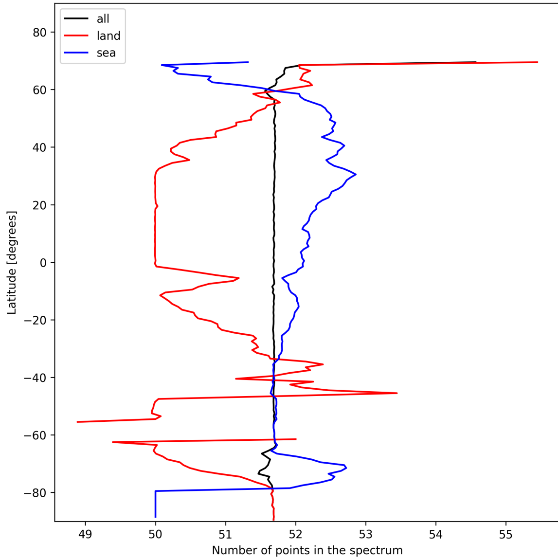
Figure 27: Zonal average of “Number of points in the spectrum” for 2024-11-15 to 2024-11-17.
