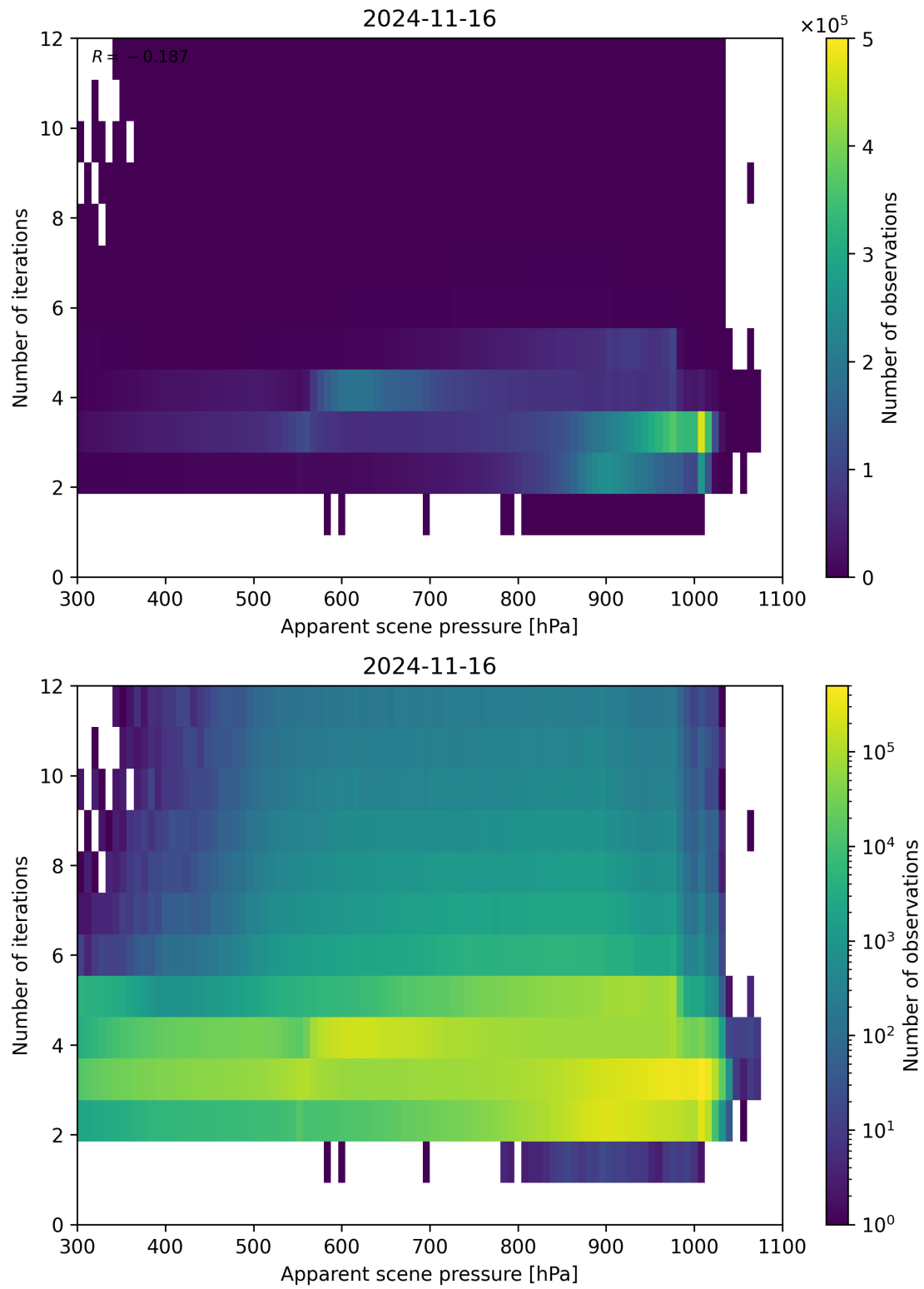
Figure 66: Scatter density plot of “Apparent scene pressure” against “Number of iterations” for 2024-11-15 to 2024-11-17.
