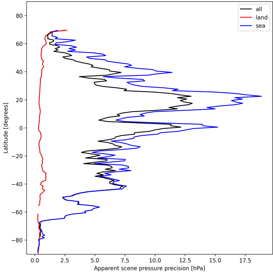
Figure 20: Zonal average of “Apparent scene pressure precision” for 2024-11-15 to 2024-11-17.
