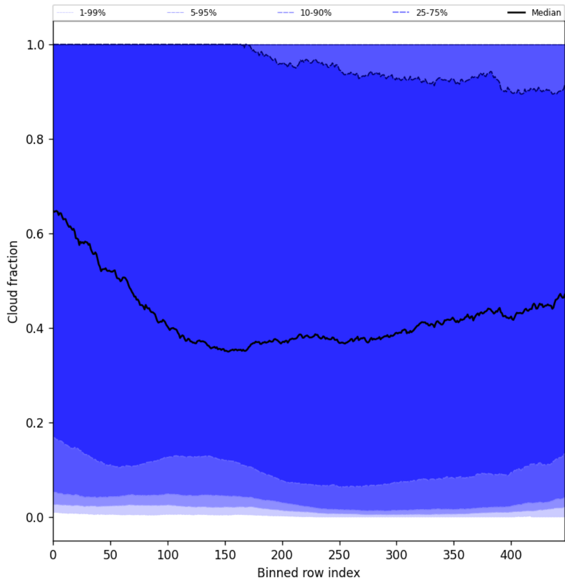
Figure 49: Along track statistics of “Cloud fraction” for 2024-11-15 to 2024-11-17
