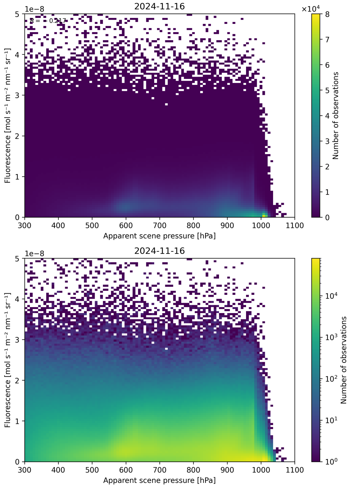
Figure 65: Scatter density plot of “Apparent scene pressure” against “Fluorescence” for 2024-11-15 to 2024-11-17.
