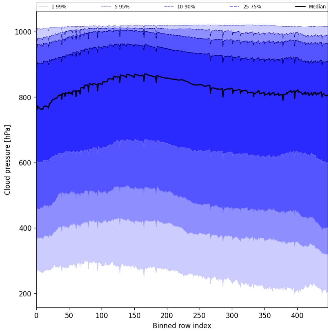
Figure 47: Along track statistics of “Cloud pressure” for 2024-11-15 to 2024-11-17
