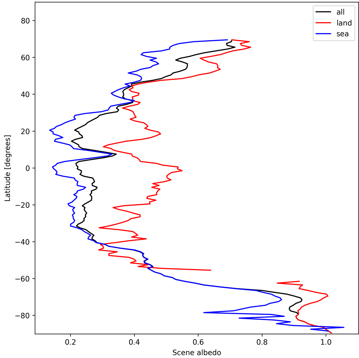
Figure 17: Zonal average of “Scene albedo” for 2024-11-15 to 2024-11-17.
