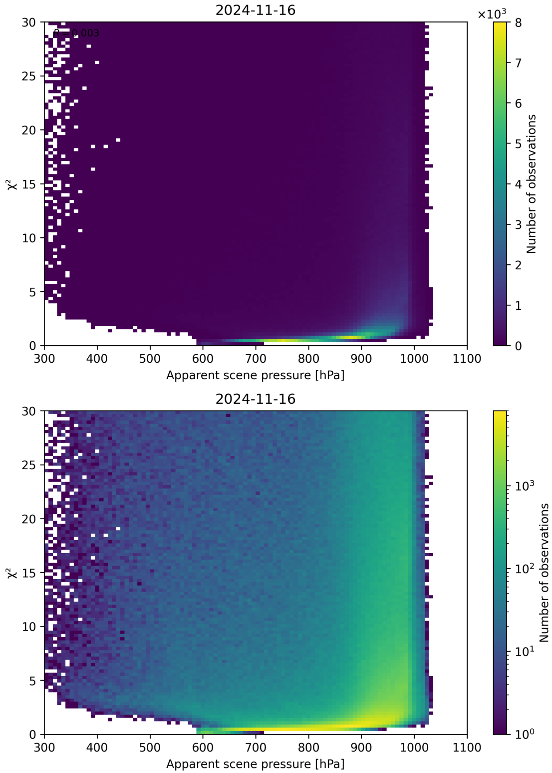
Figure 63: Scatter density plot of “Apparent scene pressure” against “ \chi^2 ” for 2024-11-15 to 2024-11-17.
