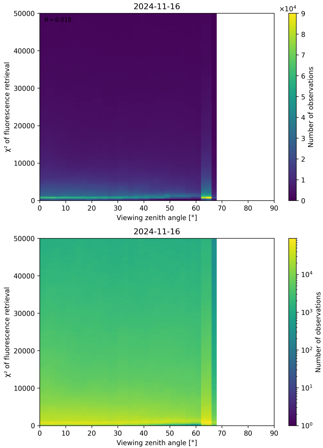
Figure 131: Scatter density plot of “Viewing zenith angle” against “ \chi^2 of fluorescence retrieval” for 2024-11-15 to 2024-11-17.
