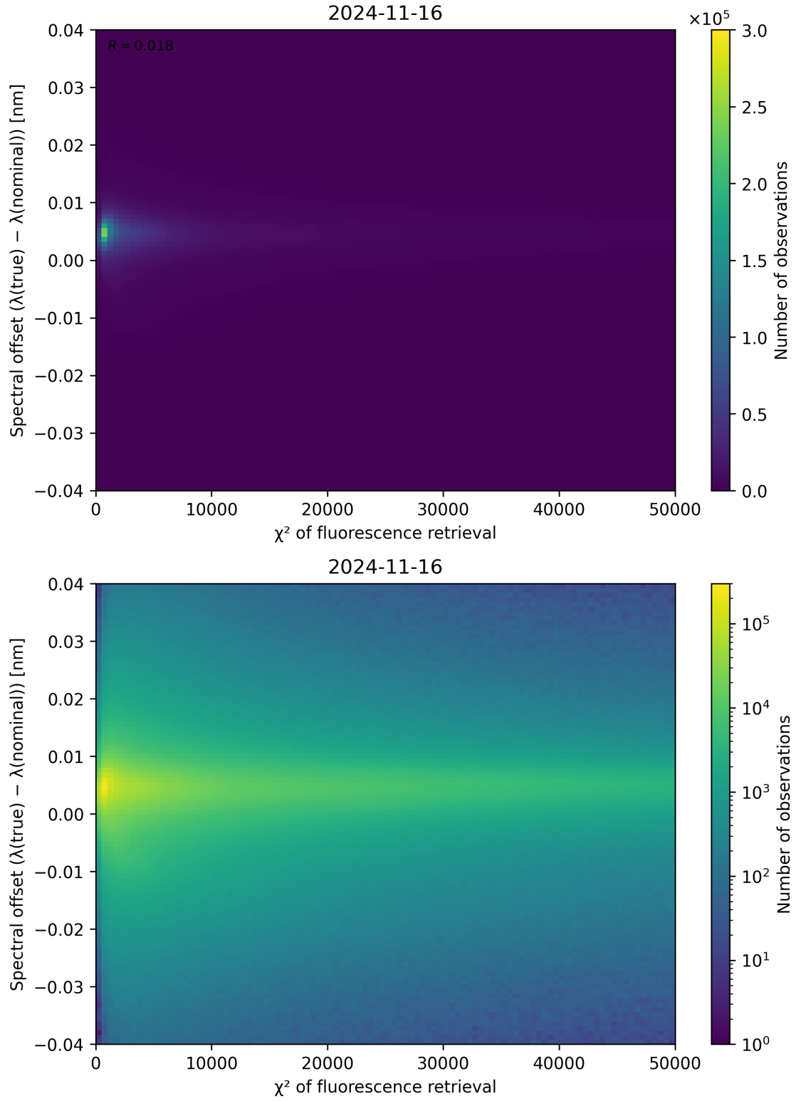
Figure 72: Scatter density plot of “ \chi^2 of fluorescence retrieval” against “Spectral offset ( \lambda_{\text{true}} - \lambda_{\text{nominal}} )” for 2024-11-15 to 2024-11-17.
