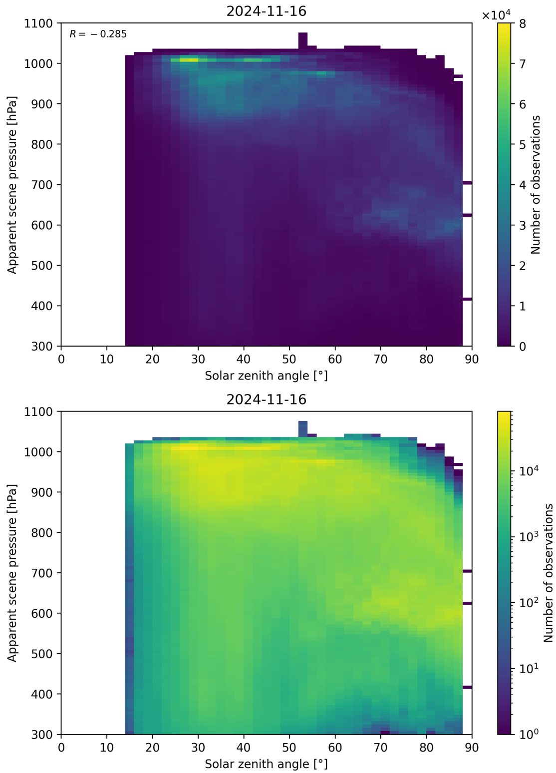
Figure 118: Scatter density plot of “Solar zenith angle” against “Apparent scene pressure” for 2024-11-15 to 2024-11-17.
