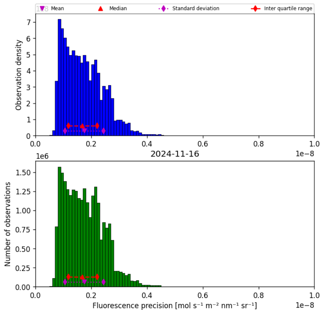
Figure 41: Histogram of “Fluorescence precision” for 2024-11-15 to 2024-11-17
