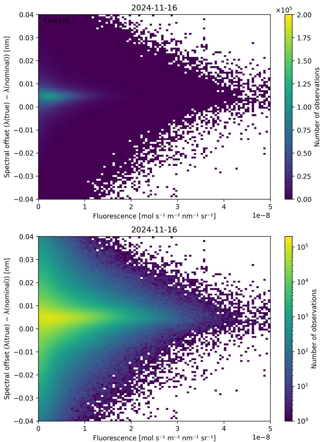
Figure 95: Scatter density plot of “Fluorescence” against “Spectral offset ( \lambda_{\text{true}} - \lambda_{\text{nominal}} )” for 2024-11-15 to 2024-11-17.
