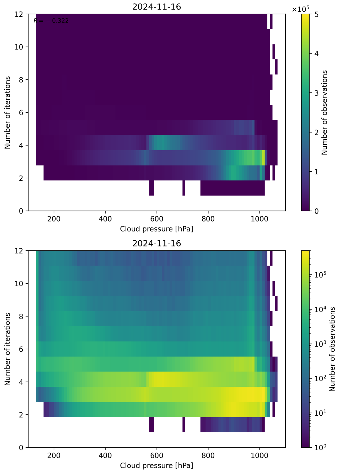
Figure 89: Scatter density plot of “Cloud pressure” against “Number of iterations” for 2024-11-15 to 2024-11-17.
