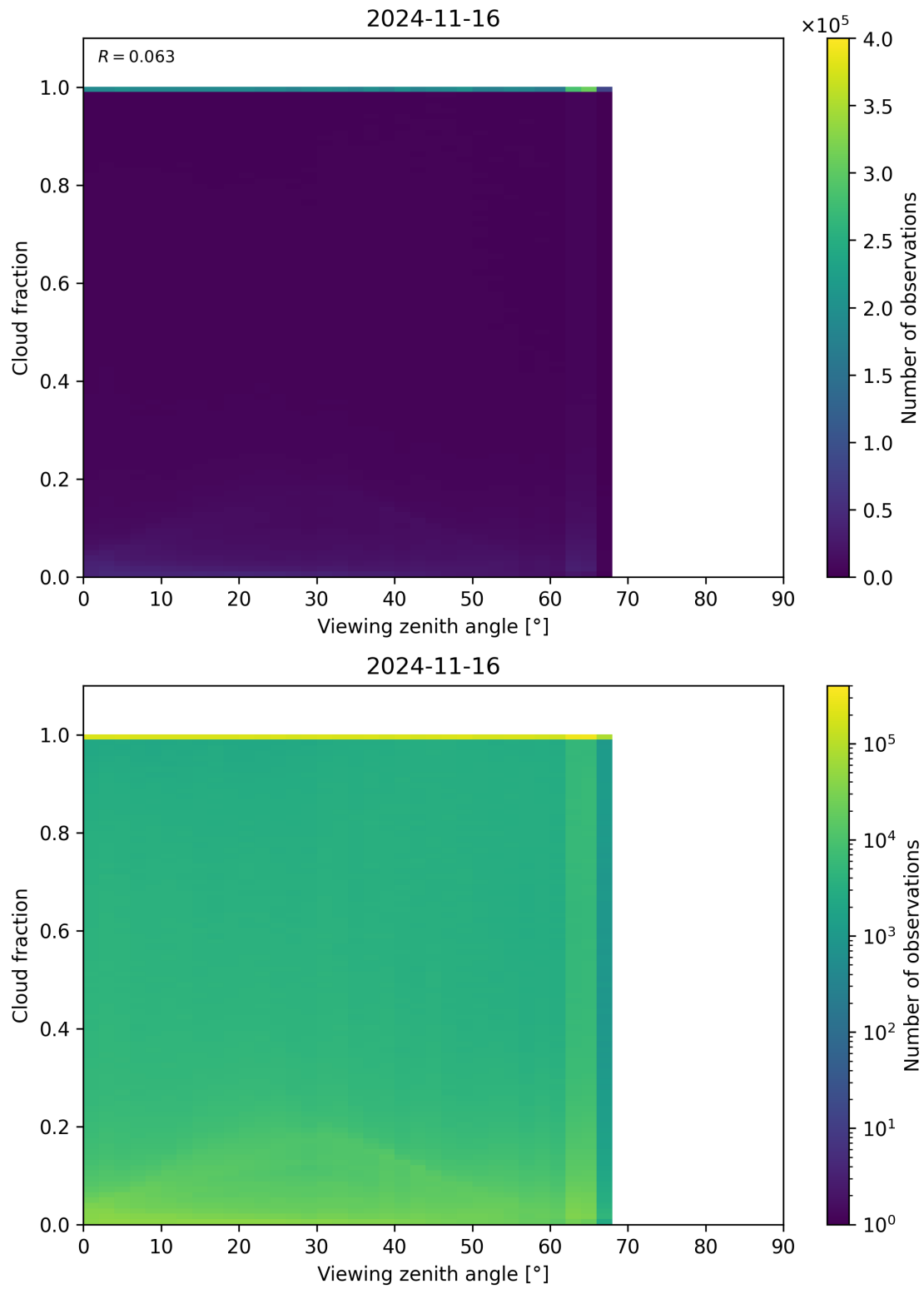
Figure 132: Scatter density plot of “Viewing zenith angle” against “Cloud fraction” for 2024-11-15 to 2024-11-17.
