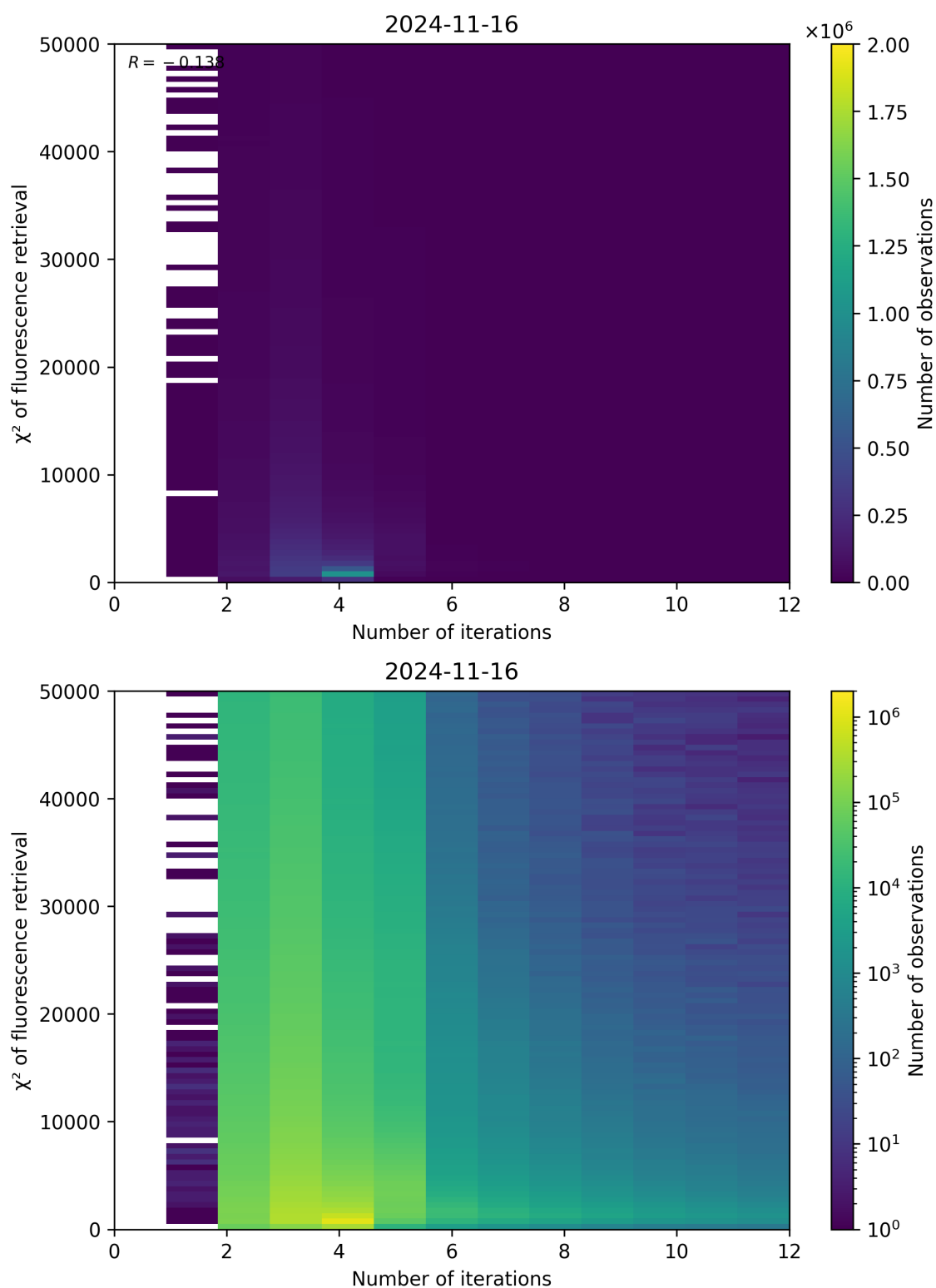
Figure 106: Scatter density plot of “Number of iterations” against “ \chi^2 of fluorescence retrieval” for 2024-11-15 to 2024-11-17.
