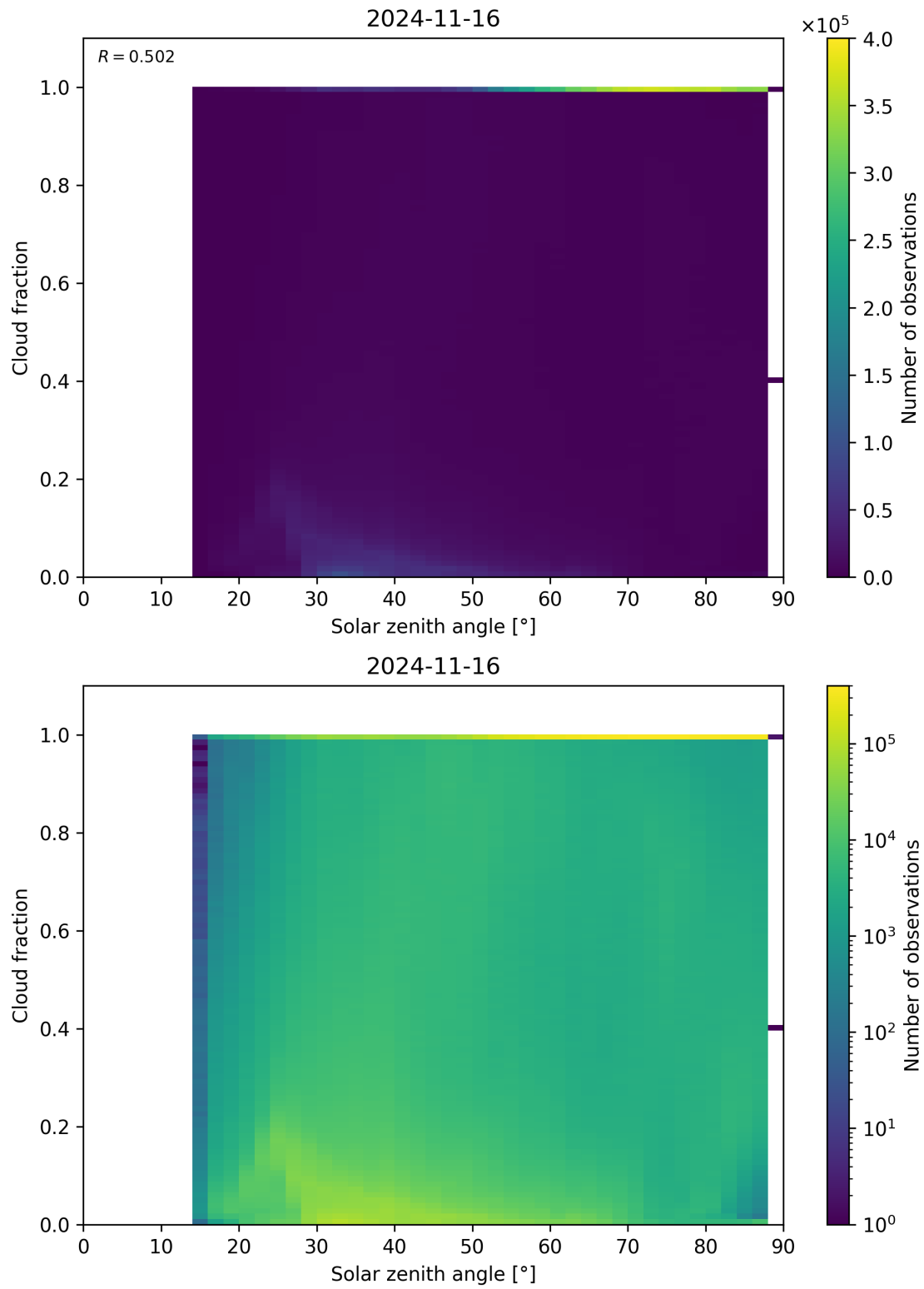
Figure 121: Scatter density plot of “Solar zenith angle” against “Cloud fraction” for 2024-11-15 to 2024-11-17.
