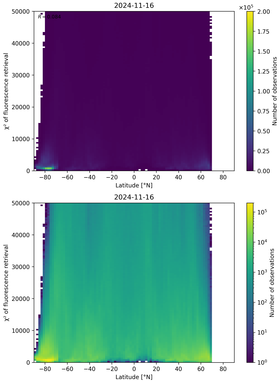
Figure 98: Scatter density plot of “Latitude” against “ \chi^2 of fluorescence retrieval” for 2024-11-15 to 2024-11-17.
