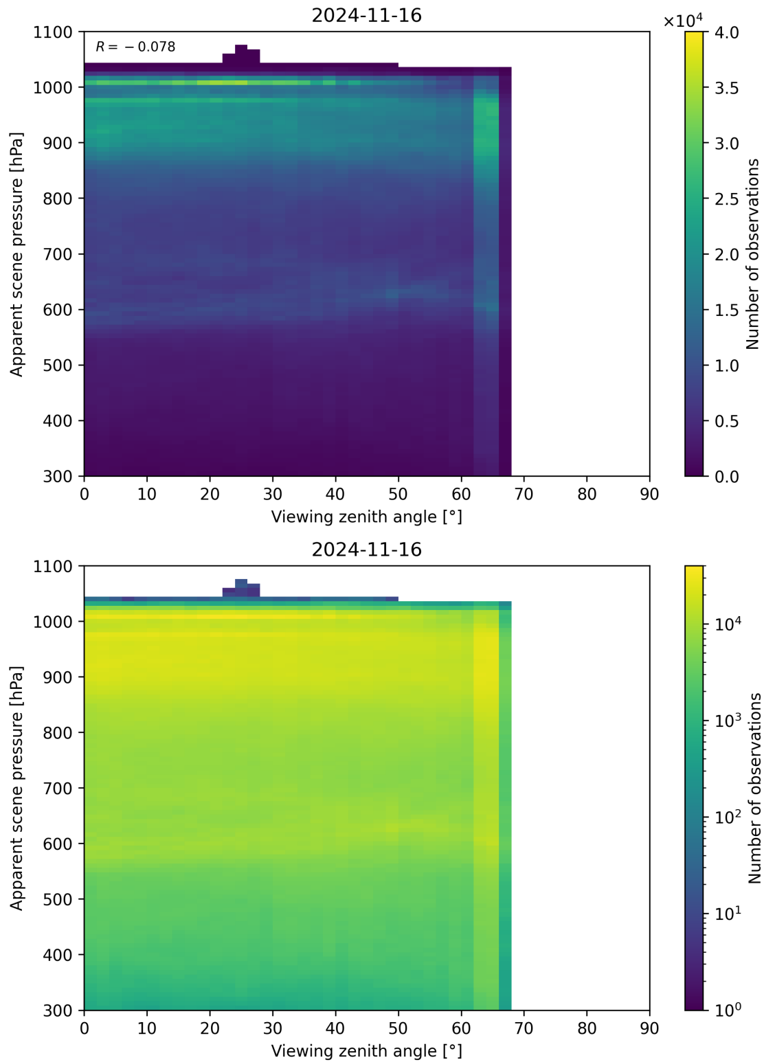
Figure 129: Scatter density plot of “Viewing zenith angle” against “Apparent scene pressure” for 2024-11-15 to 2024-11-17.
