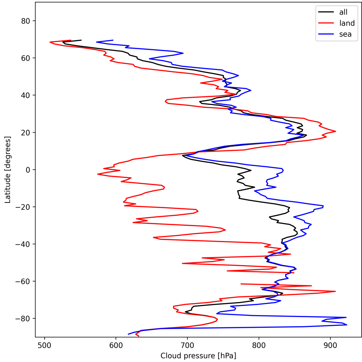
Figure 13: Zonal average of “Cloud pressure” for 2024-11-15 to 2024-11-17.
