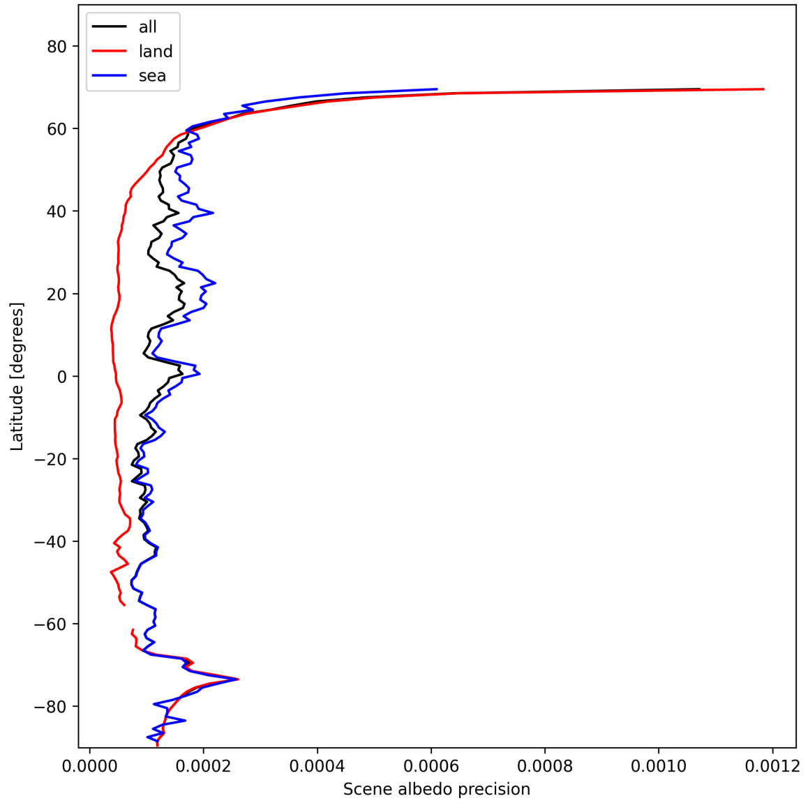
Figure 18: Zonal average of “Scene albedo precision” for 2024-11-15 to 2024-11-17.
