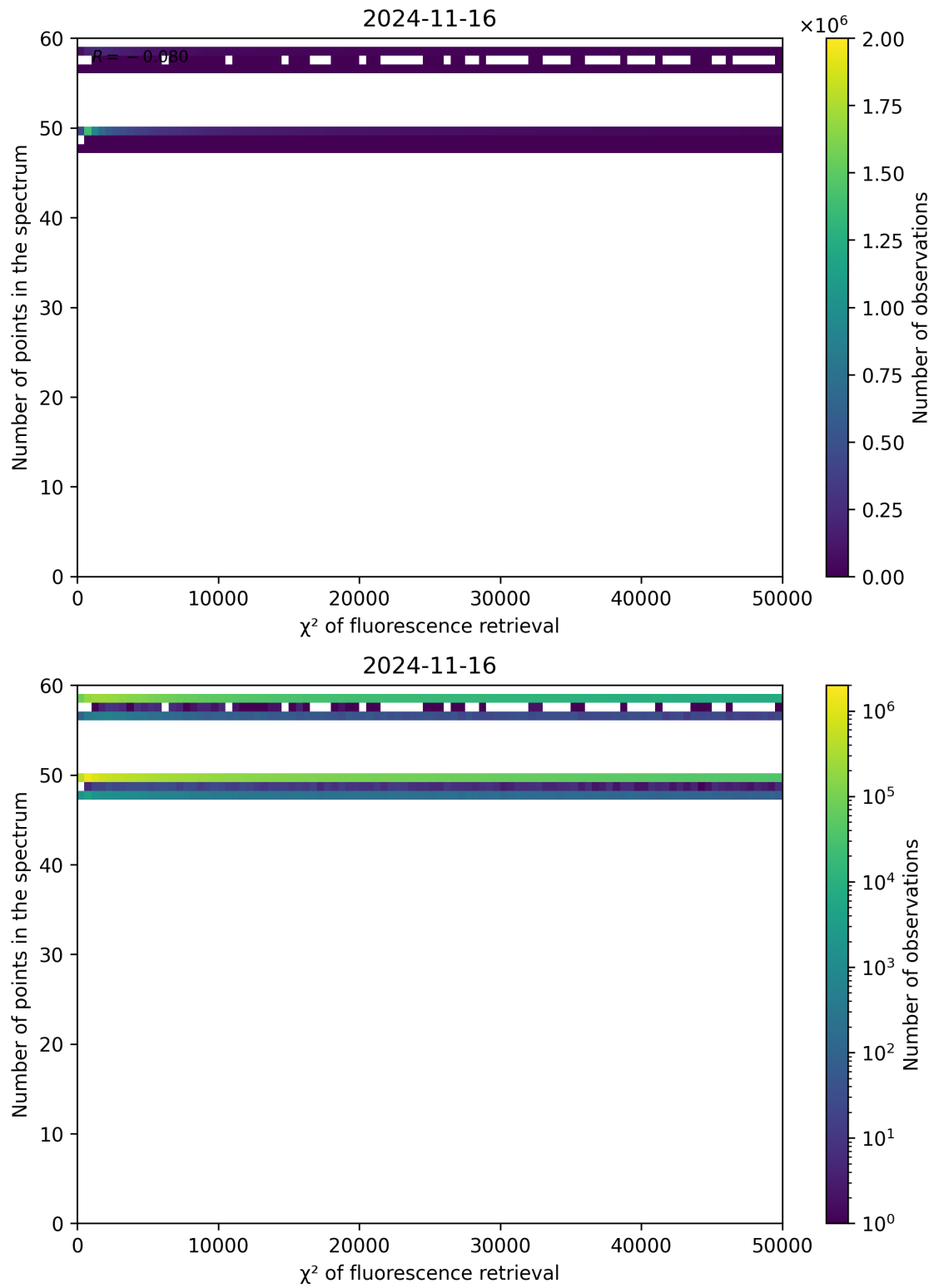
Figure 71: Scatter density plot of " \chi^2 of fluorescence retrieval" against "Number of points in the spectrum" for 2024-11-15 to 2024-11-17.
