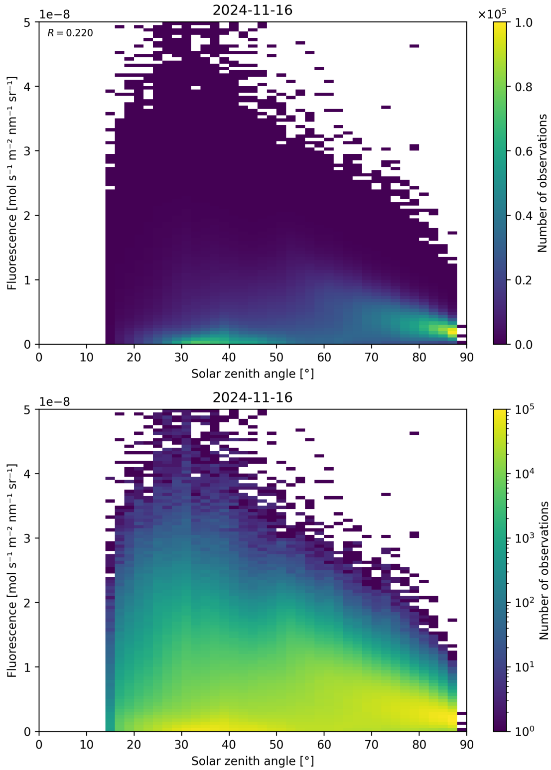
Figure 123: Scatter density plot of “Solar zenith angle” against “Fluorescence” for 2024-11-15 to 2024-11-17.
