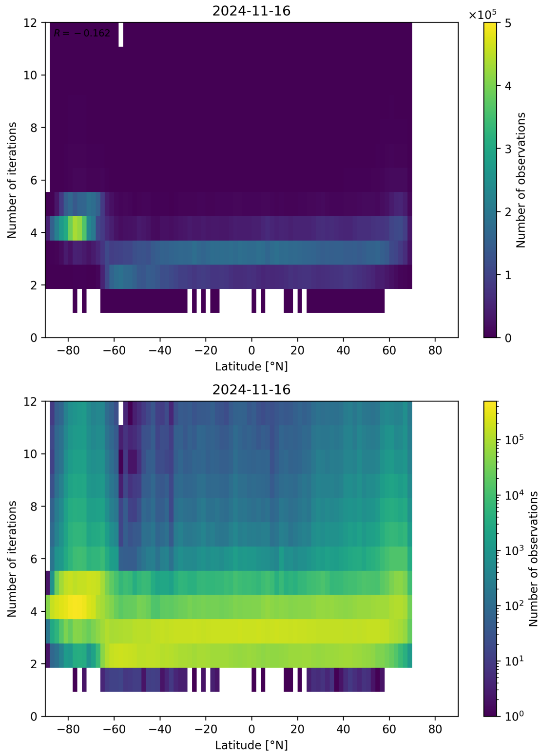
Figure 102: Scatter density plot of “Latitude” against “Number of iterations” for 2024-11-15 to 2024-11-17.
