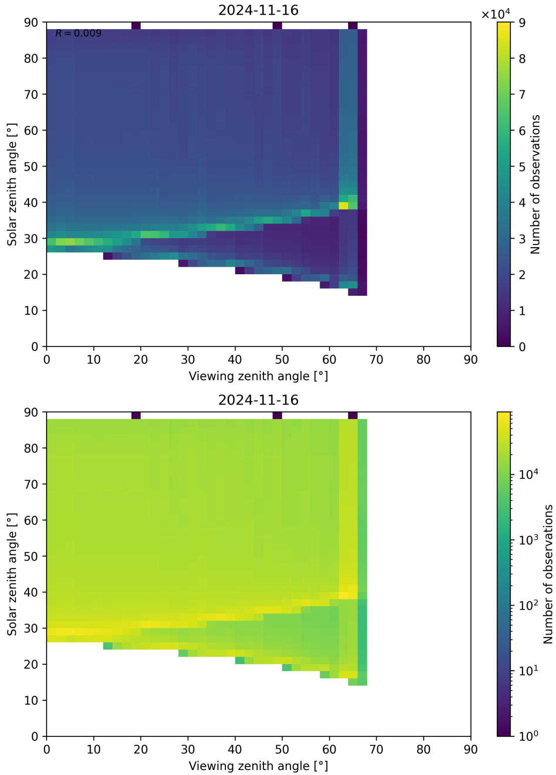
Figure 139: Scatter density plot of “Viewing zenith angle” against “Solar zenith angle” for 2024-11-15 to 2024-11-17.
