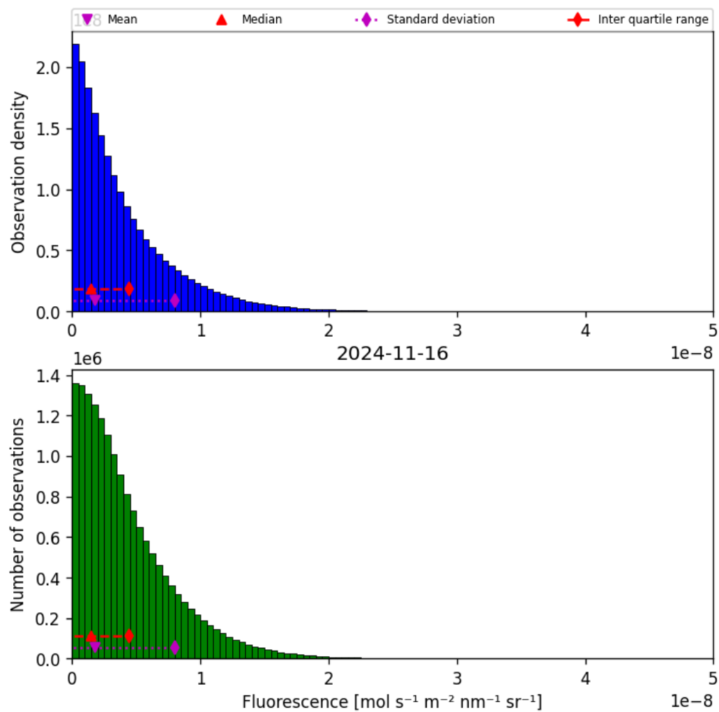
Figure 40: Histogram of “Fluorescence” for 2024-11-15 to 2024-11-17
