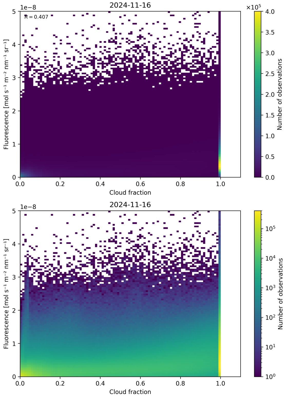
Figure 79: Scatter density plot of “Cloud fraction” against “Fluorescence” for 2024-11-15 to 2024-11-17.
