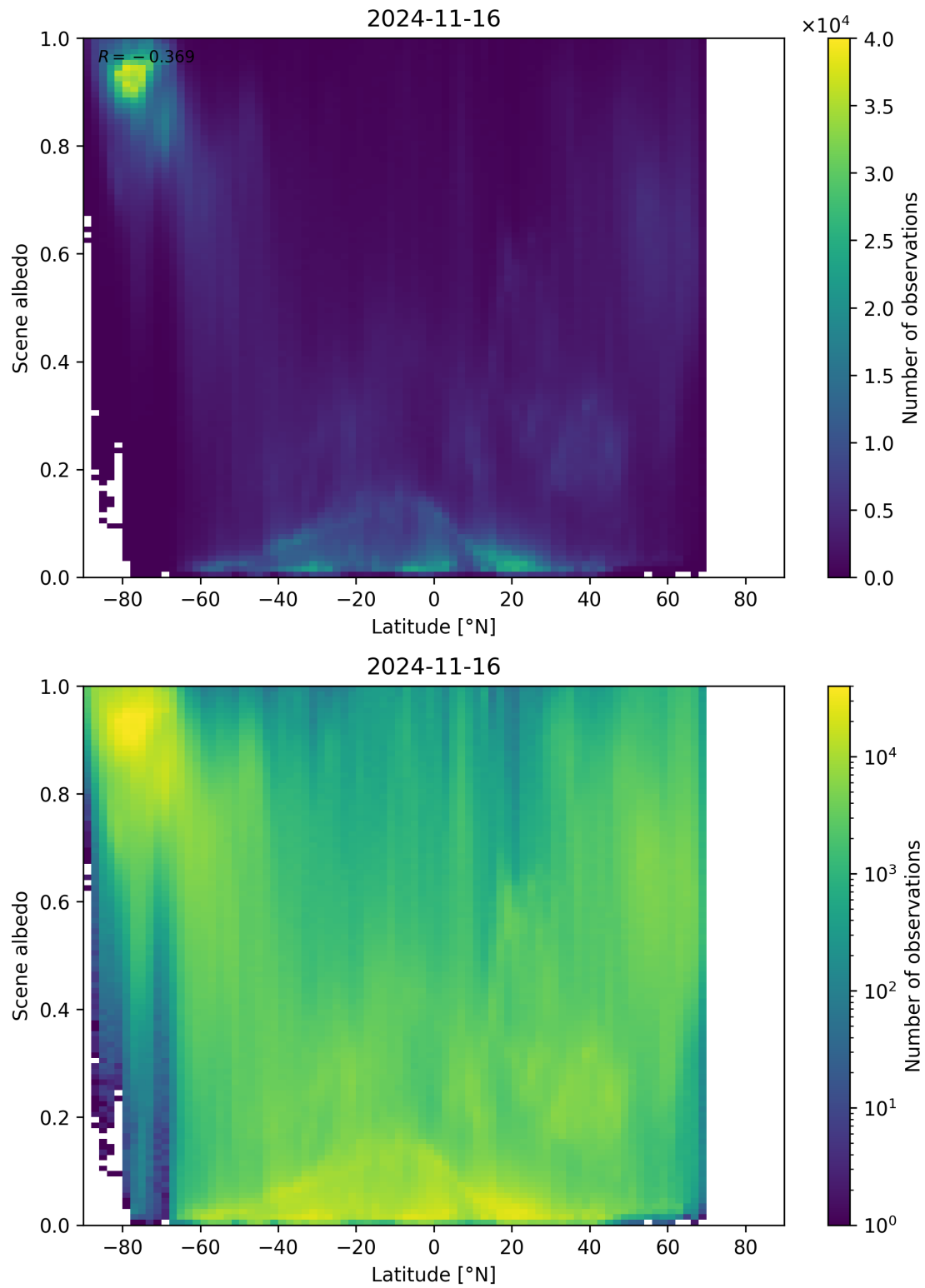
Figure 104: Scatter density plot of “Latitude” against “Scene albedo” for 2024-11-15 to 2024-11-17.
