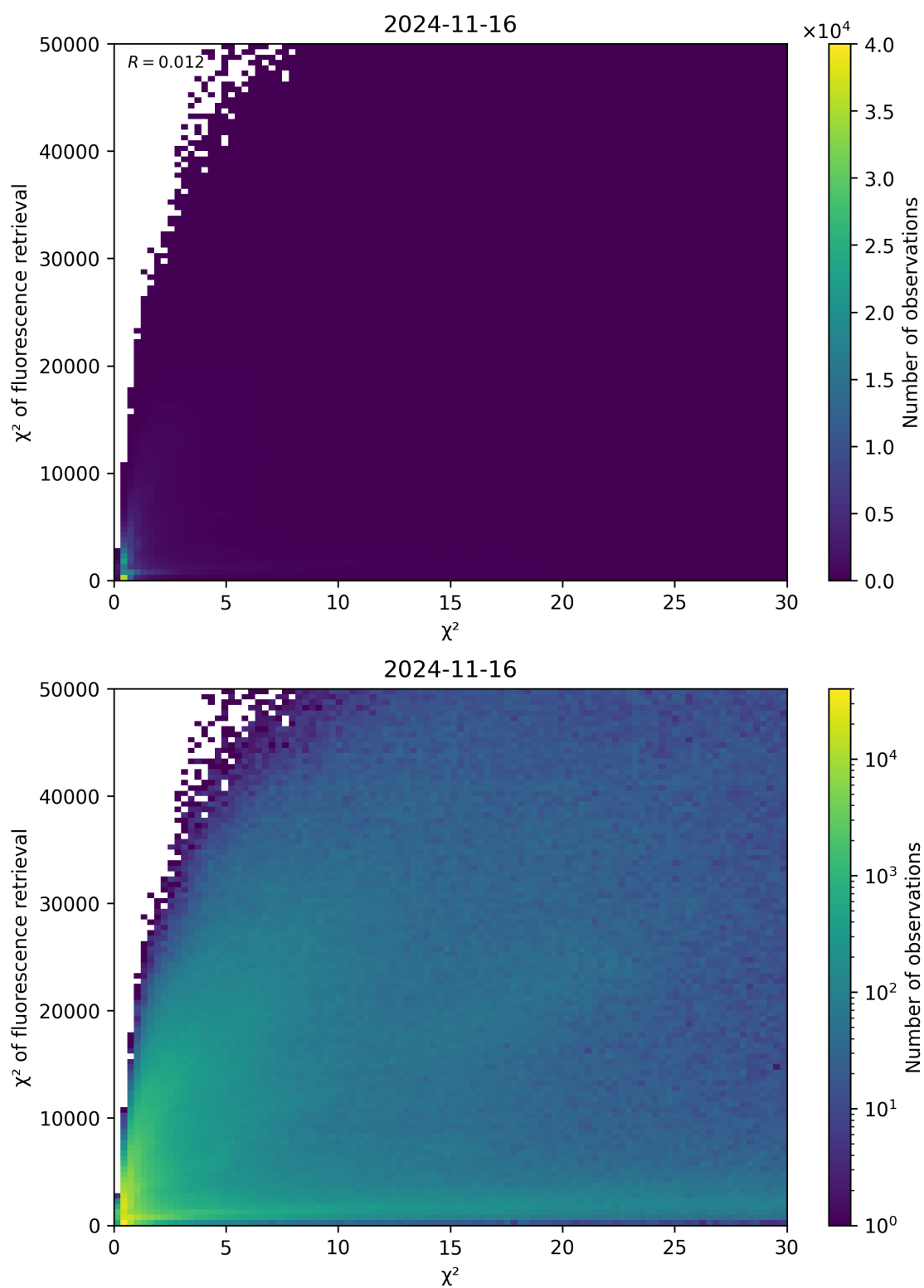
Figure 69: Scatter density plot of “ \chi^2 ” against “ \chi^2 of fluorescence retrieval” for 2024-11-15 to 2024-11-17.
