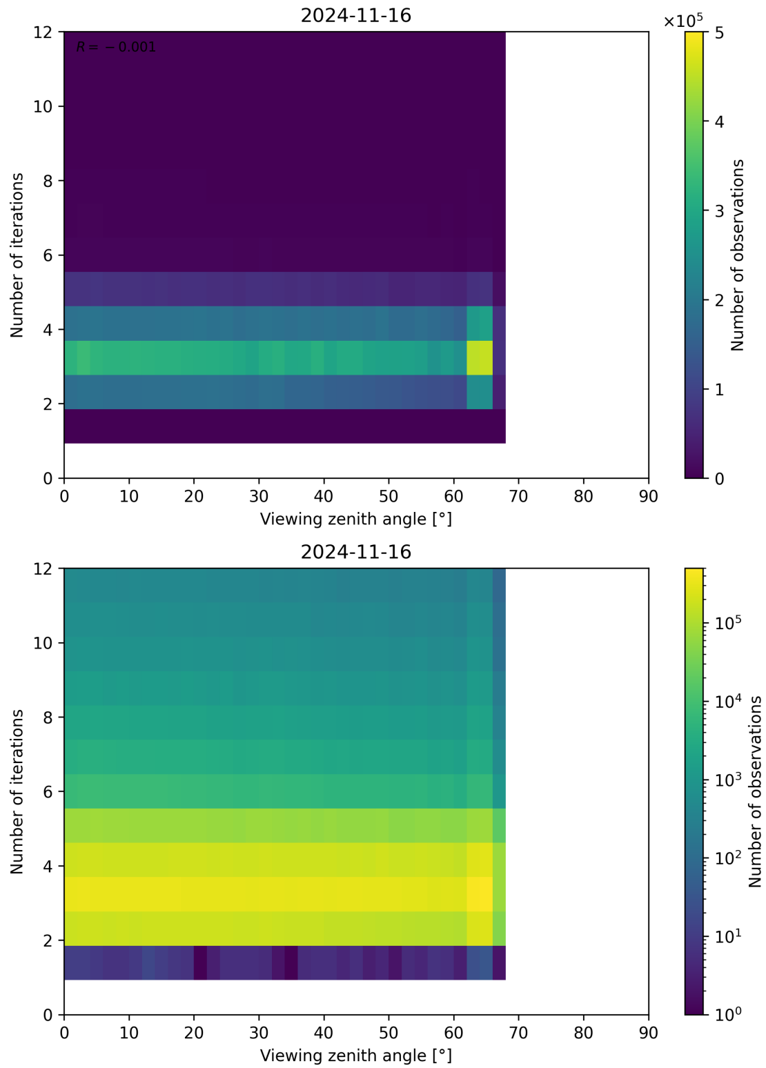
Figure 136: Scatter density plot of “Viewing zenith angle” against “Number of iterations” for 2024-11-15 to 2024-11-17.
