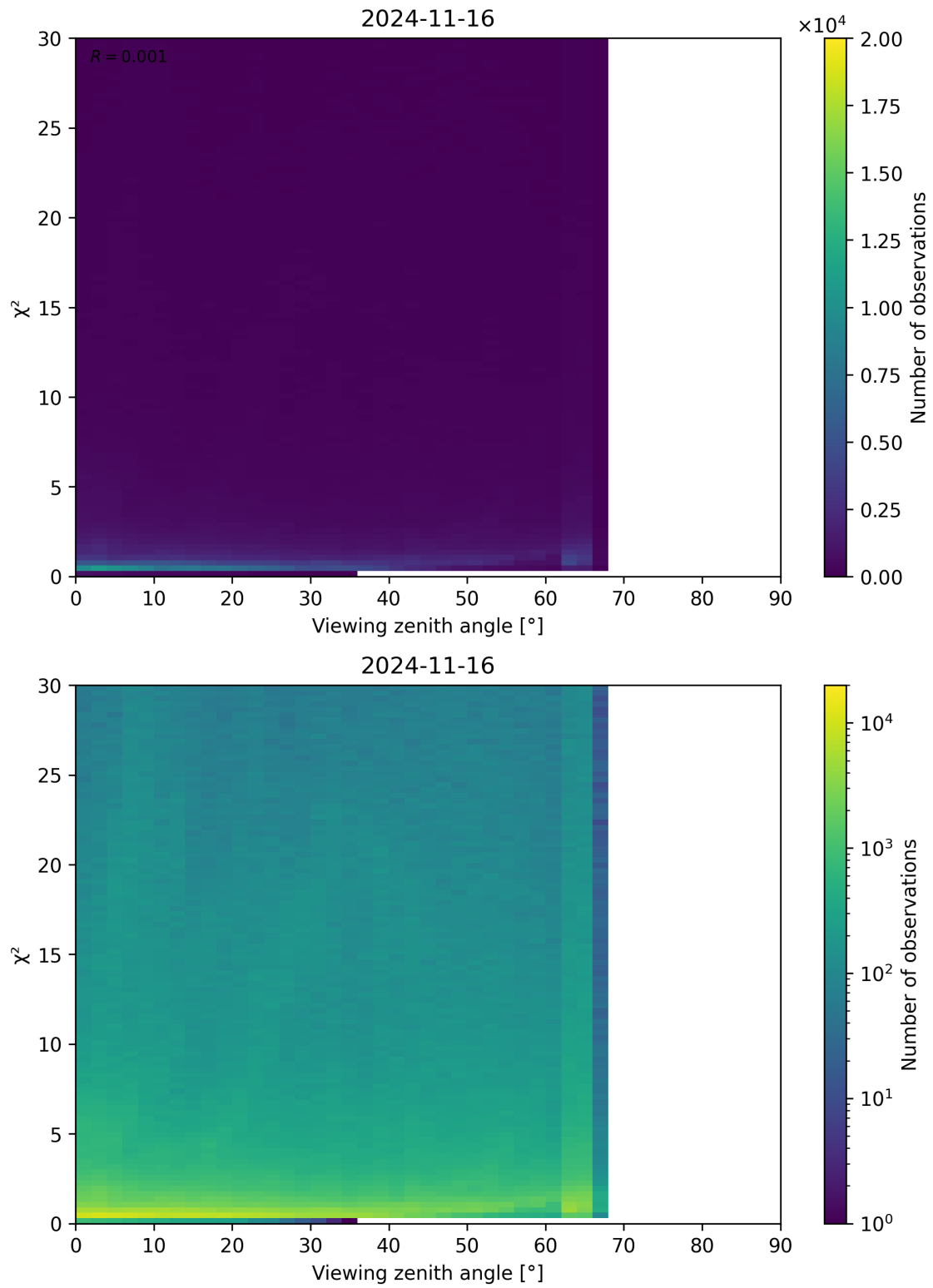
Figure 130: Scatter density plot of “Viewing zenith angle” against “ \chi^2 ” for 2024-11-15 to 2024-11-17.
