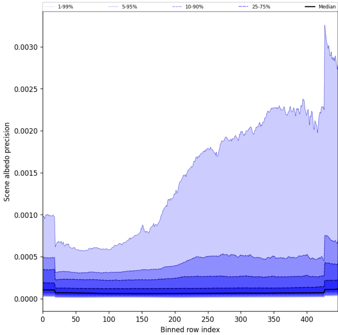
Figure 52: Along track statistics of “Scene albedo precision” for 2024-11-15 to 2024-11-17
