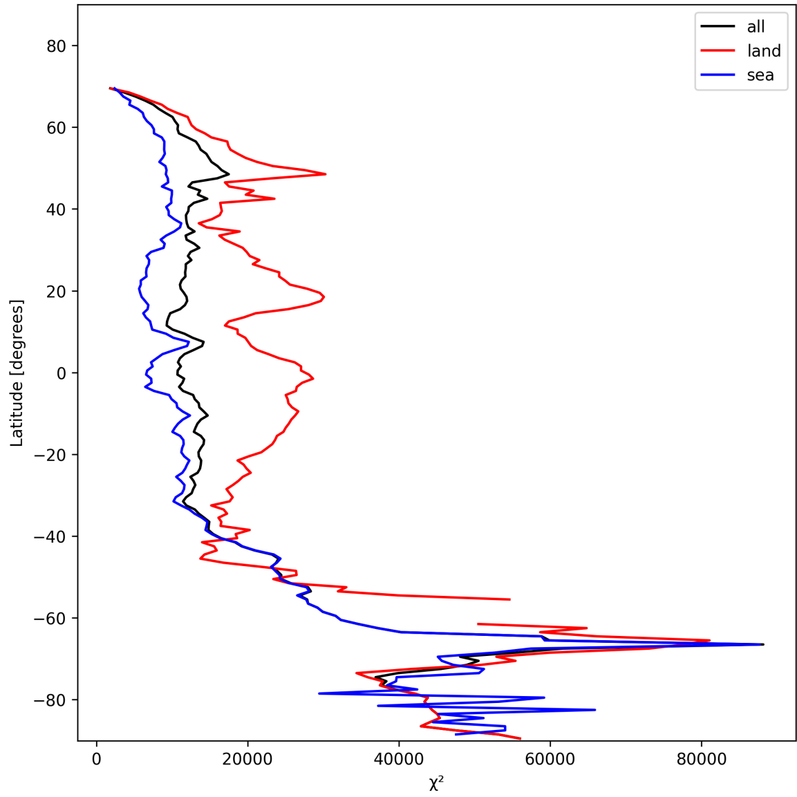
Figure 21: Zonal average of “ \chi^2 ” for 2024-11-15 to 2024-11-17.
