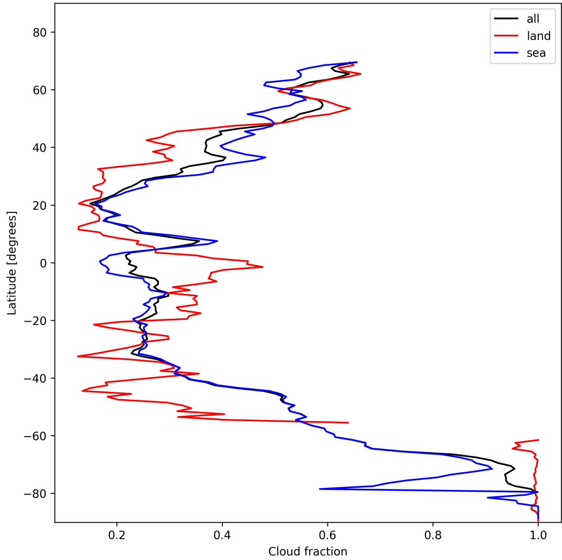
Figure 15: Zonal average of “Cloud fraction” for 2024-11-15 to 2024-11-17.
