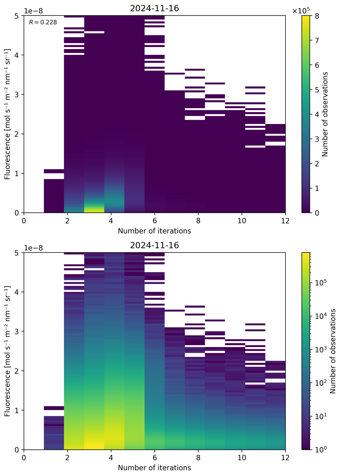
Figure 107: Scatter density plot of “Number of iterations” against “Fluorescence” for 2024-11-15 to 2024-11-17.
