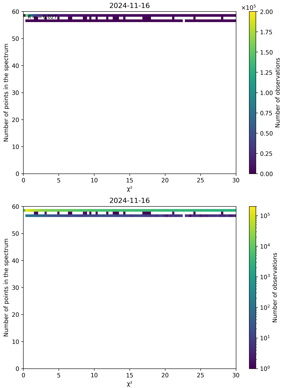
Figure 74: Scatter density plot of " \chi^2 " against "Number of points in the spectrum" for 2024-11-15 to 2024-11-17.
