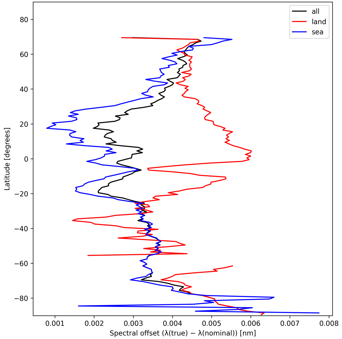
Figure 28: Zonal average of “Spectral offset ( \lambda_{\text{true}} - \lambda_{\text{nominal}} )” for 2024-11-15 to 2024-11-17.
