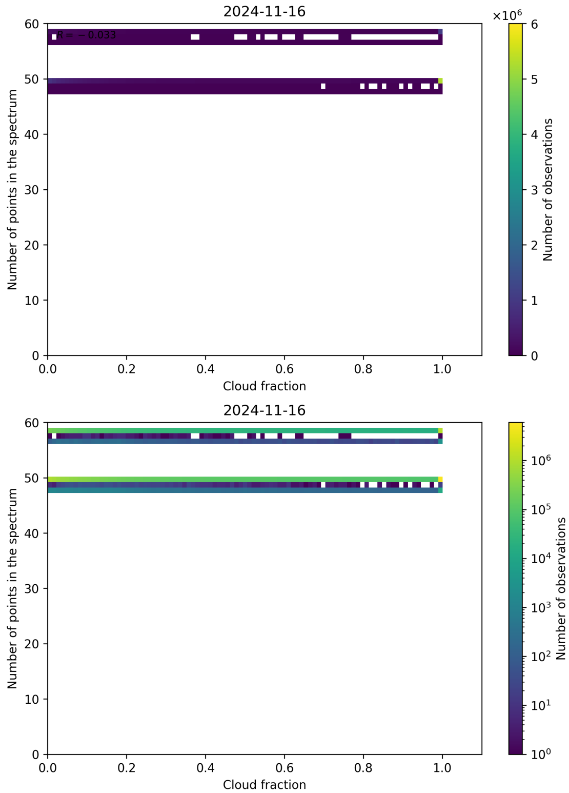
Figure 81: Scatter density plot of “Cloud fraction” against “Number of points in the spectrum” for 2024-11-15 to 2024-11-17.
