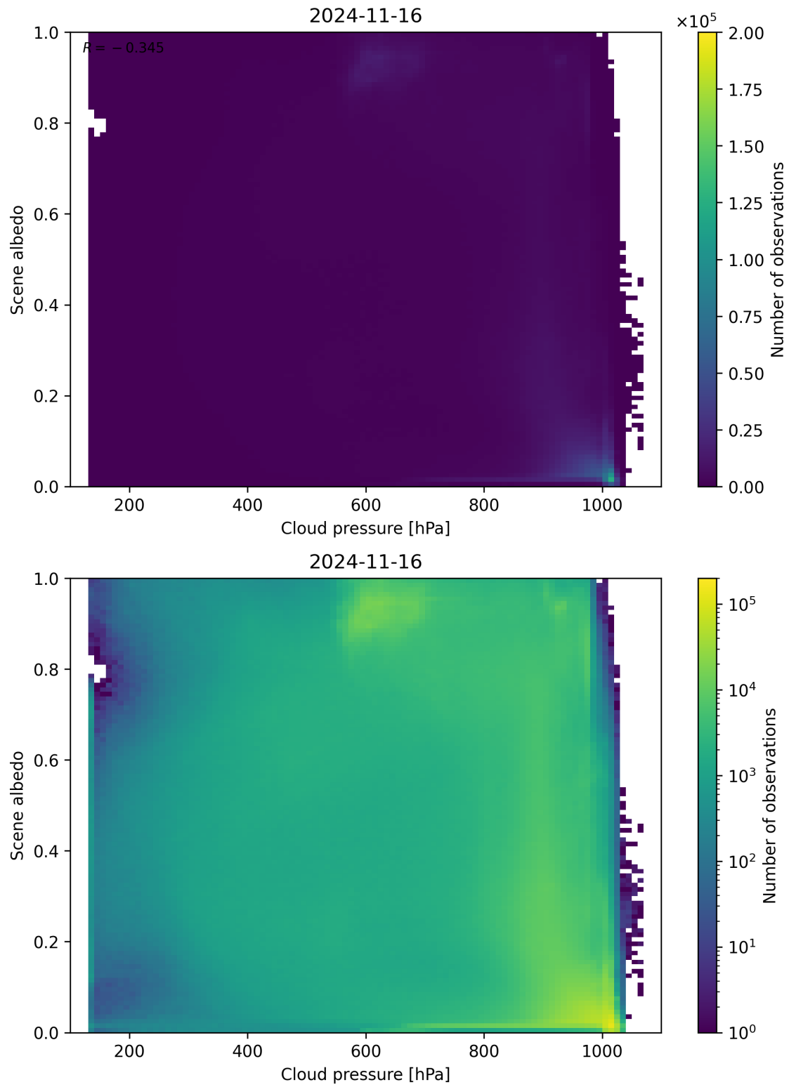
Figure 91: Scatter density plot of “Cloud pressure” against “Scene albedo” for 2024-11-15 to 2024-11-17.
