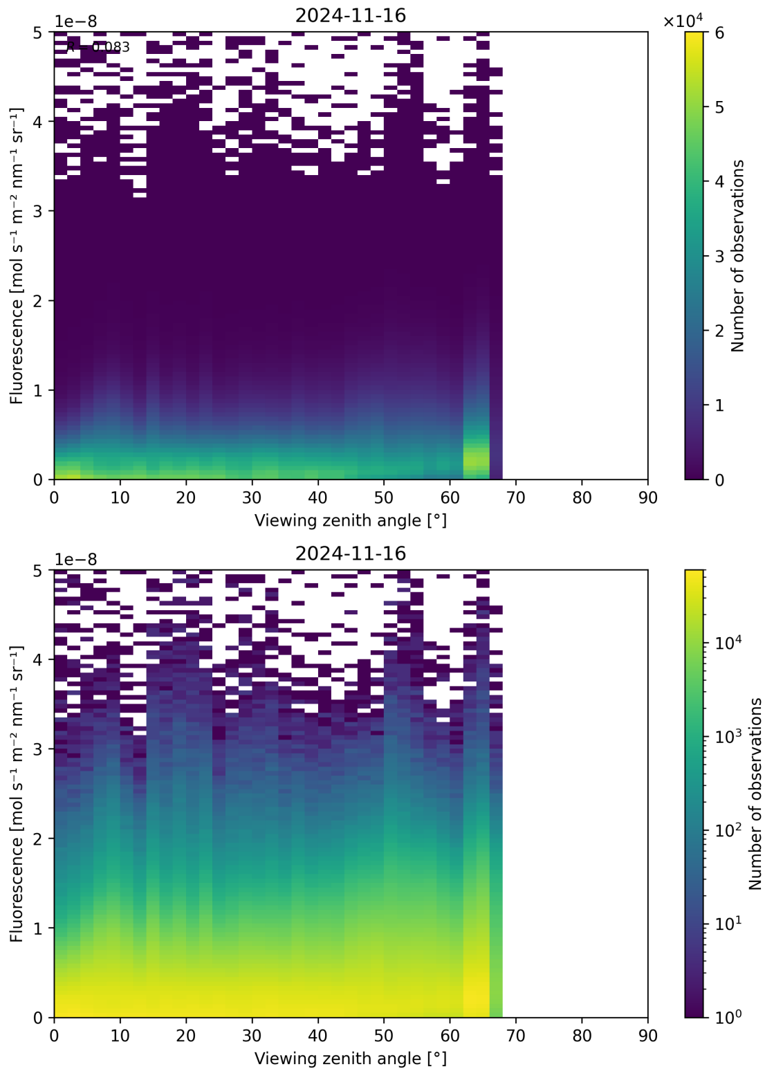
Figure 134: Scatter density plot of “Viewing zenith angle” against “Fluorescence” for 2024-11-15 to 2024-11-17.
