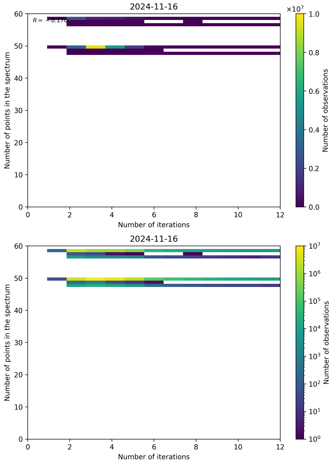
Figure 108: Scatter density plot of “Number of iterations” against “Number of points in the spectrum” for 2024-11-15 to 2024-11-17.
