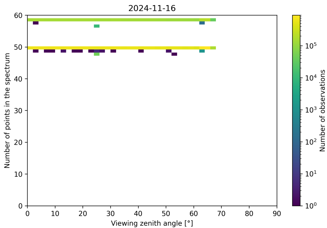
Figure 137: Scatter density plot of “Viewing zenith angle” against “Number of points in the spectrum” for 2024-11-15 to 2024-11-17.
