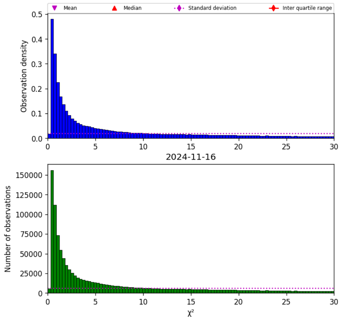
Figure 38: Histogram of “ \chi^2 ” for 2024-11-15 to 2024-11-17
