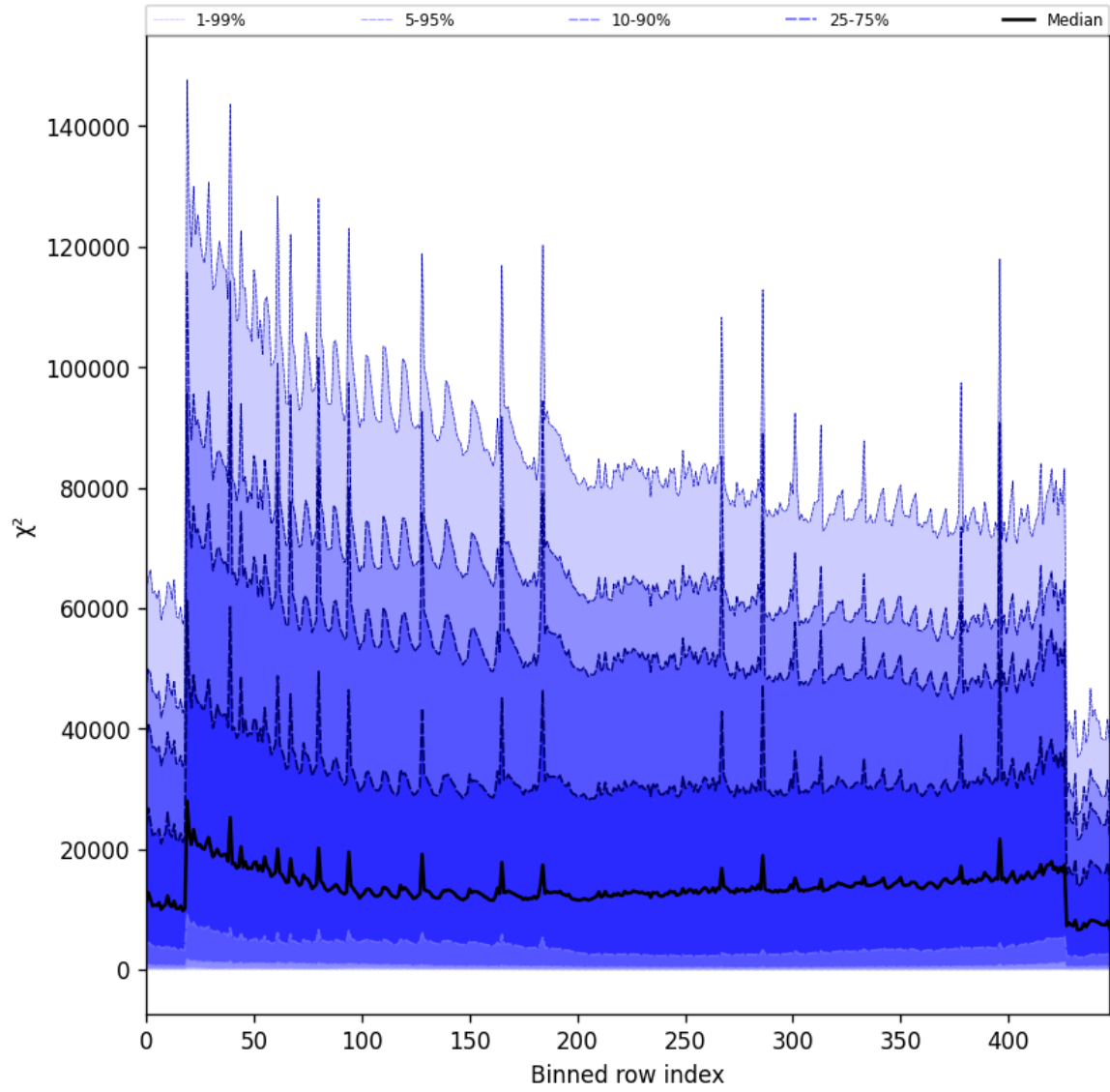
Figure 55: Along track statistics of “ \chi^2 ” for 2024-11-15 to 2024-11-17
