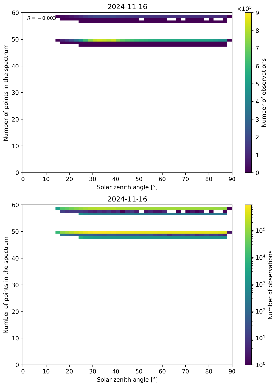
Figure 126: Scatter density plot of “Solar zenith angle” against “Number of points in the spectrum” for 2024-11-15 to 2024-11-17.
