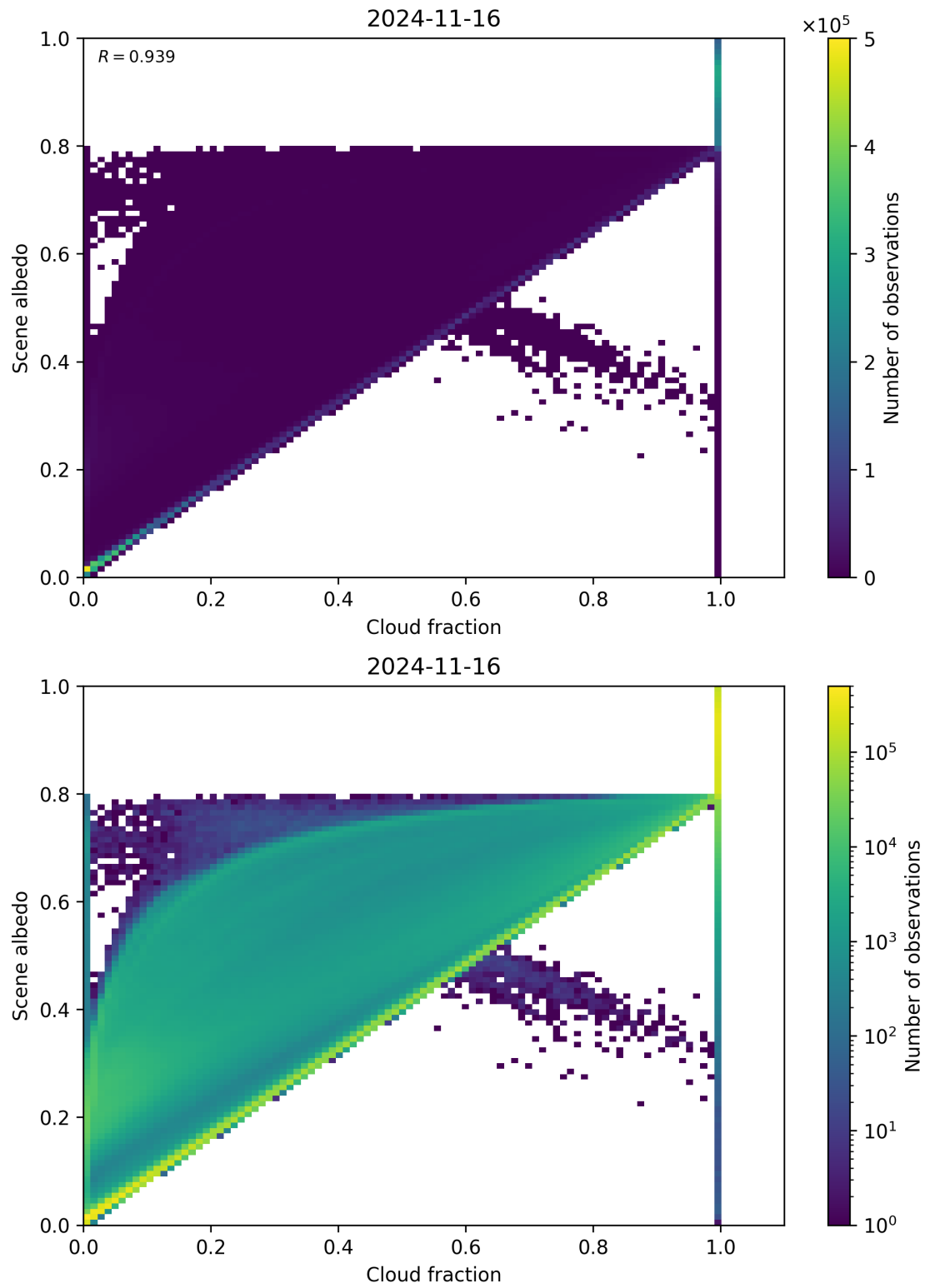
Figure 82: Scatter density plot of “Cloud fraction” against “Scene albedo” for 2024-11-15 to 2024-11-17.
