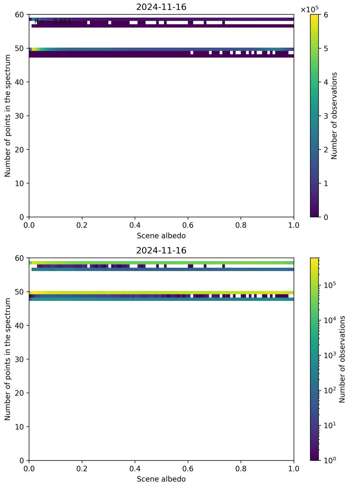
Figure 116: Scatter density plot of “Scene albedo” against “Number of points in the spectrum” for 2024-11-15 to 2024-11-17.
