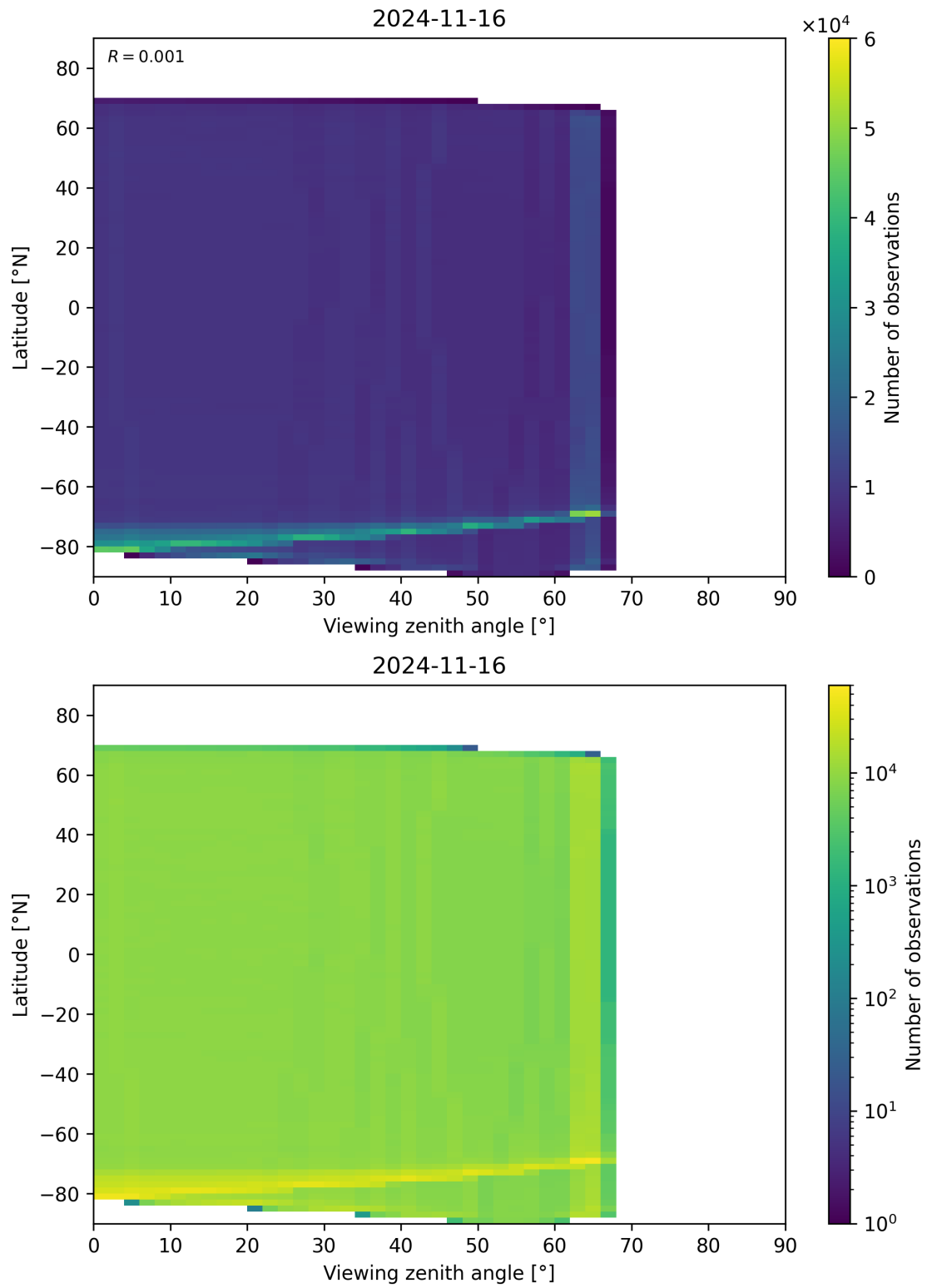
Figure 135: Scatter density plot of “Viewing zenith angle” against “Latitude” for 2024-11-15 to 2024-11-17.
