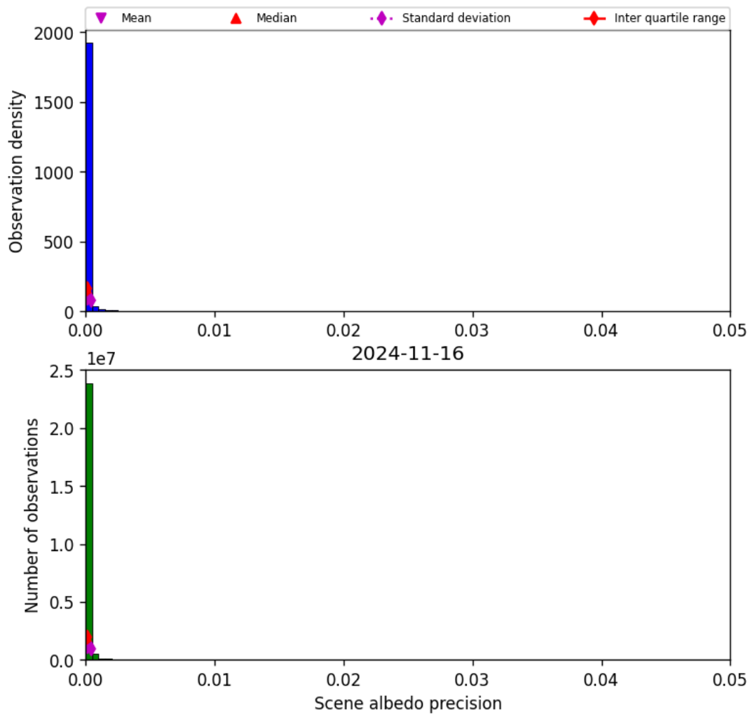
Figure 35: Histogram of “Scene albedo precision” for 2024-11-15 to 2024-11-17
