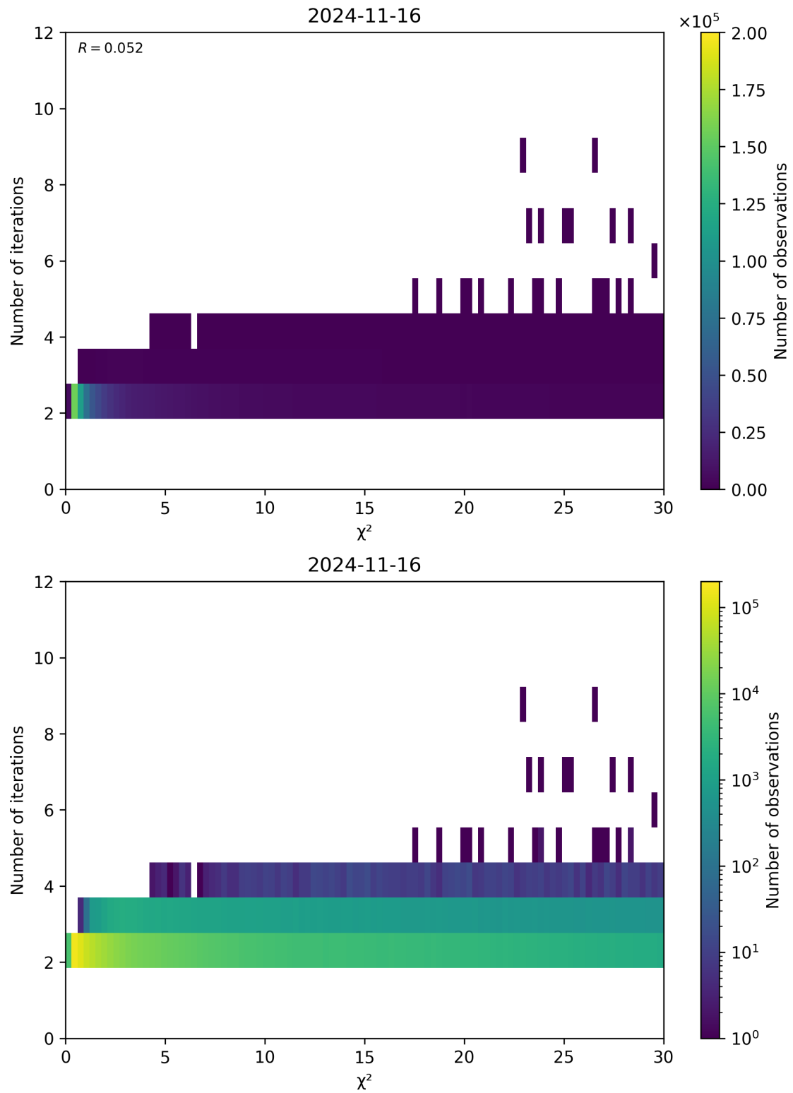
Figure 73: Scatter density plot of “ \chi^2 ” against “Number of iterations” for 2024-11-15 to 2024-11-17.
