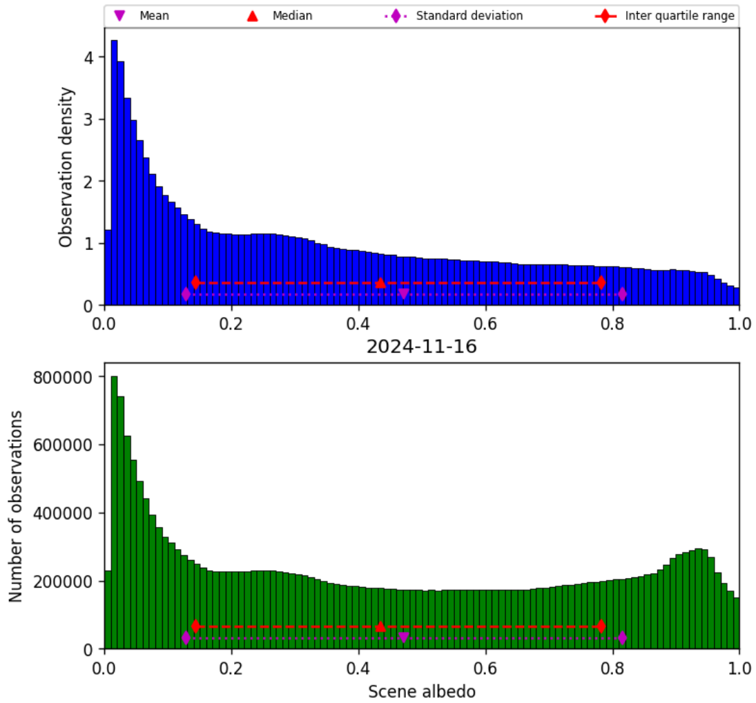
Figure 34: Histogram of “Scene albedo” for 2024-11-15 to 2024-11-17
