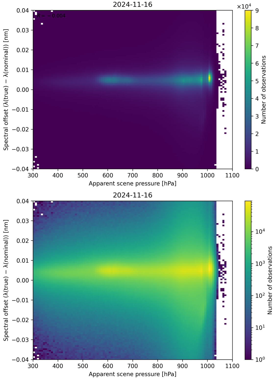
Figure 68: Scatter density plot of “Apparent scene pressure” against “Spectral offset ( \lambda_{\text{true}} - \lambda_{\text{nominal}} )” for 2024-11-15 to 2024-11-17.
