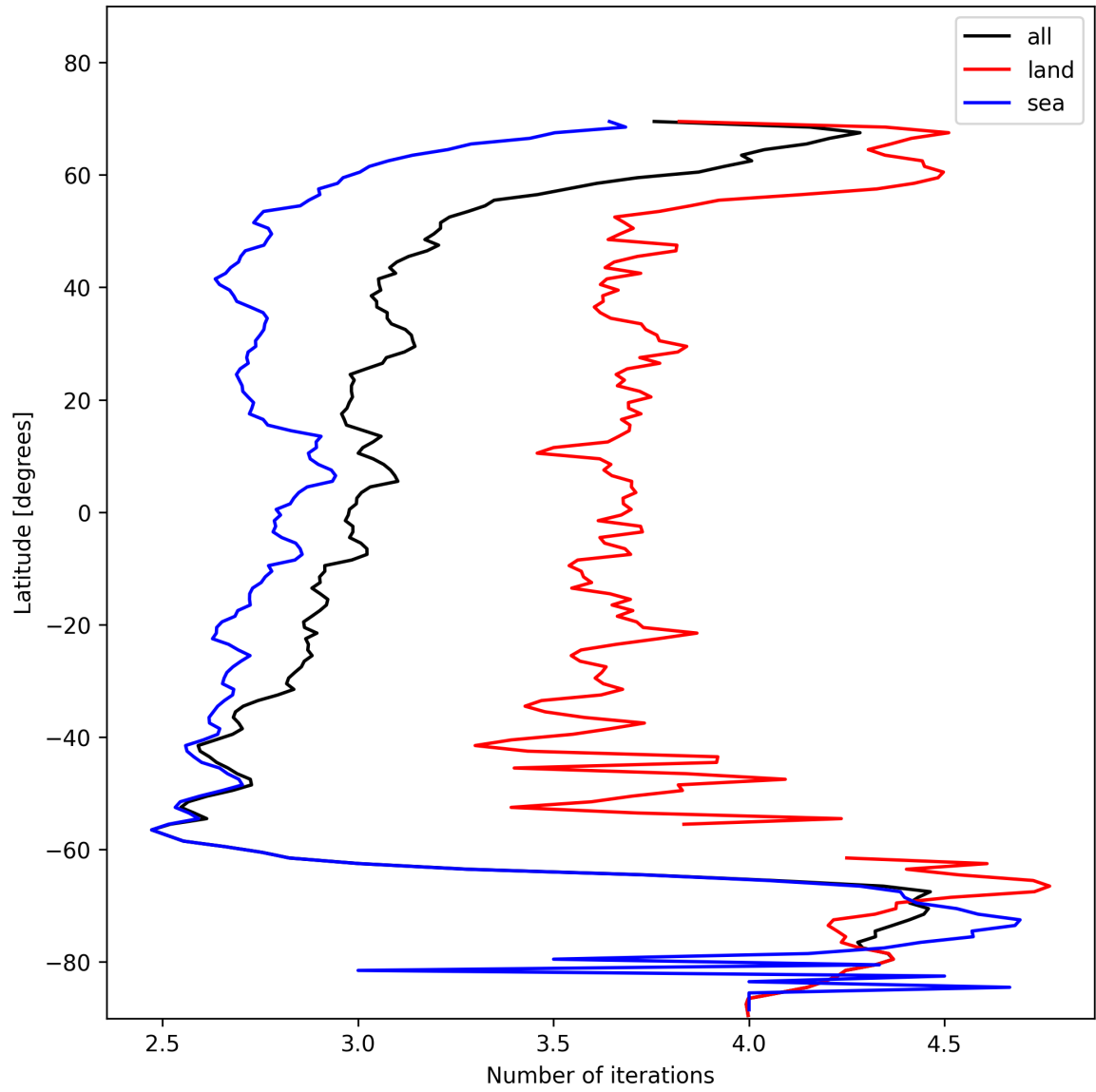
Figure 22: Zonal average of “Number of iterations” for 2024-11-15 to 2024-11-17.
