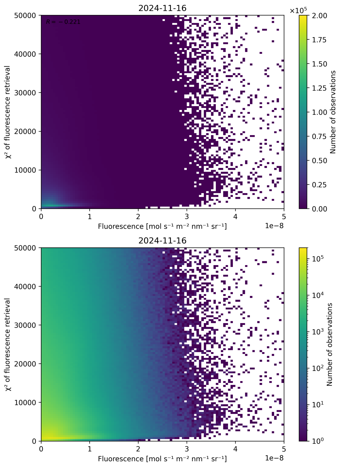
Figure 93: Scatter density plot of “Fluorescence” against “ \chi^2 of fluorescence retrieval” for 2024-11-15 to 2024-11-17.
