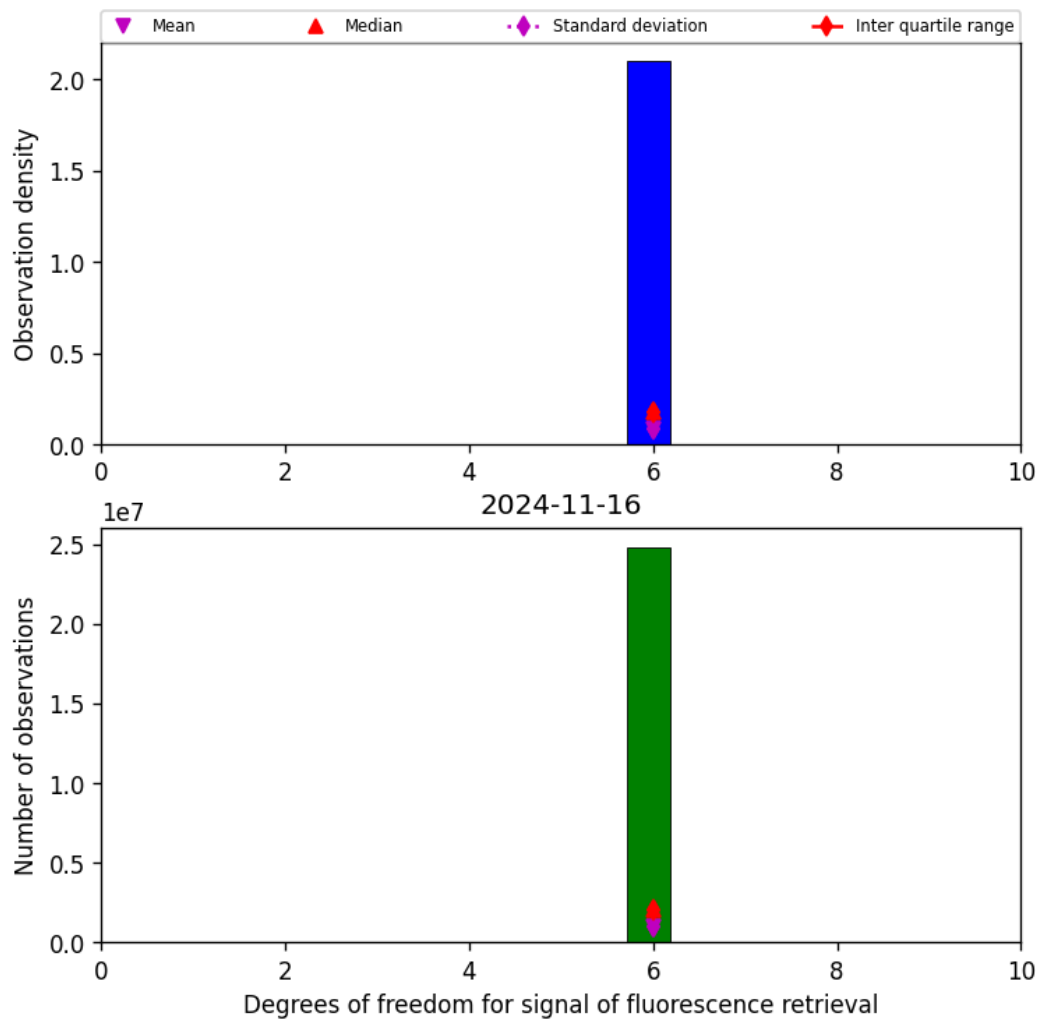
Figure 43: Histogram of “Degrees of freedom for signal of fluorescence retrieval” for 2024-11-15 to 2024-11-17
