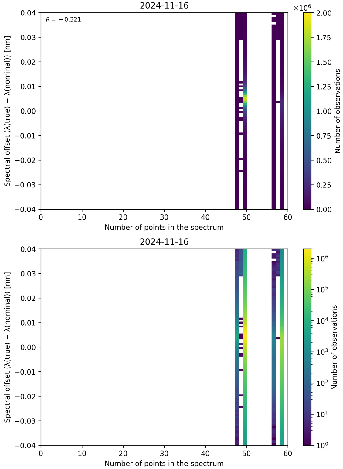
Figure 110: Scatter density plot of “Number of points in the spectrum” against “Spectral offset ( \lambda_{\text{true}} - \lambda_{\text{nominal}} )” for 2024-11-15 to 2024-11-17.
