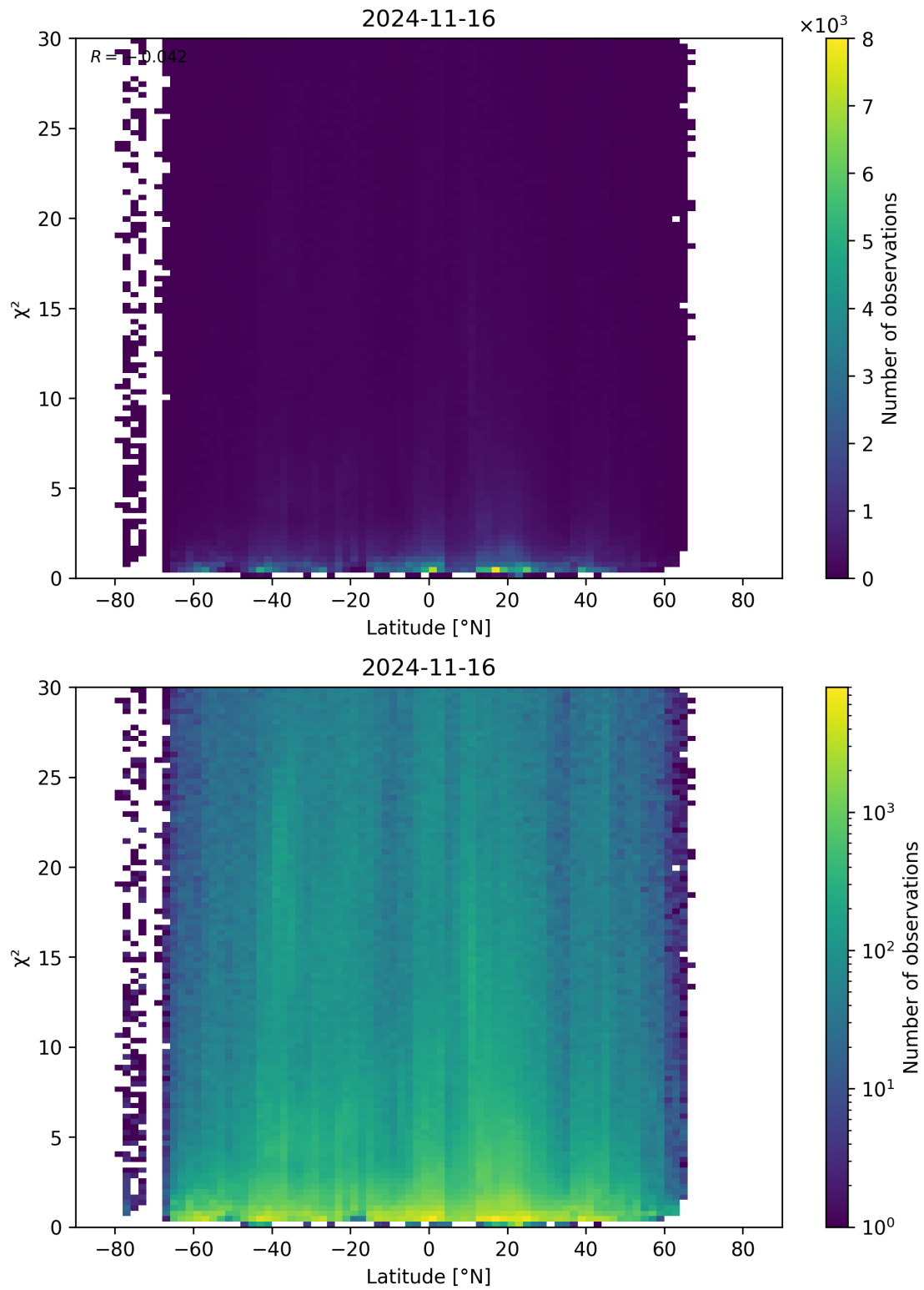
Figure 97: Scatter density plot of “Latitude” against “ \chi^2 ” for 2024-11-15 to 2024-11-17.
