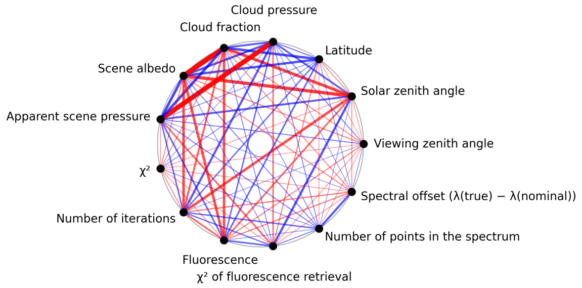
Figure 1: Map of correlation graph for 2024-11-15 to 2024-11-17.
