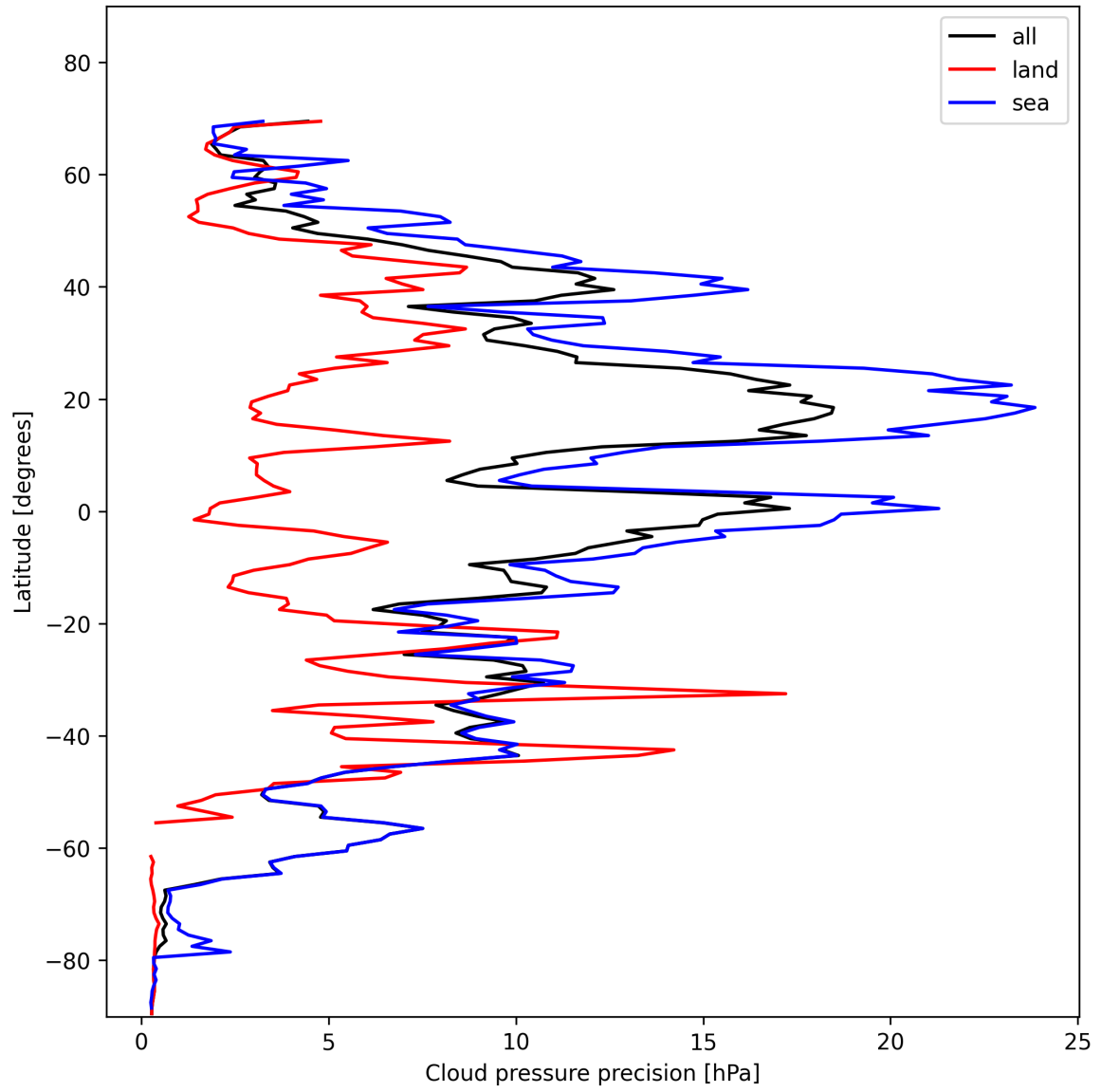
Figure 14: Zonal average of “Cloud pressure precision” for 2024-11-15 to 2024-11-17.
