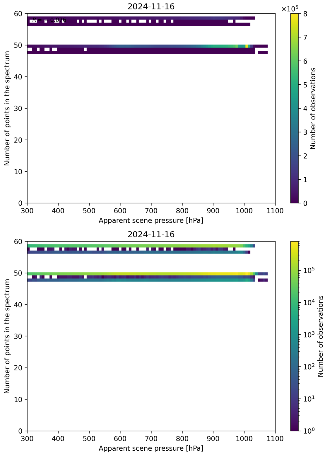
Figure 67: Scatter density plot of “Apparent scene pressure” against “Number of points in the spectrum” for 2024-11-15 to 2024-11-17.
