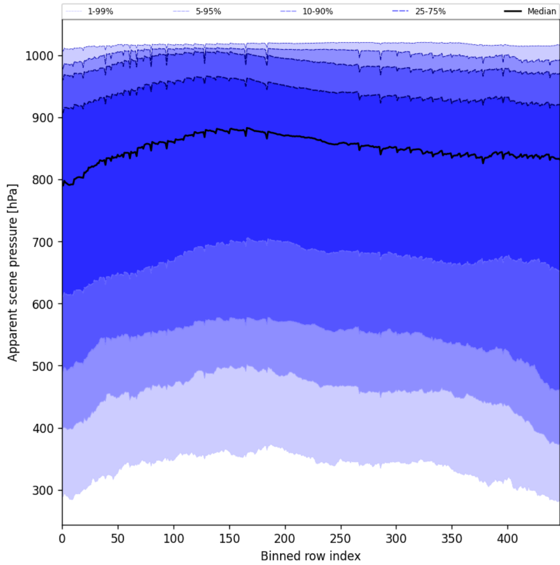
Figure 53: Along track statistics of “Apparent scene pressure” for 2024-11-15 to 2024-11-17
