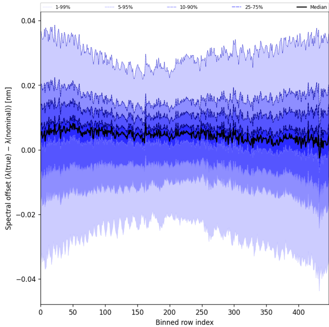
Figure 62: Along track statistics of “Spectral offset ( \lambda_{\text{true}} - \lambda_{\text{nominal}} )” for 2024-11-15 to 2024-11-17
