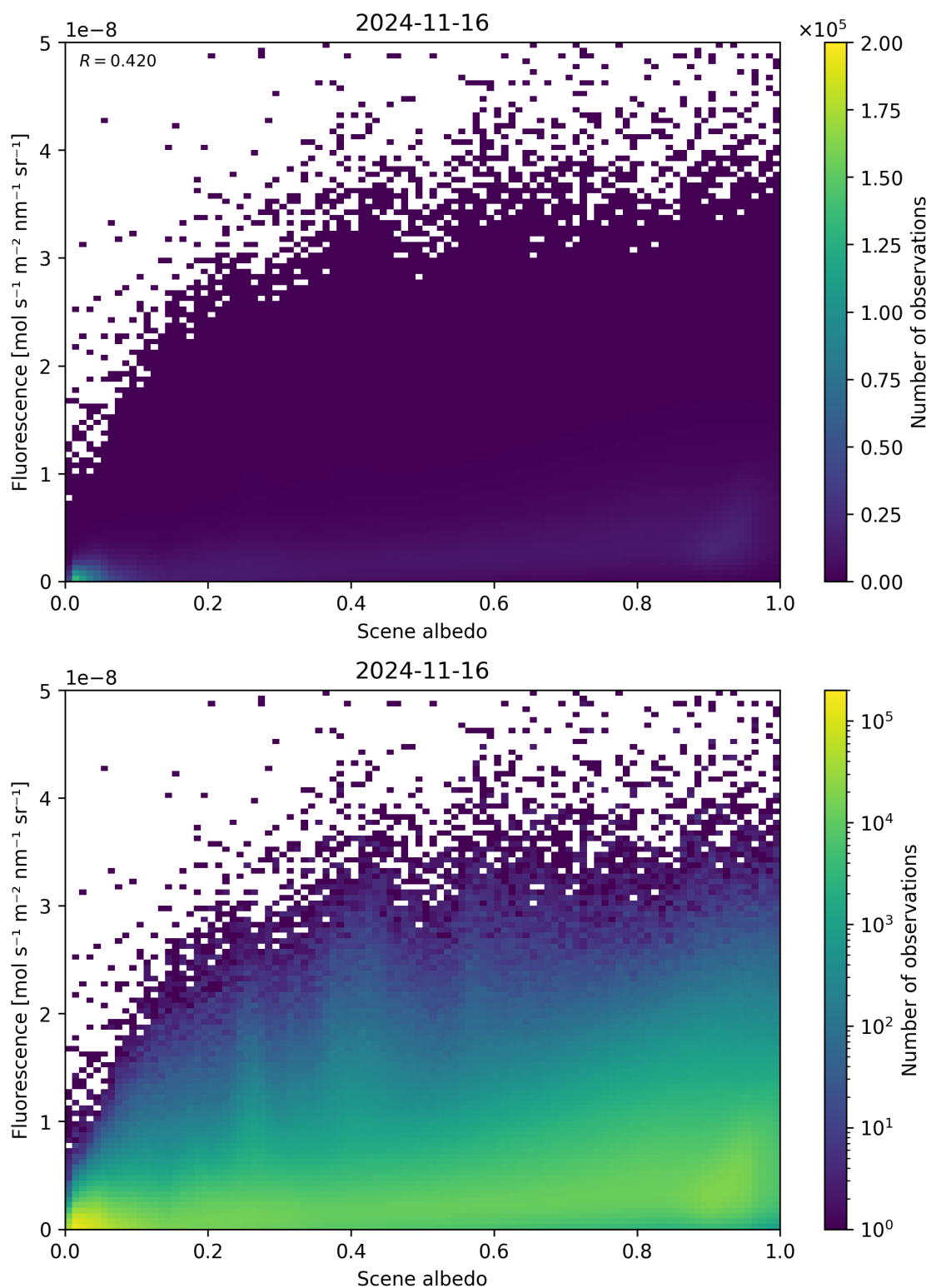
Figure 114: Scatter density plot of “Scene albedo” against “Fluorescence” for 2024-11-15 to 2024-11-17.
