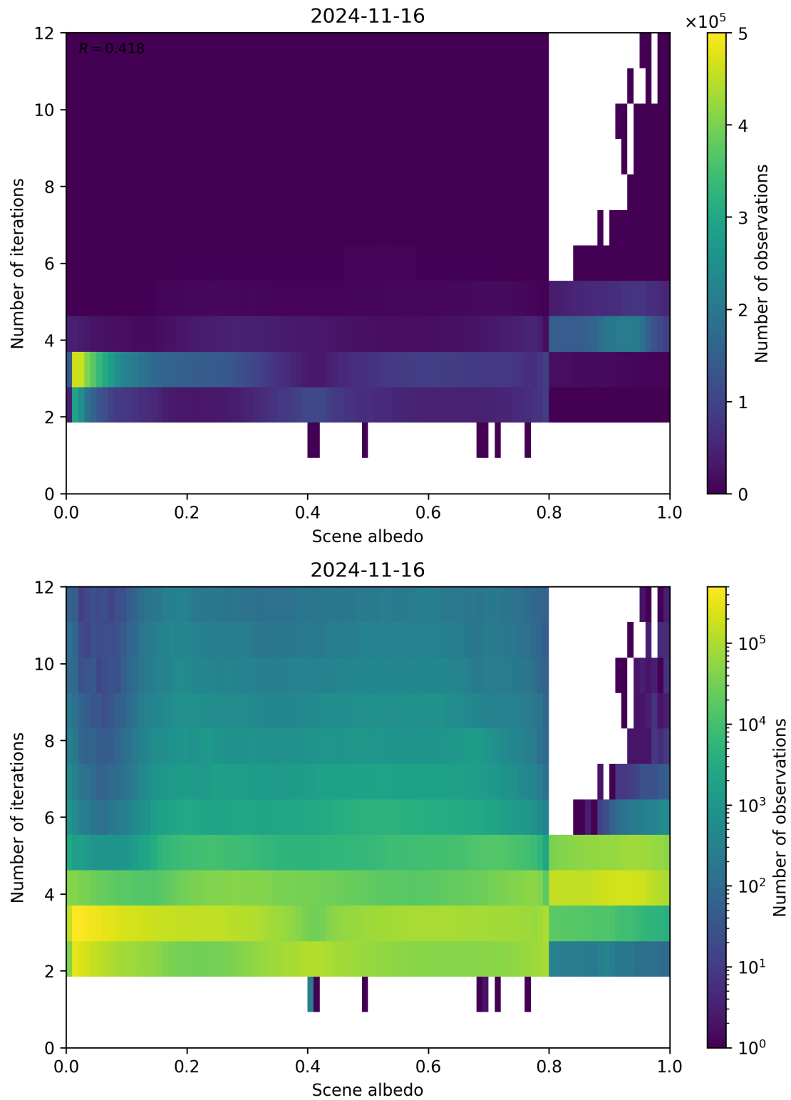
Figure 115: Scatter density plot of “Scene albedo” against “Number of iterations” for 2024-11-15 to 2024-11-17.
