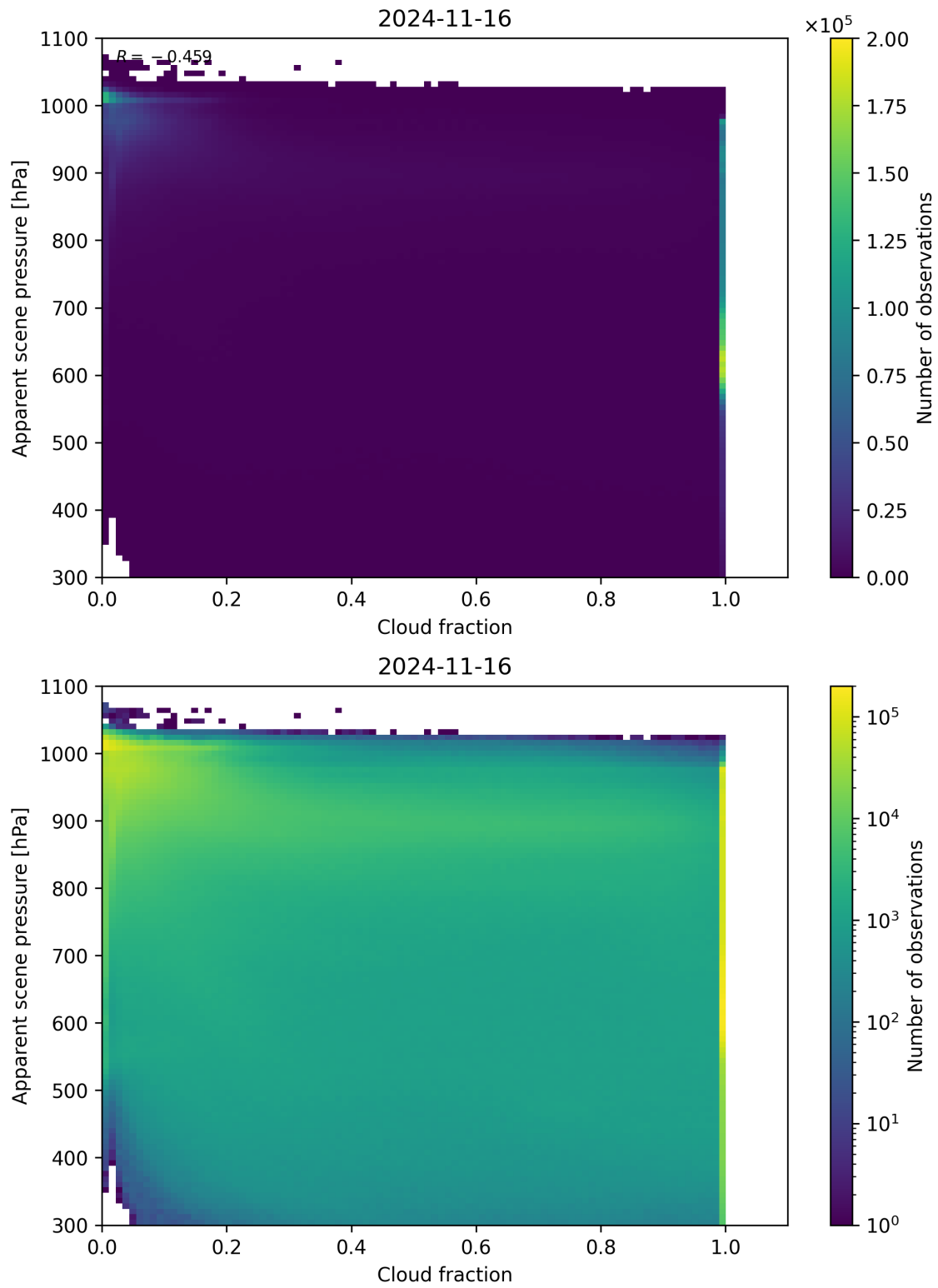
Figure 76: Scatter density plot of “Cloud fraction” against “Apparent scene pressure” for 2024-11-15 to 2024-11-17.
