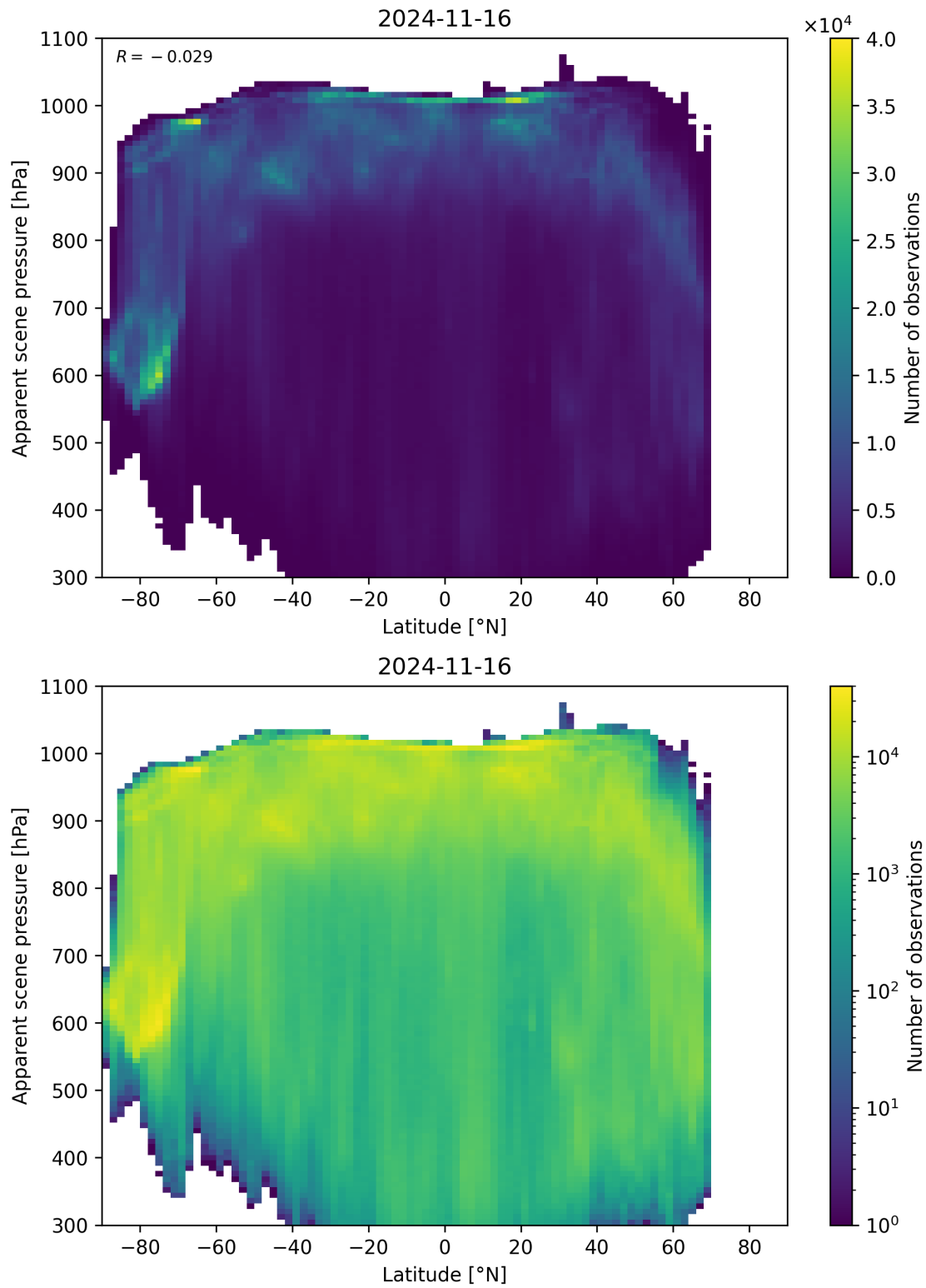
Figure 96: Scatter density plot of “Latitude” against “Apparent scene pressure” for 2024-11-15 to 2024-11-17.
