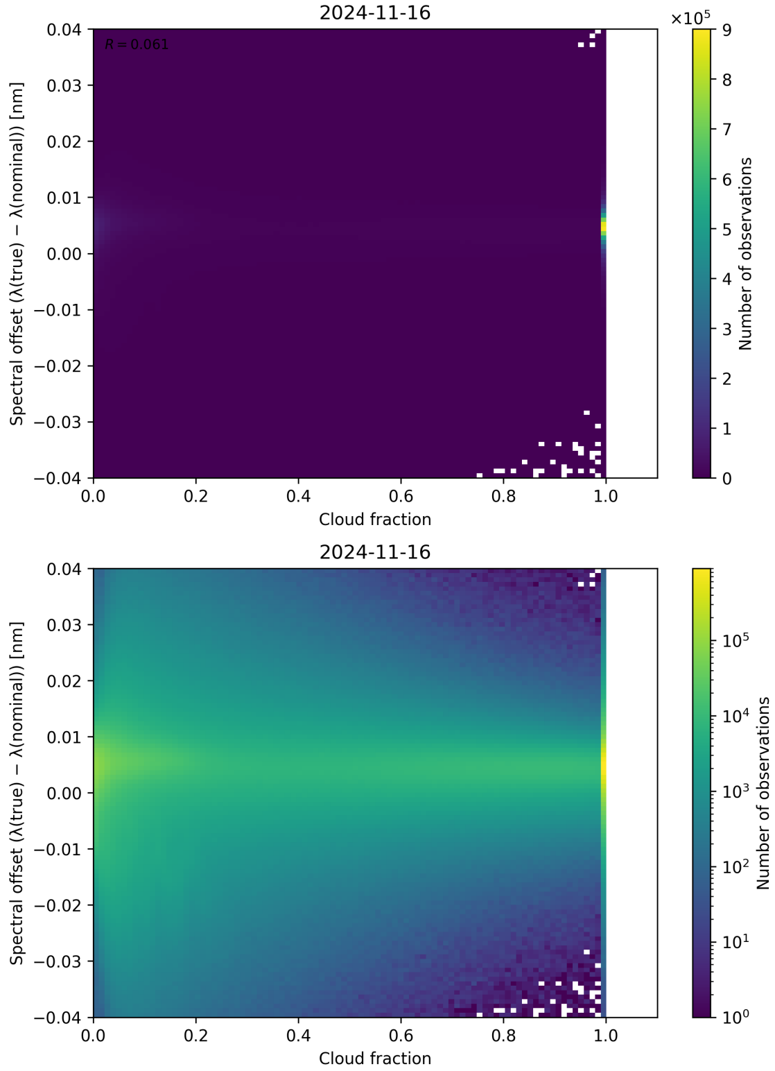
Figure 83: Scatter density plot of “Cloud fraction” against “Spectral offset ( \lambda_{\text{true}} - \lambda_{\text{nominal}} )” for 2024-11-15 to 2024-11-17.
