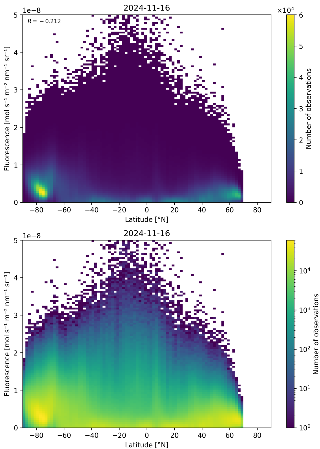
Figure 101: Scatter density plot of “Latitude” against “Fluorescence” for 2024-11-15 to 2024-11-17.
