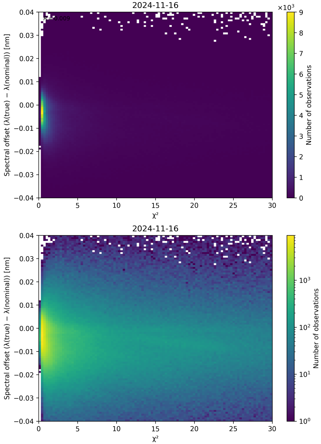
Figure 75: Scatter density plot of “ \chi^2 ” against “Spectral offset ( \lambda_{\text{true}} - \lambda_{\text{nominal}} )” for 2024-11-15 to 2024-11-17.
