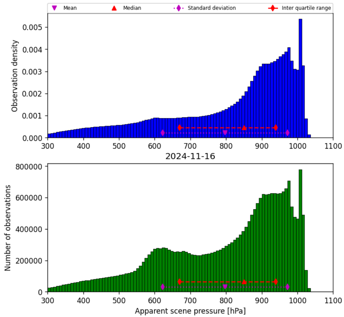
Figure 36: Histogram of “Apparent scene pressure” for 2024-11-15 to 2024-11-17
