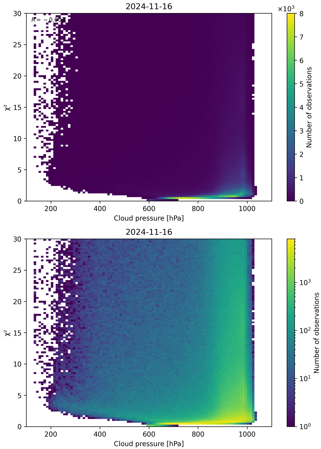
Figure 85: Scatter density plot of “Cloud pressure” against “ \chi^2 ” for 2024-11-15 to 2024-11-17.
