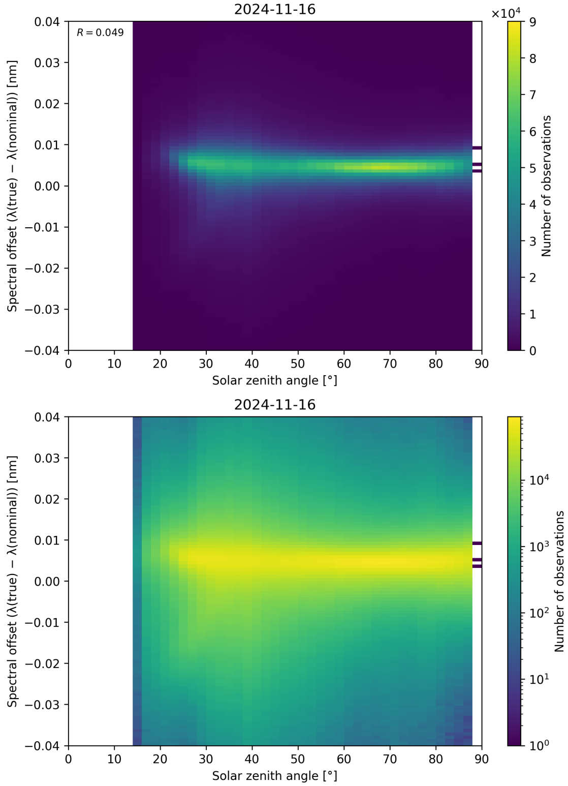
Figure 128: Scatter density plot of “Solar zenith angle” against “Spectral offset ( \lambda_{\text{true}} - \lambda_{\text{nominal}} )” for 2024-11-15 to 2024-11-17.
