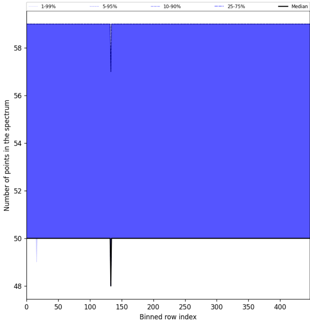
Figure 61: Along track statistics of “Number of points in the spectrum” for 2024-11-15 to 2024-11-17
