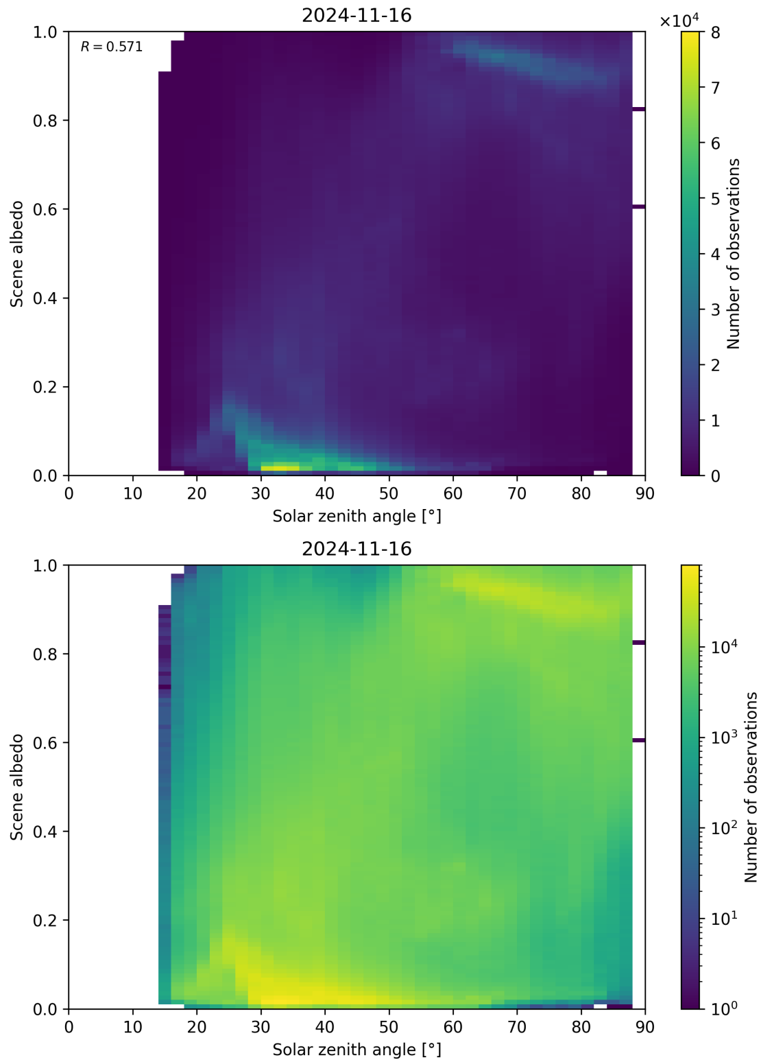
Figure 127: Scatter density plot of “Solar zenith angle” against “Scene albedo” for 2024-11-15 to 2024-11-17.
