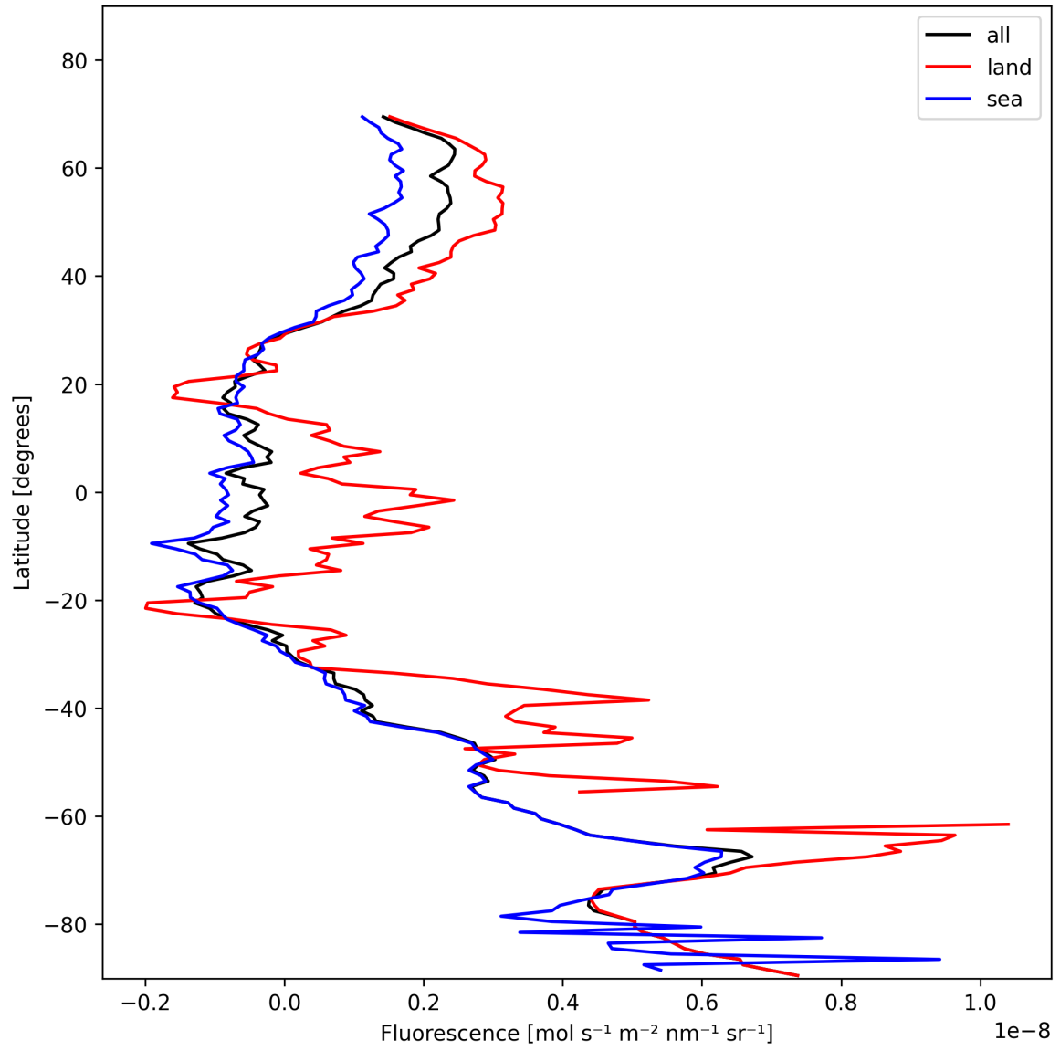
Figure 23: Zonal average of “Fluorescence” for 2024-11-15 to 2024-11-17.
