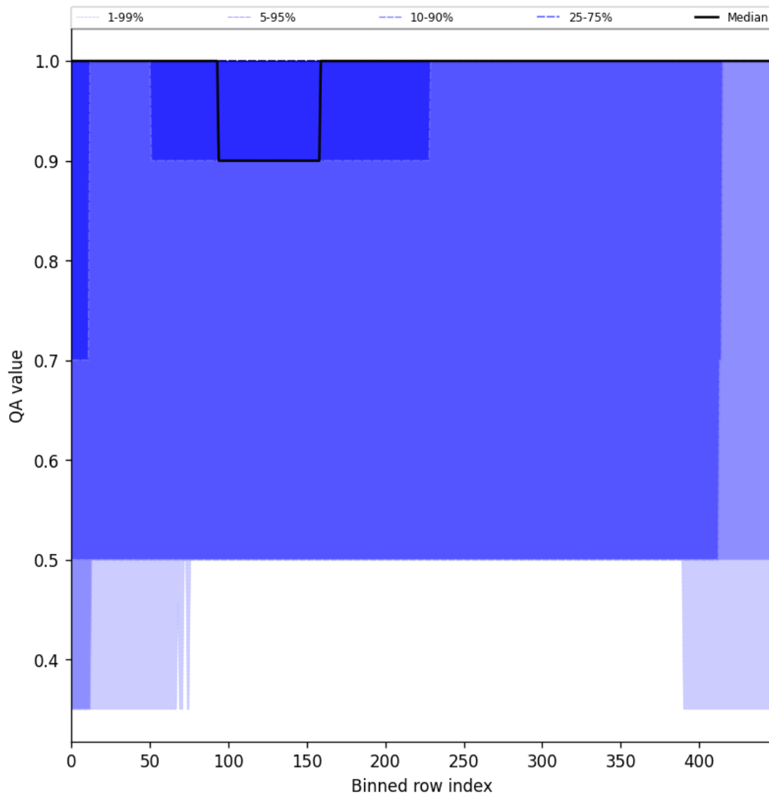
Figure 46: Along track statistics of “QA value” for 2024-11-15 to 2024-11-17
