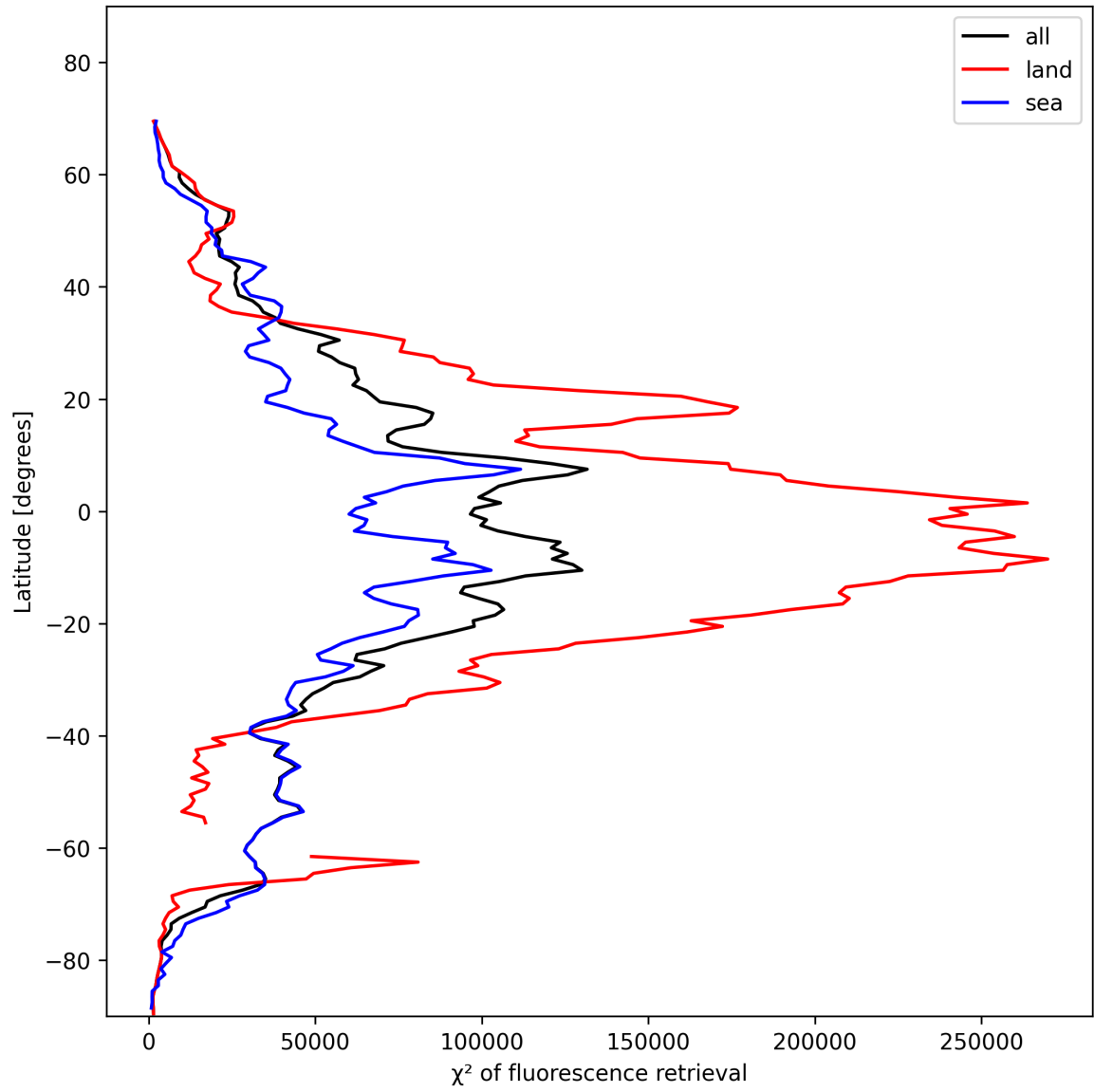
Figure 25: Zonal average of “ \chi^2 of fluorescence retrieval” for 2024-11-15 to 2024-11-17.
