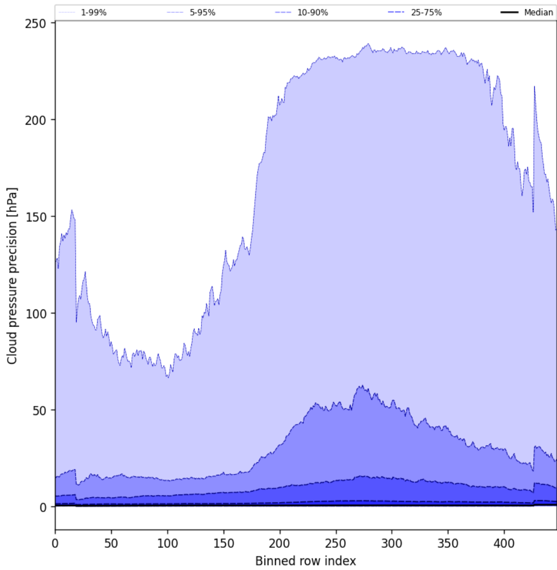
Figure 48: Along track statistics of “Cloud pressure precision” for 2024-11-15 to 2024-11-17
