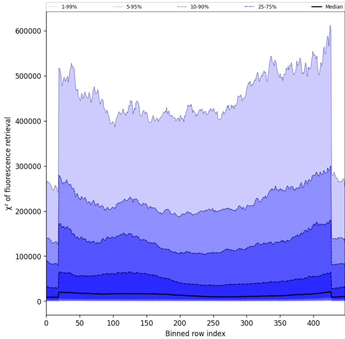
Figure 59: Along track statistics of “ \chi^2 of fluorescence retrieval” for 2024-11-15 to 2024-11-17
