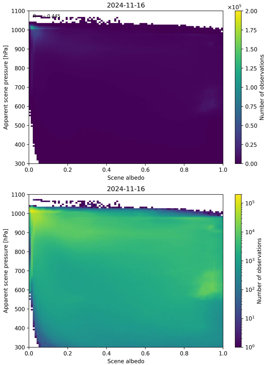
Figure 111: Scatter density plot of “Scene albedo” against “Apparent scene pressure” for 2024-11-15 to 2024-11-17.
