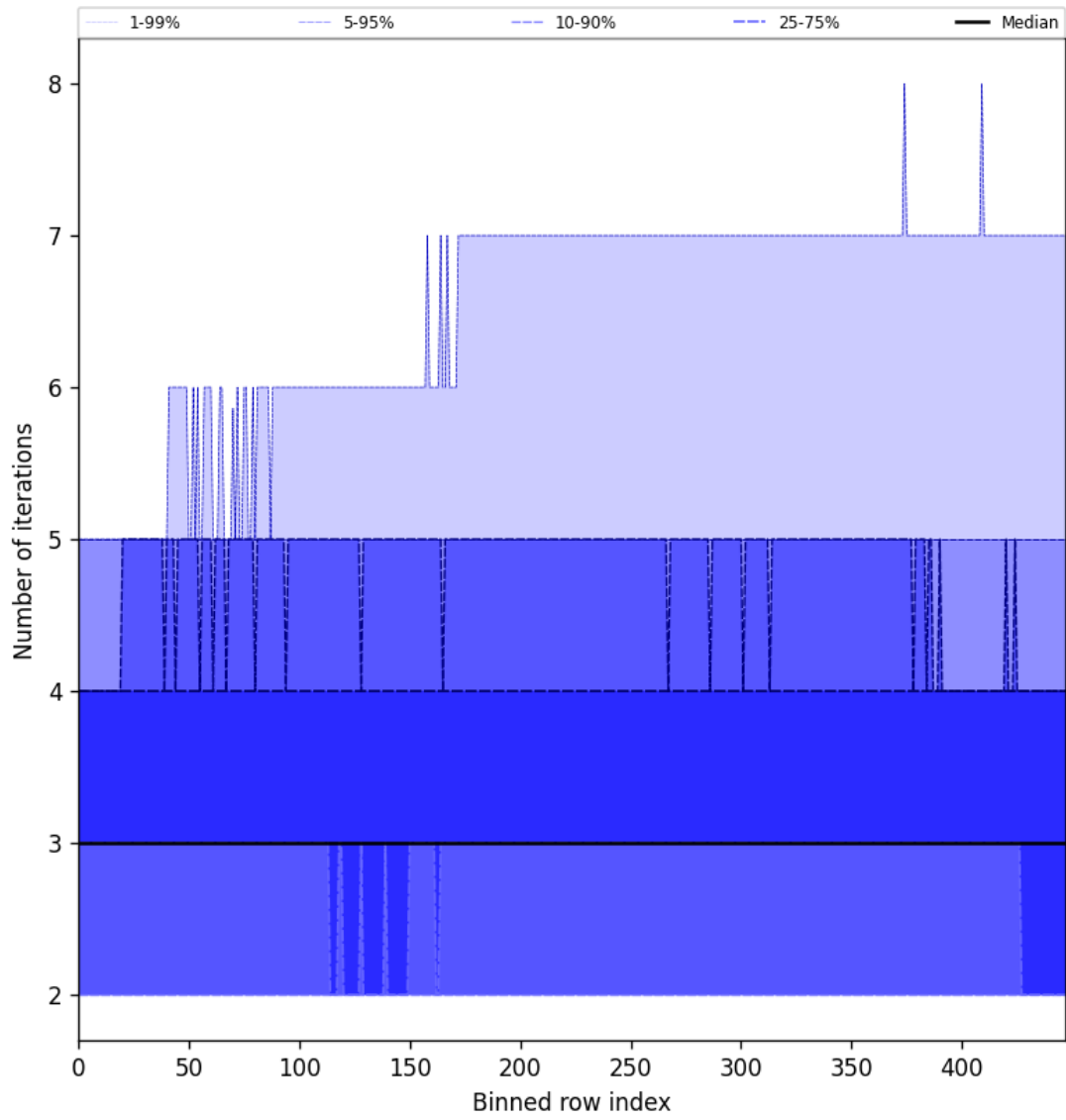
Figure 56: Along track statistics of “Number of iterations” for 2024-11-15 to 2024-11-17
