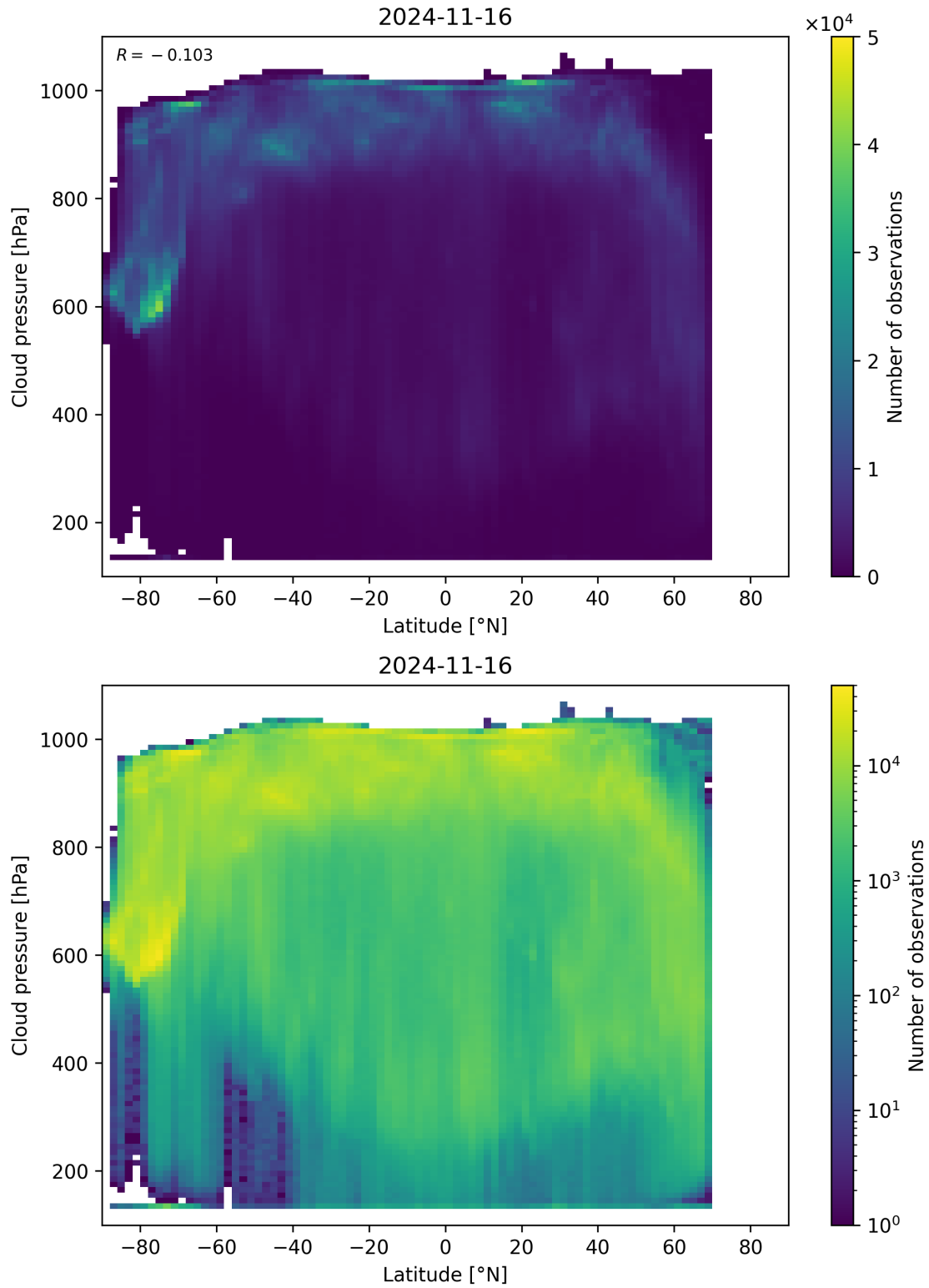
Figure 100: Scatter density plot of “Latitude” against “Cloud pressure” for 2024-11-15 to 2024-11-17.
