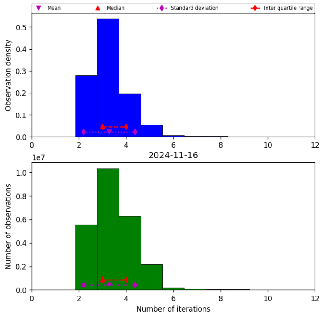
Figure 39: Histogram of “Number of iterations” for 2024-11-15 to 2024-11-17
