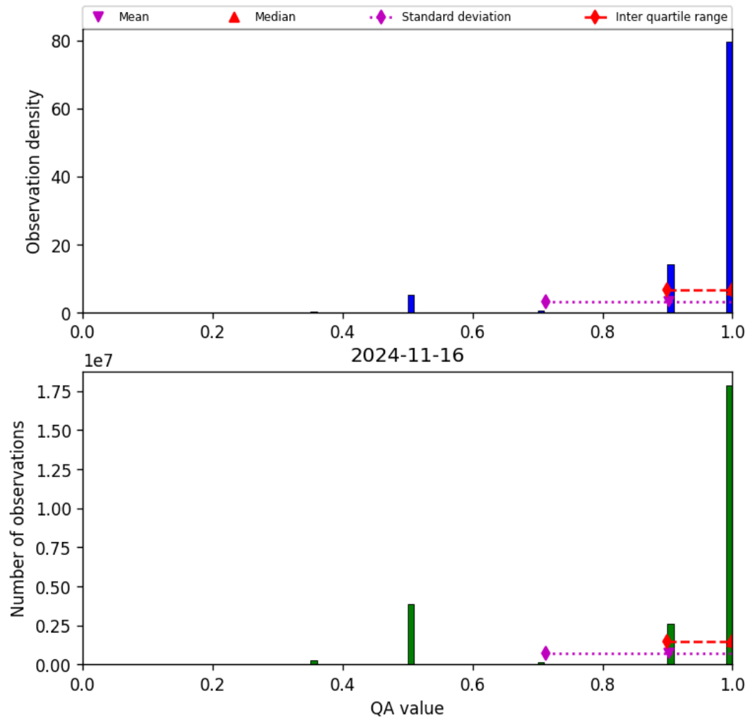
Figure 29: Histogram of “QA value” for 2024-11-15 to 2024-11-17
