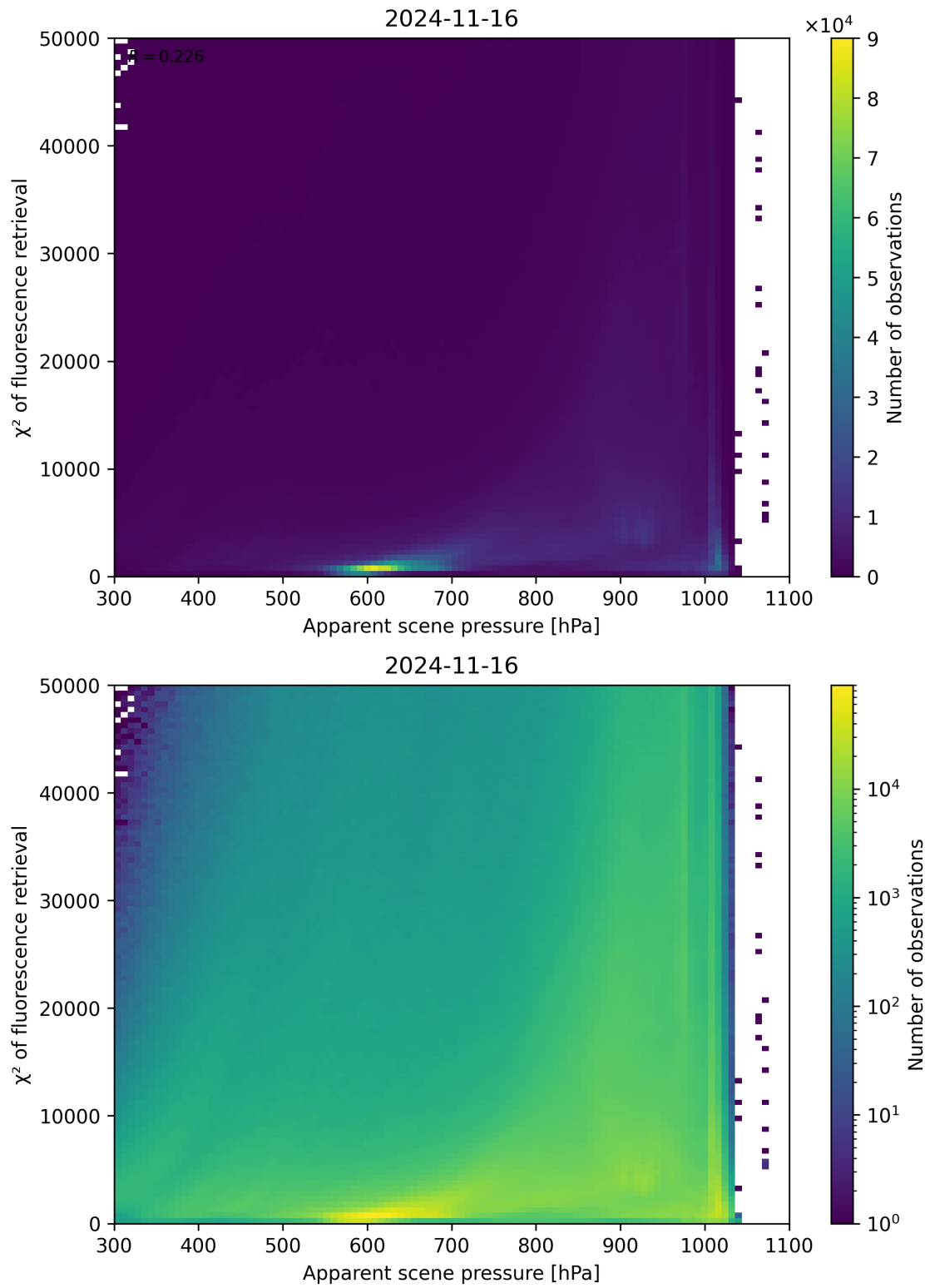
Figure 64: Scatter density plot of “Apparent scene pressure” against “ \chi^2 of fluorescence retrieval” for 2024-11-15 to 2024-11-17.
