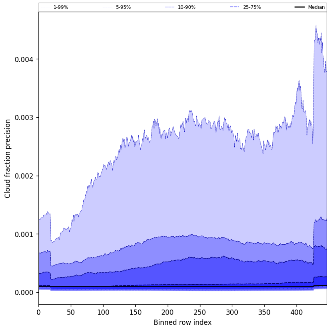
Figure 50: Along track statistics of “Cloud fraction precision” for 2024-11-15 to 2024-11-17
