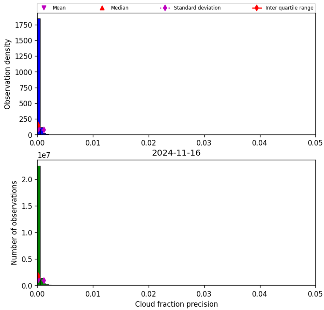
Figure 33: Histogram of “Cloud fraction precision” for 2024-11-15 to 2024-11-17
