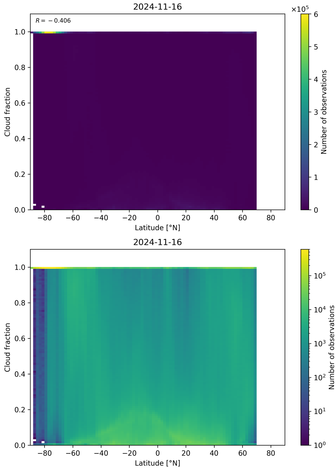
Figure 99: Scatter density plot of “Latitude” against “Cloud fraction” for 2024-11-15 to 2024-11-17.
