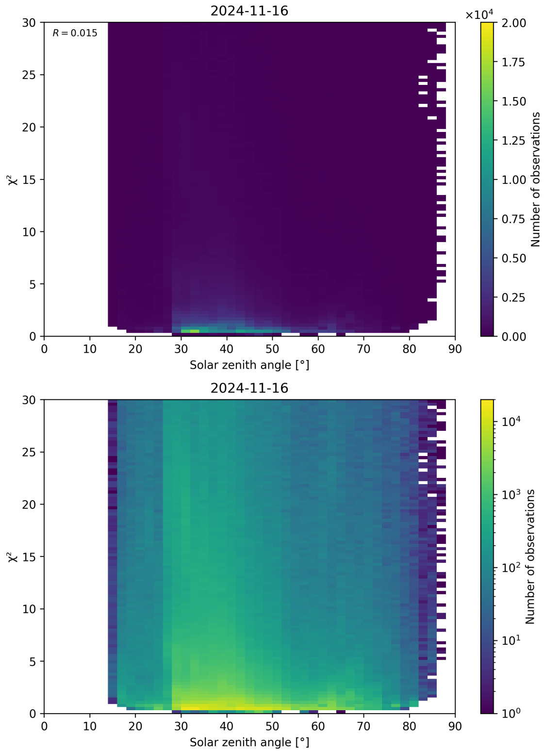
Figure 119: Scatter density plot of “Solar zenith angle” against “ \chi^2 ” for 2024-11-15 to 2024-11-17.
