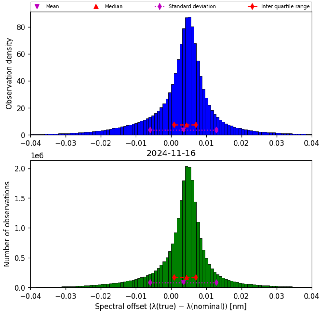
Figure 45: Histogram of “Spectral offset ( \lambda_{\text{true}} - \lambda_{\text{nominal}} )” for 2024-11-15 to 2024-11-17
