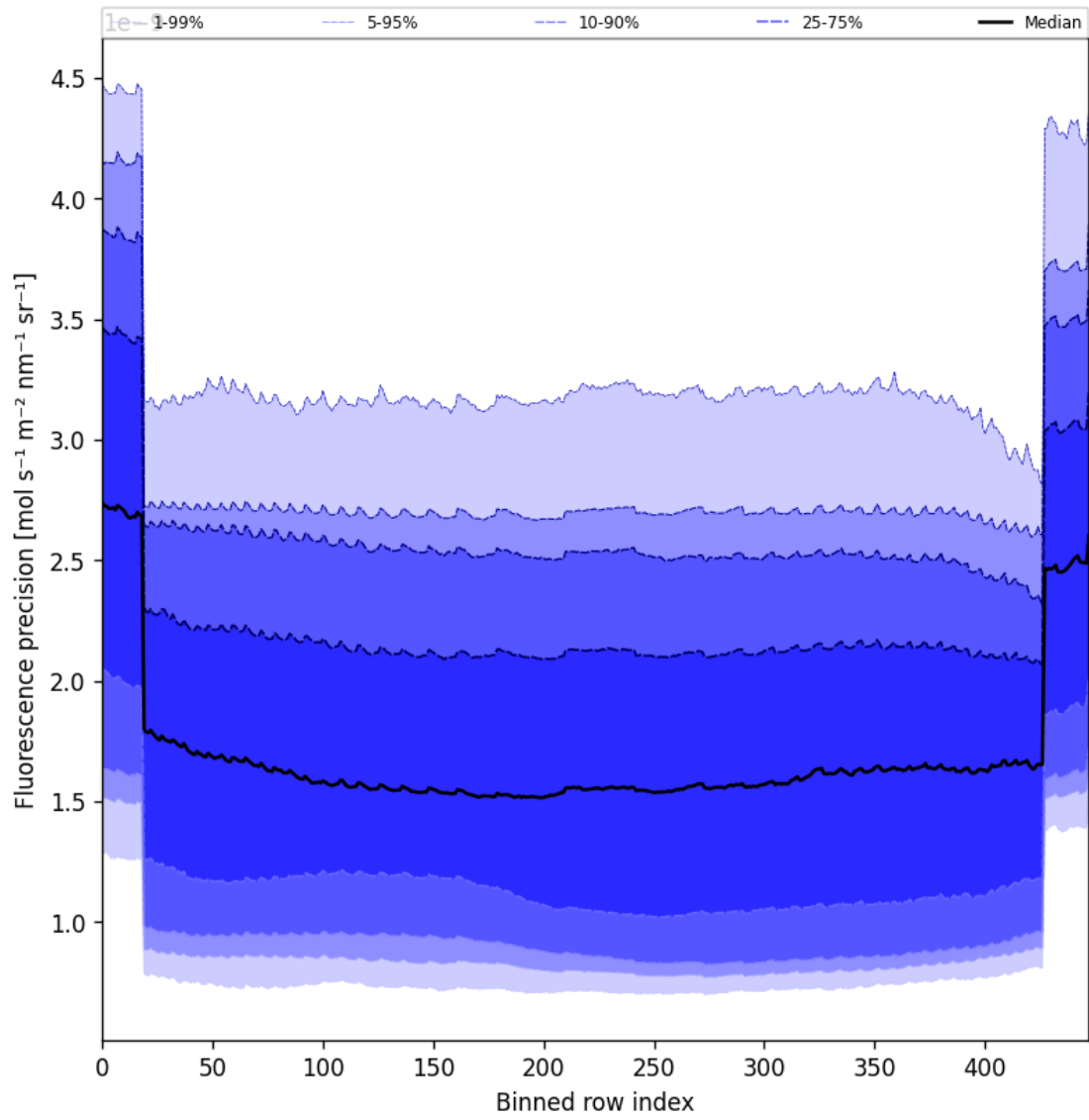
Figure 58: Along track statistics of “Fluorescence precision” for 2024-11-15 to 2024-11-17
