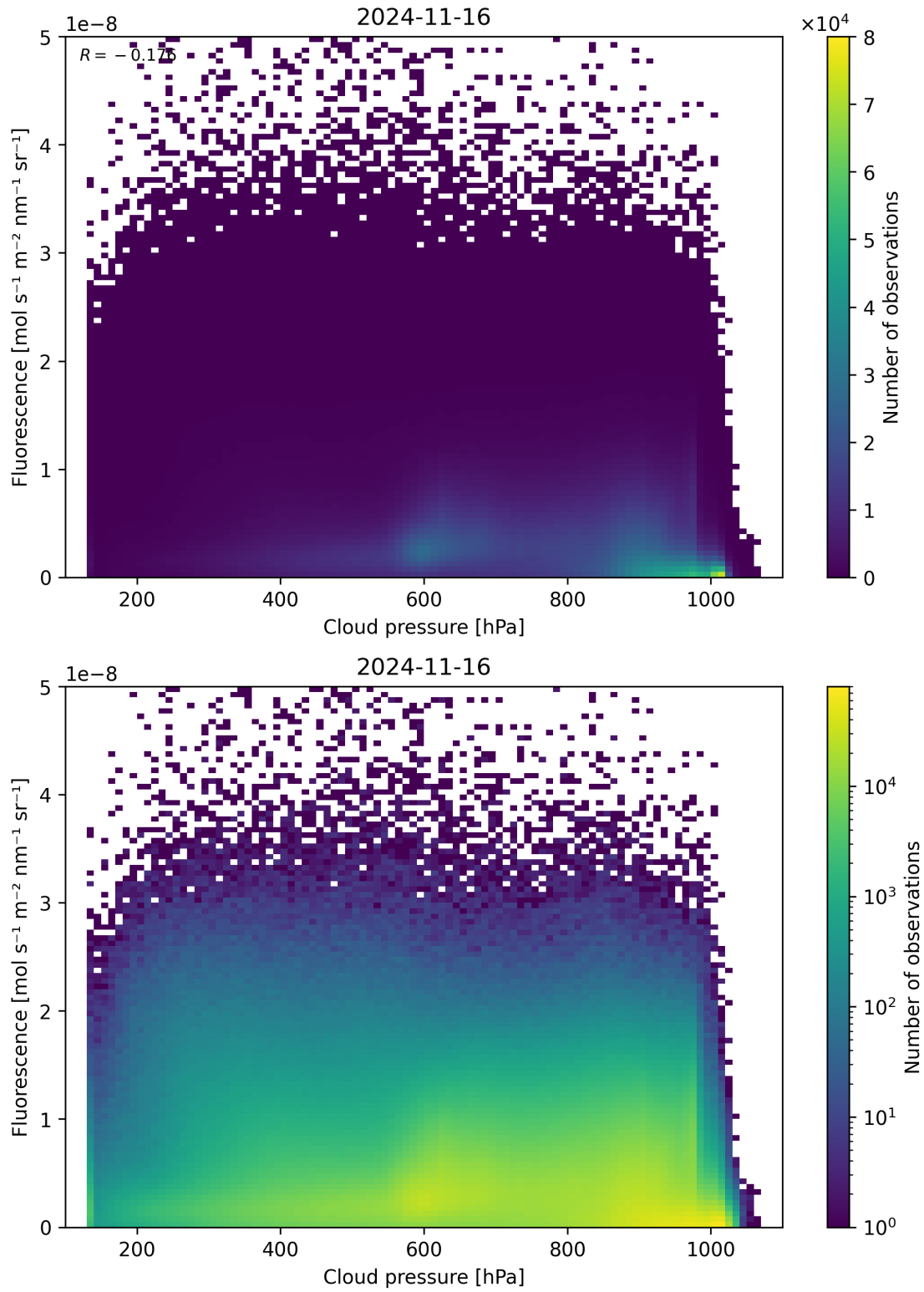
Figure 88: Scatter density plot of “Cloud pressure” against “Fluorescence” for 2024-11-15 to 2024-11-17.
