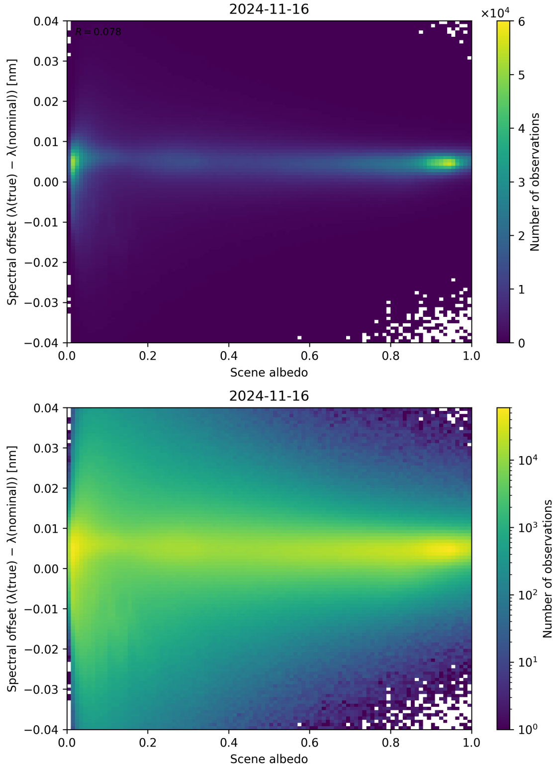
Figure 117: Scatter density plot of “Scene albedo” against “Spectral offset ( \lambda_{\text{true}} - \lambda_{\text{nominal}} )” for 2024-11-15 to 2024-11-17.
