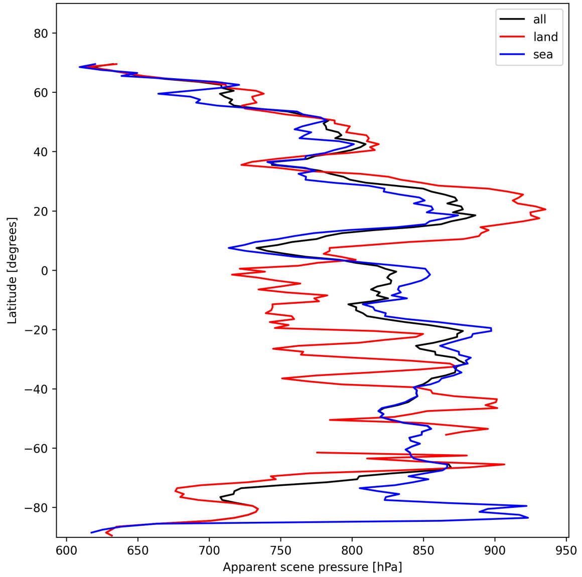
Figure 19: Zonal average of “Apparent scene pressure” for 2024-11-15 to 2024-11-17.
