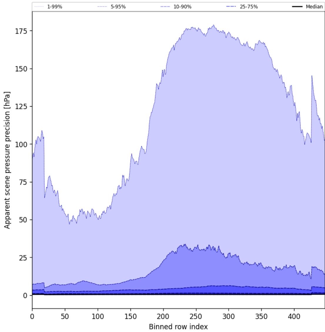
Figure 54: Along track statistics of “Apparent scene pressure precision” for 2024-11-15 to 2024-11-17
