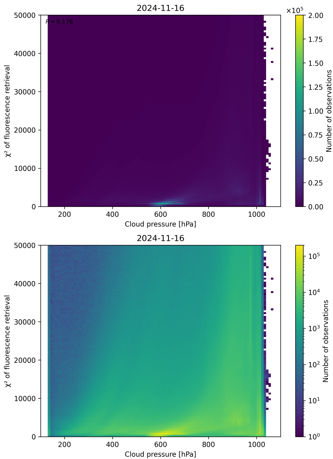
Figure 86: Scatter density plot of “Cloud pressure” against “ \chi^2 of fluorescence retrieval” for 2024-11-15 to 2024-11-17.
