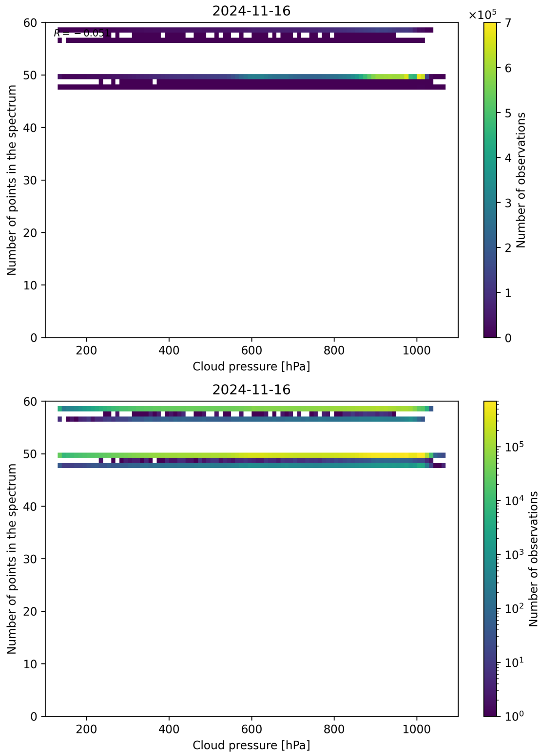
Figure 90: Scatter density plot of “Cloud pressure” against “Number of points in the spectrum” for 2024-11-15 to 2024-11-17.
