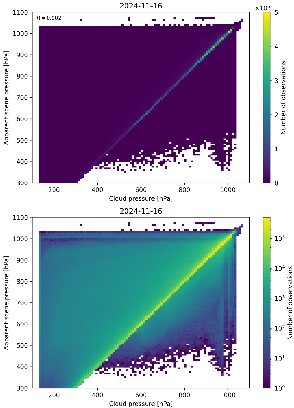
Figure 84: Scatter density plot of “Cloud pressure” against “Apparent scene pressure” for 2024-11-15 to 2024-11-17.
