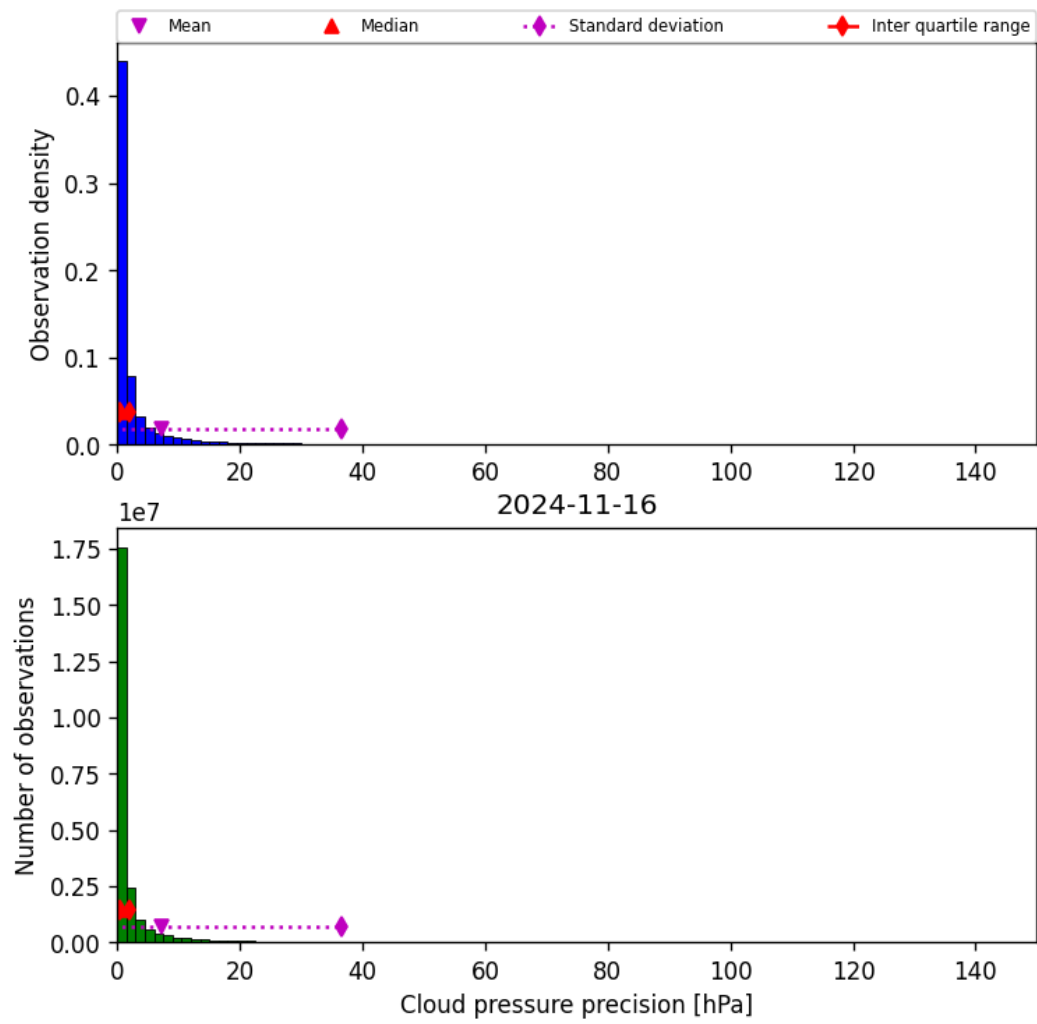
Figure 31: Histogram of “Cloud pressure precision” for 2024-11-15 to 2024-11-17
