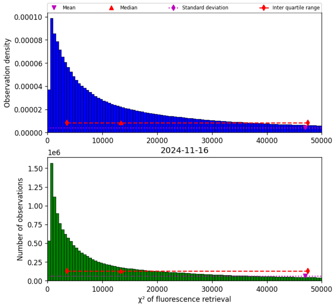
Figure 42: Histogram of “ \chi^2 of fluorescence retrieval” for 2024-11-15 to 2024-11-17
