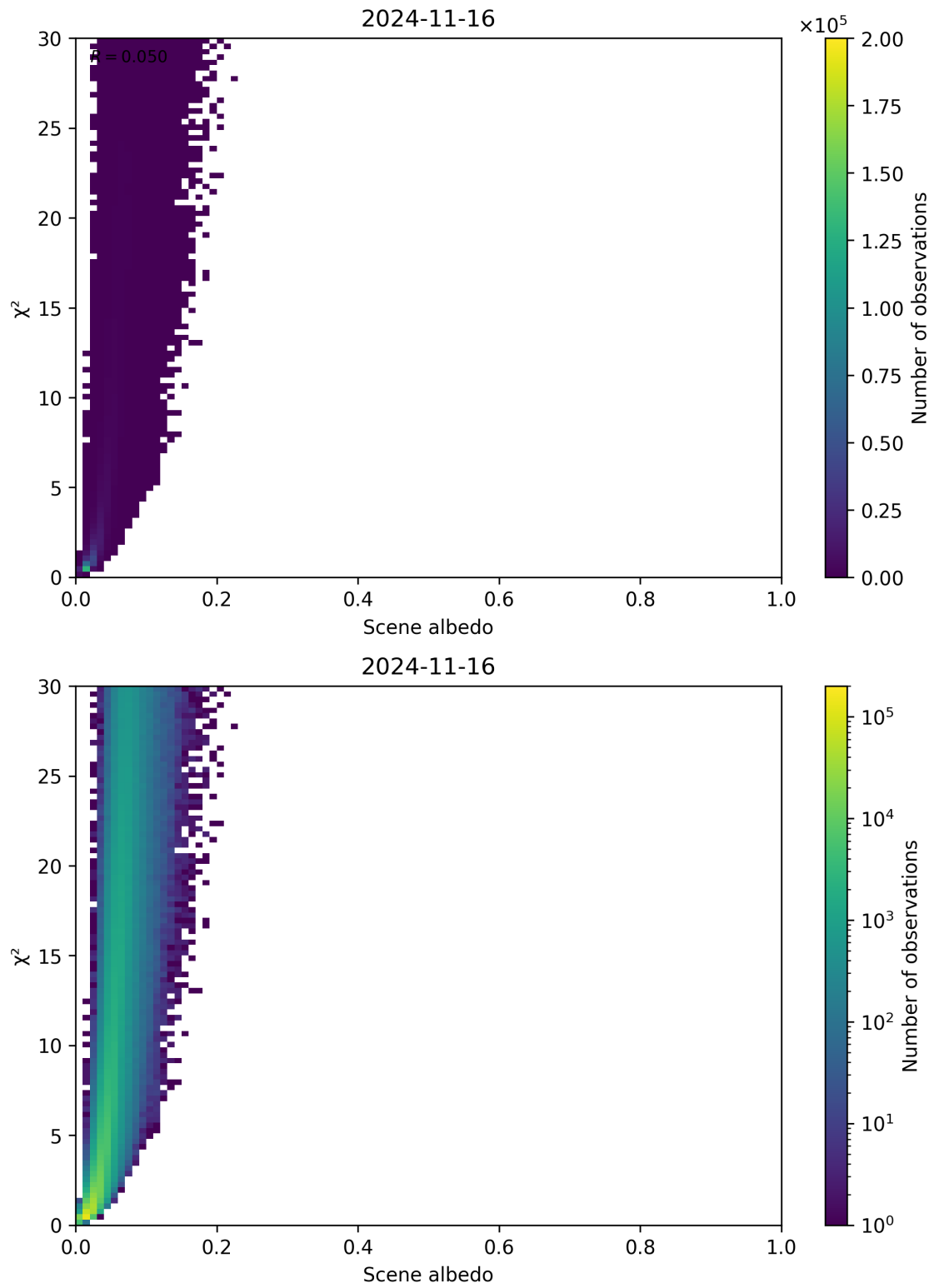
Figure 112: Scatter density plot of “Scene albedo” against “ \chi^2 ” for 2024-11-15 to 2024-11-17.
