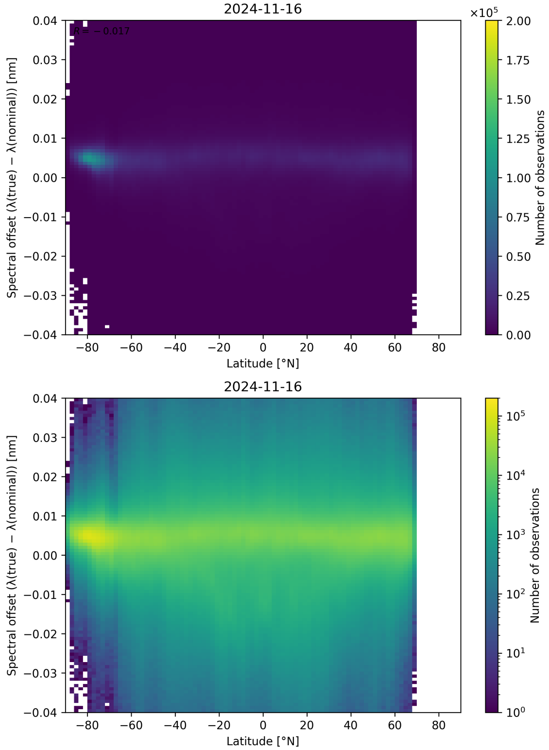
Figure 105: Scatter density plot of “Latitude” against “Spectral offset ( \lambda_{\text{true}} - \lambda_{\text{nominal}} )” for 2024-11-15 to 2024-11-17.
