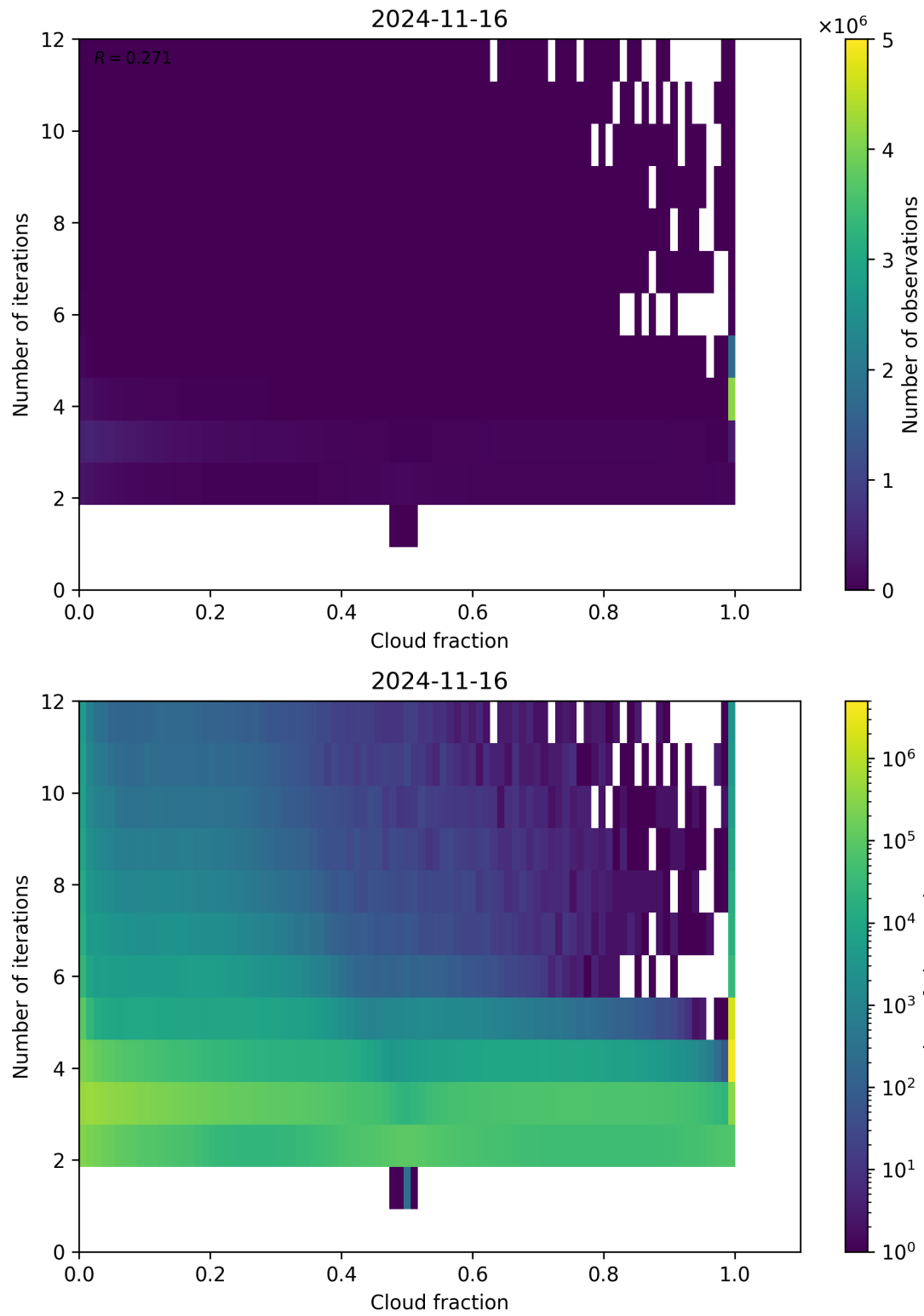
Figure 80: Scatter density plot of “Cloud fraction” against “Number of iterations” for 2024-11-15 to 2024-11-17.
