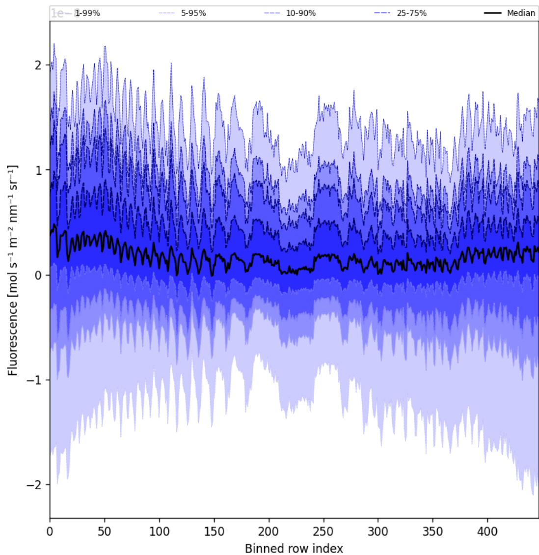
Figure 57: Along track statistics of “Fluorescence” for 2024-11-15 to 2024-11-17
