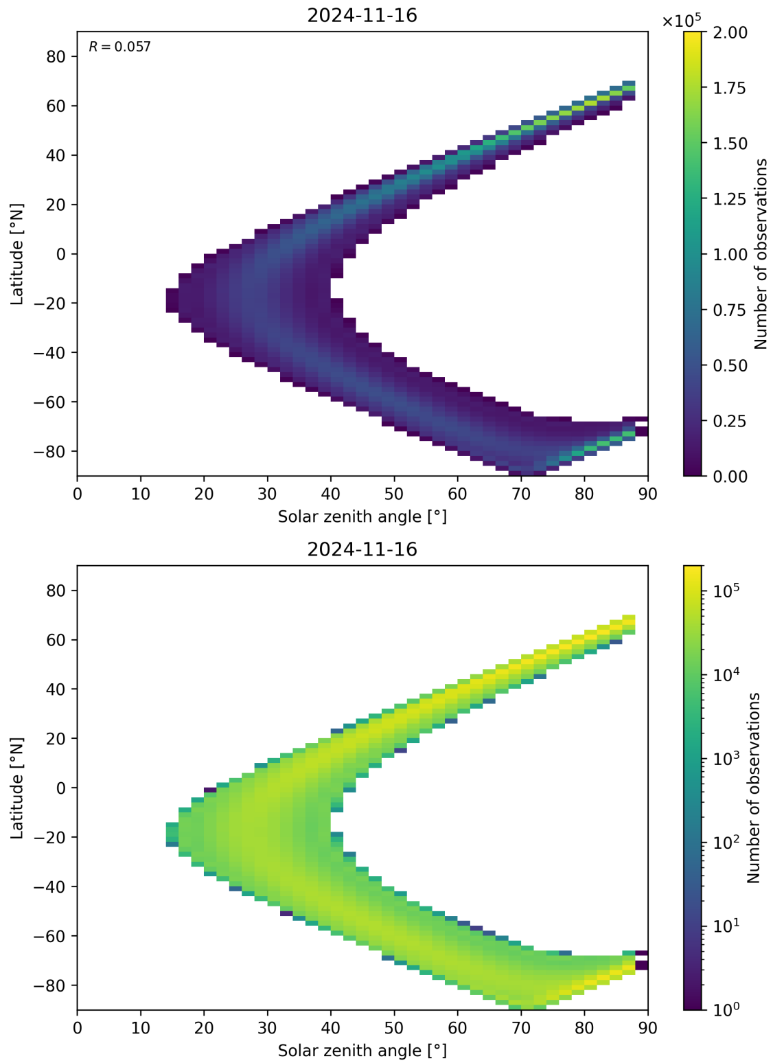
Figure 124: Scatter density plot of “Solar zenith angle” against “Latitude” for 2024-11-15 to 2024-11-17.
