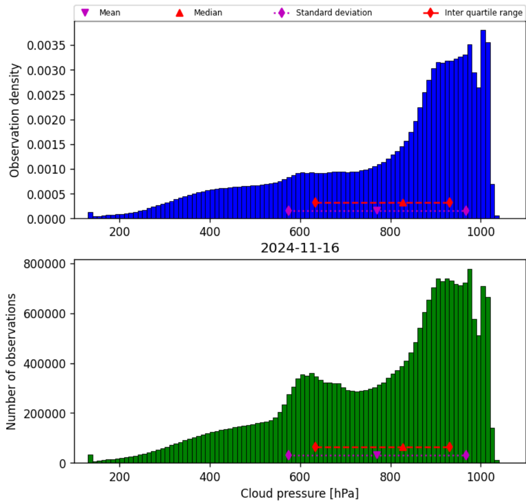
Figure 30: Histogram of “Cloud pressure” for 2024-11-15 to 2024-11-17
