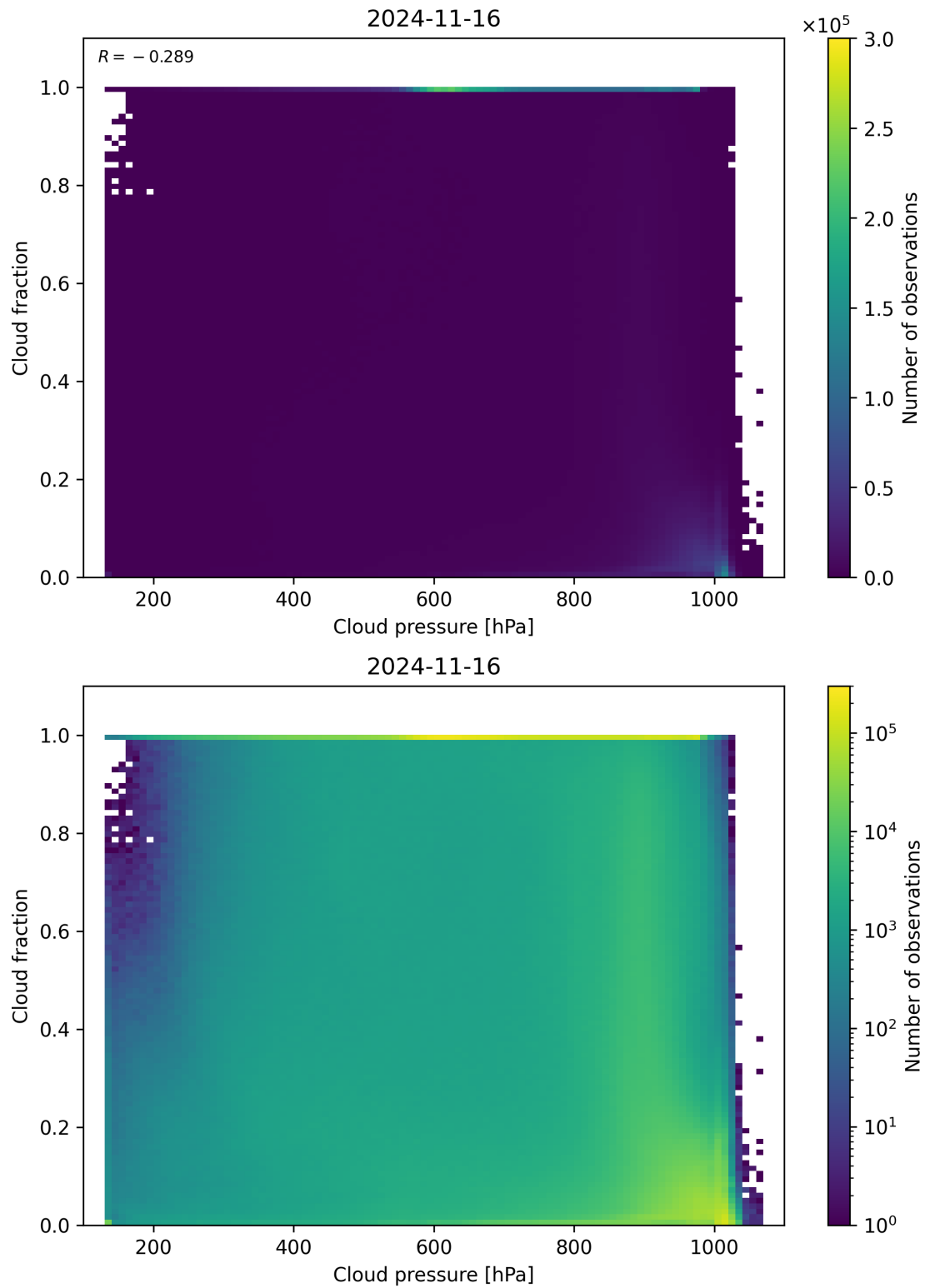
Figure 87: Scatter density plot of “Cloud pressure” against “Cloud fraction” for 2024-11-15 to 2024-11-17.
