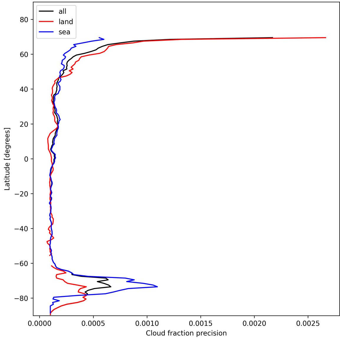
Figure 16: Zonal average of “Cloud fraction precision” for 2024-11-15 to 2024-11-17.
