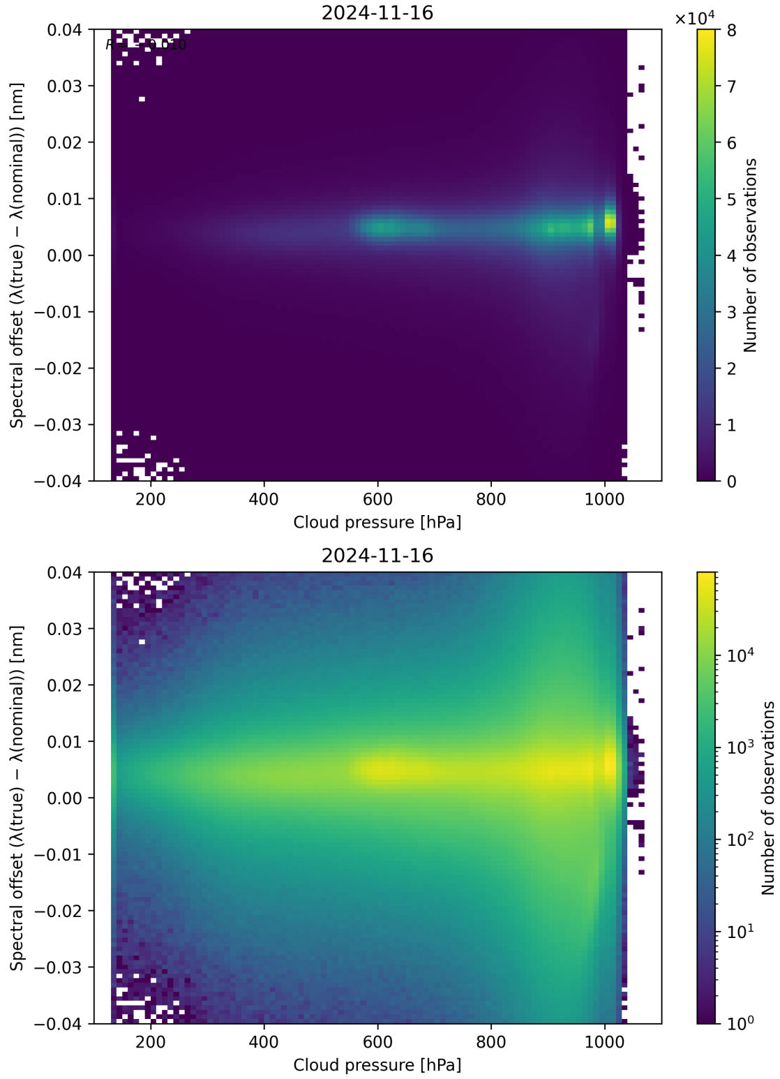
Figure 92: Scatter density plot of “Cloud pressure” against “Spectral offset ( \lambda_{\text{true}} - \lambda_{\text{nominal}} )” for 2024-11-15 to 2024-11-17.
