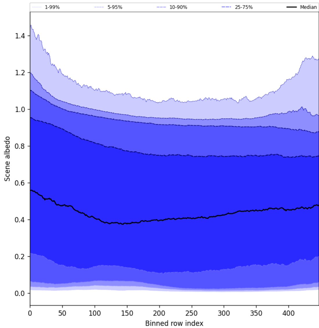
Figure 51: Along track statistics of “Scene albedo” for 2024-11-15 to 2024-11-17
