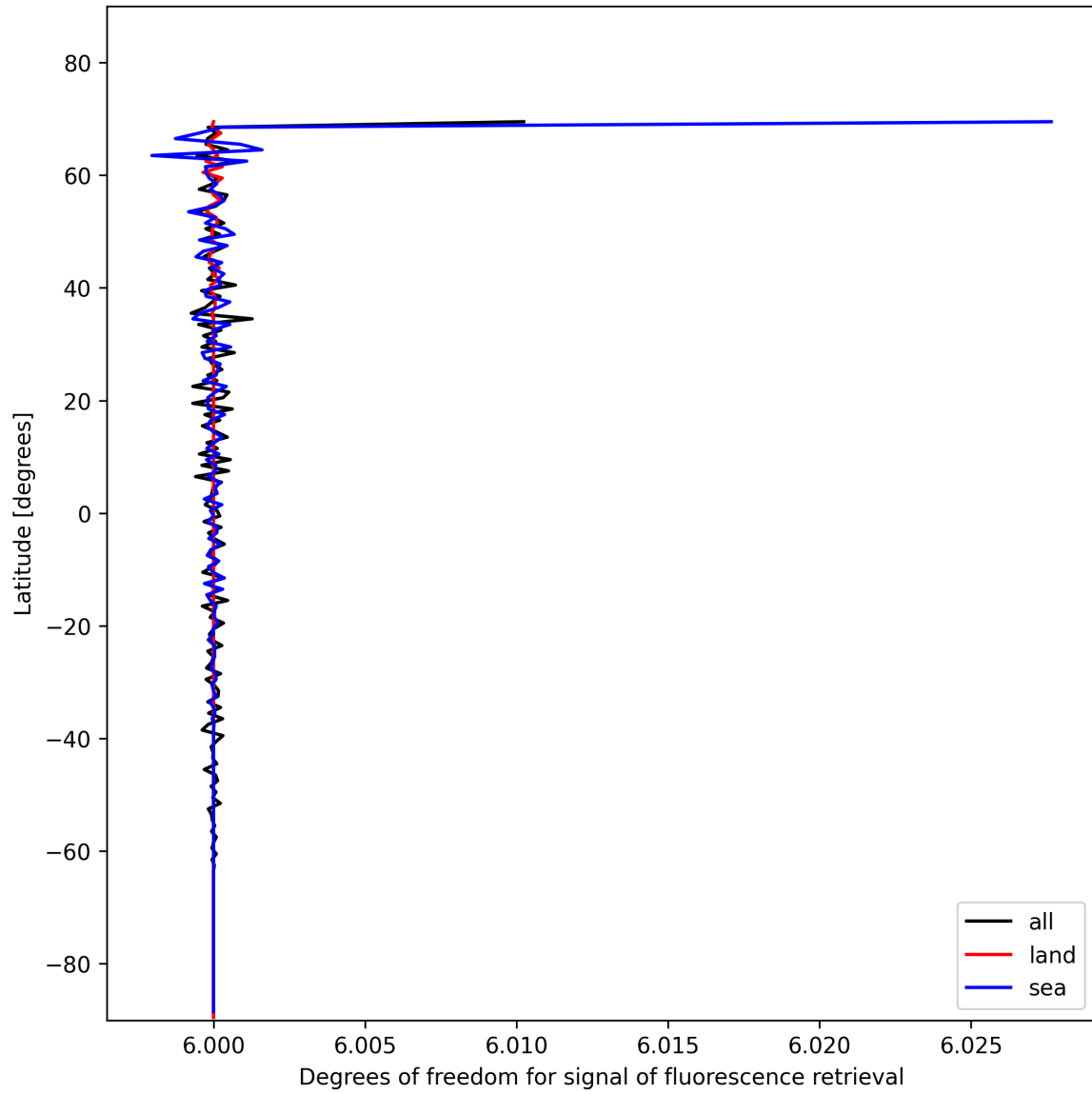
Figure 26: Zonal average of “Degrees of freedom for signal of fluorescence retrieval” for 2024-11-15 to 2024-11-17.
