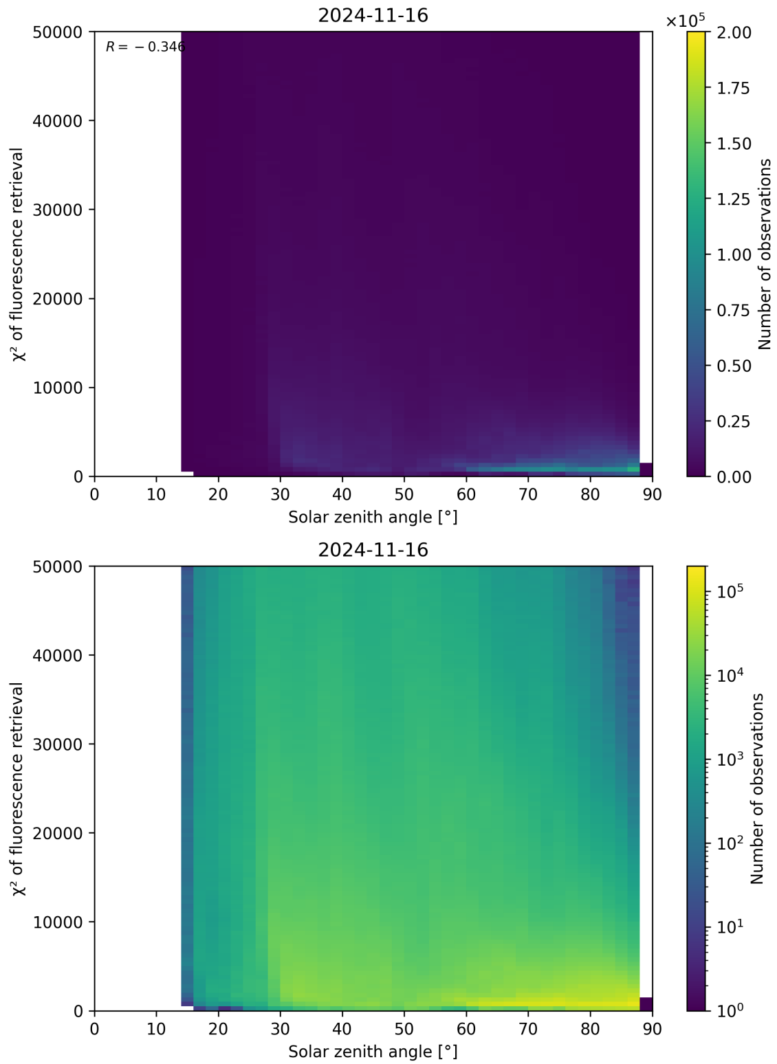
Figure 120: Scatter density plot of “Solar zenith angle” against “ \chi^2 of fluorescence retrieval” for 2024-11-15 to 2024-11-17.
