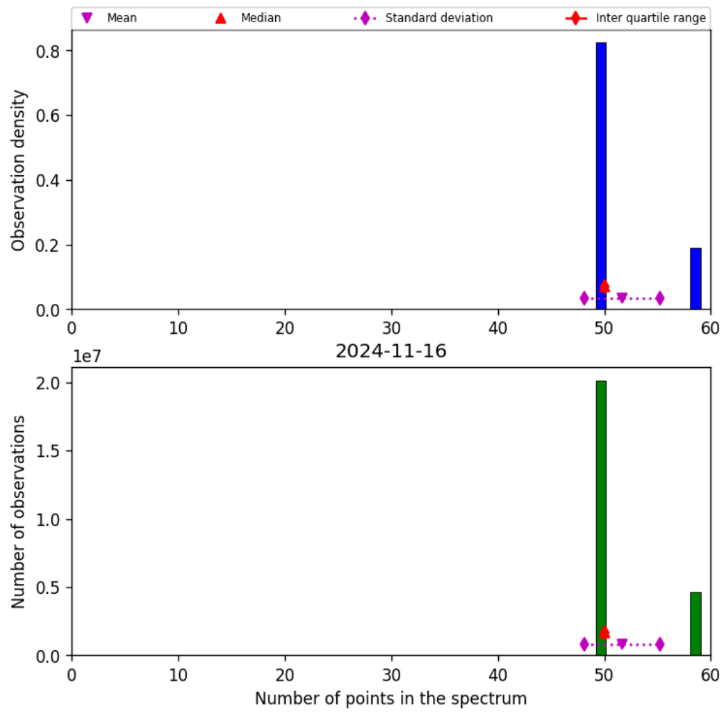
Figure 44: Histogram of “Number of points in the spectrum” for 2024-11-15 to 2024-11-17
