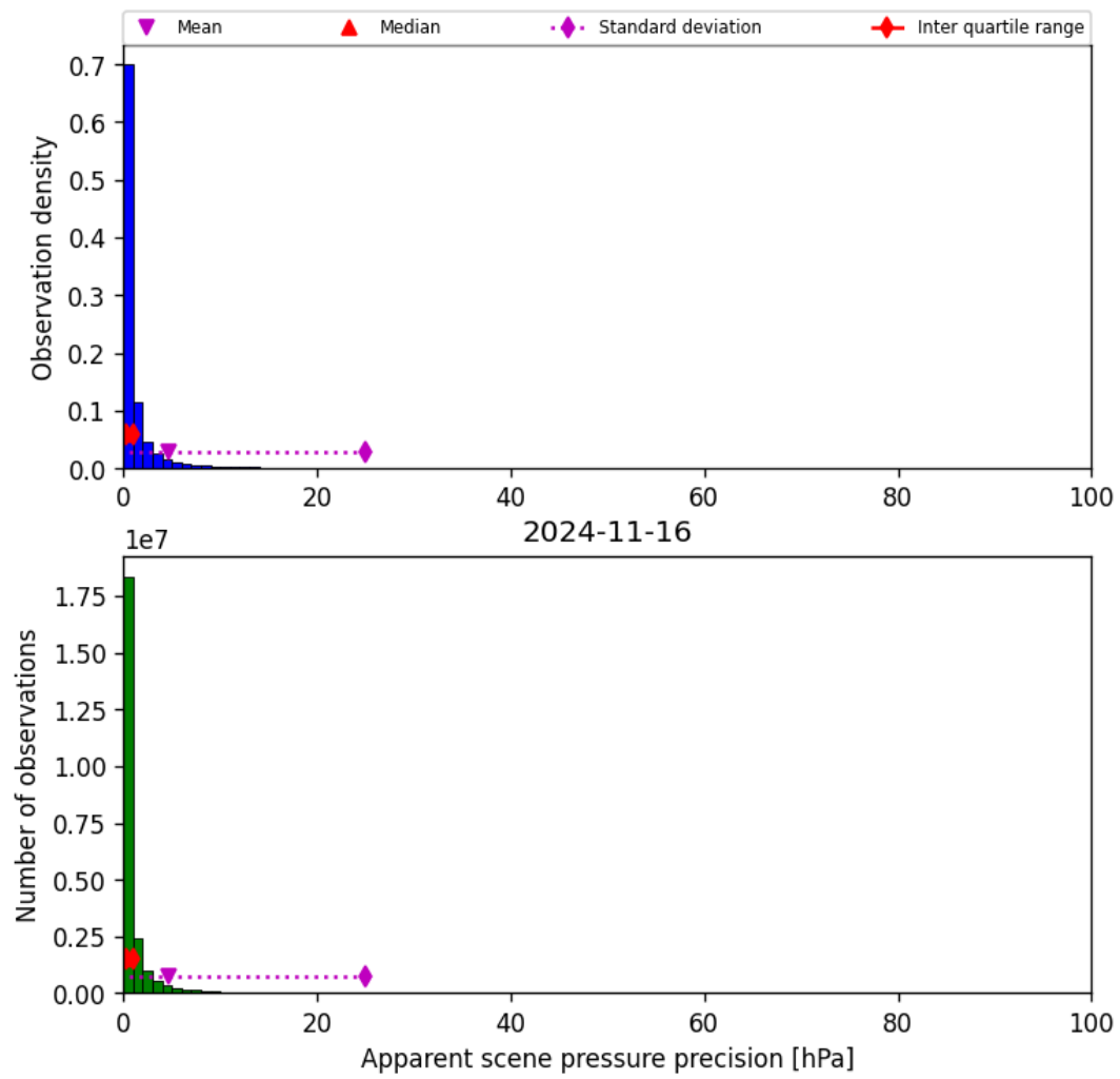
Figure 37: Histogram of “Apparent scene pressure precision” for 2024-11-15 to 2024-11-17
