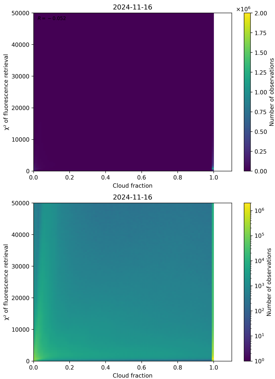
Figure 78: Scatter density plot of “Cloud fraction” against “ \chi^2 of fluorescence retrieval” for 2024-11-15 to 2024-11-17.
