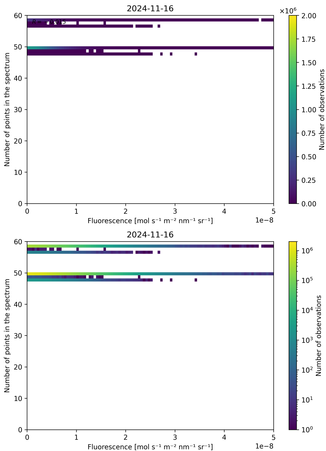
Figure 94: Scatter density plot of “Fluorescence” against “Number of points in the spectrum” for 2024-11-15 to 2024-11-17.
