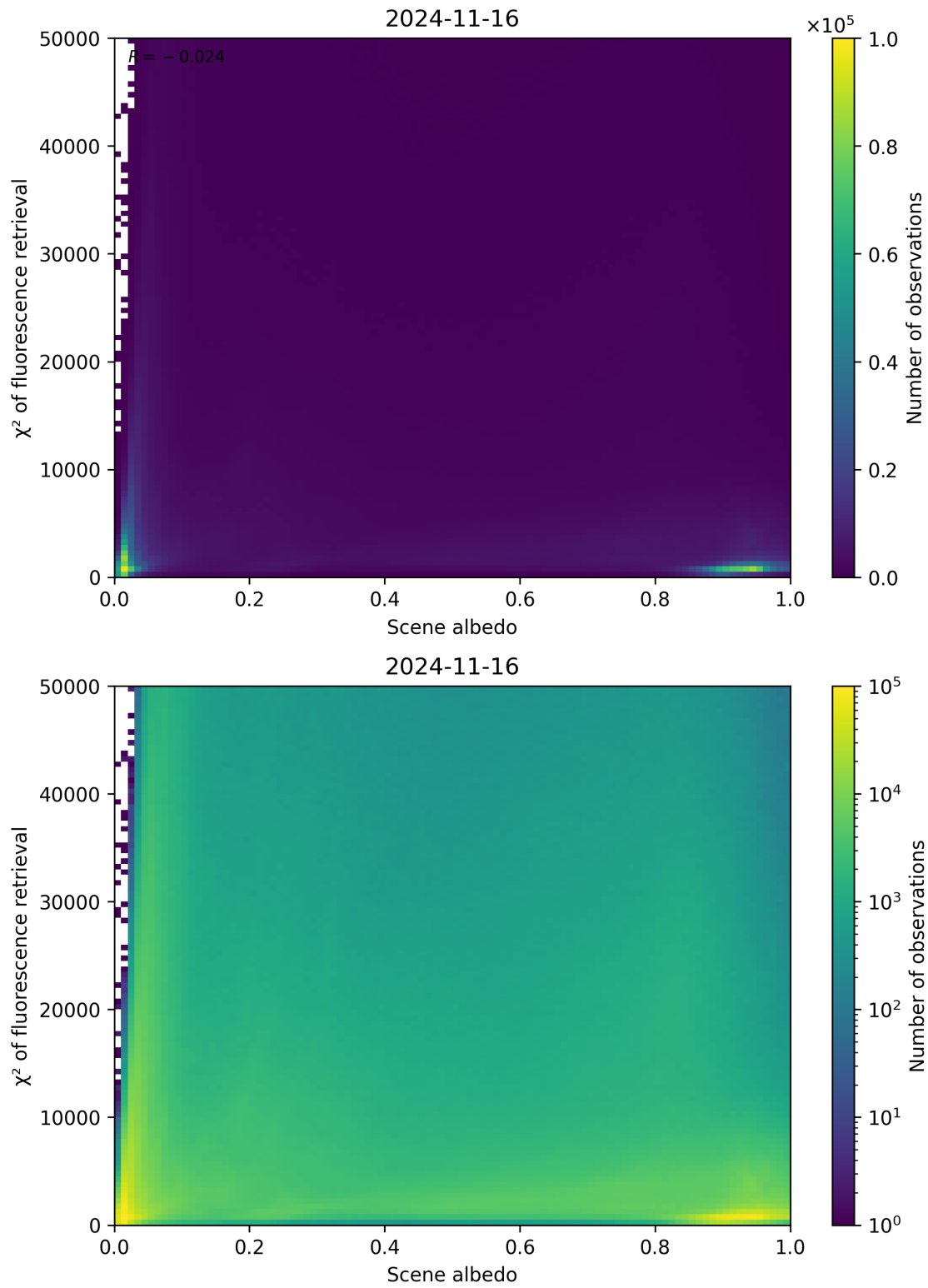
Figure 113: Scatter density plot of “Scene albedo” against “ \chi^2 of fluorescence retrieval” for 2024-11-15 to 2024-11-17.
