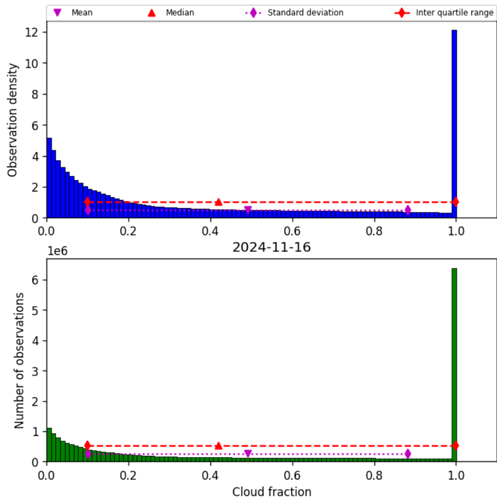
Figure 32: Histogram of “Cloud fraction” for 2024-11-15 to 2024-11-17
