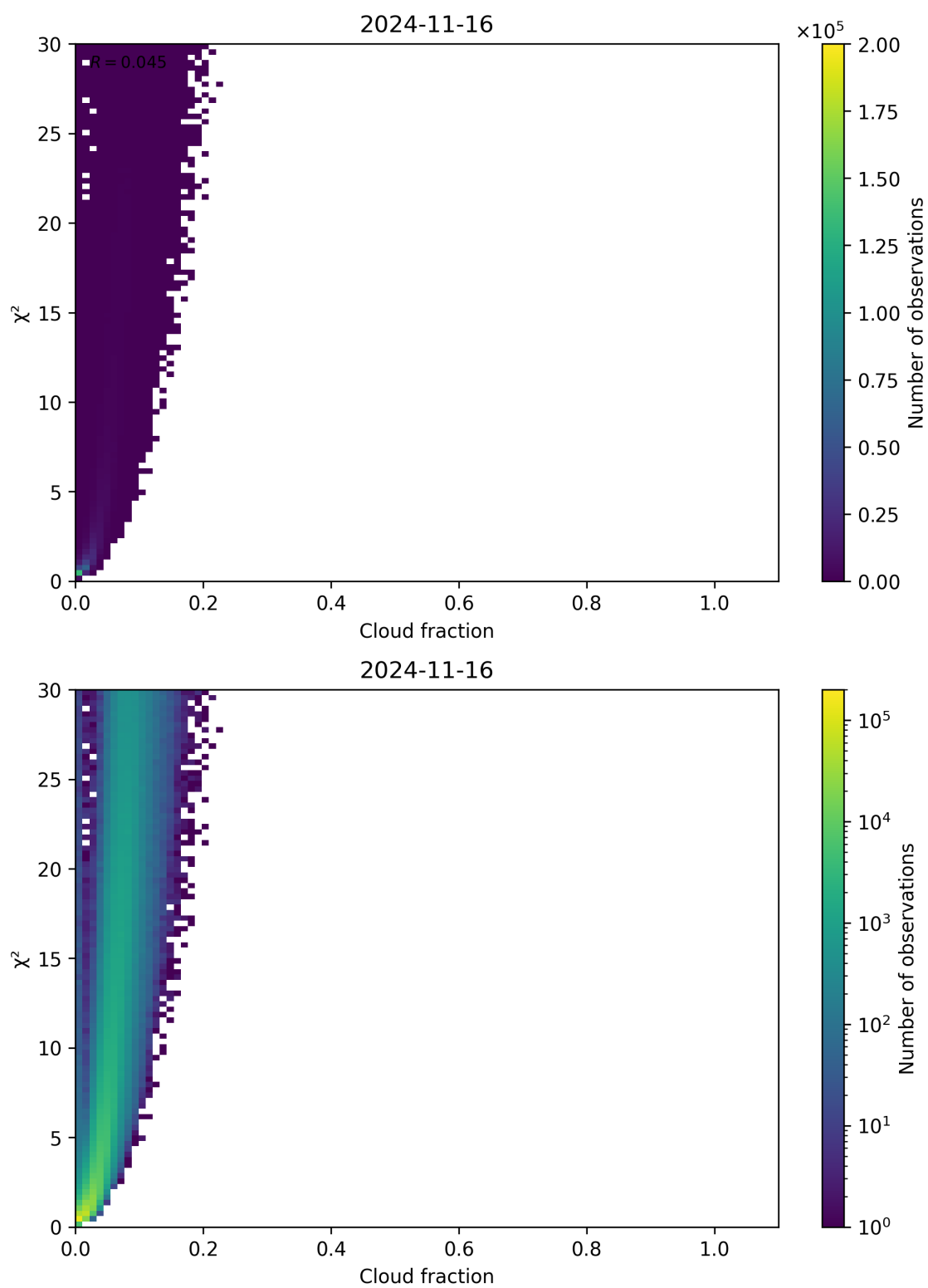
Figure 77: Scatter density plot of “Cloud fraction” against “ \chi^2 ” for 2024-11-15 to 2024-11-17.
