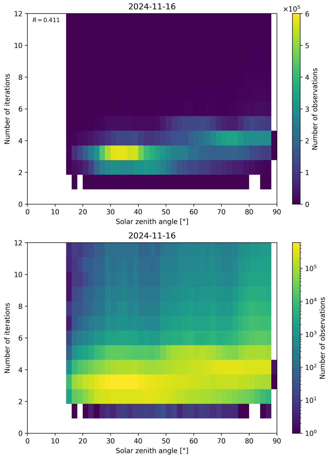
Figure 125: Scatter density plot of “Solar zenith angle” against “Number of iterations” for 2024-11-15 to 2024-11-17.
