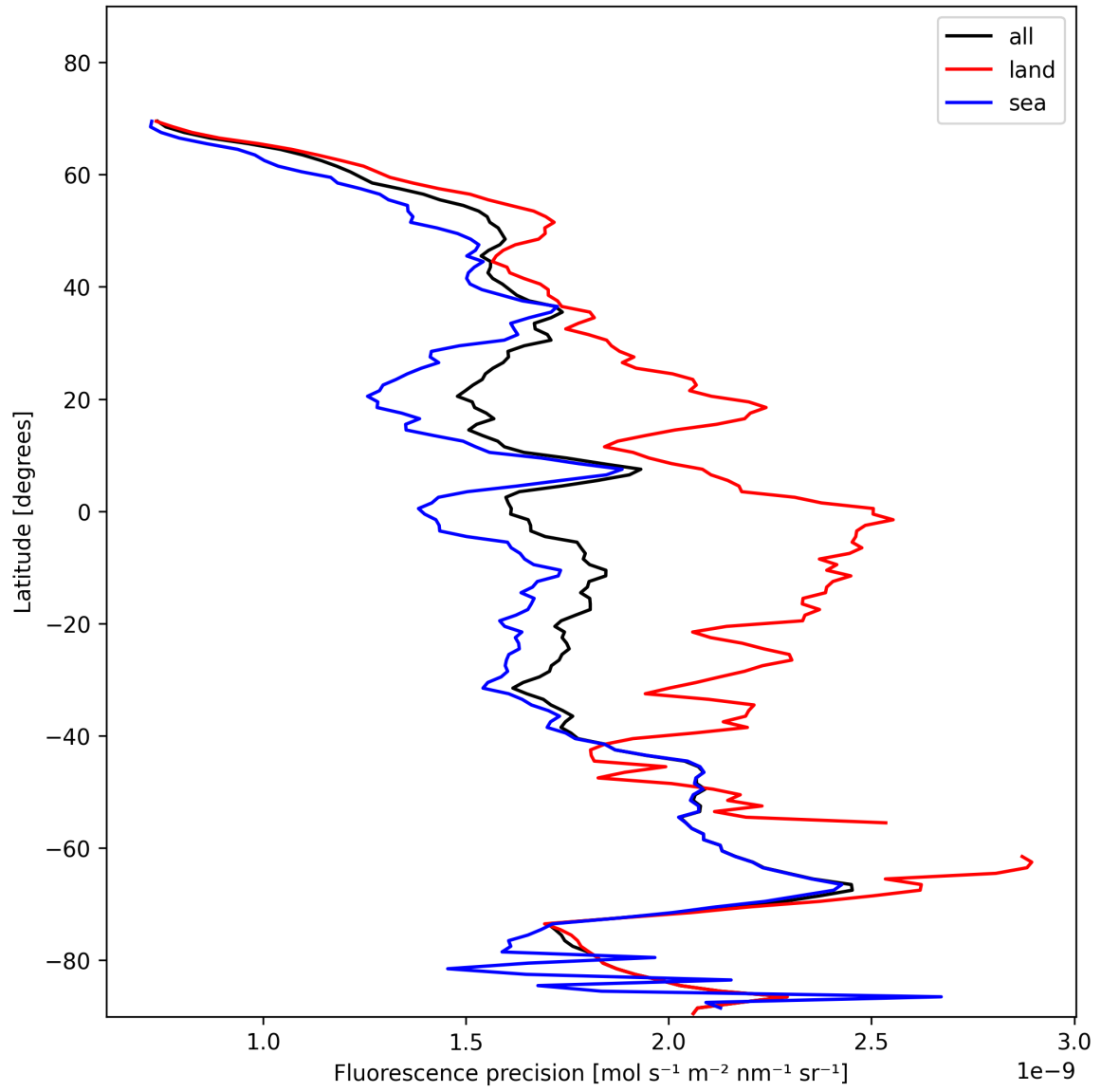
Figure 24: Zonal average of “Fluorescence precision” for 2024-11-15 to 2024-11-17.
