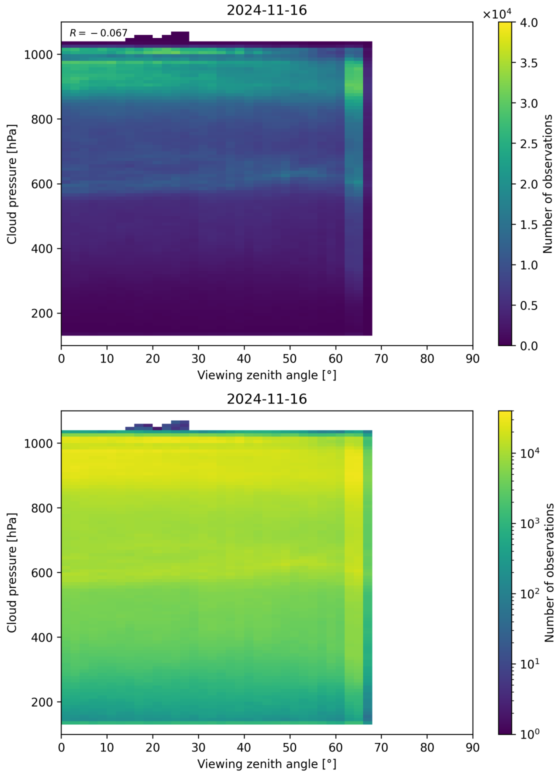
Figure 133: Scatter density plot of “Viewing zenith angle” against “Cloud pressure” for 2024-11-15 to 2024-11-17.
