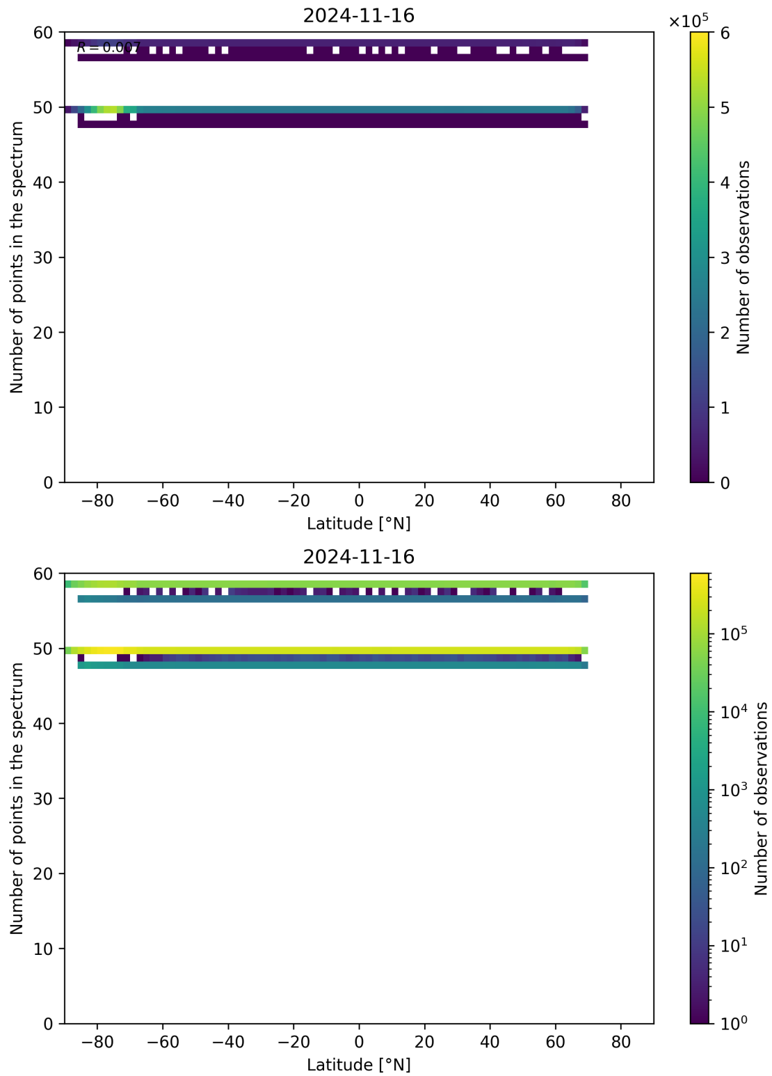
Figure 103: Scatter density plot of “Latitude” against “Number of points in the spectrum” for 2024-11-15 to 2024-11-17.
