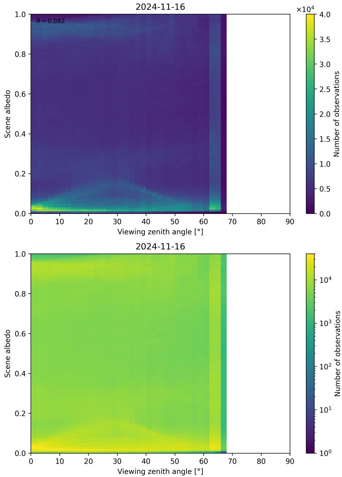
Figure 138: Scatter density plot of “Viewing zenith angle” against “Scene albedo” for 2024-11-15 to 2024-11-17.
