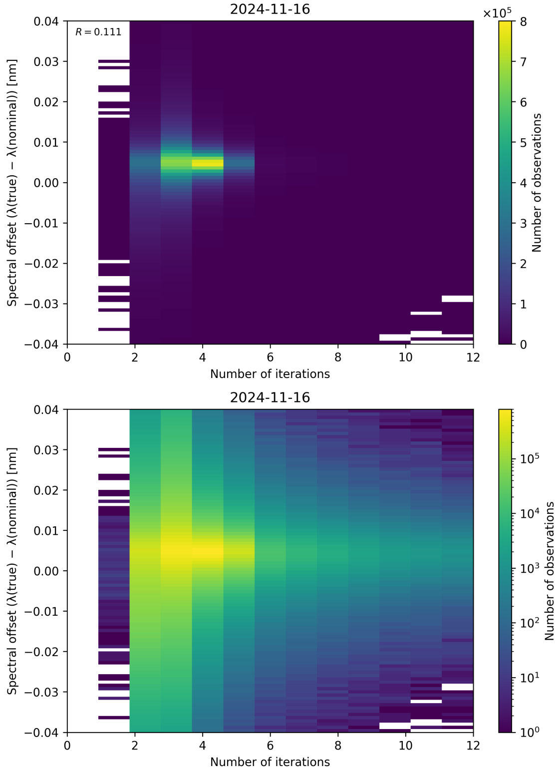
Figure 109: Scatter density plot of “Number of iterations” against “Spectral offset ( \lambda_{\text{true}} - \lambda_{\text{nominal}} )” for 2024-11-15 to 2024-11-17.
