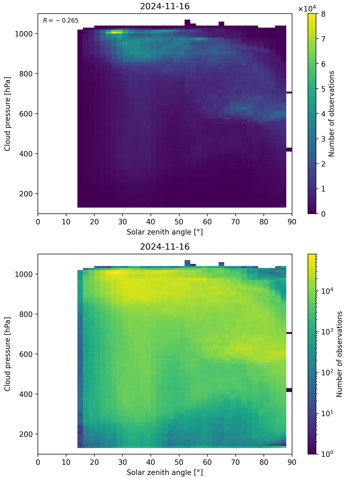
Figure 122: Scatter density plot of “Solar zenith angle” against “Cloud pressure” for 2024-11-15 to 2024-11-17.
