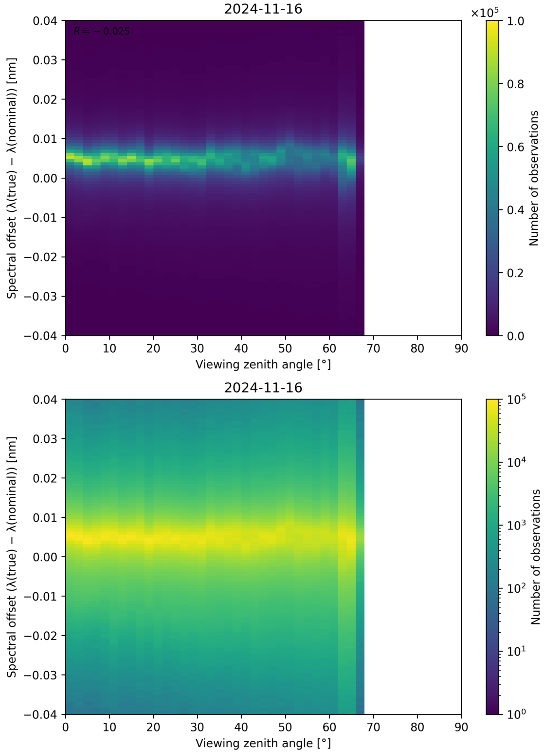
Figure 140: Scatter density plot of “Viewing zenith angle” against “Spectral offset ( \lambda_{\text{true}} - \lambda_{\text{nominal}} )” for 2024-11-15 to 2024-11-17.
