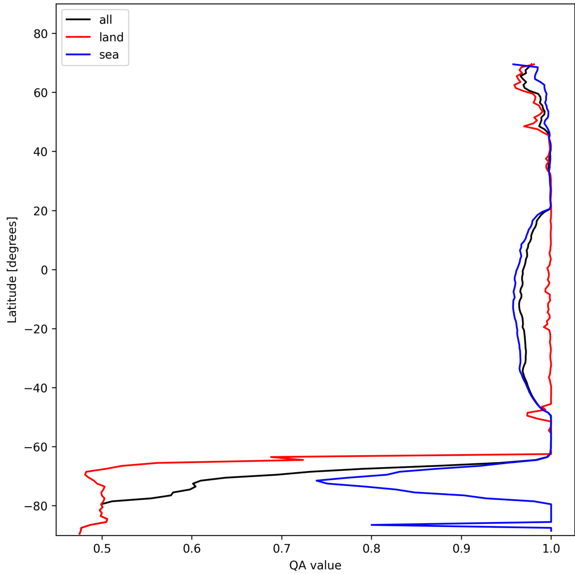
Figure 12: Zonal average of “QA value” for 2024-11-15 to 2024-11-17.
