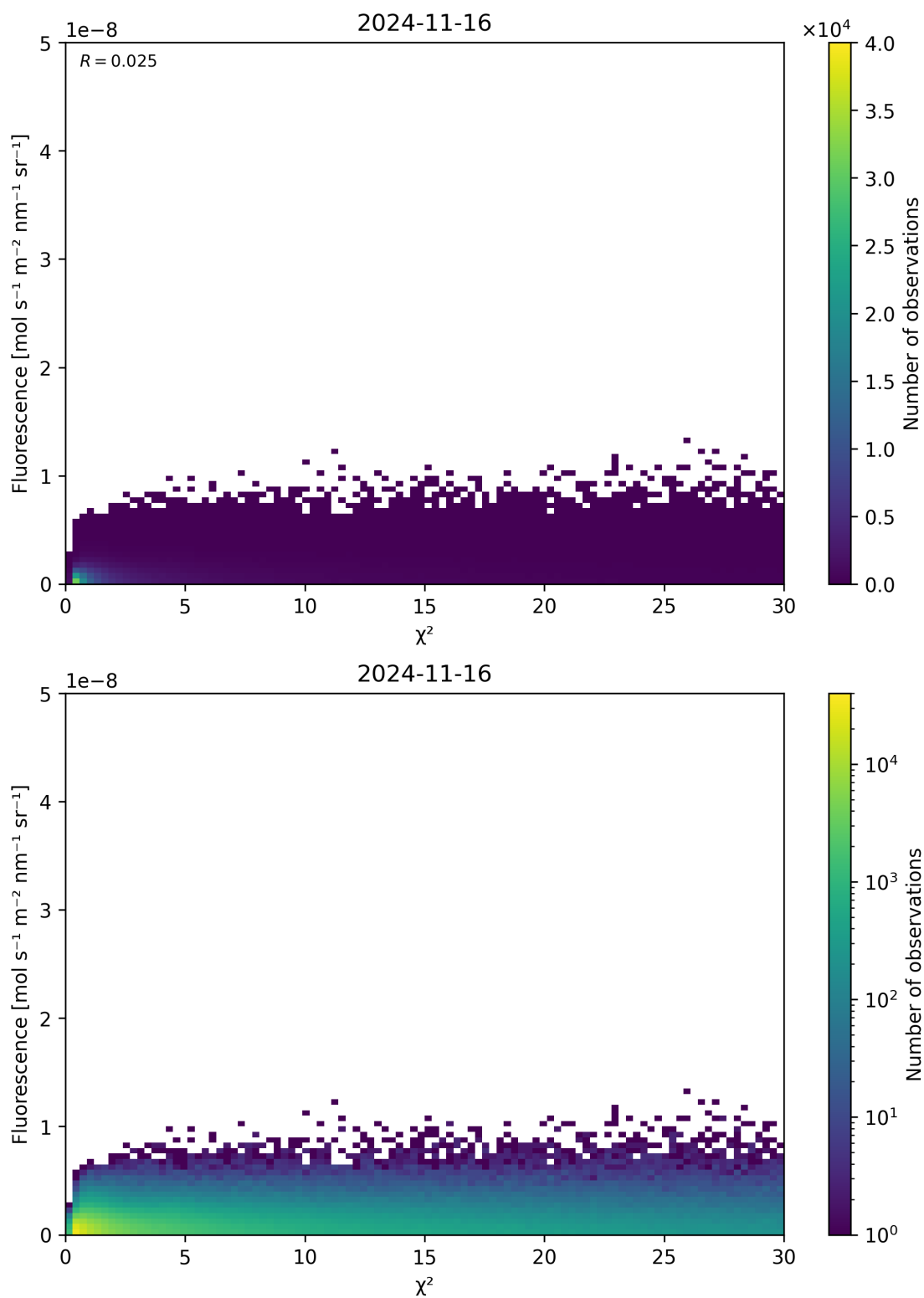
Figure 70: Scatter density plot of “ \chi^2 ” against “Fluorescence” for 2024-11-15 to 2024-11-17.
