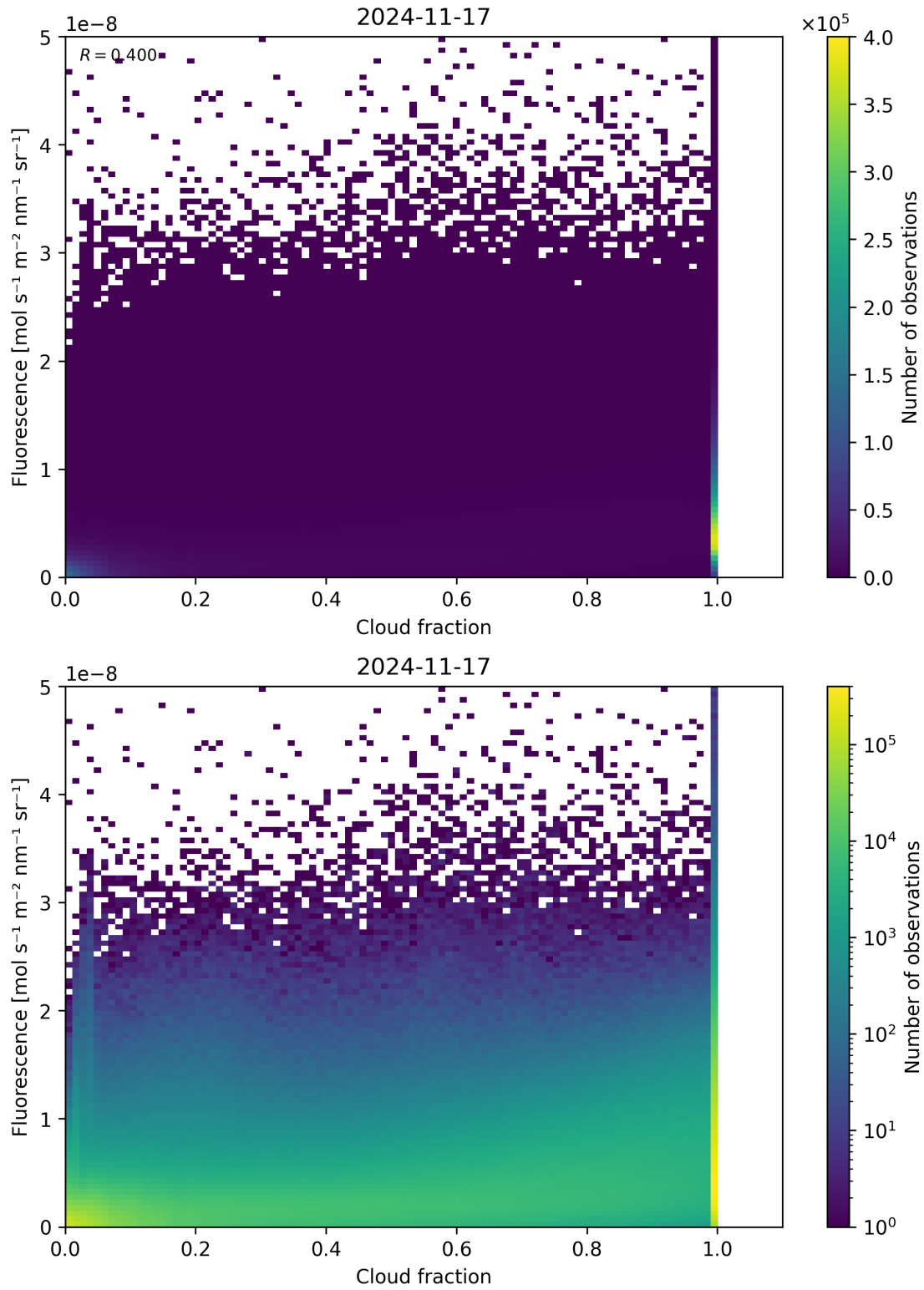
Figure 72: Scatter density plot of “Cloud fraction” against “Fluorescence” for 2024-11-17 to 2024-11-18.
