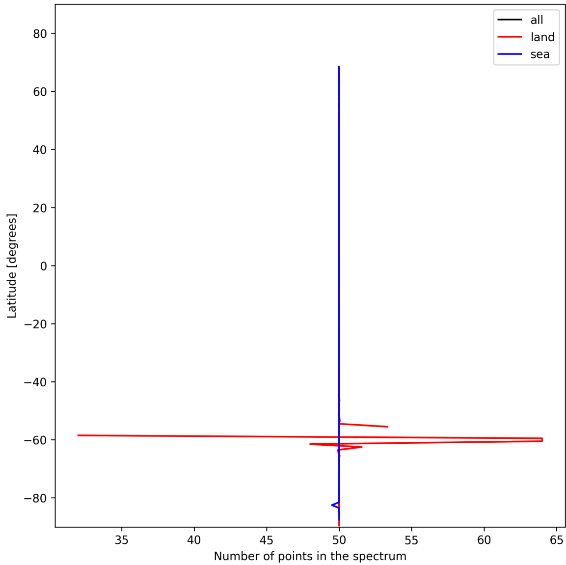
Figure 27: Zonal average of “Number of points in the spectrum” for 2024-11-17 to 2024-11-18.
