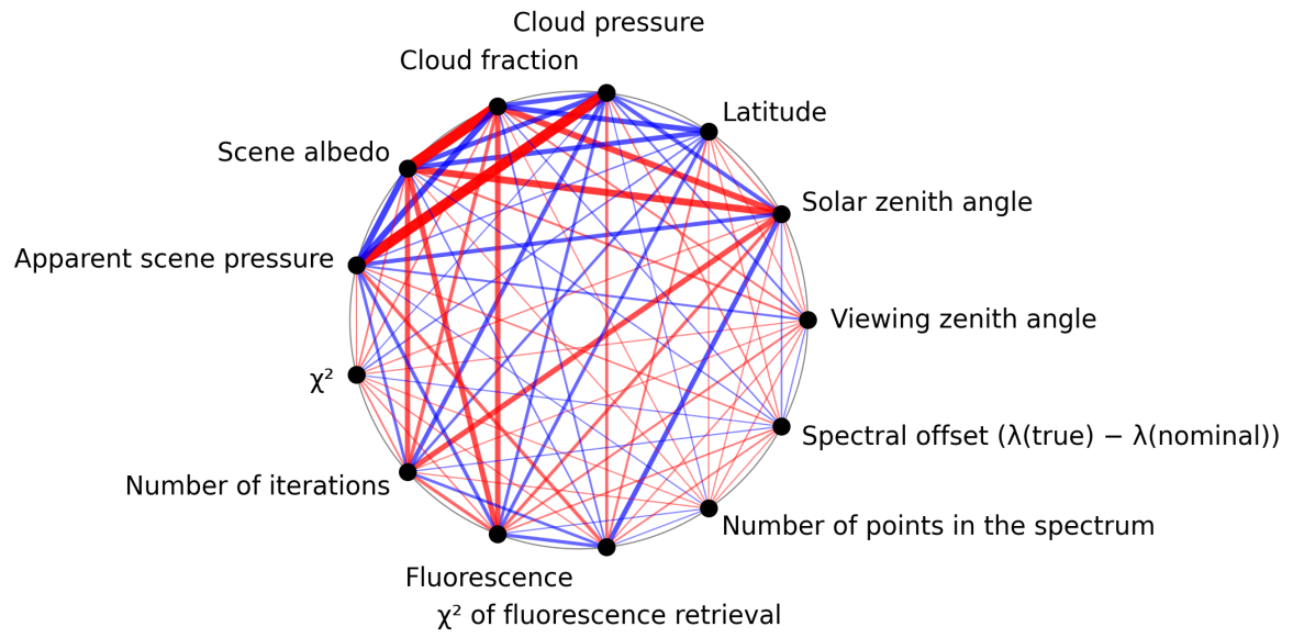
Figure 1: Map of correlation graph for 2024-11-17 to 2024-11-18.
