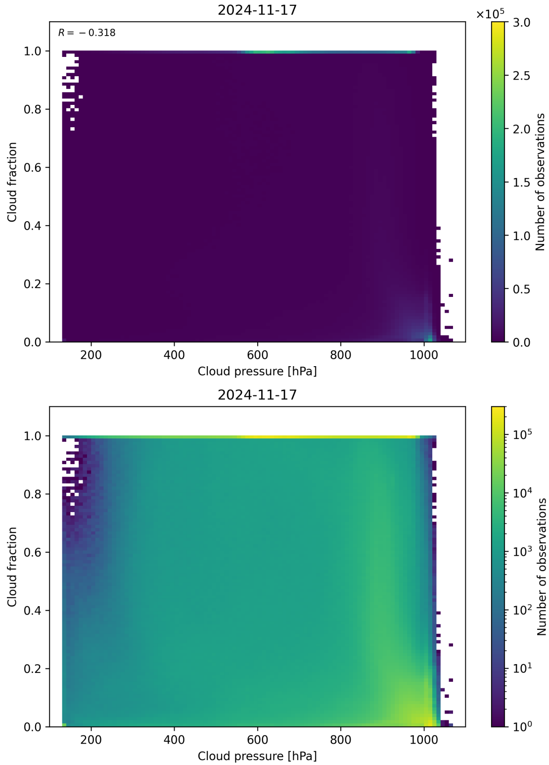
Figure 79: Scatter density plot of “Cloud pressure” against “Cloud fraction” for 2024-11-17 to 2024-11-18.
