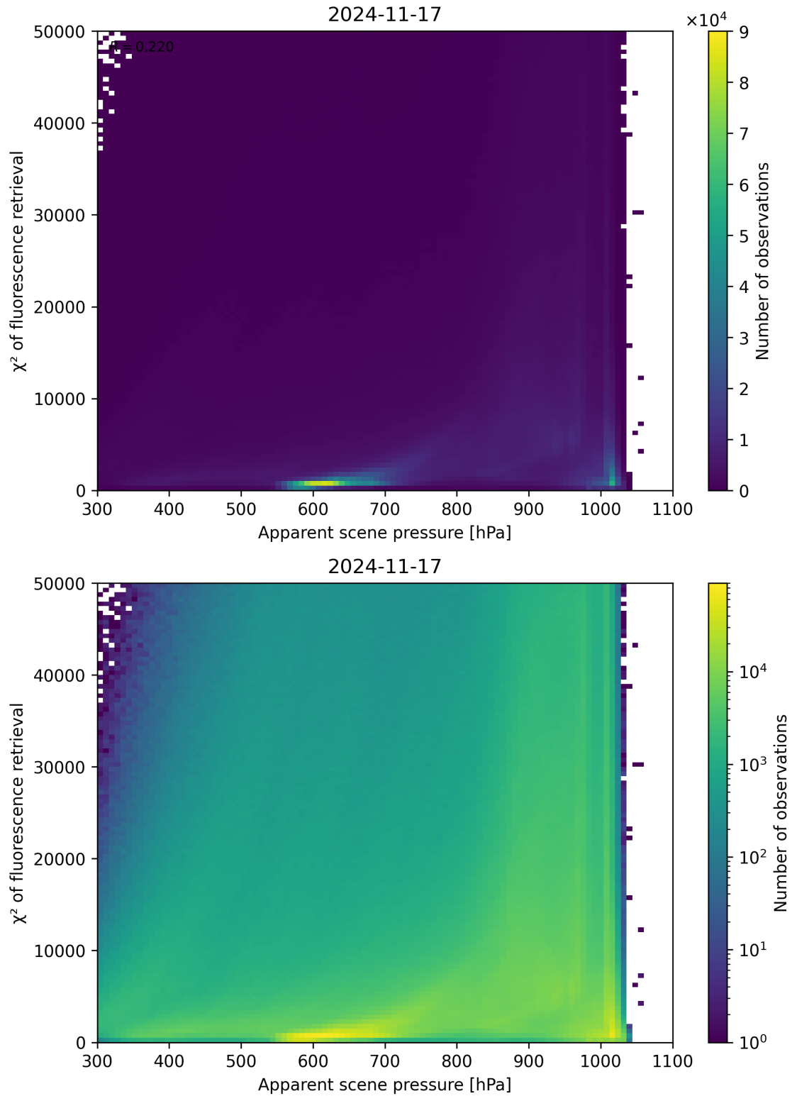
Figure 63: Scatter density plot of “Apparent scene pressure” against “ \chi^2 of fluorescence retrieval” for 2024-11-17 to 2024-11-18.
