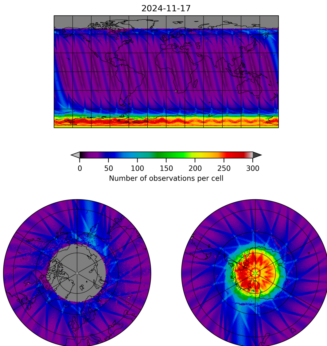
Figure 11: Map of the number of observations for 2024-11-17 to 2024-11-18
