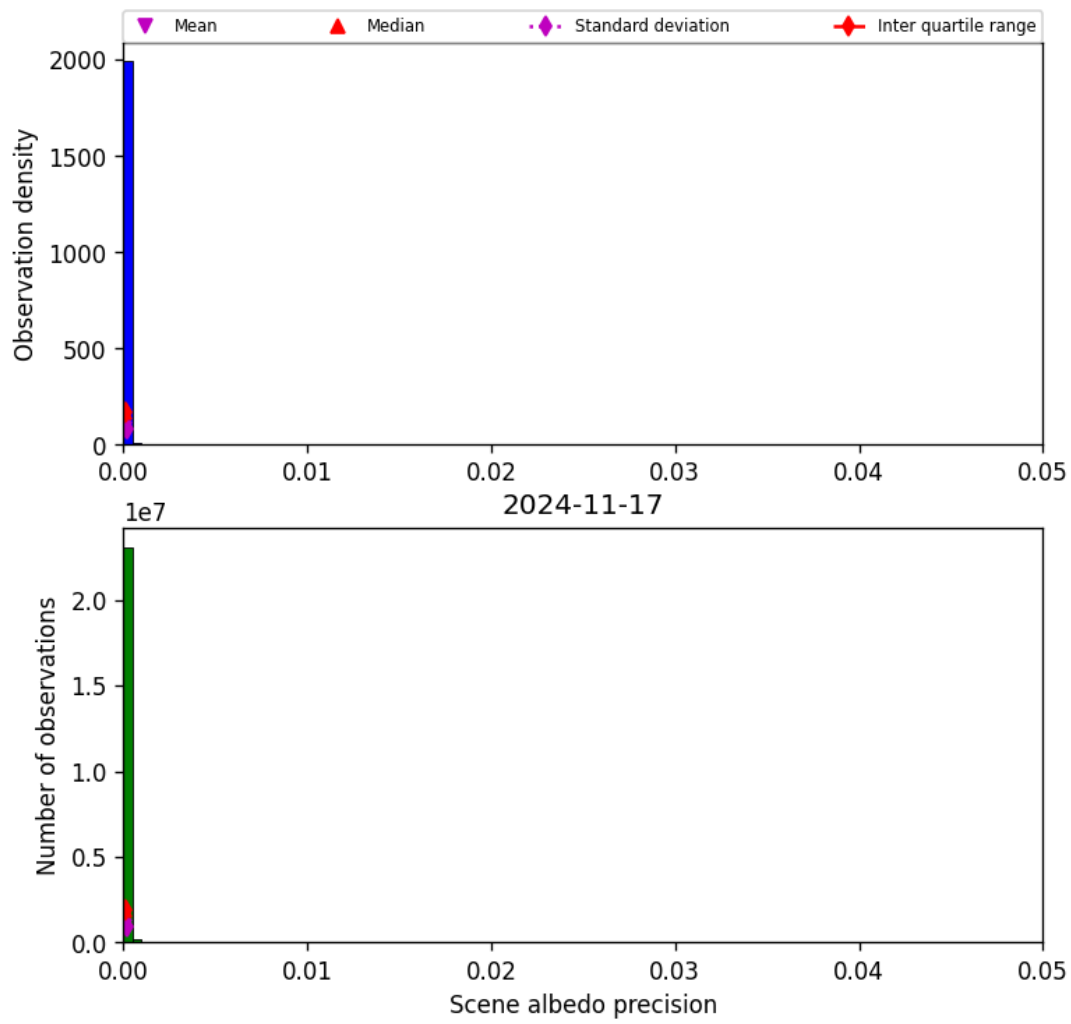
Figure 35: Histogram of “Scene albedo precision” for 2024-11-17 to 2024-11-18
