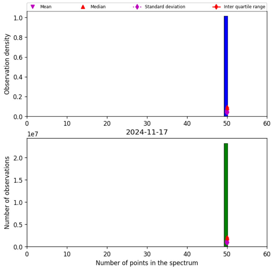
Figure 44: Histogram of “Number of points in the spectrum” for 2024-11-17 to 2024-11-18
