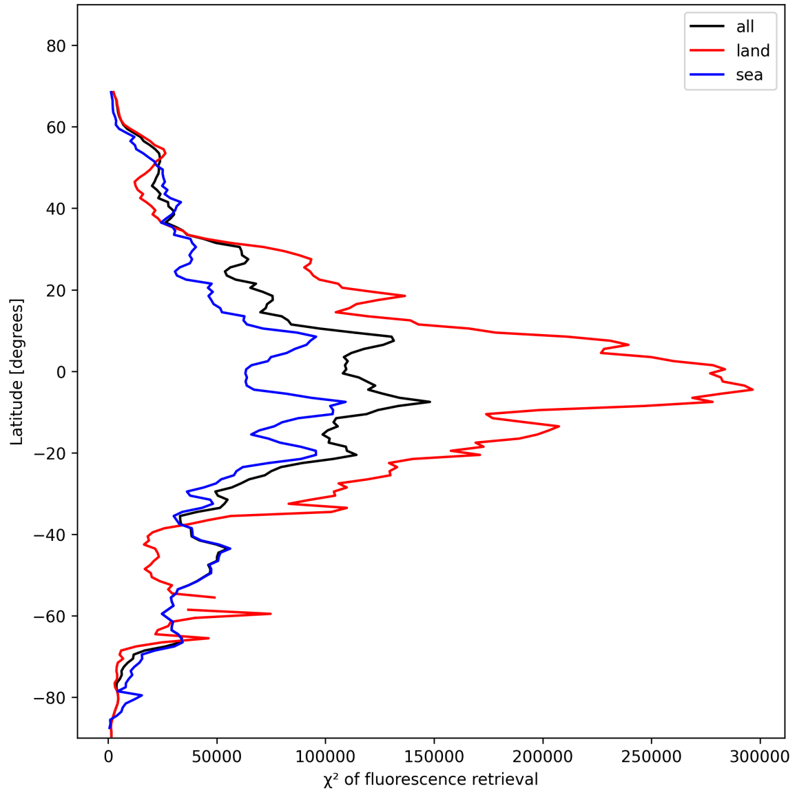
Figure 25: Zonal average of “ \chi^2 of fluorescence retrieval” for 2024-11-17 to 2024-11-18.
