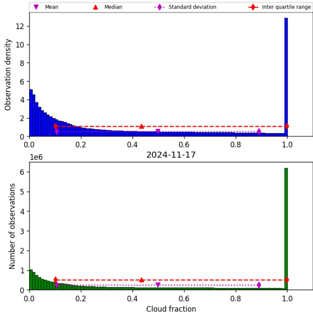
Figure 32: Histogram of “Cloud fraction” for 2024-11-17 to 2024-11-18
