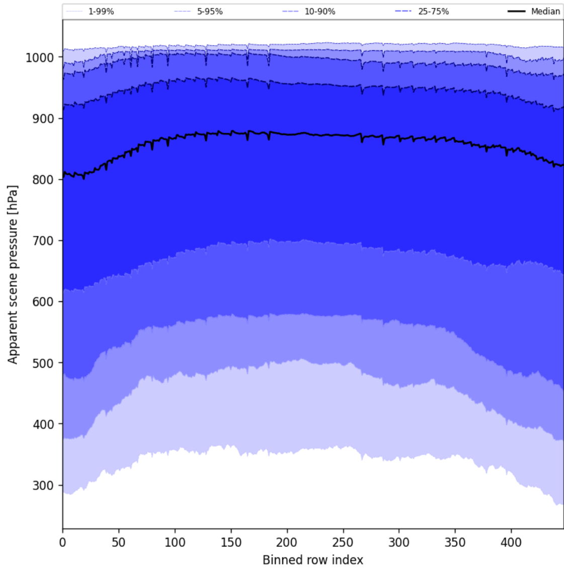
Figure 53: Along track statistics of “Apparent scene pressure” for 2024-11-17 to 2024-11-18
