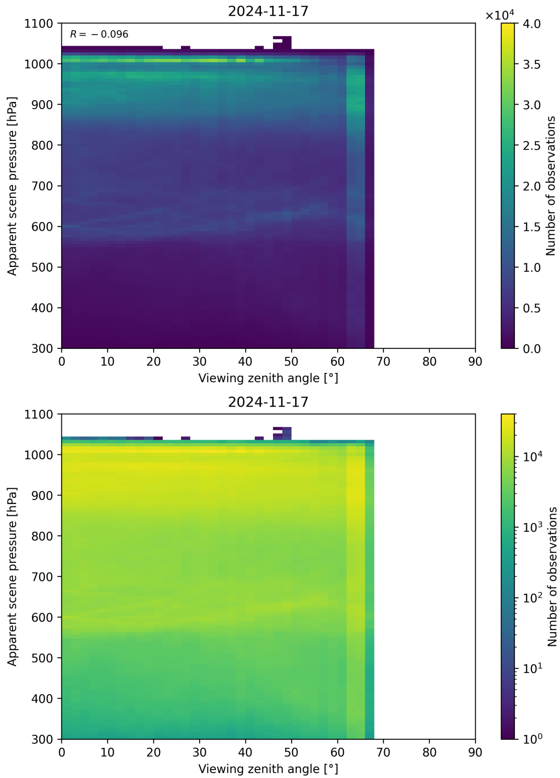
Figure 118: Scatter density plot of “Viewing zenith angle” against “Apparent scene pressure” for 2024-11-17 to 2024-11-18.
