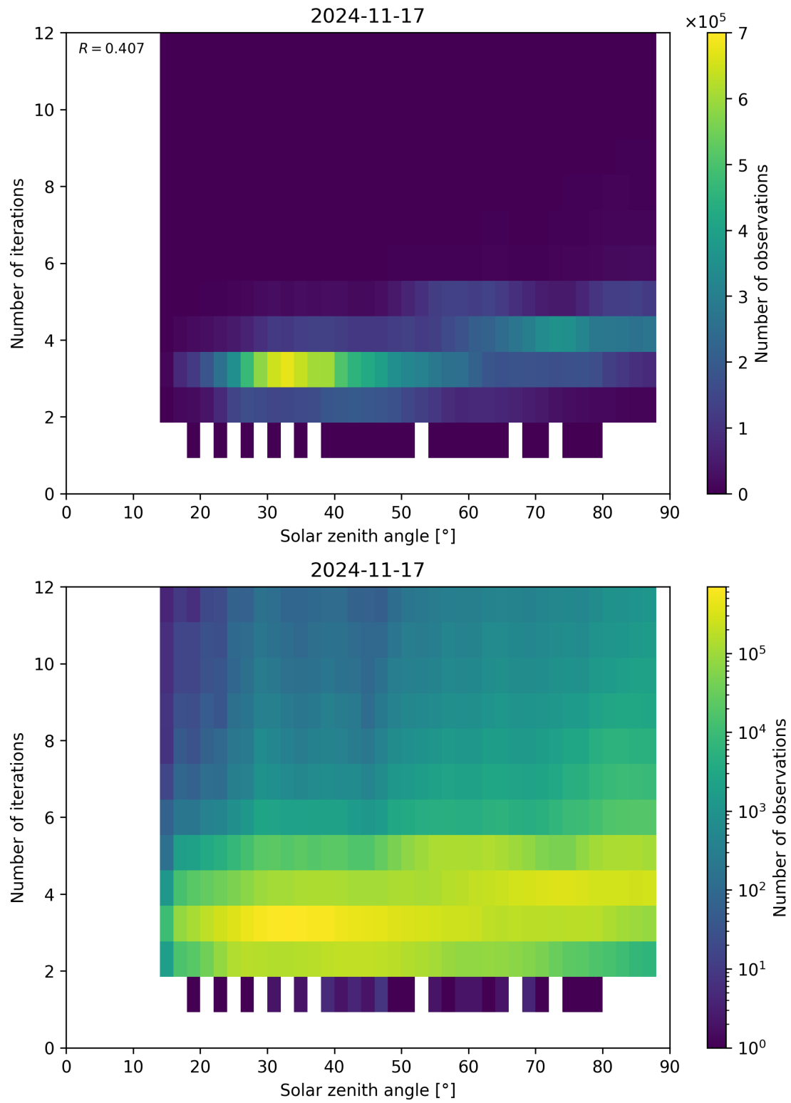
Figure 114: Scatter density plot of “Solar zenith angle” against “Number of iterations” for 2024-11-17 to 2024-11-18.
