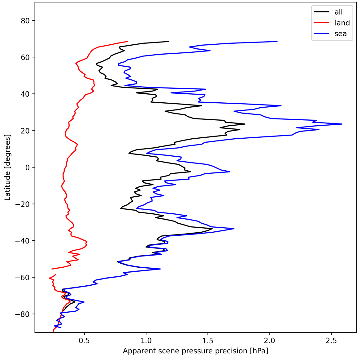
Figure 20: Zonal average of “Apparent scene pressure precision” for 2024-11-17 to 2024-11-18.
