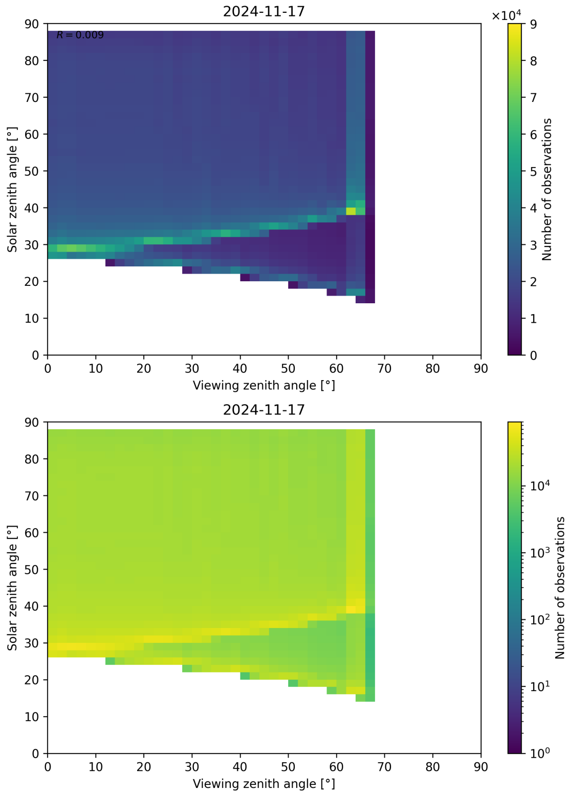
Figure 127: Scatter density plot of “Viewing zenith angle” against “Solar zenith angle” for 2024-11-17 to 2024-11-18.
