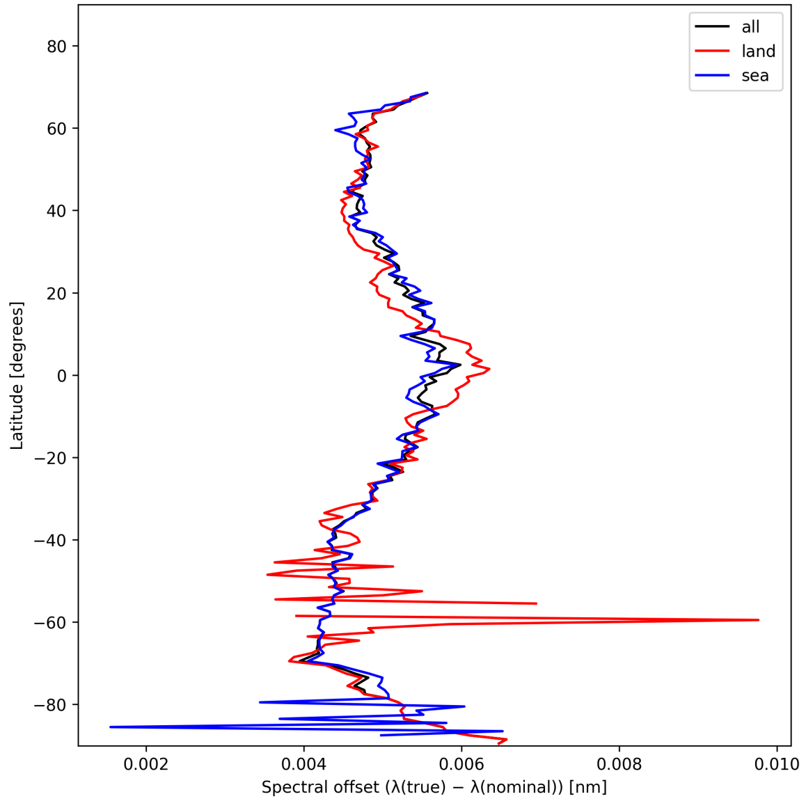
Figure 28: Zonal average of “Spectral offset ( \lambda_{\text{true}} - \lambda_{\text{nominal}} )” for 2024-11-17 to 2024-11-18.
