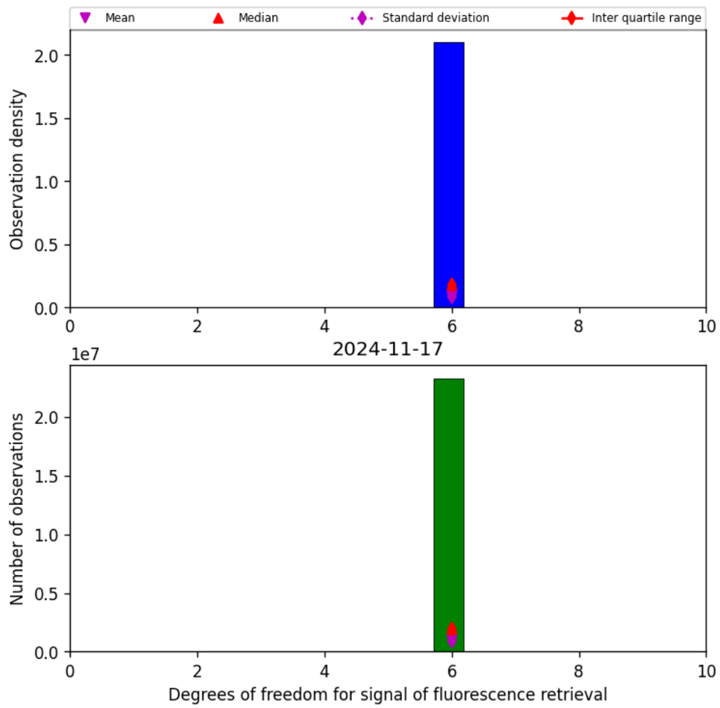
Figure 43: Histogram of “Degrees of freedom for signal of fluorescence retrieval” for 2024-11-17 to 2024-11-18
