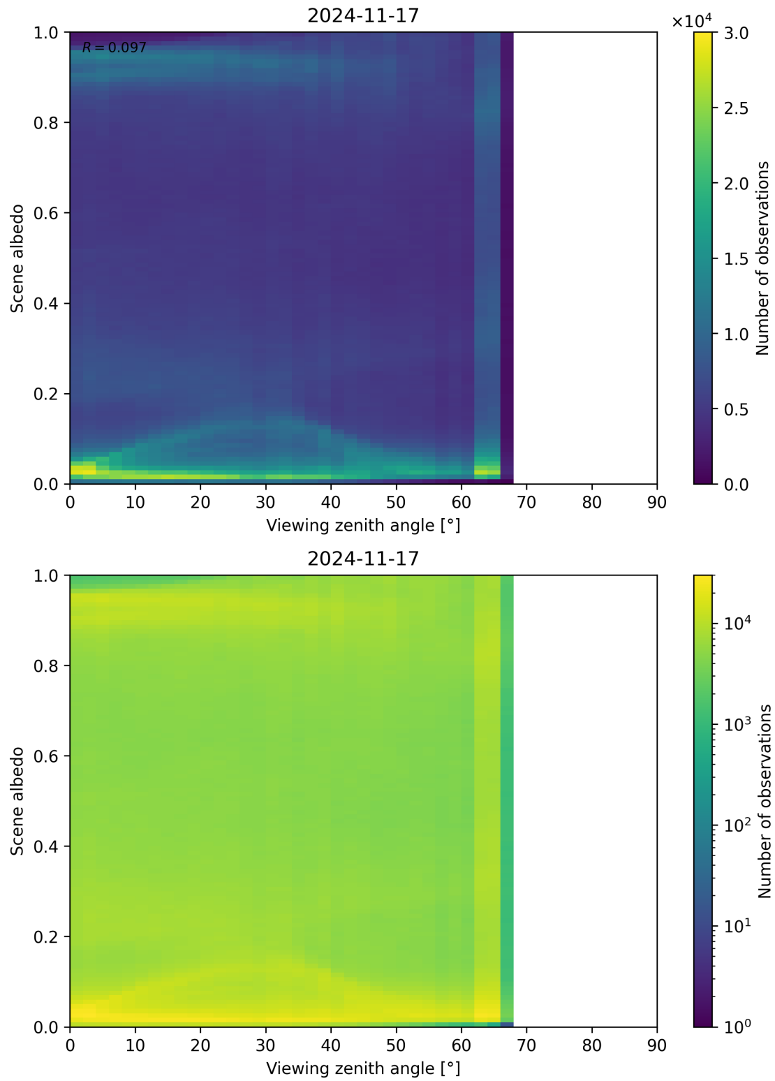
Figure 126: Scatter density plot of “Viewing zenith angle” against “Scene albedo” for 2024-11-17 to 2024-11-18.
