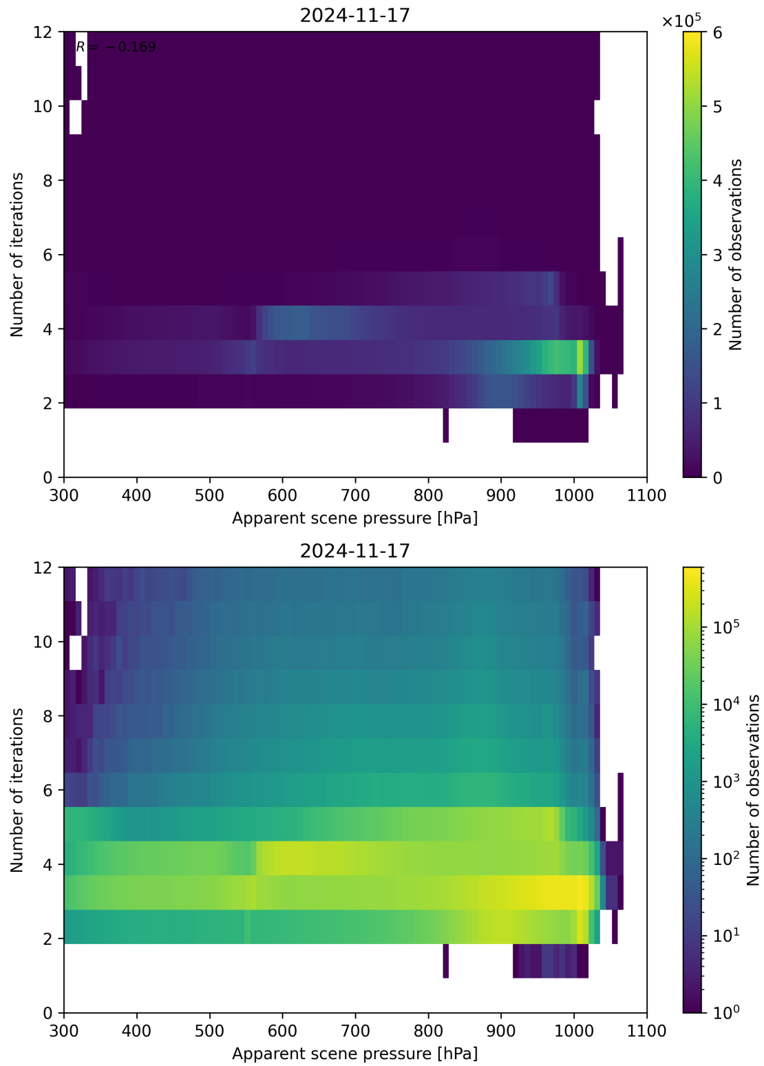
Figure 65: Scatter density plot of “Apparent scene pressure” against “Number of iterations” for 2024-11-17 to 2024-11-18.
