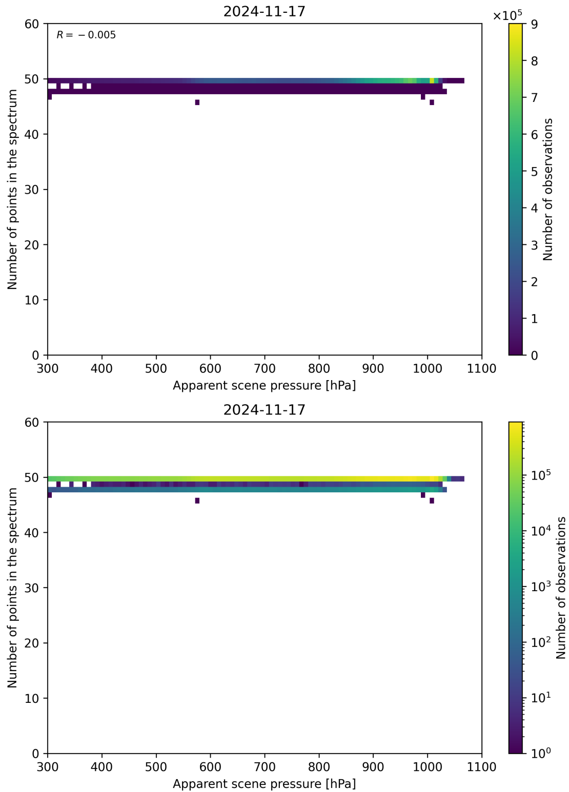
Figure 66: Scatter density plot of “Apparent scene pressure” against “Number of points in the spectrum” for 2024-11-17 to 2024-11-18.
