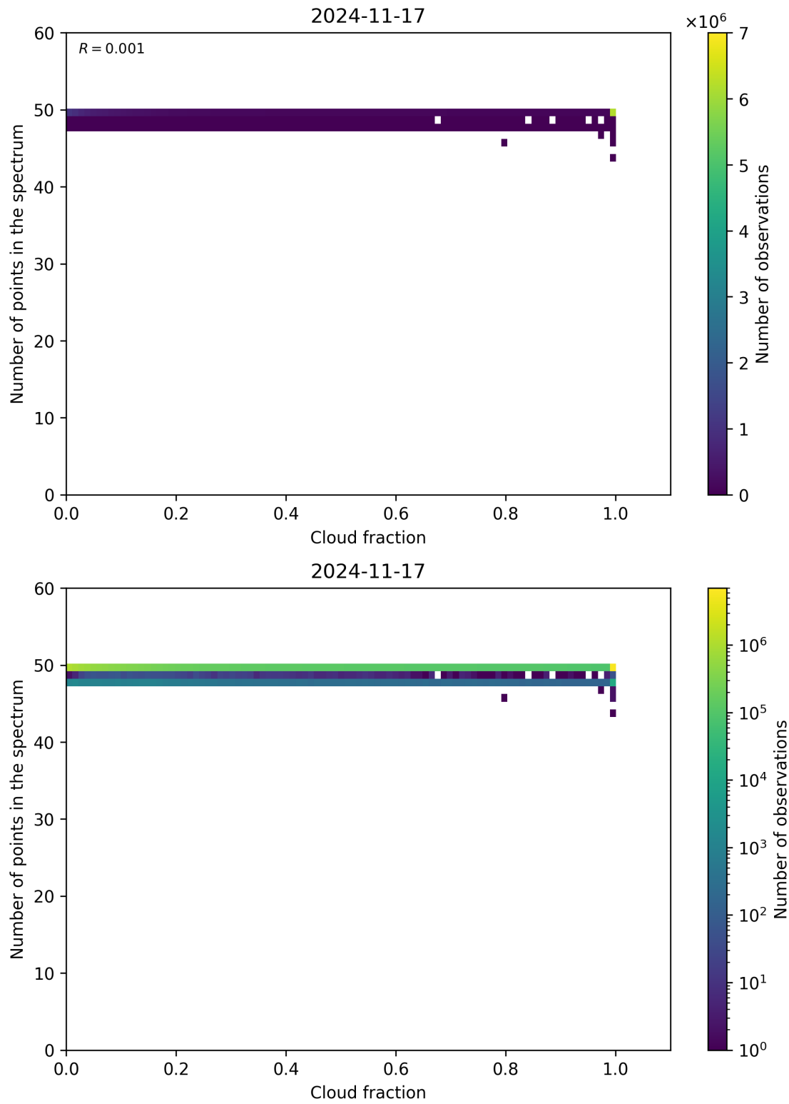
Figure 74: Scatter density plot of “Cloud fraction” against “Number of points in the spectrum” for 2024-11-17 to 2024-11-18.
