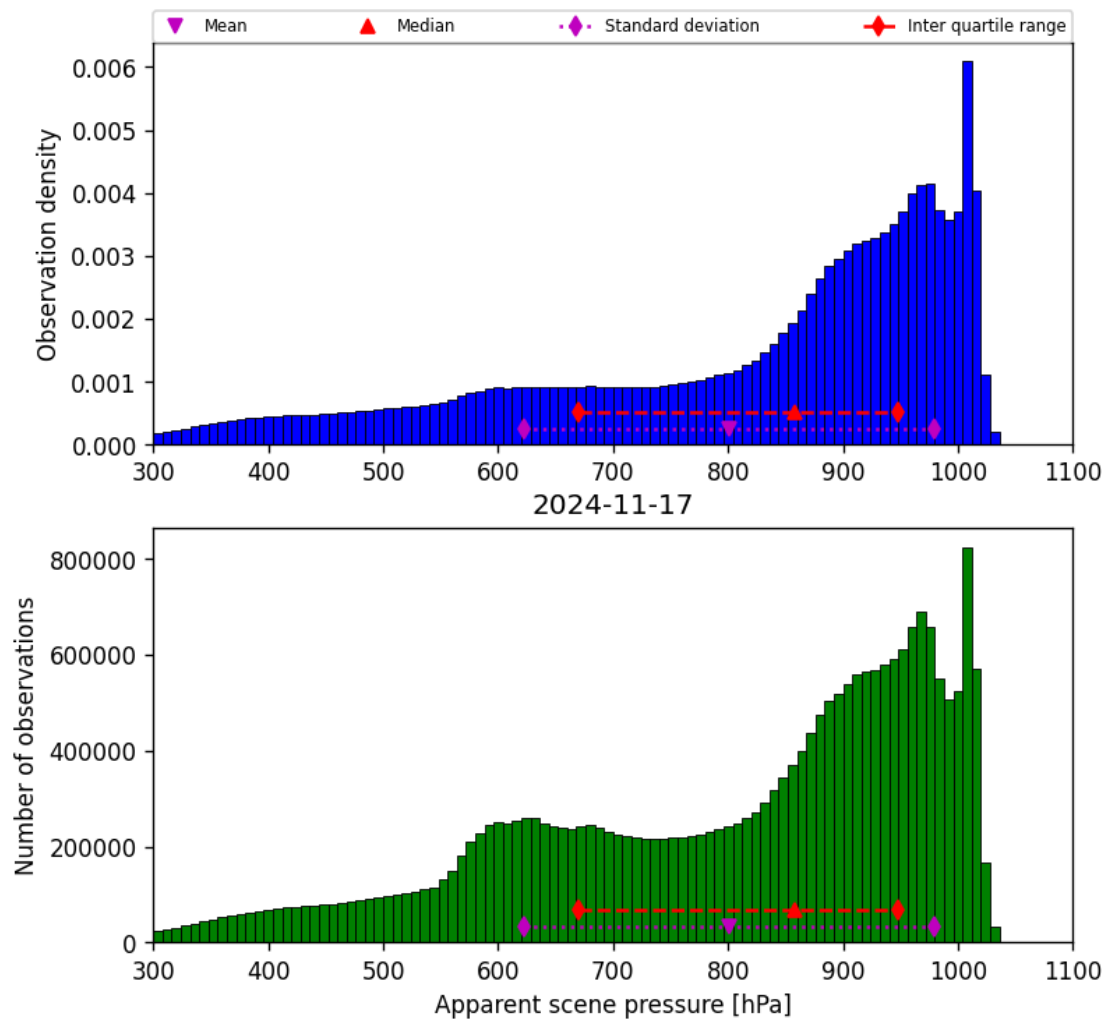
Figure 36: Histogram of “Apparent scene pressure” for 2024-11-17 to 2024-11-18
