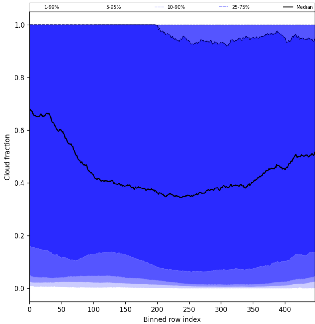
Figure 49: Along track statistics of “Cloud fraction” for 2024-11-17 to 2024-11-18
