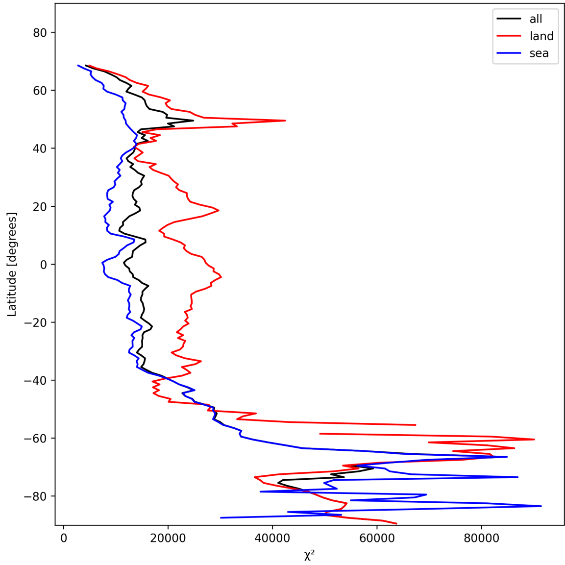
Figure 21: Zonal average of “ \chi^2 ” for 2024-11-17 to 2024-11-18.
