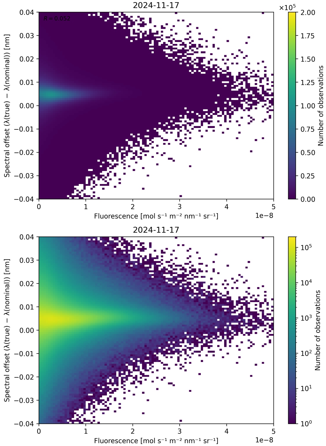
Figure 87: Scatter density plot of “Fluorescence” against “Spectral offset ( \lambda_{\text{true}} - \lambda_{\text{nominal}} )” for 2024-11-17 to 2024-11-18.
