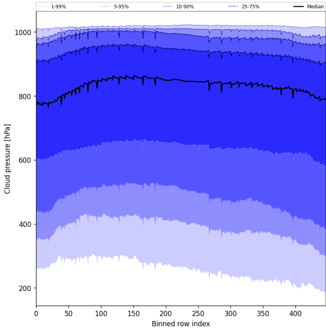
Figure 47: Along track statistics of “Cloud pressure” for 2024-11-17 to 2024-11-18
