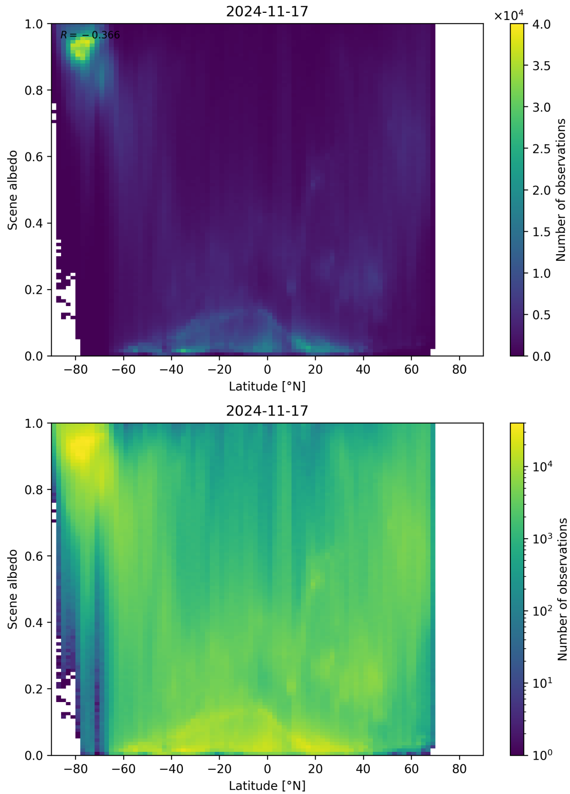
Figure 95: Scatter density plot of “Latitude” against “Scene albedo” for 2024-11-17 to 2024-11-18.
