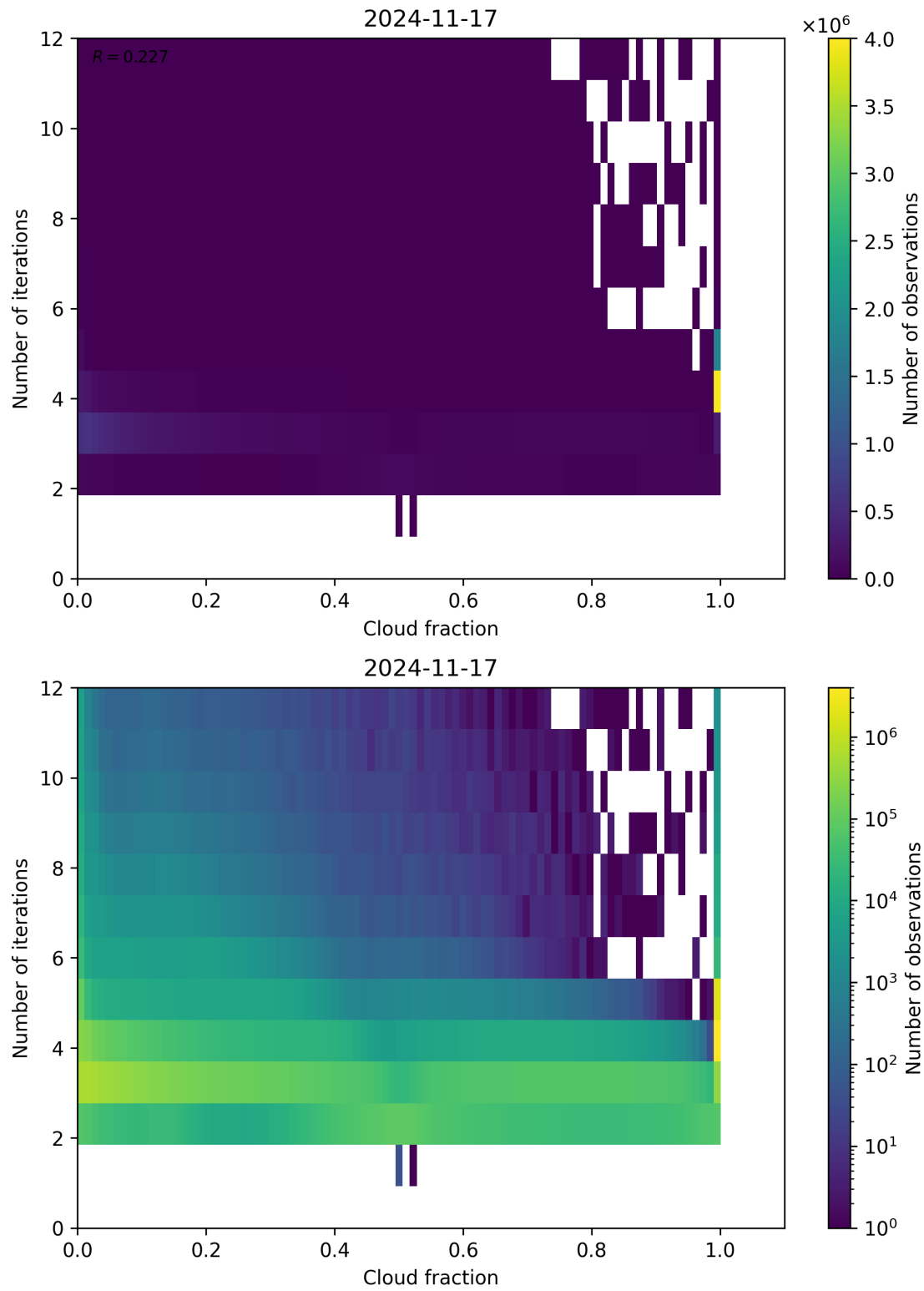
Figure 73: Scatter density plot of “Cloud fraction” against “Number of iterations” for 2024-11-17 to 2024-11-18.
