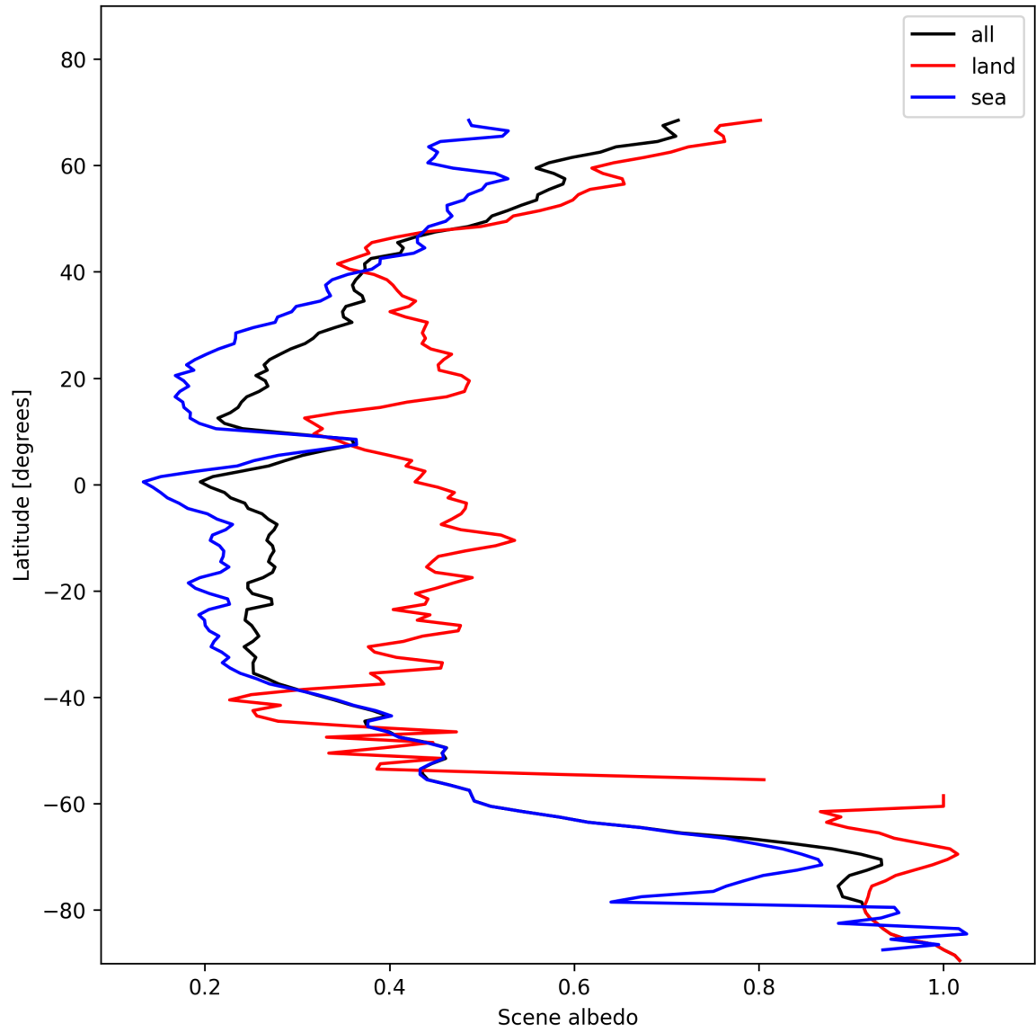
Figure 17: Zonal average of “Scene albedo” for 2024-11-17 to 2024-11-18.
