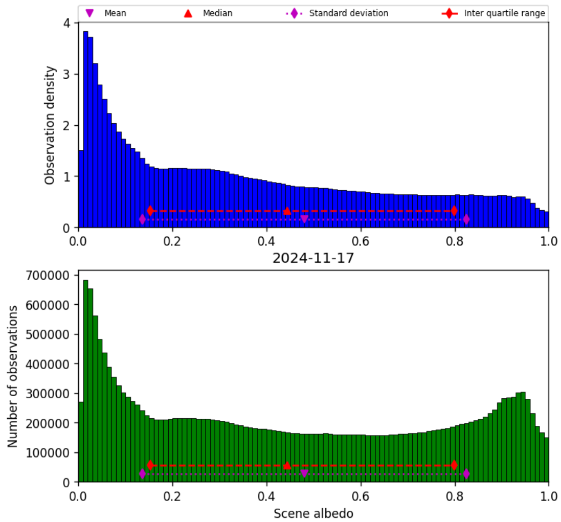
Figure 34: Histogram of “Scene albedo” for 2024-11-17 to 2024-11-18
