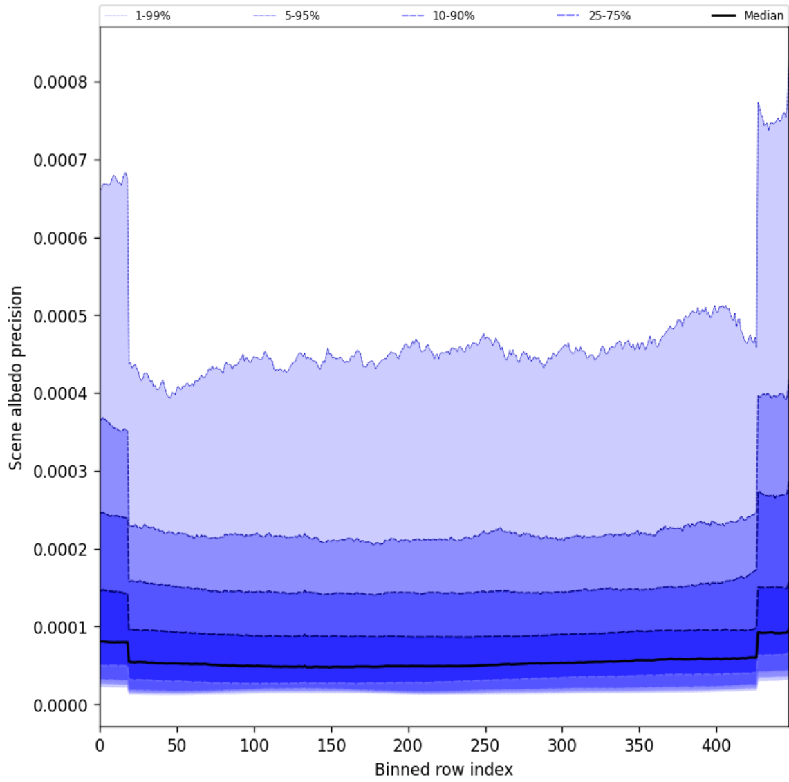
Figure 52: Along track statistics of “Scene albedo precision” for 2024-11-17 to 2024-11-18
