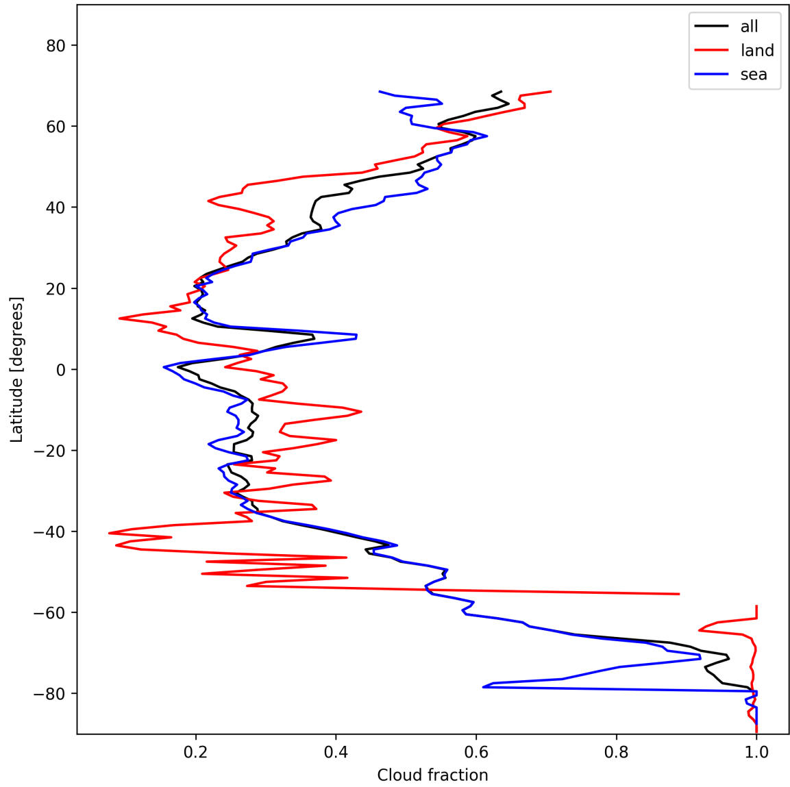
Figure 15: Zonal average of “Cloud fraction” for 2024-11-17 to 2024-11-18.
