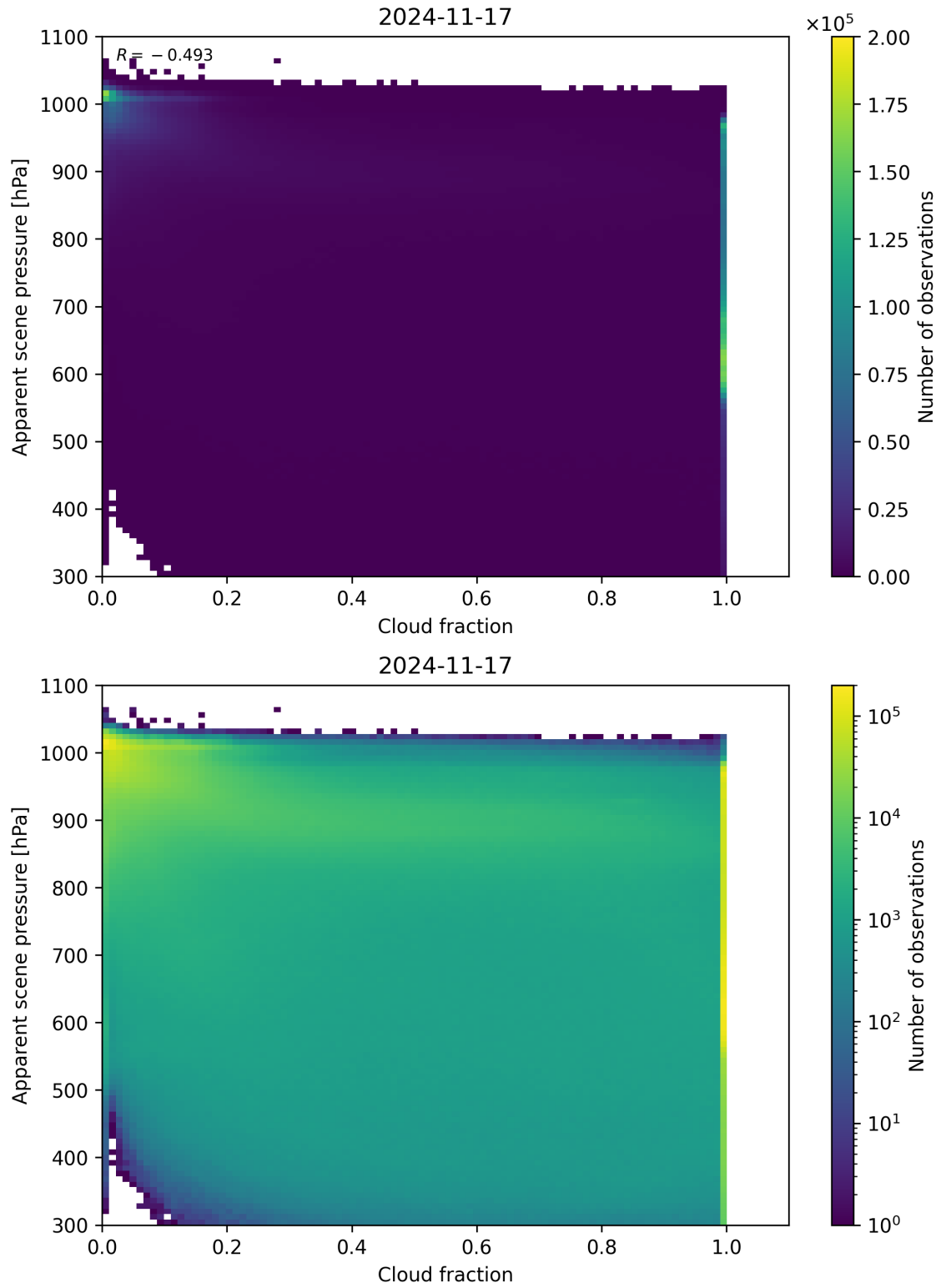
Figure 70: Scatter density plot of “Cloud fraction” against “Apparent scene pressure” for 2024-11-17 to 2024-11-18.
