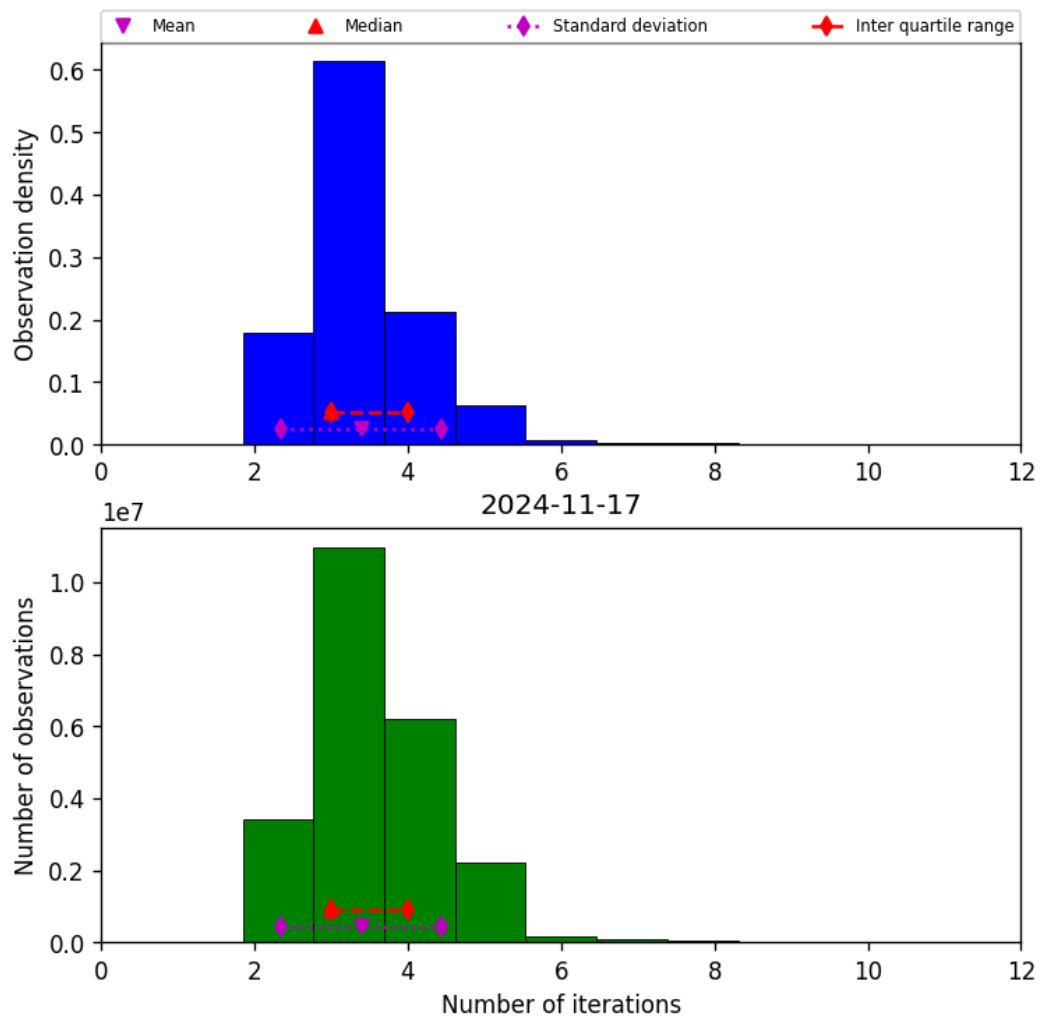
Figure 39: Histogram of “Number of iterations” for 2024-11-17 to 2024-11-18
