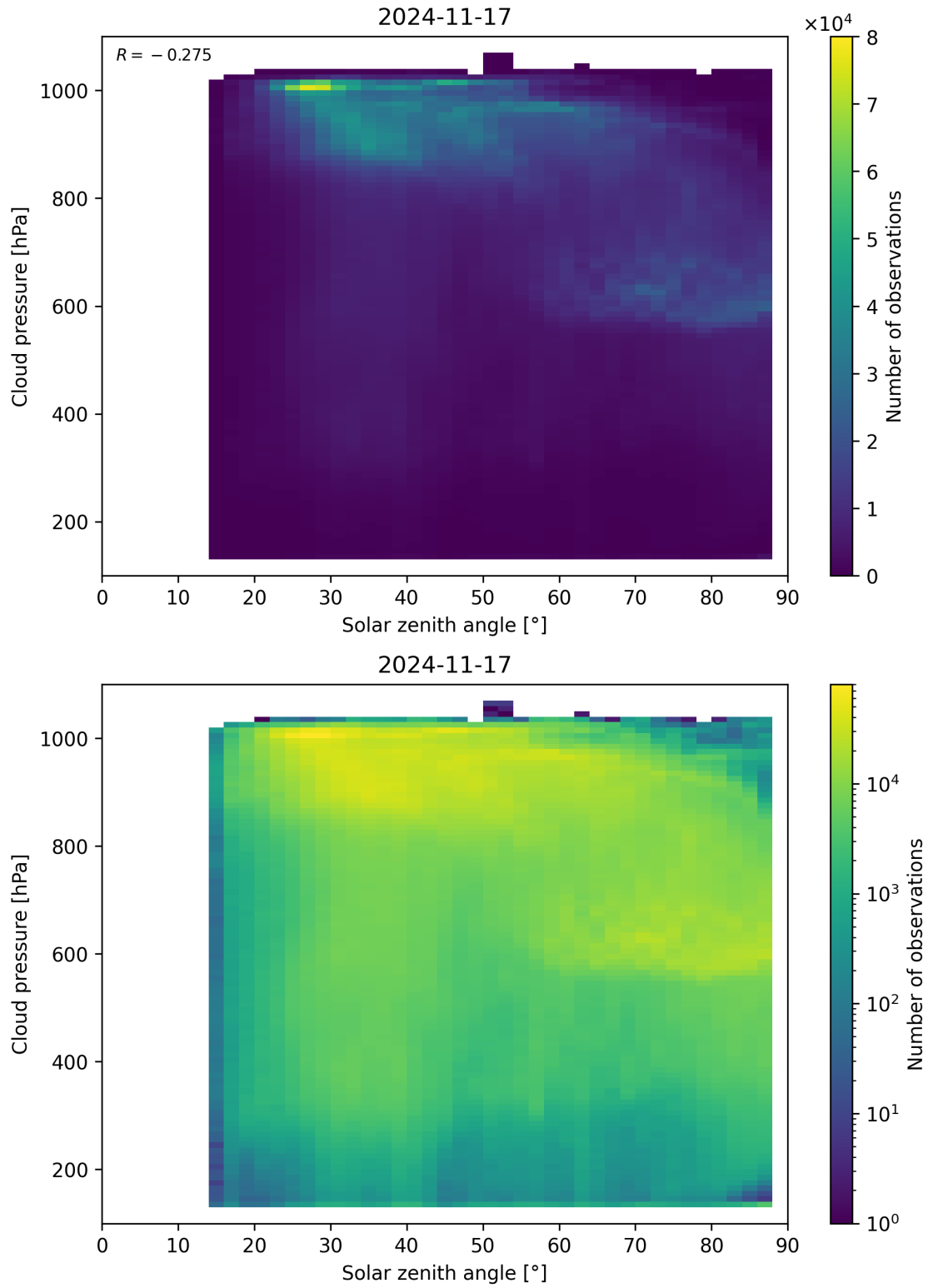
Figure 111: Scatter density plot of “Solar zenith angle” against “Cloud pressure” for 2024-11-17 to 2024-11-18.
