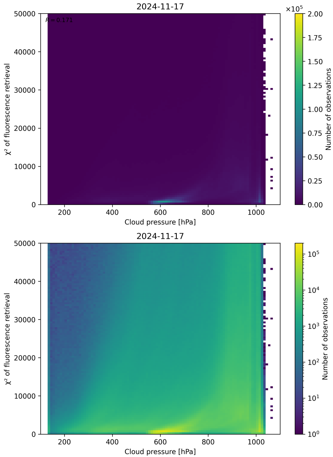
Figure 78: Scatter density plot of “Cloud pressure” against “ \chi^2 of fluorescence retrieval” for 2024-11-17 to 2024-11-18.
