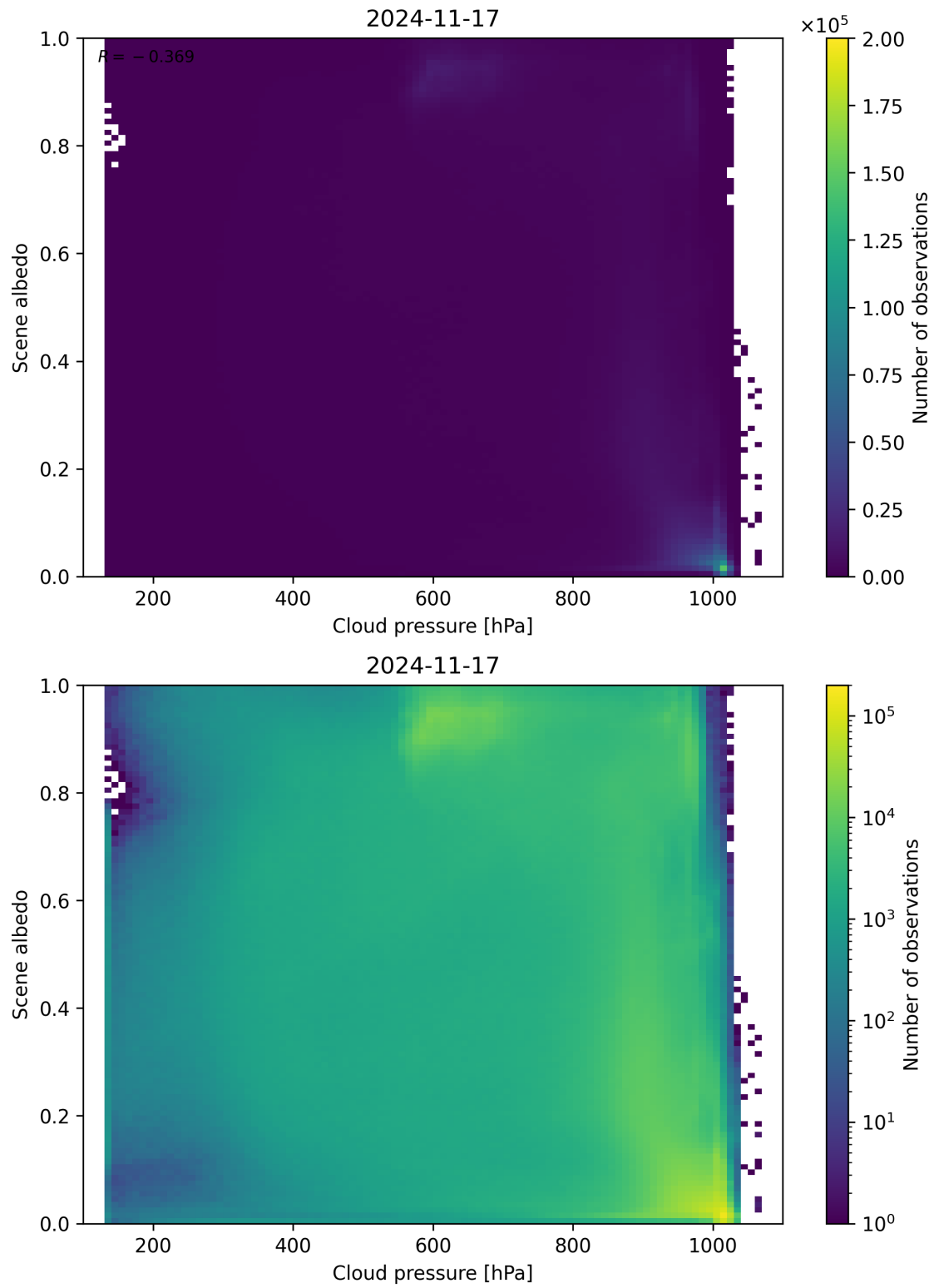
Figure 83: Scatter density plot of “Cloud pressure” against “Scene albedo” for 2024-11-17 to 2024-11-18.
