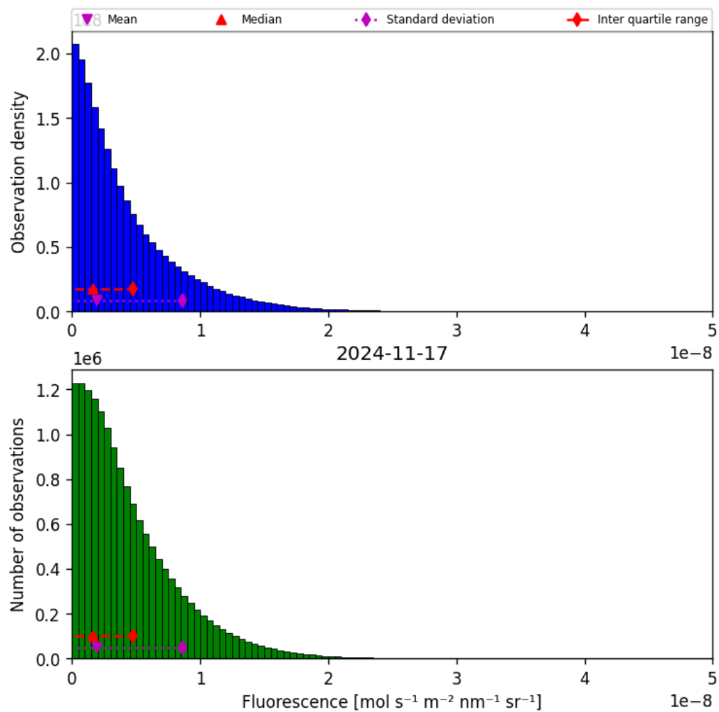
Figure 40: Histogram of “Fluorescence” for 2024-11-17 to 2024-11-18
