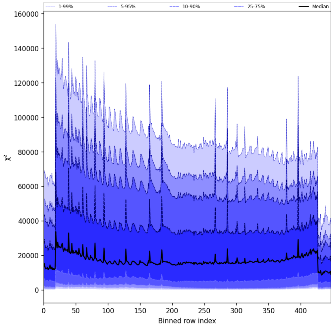
Figure 55: Along track statistics of “ \chi^2 ” for 2024-11-17 to 2024-11-18
