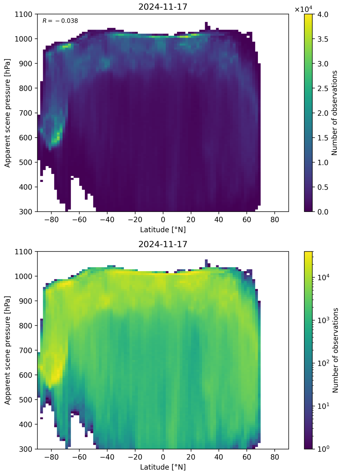
Figure 88: Scatter density plot of “Latitude” against “Apparent scene pressure” for 2024-11-17 to 2024-11-18.
