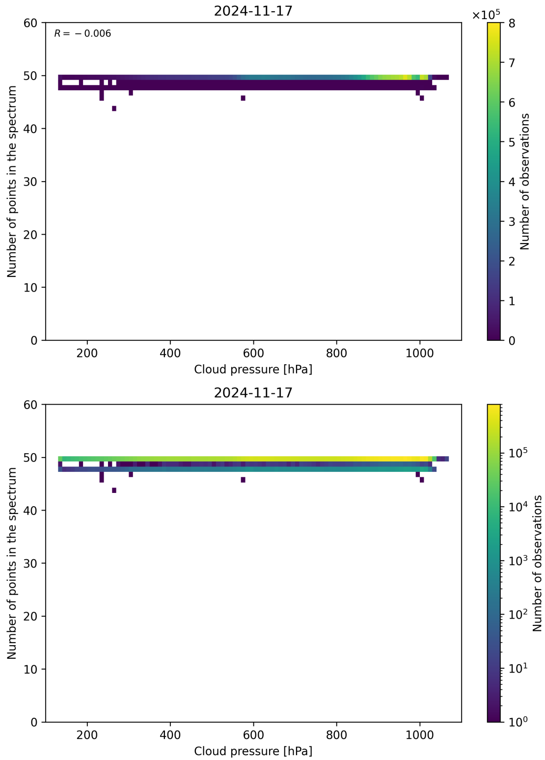
Figure 82: Scatter density plot of “Cloud pressure” against “Number of points in the spectrum” for 2024-11-17 to 2024-11-18.
