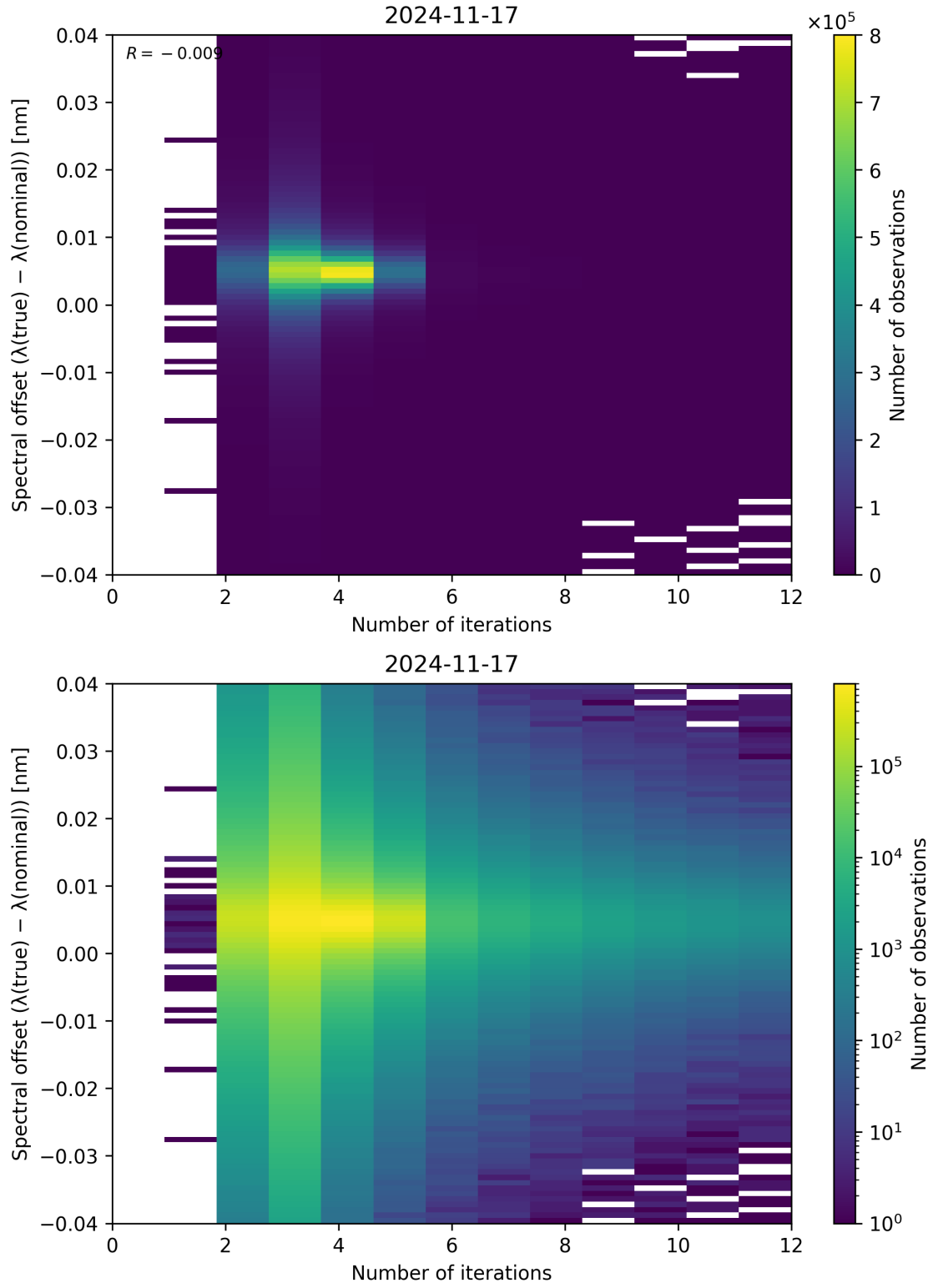
Figure 100: Scatter density plot of “Number of iterations” against “Spectral offset ( \lambda_{\text{true}} - \lambda_{\text{nominal}} )” for 2024-11-17 to 2024-11-18.
