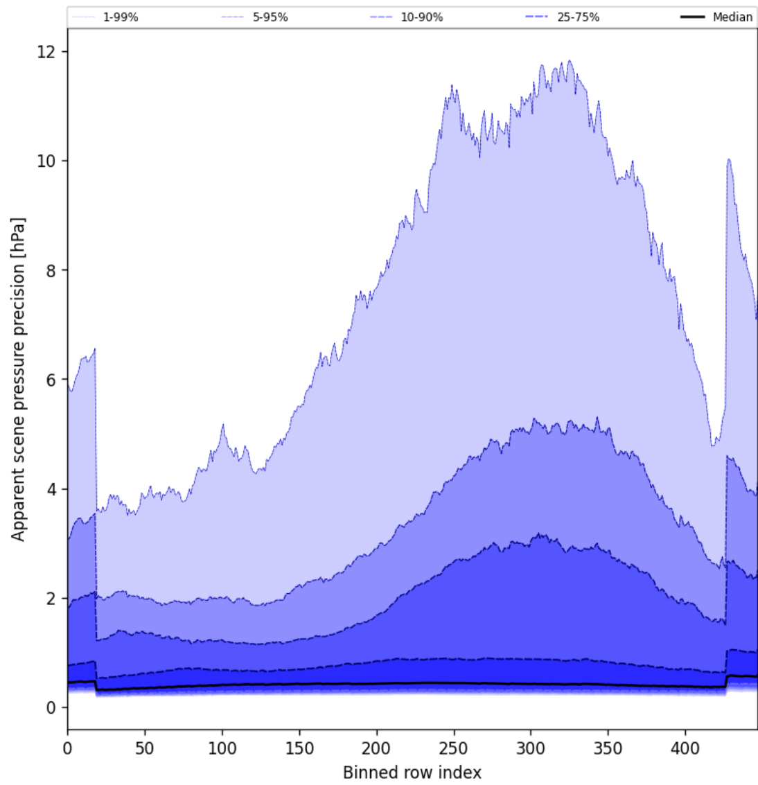
Figure 54: Along track statistics of “Apparent scene pressure precision” for 2024-11-17 to 2024-11-18
