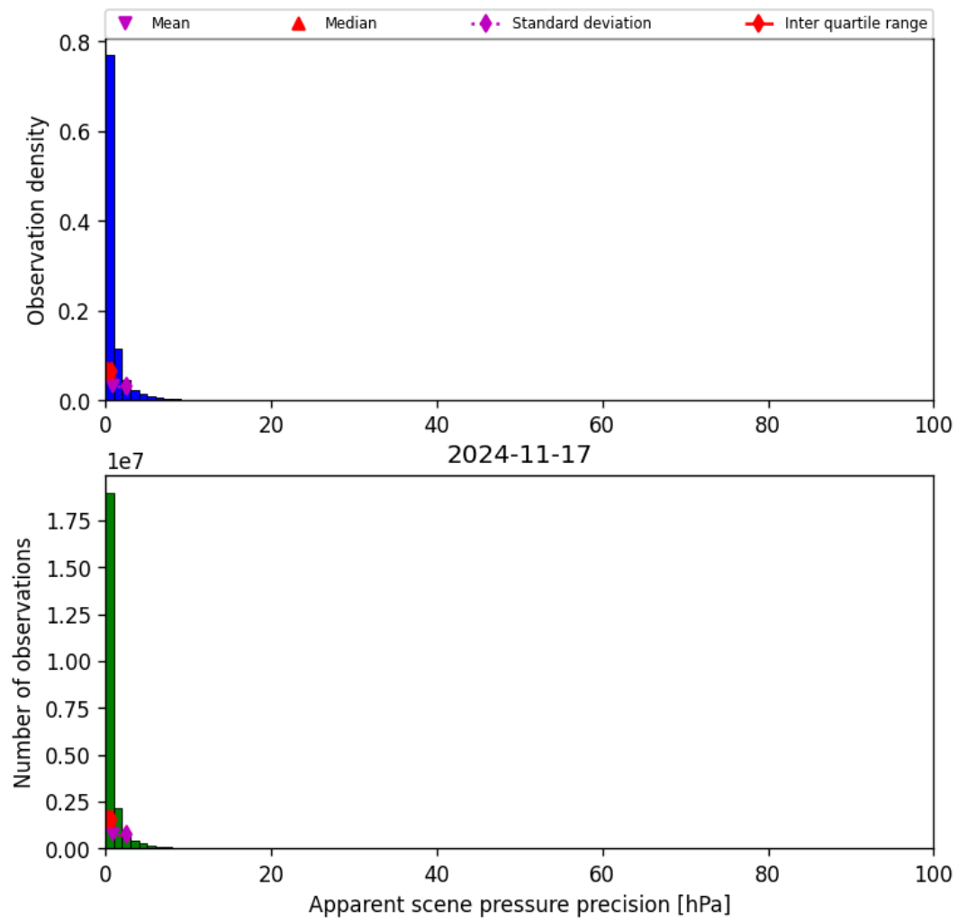
Figure 37: Histogram of “Apparent scene pressure precision” for 2024-11-17 to 2024-11-18
