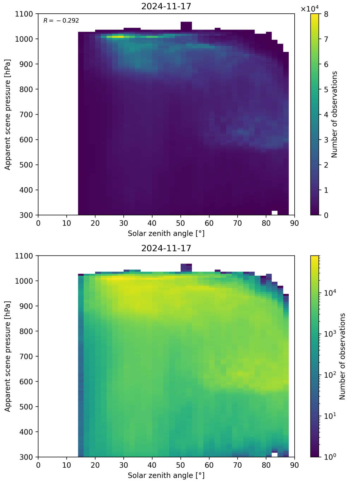
Figure 108: Scatter density plot of “Solar zenith angle” against “Apparent scene pressure” for 2024-11-17 to 2024-11-18.
