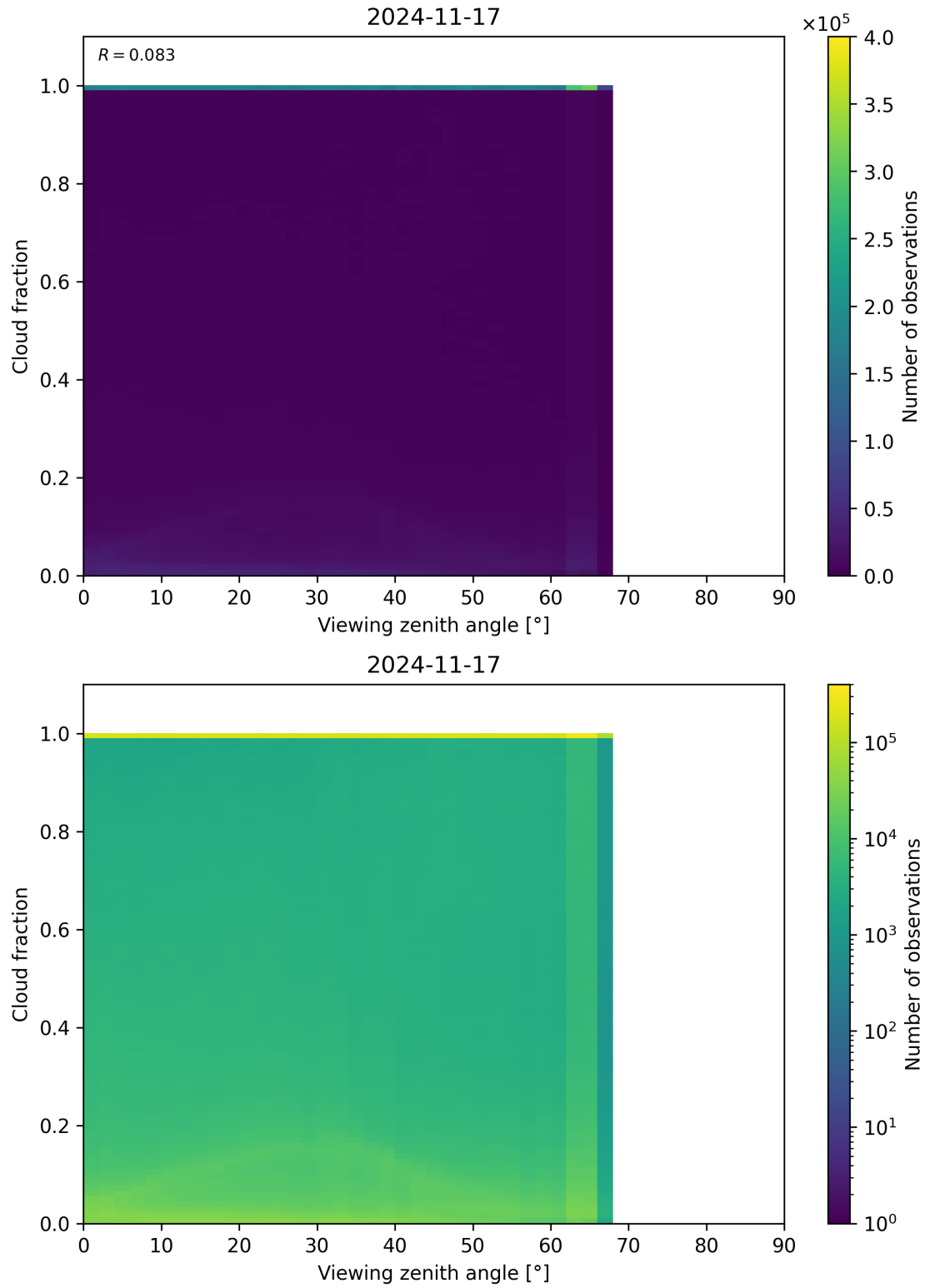
Figure 120: Scatter density plot of “Viewing zenith angle” against “Cloud fraction” for 2024-11-17 to 2024-11-18.
