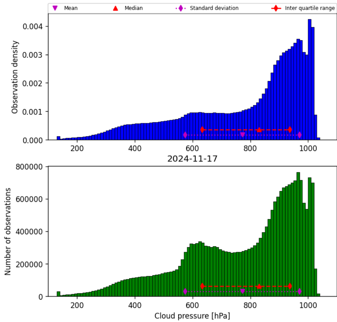
Figure 30: Histogram of “Cloud pressure” for 2024-11-17 to 2024-11-18
