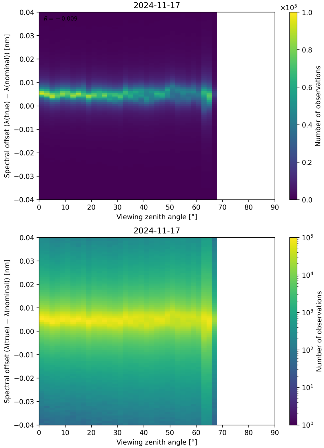
Figure 128: Scatter density plot of “Viewing zenith angle” against “Spectral offset ( \lambda_{\text{true}} - \lambda_{\text{nominal}} )” for 2024-11-17 to 2024-11-18.
