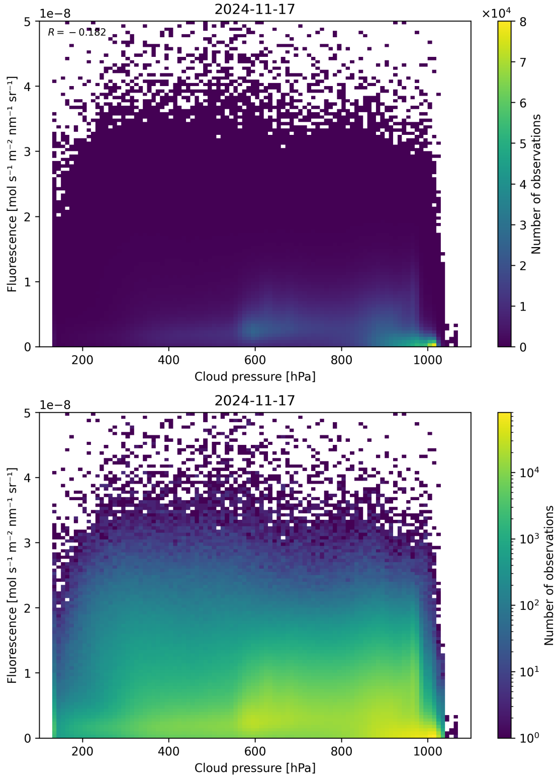
Figure 80: Scatter density plot of “Cloud pressure” against “Fluorescence” for 2024-11-17 to 2024-11-18.
