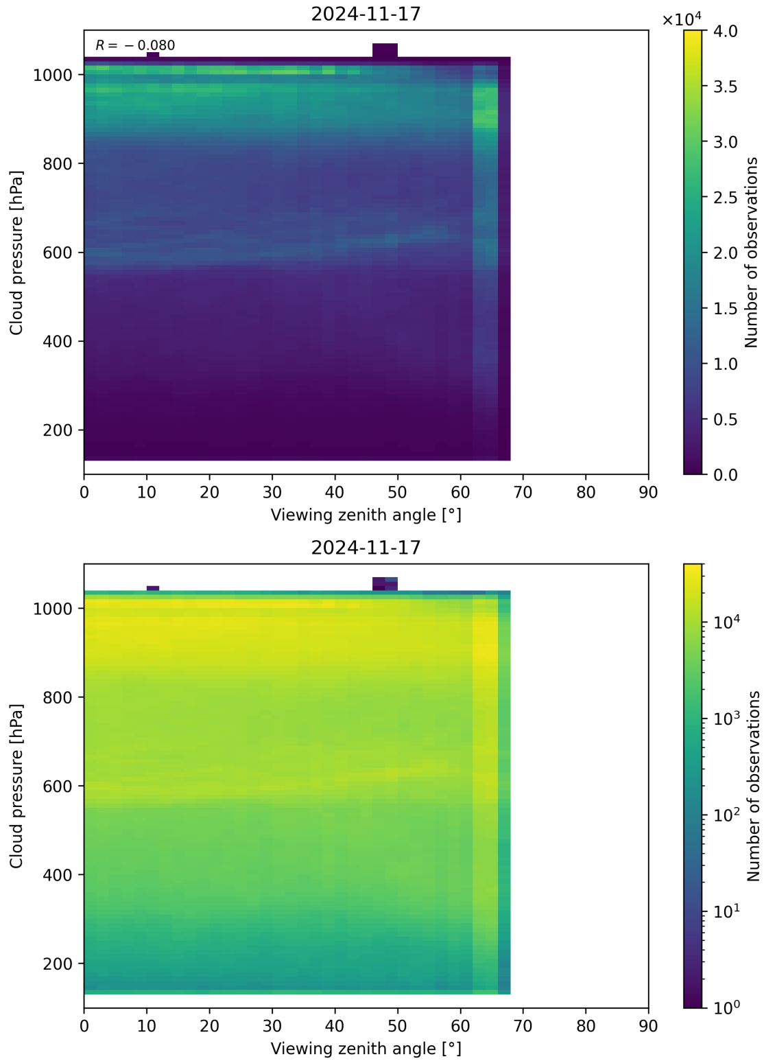
Figure 121: Scatter density plot of “Viewing zenith angle” against “Cloud pressure” for 2024-11-17 to 2024-11-18.
