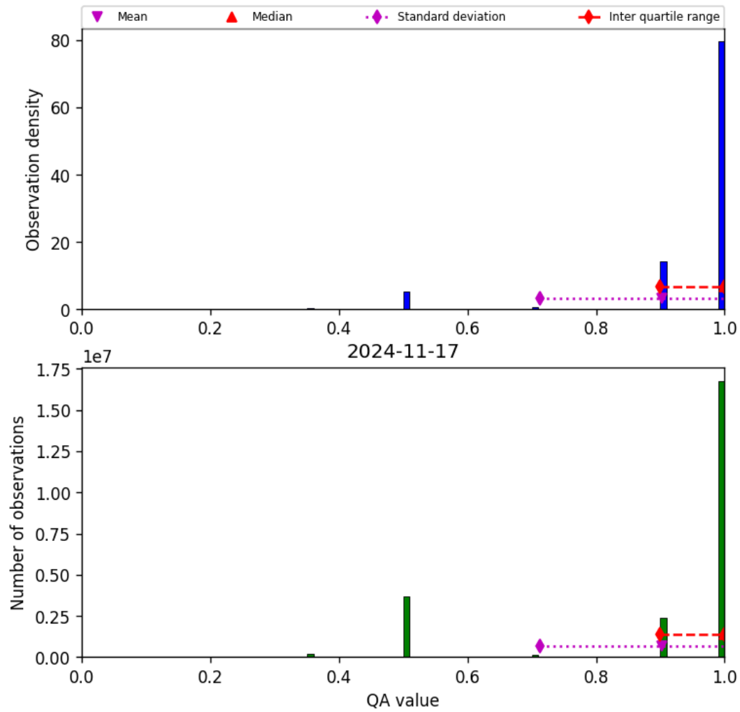
Figure 29: Histogram of “QA value” for 2024-11-17 to 2024-11-18
