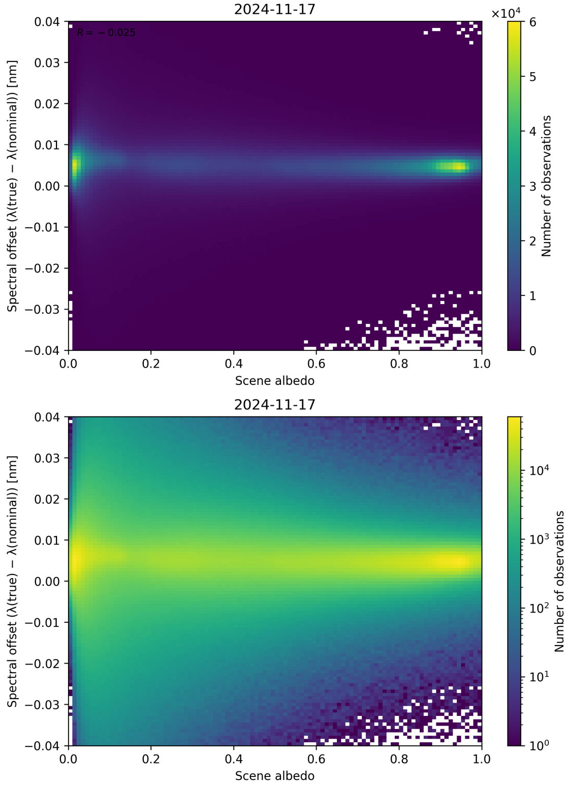
Figure 107: Scatter density plot of “Scene albedo” against “Spectral offset ( \lambda_{\text{true}} - \lambda_{\text{nominal}} )” for 2024-11-17 to 2024-11-18.
