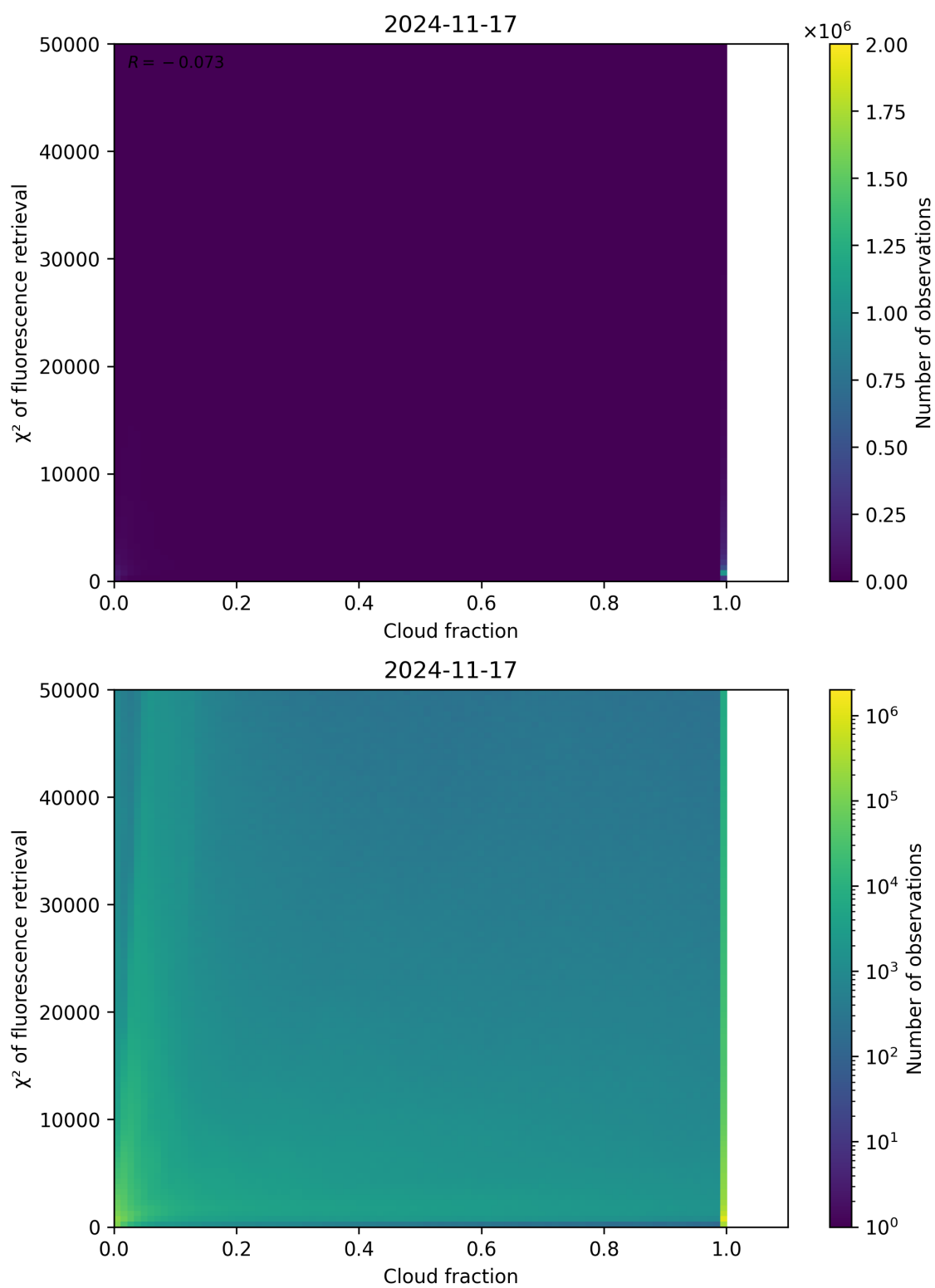
Figure 71: Scatter density plot of “Cloud fraction” against “ \chi^2 of fluorescence retrieval” for 2024-11-17 to 2024-11-18.
