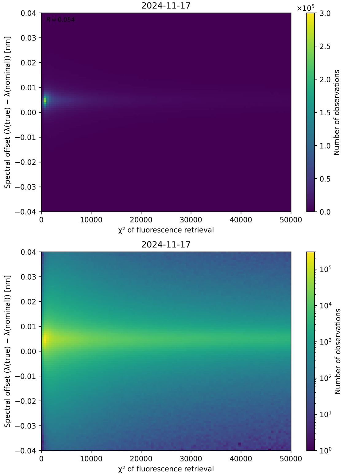
Figure 69: Scatter density plot of “ \chi^2 of fluorescence retrieval” against “Spectral offset ( \lambda_{\text{true}} - \lambda_{\text{nominal}} )” for 2024-11-17 to 2024-11-18.
