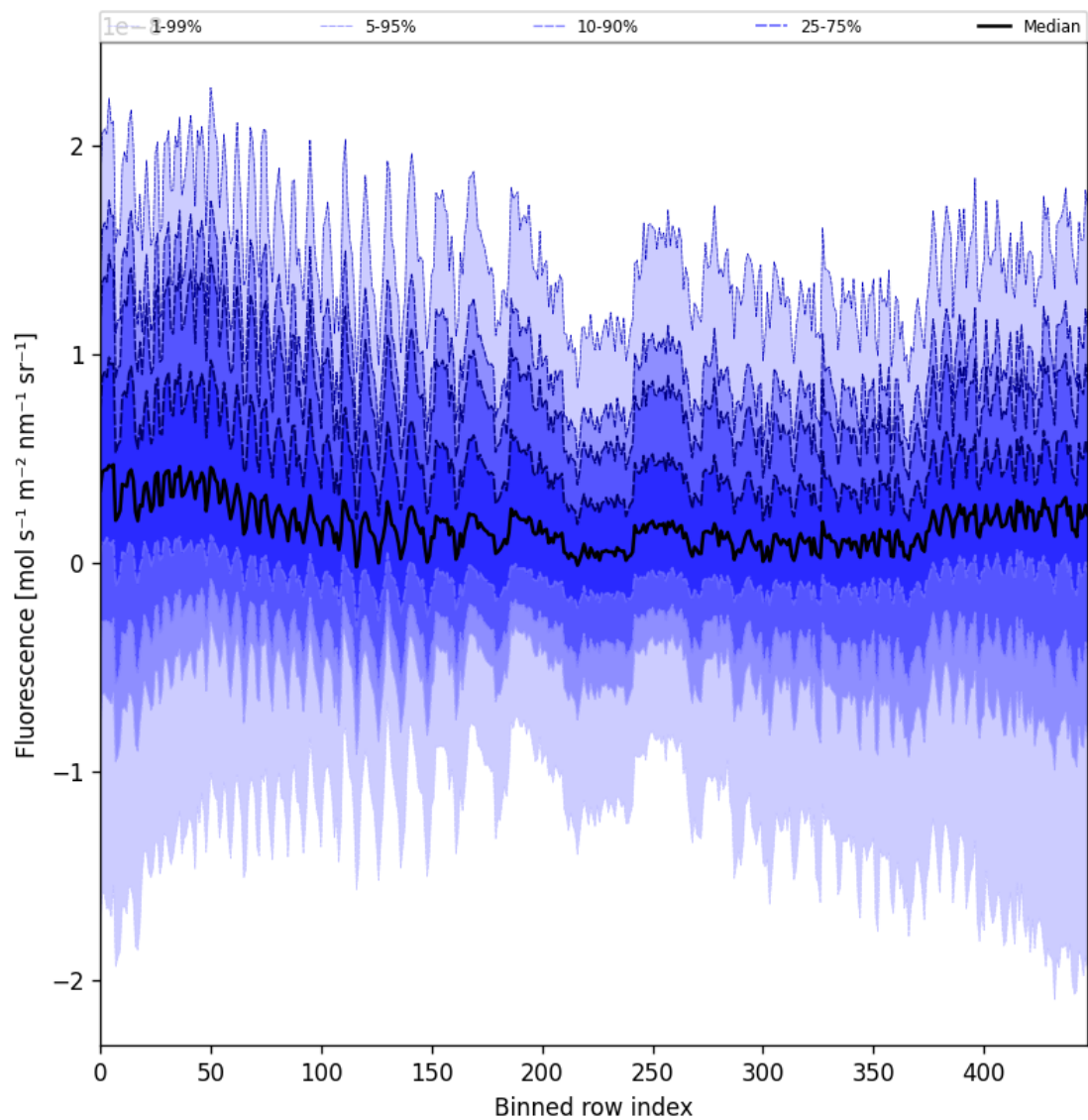
Figure 57: Along track statistics of “Fluorescence” for 2024-11-17 to 2024-11-18
