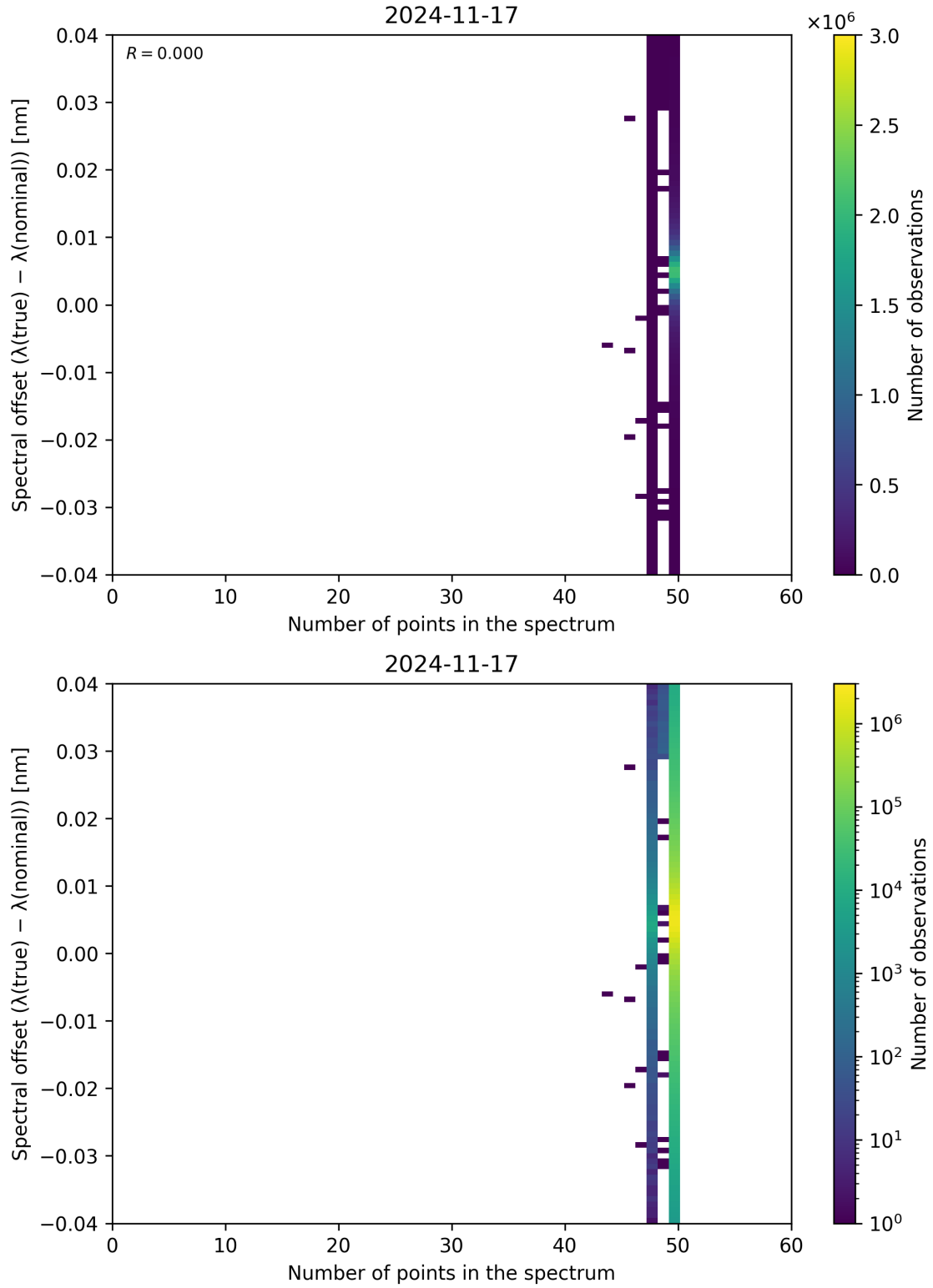
Figure 101: Scatter density plot of “Number of points in the spectrum” against “Spectral offset ( \lambda_{\text{true}} - \lambda_{\text{nominal}} )” for 2024-11-17 to 2024-11-18.
