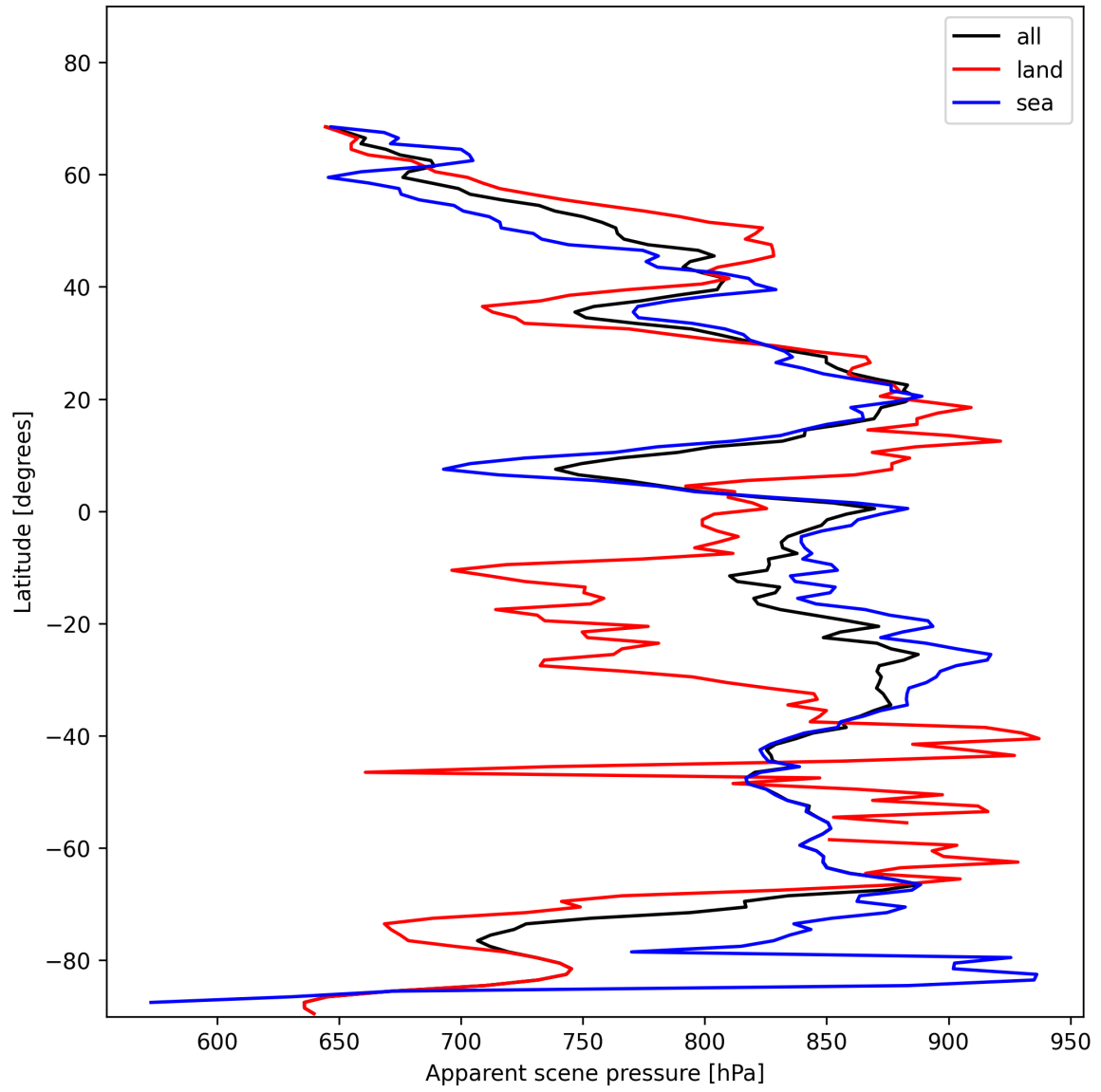
Figure 19: Zonal average of “Apparent scene pressure” for 2024-11-17 to 2024-11-18.
