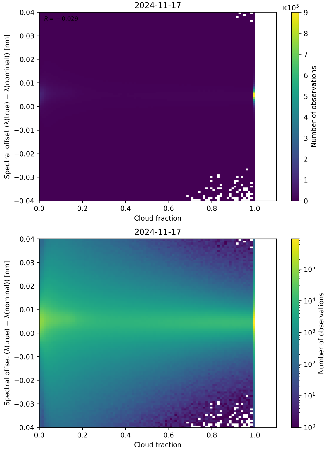
Figure 76: Scatter density plot of “Cloud fraction” against “Spectral offset ( \lambda_{\text{true}} - \lambda_{\text{nominal}} )” for 2024-11-17 to 2024-11-18.
