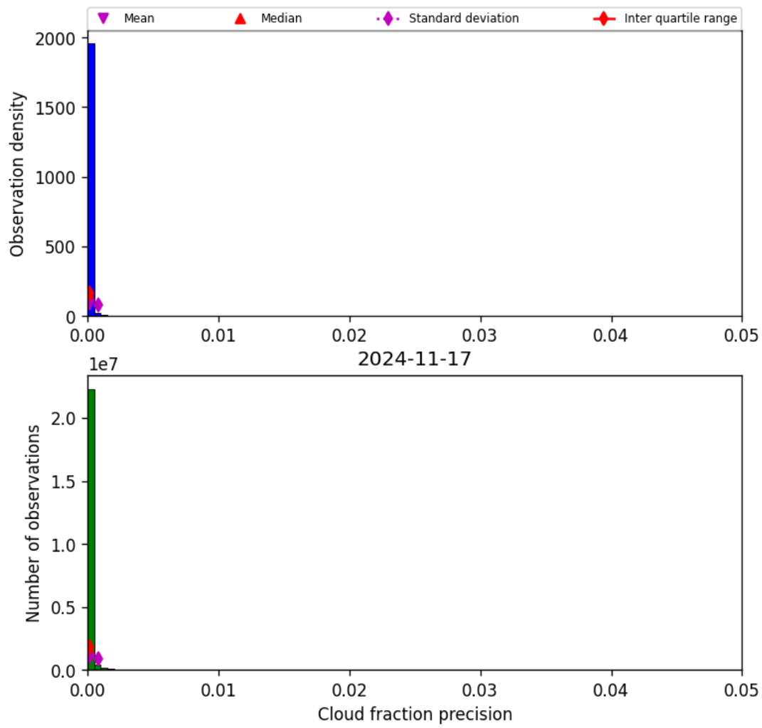
Figure 33: Histogram of “Cloud fraction precision” for 2024-11-17 to 2024-11-18
