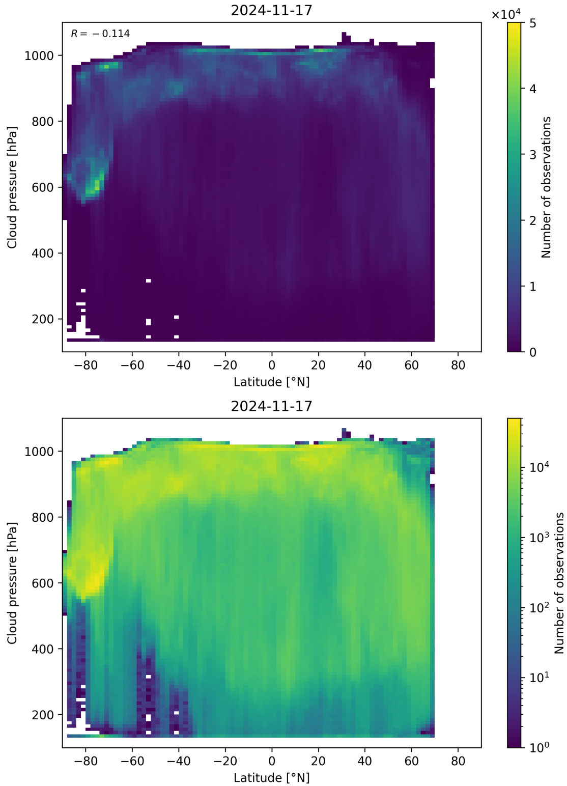
Figure 91: Scatter density plot of “Latitude” against “Cloud pressure” for 2024-11-17 to 2024-11-18.
