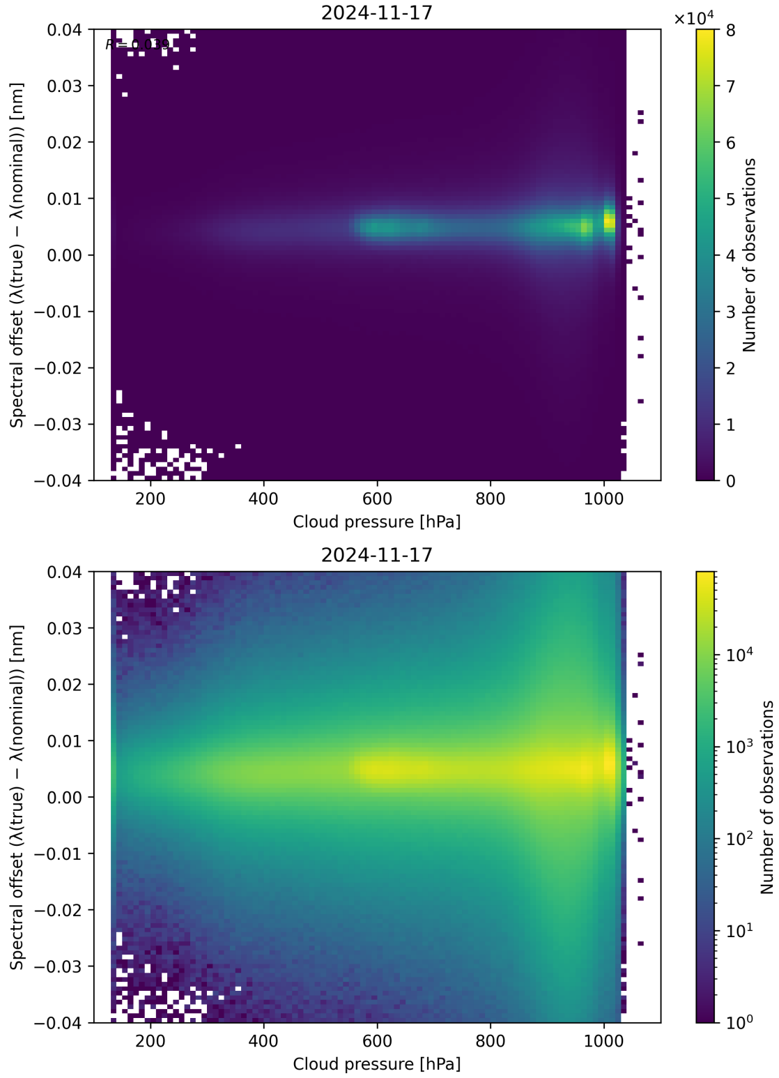
Figure 84: Scatter density plot of “Cloud pressure” against “Spectral offset ( \lambda_{\text{true}} - \lambda_{\text{nominal}} )” for 2024-11-17 to 2024-11-18.
