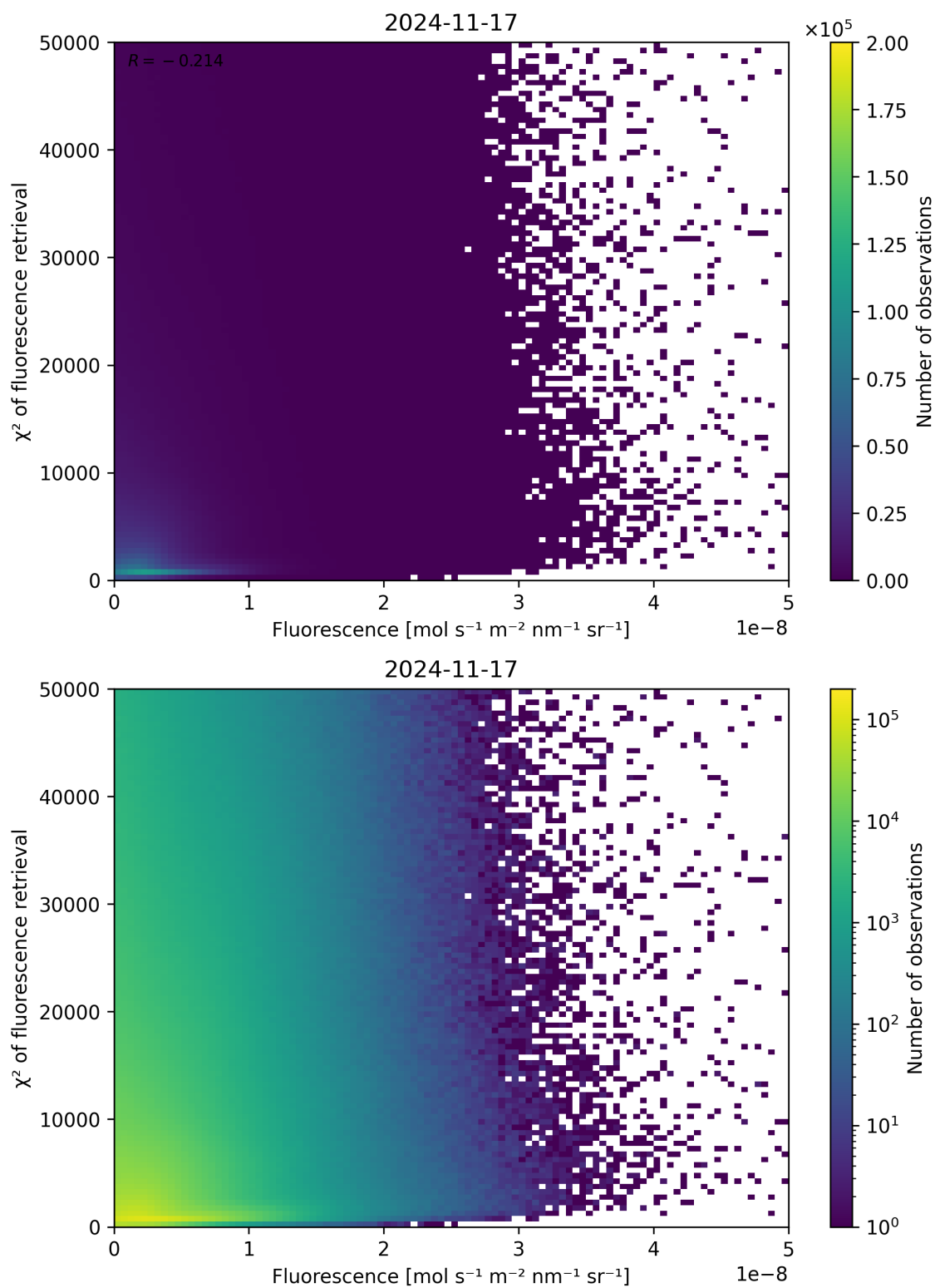
Figure 85: Scatter density plot of “Fluorescence” against “ \chi^2 of fluorescence retrieval” for 2024-11-17 to 2024-11-18.
