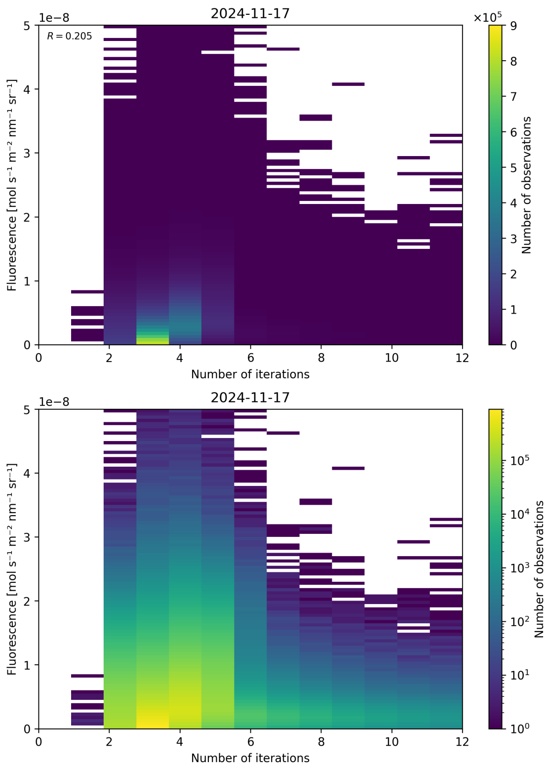
Figure 98: Scatter density plot of “Number of iterations” against “Fluorescence” for 2024-11-17 to 2024-11-18.
