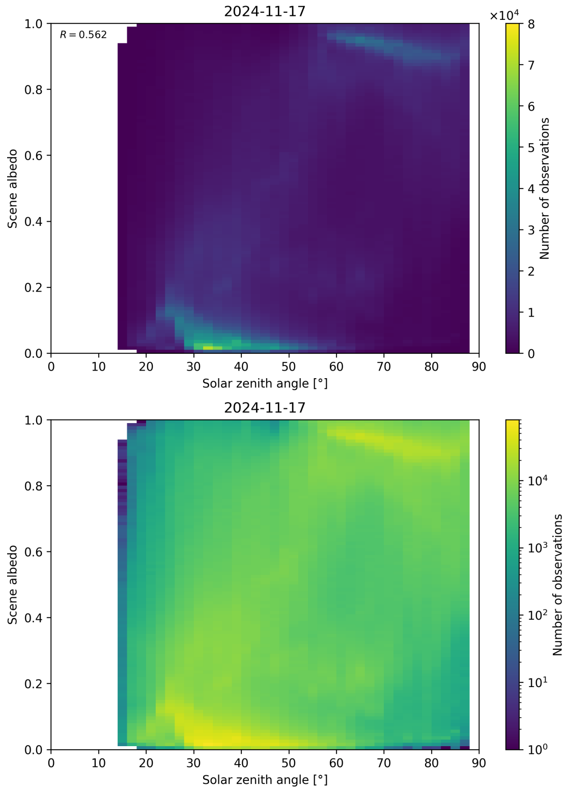
Figure 116: Scatter density plot of “Solar zenith angle” against “Scene albedo” for 2024-11-17 to 2024-11-18.
