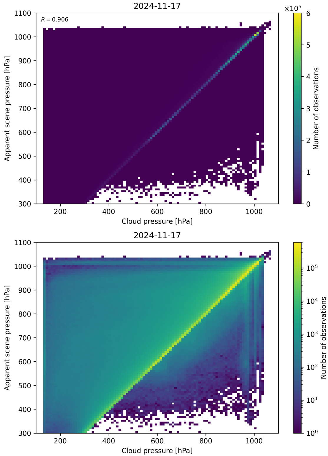
Figure 77: Scatter density plot of “Cloud pressure” against “Apparent scene pressure” for 2024-11-17 to 2024-11-18.
