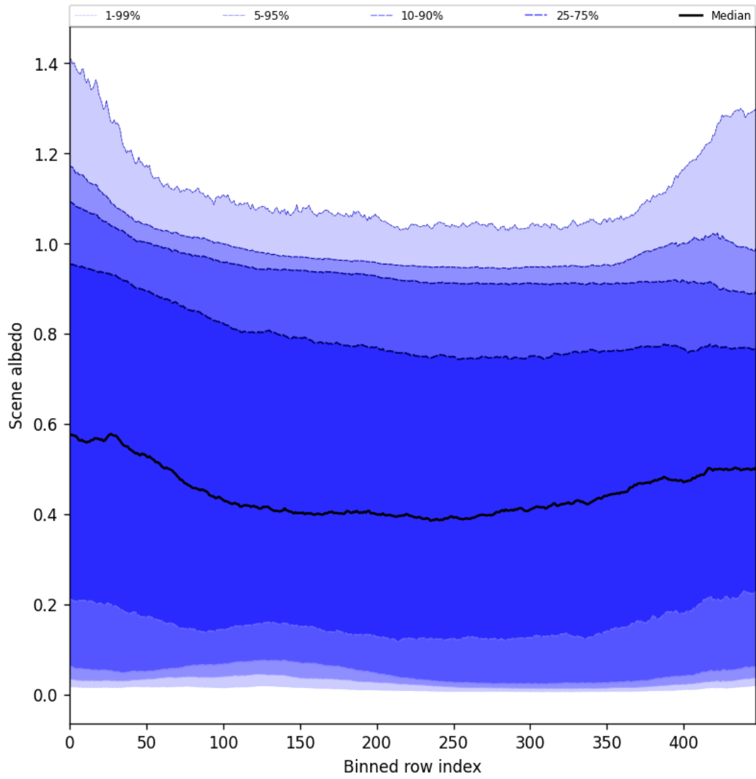
Figure 51: Along track statistics of “Scene albedo” for 2024-11-17 to 2024-11-18
