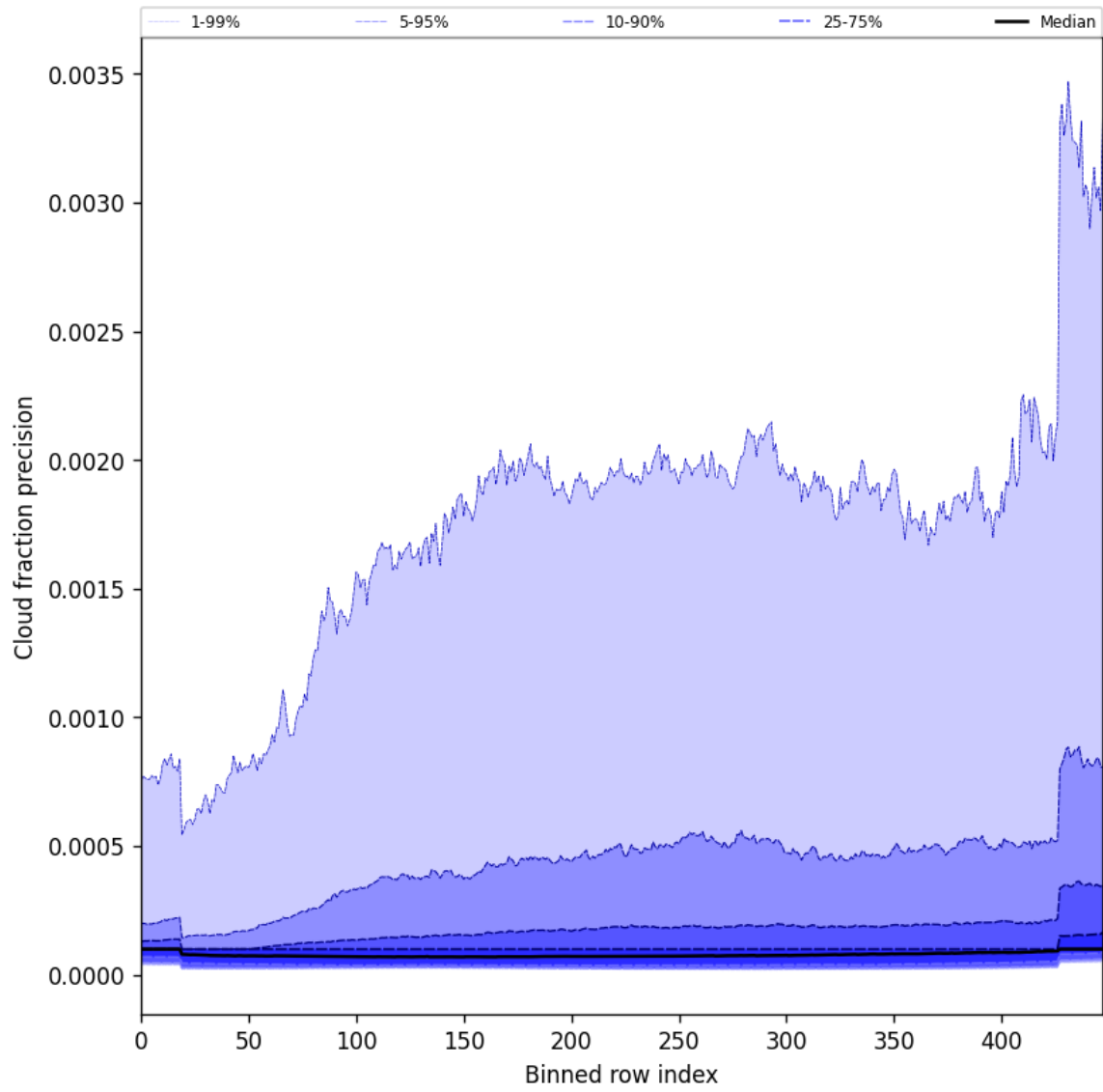
Figure 50: Along track statistics of “Cloud fraction precision” for 2024-11-17 to 2024-11-18
