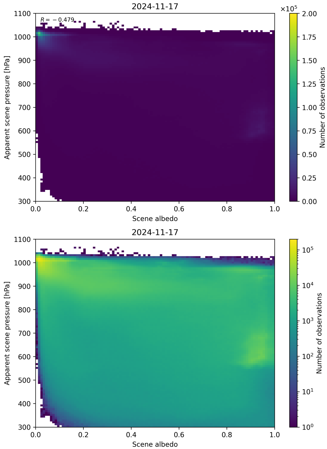
Figure 102: Scatter density plot of “Scene albedo” against “Apparent scene pressure” for 2024-11-17 to 2024-11-18.
