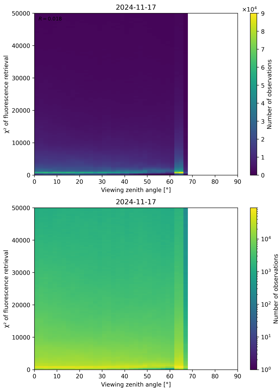
Figure 119: Scatter density plot of “Viewing zenith angle” against “ \chi^2 of fluorescence retrieval” for 2024-11-17 to 2024-11-18.
