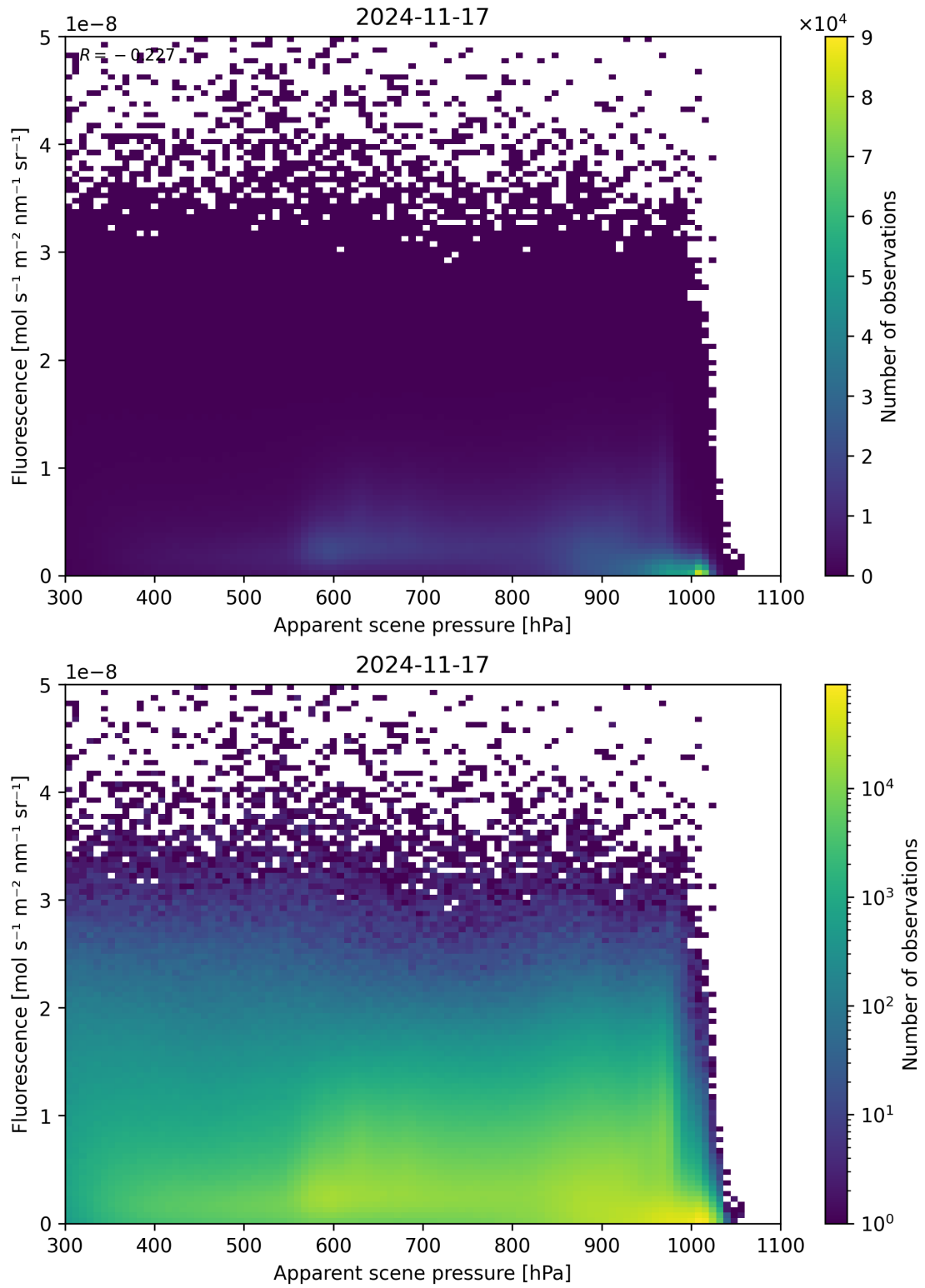
Figure 64: Scatter density plot of “Apparent scene pressure” against “Fluorescence” for 2024-11-17 to 2024-11-18.
