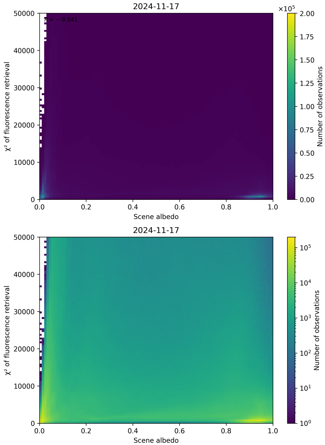
Figure 103: Scatter density plot of “Scene albedo” against “ \chi^2 of fluorescence retrieval” for 2024-11-17 to 2024-11-18.
