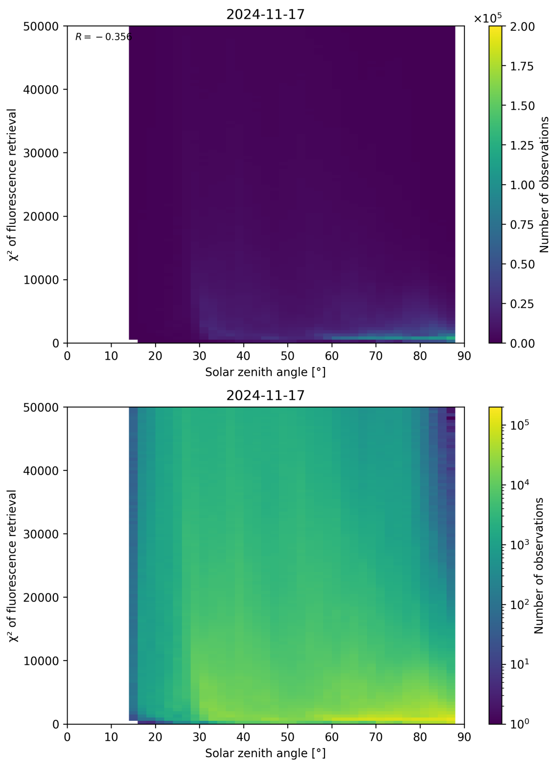
Figure 109: Scatter density plot of “Solar zenith angle” against “ \chi^2 of fluorescence retrieval” for 2024-11-17 to 2024-11-18.
