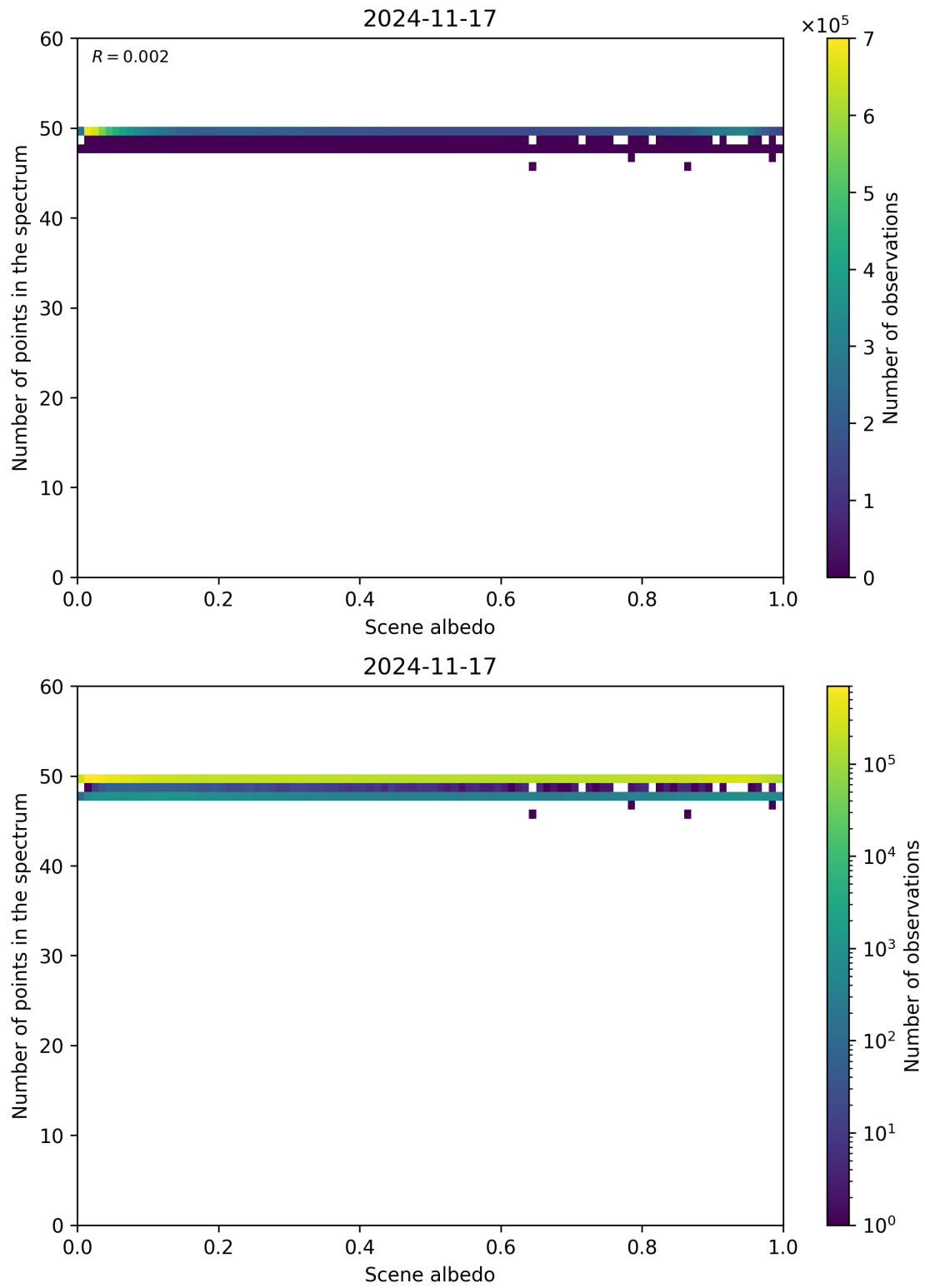
Figure 106: Scatter density plot of “Scene albedo” against “Number of points in the spectrum” for 2024-11-17 to 2024-11-18.
