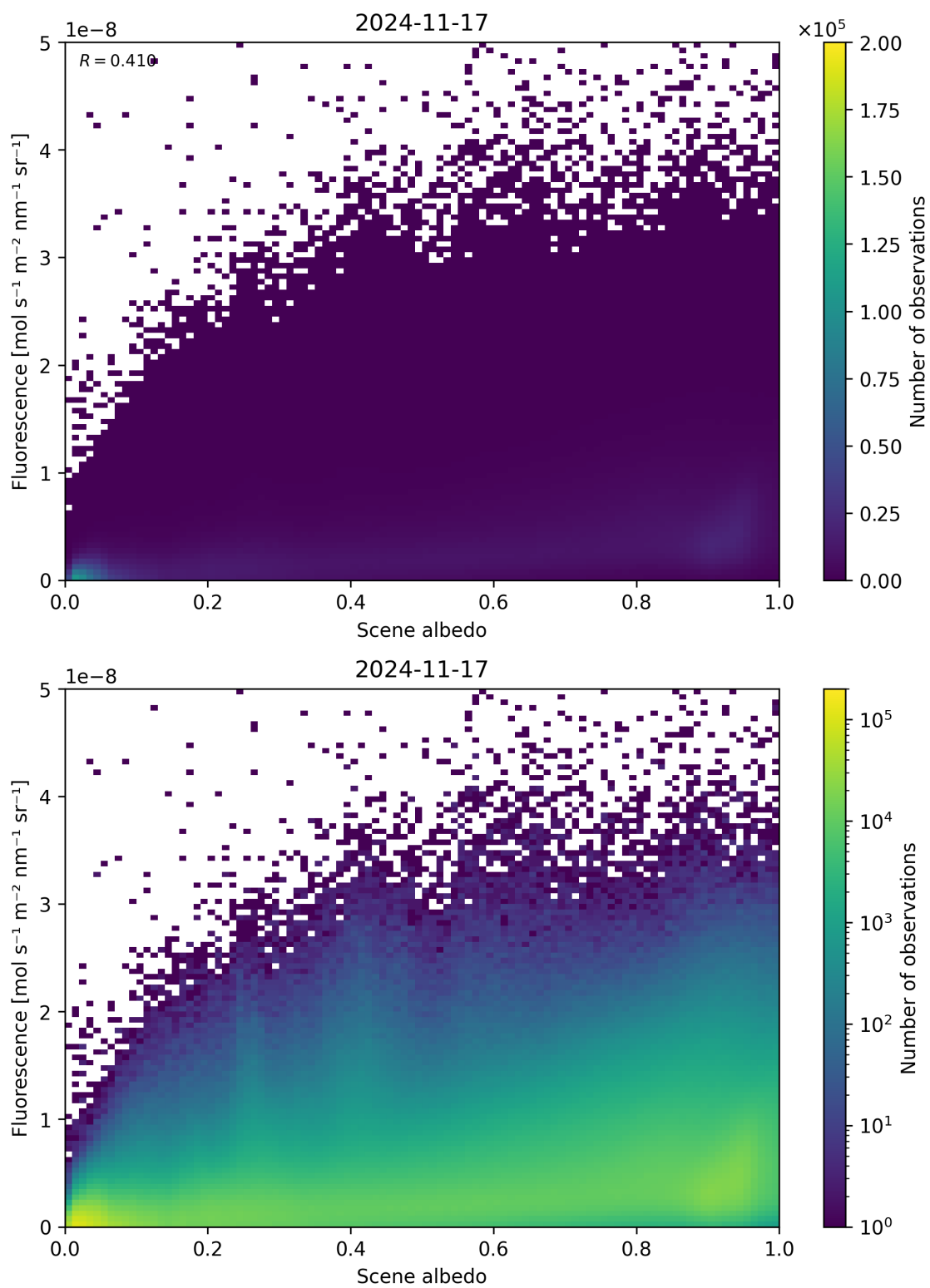
Figure 104: Scatter density plot of “Scene albedo” against “Fluorescence” for 2024-11-17 to 2024-11-18.
