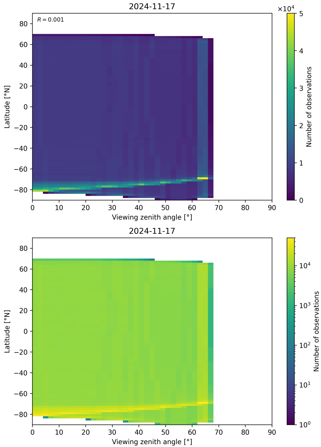
Figure 123: Scatter density plot of “Viewing zenith angle” against “Latitude” for 2024-11-17 to 2024-11-18.
