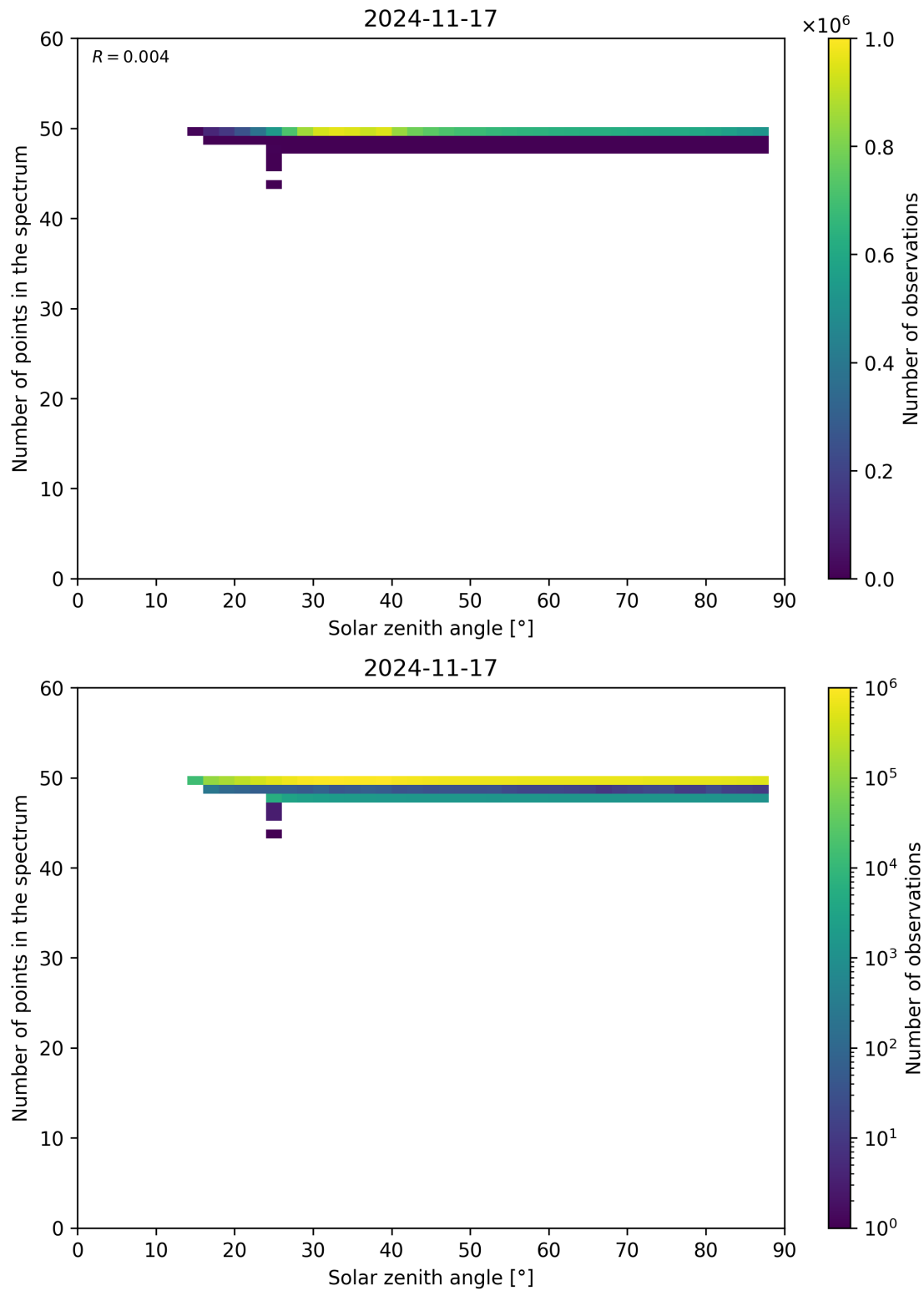
Figure 115: Scatter density plot of “Solar zenith angle” against “Number of points in the spectrum” for 2024-11-17 to 2024-11-18.
