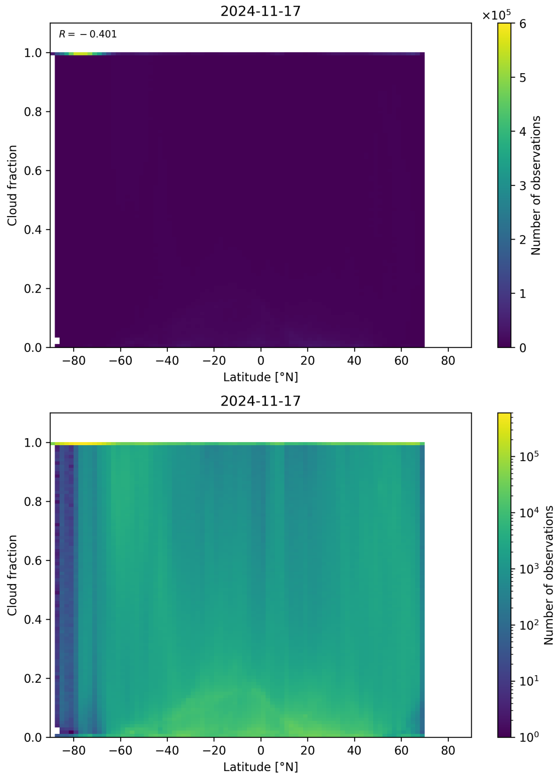
Figure 90: Scatter density plot of “Latitude” against “Cloud fraction” for 2024-11-17 to 2024-11-18.
