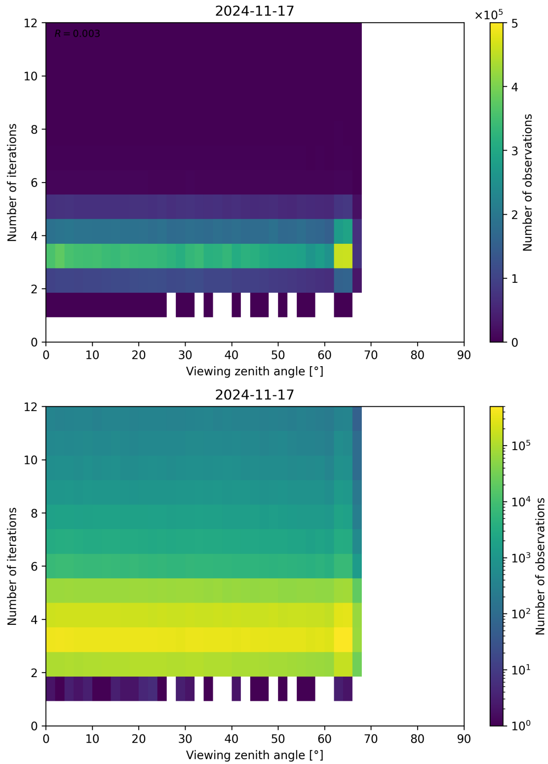
Figure 124: Scatter density plot of “Viewing zenith angle” against “Number of iterations” for 2024-11-17 to 2024-11-18.
