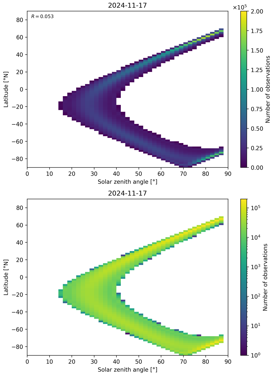
Figure 113: Scatter density plot of “Solar zenith angle” against “Latitude” for 2024-11-17 to 2024-11-18.
