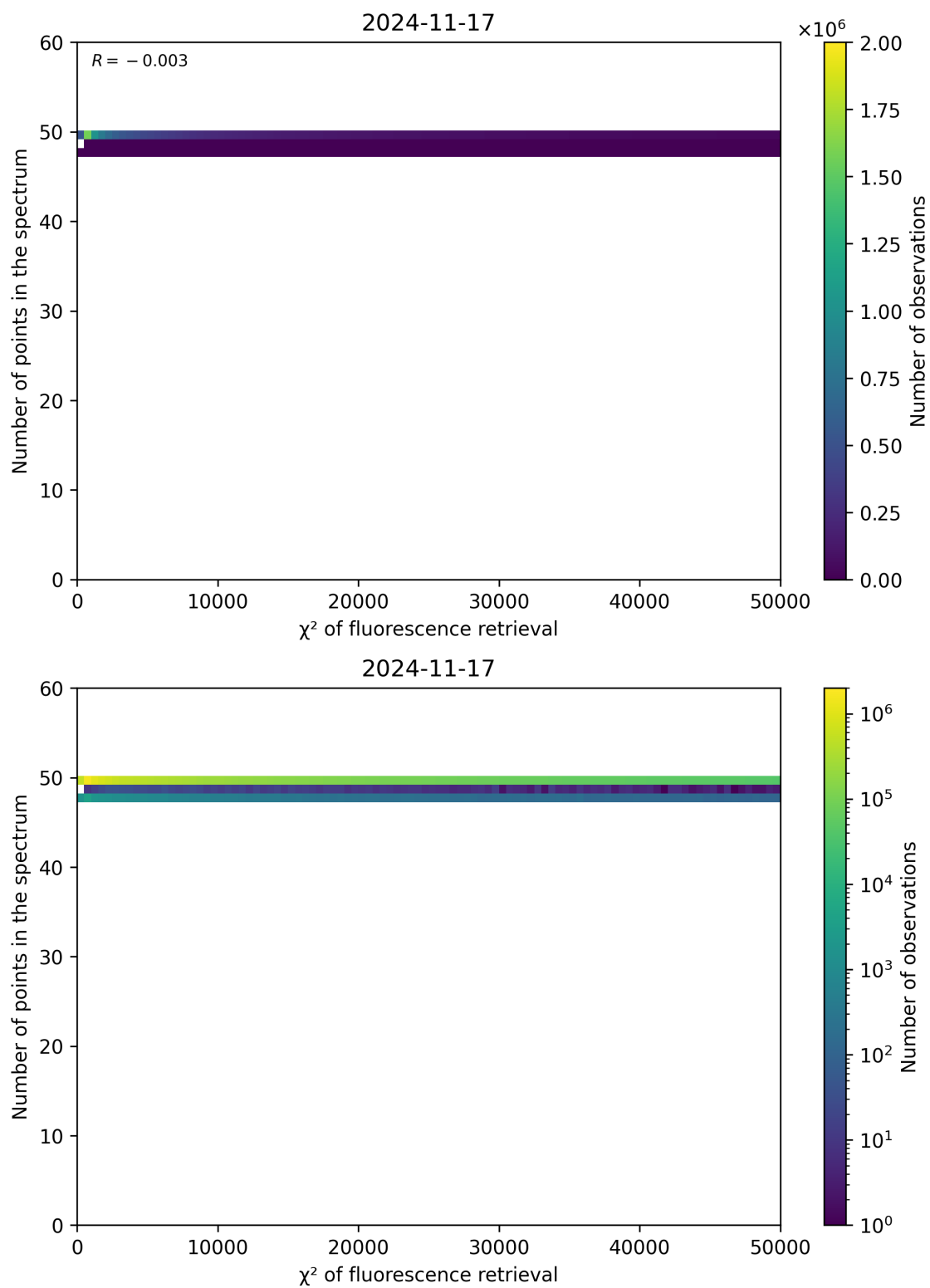
Figure 68: Scatter density plot of “ \chi^2 of fluorescence retrieval” against “Number of points in the spectrum” for 2024-11-17 to 2024-11-18.
