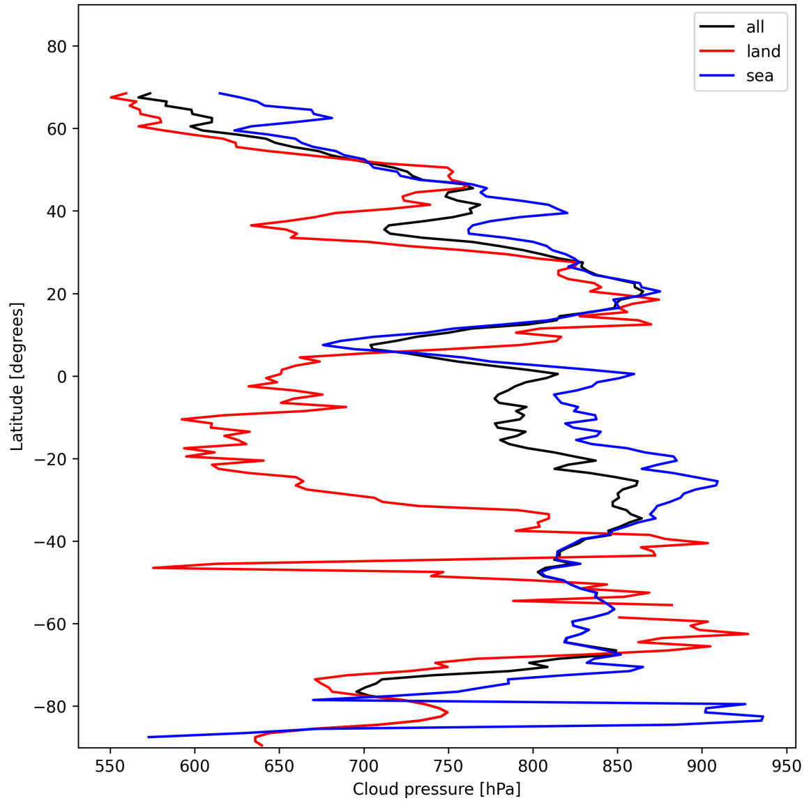
Figure 13: Zonal average of “Cloud pressure” for 2024-11-17 to 2024-11-18.
