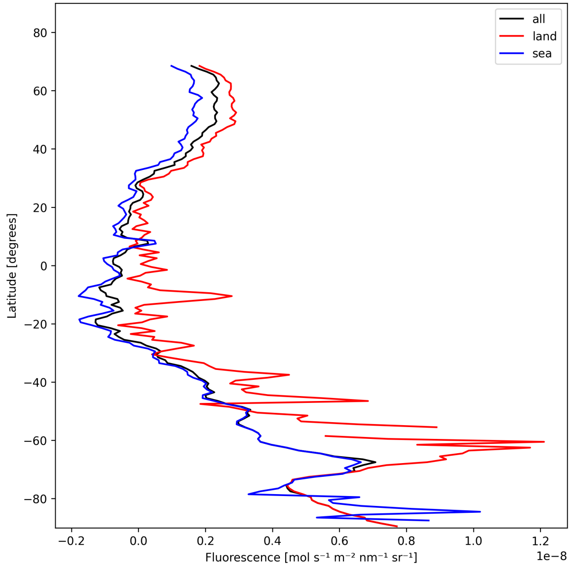
Figure 23: Zonal average of “Fluorescence” for 2024-11-17 to 2024-11-18.
