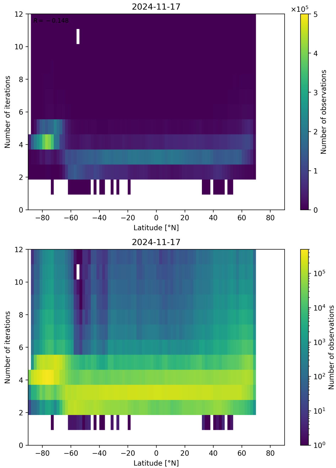
Figure 93: Scatter density plot of “Latitude” against “Number of iterations” for 2024-11-17 to 2024-11-18.
