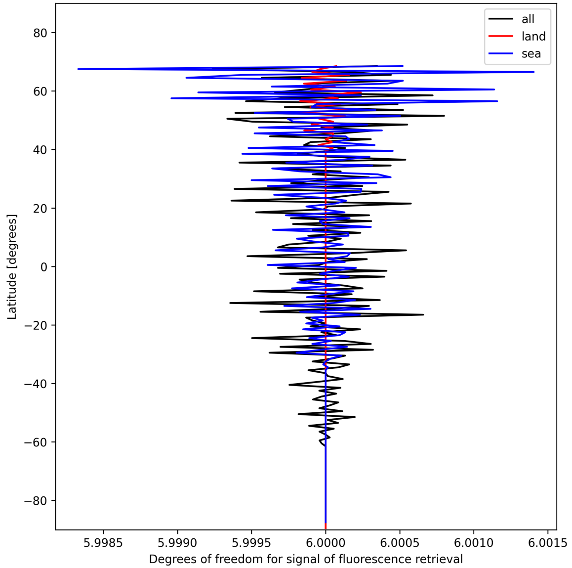
Figure 26: Zonal average of “Degrees of freedom for signal of fluorescence retrieval” for 2024-11-17 to 2024-11-18.
