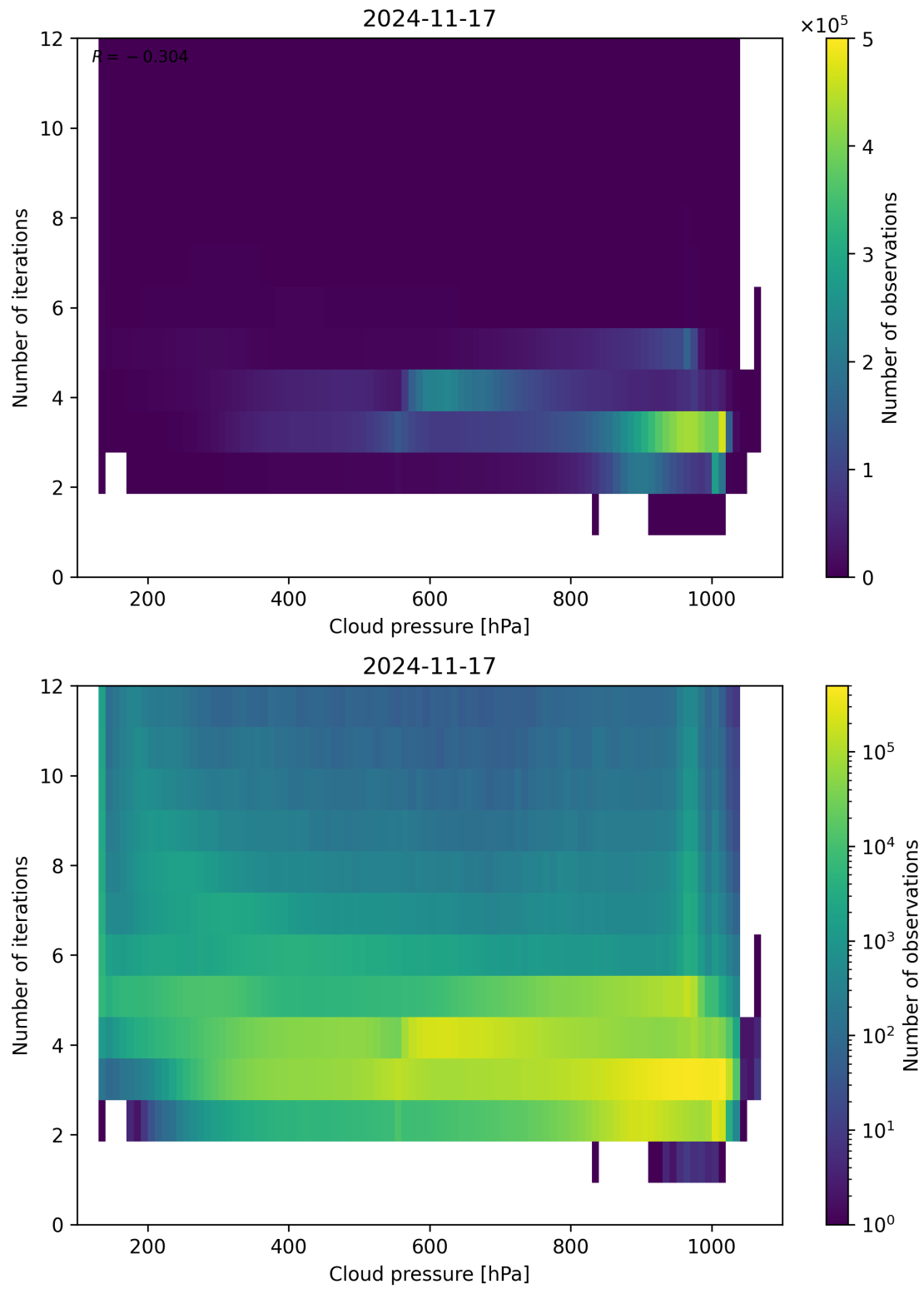
Figure 81: Scatter density plot of “Cloud pressure” against “Number of iterations” for 2024-11-17 to 2024-11-18.
