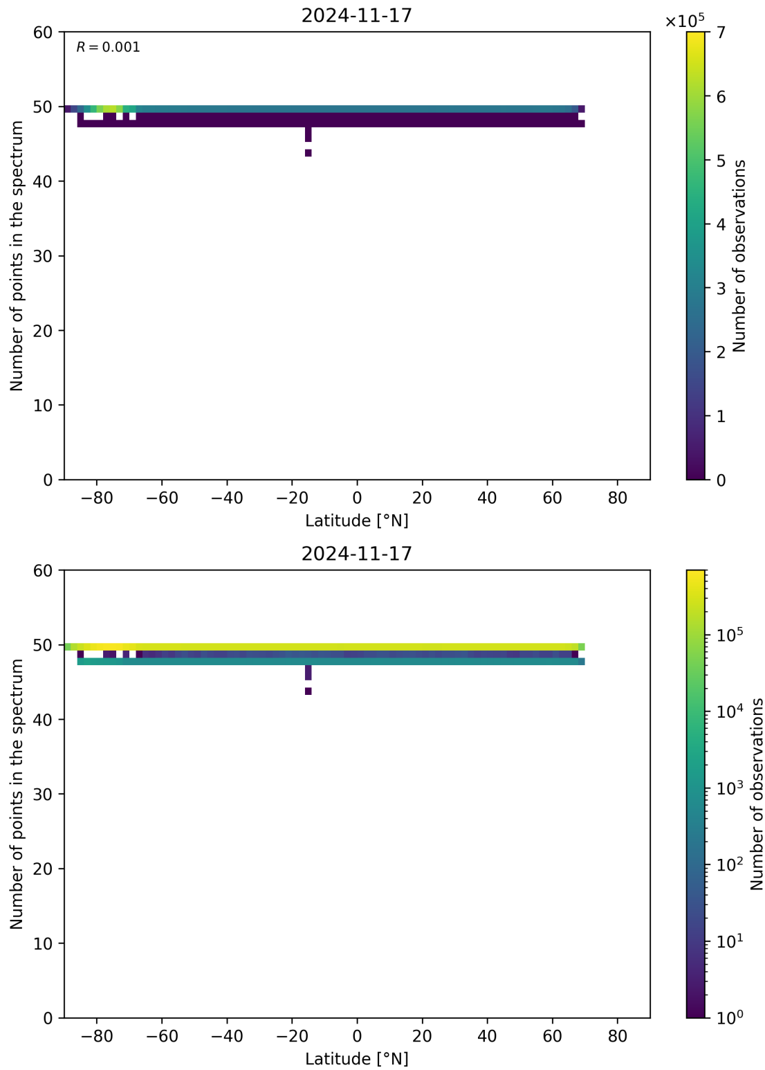
Figure 94: Scatter density plot of “Latitude” against “Number of points in the spectrum” for 2024-11-17 to 2024-11-18.
