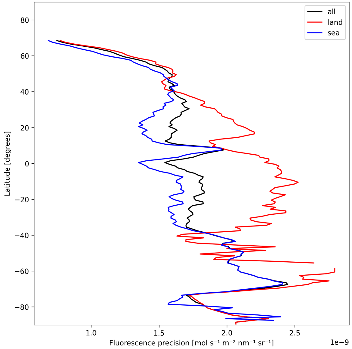
Figure 24: Zonal average of “Fluorescence precision” for 2024-11-17 to 2024-11-18.
