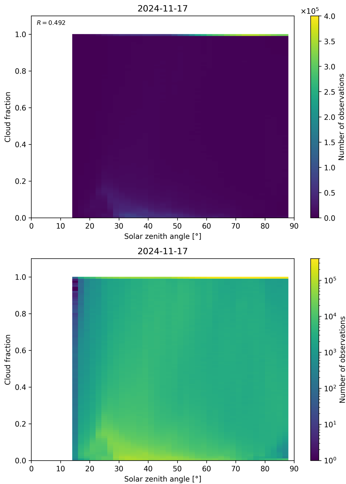
Figure 110: Scatter density plot of “Solar zenith angle” against “Cloud fraction” for 2024-11-17 to 2024-11-18.
