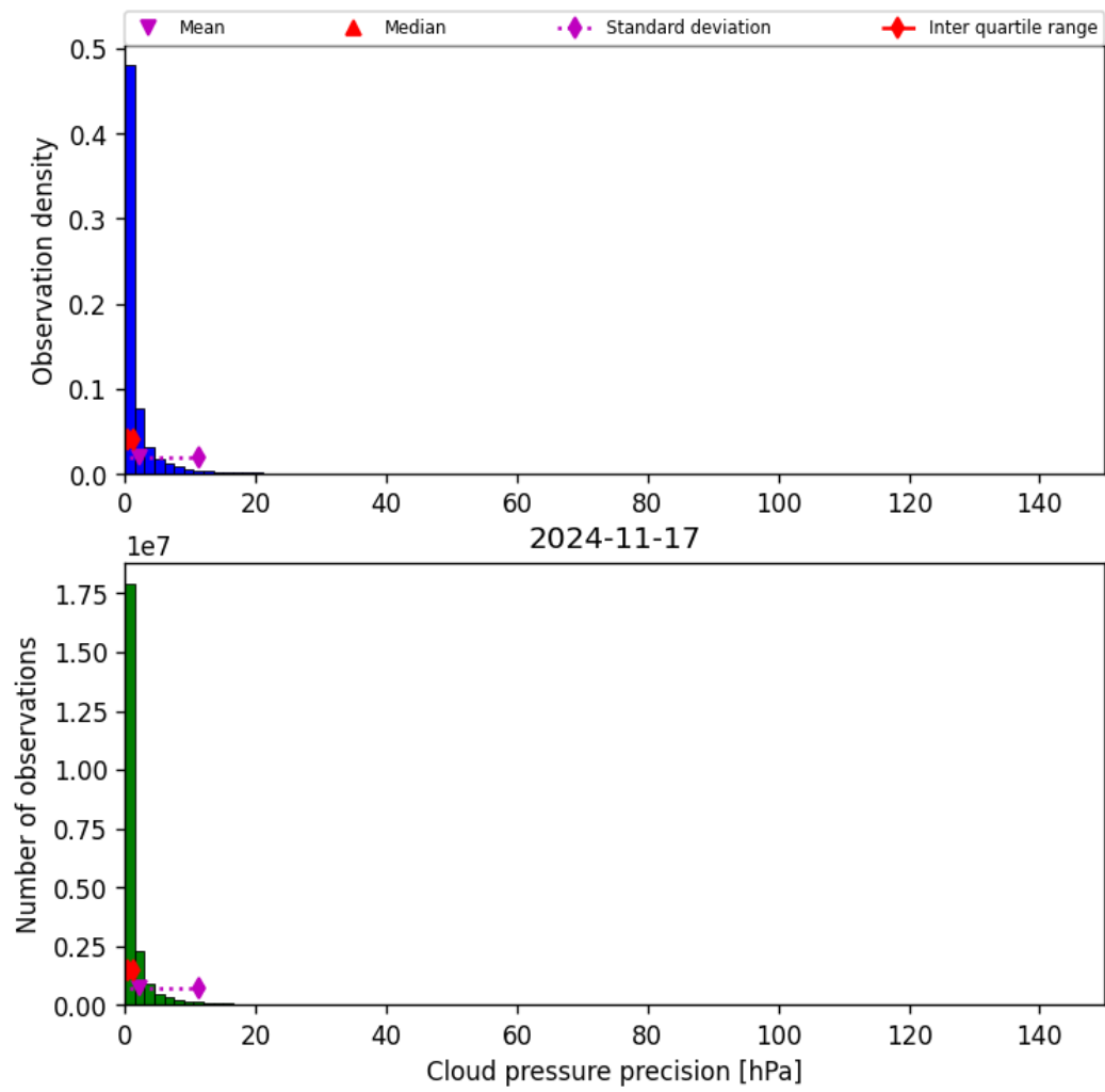
Figure 31: Histogram of “Cloud pressure precision” for 2024-11-17 to 2024-11-18
