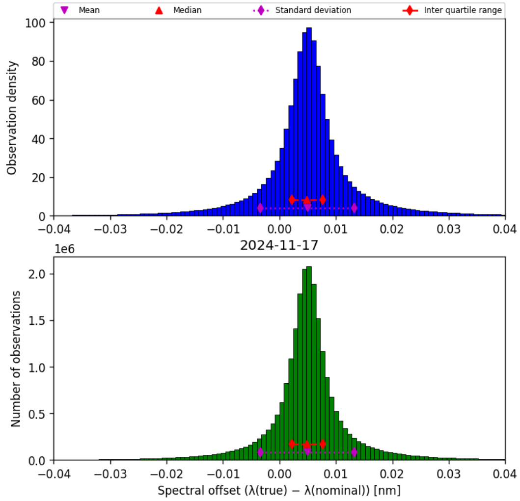
Figure 45: Histogram of “Spectral offset ( \lambda_{\text{true}} - \lambda_{\text{nominal}} )” for 2024-11-17 to 2024-11-18
