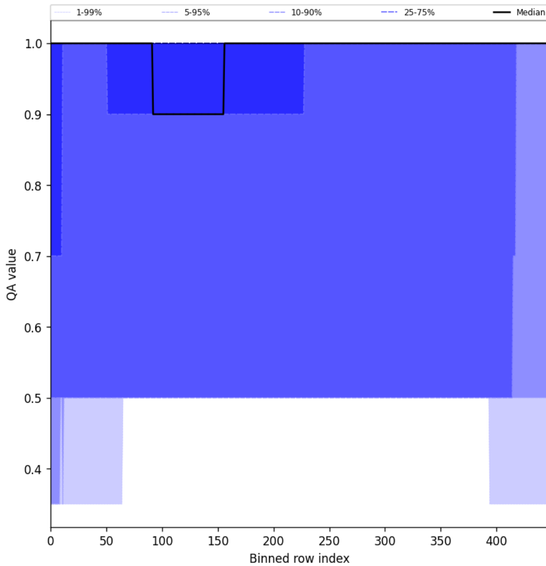
Figure 46: Along track statistics of “QA value” for 2024-11-17 to 2024-11-18
