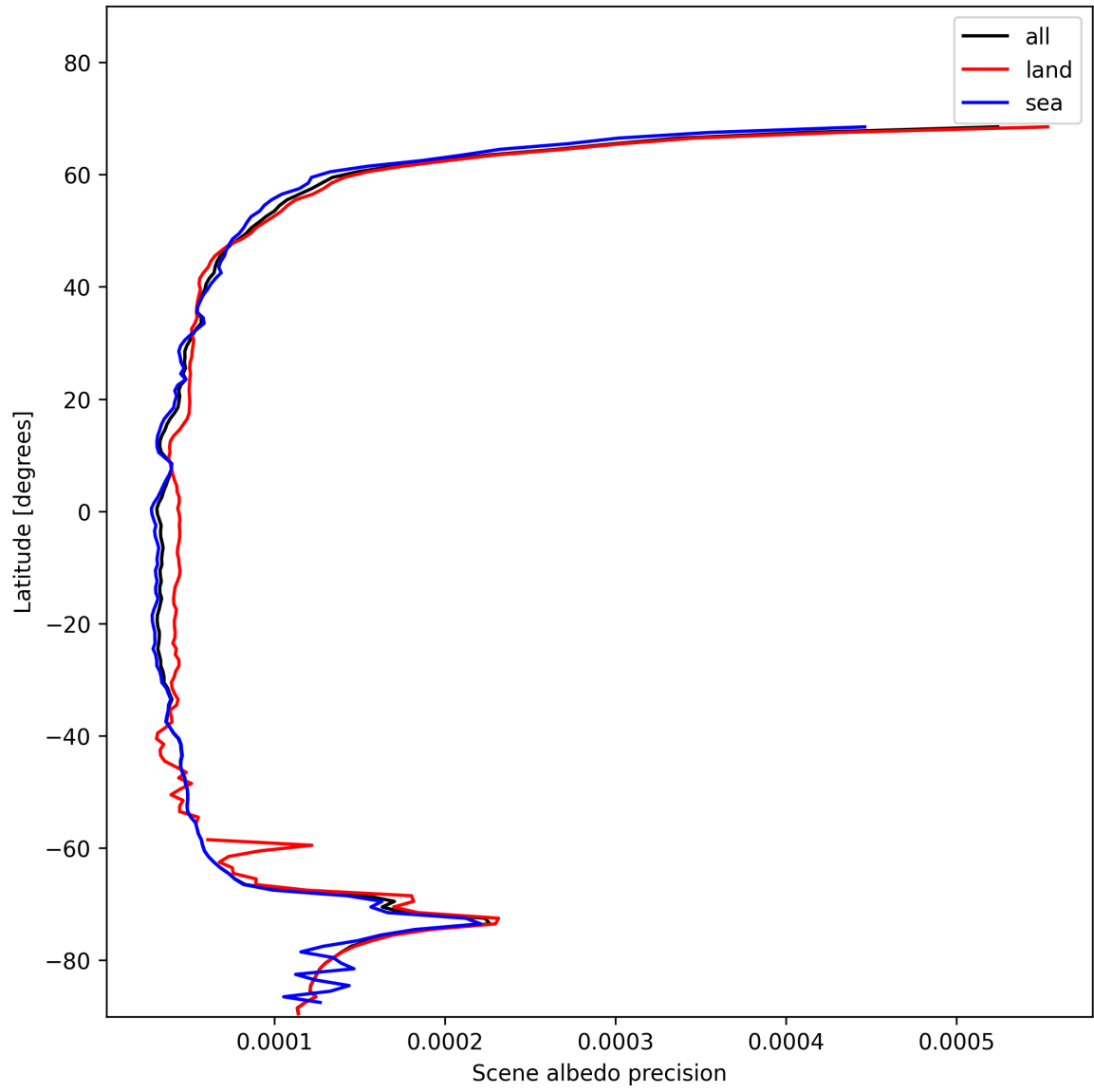
Figure 18: Zonal average of “Scene albedo precision” for 2024-11-17 to 2024-11-18.
