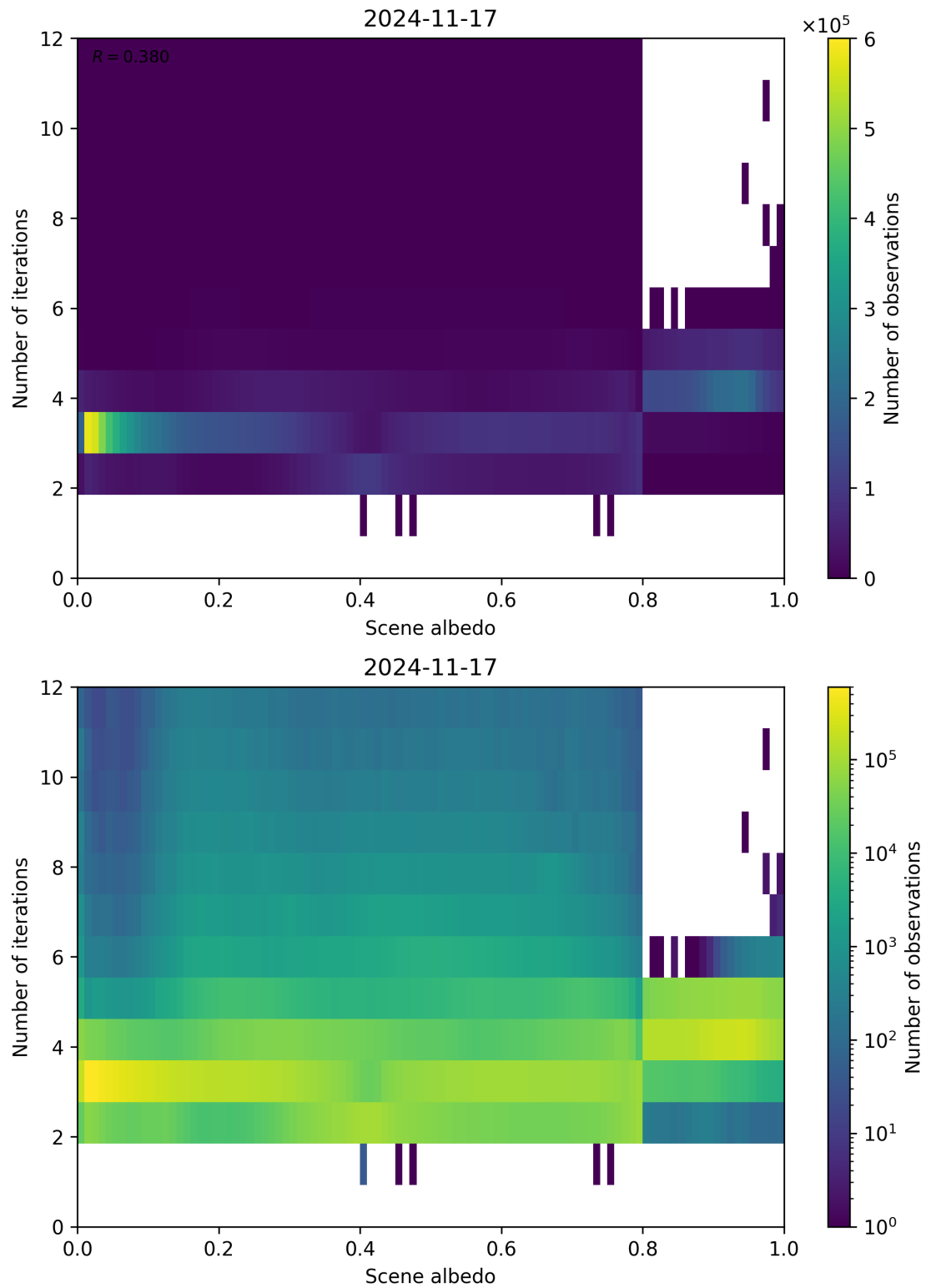
Figure 105: Scatter density plot of “Scene albedo” against “Number of iterations” for 2024-11-17 to 2024-11-18.
