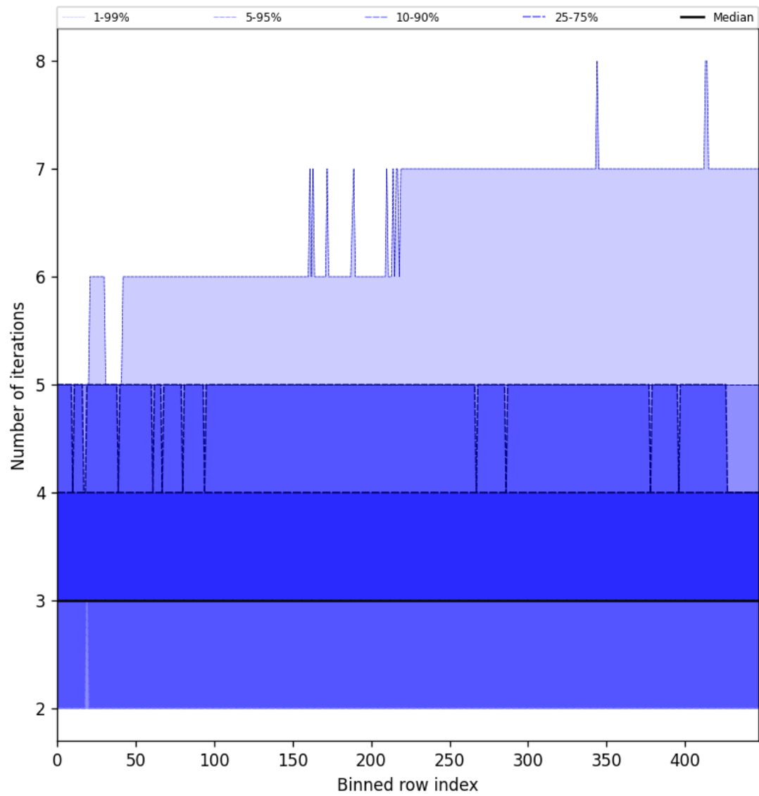
Figure 56: Along track statistics of “Number of iterations” for 2024-11-17 to 2024-11-18
