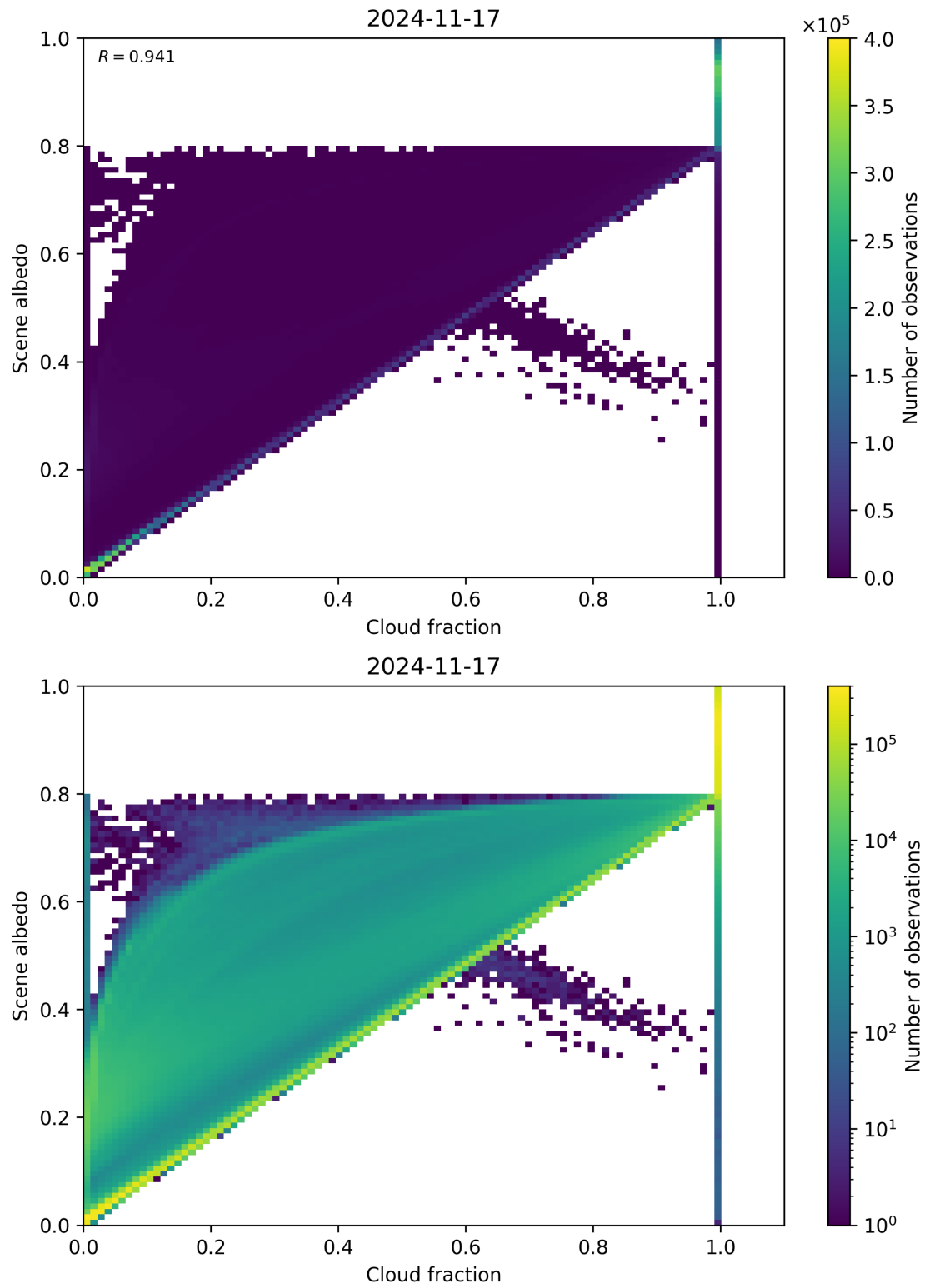
Figure 75: Scatter density plot of “Cloud fraction” against “Scene albedo” for 2024-11-17 to 2024-11-18.
