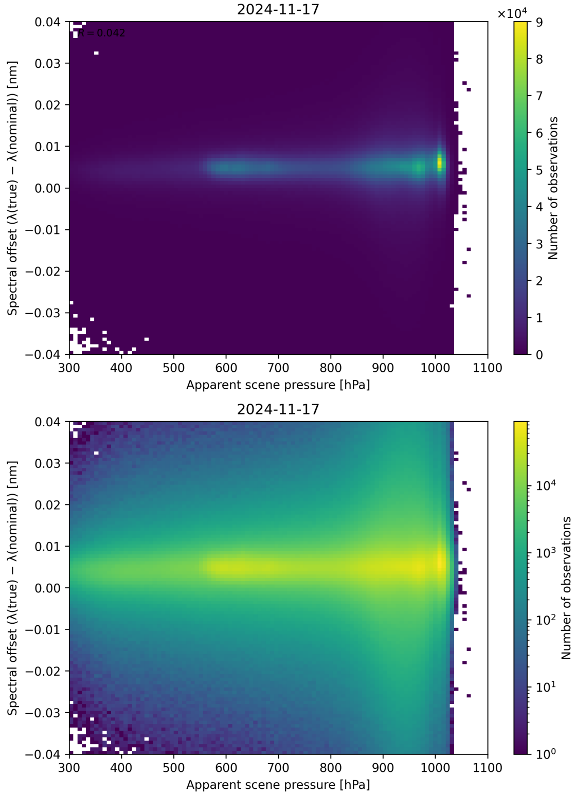
Figure 67: Scatter density plot of “Apparent scene pressure” against “Spectral offset ( \lambda_{\text{true}} - \lambda_{\text{nominal}} )” for 2024-11-17 to 2024-11-18.
