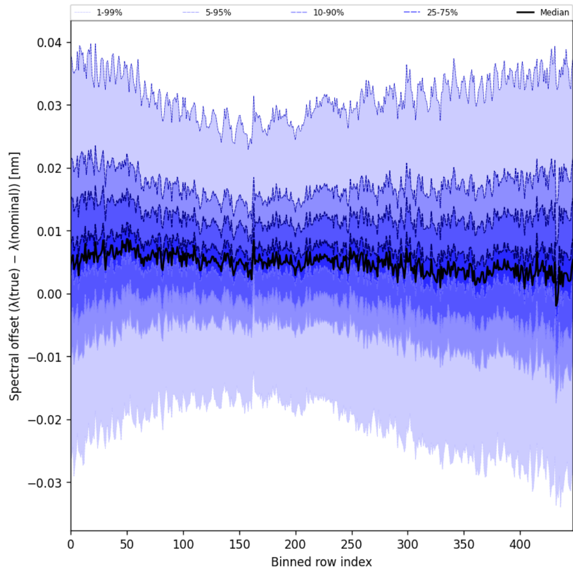
Figure 62: Along track statistics of “Spectral offset ( \lambda_{\text{true}} - \lambda_{\text{nominal}} )” for 2024-11-17 to 2024-11-18
