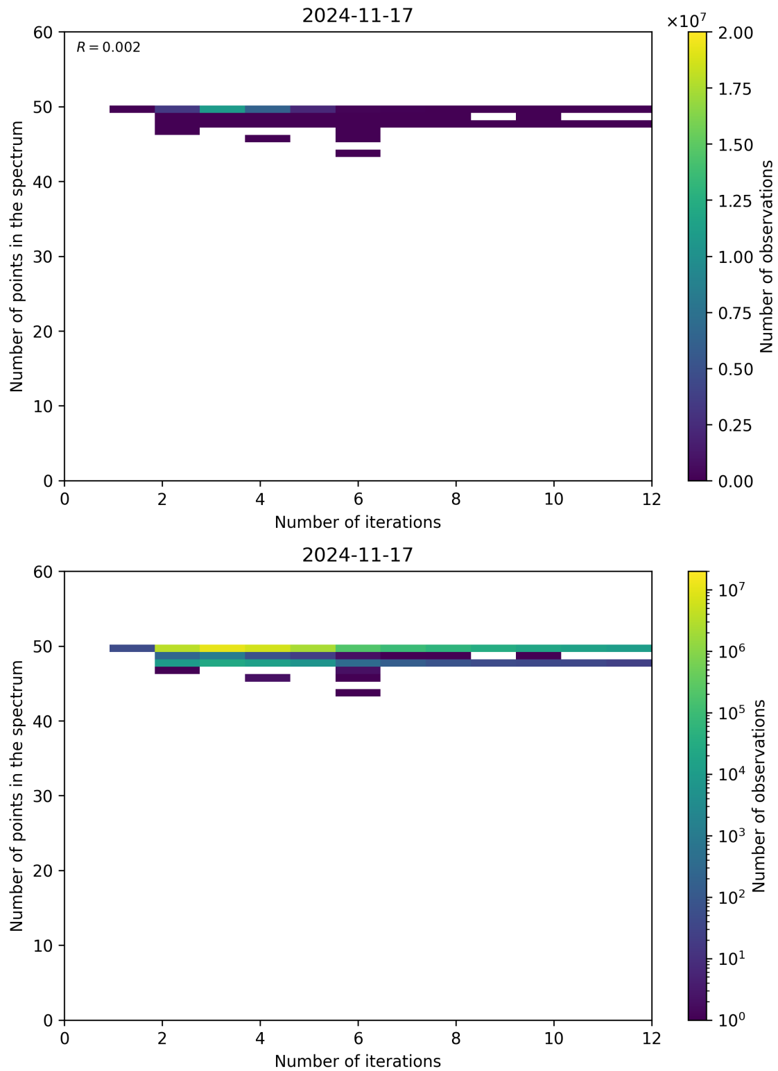
Figure 99: Scatter density plot of “Number of iterations” against “Number of points in the spectrum” for 2024-11-17 to 2024-11-18.
