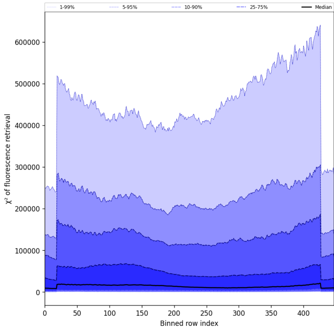
Figure 59: Along track statistics of “ \chi^2 of fluorescence retrieval” for 2024-11-17 to 2024-11-18
