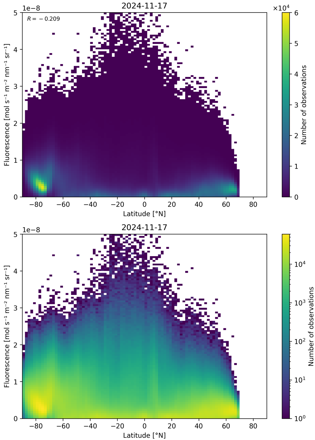
Figure 92: Scatter density plot of “Latitude” against “Fluorescence” for 2024-11-17 to 2024-11-18.
