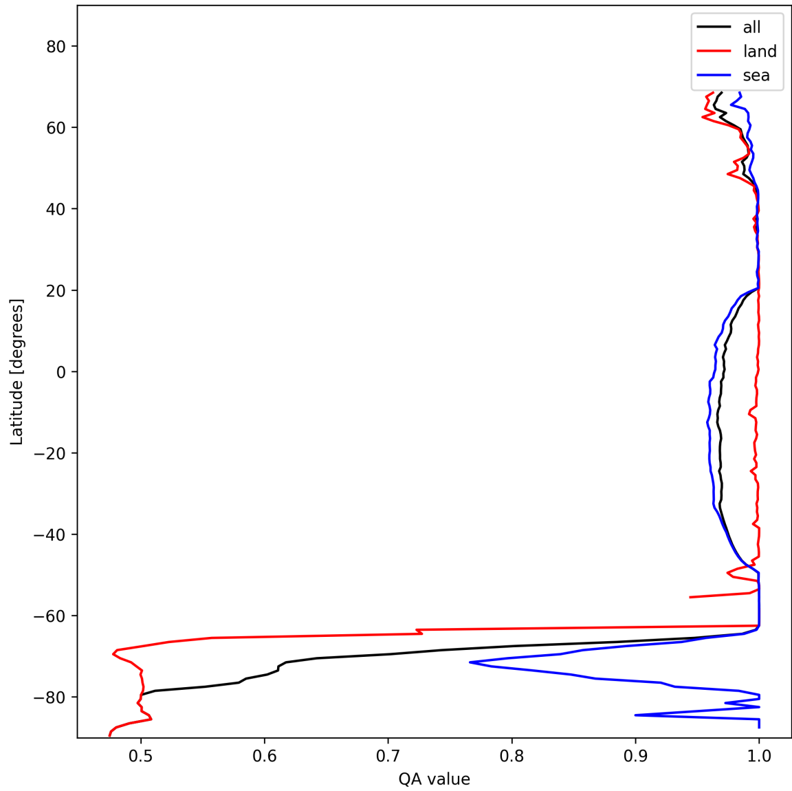
Figure 12: Zonal average of “QA value” for 2024-11-17 to 2024-11-18.
