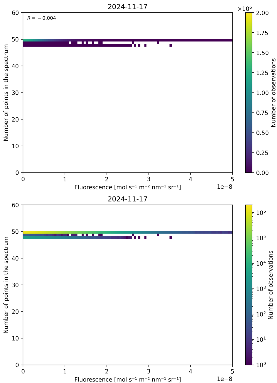
Figure 86: Scatter density plot of “Fluorescence” against “Number of points in the spectrum” for 2024-11-17 to 2024-11-18.
