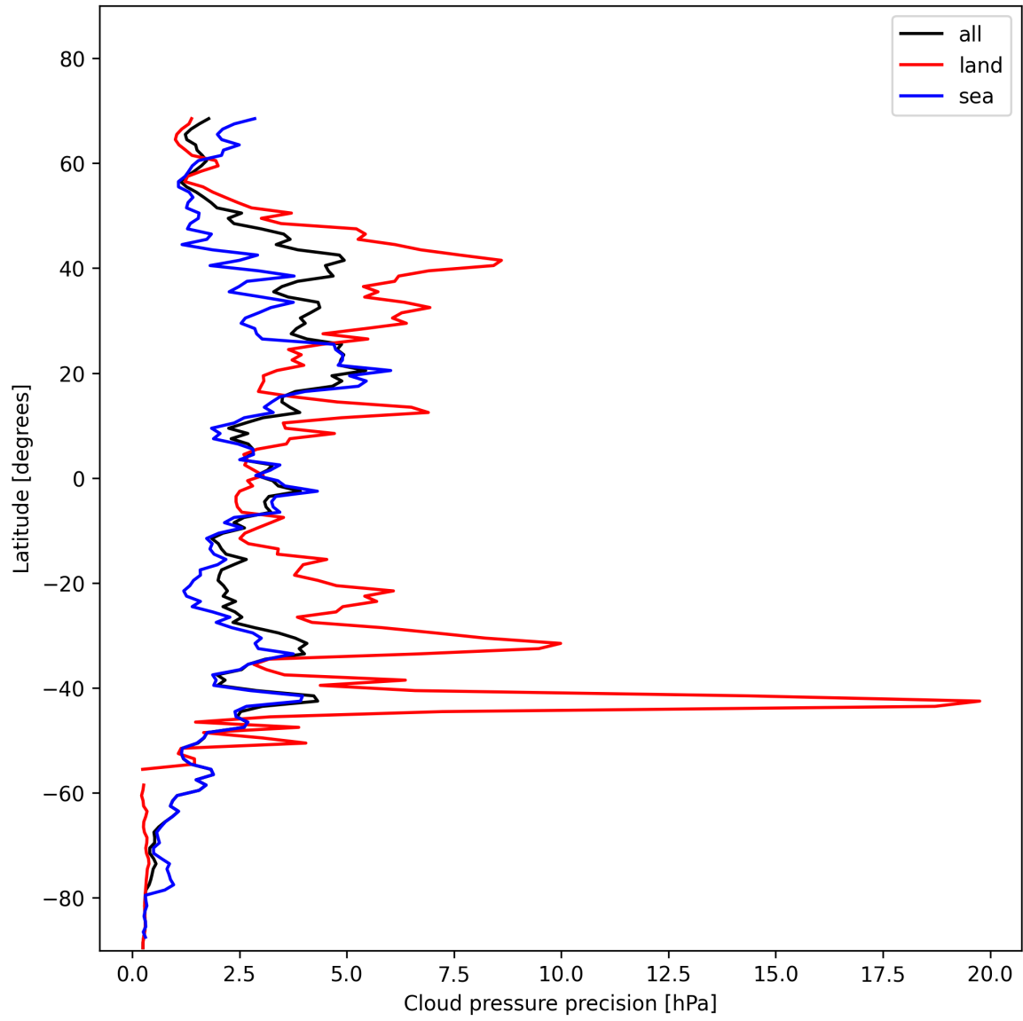
Figure 14: Zonal average of “Cloud pressure precision” for 2024-11-17 to 2024-11-18.
