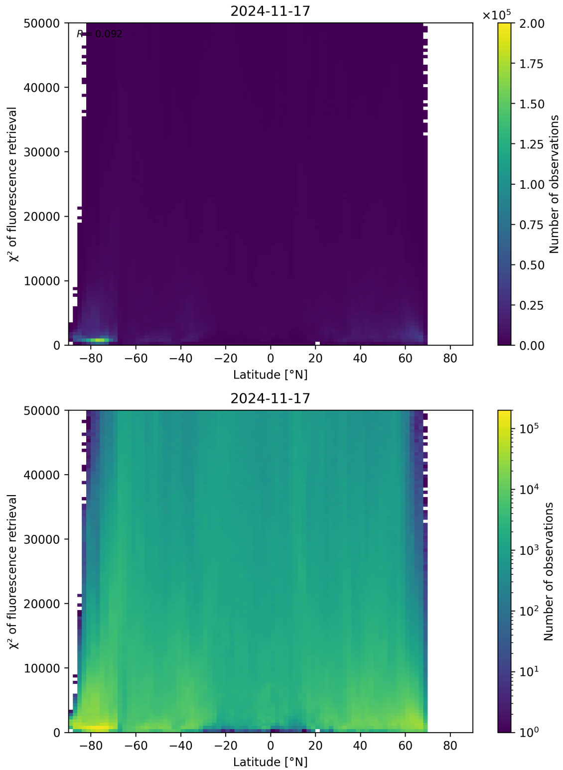
Figure 89: Scatter density plot of “Latitude” against “ \chi^2 of fluorescence retrieval” for 2024-11-17 to 2024-11-18.
