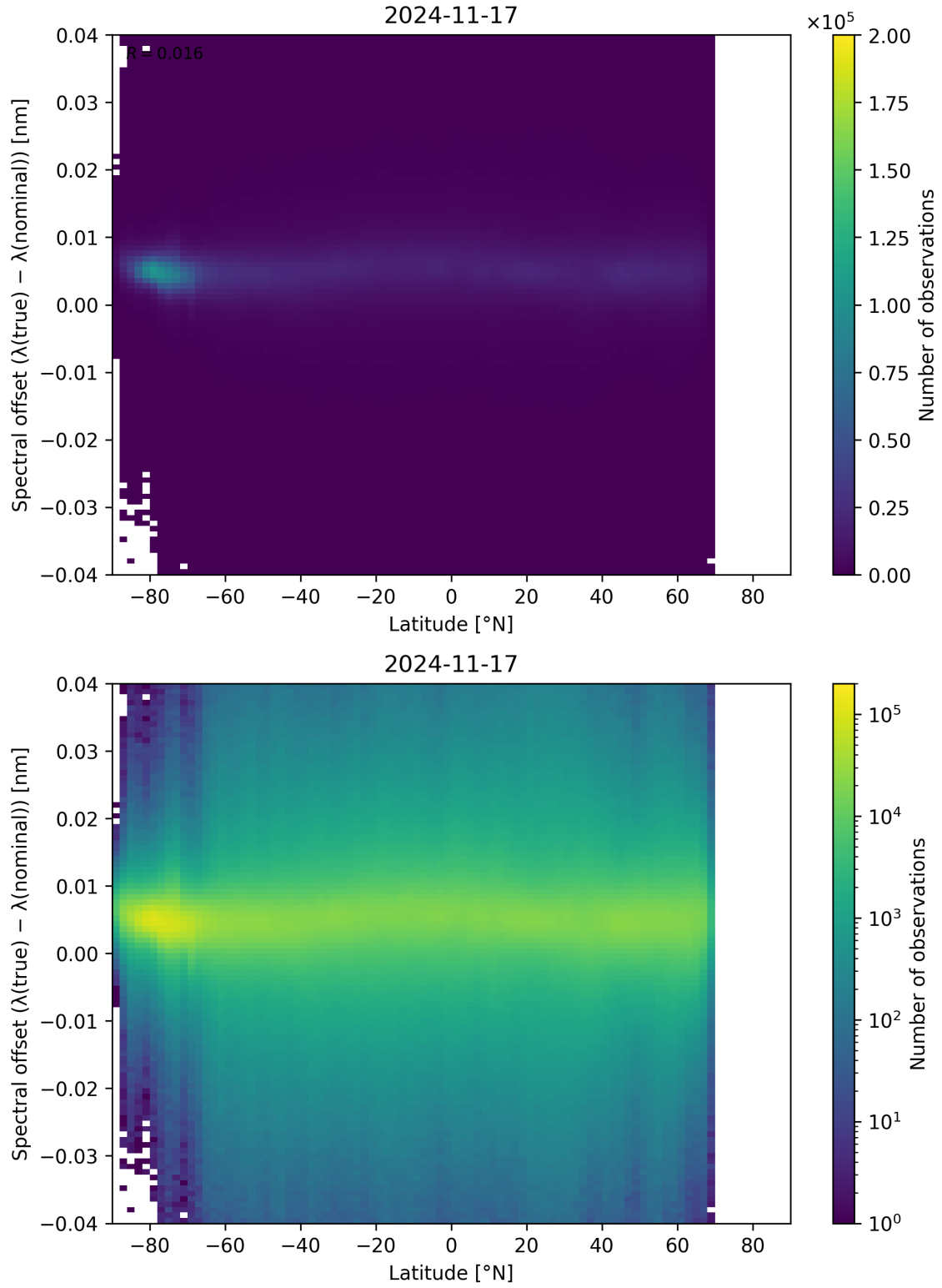
Figure 96: Scatter density plot of “Latitude” against “Spectral offset ( \lambda_{\text{true}} - \lambda_{\text{nominal}} )” for 2024-11-17 to 2024-11-18.
