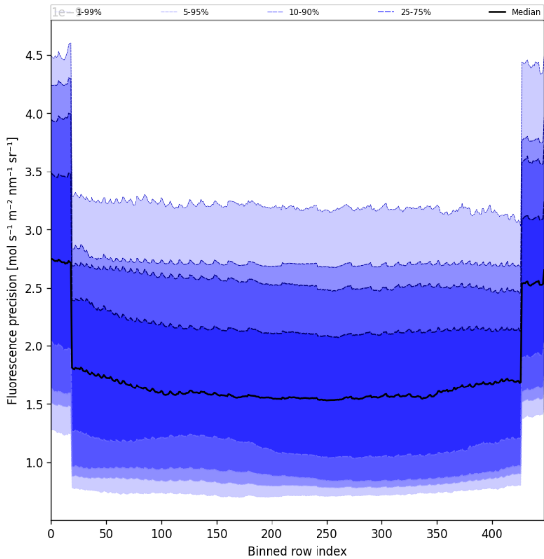
Figure 58: Along track statistics of “Fluorescence precision” for 2024-11-17 to 2024-11-18
