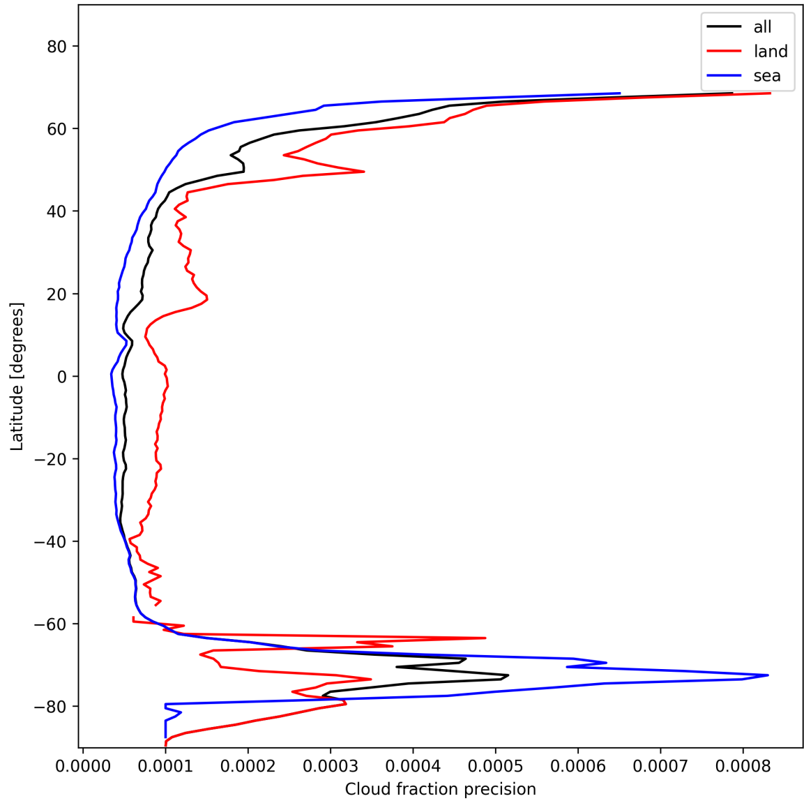
Figure 16: Zonal average of “Cloud fraction precision” for 2024-11-17 to 2024-11-18.
