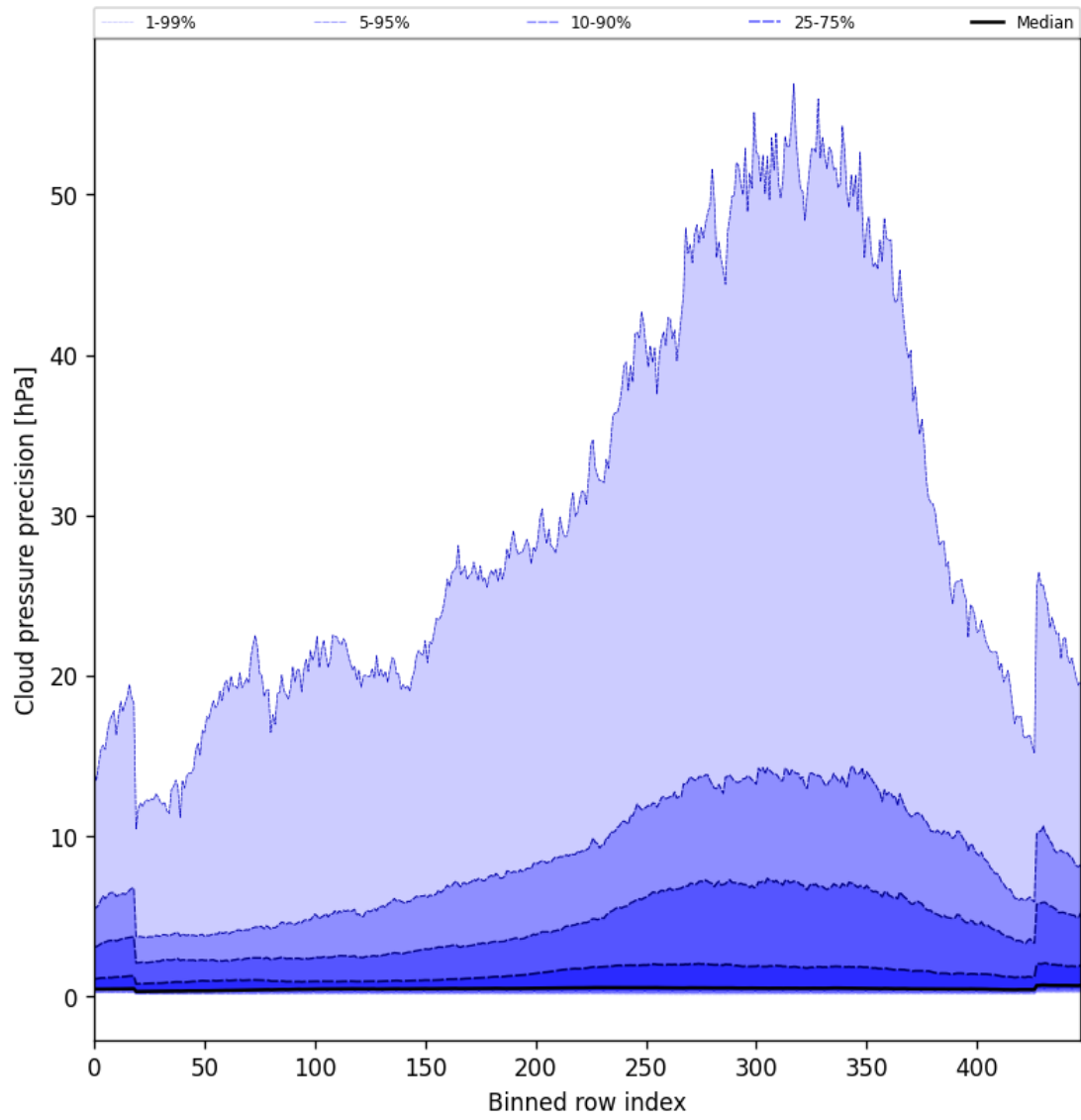
Figure 48: Along track statistics of “Cloud pressure precision” for 2024-11-17 to 2024-11-18
