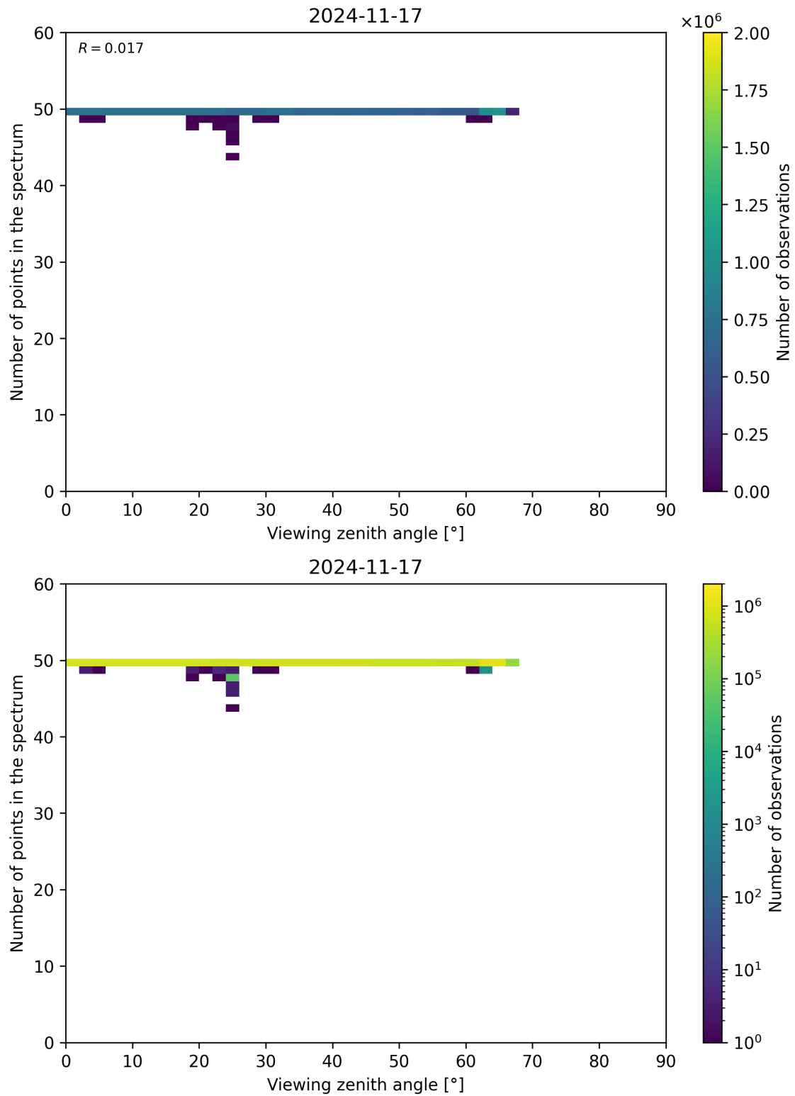
Figure 125: Scatter density plot of “Viewing zenith angle” against “Number of points in the spectrum” for 2024-11-17 to 2024-11-18.
