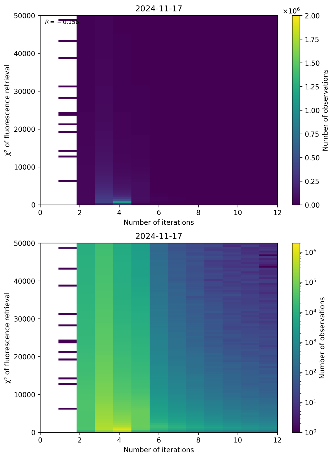
Figure 97: Scatter density plot of “Number of iterations” against “ \chi^2 of fluorescence retrieval” for 2024-11-17 to 2024-11-18.
