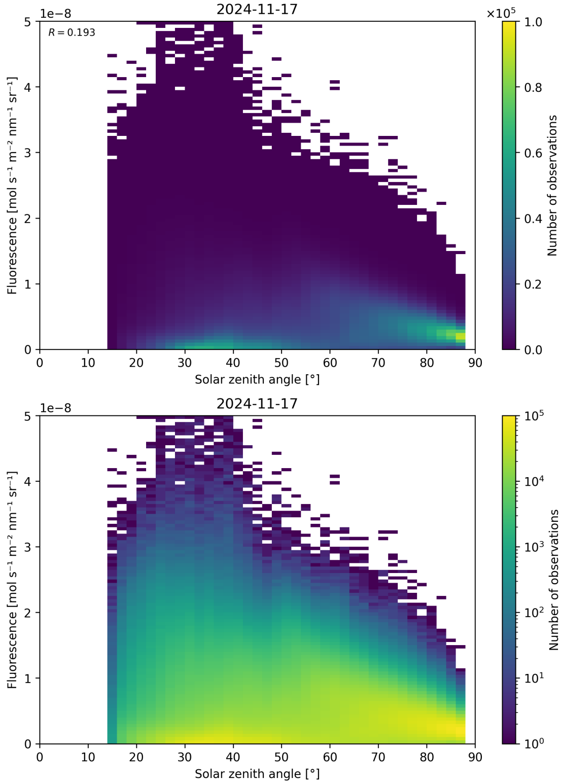
Figure 112: Scatter density plot of “Solar zenith angle” against “Fluorescence” for 2024-11-17 to 2024-11-18.
