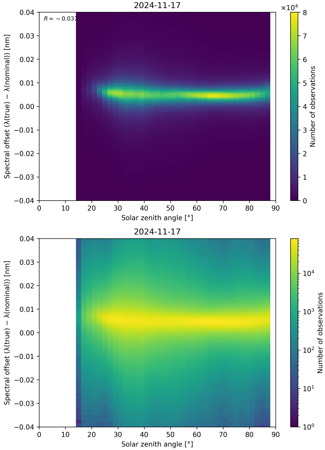
Figure 117: Scatter density plot of “Solar zenith angle” against “Spectral offset ( \lambda_{\text{true}} - \lambda_{\text{nominal}} )” for 2024-11-17 to 2024-11-18.
