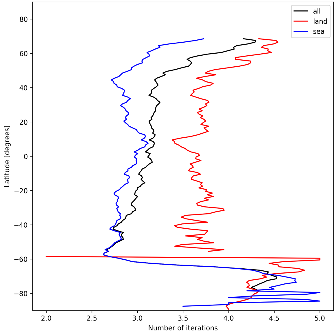
Figure 22: Zonal average of “Number of iterations” for 2024-11-17 to 2024-11-18.
