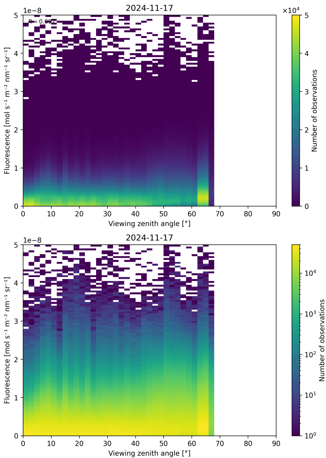
Figure 122: Scatter density plot of “Viewing zenith angle” against “Fluorescence” for 2024-11-17 to 2024-11-18.
