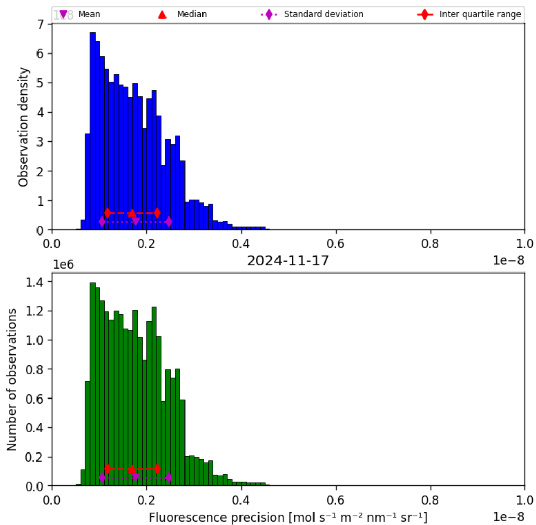
Figure 41: Histogram of “Fluorescence precision” for 2024-11-17 to 2024-11-18
