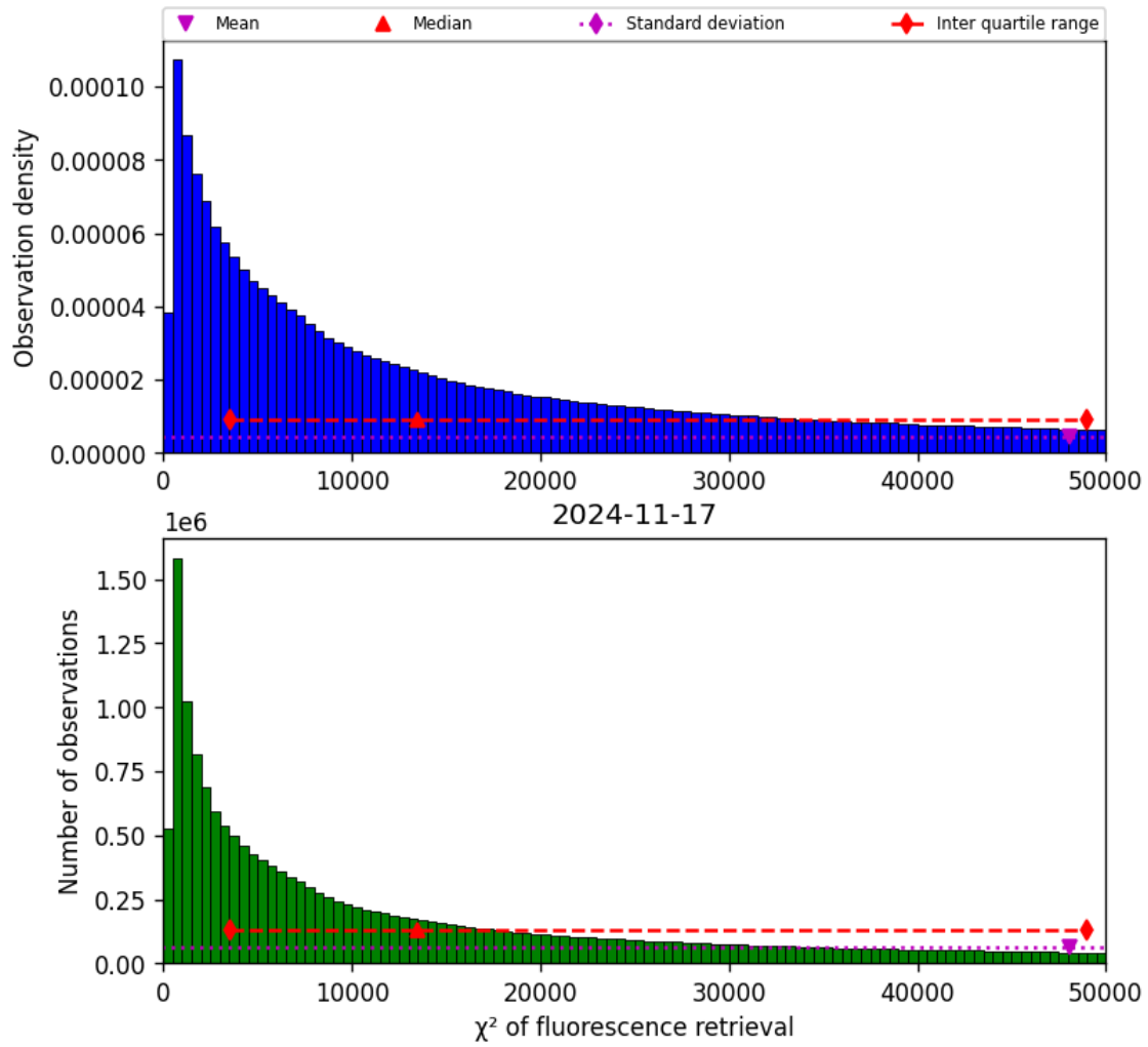
Figure 42: Histogram of “ \chi^2 of fluorescence retrieval” for 2024-11-17 to 2024-11-18
