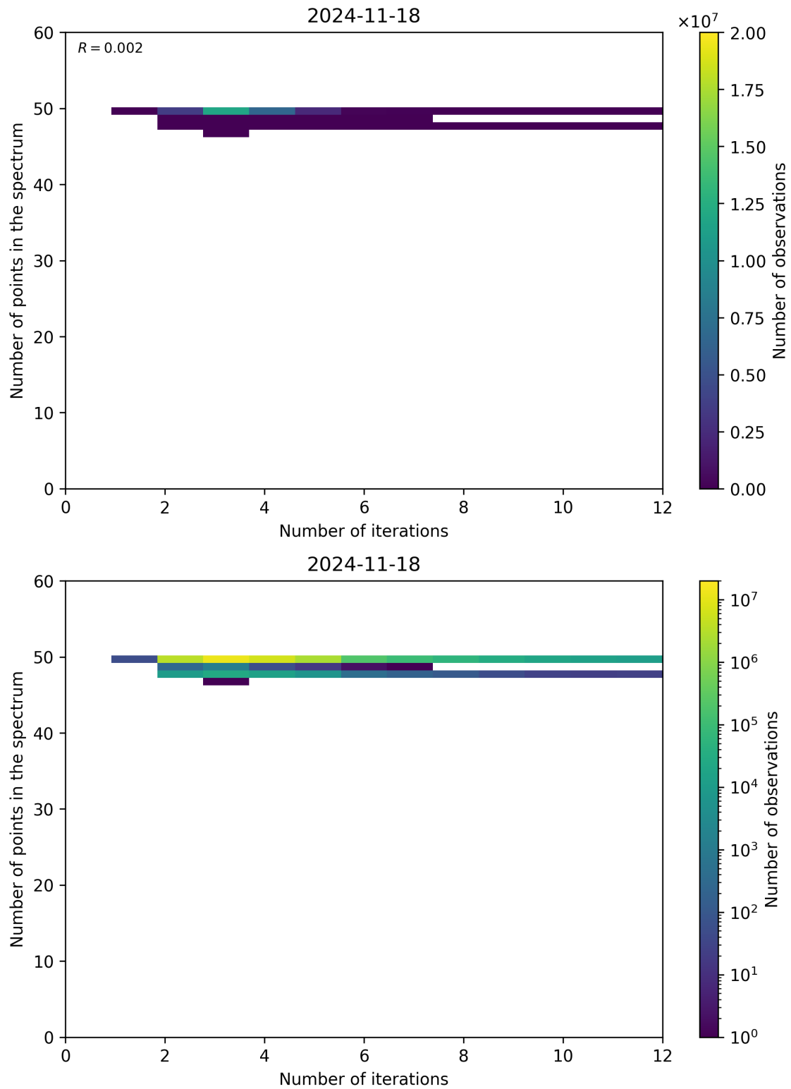
Figure 99: Scatter density plot of “Number of iterations” against “Number of points in the spectrum” for 2024-11-17 to 2024-11-19.
