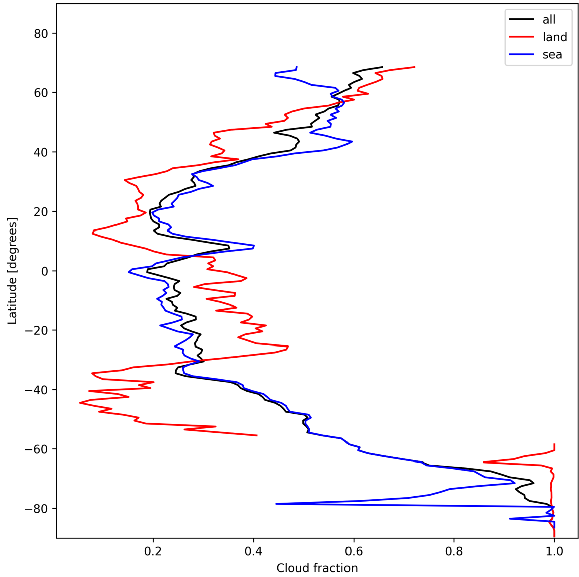
Figure 15: Zonal average of “Cloud fraction” for 2024-11-17 to 2024-11-19.
