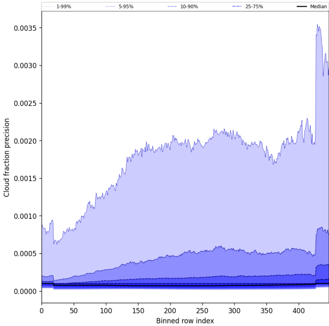
Figure 50: Along track statistics of “Cloud fraction precision” for 2024-11-17 to 2024-11-19
