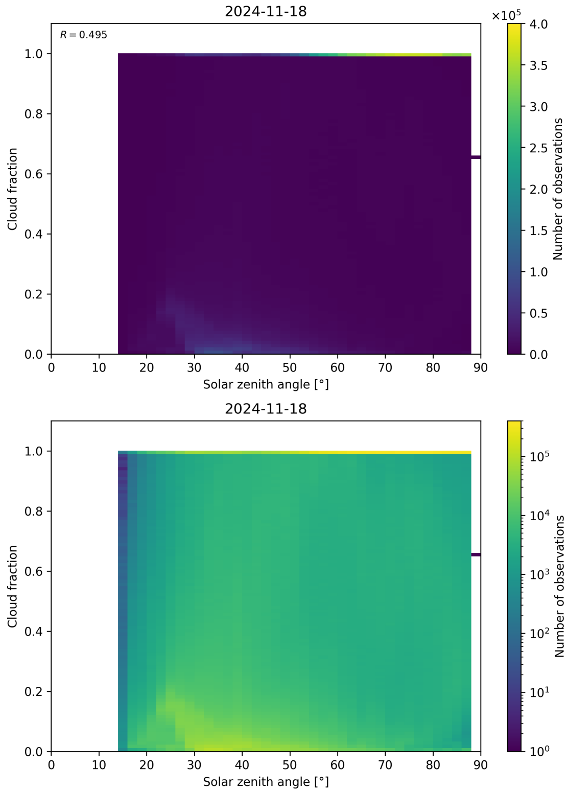
Figure 110: Scatter density plot of “Solar zenith angle” against “Cloud fraction” for 2024-11-17 to 2024-11-19.
