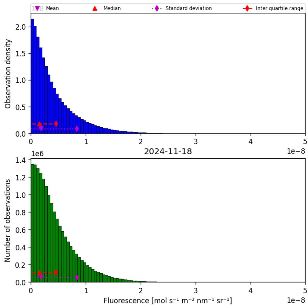
Figure 40: Histogram of “Fluorescence” for 2024-11-17 to 2024-11-19
