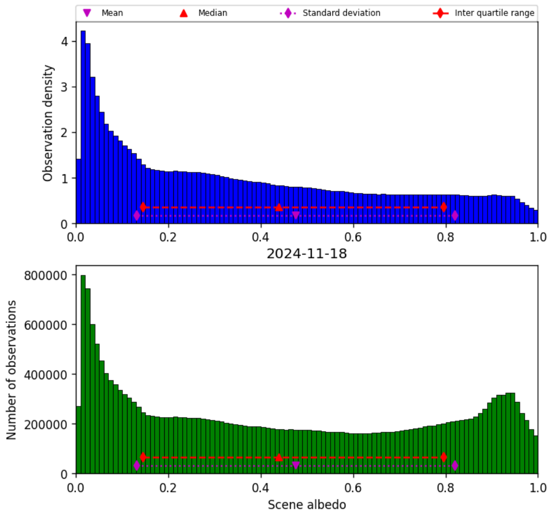
Figure 34: Histogram of “Scene albedo” for 2024-11-17 to 2024-11-19
