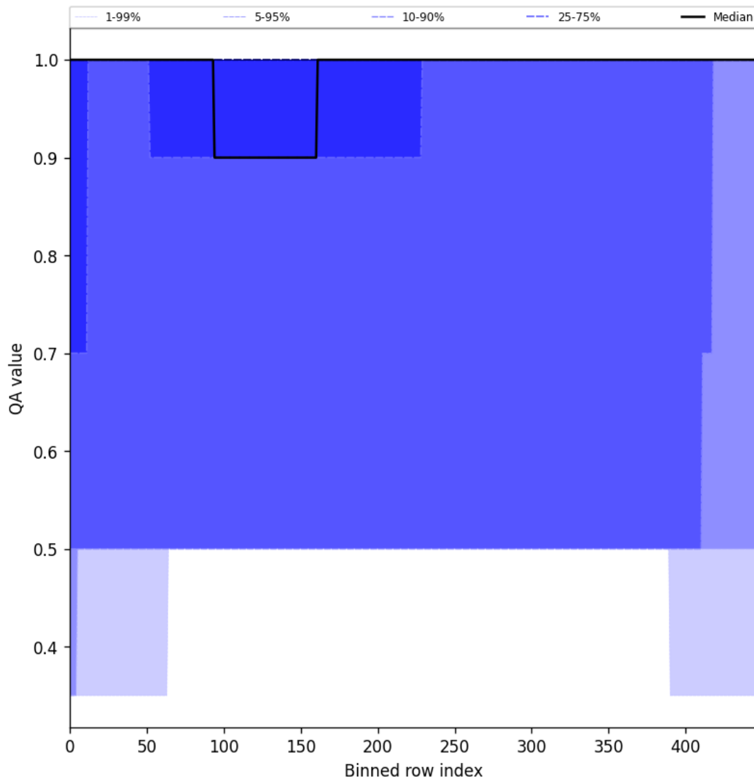
Figure 46: Along track statistics of “QA value” for 2024-11-17 to 2024-11-19
