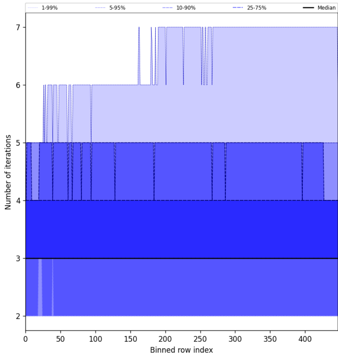
Figure 56: Along track statistics of “Number of iterations” for 2024-11-17 to 2024-11-19
