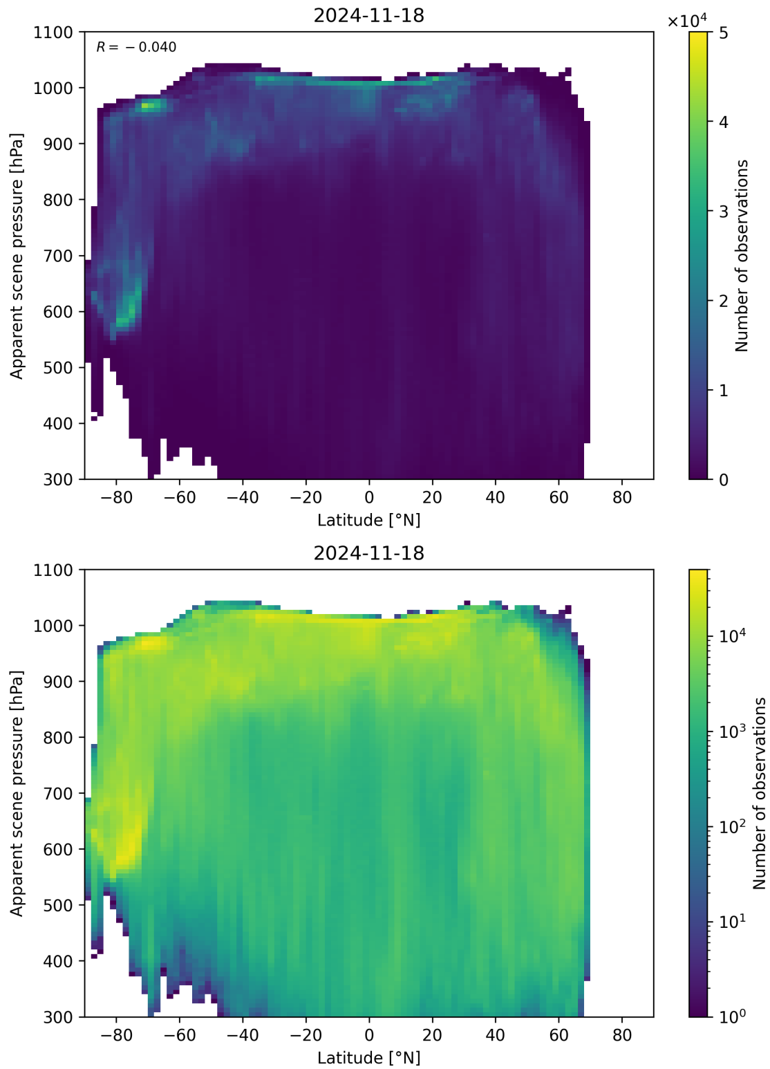
Figure 88: Scatter density plot of “Latitude” against “Apparent scene pressure” for 2024-11-17 to 2024-11-19.
