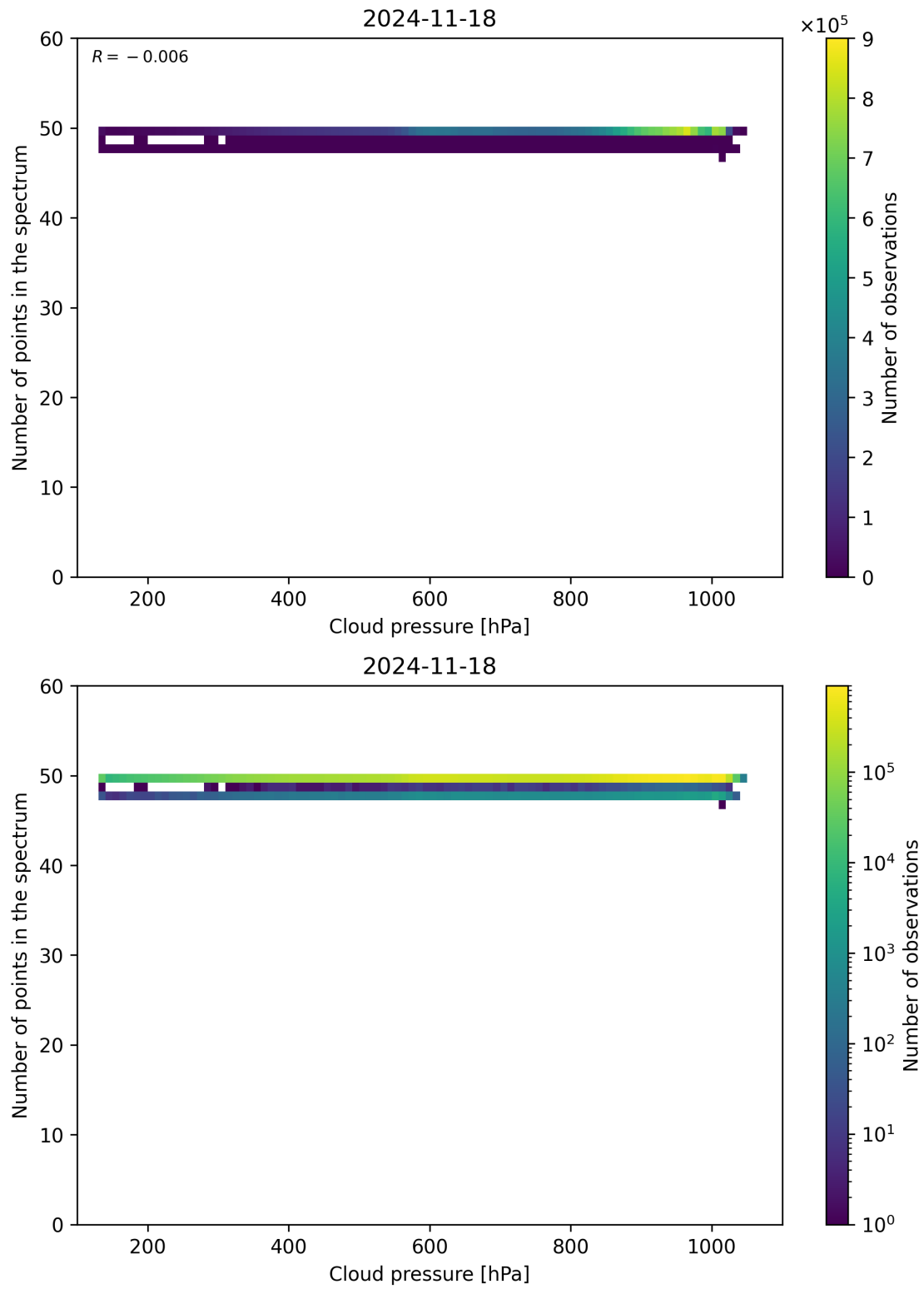
Figure 82: Scatter density plot of “Cloud pressure” against “Number of points in the spectrum” for 2024-11-17 to 2024-11-19.
