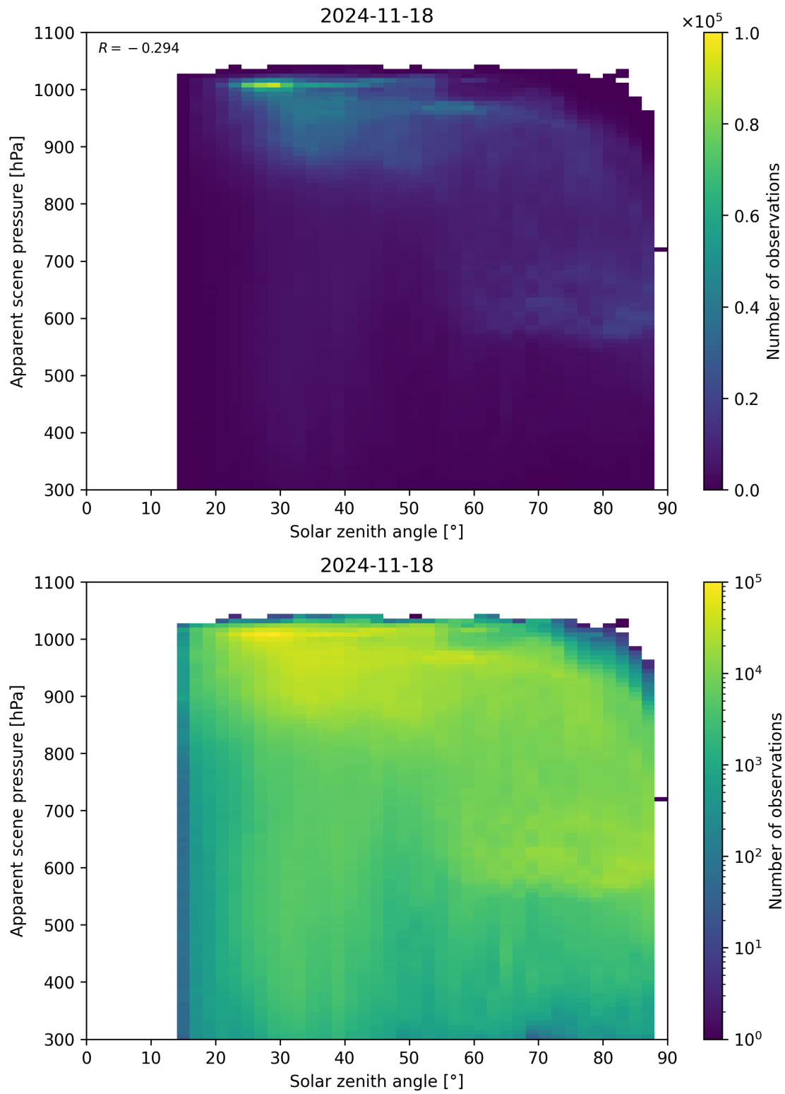
Figure 108: Scatter density plot of “Solar zenith angle” against “Apparent scene pressure” for 2024-11-17 to 2024-11-19.
