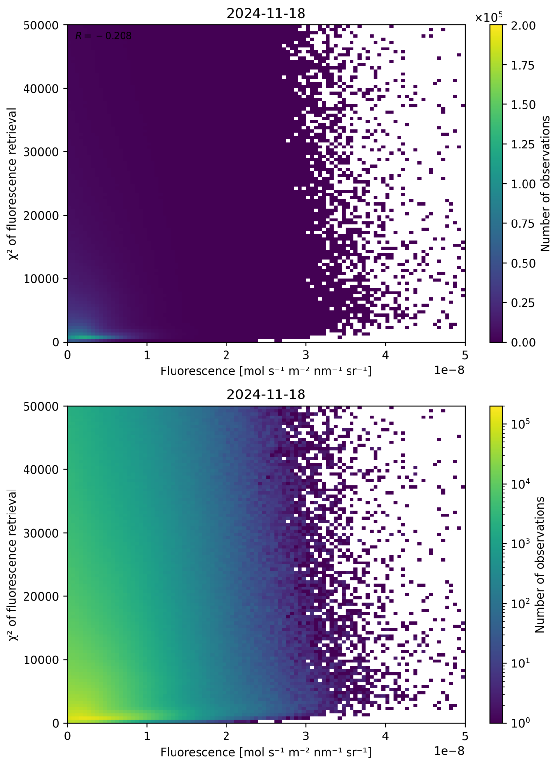
Figure 85: Scatter density plot of “Fluorescence” against “ \chi^2 of fluorescence retrieval” for 2024-11-17 to 2024-11-19.
