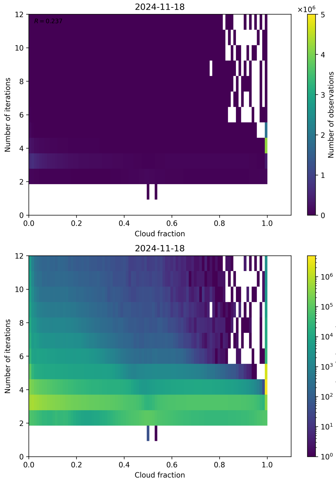
Figure 73: Scatter density plot of “Cloud fraction” against “Number of iterations” for 2024-11-17 to 2024-11-19.
