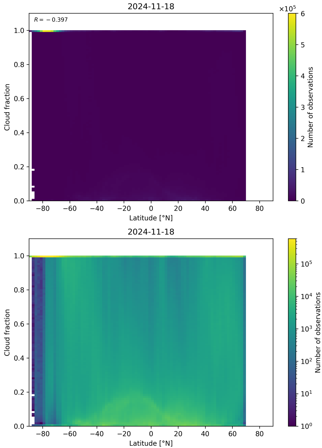
Figure 90: Scatter density plot of “Latitude” against “Cloud fraction” for 2024-11-17 to 2024-11-19.
