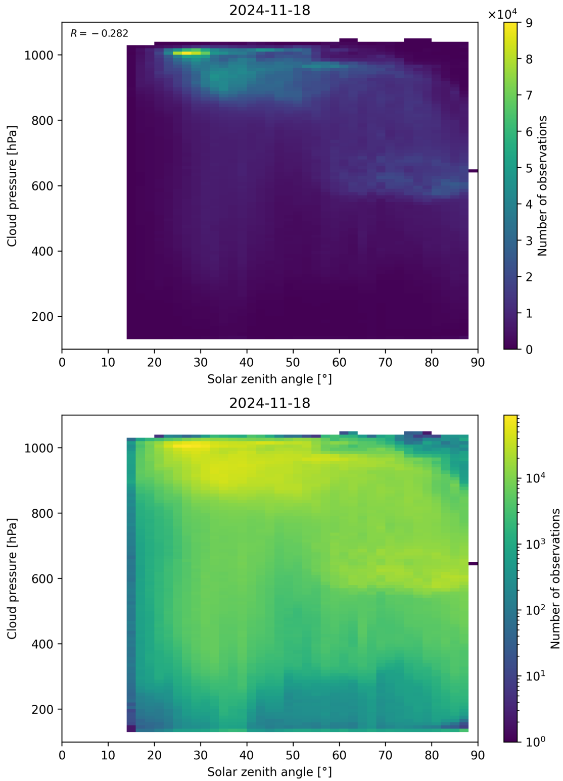
Figure 111: Scatter density plot of “Solar zenith angle” against “Cloud pressure” for 2024-11-17 to 2024-11-19.
