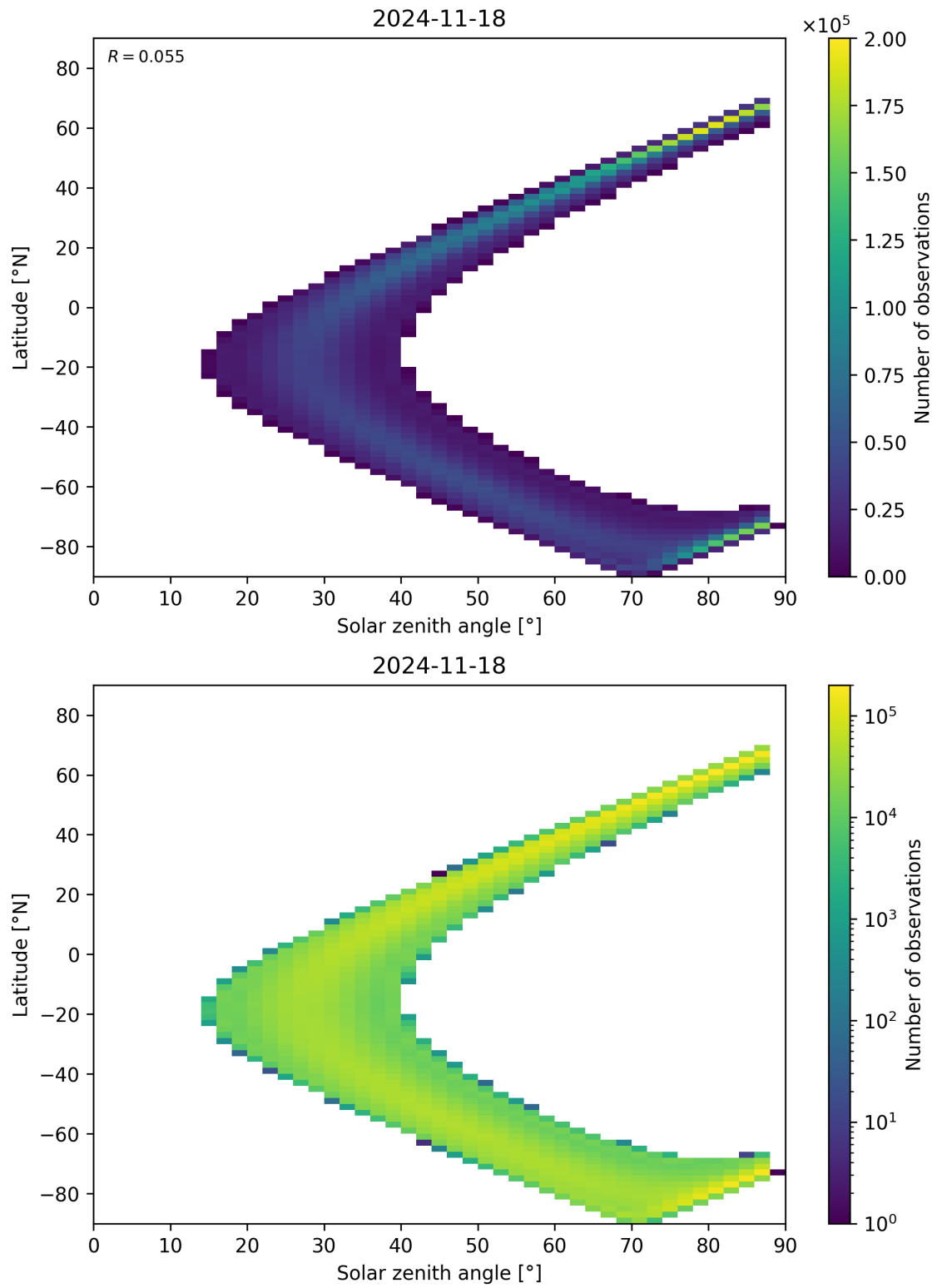
Figure 113: Scatter density plot of “Solar zenith angle” against “Latitude” for 2024-11-17 to 2024-11-19.
