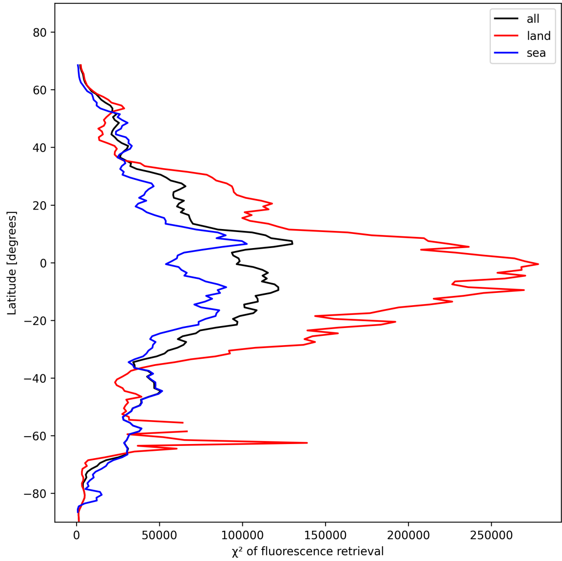
Figure 25: Zonal average of “ \chi^2 of fluorescence retrieval” for 2024-11-17 to 2024-11-19.
