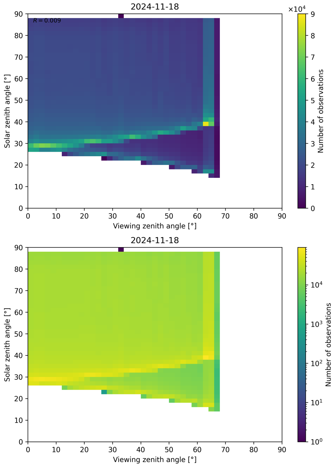
Figure 127: Scatter density plot of “Viewing zenith angle” against “Solar zenith angle” for 2024-11-17 to 2024-11-19.
