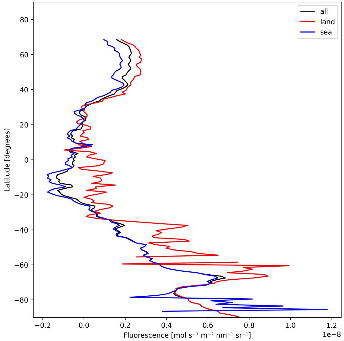
Figure 23: Zonal average of “Fluorescence” for 2024-11-17 to 2024-11-19.
