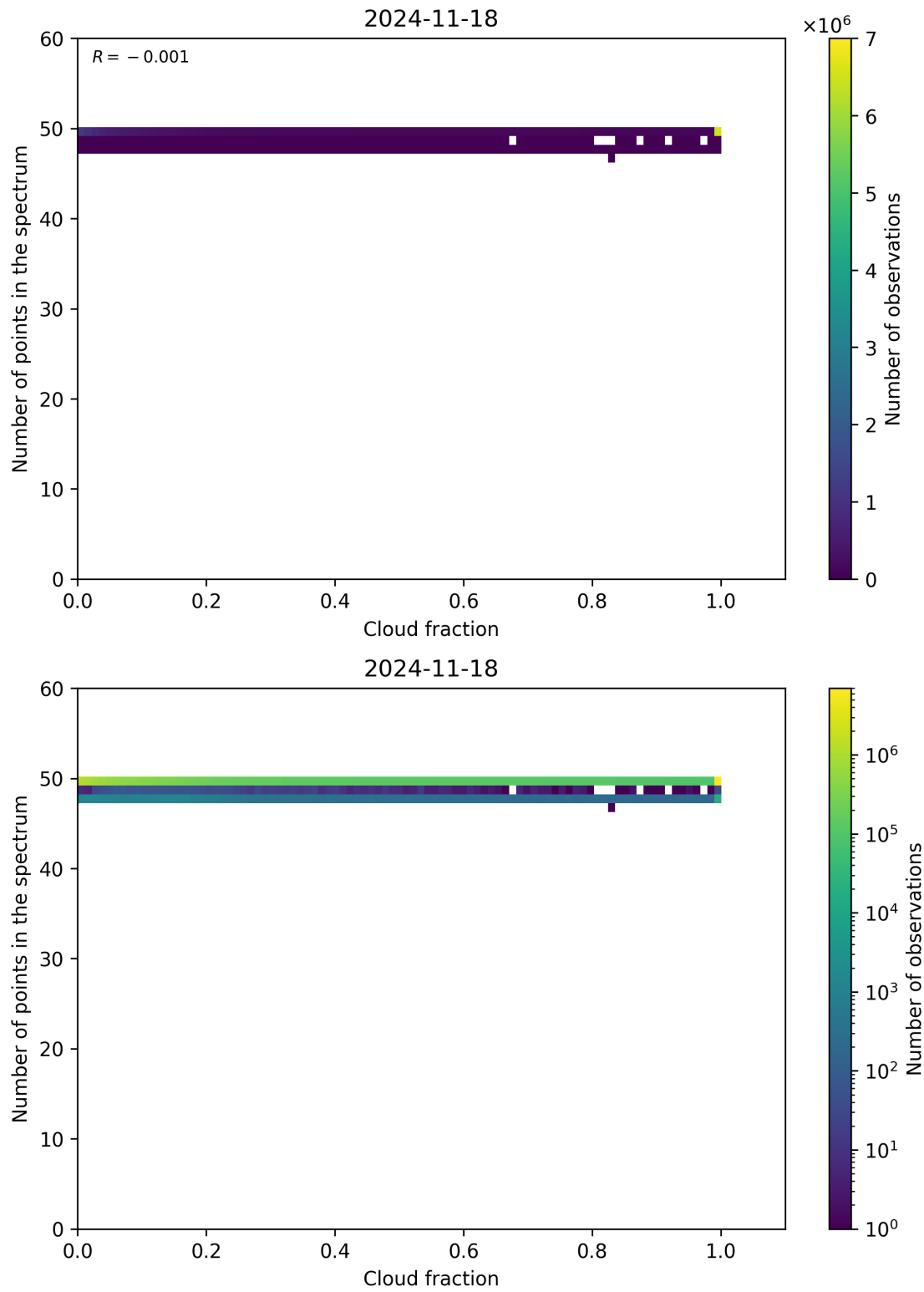
Figure 74: Scatter density plot of “Cloud fraction” against “Number of points in the spectrum” for 2024-11-17 to 2024-11-19.
