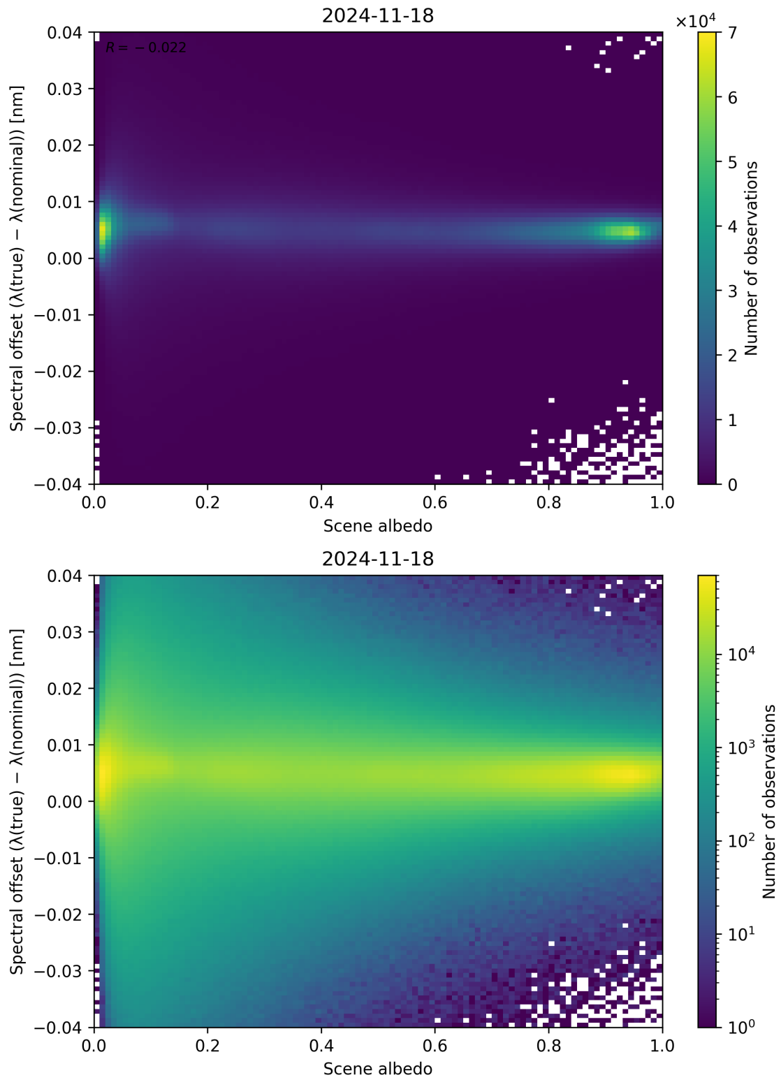
Figure 107: Scatter density plot of “Scene albedo” against “Spectral offset ( \lambda_{\text{true}} - \lambda_{\text{nominal}} )” for 2024-11-17 to 2024-11-19.
