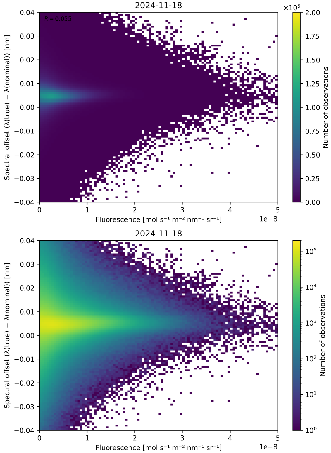
Figure 87: Scatter density plot of “Fluorescence” against “Spectral offset ( \lambda_{\text{true}} - \lambda_{\text{nominal}} )” for 2024-11-17 to 2024-11-19.
