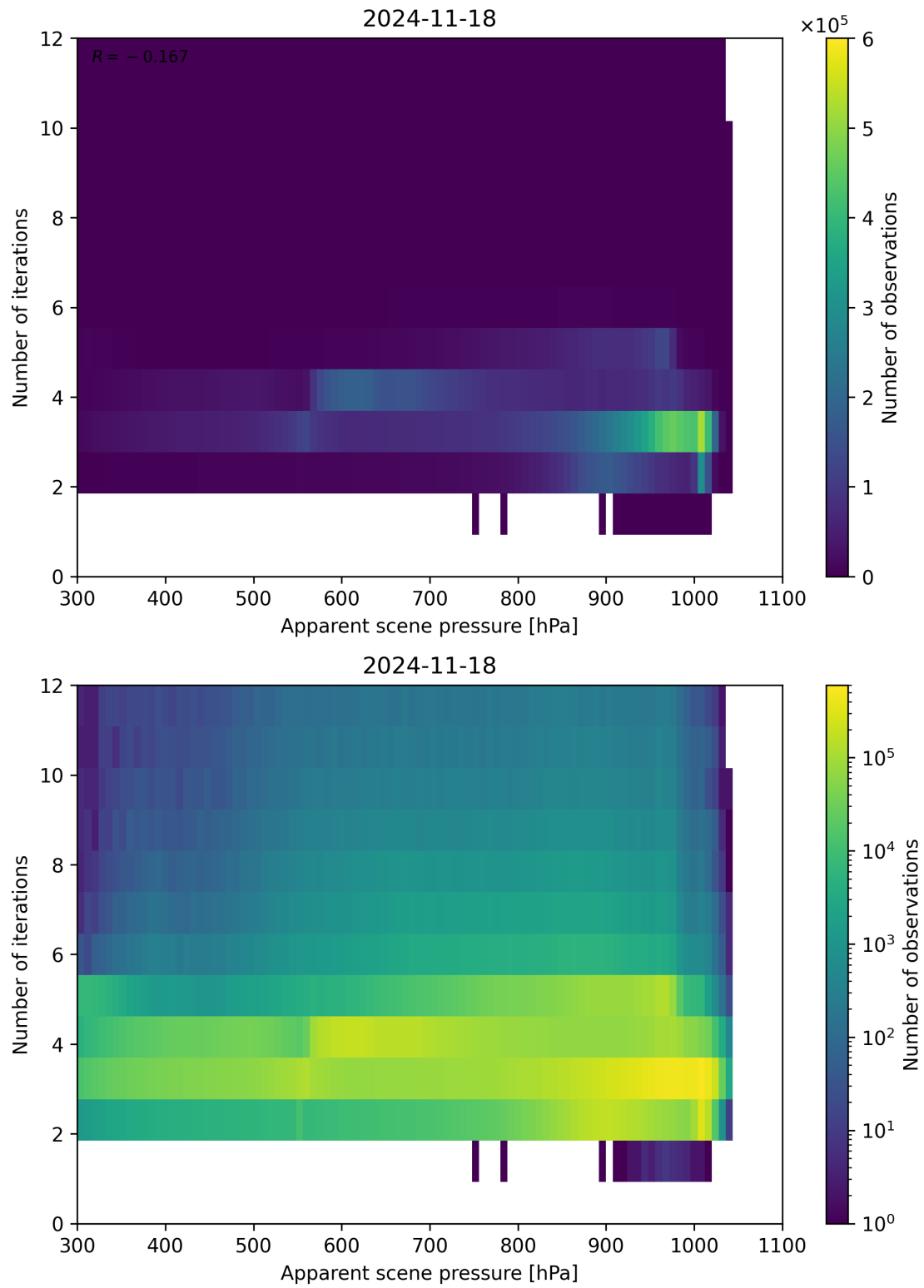
Figure 65: Scatter density plot of “Apparent scene pressure” against “Number of iterations” for 2024-11-17 to 2024-11-19.
