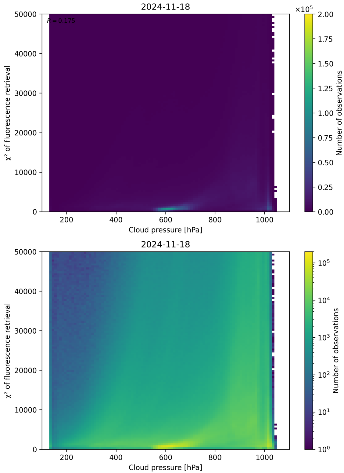
Figure 78: Scatter density plot of “Cloud pressure” against “ \chi^2 of fluorescence retrieval” for 2024-11-17 to 2024-11-19.
