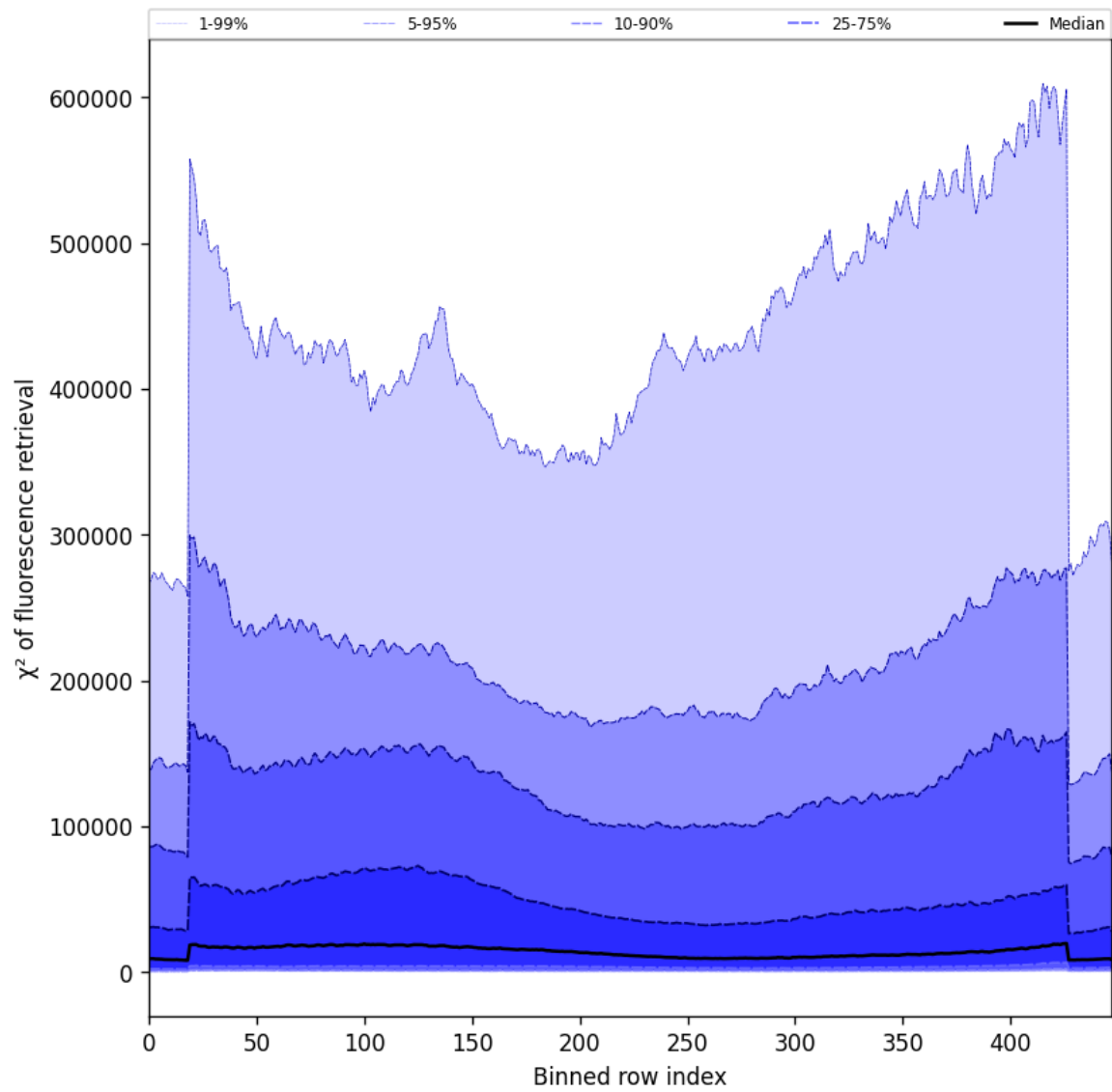
Figure 59: Along track statistics of “ \chi^2 of fluorescence retrieval” for 2024-11-17 to 2024-11-19
