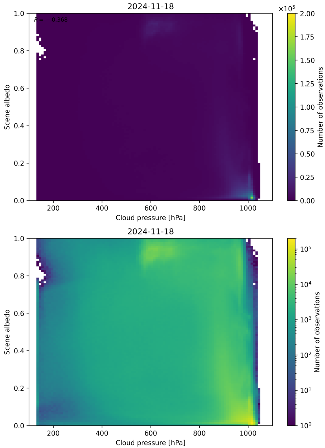
Figure 83: Scatter density plot of “Cloud pressure” against “Scene albedo” for 2024-11-17 to 2024-11-19.
