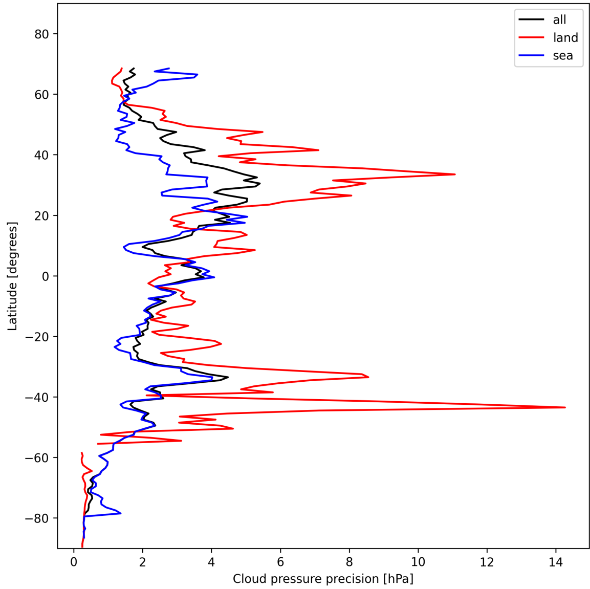
Figure 14: Zonal average of “Cloud pressure precision” for 2024-11-17 to 2024-11-19.
