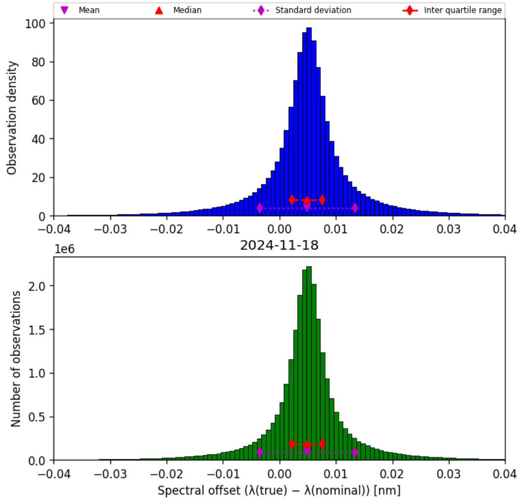
Figure 45: Histogram of “Spectral offset ( \lambda_{\text{true}} - \lambda_{\text{nominal}} )” for 2024-11-17 to 2024-11-19
