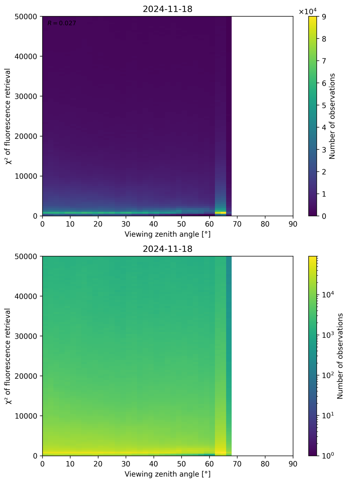
Figure 119: Scatter density plot of “Viewing zenith angle” against “ \chi^2 of fluorescence retrieval” for 2024-11-17 to 2024-11-19.
