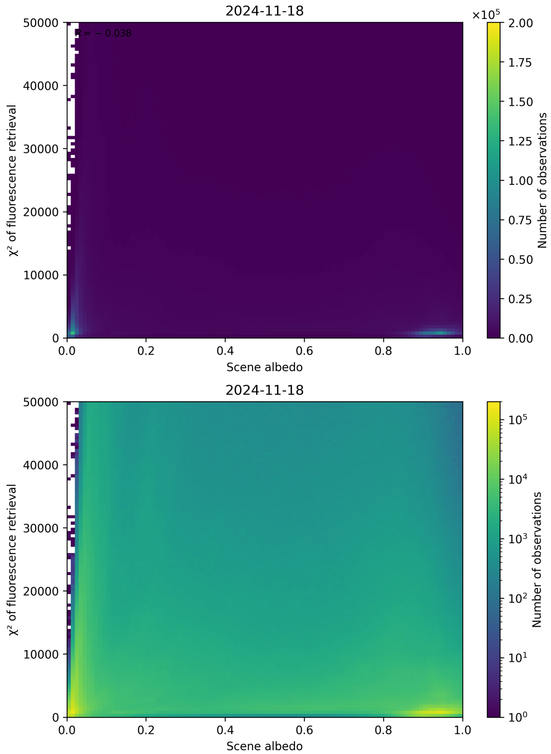
Figure 103: Scatter density plot of “Scene albedo” against “ \chi^2 of fluorescence retrieval” for 2024-11-17 to 2024-11-19.
