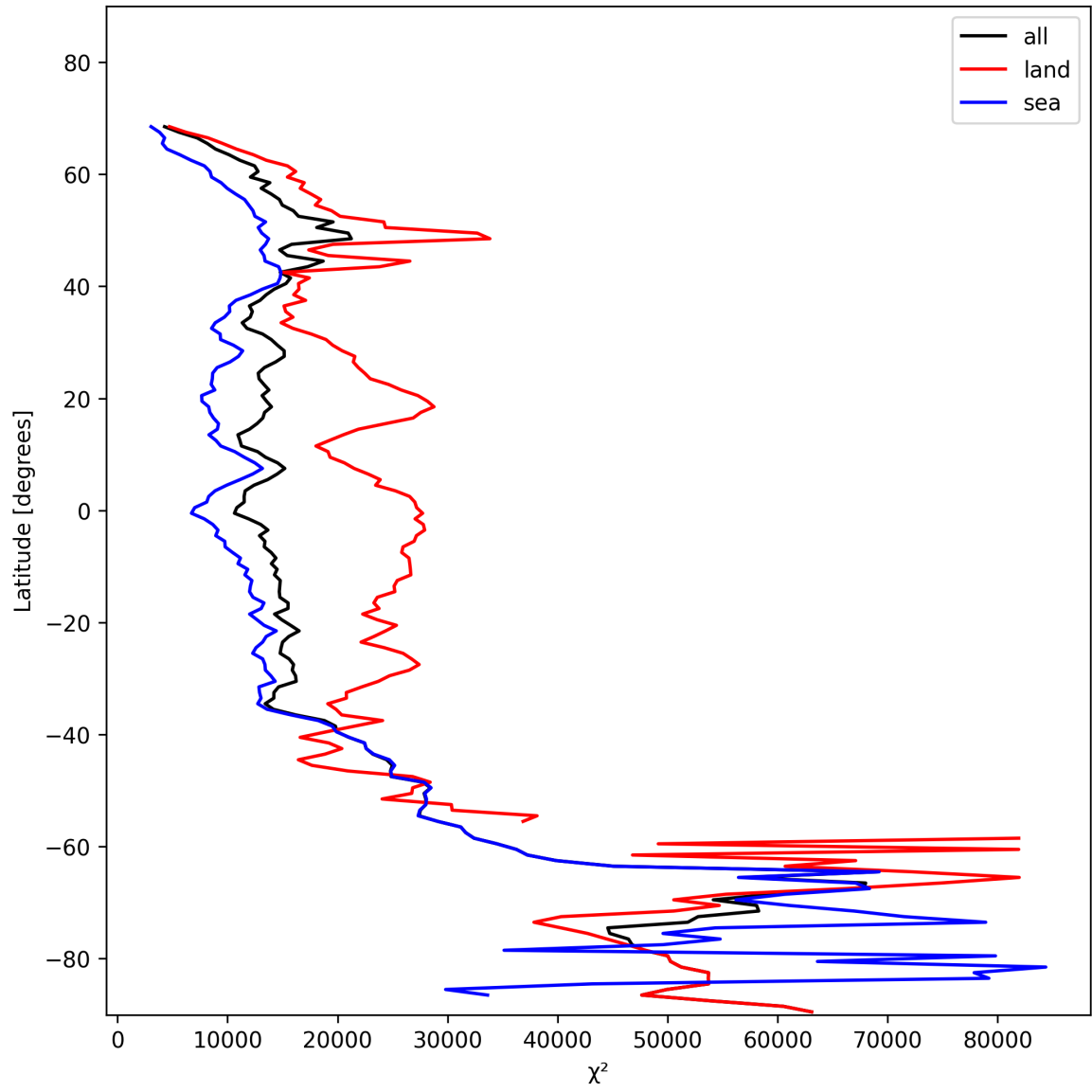
Figure 21: Zonal average of “ \chi^2 ” for 2024-11-17 to 2024-11-19.
