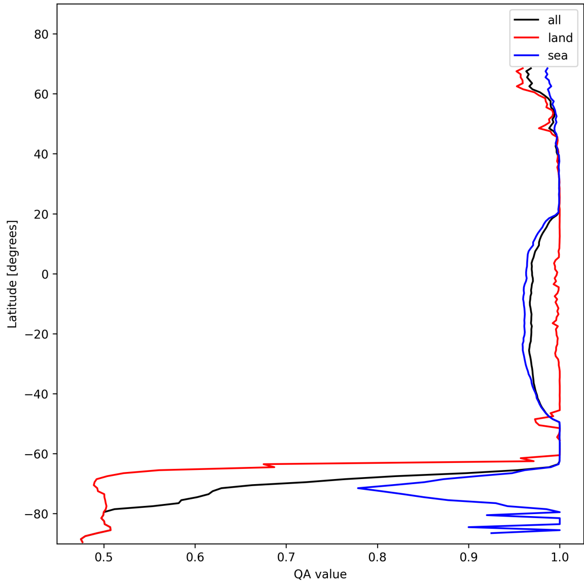
Figure 12: Zonal average of “QA value” for 2024-11-17 to 2024-11-19.
