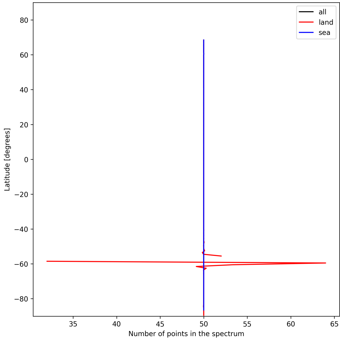
Figure 27: Zonal average of “Number of points in the spectrum” for 2024-11-17 to 2024-11-19.
