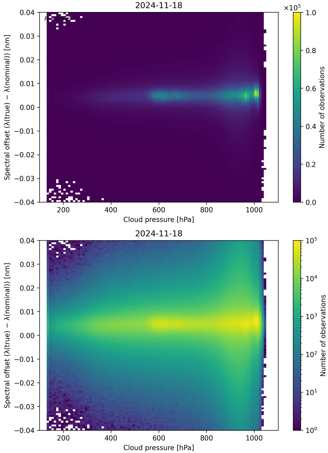
Figure 84: Scatter density plot of “Cloud pressure” against “Spectral offset ( \lambda_{\text{true}} - \lambda_{\text{nominal}} )” for 2024-11-17 to 2024-11-19.
