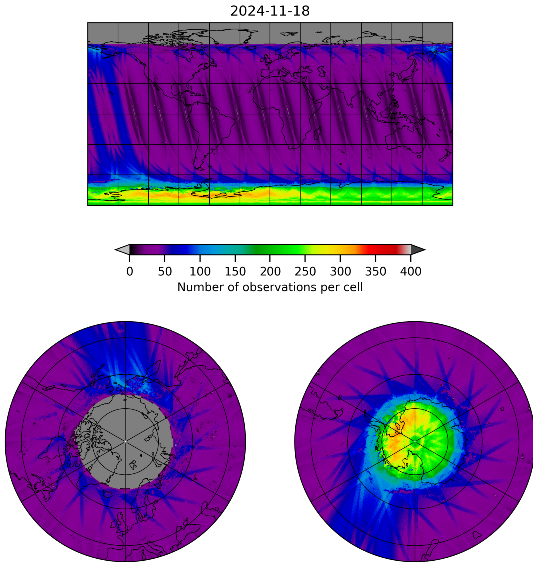
Figure 11: Map of the number of observations for 2024-11-17 to 2024-11-19
