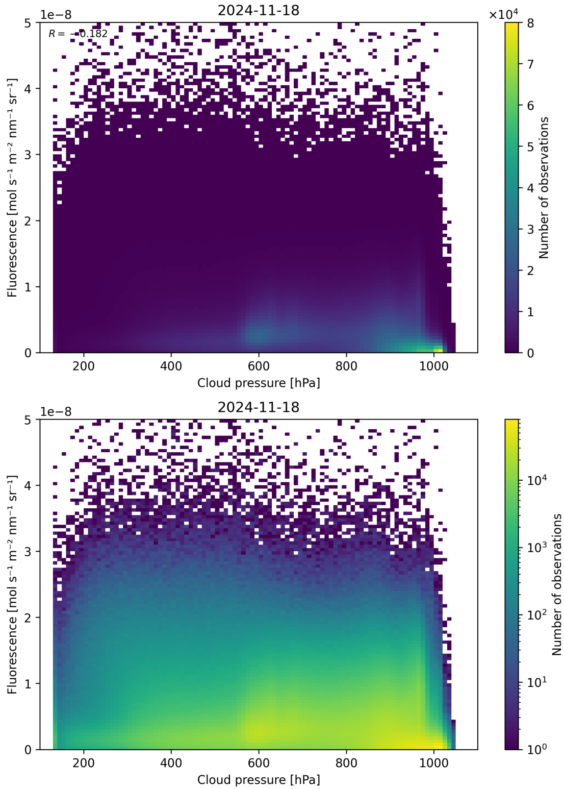
Figure 80: Scatter density plot of “Cloud pressure” against “Fluorescence” for 2024-11-17 to 2024-11-19.
