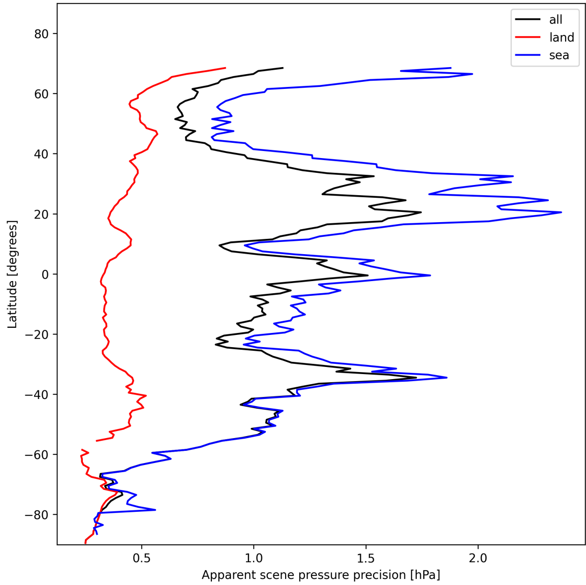
Figure 20: Zonal average of “Apparent scene pressure precision” for 2024-11-17 to 2024-11-19.
