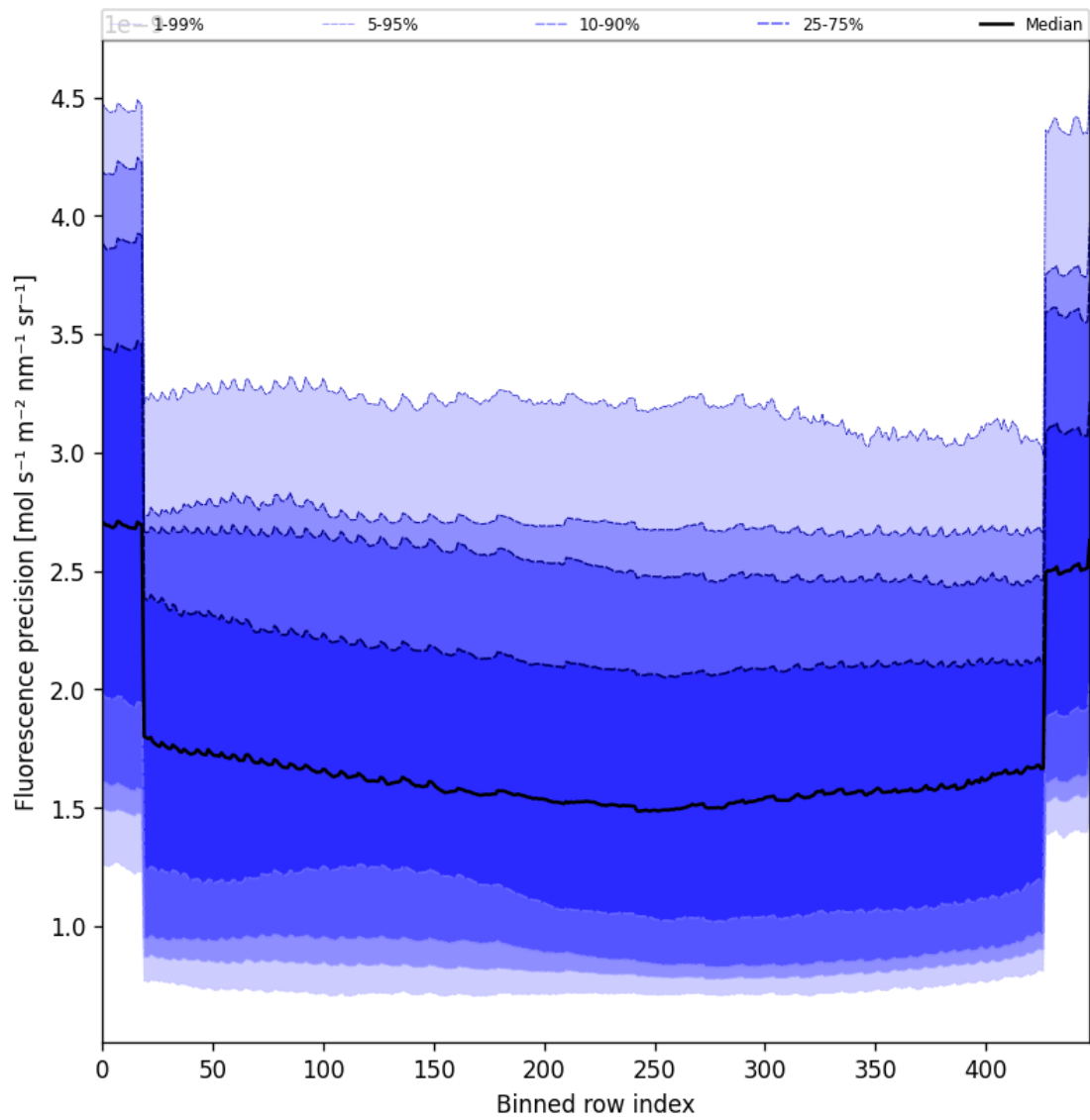
Figure 58: Along track statistics of “Fluorescence precision” for 2024-11-17 to 2024-11-19
