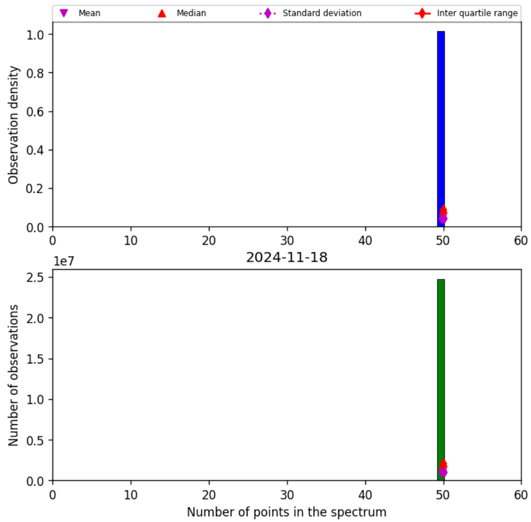
Figure 44: Histogram of “Number of points in the spectrum” for 2024-11-17 to 2024-11-19
