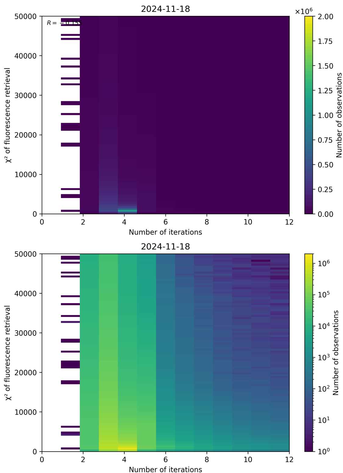
Figure 97: Scatter density plot of “Number of iterations” against “ \chi^2 of fluorescence retrieval” for 2024-11-17 to 2024-11-19.
