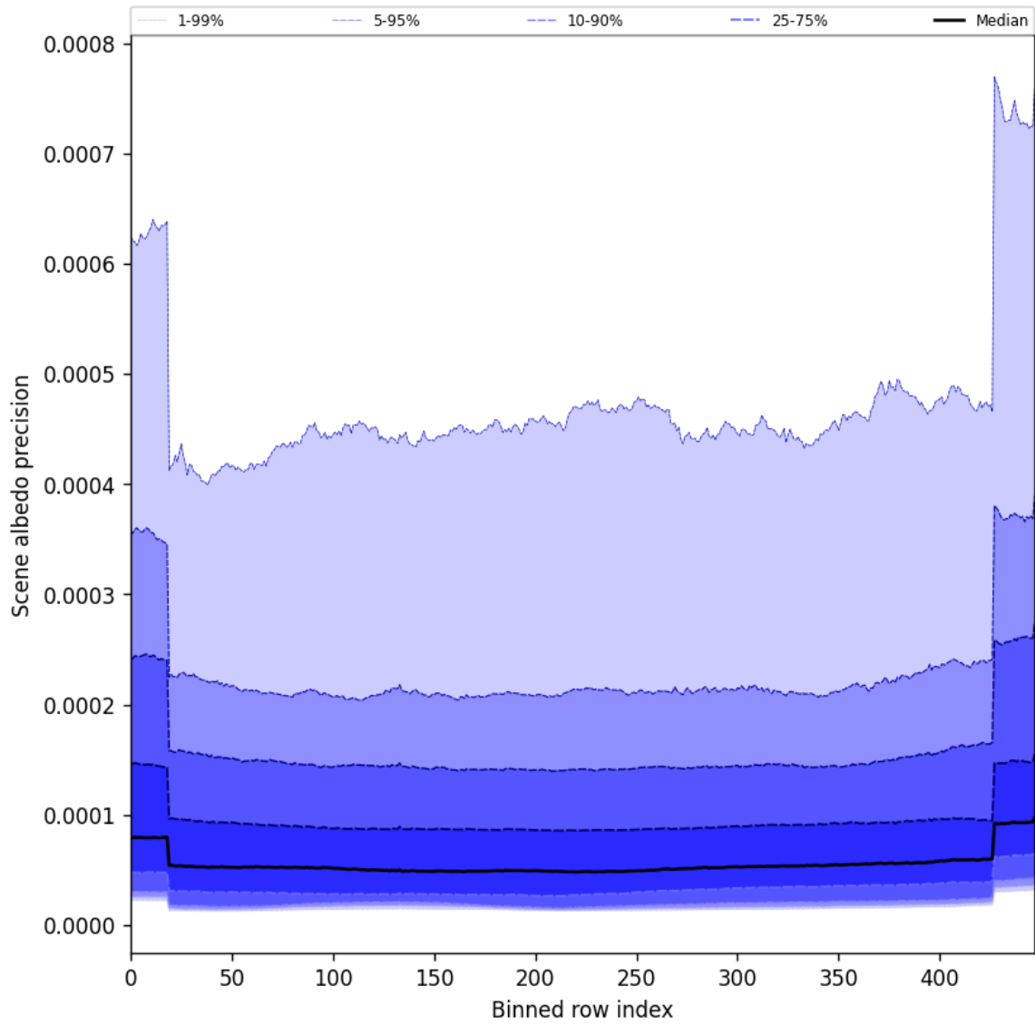
Figure 52: Along track statistics of “Scene albedo precision” for 2024-11-17 to 2024-11-19
