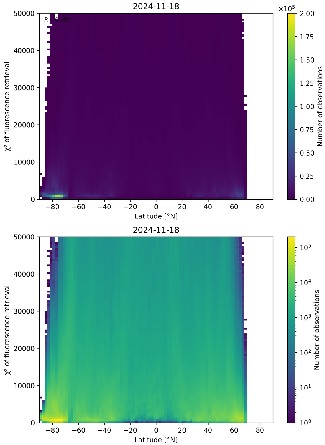
Figure 89: Scatter density plot of “Latitude” against “ \chi^2 of fluorescence retrieval” for 2024-11-17 to 2024-11-19.
