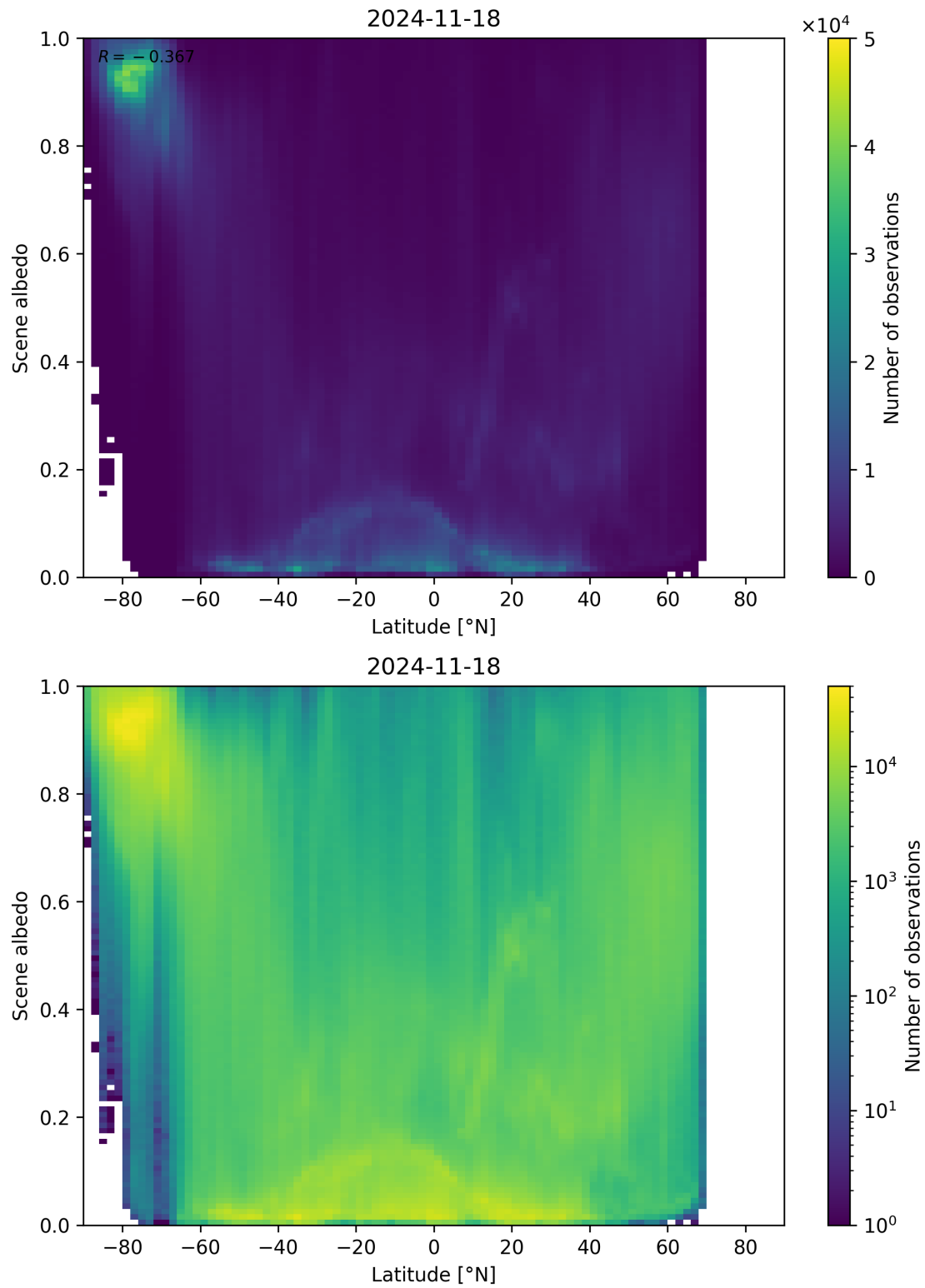
Figure 95: Scatter density plot of “Latitude” against “Scene albedo” for 2024-11-17 to 2024-11-19.
