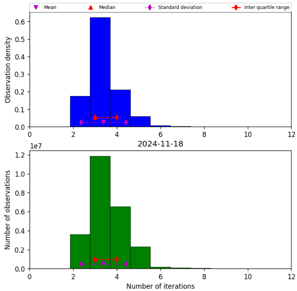
Figure 39: Histogram of “Number of iterations” for 2024-11-17 to 2024-11-19
