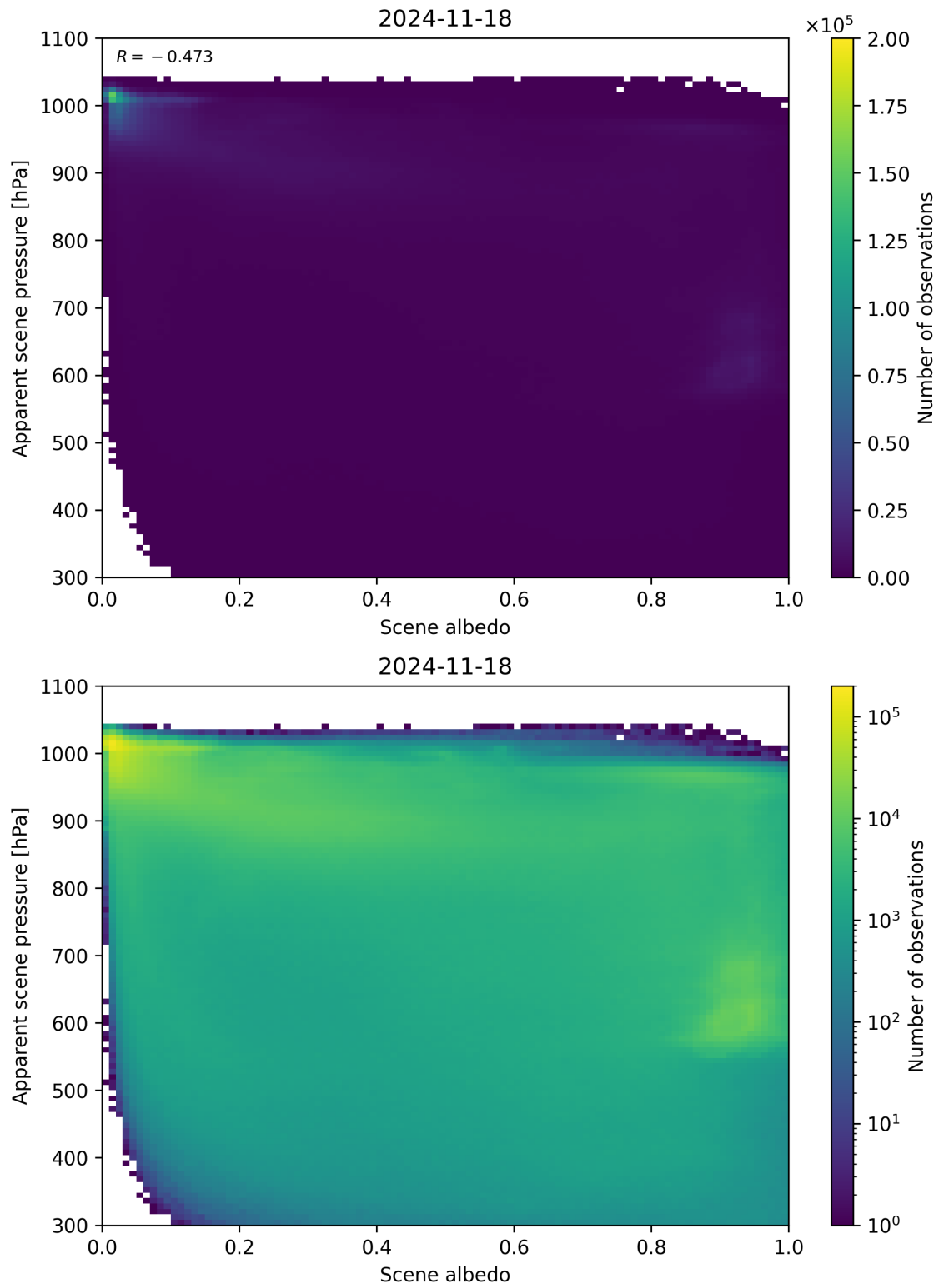
Figure 102: Scatter density plot of “Scene albedo” against “Apparent scene pressure” for 2024-11-17 to 2024-11-19.
