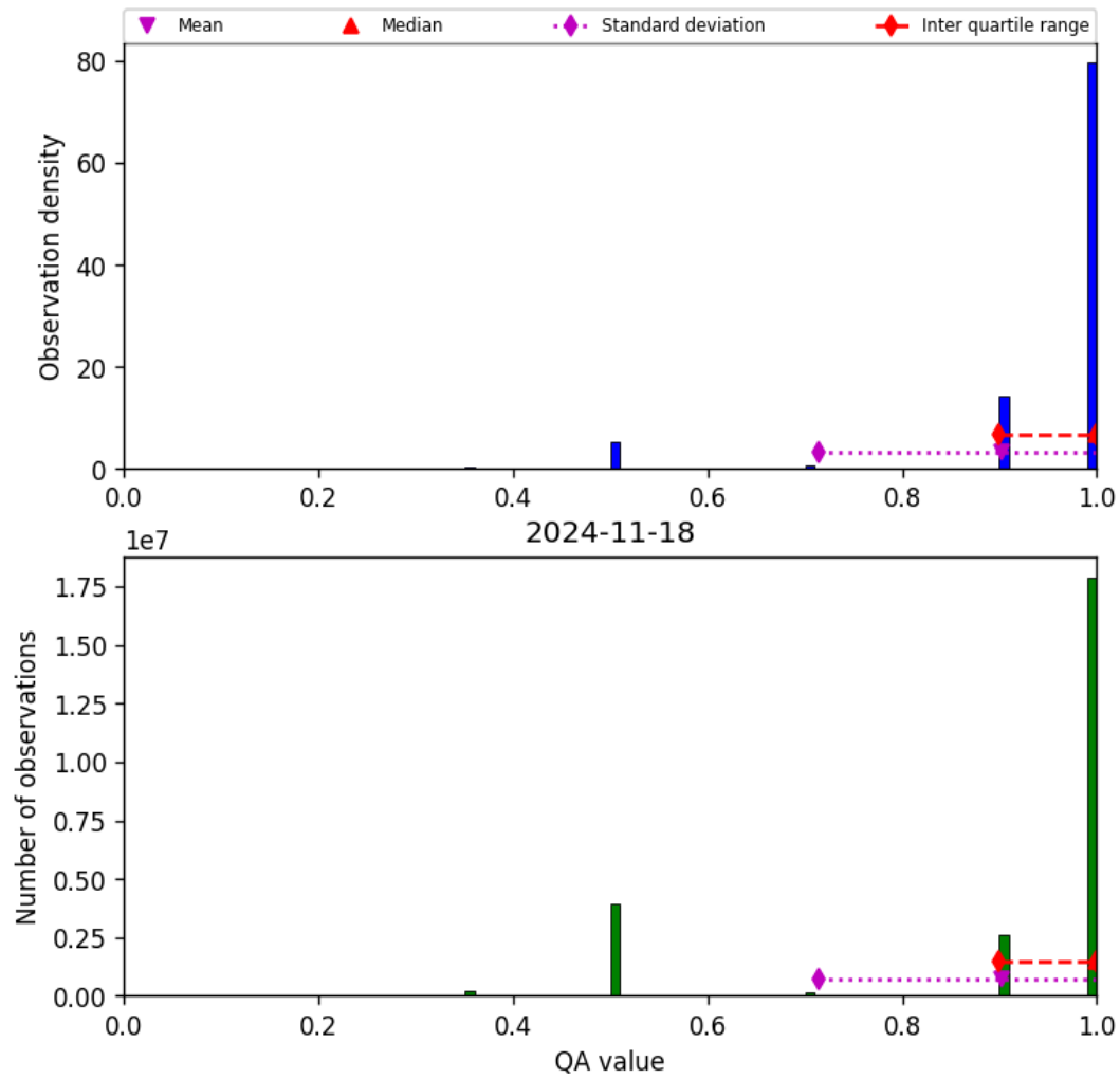
Figure 29: Histogram of “QA value” for 2024-11-17 to 2024-11-19
