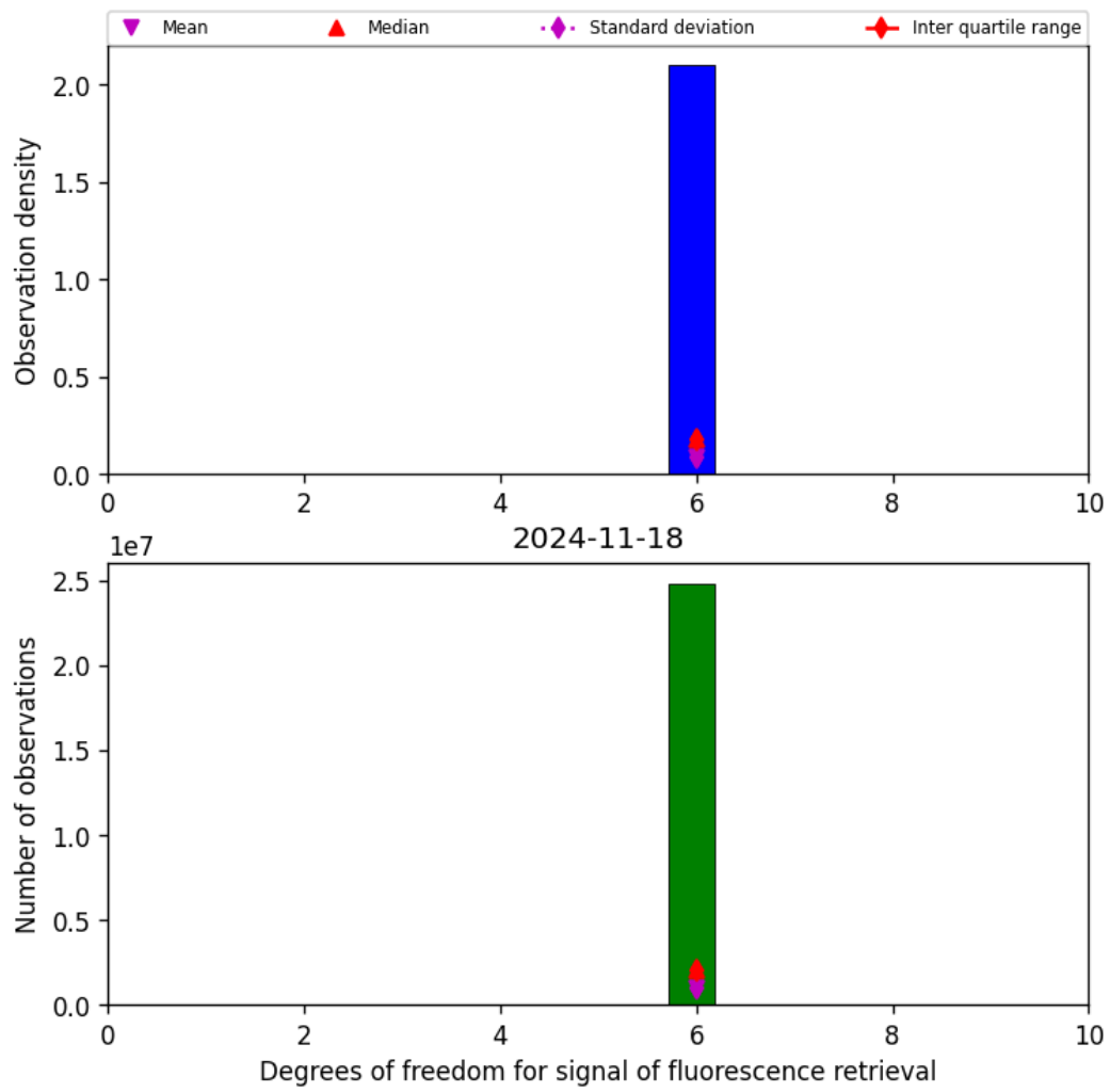
Figure 43: Histogram of “Degrees of freedom for signal of fluorescence retrieval” for 2024-11-17 to 2024-11-19
