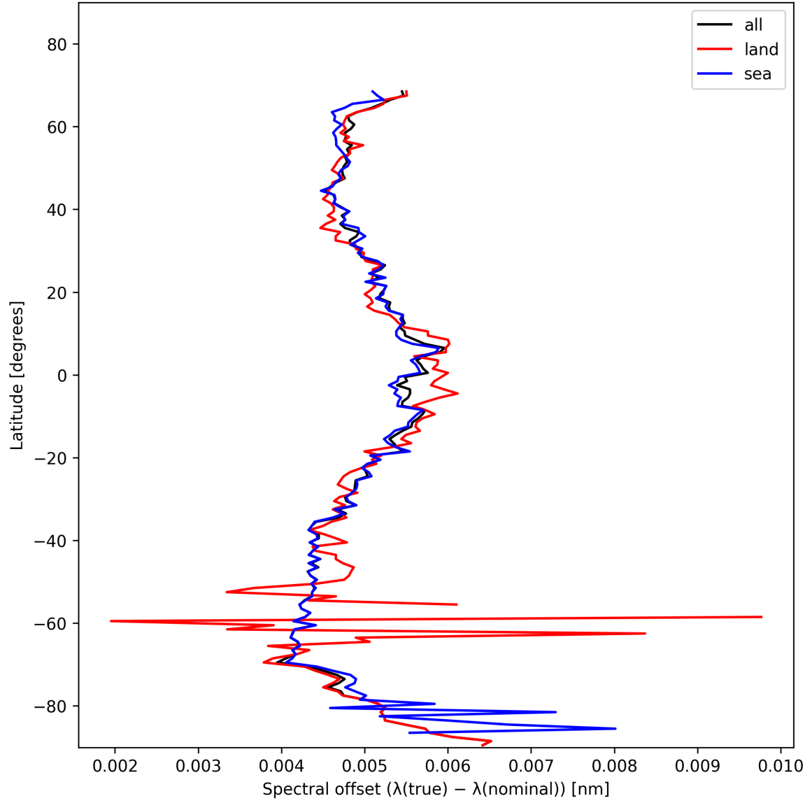
Figure 28: Zonal average of “Spectral offset ( \lambda_{\text{true}} - \lambda_{\text{nominal}} )” for 2024-11-17 to 2024-11-19.
