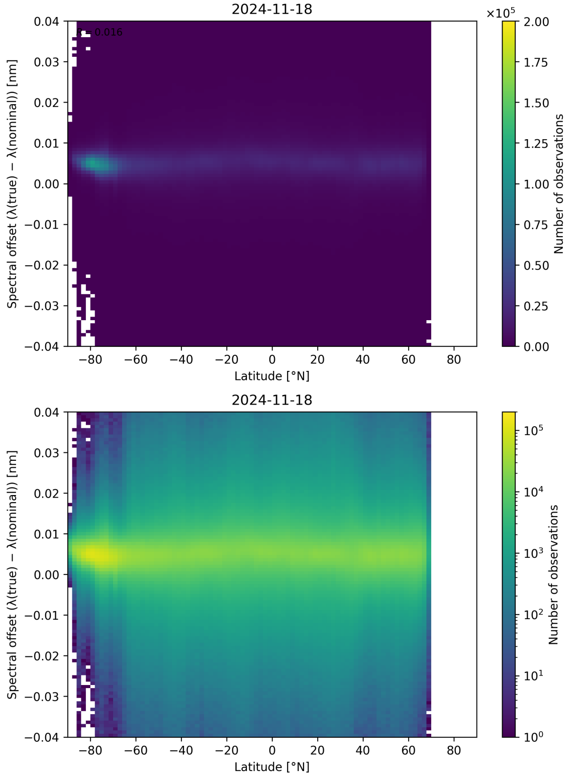
Figure 96: Scatter density plot of “Latitude” against “Spectral offset ( \lambda_{\text{true}} - \lambda_{\text{nominal}} )” for 2024-11-17 to 2024-11-19.
