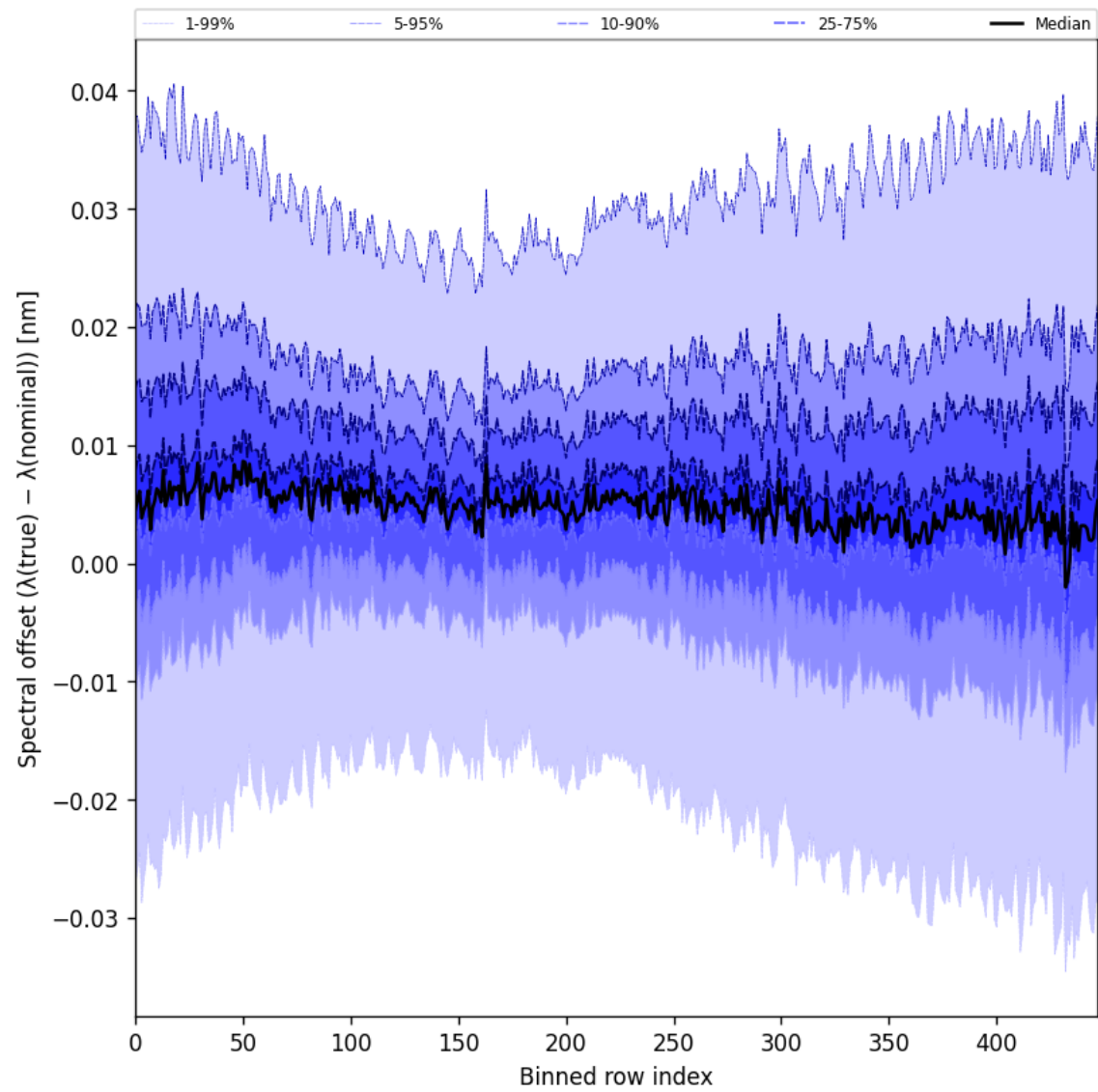
Figure 62: Along track statistics of “Spectral offset ( \lambda_{\text{true}} - \lambda_{\text{nominal}} )” for 2024-11-17 to 2024-11-19
