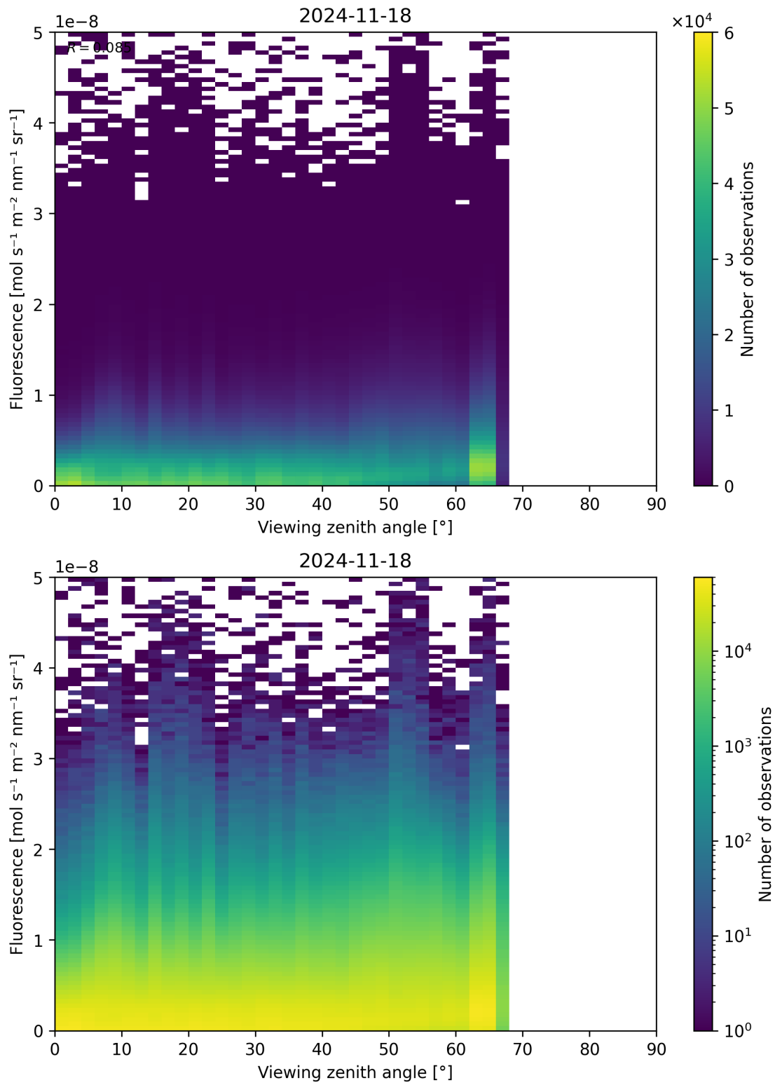
Figure 122: Scatter density plot of “Viewing zenith angle” against “Fluorescence” for 2024-11-17 to 2024-11-19.
