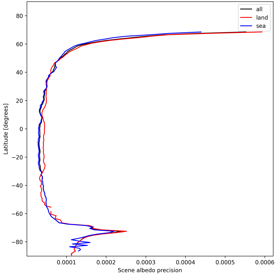
Figure 18: Zonal average of “Scene albedo precision” for 2024-11-17 to 2024-11-19.
