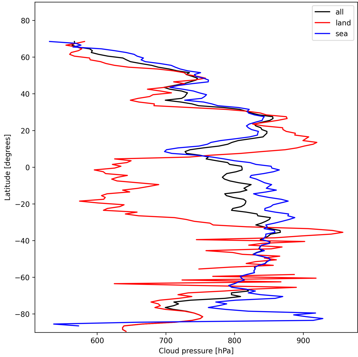
Figure 13: Zonal average of “Cloud pressure” for 2024-11-17 to 2024-11-19.
