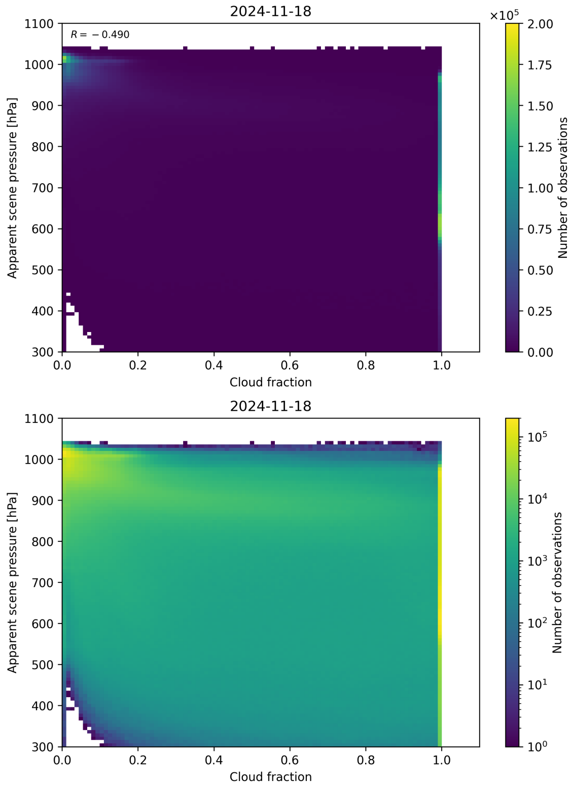
Figure 70: Scatter density plot of “Cloud fraction” against “Apparent scene pressure” for 2024-11-17 to 2024-11-19.
