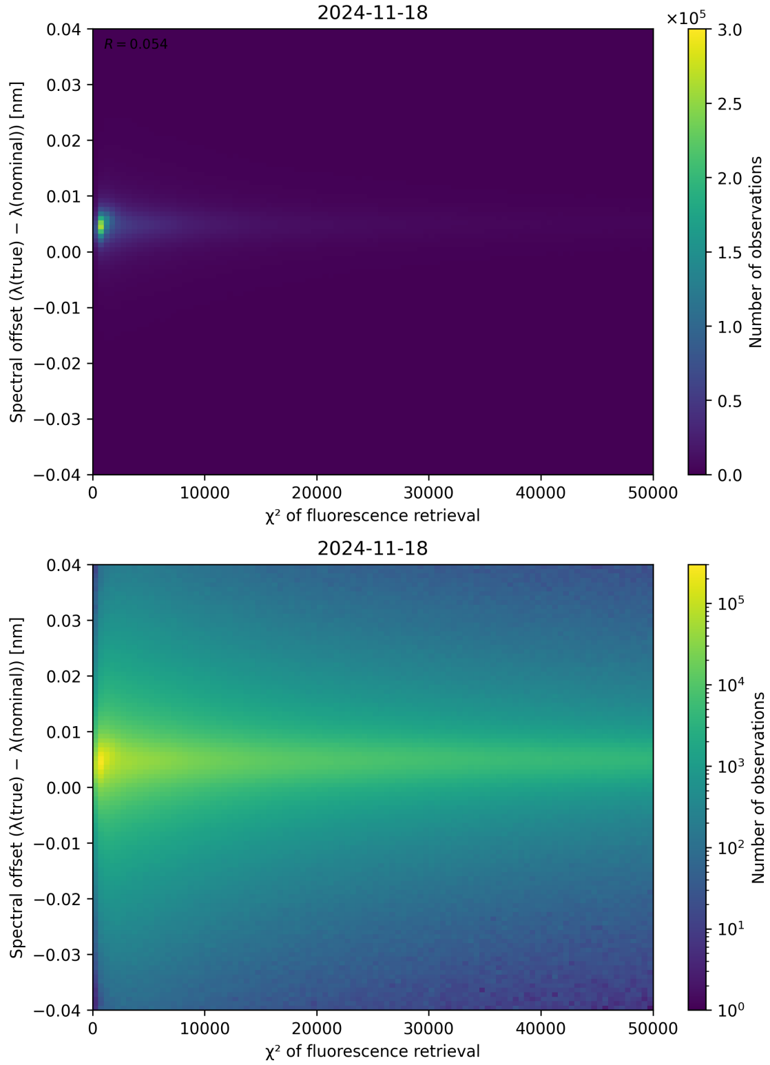
Figure 69: Scatter density plot of “ \chi^2 of fluorescence retrieval” against “Spectral offset ( \lambda_{\text{true}} - \lambda_{\text{nominal}} )” for 2024-11-17 to 2024-11-19.
