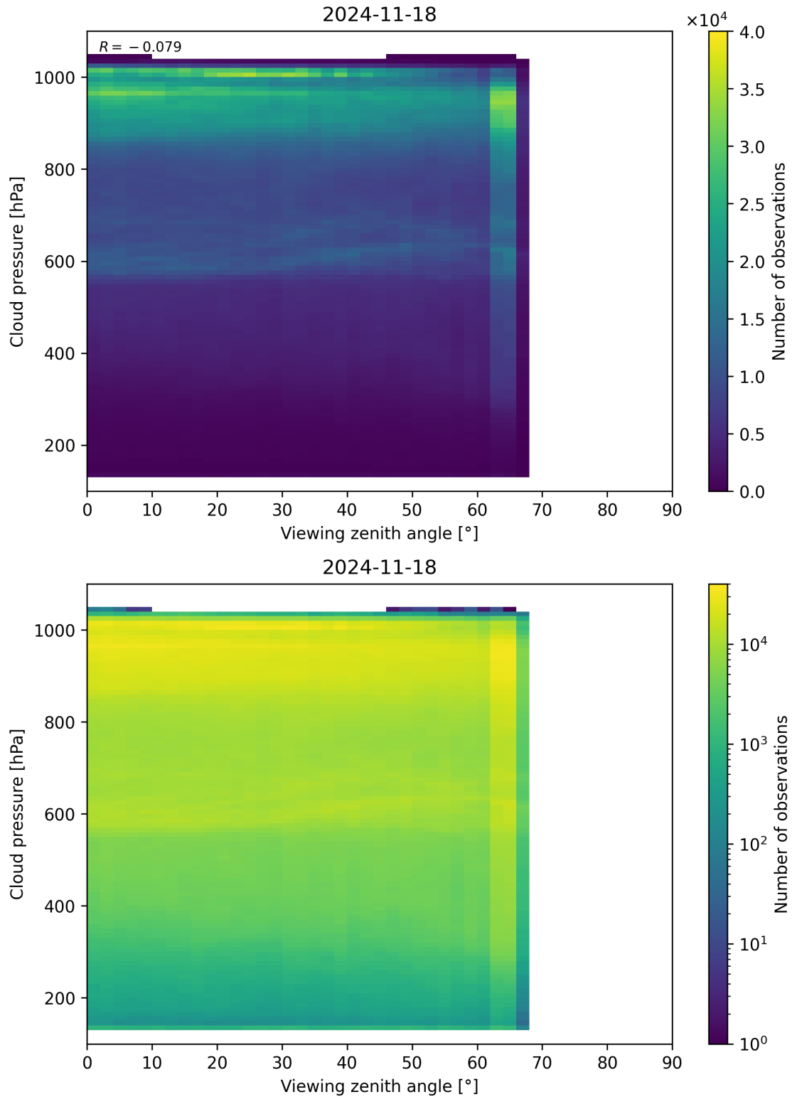
Figure 121: Scatter density plot of “Viewing zenith angle” against “Cloud pressure” for 2024-11-17 to 2024-11-19.
