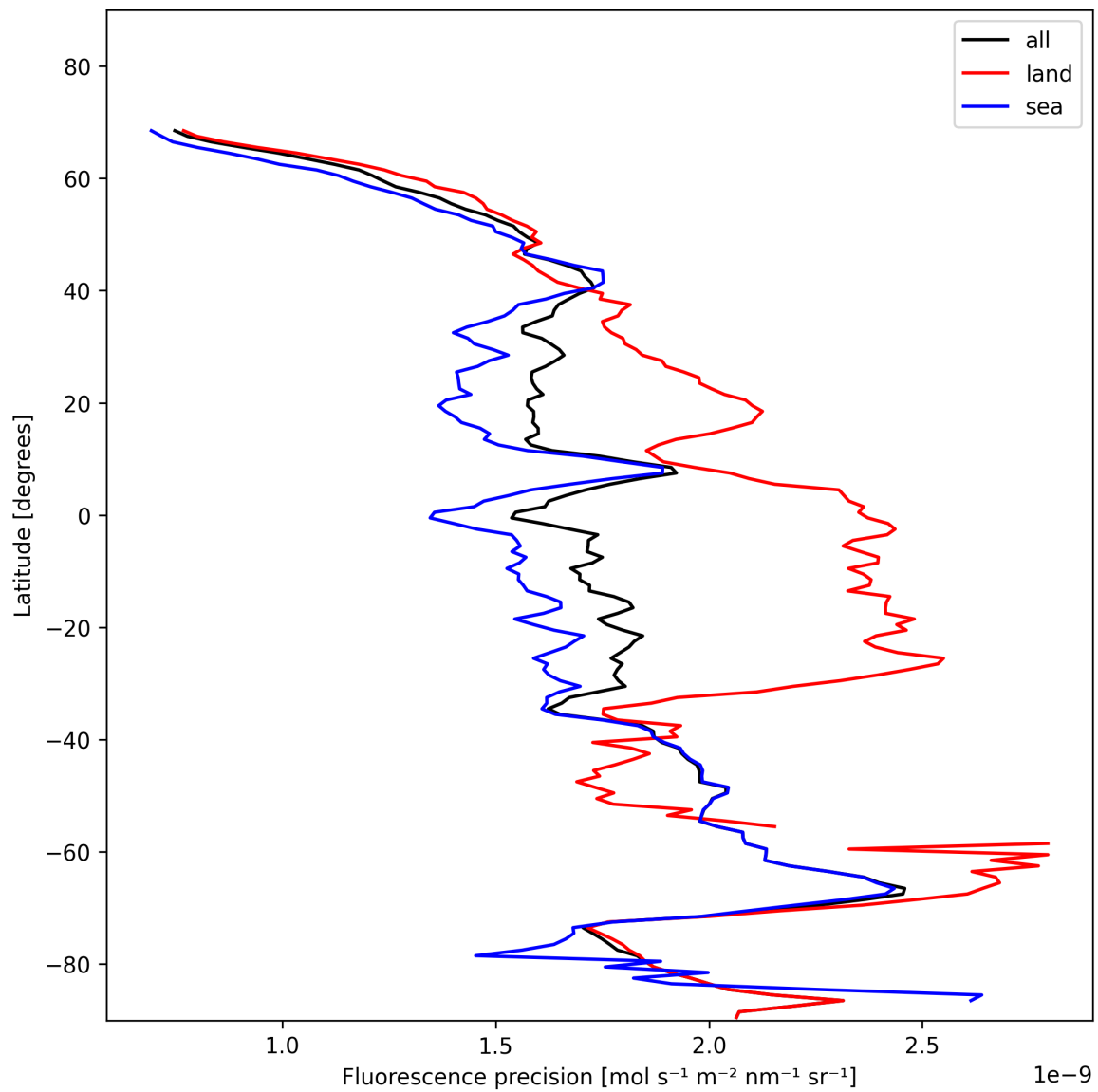
Figure 24: Zonal average of “Fluorescence precision” for 2024-11-17 to 2024-11-19.
