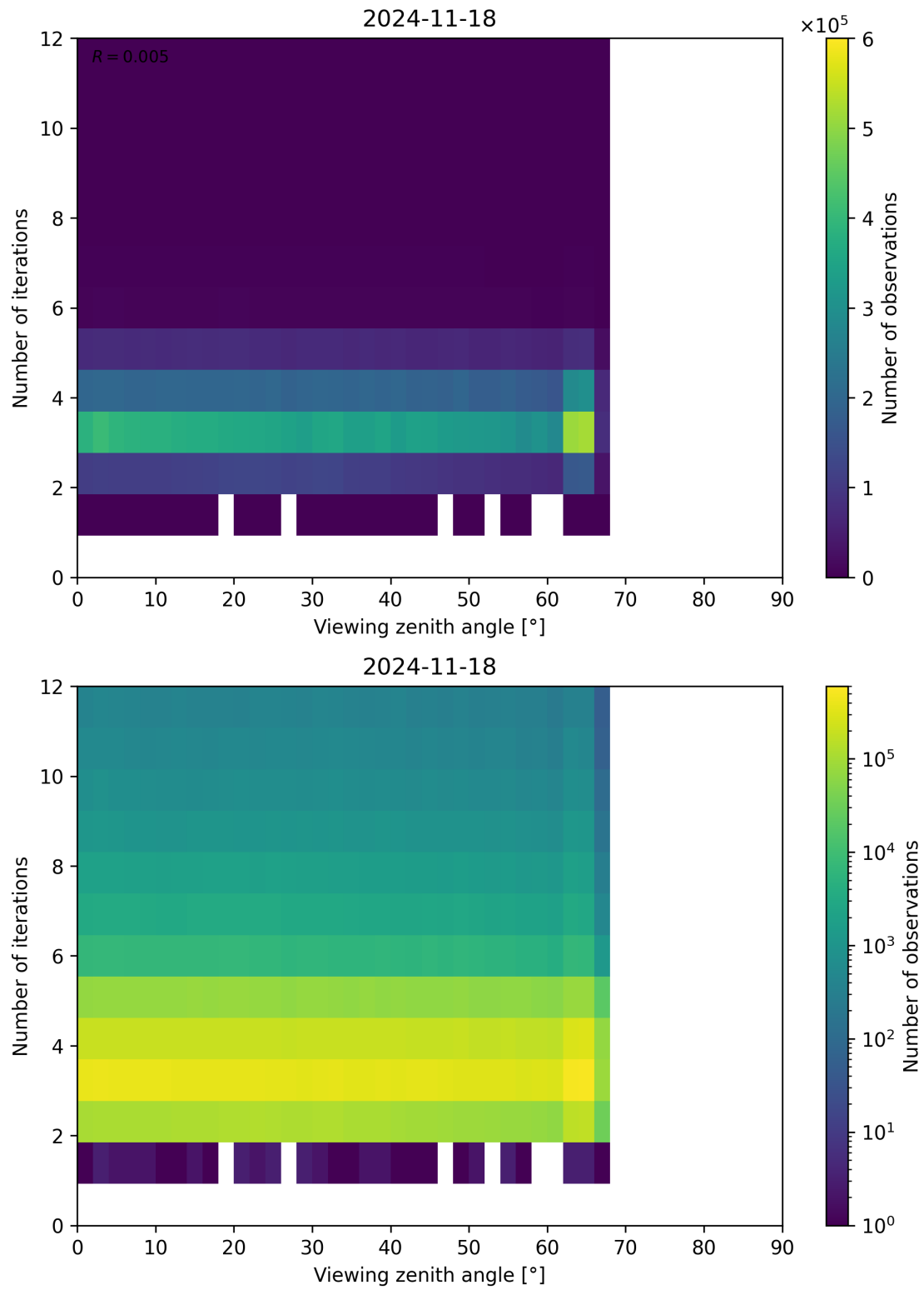
Figure 124: Scatter density plot of “Viewing zenith angle” against “Number of iterations” for 2024-11-17 to 2024-11-19.
