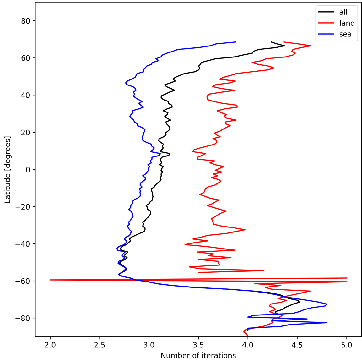
Figure 22: Zonal average of “Number of iterations” for 2024-11-17 to 2024-11-19.
