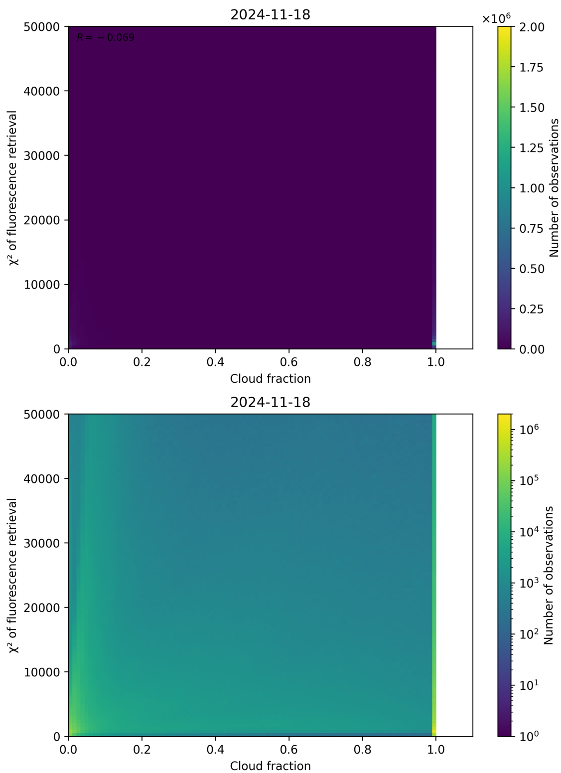
Figure 71: Scatter density plot of “Cloud fraction” against “ \chi^2 of fluorescence retrieval” for 2024-11-17 to 2024-11-19.
