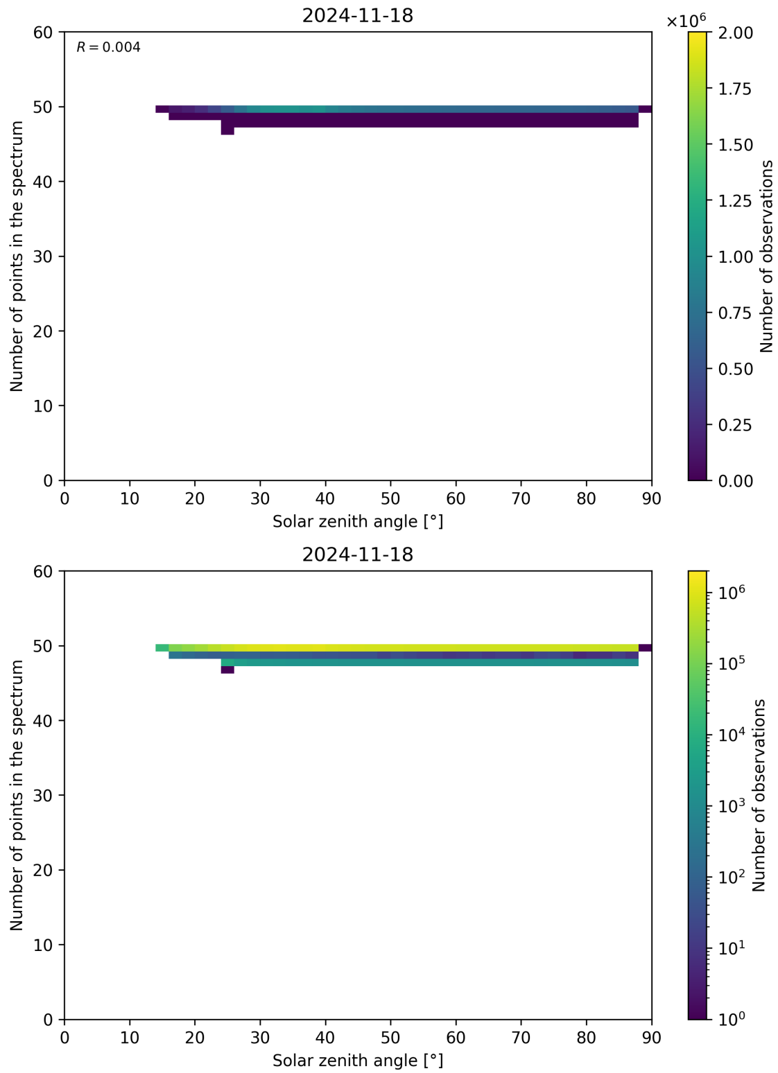
Figure 115: Scatter density plot of “Solar zenith angle” against “Number of points in the spectrum” for 2024-11-17 to 2024-11-19.
