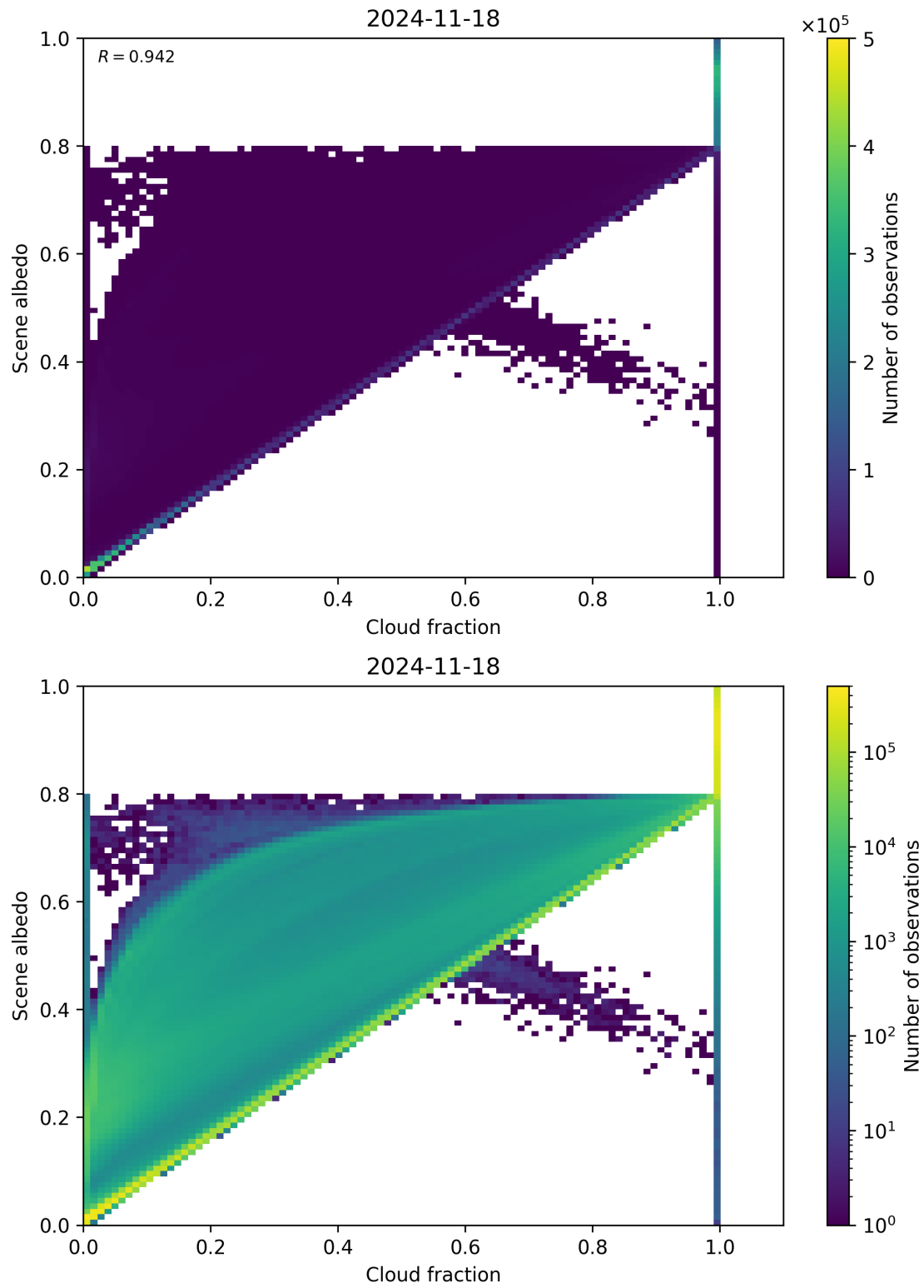
Figure 75: Scatter density plot of “Cloud fraction” against “Scene albedo” for 2024-11-17 to 2024-11-19.
