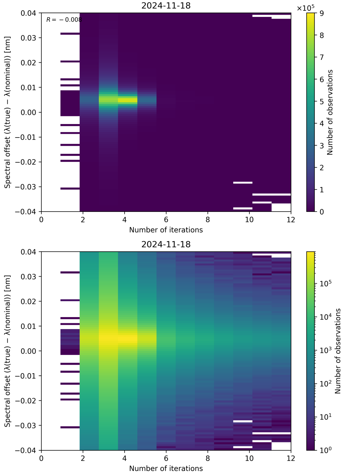
Figure 100: Scatter density plot of “Number of iterations” against “Spectral offset ( \lambda_{\text{true}} - \lambda_{\text{nominal}} )” for 2024-11-17 to 2024-11-19.
