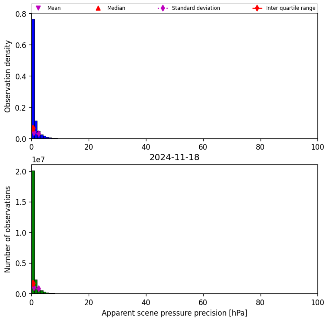
Figure 37: Histogram of “Apparent scene pressure precision” for 2024-11-17 to 2024-11-19
