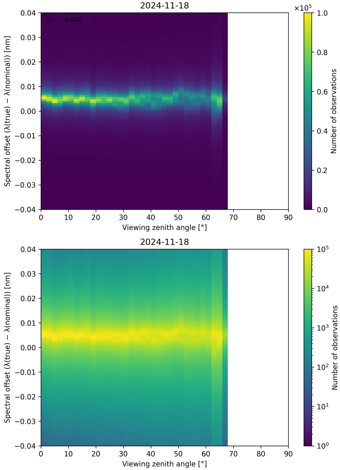
Figure 128: Scatter density plot of “Viewing zenith angle” against “Spectral offset ( \lambda_{\text{true}} - \lambda_{\text{nominal}} )” for 2024-11-17 to 2024-11-19.
