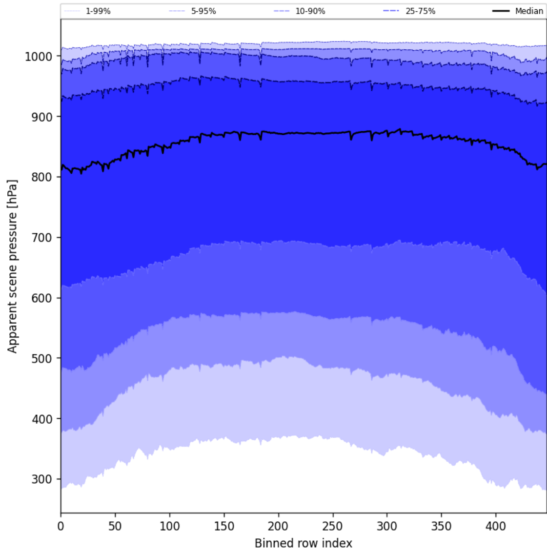
Figure 53: Along track statistics of “Apparent scene pressure” for 2024-11-17 to 2024-11-19
