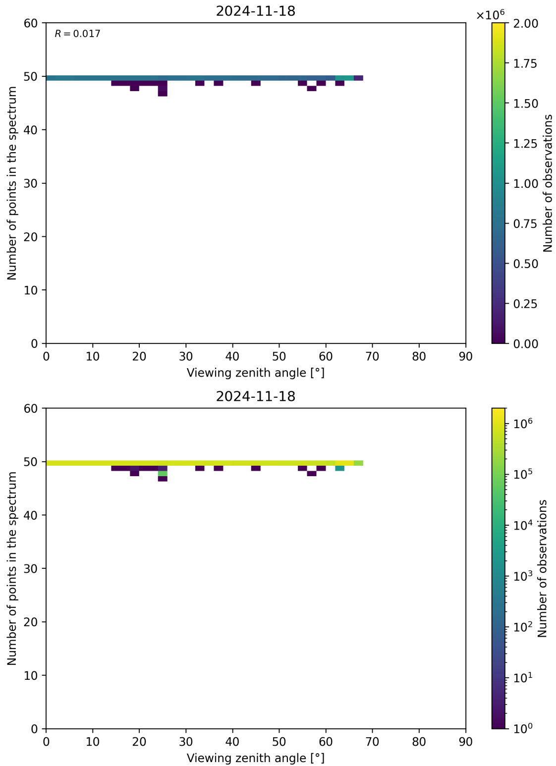
Figure 125: Scatter density plot of “Viewing zenith angle” against “Number of points in the spectrum” for 2024-11-17 to 2024-11-19.
