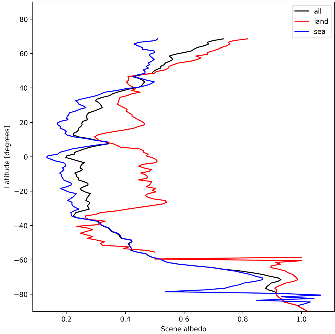
Figure 17: Zonal average of “Scene albedo” for 2024-11-17 to 2024-11-19.
