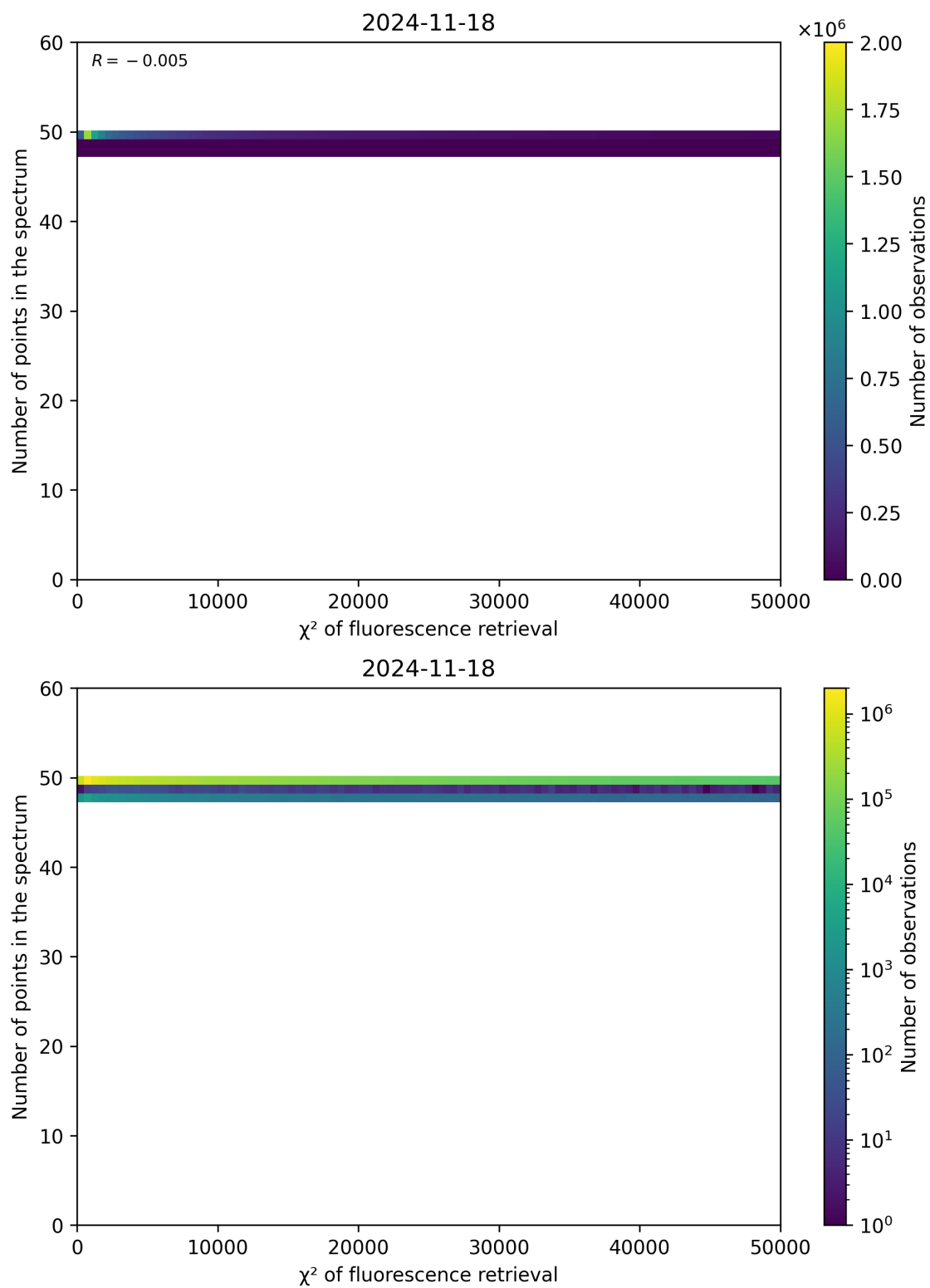
Figure 68: Scatter density plot of “ \chi^2 of fluorescence retrieval” against “Number of points in the spectrum” for 2024-11-17 to 2024-11-19.
