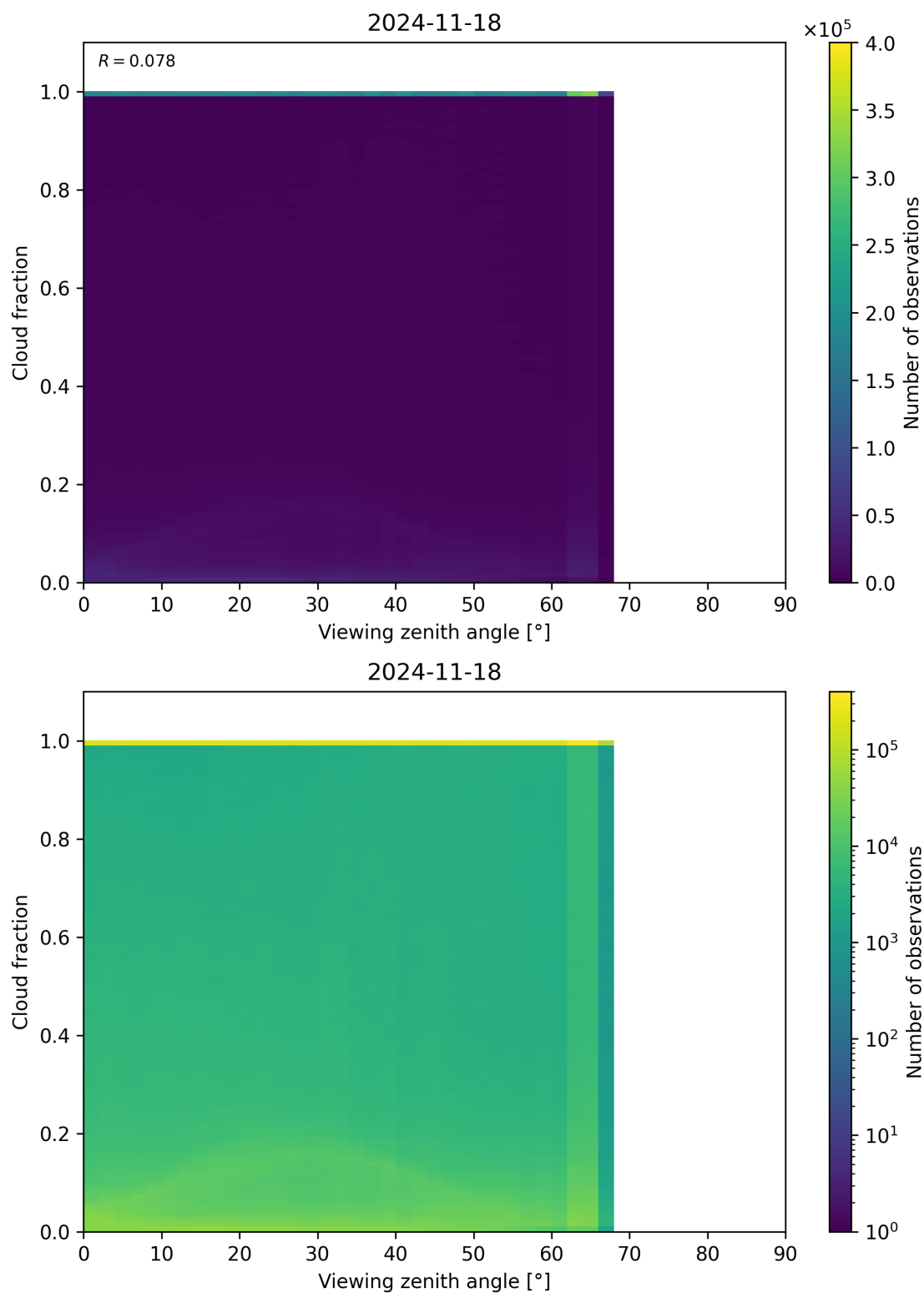
Figure 120: Scatter density plot of “Viewing zenith angle” against “Cloud fraction” for 2024-11-17 to 2024-11-19.
