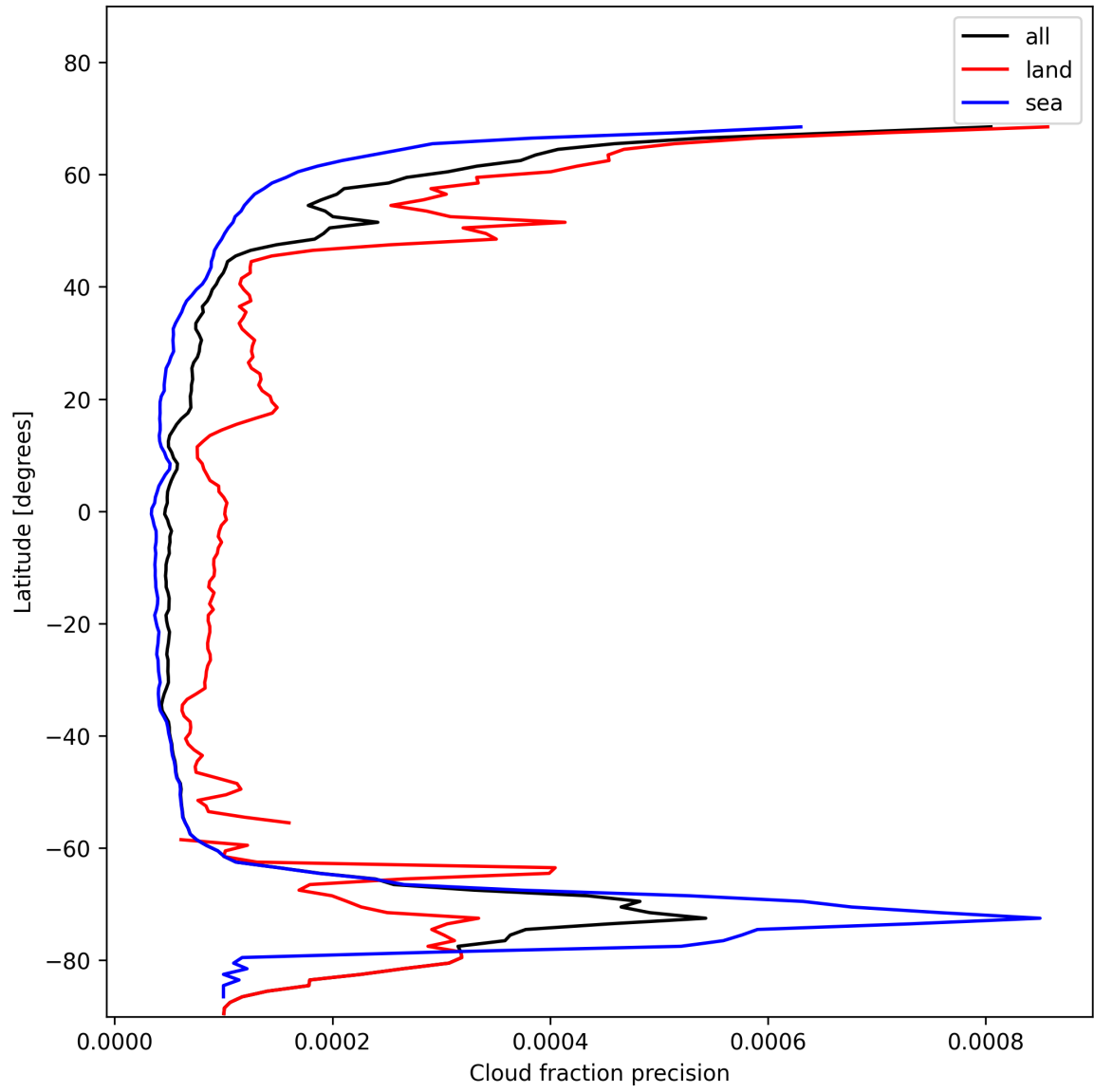
Figure 16: Zonal average of “Cloud fraction precision” for 2024-11-17 to 2024-11-19.
