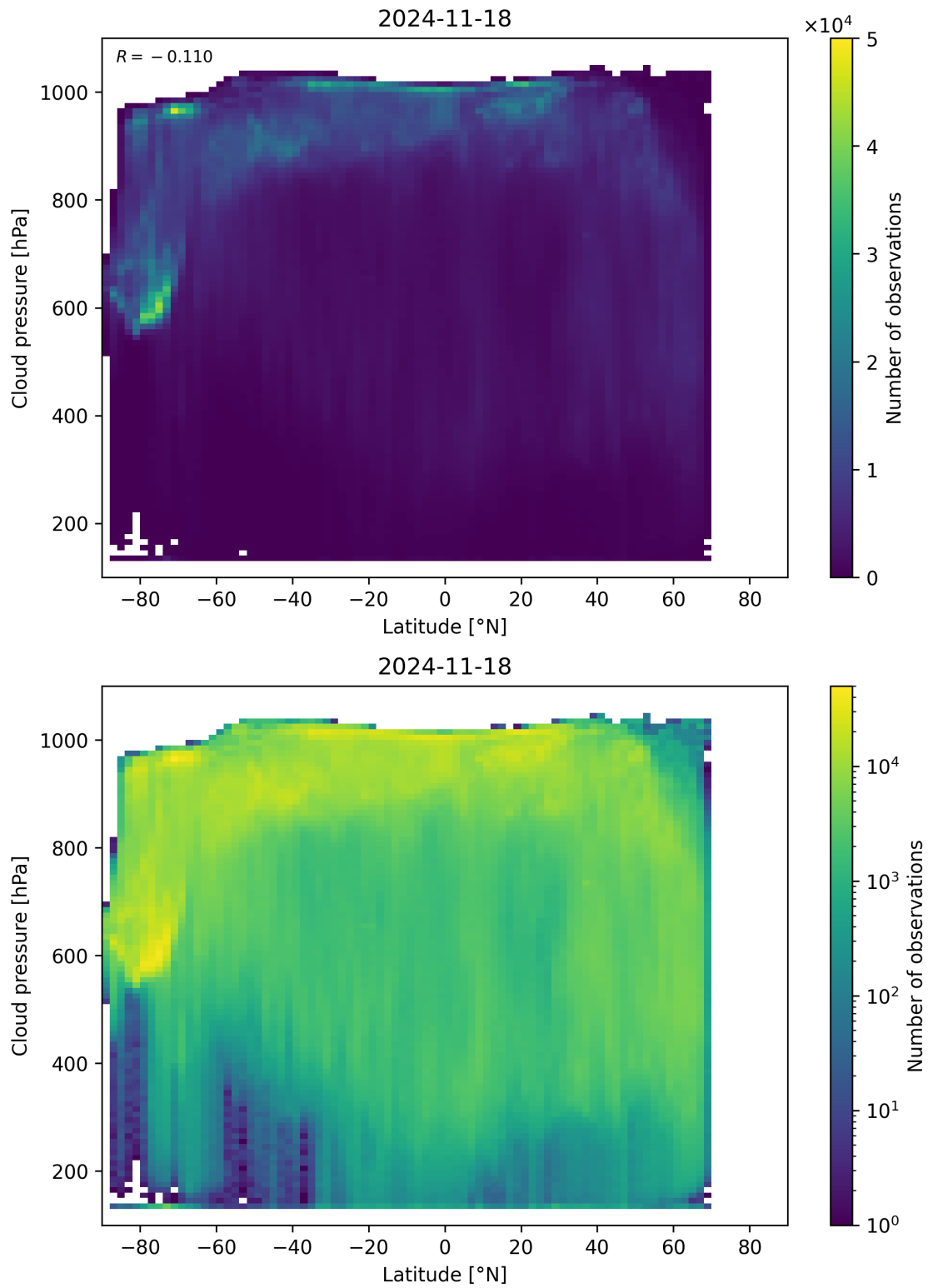
Figure 91: Scatter density plot of “Latitude” against “Cloud pressure” for 2024-11-17 to 2024-11-19.
