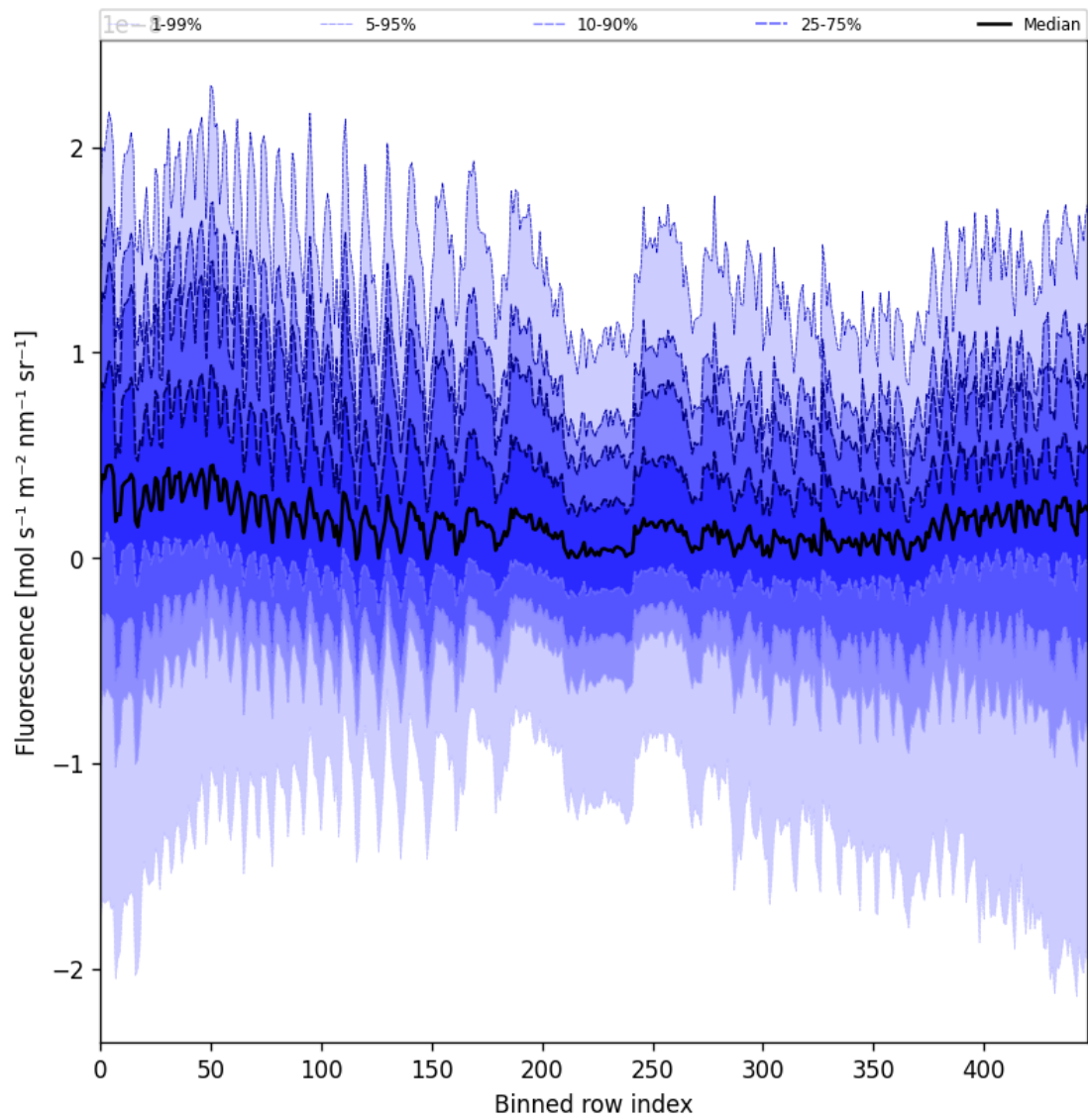
Figure 57: Along track statistics of “Fluorescence” for 2024-11-17 to 2024-11-19
