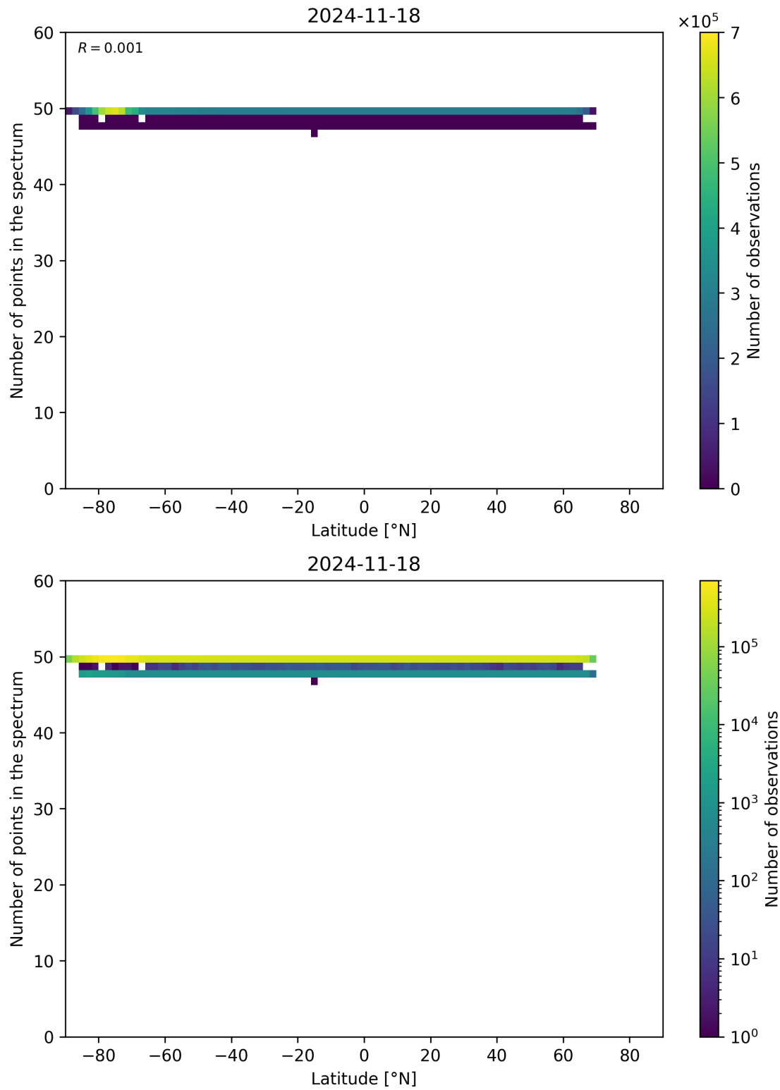
Figure 94: Scatter density plot of “Latitude” against “Number of points in the spectrum” for 2024-11-17 to 2024-11-19.
