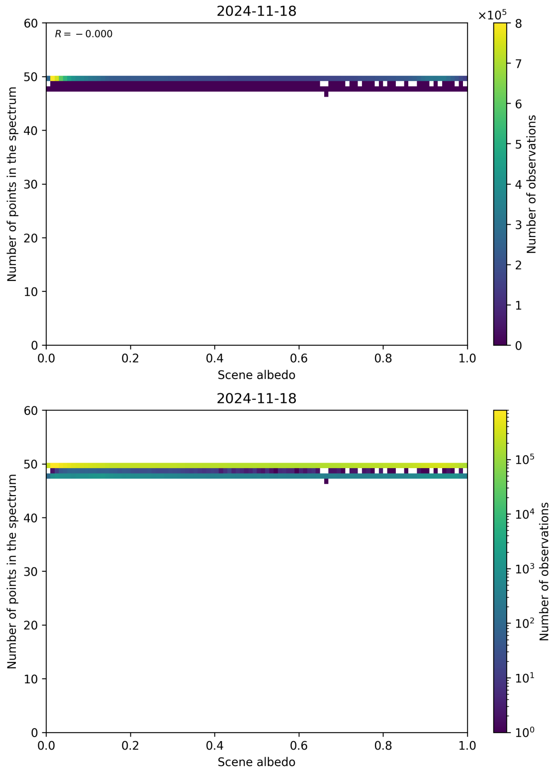
Figure 106: Scatter density plot of “Scene albedo” against “Number of points in the spectrum” for 2024-11-17 to 2024-11-19.
