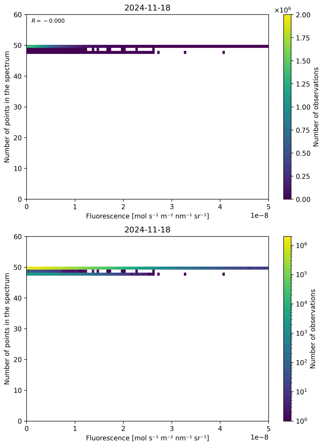
Figure 86: Scatter density plot of “Fluorescence” against “Number of points in the spectrum” for 2024-11-17 to 2024-11-19.
