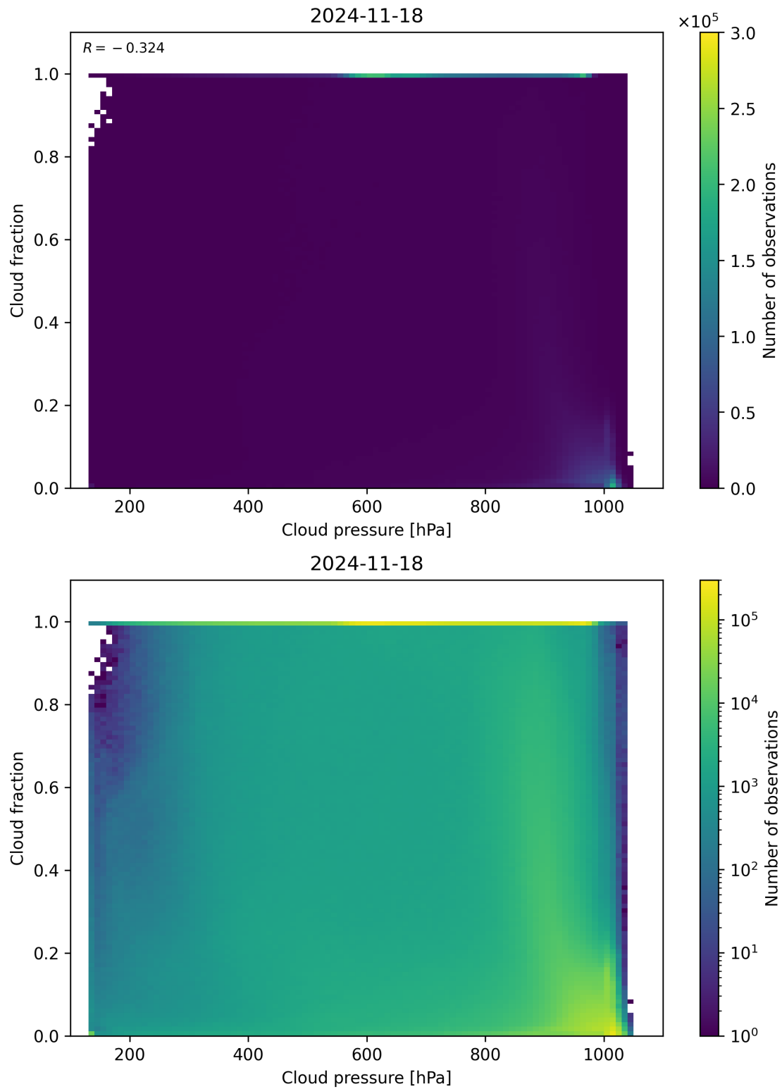
Figure 79: Scatter density plot of “Cloud pressure” against “Cloud fraction” for 2024-11-17 to 2024-11-19.
