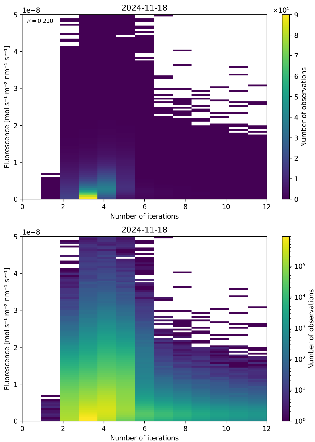
Figure 98: Scatter density plot of “Number of iterations” against “Fluorescence” for 2024-11-17 to 2024-11-19.
