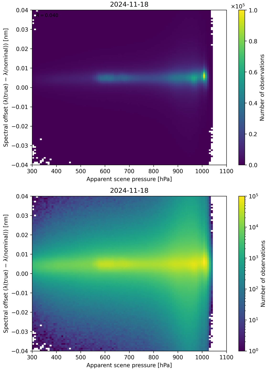
Figure 67: Scatter density plot of “Apparent scene pressure” against “Spectral offset ( \lambda_{\text{true}} - \lambda_{\text{nominal}} )” for 2024-11-17 to 2024-11-19.
