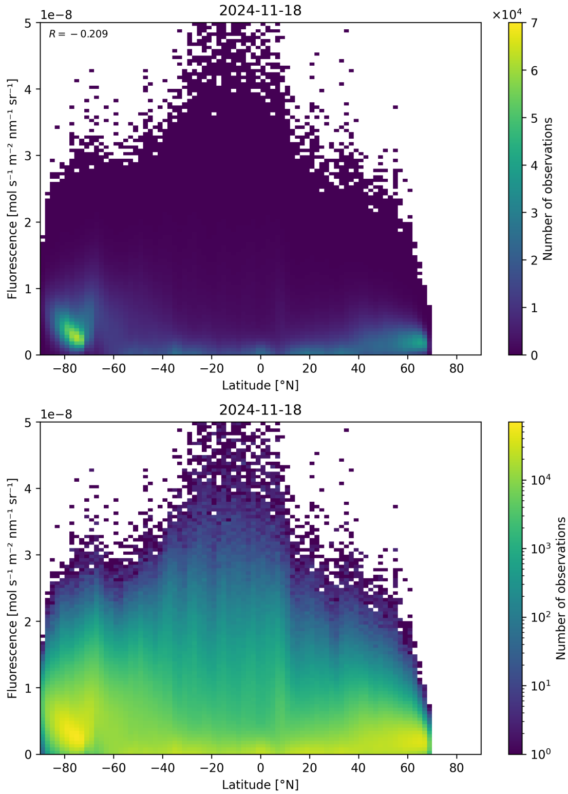
Figure 92: Scatter density plot of “Latitude” against “Fluorescence” for 2024-11-17 to 2024-11-19.
