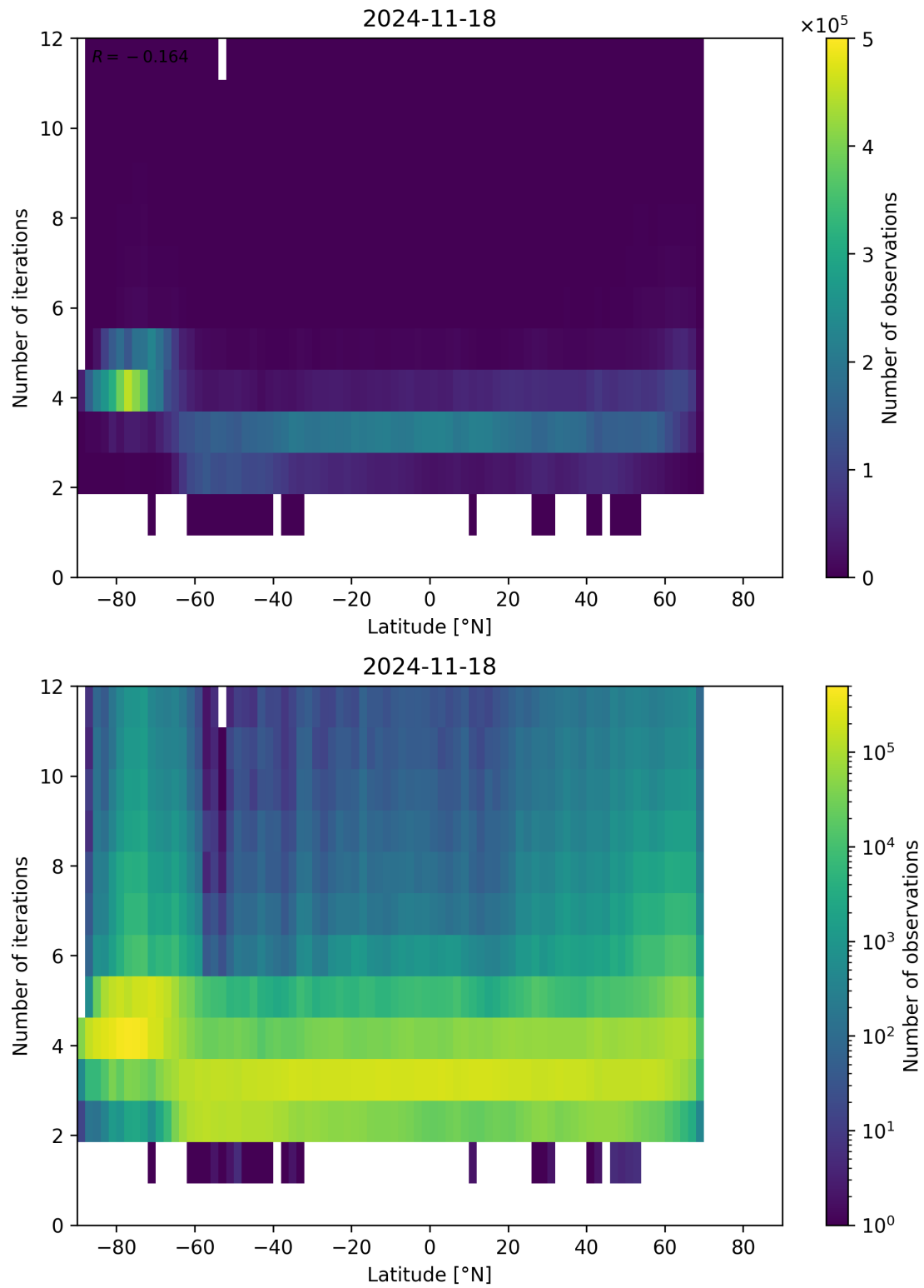
Figure 93: Scatter density plot of “Latitude” against “Number of iterations” for 2024-11-17 to 2024-11-19.
