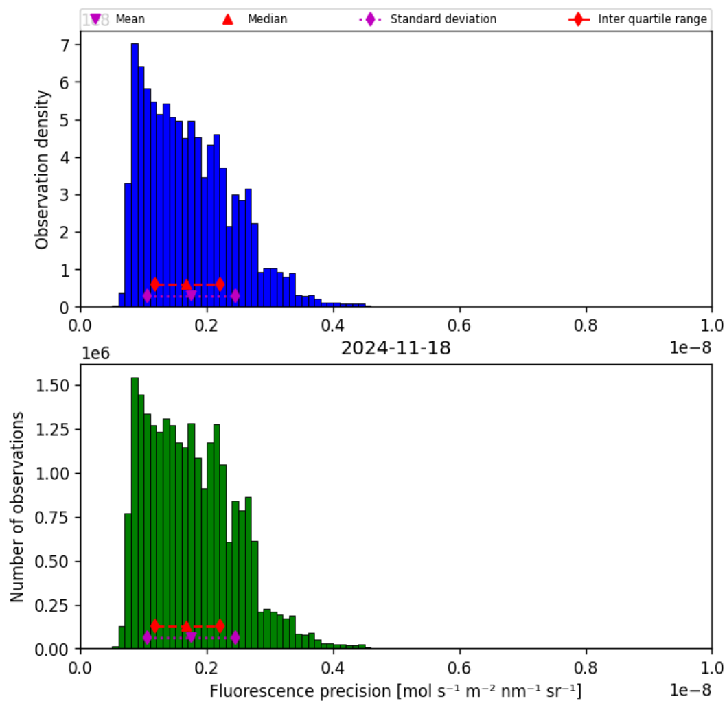
Figure 41: Histogram of “Fluorescence precision” for 2024-11-17 to 2024-11-19
