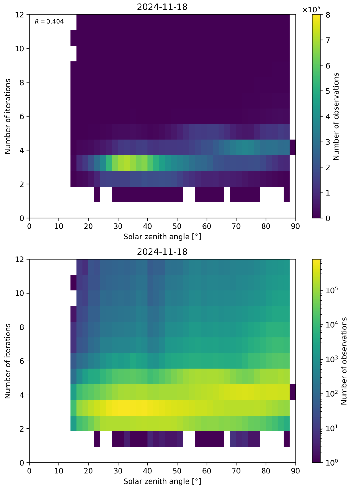
Figure 114: Scatter density plot of “Solar zenith angle” against “Number of iterations” for 2024-11-17 to 2024-11-19.
