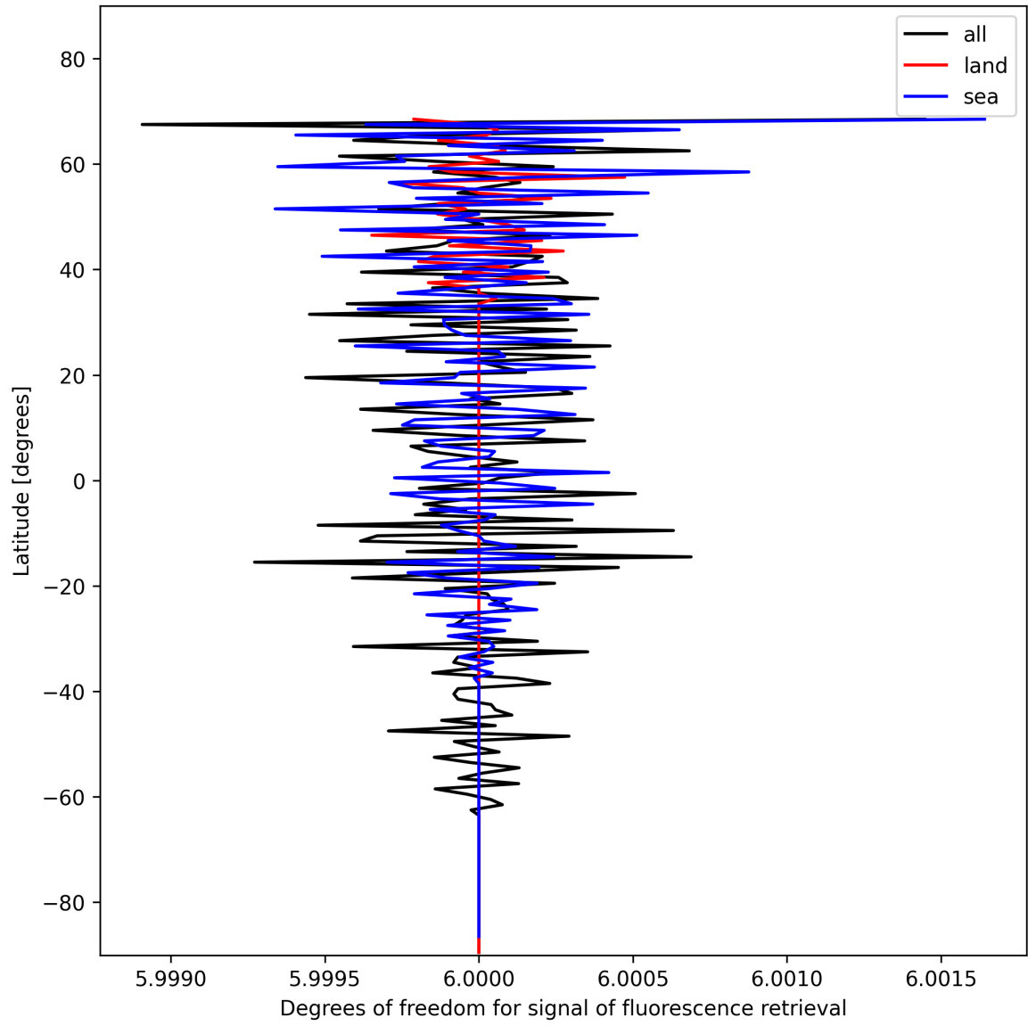
Figure 26: Zonal average of “Degrees of freedom for signal of fluorescence retrieval” for 2024-11-17 to 2024-11-19.
