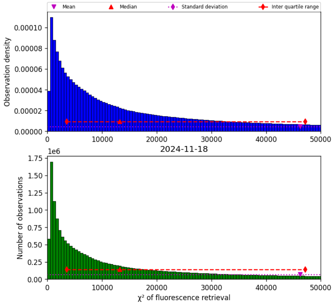
Figure 42: Histogram of “ \chi^2 of fluorescence retrieval” for 2024-11-17 to 2024-11-19
