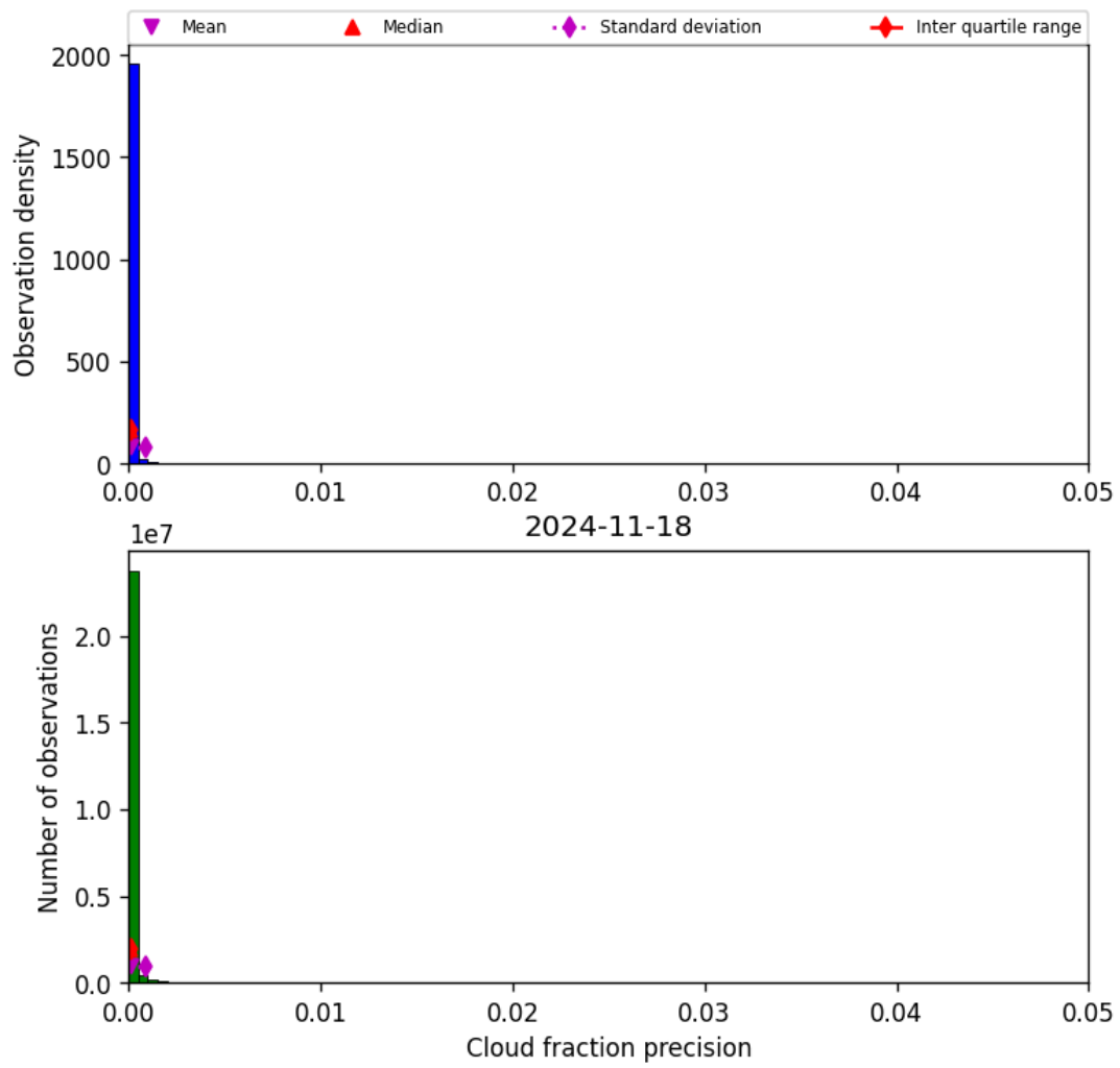
Figure 33: Histogram of “Cloud fraction precision” for 2024-11-17 to 2024-11-19
