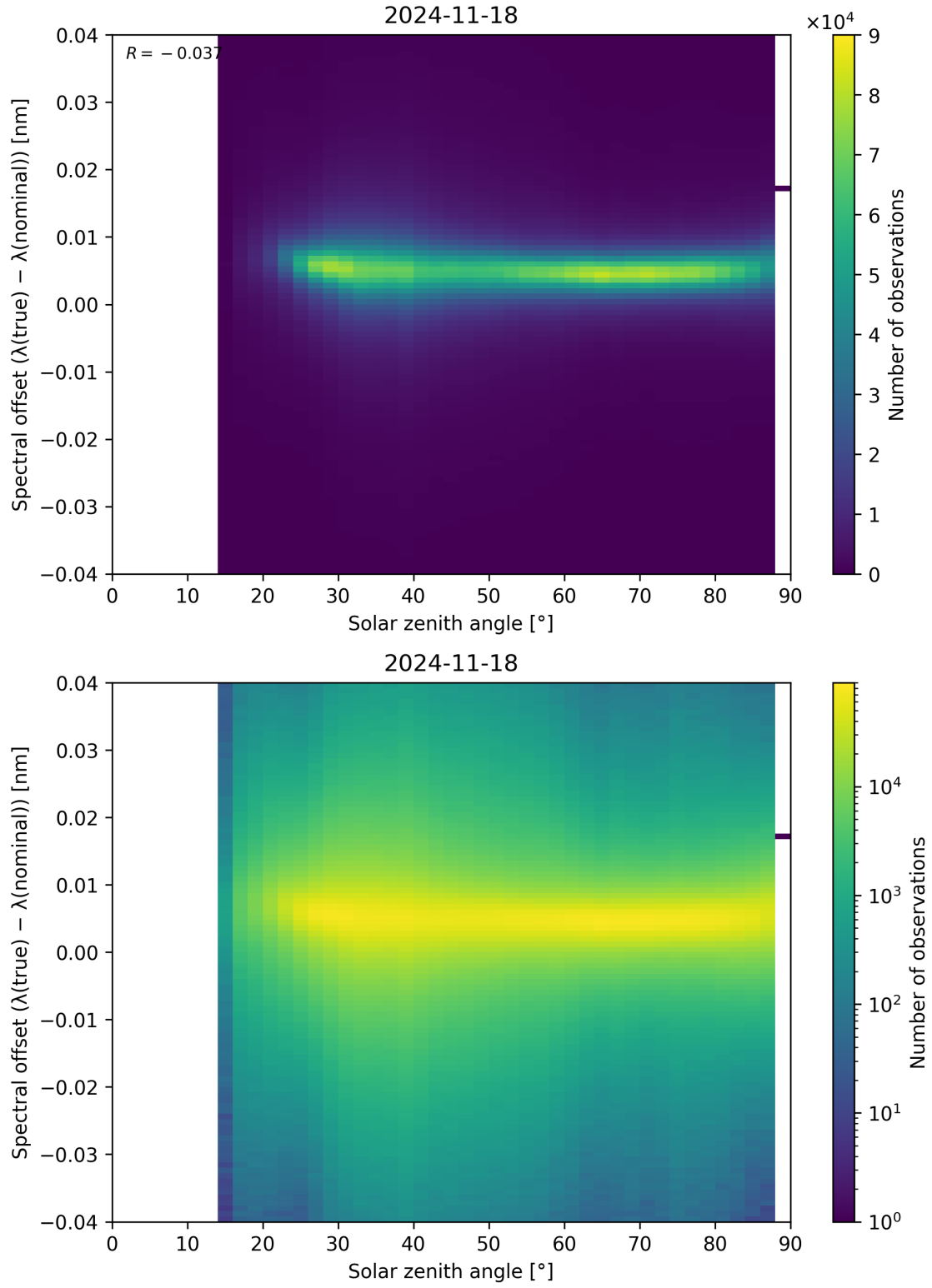
Figure 117: Scatter density plot of “Solar zenith angle” against “Spectral offset ( \lambda_{\text{true}} - \lambda_{\text{nominal}} )” for 2024-11-17 to 2024-11-19.
