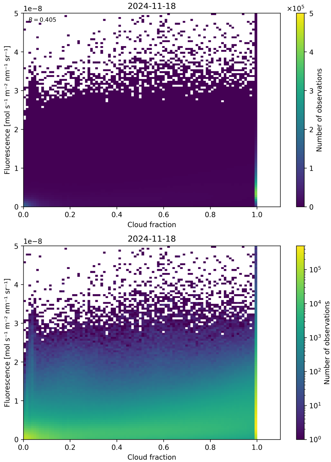
Figure 72: Scatter density plot of “Cloud fraction” against “Fluorescence” for 2024-11-17 to 2024-11-19.
