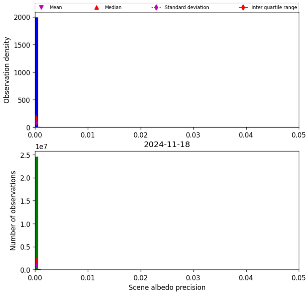
Figure 35: Histogram of “Scene albedo precision” for 2024-11-17 to 2024-11-19
