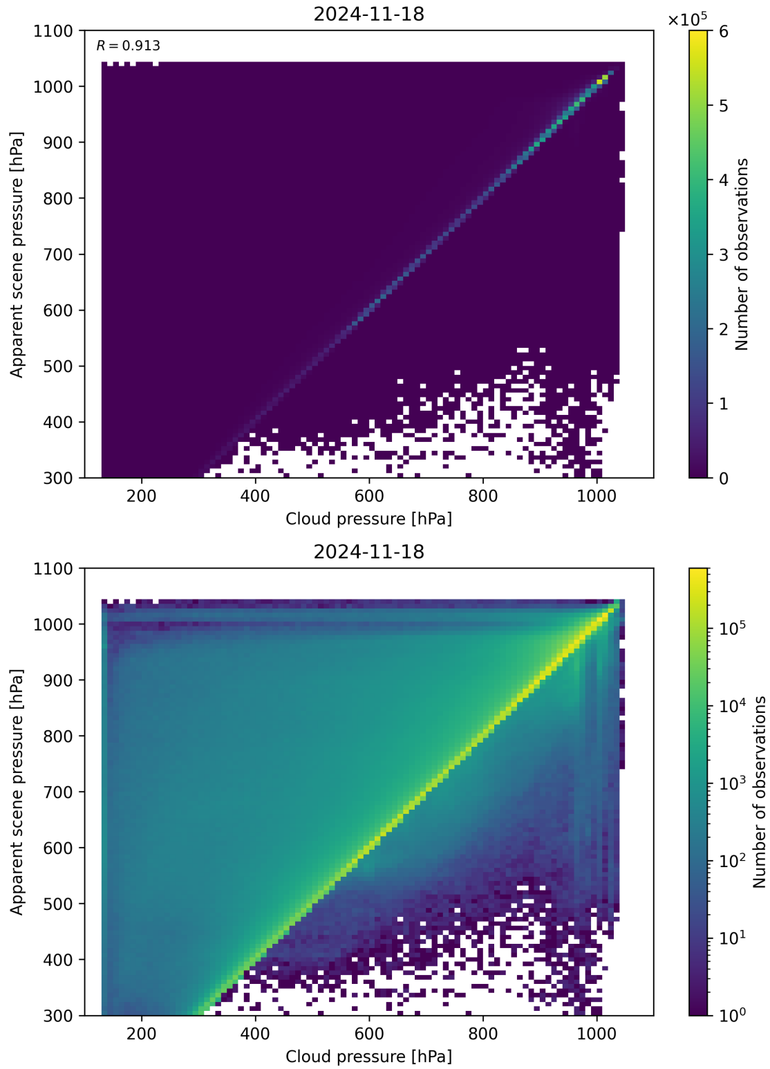
Figure 77: Scatter density plot of “Cloud pressure” against “Apparent scene pressure” for 2024-11-17 to 2024-11-19.
