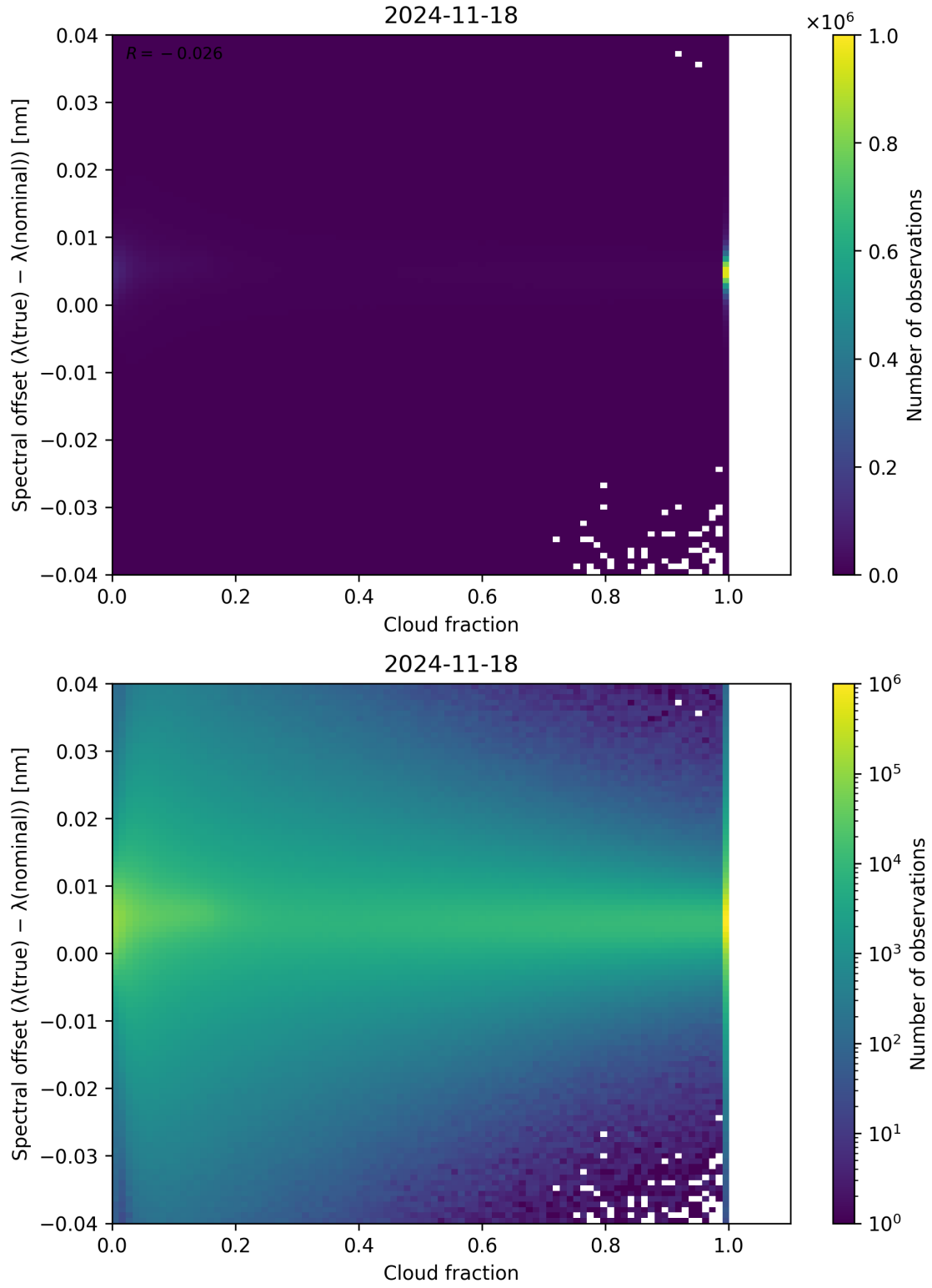
Figure 76: Scatter density plot of “Cloud fraction” against “Spectral offset ( \lambda_{\text{true}} - \lambda_{\text{nominal}} )” for 2024-11-17 to 2024-11-19.
