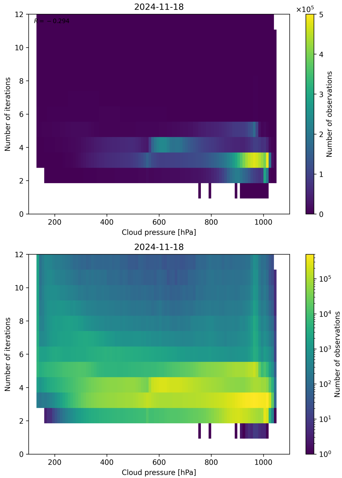
Figure 81: Scatter density plot of “Cloud pressure” against “Number of iterations” for 2024-11-17 to 2024-11-19.
