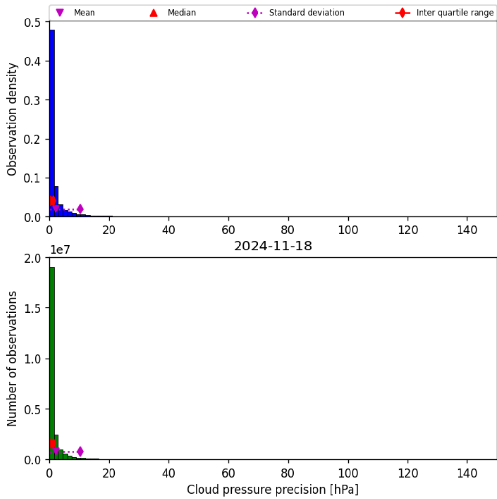
Figure 31: Histogram of “Cloud pressure precision” for 2024-11-17 to 2024-11-19
