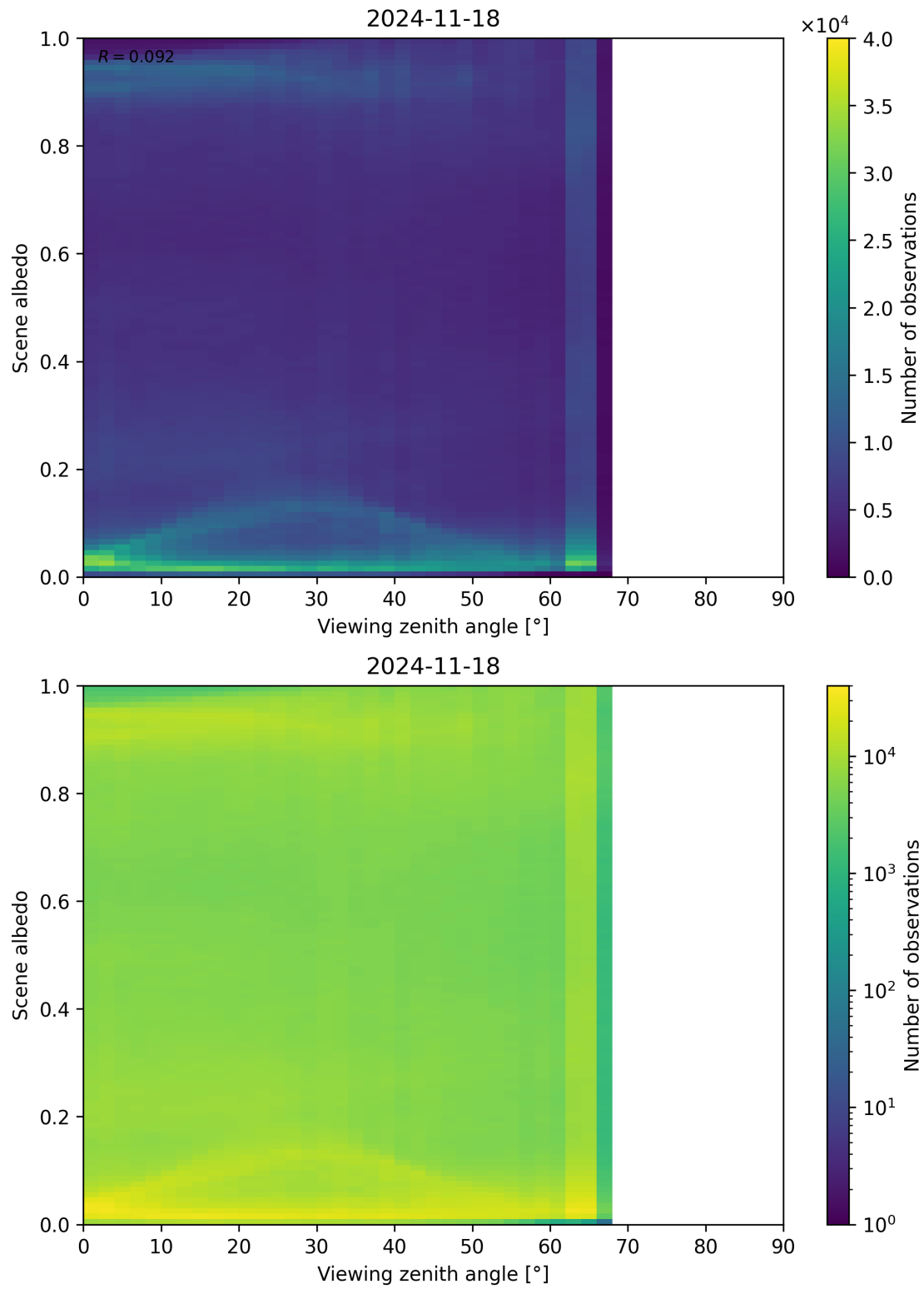
Figure 126: Scatter density plot of “Viewing zenith angle” against “Scene albedo” for 2024-11-17 to 2024-11-19.
