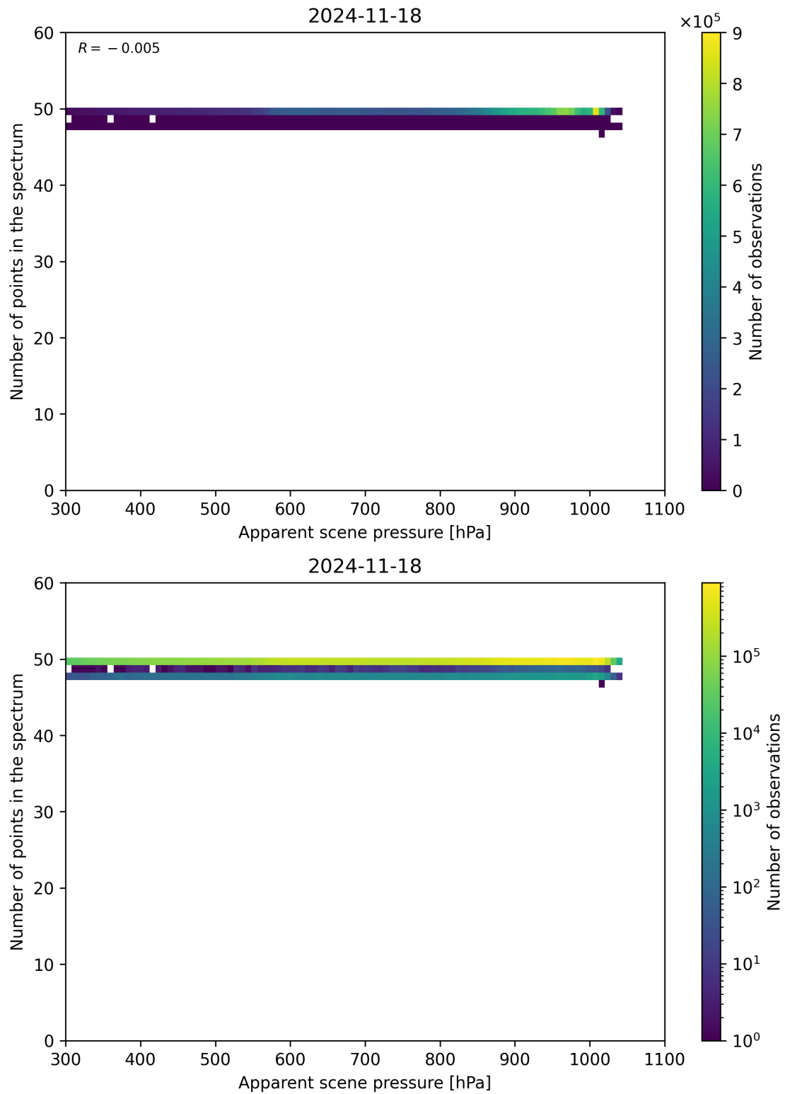
Figure 66: Scatter density plot of “Apparent scene pressure” against “Number of points in the spectrum” for 2024-11-17 to 2024-11-19.
