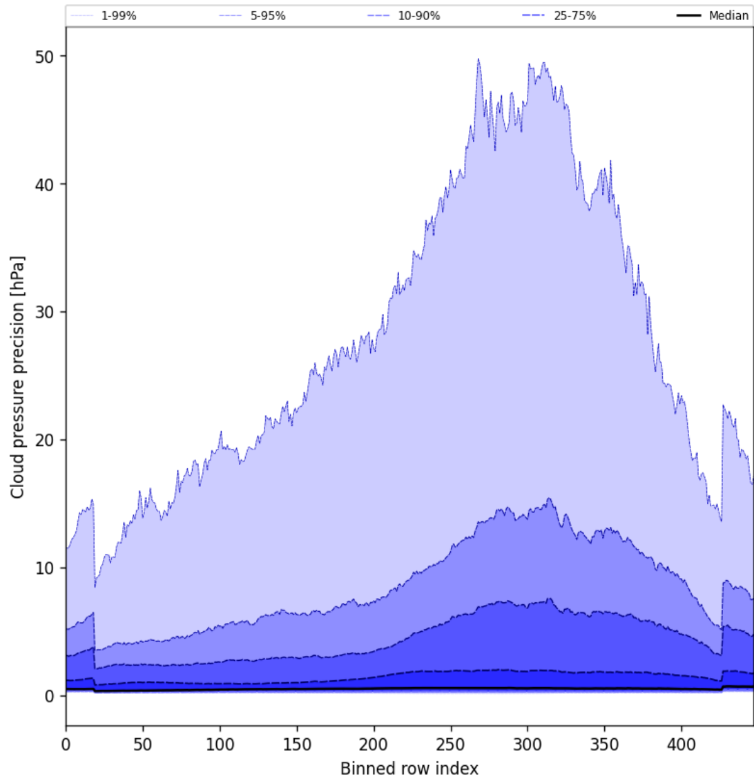
Figure 48: Along track statistics of “Cloud pressure precision” for 2024-11-17 to 2024-11-19
