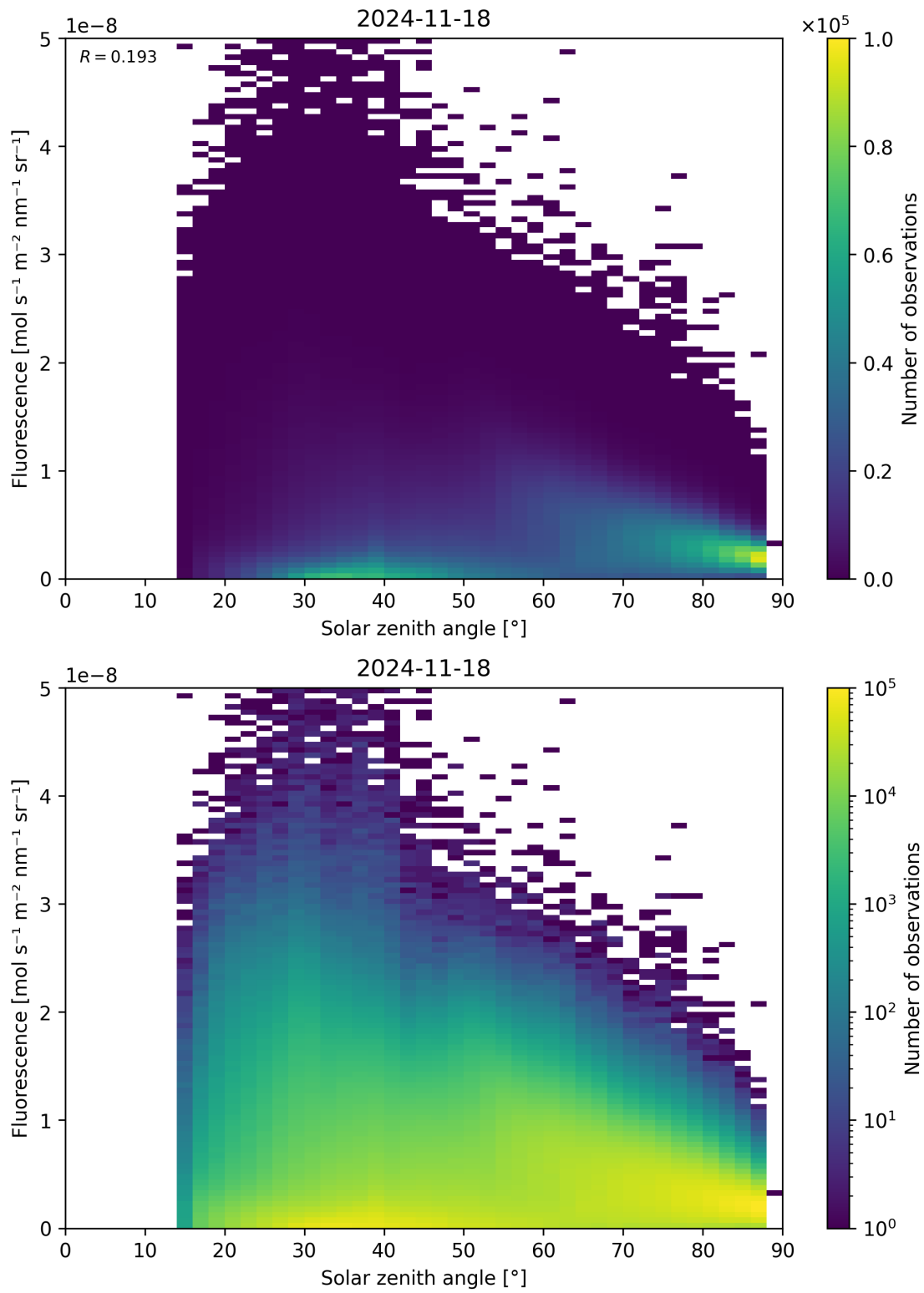
Figure 112: Scatter density plot of “Solar zenith angle” against “Fluorescence” for 2024-11-17 to 2024-11-19.
