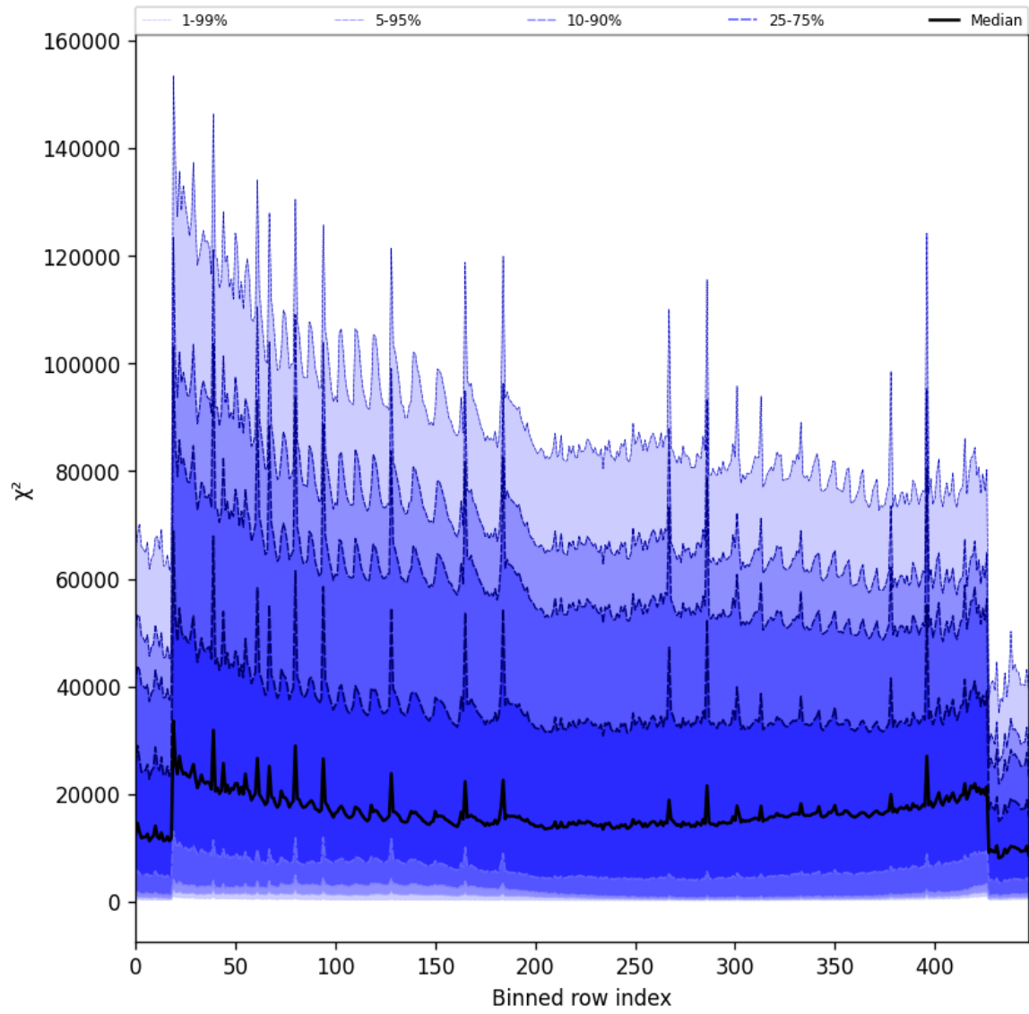
Figure 55: Along track statistics of “ \chi^2 ” for 2024-11-17 to 2024-11-19
