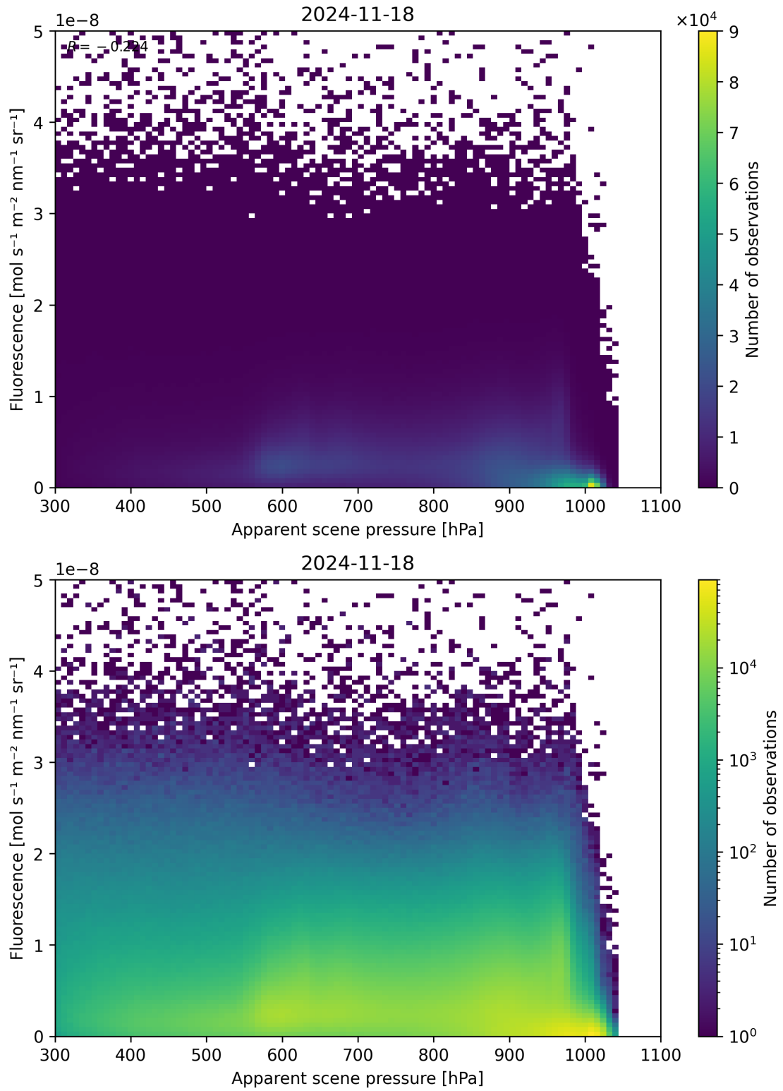
Figure 64: Scatter density plot of “Apparent scene pressure” against “Fluorescence” for 2024-11-17 to 2024-11-19.
