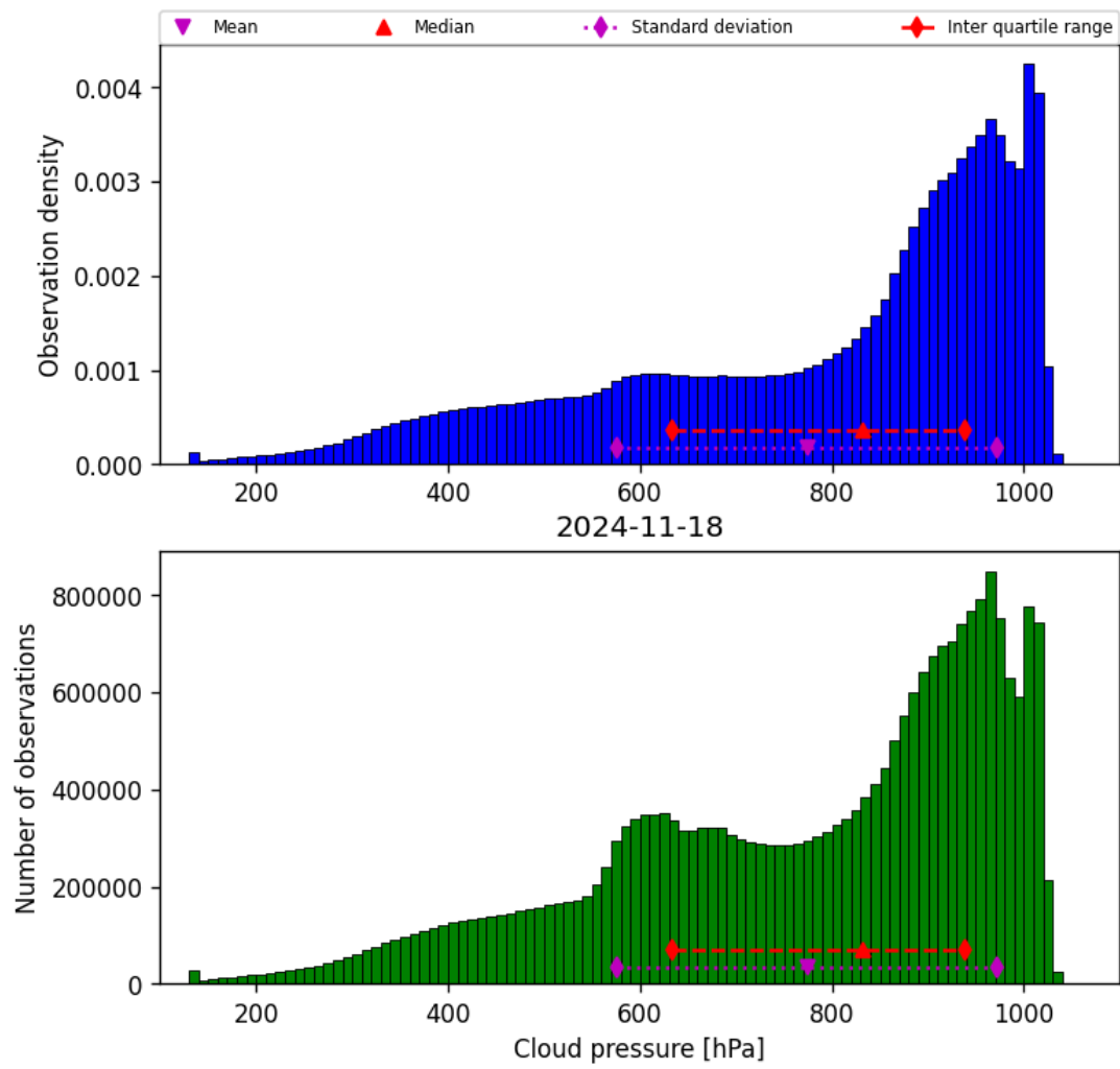
Figure 30: Histogram of “Cloud pressure” for 2024-11-17 to 2024-11-19
