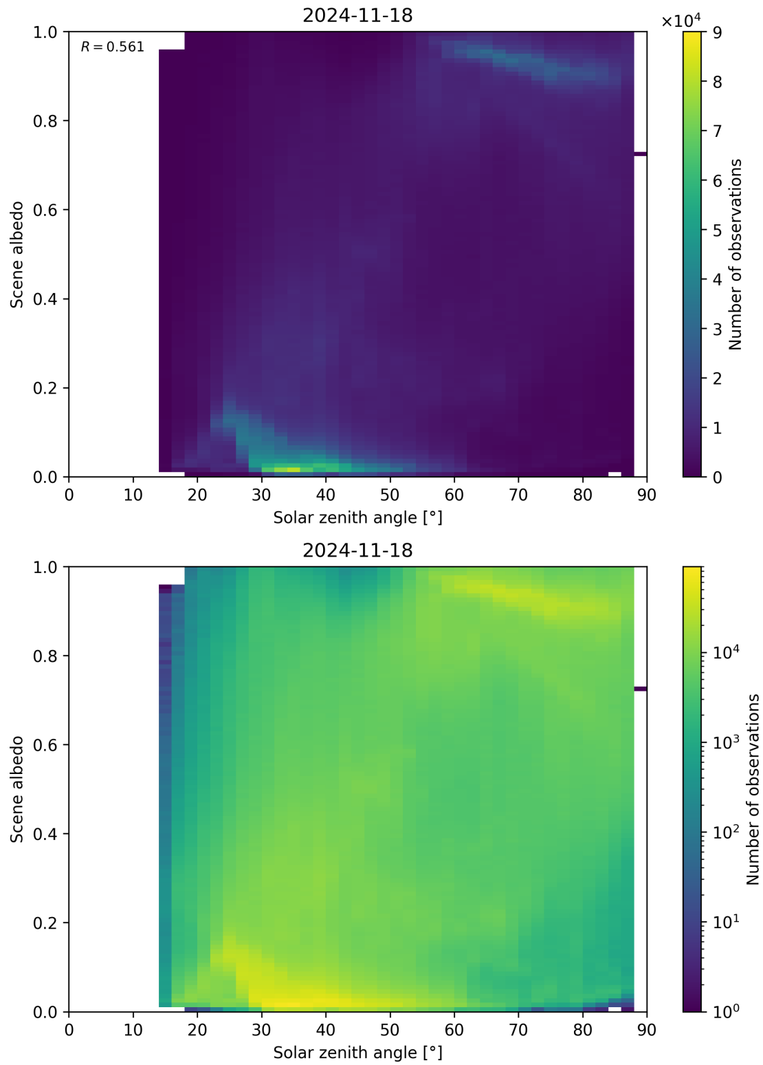
Figure 116: Scatter density plot of “Solar zenith angle” against “Scene albedo” for 2024-11-17 to 2024-11-19.
