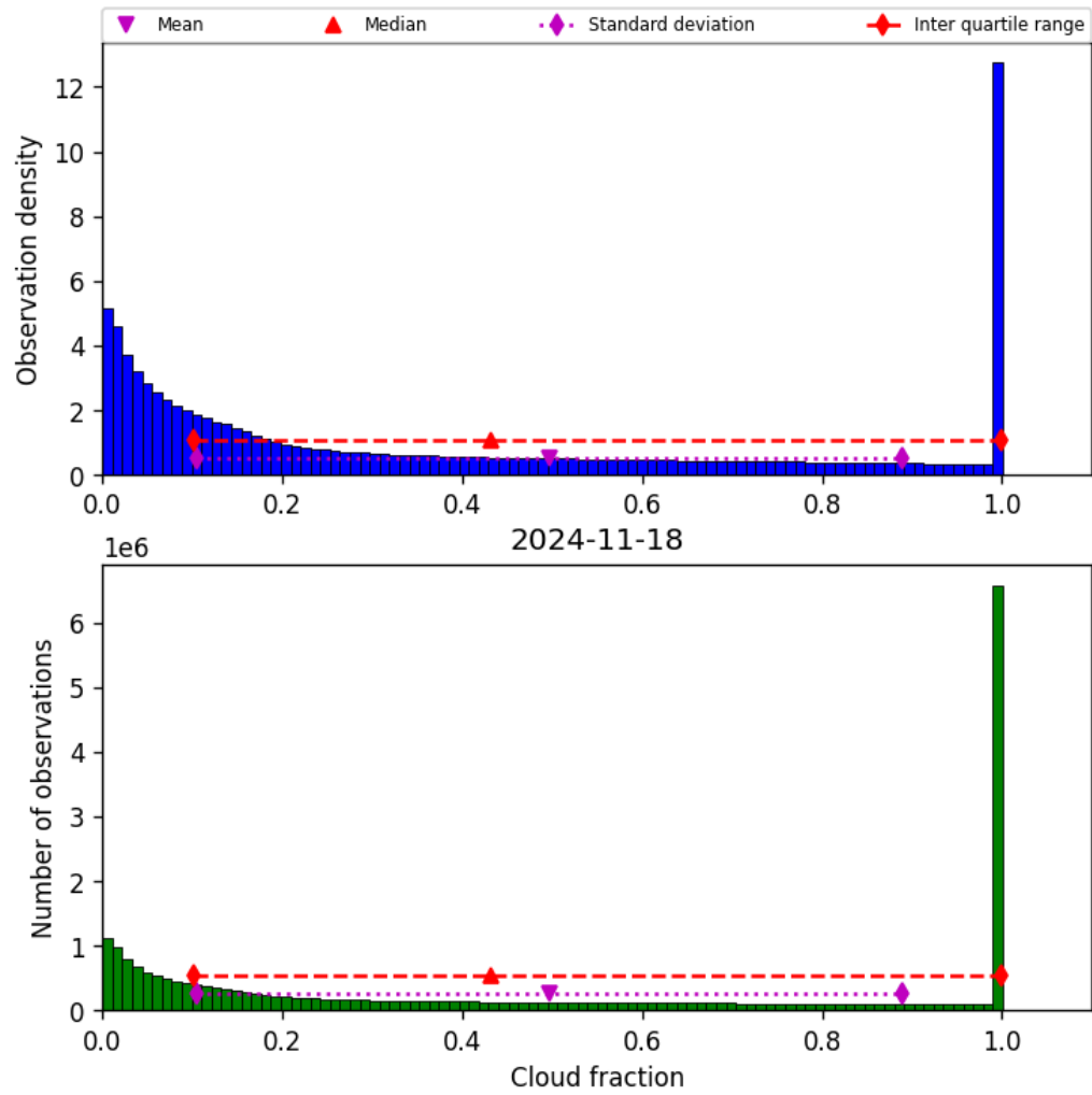
Figure 32: Histogram of "Cloud fraction" for 2024-11-17 to 2024-11-19
