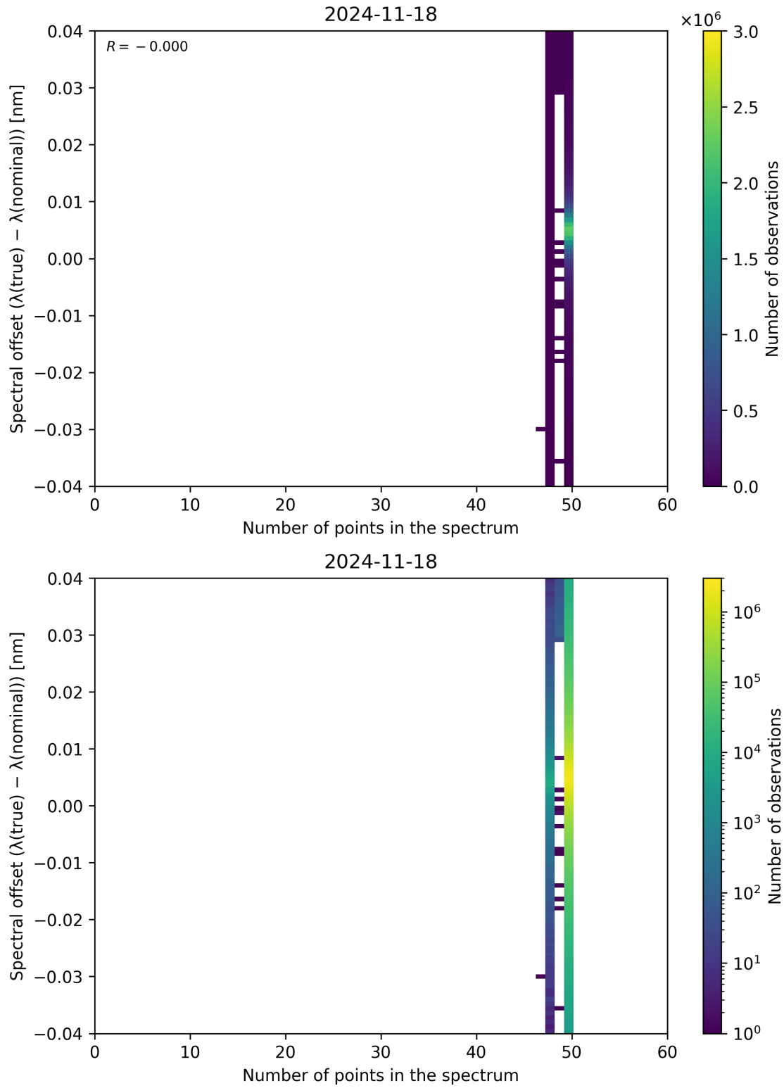
Figure 101: Scatter density plot of “Number of points in the spectrum” against “Spectral offset ( \lambda_{\text{true}} - \lambda_{\text{nominal}} )” for 2024-11-17 to 2024-11-19.
