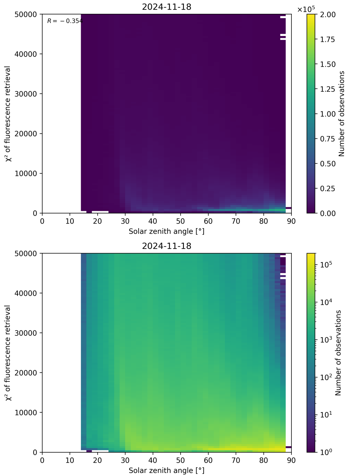
Figure 109: Scatter density plot of “Solar zenith angle” against “ \chi^2 of fluorescence retrieval” for 2024-11-17 to 2024-11-19.
