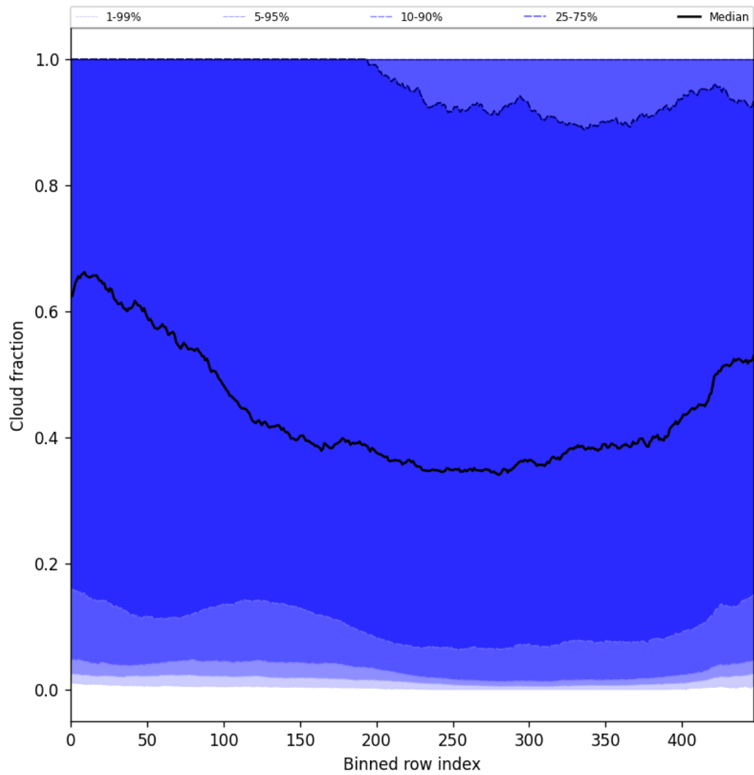
Figure 49: Along track statistics of “Cloud fraction” for 2024-11-17 to 2024-11-19
