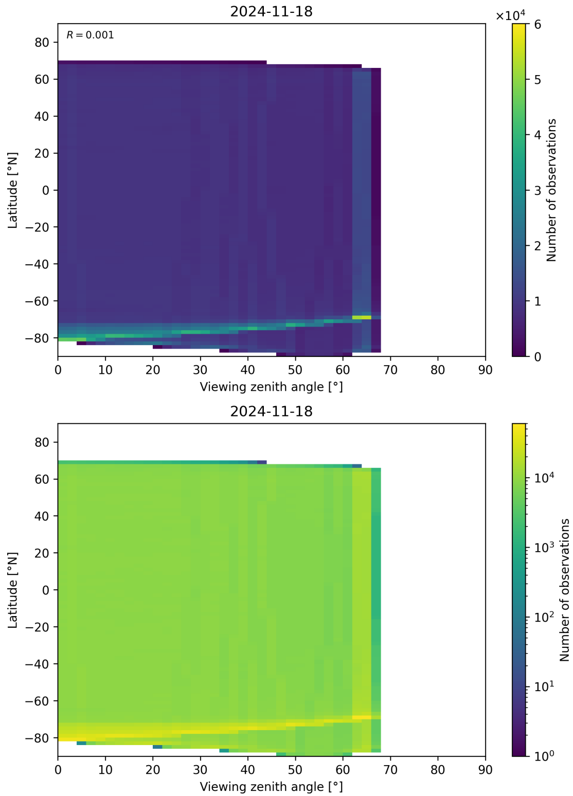
Figure 123: Scatter density plot of “Viewing zenith angle” against “Latitude” for 2024-11-17 to 2024-11-19.
