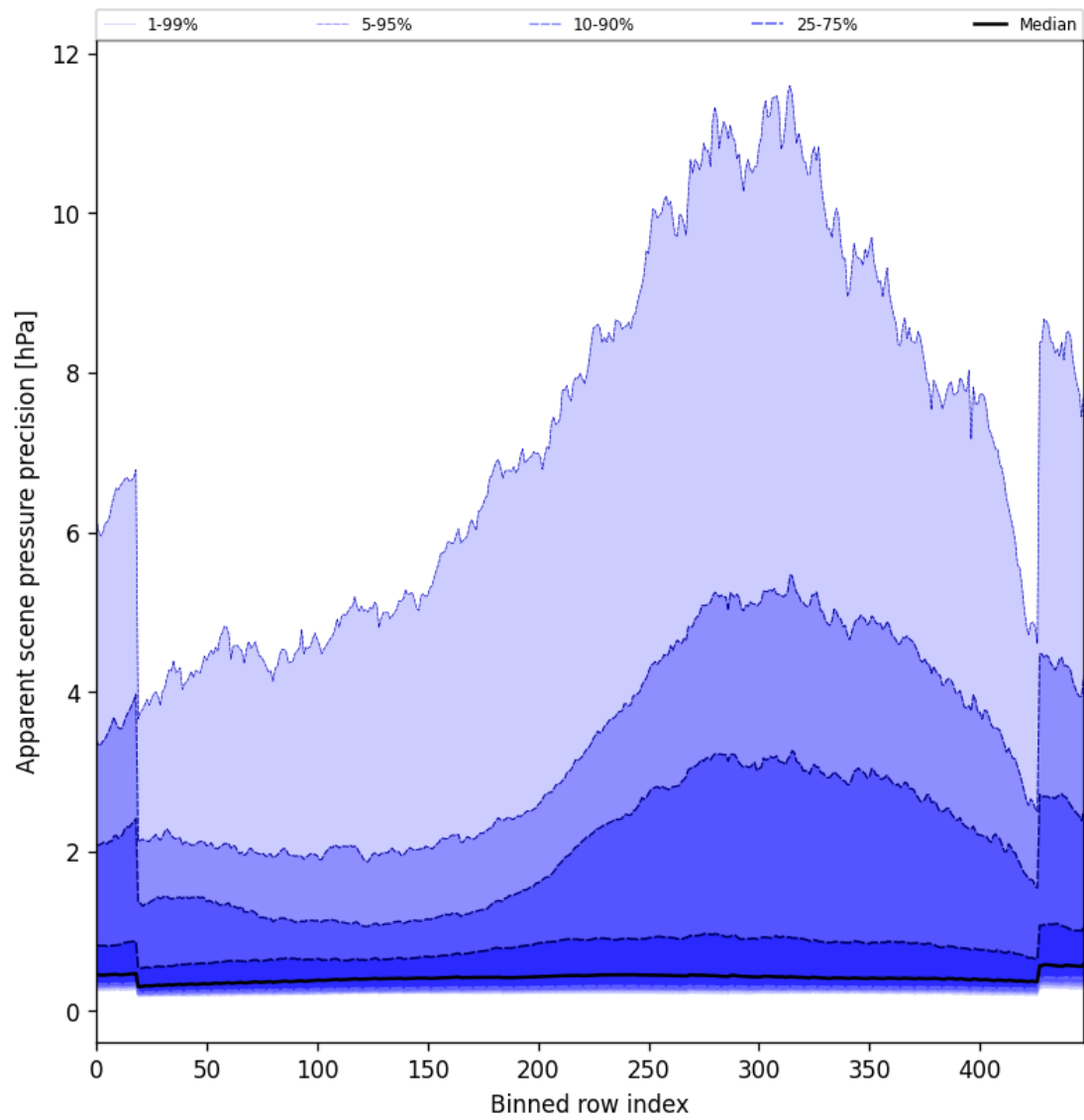
Figure 54: Along track statistics of “Apparent scene pressure precision” for 2024-11-17 to 2024-11-19
