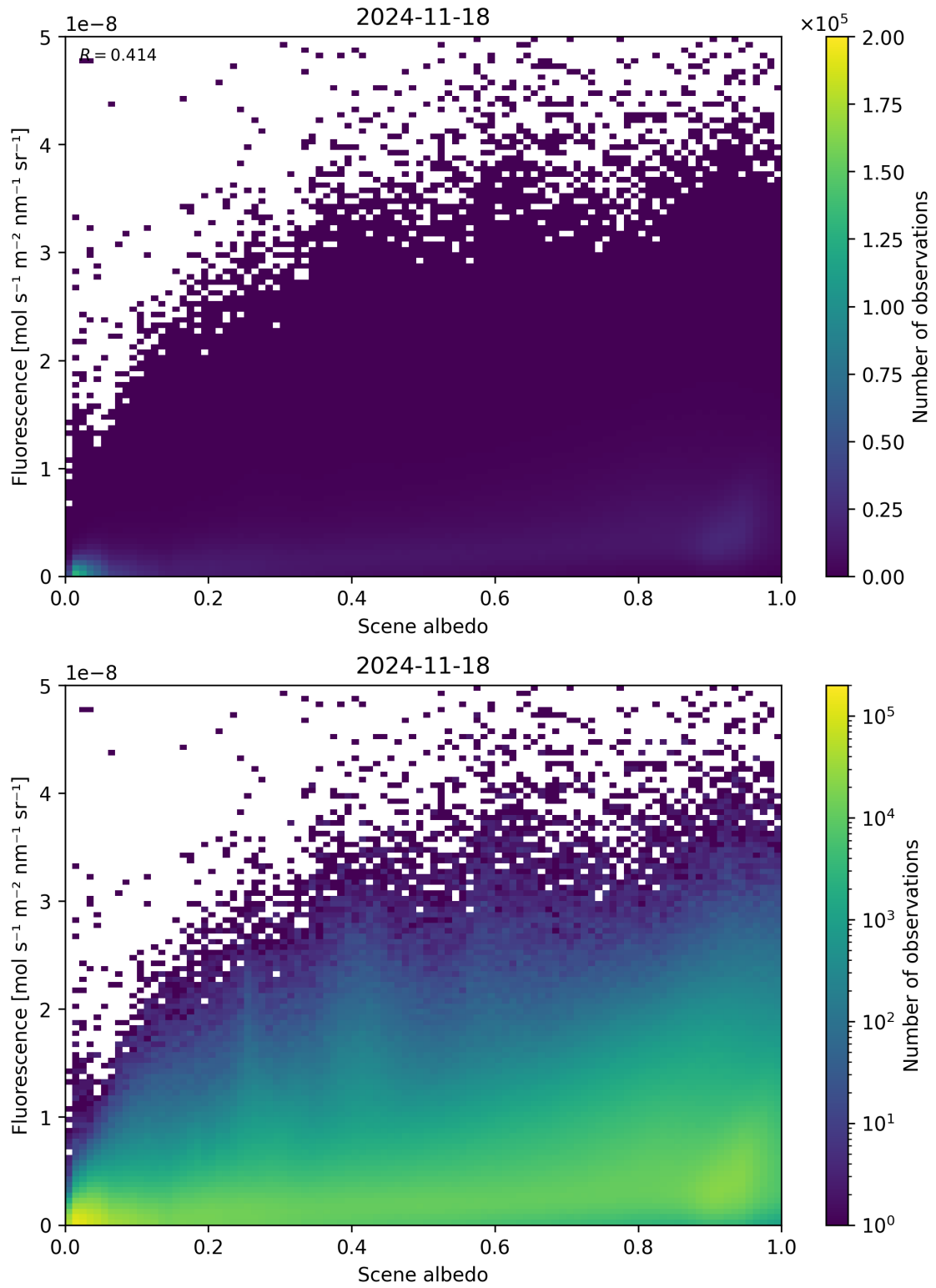
Figure 104: Scatter density plot of “Scene albedo” against “Fluorescence” for 2024-11-17 to 2024-11-19.
