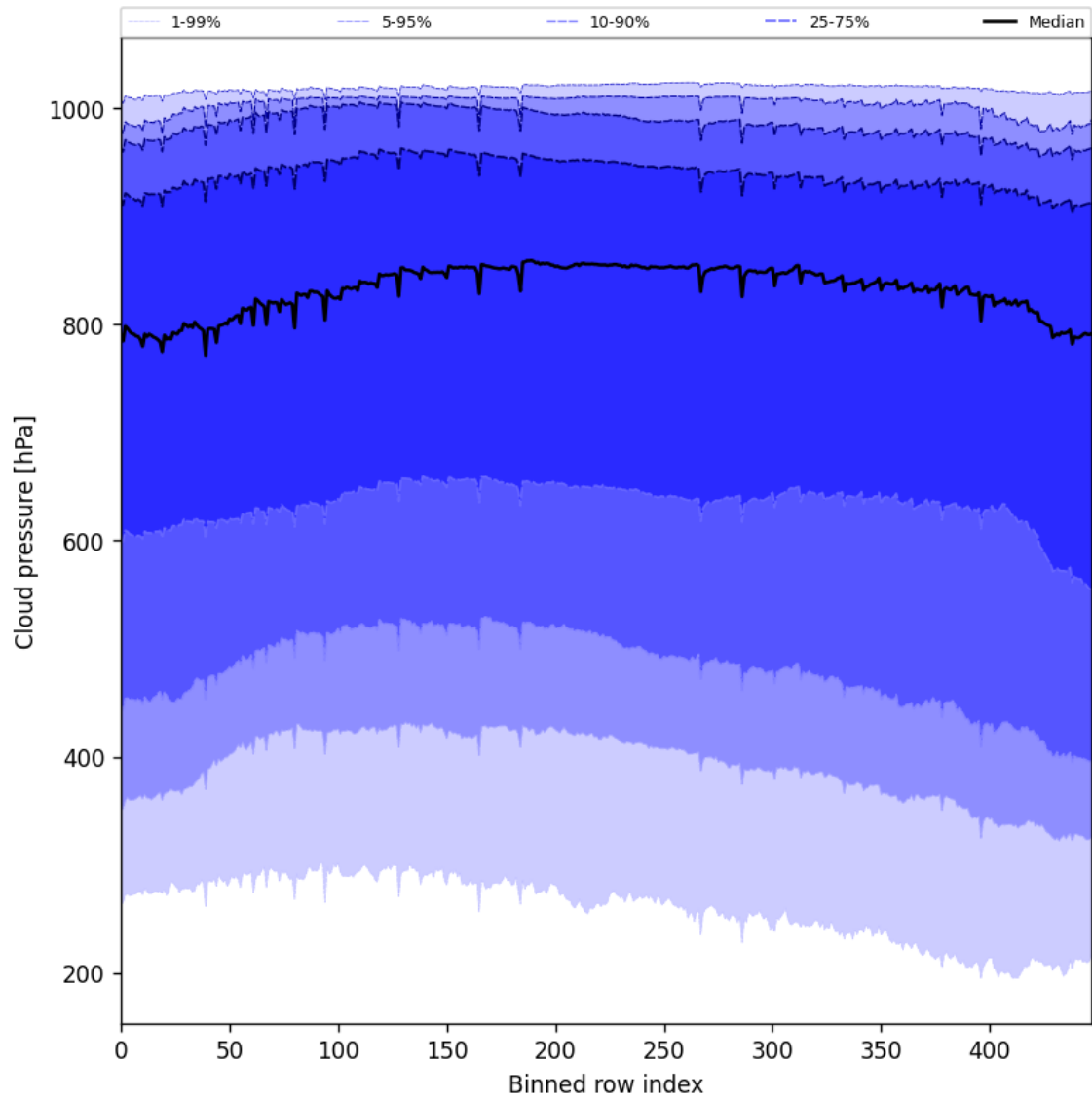
Figure 47: Along track statistics of “Cloud pressure” for 2024-11-17 to 2024-11-19
