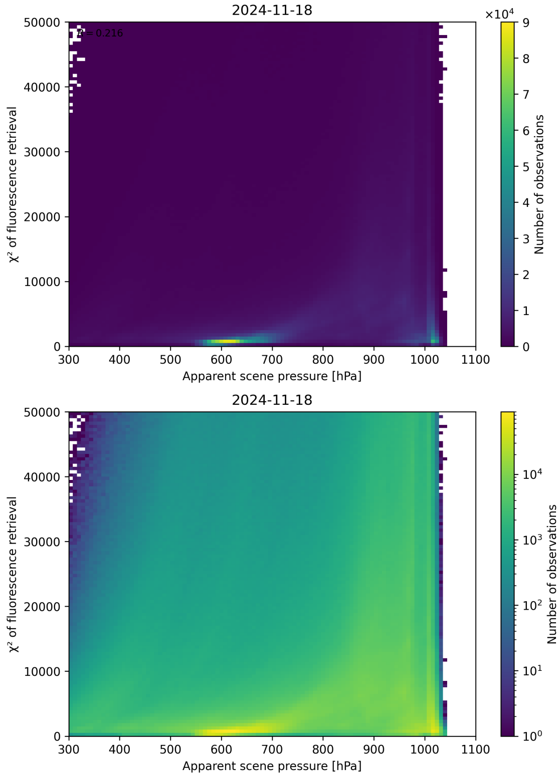
Figure 63: Scatter density plot of “Apparent scene pressure” against “ \chi^2 of fluorescence retrieval” for 2024-11-17 to 2024-11-19.
