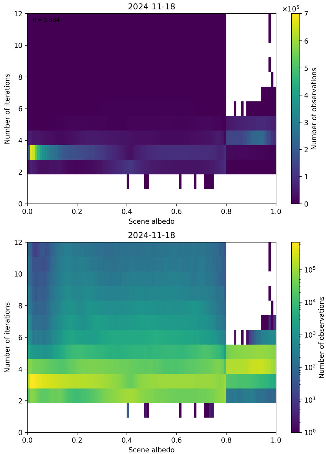
Figure 105: Scatter density plot of “Scene albedo” against “Number of iterations” for 2024-11-17 to 2024-11-19.
