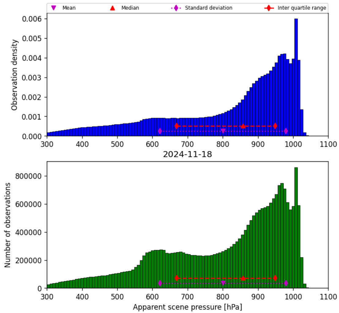
Figure 36: Histogram of “Apparent scene pressure” for 2024-11-17 to 2024-11-19
