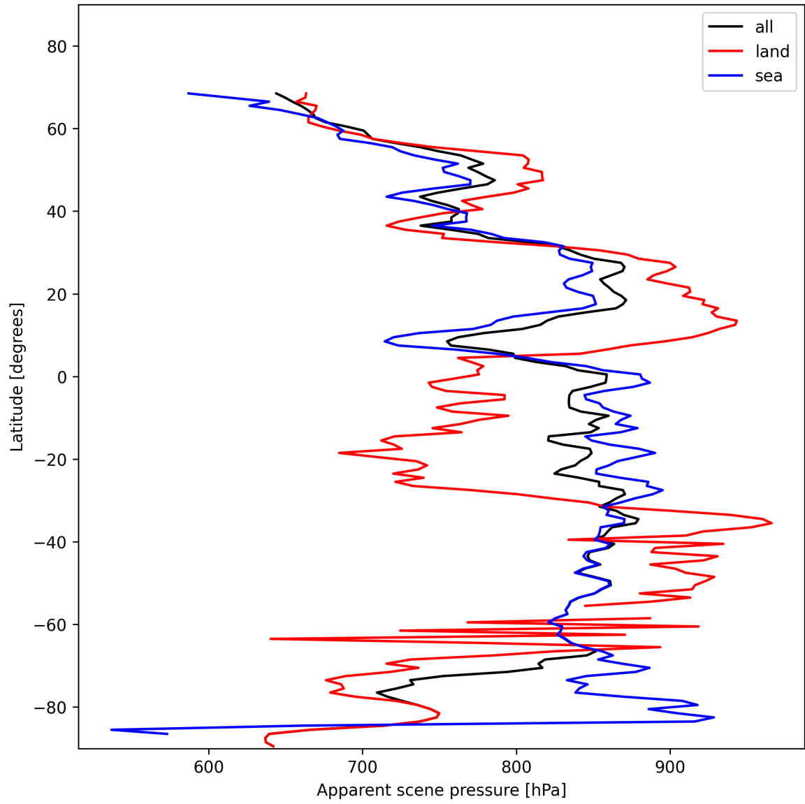
Figure 19: Zonal average of “Apparent scene pressure” for 2024-11-17 to 2024-11-19.
