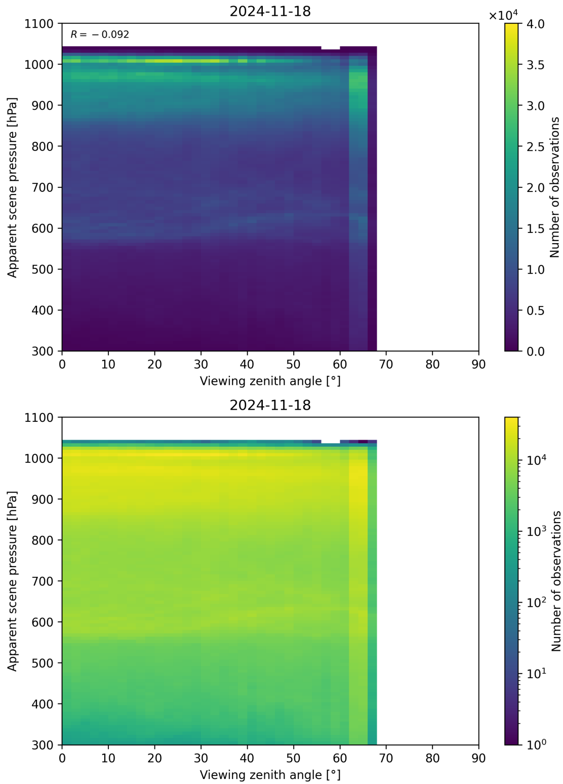
Figure 118: Scatter density plot of “Viewing zenith angle” against “Apparent scene pressure” for 2024-11-17 to 2024-11-19.
