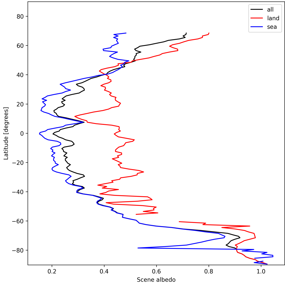
Figure 17: Zonal average of “Scene albedo” for 2024-11-18 to 2024-11-20.
