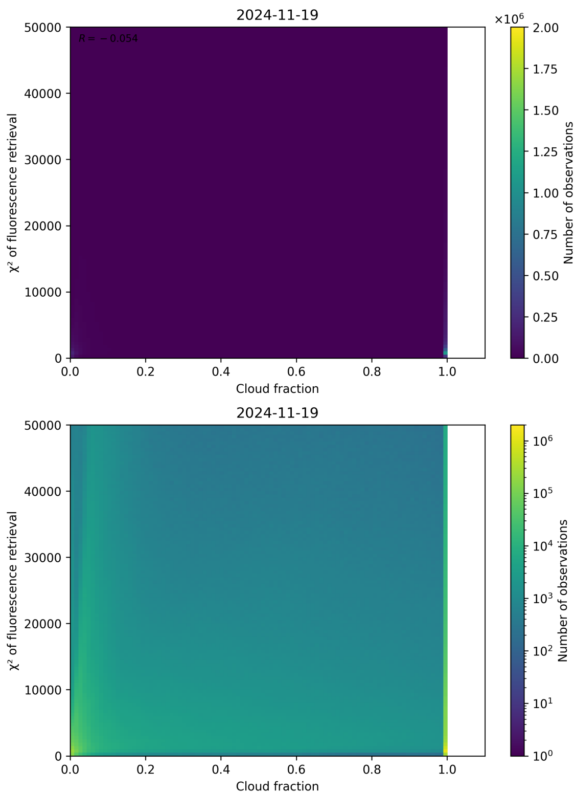
Figure 71: Scatter density plot of “Cloud fraction” against “ \chi^2 of fluorescence retrieval” for 2024-11-18 to 2024-11-20.
