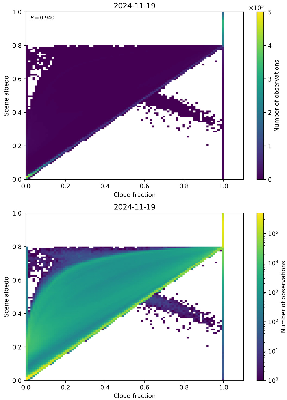
Figure 75: Scatter density plot of “Cloud fraction” against “Scene albedo” for 2024-11-18 to 2024-11-20.
