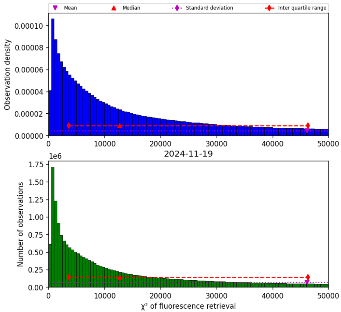
Figure 42: Histogram of “ \chi^2 of fluorescence retrieval” for 2024-11-18 to 2024-11-20
