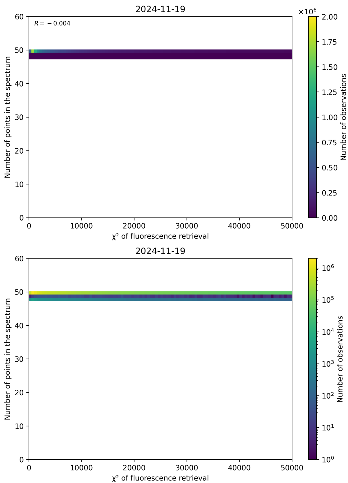
Figure 68: Scatter density plot of " \chi^2 of fluorescence retrieval" against "Number of points in the spectrum" for 2024-11-18 to 2024-11-20.
