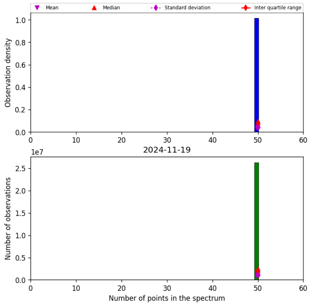
Figure 44: Histogram of “Number of points in the spectrum” for 2024-11-18 to 2024-11-20
