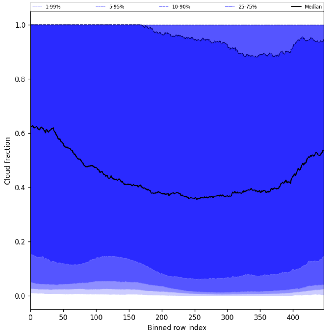
Figure 49: Along track statistics of “Cloud fraction” for 2024-11-18 to 2024-11-20
