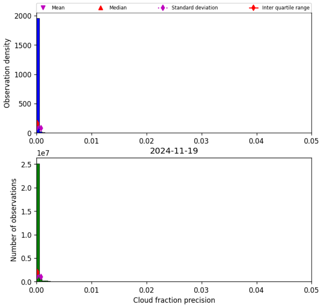
Figure 33: Histogram of “Cloud fraction precision” for 2024-11-18 to 2024-11-20
