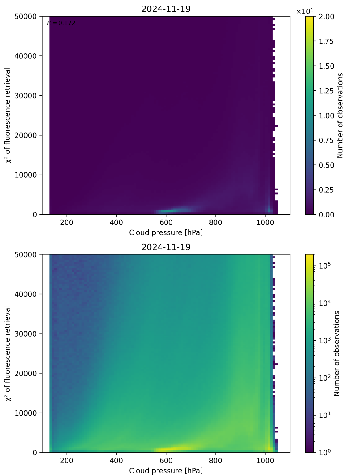
Figure 78: Scatter density plot of “Cloud pressure” against “ \chi^2 of fluorescence retrieval” for 2024-11-18 to 2024-11-20.
