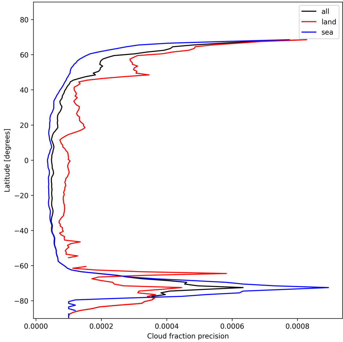
Figure 16: Zonal average of “Cloud fraction precision” for 2024-11-18 to 2024-11-20.
