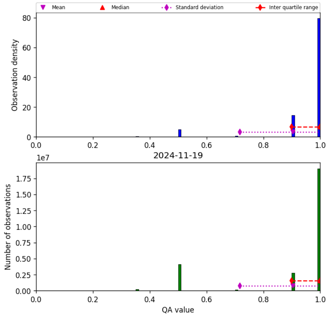
Figure 29: Histogram of “QA value” for 2024-11-18 to 2024-11-20
