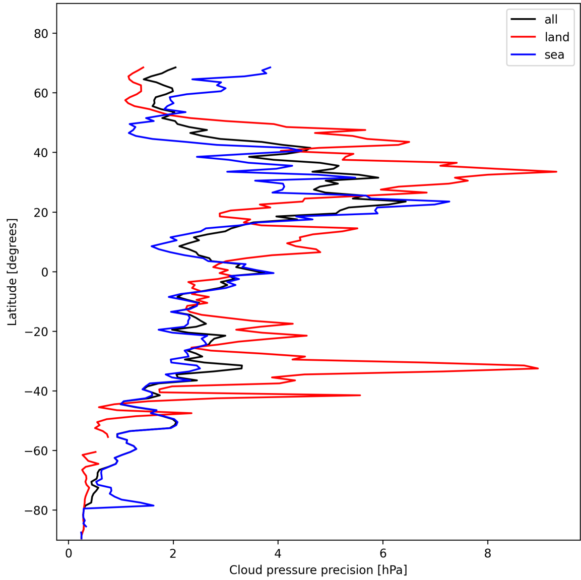
Figure 14: Zonal average of “Cloud pressure precision” for 2024-11-18 to 2024-11-20.
