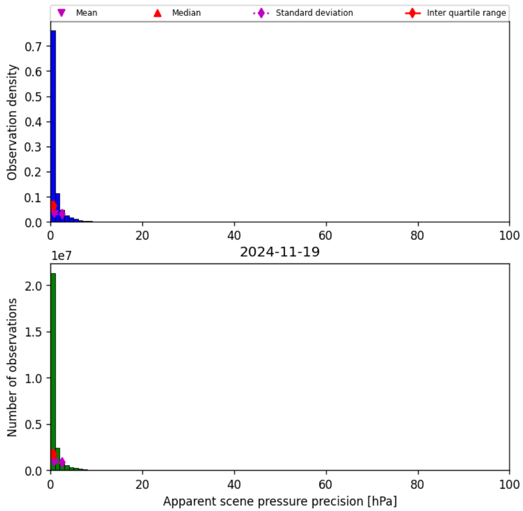
Figure 37: Histogram of “Apparent scene pressure precision” for 2024-11-18 to 2024-11-20
