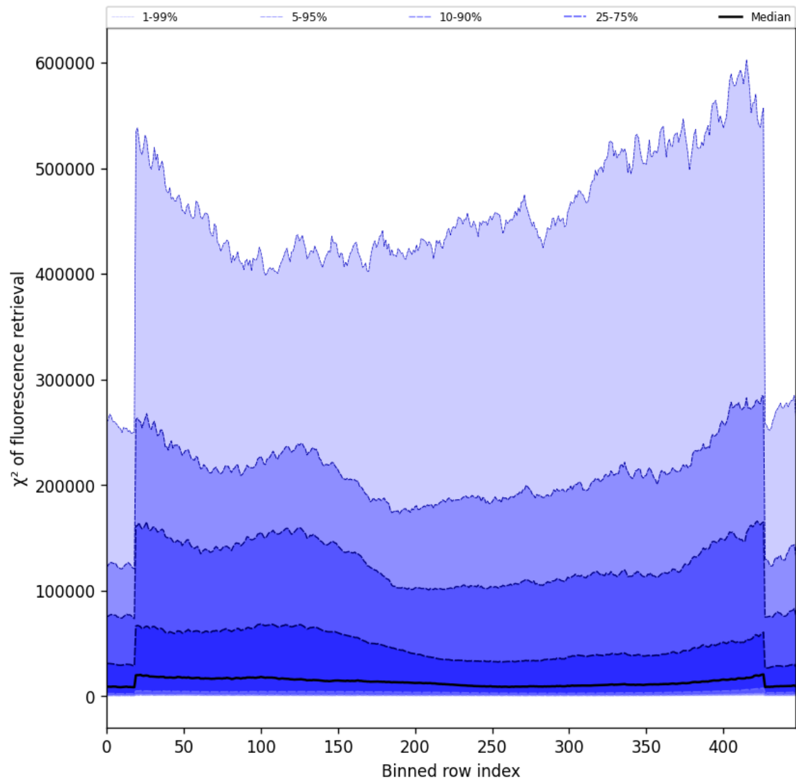
Figure 59: Along track statistics of “ \chi^2 of fluorescence retrieval” for 2024-11-18 to 2024-11-20
