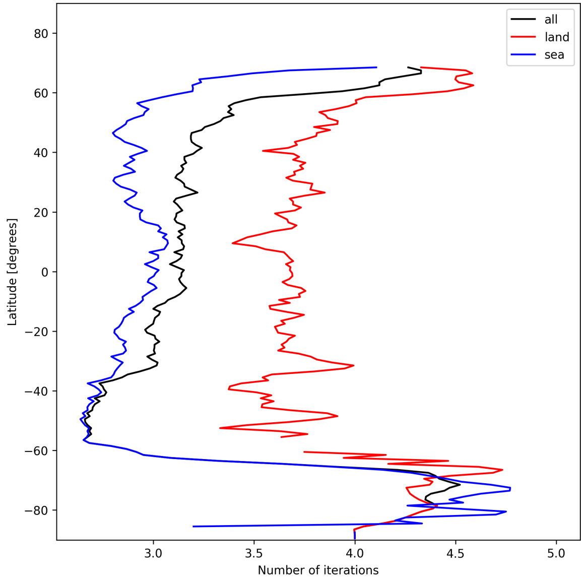
Figure 22: Zonal average of “Number of iterations” for 2024-11-18 to 2024-11-20.
