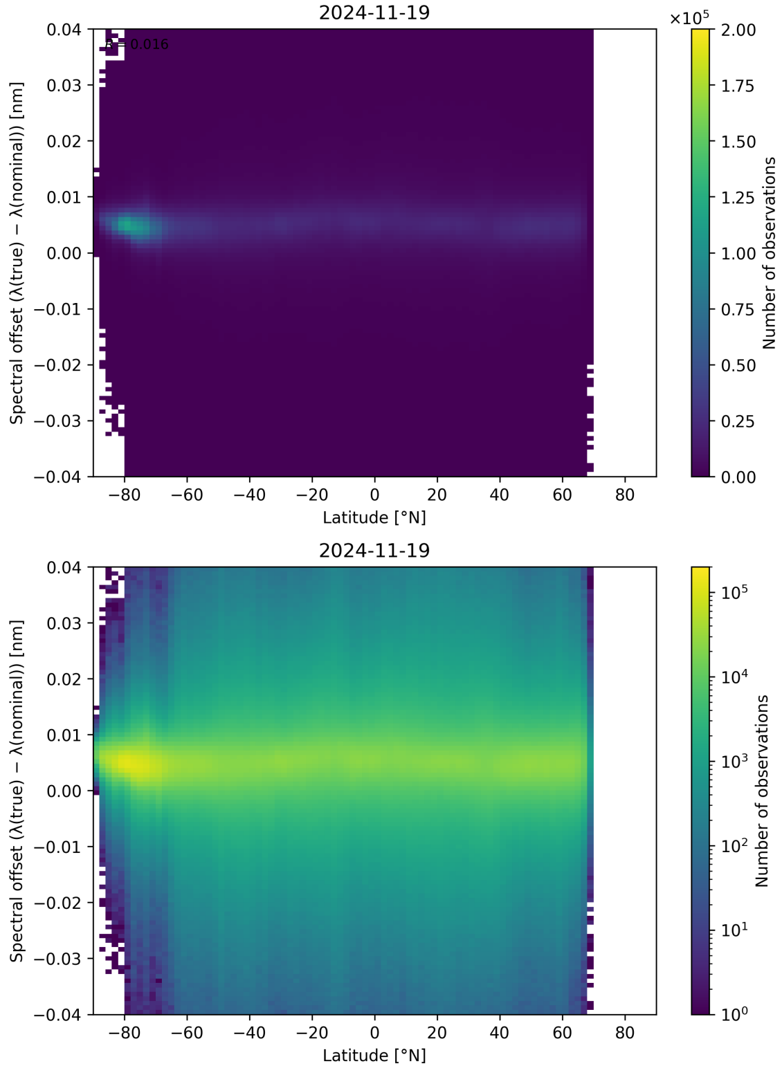
Figure 96: Scatter density plot of “Latitude” against “Spectral offset ( \lambda_{\text{true}} - \lambda_{\text{nominal}} )” for 2024-11-18 to 2024-11-20.
