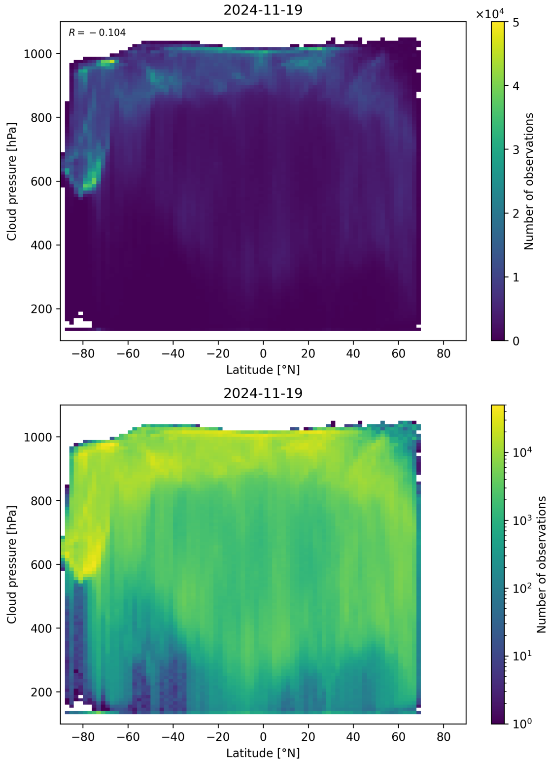
Figure 91: Scatter density plot of “Latitude” against “Cloud pressure” for 2024-11-18 to 2024-11-20.
