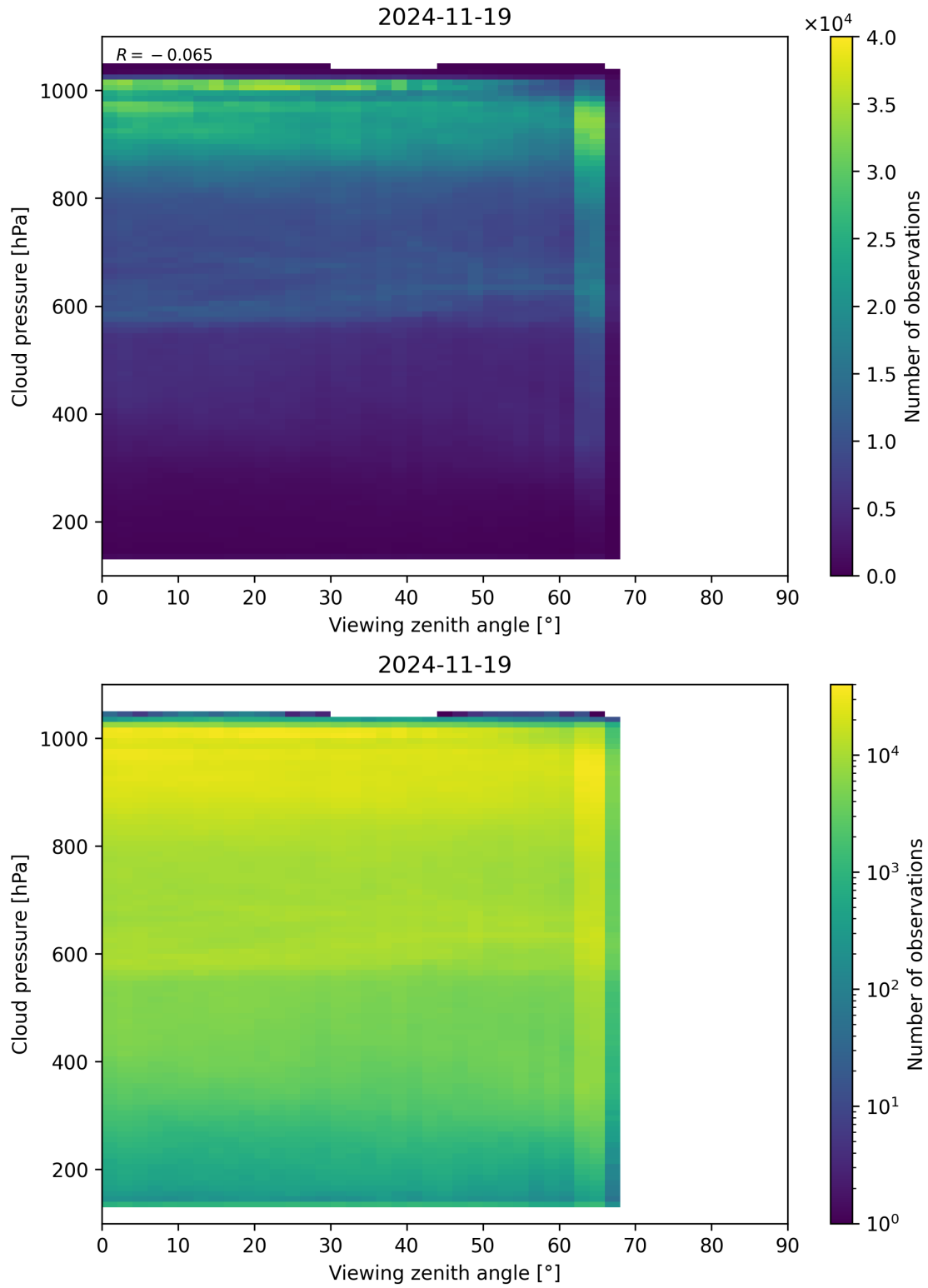
Figure 121: Scatter density plot of “Viewing zenith angle” against “Cloud pressure” for 2024-11-18 to 2024-11-20.
