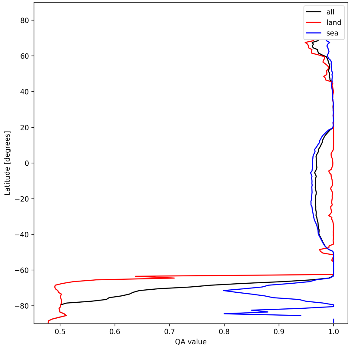
Figure 12: Zonal average of “QA value” for 2024-11-18 to 2024-11-20.
