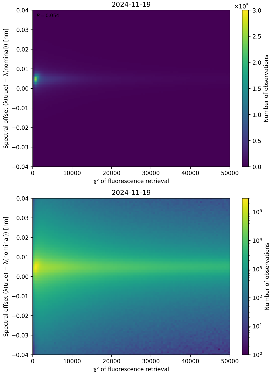
Figure 69: Scatter density plot of “ \chi^2 of fluorescence retrieval” against “Spectral offset ( \lambda_{\text{true}} - \lambda_{\text{nominal}} )” for 2024-11-18 to 2024-11-20.
