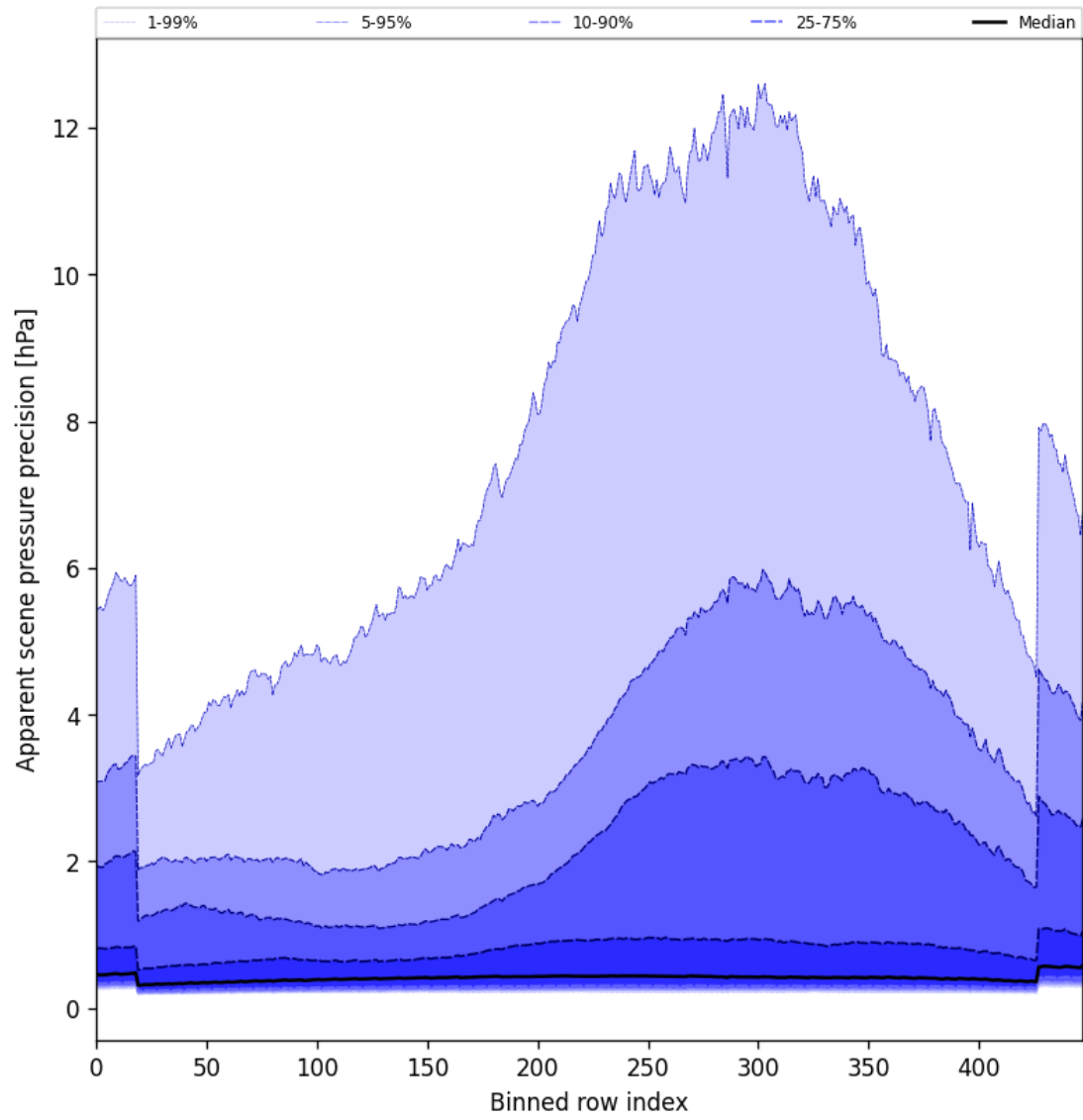
Figure 54: Along track statistics of “Apparent scene pressure precision” for 2024-11-18 to 2024-11-20
