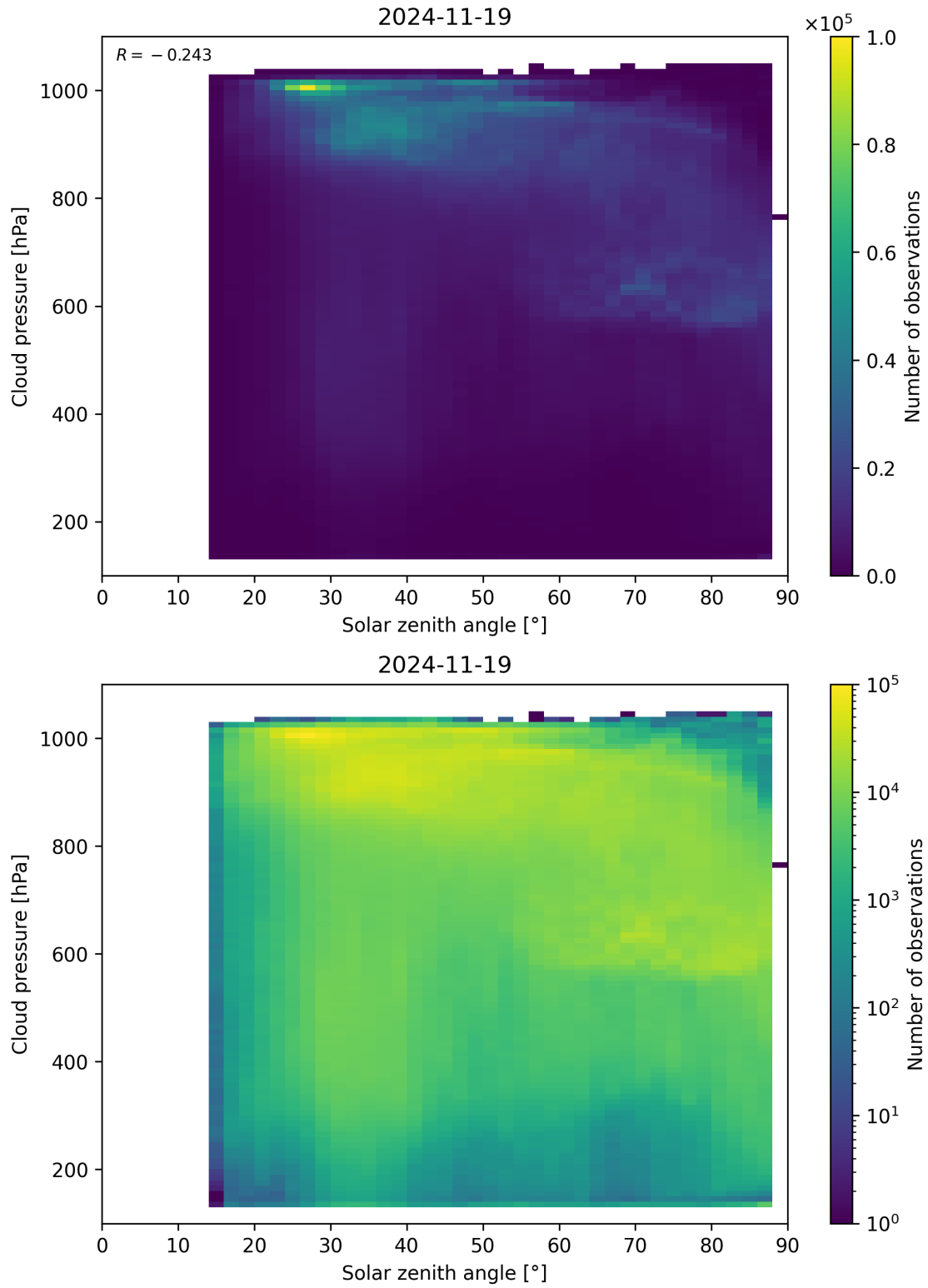
Figure 111: Scatter density plot of “Solar zenith angle” against “Cloud pressure” for 2024-11-18 to 2024-11-20.
