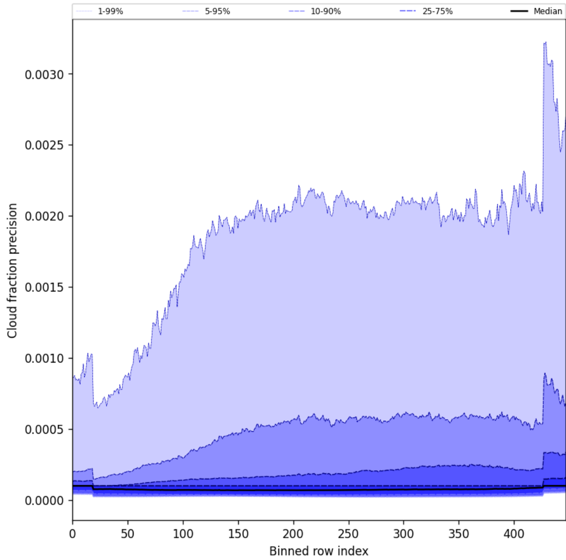
Figure 50: Along track statistics of “Cloud fraction precision” for 2024-11-18 to 2024-11-20
