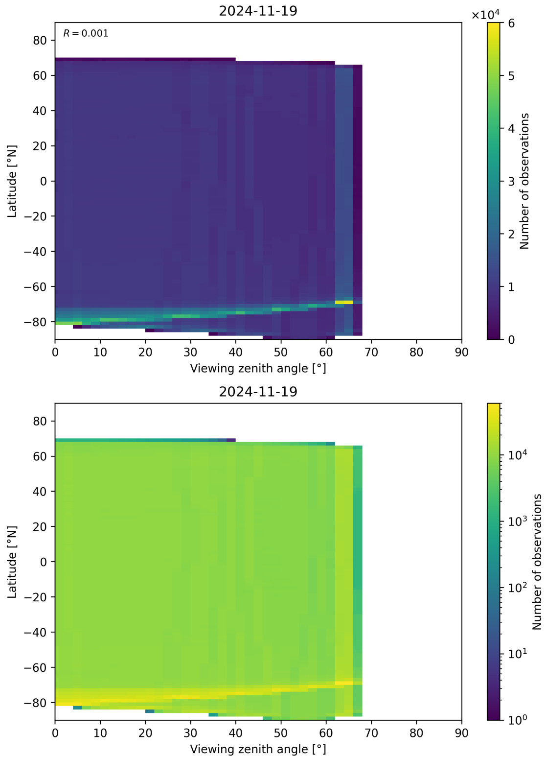
Figure 123: Scatter density plot of “Viewing zenith angle” against “Latitude” for 2024-11-18 to 2024-11-20.
