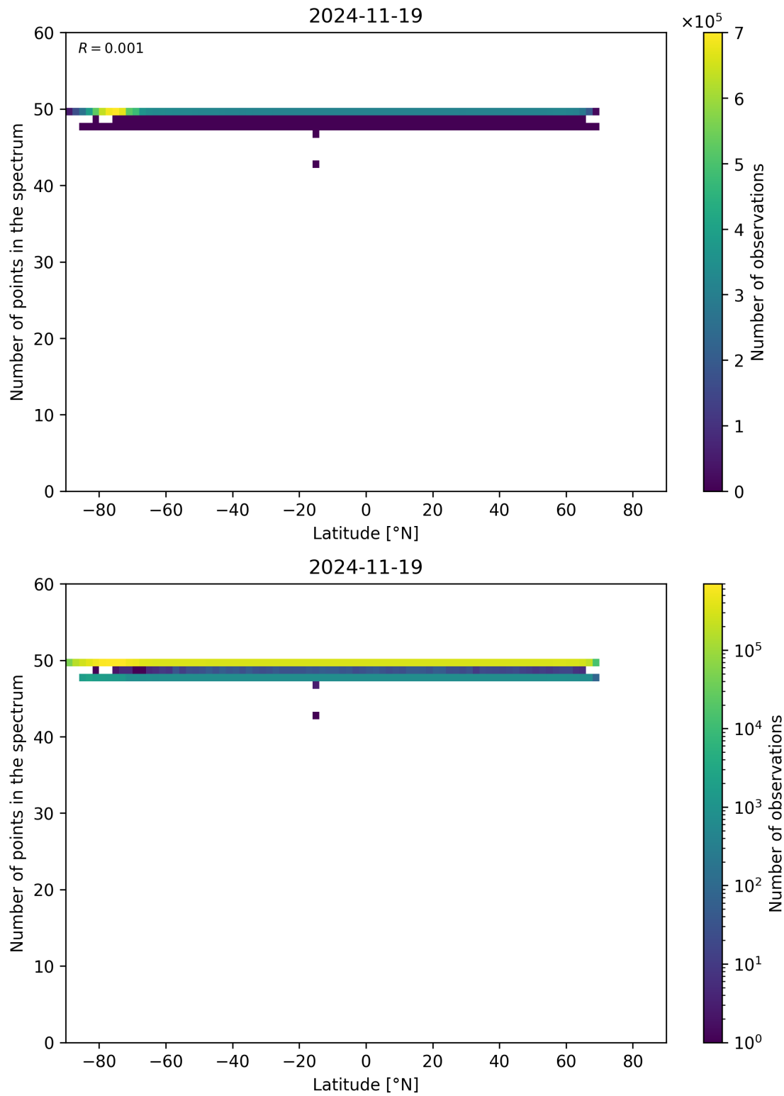
Figure 94: Scatter density plot of “Latitude” against “Number of points in the spectrum” for 2024-11-18 to 2024-11-20.
