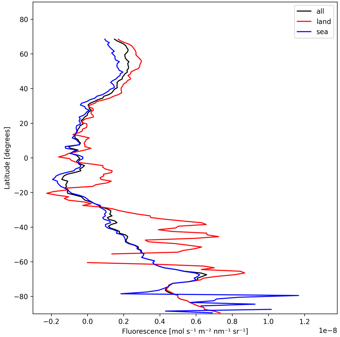
Figure 23: Zonal average of “Fluorescence” for 2024-11-18 to 2024-11-20.
