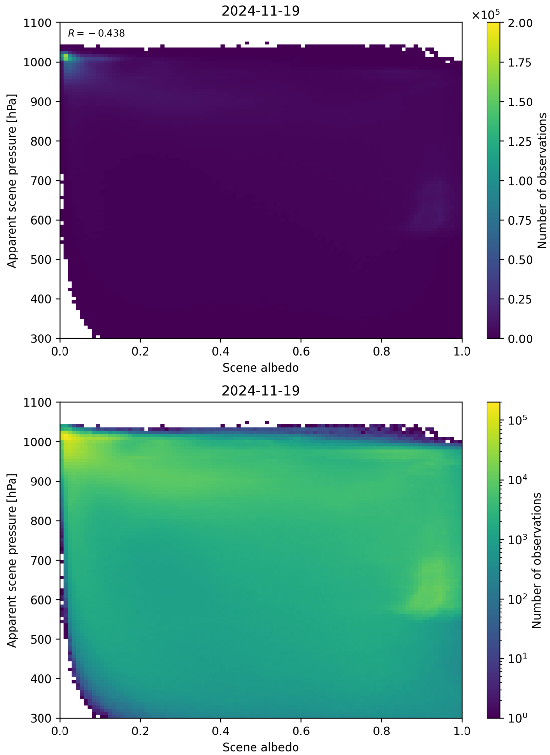
Figure 102: Scatter density plot of “Scene albedo” against “Apparent scene pressure” for 2024-11-18 to 2024-11-20.
