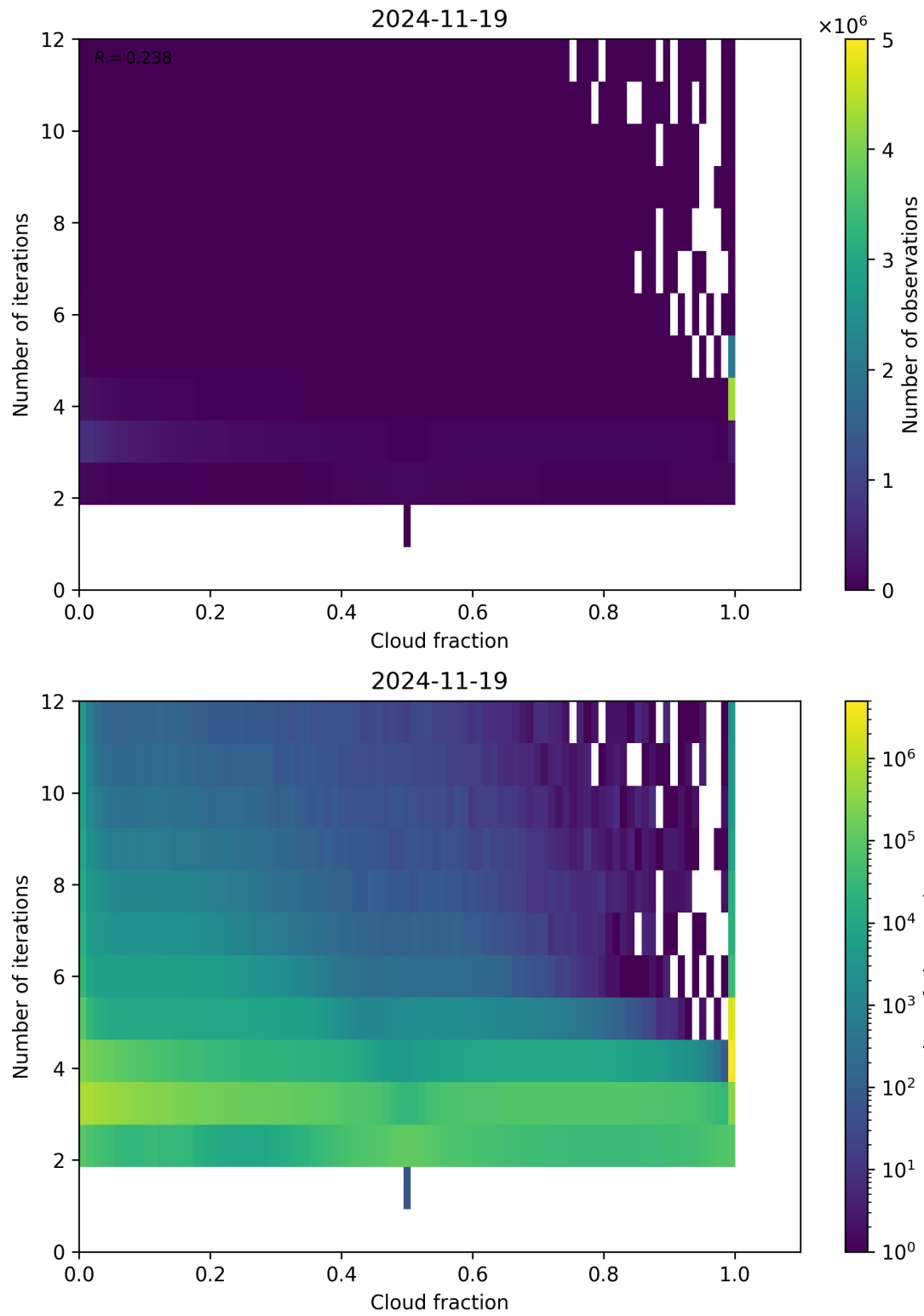
Figure 73: Scatter density plot of “Cloud fraction” against “Number of iterations” for 2024-11-18 to 2024-11-20.
