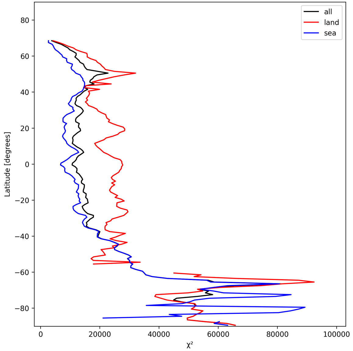
Figure 21: Zonal average of “ \chi^2 ” for 2024-11-18 to 2024-11-20.
