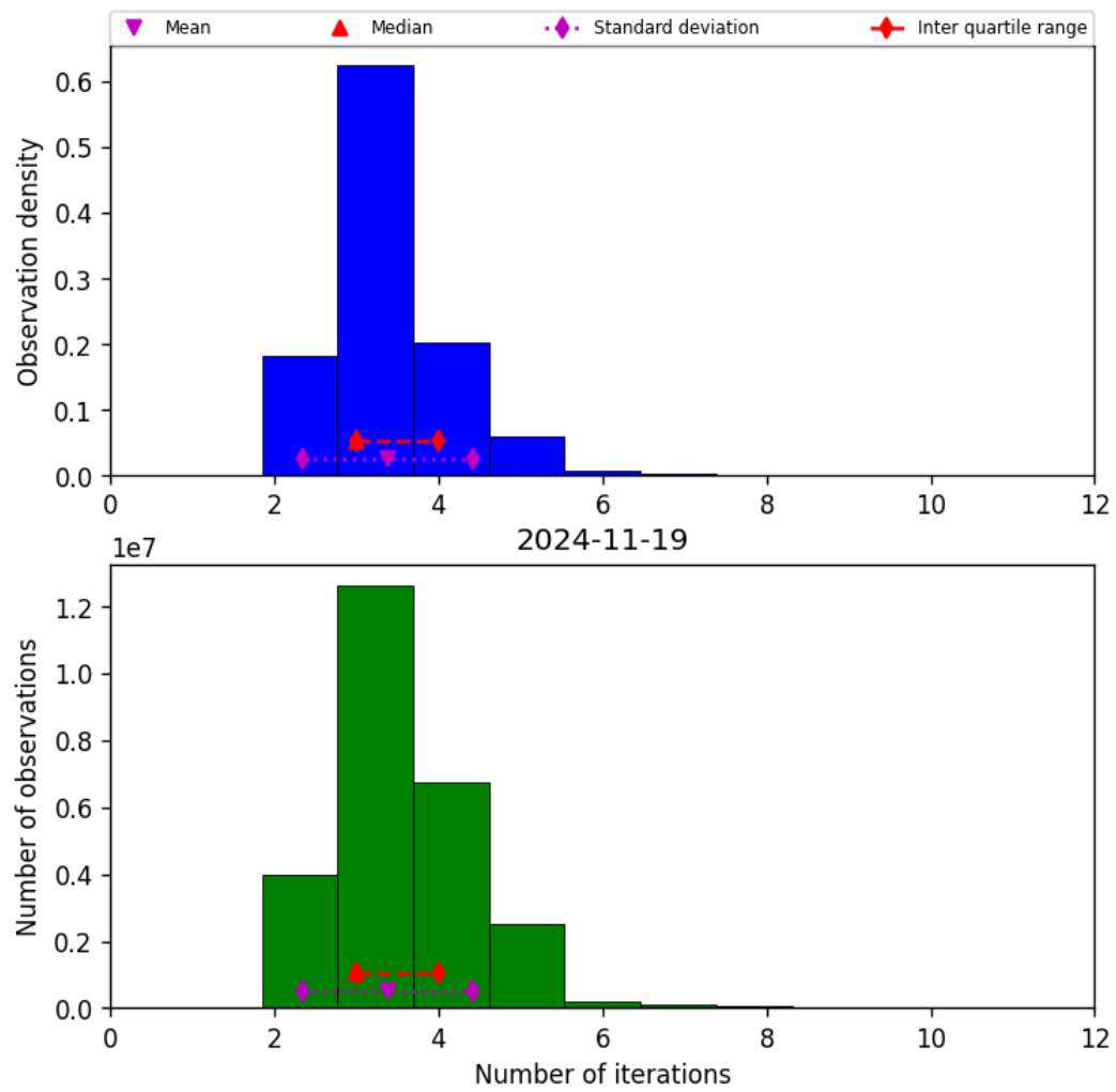
Figure 39: Histogram of “Number of iterations” for 2024-11-18 to 2024-11-20
