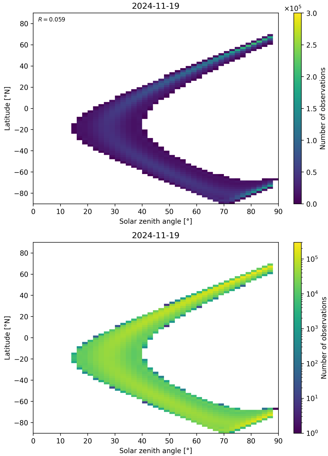
Figure 113: Scatter density plot of “Solar zenith angle” against “Latitude” for 2024-11-18 to 2024-11-20.
