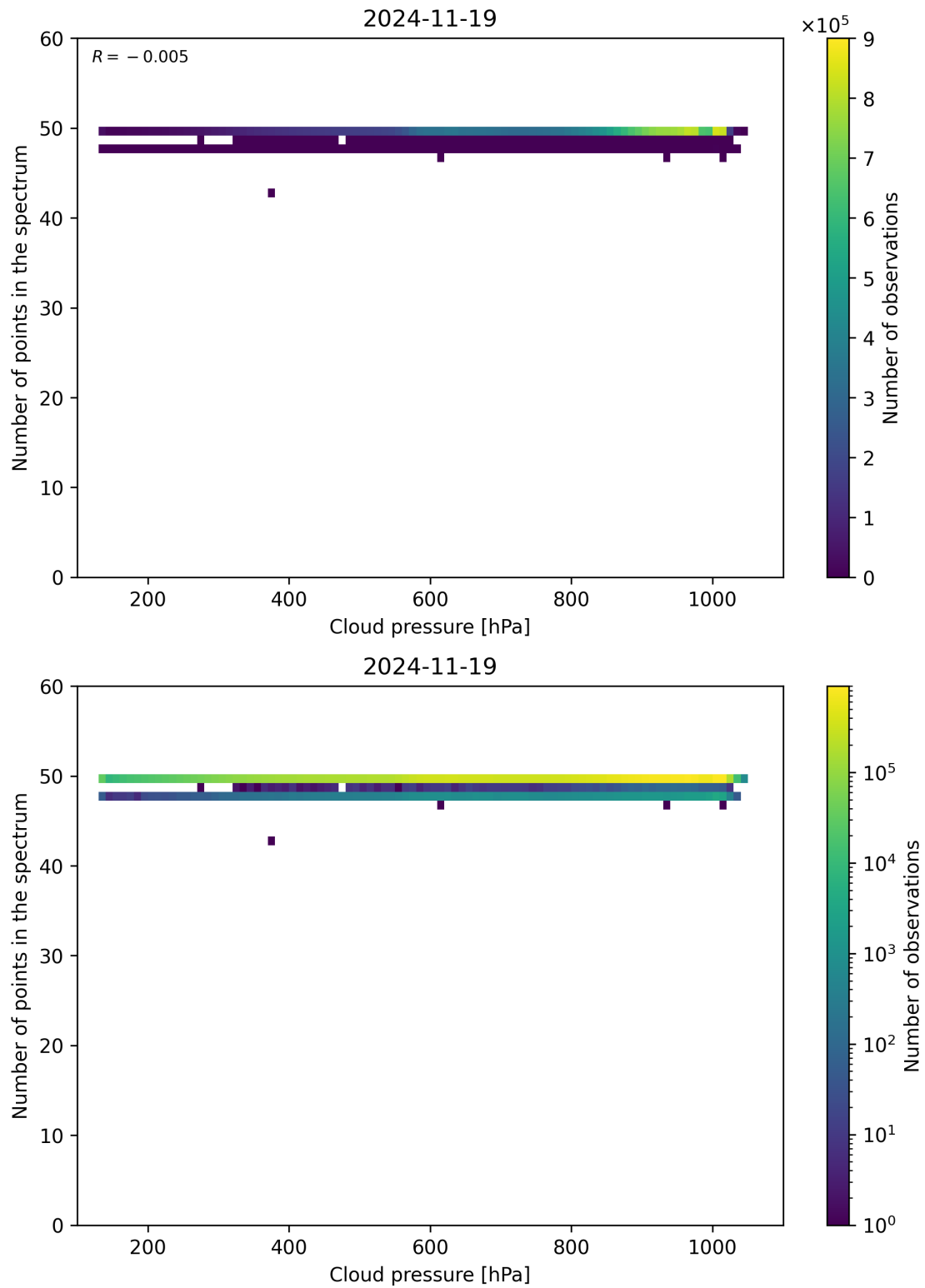
Figure 82: Scatter density plot of “Cloud pressure” against “Number of points in the spectrum” for 2024-11-18 to 2024-11-20.
