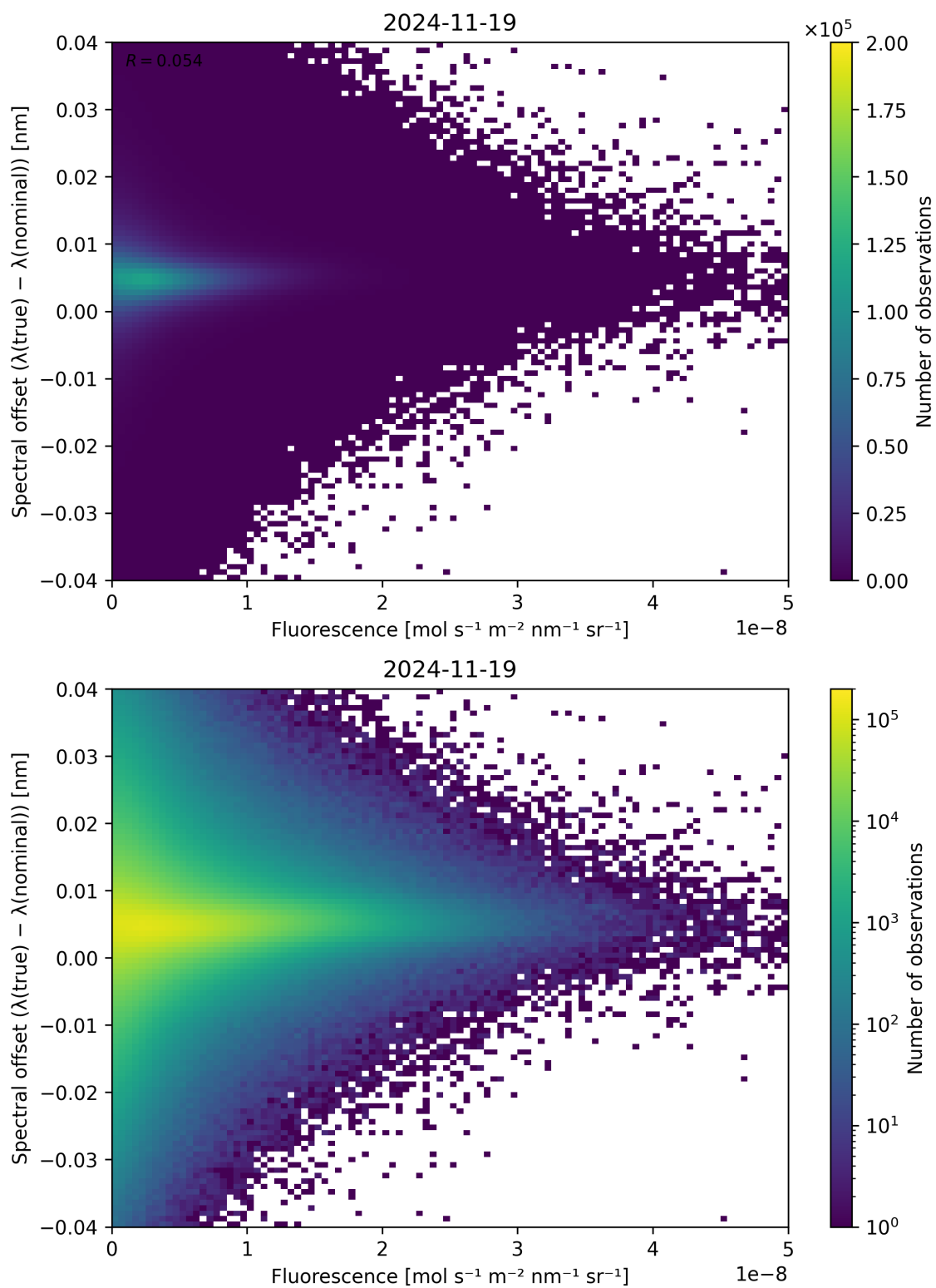
Figure 87: Scatter density plot of “Fluorescence” against “Spectral offset ( \lambda_{\text{true}} - \lambda_{\text{nominal}} )” for 2024-11-18 to 2024-11-20.
