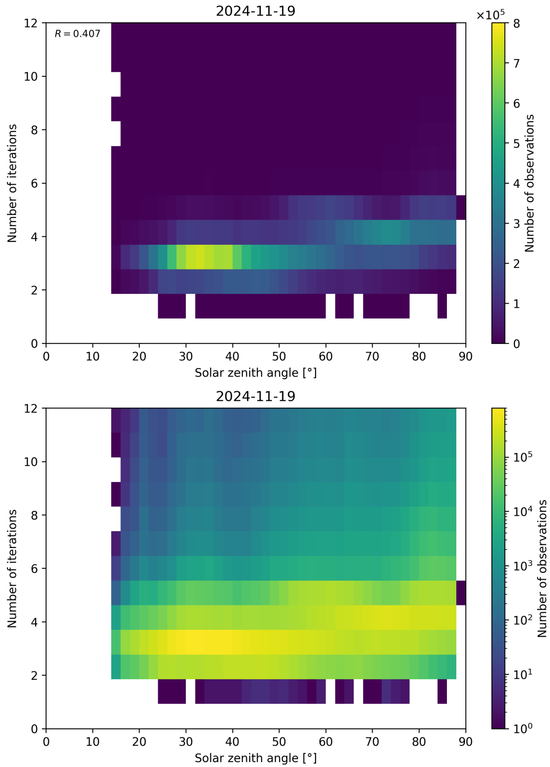
Figure 114: Scatter density plot of “Solar zenith angle” against “Number of iterations” for 2024-11-18 to 2024-11-20.
