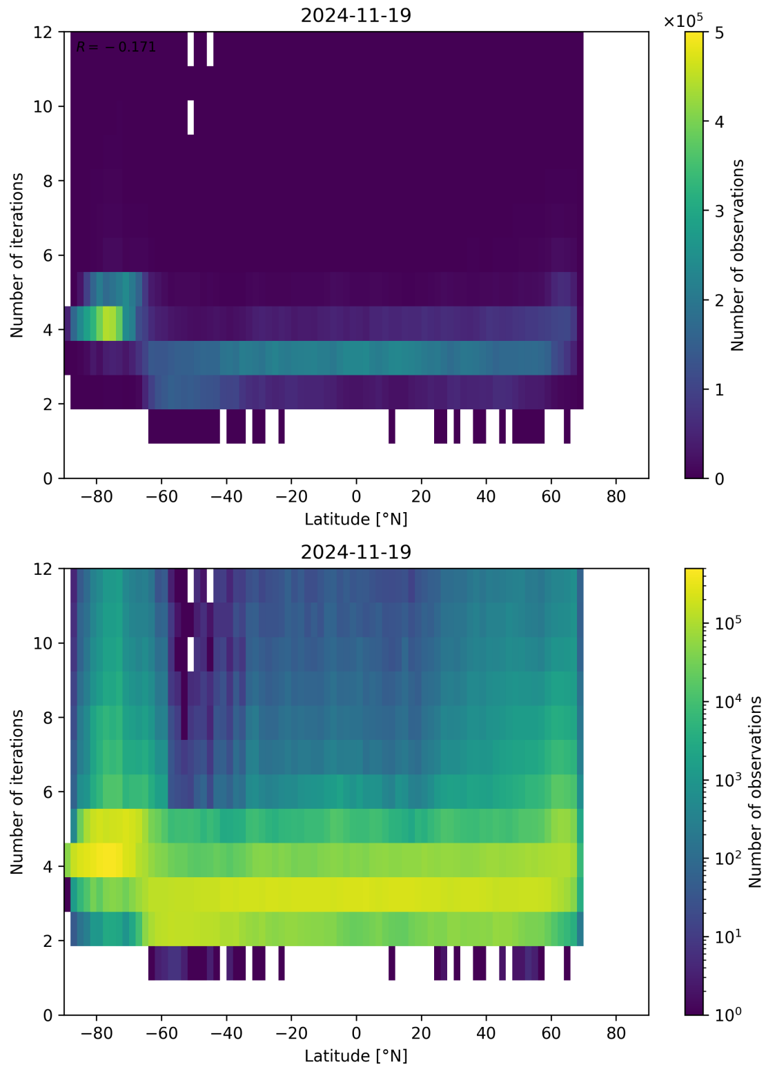
Figure 93: Scatter density plot of “Latitude” against “Number of iterations” for 2024-11-18 to 2024-11-20.
