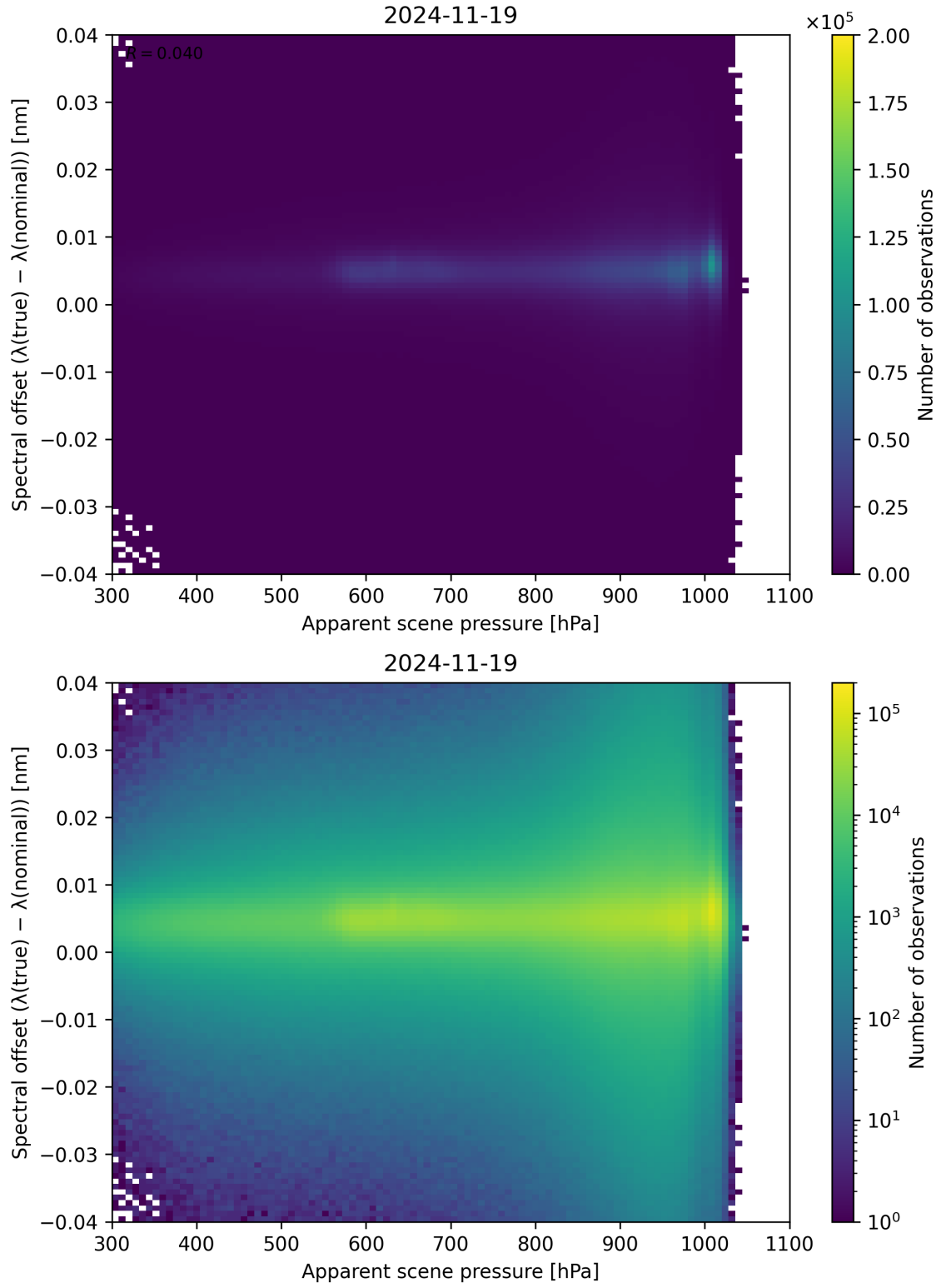
Figure 67: Scatter density plot of “Apparent scene pressure” against “Spectral offset ( \lambda_{\text{true}} - \lambda_{\text{nominal}} )” for 2024-11-18 to 2024-11-20.
