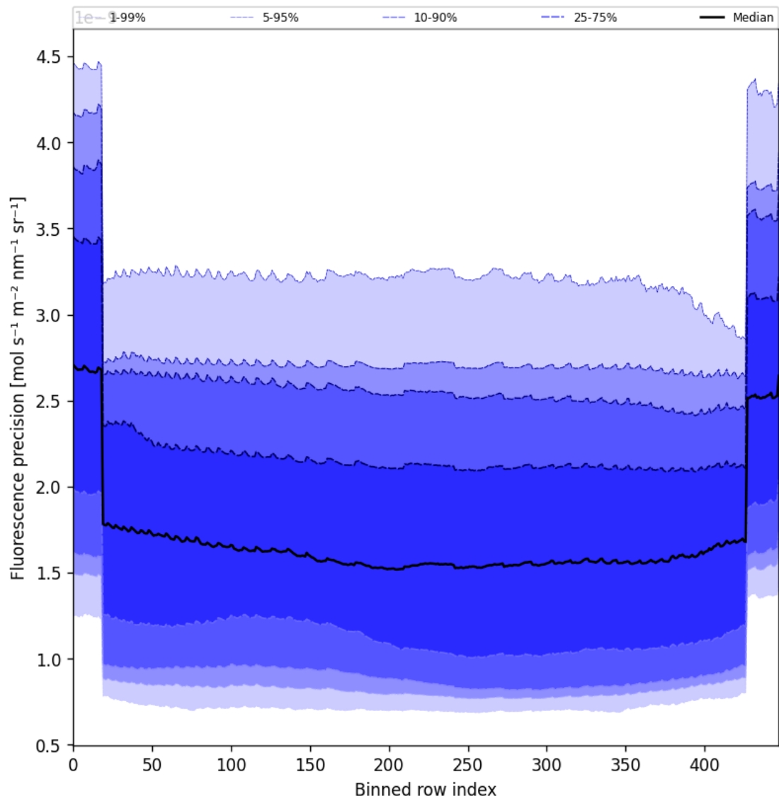
Figure 58: Along track statistics of “Fluorescence precision” for 2024-11-18 to 2024-11-20
