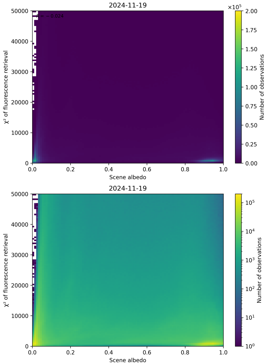
Figure 103: Scatter density plot of “Scene albedo” against “ \chi^2 of fluorescence retrieval” for 2024-11-18 to 2024-11-20.
