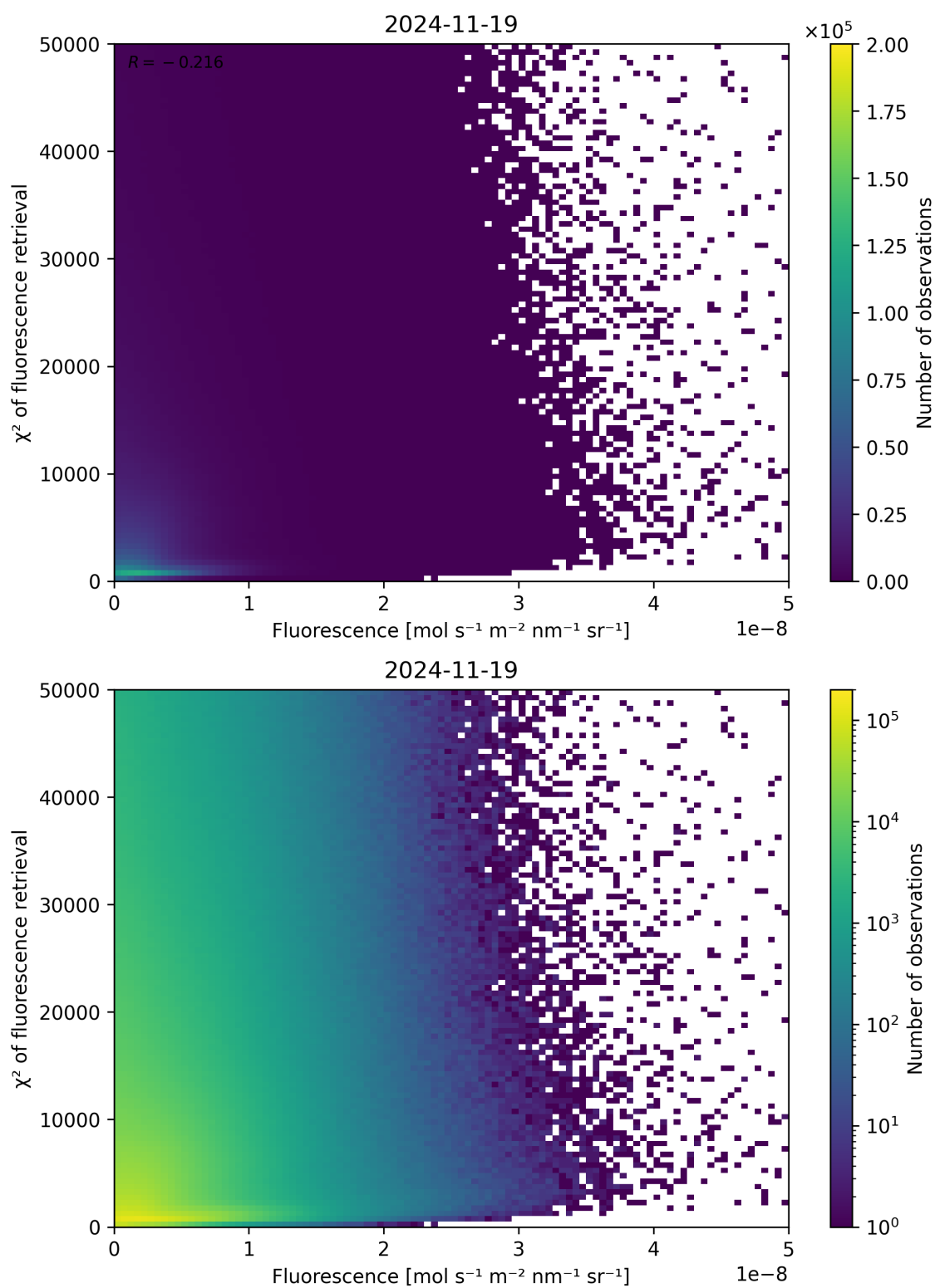
Figure 85: Scatter density plot of “Fluorescence” against “ \chi^2 of fluorescence retrieval” for 2024-11-18 to 2024-11-20.
