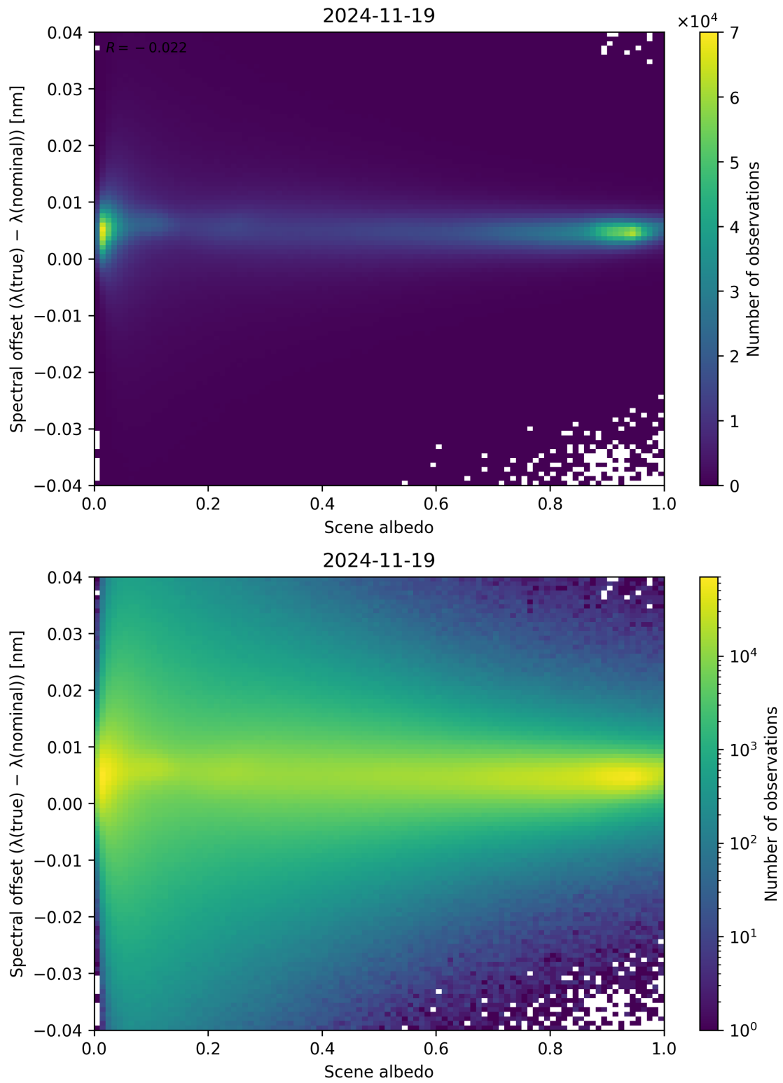
Figure 107: Scatter density plot of “Scene albedo” against “Spectral offset ( \lambda_{\text{true}} - \lambda_{\text{nominal}} )” for 2024-11-18 to 2024-11-20.
