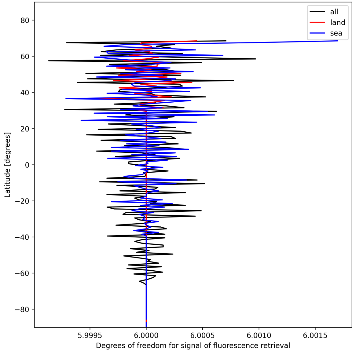
Figure 26: Zonal average of “Degrees of freedom for signal of fluorescence retrieval” for 2024-11-18 to 2024-11-20.
