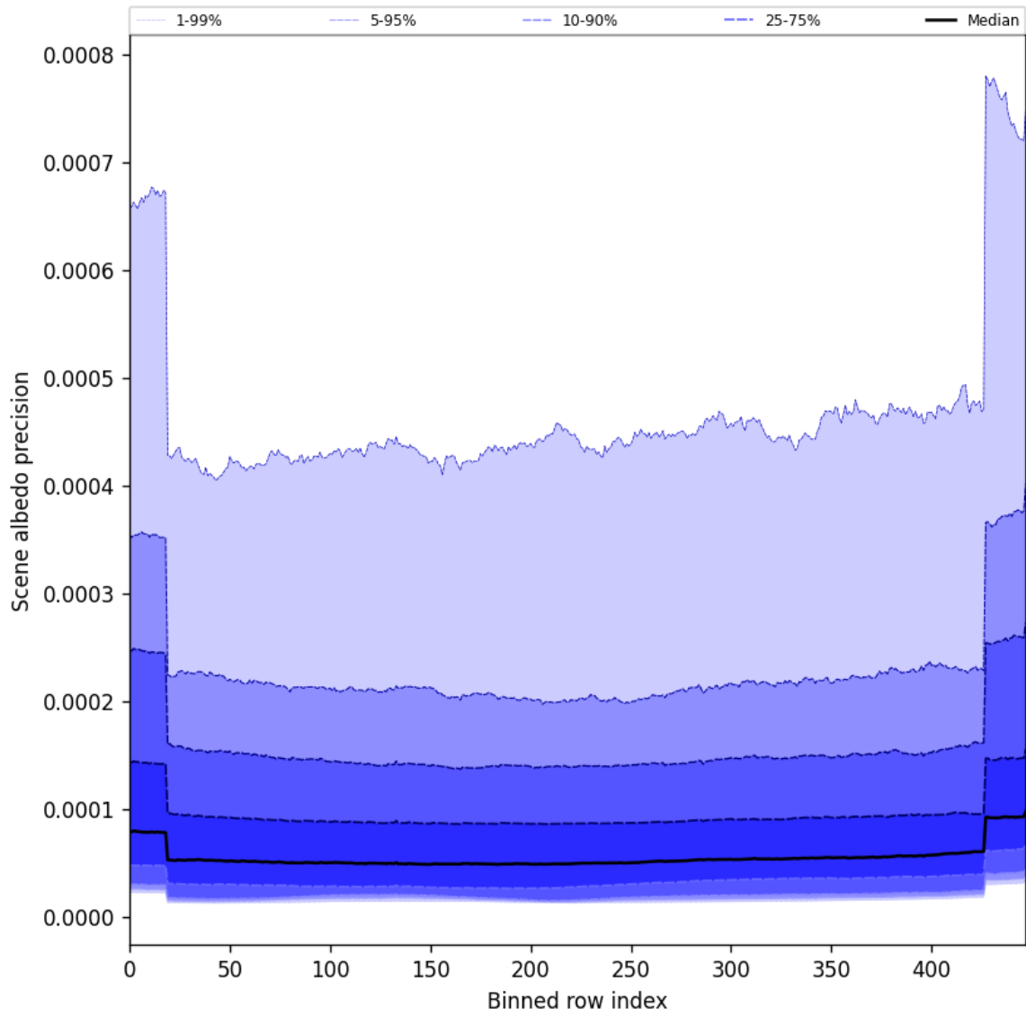
Figure 52: Along track statistics of “Scene albedo precision” for 2024-11-18 to 2024-11-20
