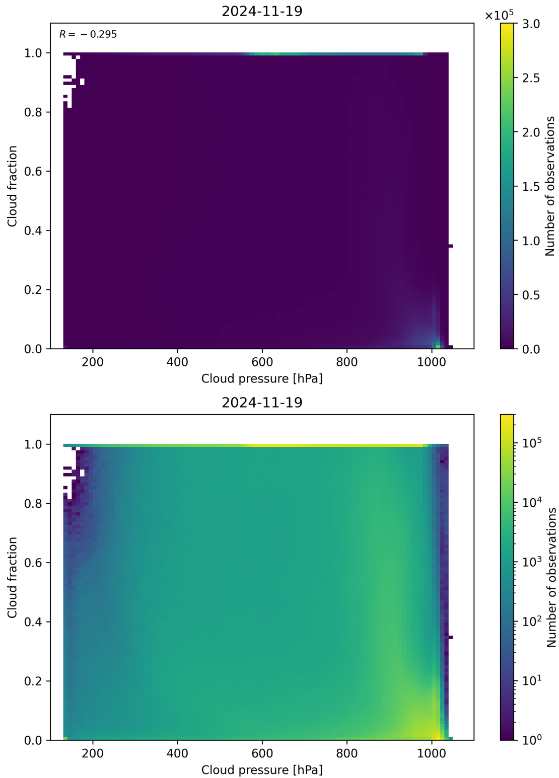
Figure 79: Scatter density plot of “Cloud pressure” against “Cloud fraction” for 2024-11-18 to 2024-11-20.
