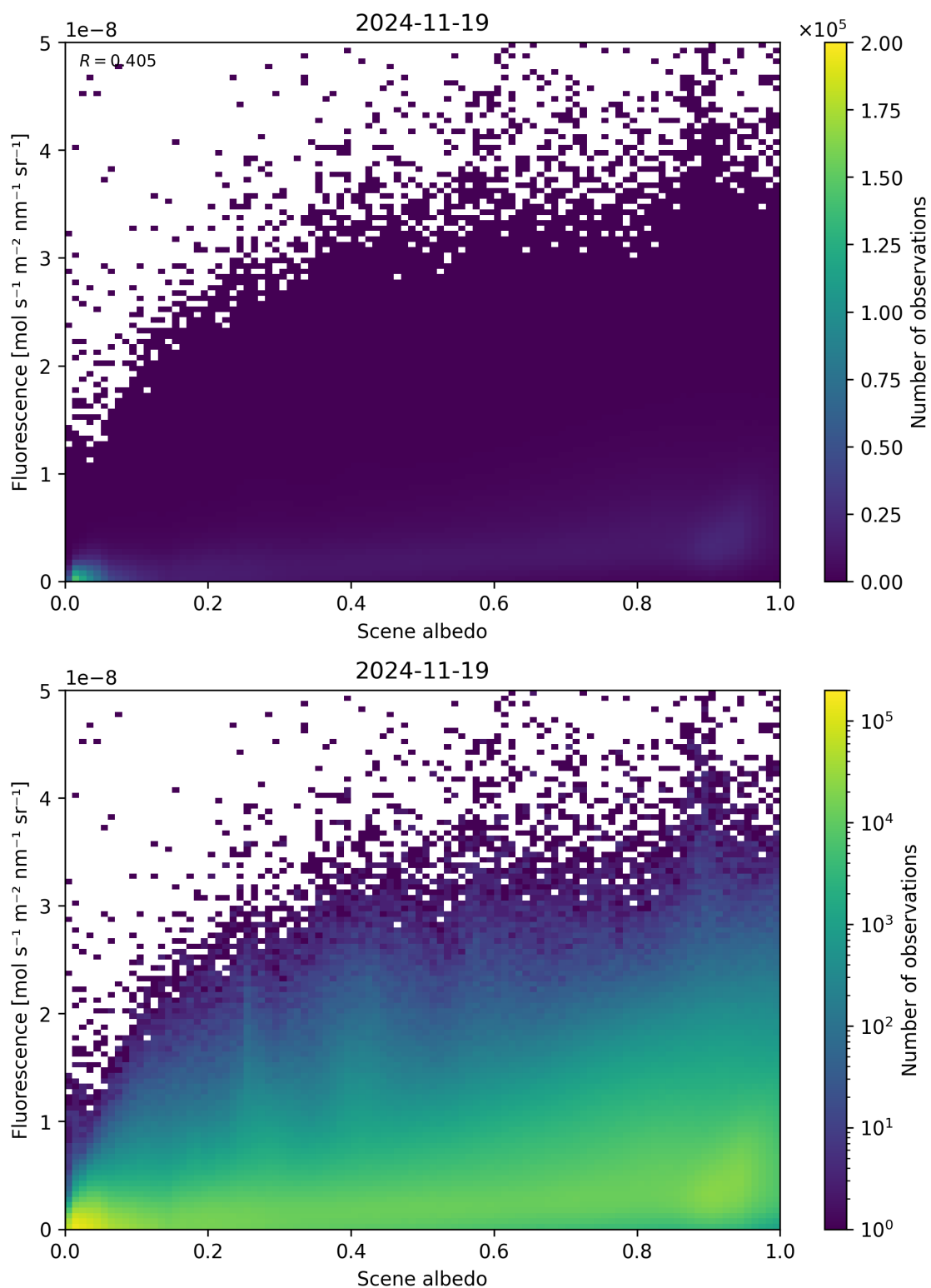
Figure 104: Scatter density plot of “Scene albedo” against “Fluorescence” for 2024-11-18 to 2024-11-20.
