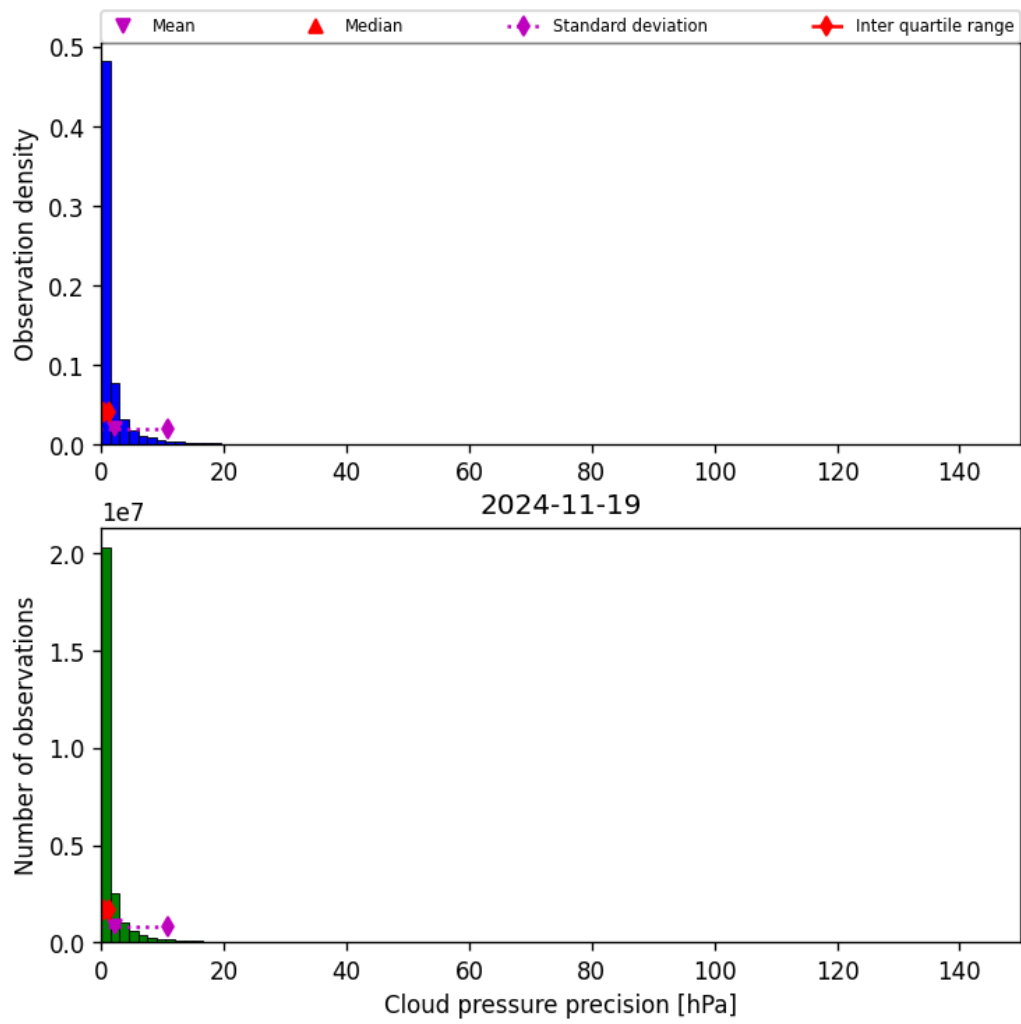
Figure 31: Histogram of “Cloud pressure precision” for 2024-11-18 to 2024-11-20
