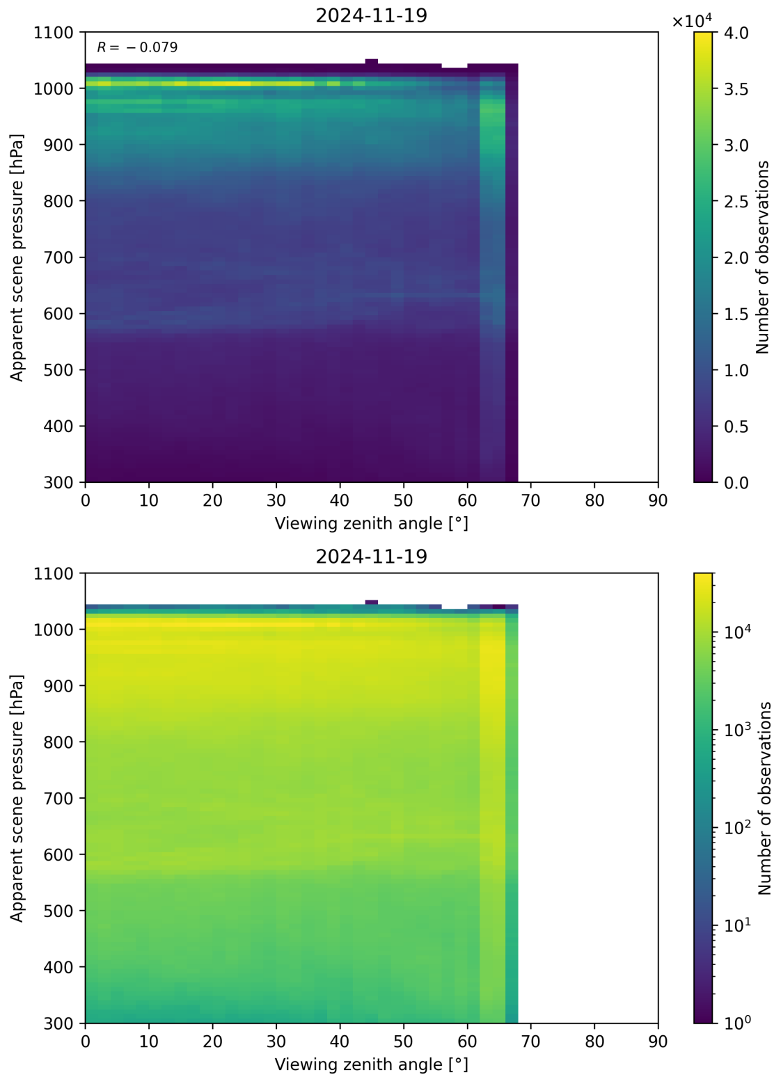
Figure 118: Scatter density plot of “Viewing zenith angle” against “Apparent scene pressure” for 2024-11-18 to 2024-11-20.
