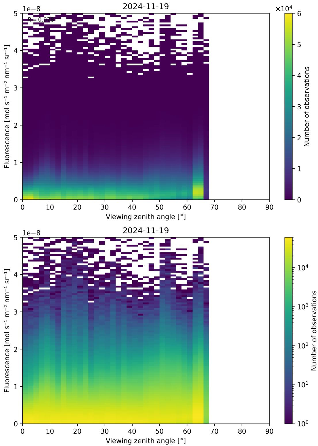
Figure 122: Scatter density plot of “Viewing zenith angle” against “Fluorescence” for 2024-11-18 to 2024-11-20.
