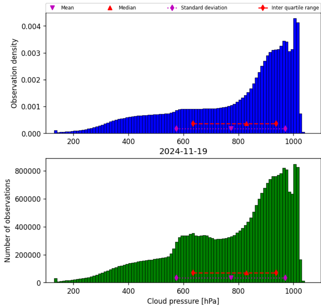
Figure 30: Histogram of “Cloud pressure” for 2024-11-18 to 2024-11-20
