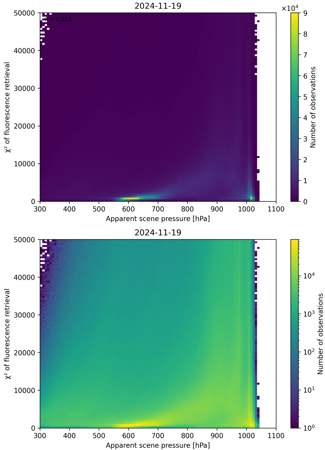
Figure 63: Scatter density plot of “Apparent scene pressure” against “ \chi^2 of fluorescence retrieval” for 2024-11-18 to 2024-11-20.
