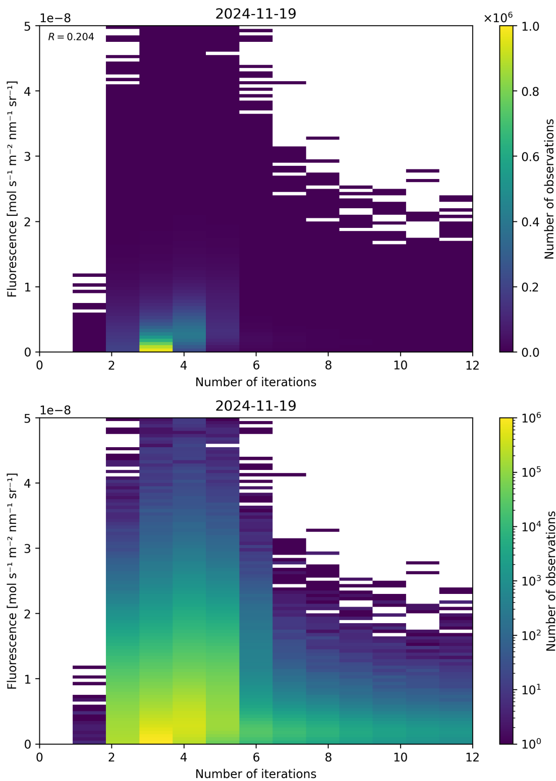
Figure 98: Scatter density plot of “Number of iterations” against “Fluorescence” for 2024-11-18 to 2024-11-20.
