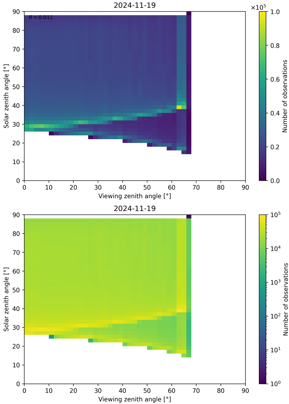
Figure 127: Scatter density plot of “Viewing zenith angle” against “Solar zenith angle” for 2024-11-18 to 2024-11-20.
