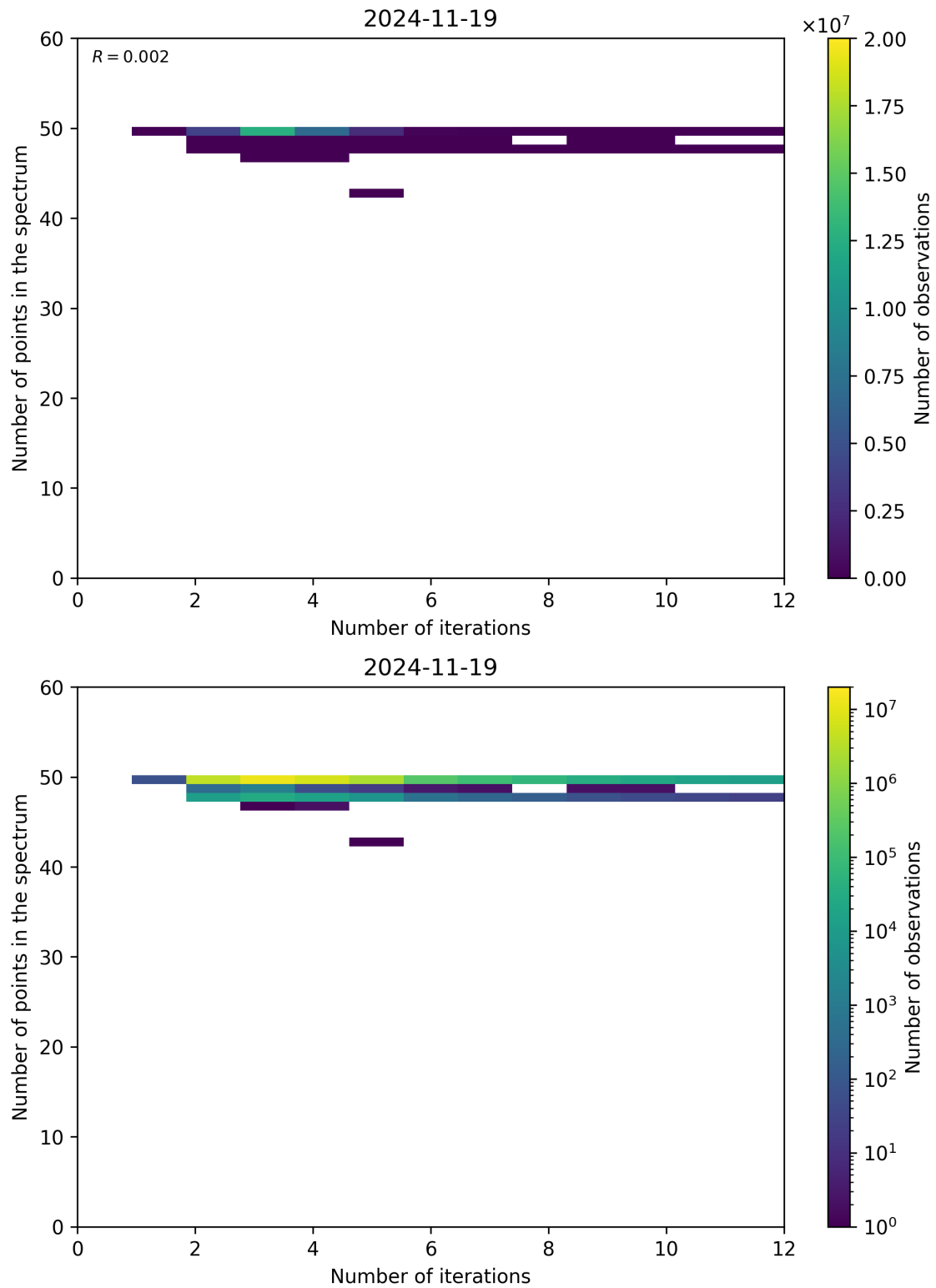
Figure 99: Scatter density plot of “Number of iterations” against “Number of points in the spectrum” for 2024-11-18 to 2024-11-20.
