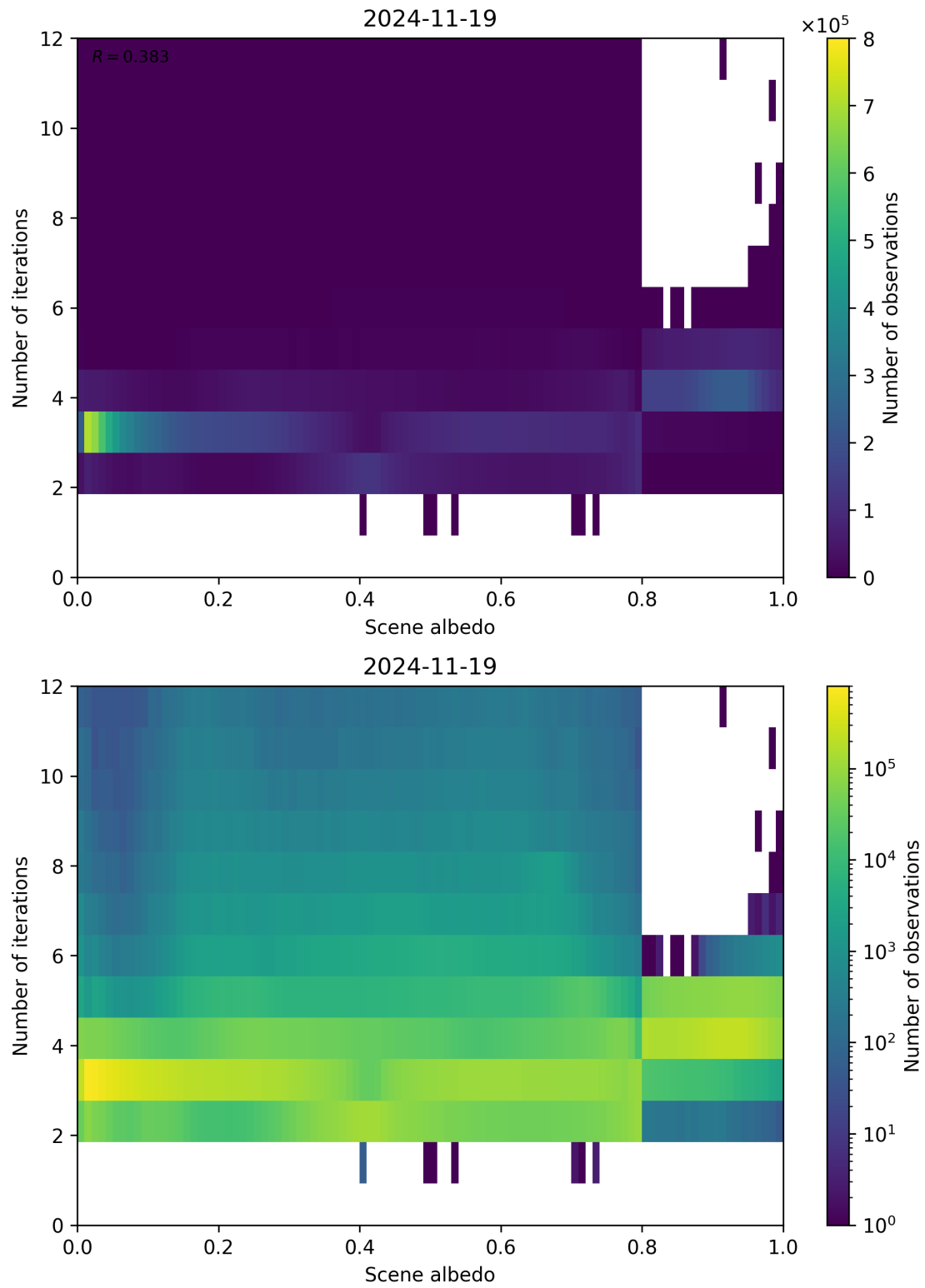
Figure 105: Scatter density plot of “Scene albedo” against “Number of iterations” for 2024-11-18 to 2024-11-20.
