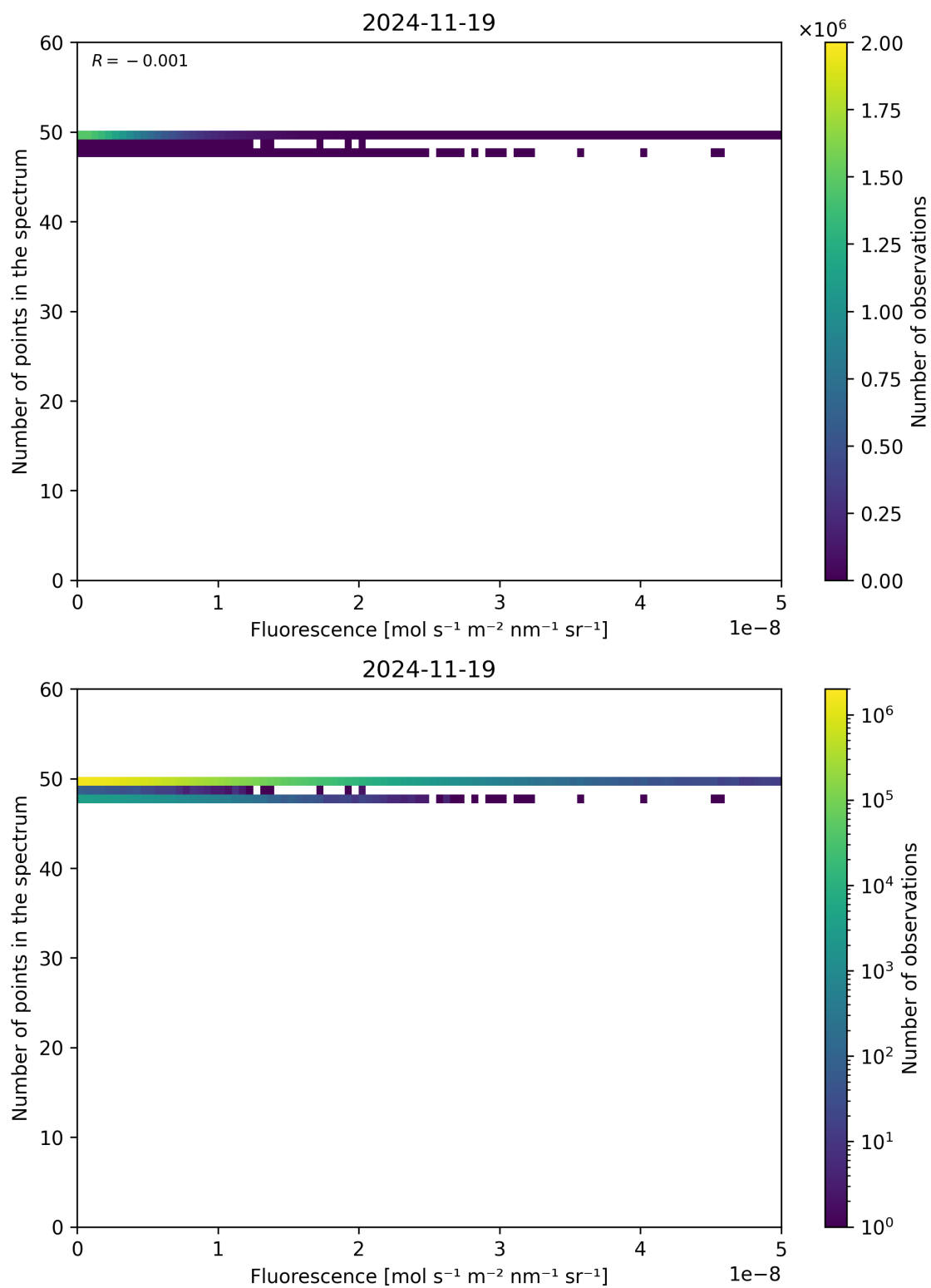
Figure 86: Scatter density plot of “Fluorescence” against “Number of points in the spectrum” for 2024-11-18 to 2024-11-20.
