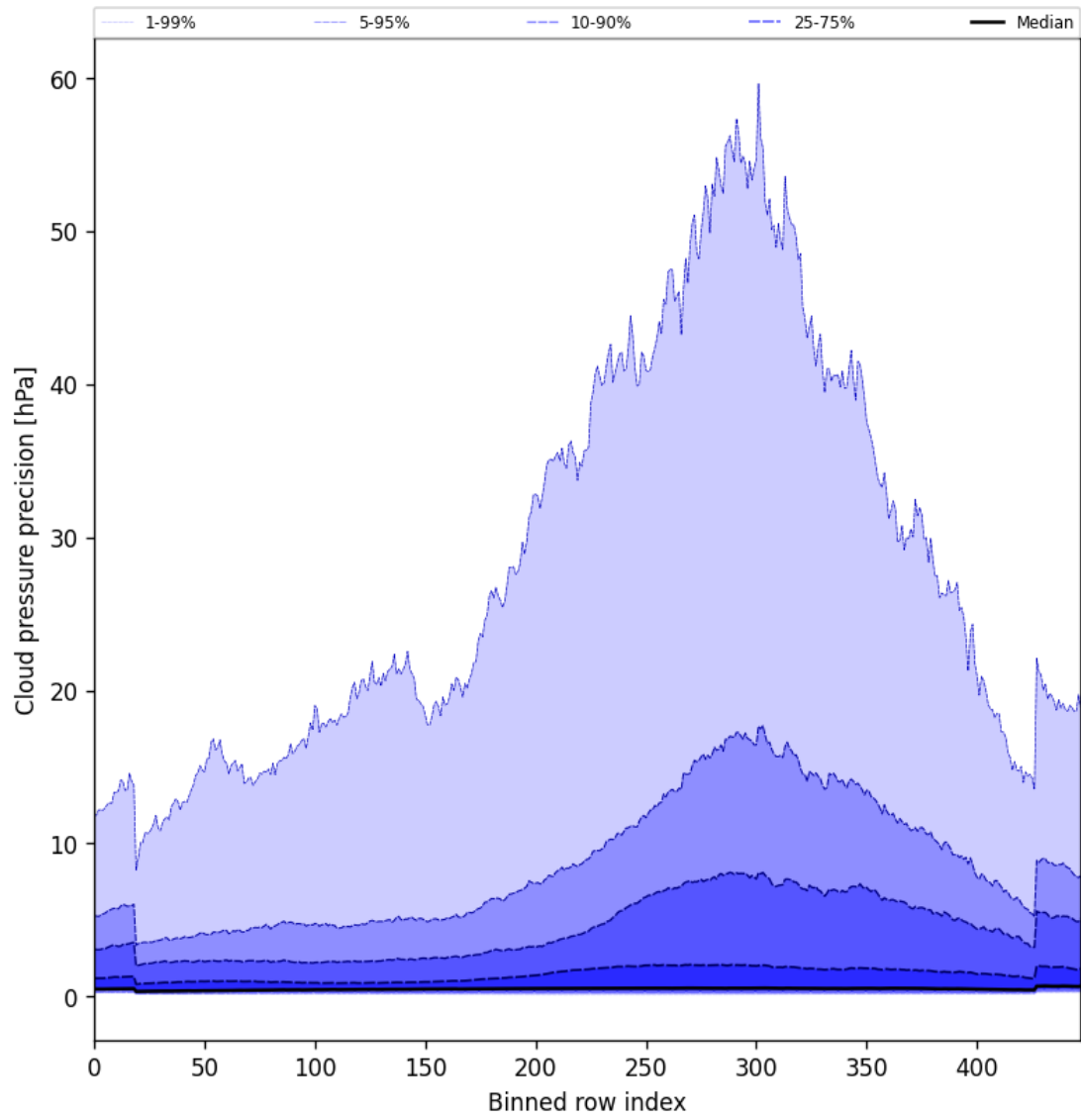
Figure 48: Along track statistics of “Cloud pressure precision” for 2024-11-18 to 2024-11-20
