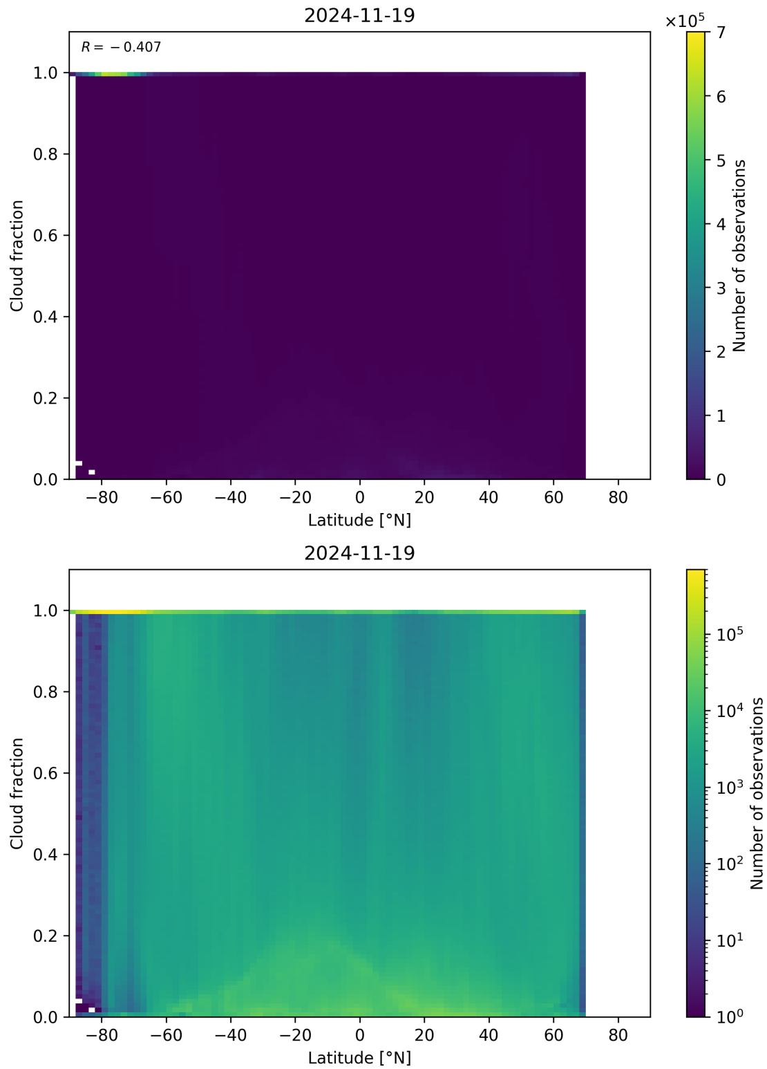
Figure 90: Scatter density plot of “Latitude” against “Cloud fraction” for 2024-11-18 to 2024-11-20.
