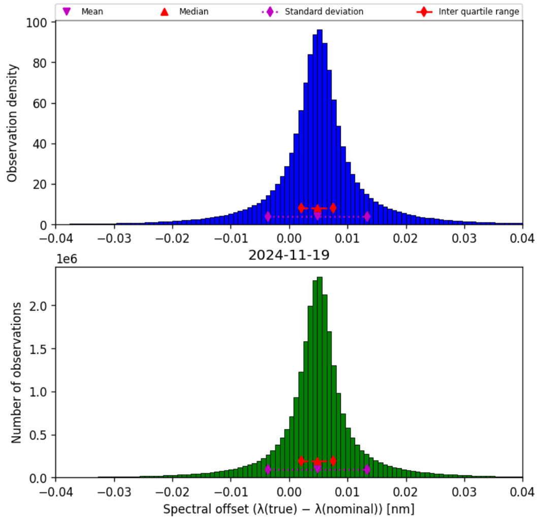
Figure 45: Histogram of “Spectral offset ( \lambda_{\text{true}} - \lambda_{\text{nominal}} )” for 2024-11-18 to 2024-11-20
