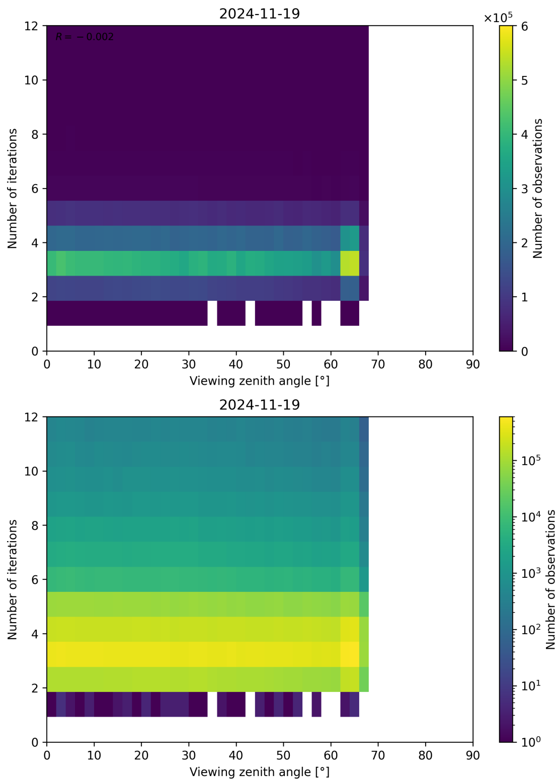
Figure 124: Scatter density plot of “Viewing zenith angle” against “Number of iterations” for 2024-11-18 to 2024-11-20.
