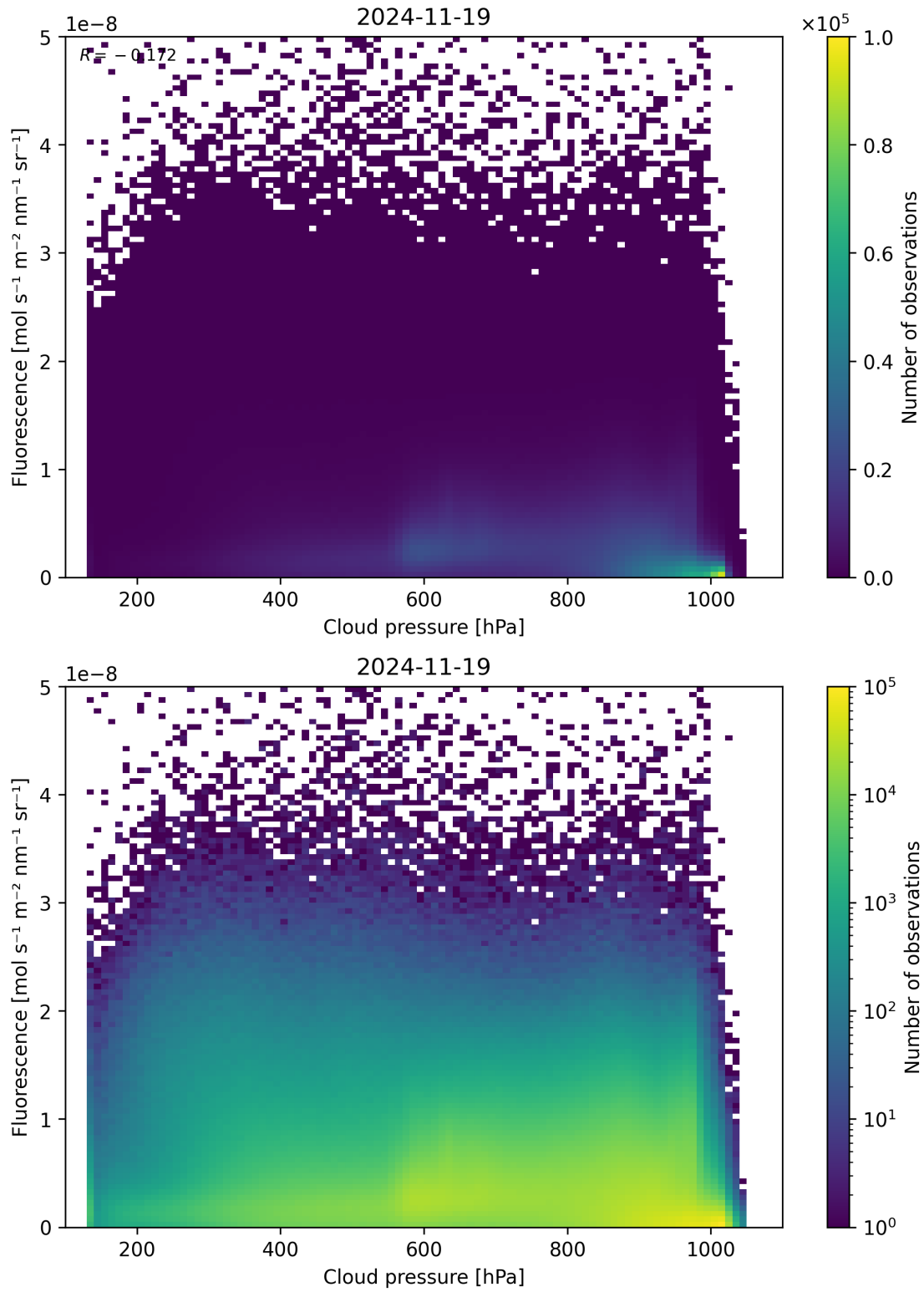
Figure 80: Scatter density plot of “Cloud pressure” against “Fluorescence” for 2024-11-18 to 2024-11-20.
