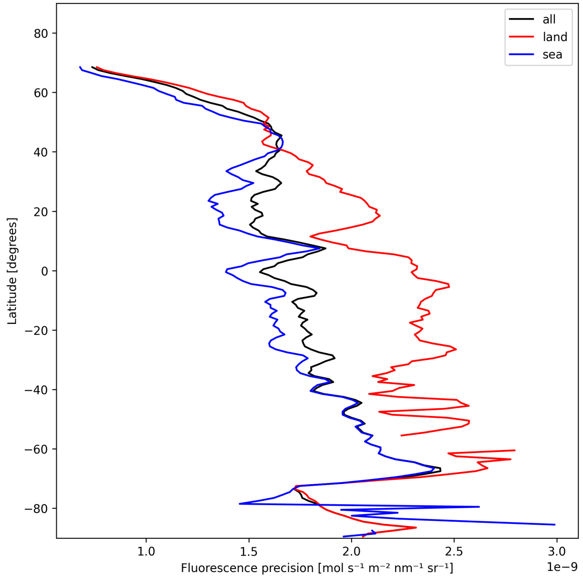
Figure 24: Zonal average of “Fluorescence precision” for 2024-11-18 to 2024-11-20.
