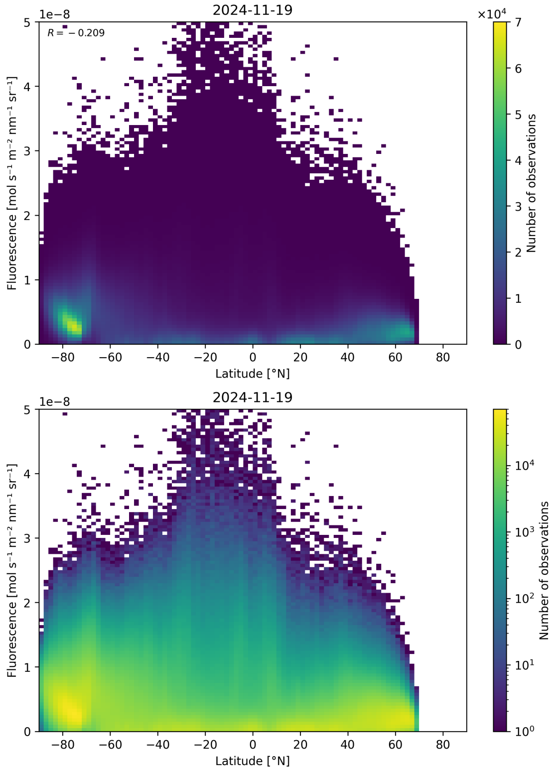
Figure 92: Scatter density plot of “Latitude” against “Fluorescence” for 2024-11-18 to 2024-11-20.
