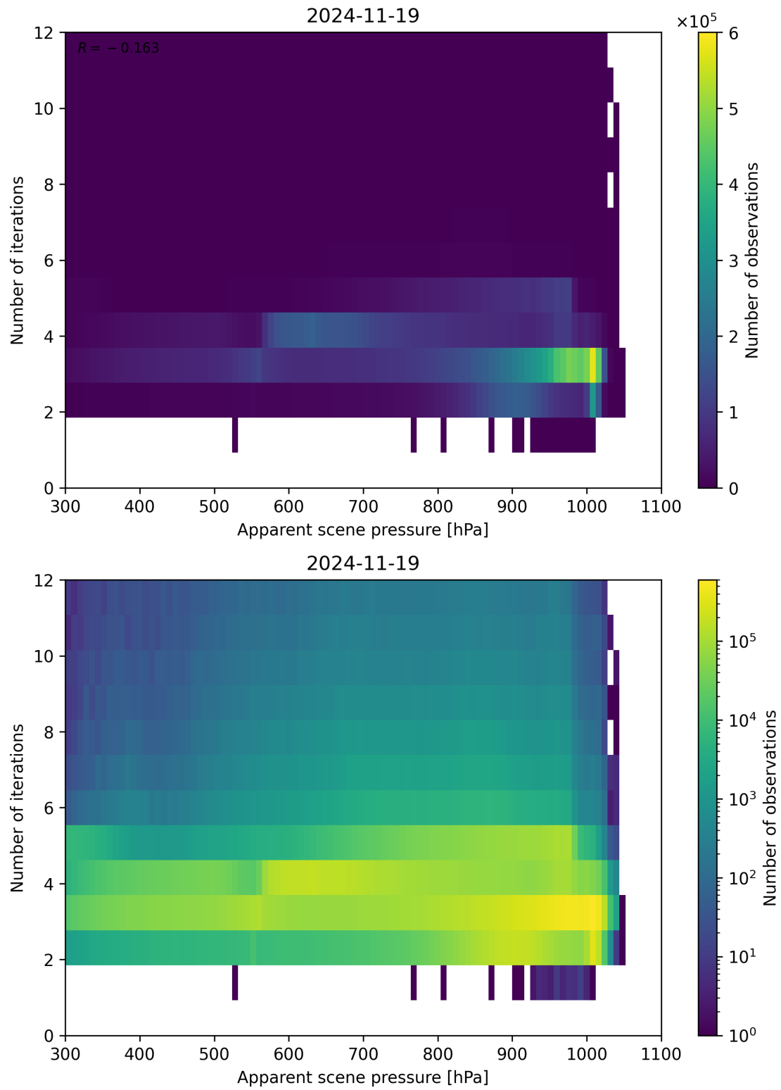
Figure 65: Scatter density plot of “Apparent scene pressure” against “Number of iterations” for 2024-11-18 to 2024-11-20.
