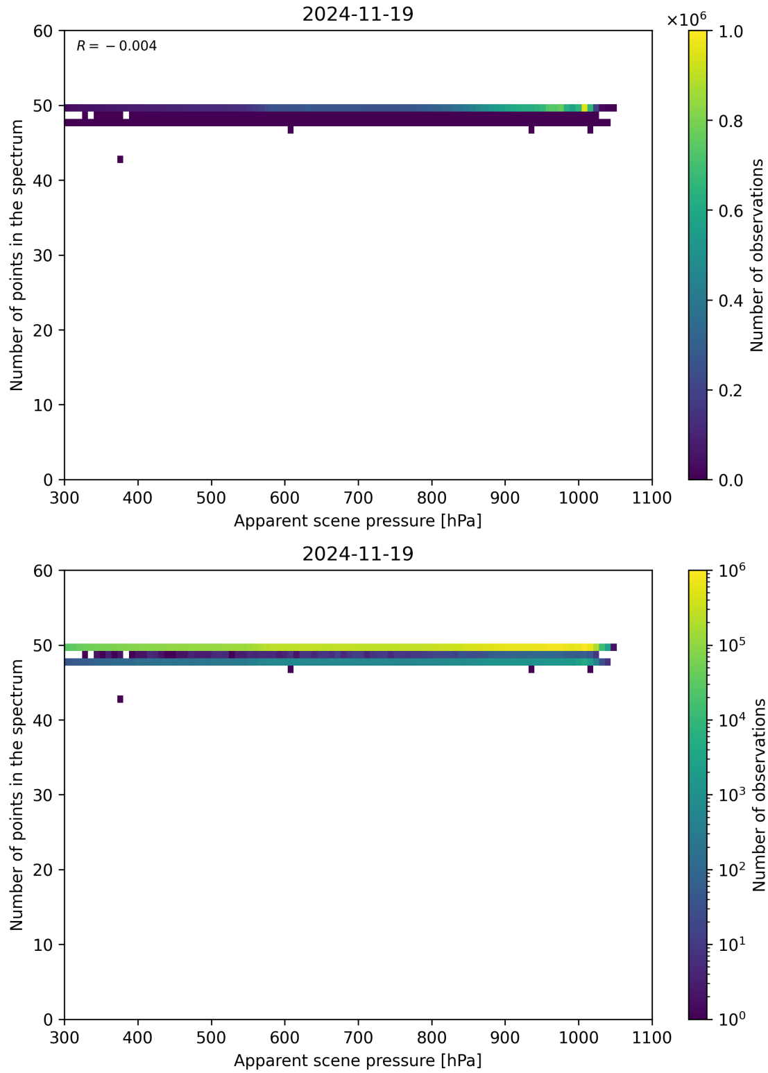
Figure 66: Scatter density plot of “Apparent scene pressure” against “Number of points in the spectrum” for 2024-11-18 to 2024-11-20.
