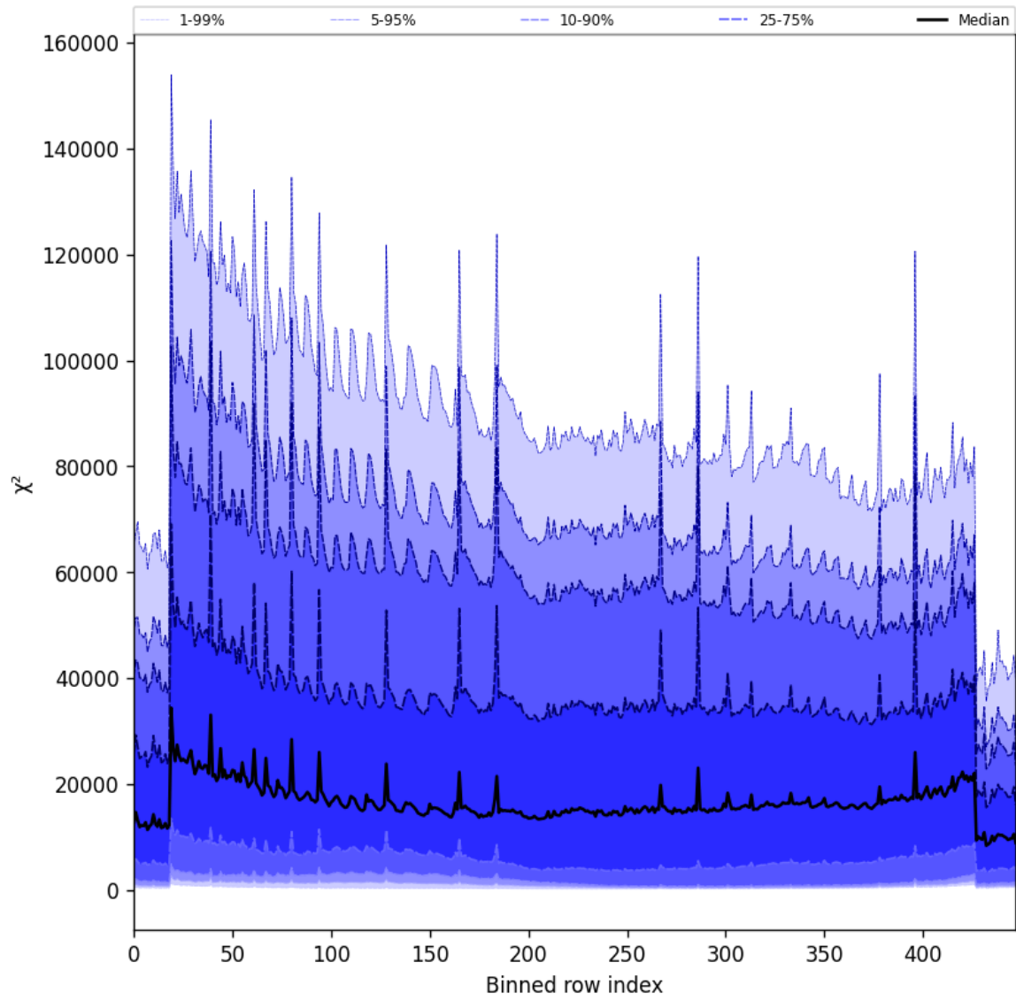
Figure 55: Along track statistics of “ \chi^2 ” for 2024-11-18 to 2024-11-20
