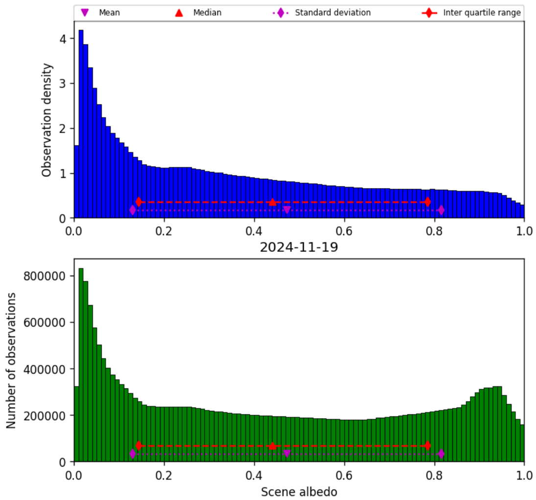
Figure 34: Histogram of “Scene albedo” for 2024-11-18 to 2024-11-20
