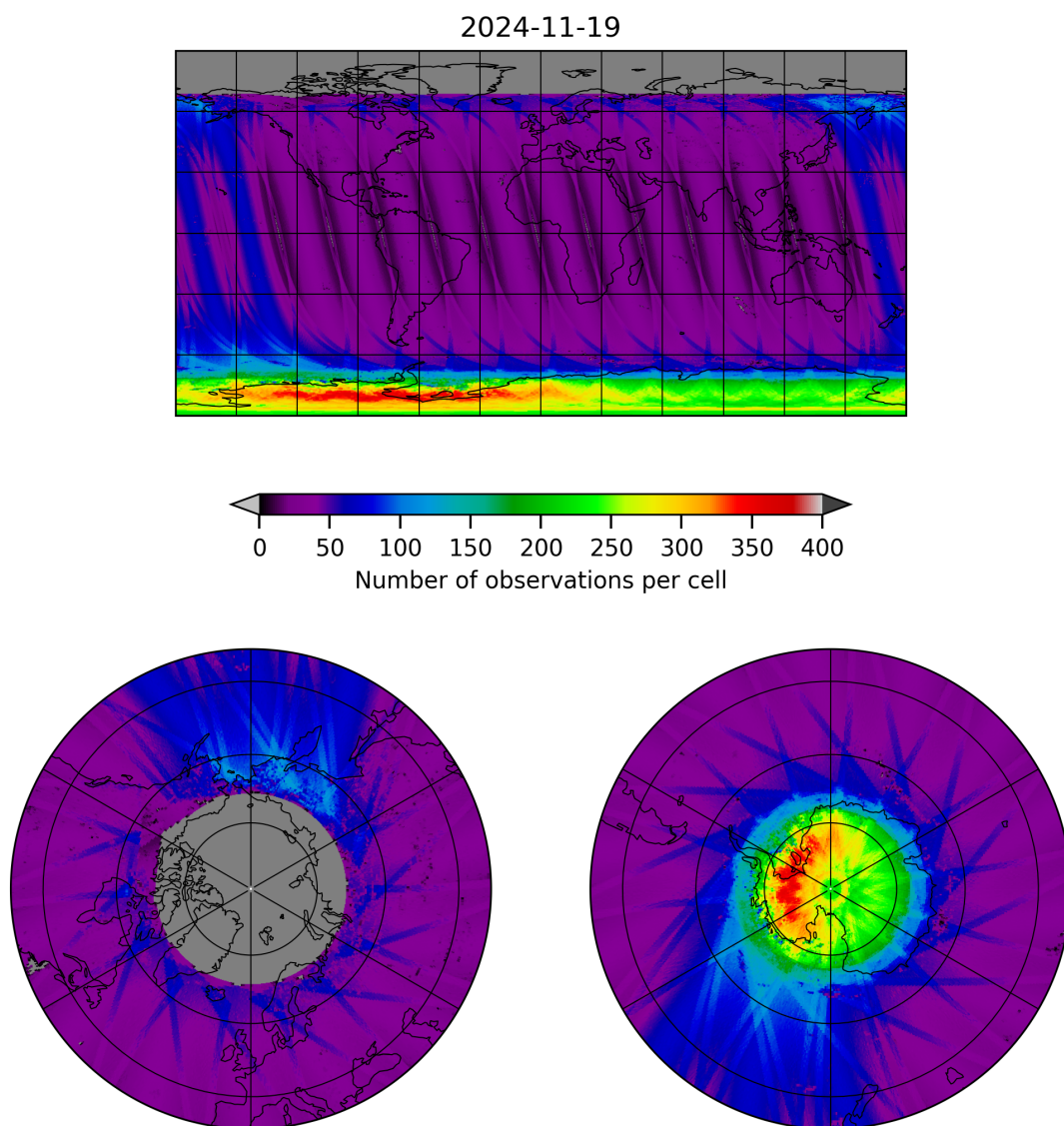
Figure 11: Map of the number of observations for 2024-11-18 to 2024-11-20
