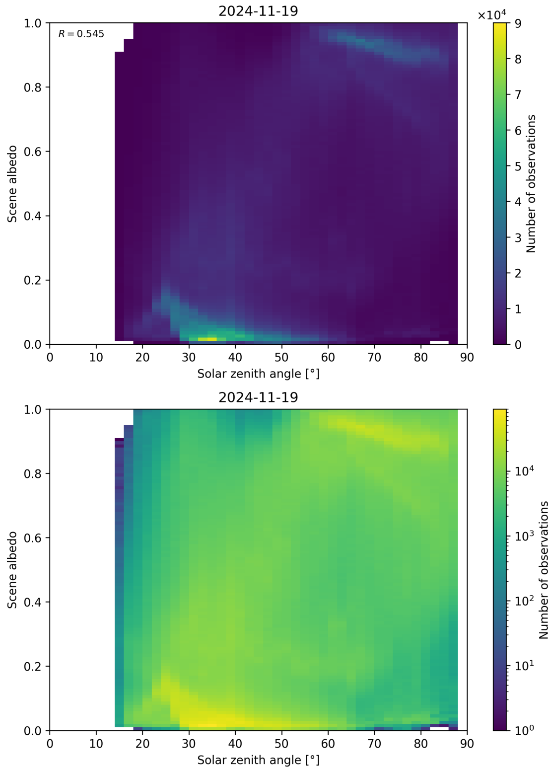
Figure 116: Scatter density plot of “Solar zenith angle” against “Scene albedo” for 2024-11-18 to 2024-11-20.
