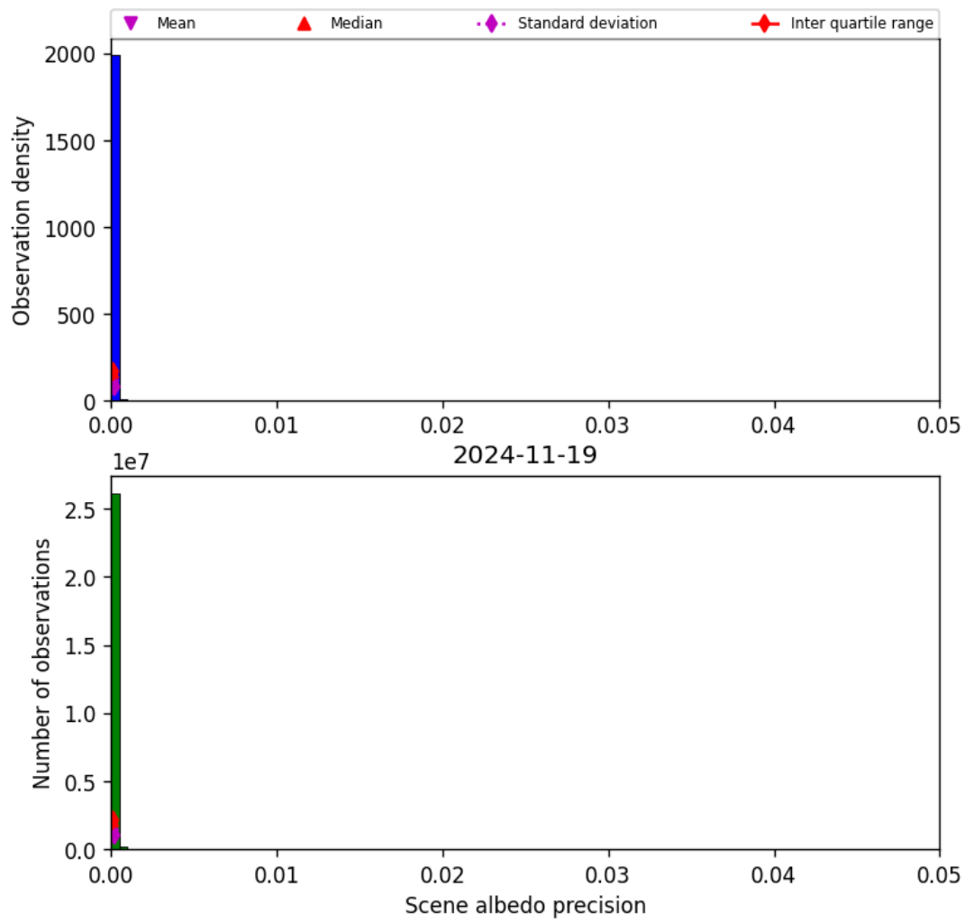
Figure 35: Histogram of “Scene albedo precision” for 2024-11-18 to 2024-11-20
