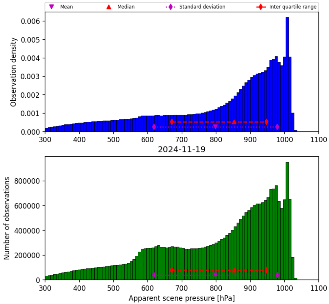
Figure 36: Histogram of “Apparent scene pressure” for 2024-11-18 to 2024-11-20
