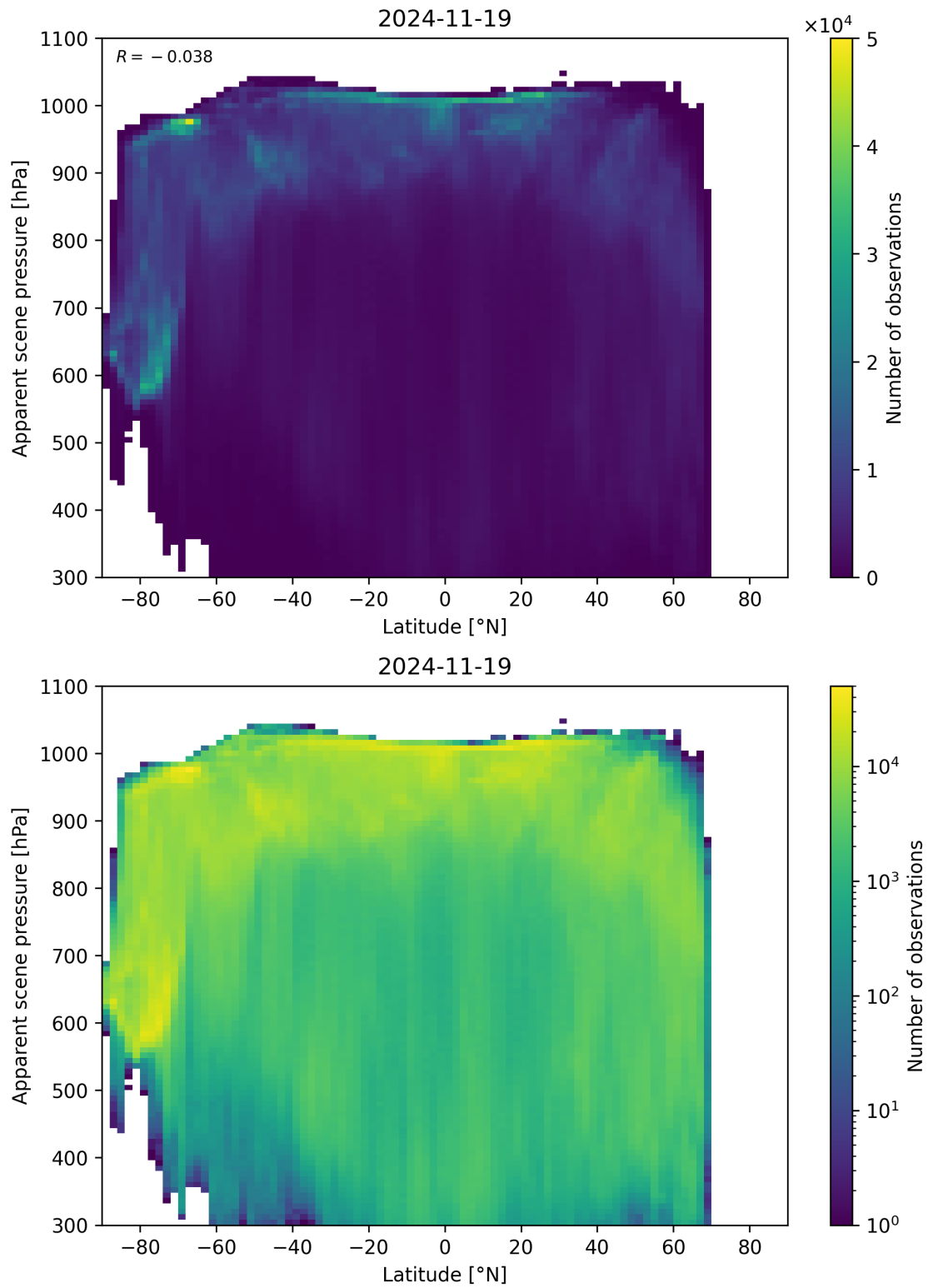
Figure 88: Scatter density plot of “Latitude” against “Apparent scene pressure” for 2024-11-18 to 2024-11-20.
