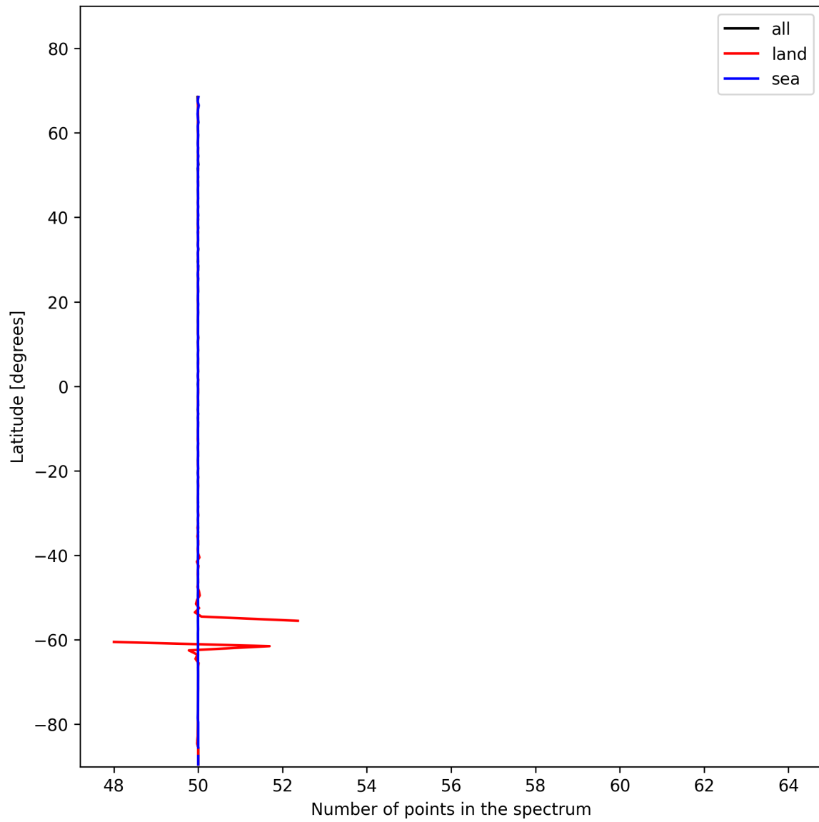
Figure 27: Zonal average of “Number of points in the spectrum” for 2024-11-18 to 2024-11-20.
