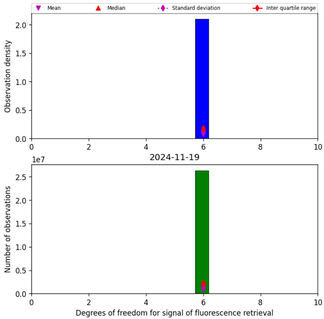
Figure 43: Histogram of "Degrees of freedom for signal of fluorescence retrieval" for 2024-11-18 to 2024-11-20
