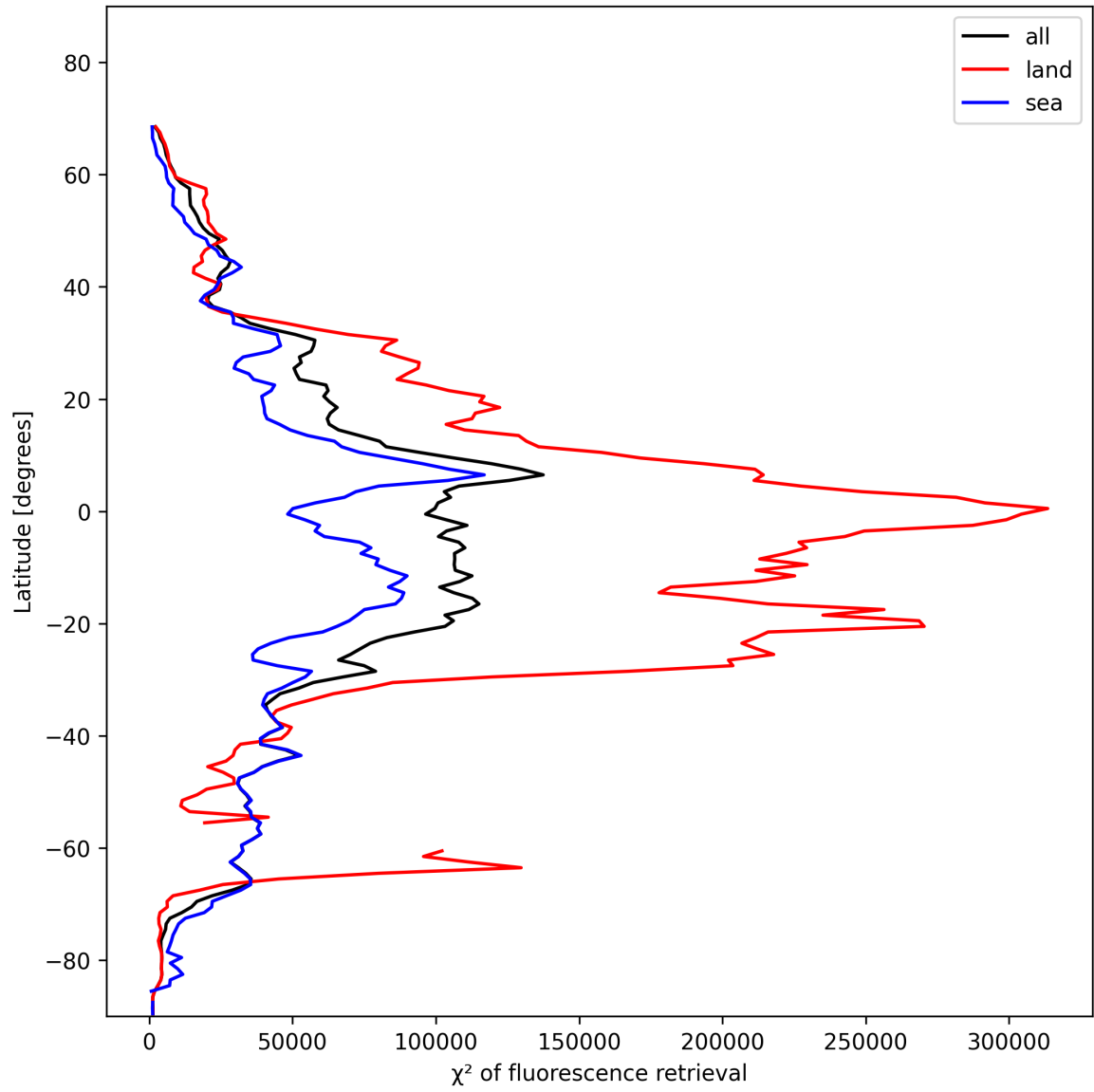
Figure 25: Zonal average of “ \chi^2 of fluorescence retrieval” for 2024-11-18 to 2024-11-20.
