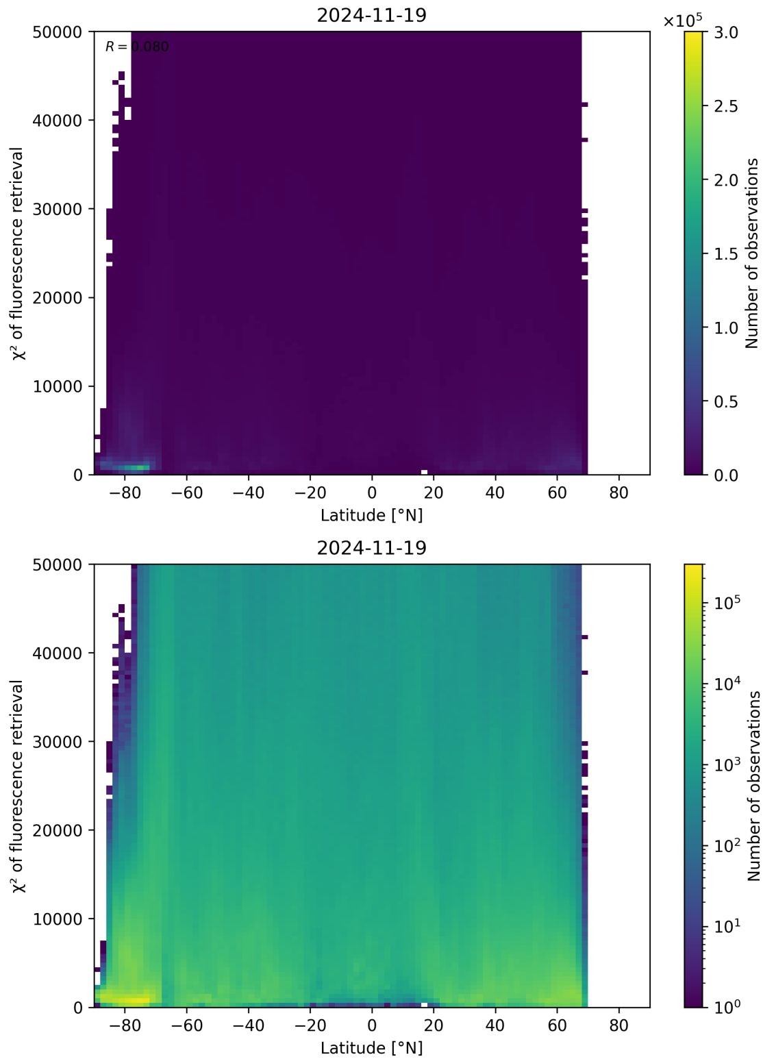
Figure 89: Scatter density plot of “Latitude” against “ \chi^2 of fluorescence retrieval” for 2024-11-18 to 2024-11-20.
