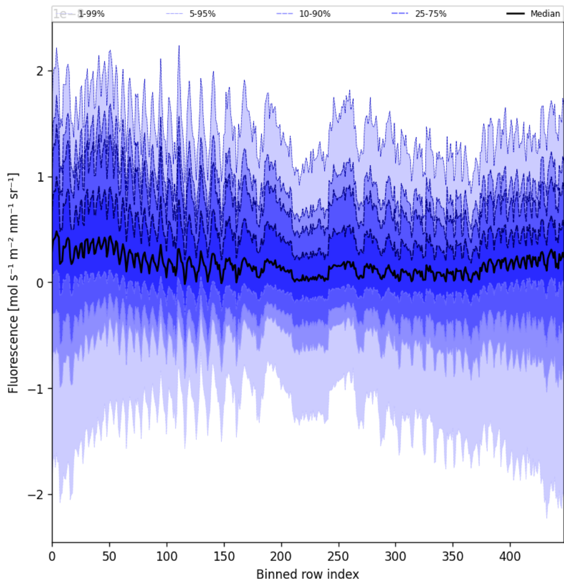
Figure 57: Along track statistics of “Fluorescence” for 2024-11-18 to 2024-11-20
