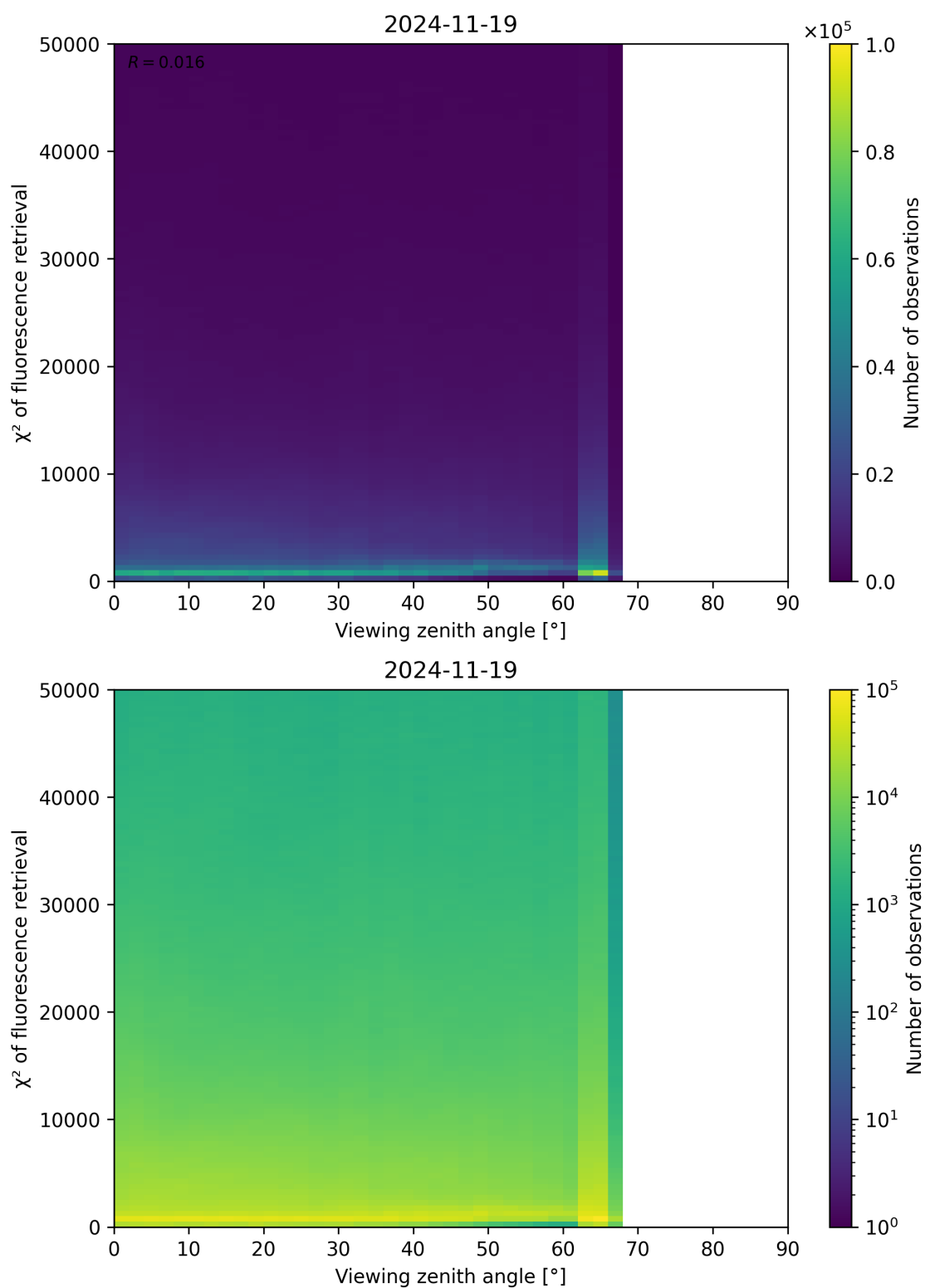
Figure 119: Scatter density plot of “Viewing zenith angle” against “ \chi^2 of fluorescence retrieval” for 2024-11-18 to 2024-11-20.
