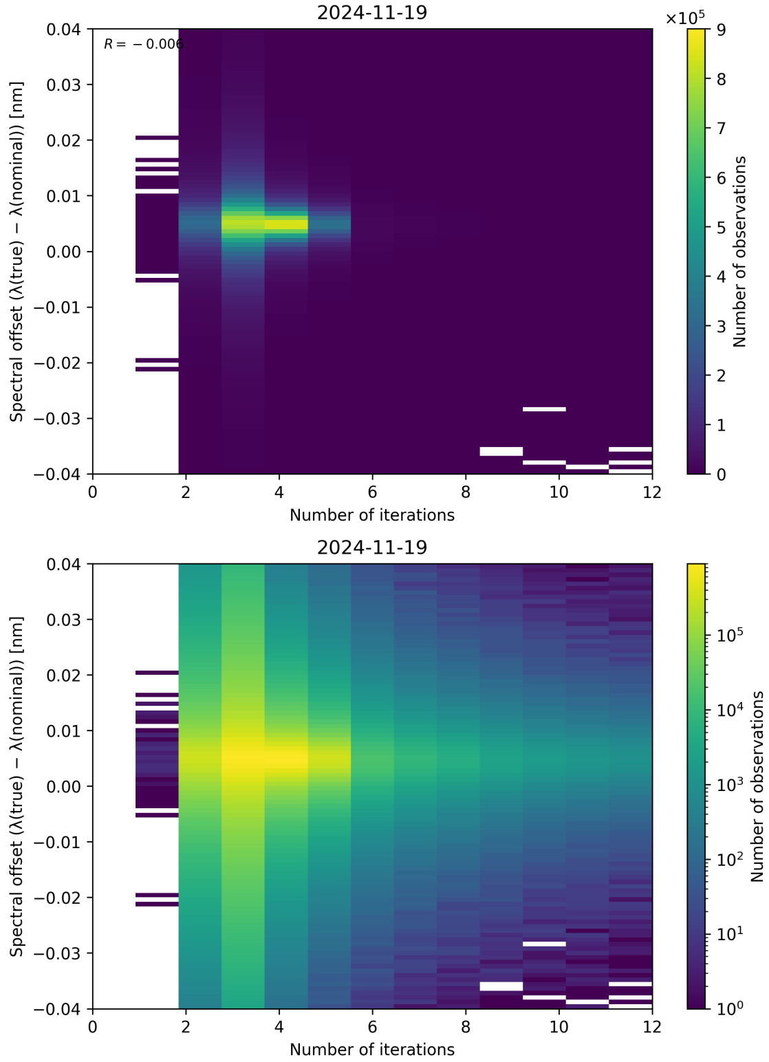
Figure 100: Scatter density plot of “Number of iterations” against “Spectral offset ( \lambda_{\text{true}} - \lambda_{\text{nominal}} )” for 2024-11-18 to 2024-11-20.
