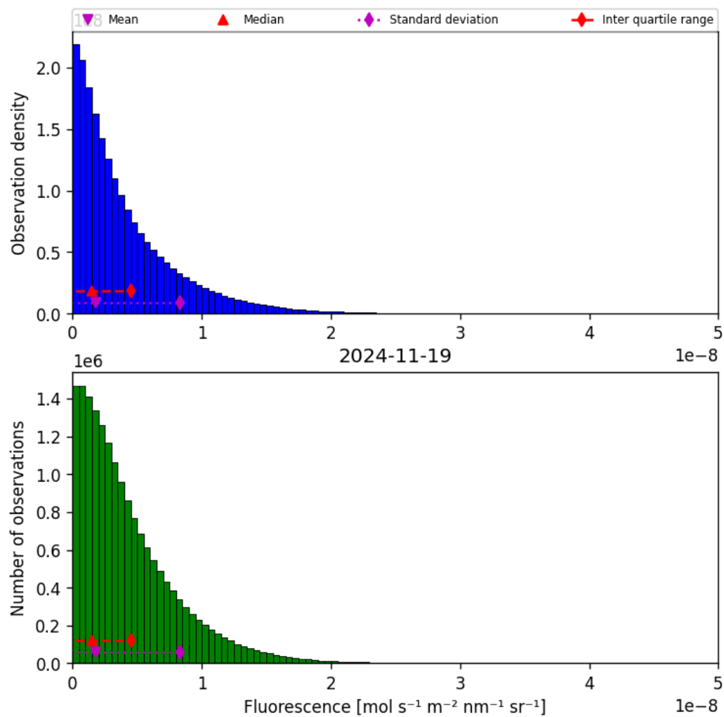
Figure 40: Histogram of “Fluorescence” for 2024-11-18 to 2024-11-20
