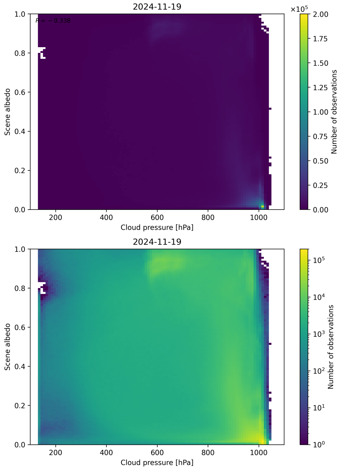
Figure 83: Scatter density plot of “Cloud pressure” against “Scene albedo” for 2024-11-18 to 2024-11-20.
