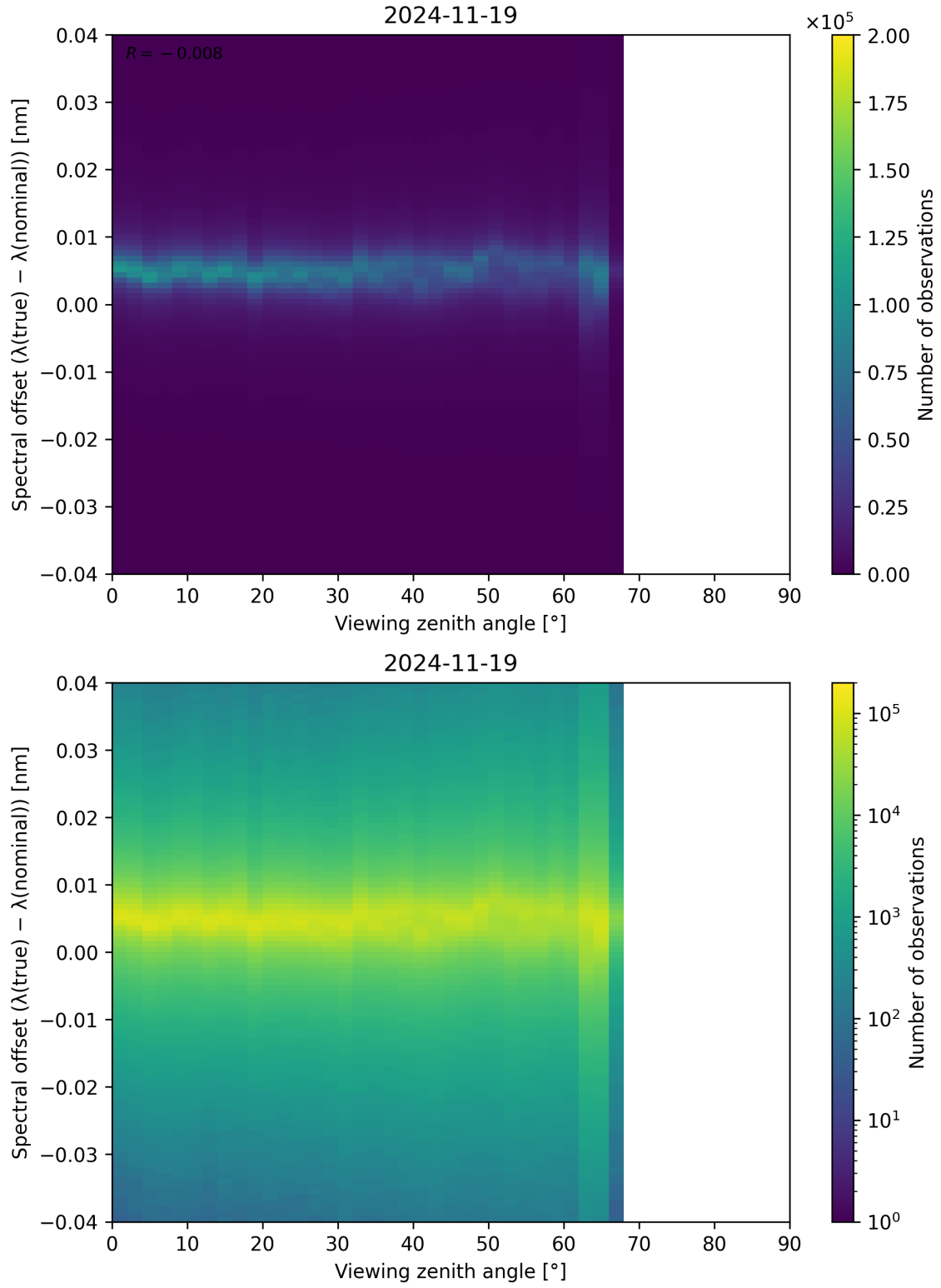
Figure 128: Scatter density plot of “Viewing zenith angle” against “Spectral offset ( \lambda_{\text{true}} - \lambda_{\text{nominal}} )” for 2024-11-18 to 2024-11-20.
