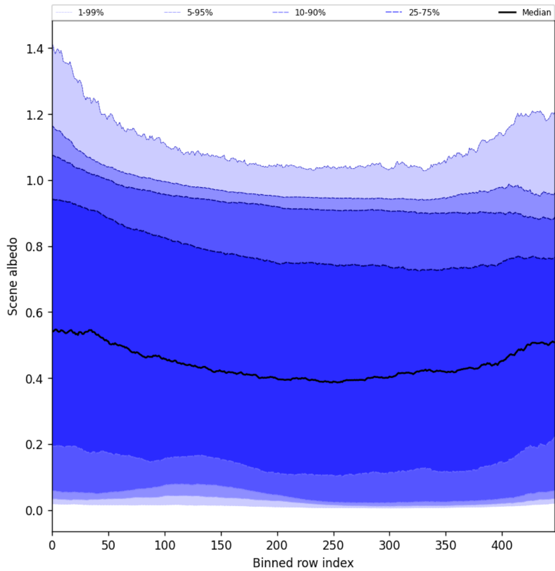
Figure 51: Along track statistics of “Scene albedo” for 2024-11-18 to 2024-11-20
