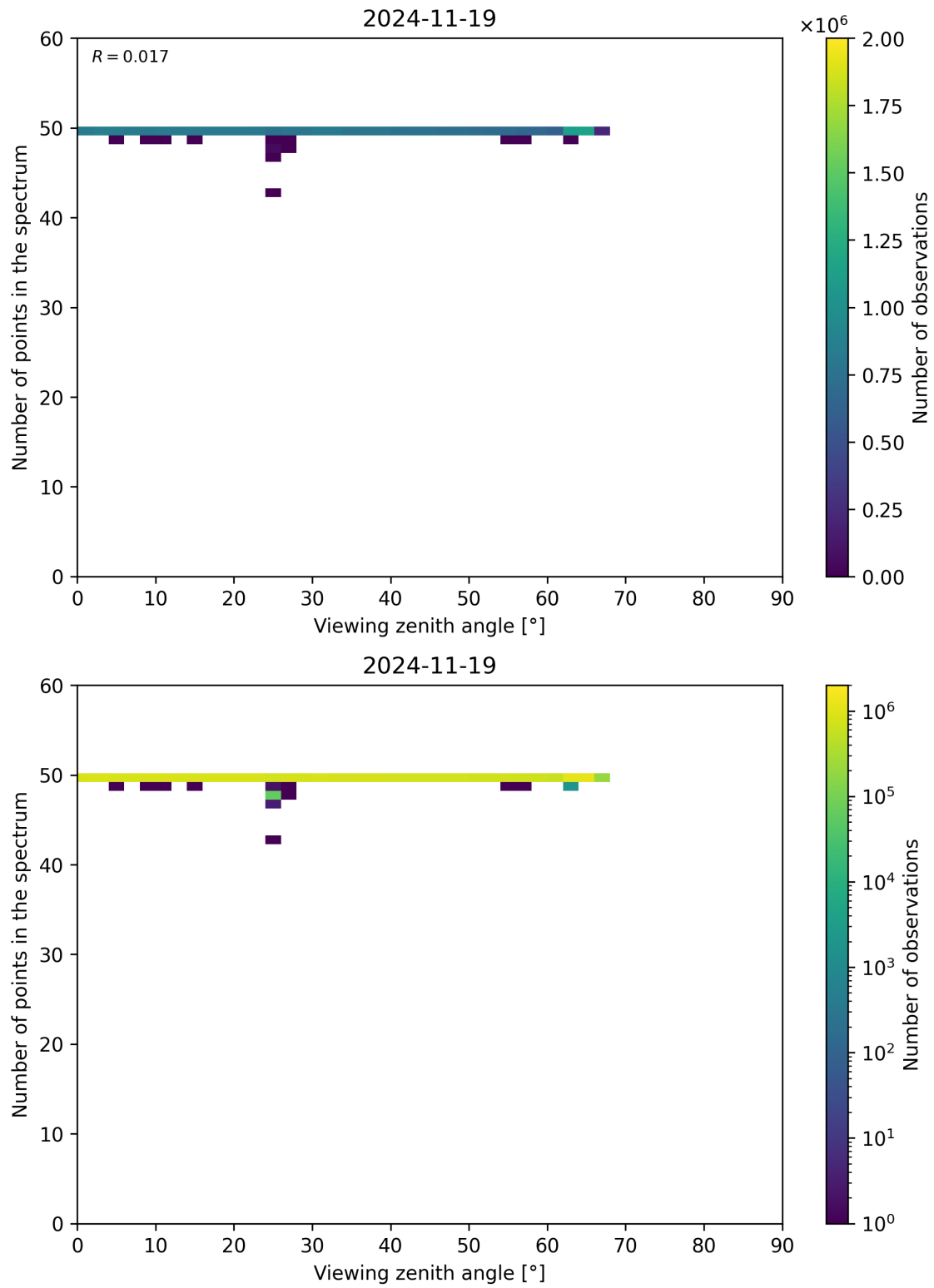
Figure 125: Scatter density plot of “Viewing zenith angle” against “Number of points in the spectrum” for 2024-11-18 to 2024-11-20.
