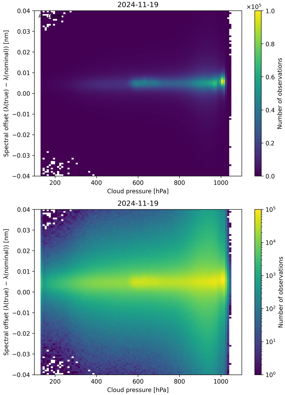
Figure 84: Scatter density plot of “Cloud pressure” against “Spectral offset ( \lambda_{\text{true}} - \lambda_{\text{nominal}} )” for 2024-11-18 to 2024-11-20.
