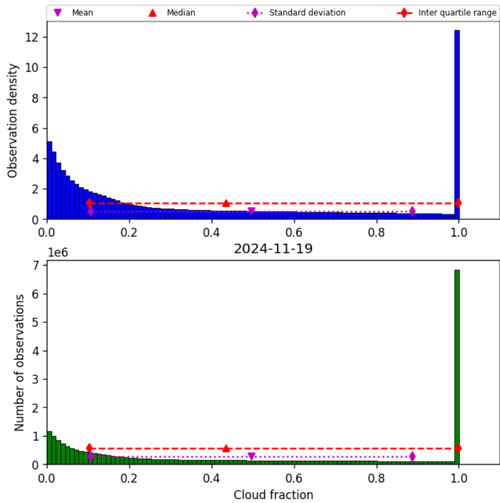
Figure 32: Histogram of “Cloud fraction” for 2024-11-18 to 2024-11-20
