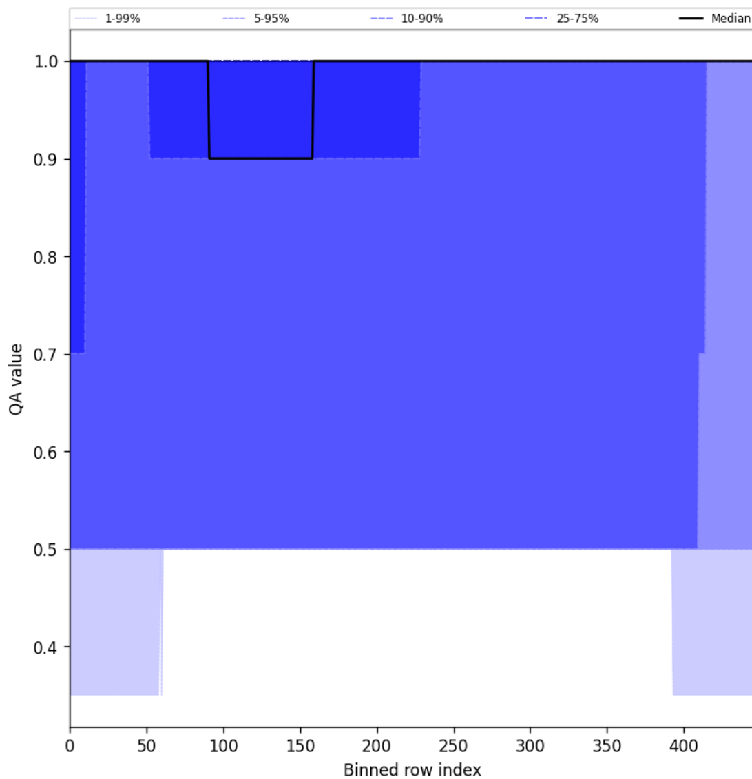
Figure 46: Along track statistics of “QA value” for 2024-11-18 to 2024-11-20
