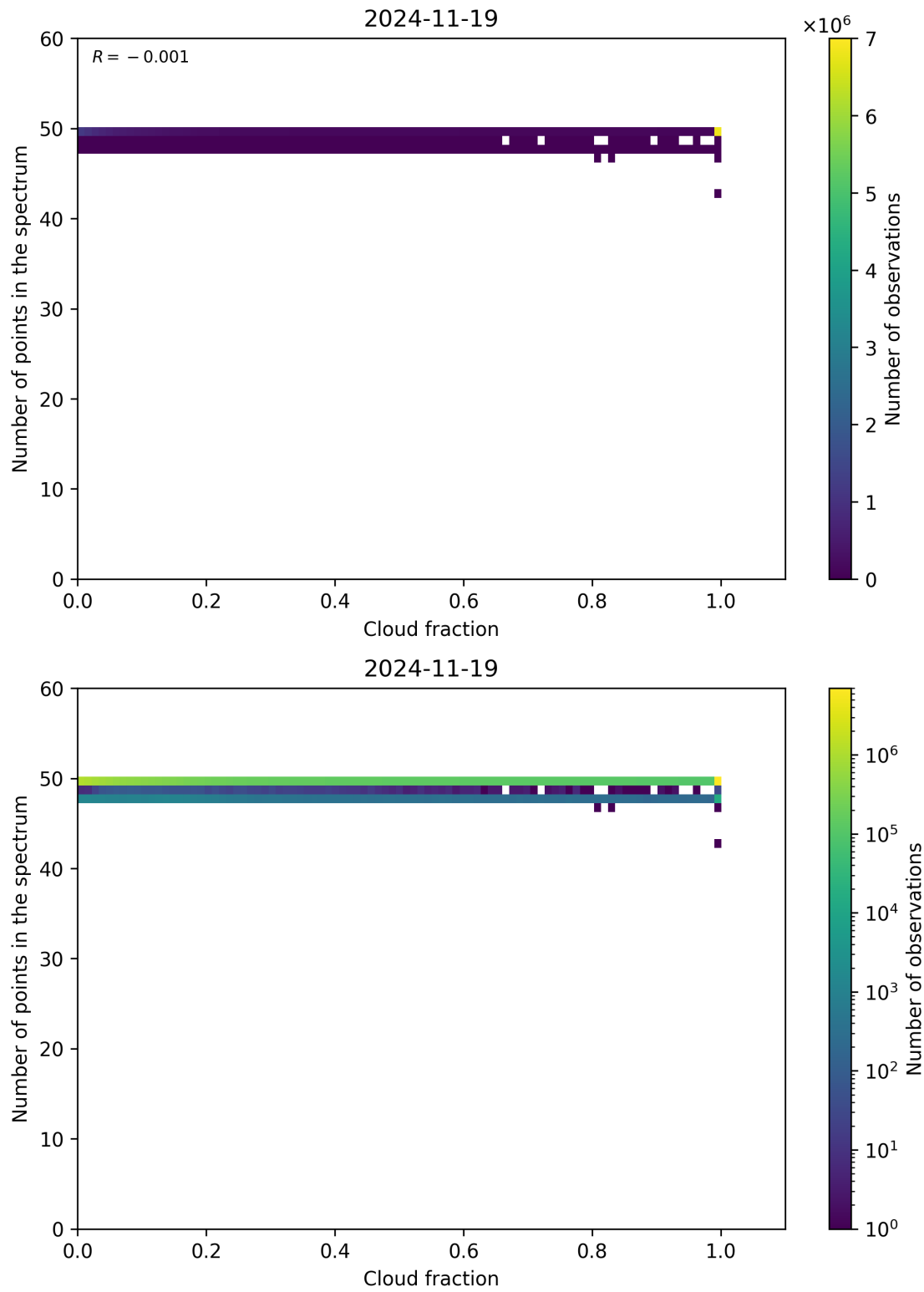
Figure 74: Scatter density plot of “Cloud fraction” against “Number of points in the spectrum” for 2024-11-18 to 2024-11-20.
