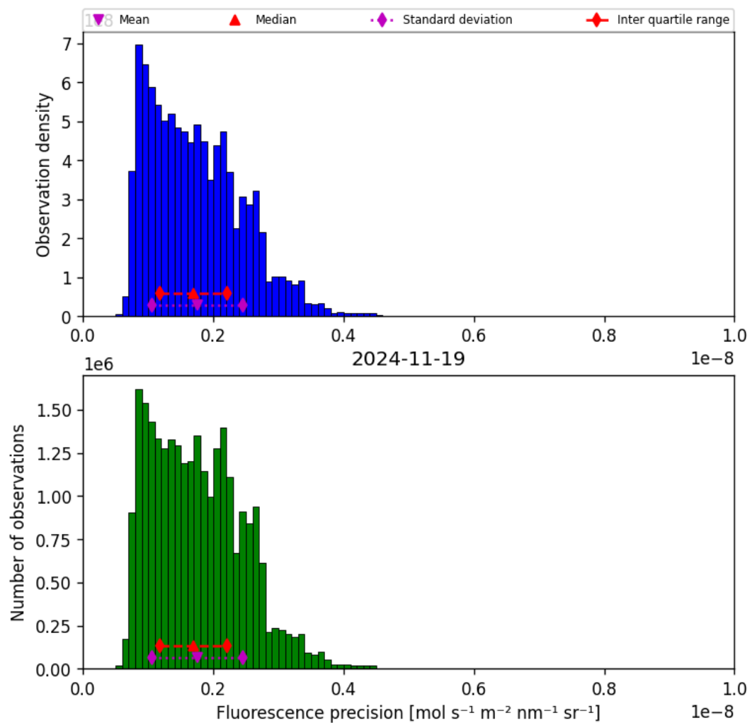
Figure 41: Histogram of “Fluorescence precision” for 2024-11-18 to 2024-11-20
