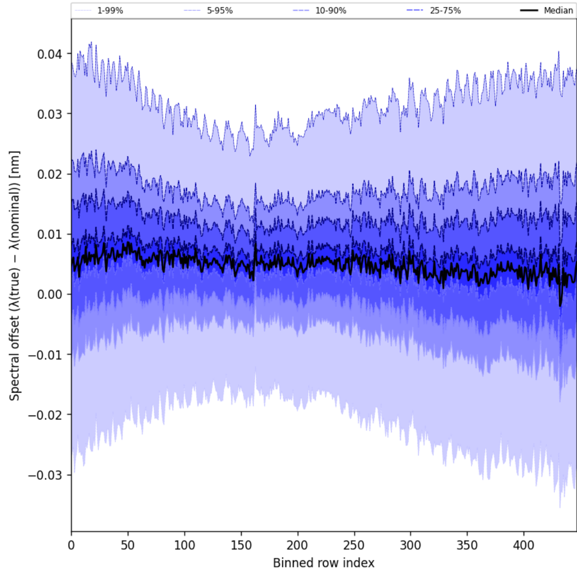
Figure 62: Along track statistics of “Spectral offset ( \lambda_{\text{true}} - \lambda_{\text{nominal}} )” for 2024-11-18 to 2024-11-20
