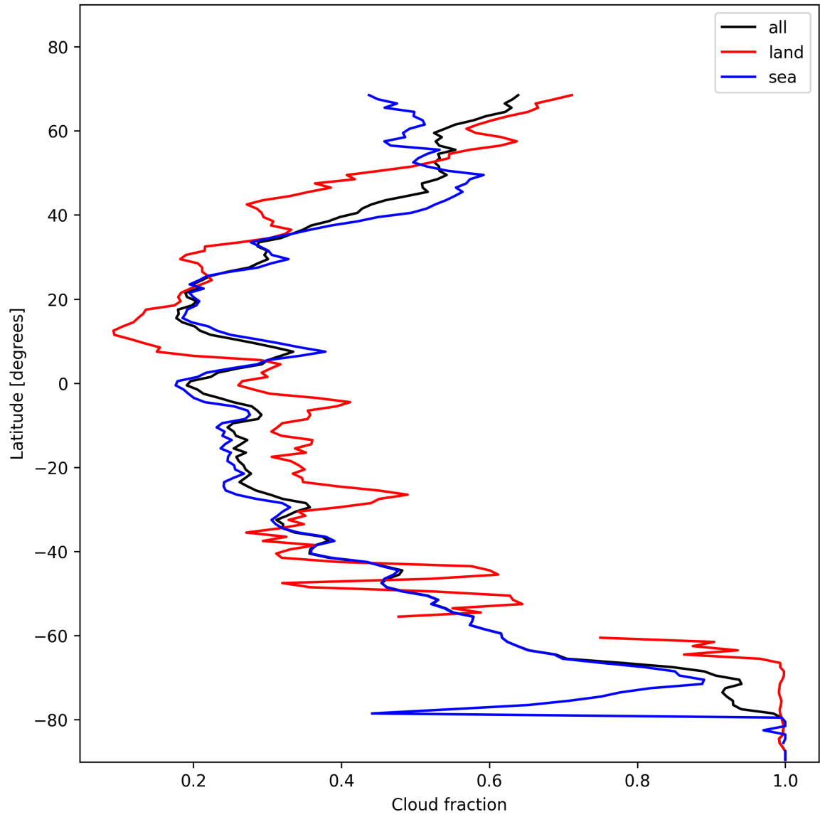
Figure 15: Zonal average of “Cloud fraction” for 2024-11-18 to 2024-11-20.
