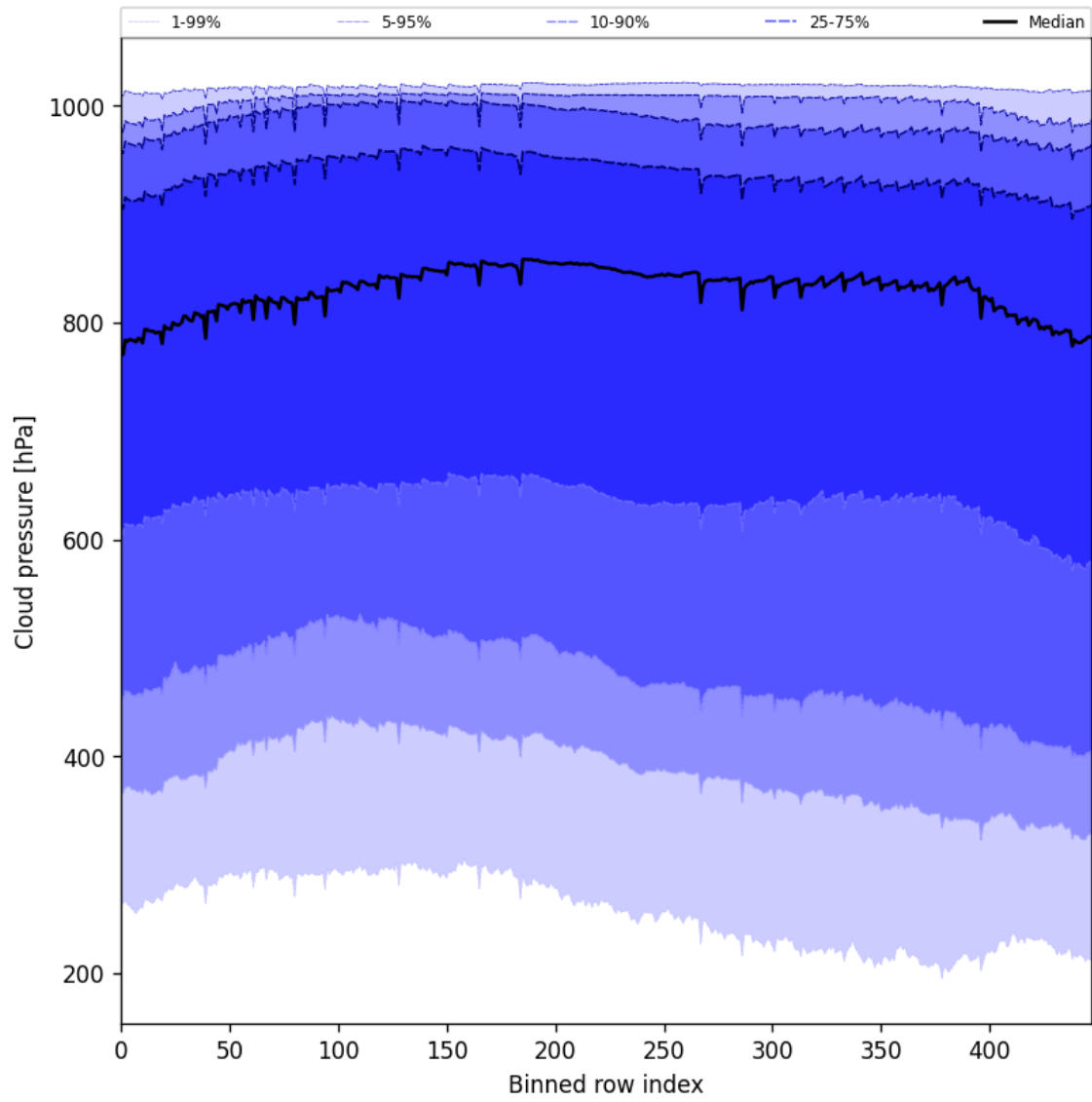
Figure 47: Along track statistics of “Cloud pressure” for 2024-11-18 to 2024-11-20
