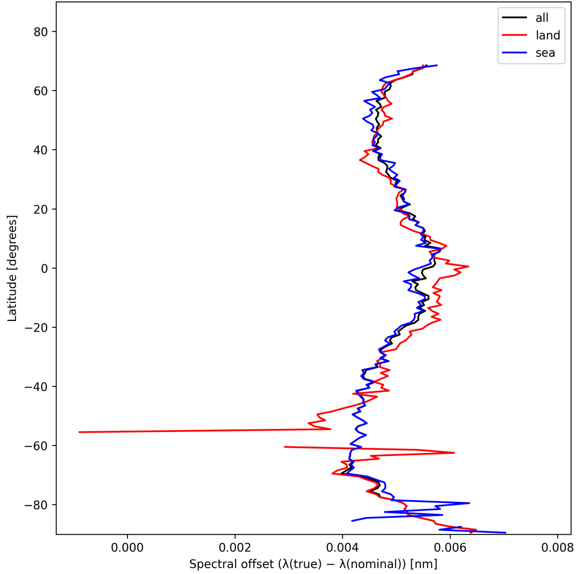
Figure 28: Zonal average of “Spectral offset ( \lambda_{\text{true}} - \lambda_{\text{nominal}} )” for 2024-11-18 to 2024-11-20.
