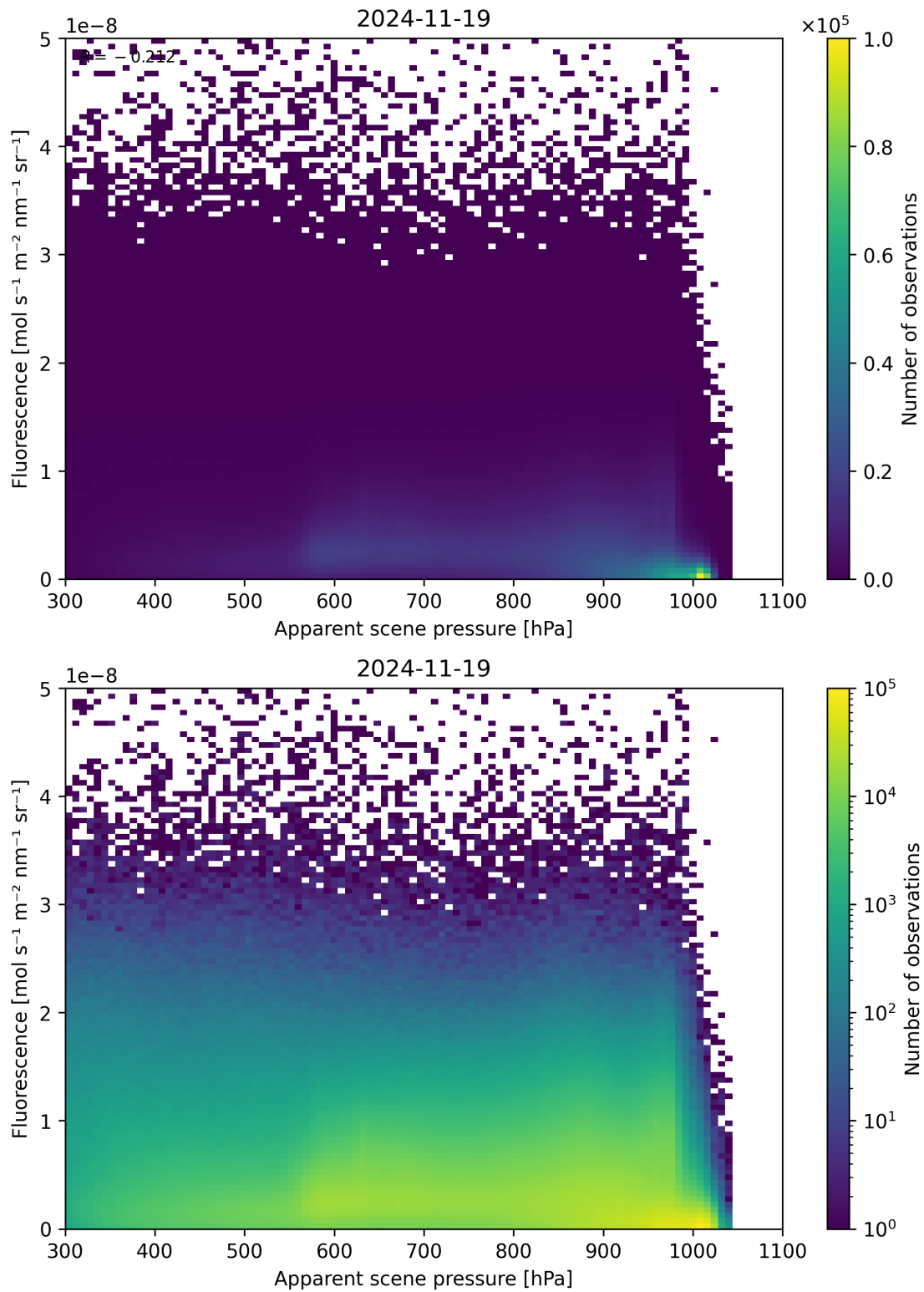
Figure 64: Scatter density plot of “Apparent scene pressure” against “Fluorescence” for 2024-11-18 to 2024-11-20.
