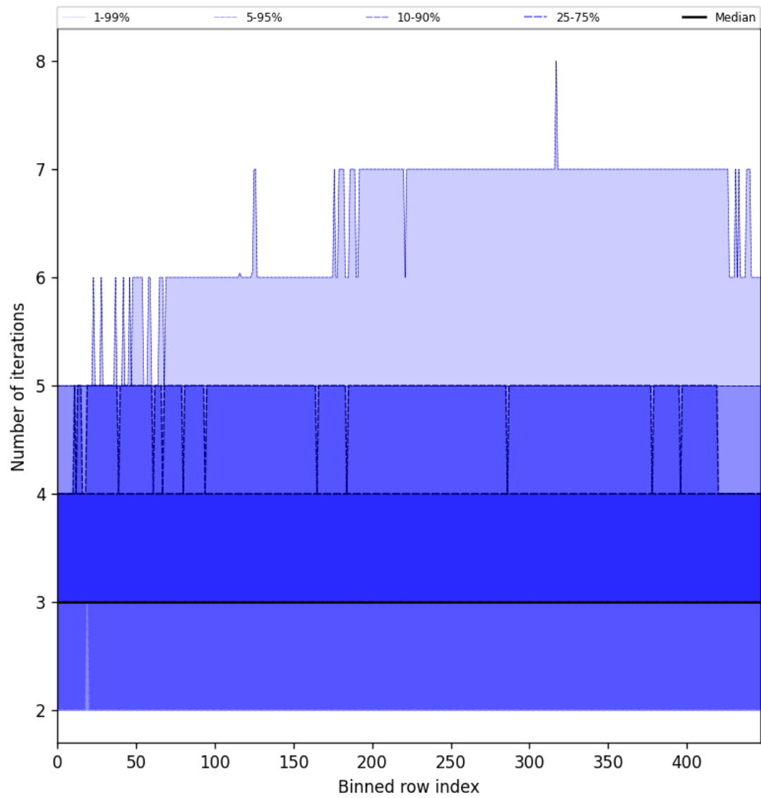
Figure 56: Along track statistics of “Number of iterations” for 2024-11-18 to 2024-11-20
