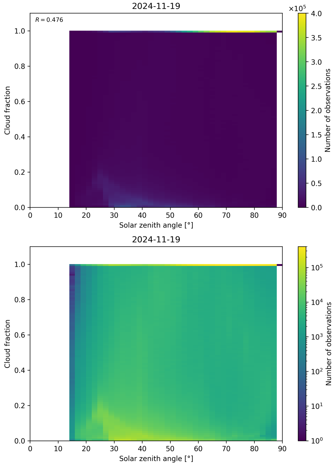
Figure 110: Scatter density plot of “Solar zenith angle” against “Cloud fraction” for 2024-11-18 to 2024-11-20.
