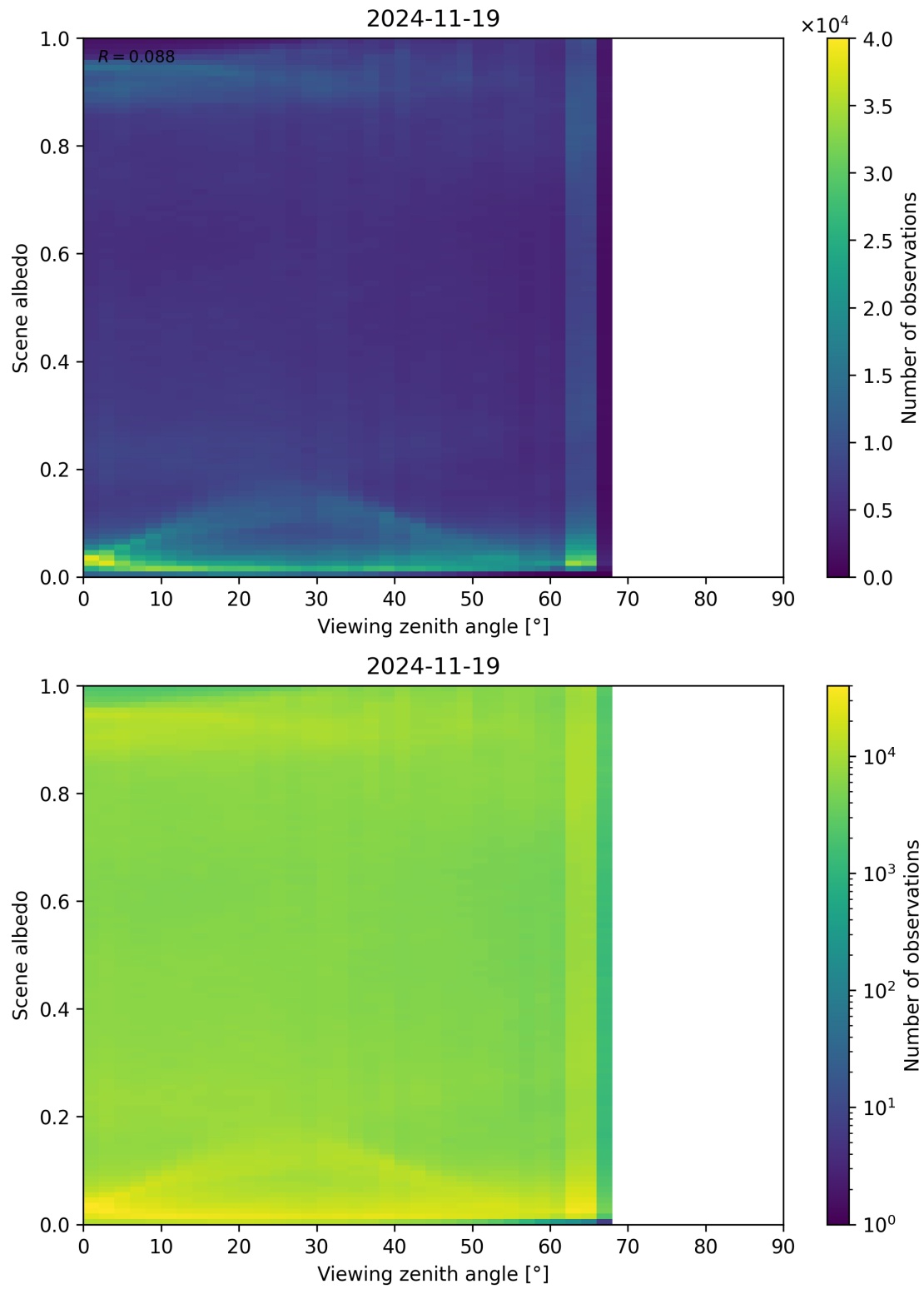
Figure 126: Scatter density plot of “Viewing zenith angle” against “Scene albedo” for 2024-11-18 to 2024-11-20.
