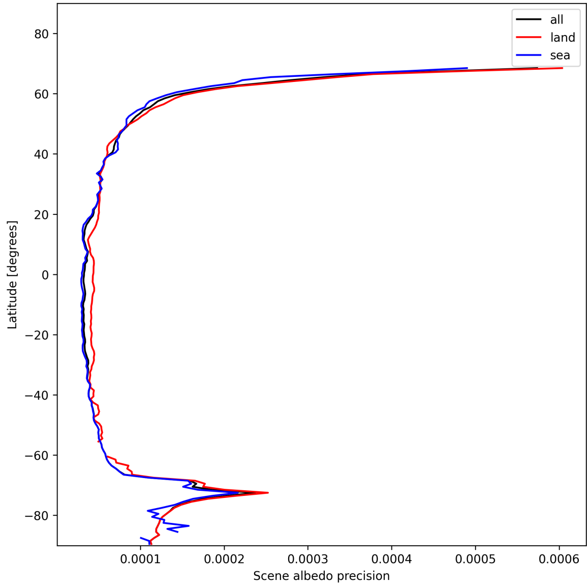
Figure 18: Zonal average of “Scene albedo precision” for 2024-11-18 to 2024-11-20.
