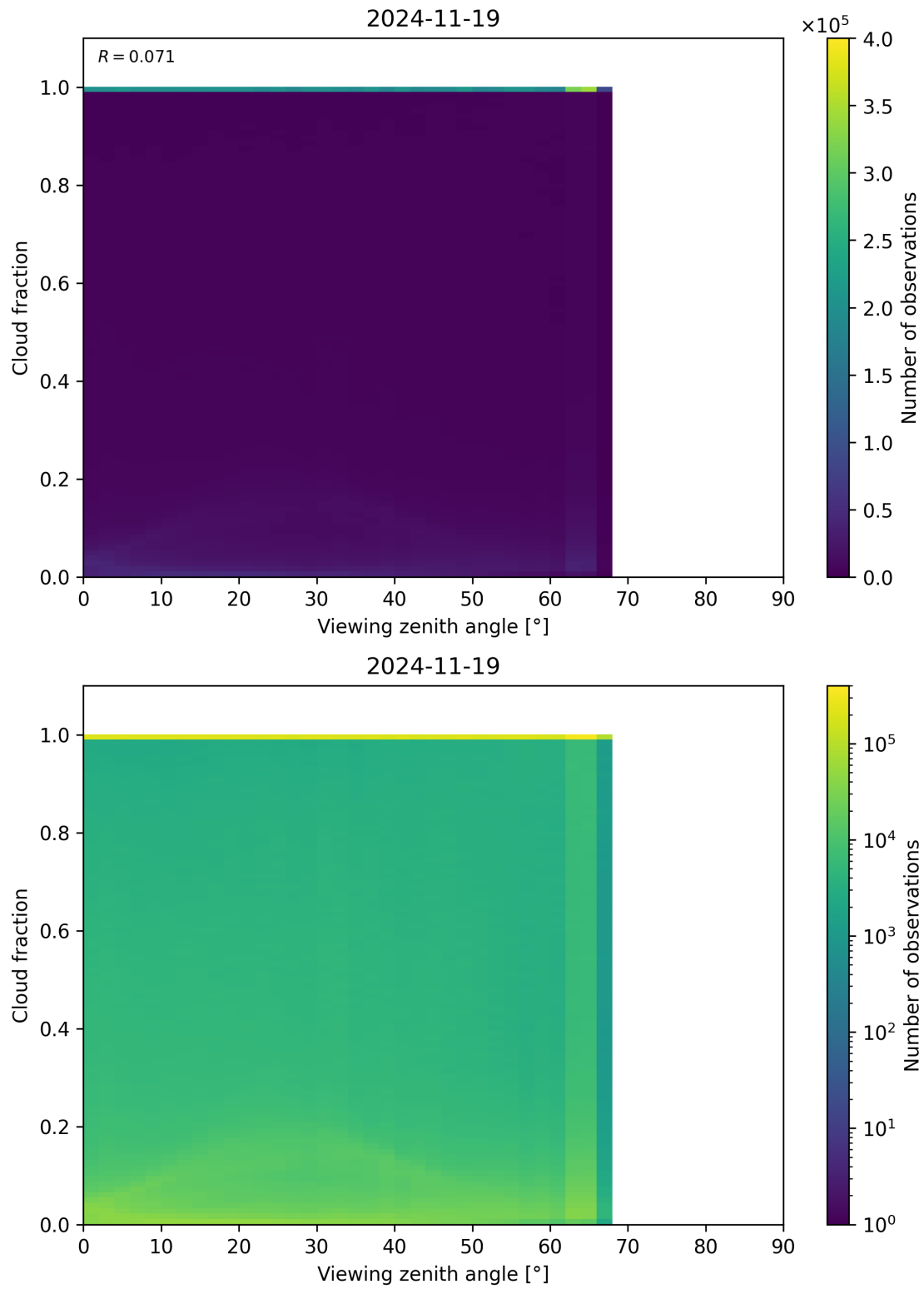
Figure 120: Scatter density plot of “Viewing zenith angle” against “Cloud fraction” for 2024-11-18 to 2024-11-20.
