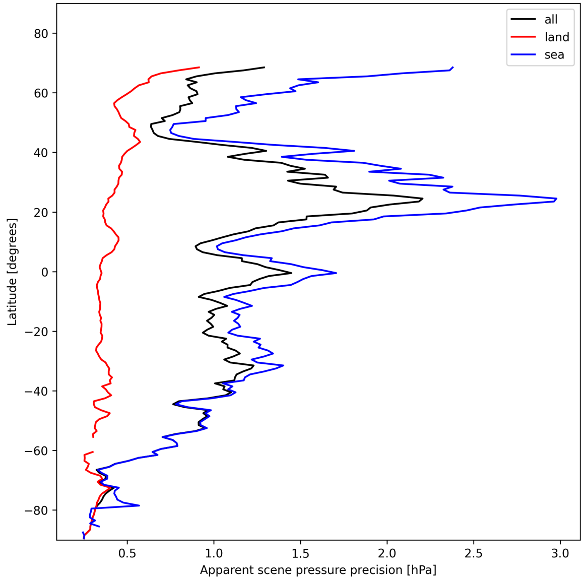
Figure 20: Zonal average of “Apparent scene pressure precision” for 2024-11-18 to 2024-11-20.
