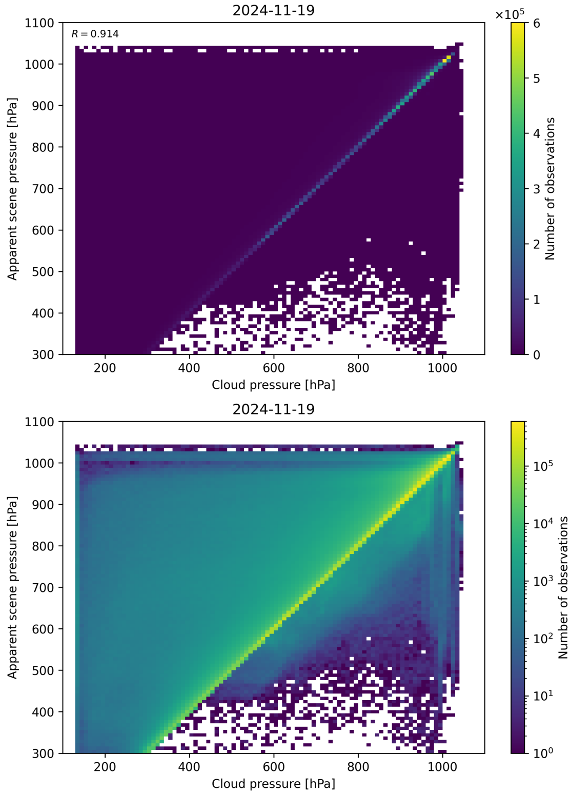
Figure 77: Scatter density plot of “Cloud pressure” against “Apparent scene pressure” for 2024-11-18 to 2024-11-20.
