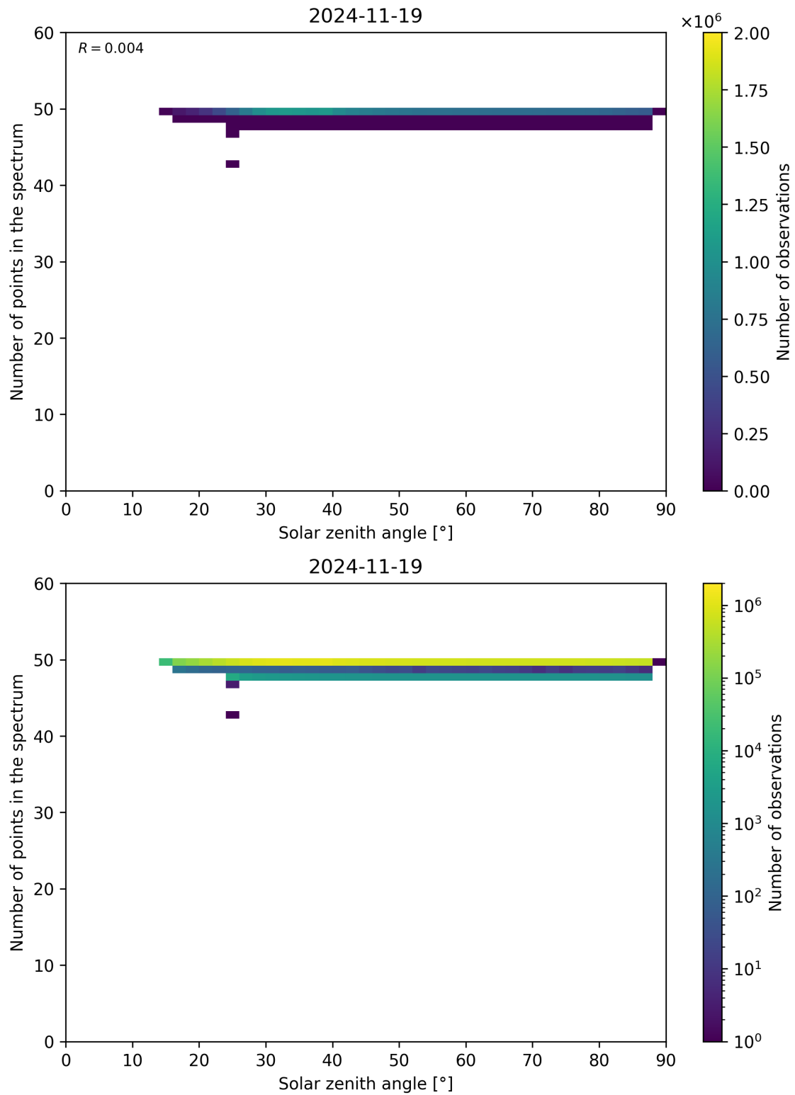
Figure 115: Scatter density plot of “Solar zenith angle” against “Number of points in the spectrum” for 2024-11-18 to 2024-11-20.
