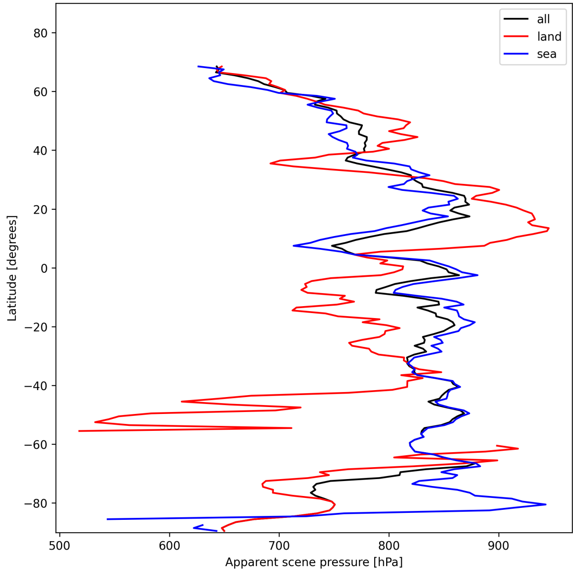
Figure 19: Zonal average of “Apparent scene pressure” for 2024-11-18 to 2024-11-20.
