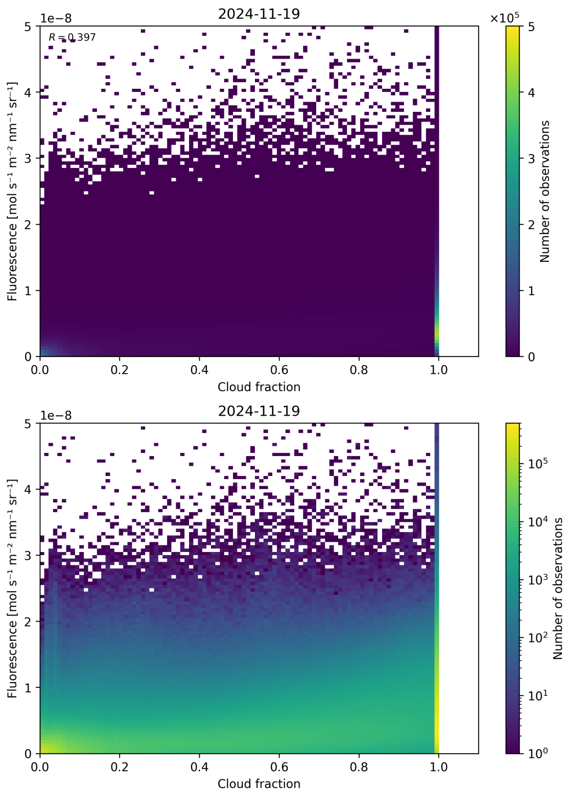
Figure 72: Scatter density plot of “Cloud fraction” against “Fluorescence” for 2024-11-18 to 2024-11-20.
