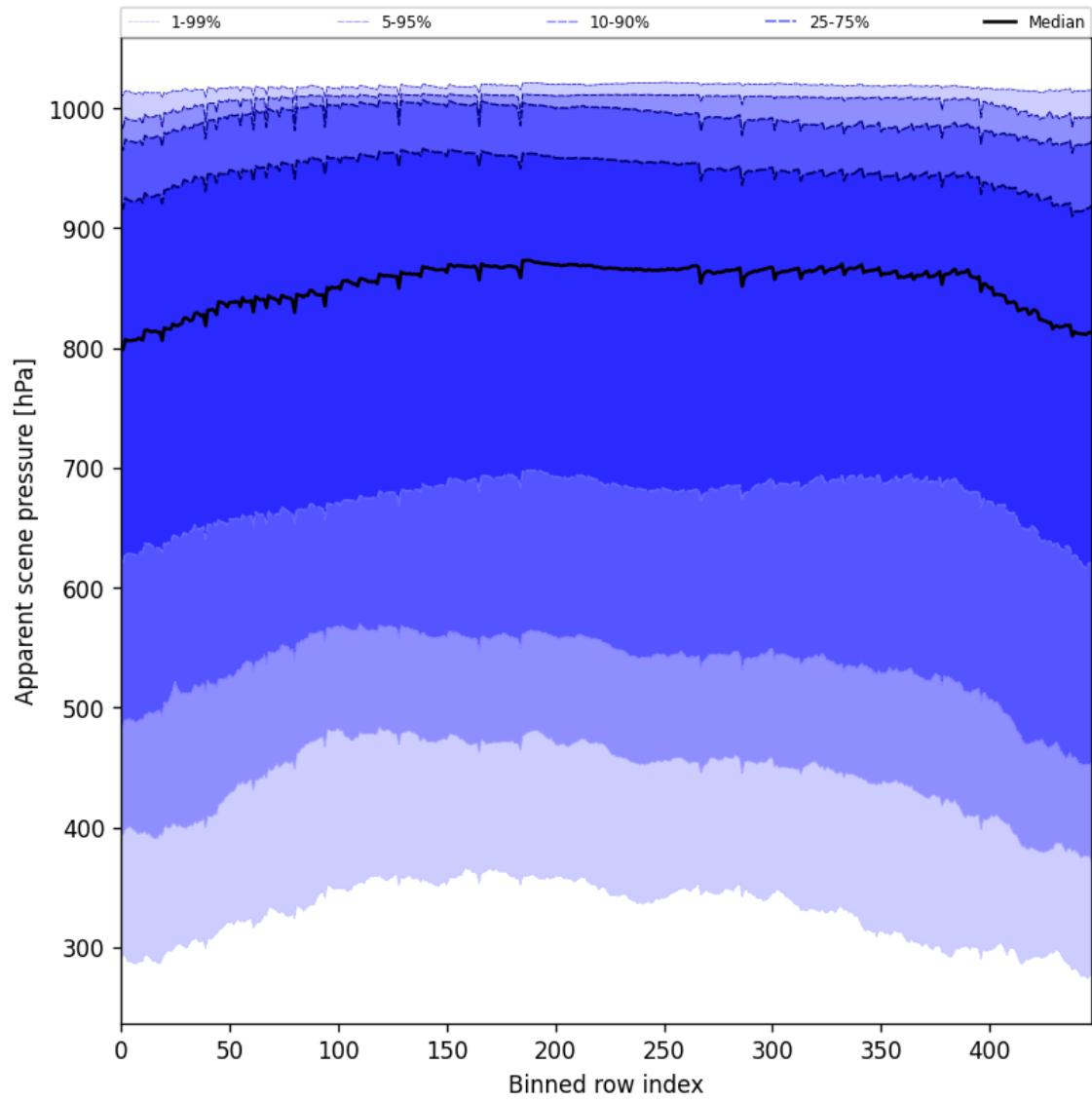
Figure 53: Along track statistics of “Apparent scene pressure” for 2024-11-18 to 2024-11-20
