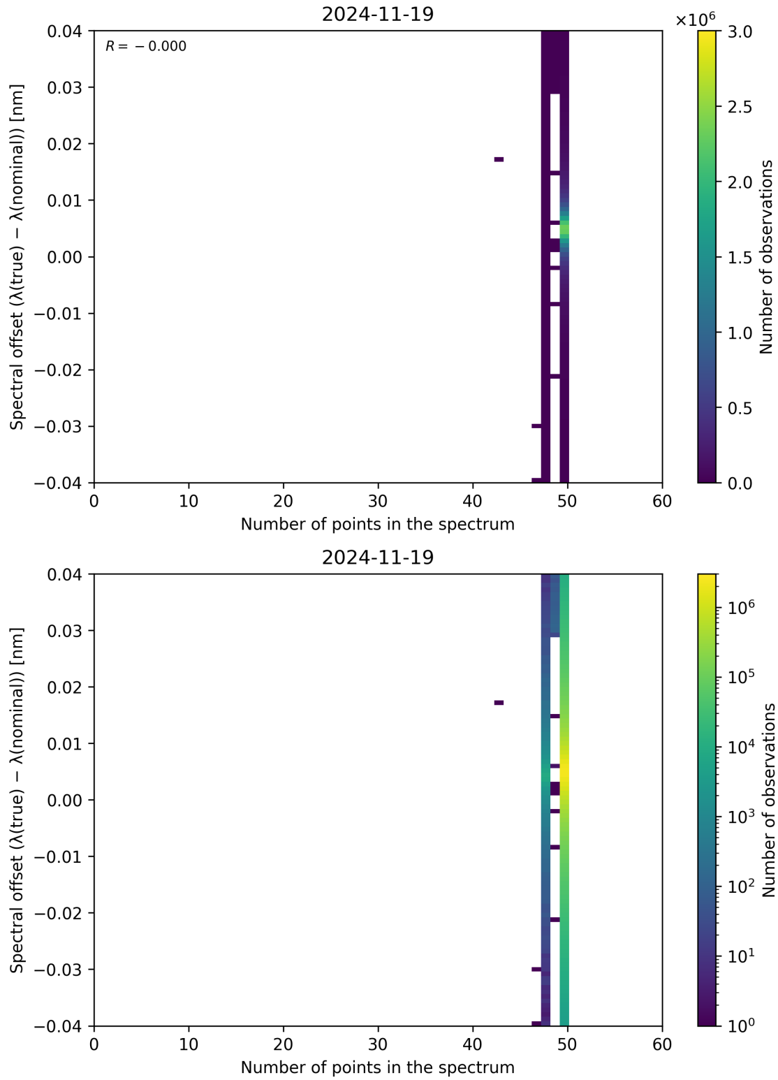
Figure 101: Scatter density plot of “Number of points in the spectrum” against “Spectral offset ( \lambda_{\text{true}} - \lambda_{\text{nominal}} )” for 2024-11-18 to 2024-11-20.
