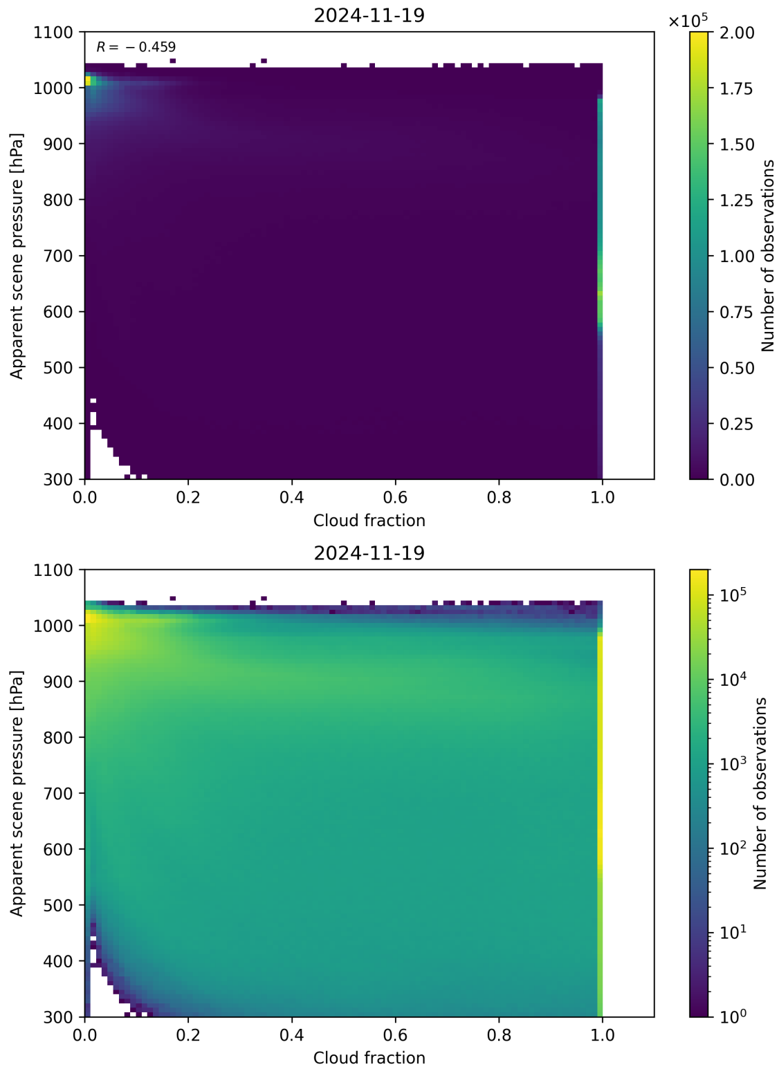
Figure 70: Scatter density plot of “Cloud fraction” against “Apparent scene pressure” for 2024-11-18 to 2024-11-20.
