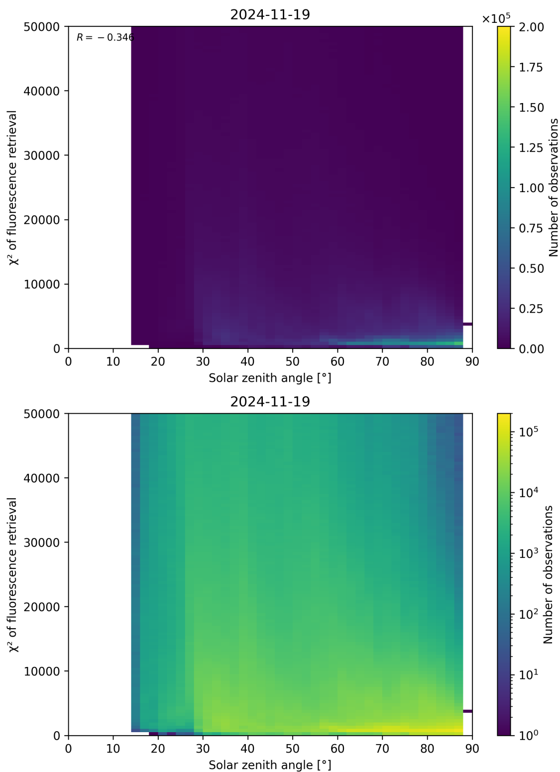
Figure 109: Scatter density plot of “Solar zenith angle” against “ \chi^2 of fluorescence retrieval” for 2024-11-18 to 2024-11-20.
