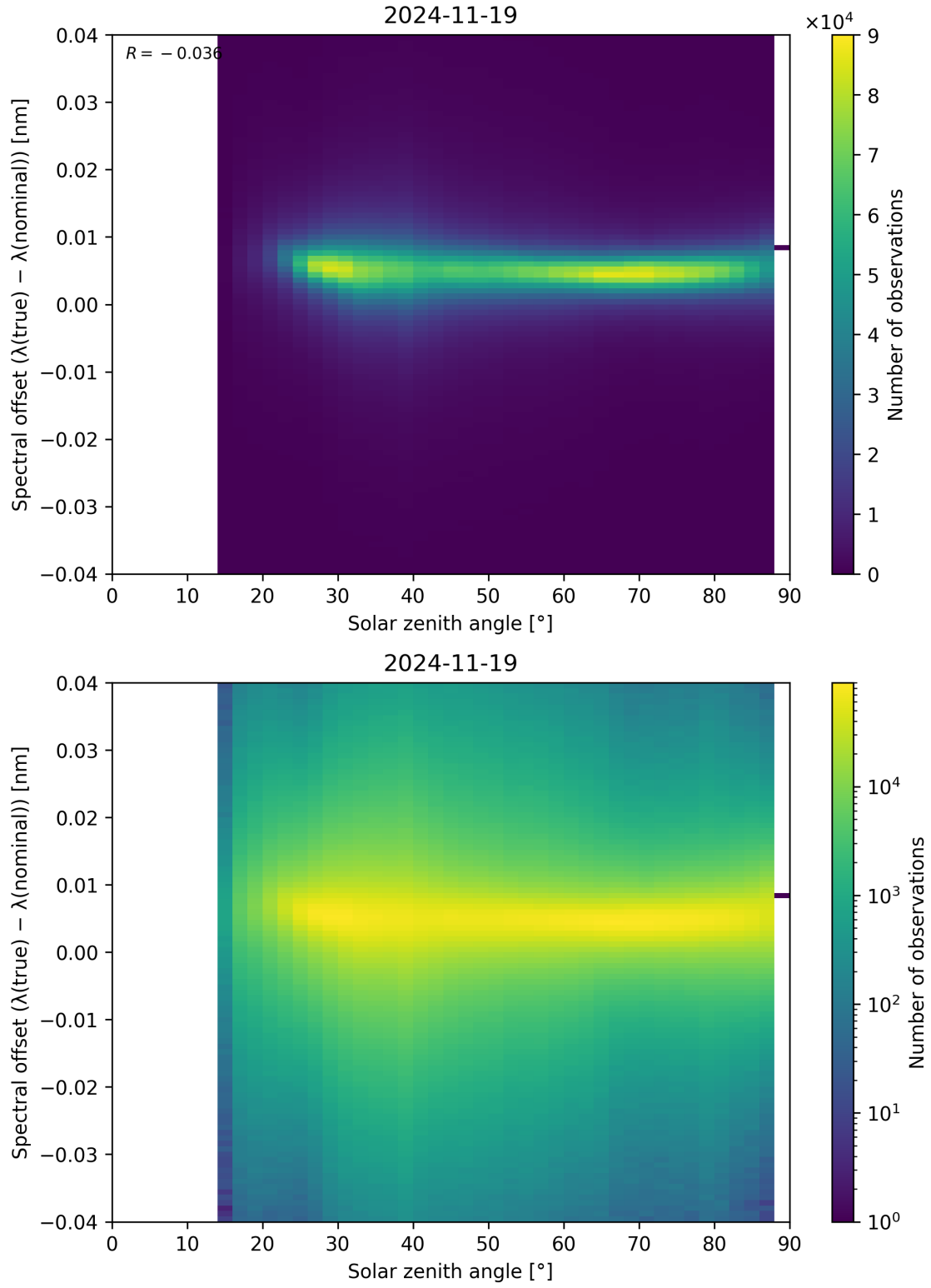
Figure 117: Scatter density plot of “Solar zenith angle” against “Spectral offset ( \lambda_{\text{true}} - \lambda_{\text{nominal}} )” for 2024-11-18 to 2024-11-20.
