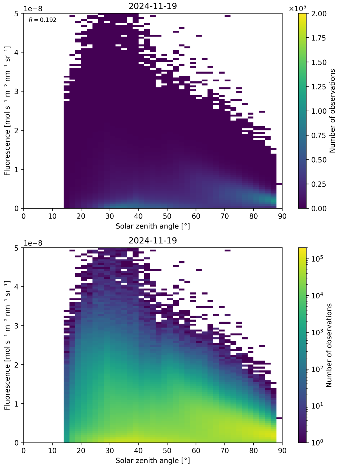
Figure 112: Scatter density plot of “Solar zenith angle” against “Fluorescence” for 2024-11-18 to 2024-11-20.
