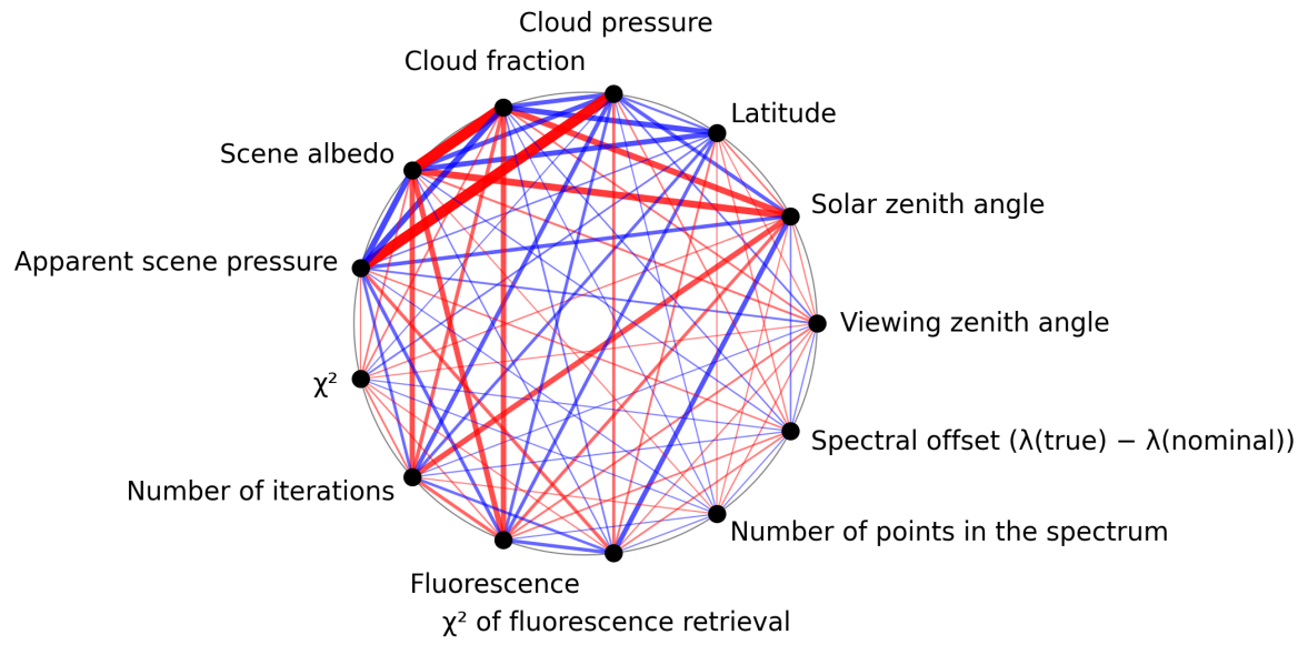
Figure 1: Map of correlation graph for 2024-11-18 to 2024-11-20.
