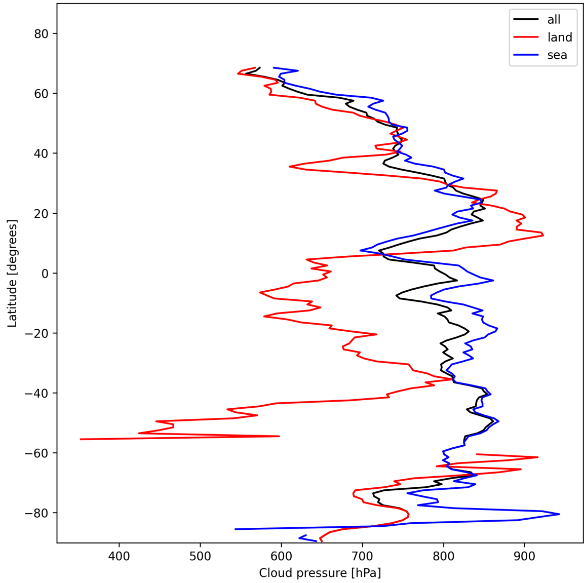
Figure 13: Zonal average of “Cloud pressure” for 2024-11-18 to 2024-11-20.
