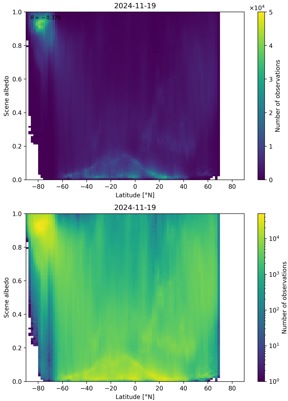
Figure 95: Scatter density plot of “Latitude” against “Scene albedo” for 2024-11-18 to 2024-11-20.
