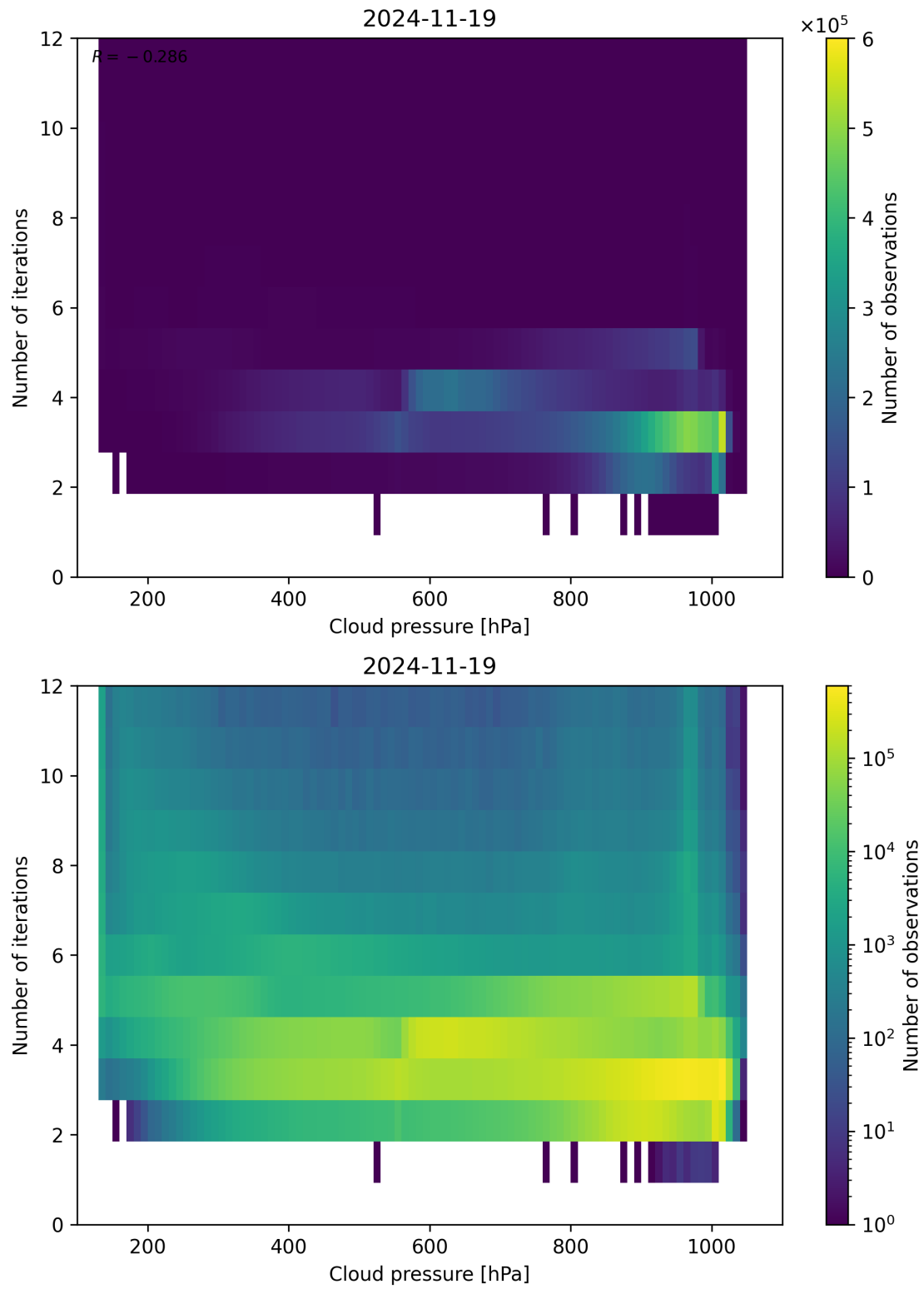
Figure 81: Scatter density plot of “Cloud pressure” against “Number of iterations” for 2024-11-18 to 2024-11-20.
