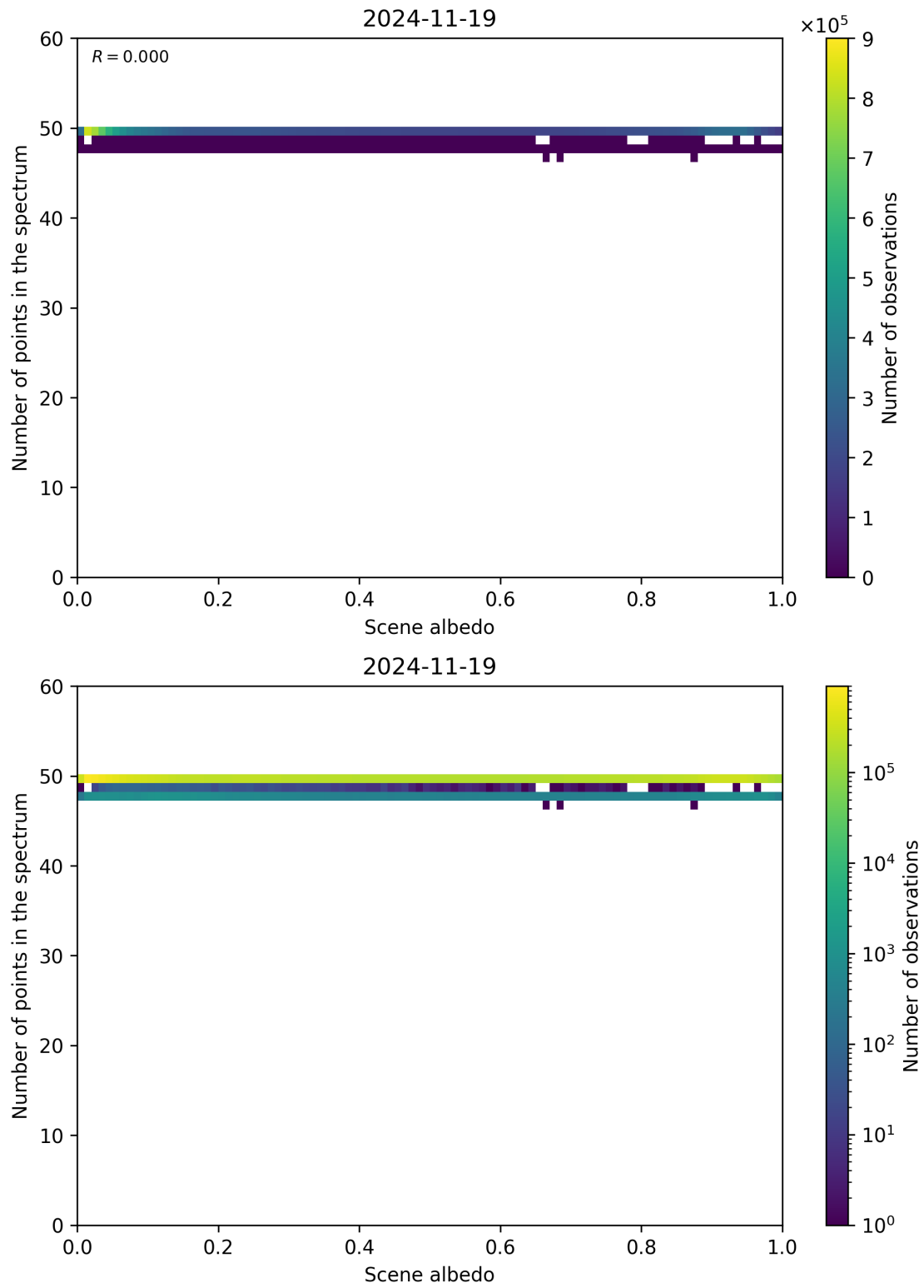
Figure 106: Scatter density plot of “Scene albedo” against “Number of points in the spectrum” for 2024-11-18 to 2024-11-20.
