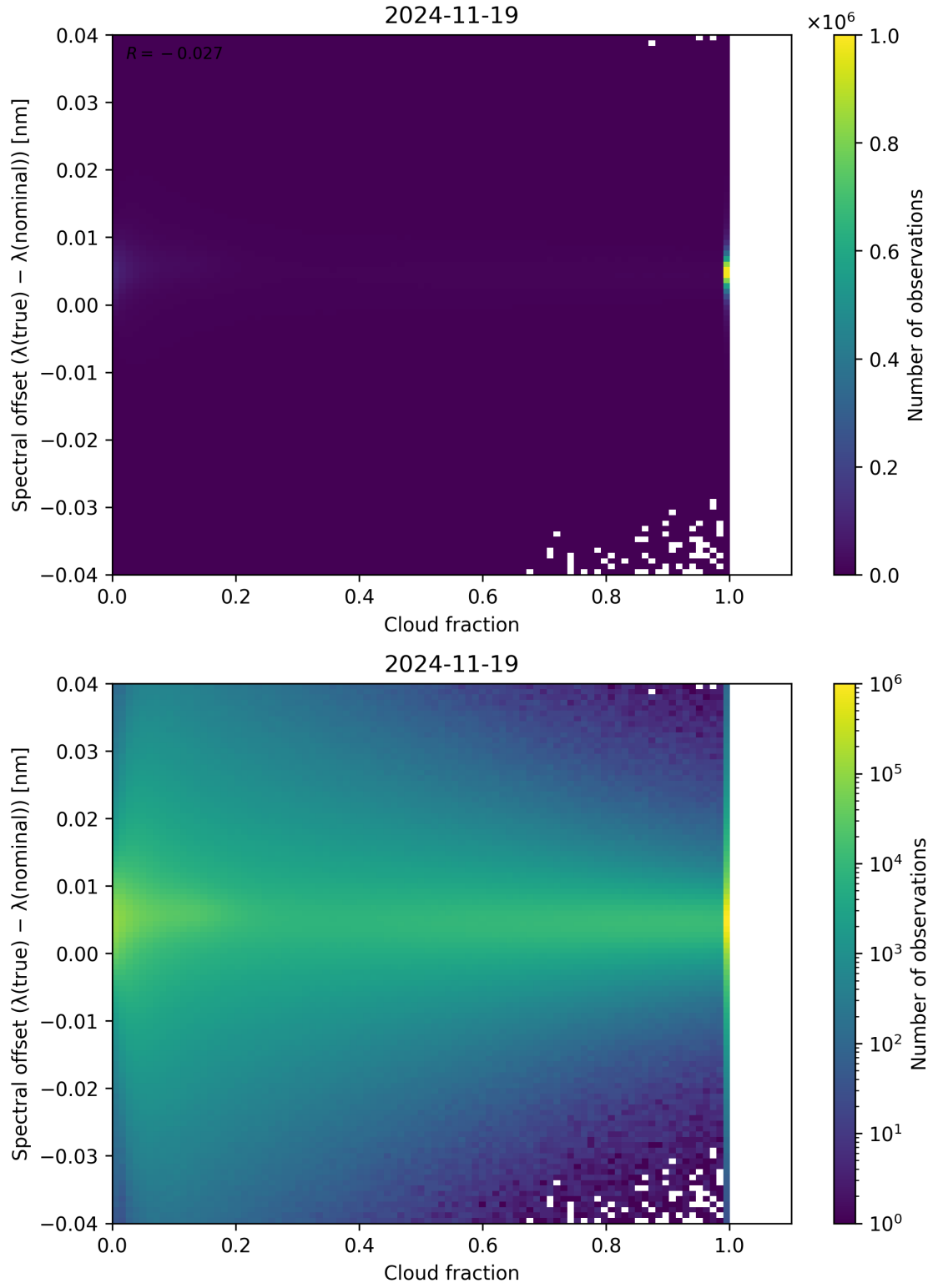
Figure 76: Scatter density plot of “Cloud fraction” against “Spectral offset ( \lambda_{\text{true}} - \lambda_{\text{nominal}} )” for 2024-11-18 to 2024-11-20.
