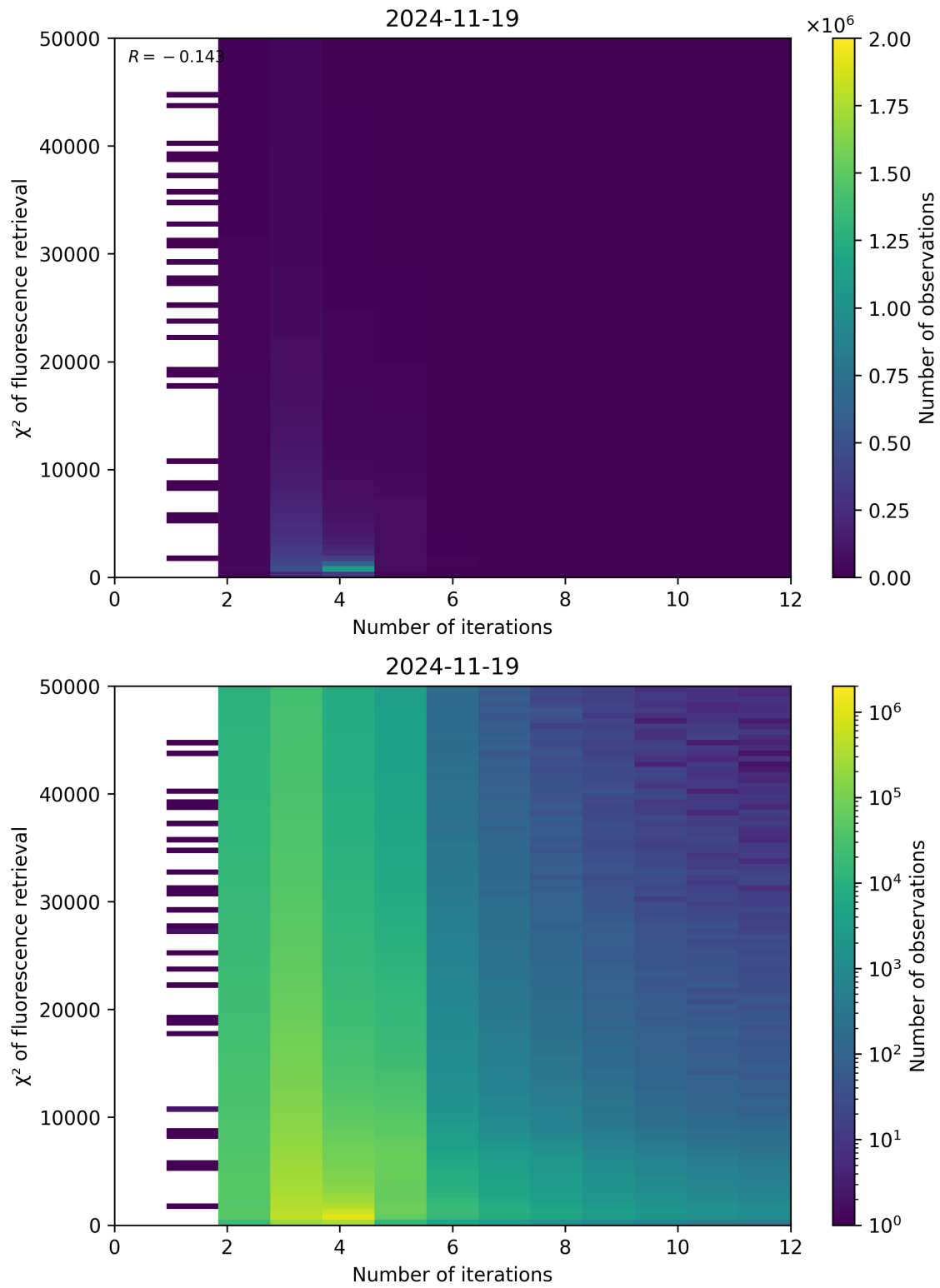
Figure 97: Scatter density plot of “Number of iterations” against “ \chi^2 of fluorescence retrieval” for 2024-11-18 to 2024-11-20.
