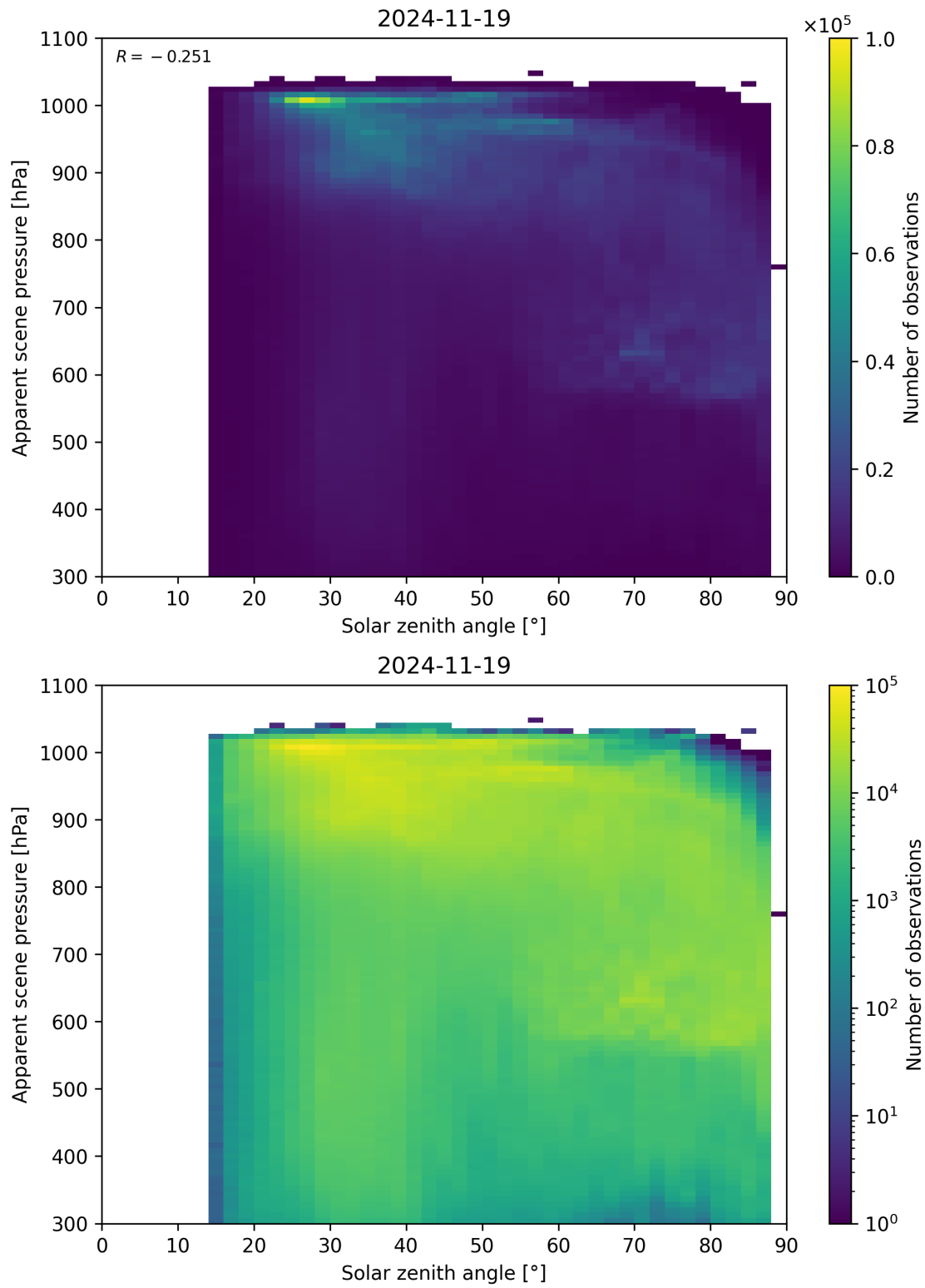
Figure 108: Scatter density plot of “Solar zenith angle” against “Apparent scene pressure” for 2024-11-18 to 2024-11-20.
