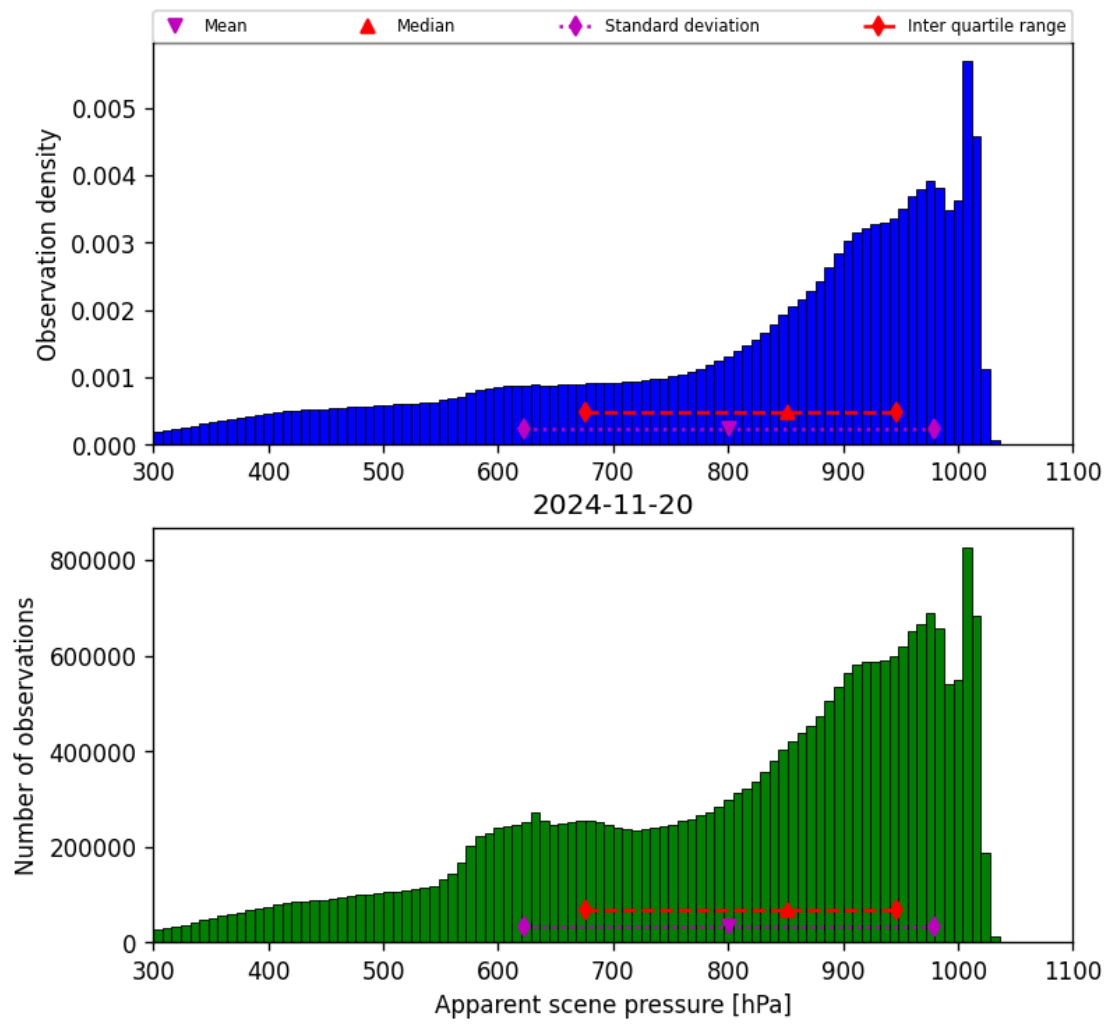
Figure 36: Histogram of “Apparent scene pressure” for 2024-11-20 to 2024-11-21
