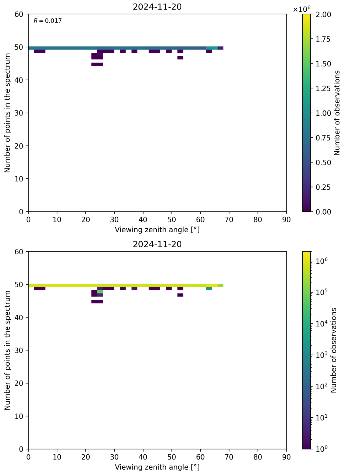
Figure 125: Scatter density plot of “Viewing zenith angle” against “Number of points in the spectrum” for 2024-11-20 to 2024-11-21.
