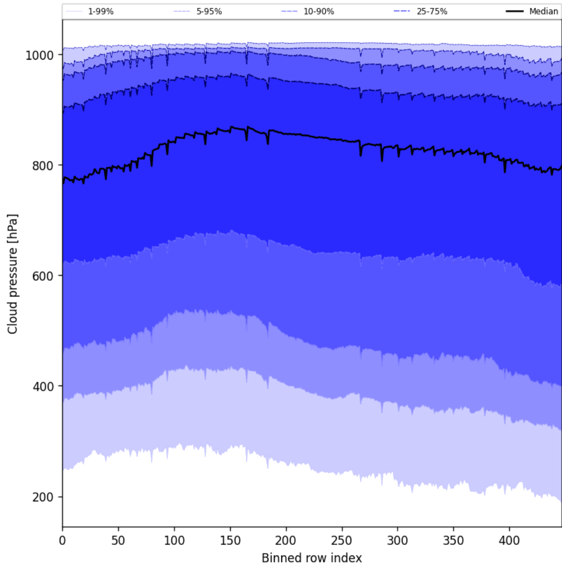
Figure 47: Along track statistics of “Cloud pressure” for 2024-11-20 to 2024-11-21
