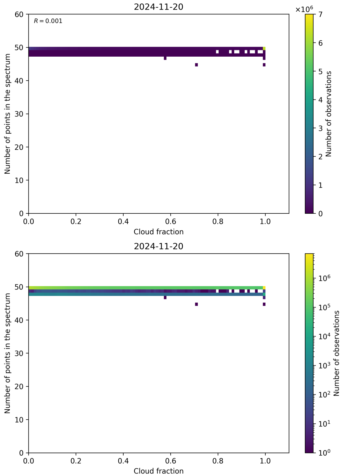
Figure 74: Scatter density plot of “Cloud fraction” against “Number of points in the spectrum” for 2024-11-20 to 2024-11-21.
