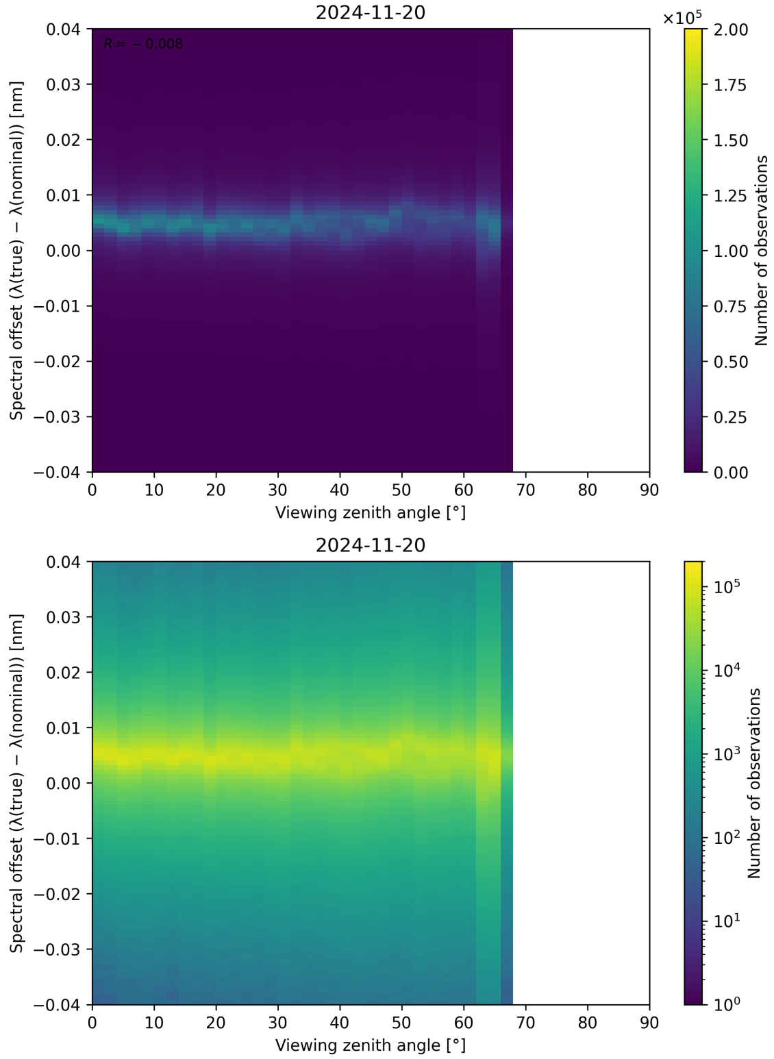
Figure 128: Scatter density plot of “Viewing zenith angle” against “Spectral offset ( \lambda_{\text{true}} - \lambda_{\text{nominal}} )” for 2024-11-20 to 2024-11-21.
