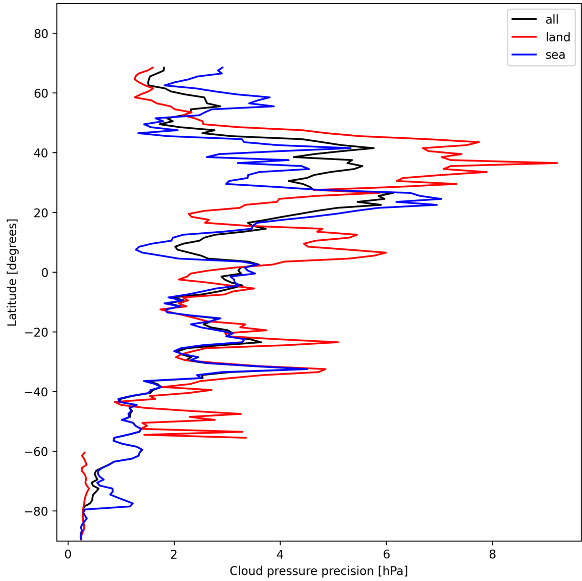
Figure 14: Zonal average of “Cloud pressure precision” for 2024-11-20 to 2024-11-21.
