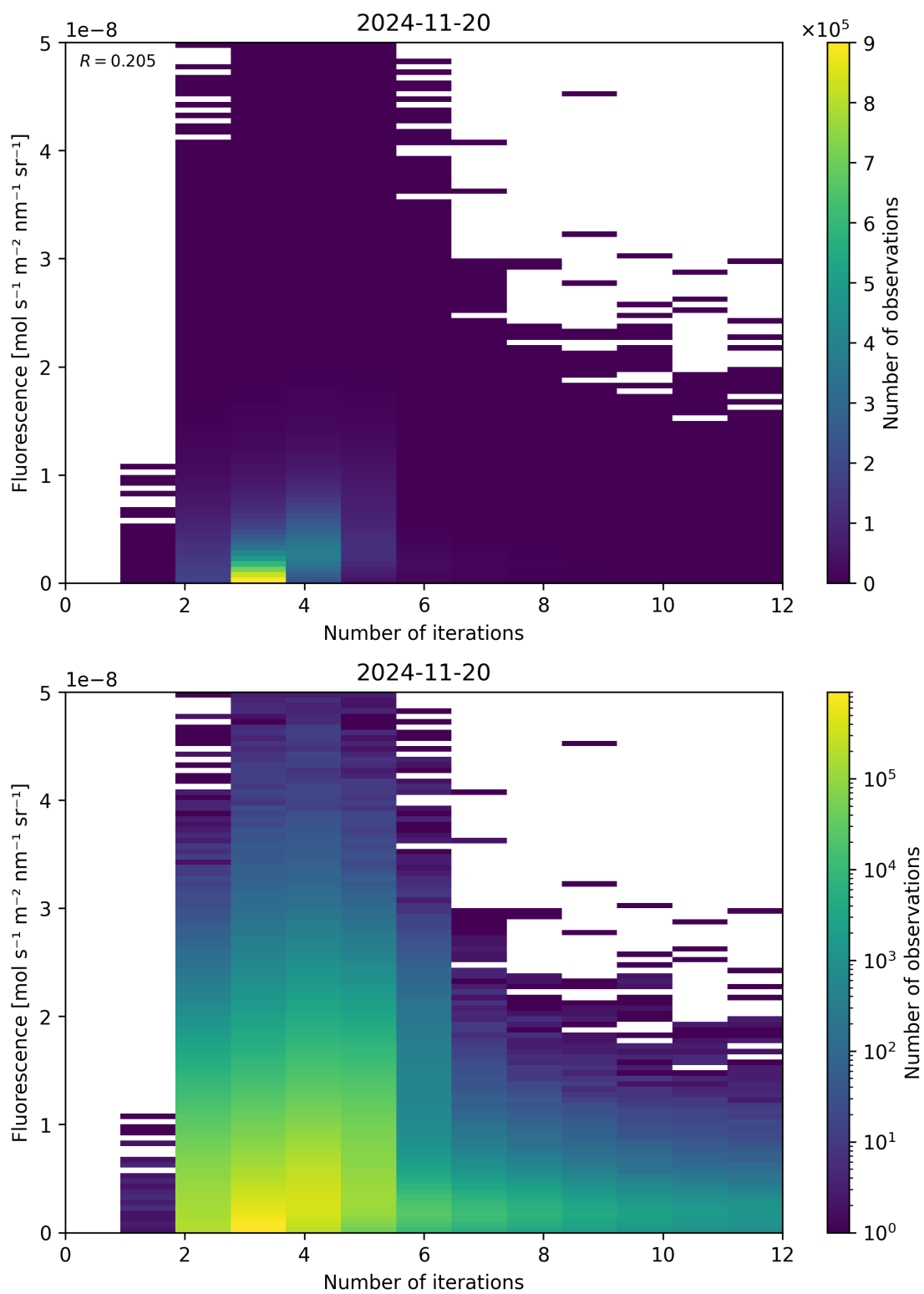
Figure 98: Scatter density plot of “Number of iterations” against “Fluorescence” for 2024-11-20 to 2024-11-21.
