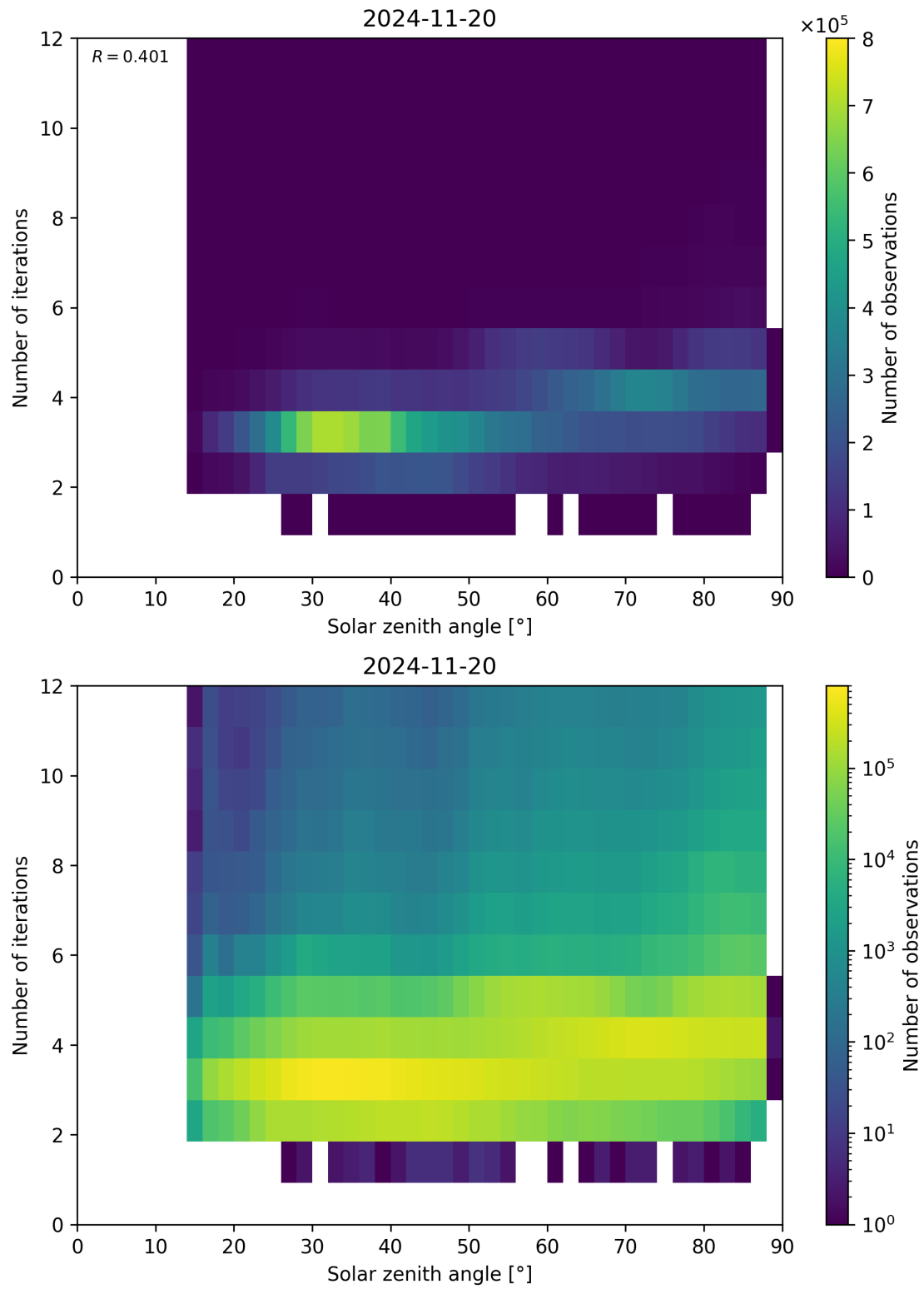
Figure 114: Scatter density plot of “Solar zenith angle” against “Number of iterations” for 2024-11-20 to 2024-11-21.
