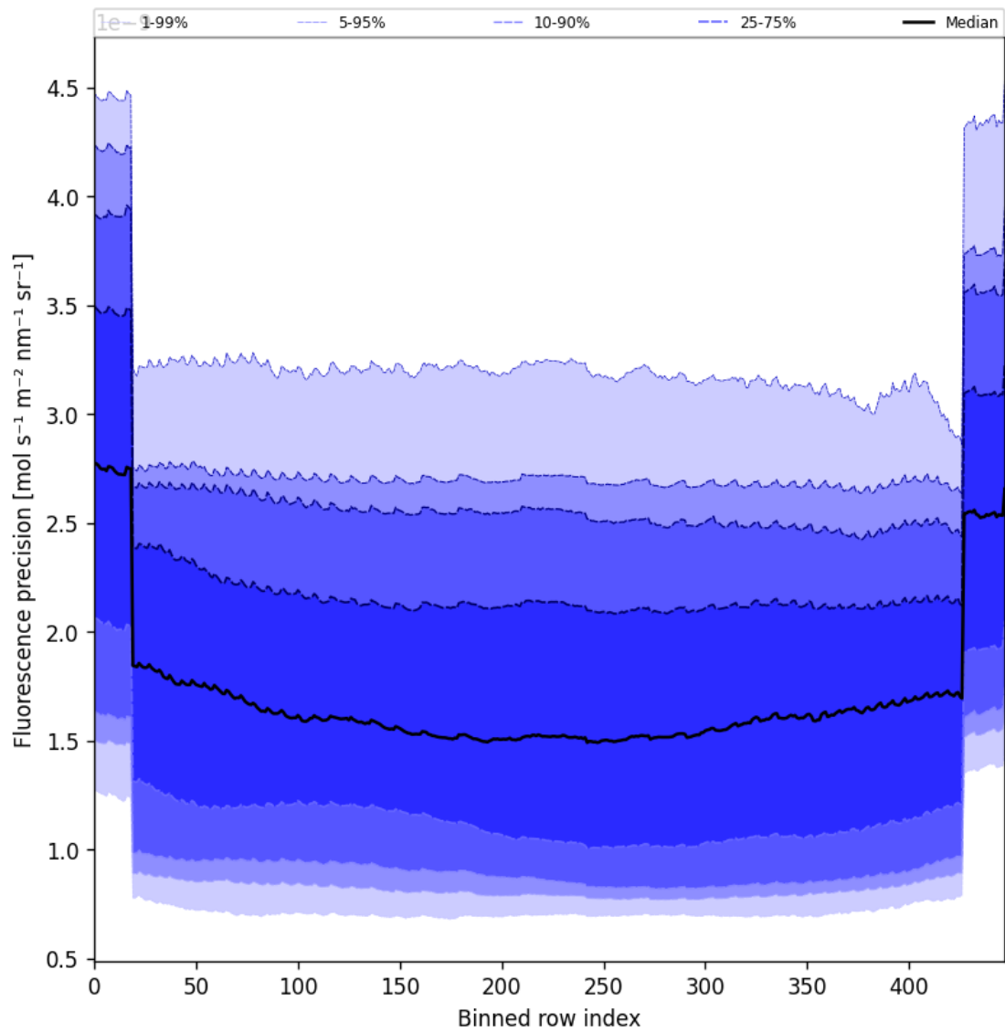
Figure 58: Along track statistics of “Fluorescence precision” for 2024-11-20 to 2024-11-21
