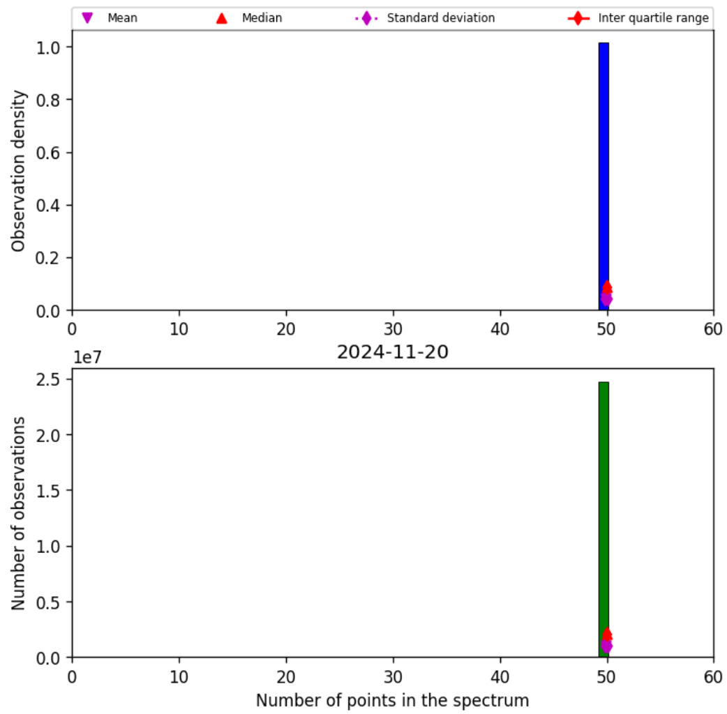
Figure 44: Histogram of “Number of points in the spectrum” for 2024-11-20 to 2024-11-21
