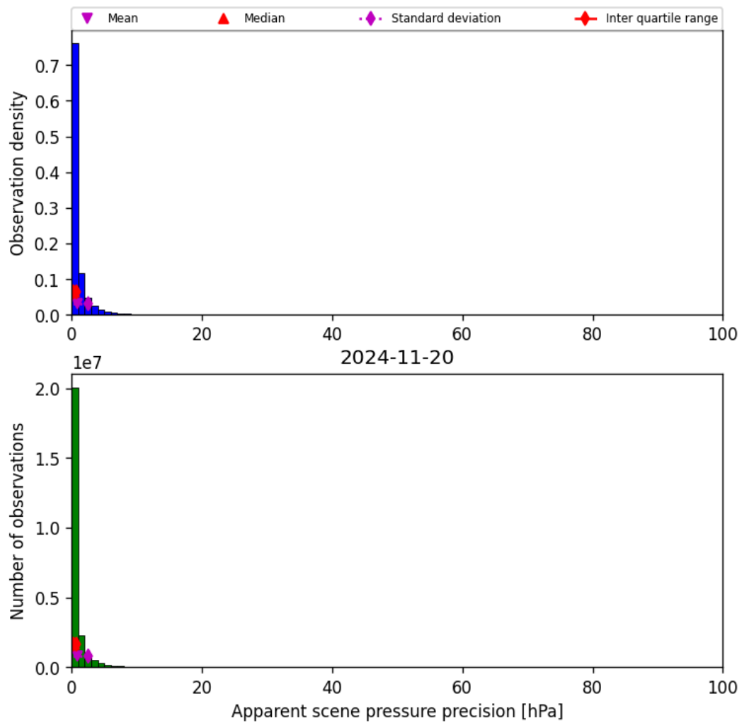
Figure 37: Histogram of “Apparent scene pressure precision” for 2024-11-20 to 2024-11-21
