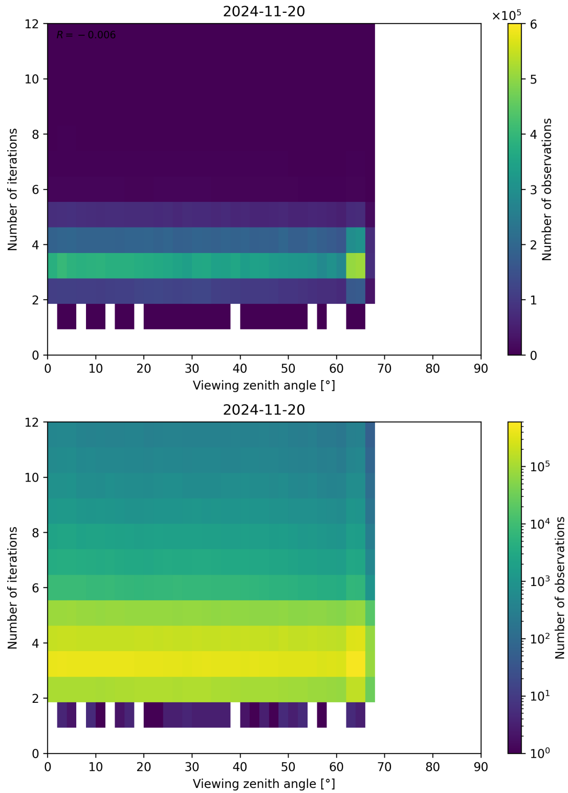
Figure 124: Scatter density plot of “Viewing zenith angle” against “Number of iterations” for 2024-11-20 to 2024-11-21.
