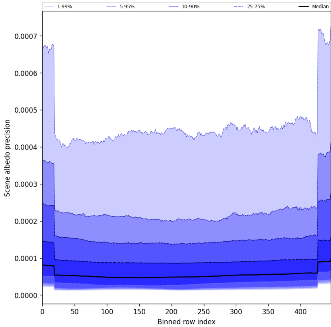
Figure 52: Along track statistics of “Scene albedo precision” for 2024-11-20 to 2024-11-21
