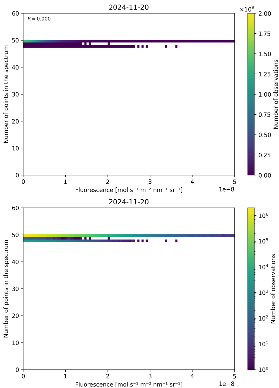
Figure 86: Scatter density plot of “Fluorescence” against “Number of points in the spectrum” for 2024-11-20 to 2024-11-21.
