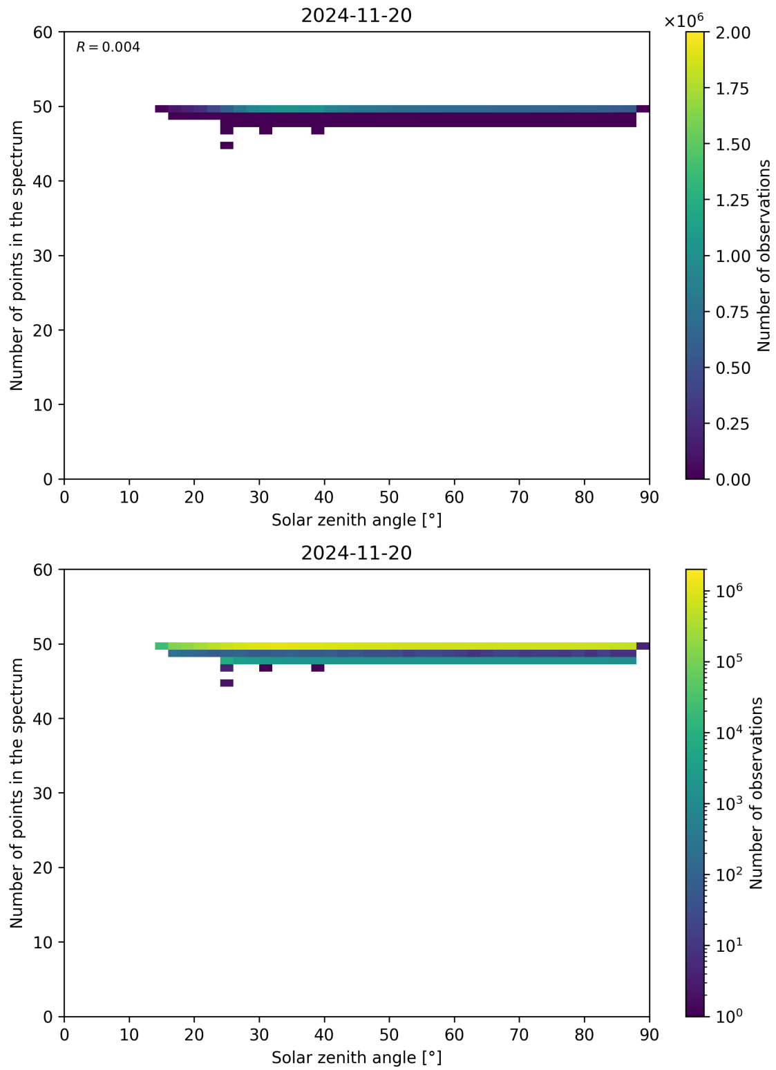
Figure 115: Scatter density plot of “Solar zenith angle” against “Number of points in the spectrum” for 2024-11-20 to 2024-11-21.
