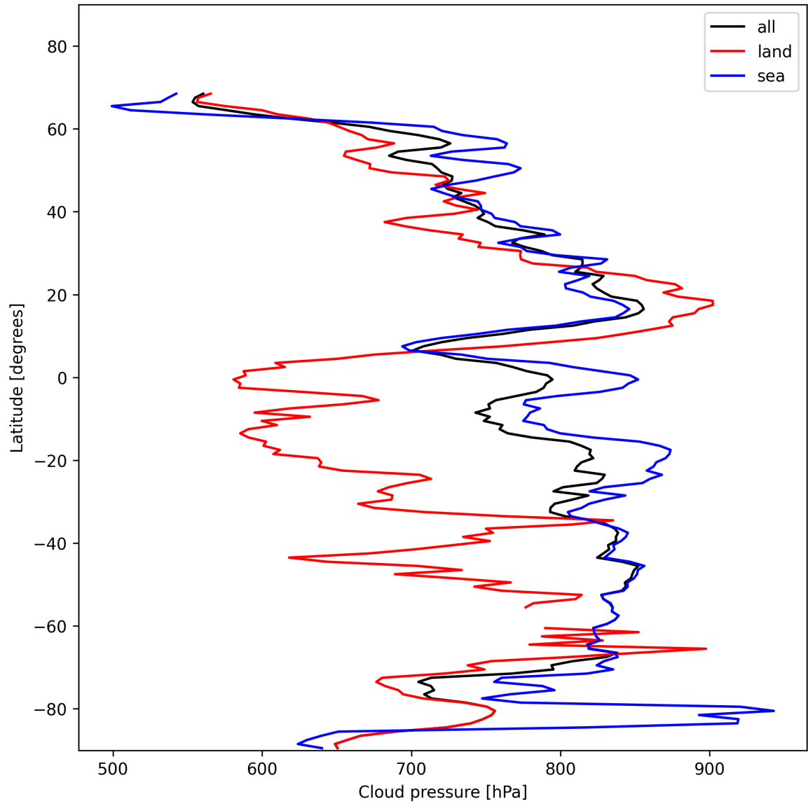
Figure 13: Zonal average of “Cloud pressure” for 2024-11-20 to 2024-11-21.
