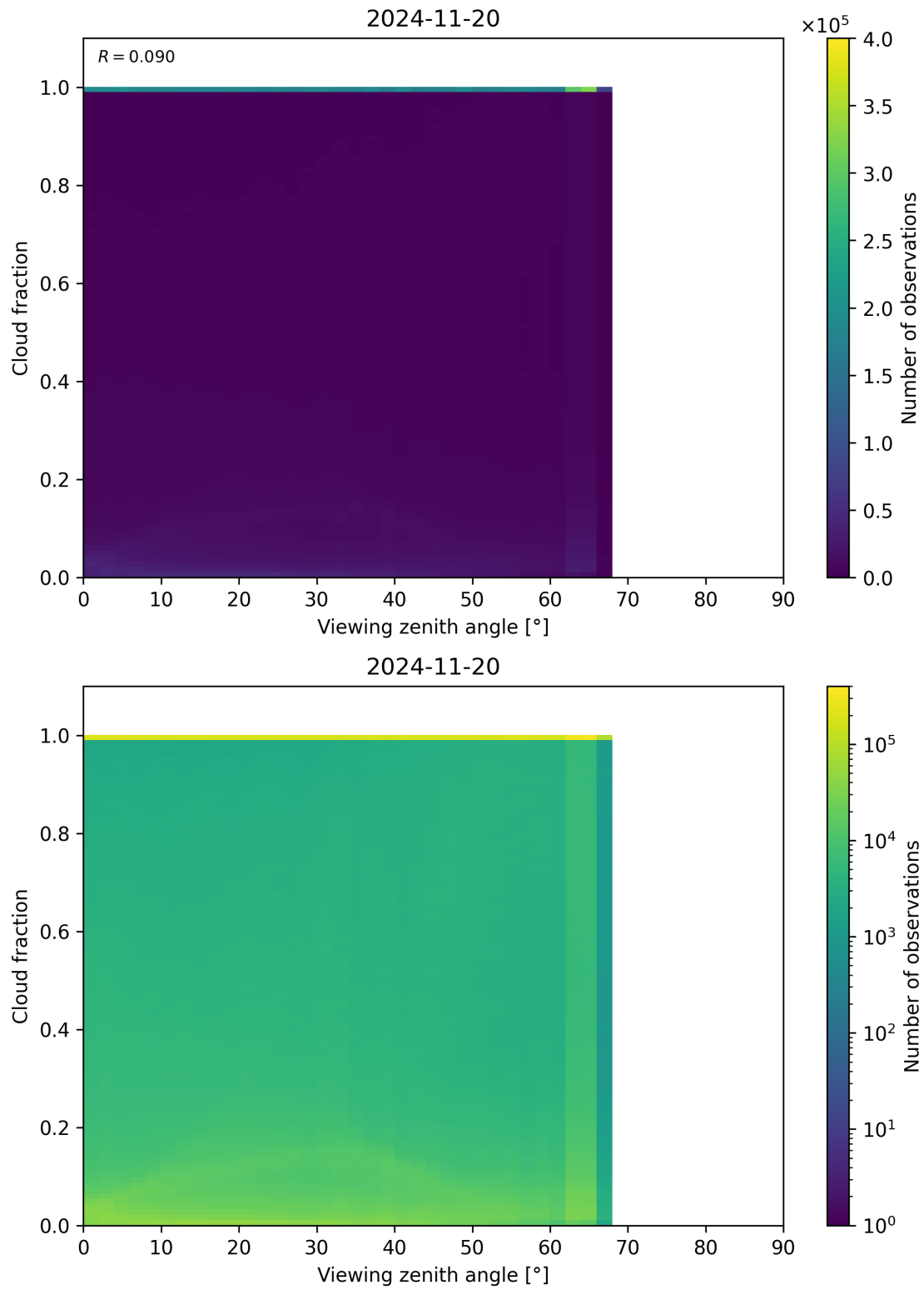
Figure 120: Scatter density plot of “Viewing zenith angle” against “Cloud fraction” for 2024-11-20 to 2024-11-21.
