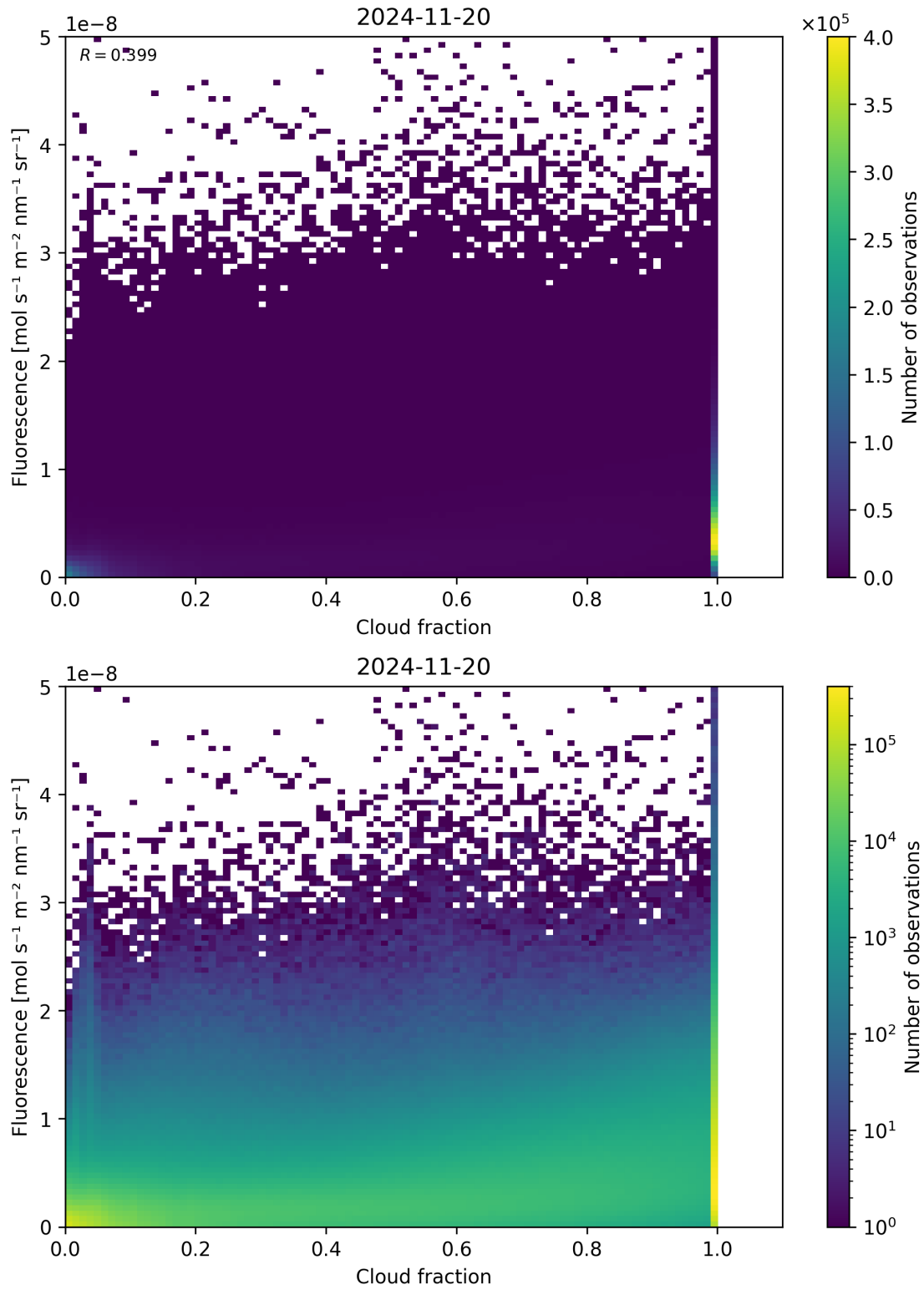
Figure 72: Scatter density plot of “Cloud fraction” against “Fluorescence” for 2024-11-20 to 2024-11-21.
