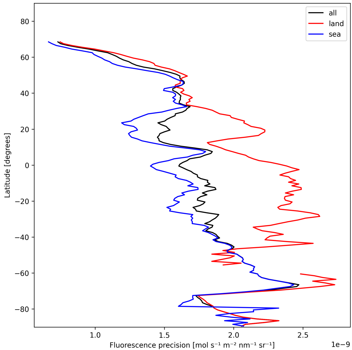
Figure 24: Zonal average of “Fluorescence precision” for 2024-11-20 to 2024-11-21.
