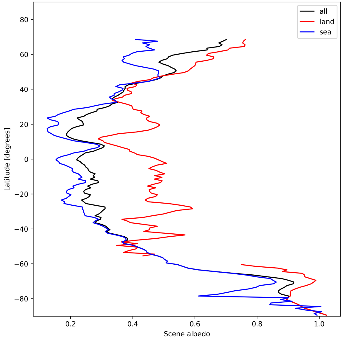
Figure 17: Zonal average of “Scene albedo” for 2024-11-20 to 2024-11-21.
