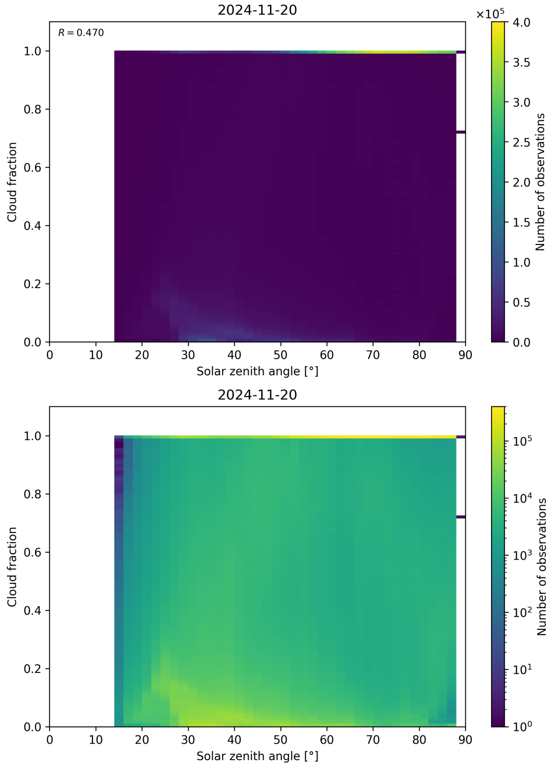
Figure 110: Scatter density plot of “Solar zenith angle” against “Cloud fraction” for 2024-11-20 to 2024-11-21.
