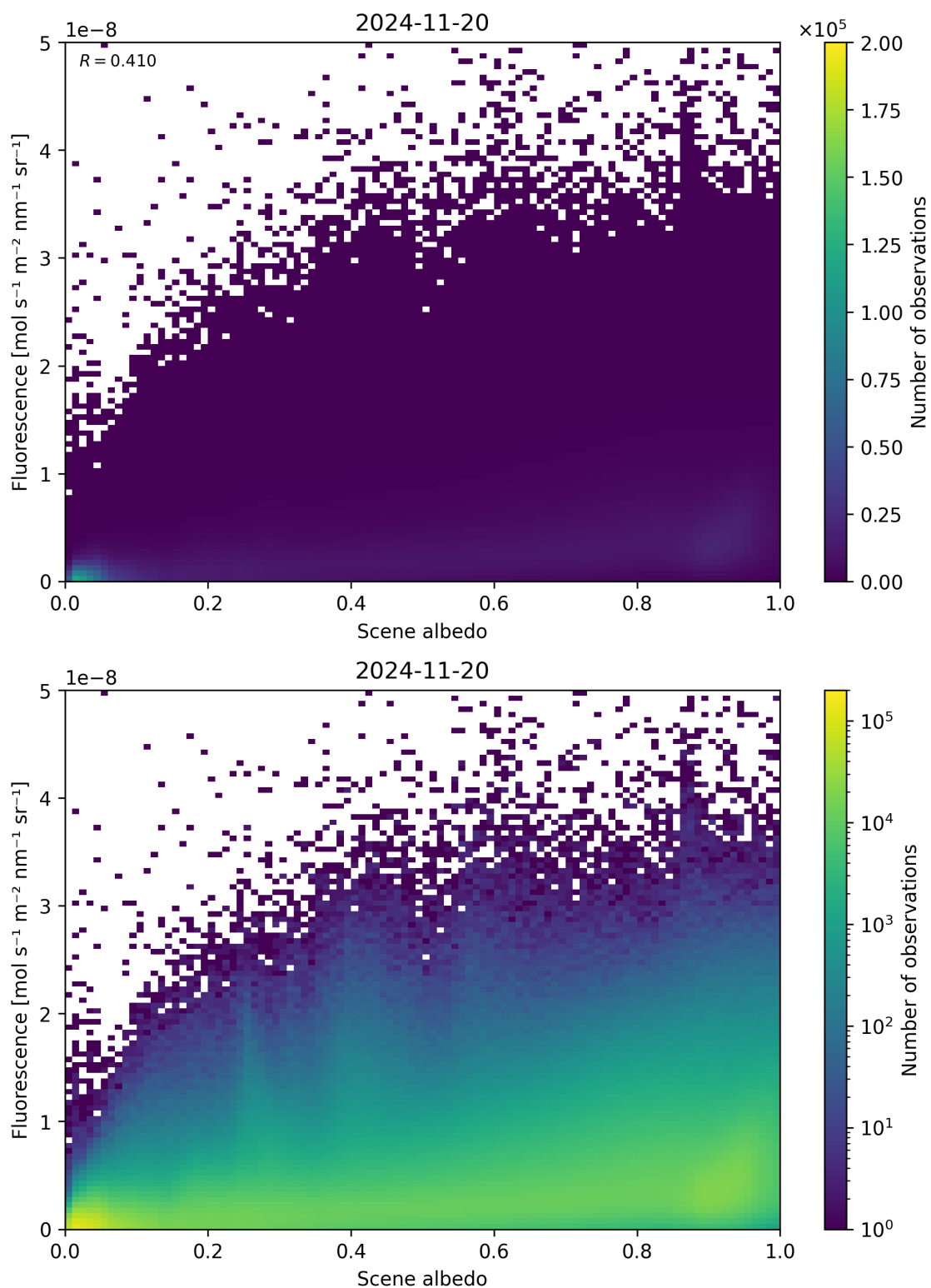
Figure 104: Scatter density plot of “Scene albedo” against “Fluorescence” for 2024-11-20 to 2024-11-21.
