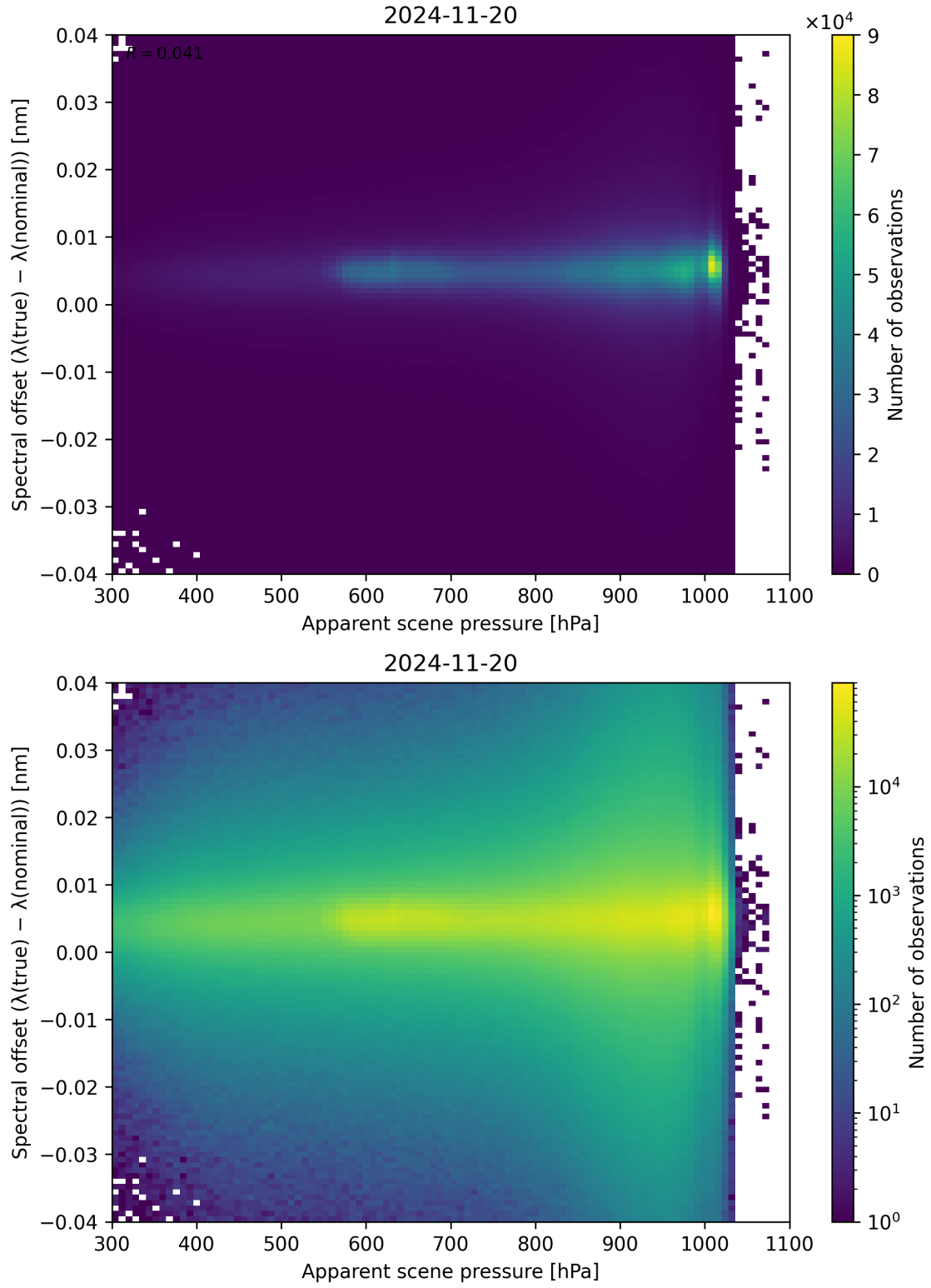
Figure 67: Scatter density plot of “Apparent scene pressure” against “Spectral offset ( \lambda_{\text{true}} - \lambda_{\text{nominal}} )” for 2024-11-20 to 2024-11-21.
