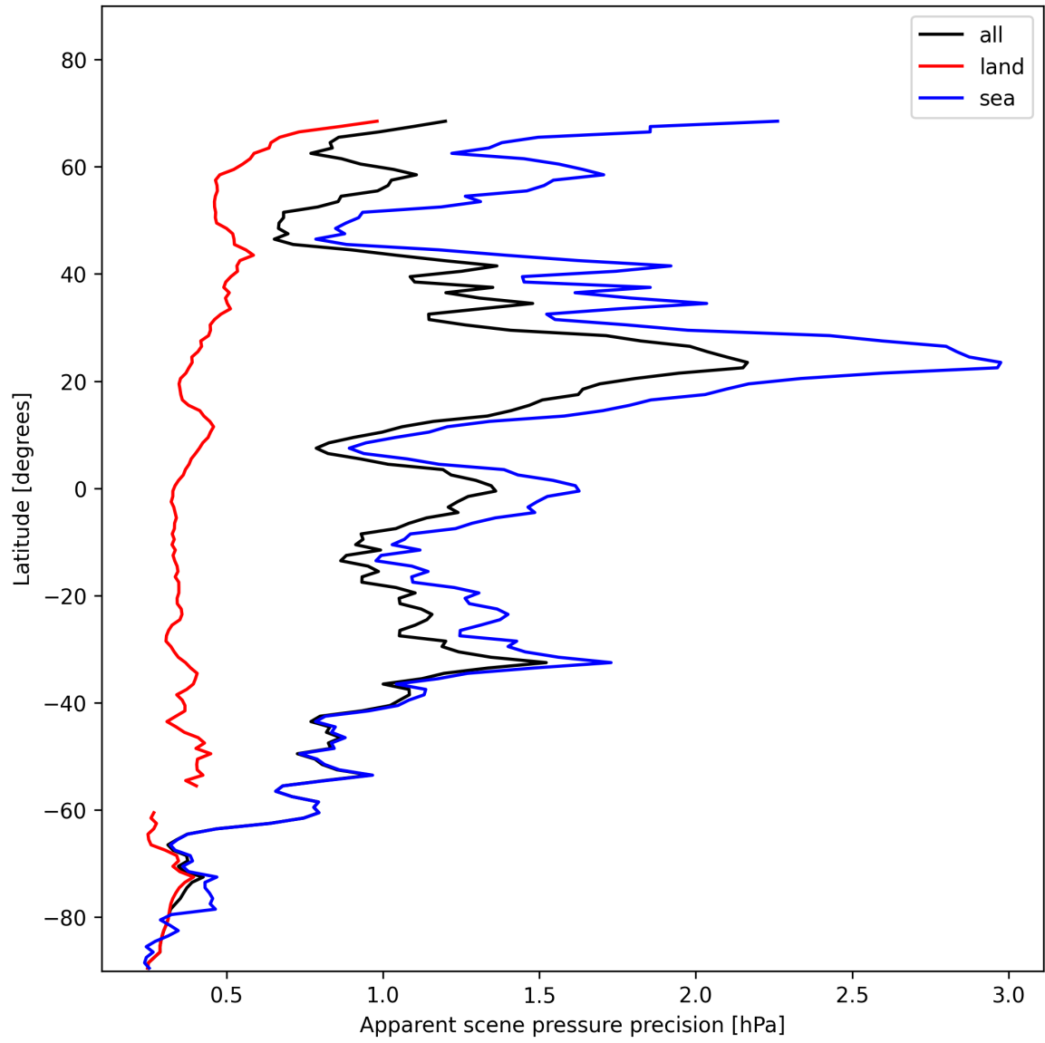
Figure 20: Zonal average of “Apparent scene pressure precision” for 2024-11-20 to 2024-11-21.
