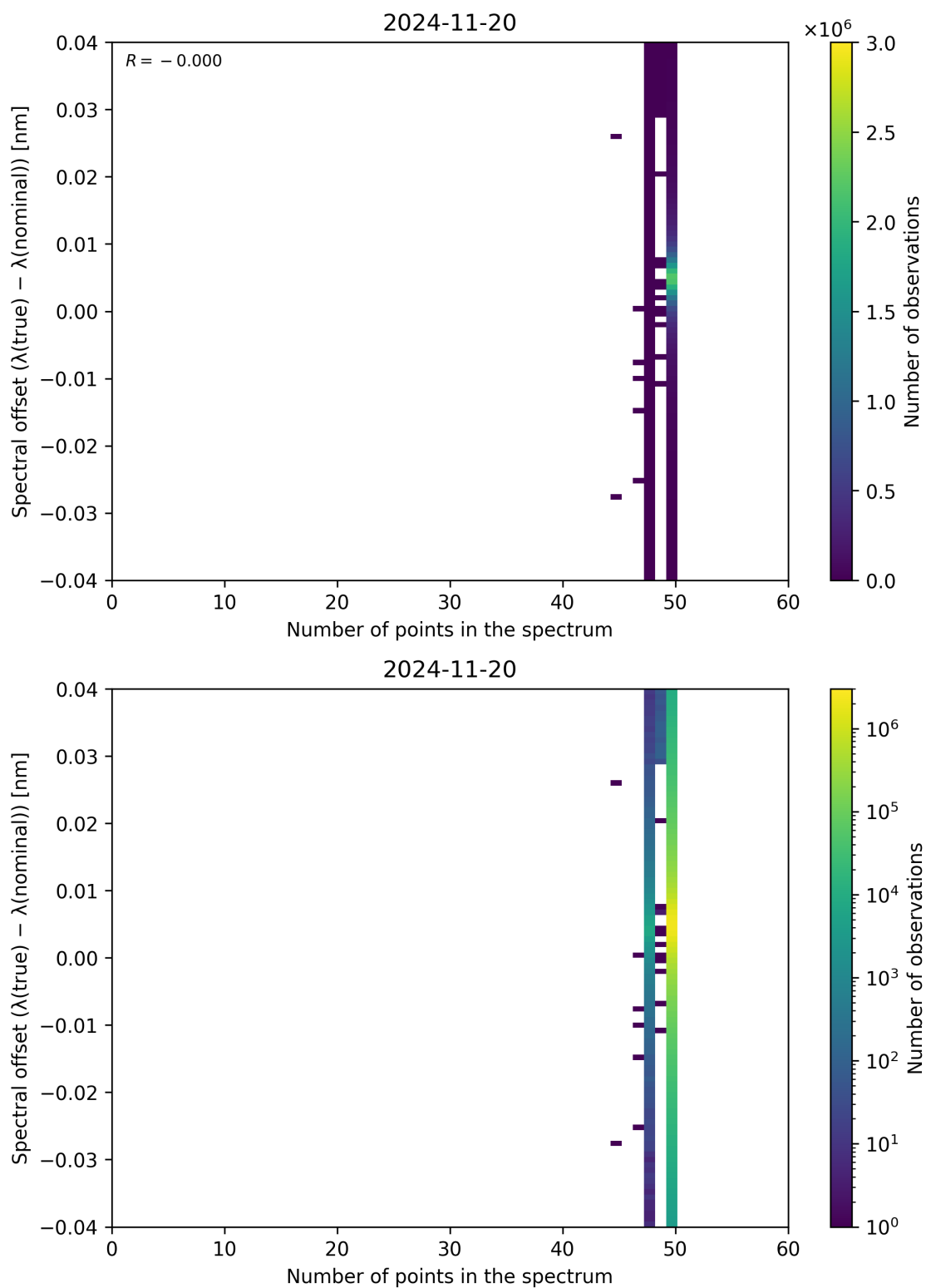
Figure 101: Scatter density plot of “Number of points in the spectrum” against “Spectral offset ( \lambda_{\text{true}} - \lambda_{\text{nominal}} )” for 2024-11-20 to 2024-11-21.
