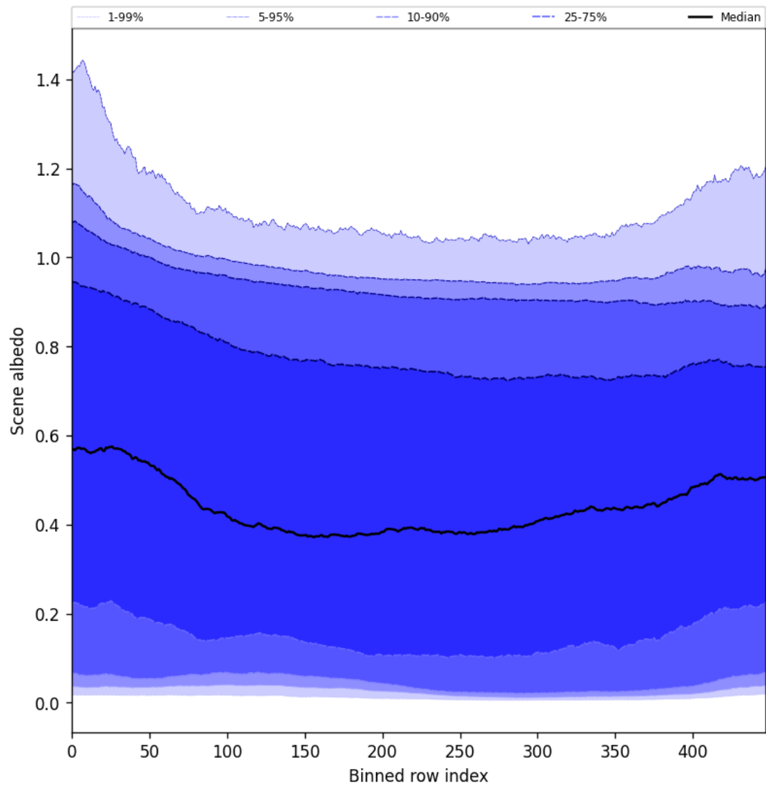
Figure 51: Along track statistics of “Scene albedo” for 2024-11-20 to 2024-11-21
