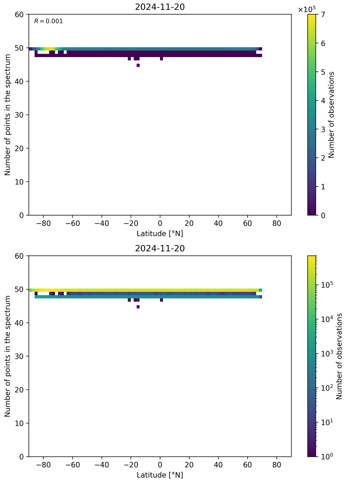
Figure 94: Scatter density plot of “Latitude” against “Number of points in the spectrum” for 2024-11-20 to 2024-11-21.
