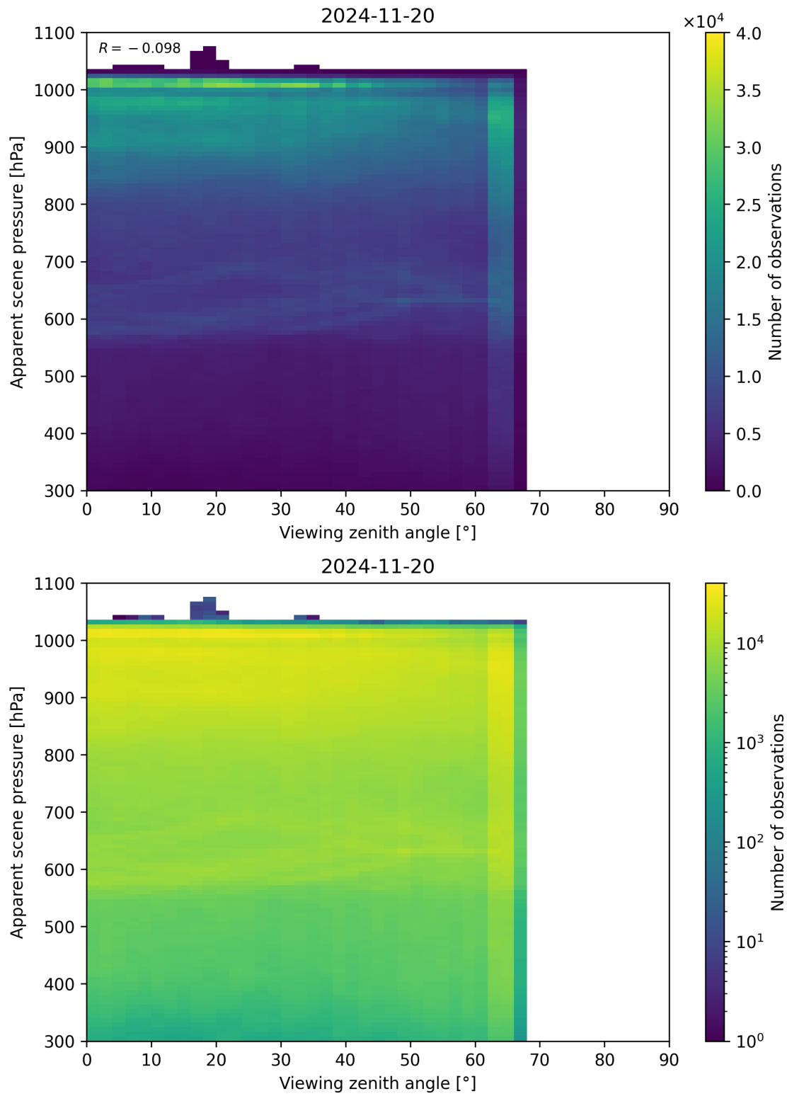
Figure 118: Scatter density plot of “Viewing zenith angle” against “Apparent scene pressure” for 2024-11-20 to 2024-11-21.
