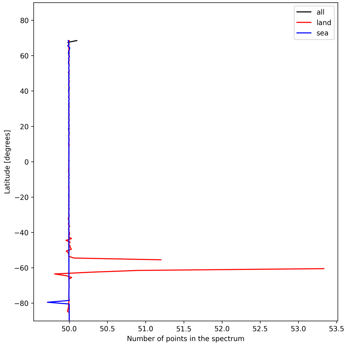
Figure 27: Zonal average of “Number of points in the spectrum” for 2024-11-20 to 2024-11-21.
