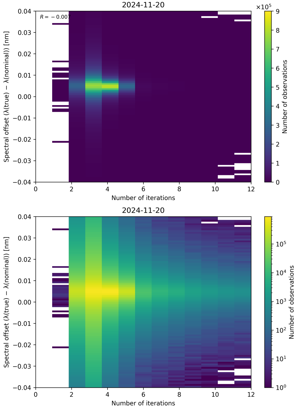
Figure 100: Scatter density plot of “Number of iterations” against “Spectral offset ( \lambda_{\text{true}} - \lambda_{\text{nominal}} )” for 2024-11-20 to 2024-11-21.
