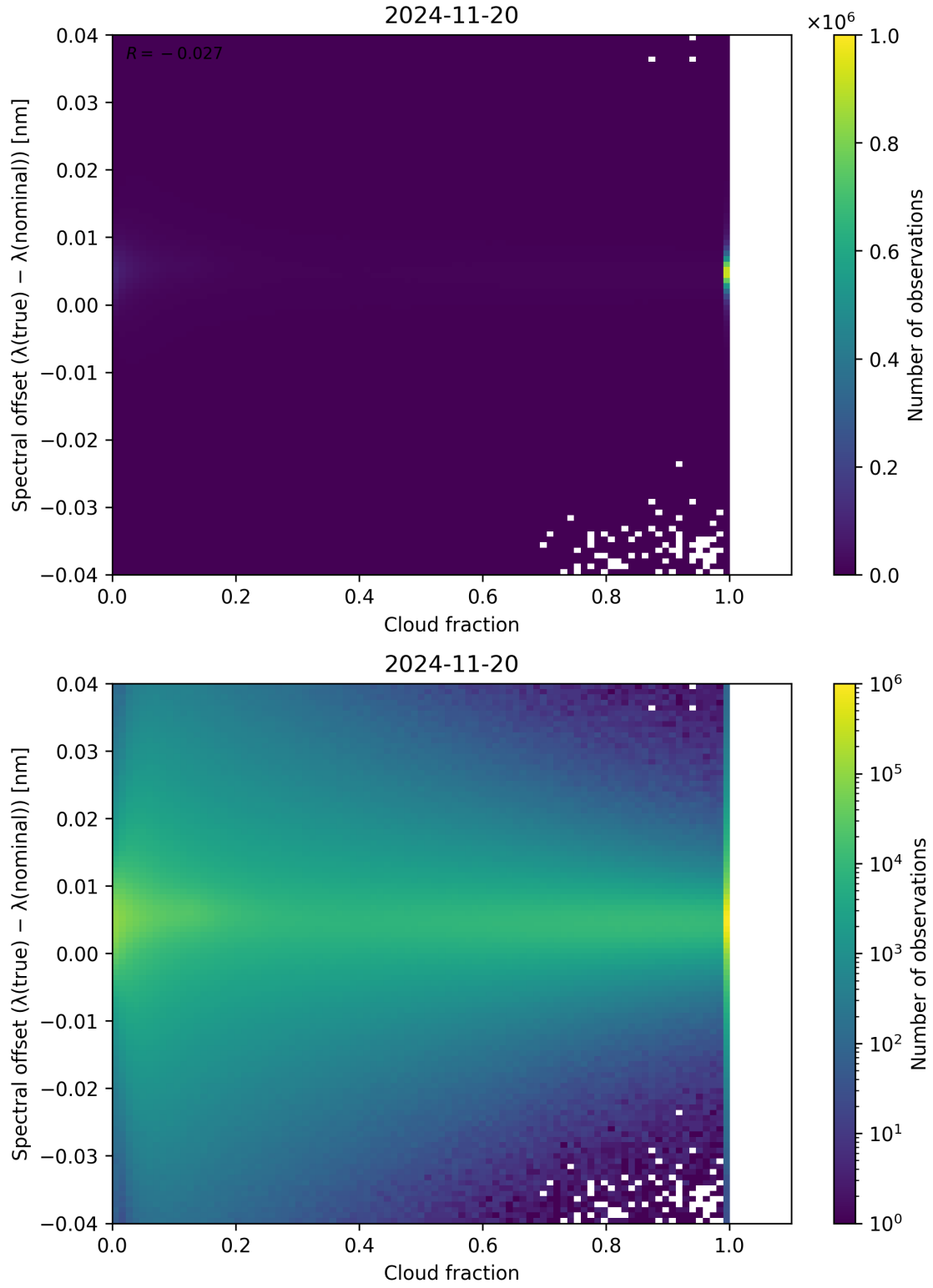
Figure 76: Scatter density plot of “Cloud fraction” against “Spectral offset ( \lambda_{\text{true}} - \lambda_{\text{nominal}} )” for 2024-11-20 to 2024-11-21.
