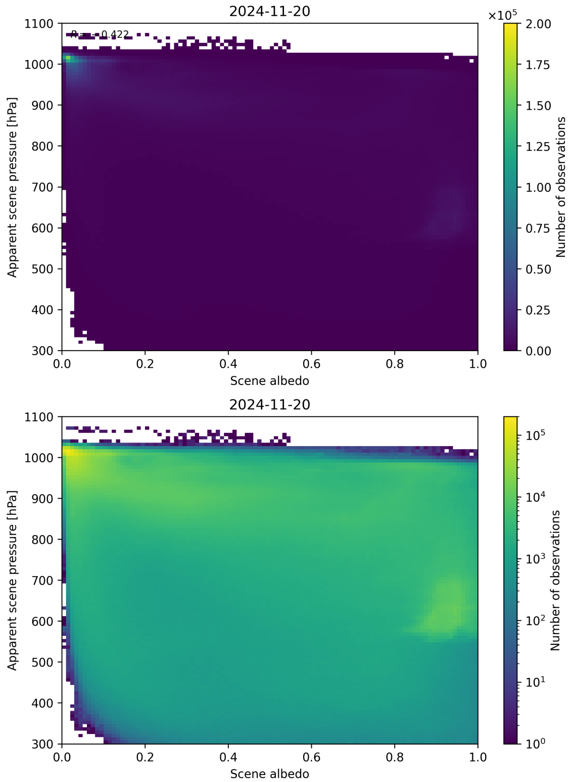
Figure 102: Scatter density plot of “Scene albedo” against “Apparent scene pressure” for 2024-11-20 to 2024-11-21.
