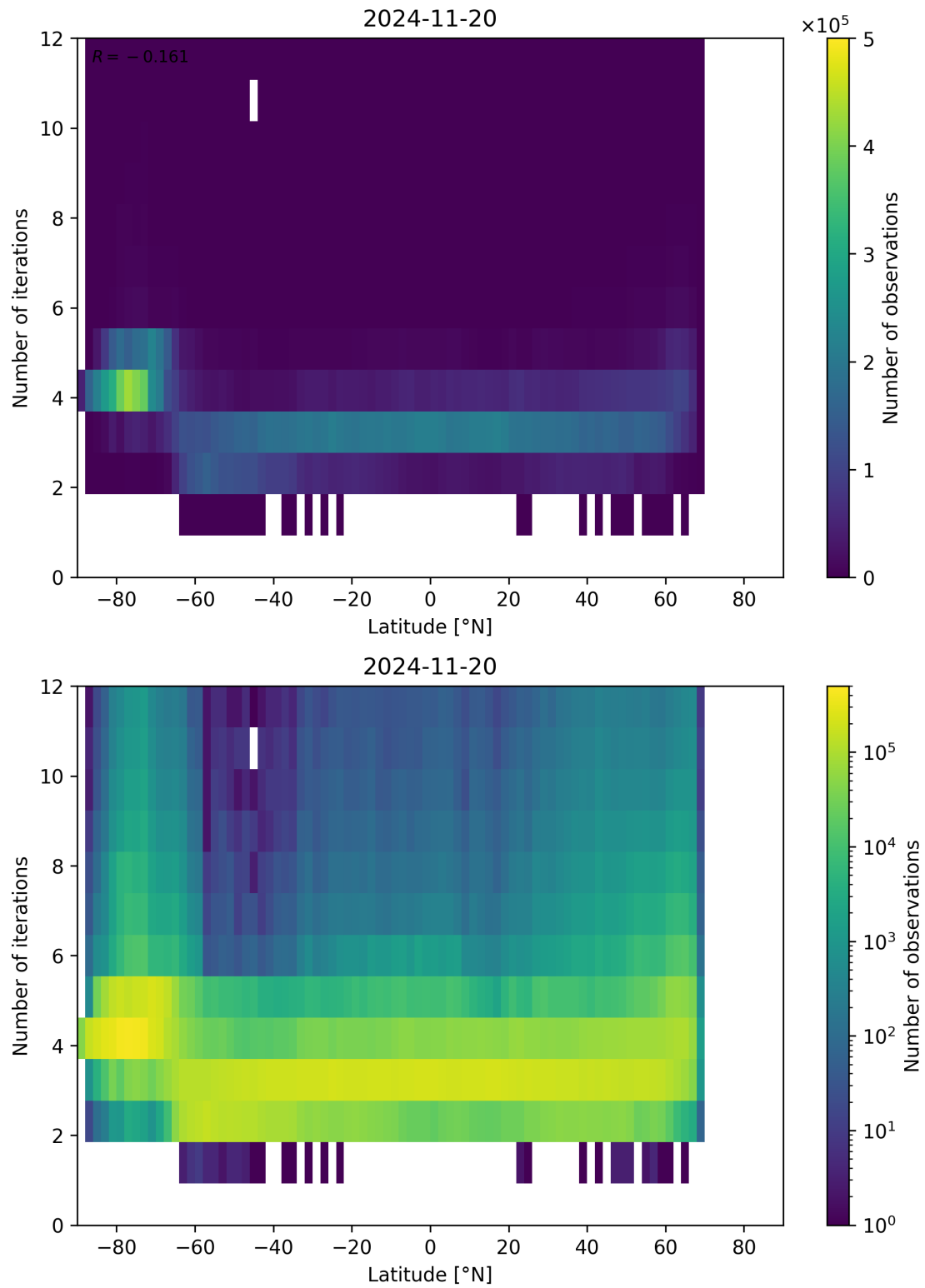
Figure 93: Scatter density plot of “Latitude” against “Number of iterations” for 2024-11-20 to 2024-11-21.
