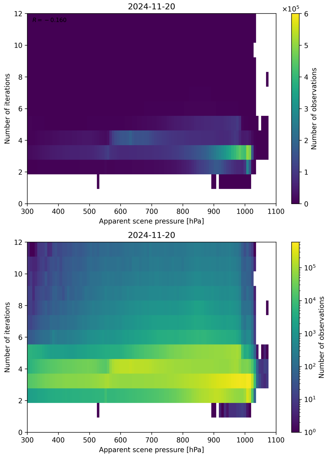
Figure 65: Scatter density plot of “Apparent scene pressure” against “Number of iterations” for 2024-11-20 to 2024-11-21.
