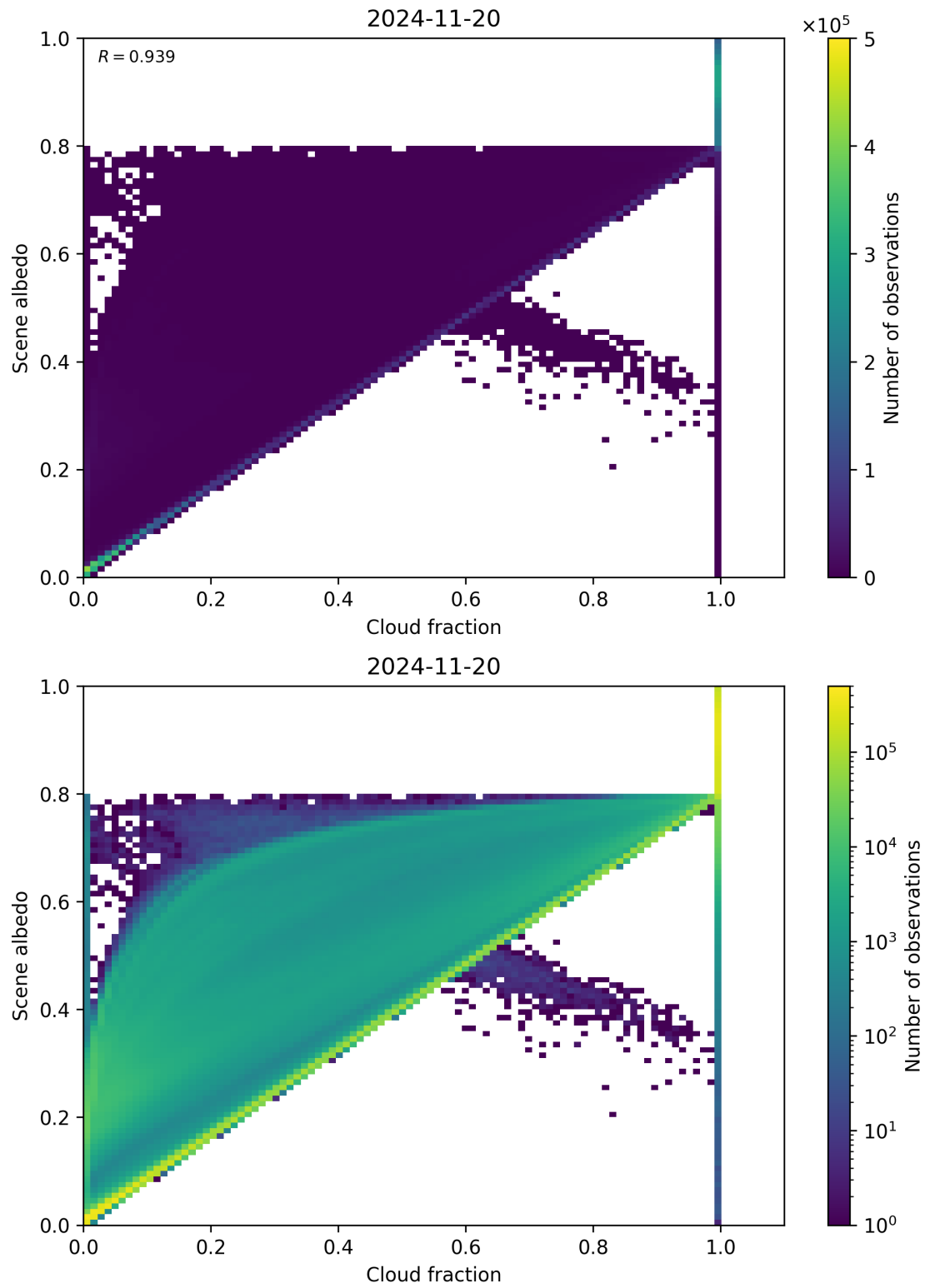
Figure 75: Scatter density plot of “Cloud fraction” against “Scene albedo” for 2024-11-20 to 2024-11-21.
