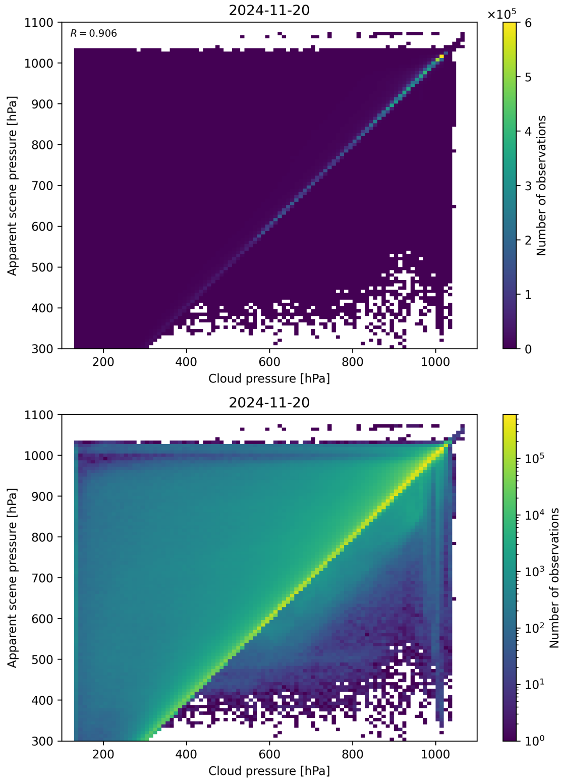
Figure 77: Scatter density plot of “Cloud pressure” against “Apparent scene pressure” for 2024-11-20 to 2024-11-21.
