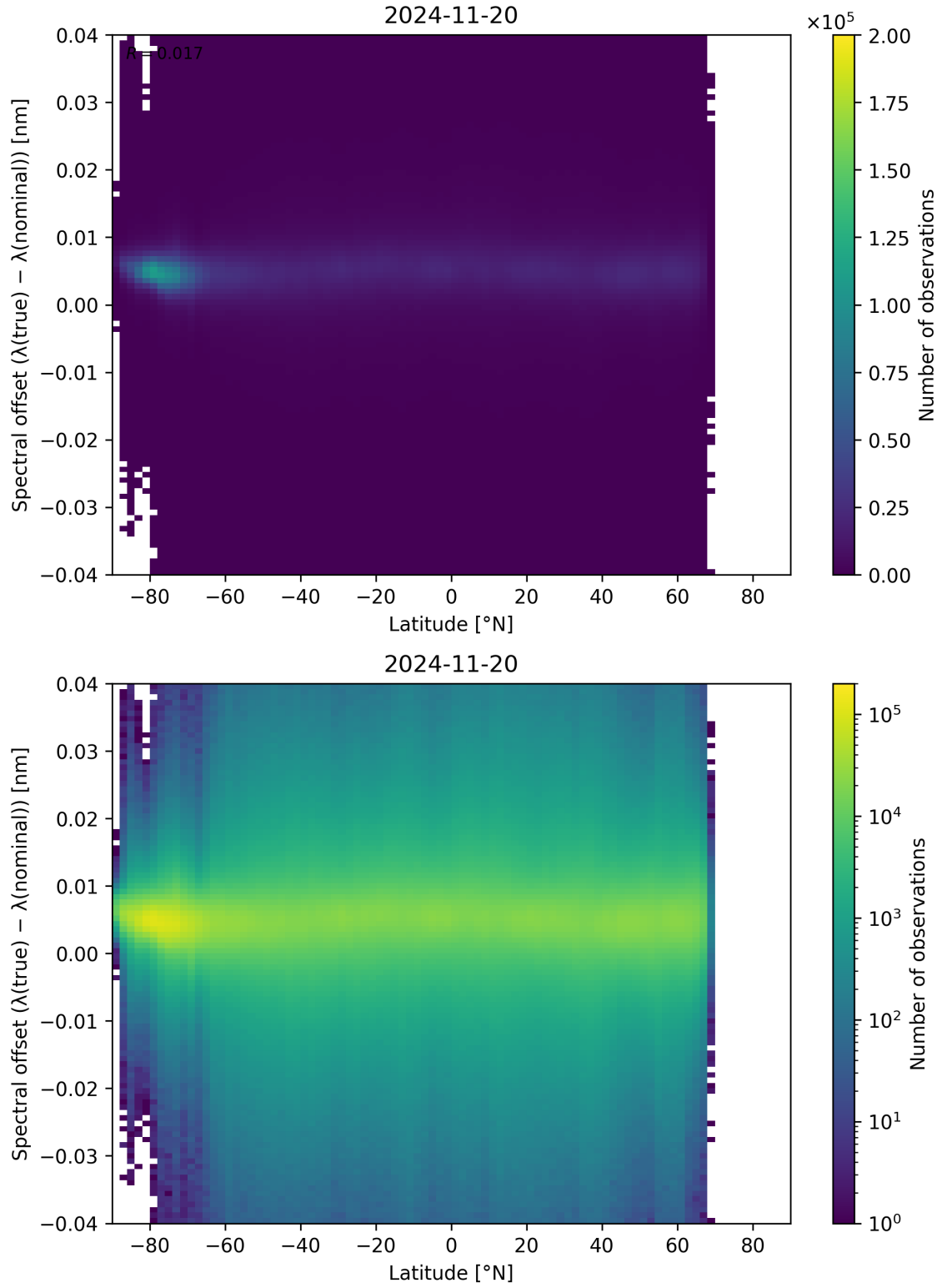
Figure 96: Scatter density plot of “Latitude” against “Spectral offset ( \lambda_{\text{true}} - \lambda_{\text{nominal}} )” for 2024-11-20 to 2024-11-21.
