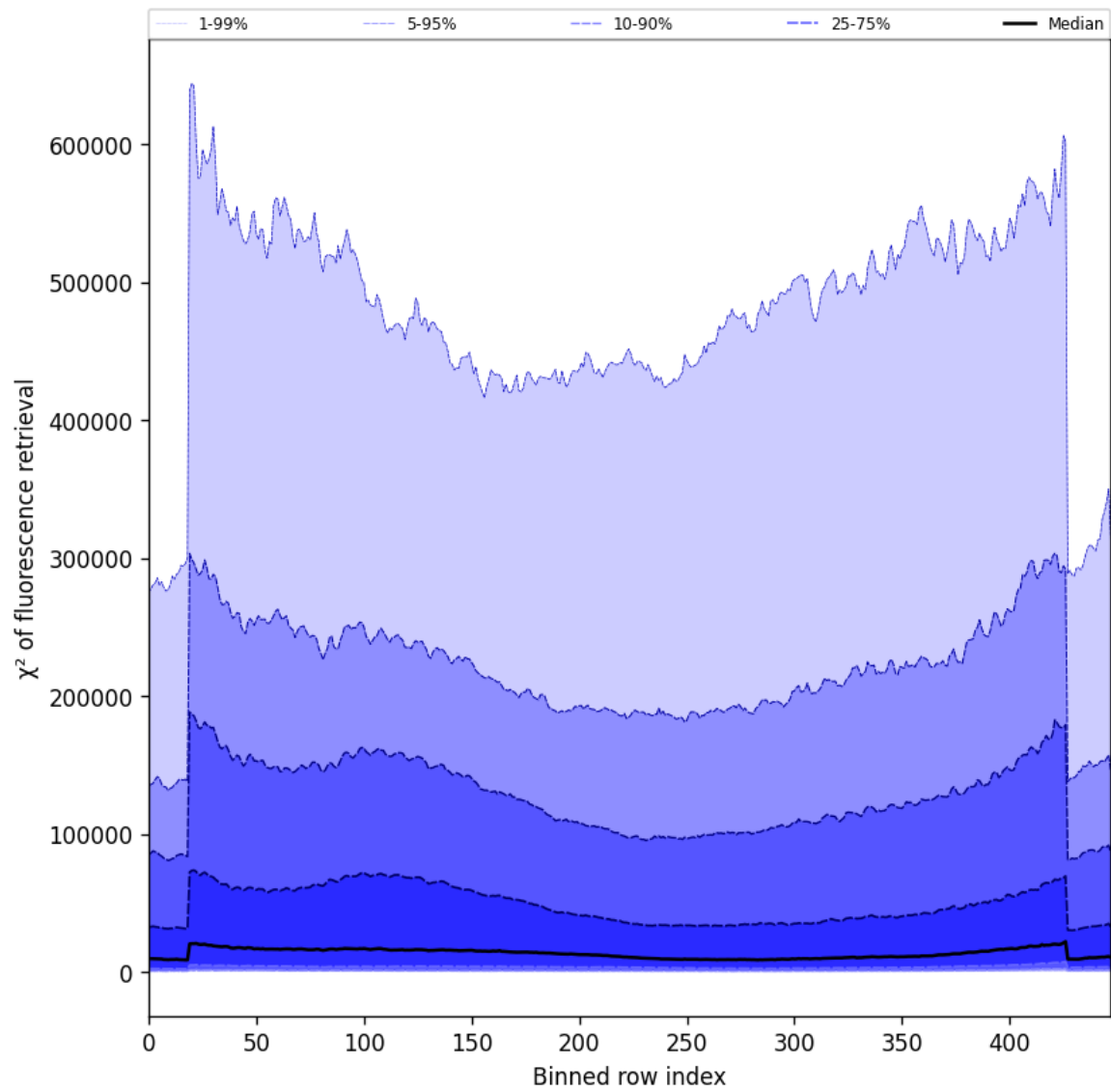
Figure 59: Along track statistics of “ \chi^2 of fluorescence retrieval” for 2024-11-20 to 2024-11-21
