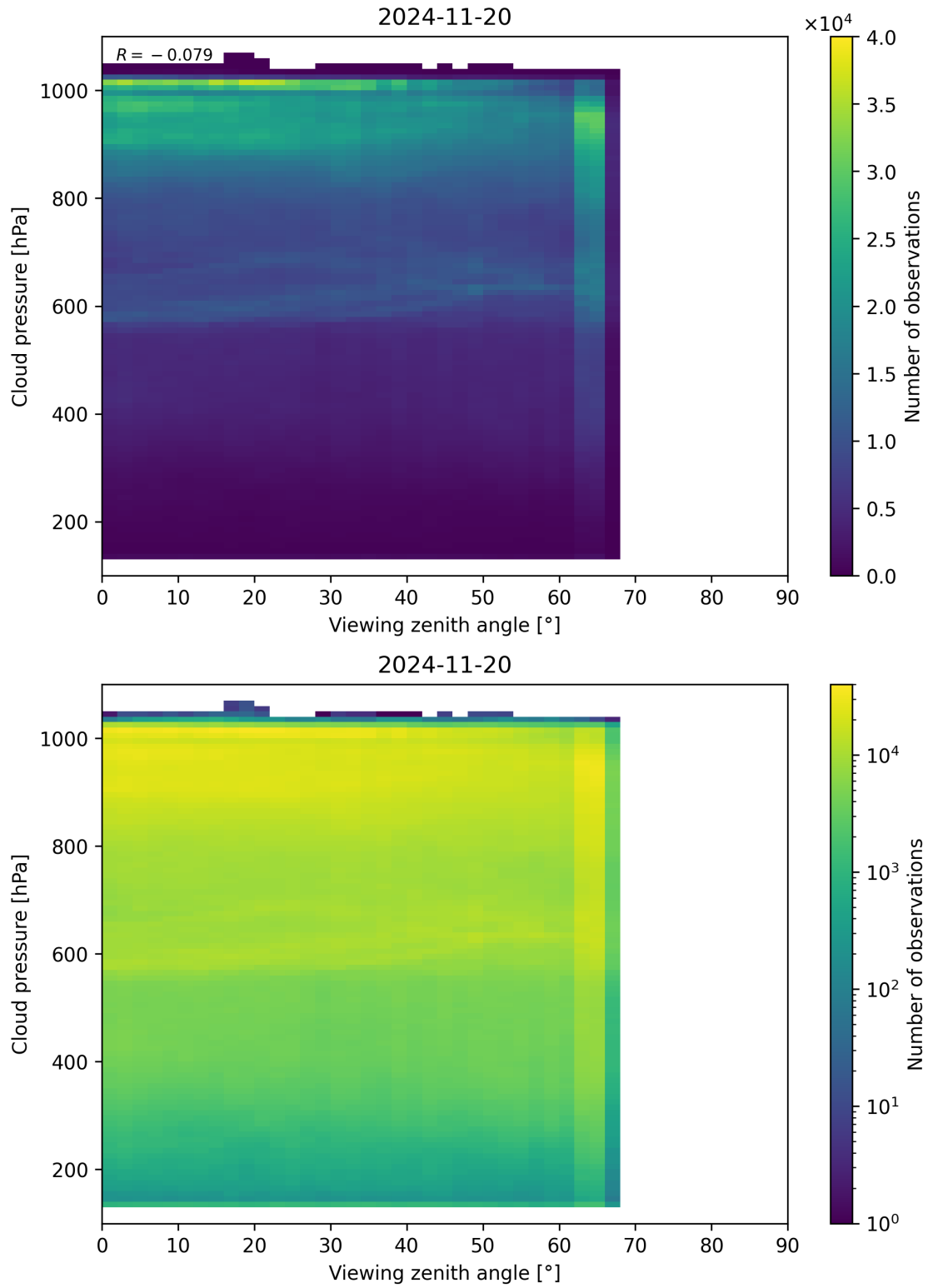
Figure 121: Scatter density plot of “Viewing zenith angle” against “Cloud pressure” for 2024-11-20 to 2024-11-21.
