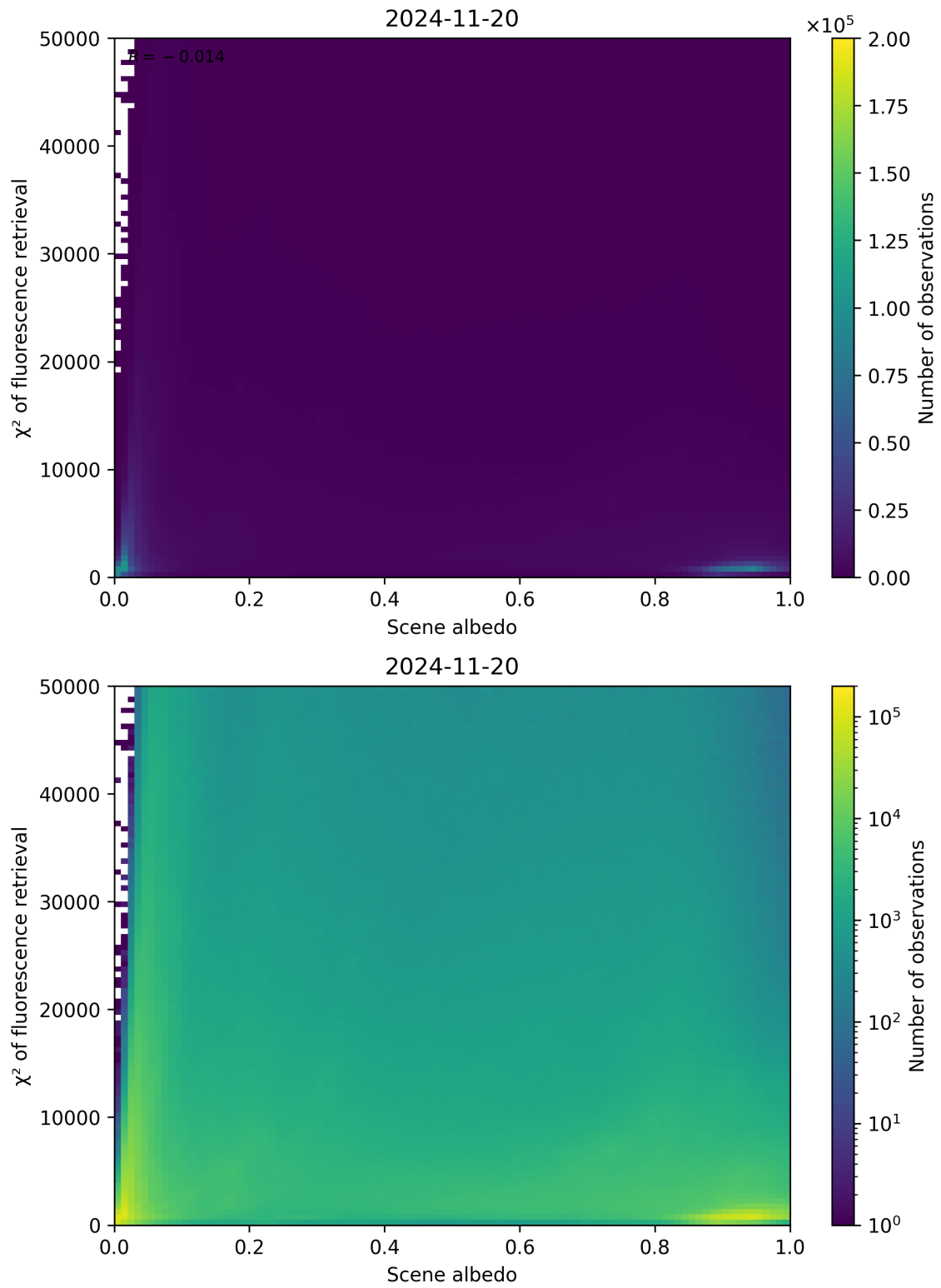
Figure 103: Scatter density plot of “Scene albedo” against “ \chi^2 of fluorescence retrieval” for 2024-11-20 to 2024-11-21.
