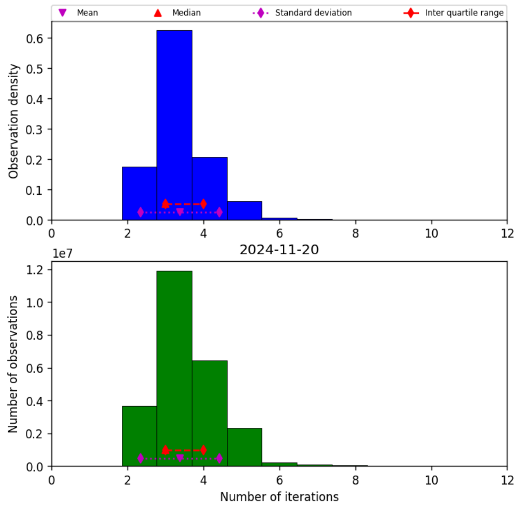
Figure 39: Histogram of “Number of iterations” for 2024-11-20 to 2024-11-21
