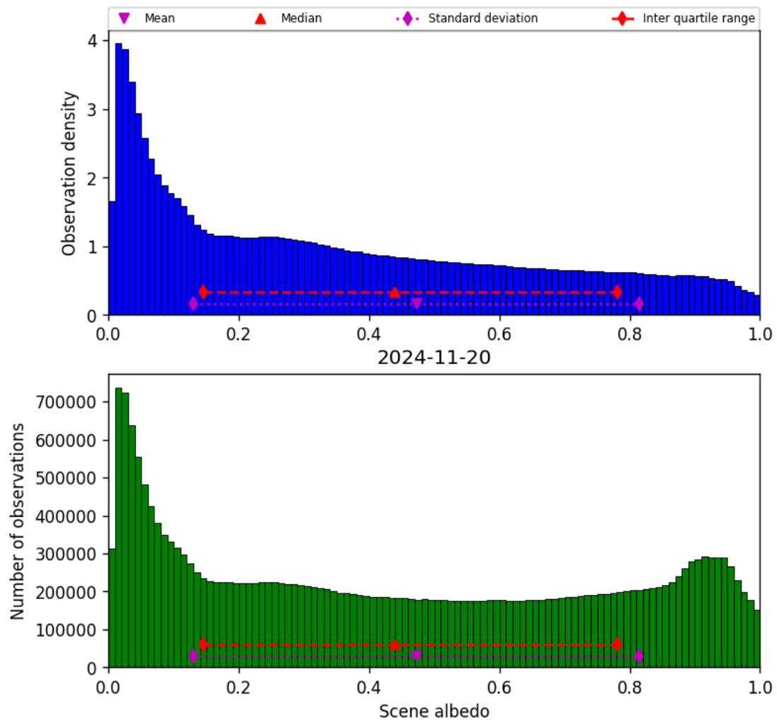
Figure 34: Histogram of “Scene albedo” for 2024-11-20 to 2024-11-21
