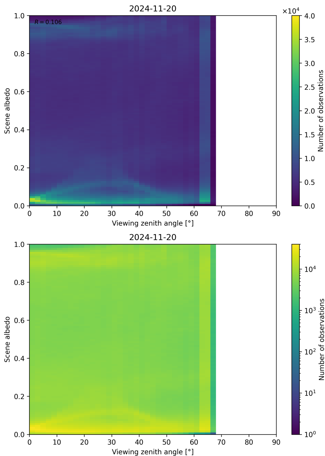
Figure 126: Scatter density plot of “Viewing zenith angle” against “Scene albedo” for 2024-11-20 to 2024-11-21.
