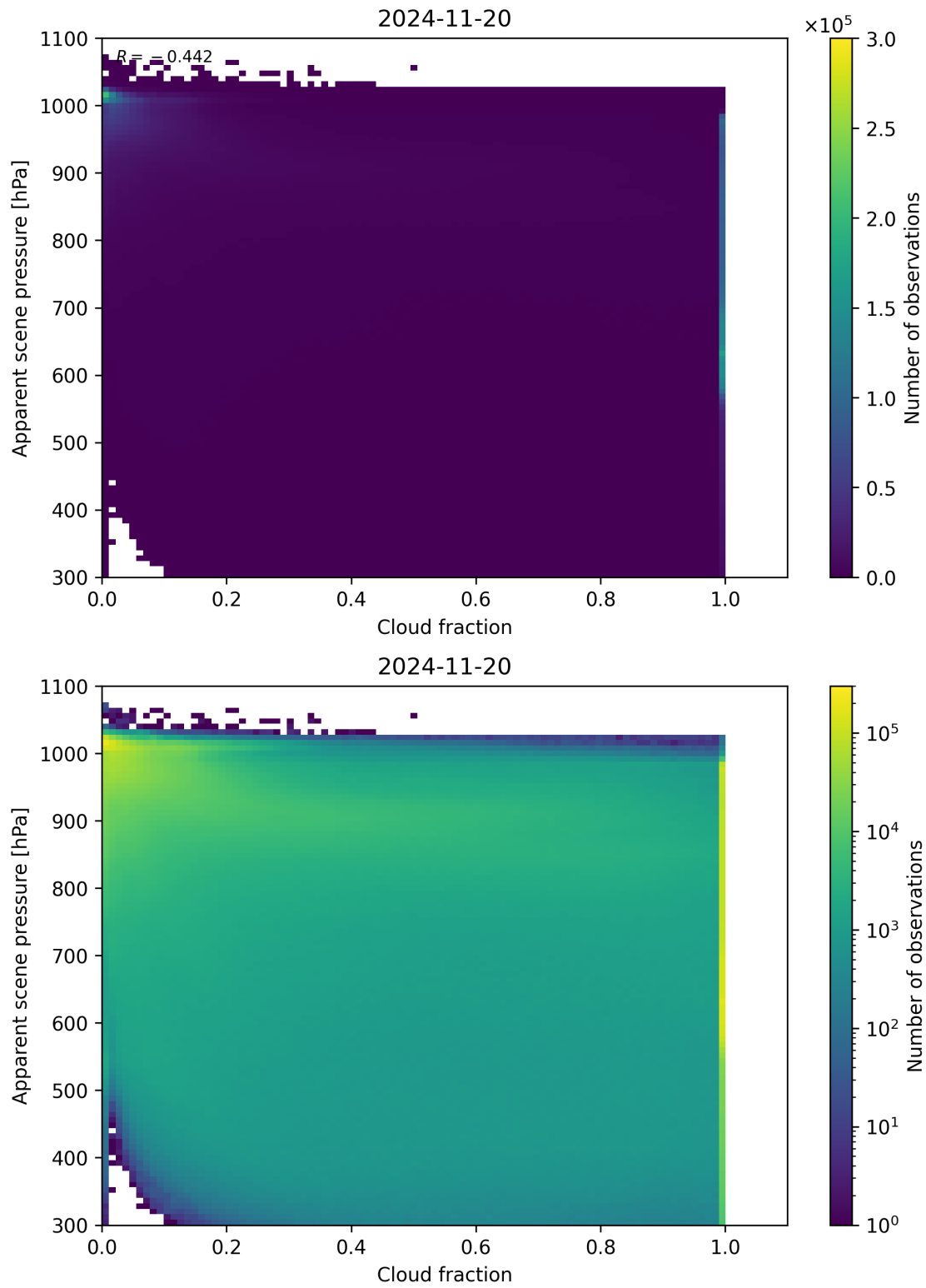
Figure 70: Scatter density plot of “Cloud fraction” against “Apparent scene pressure” for 2024-11-20 to 2024-11-21.
