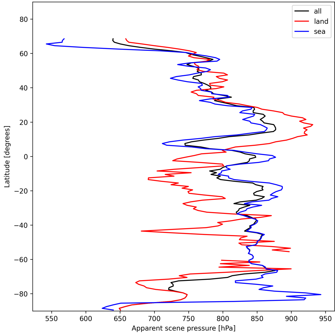
Figure 19: Zonal average of “Apparent scene pressure” for 2024-11-20 to 2024-11-21.
