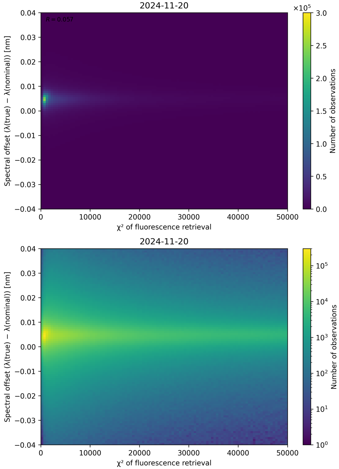
Figure 69: Scatter density plot of “ \chi^2 of fluorescence retrieval” against “Spectral offset ( \lambda_{\text{true}} - \lambda_{\text{nominal}} )” for 2024-11-20 to 2024-11-21.
