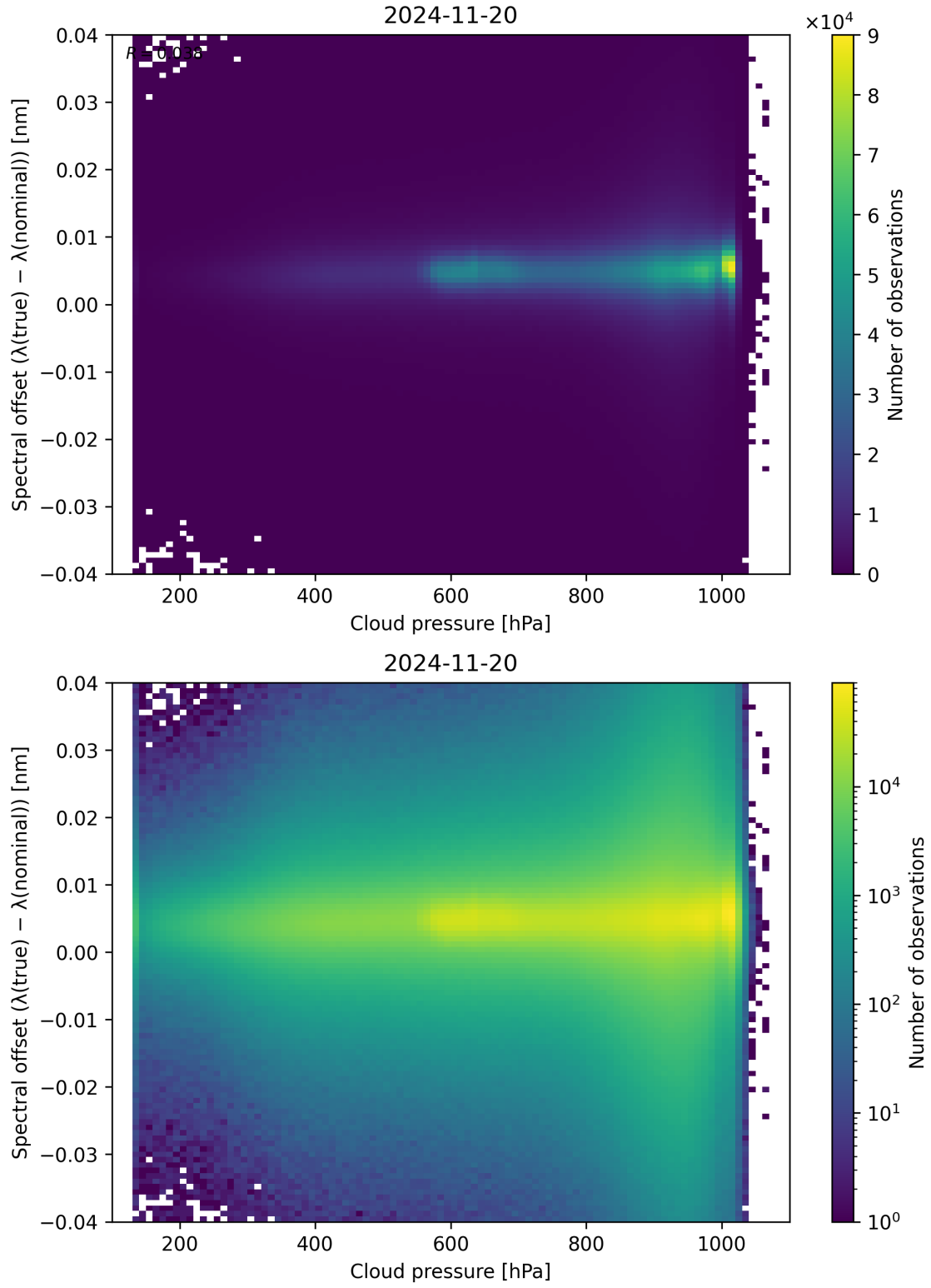
Figure 84: Scatter density plot of “Cloud pressure” against “Spectral offset ( \lambda_{\text{true}} - \lambda_{\text{nominal}} )” for 2024-11-20 to 2024-11-21.
