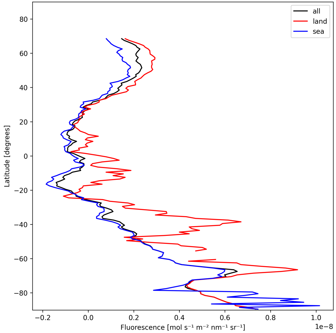
Figure 23: Zonal average of “Fluorescence” for 2024-11-20 to 2024-11-21.
