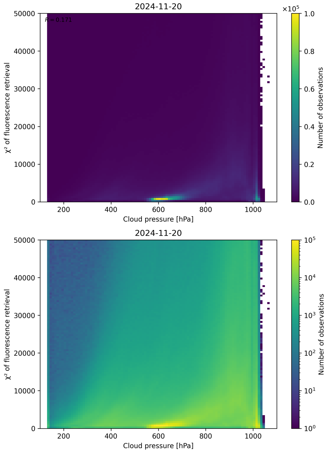
Figure 78: Scatter density plot of “Cloud pressure” against “ \chi^2 of fluorescence retrieval” for 2024-11-20 to 2024-11-21.
