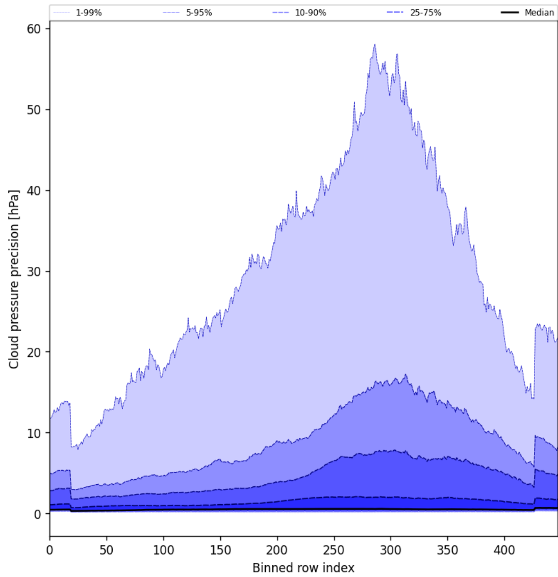
Figure 48: Along track statistics of “Cloud pressure precision” for 2024-11-20 to 2024-11-21
