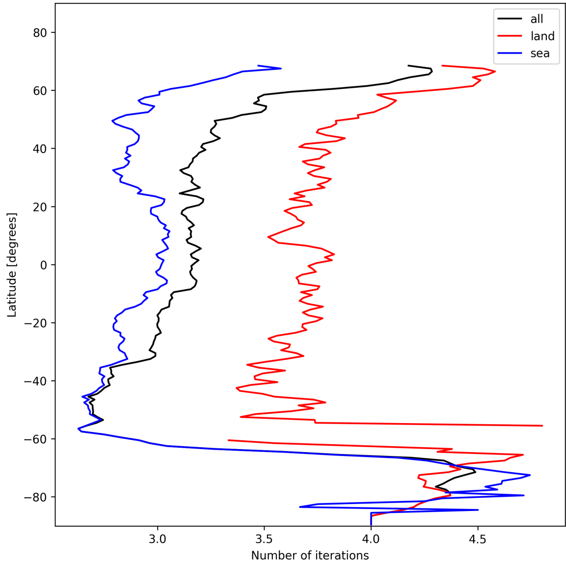
Figure 22: Zonal average of “Number of iterations” for 2024-11-20 to 2024-11-21.
