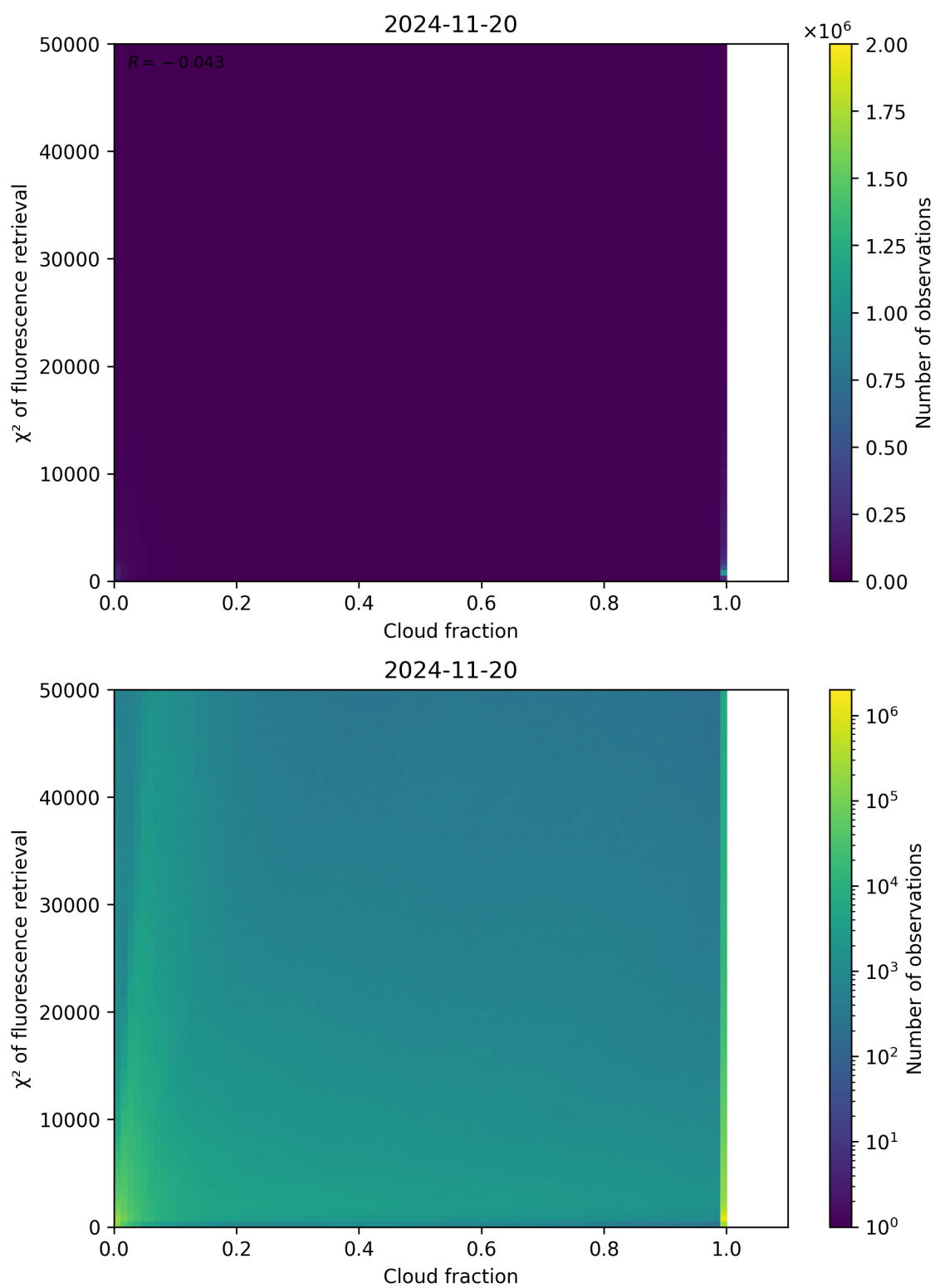
Figure 71: Scatter density plot of “Cloud fraction” against “ \chi^2 of fluorescence retrieval” for 2024-11-20 to 2024-11-21.
