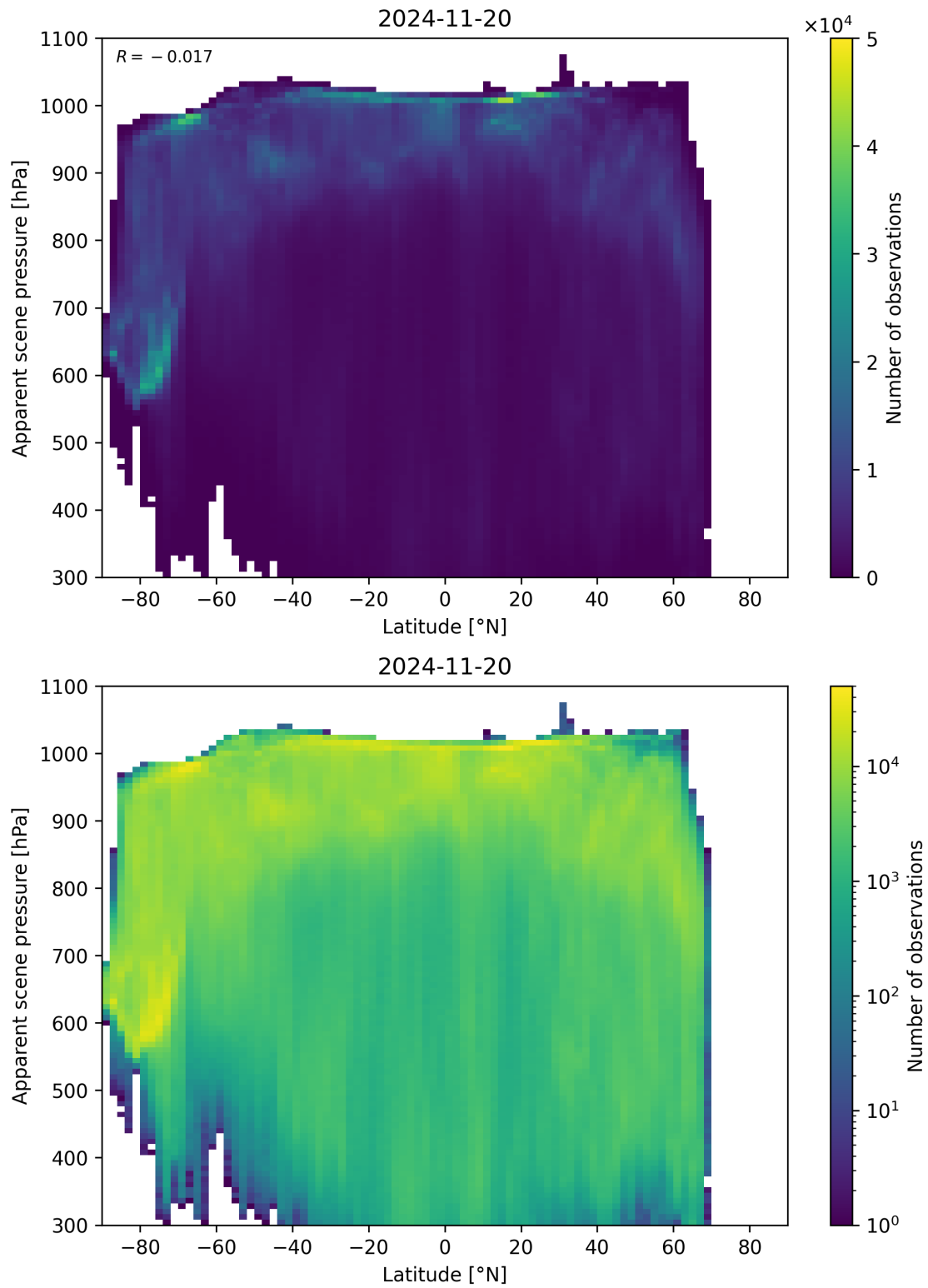
Figure 88: Scatter density plot of “Latitude” against “Apparent scene pressure” for 2024-11-20 to 2024-11-21.
