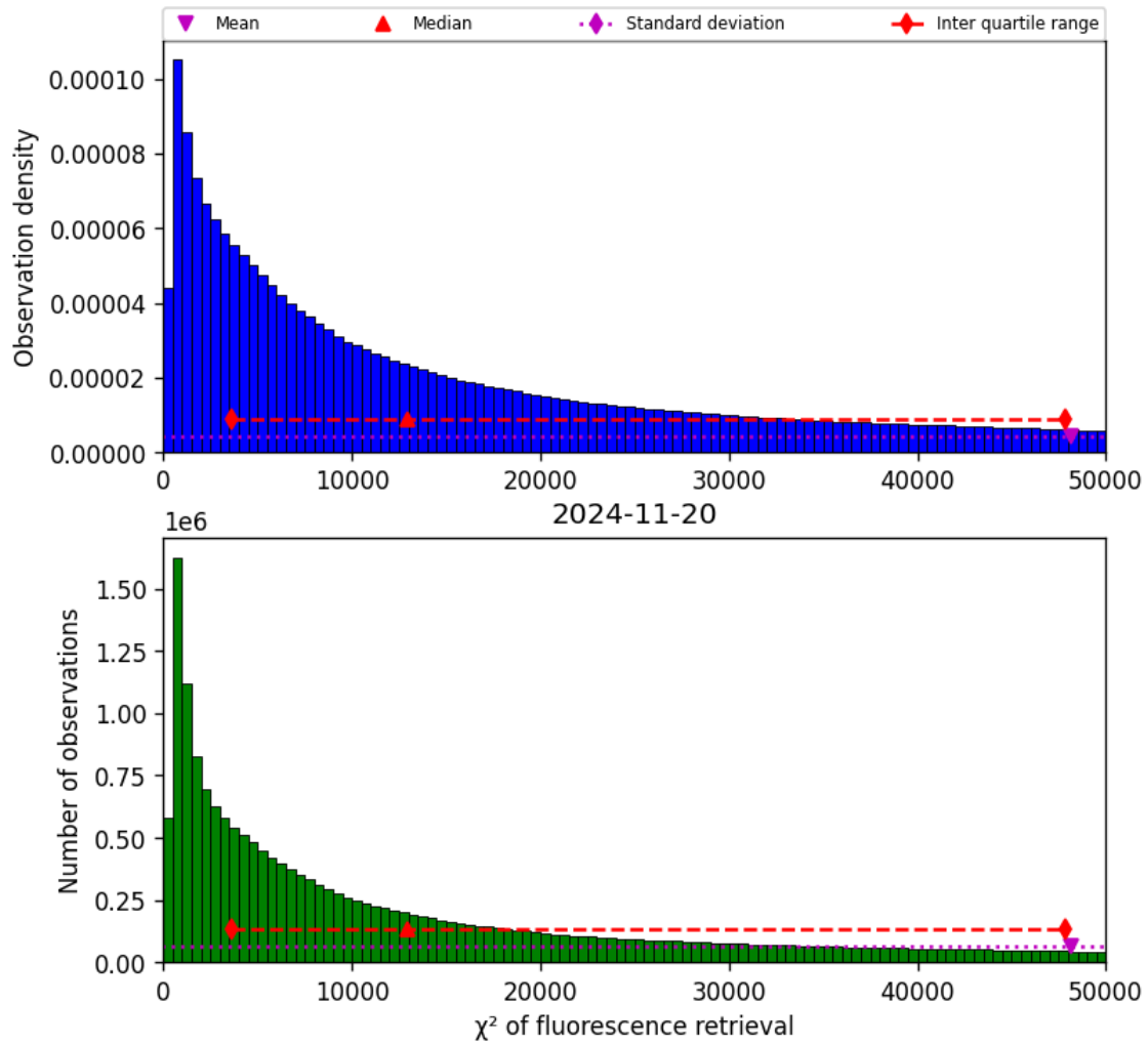
Figure 42: Histogram of “ \chi^2 of fluorescence retrieval” for 2024-11-20 to 2024-11-21
