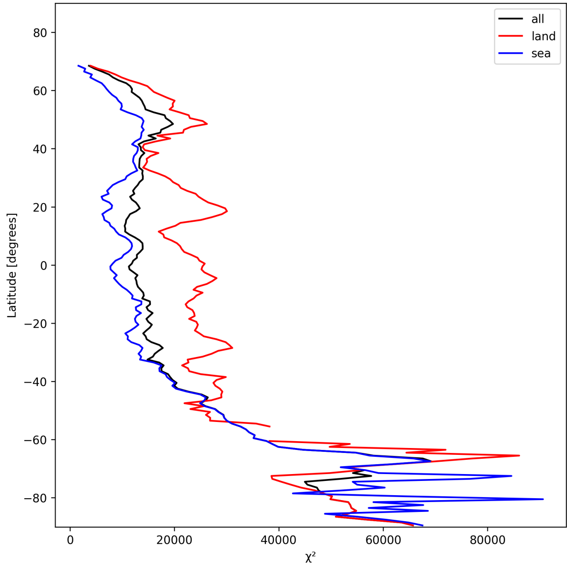
Figure 21: Zonal average of “ \chi^2 ” for 2024-11-20 to 2024-11-21.
