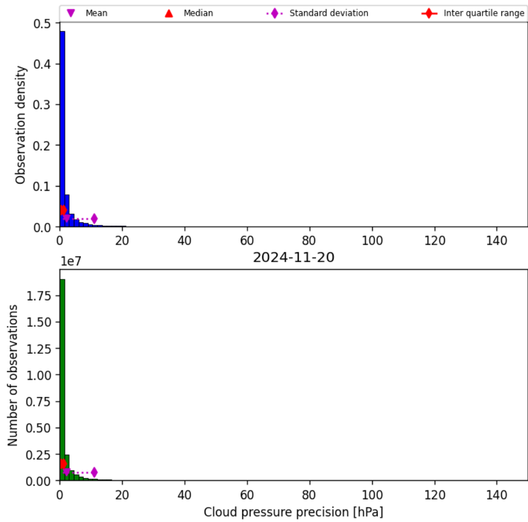
Figure 31: Histogram of “Cloud pressure precision” for 2024-11-20 to 2024-11-21
