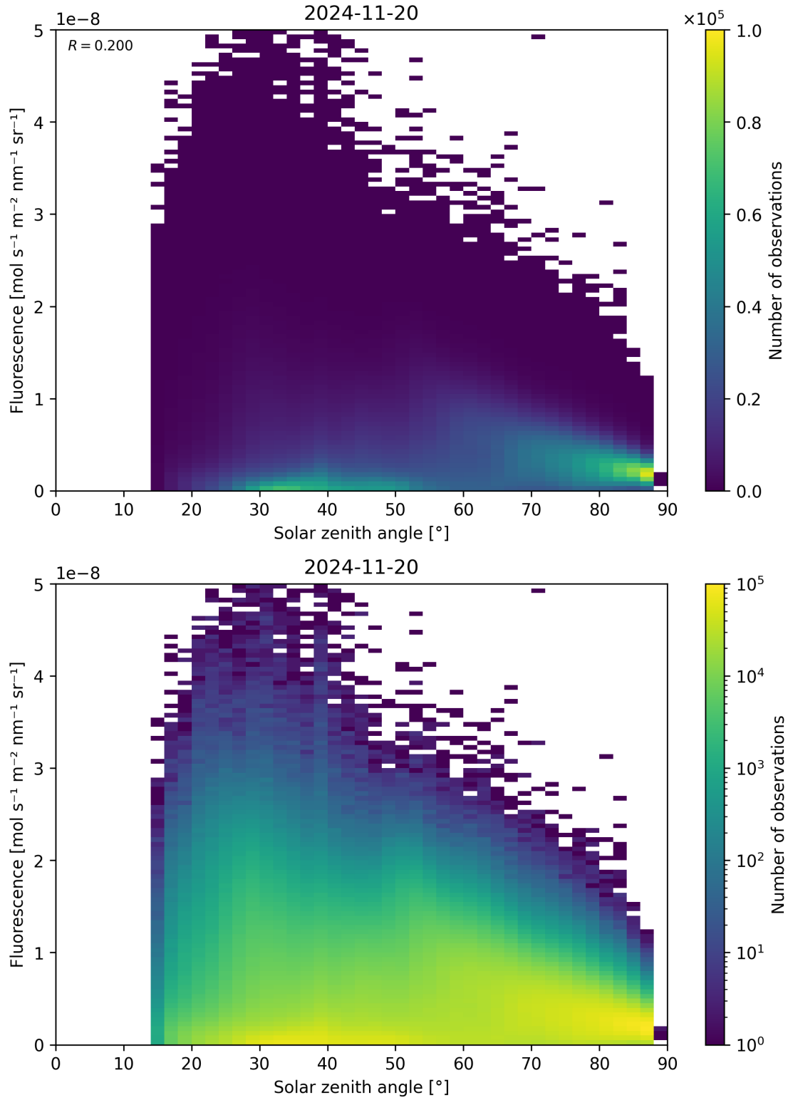
Figure 112: Scatter density plot of “Solar zenith angle” against “Fluorescence” for 2024-11-20 to 2024-11-21.
