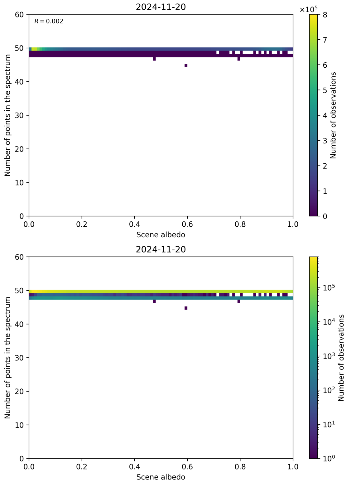
Figure 106: Scatter density plot of “Scene albedo” against “Number of points in the spectrum” for 2024-11-20 to 2024-11-21.
