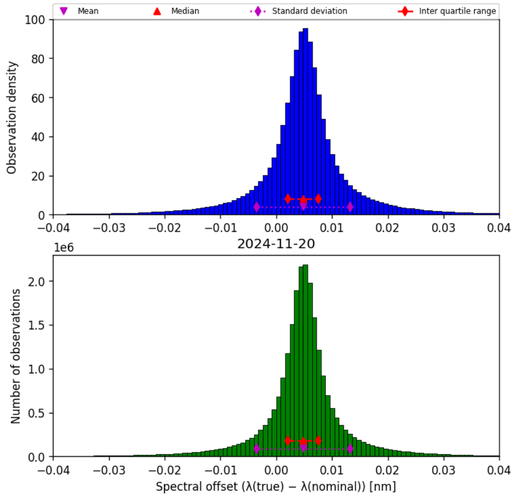
Figure 45: Histogram of “Spectral offset ( \lambda_{\text{true}} - \lambda_{\text{nominal}} )” for 2024-11-20 to 2024-11-21
