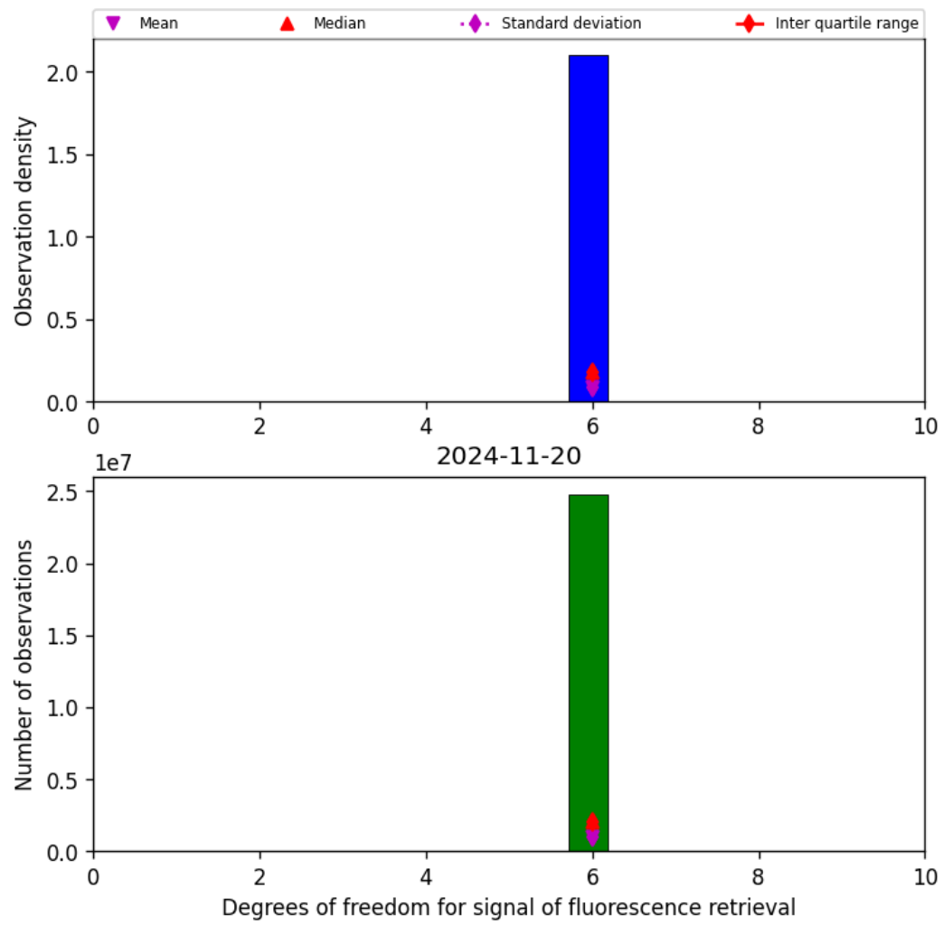
Figure 43: Histogram of “Degrees of freedom for signal of fluorescence retrieval” for 2024-11-20 to 2024-11-21
