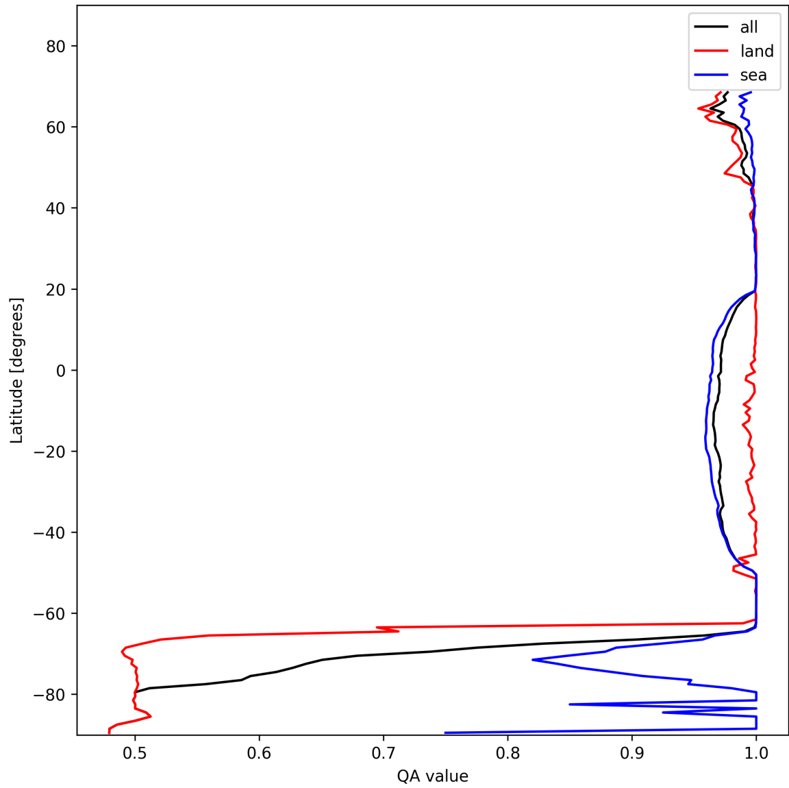
Figure 12: Zonal average of “QA value” for 2024-11-20 to 2024-11-21.
