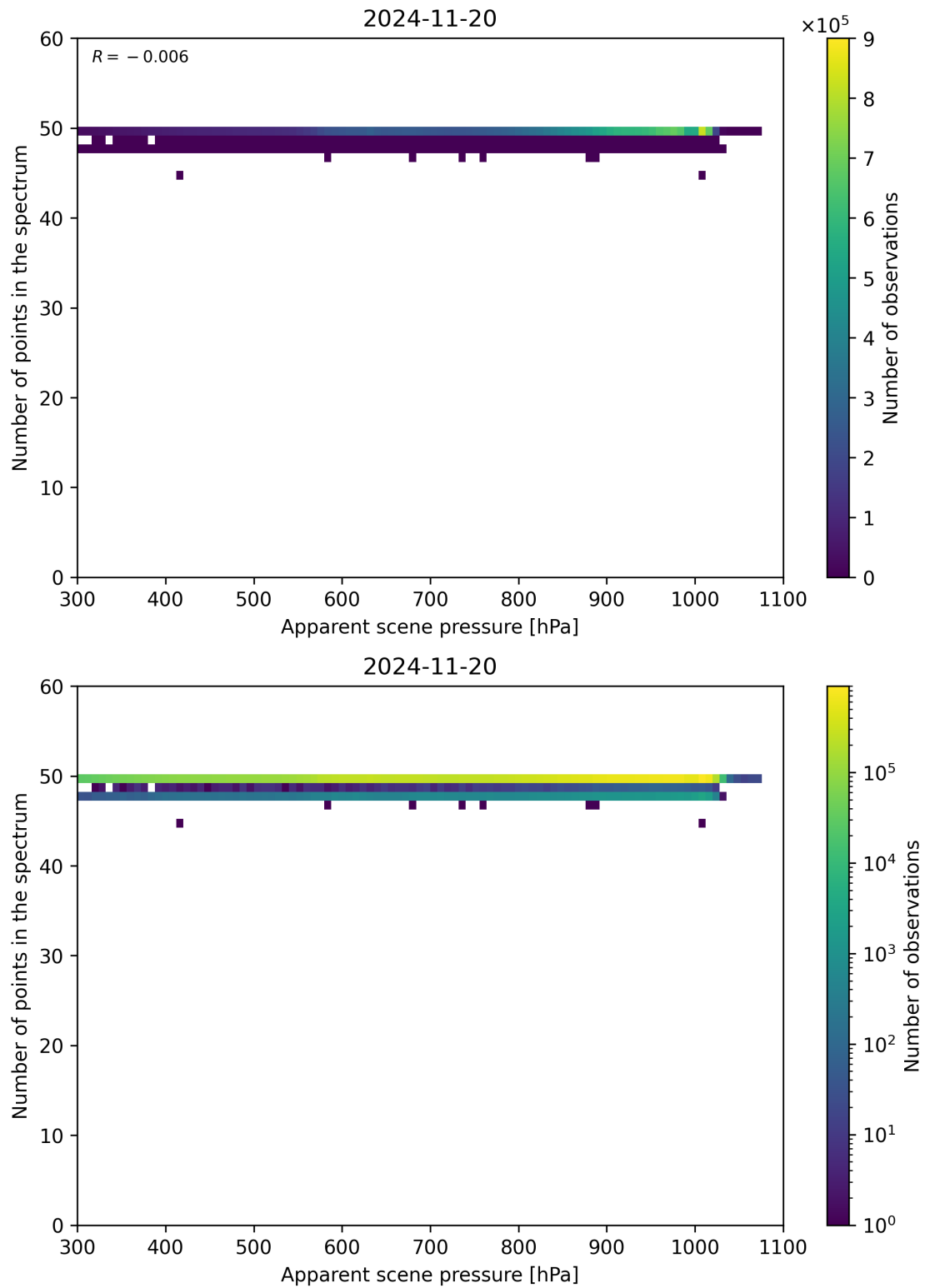
Figure 66: Scatter density plot of “Apparent scene pressure” against “Number of points in the spectrum” for 2024-11-20 to 2024-11-21.
