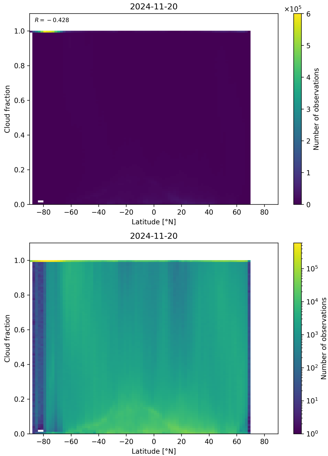
Figure 90: Scatter density plot of “Latitude” against “Cloud fraction” for 2024-11-20 to 2024-11-21.
