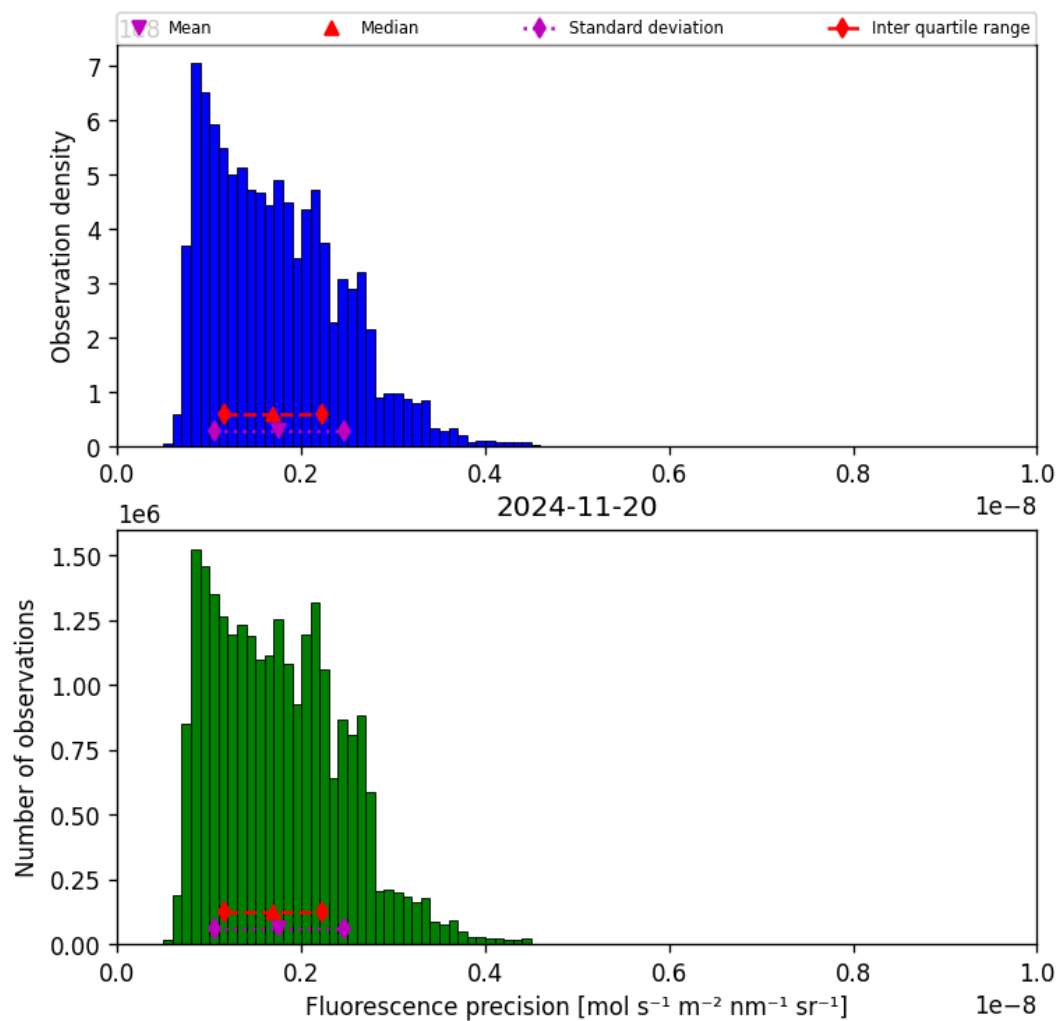
Figure 41: Histogram of “Fluorescence precision” for 2024-11-20 to 2024-11-21
