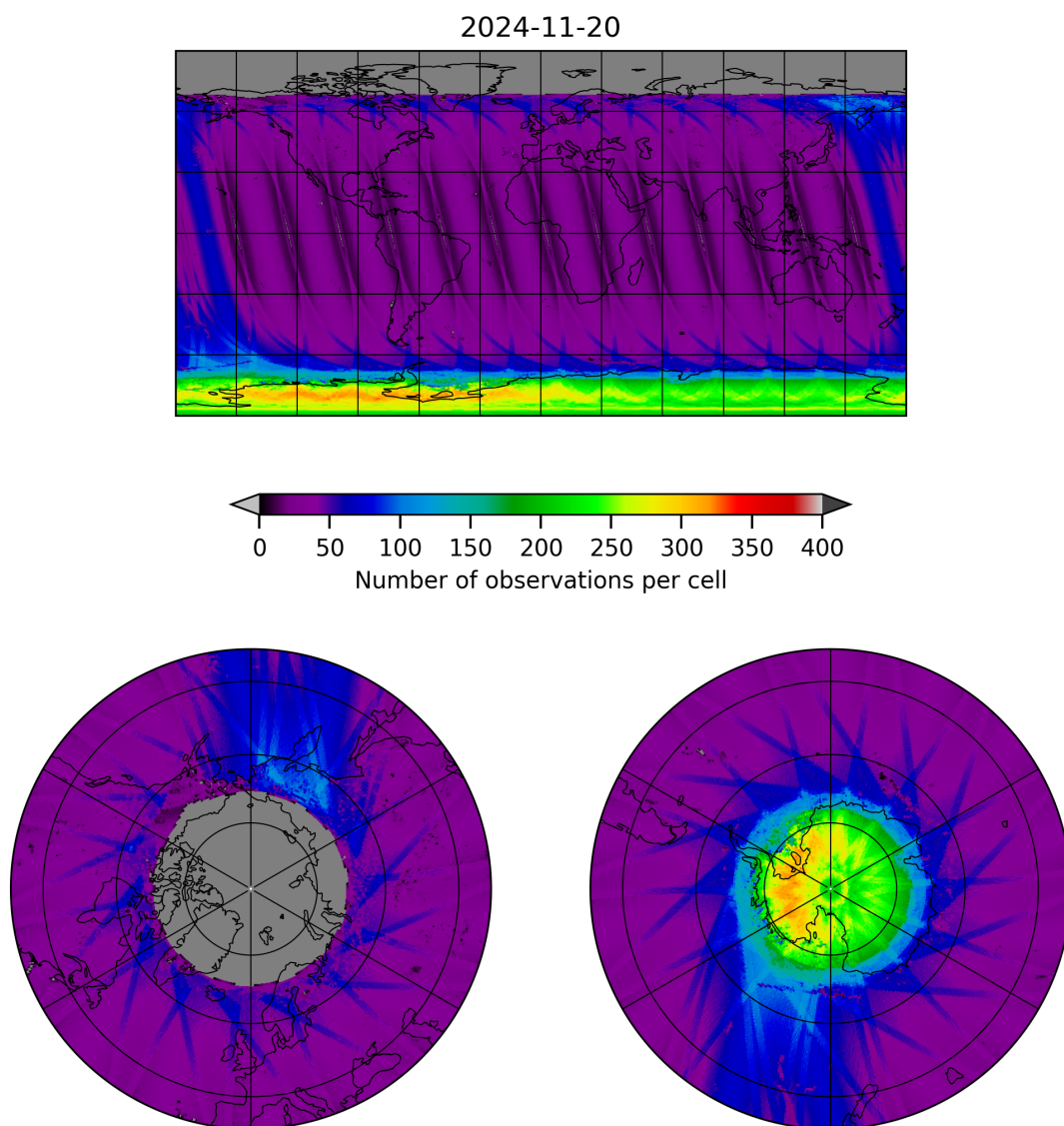
Figure 11: Map of the number of observations for 2024-11-20 to 2024-11-21
