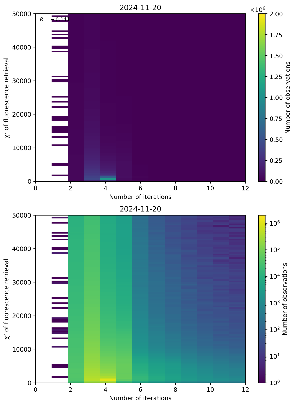
Figure 97: Scatter density plot of “Number of iterations” against “ \chi^2 of fluorescence retrieval” for 2024-11-20 to 2024-11-21.
