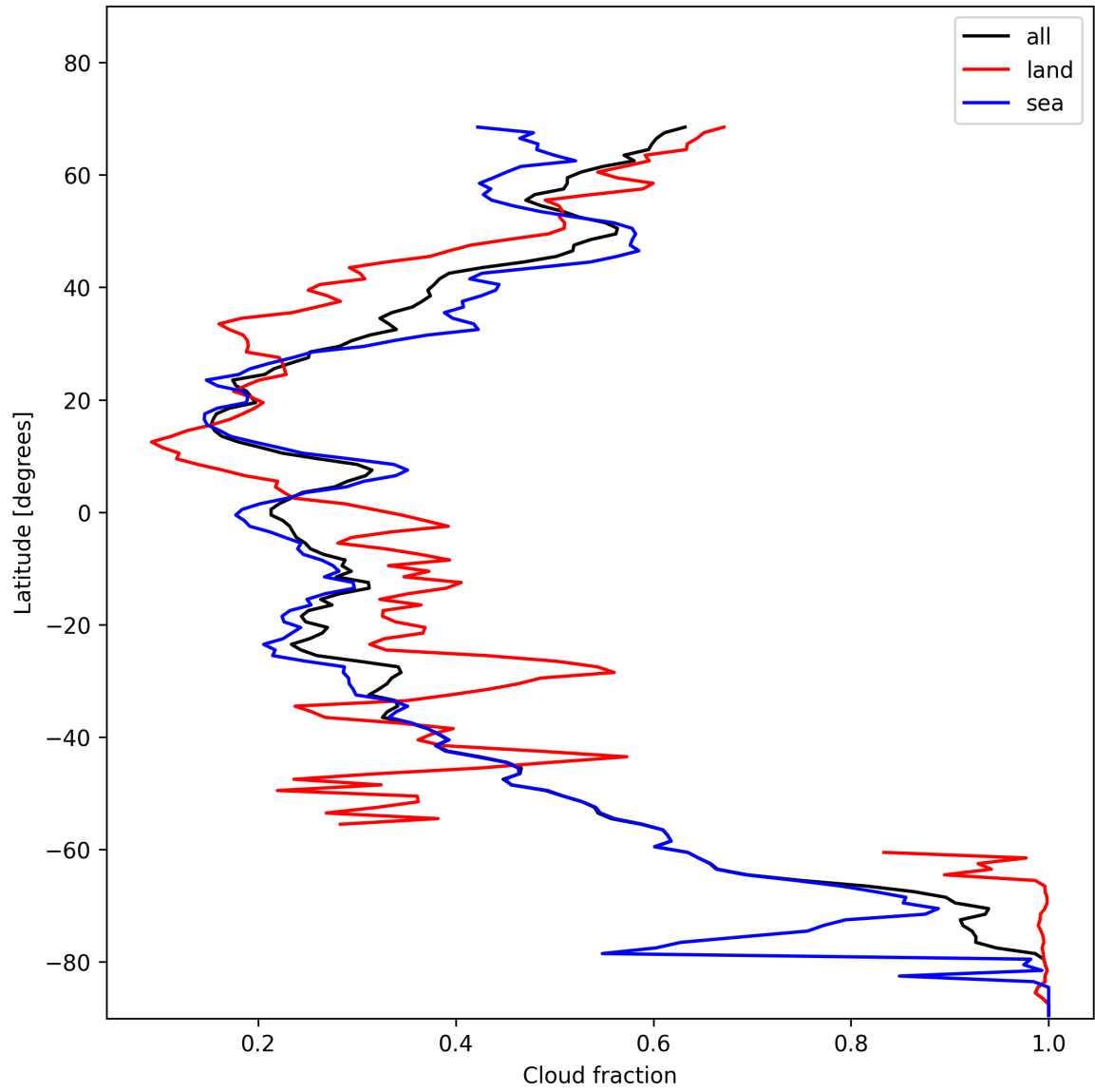
Figure 15: Zonal average of “Cloud fraction” for 2024-11-20 to 2024-11-21.
