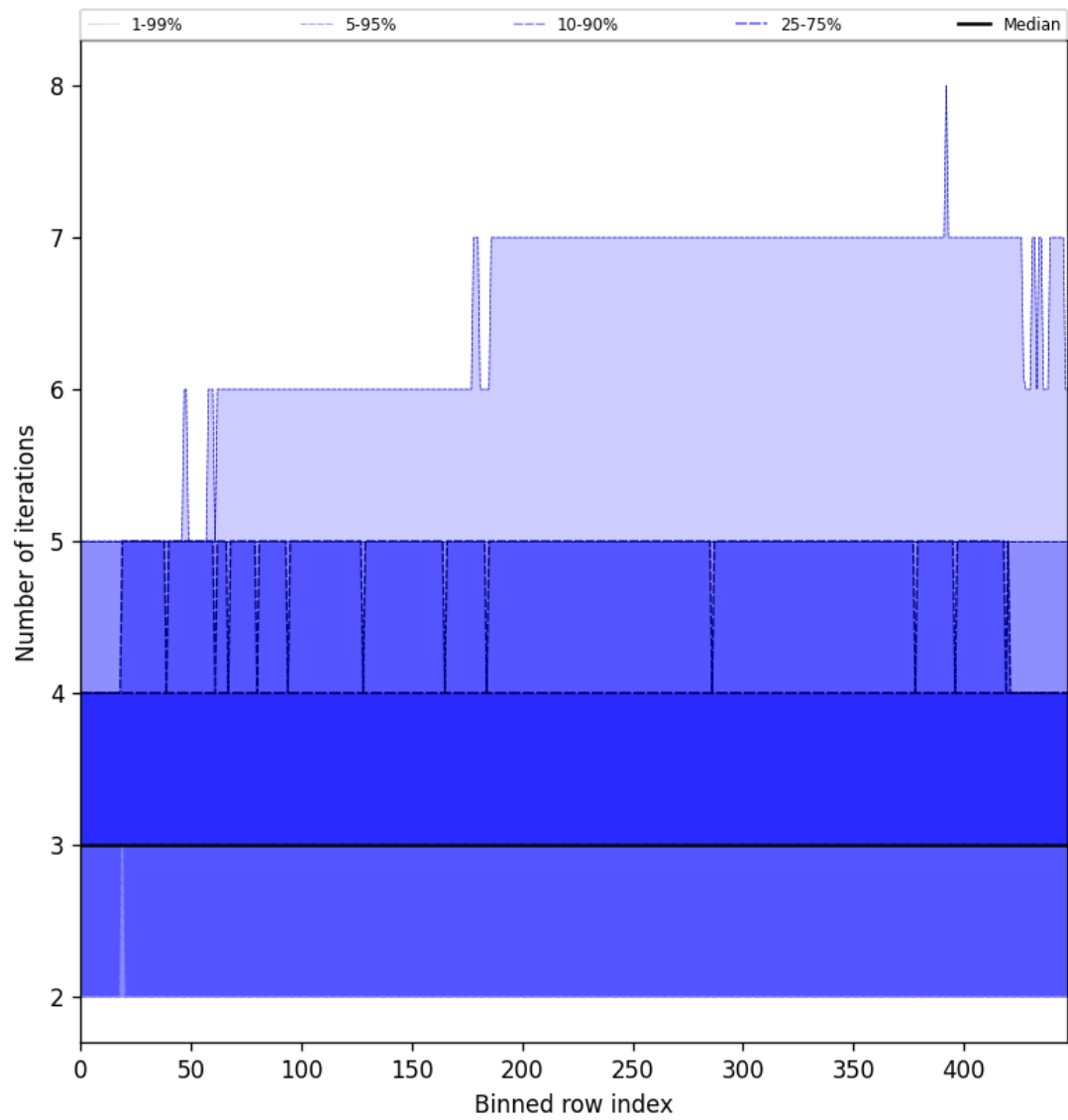
Figure 56: Along track statistics of “Number of iterations” for 2024-11-20 to 2024-11-21
