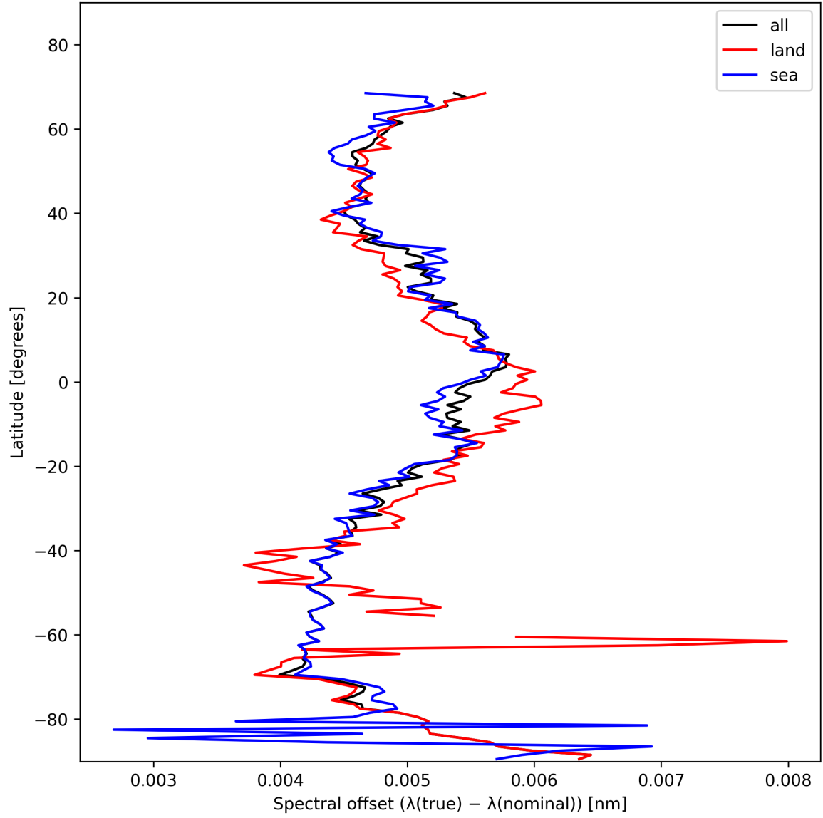
Figure 28: Zonal average of “Spectral offset ( \lambda_{\text{true}} - \lambda_{\text{nominal}} )” for 2024-11-20 to 2024-11-21.
