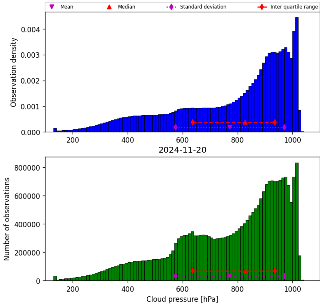
Figure 30: Histogram of “Cloud pressure” for 2024-11-20 to 2024-11-21
