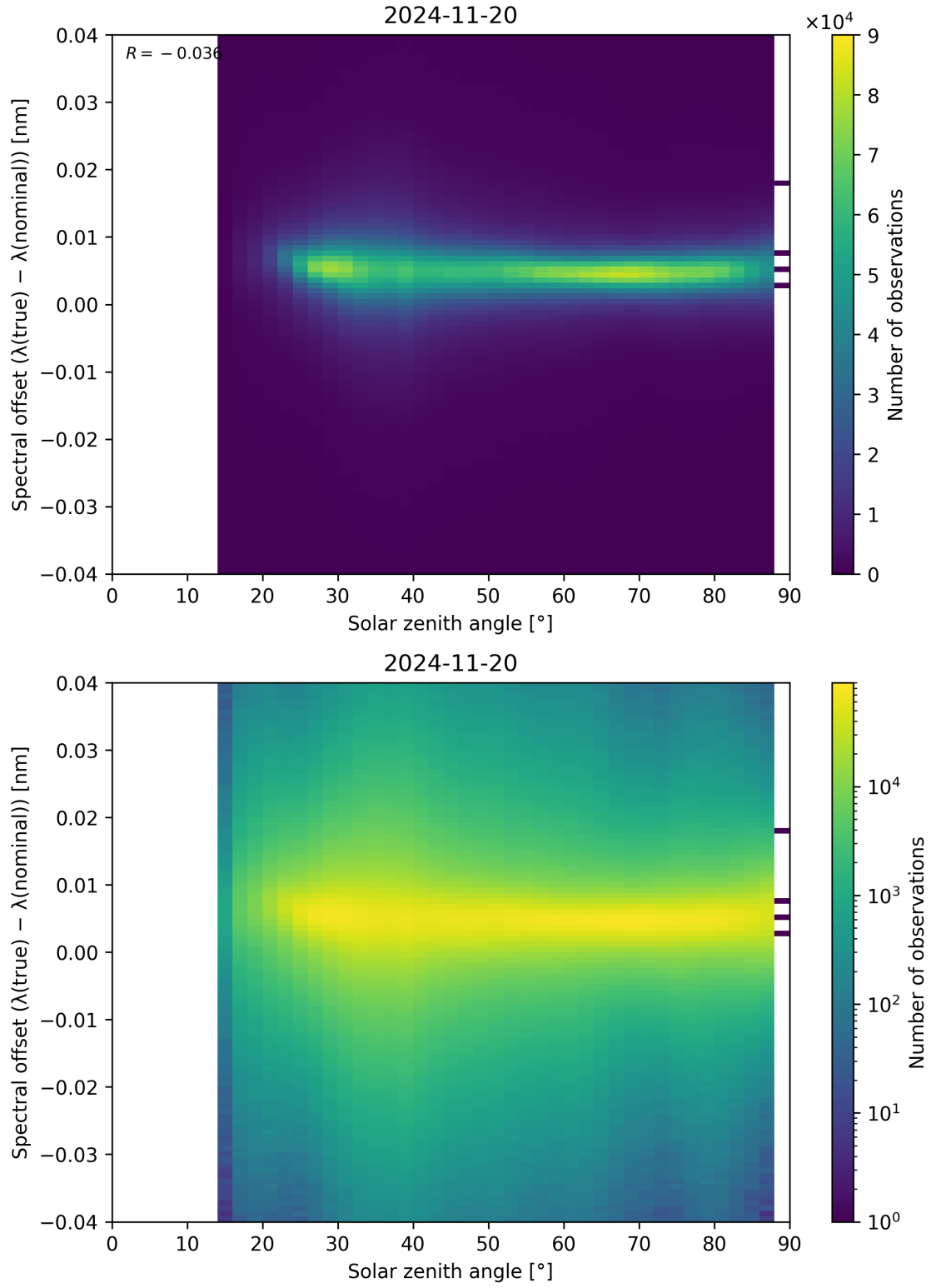
Figure 117: Scatter density plot of “Solar zenith angle” against “Spectral offset ( \lambda_{\text{true}} - \lambda_{\text{nominal}} )” for 2024-11-20 to 2024-11-21.
