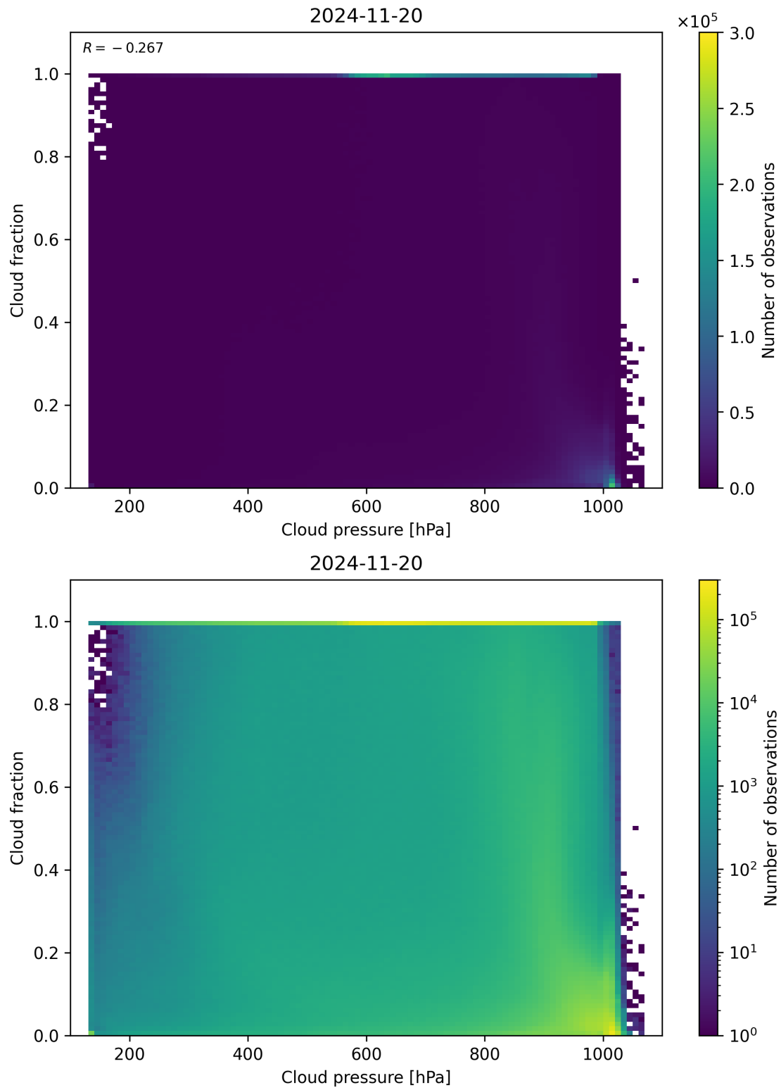
Figure 79: Scatter density plot of “Cloud pressure” against “Cloud fraction” for 2024-11-20 to 2024-11-21.
