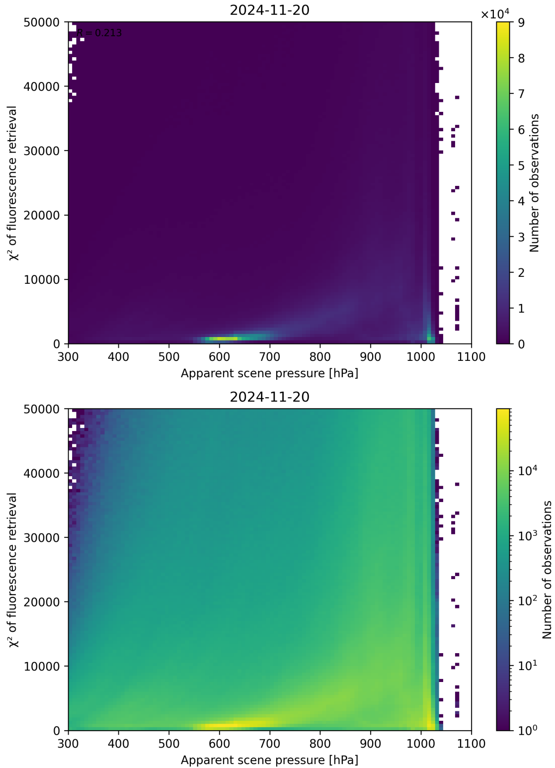
Figure 63: Scatter density plot of “Apparent scene pressure” against “ \chi^2 of fluorescence retrieval” for 2024-11-20 to 2024-11-21.
