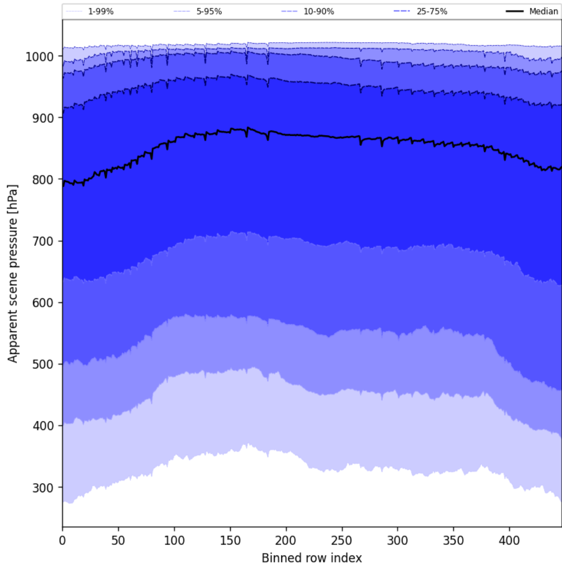
Figure 53: Along track statistics of “Apparent scene pressure” for 2024-11-20 to 2024-11-21
