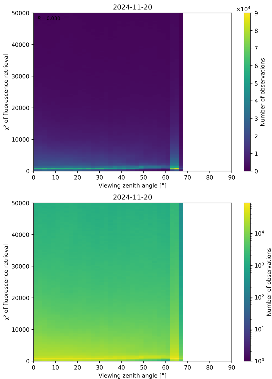
Figure 119: Scatter density plot of “Viewing zenith angle” against “ \chi^2 of fluorescence retrieval” for 2024-11-20 to 2024-11-21.
