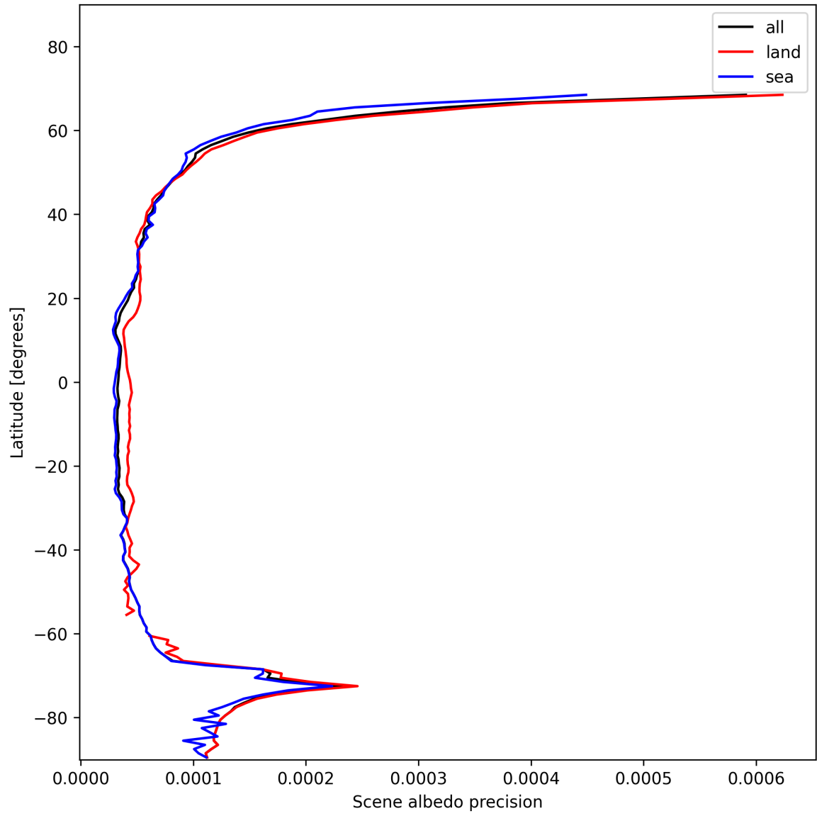
Figure 18: Zonal average of “Scene albedo precision” for 2024-11-20 to 2024-11-21.
