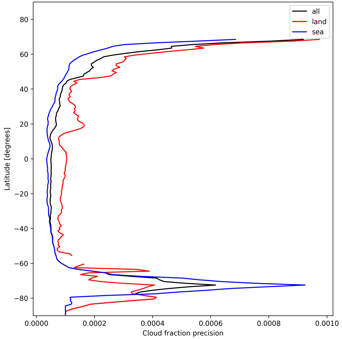
Figure 16: Zonal average of “Cloud fraction precision” for 2024-11-20 to 2024-11-21.
