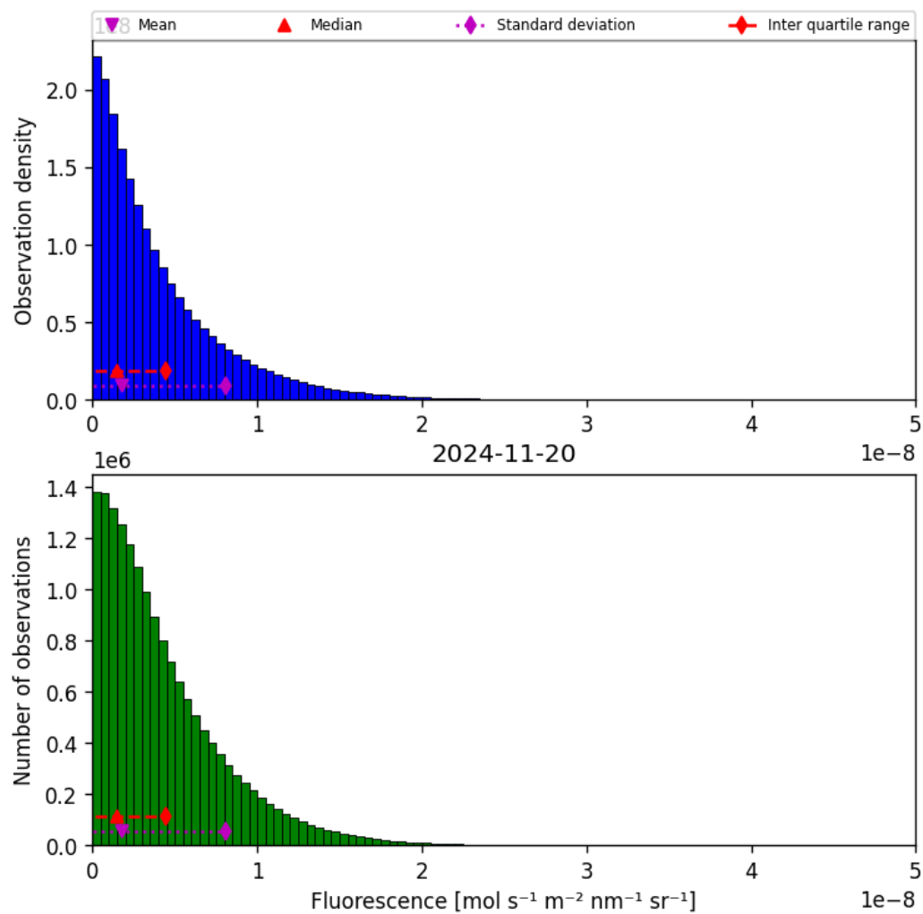
Figure 40: Histogram of “Fluorescence” for 2024-11-20 to 2024-11-21
