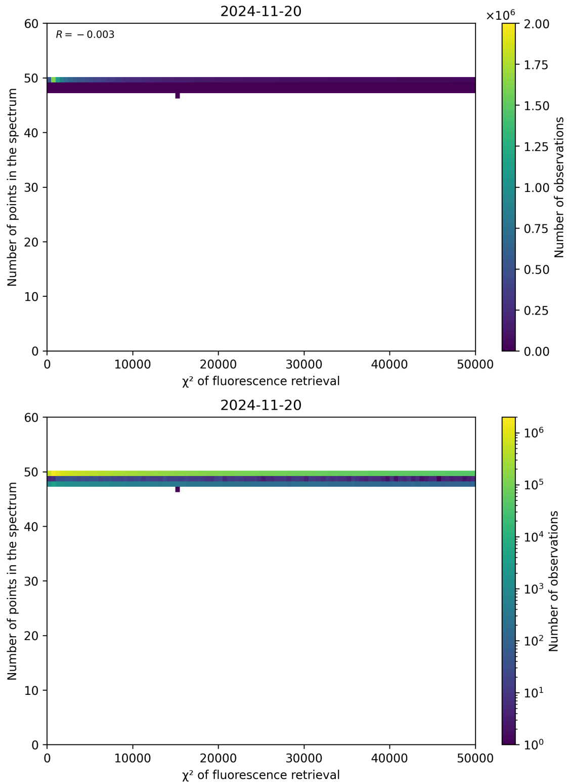
Figure 68: Scatter density plot of “ \chi^2 of fluorescence retrieval” against “Number of points in the spectrum” for 2024-11-20 to 2024-11-21.
