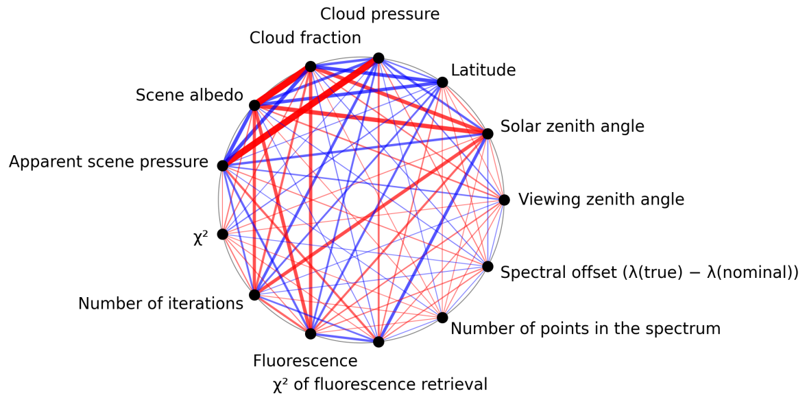
Figure 1: Map of correlation graph for 2024-11-20 to 2024-11-21.
