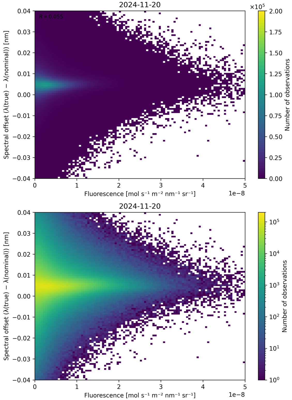
Figure 87: Scatter density plot of “Fluorescence” against “Spectral offset ( \lambda_{\text{true}} - \lambda_{\text{nominal}} )” for 2024-11-20 to 2024-11-21.
