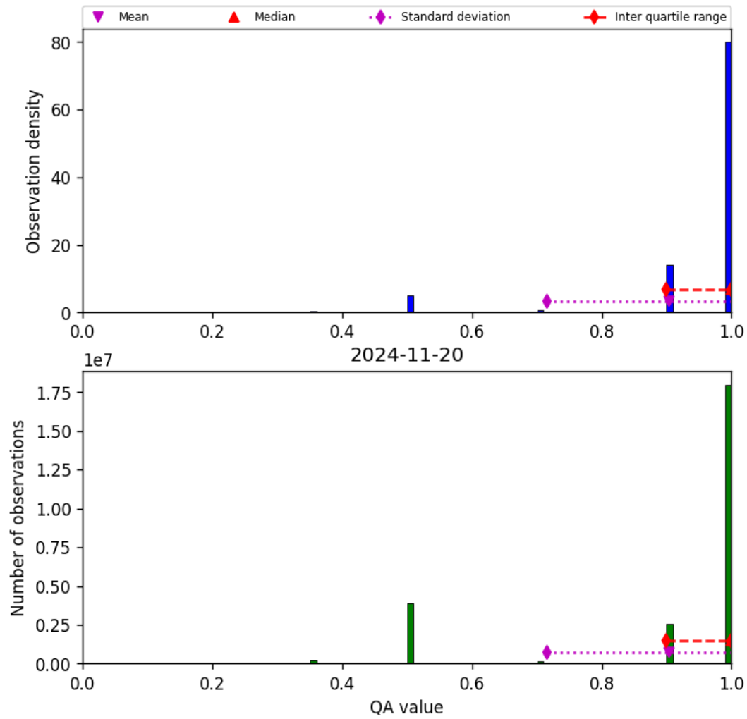
Figure 29: Histogram of “QA value” for 2024-11-20 to 2024-11-21
