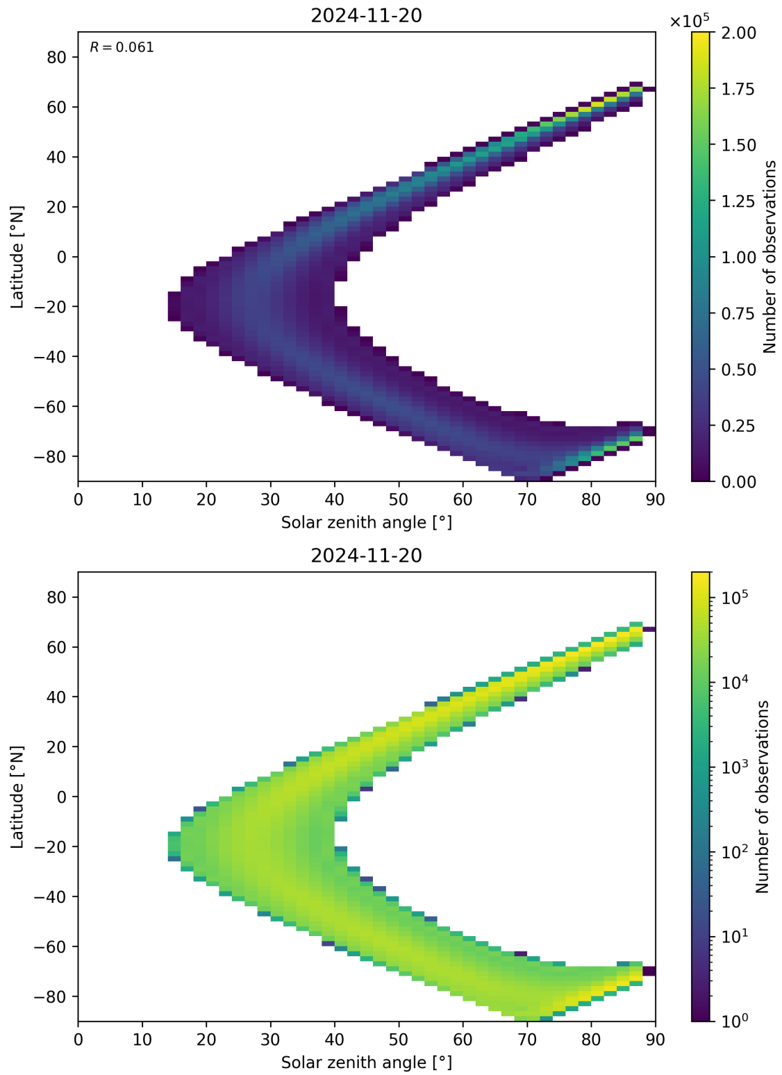
Figure 113: Scatter density plot of “Solar zenith angle” against “Latitude” for 2024-11-20 to 2024-11-21.
