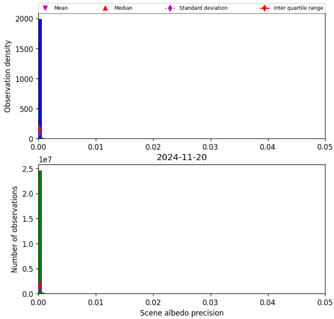
Figure 35: Histogram of “Scene albedo precision” for 2024-11-20 to 2024-11-21
