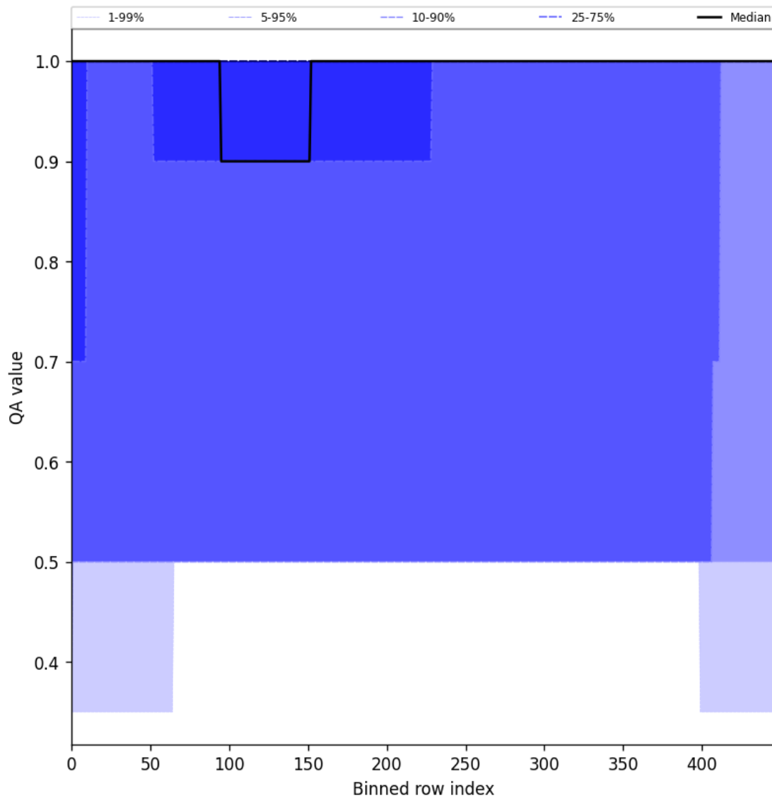
Figure 46: Along track statistics of “QA value” for 2024-11-20 to 2024-11-21
