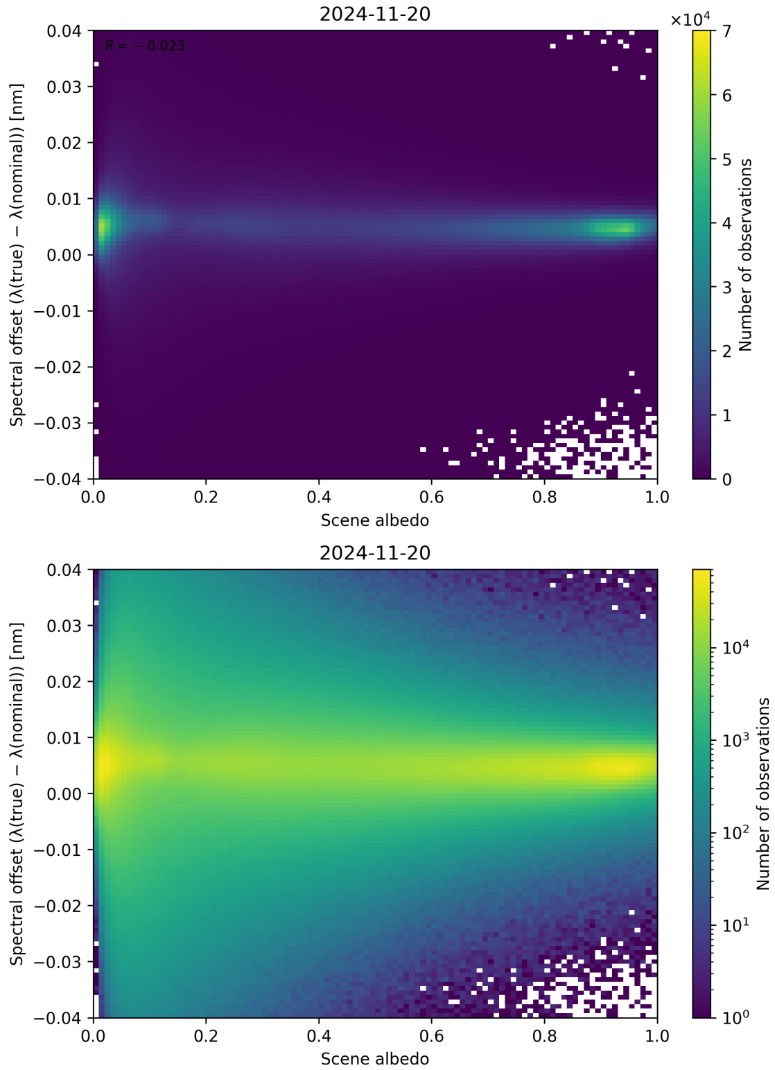
Figure 107: Scatter density plot of “Scene albedo” against “Spectral offset ( \lambda_{\text{true}} - \lambda_{\text{nominal}} )” for 2024-11-20 to 2024-11-21.
