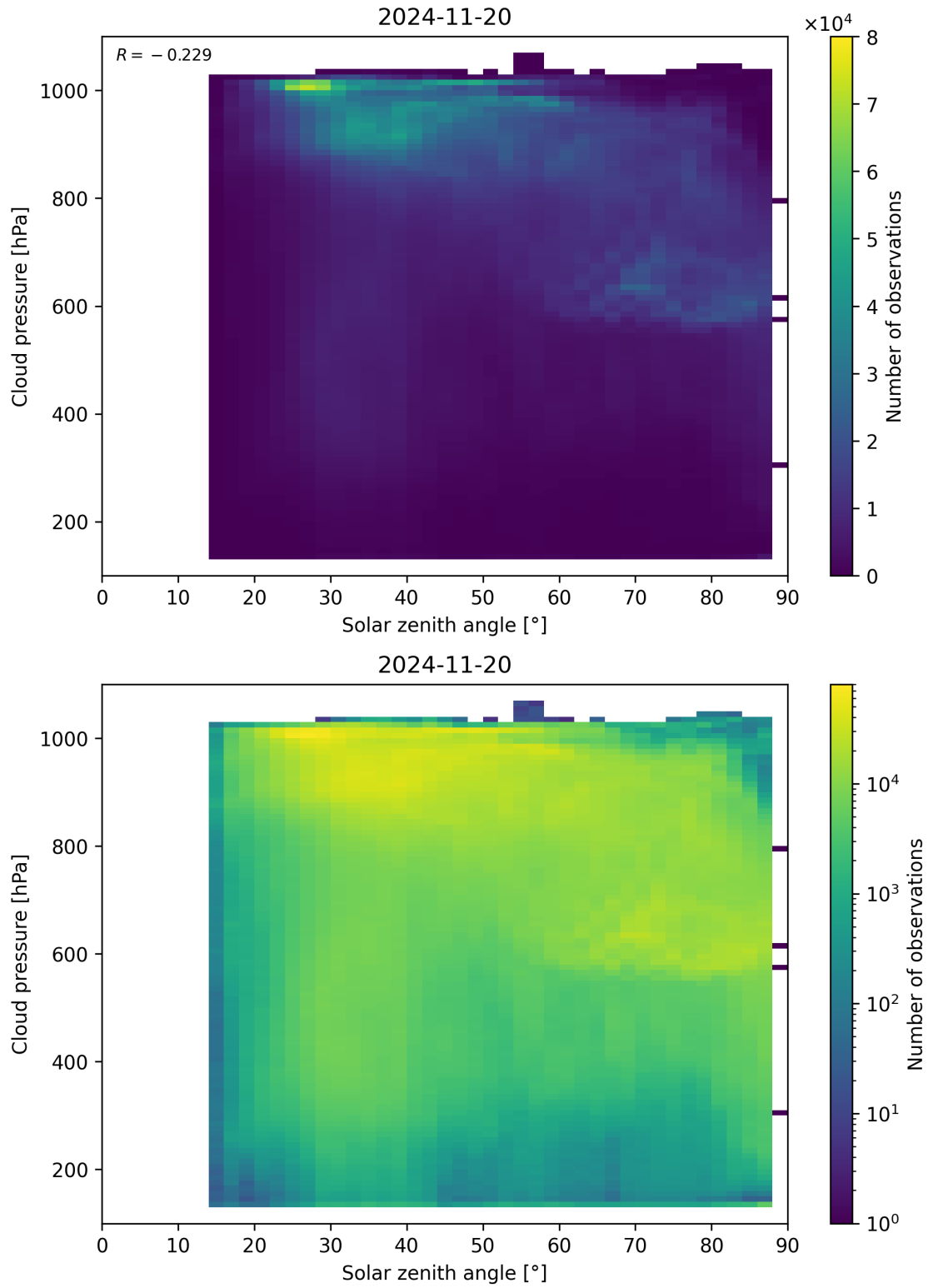
Figure 111: Scatter density plot of “Solar zenith angle” against “Cloud pressure” for 2024-11-20 to 2024-11-21.
