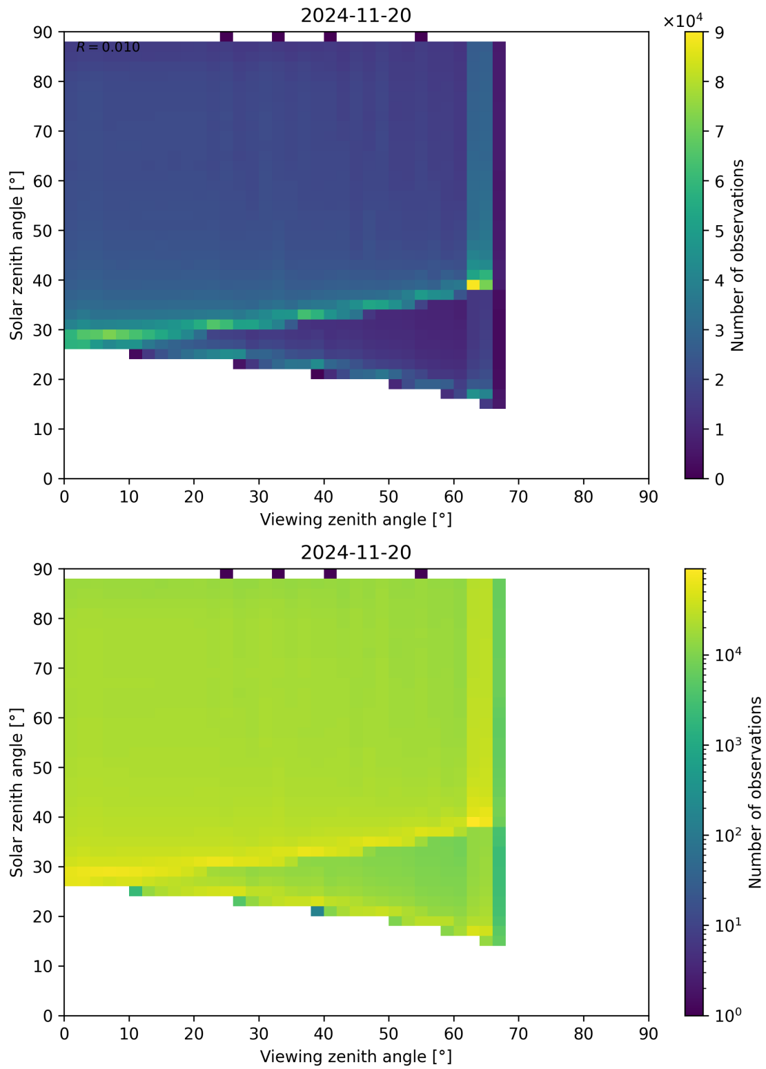
Figure 127: Scatter density plot of “Viewing zenith angle” against “Solar zenith angle” for 2024-11-20 to 2024-11-21.
