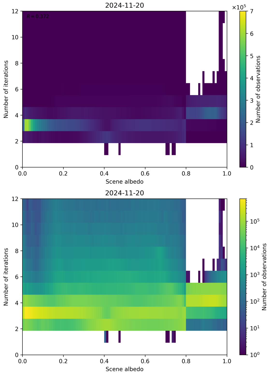
Figure 105: Scatter density plot of “Scene albedo” against “Number of iterations” for 2024-11-20 to 2024-11-21.
