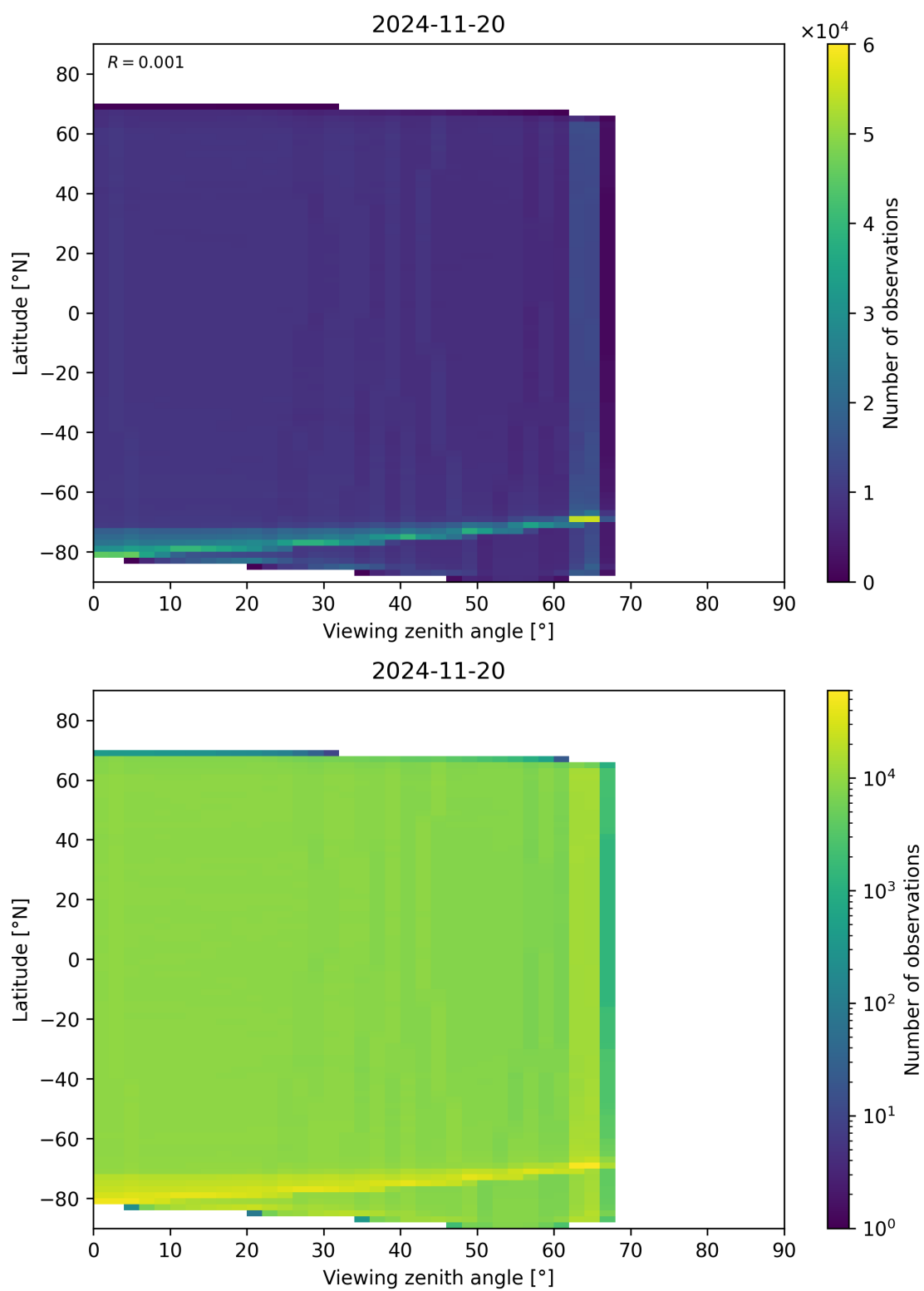
Figure 123: Scatter density plot of “Viewing zenith angle” against “Latitude” for 2024-11-20 to 2024-11-21.
