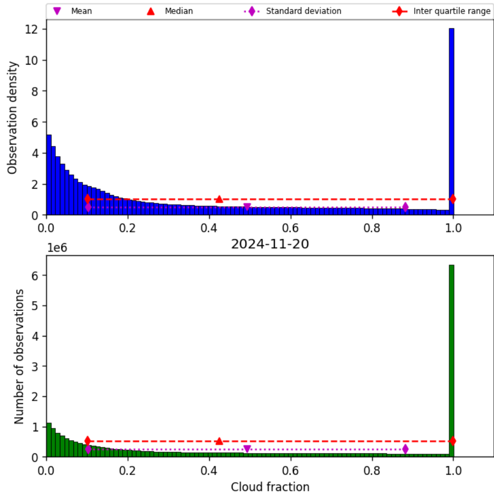
Figure 32: Histogram of “Cloud fraction” for 2024-11-20 to 2024-11-21
