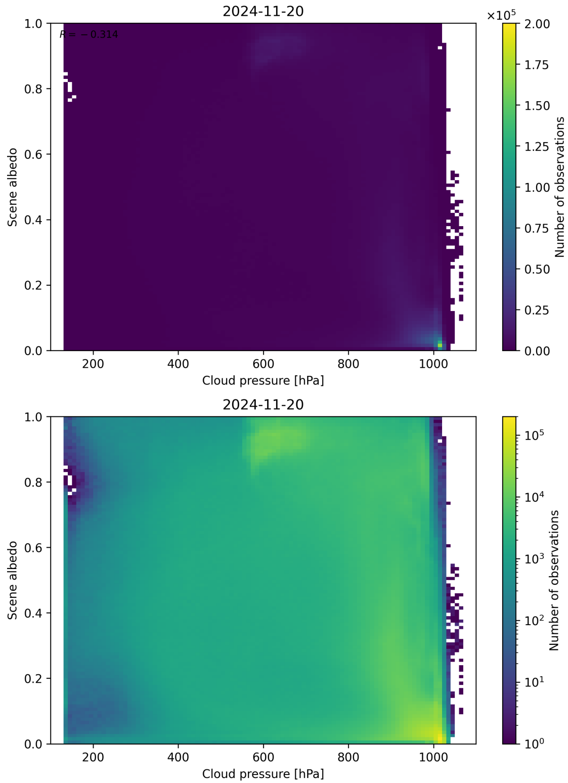
Figure 83: Scatter density plot of “Cloud pressure” against “Scene albedo” for 2024-11-20 to 2024-11-21.
