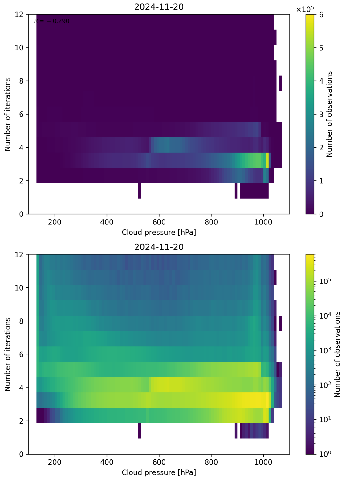
Figure 81: Scatter density plot of “Cloud pressure” against “Number of iterations” for 2024-11-20 to 2024-11-21.
