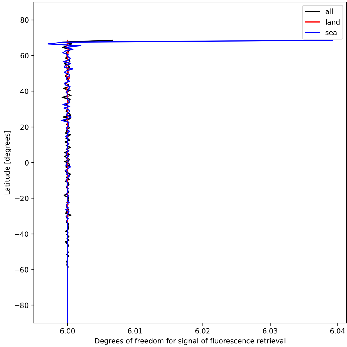
Figure 26: Zonal average of “Degrees of freedom for signal of fluorescence retrieval” for 2024-11-20 to 2024-11-21.
