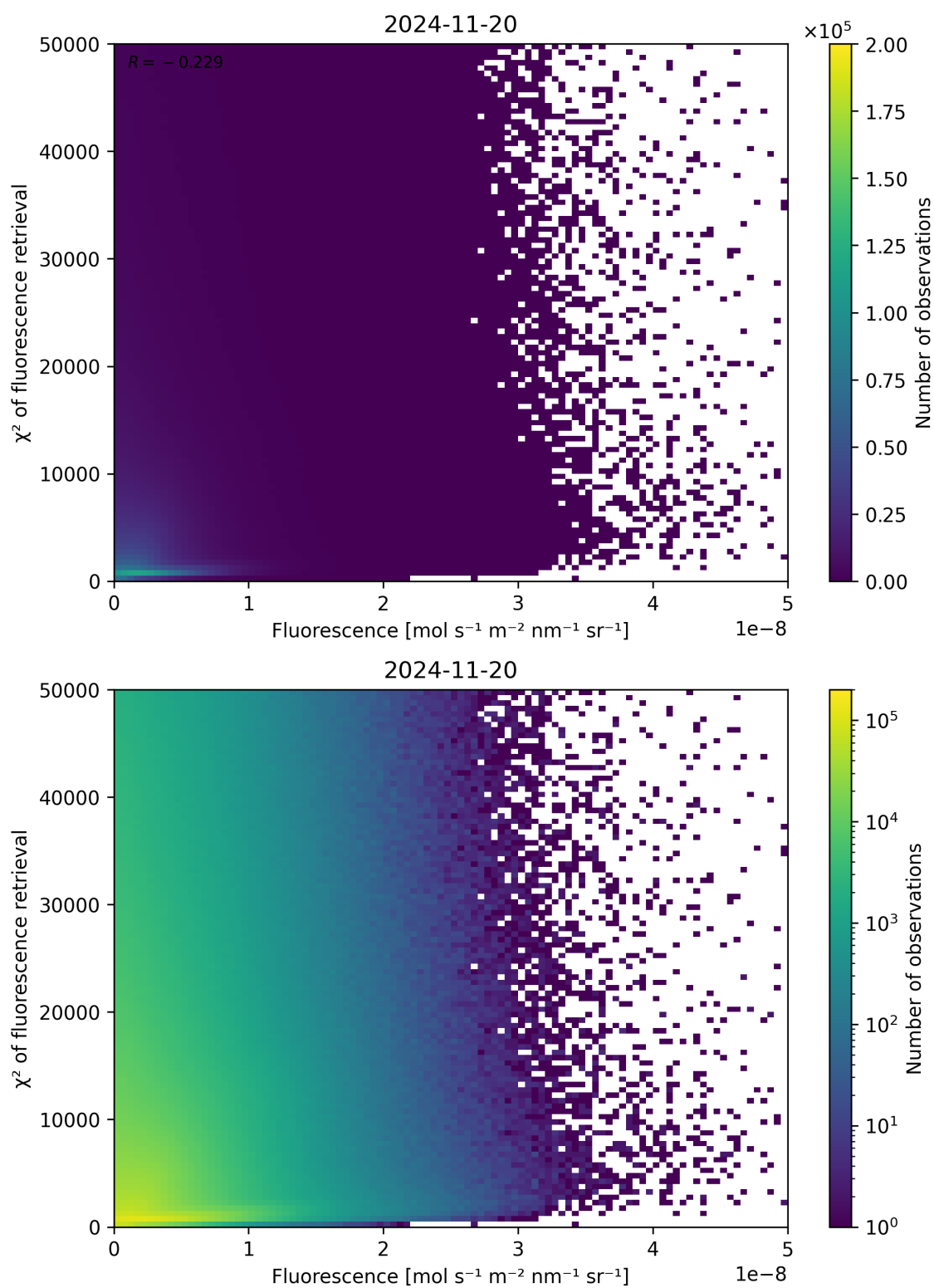
Figure 85: Scatter density plot of “Fluorescence” against “ \chi^2 of fluorescence retrieval” for 2024-11-20 to 2024-11-21.
