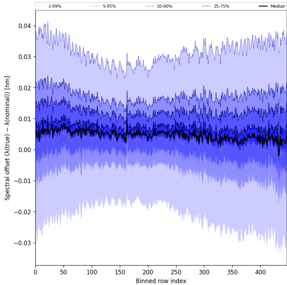
Figure 62: Along track statistics of “Spectral offset ( \lambda_{\text{true}} - \lambda_{\text{nominal}} )” for 2024-11-20 to 2024-11-21
