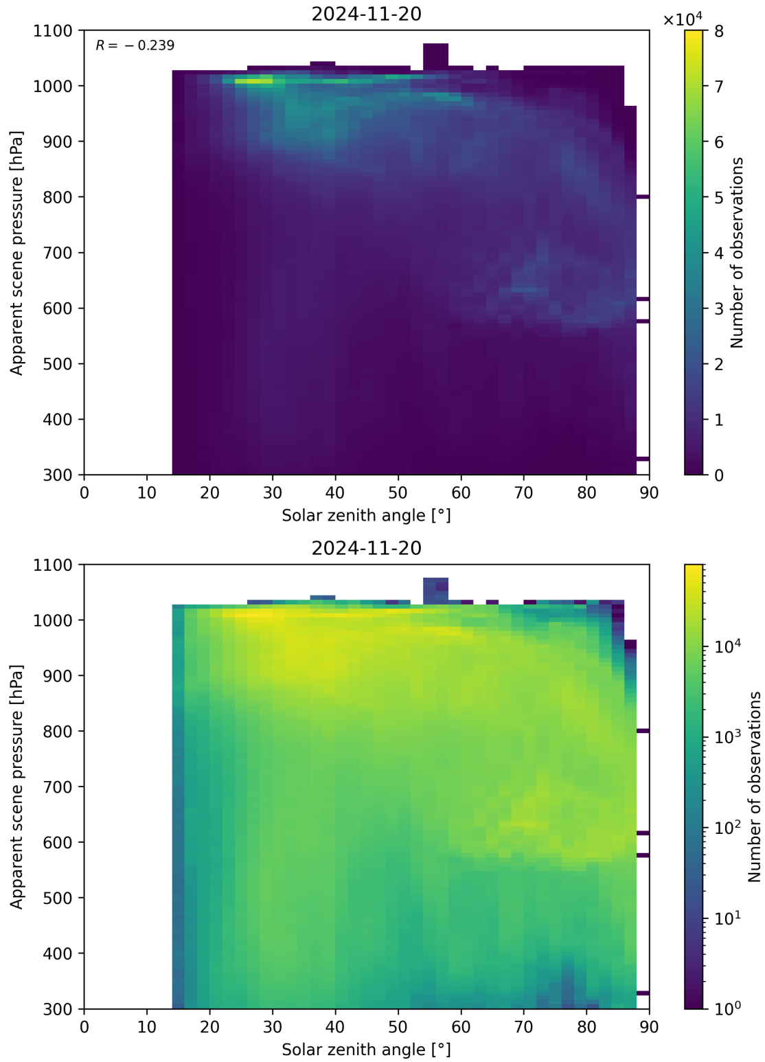
Figure 108: Scatter density plot of “Solar zenith angle” against “Apparent scene pressure” for 2024-11-20 to 2024-11-21.
