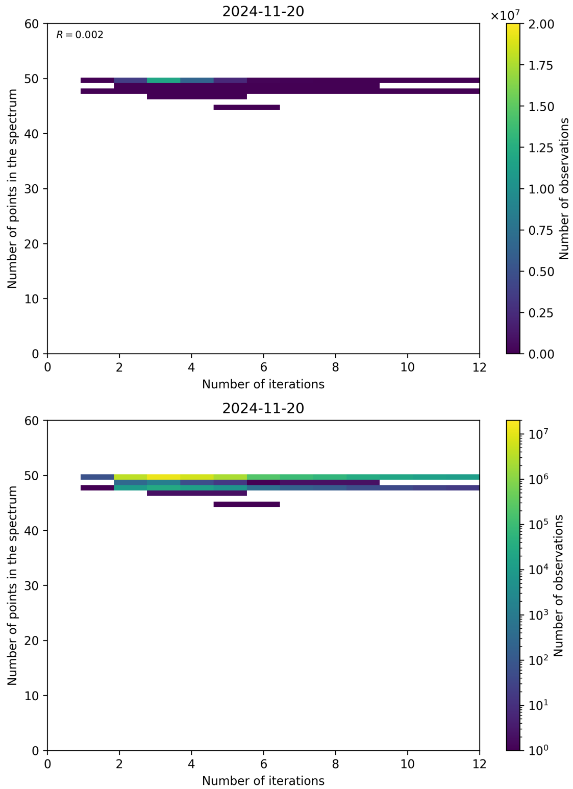
Figure 99: Scatter density plot of “Number of iterations” against “Number of points in the spectrum” for 2024-11-20 to 2024-11-21.
