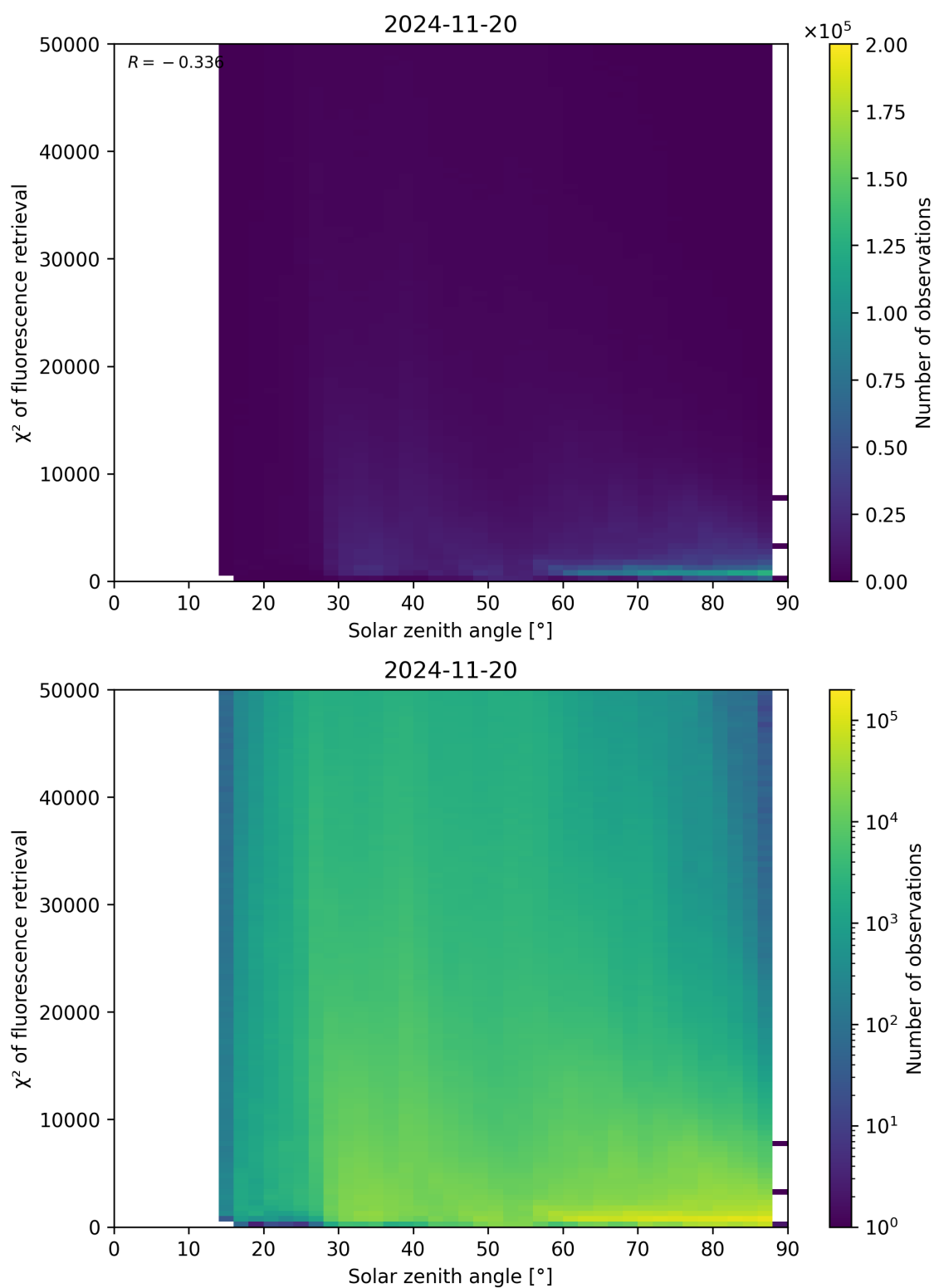
Figure 109: Scatter density plot of “Solar zenith angle” against “ \chi^2 of fluorescence retrieval” for 2024-11-20 to 2024-11-21.
