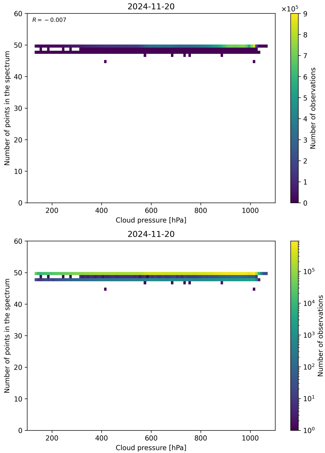
Figure 82: Scatter density plot of “Cloud pressure” against “Number of points in the spectrum” for 2024-11-20 to 2024-11-21.
