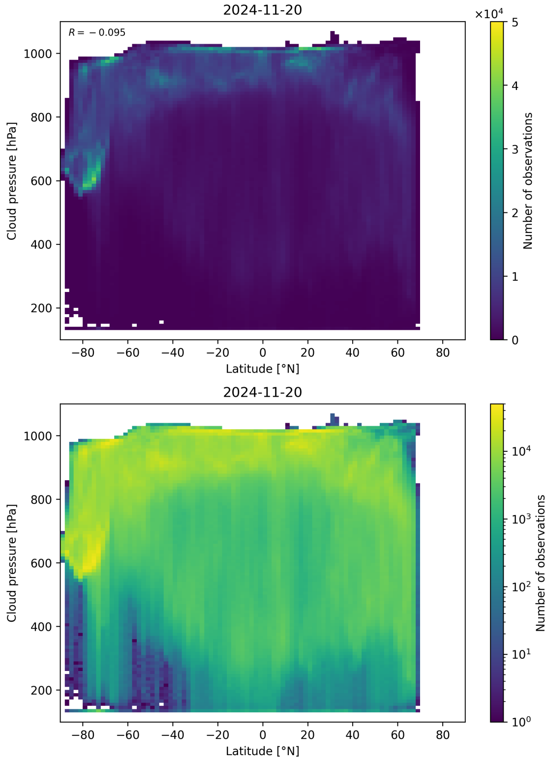
Figure 91: Scatter density plot of “Latitude” against “Cloud pressure” for 2024-11-20 to 2024-11-21.
