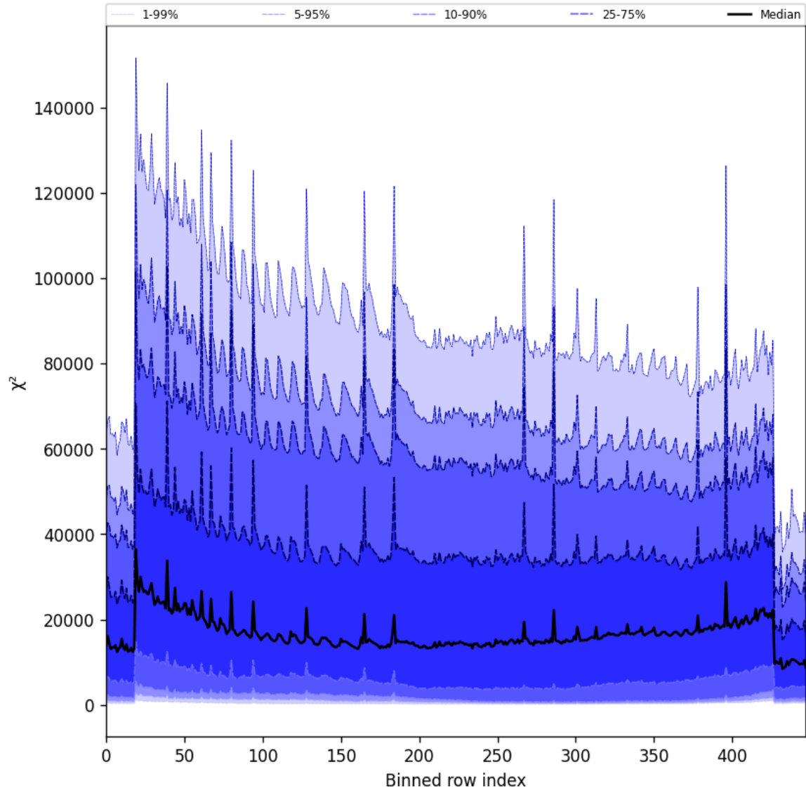
Figure 55: Along track statistics of “ \chi^2 ” for 2024-11-20 to 2024-11-21
