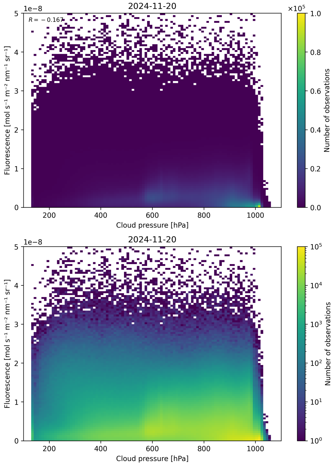
Figure 80: Scatter density plot of “Cloud pressure” against “Fluorescence” for 2024-11-20 to 2024-11-21.
