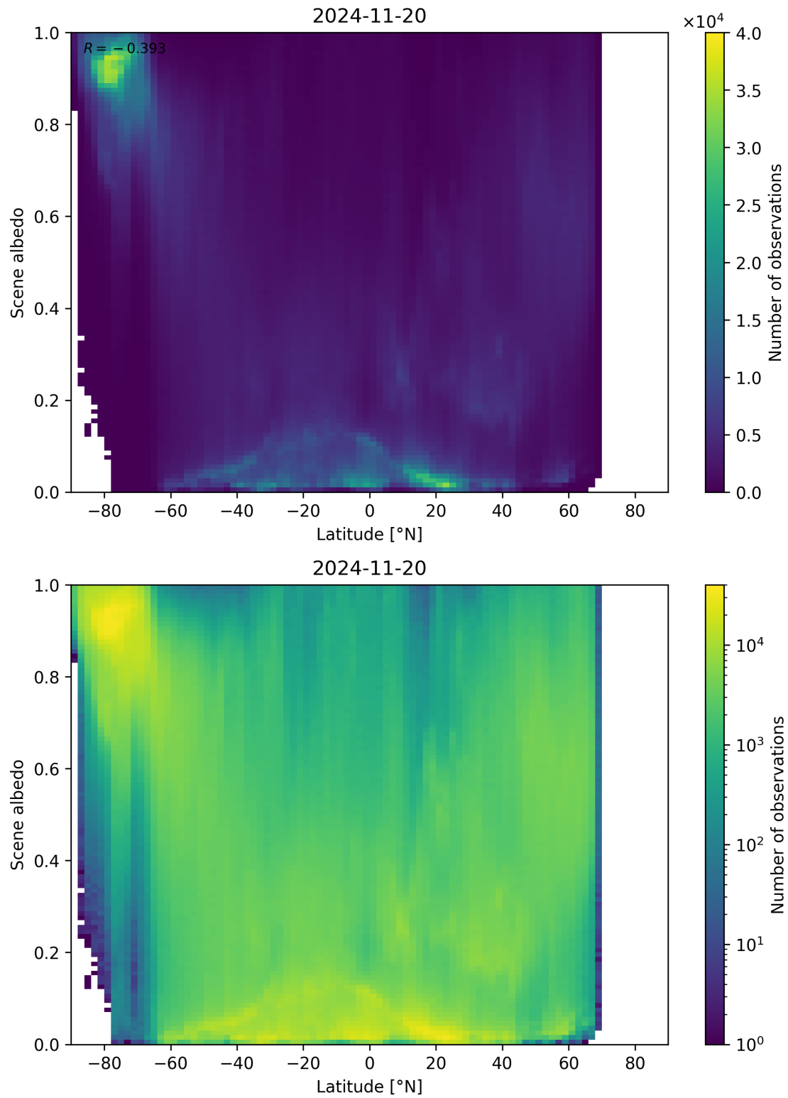
Figure 95: Scatter density plot of “Latitude” against “Scene albedo” for 2024-11-20 to 2024-11-21.
