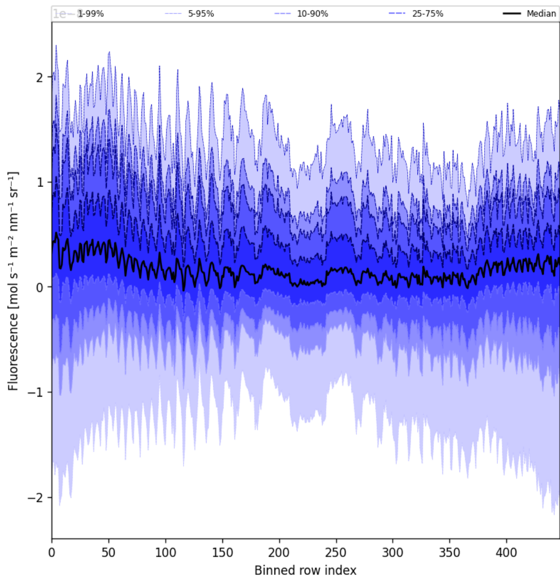
Figure 57: Along track statistics of “Fluorescence” for 2024-11-20 to 2024-11-21
