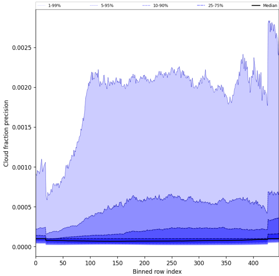
Figure 50: Along track statistics of “Cloud fraction precision” for 2024-11-20 to 2024-11-21
