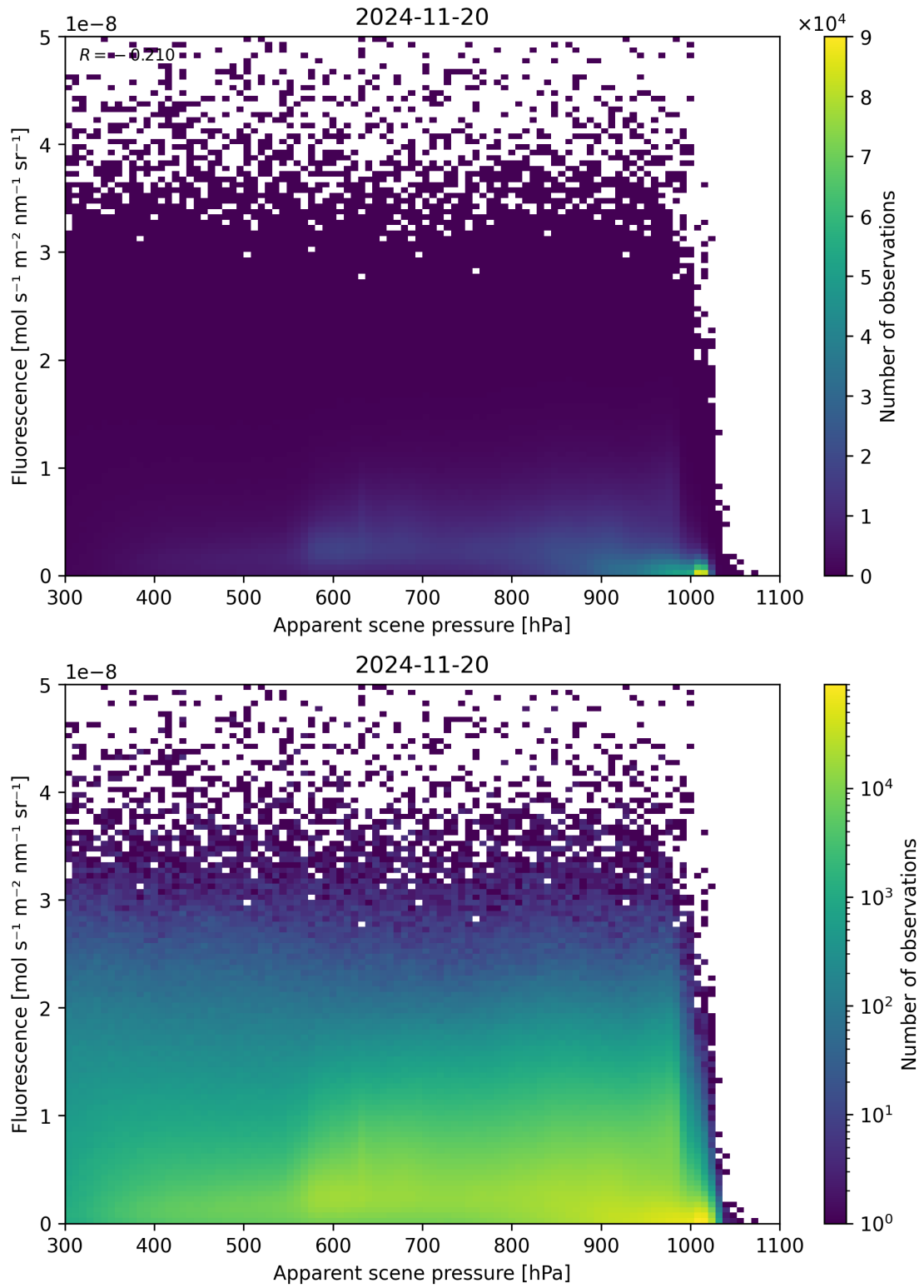
Figure 64: Scatter density plot of “Apparent scene pressure” against “Fluorescence” for 2024-11-20 to 2024-11-21.
