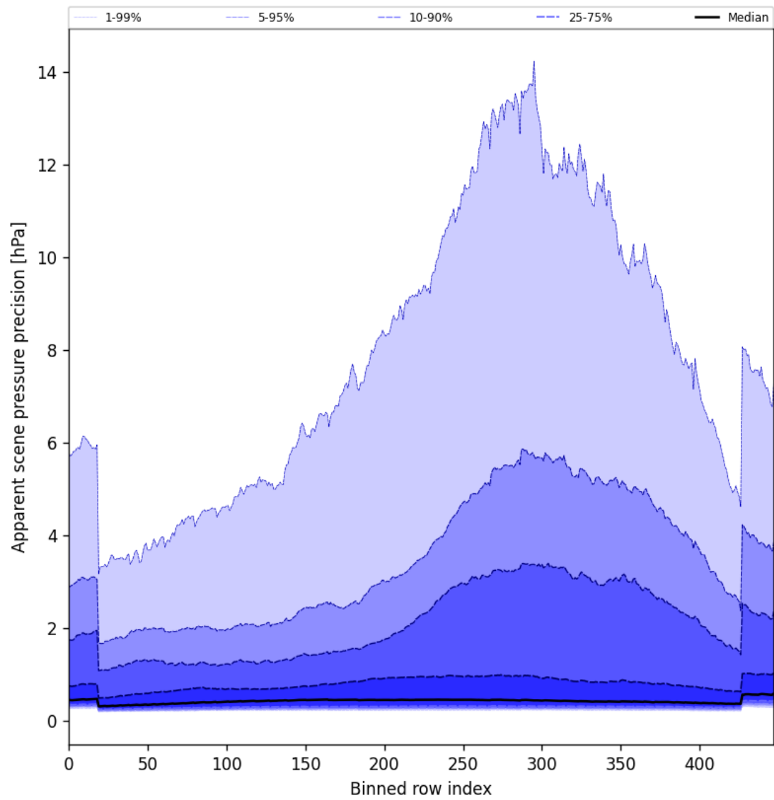
Figure 54: Along track statistics of “Apparent scene pressure precision” for 2024-11-20 to 2024-11-21
