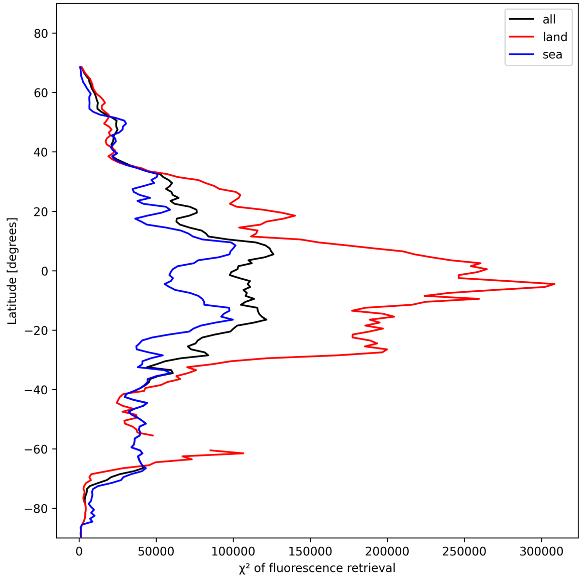
Figure 25: Zonal average of “ \chi^2 of fluorescence retrieval” for 2024-11-20 to 2024-11-21.
