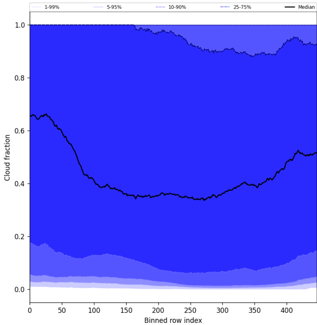
Figure 49: Along track statistics of “Cloud fraction” for 2024-11-20 to 2024-11-21
