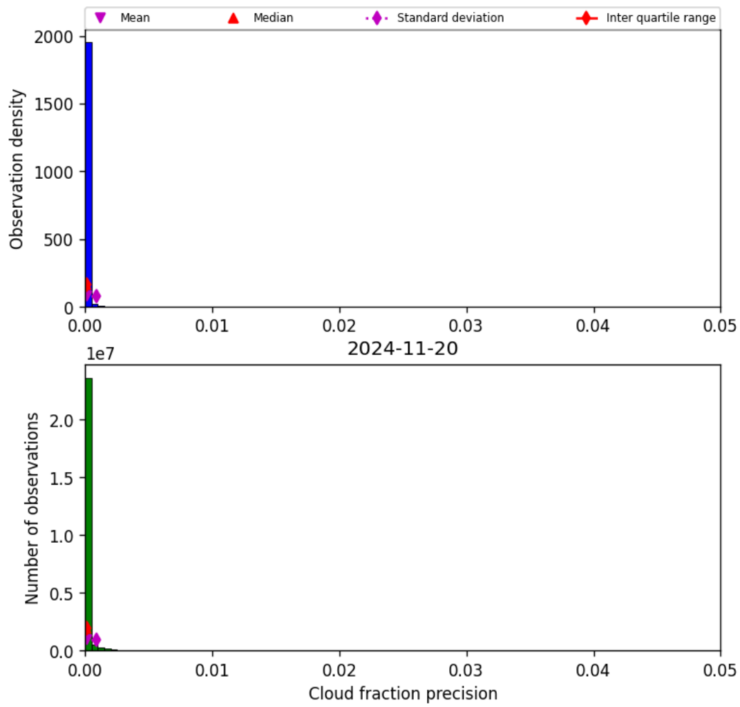
Figure 33: Histogram of “Cloud fraction precision” for 2024-11-20 to 2024-11-21
