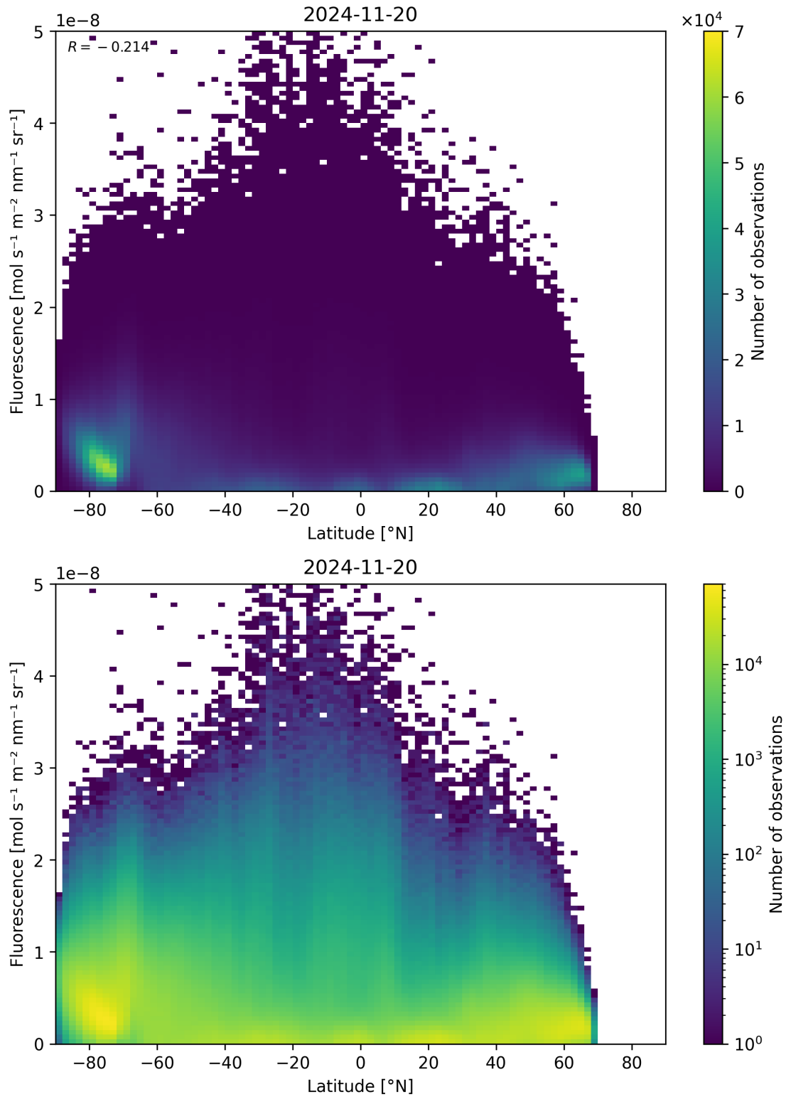
Figure 92: Scatter density plot of “Latitude” against “Fluorescence” for 2024-11-20 to 2024-11-21.
