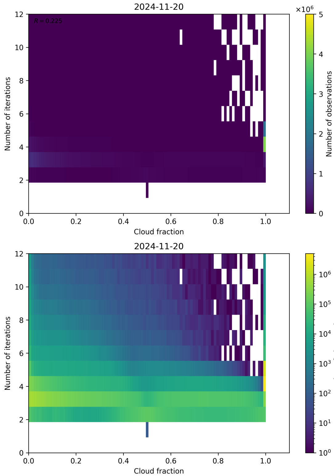
Figure 73: Scatter density plot of “Cloud fraction” against “Number of iterations” for 2024-11-20 to 2024-11-21.
