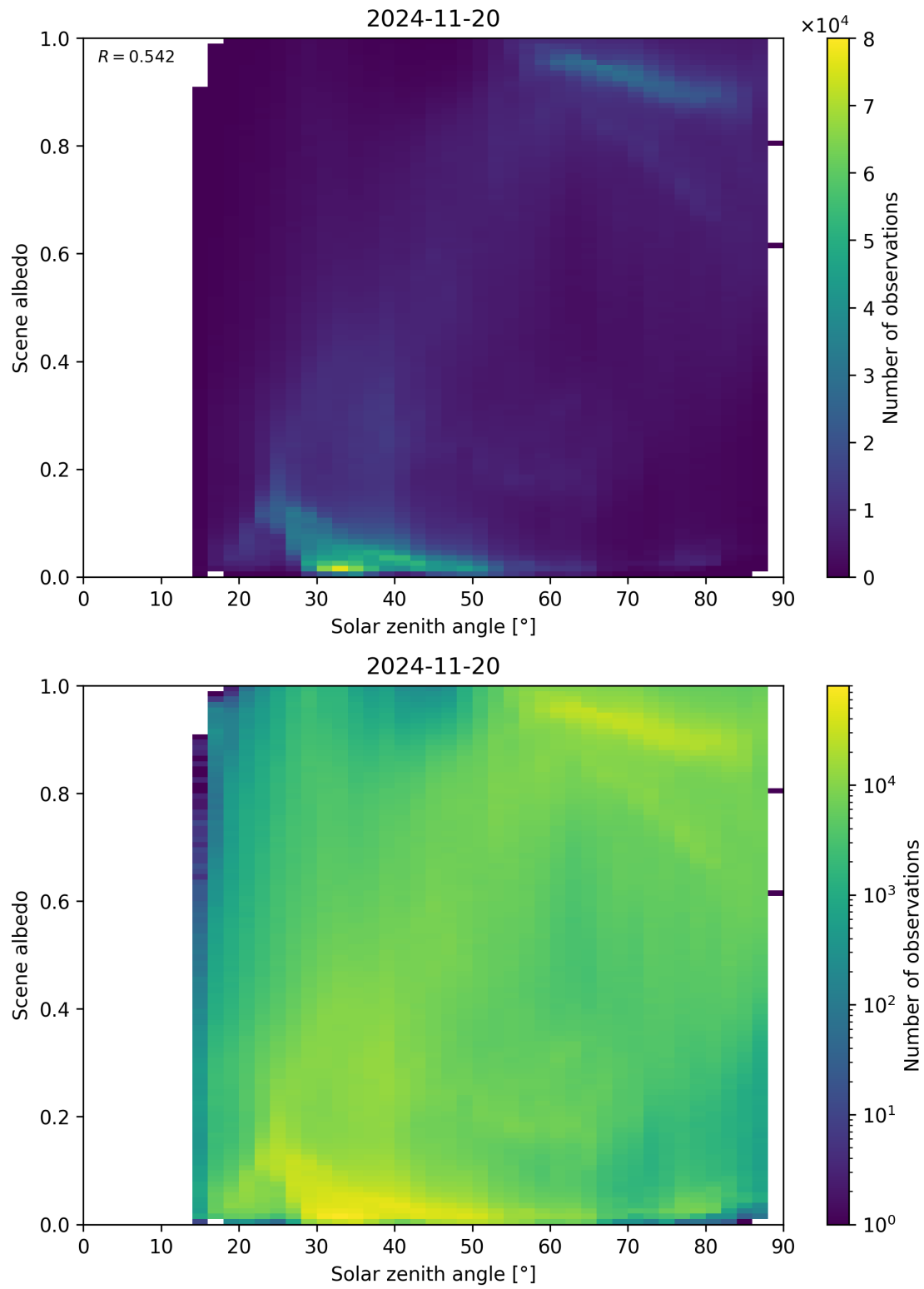
Figure 116: Scatter density plot of “Solar zenith angle” against “Scene albedo” for 2024-11-20 to 2024-11-21.
