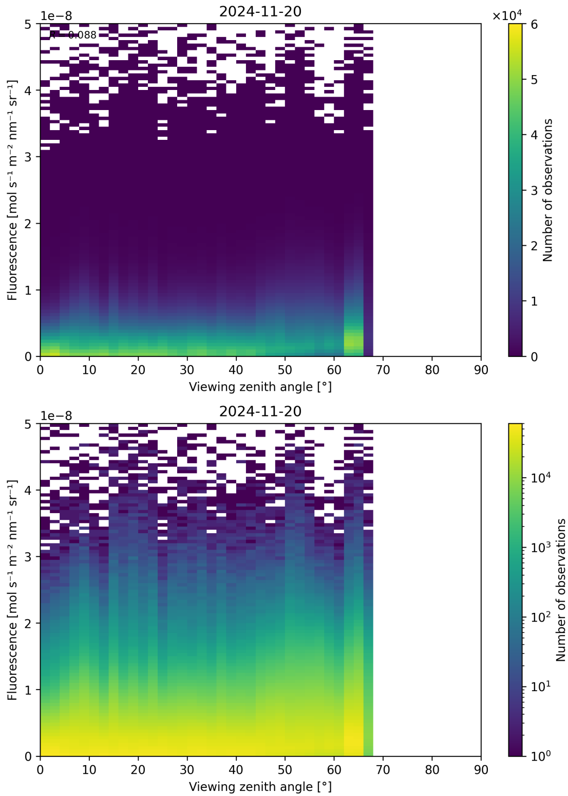
Figure 122: Scatter density plot of “Viewing zenith angle” against “Fluorescence” for 2024-11-20 to 2024-11-21.
