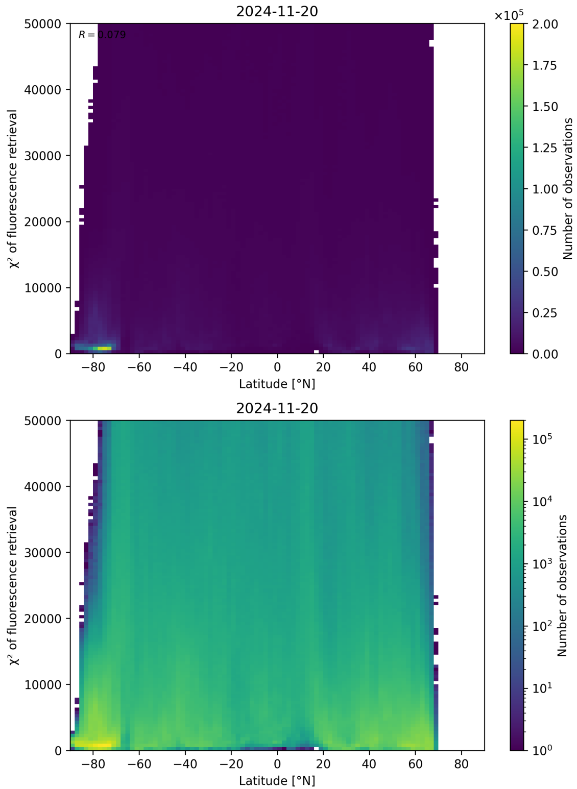
Figure 89: Scatter density plot of “Latitude” against “ \chi^2 of fluorescence retrieval” for 2024-11-20 to 2024-11-21.
