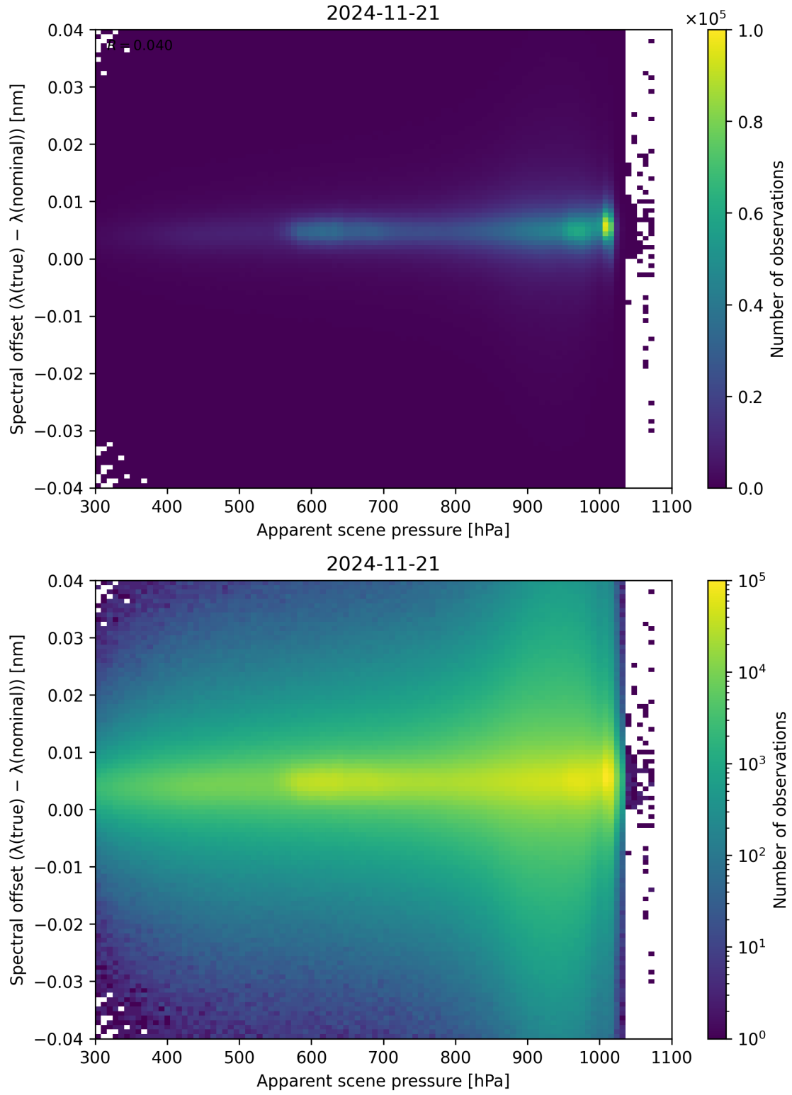
Figure 67: Scatter density plot of “Apparent scene pressure” against “Spectral offset ( \lambda_{\text{true}} - \lambda_{\text{nominal}} )” for 2024-11-20 to 2024-11-22.
