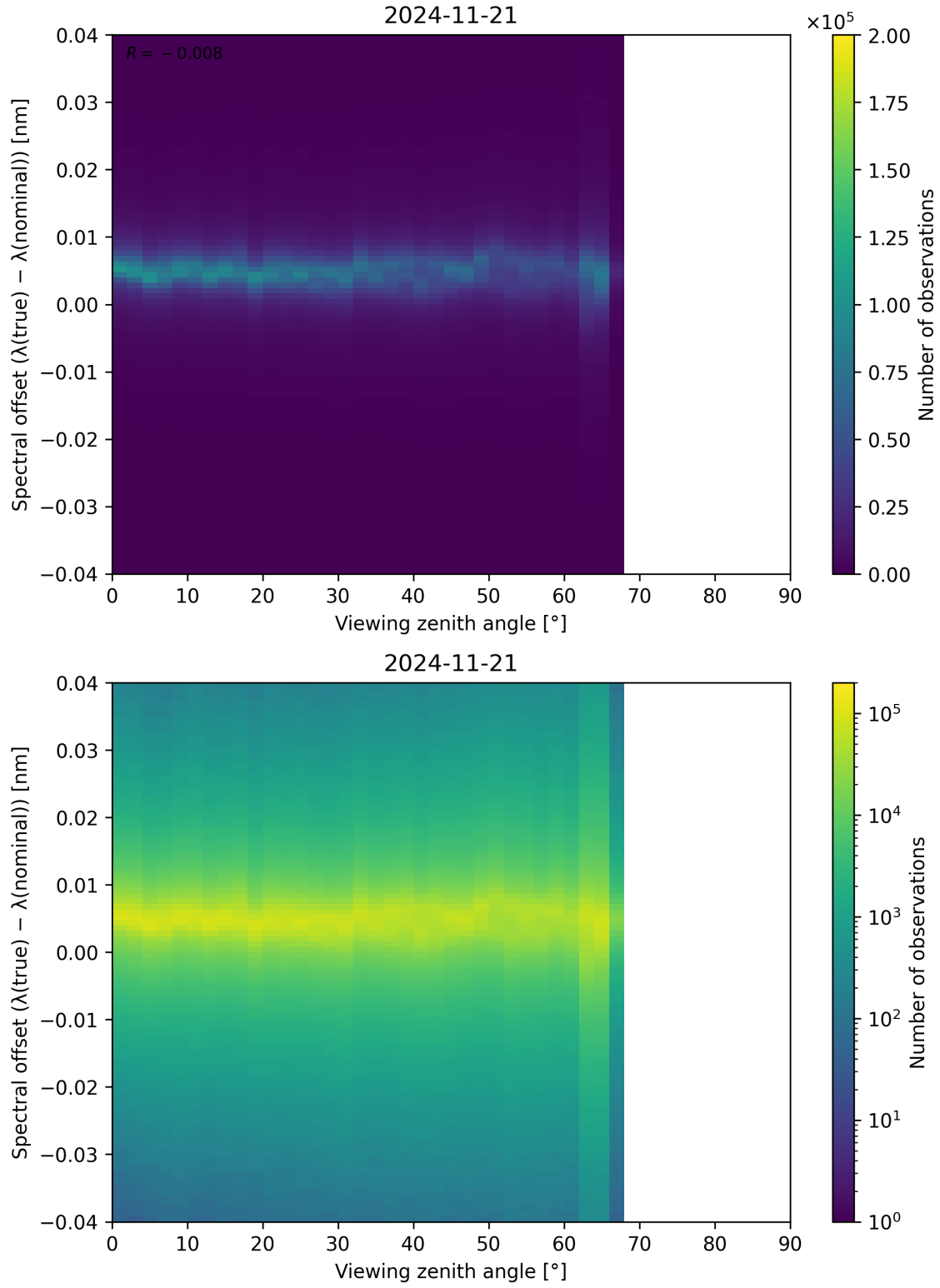
Figure 128: Scatter density plot of “Viewing zenith angle” against “Spectral offset ( \lambda_{\text{true}} - \lambda_{\text{nominal}} )” for 2024-11-20 to 2024-11-22.
