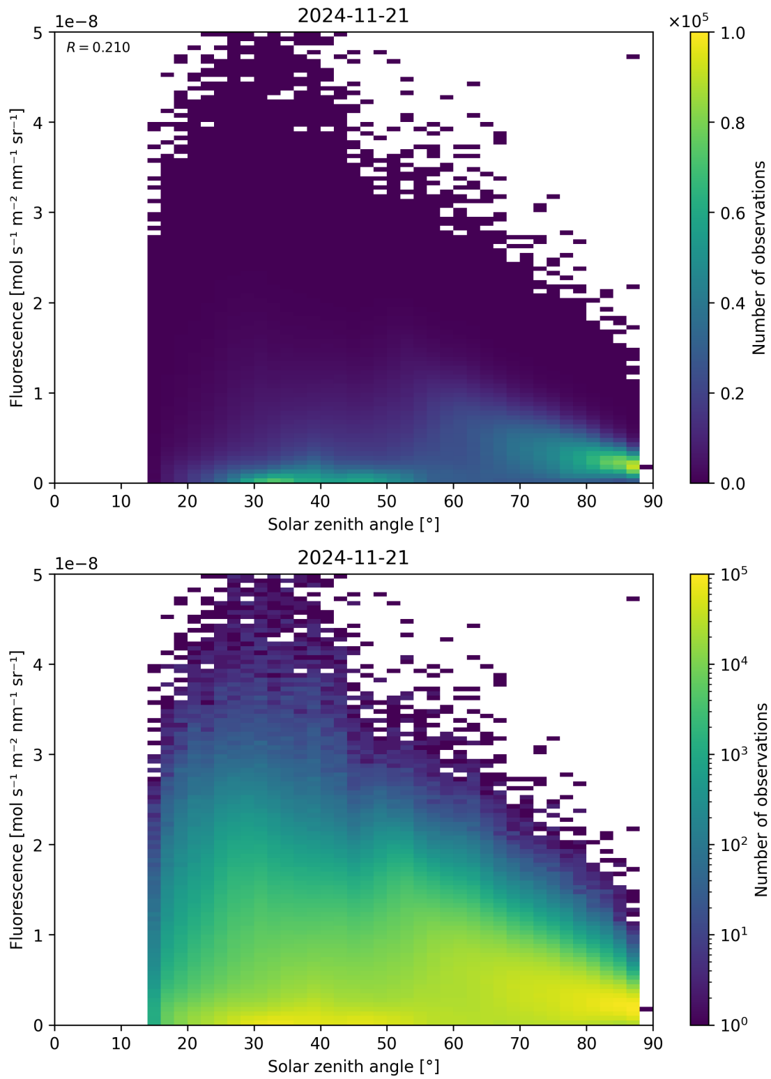
Figure 112: Scatter density plot of “Solar zenith angle” against “Fluorescence” for 2024-11-20 to 2024-11-22.
