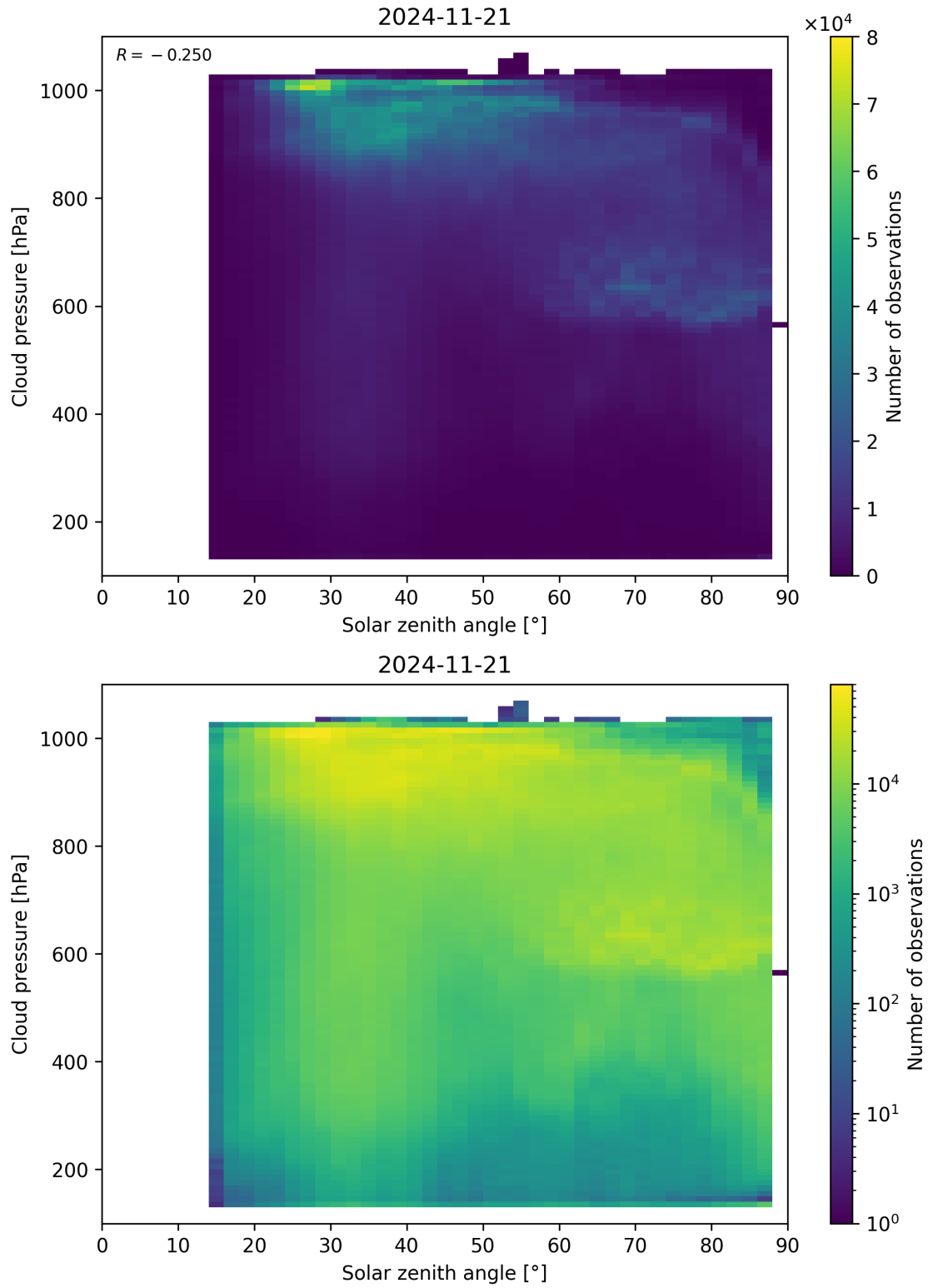
Figure 111: Scatter density plot of “Solar zenith angle” against “Cloud pressure” for 2024-11-20 to 2024-11-22.
