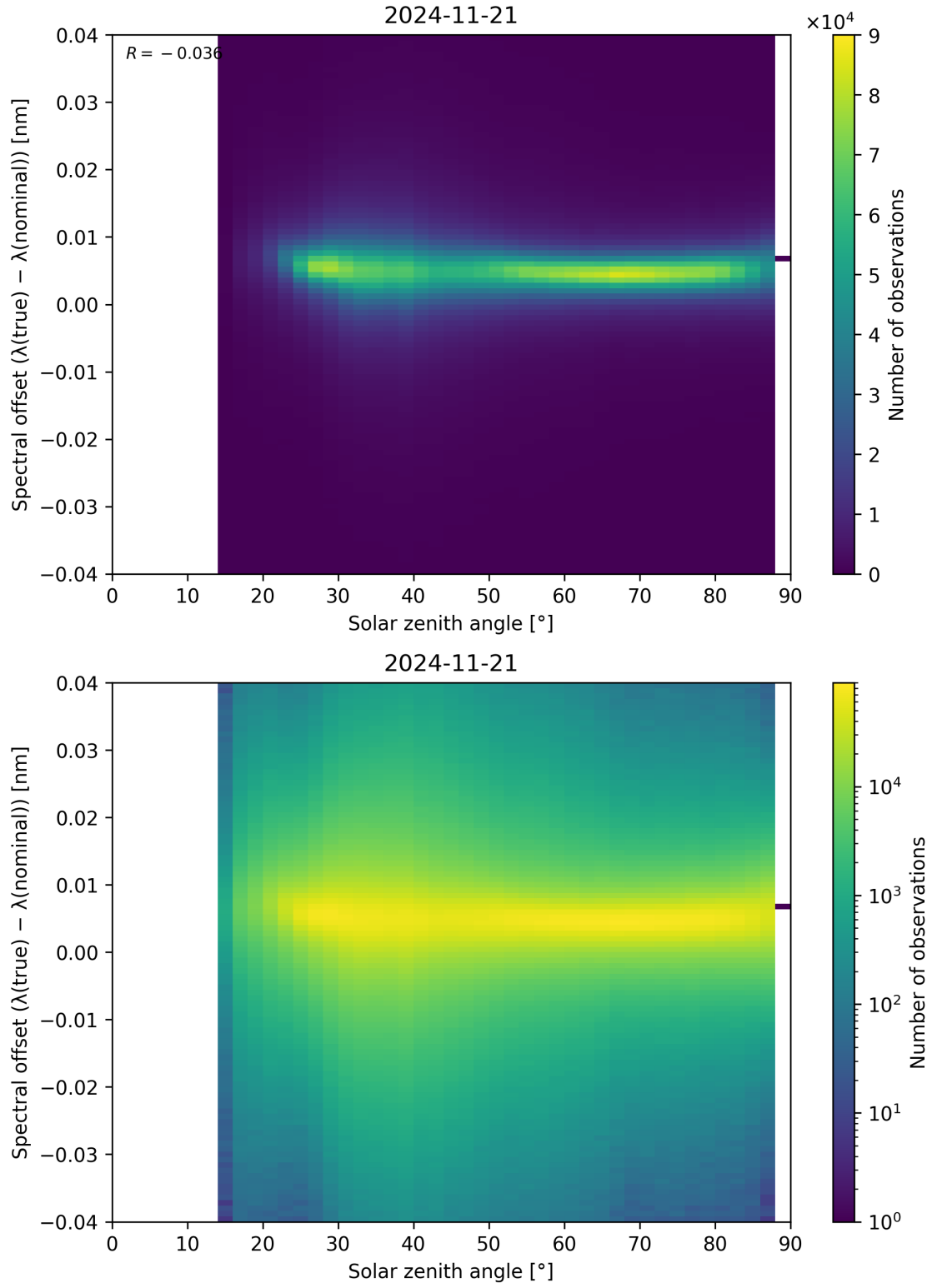
Figure 117: Scatter density plot of “Solar zenith angle” against “Spectral offset ( \lambda_{\text{true}} - \lambda_{\text{nominal}} )” for 2024-11-20 to 2024-11-22.
