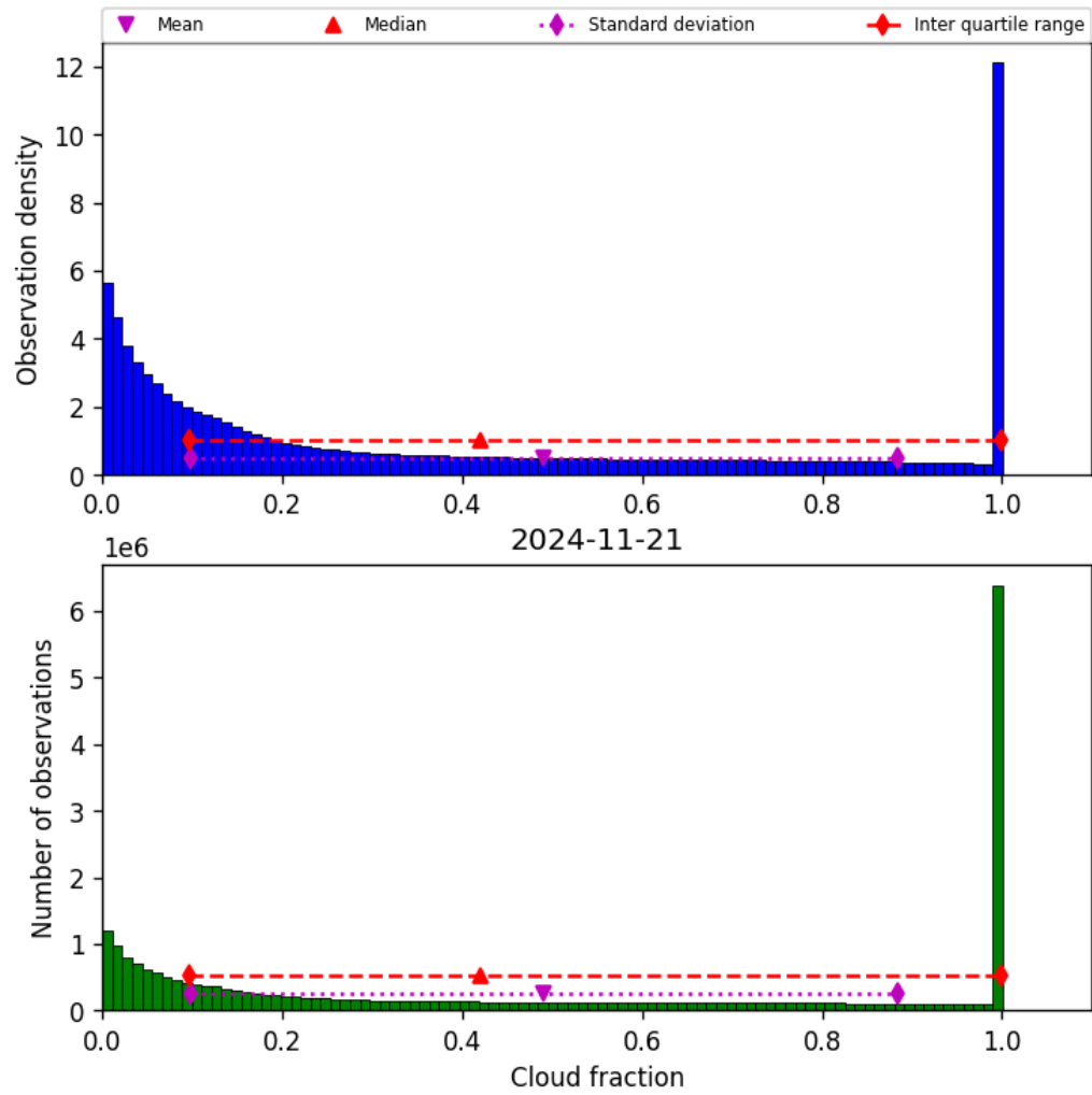
Figure 32: Histogram of “Cloud fraction” for 2024-11-20 to 2024-11-22
