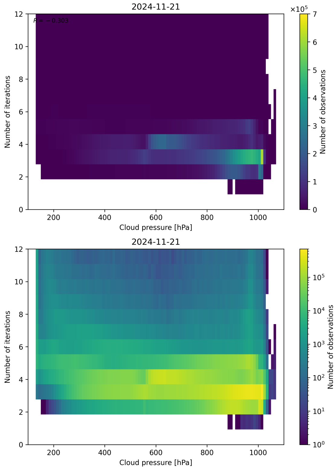
Figure 81: Scatter density plot of “Cloud pressure” against “Number of iterations” for 2024-11-20 to 2024-11-22.
