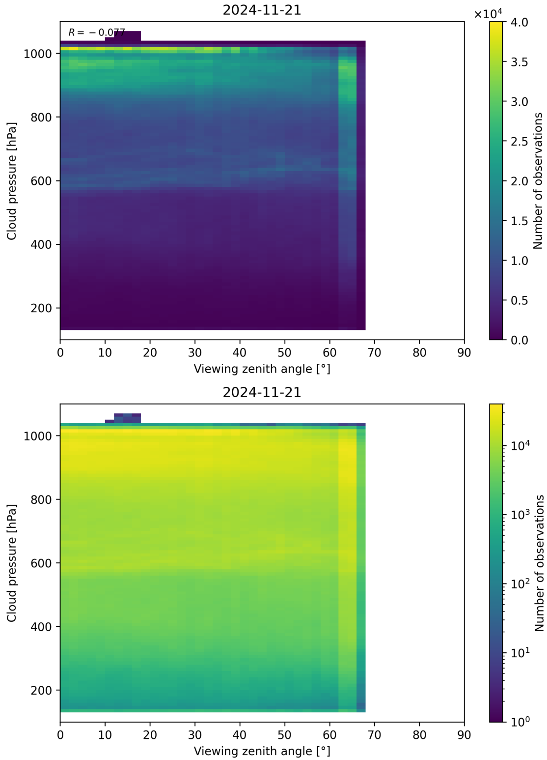
Figure 121: Scatter density plot of “Viewing zenith angle” against “Cloud pressure” for 2024-11-20 to 2024-11-22.
