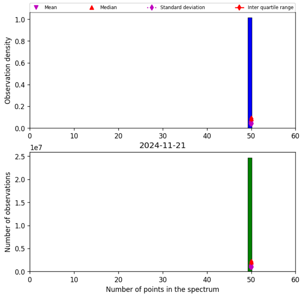
Figure 44: Histogram of “Number of points in the spectrum” for 2024-11-20 to 2024-11-22
