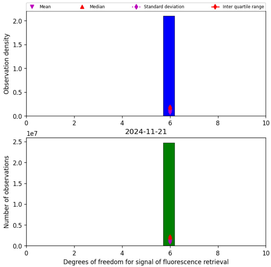
Figure 43: Histogram of “Degrees of freedom for signal of fluorescence retrieval” for 2024-11-20 to 2024-11-22
