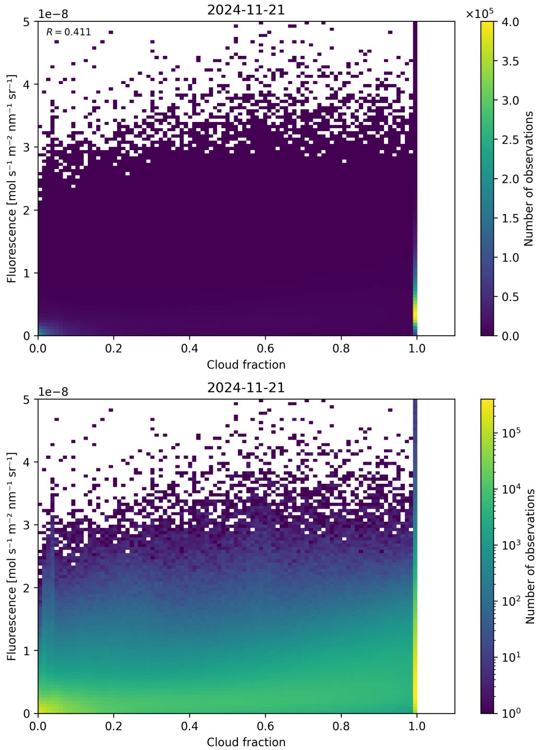
Figure 72: Scatter density plot of “Cloud fraction” against “Fluorescence” for 2024-11-20 to 2024-11-22.
