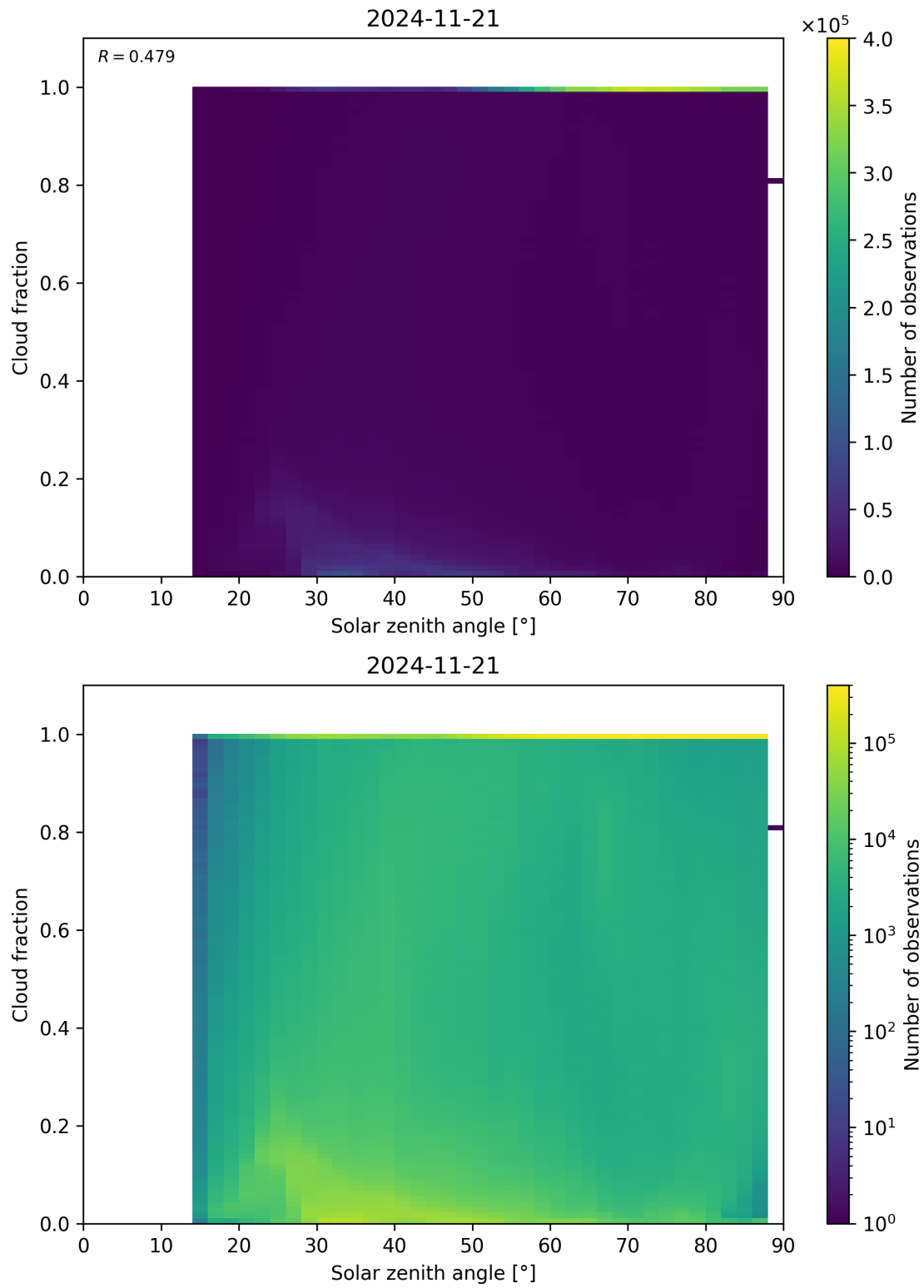
Figure 110: Scatter density plot of “Solar zenith angle” against “Cloud fraction” for 2024-11-20 to 2024-11-22.
