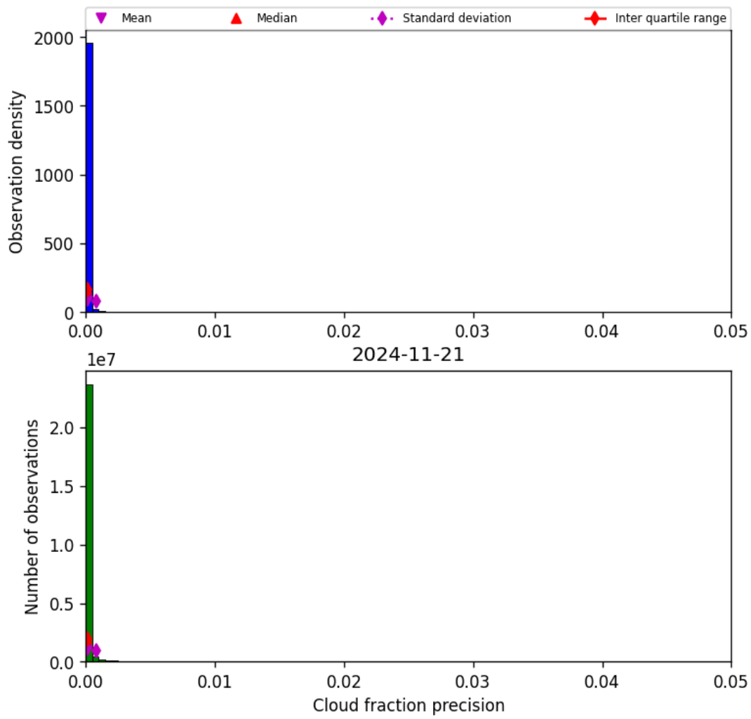
Figure 33: Histogram of “Cloud fraction precision” for 2024-11-20 to 2024-11-22
