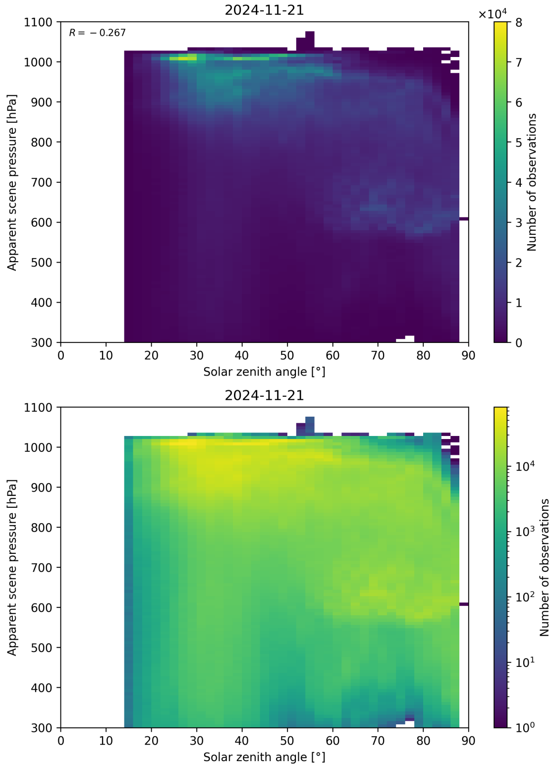
Figure 108: Scatter density plot of “Solar zenith angle” against “Apparent scene pressure” for 2024-11-20 to 2024-11-22.
