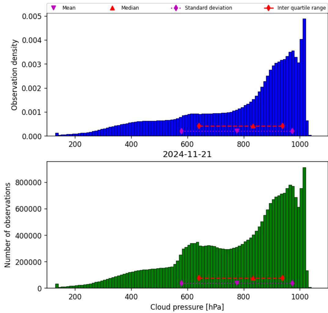
Figure 30: Histogram of “Cloud pressure” for 2024-11-20 to 2024-11-22
