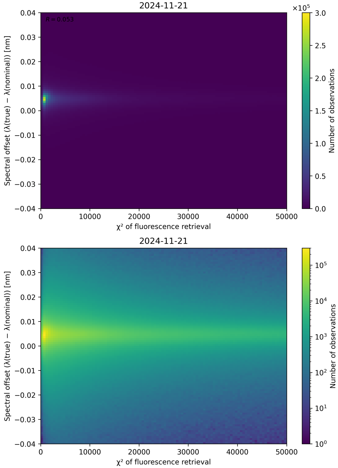
Figure 69: Scatter density plot of “ \chi^2 of fluorescence retrieval” against “Spectral offset ( \lambda_{\text{true}} - \lambda_{\text{nominal}} )” for 2024-11-20 to 2024-11-22.
