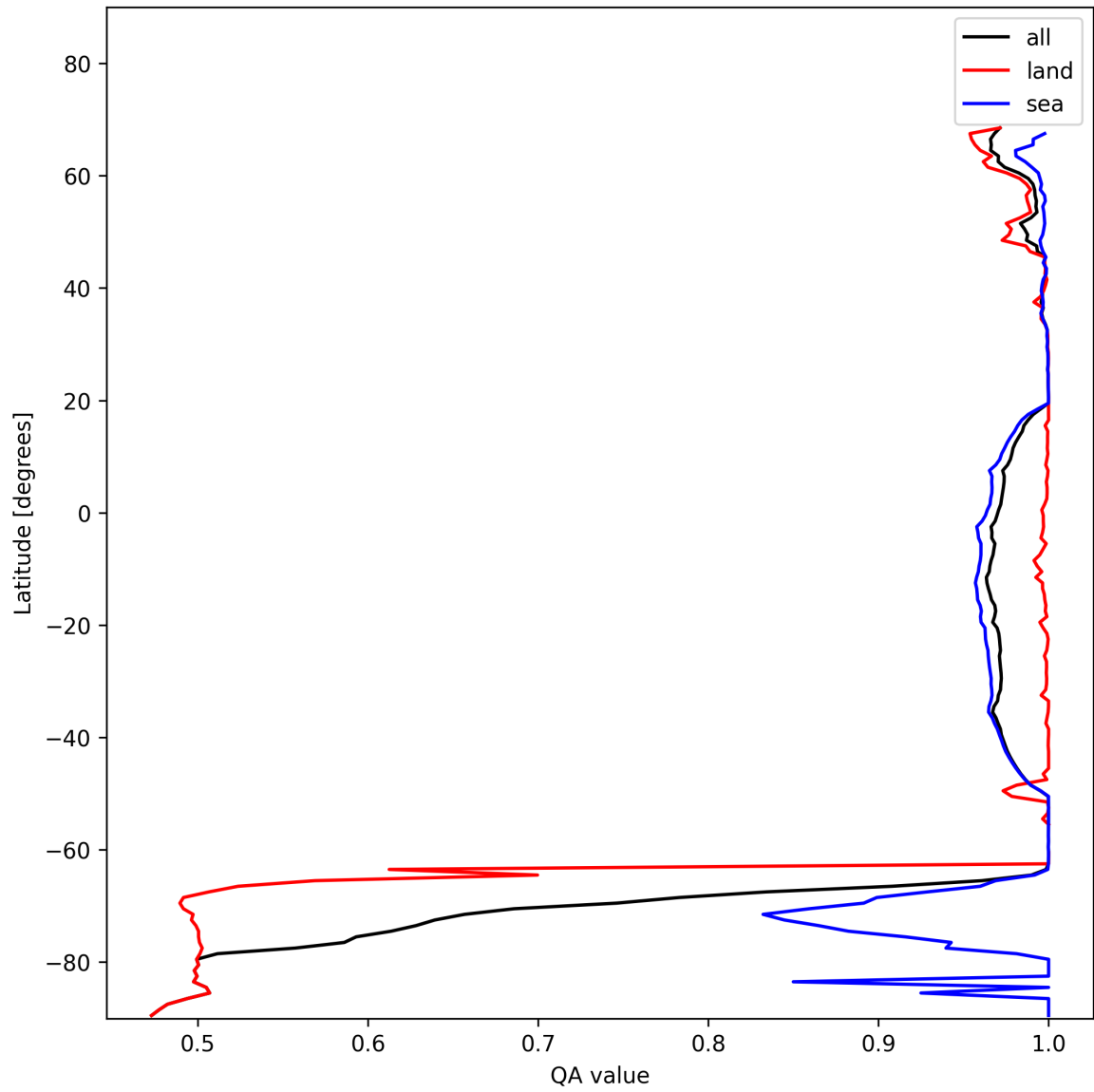
Figure 12: Zonal average of “QA value” for 2024-11-20 to 2024-11-22.
