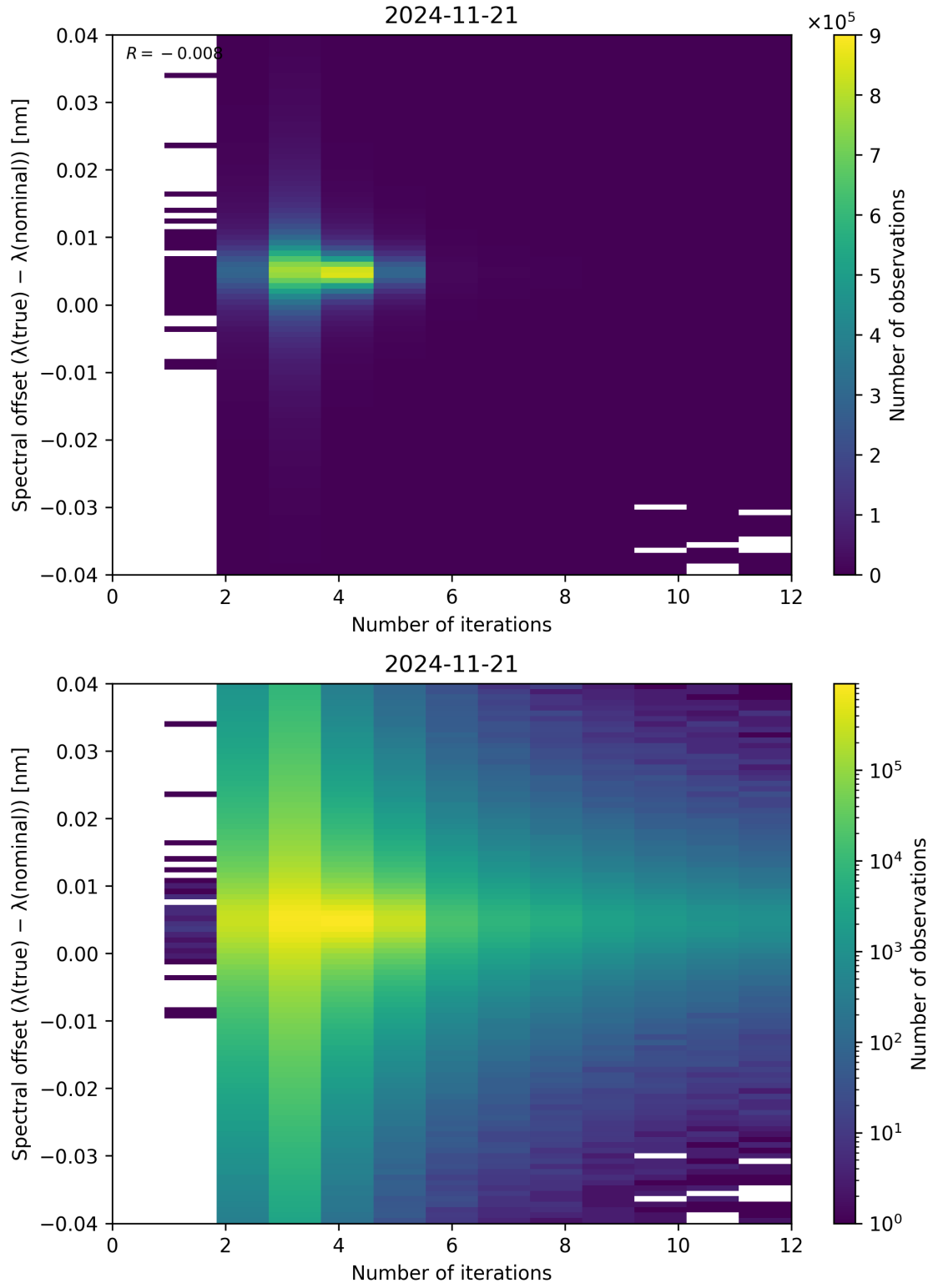
Figure 100: Scatter density plot of “Number of iterations” against “Spectral offset ( \lambda_{\text{true}} - \lambda_{\text{nominal}} )” for 2024-11-20 to 2024-11-22.
