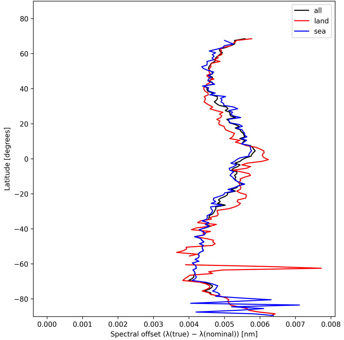
Figure 28: Zonal average of “Spectral offset ( \lambda_{\text{true}} - \lambda_{\text{nominal}} )” for 2024-11-20 to 2024-11-22.
