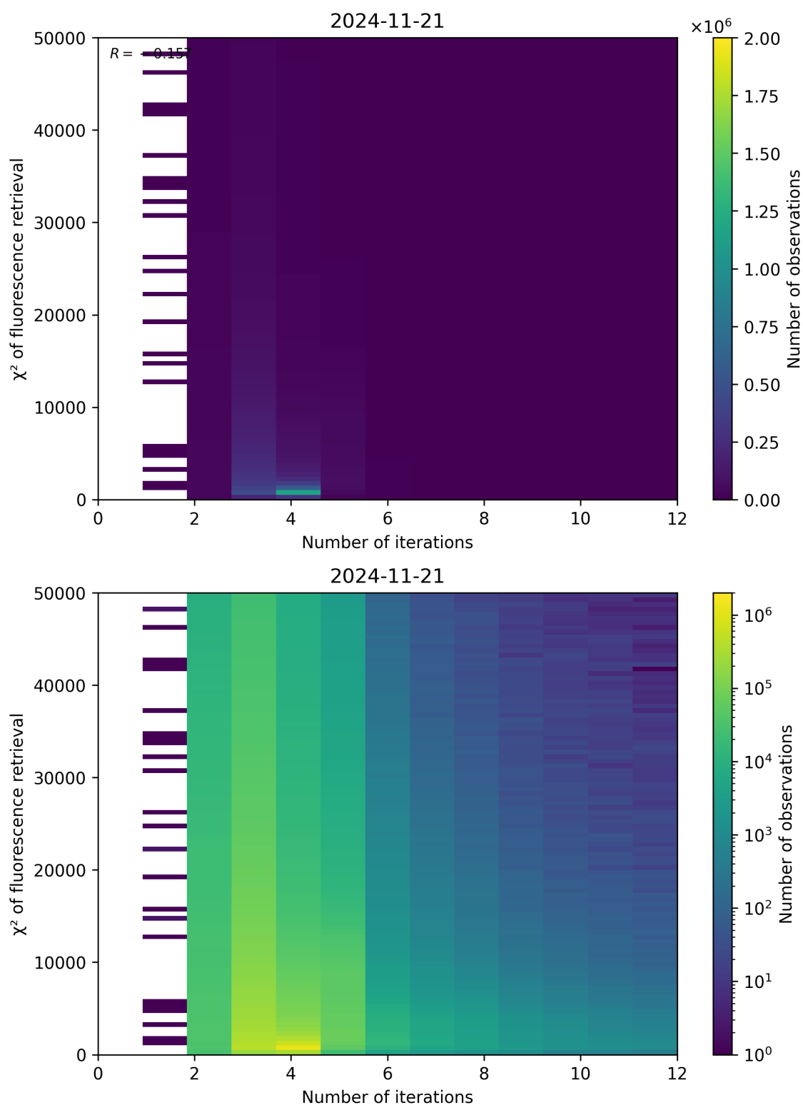
Figure 97: Scatter density plot of “Number of iterations” against “ \chi^2 of fluorescence retrieval” for 2024-11-20 to 2024-11-22.
