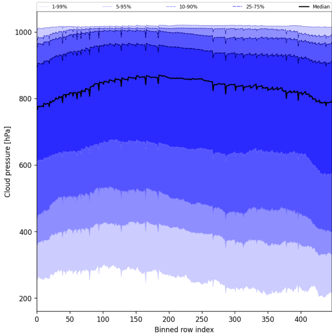
Figure 47: Along track statistics of “Cloud pressure” for 2024-11-20 to 2024-11-22
