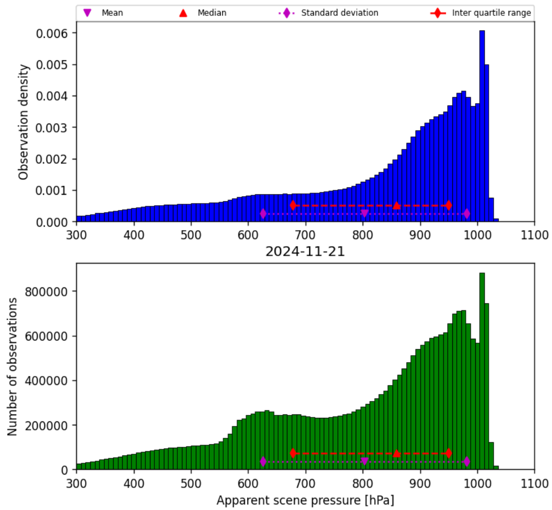
Figure 36: Histogram of “Apparent scene pressure” for 2024-11-20 to 2024-11-22
