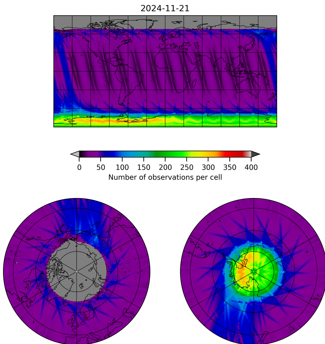
Figure 11: Map of the number of observations for 2024-11-20 to 2024-11-22
