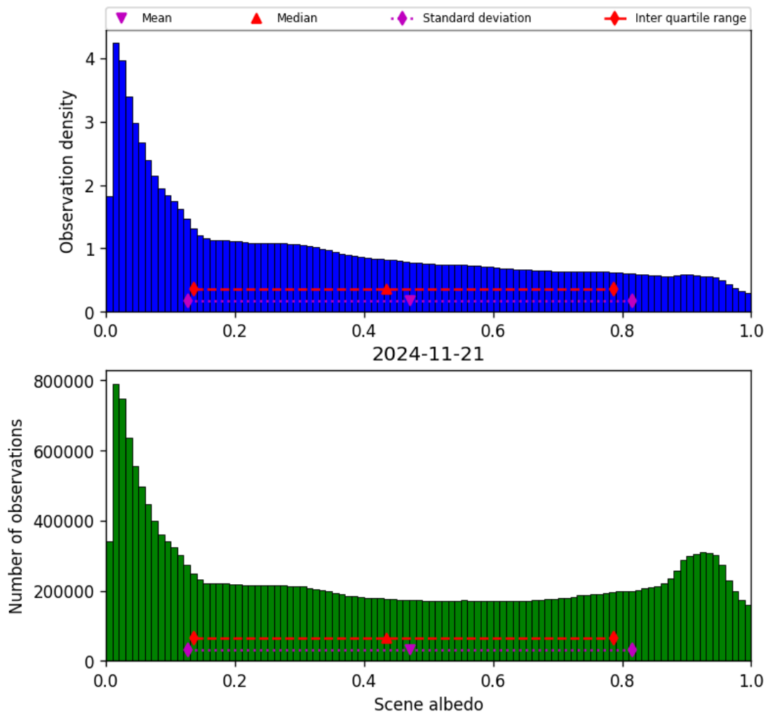
Figure 34: Histogram of “Scene albedo” for 2024-11-20 to 2024-11-22
