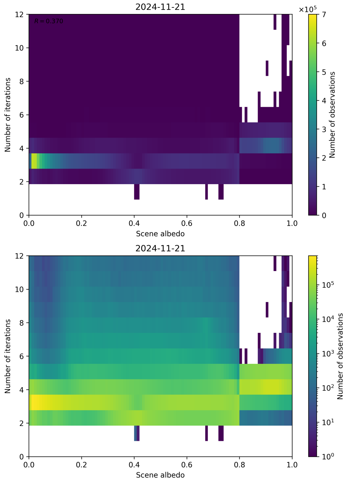
Figure 105: Scatter density plot of “Scene albedo” against “Number of iterations” for 2024-11-20 to 2024-11-22.
