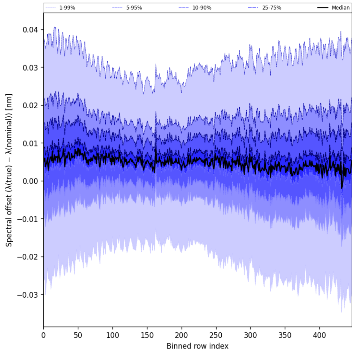
Figure 62: Along track statistics of “Spectral offset ( \lambda_{\text{true}} - \lambda_{\text{nominal}} )” for 2024-11-20 to 2024-11-22
