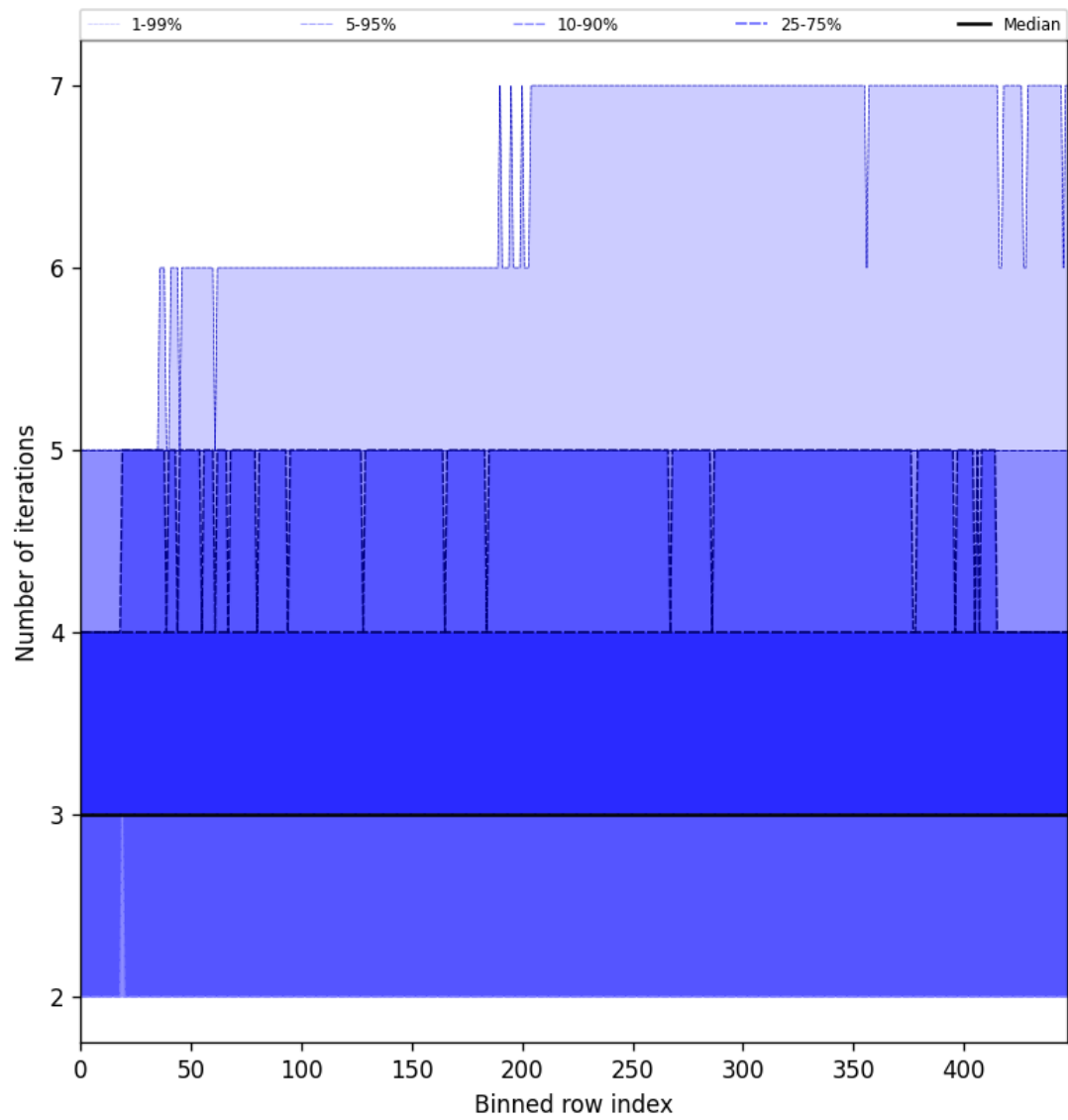
Figure 56: Along track statistics of “Number of iterations” for 2024-11-20 to 2024-11-22
