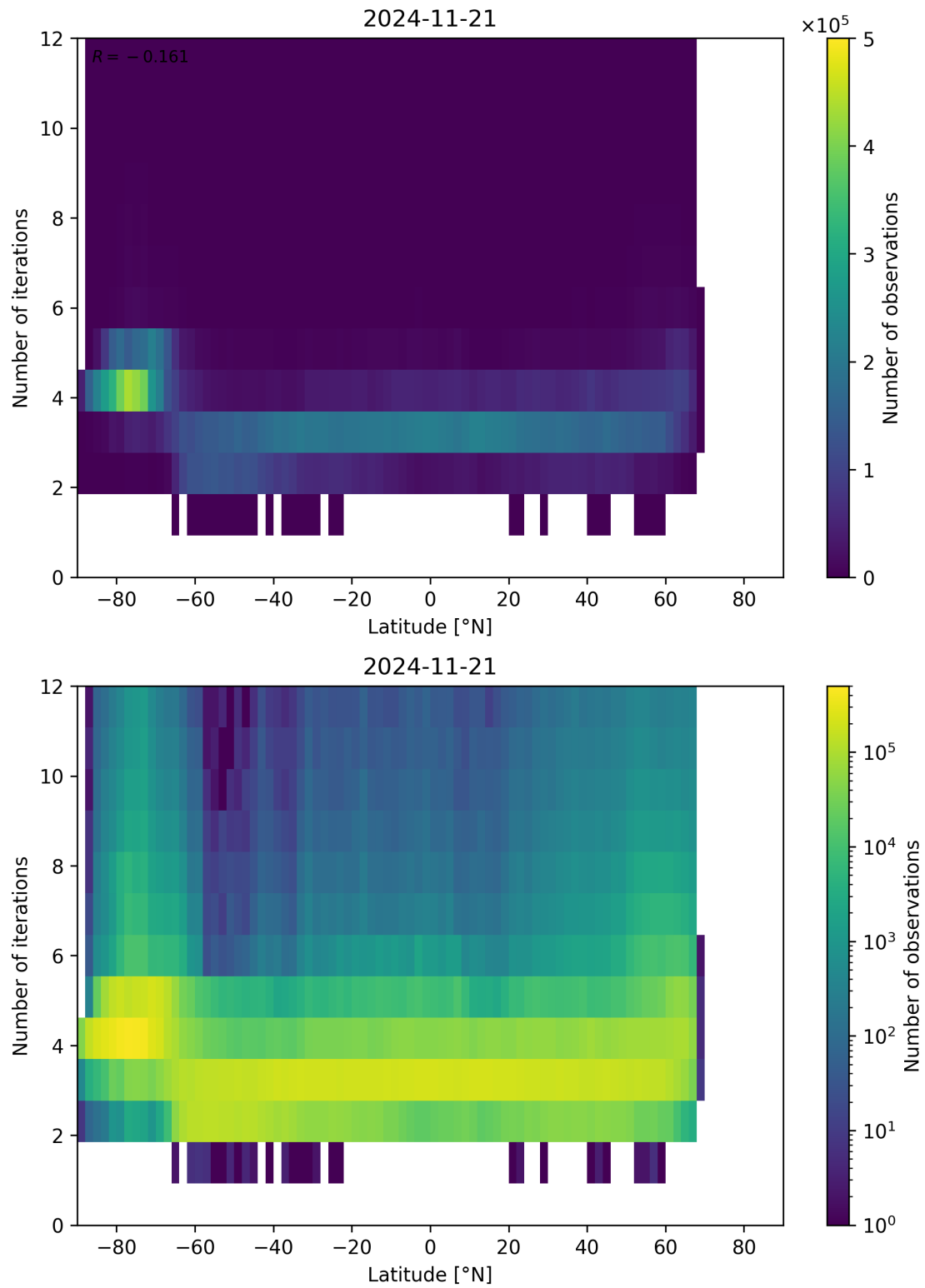
Figure 93: Scatter density plot of “Latitude” against “Number of iterations” for 2024-11-20 to 2024-11-22.
