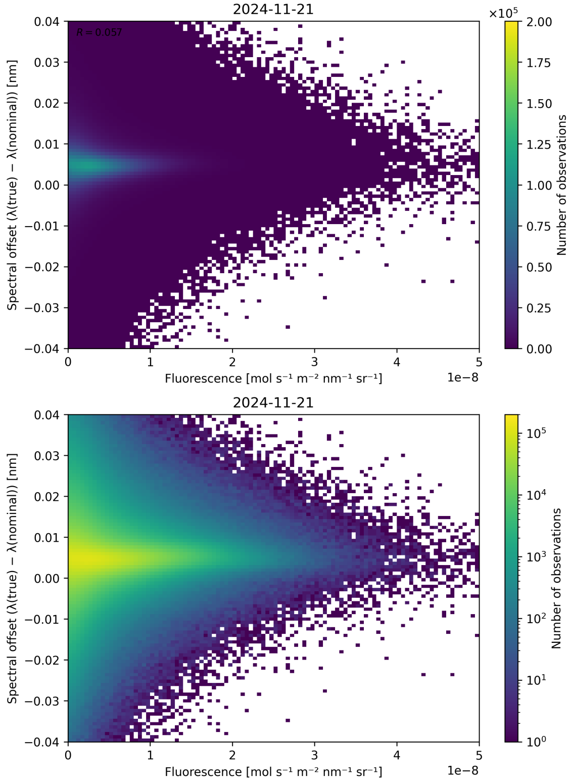
Figure 87: Scatter density plot of “Fluorescence” against “Spectral offset ( \lambda_{\text{true}} - \lambda_{\text{nominal}} )” for 2024-11-20 to 2024-11-22.
