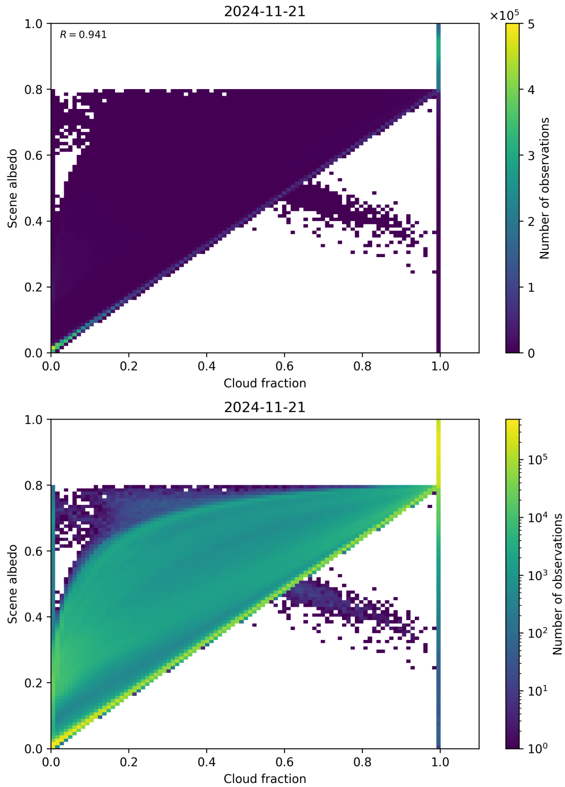
Figure 75: Scatter density plot of “Cloud fraction” against “Scene albedo” for 2024-11-20 to 2024-11-22.
