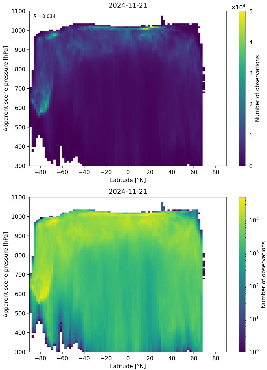
Figure 88: Scatter density plot of “Latitude” against “Apparent scene pressure” for 2024-11-20 to 2024-11-22.
