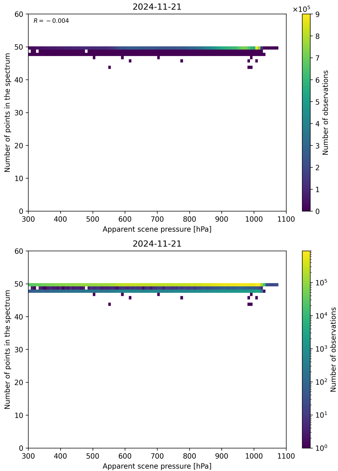
Figure 66: Scatter density plot of “Apparent scene pressure” against “Number of points in the spectrum” for 2024-11-20 to 2024-11-22.
