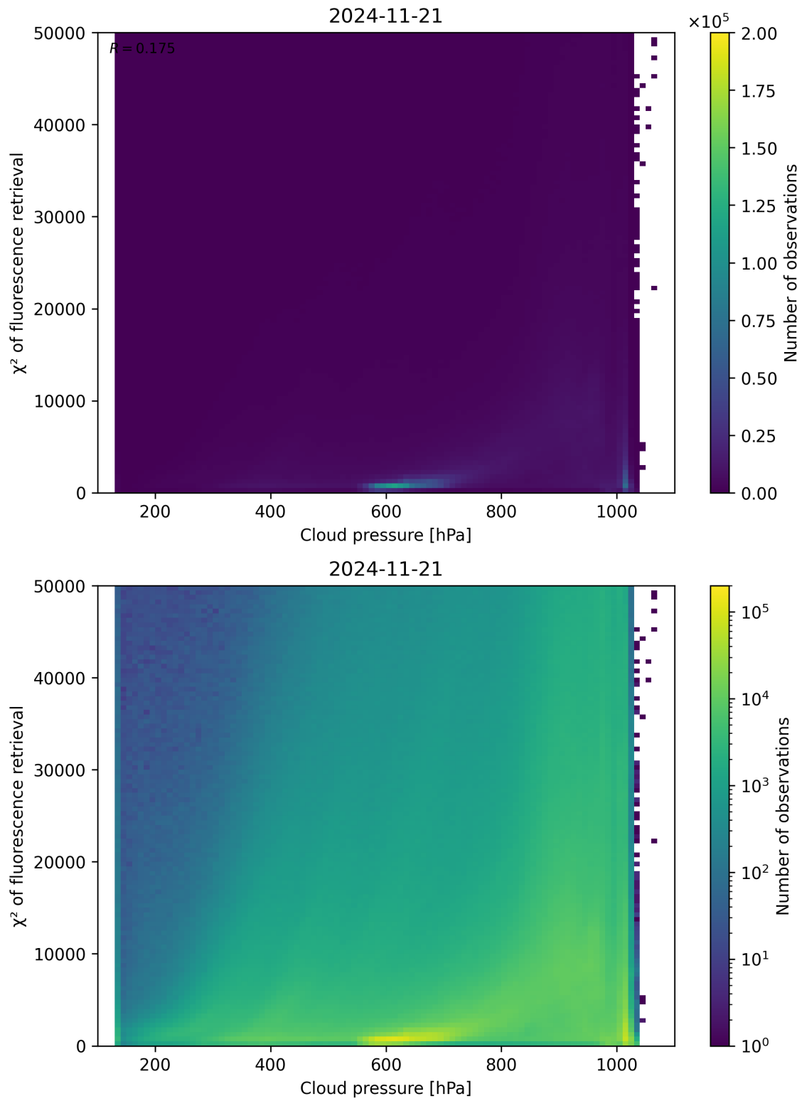
Figure 78: Scatter density plot of “Cloud pressure” against “ \chi^2 of fluorescence retrieval” for 2024-11-20 to 2024-11-22.
