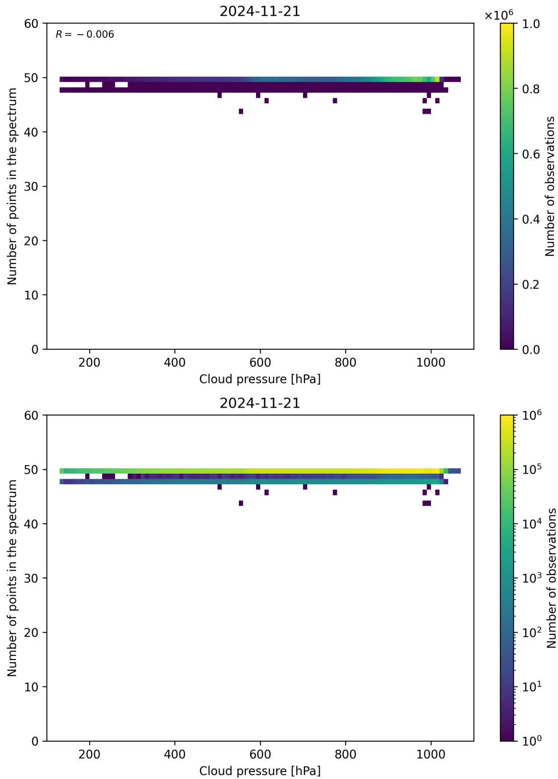
Figure 82: Scatter density plot of “Cloud pressure” against “Number of points in the spectrum” for 2024-11-20 to 2024-11-22.
