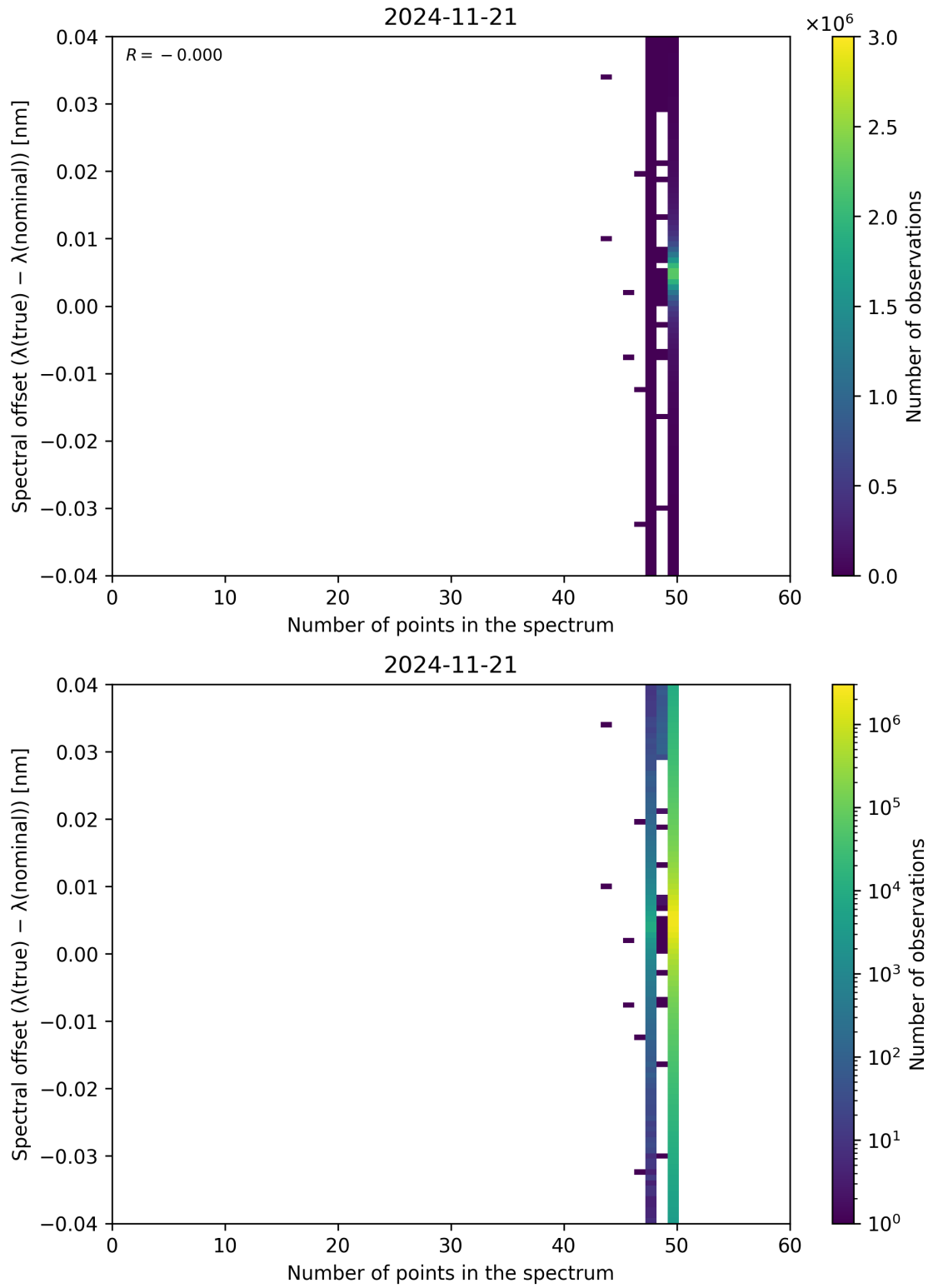
Figure 101: Scatter density plot of “Number of points in the spectrum” against “Spectral offset ( \lambda_{\text{true}} - \lambda_{\text{nominal}} )” for 2024-11-20 to 2024-11-22.
