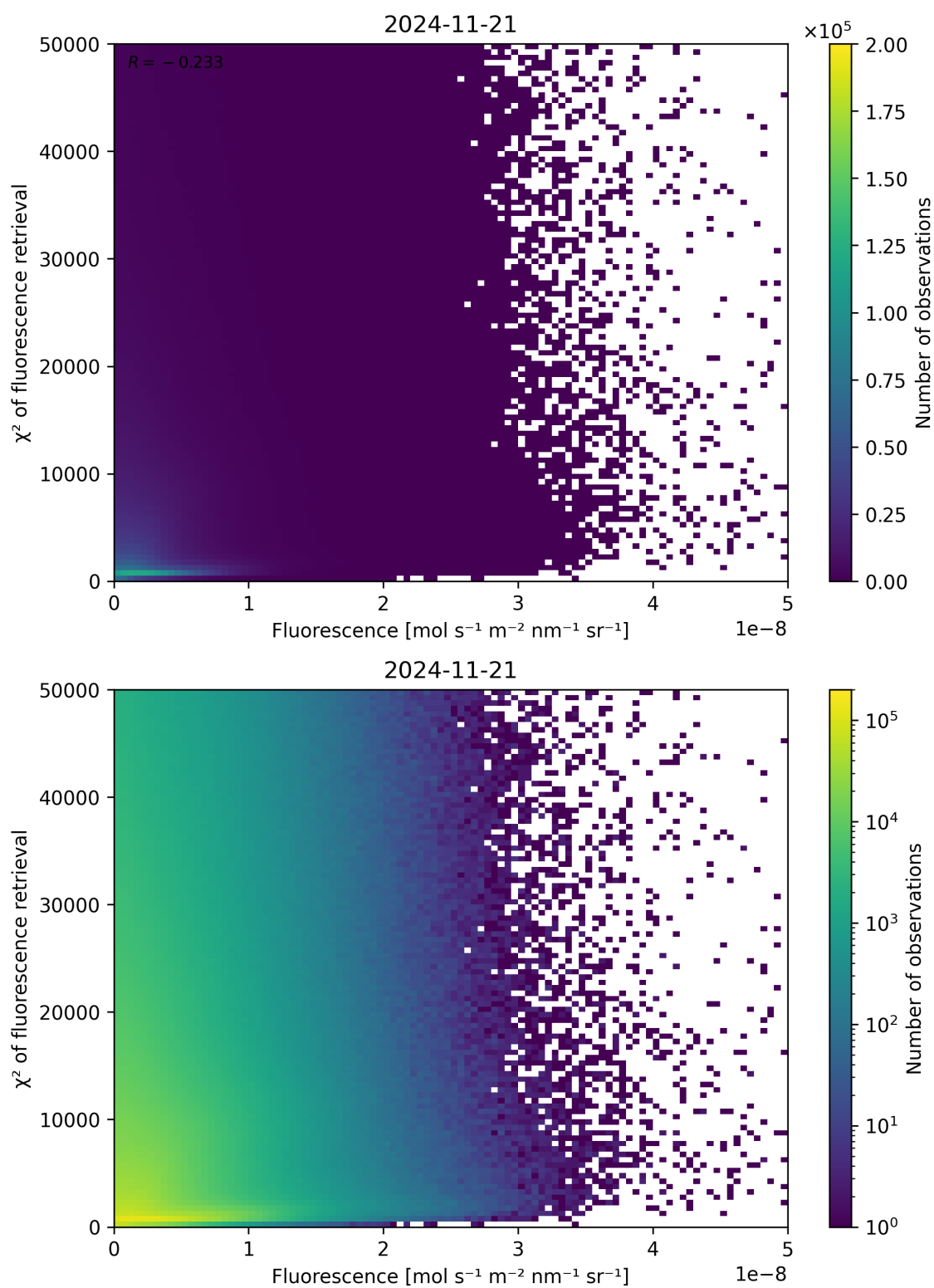
Figure 85: Scatter density plot of “Fluorescence” against “ \chi^2 of fluorescence retrieval” for 2024-11-20 to 2024-11-22.
