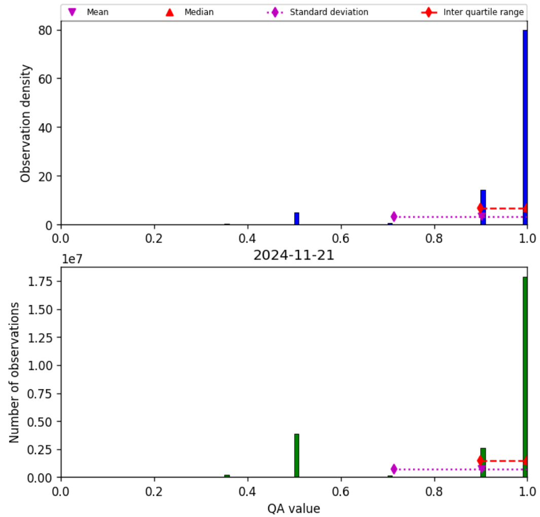
Figure 29: Histogram of “QA value” for 2024-11-20 to 2024-11-22
