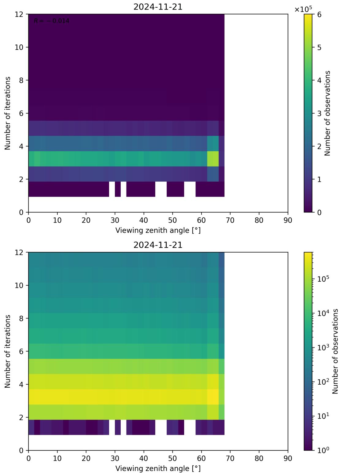
Figure 124: Scatter density plot of “Viewing zenith angle” against “Number of iterations” for 2024-11-20 to 2024-11-22.
