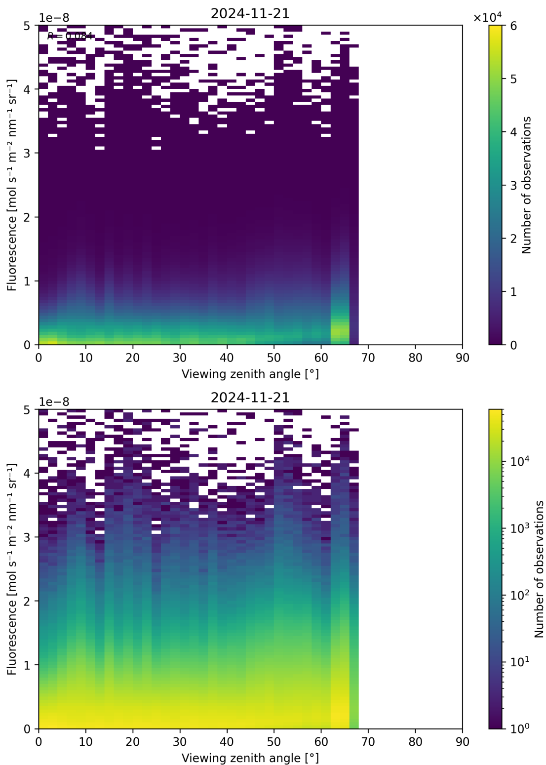
Figure 122: Scatter density plot of “Viewing zenith angle” against “Fluorescence” for 2024-11-20 to 2024-11-22.
