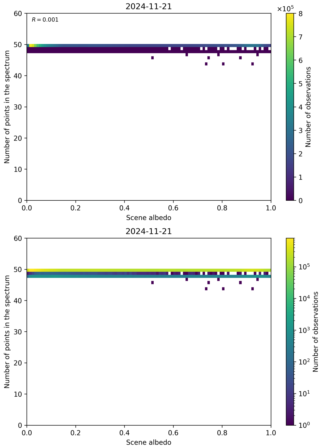
Figure 106: Scatter density plot of “Scene albedo” against “Number of points in the spectrum” for 2024-11-20 to 2024-11-22.
