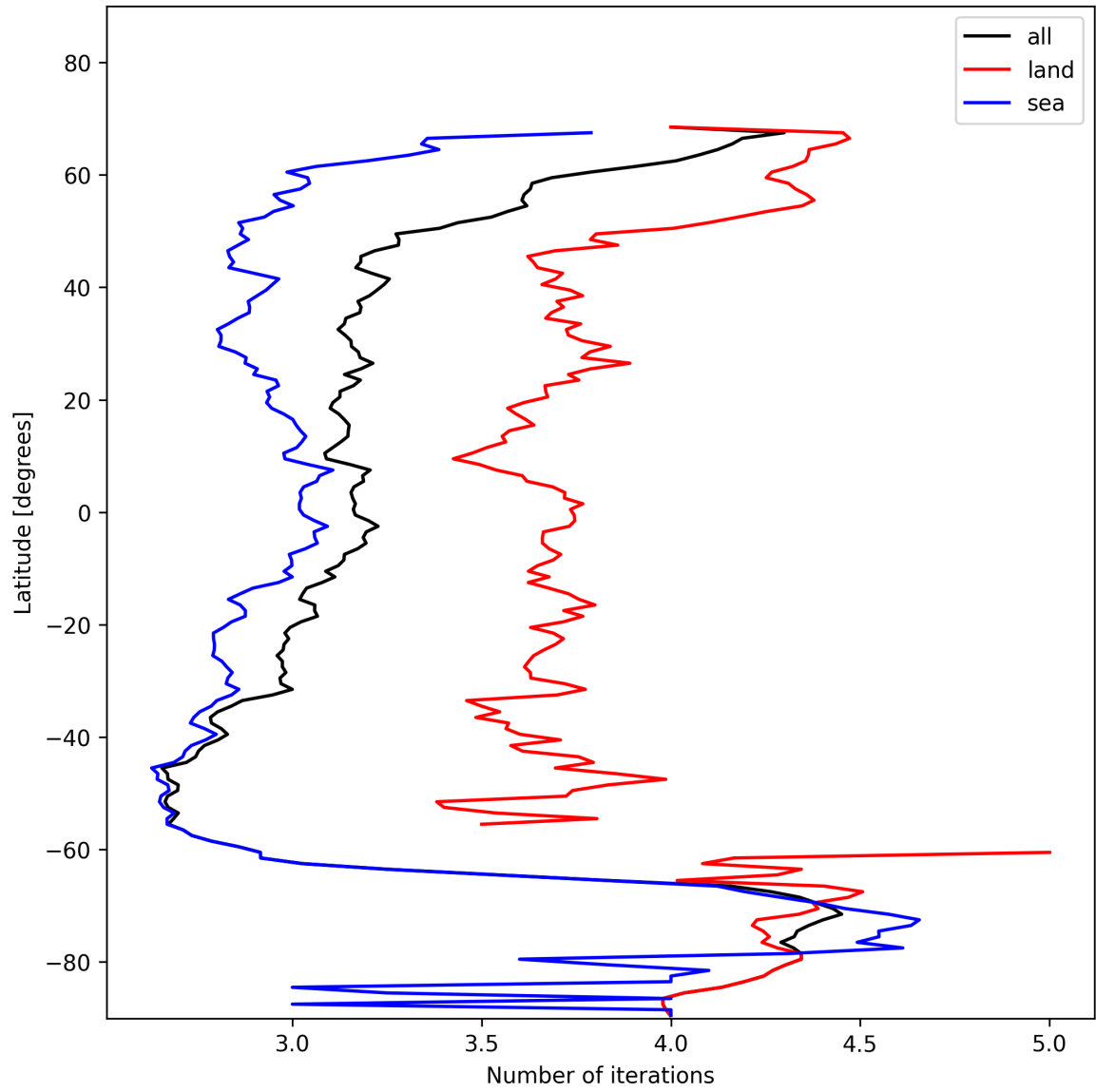
Figure 22: Zonal average of “Number of iterations” for 2024-11-20 to 2024-11-22.
