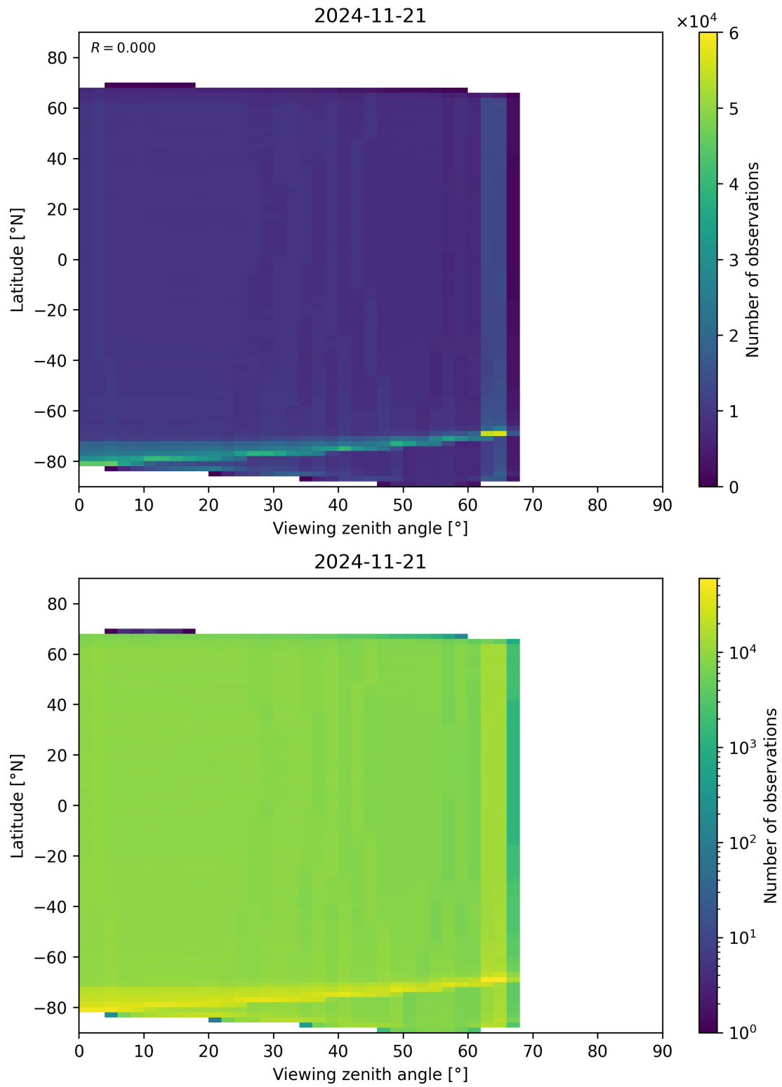
Figure 123: Scatter density plot of “Viewing zenith angle” against “Latitude” for 2024-11-20 to 2024-11-22.
