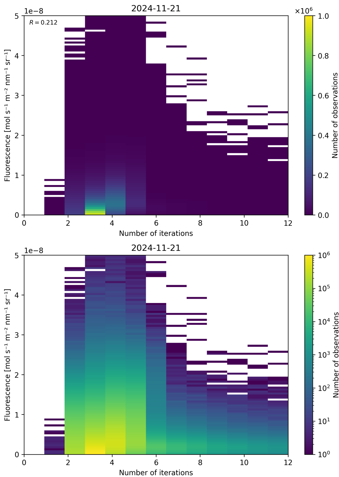
Figure 98: Scatter density plot of “Number of iterations” against “Fluorescence” for 2024-11-20 to 2024-11-22.
