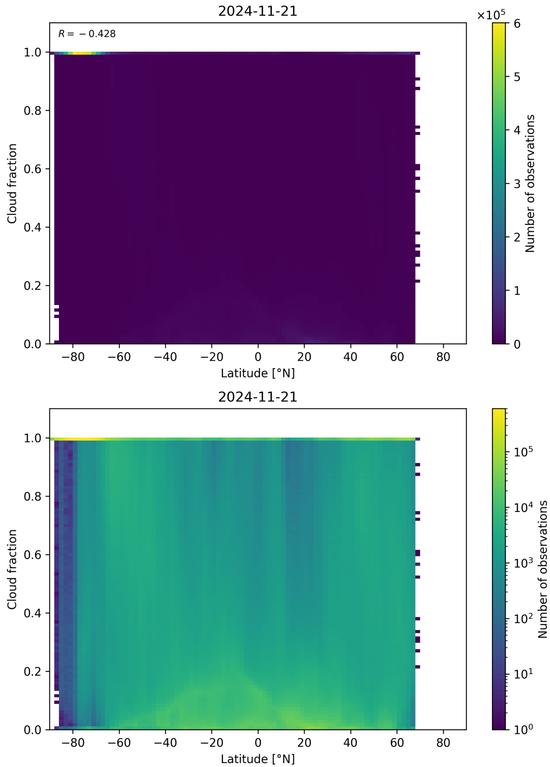
Figure 90: Scatter density plot of “Latitude” against “Cloud fraction” for 2024-11-20 to 2024-11-22.
