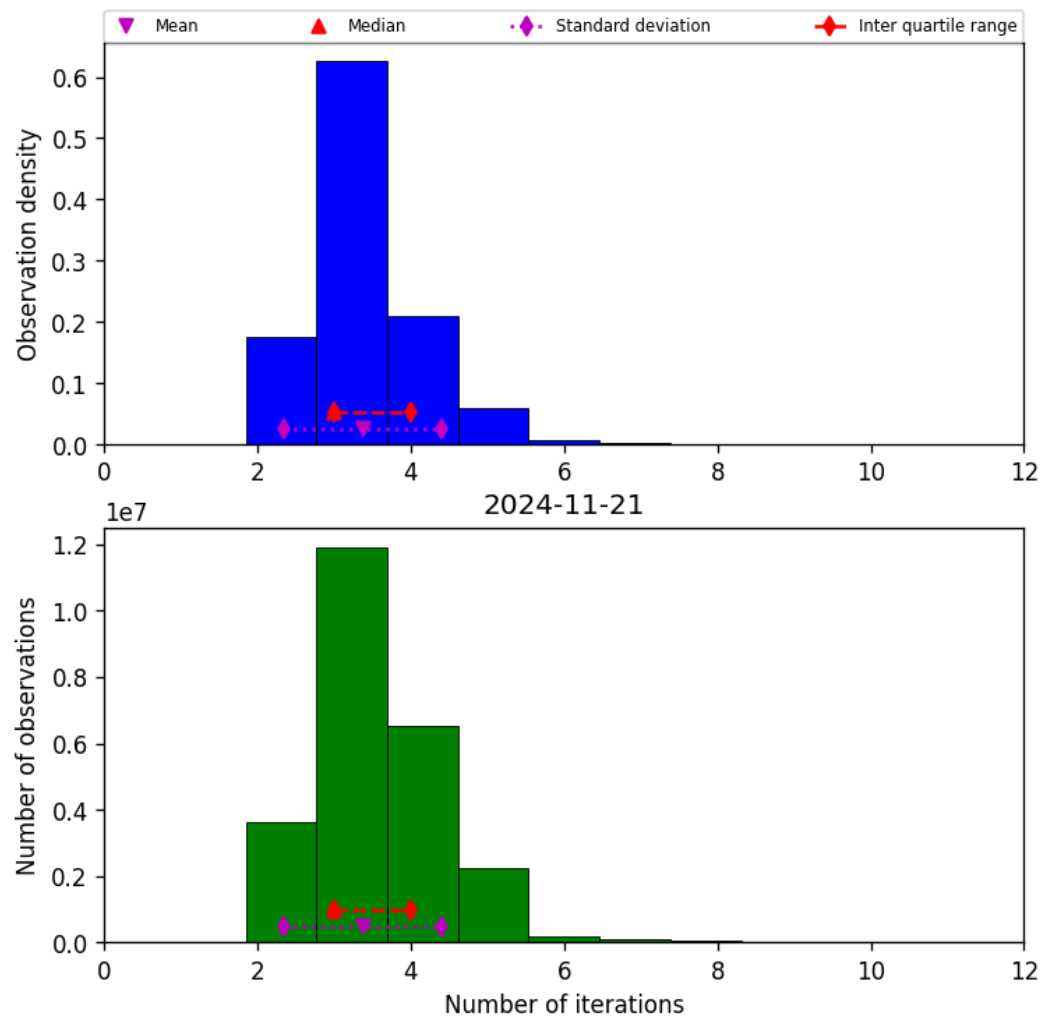
Figure 39: Histogram of “Number of iterations” for 2024-11-20 to 2024-11-22
