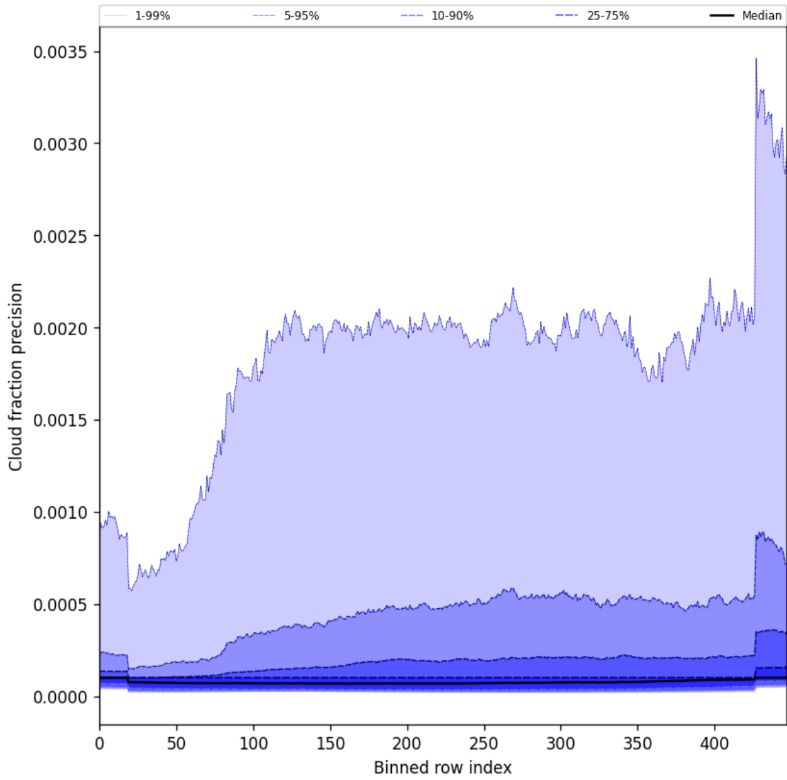
Figure 50: Along track statistics of “Cloud fraction precision” for 2024-11-20 to 2024-11-22
