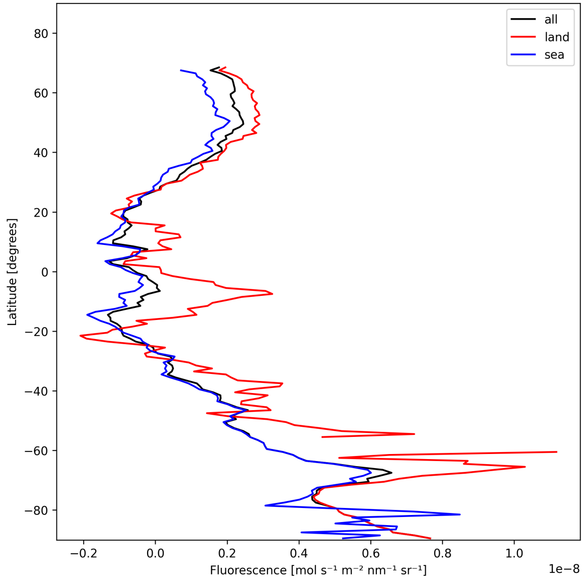
Figure 23: Zonal average of “Fluorescence” for 2024-11-20 to 2024-11-22.
