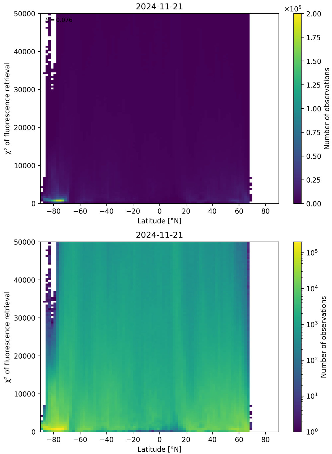
Figure 89: Scatter density plot of “Latitude” against “ \chi^2 of fluorescence retrieval” for 2024-11-20 to 2024-11-22.
