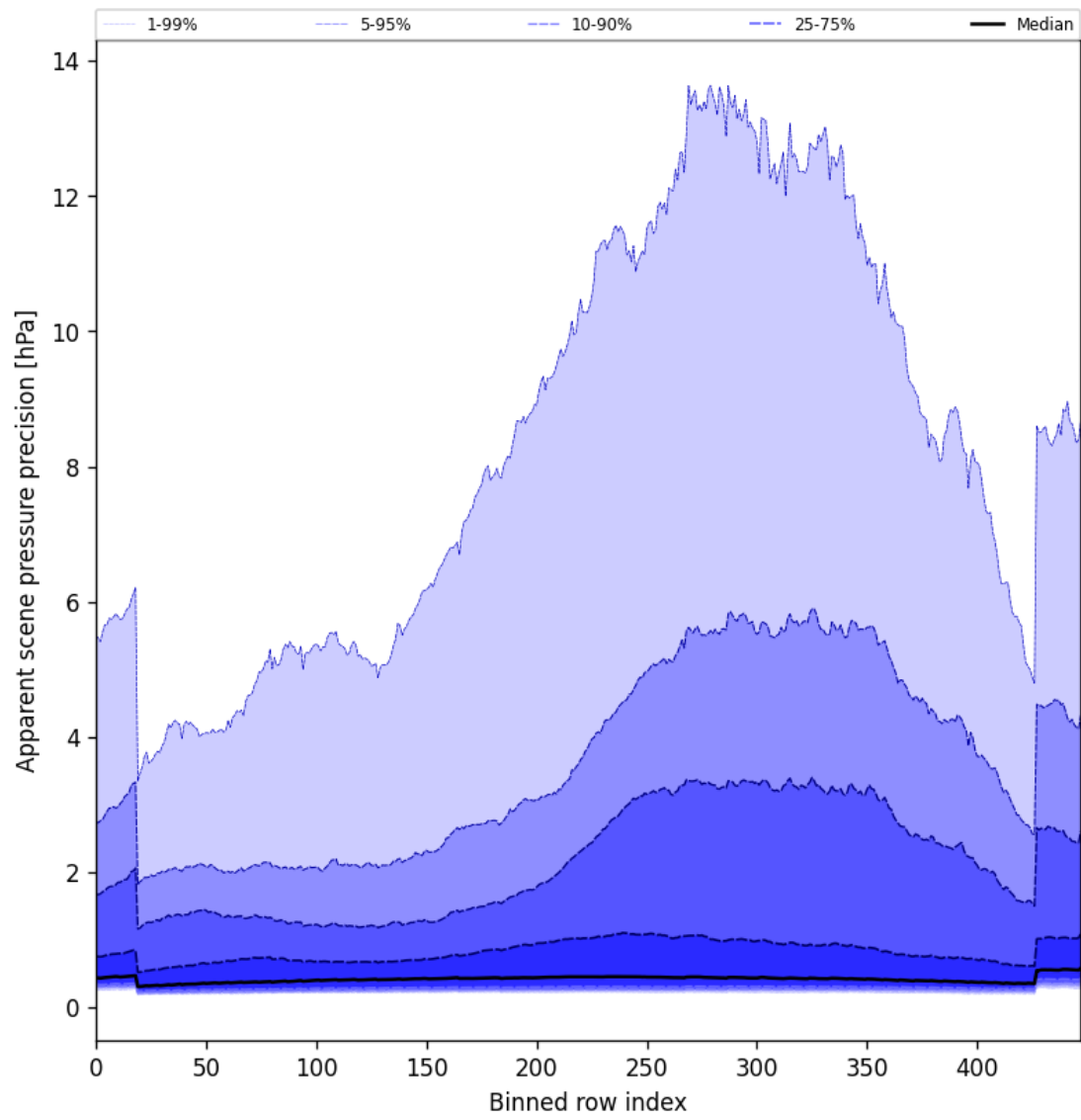
Figure 54: Along track statistics of “Apparent scene pressure precision” for 2024-11-20 to 2024-11-22
