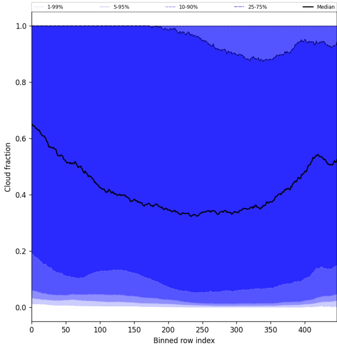
Figure 49: Along track statistics of “Cloud fraction” for 2024-11-20 to 2024-11-22
