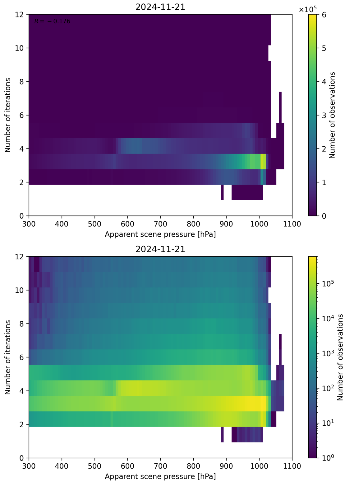
Figure 65: Scatter density plot of “Apparent scene pressure” against “Number of iterations” for 2024-11-20 to 2024-11-22.
