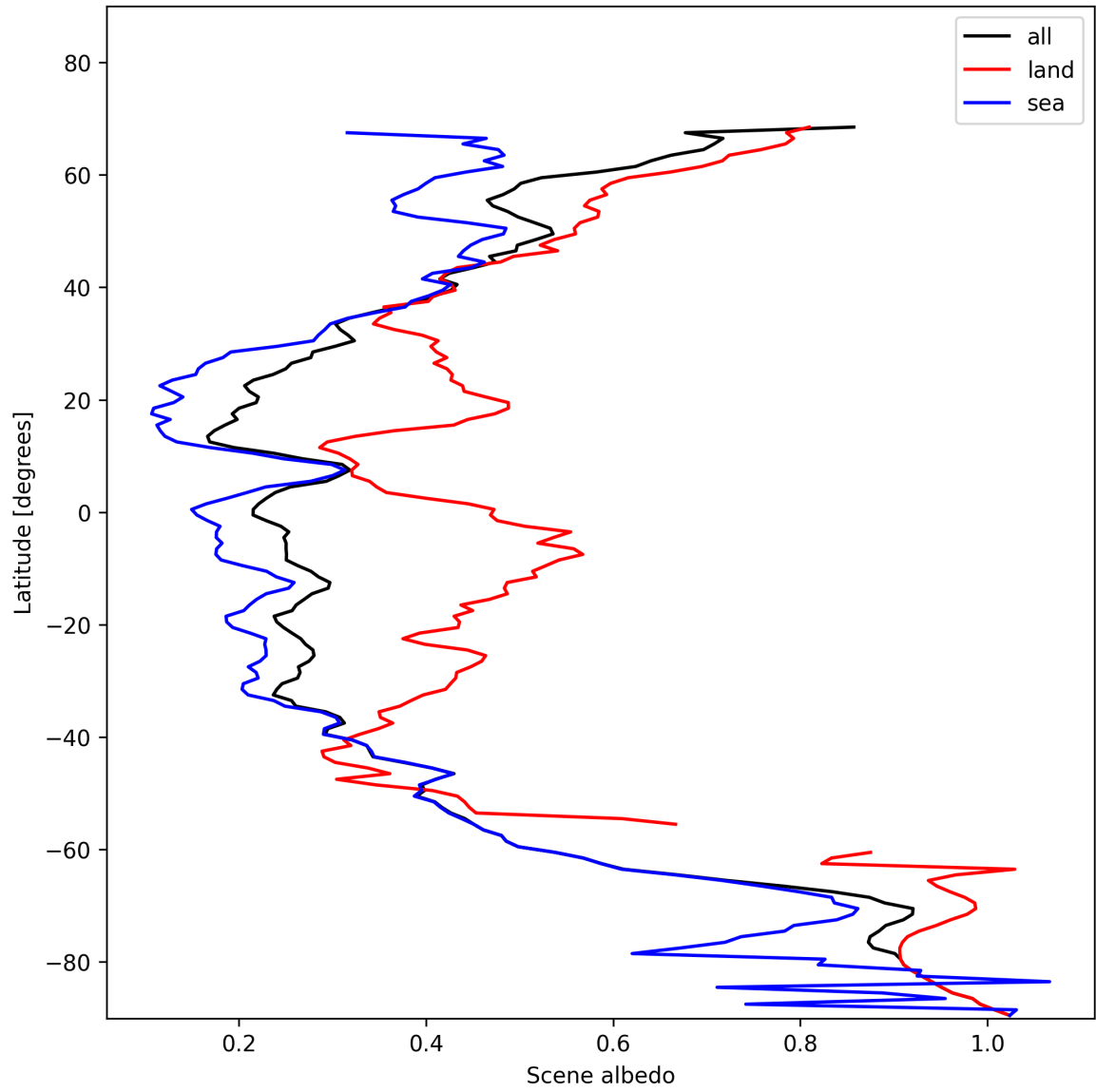
Figure 17: Zonal average of “Scene albedo” for 2024-11-20 to 2024-11-22.
