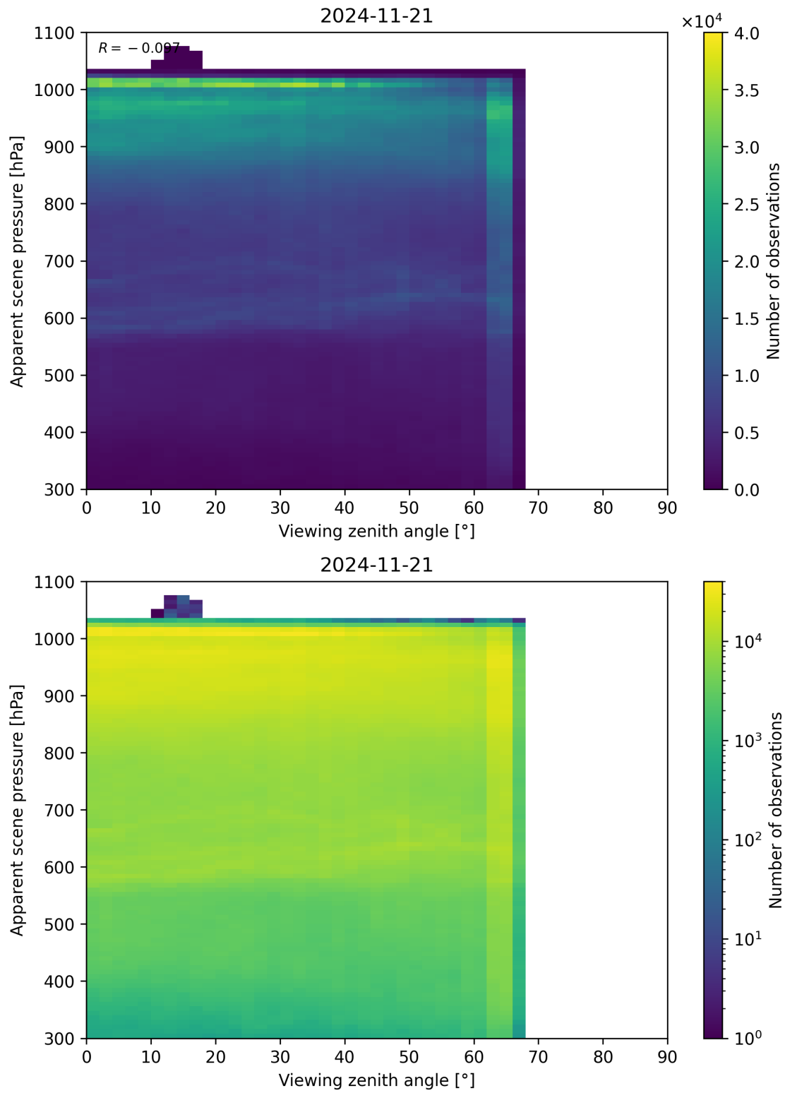
Figure 118: Scatter density plot of “Viewing zenith angle” against “Apparent scene pressure” for 2024-11-20 to 2024-11-22.
