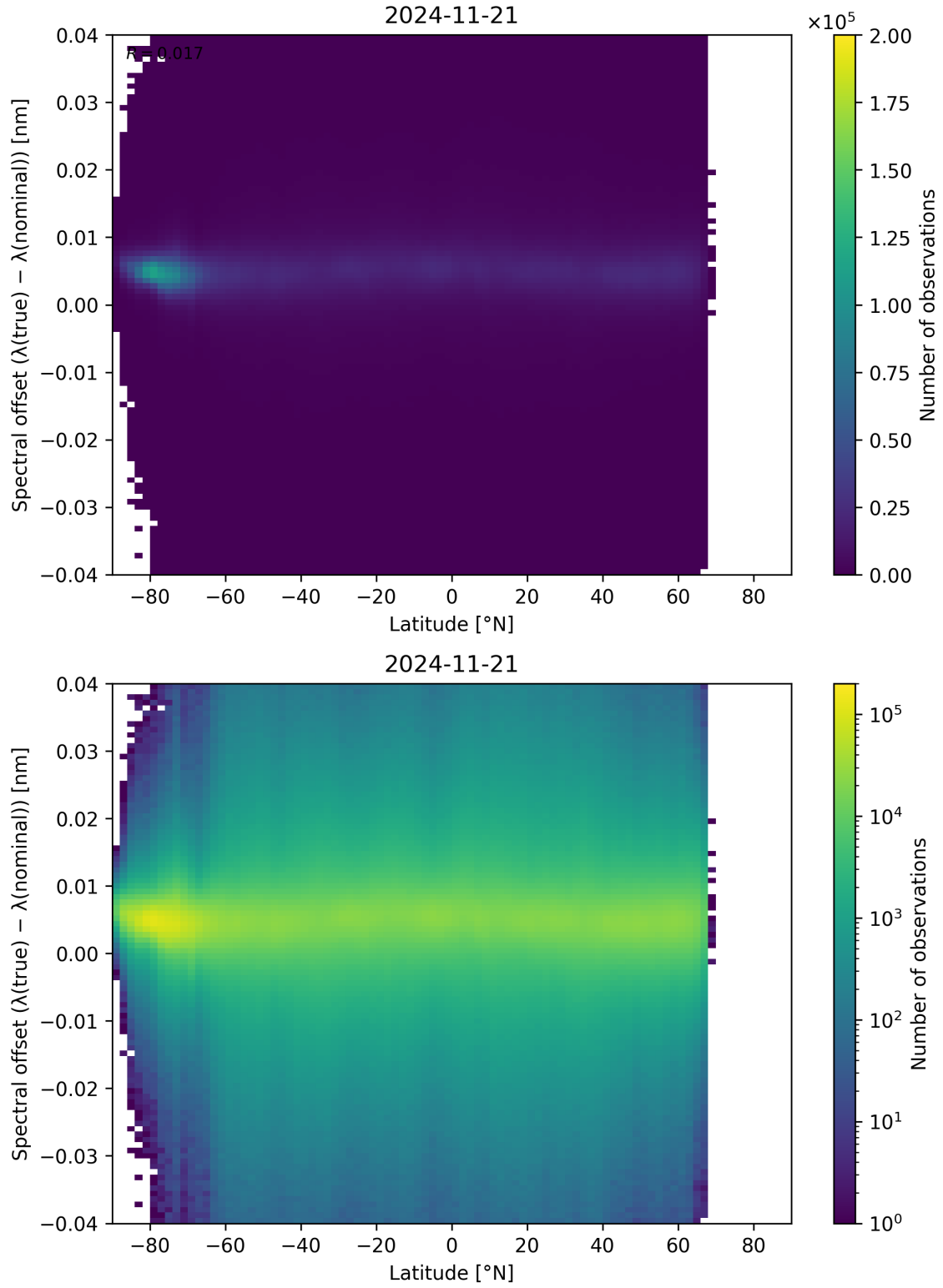
Figure 96: Scatter density plot of “Latitude” against “Spectral offset ( \lambda_{\text{true}} - \lambda_{\text{nominal}} )” for 2024-11-20 to 2024-11-22.
