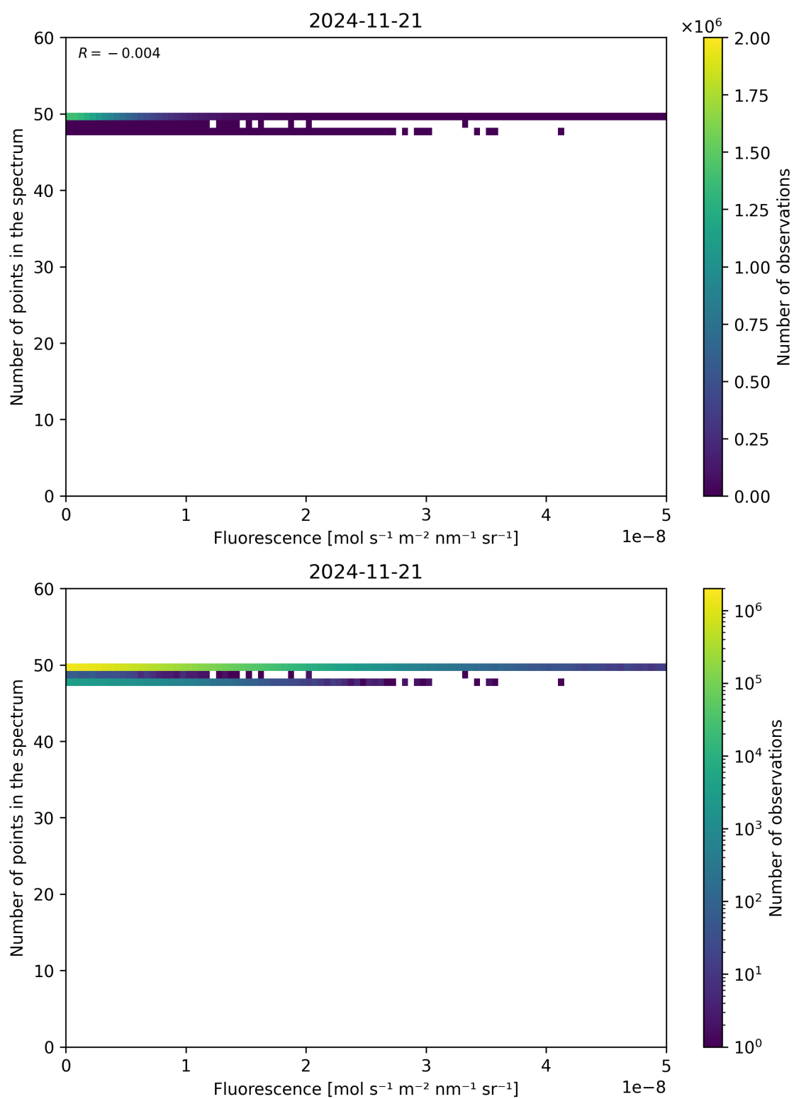
Figure 86: Scatter density plot of “Fluorescence” against “Number of points in the spectrum” for 2024-11-20 to 2024-11-22.
