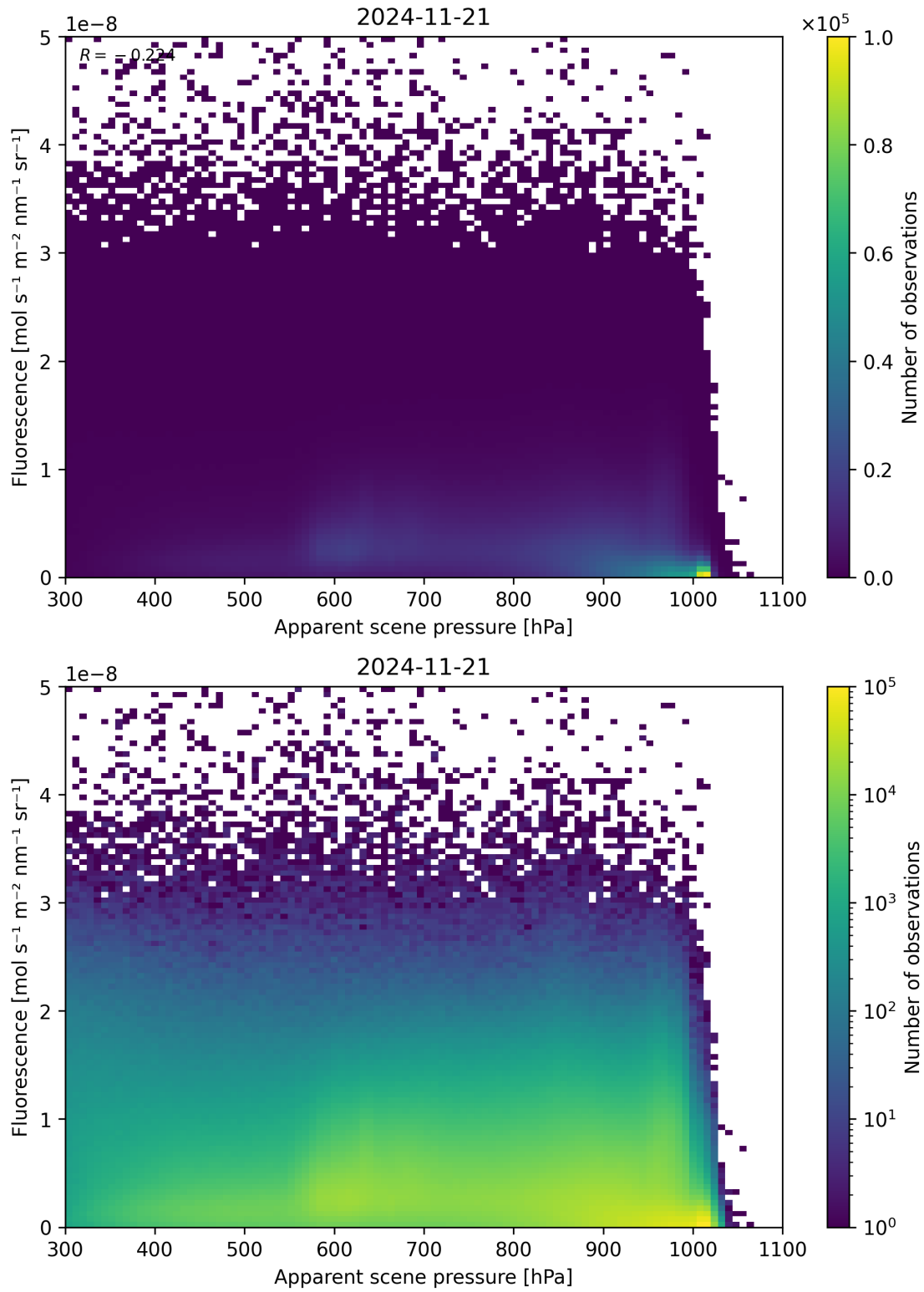
Figure 64: Scatter density plot of “Apparent scene pressure” against “Fluorescence” for 2024-11-20 to 2024-11-22.
