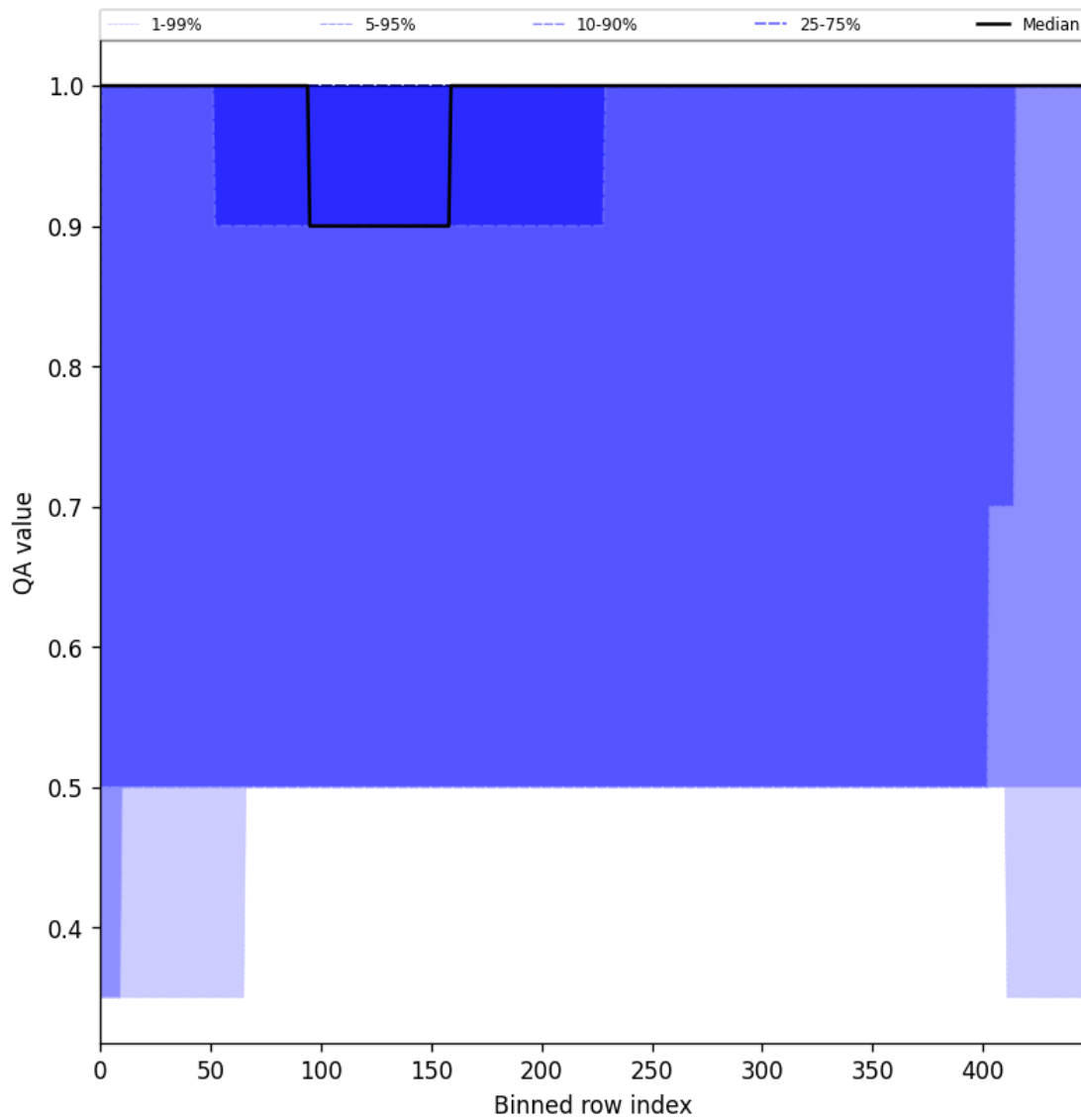
Figure 46: Along track statistics of “QA value” for 2024-11-20 to 2024-11-22
