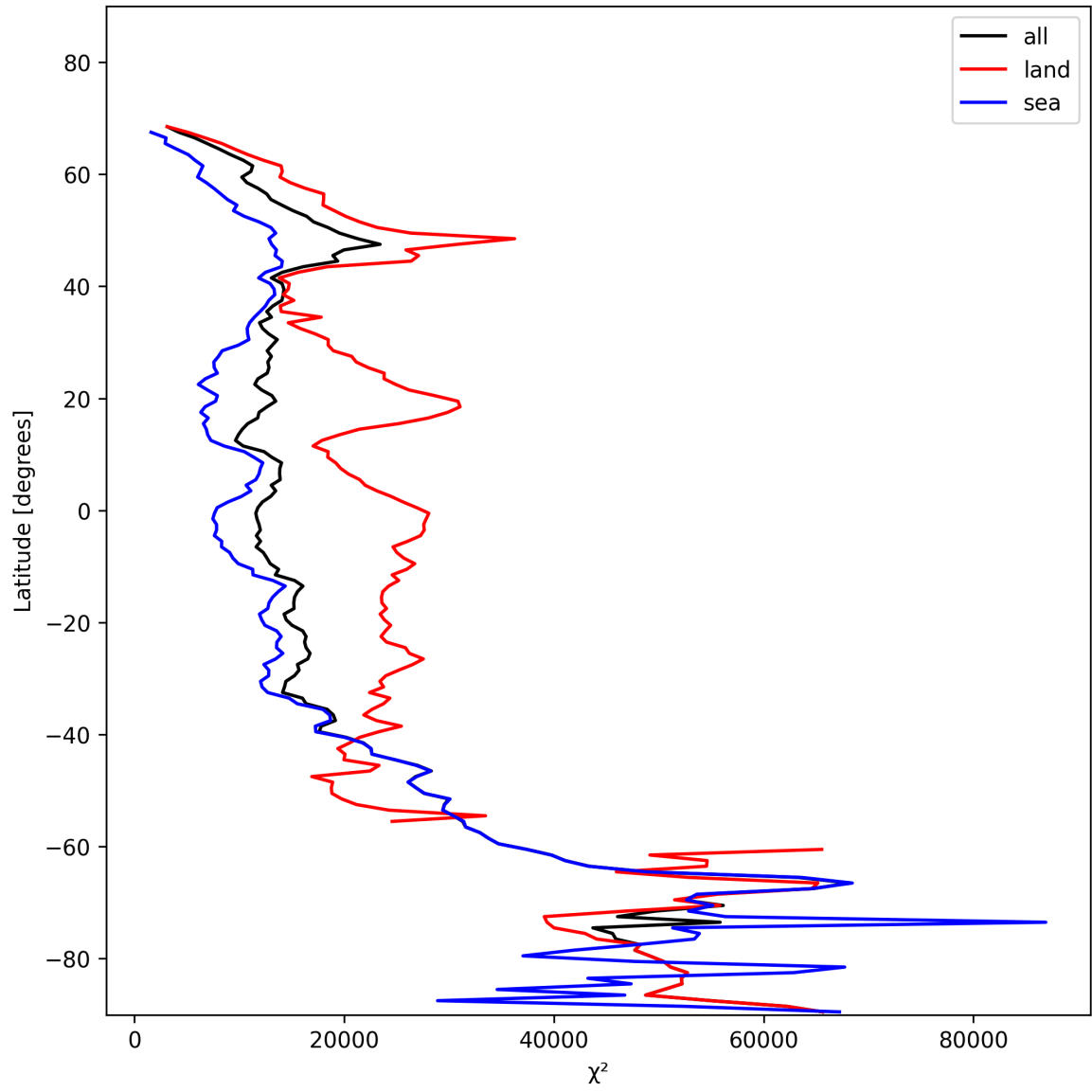
Figure 21: Zonal average of “ \chi^2 ” for 2024-11-20 to 2024-11-22.
