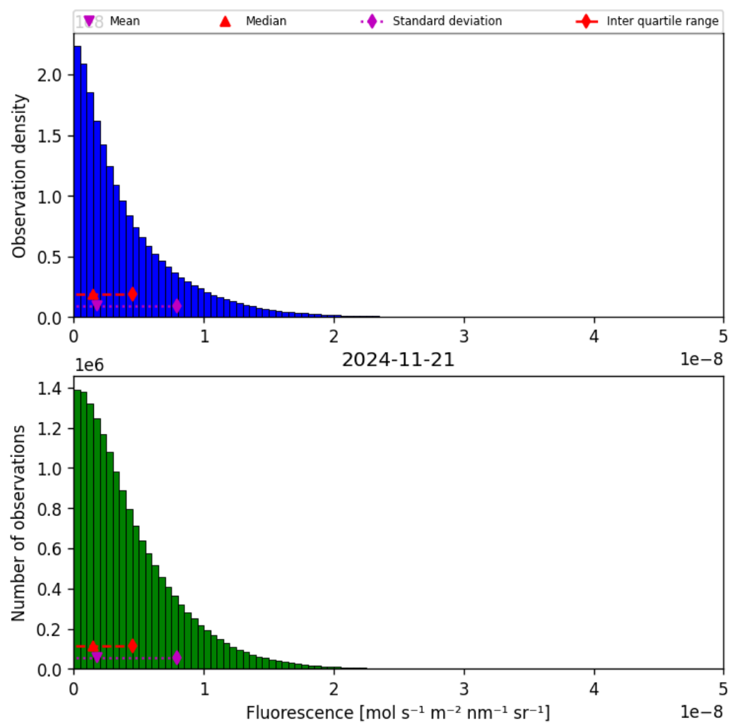
Figure 40: Histogram of “Fluorescence” for 2024-11-20 to 2024-11-22
