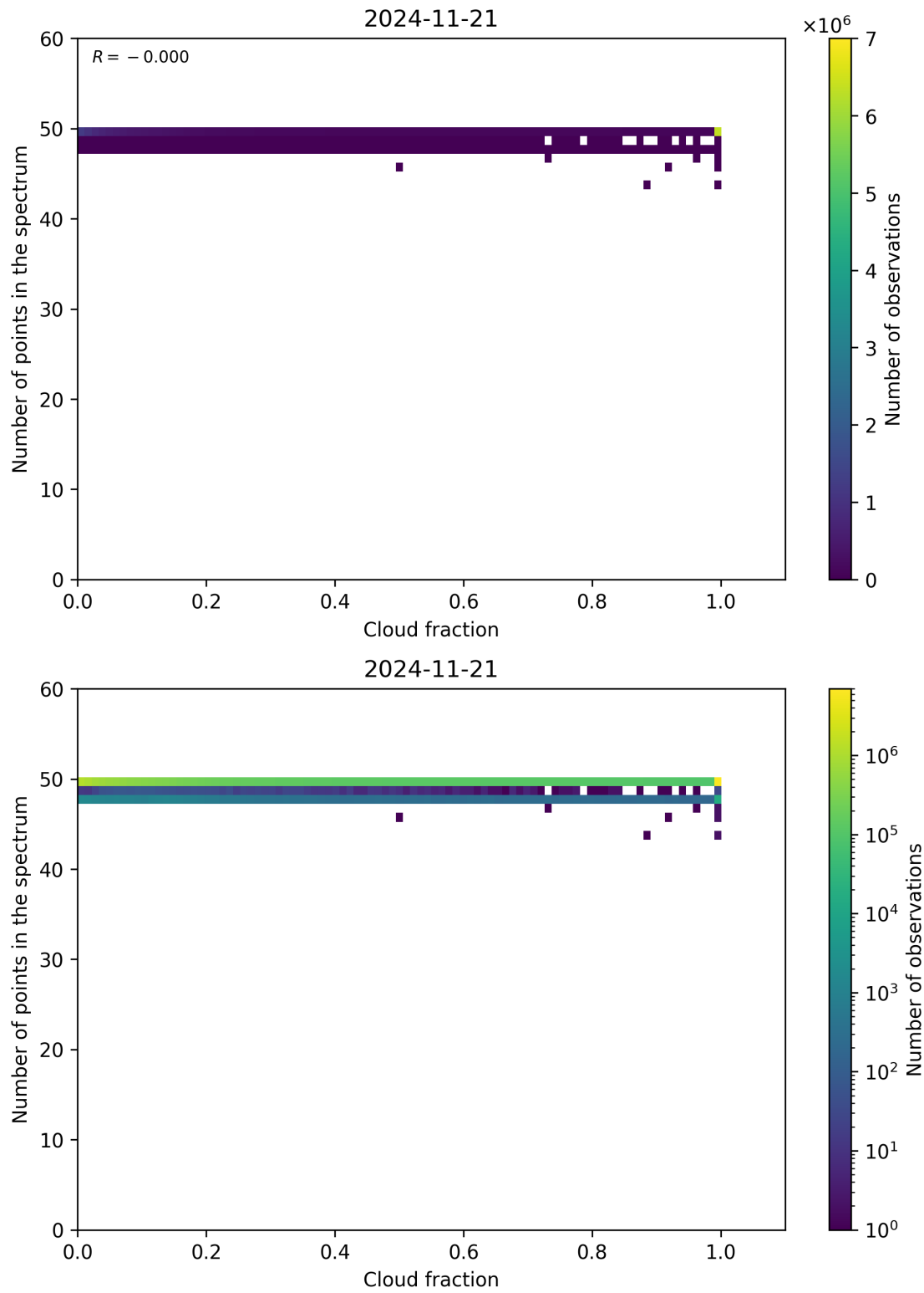
Figure 74: Scatter density plot of “Cloud fraction” against “Number of points in the spectrum” for 2024-11-20 to 2024-11-22.
