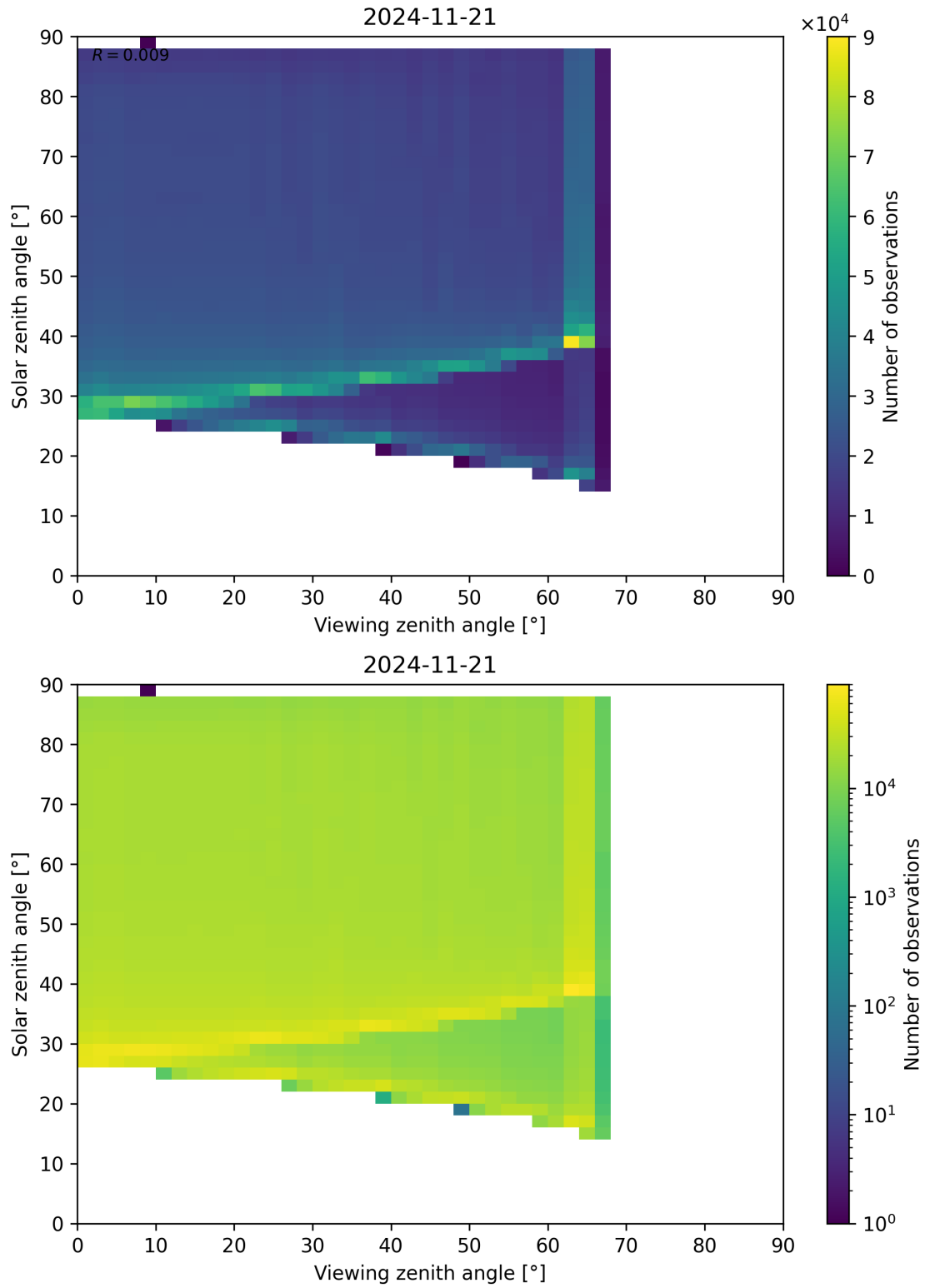
Figure 127: Scatter density plot of “Viewing zenith angle” against “Solar zenith angle” for 2024-11-20 to 2024-11-22.
