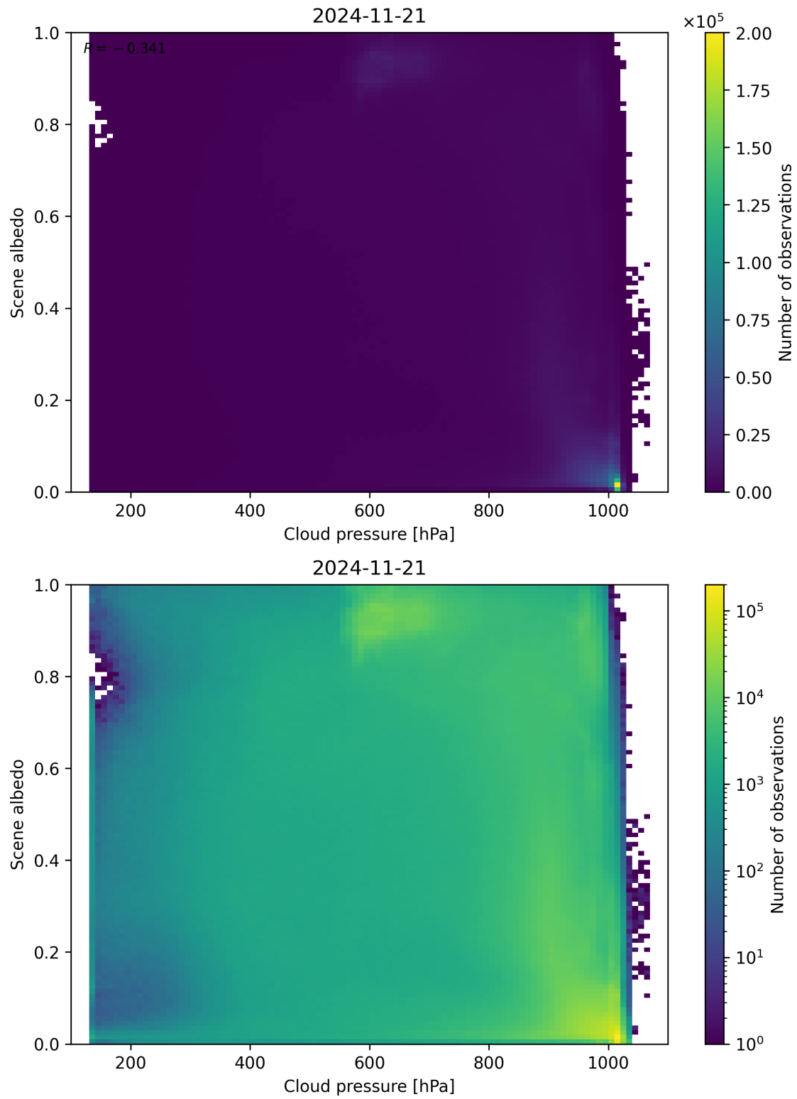
Figure 83: Scatter density plot of “Cloud pressure” against “Scene albedo” for 2024-11-20 to 2024-11-22.
