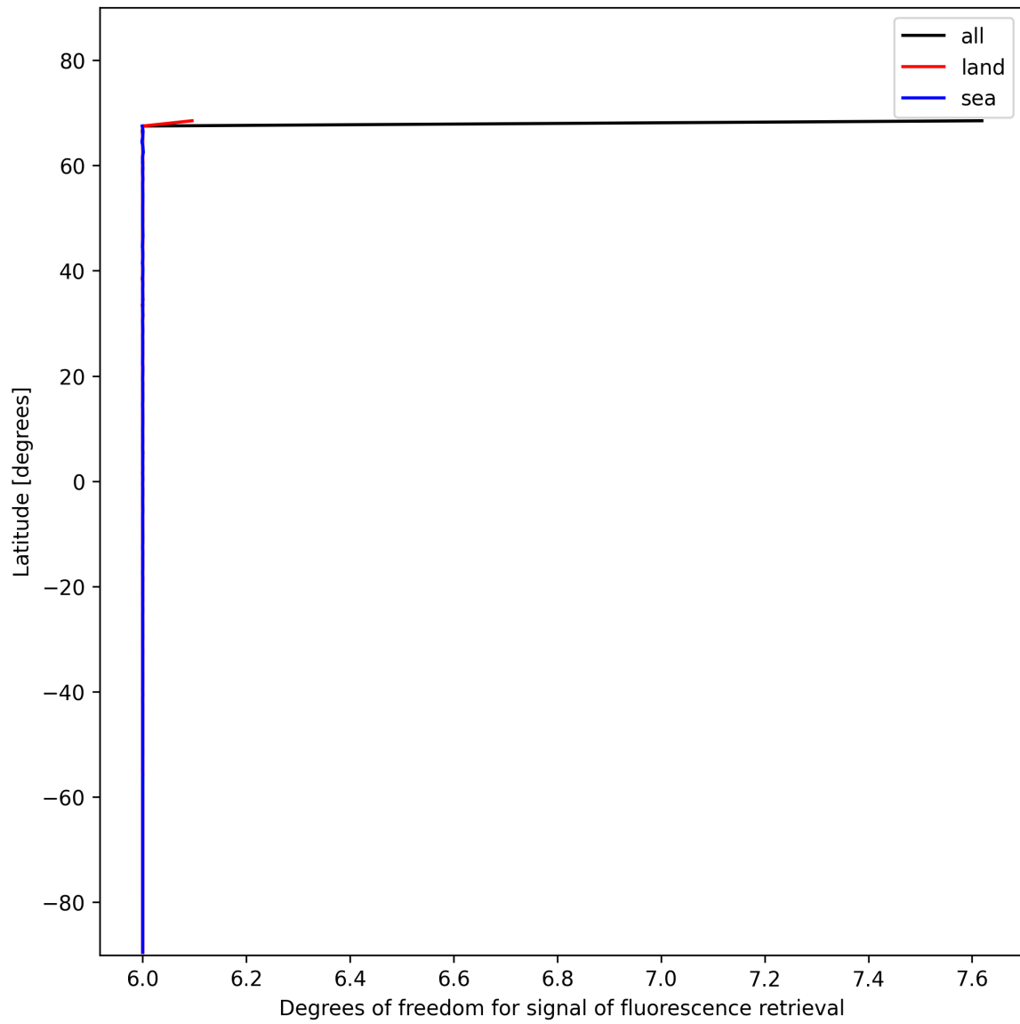
Figure 26: Zonal average of “Degrees of freedom for signal of fluorescence retrieval” for 2024-11-20 to 2024-11-22.
