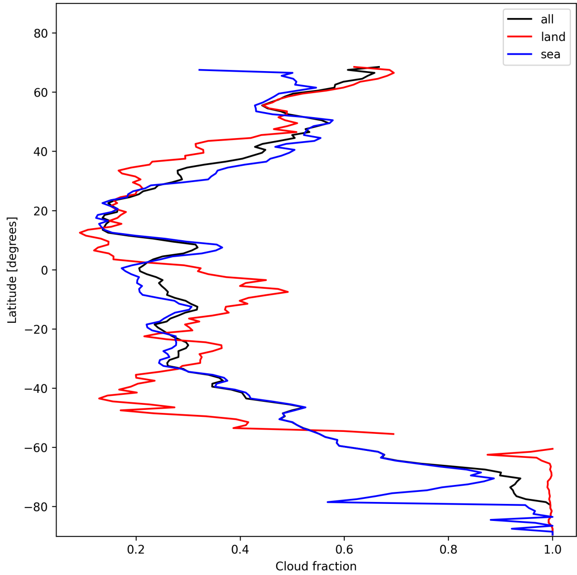
Figure 15: Zonal average of “Cloud fraction” for 2024-11-20 to 2024-11-22.
