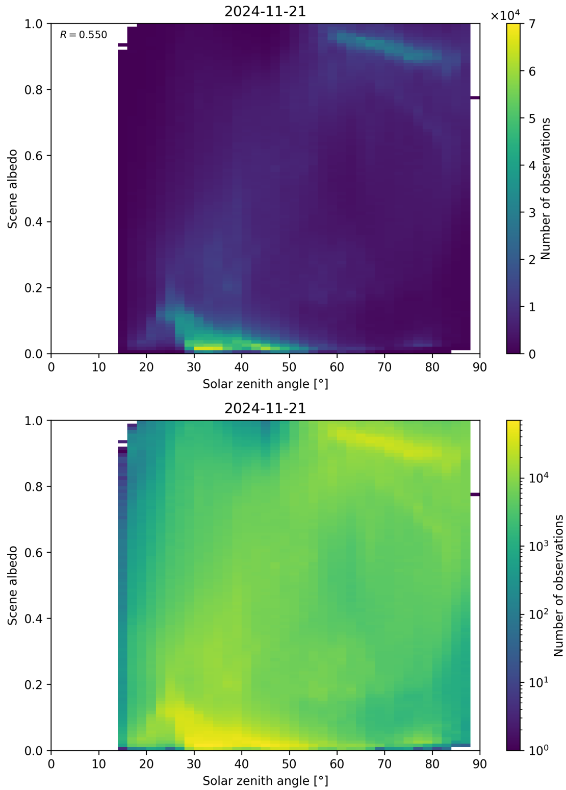
Figure 116: Scatter density plot of “Solar zenith angle” against “Scene albedo” for 2024-11-20 to 2024-11-22.
