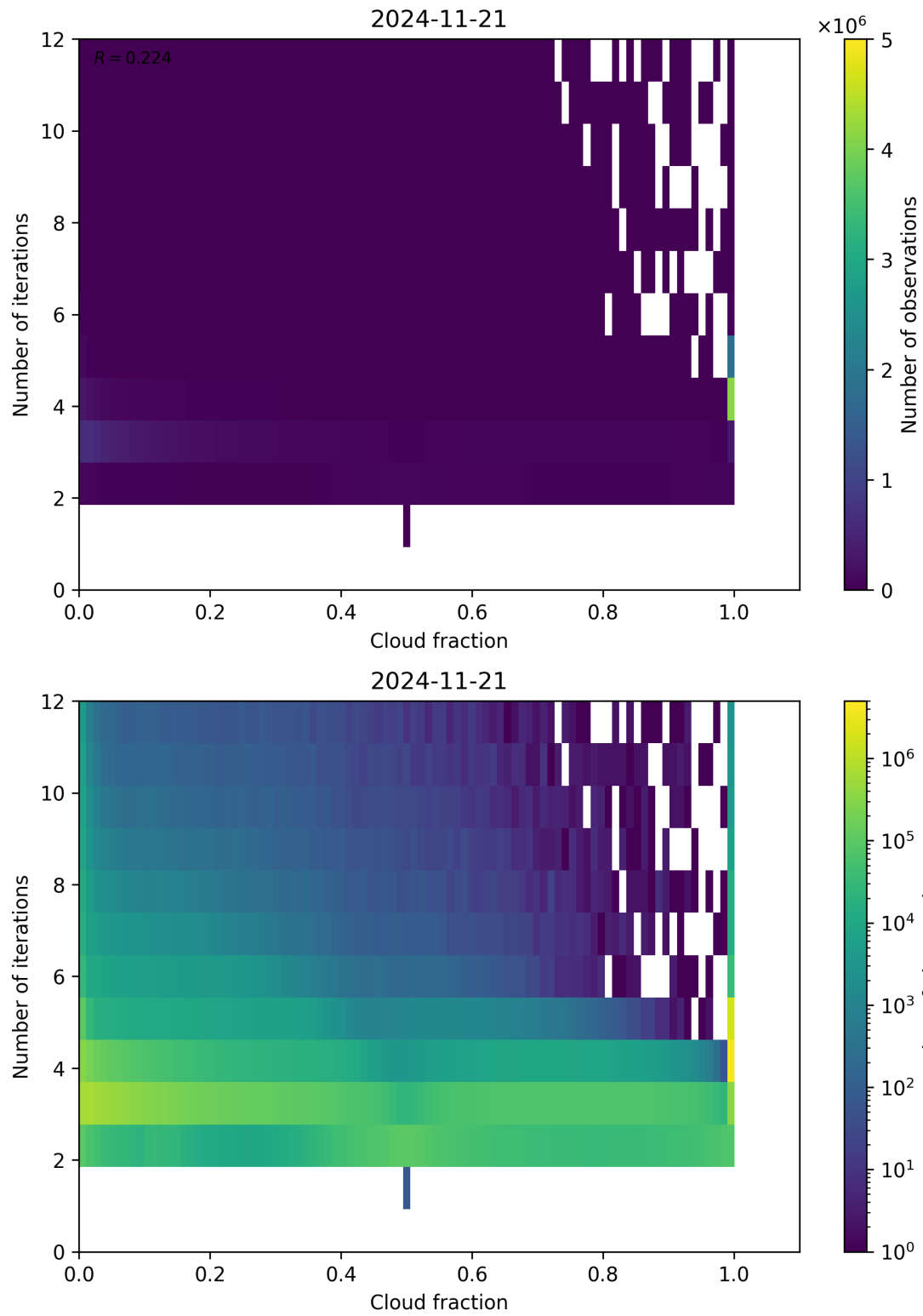
Figure 73: Scatter density plot of “Cloud fraction” against “Number of iterations” for 2024-11-20 to 2024-11-22.
