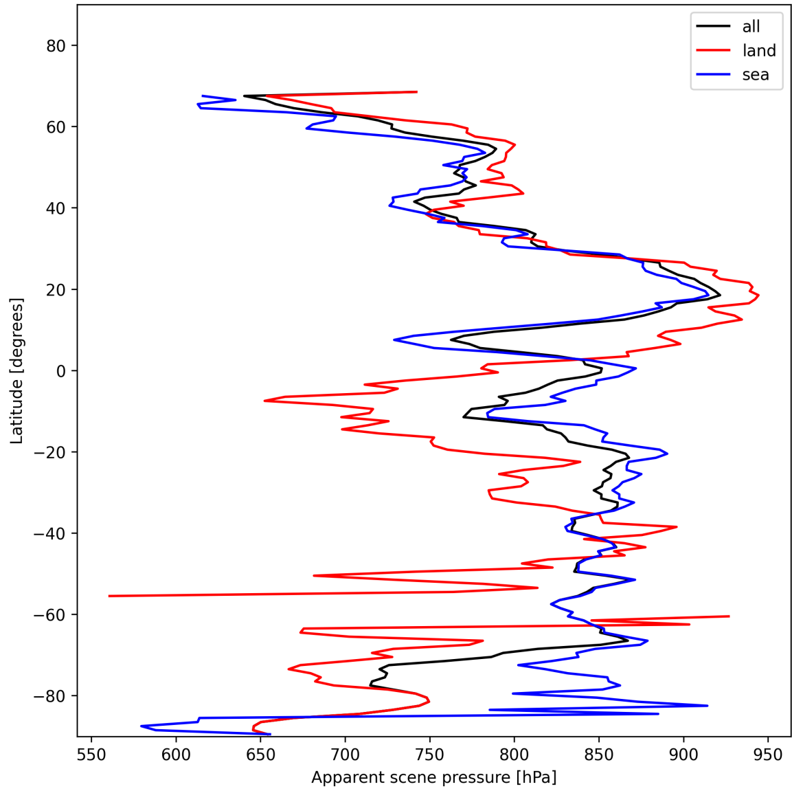
Figure 19: Zonal average of “Apparent scene pressure” for 2024-11-20 to 2024-11-22.
