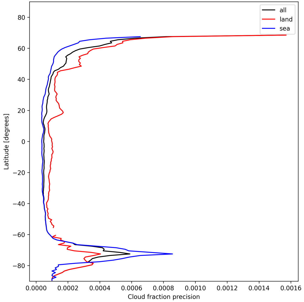
Figure 16: Zonal average of “Cloud fraction precision” for 2024-11-20 to 2024-11-22.
