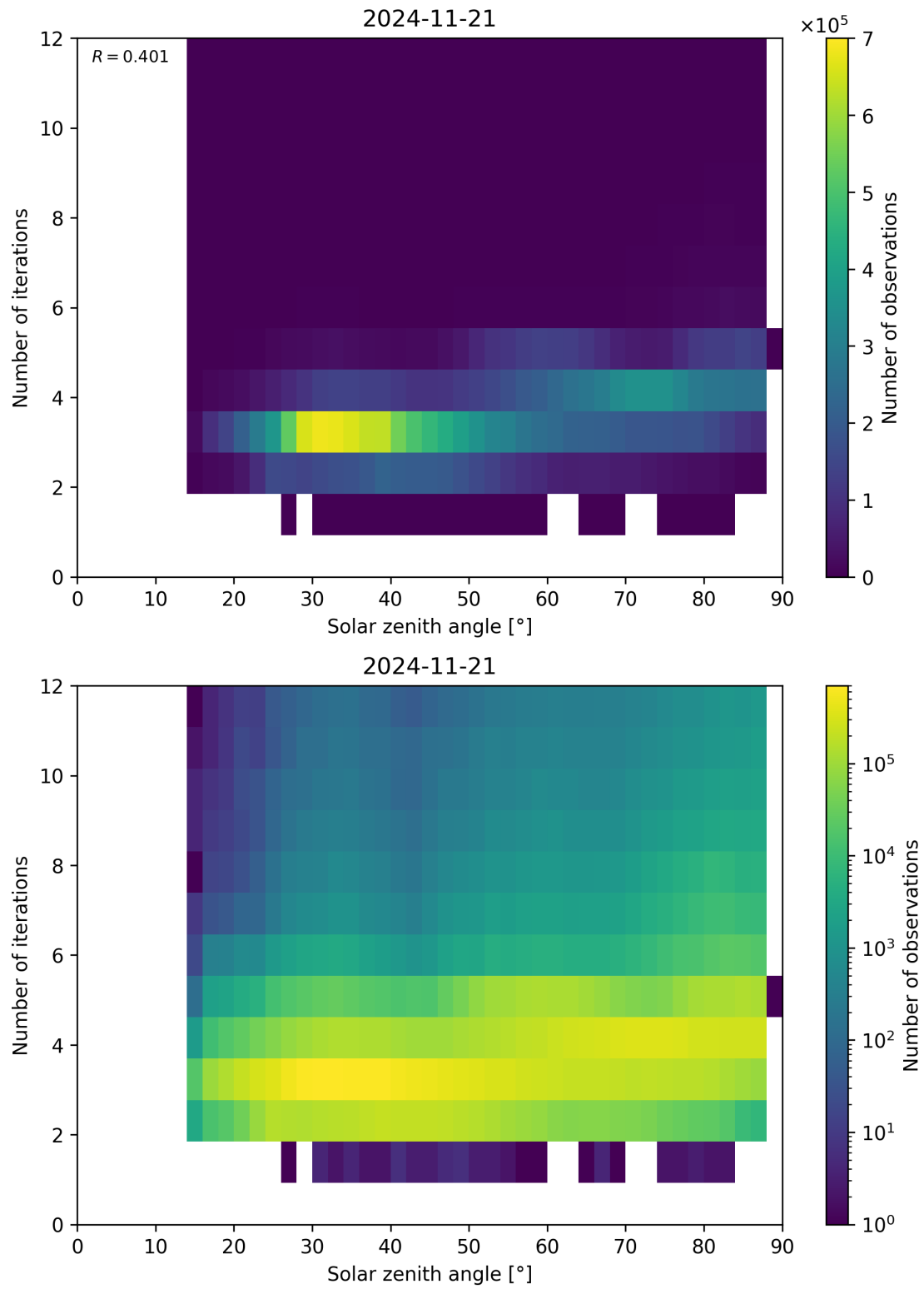
Figure 114: Scatter density plot of “Solar zenith angle” against “Number of iterations” for 2024-11-20 to 2024-11-22.
