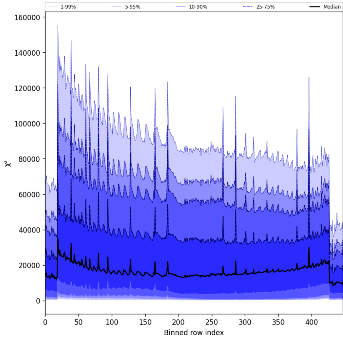
Figure 55: Along track statistics of “ \chi^2 ” for 2024-11-20 to 2024-11-22
