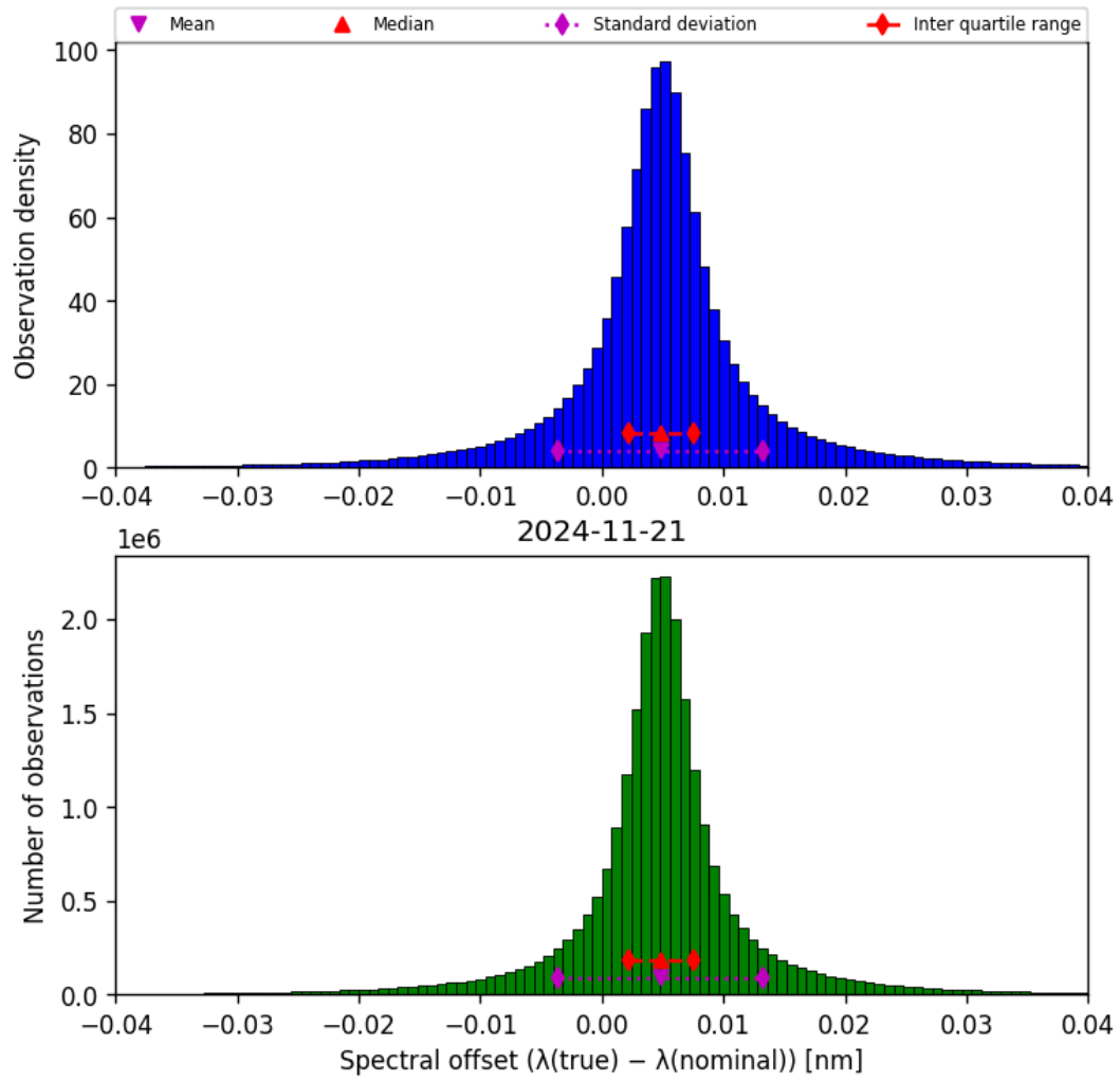
Figure 45: Histogram of “Spectral offset ( \lambda_{\text{true}} - \lambda_{\text{nominal}} )” for 2024-11-20 to 2024-11-22
