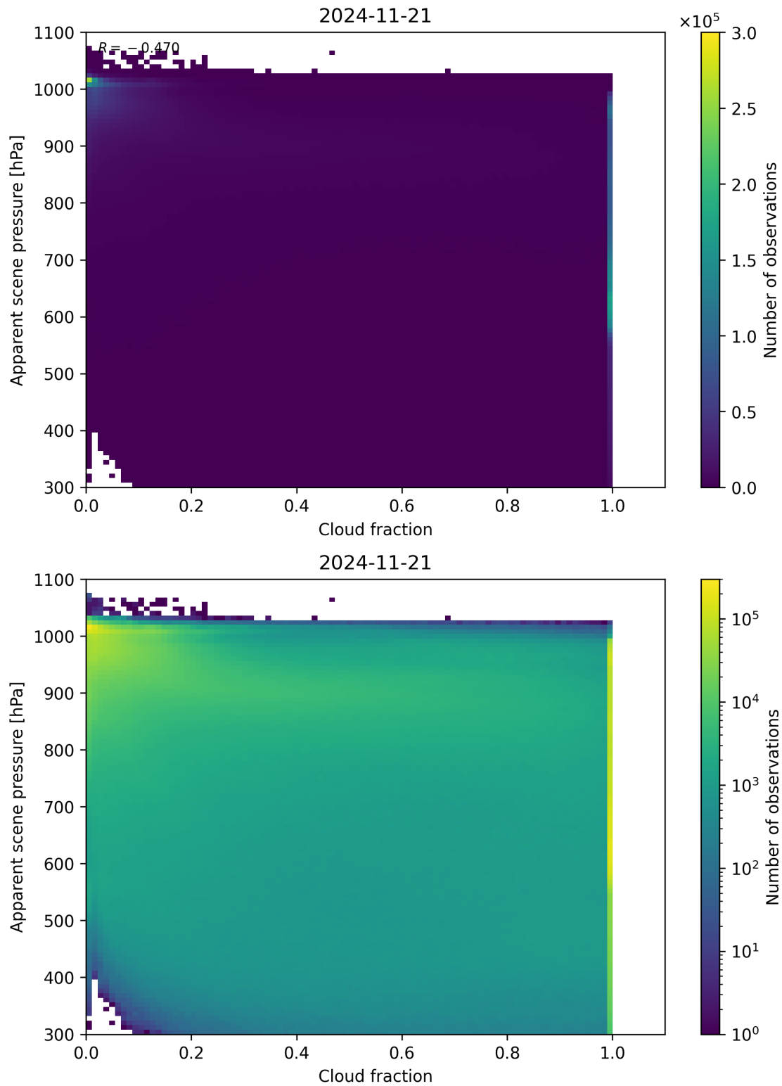
Figure 70: Scatter density plot of “Cloud fraction” against “Apparent scene pressure” for 2024-11-20 to 2024-11-22.
