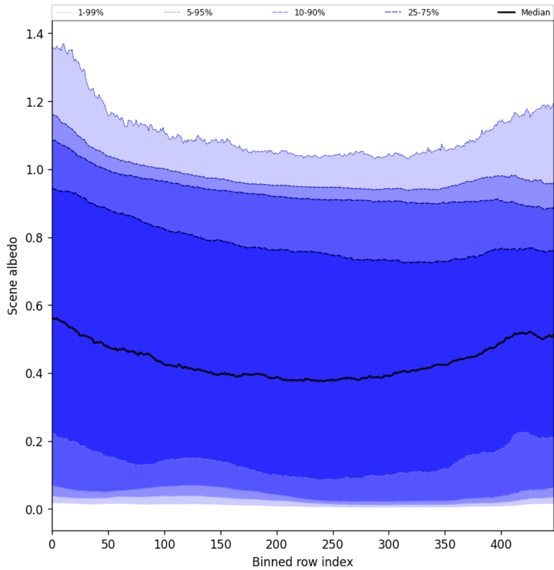
Figure 51: Along track statistics of “Scene albedo” for 2024-11-20 to 2024-11-22
