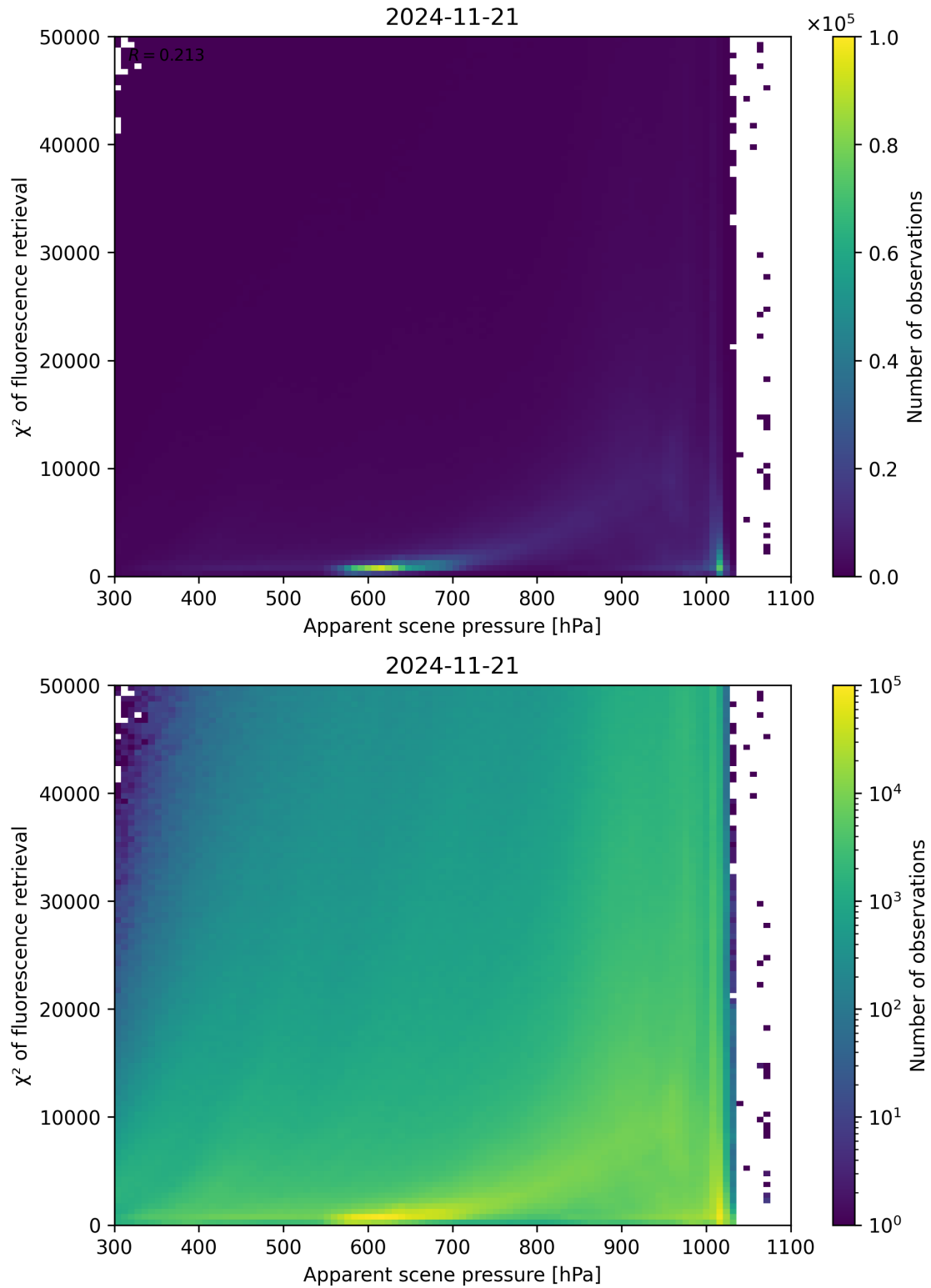
Figure 63: Scatter density plot of “Apparent scene pressure” against “ \chi^2 of fluorescence retrieval” for 2024-11-20 to 2024-11-22.
