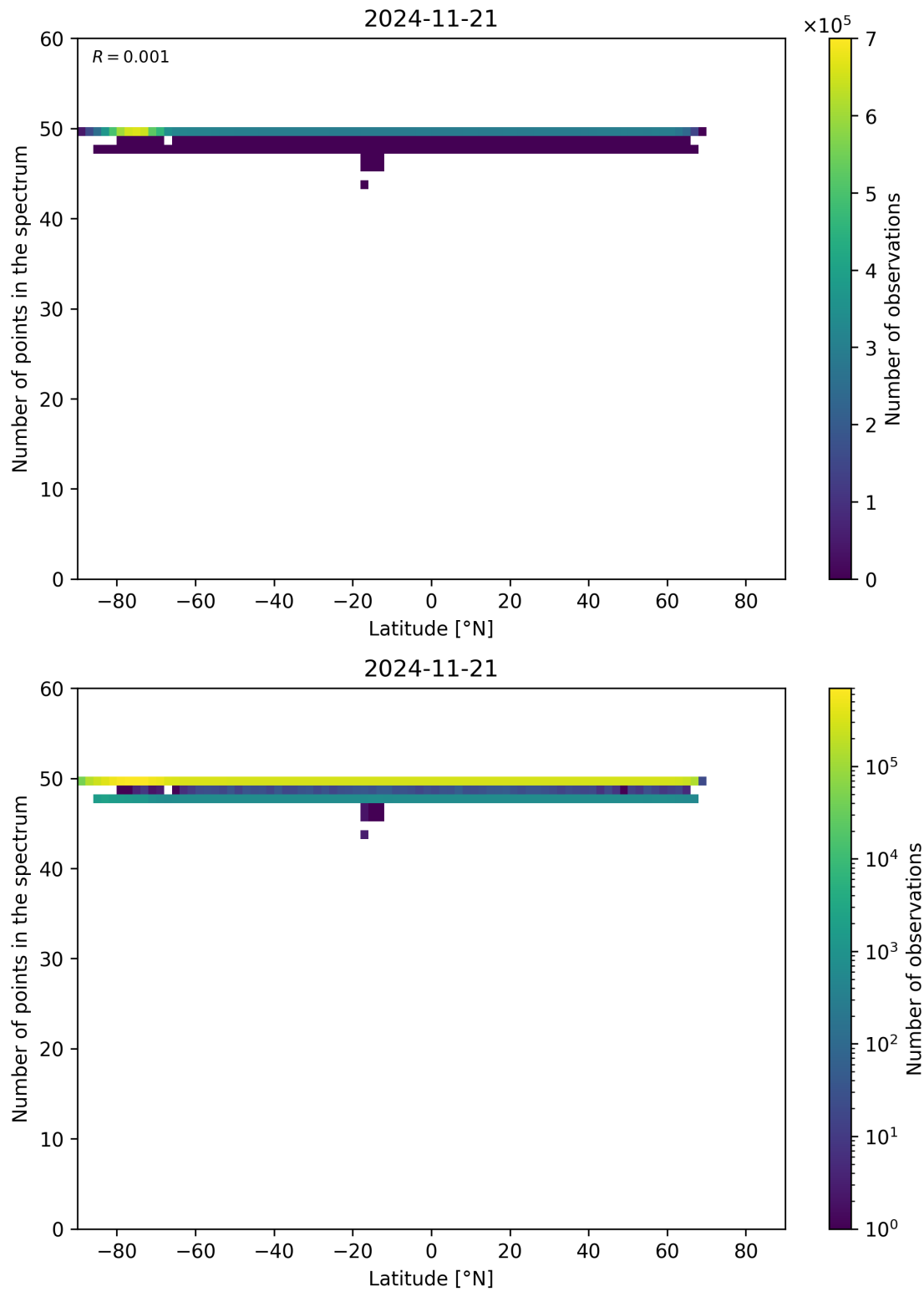
Figure 94: Scatter density plot of “Latitude” against “Number of points in the spectrum” for 2024-11-20 to 2024-11-22.
