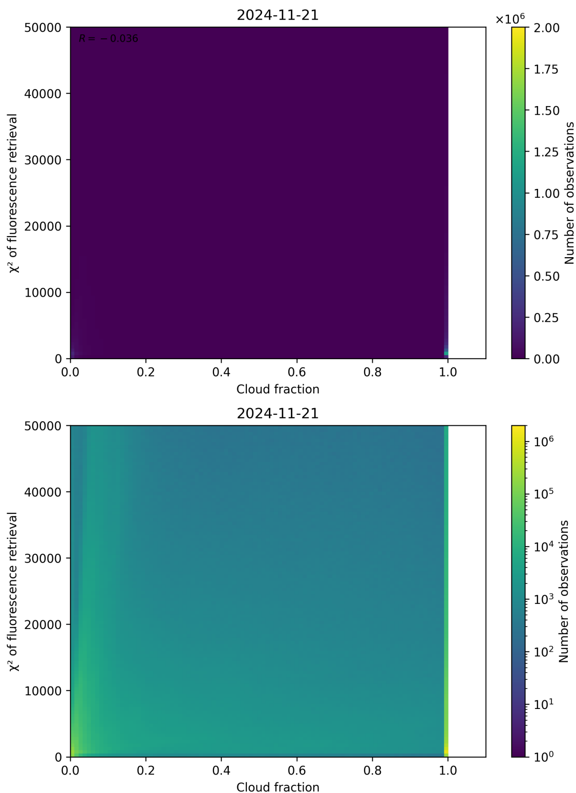
Figure 71: Scatter density plot of “Cloud fraction” against “ \chi^2 of fluorescence retrieval” for 2024-11-20 to 2024-11-22.
