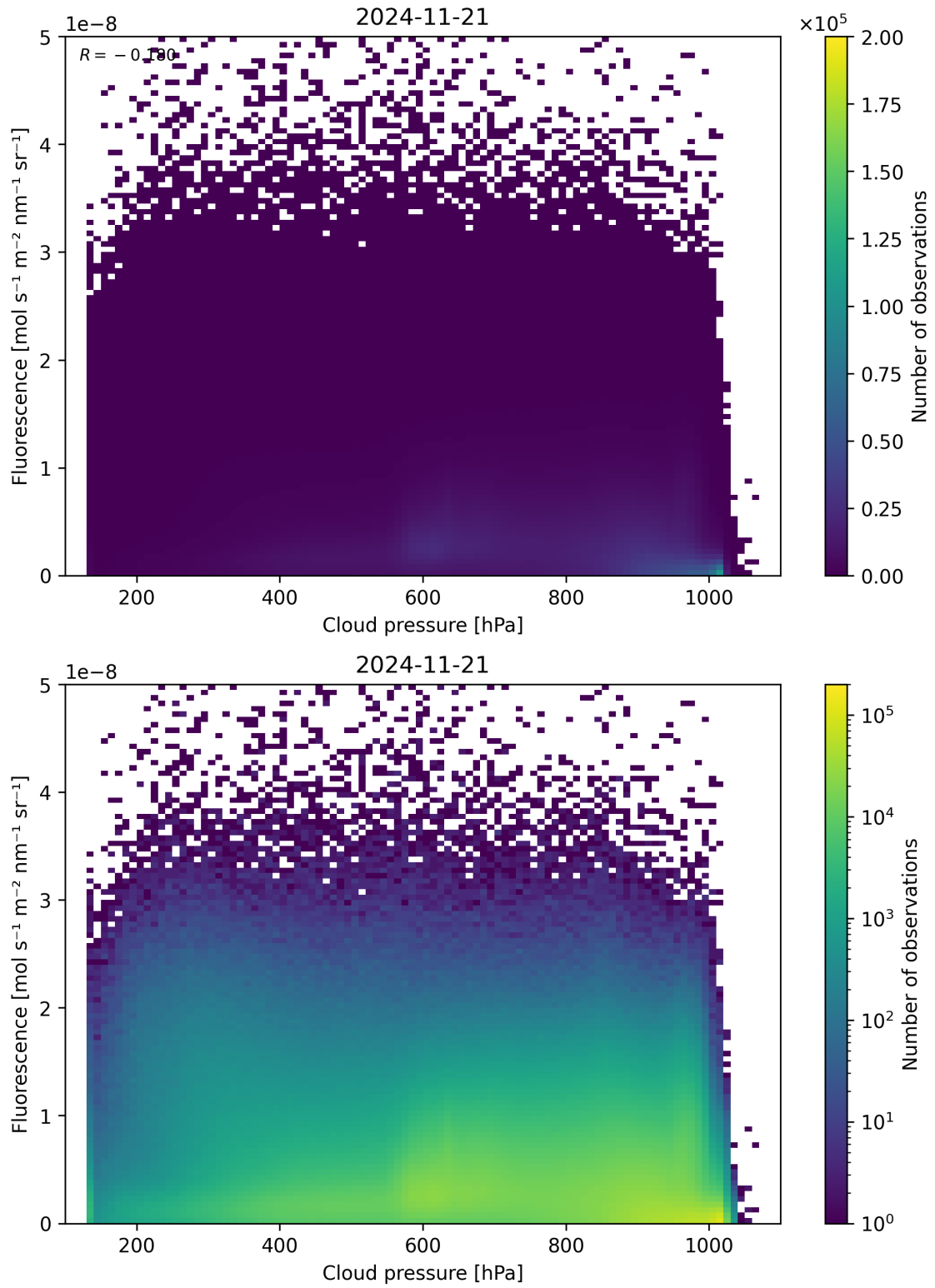
Figure 80: Scatter density plot of “Cloud pressure” against “Fluorescence” for 2024-11-20 to 2024-11-22.
