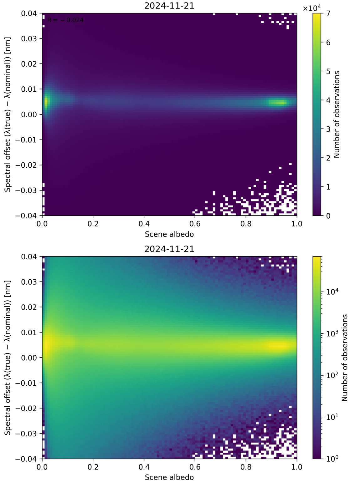
Figure 107: Scatter density plot of “Scene albedo” against “Spectral offset ( \lambda_{\text{true}} - \lambda_{\text{nominal}} )” for 2024-11-20 to 2024-11-22.
