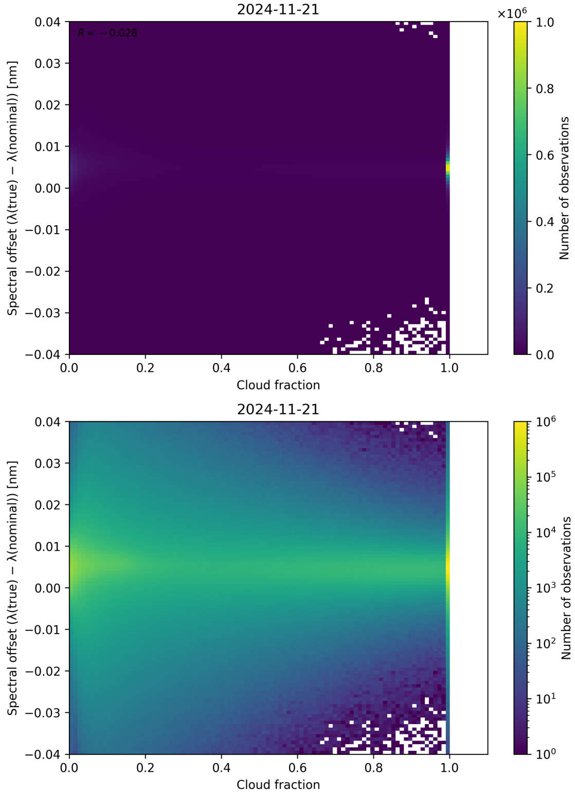
Figure 76: Scatter density plot of “Cloud fraction” against “Spectral offset ( \lambda_{\text{true}} - \lambda_{\text{nominal}} )” for 2024-11-20 to 2024-11-22.
