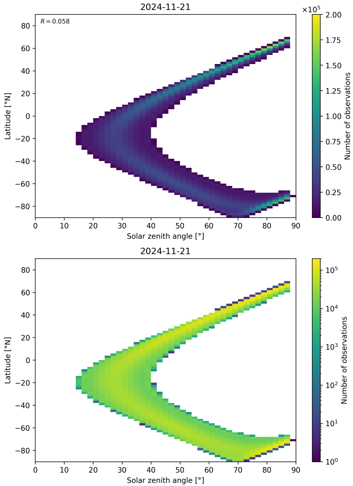
Figure 113: Scatter density plot of “Solar zenith angle” against “Latitude” for 2024-11-20 to 2024-11-22.
