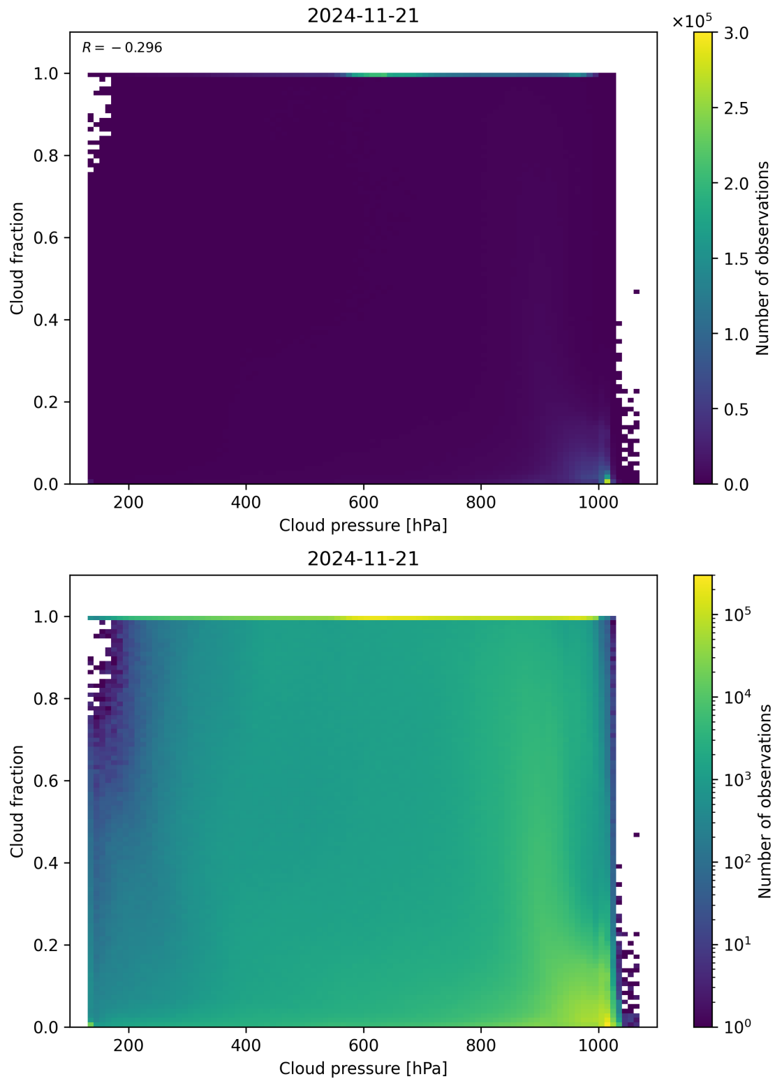
Figure 79: Scatter density plot of “Cloud pressure” against “Cloud fraction” for 2024-11-20 to 2024-11-22.
