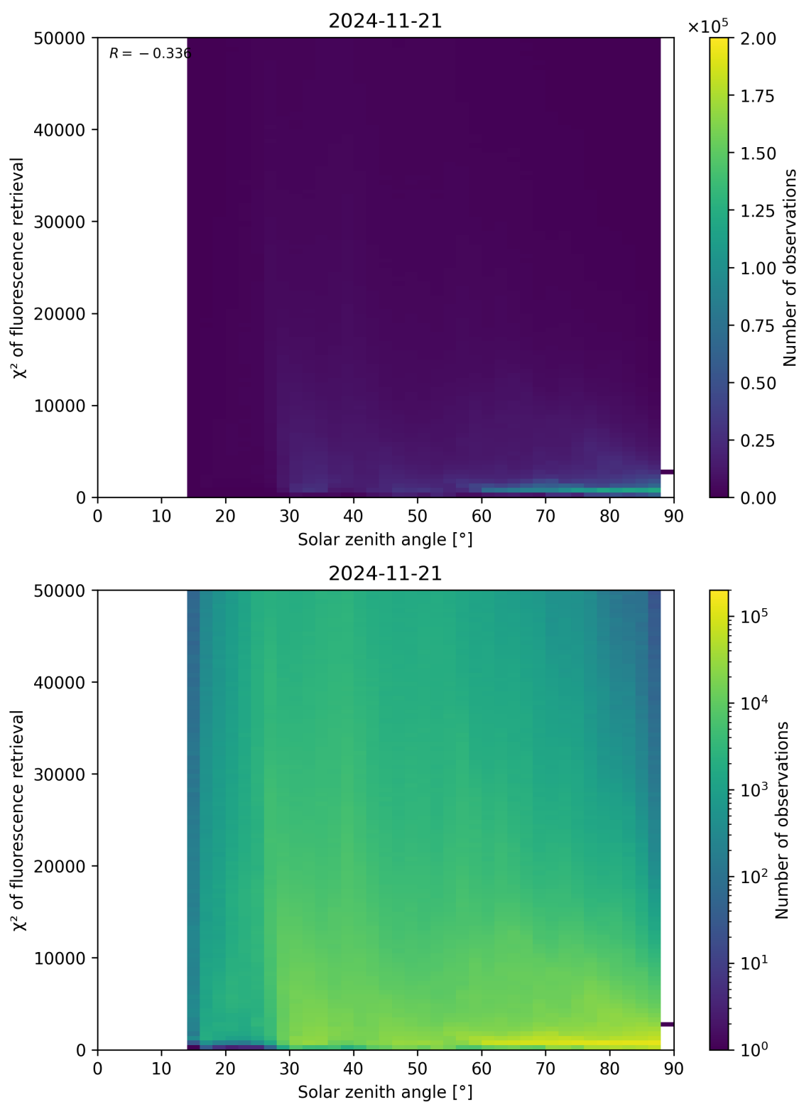
Figure 109: Scatter density plot of “Solar zenith angle” against “ \chi^2 of fluorescence retrieval” for 2024-11-20 to 2024-11-22.
