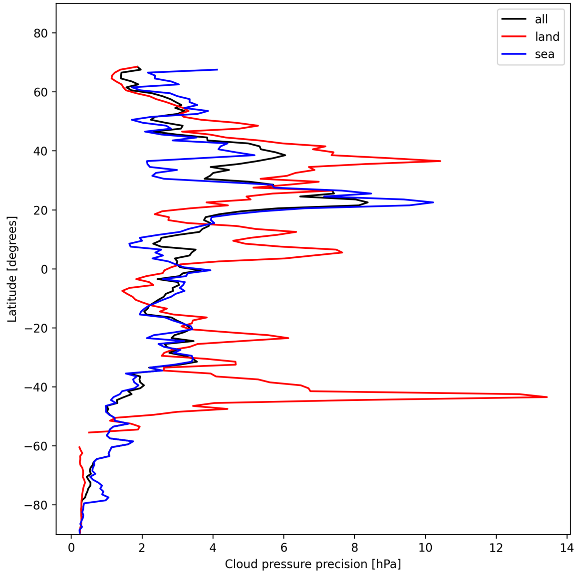
Figure 14: Zonal average of “Cloud pressure precision” for 2024-11-20 to 2024-11-22.
