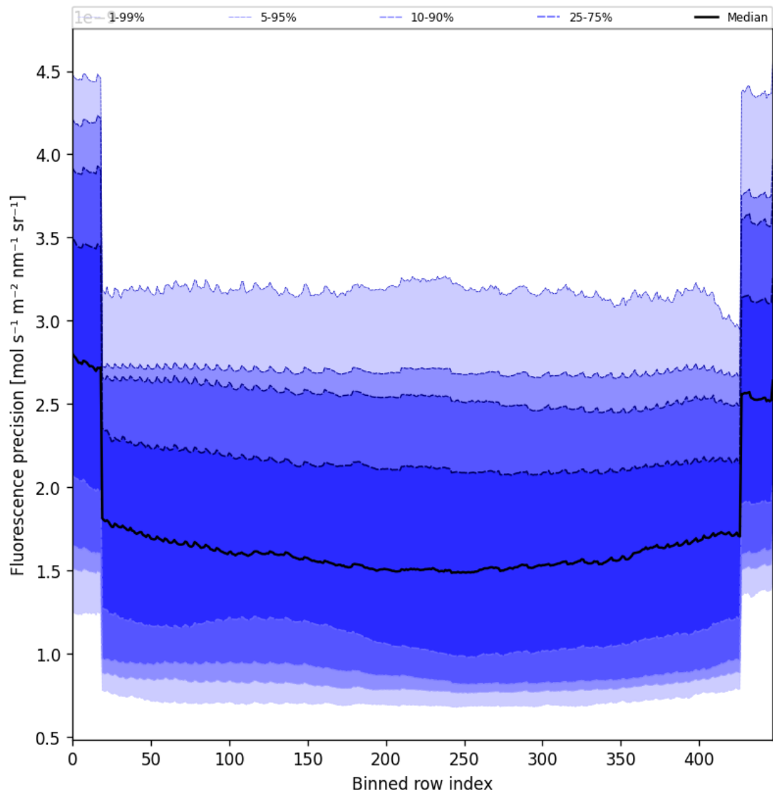
Figure 58: Along track statistics of “Fluorescence precision” for 2024-11-20 to 2024-11-22
