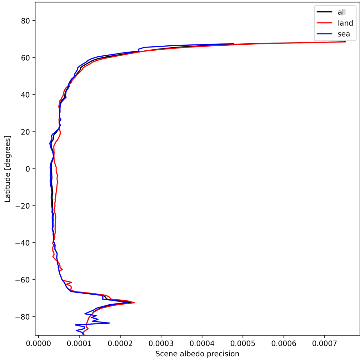
Figure 18: Zonal average of “Scene albedo precision” for 2024-11-20 to 2024-11-22.
