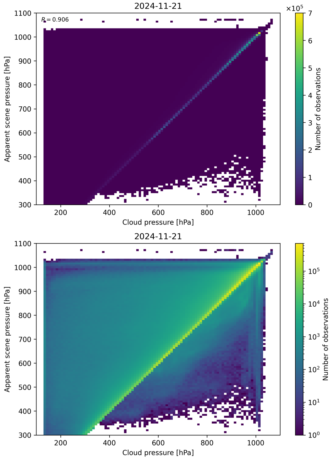
Figure 77: Scatter density plot of “Cloud pressure” against “Apparent scene pressure” for 2024-11-20 to 2024-11-22.
