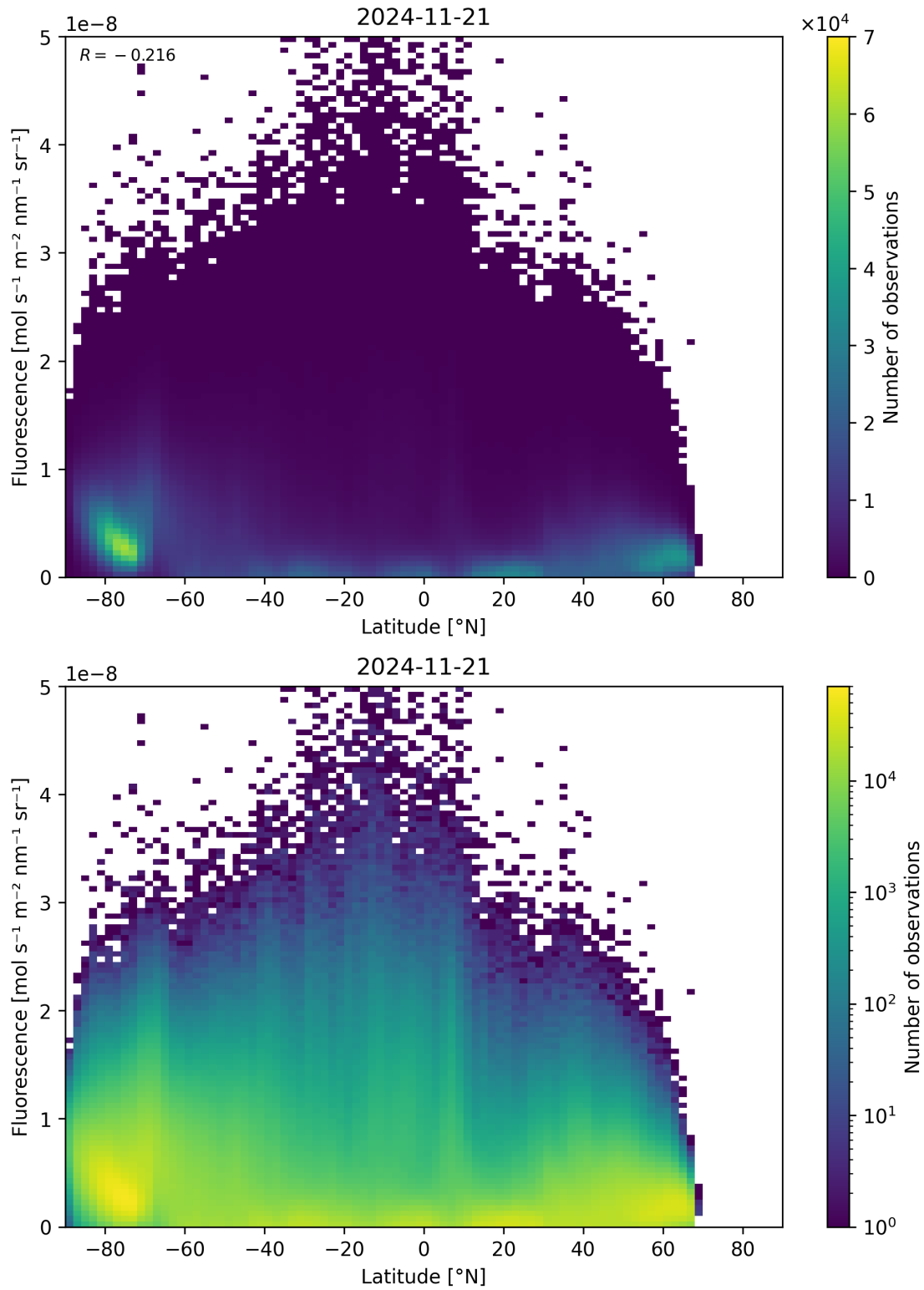
Figure 92: Scatter density plot of “Latitude” against “Fluorescence” for 2024-11-20 to 2024-11-22.
