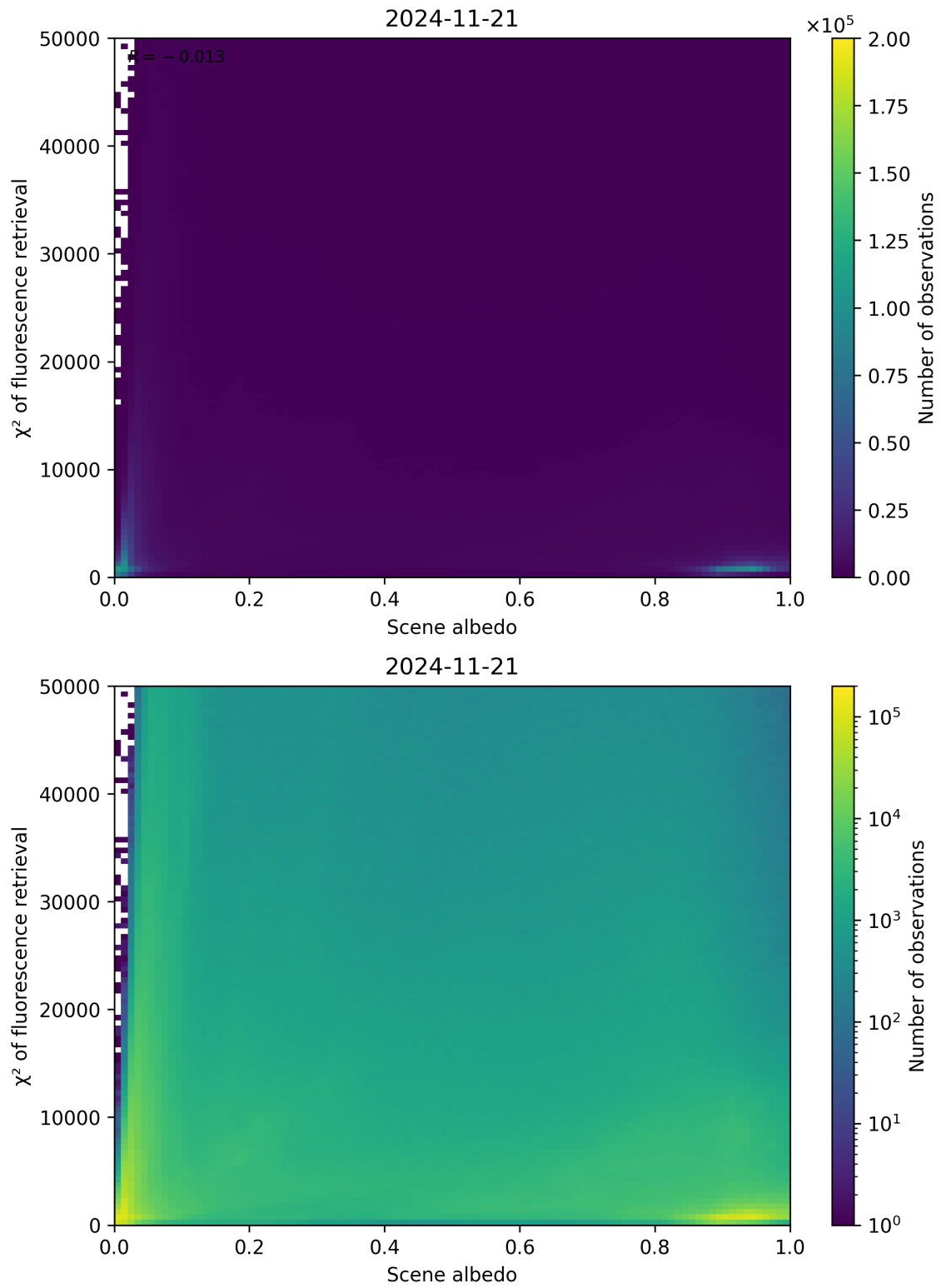
Figure 103: Scatter density plot of “Scene albedo” against “ \chi^2 of fluorescence retrieval” for 2024-11-20 to 2024-11-22.
