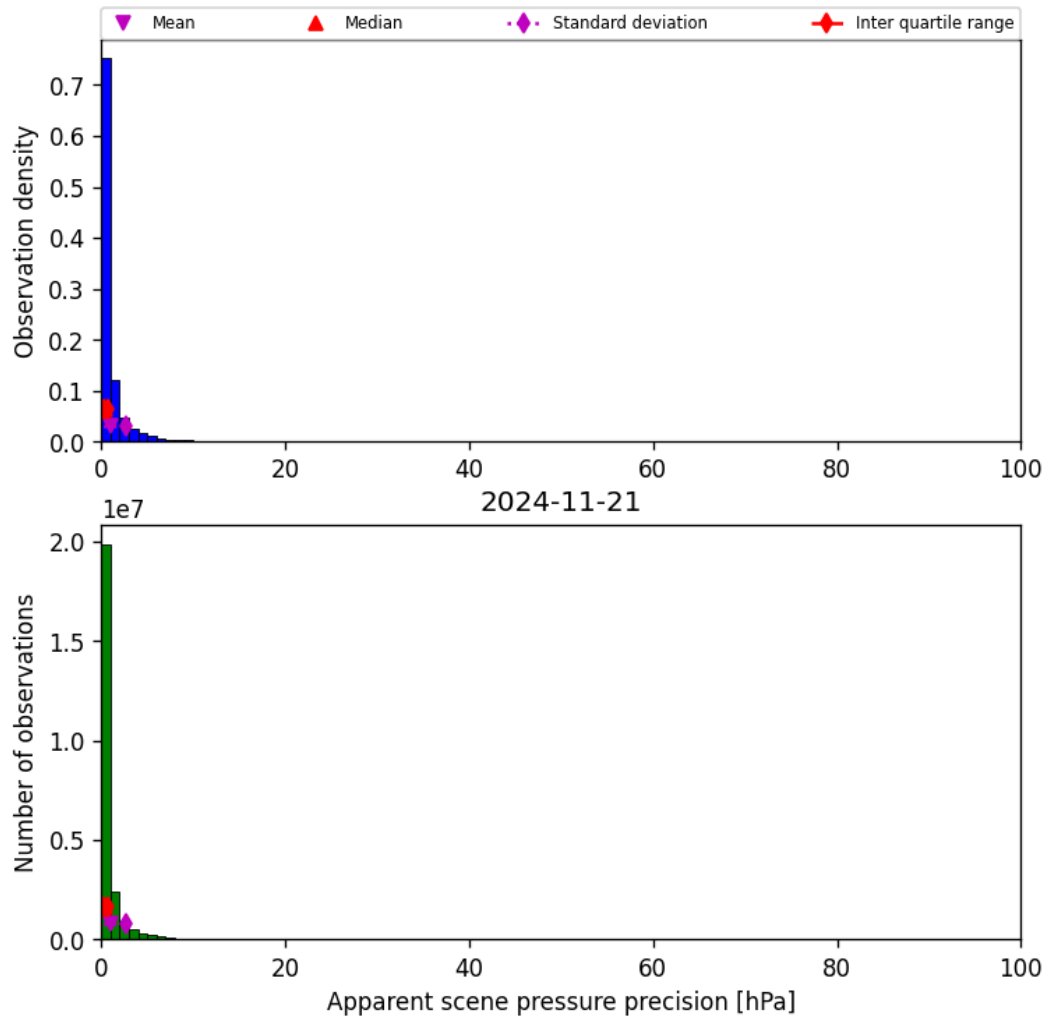
Figure 37: Histogram of “Apparent scene pressure precision” for 2024-11-20 to 2024-11-22
