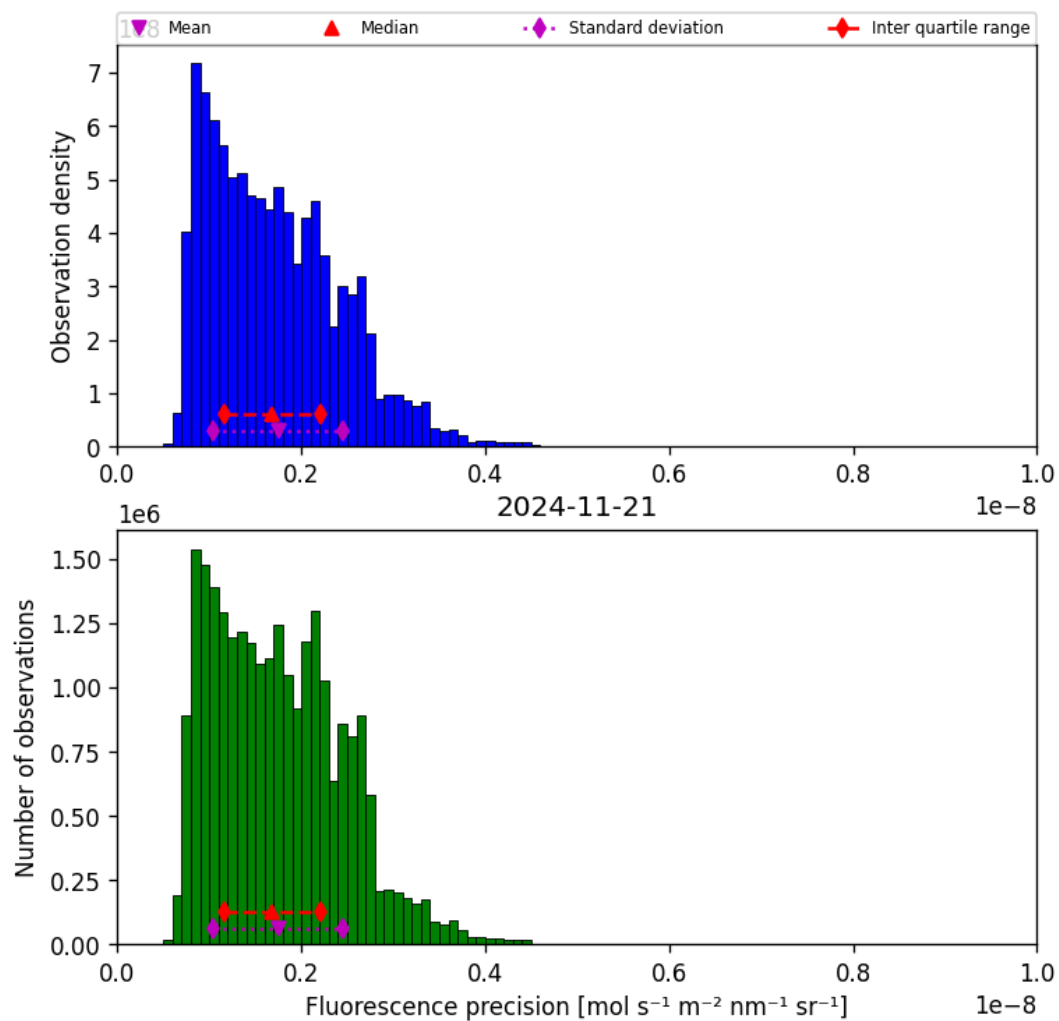
Figure 41: Histogram of “Fluorescence precision” for 2024-11-20 to 2024-11-22
