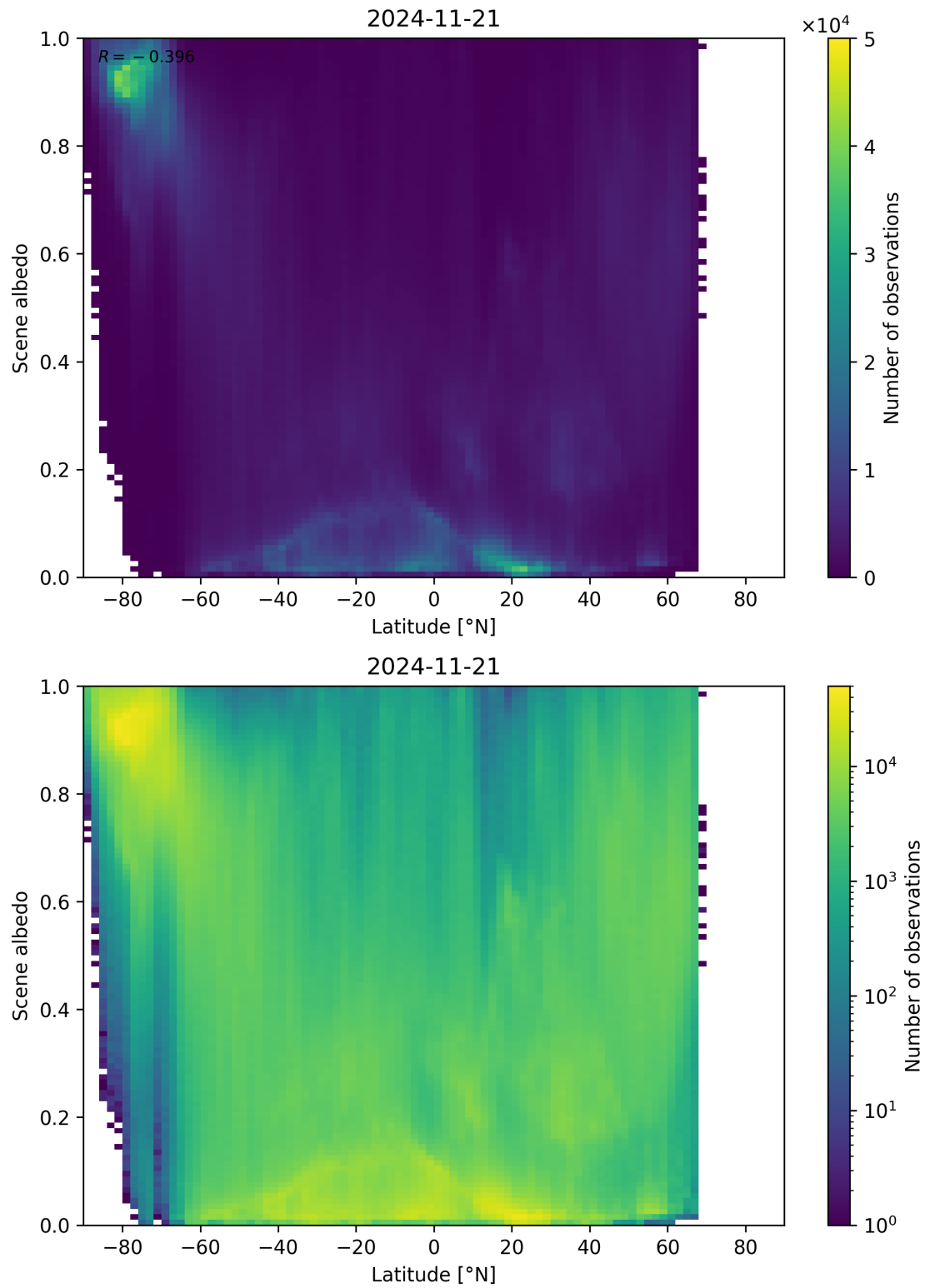
Figure 95: Scatter density plot of “Latitude” against “Scene albedo” for 2024-11-20 to 2024-11-22.
