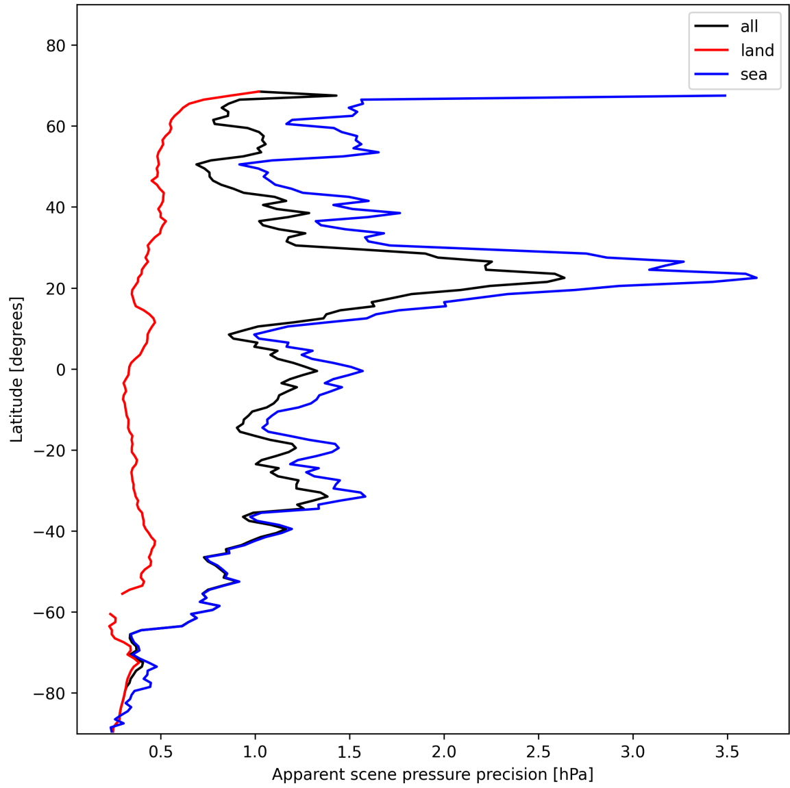
Figure 20: Zonal average of “Apparent scene pressure precision” for 2024-11-20 to 2024-11-22.
