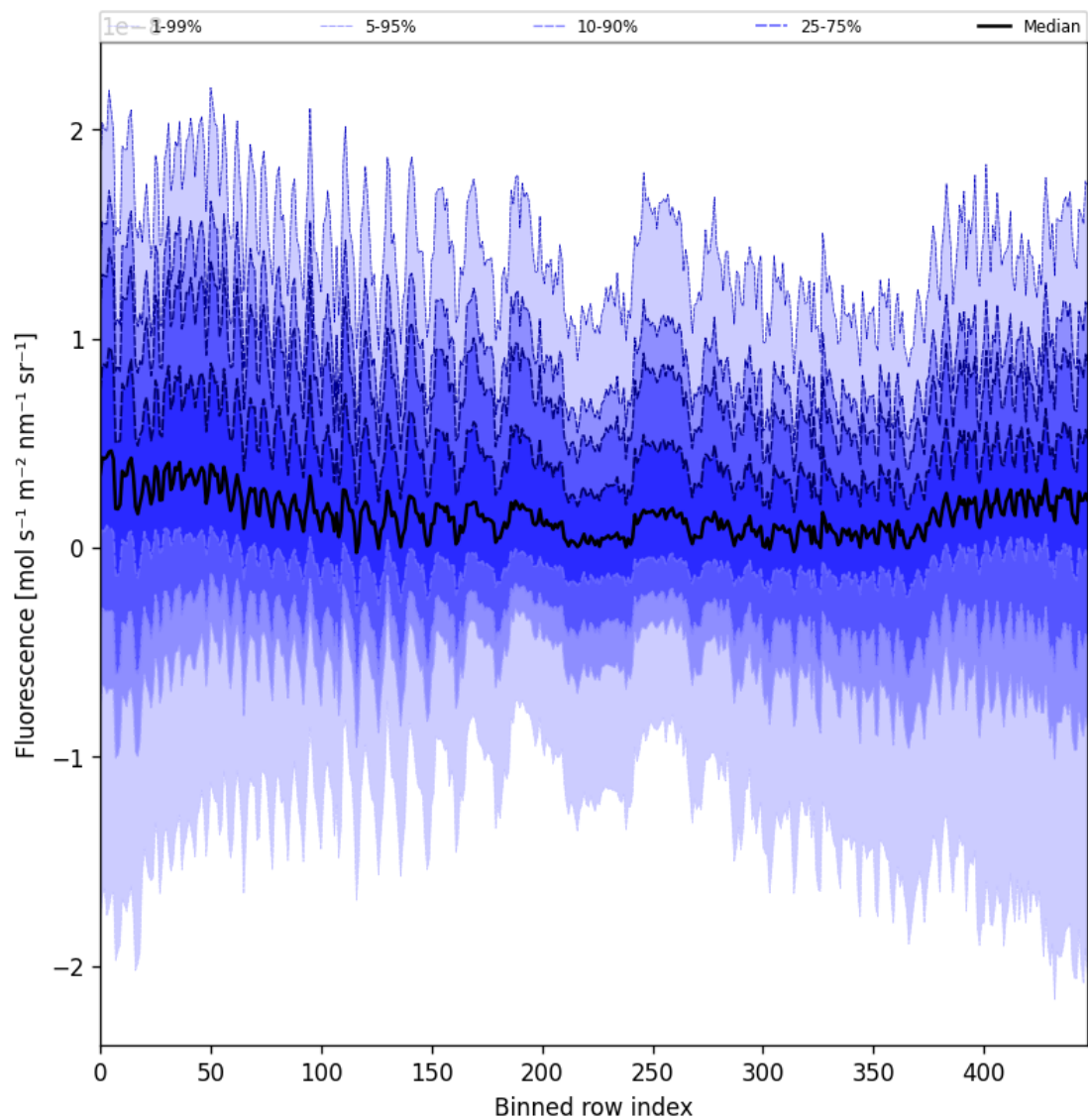
Figure 57: Along track statistics of “Fluorescence” for 2024-11-20 to 2024-11-22
