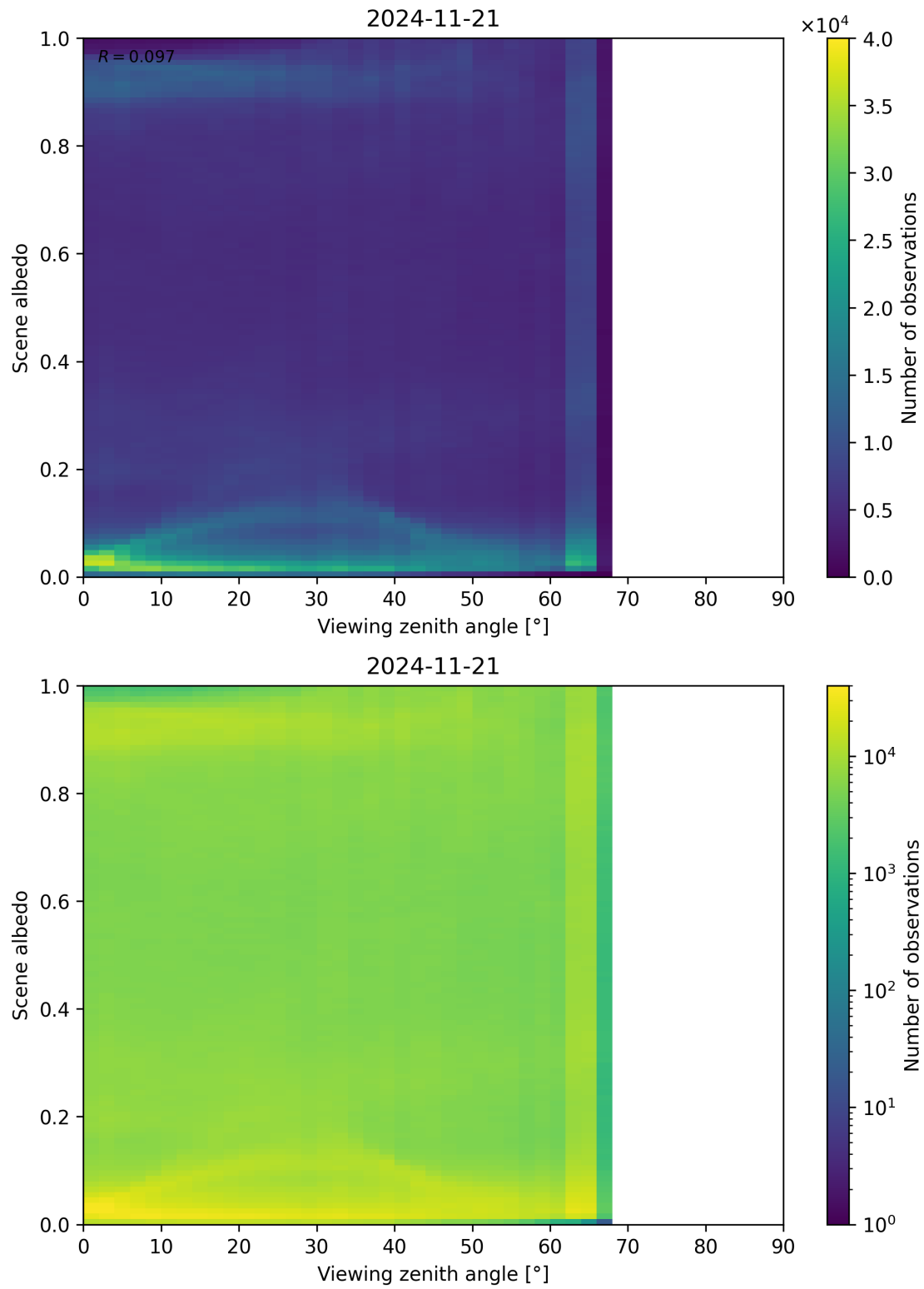
Figure 126: Scatter density plot of “Viewing zenith angle” against “Scene albedo” for 2024-11-20 to 2024-11-22.
