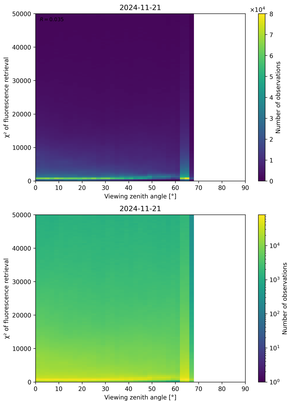
Figure 119: Scatter density plot of “Viewing zenith angle” against “ \chi^2 of fluorescence retrieval” for 2024-11-20 to 2024-11-22.
