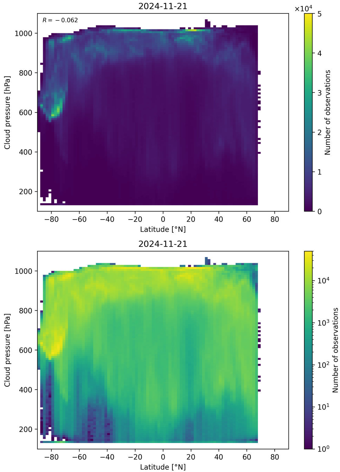
Figure 91: Scatter density plot of “Latitude” against “Cloud pressure” for 2024-11-20 to 2024-11-22.
