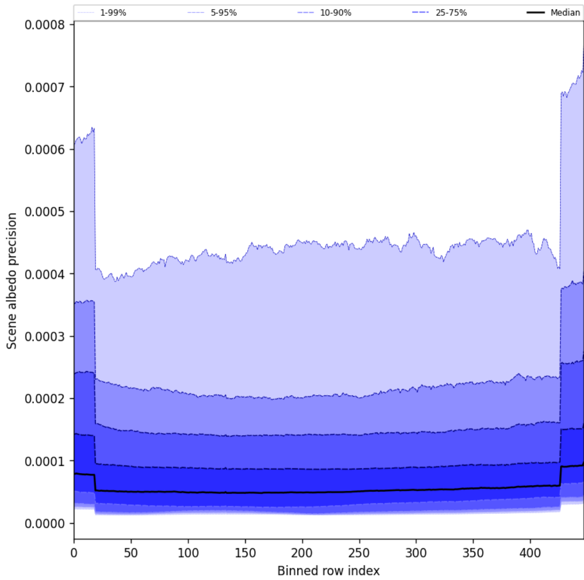
Figure 52: Along track statistics of “Scene albedo precision” for 2024-11-20 to 2024-11-22
