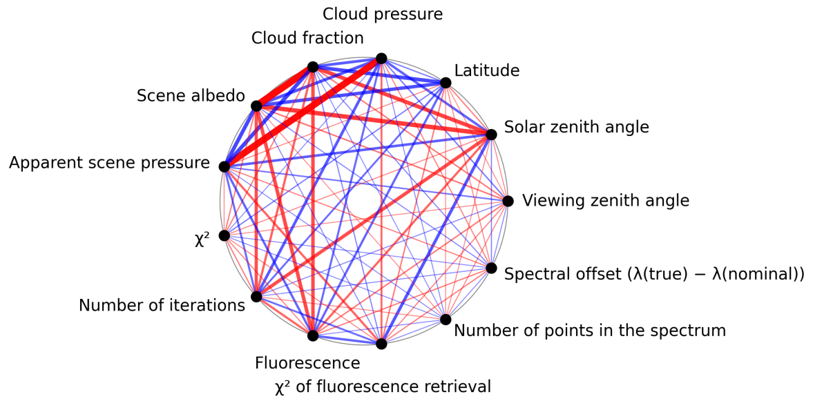
Figure 1: Map of correlation graph for 2024-11-20 to 2024-11-22.
