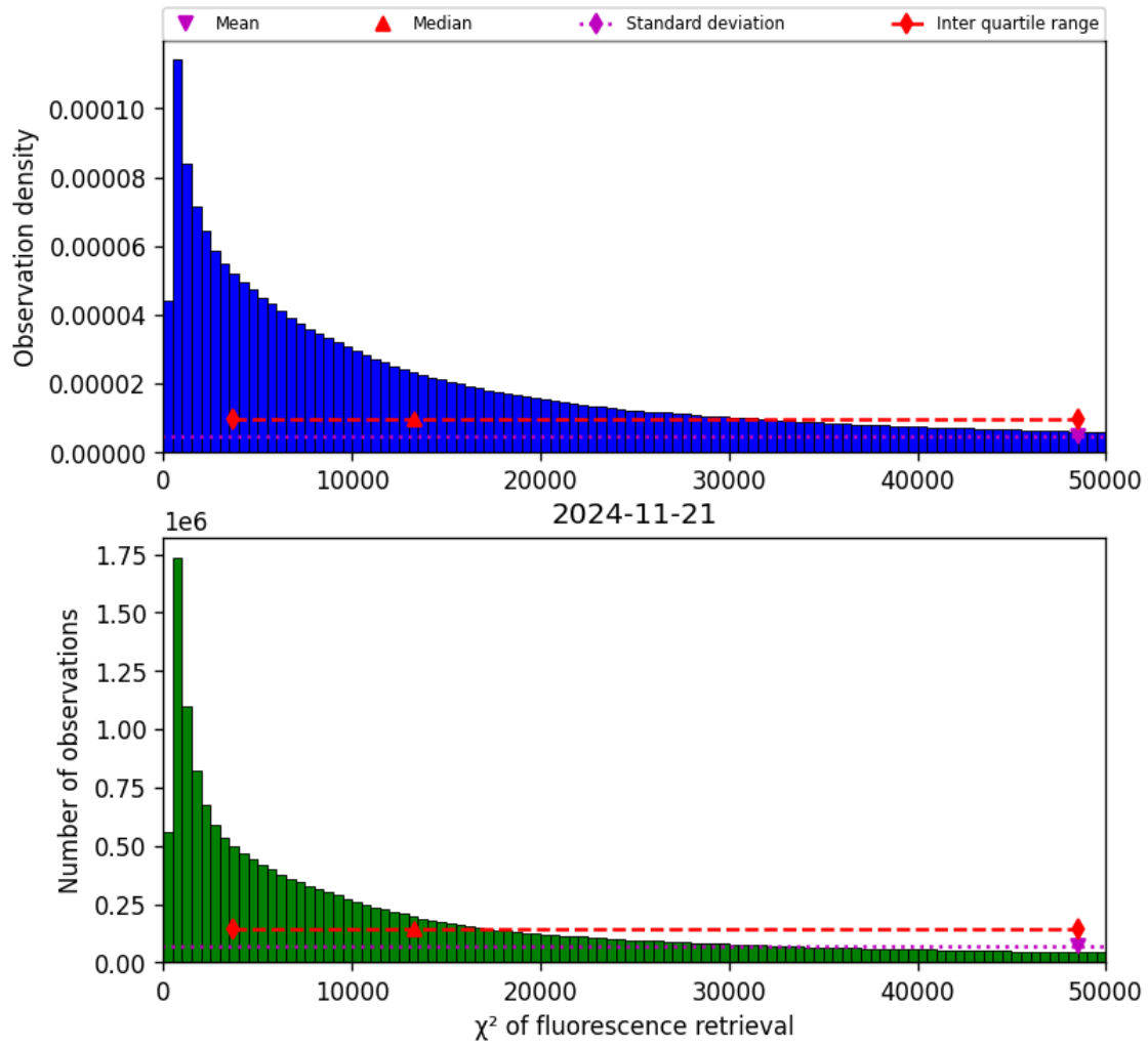
Figure 42: Histogram of “ \chi^2 of fluorescence retrieval” for 2024-11-20 to 2024-11-22
