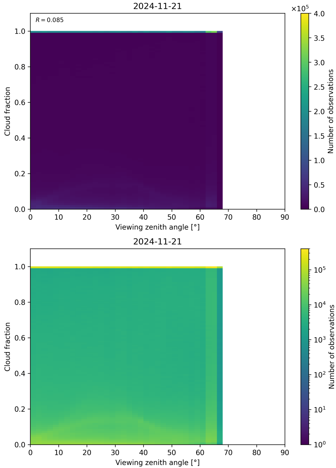
Figure 120: Scatter density plot of “Viewing zenith angle” against “Cloud fraction” for 2024-11-20 to 2024-11-22.
