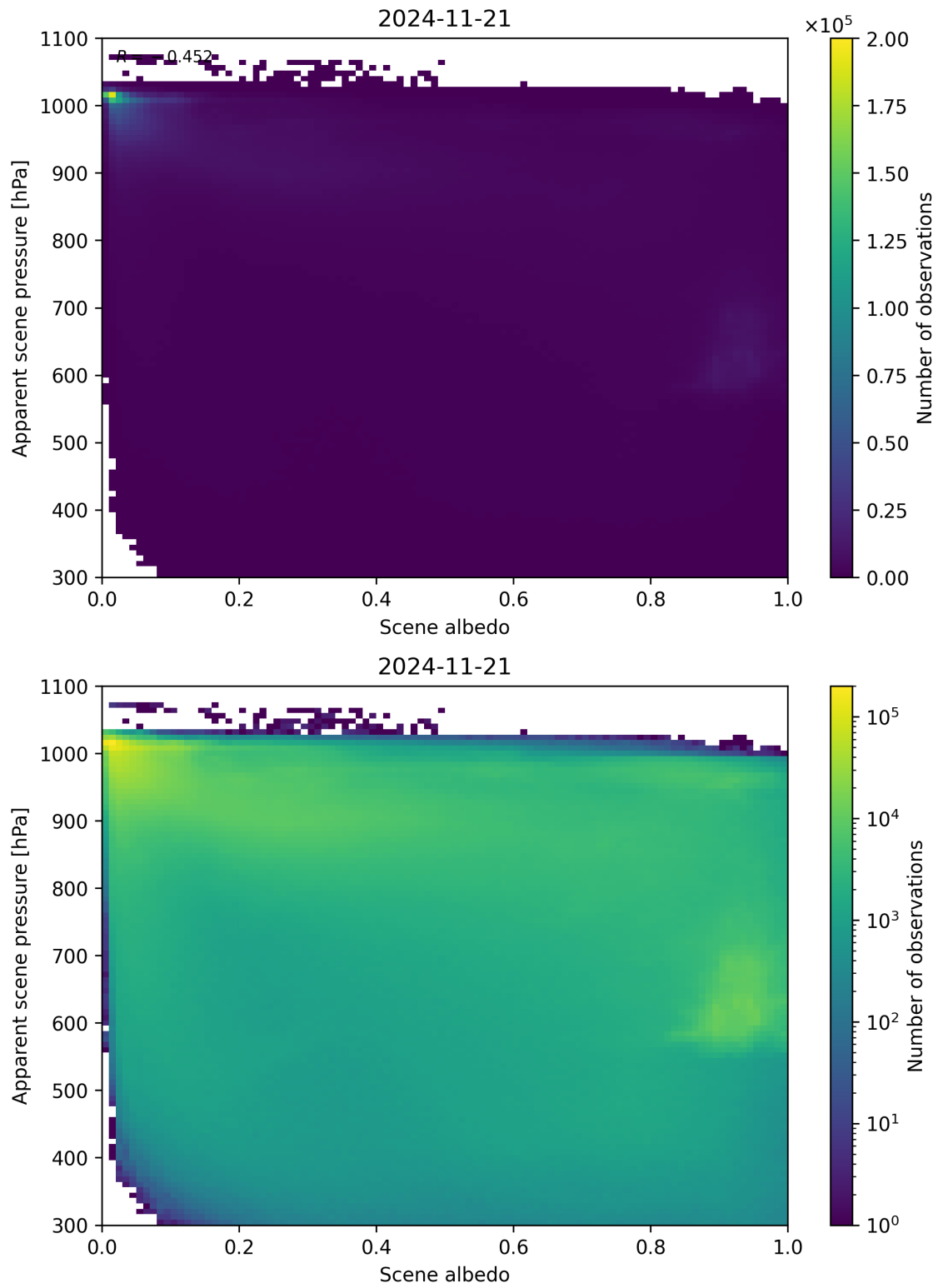
Figure 102: Scatter density plot of “Scene albedo” against “Apparent scene pressure” for 2024-11-20 to 2024-11-22.
