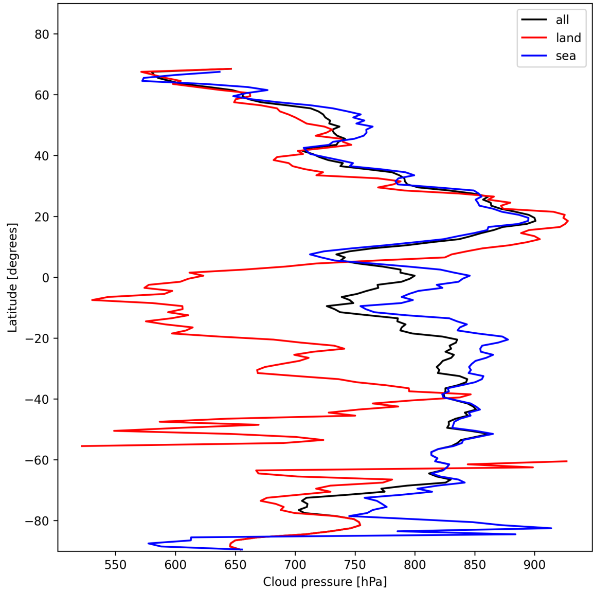
Figure 13: Zonal average of “Cloud pressure” for 2024-11-20 to 2024-11-22.
