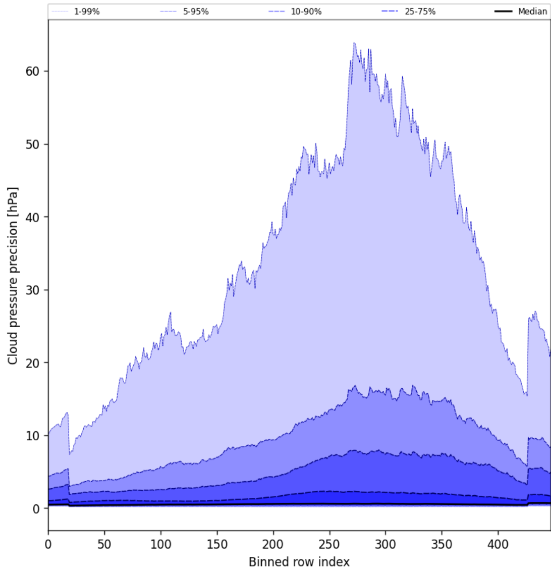
Figure 48: Along track statistics of “Cloud pressure precision” for 2024-11-20 to 2024-11-22
