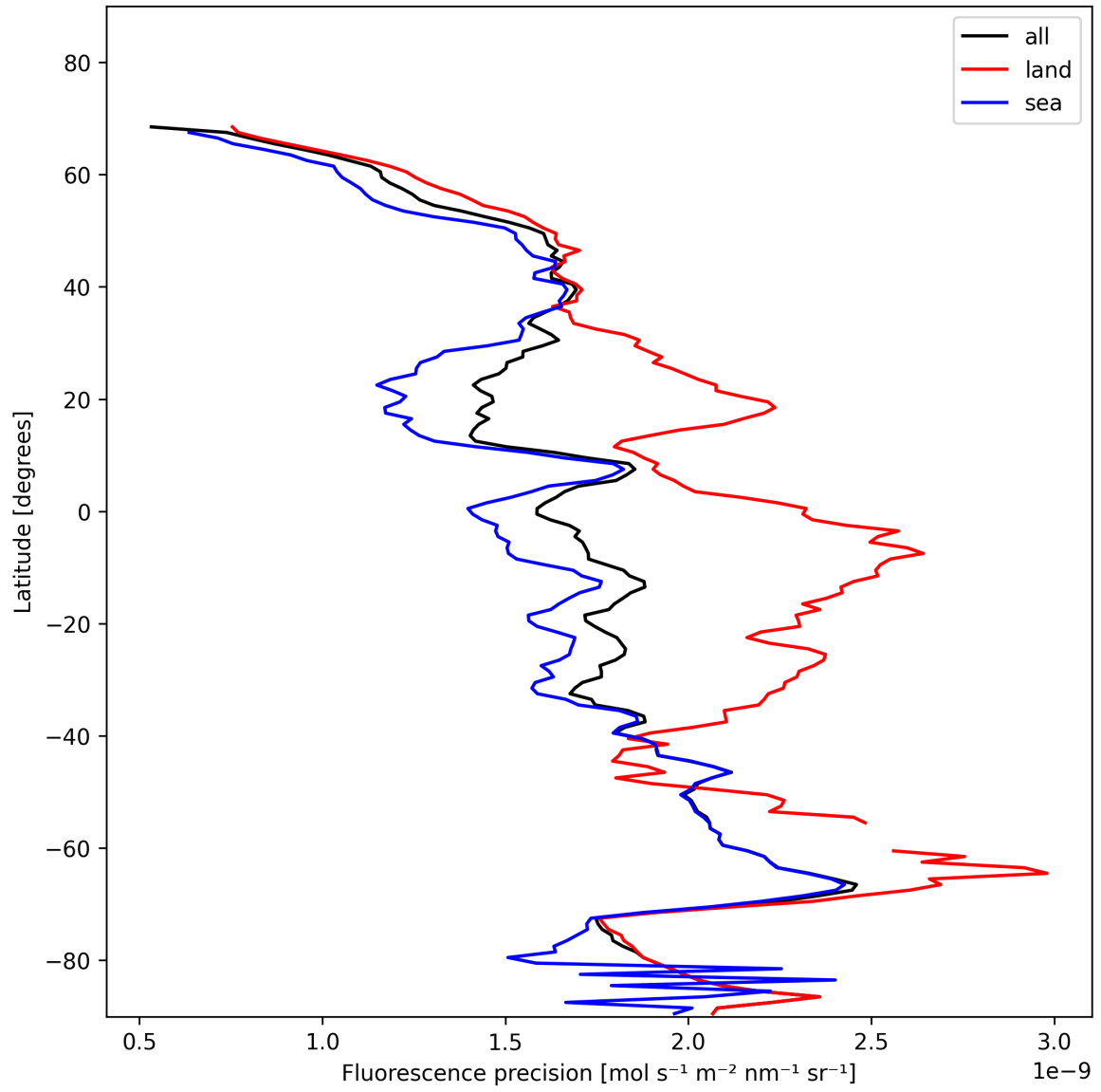
Figure 24: Zonal average of “Fluorescence precision” for 2024-11-20 to 2024-11-22.
