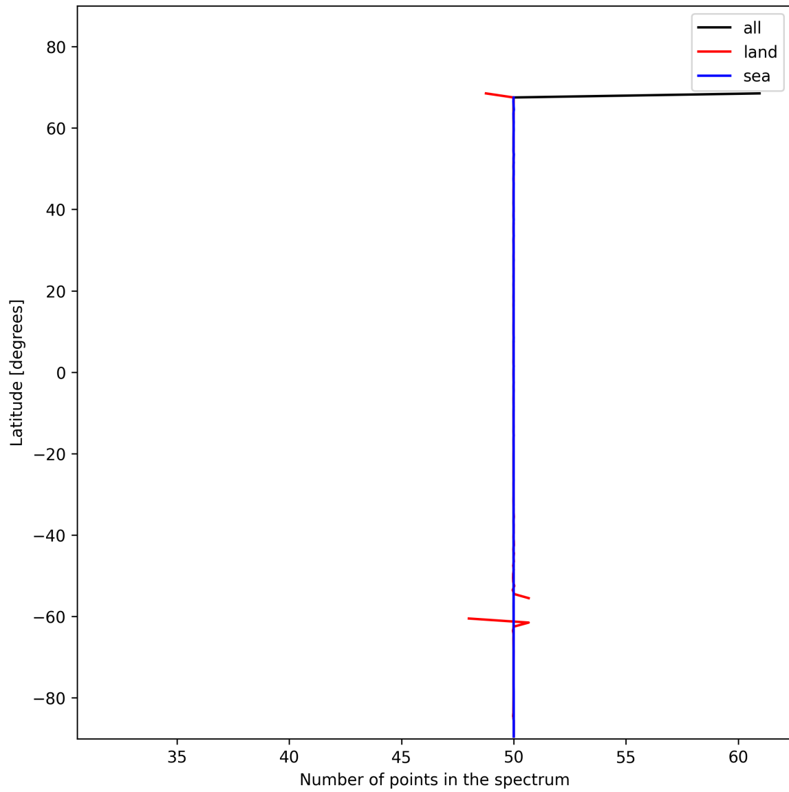
Figure 27: Zonal average of “Number of points in the spectrum” for 2024-11-20 to 2024-11-22.
