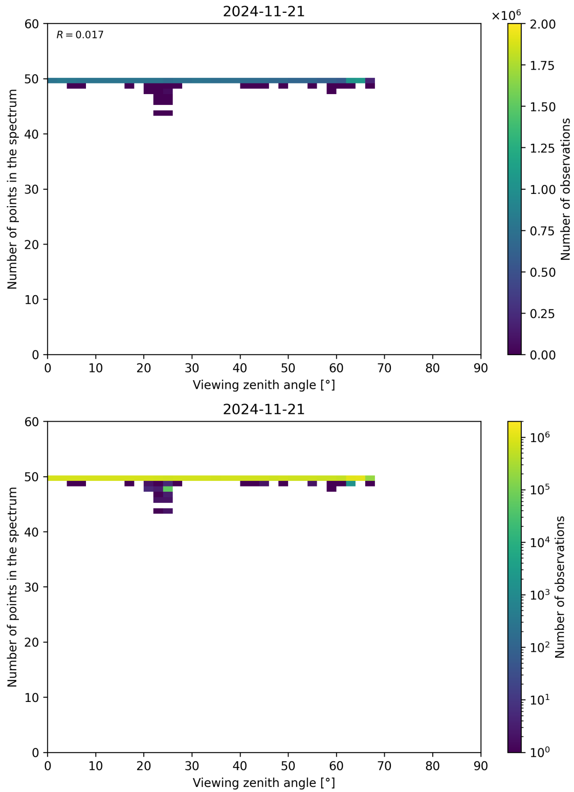
Figure 125: Scatter density plot of “Viewing zenith angle” against “Number of points in the spectrum” for 2024-11-20 to 2024-11-22.
