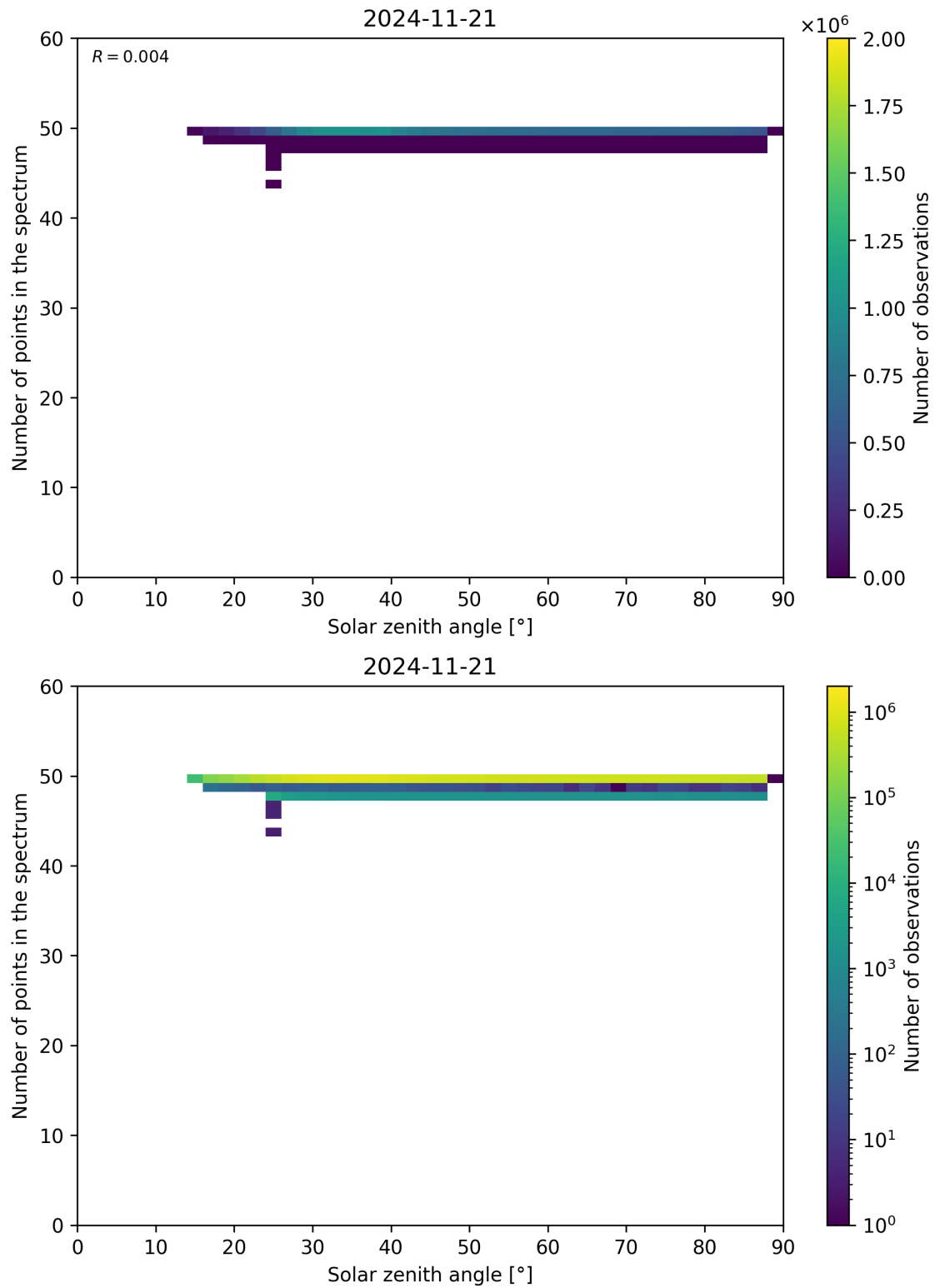
Figure 115: Scatter density plot of “Solar zenith angle” against “Number of points in the spectrum” for 2024-11-20 to 2024-11-22.
