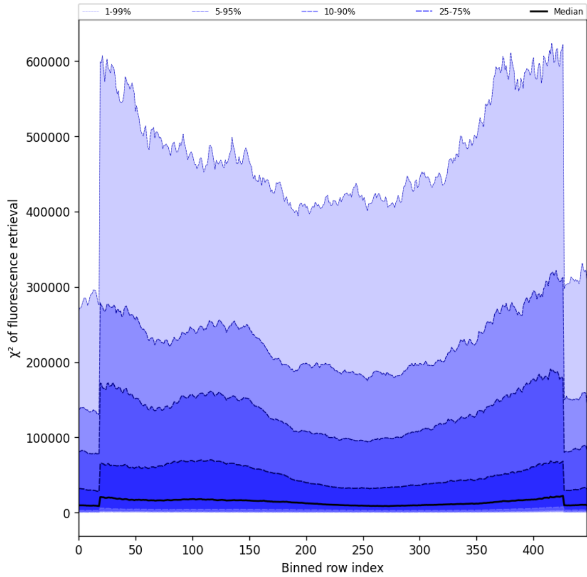
Figure 59: Along track statistics of “ \chi^2 of fluorescence retrieval” for 2024-11-20 to 2024-11-22
