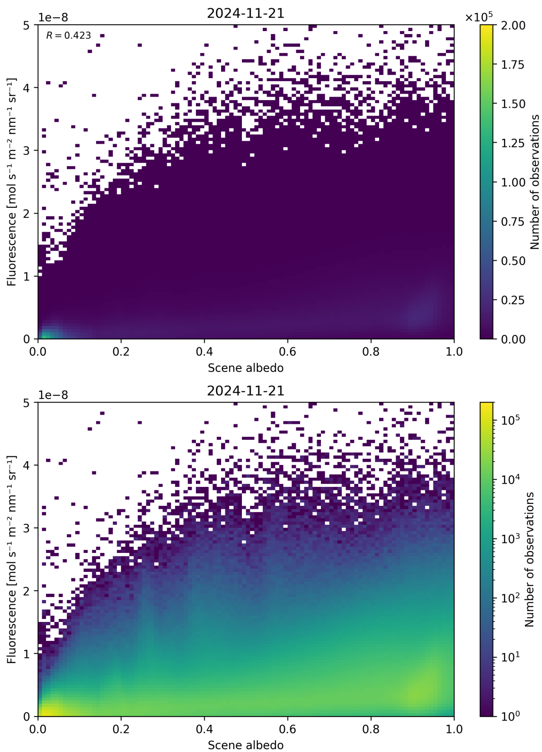
Figure 104: Scatter density plot of “Scene albedo” against “Fluorescence” for 2024-11-20 to 2024-11-22.
