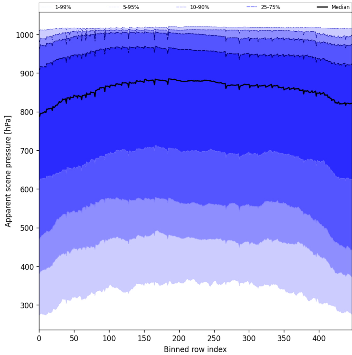
Figure 53: Along track statistics of “Apparent scene pressure” for 2024-11-20 to 2024-11-22
