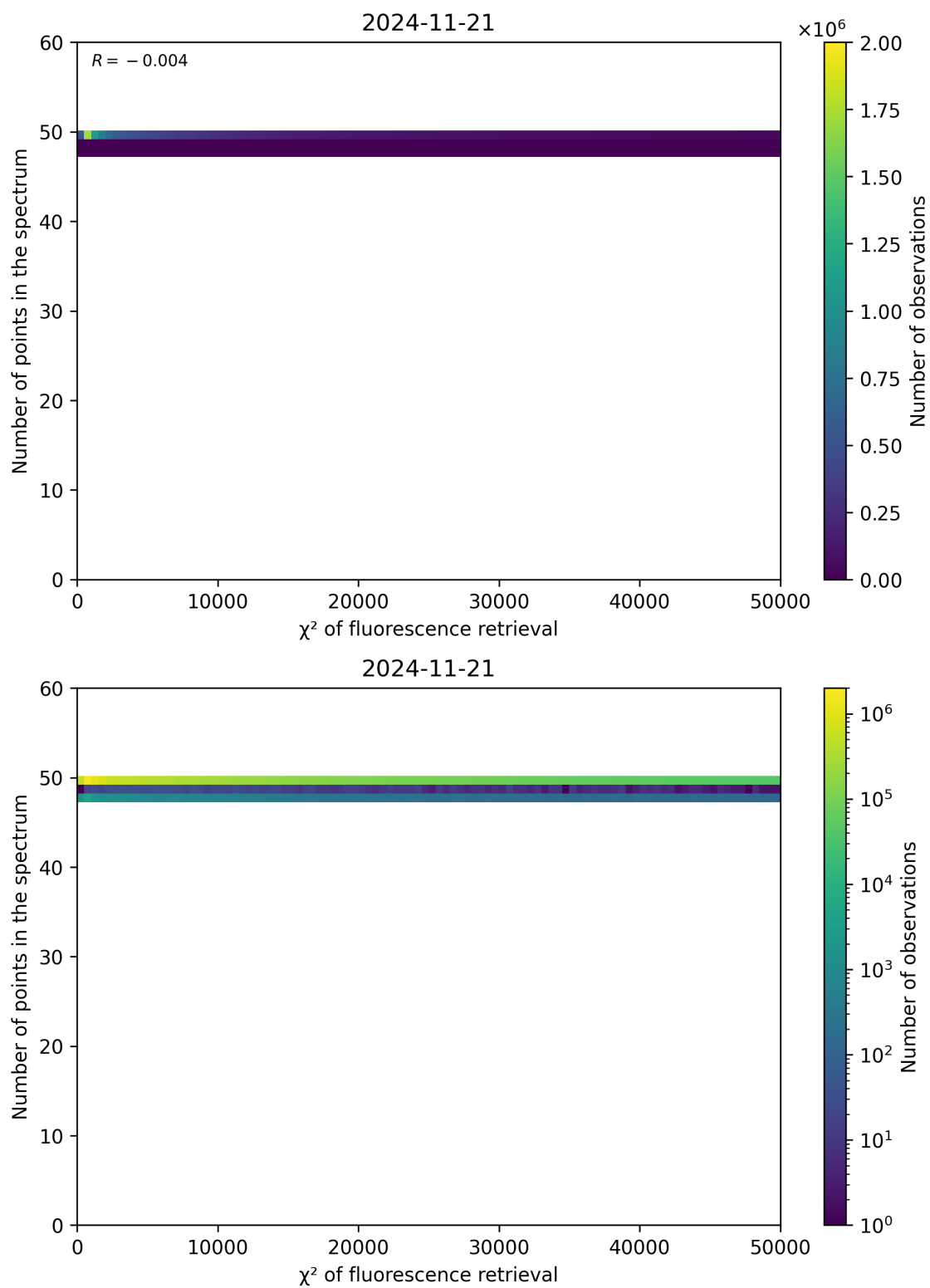
Figure 68: Scatter density plot of “ \chi^2 of fluorescence retrieval” against “Number of points in the spectrum” for 2024-11-20 to 2024-11-22.
