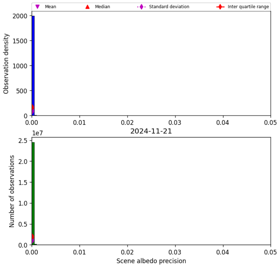
Figure 35: Histogram of “Scene albedo precision” for 2024-11-20 to 2024-11-22
