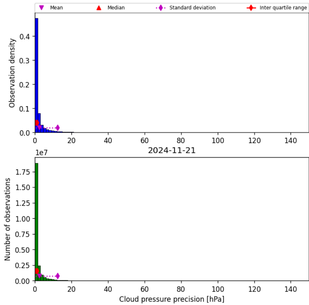
Figure 31: Histogram of “Cloud pressure precision” for 2024-11-20 to 2024-11-22
