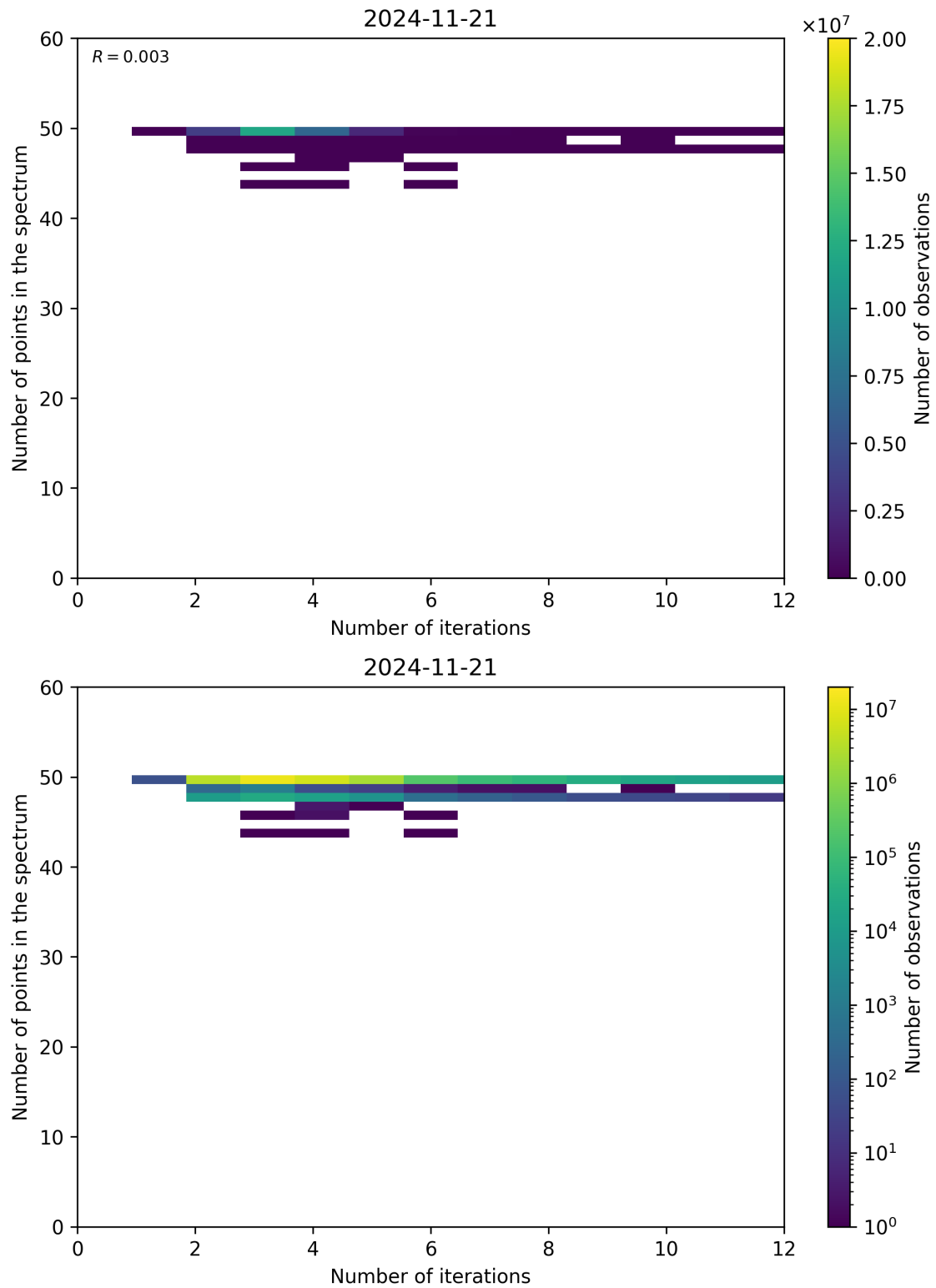
Figure 99: Scatter density plot of “Number of iterations” against “Number of points in the spectrum” for 2024-11-20 to 2024-11-22.
