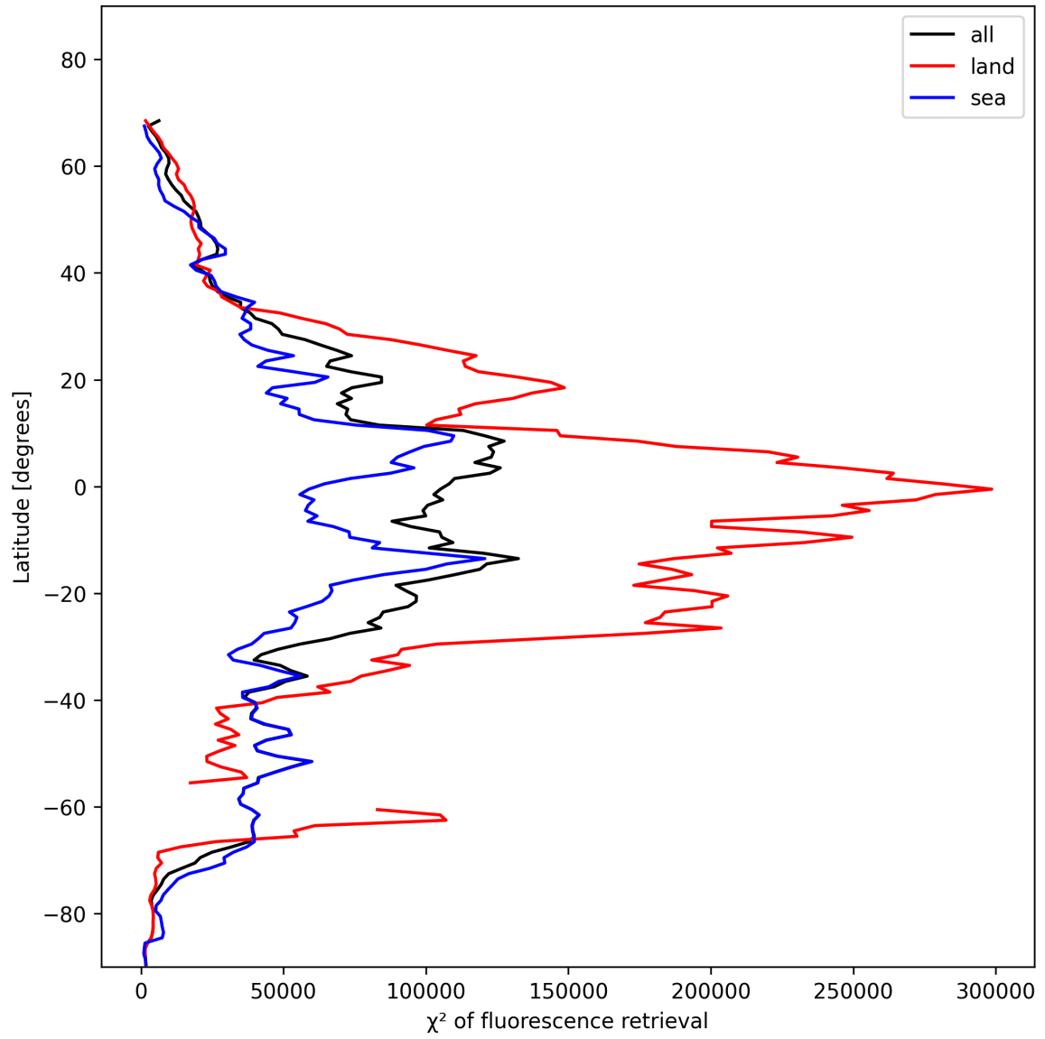
Figure 25: Zonal average of “ \chi^2 of fluorescence retrieval” for 2024-11-20 to 2024-11-22.
