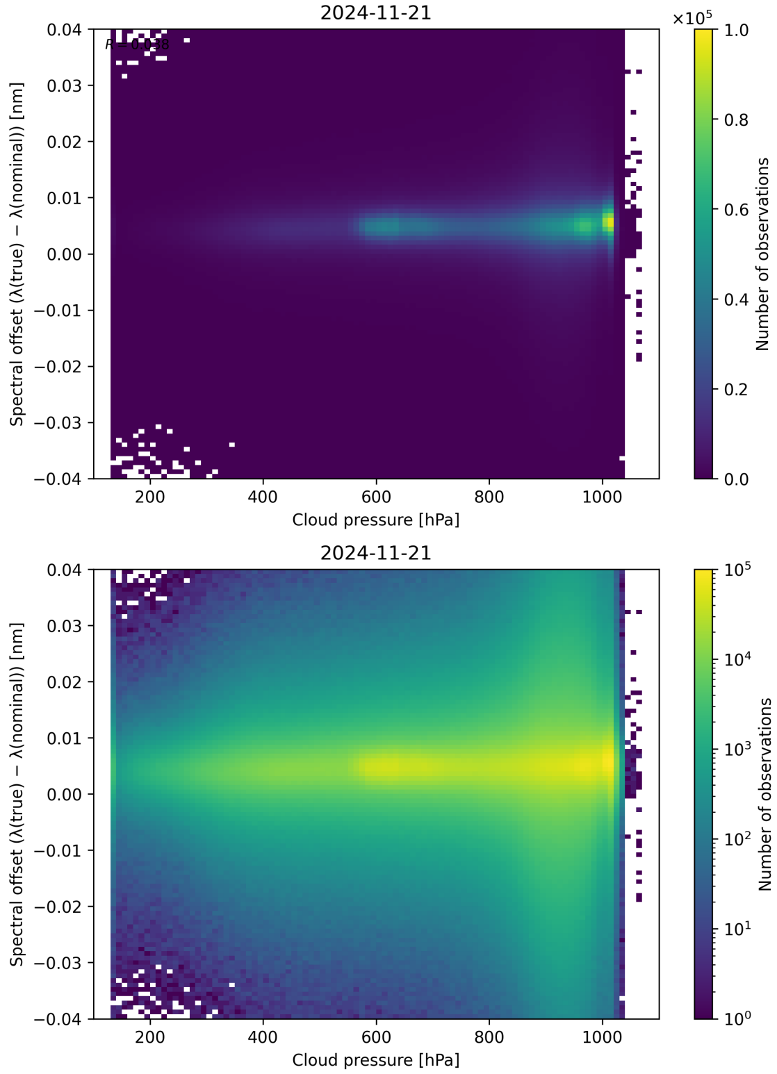
Figure 84: Scatter density plot of “Cloud pressure” against “Spectral offset ( \lambda_{\text{true}} - \lambda_{\text{nominal}} )” for 2024-11-20 to 2024-11-22.
