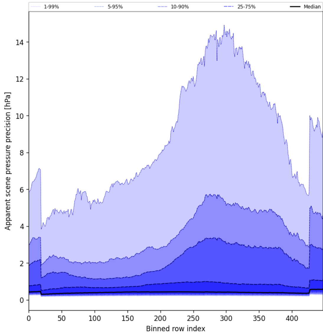
Figure 54: Along track statistics of “Apparent scene pressure precision” for 2024-11-22 to 2024-11-24
