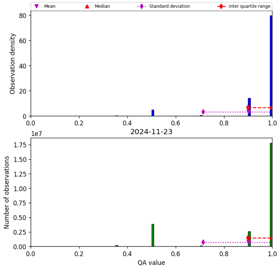
Figure 29: Histogram of “QA value” for 2024-11-22 to 2024-11-24
