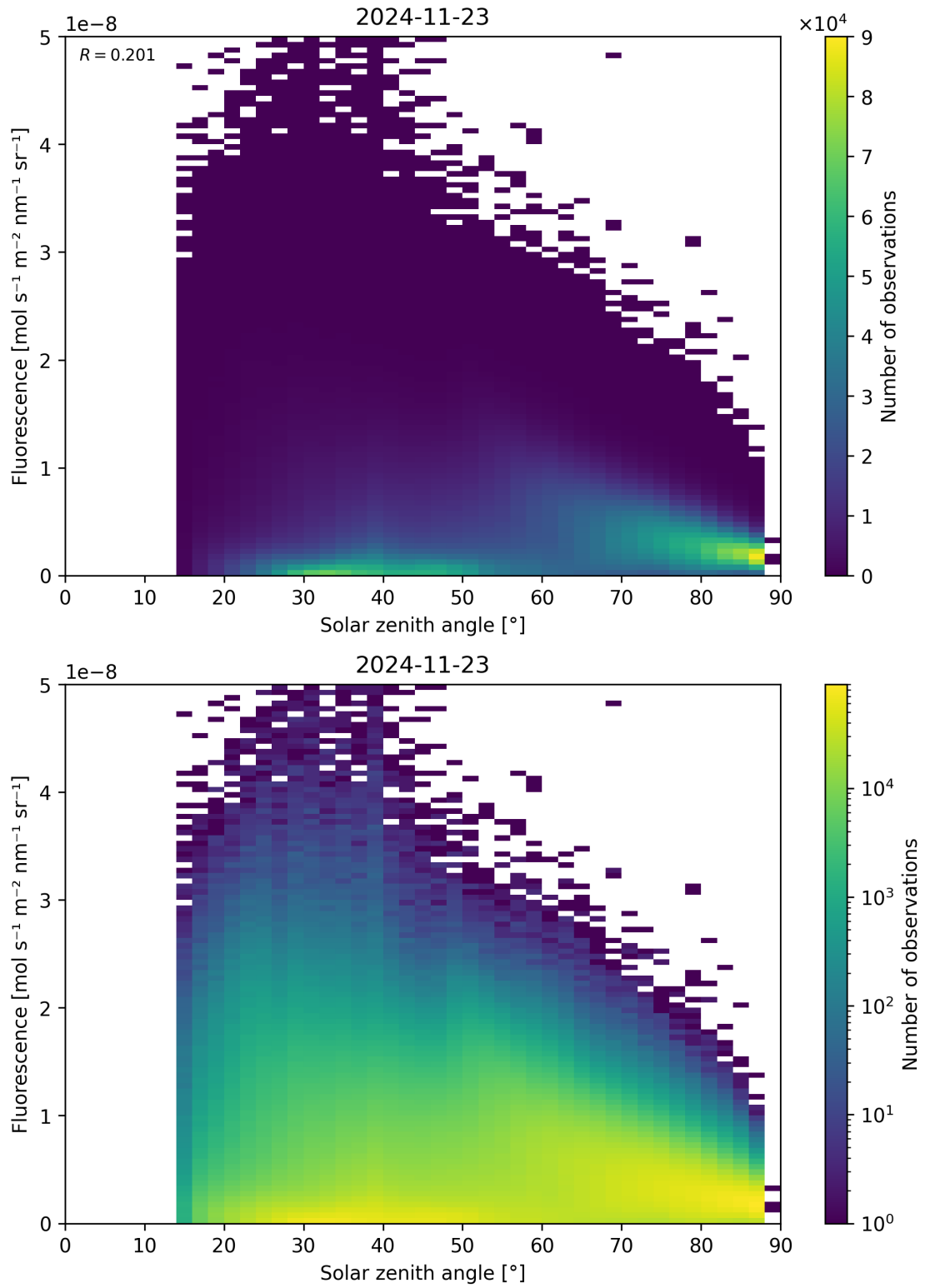
Figure 112: Scatter density plot of “Solar zenith angle” against “Fluorescence” for 2024-11-22 to 2024-11-24.
