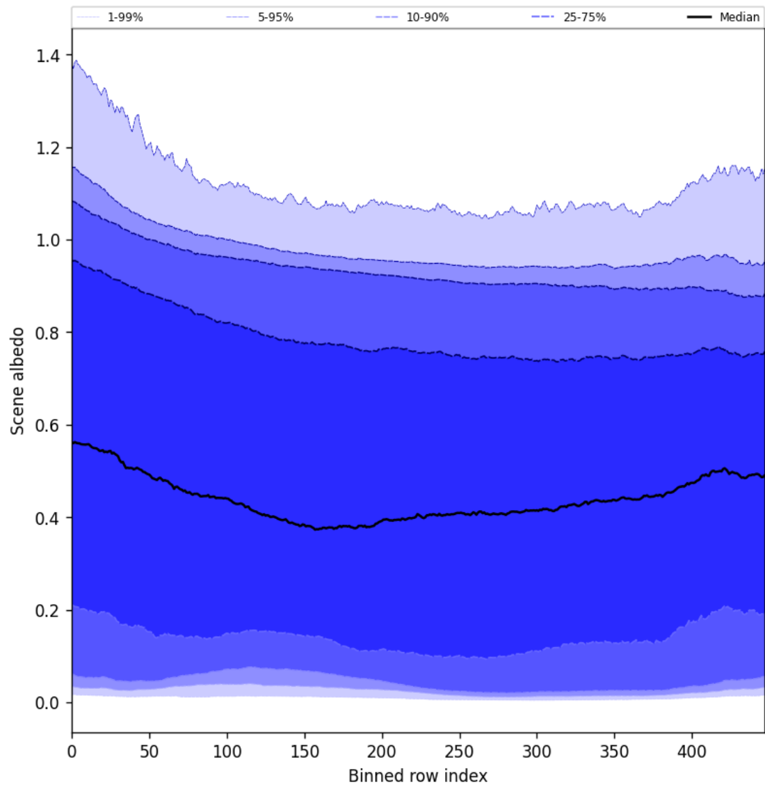
Figure 51: Along track statistics of “Scene albedo” for 2024-11-22 to 2024-11-24
