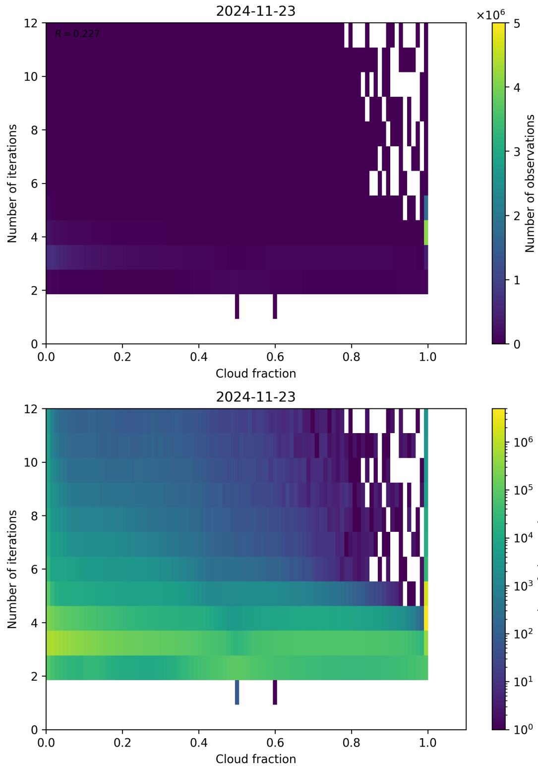
Figure 73: Scatter density plot of “Cloud fraction” against “Number of iterations” for 2024-11-22 to 2024-11-24.
