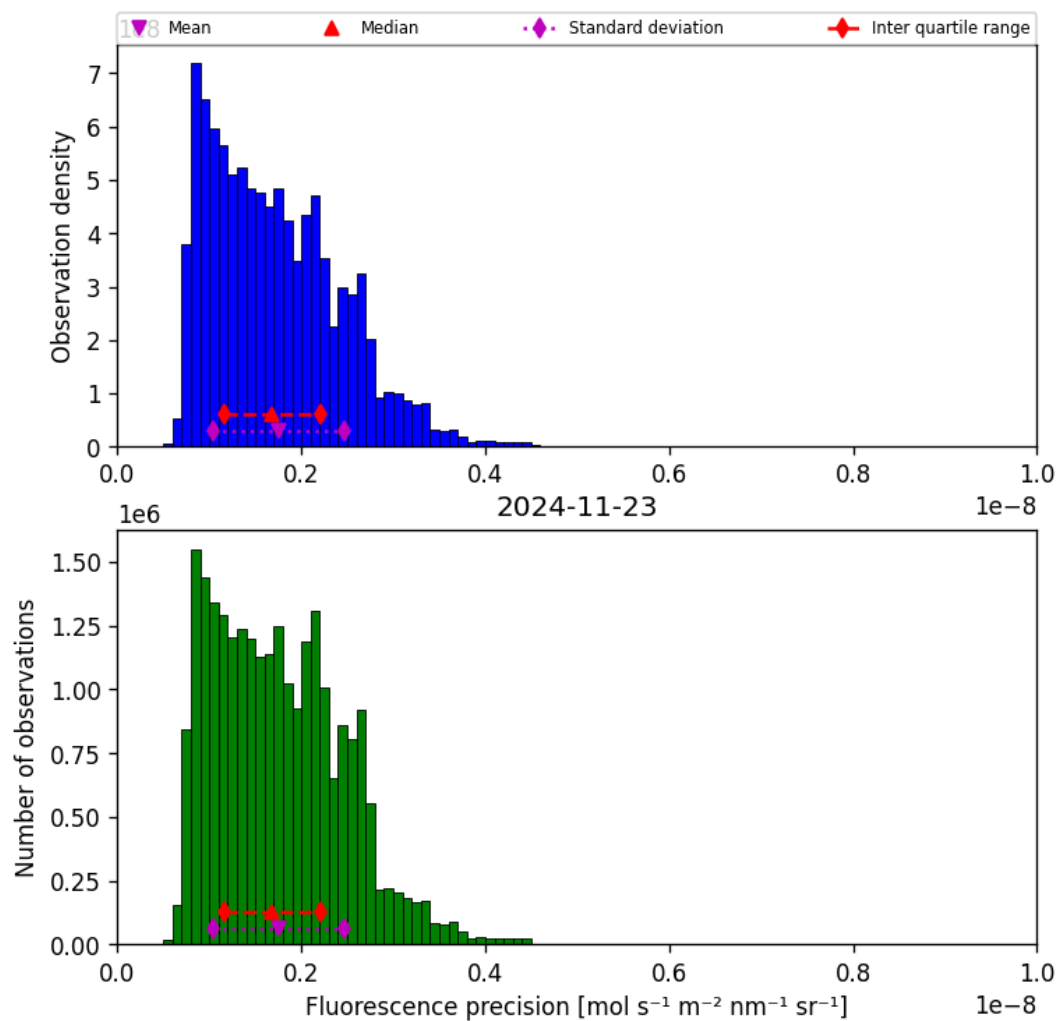
Figure 41: Histogram of “Fluorescence precision” for 2024-11-22 to 2024-11-24
