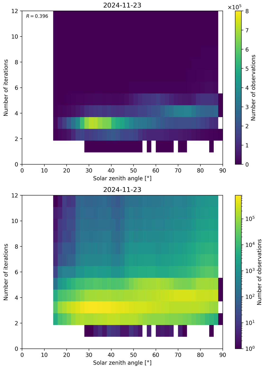
Figure 114: Scatter density plot of “Solar zenith angle” against “Number of iterations” for 2024-11-22 to 2024-11-24.
