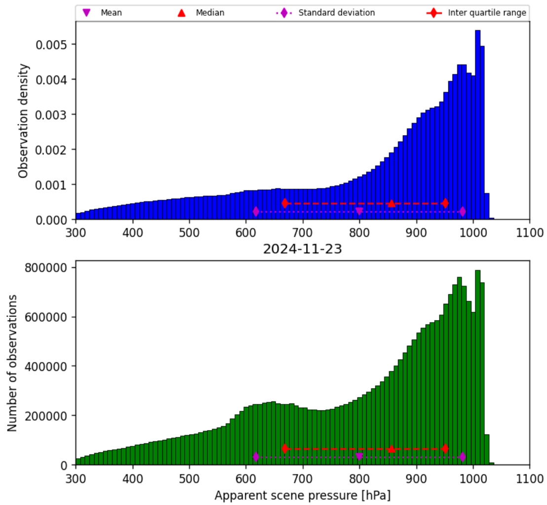
Figure 36: Histogram of “Apparent scene pressure” for 2024-11-22 to 2024-11-24
