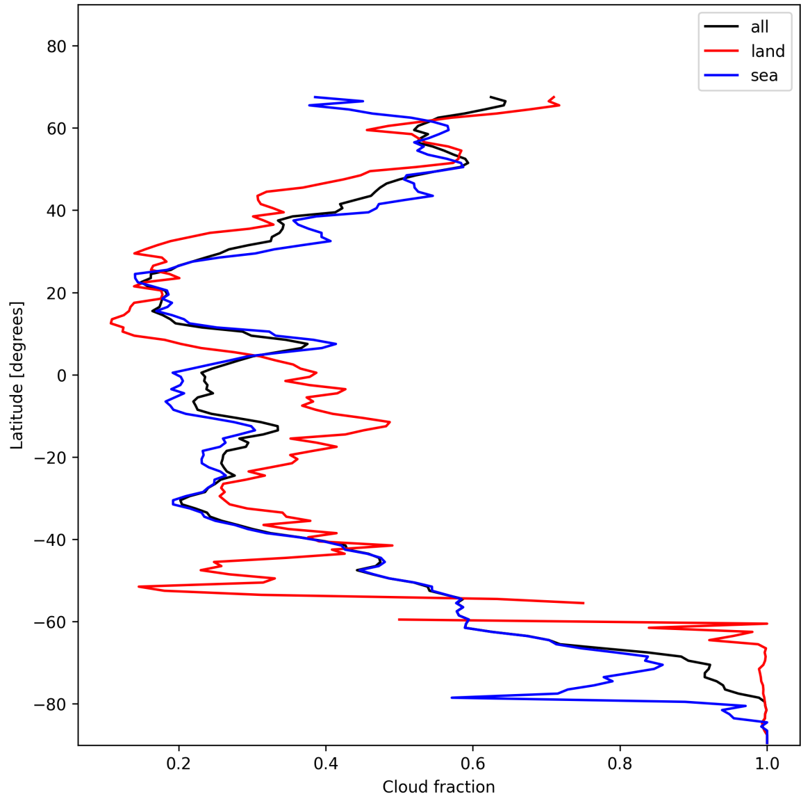
Figure 15: Zonal average of “Cloud fraction” for 2024-11-22 to 2024-11-24.
