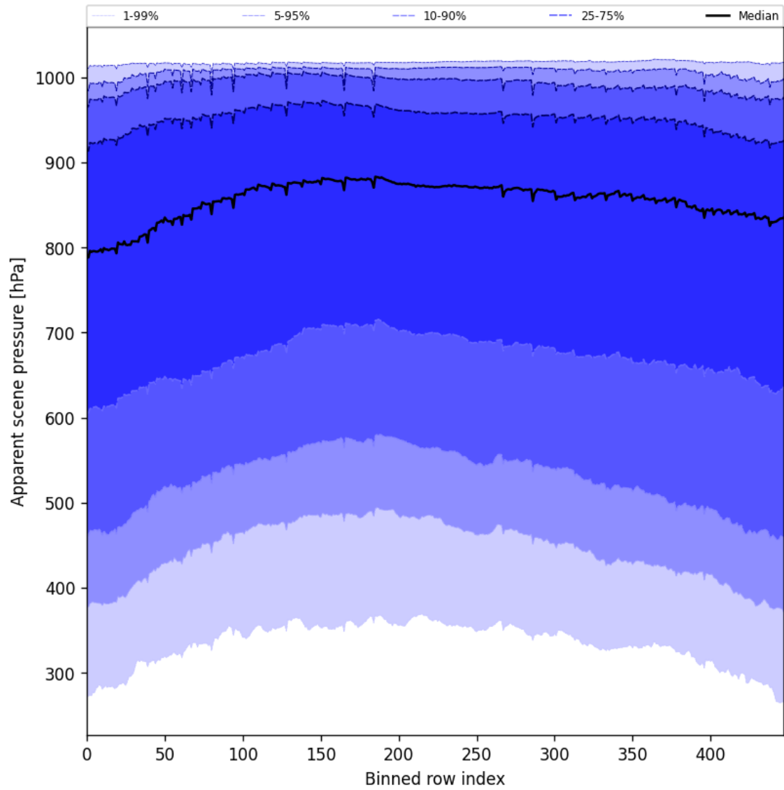
Figure 53: Along track statistics of “Apparent scene pressure” for 2024-11-22 to 2024-11-24
