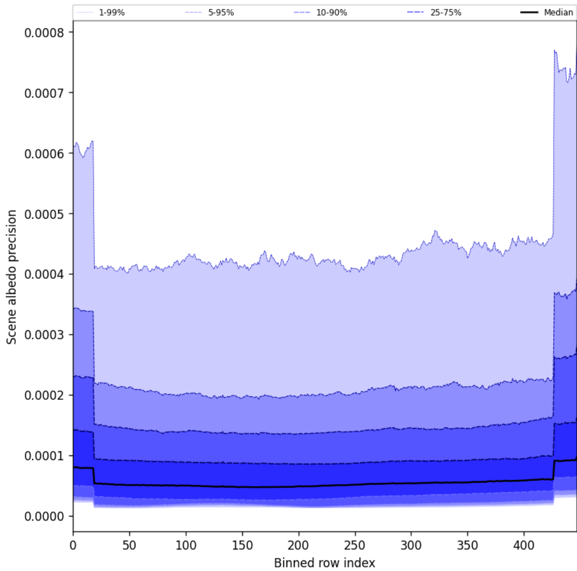
Figure 52: Along track statistics of “Scene albedo precision” for 2024-11-22 to 2024-11-24
