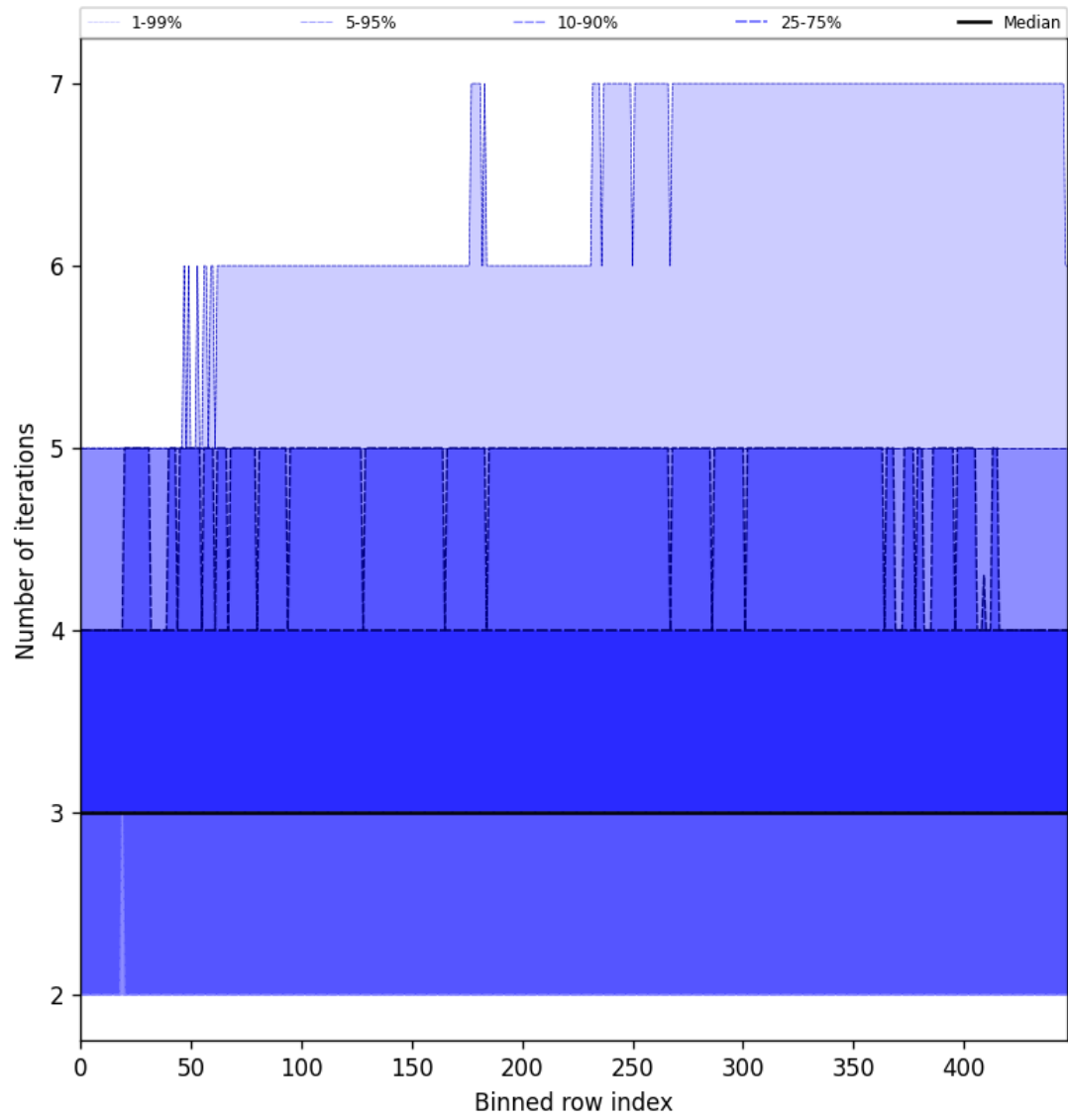
Figure 56: Along track statistics of “Number of iterations” for 2024-11-22 to 2024-11-24
