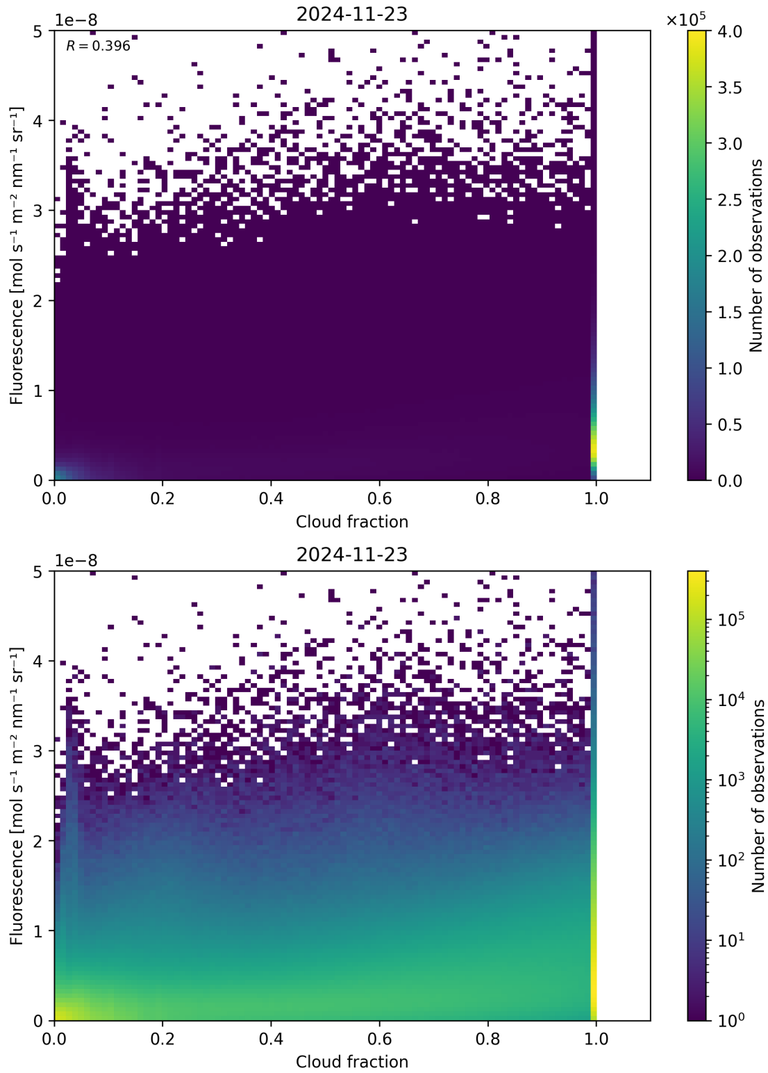
Figure 72: Scatter density plot of “Cloud fraction” against “Fluorescence” for 2024-11-22 to 2024-11-24.
