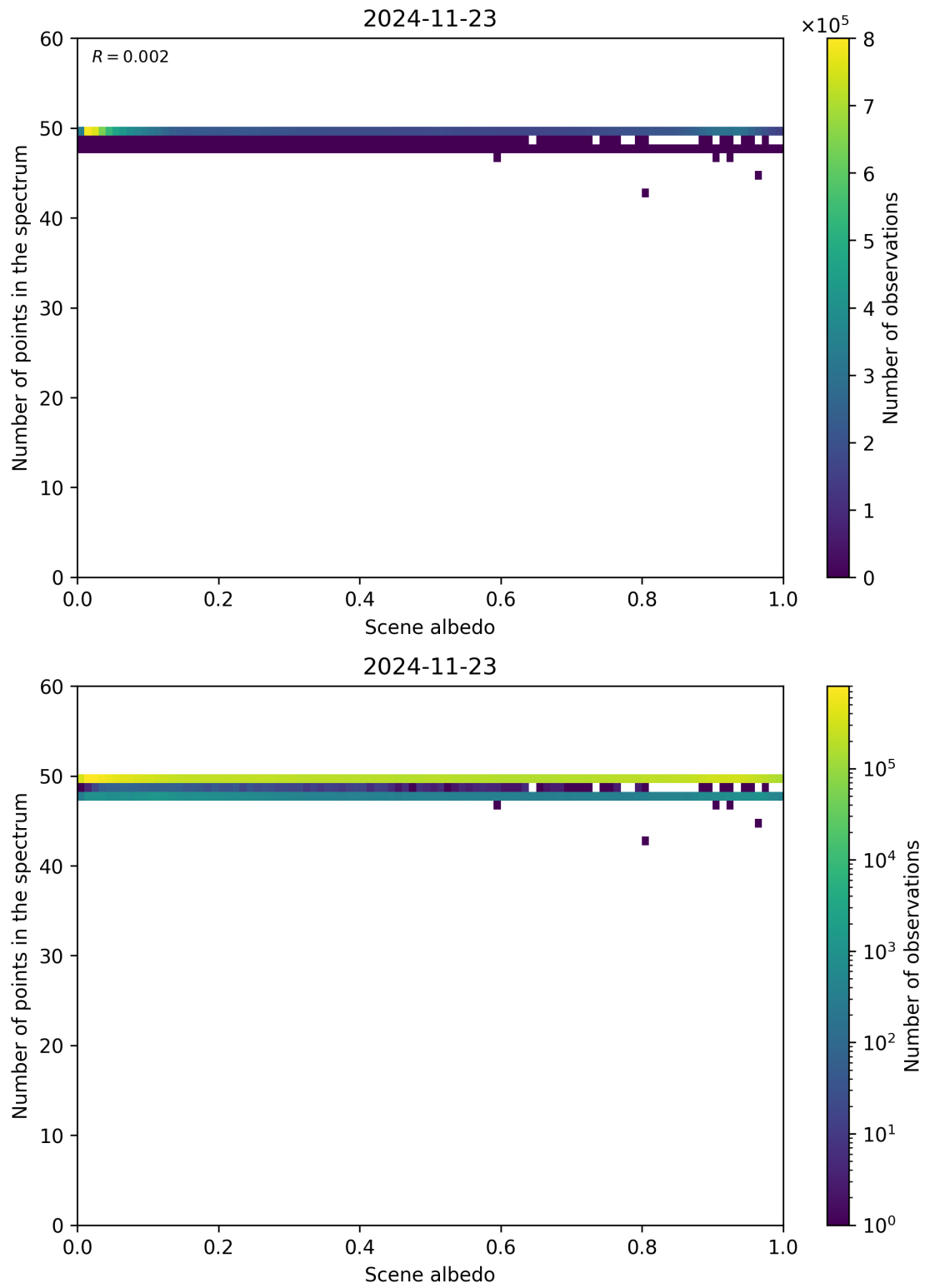
Figure 106: Scatter density plot of “Scene albedo” against “Number of points in the spectrum” for 2024-11-22 to 2024-11-24.
