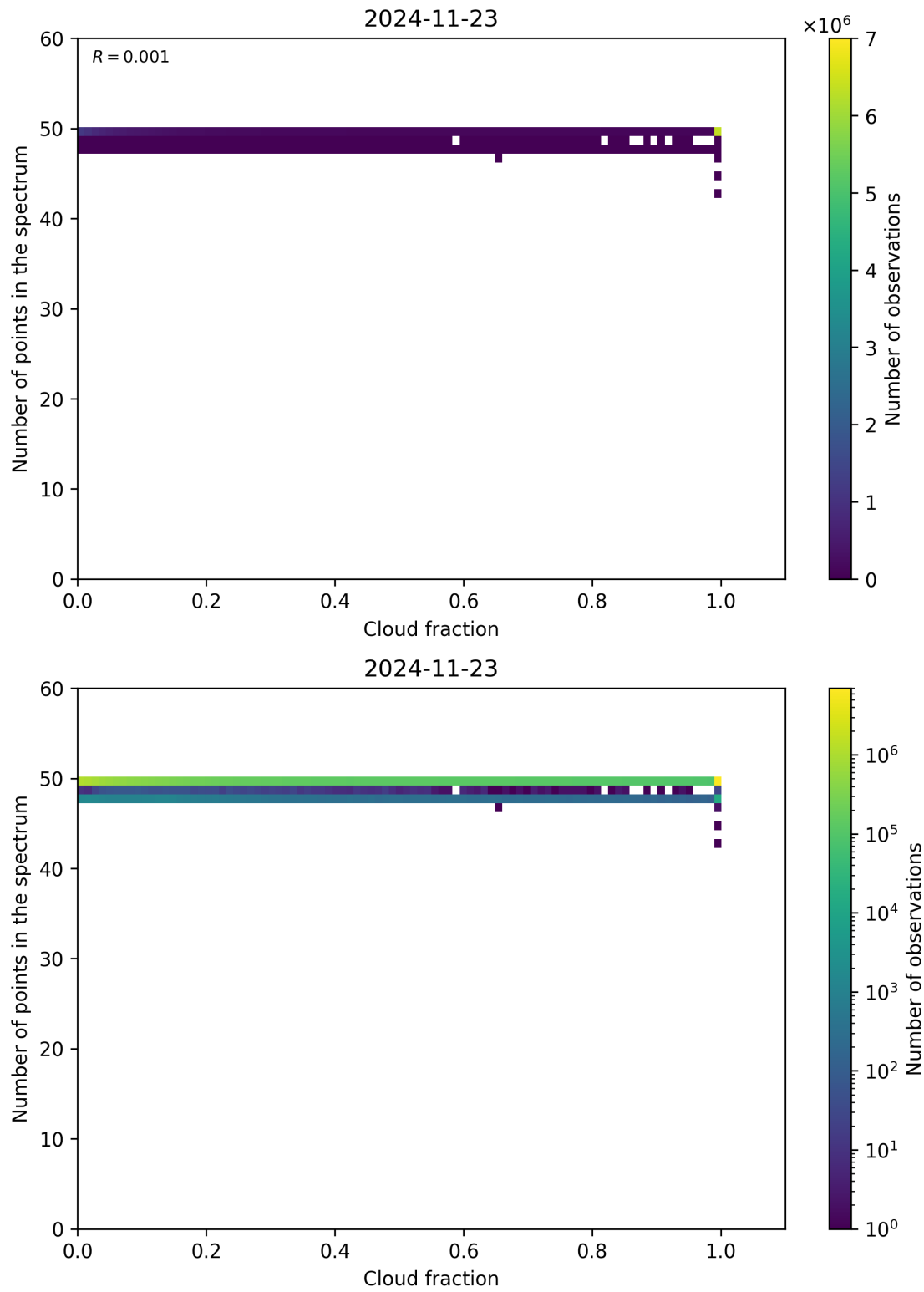
Figure 74: Scatter density plot of “Cloud fraction” against “Number of points in the spectrum” for 2024-11-22 to 2024-11-24.
