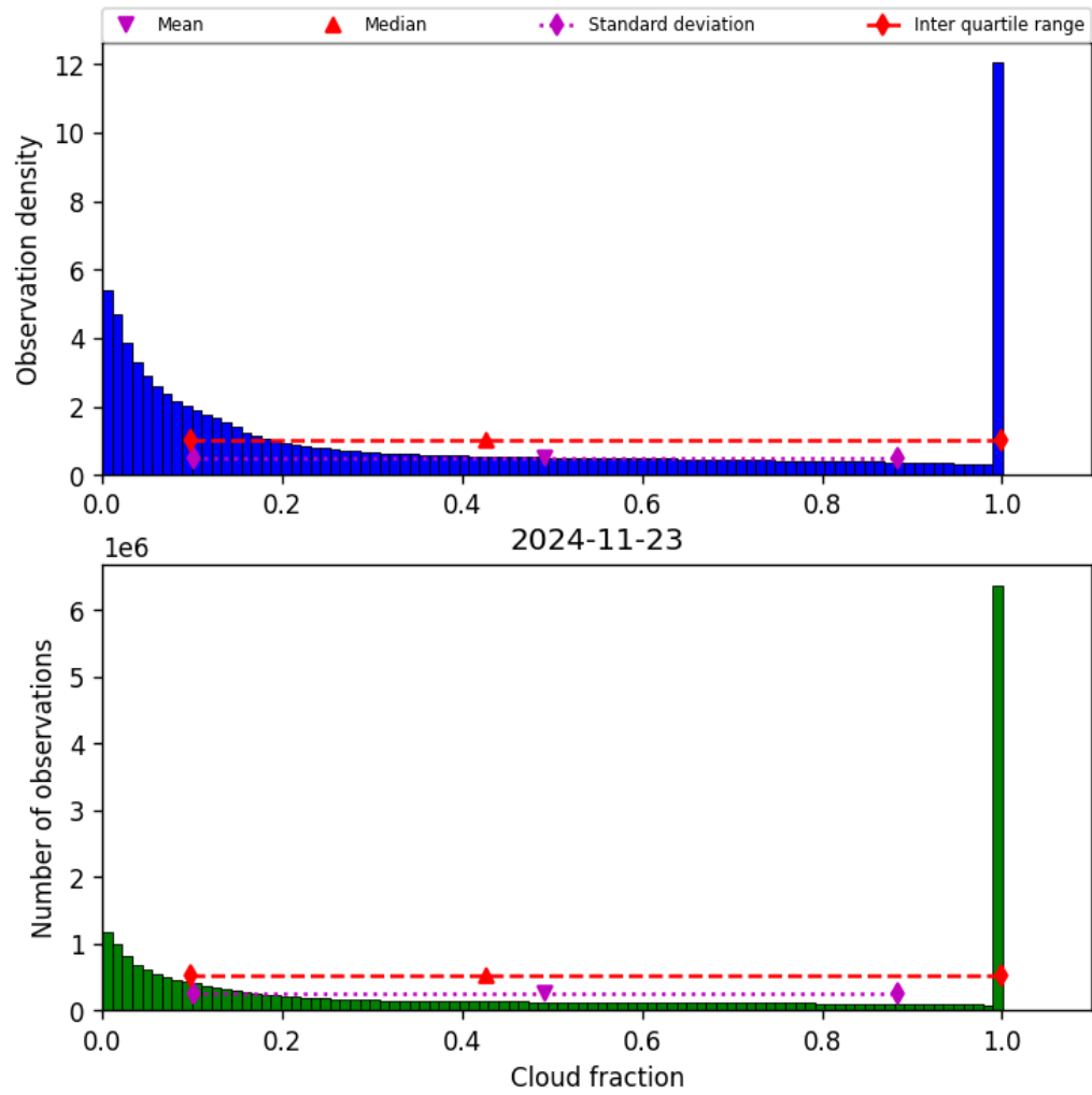
Figure 32: Histogram of “Cloud fraction” for 2024-11-22 to 2024-11-24
