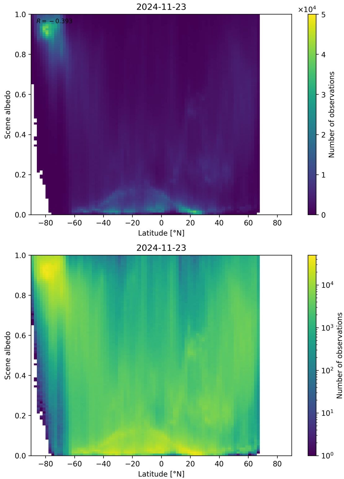
Figure 95: Scatter density plot of “Latitude” against “Scene albedo” for 2024-11-22 to 2024-11-24.
