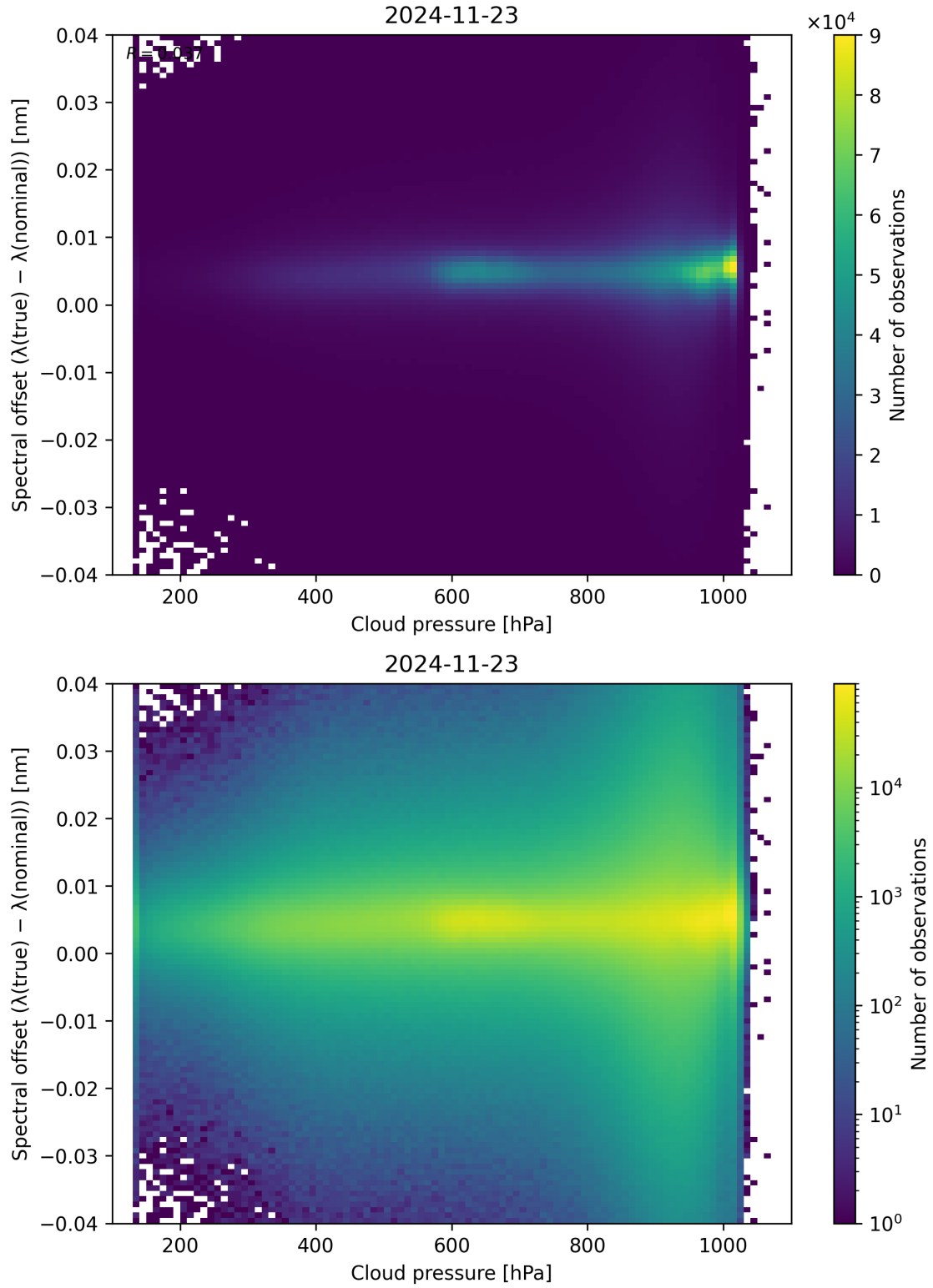
Figure 84: Scatter density plot of “Cloud pressure” against “Spectral offset ( \lambda_{\text{true}} - \lambda_{\text{nominal}} )” for 2024-11-22 to 2024-11-24.
