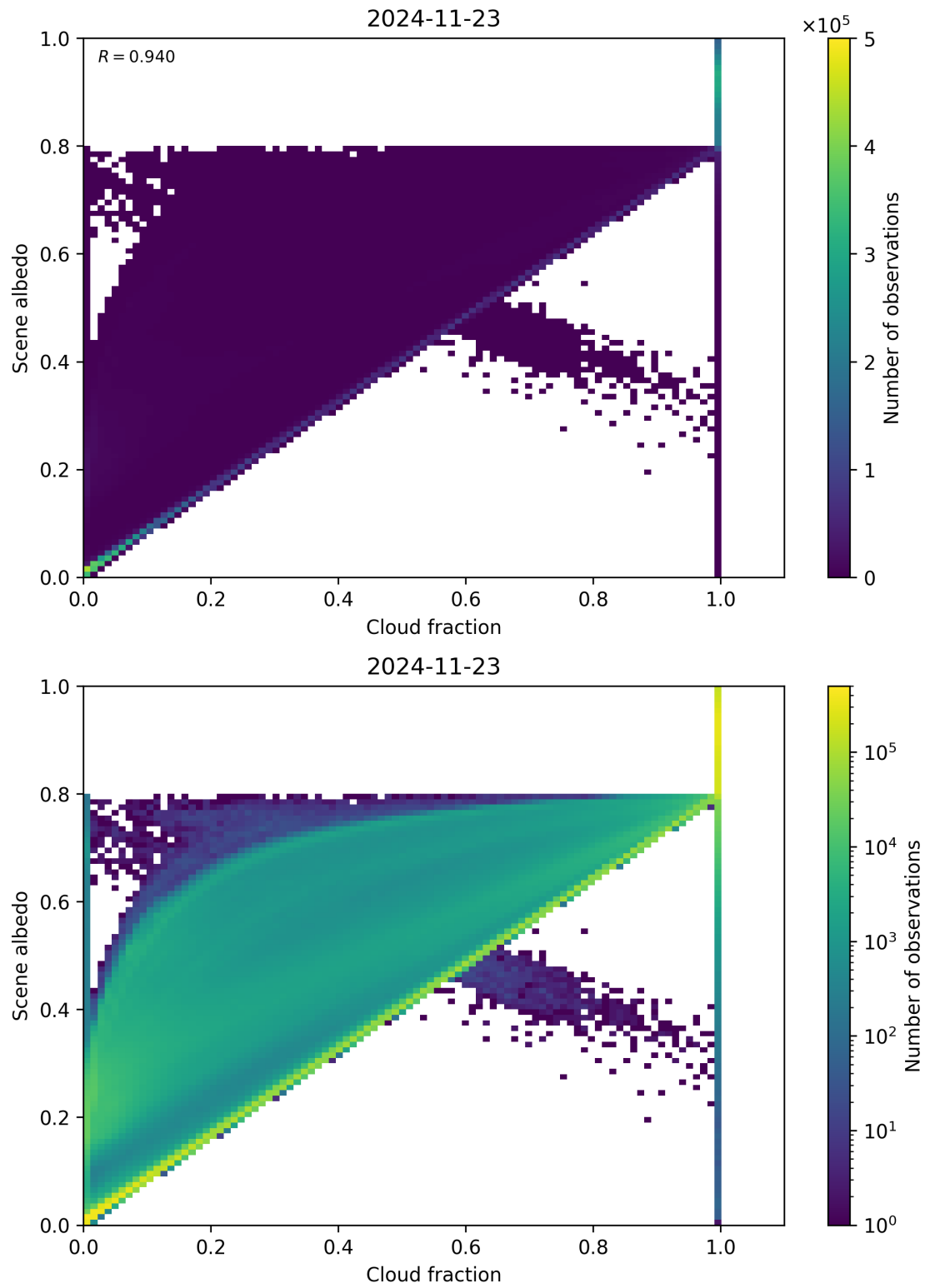
Figure 75: Scatter density plot of “Cloud fraction” against “Scene albedo” for 2024-11-22 to 2024-11-24.
