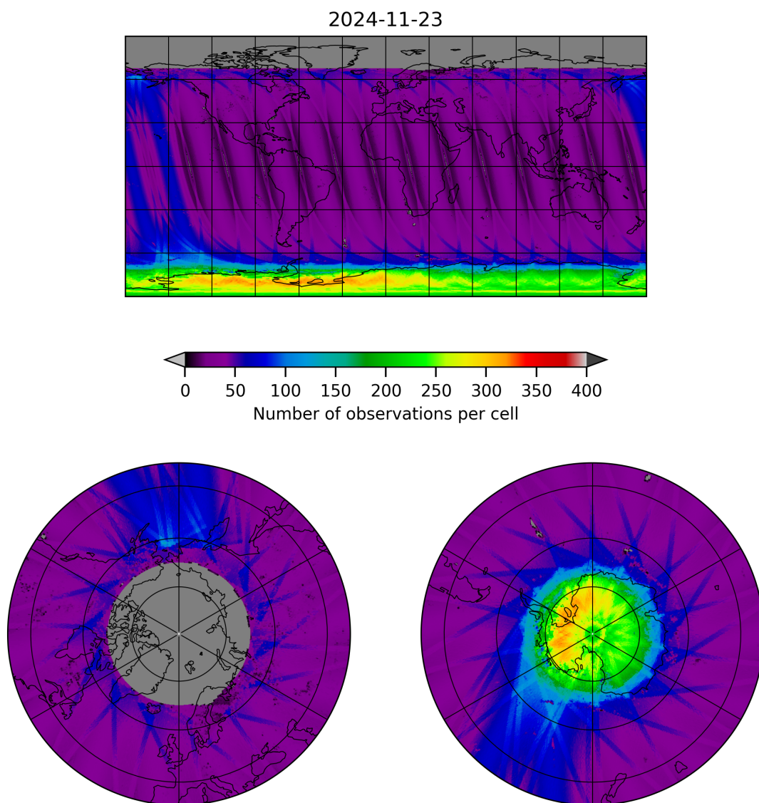
Figure 11: Map of the number of observations for 2024-11-22 to 2024-11-24
