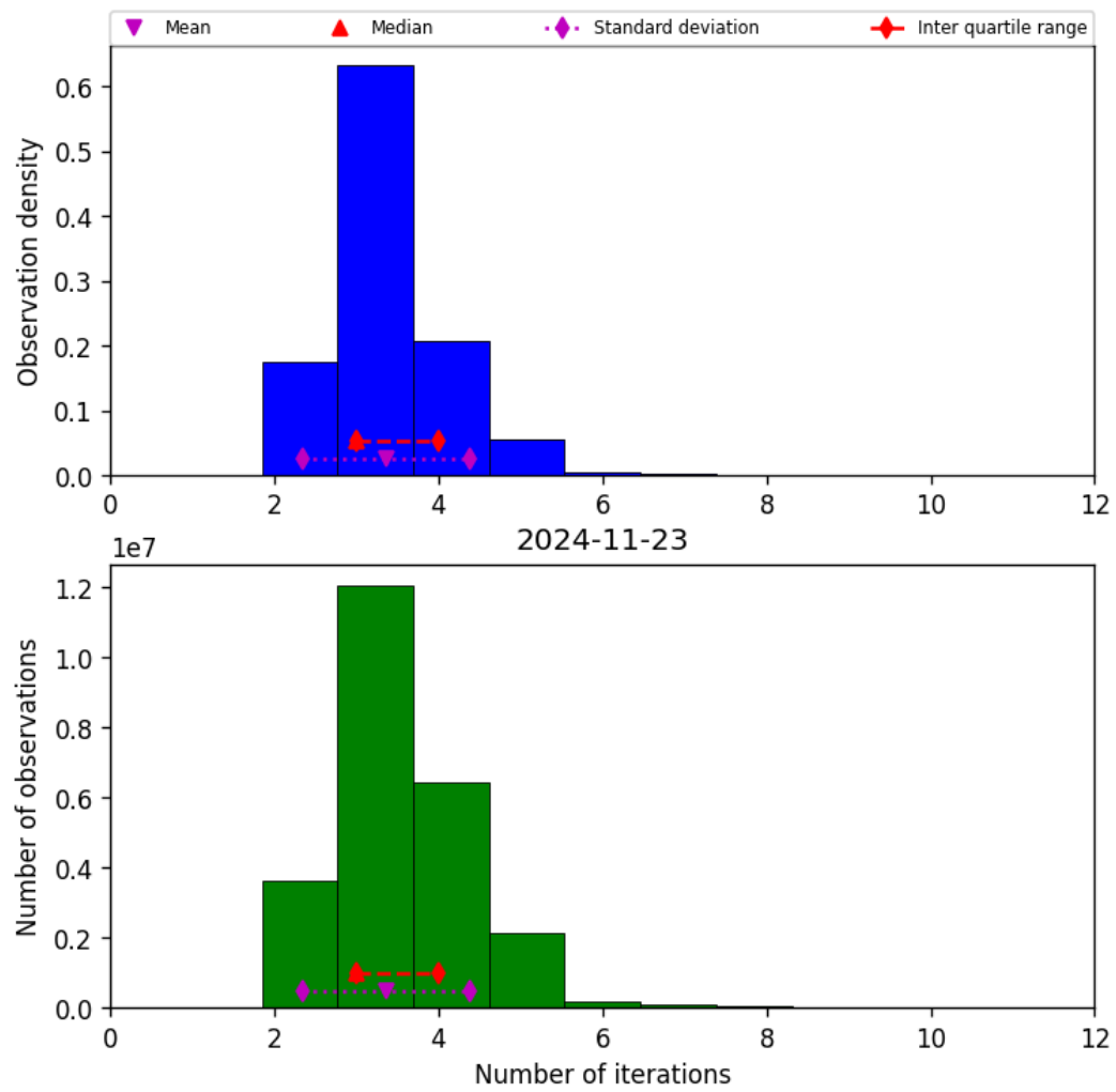
Figure 39: Histogram of “Number of iterations” for 2024-11-22 to 2024-11-24
