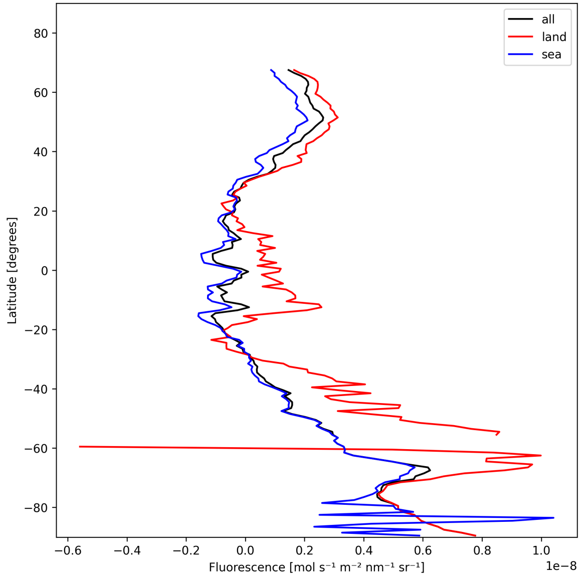
Figure 23: Zonal average of “Fluorescence” for 2024-11-22 to 2024-11-24.
