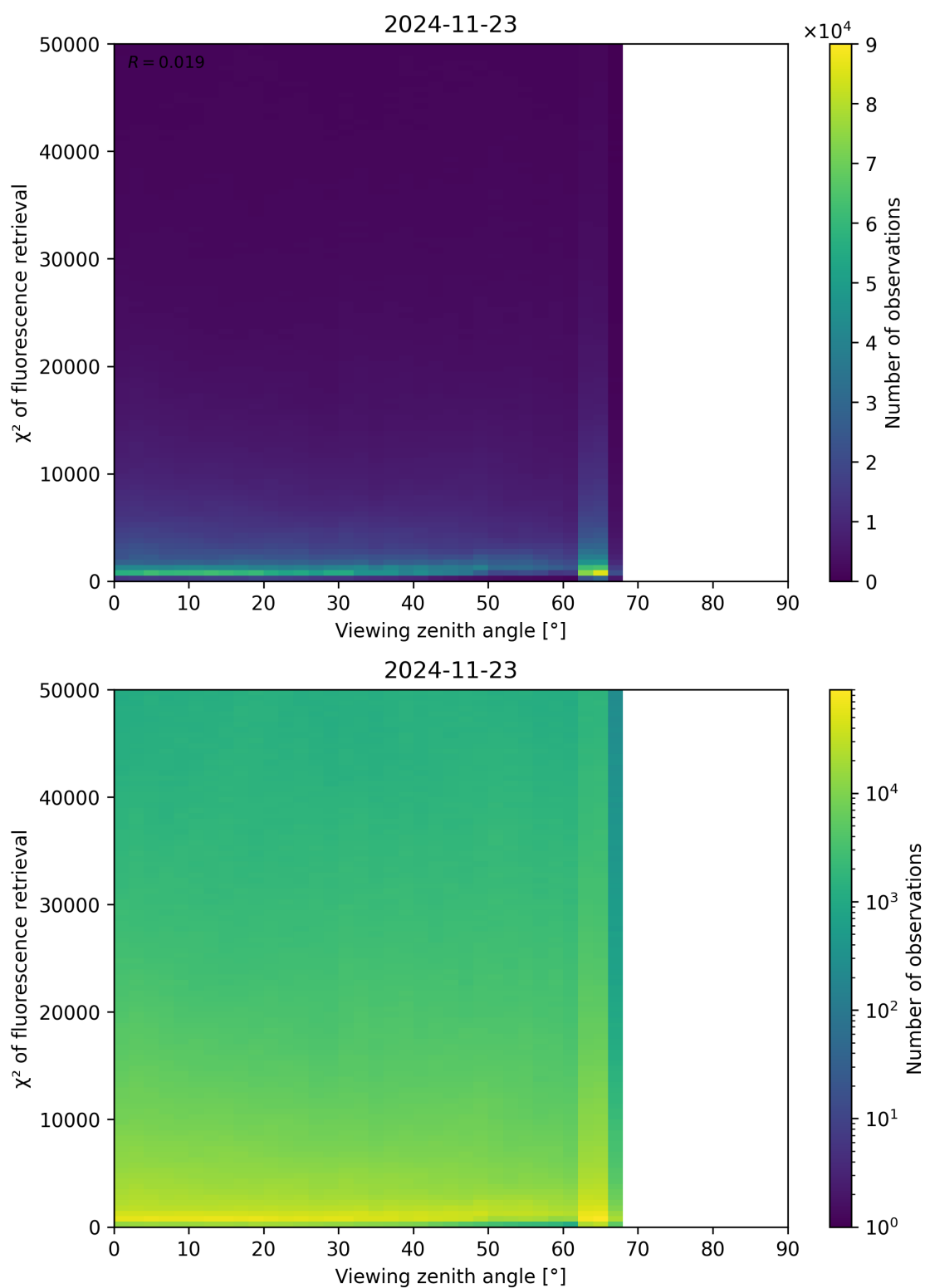
Figure 119: Scatter density plot of “Viewing zenith angle” against “ \chi^2 of fluorescence retrieval” for 2024-11-22 to 2024-11-24.
