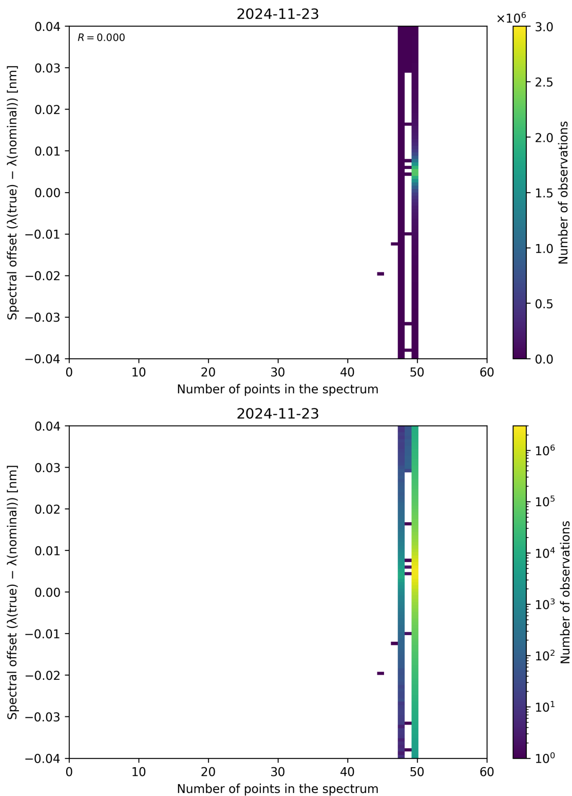
Figure 101: Scatter density plot of “Number of points in the spectrum” against “Spectral offset ( \lambda_{\text{true}} - \lambda_{\text{nominal}} )” for 2024-11-22 to 2024-11-24.
