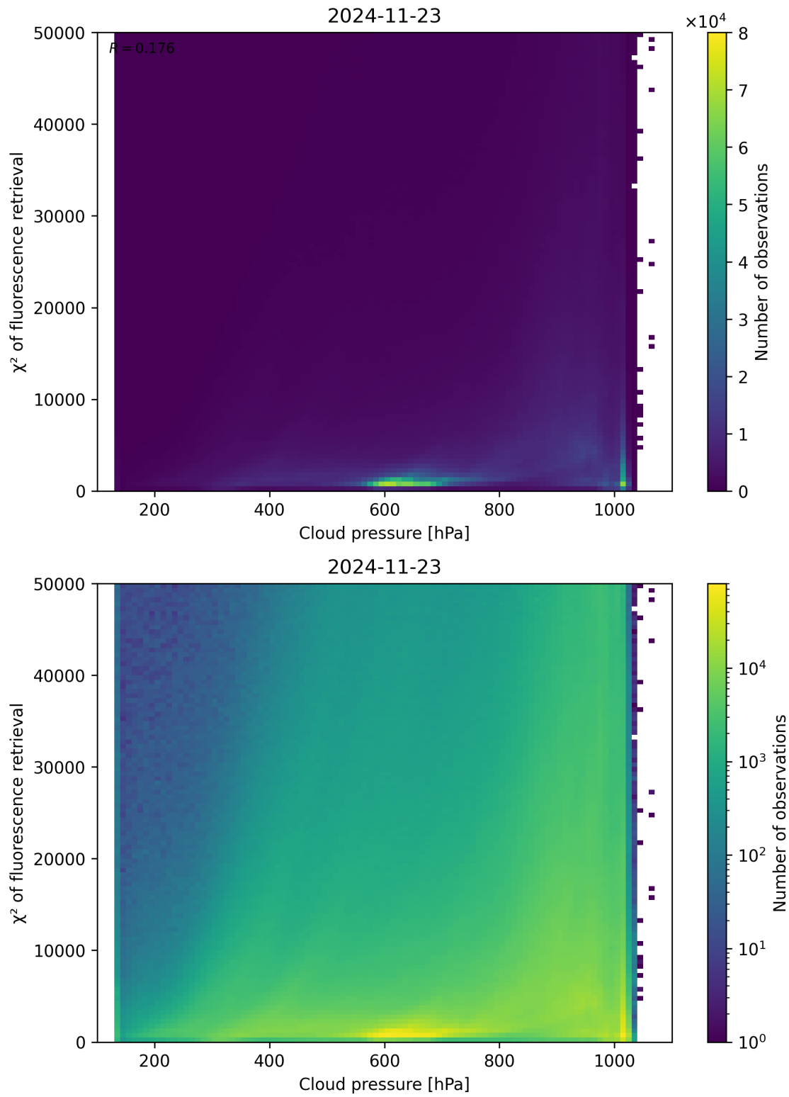
Figure 78: Scatter density plot of “Cloud pressure” against “ \chi^2 of fluorescence retrieval” for 2024-11-22 to 2024-11-24.
