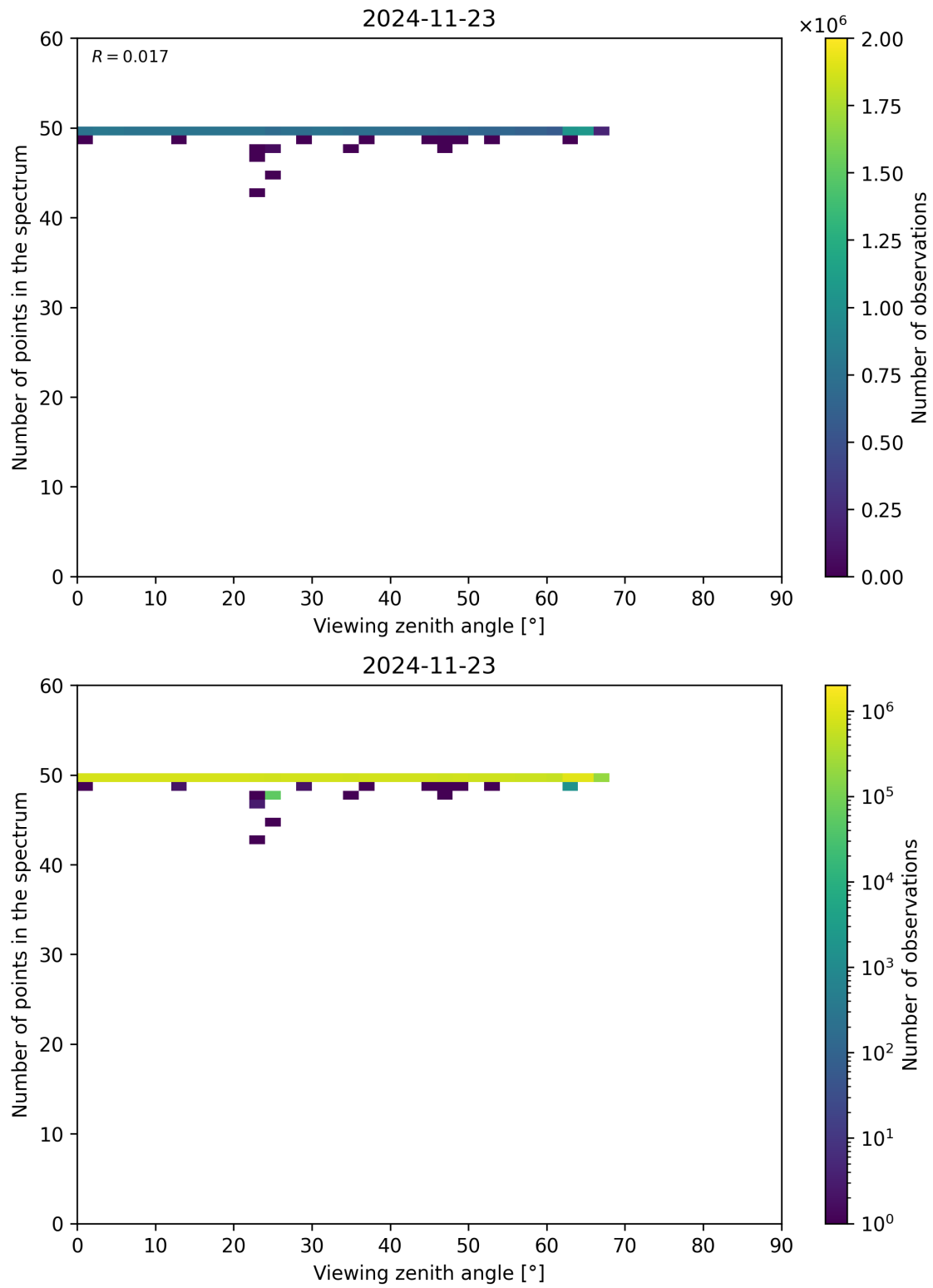
Figure 125: Scatter density plot of “Viewing zenith angle” against “Number of points in the spectrum” for 2024-11-22 to 2024-11-24.
