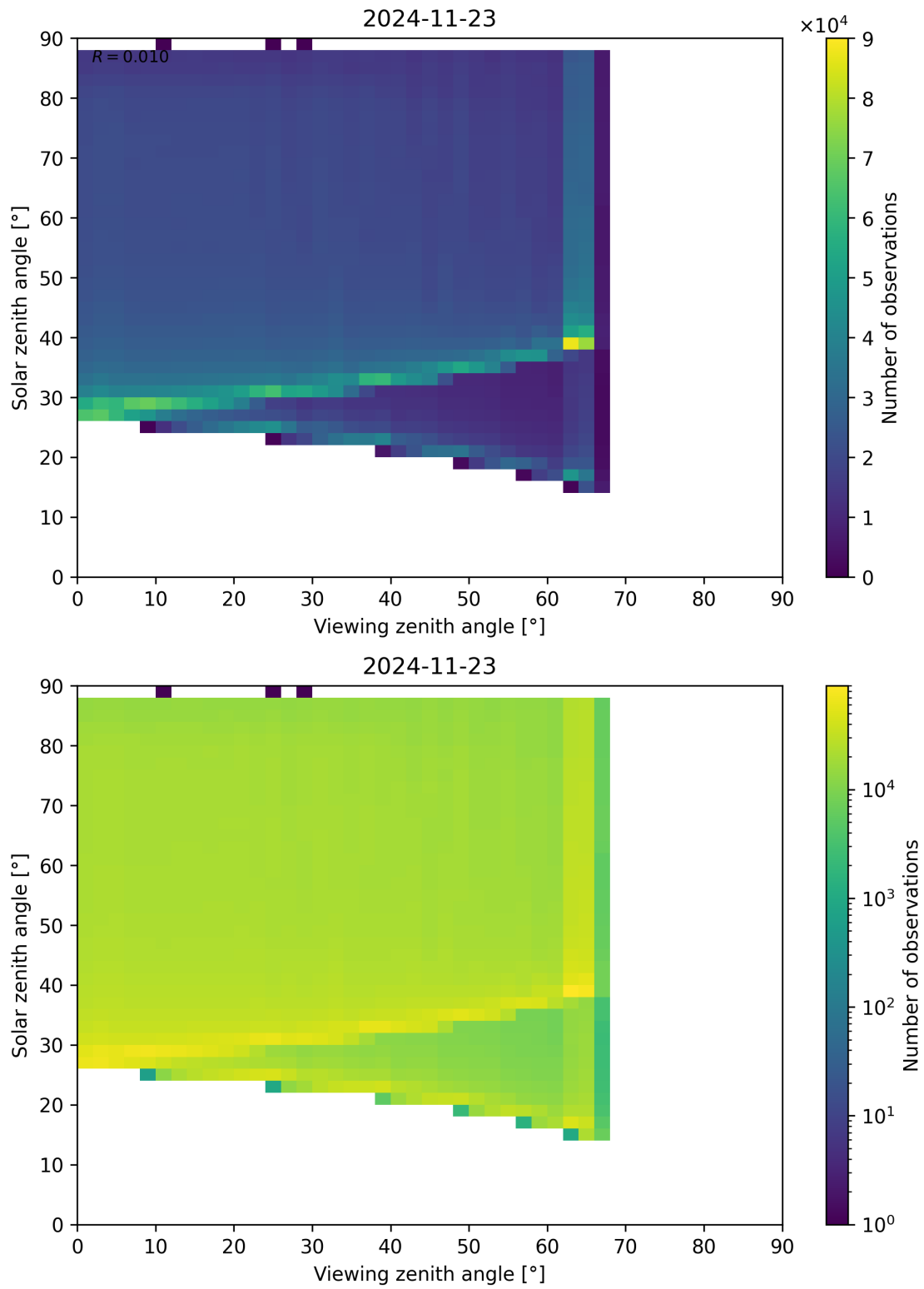
Figure 127: Scatter density plot of “Viewing zenith angle” against “Solar zenith angle” for 2024-11-22 to 2024-11-24.
