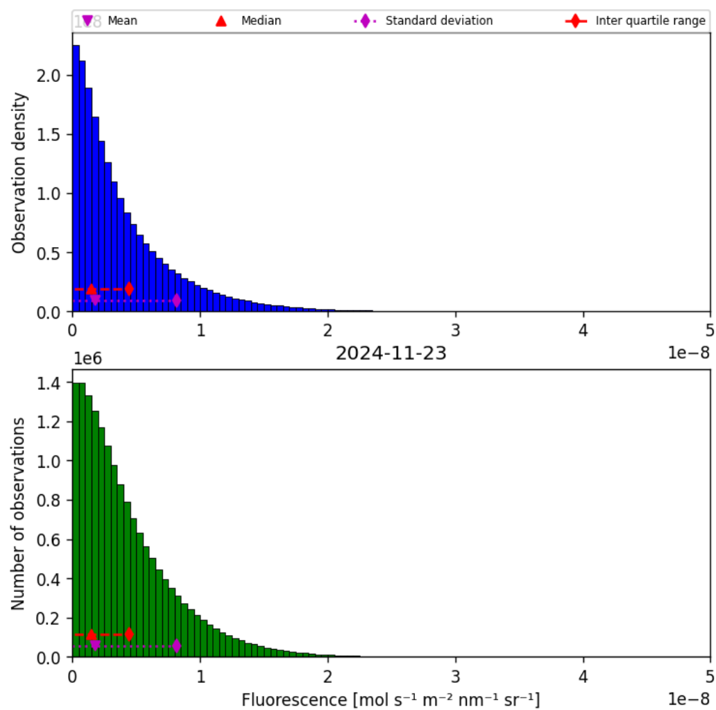
Figure 40: Histogram of “Fluorescence” for 2024-11-22 to 2024-11-24
