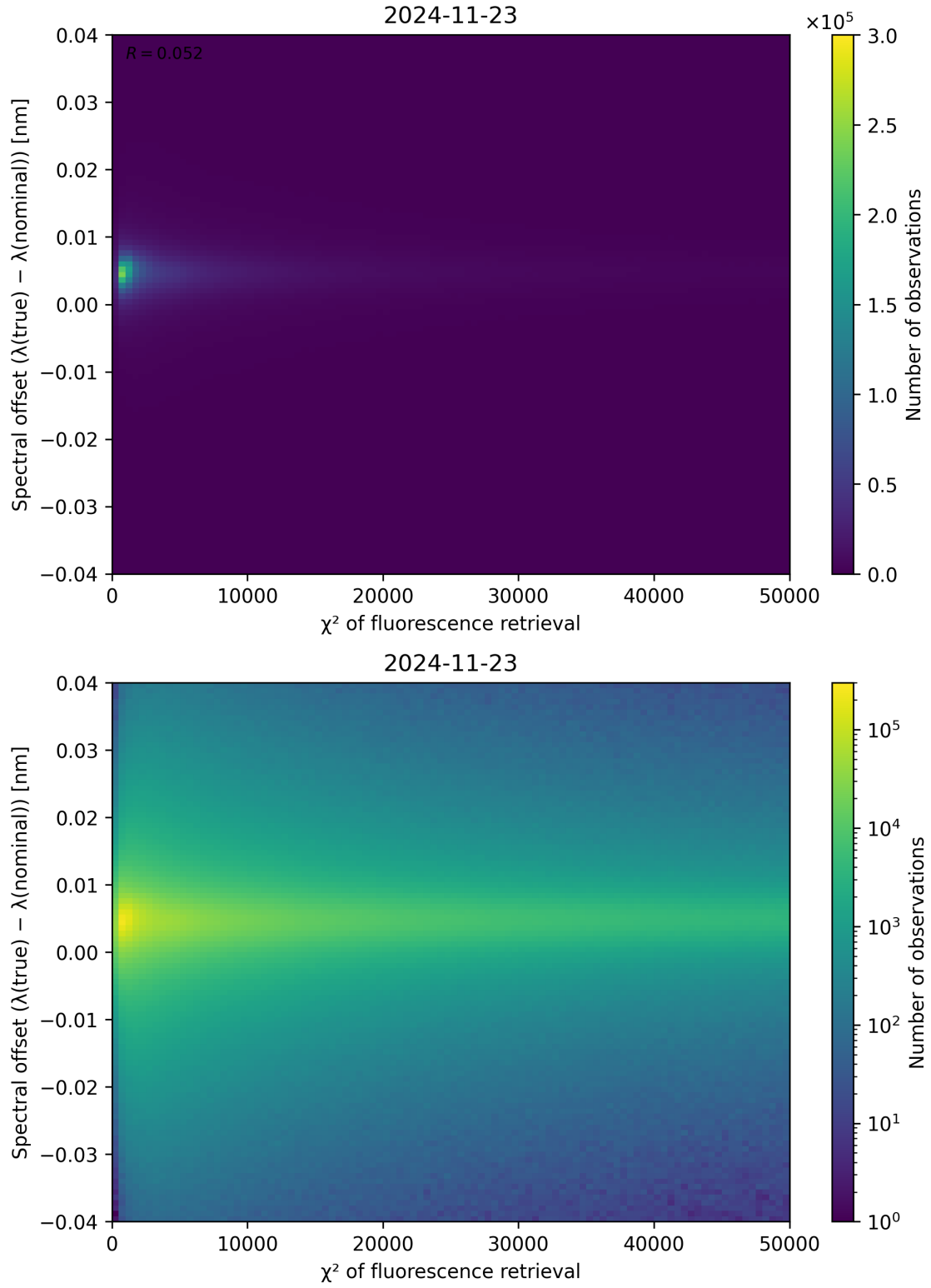
Figure 69: Scatter density plot of “ \chi^2 of fluorescence retrieval” against “Spectral offset ( \lambda_{\text{true}} - \lambda_{\text{nominal}} )” for 2024-11-22 to 2024-11-24.
