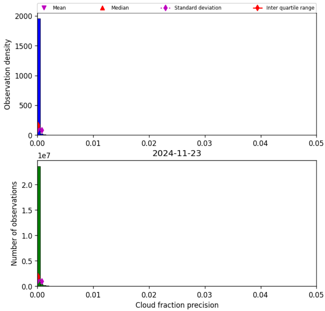
Figure 33: Histogram of “Cloud fraction precision” for 2024-11-22 to 2024-11-24
