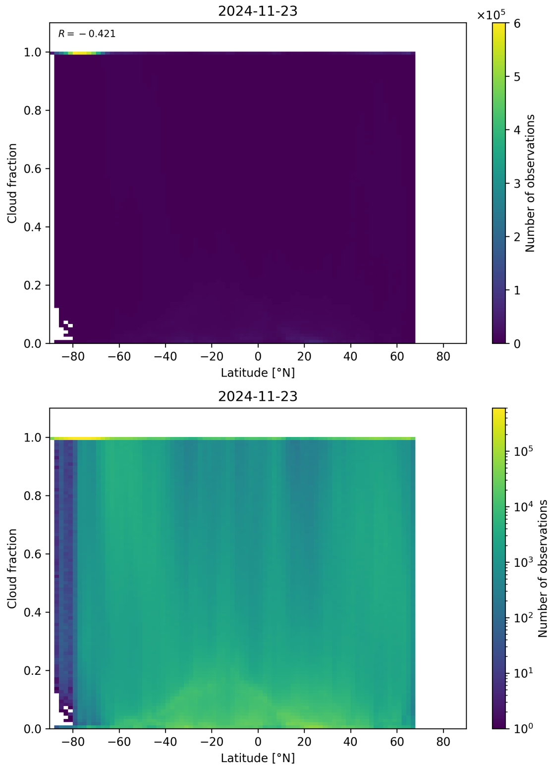
Figure 90: Scatter density plot of “Latitude” against “Cloud fraction” for 2024-11-22 to 2024-11-24.
