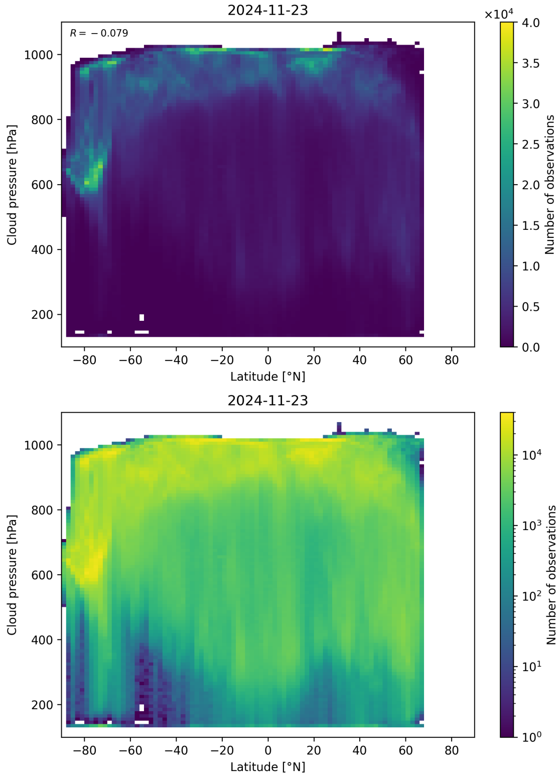
Figure 91: Scatter density plot of “Latitude” against “Cloud pressure” for 2024-11-22 to 2024-11-24.
