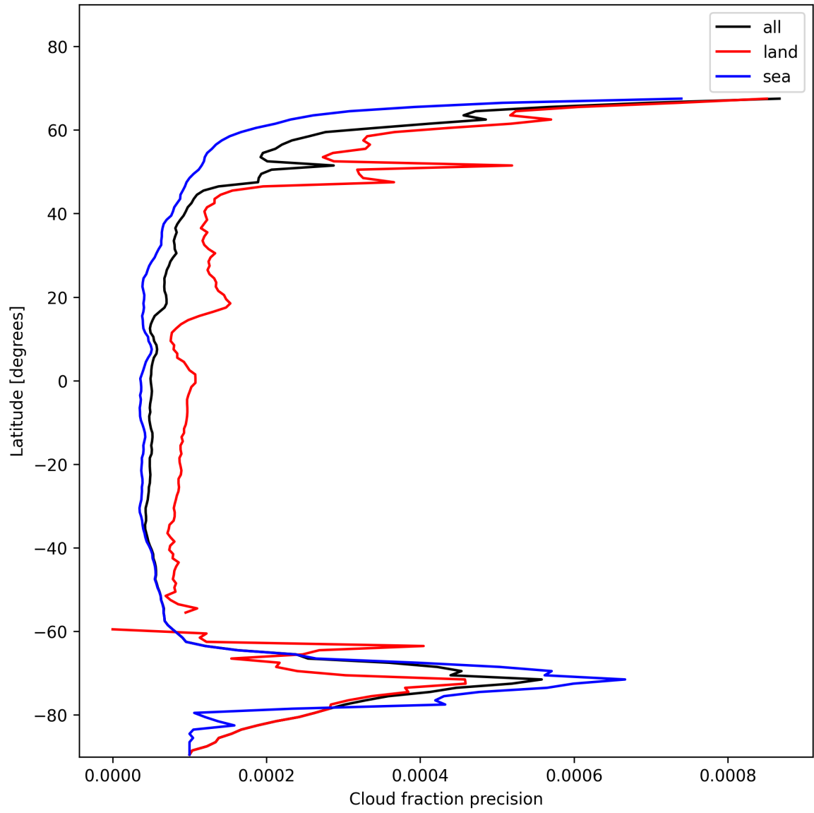
Figure 16: Zonal average of “Cloud fraction precision” for 2024-11-22 to 2024-11-24.
