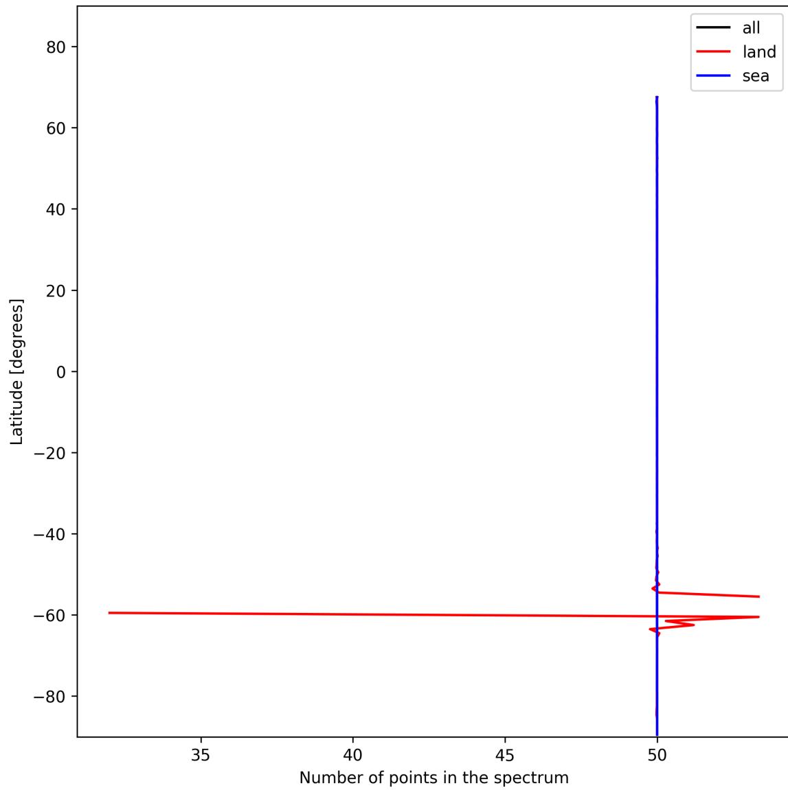
Figure 27: Zonal average of “Number of points in the spectrum” for 2024-11-22 to 2024-11-24.
