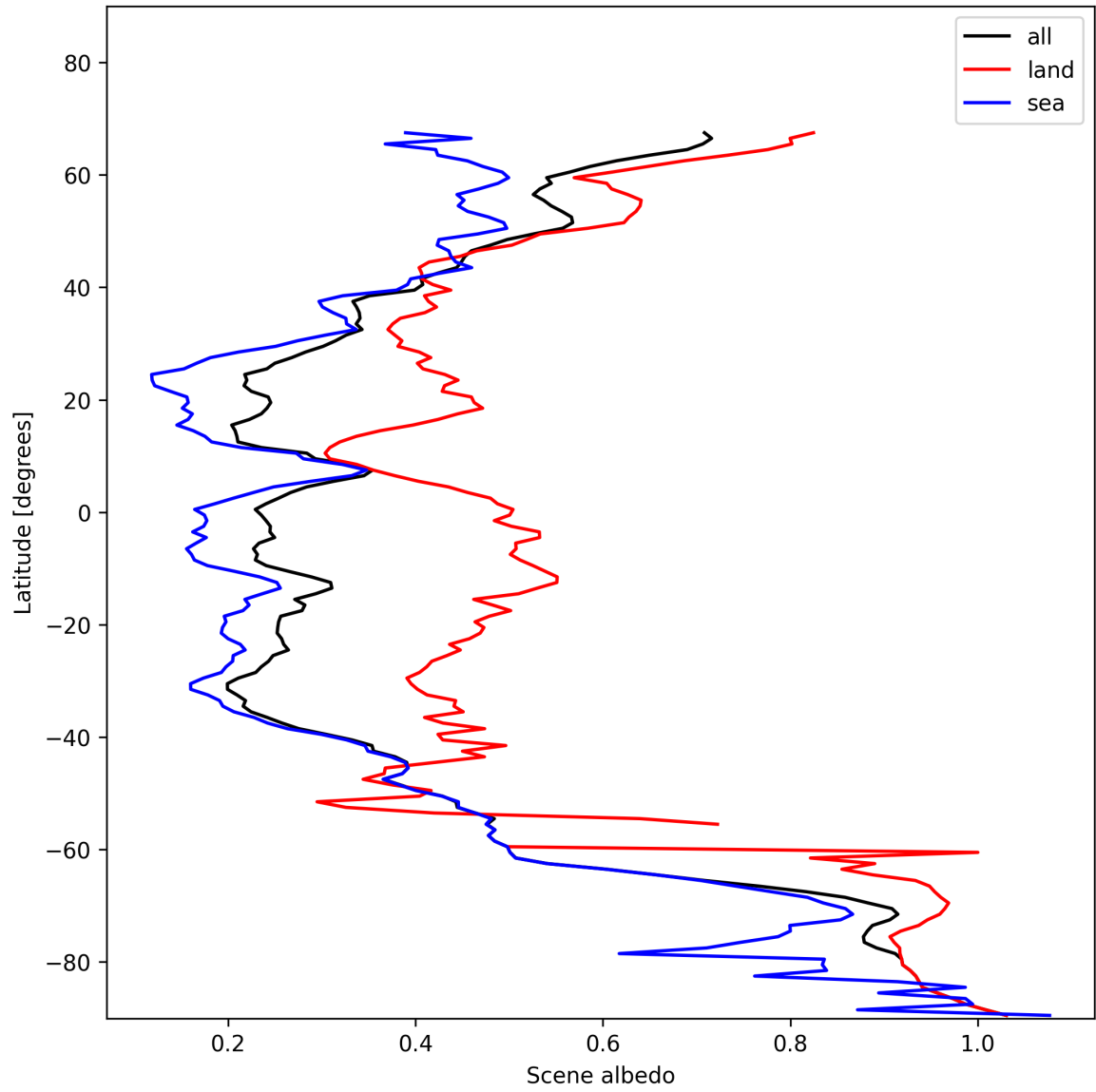
Figure 17: Zonal average of “Scene albedo” for 2024-11-22 to 2024-11-24.
