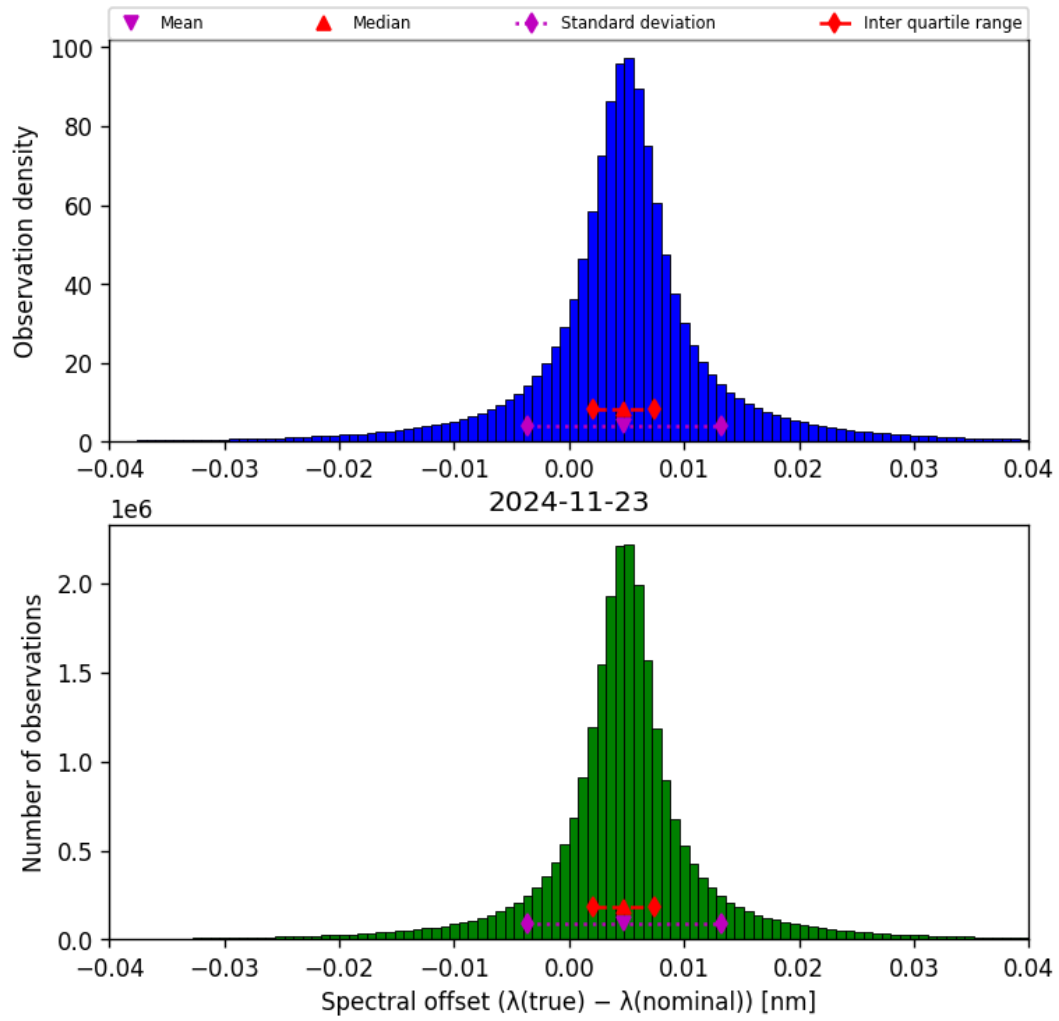
Figure 45: Histogram of “Spectral offset ( \lambda_{\text{true}} - \lambda_{\text{nominal}} )” for 2024-11-22 to 2024-11-24
