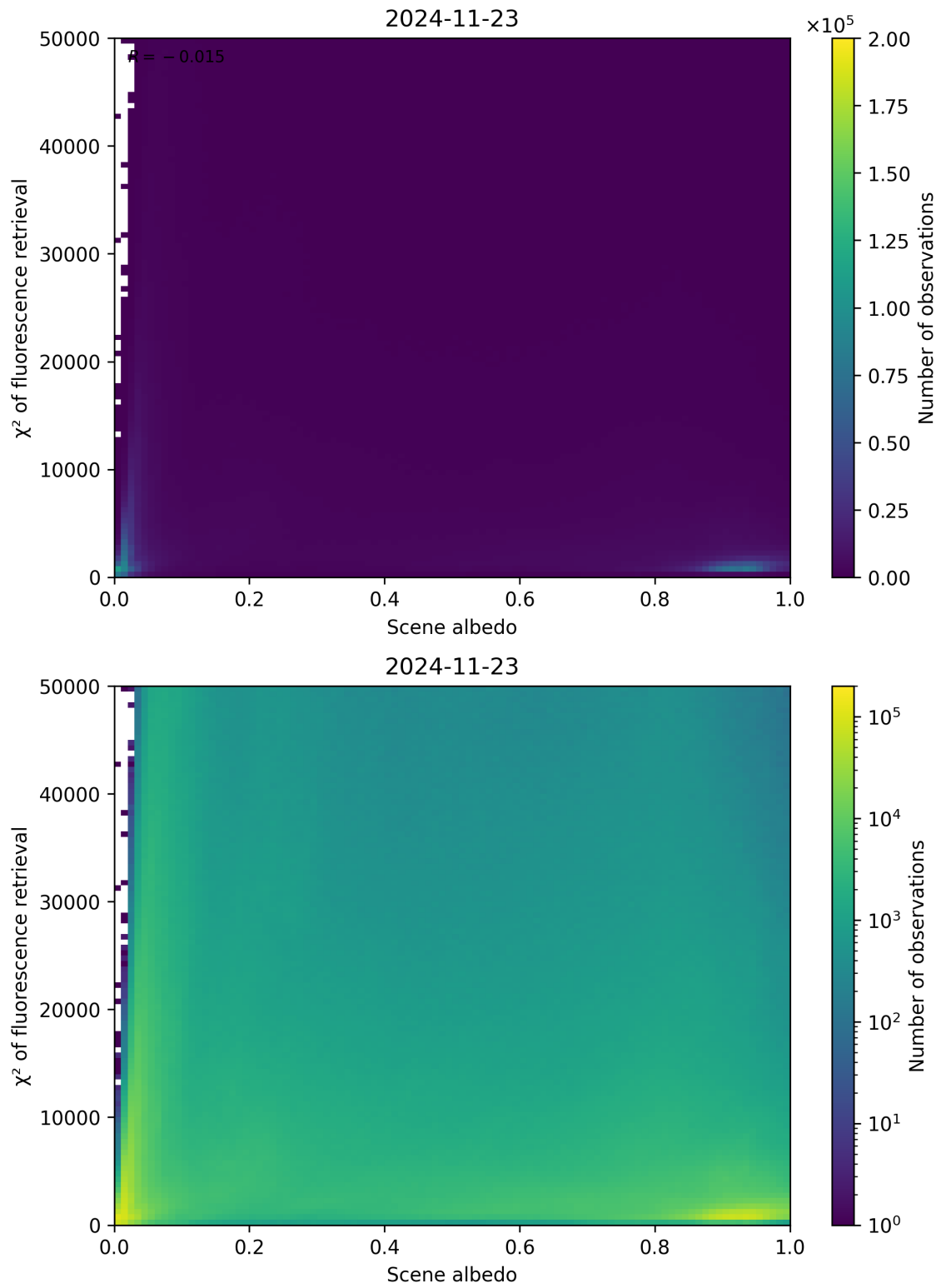
Figure 103: Scatter density plot of “Scene albedo” against “ \chi^2 of fluorescence retrieval” for 2024-11-22 to 2024-11-24.
