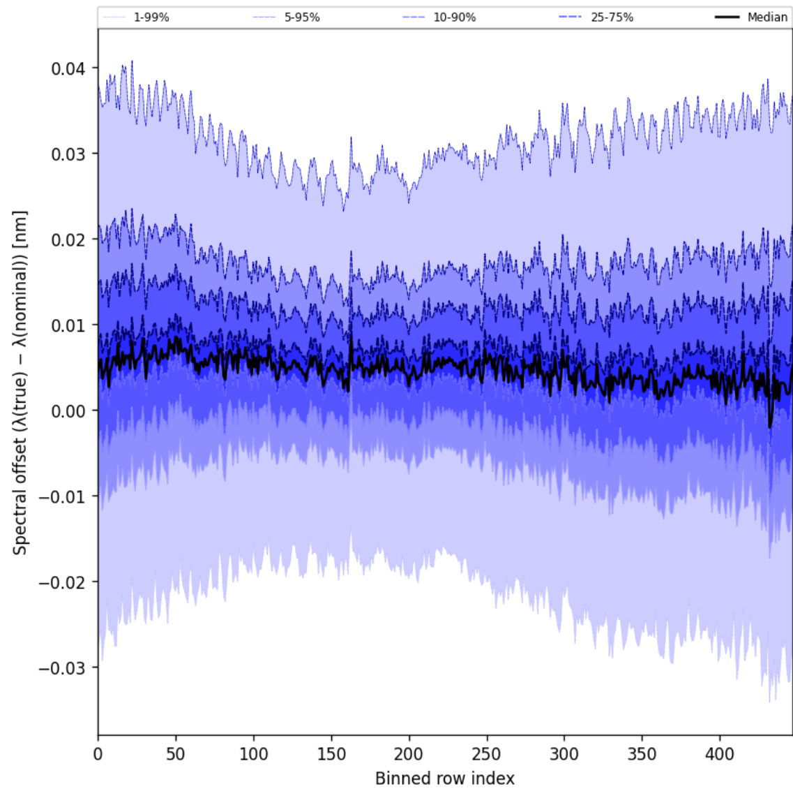
Figure 62: Along track statistics of “Spectral offset ( \lambda_{\text{true}} - \lambda_{\text{nominal}} )” for 2024-11-22 to 2024-11-24
