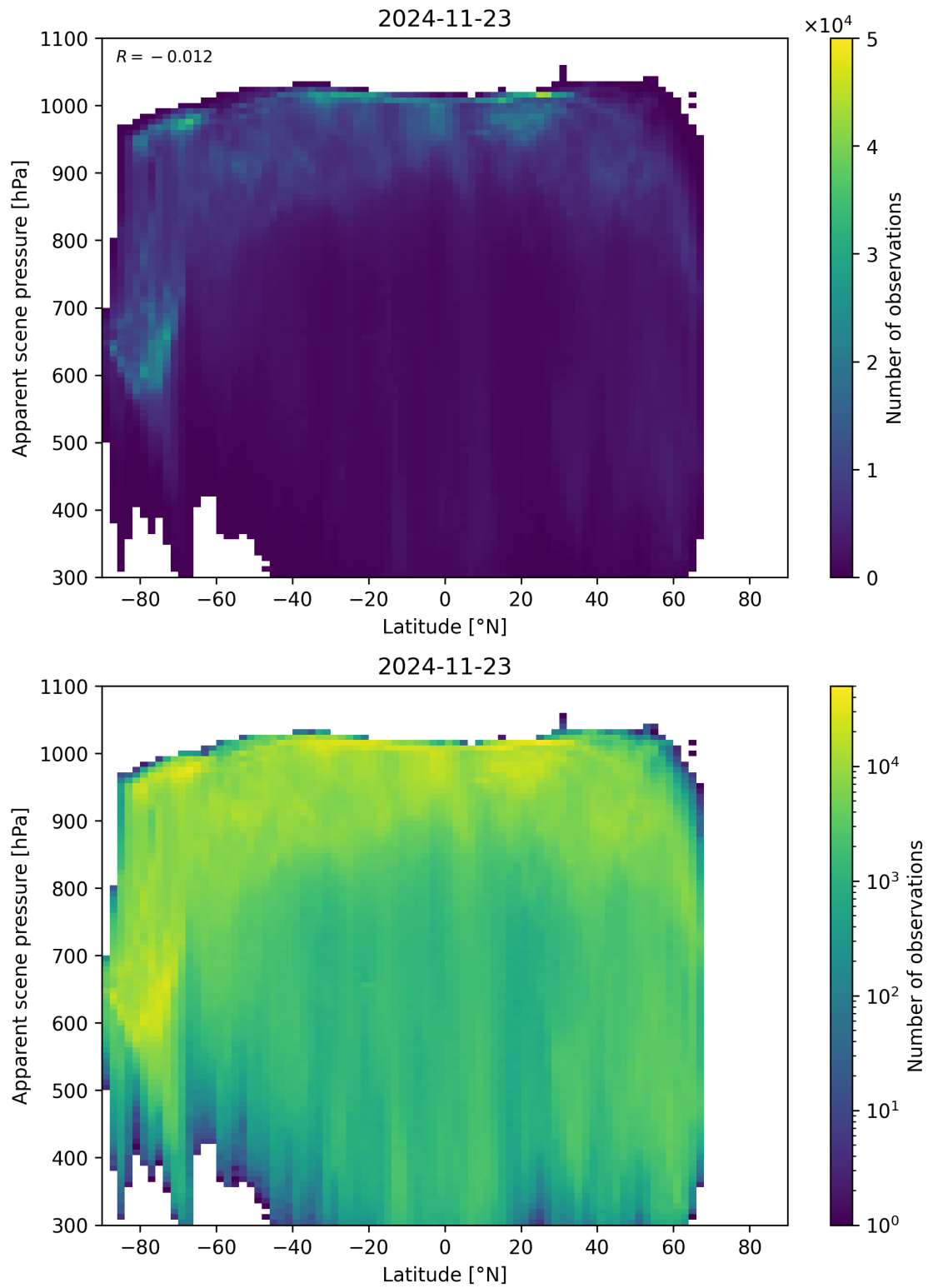
Figure 88: Scatter density plot of “Latitude” against “Apparent scene pressure” for 2024-11-22 to 2024-11-24.
