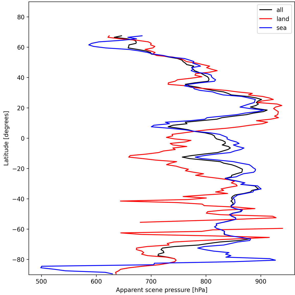
Figure 19: Zonal average of “Apparent scene pressure” for 2024-11-22 to 2024-11-24.
