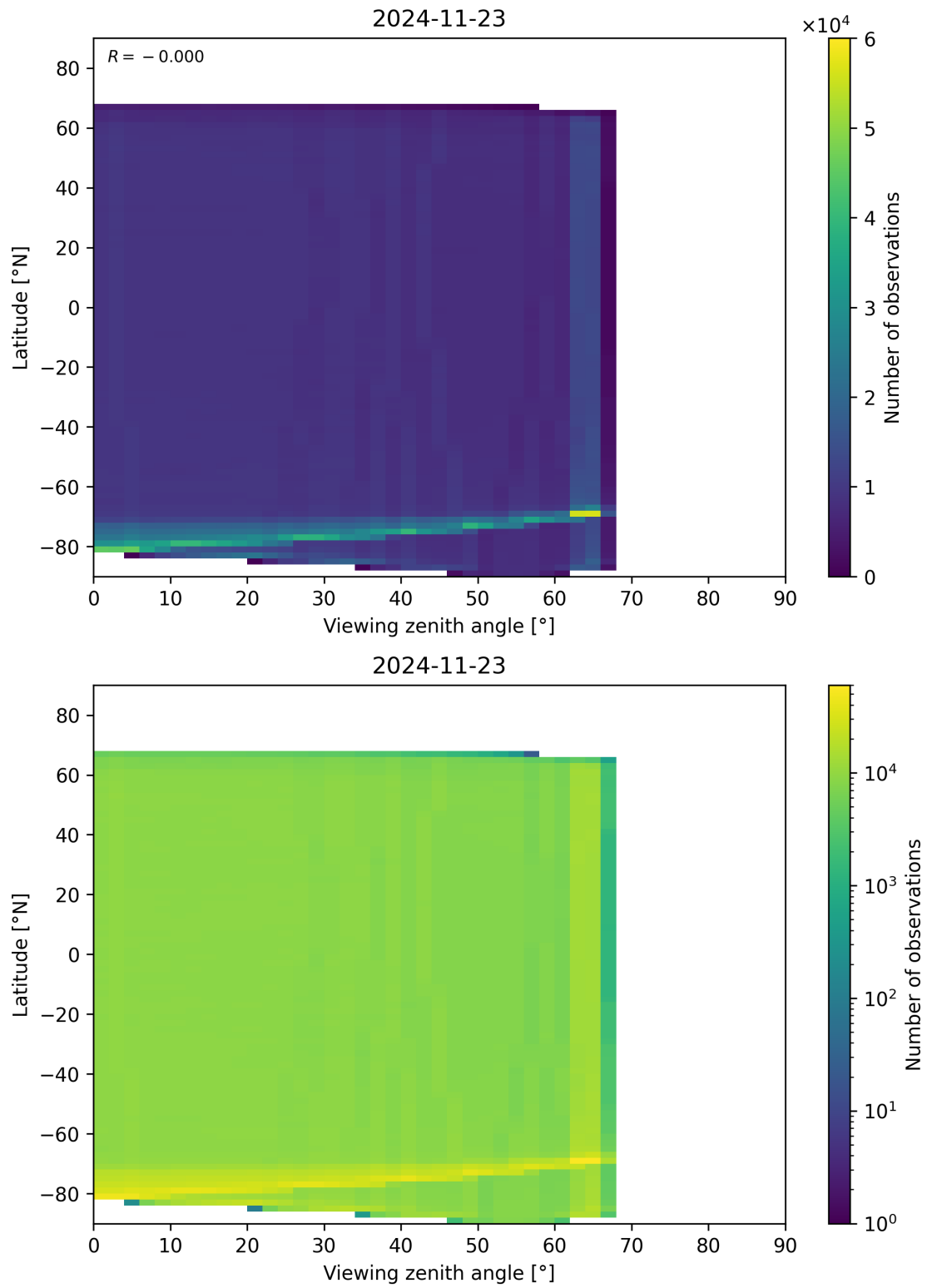
Figure 123: Scatter density plot of “Viewing zenith angle” against “Latitude” for 2024-11-22 to 2024-11-24.
