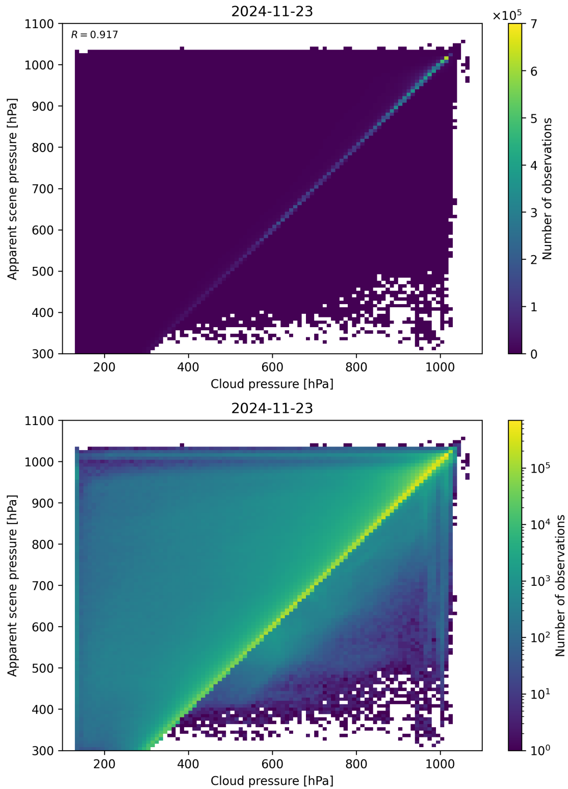
Figure 77: Scatter density plot of “Cloud pressure” against “Apparent scene pressure” for 2024-11-22 to 2024-11-24.
