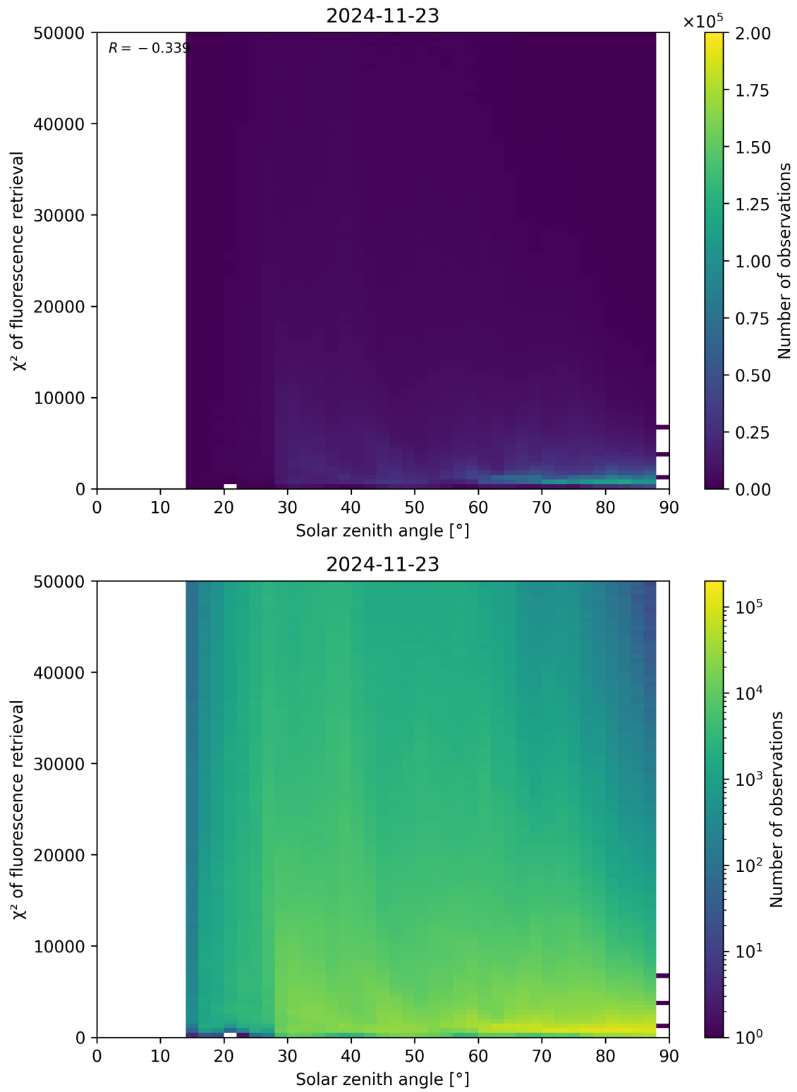
Figure 109: Scatter density plot of “Solar zenith angle” against “ \chi^2 of fluorescence retrieval” for 2024-11-22 to 2024-11-24.
