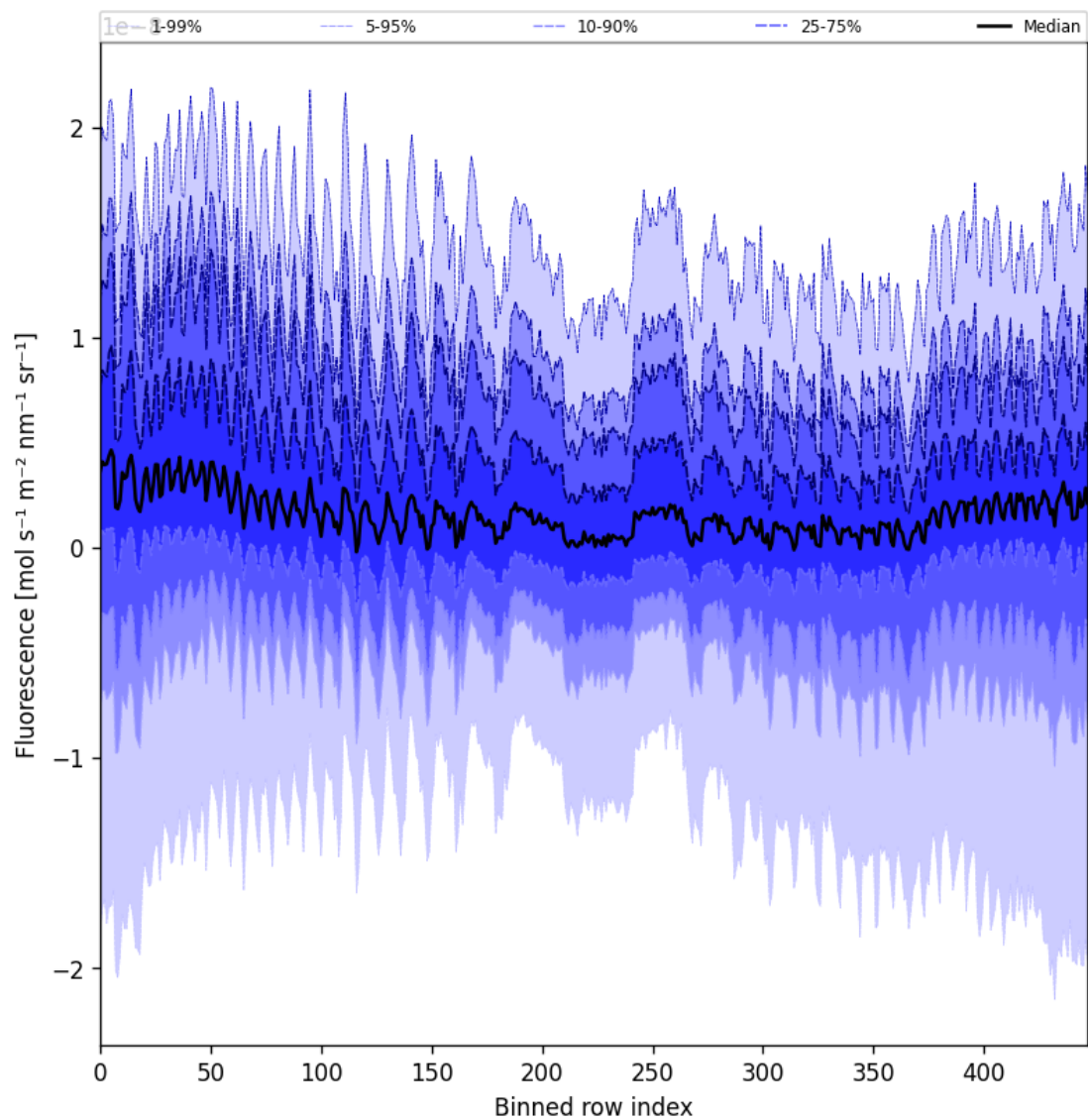
Figure 57: Along track statistics of “Fluorescence” for 2024-11-22 to 2024-11-24
