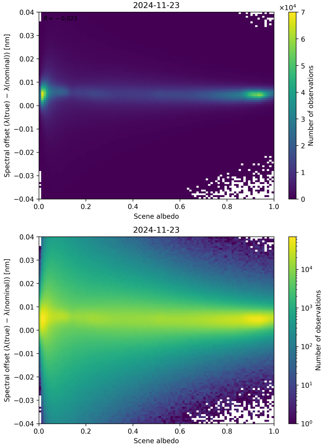
Figure 107: Scatter density plot of “Scene albedo” against “Spectral offset ( \lambda_{\text{true}} - \lambda_{\text{nominal}} )” for 2024-11-22 to 2024-11-24.
