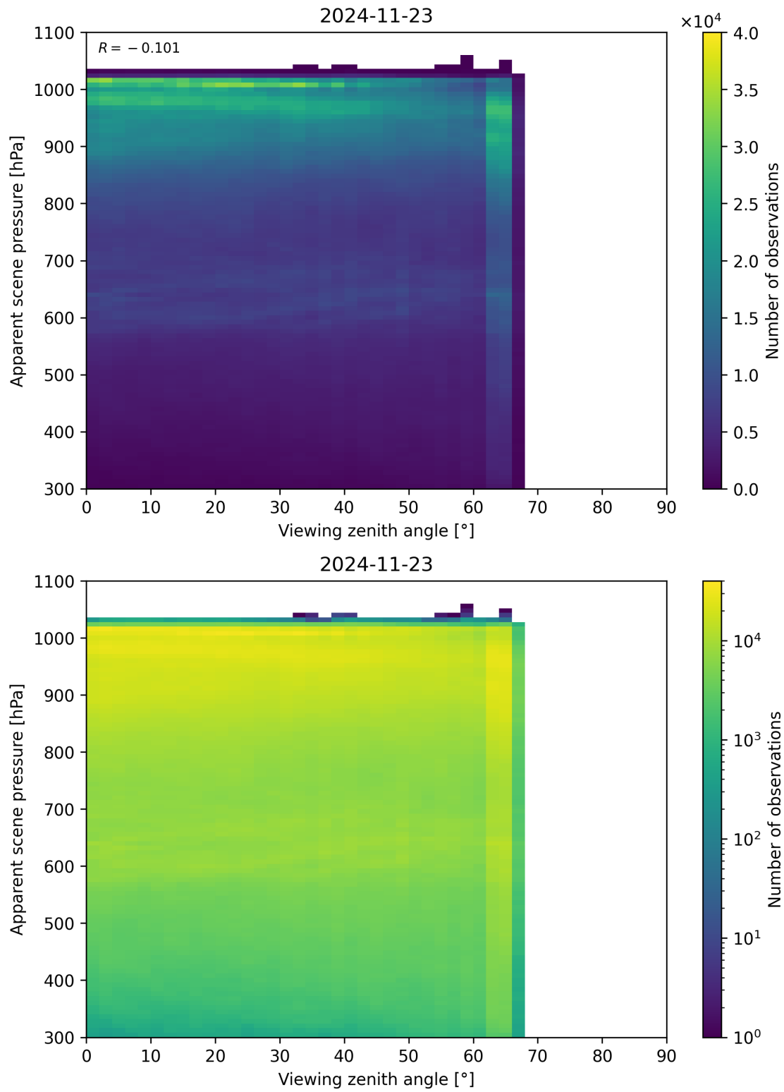
Figure 118: Scatter density plot of “Viewing zenith angle” against “Apparent scene pressure” for 2024-11-22 to 2024-11-24.
