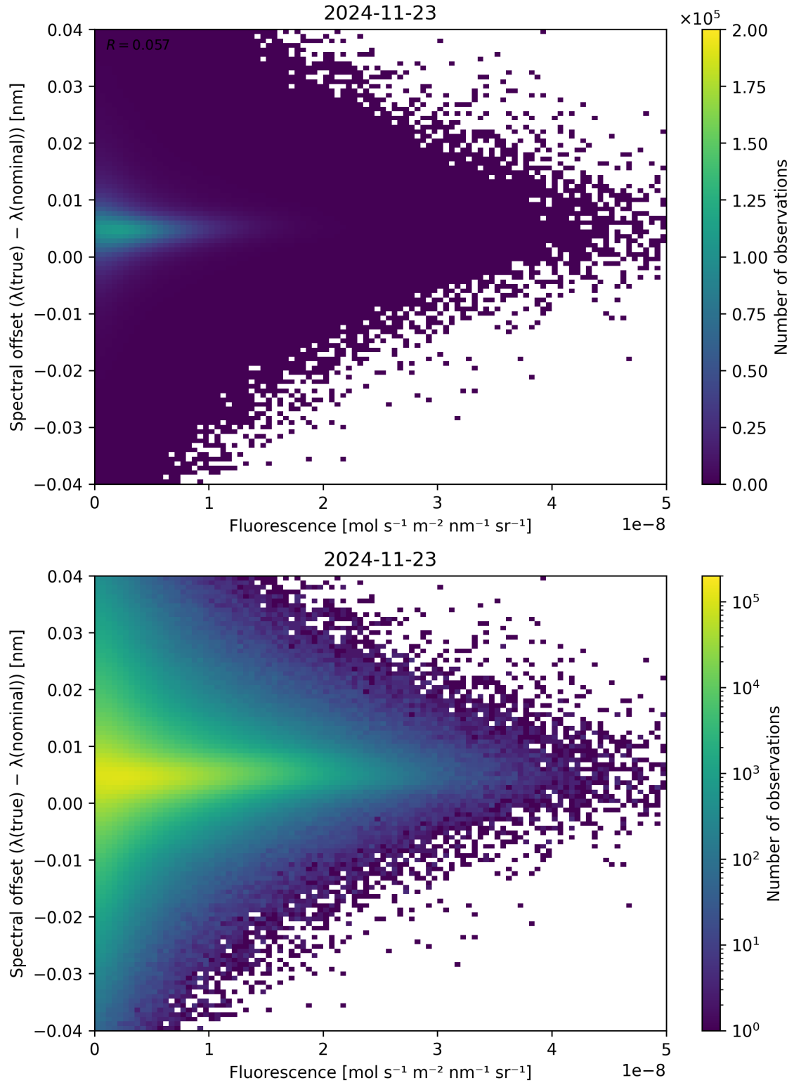
Figure 87: Scatter density plot of “Fluorescence” against “Spectral offset ( \lambda_{\text{true}} - \lambda_{\text{nominal}} )” for 2024-11-22 to 2024-11-24.
