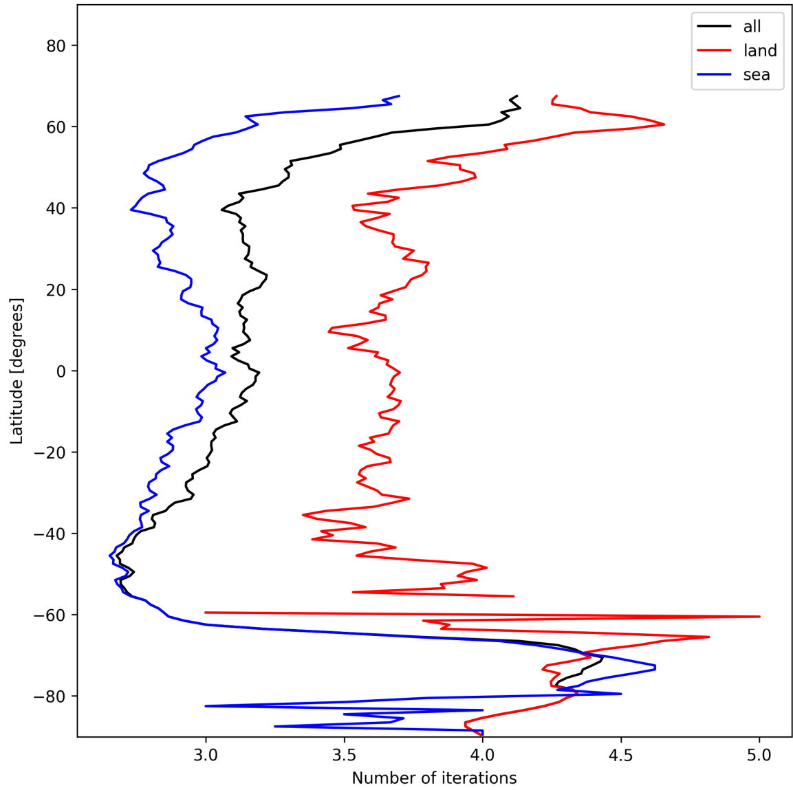
Figure 22: Zonal average of “Number of iterations” for 2024-11-22 to 2024-11-24.
