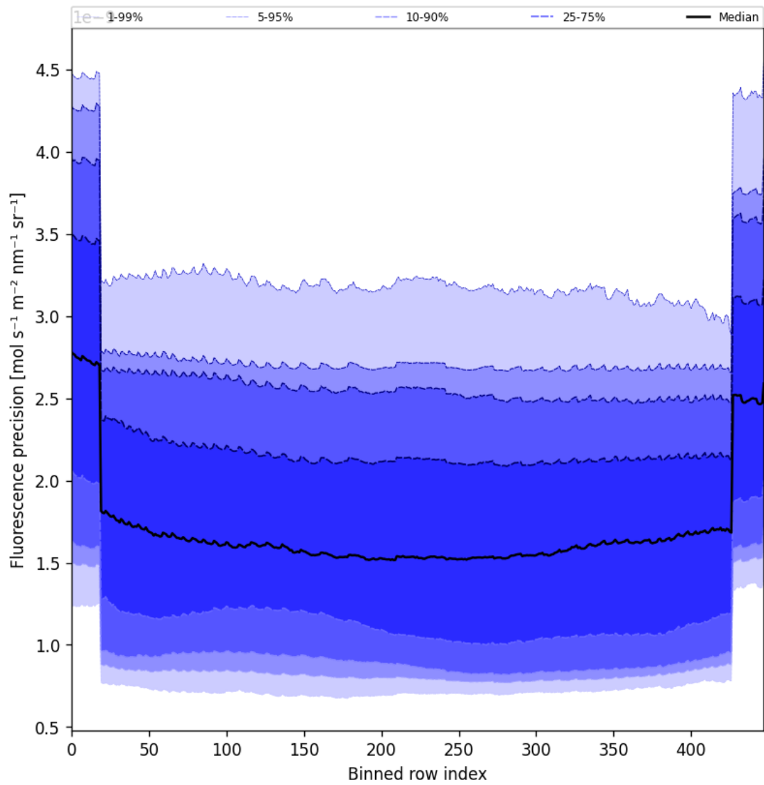
Figure 58: Along track statistics of “Fluorescence precision” for 2024-11-22 to 2024-11-24
