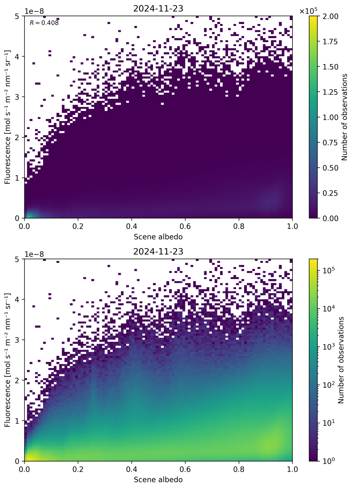
Figure 104: Scatter density plot of “Scene albedo” against “Fluorescence” for 2024-11-22 to 2024-11-24.
