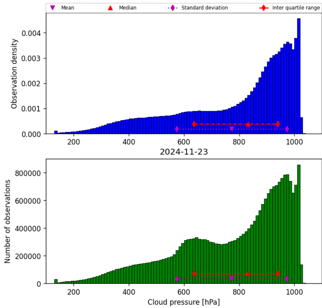
Figure 30: Histogram of “Cloud pressure” for 2024-11-22 to 2024-11-24
