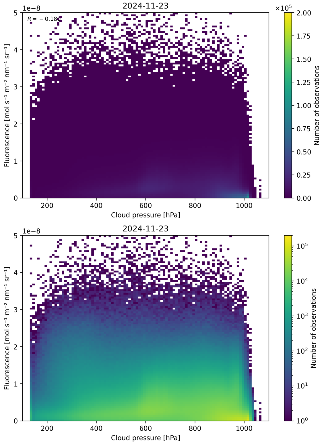
Figure 80: Scatter density plot of “Cloud pressure” against “Fluorescence” for 2024-11-22 to 2024-11-24.
