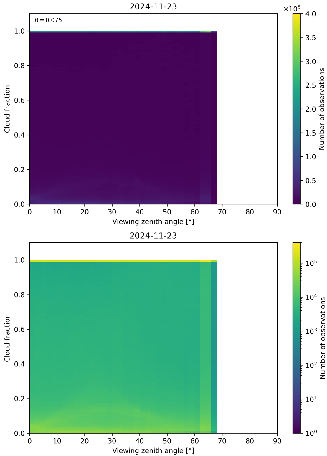
Figure 120: Scatter density plot of “Viewing zenith angle” against “Cloud fraction” for 2024-11-22 to 2024-11-24.
