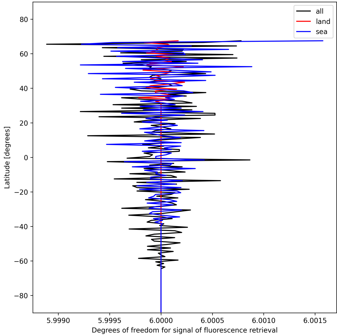
Figure 26: Zonal average of “Degrees of freedom for signal of fluorescence retrieval” for 2024-11-22 to 2024-11-24.
