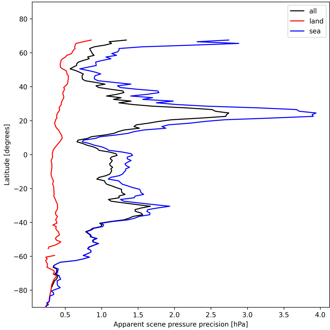
Figure 20: Zonal average of “Apparent scene pressure precision” for 2024-11-22 to 2024-11-24.
