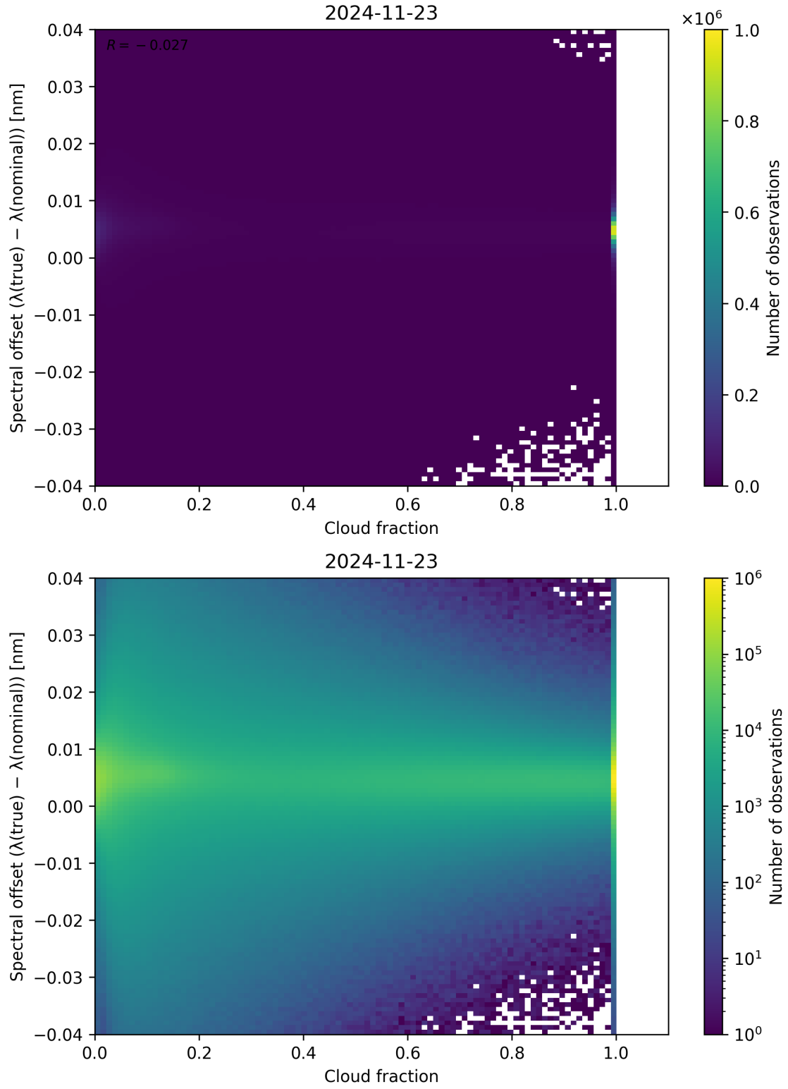
Figure 76: Scatter density plot of “Cloud fraction” against “Spectral offset ( \lambda_{\text{true}} - \lambda_{\text{nominal}} )” for 2024-11-22 to 2024-11-24.
