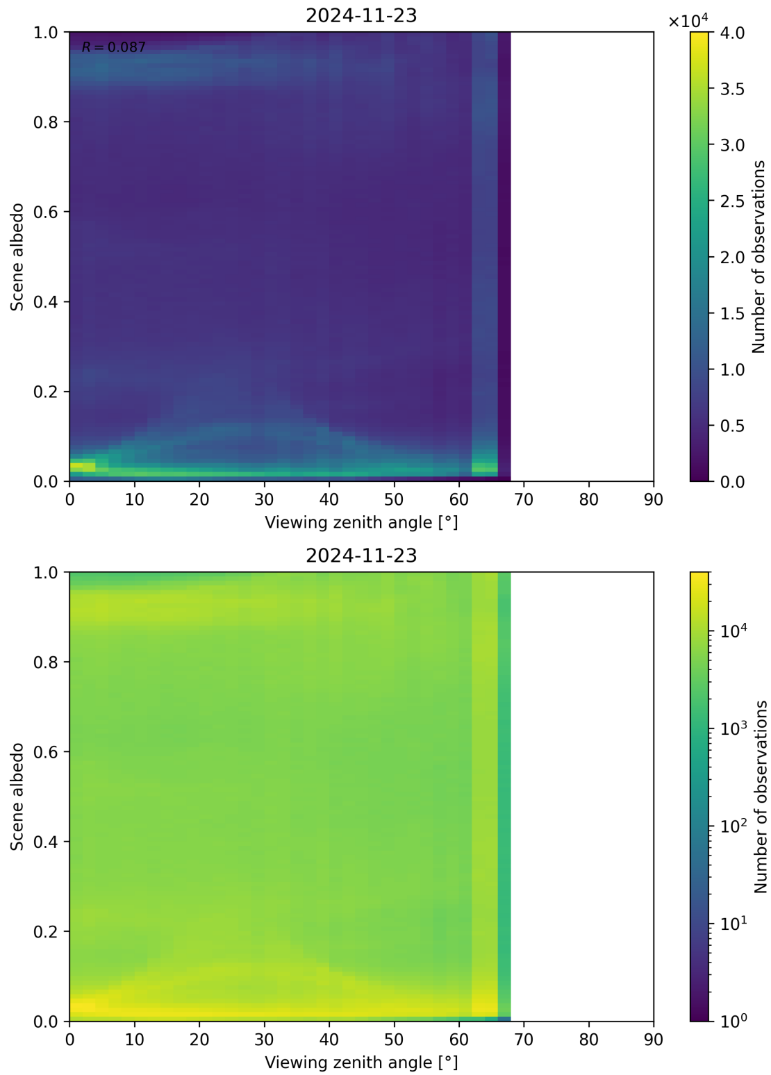
Figure 126: Scatter density plot of “Viewing zenith angle” against “Scene albedo” for 2024-11-22 to 2024-11-24.
