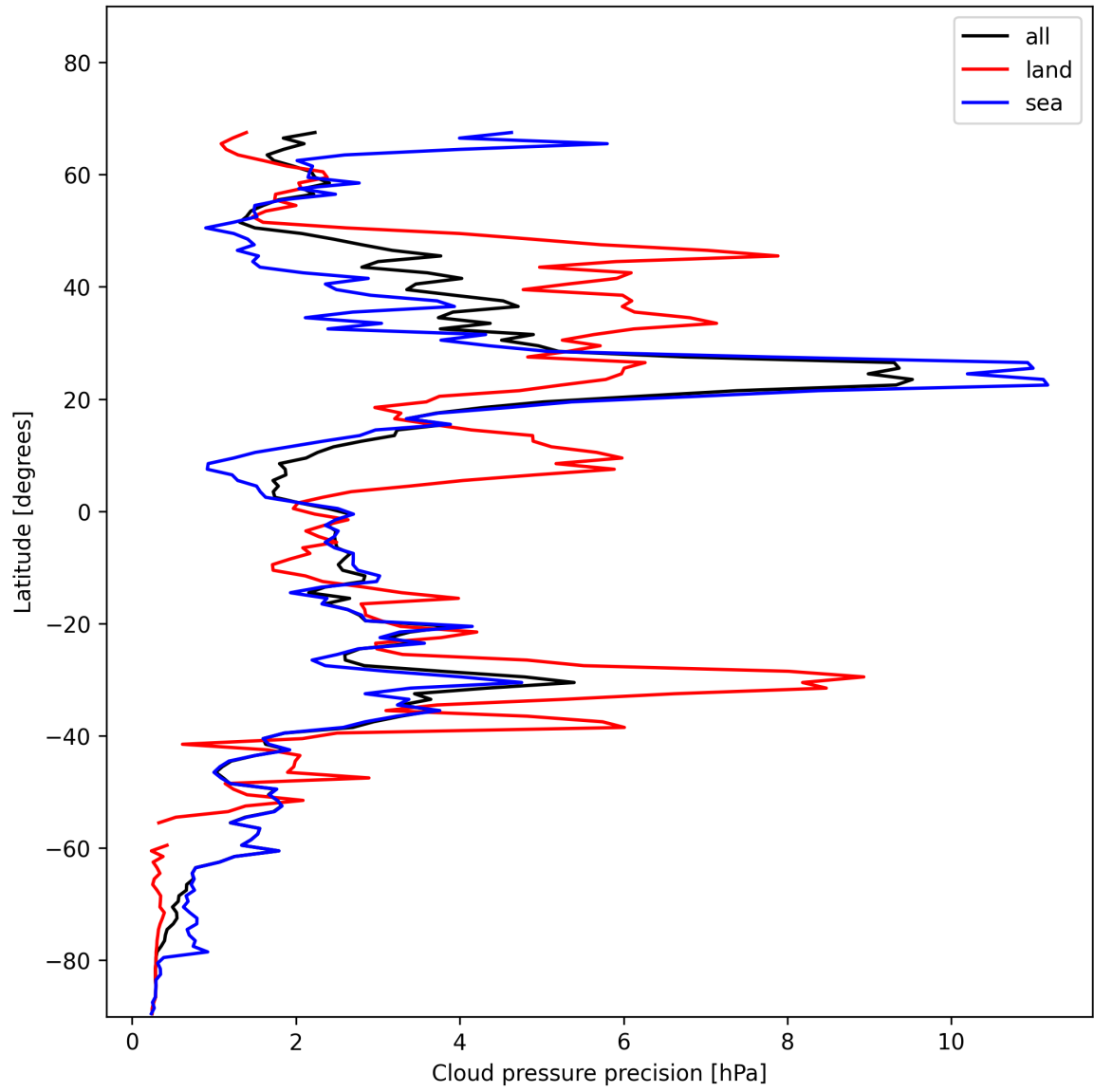
Figure 14: Zonal average of “Cloud pressure precision” for 2024-11-22 to 2024-11-24.
