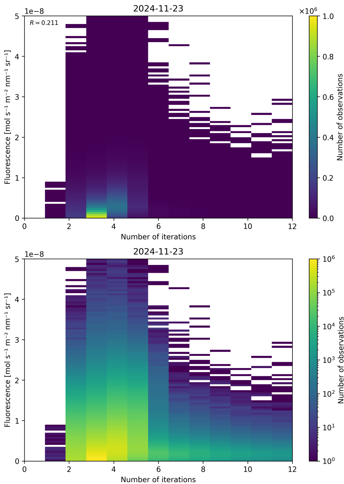
Figure 98: Scatter density plot of “Number of iterations” against “Fluorescence” for 2024-11-22 to 2024-11-24.
