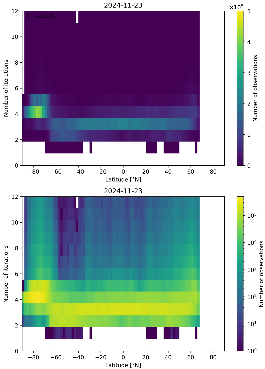
Figure 93: Scatter density plot of “Latitude” against “Number of iterations” for 2024-11-22 to 2024-11-24.
