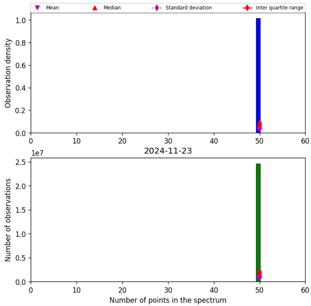
Figure 44: Histogram of “Number of points in the spectrum” for 2024-11-22 to 2024-11-24
