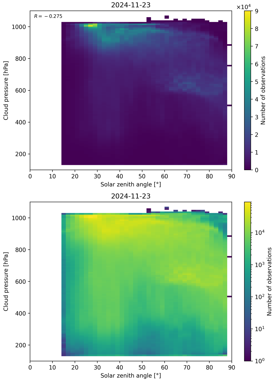
Figure 111: Scatter density plot of “Solar zenith angle” against “Cloud pressure” for 2024-11-22 to 2024-11-24.
