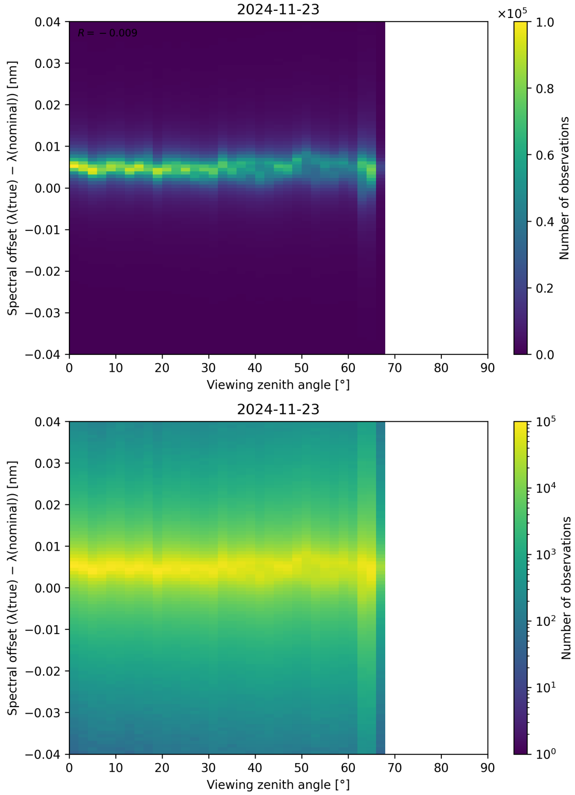
Figure 128: Scatter density plot of “Viewing zenith angle” against “Spectral offset ( \lambda_{\text{true}} - \lambda_{\text{nominal}} )” for 2024-11-22 to 2024-11-24.
