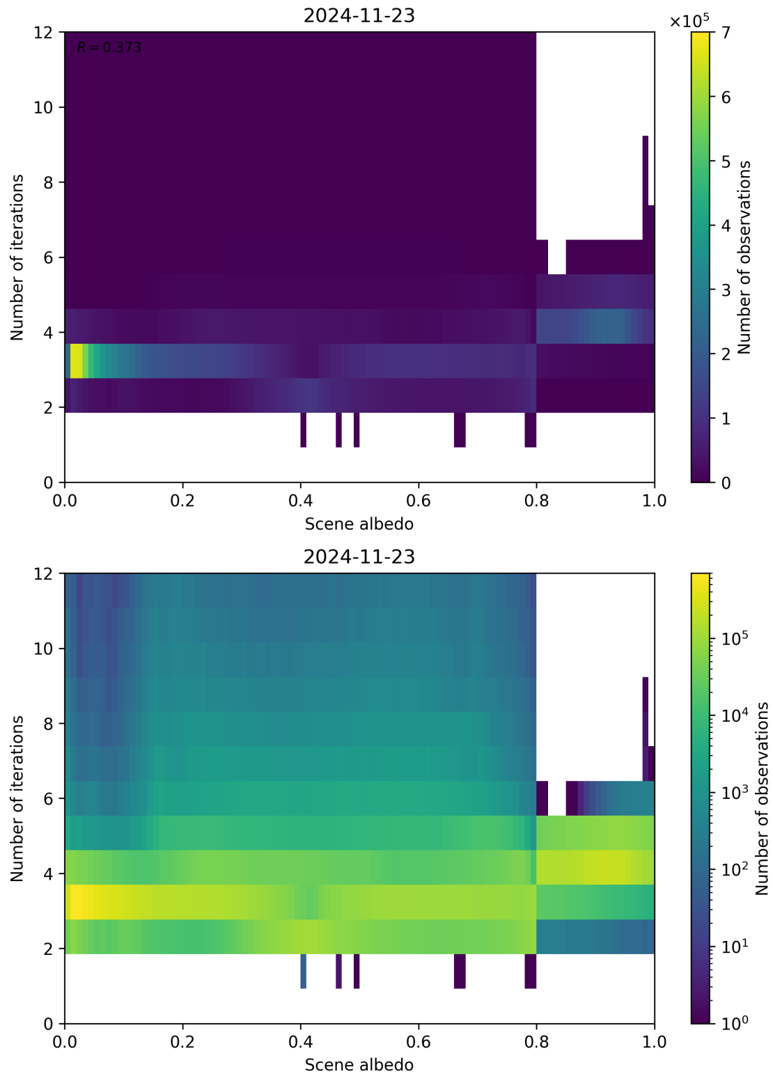
Figure 105: Scatter density plot of “Scene albedo” against “Number of iterations” for 2024-11-22 to 2024-11-24.
