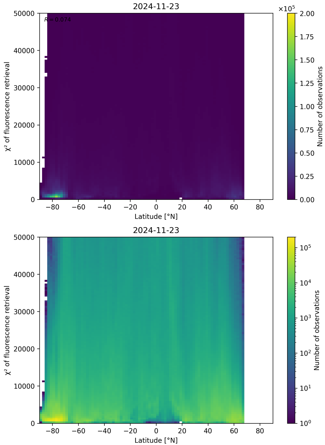
Figure 89: Scatter density plot of “Latitude” against “ \chi^2 of fluorescence retrieval” for 2024-11-22 to 2024-11-24.
