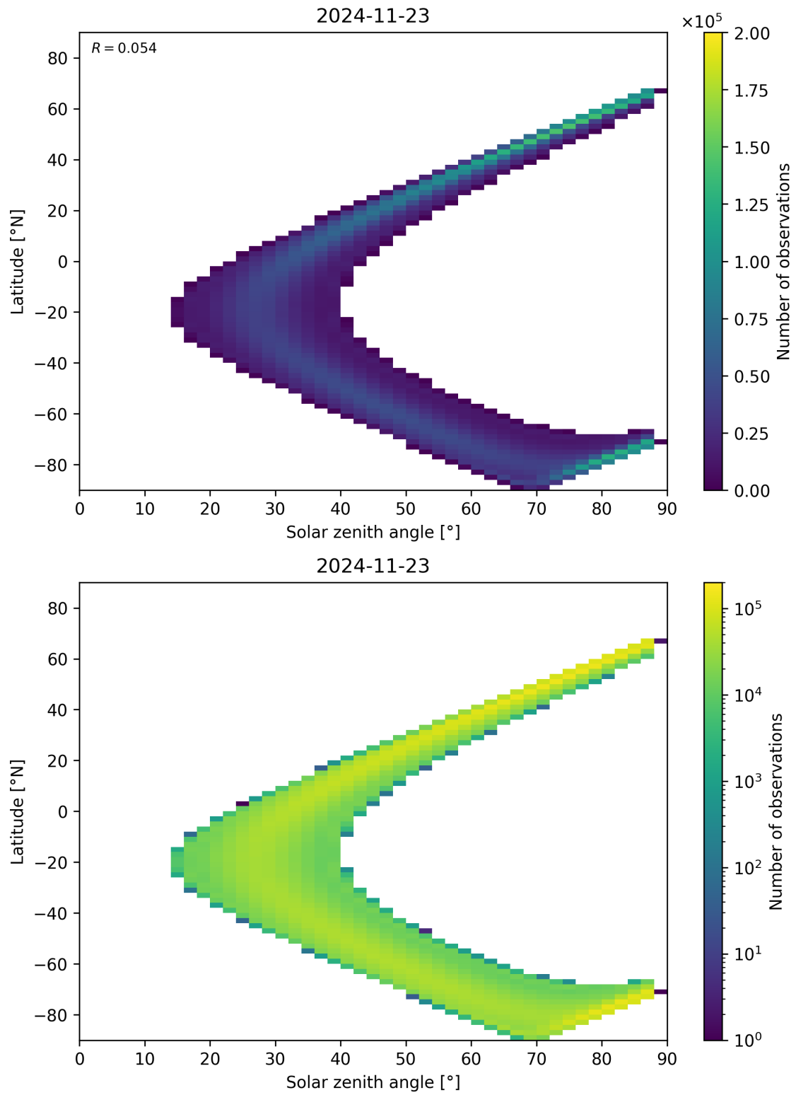
Figure 113: Scatter density plot of “Solar zenith angle” against “Latitude” for 2024-11-22 to 2024-11-24.
