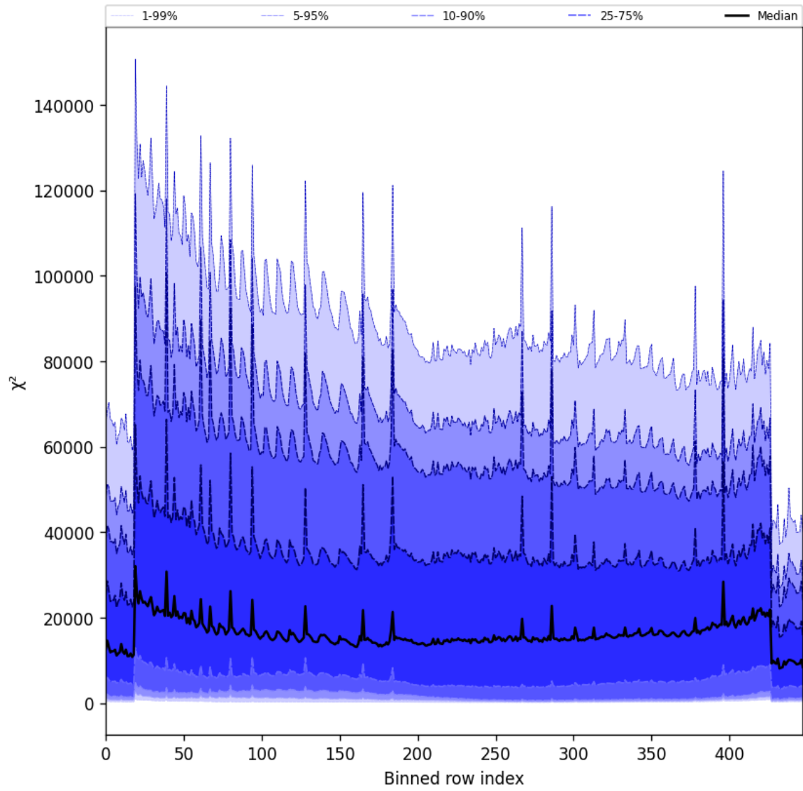
Figure 55: Along track statistics of “ \chi^2 ” for 2024-11-22 to 2024-11-24
