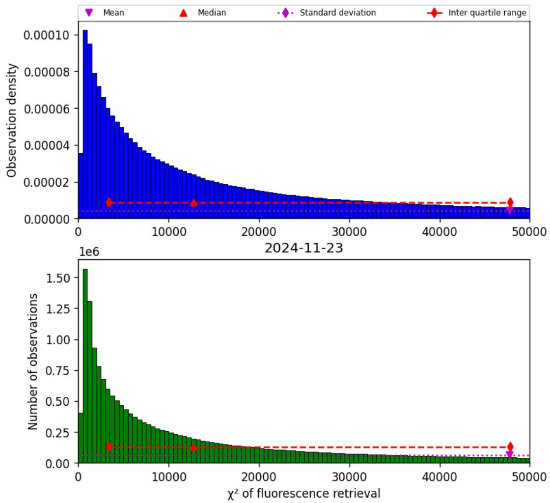
Figure 42: Histogram of “ \chi^2 of fluorescence retrieval” for 2024-11-22 to 2024-11-24
