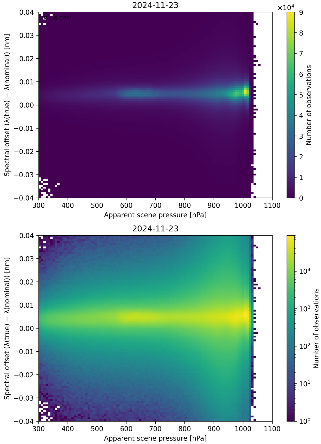
Figure 67: Scatter density plot of “Apparent scene pressure” against “Spectral offset ( \lambda_{\text{true}} - \lambda_{\text{nominal}} )” for 2024-11-22 to 2024-11-24.
