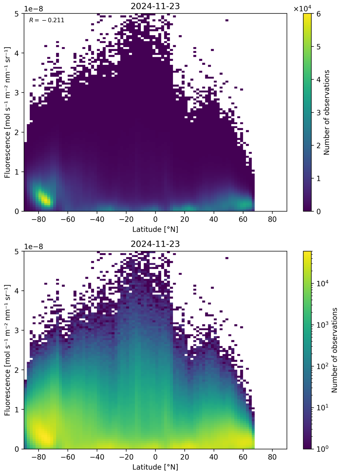
Figure 92: Scatter density plot of “Latitude” against “Fluorescence” for 2024-11-22 to 2024-11-24.
