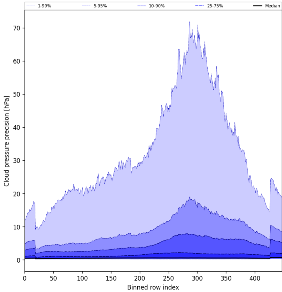
Figure 48: Along track statistics of “Cloud pressure precision” for 2024-11-22 to 2024-11-24
