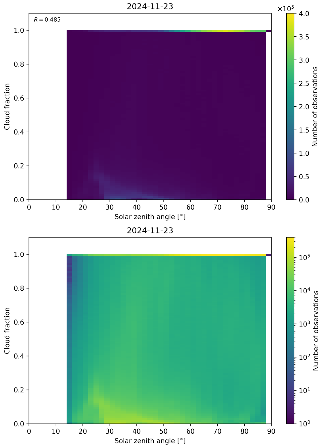
Figure 110: Scatter density plot of “Solar zenith angle” against “Cloud fraction” for 2024-11-22 to 2024-11-24.
