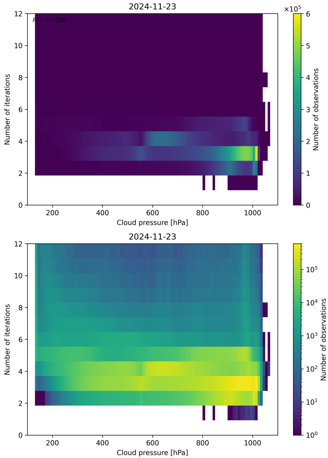
Figure 81: Scatter density plot of “Cloud pressure” against “Number of iterations” for 2024-11-22 to 2024-11-24.
