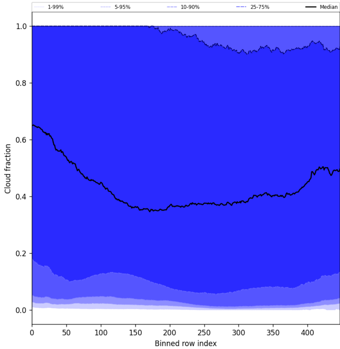
Figure 49: Along track statistics of “Cloud fraction” for 2024-11-22 to 2024-11-24
