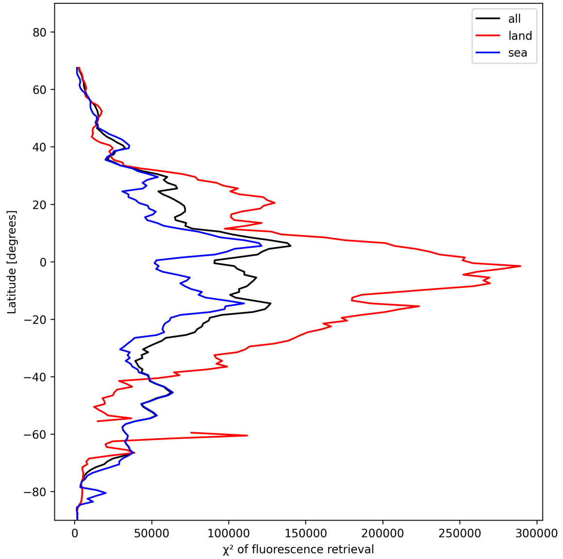
Figure 25: Zonal average of “ \chi^2 of fluorescence retrieval” for 2024-11-22 to 2024-11-24.
