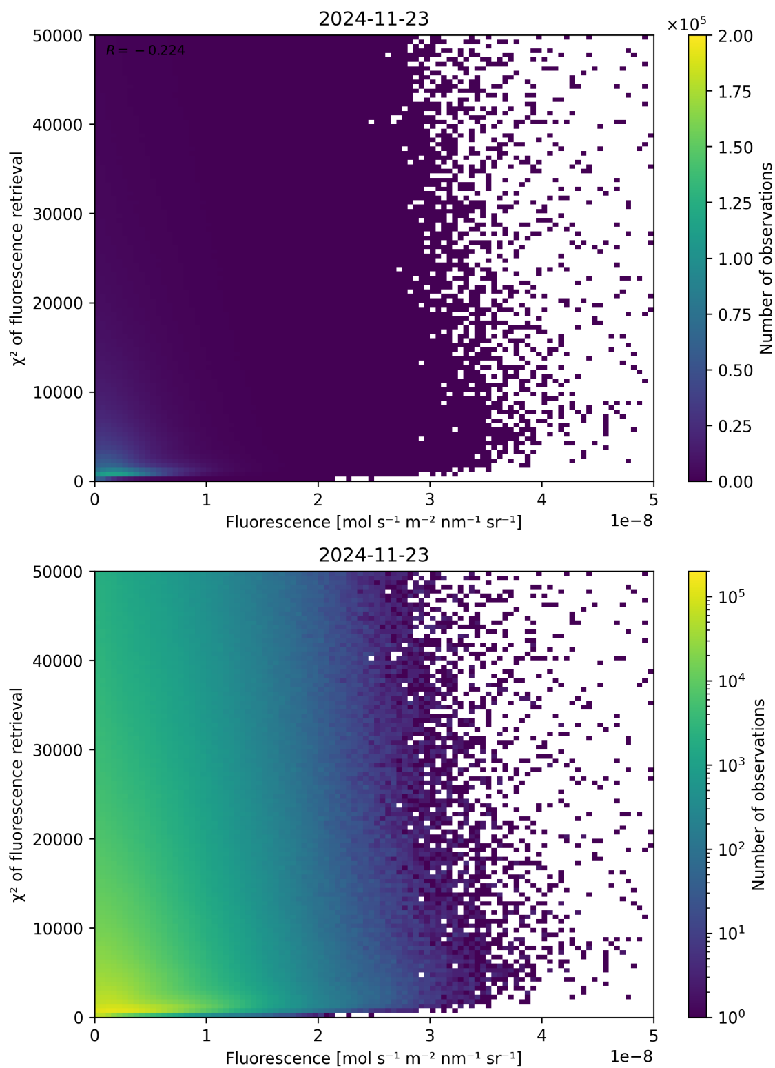
Figure 85: Scatter density plot of “Fluorescence” against “ \chi^2 of fluorescence retrieval” for 2024-11-22 to 2024-11-24.
