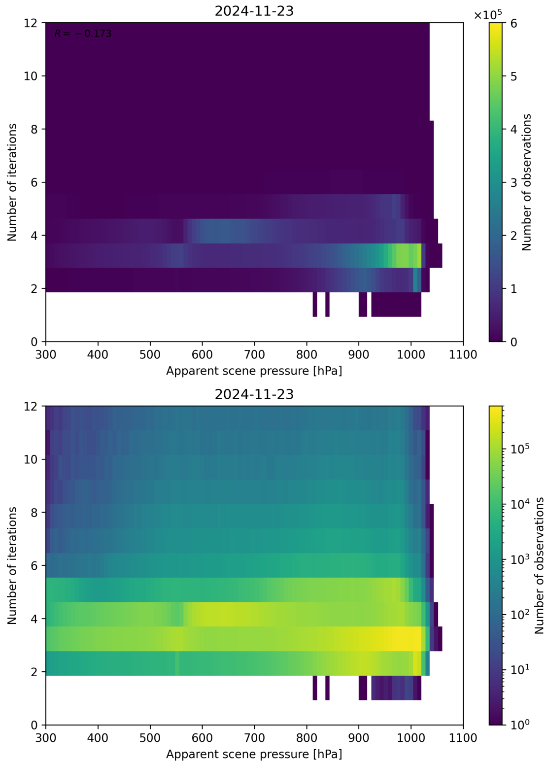
Figure 65: Scatter density plot of “Apparent scene pressure” against “Number of iterations” for 2024-11-22 to 2024-11-24.
