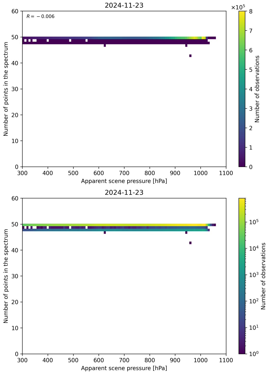
Figure 66: Scatter density plot of “Apparent scene pressure” against “Number of points in the spectrum” for 2024-11-22 to 2024-11-24.
