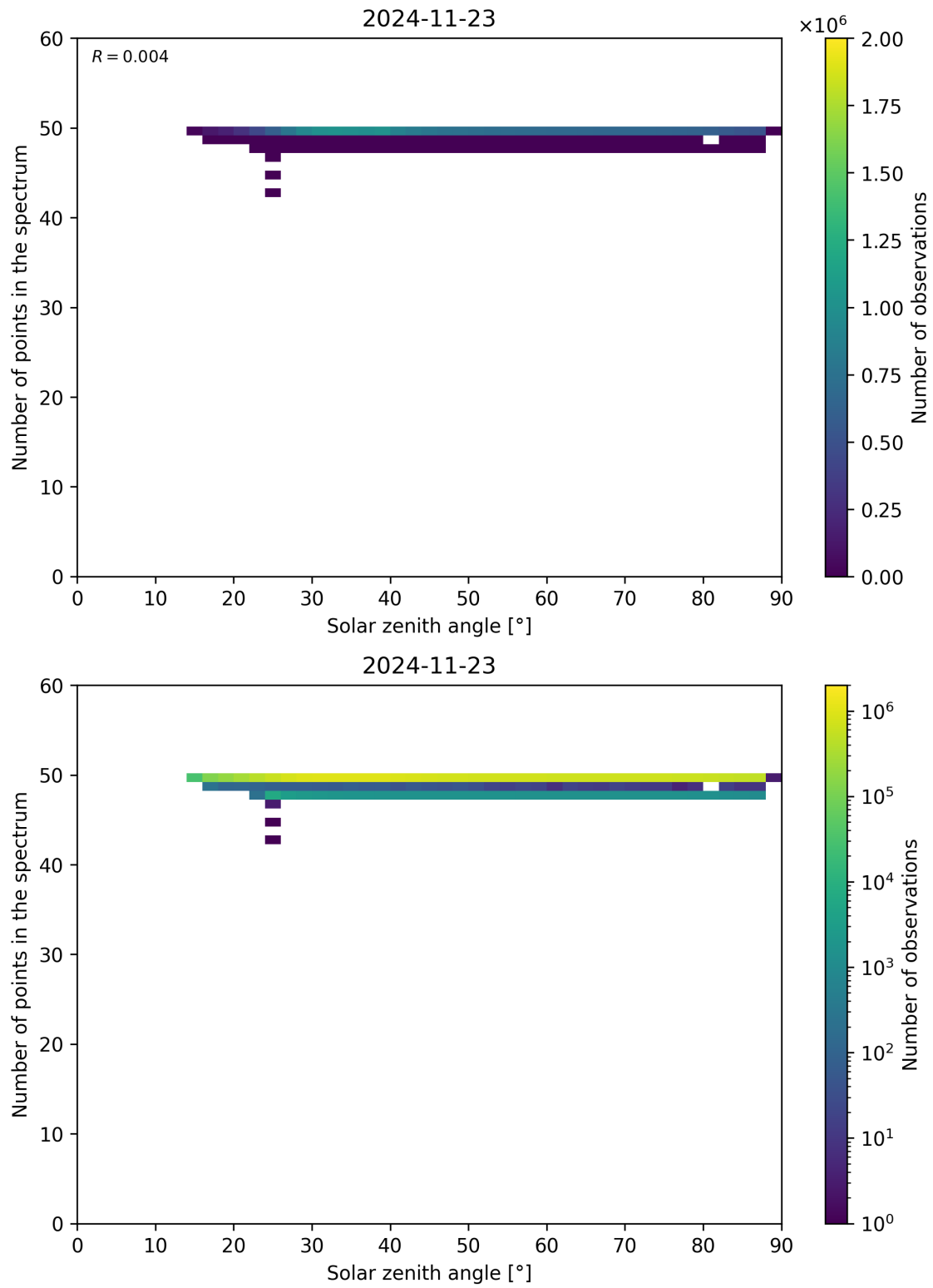
Figure 115: Scatter density plot of “Solar zenith angle” against “Number of points in the spectrum” for 2024-11-22 to 2024-11-24.
