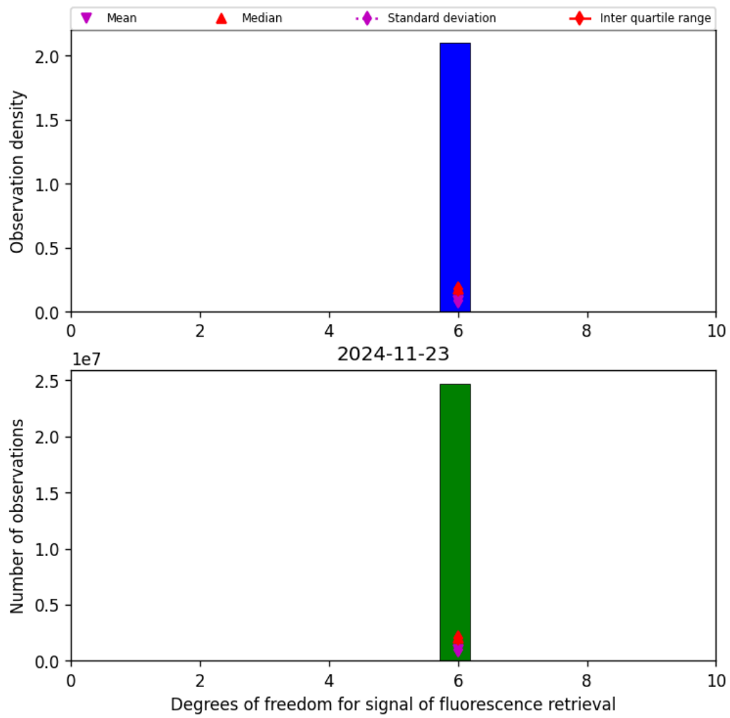
Figure 43: Histogram of "Degrees of freedom for signal of fluorescence retrieval" for 2024-11-22 to 2024-11-24
