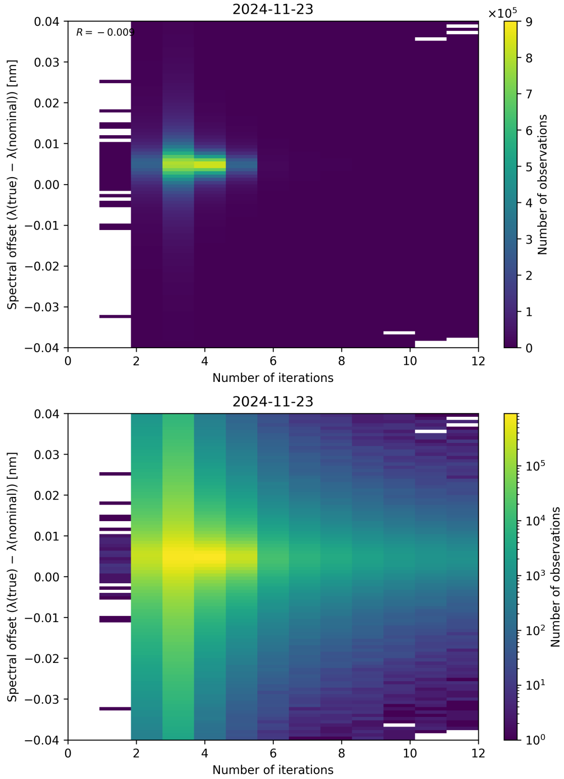
Figure 100: Scatter density plot of “Number of iterations” against “Spectral offset ( \lambda_{\text{true}} - \lambda_{\text{nominal}} )” for 2024-11-22 to 2024-11-24.
