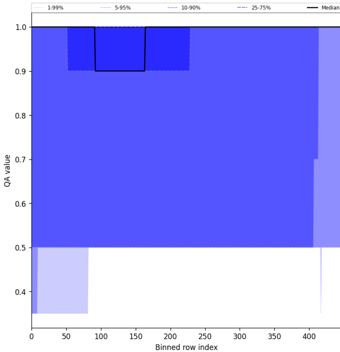
Figure 46: Along track statistics of “QA value” for 2024-11-22 to 2024-11-24
