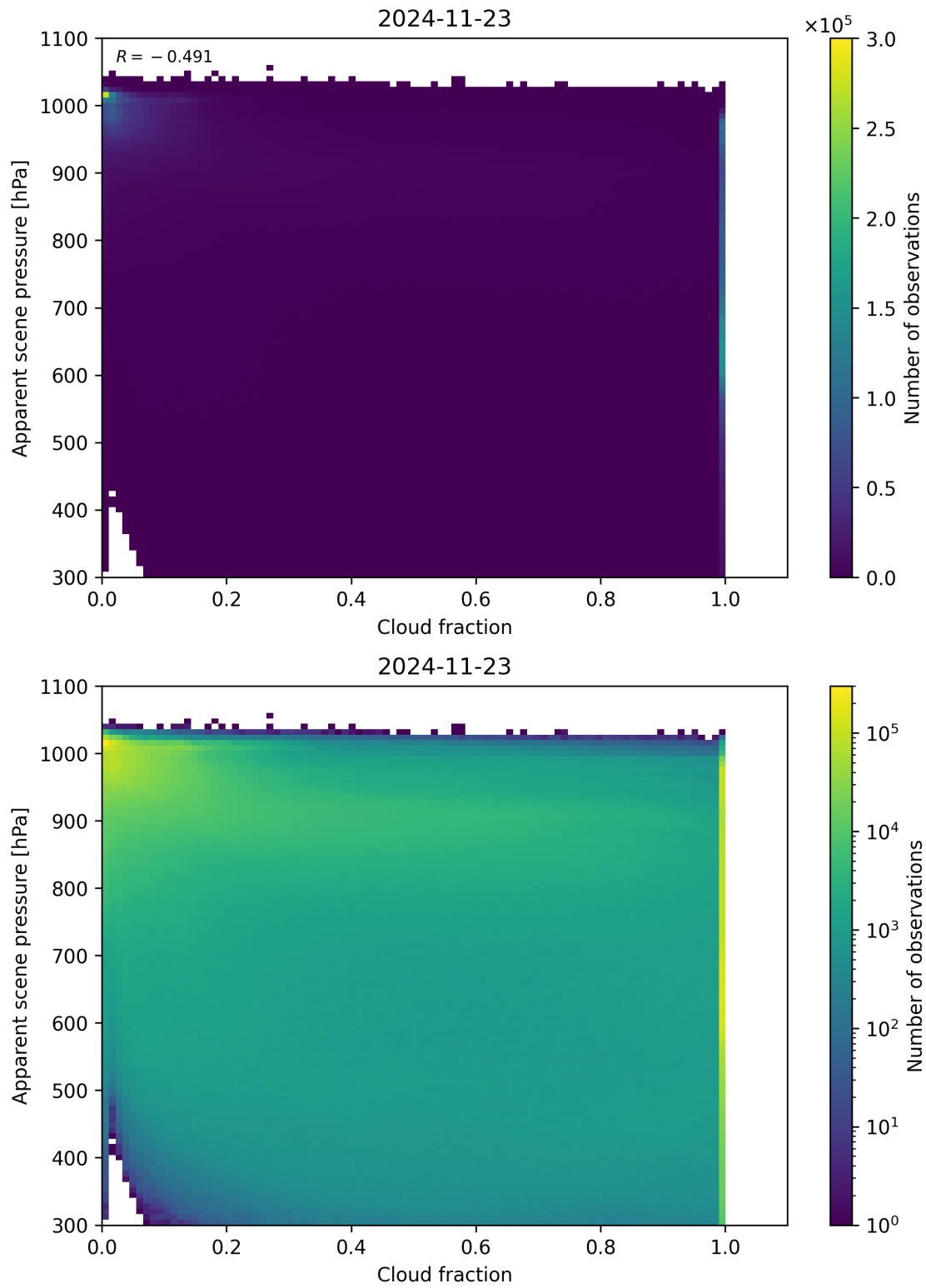
Figure 70: Scatter density plot of “Cloud fraction” against “Apparent scene pressure” for 2024-11-22 to 2024-11-24.
