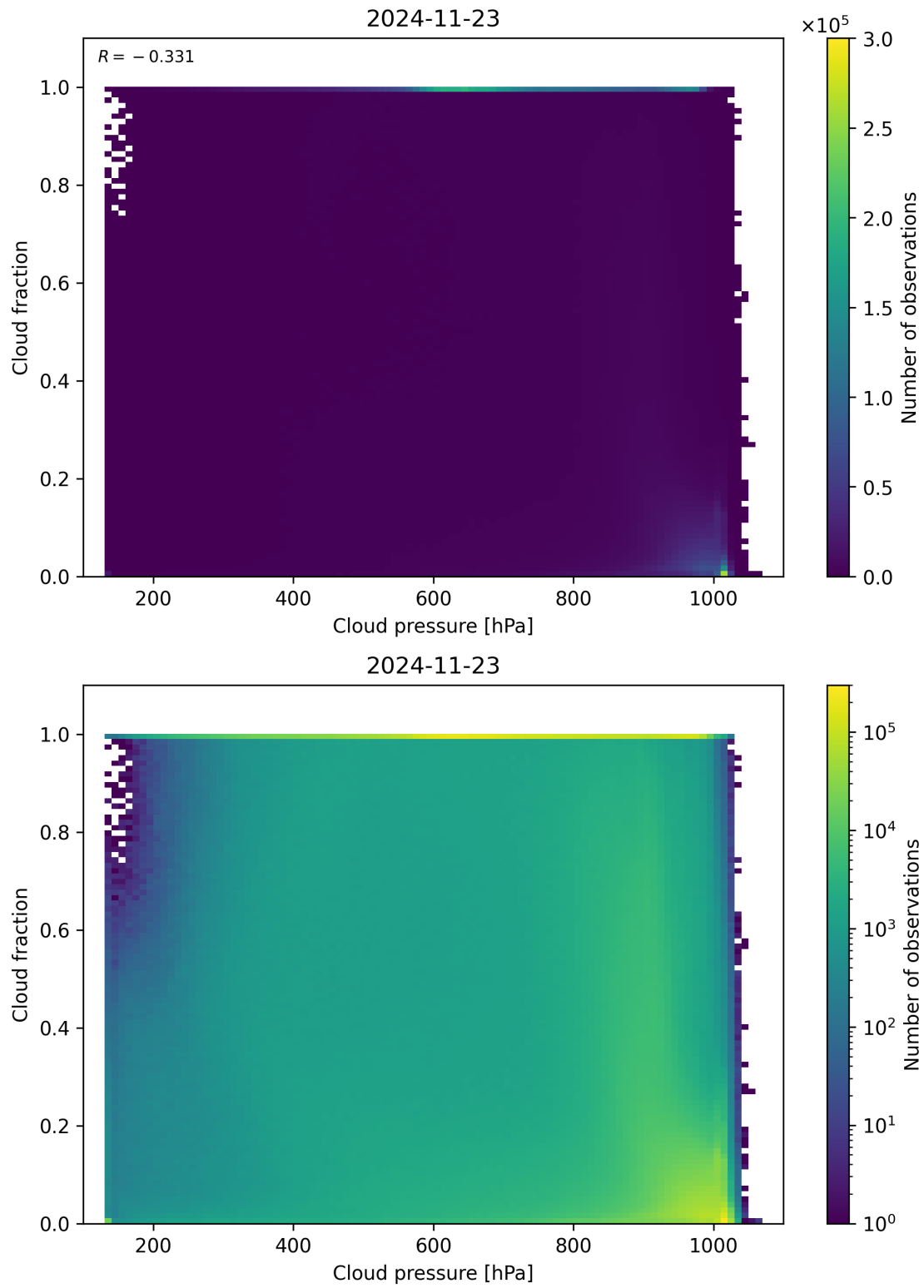
Figure 79: Scatter density plot of “Cloud pressure” against “Cloud fraction” for 2024-11-22 to 2024-11-24.
