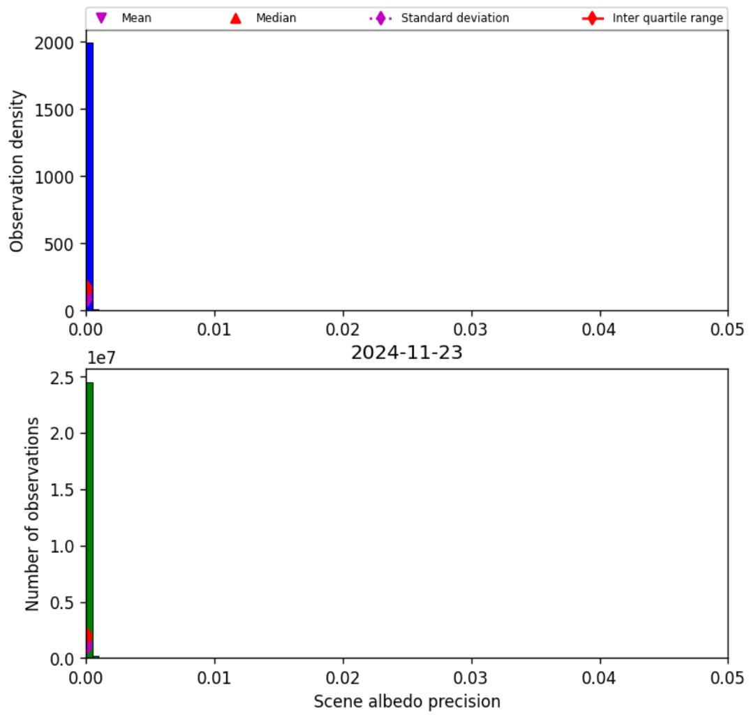
Figure 35: Histogram of “Scene albedo precision” for 2024-11-22 to 2024-11-24
