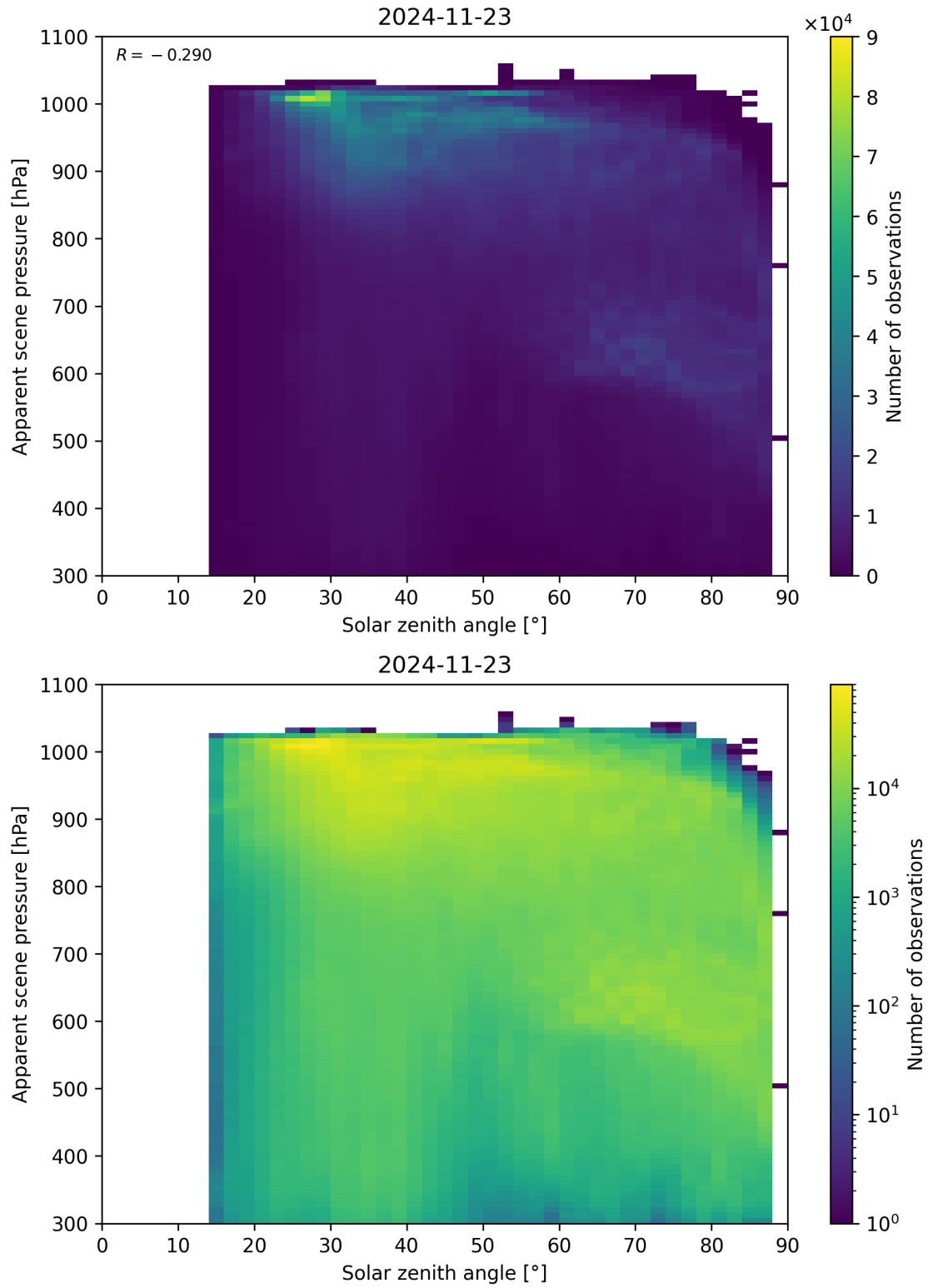
Figure 108: Scatter density plot of “Solar zenith angle” against “Apparent scene pressure” for 2024-11-22 to 2024-11-24.
