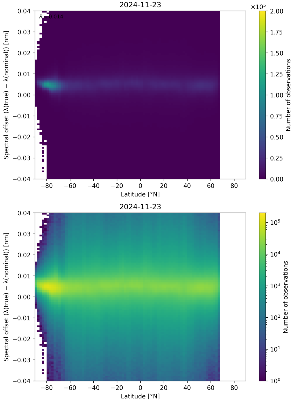
Figure 96: Scatter density plot of “Latitude” against “Spectral offset ( \lambda_{\text{true}} - \lambda_{\text{nominal}} )” for 2024-11-22 to 2024-11-24.
