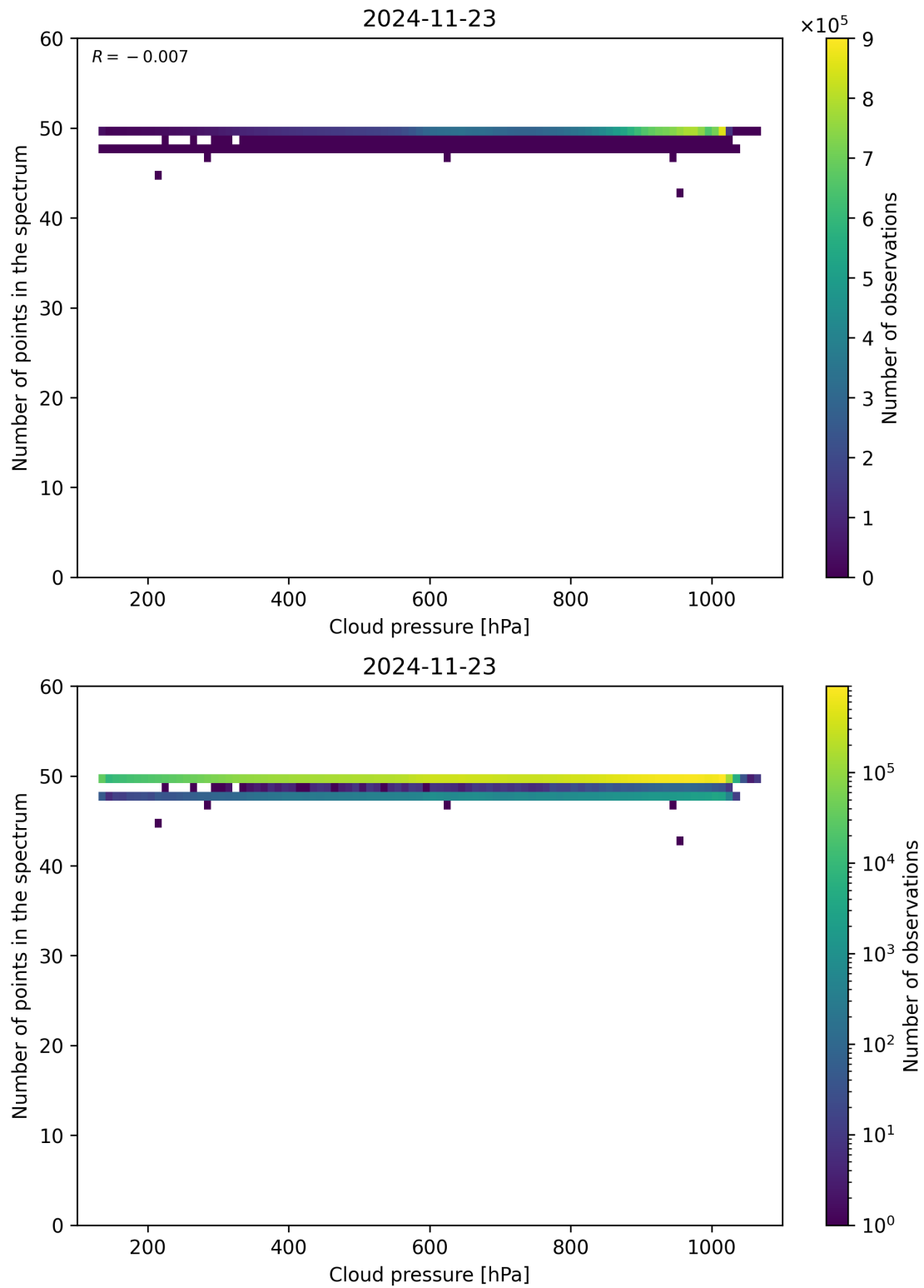
Figure 82: Scatter density plot of “Cloud pressure” against “Number of points in the spectrum” for 2024-11-22 to 2024-11-24.
