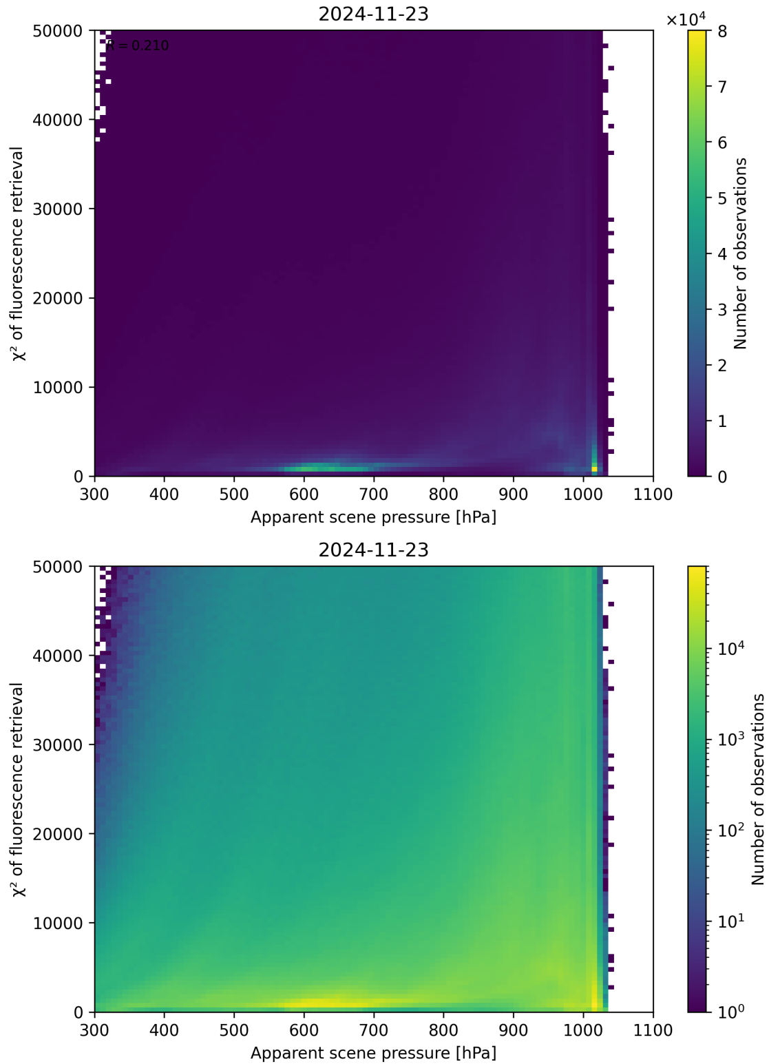
Figure 63: Scatter density plot of “Apparent scene pressure” against “ \chi^2 of fluorescence retrieval” for 2024-11-22 to 2024-11-24.
