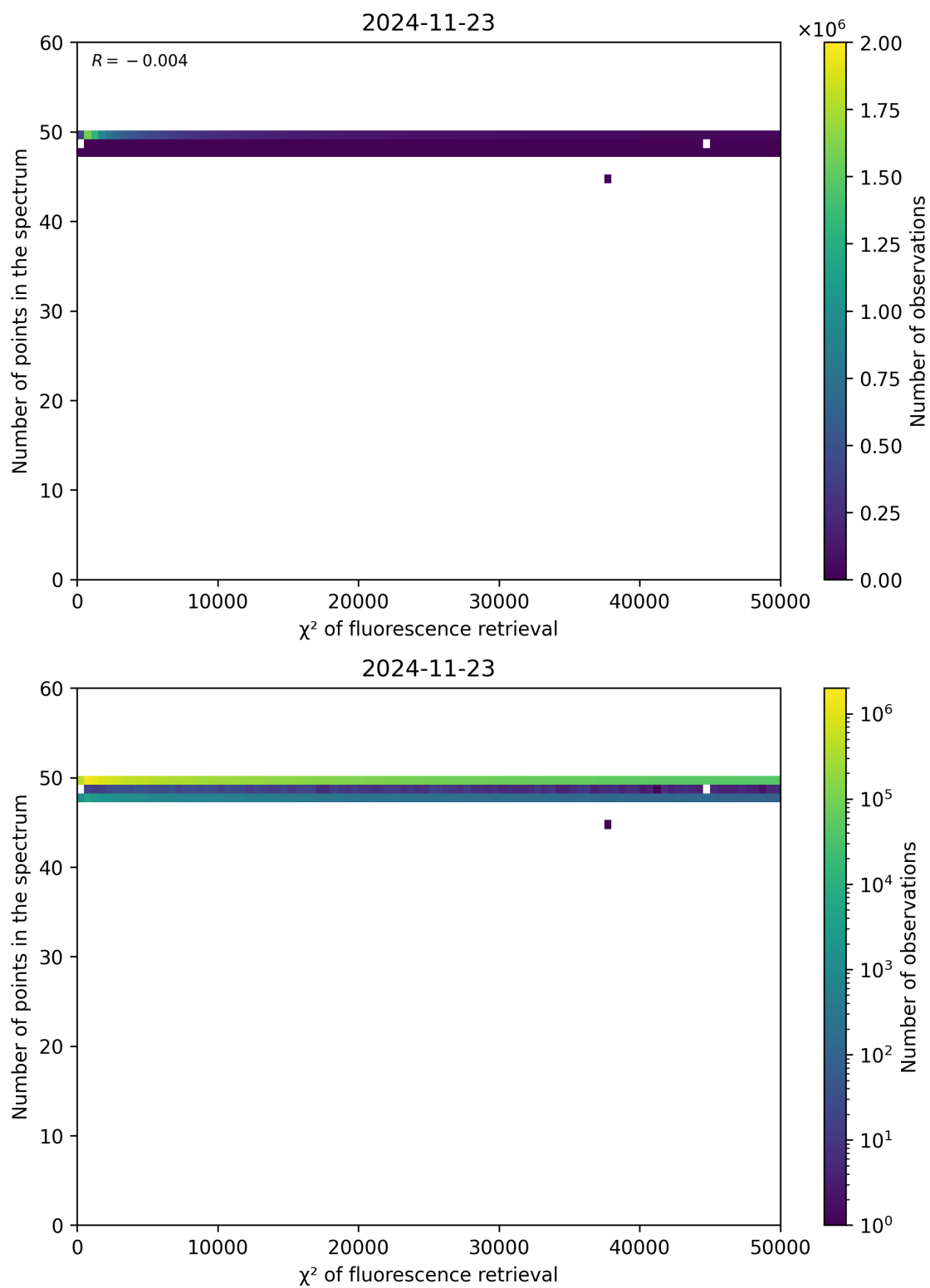
Figure 68: Scatter density plot of “ \chi^2 of fluorescence retrieval” against “Number of points in the spectrum” for 2024-11-22 to 2024-11-24.
