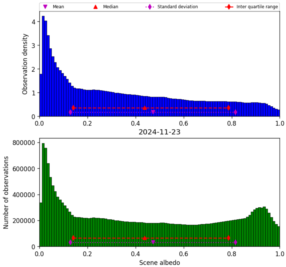
Figure 34: Histogram of “Scene albedo” for 2024-11-22 to 2024-11-24
