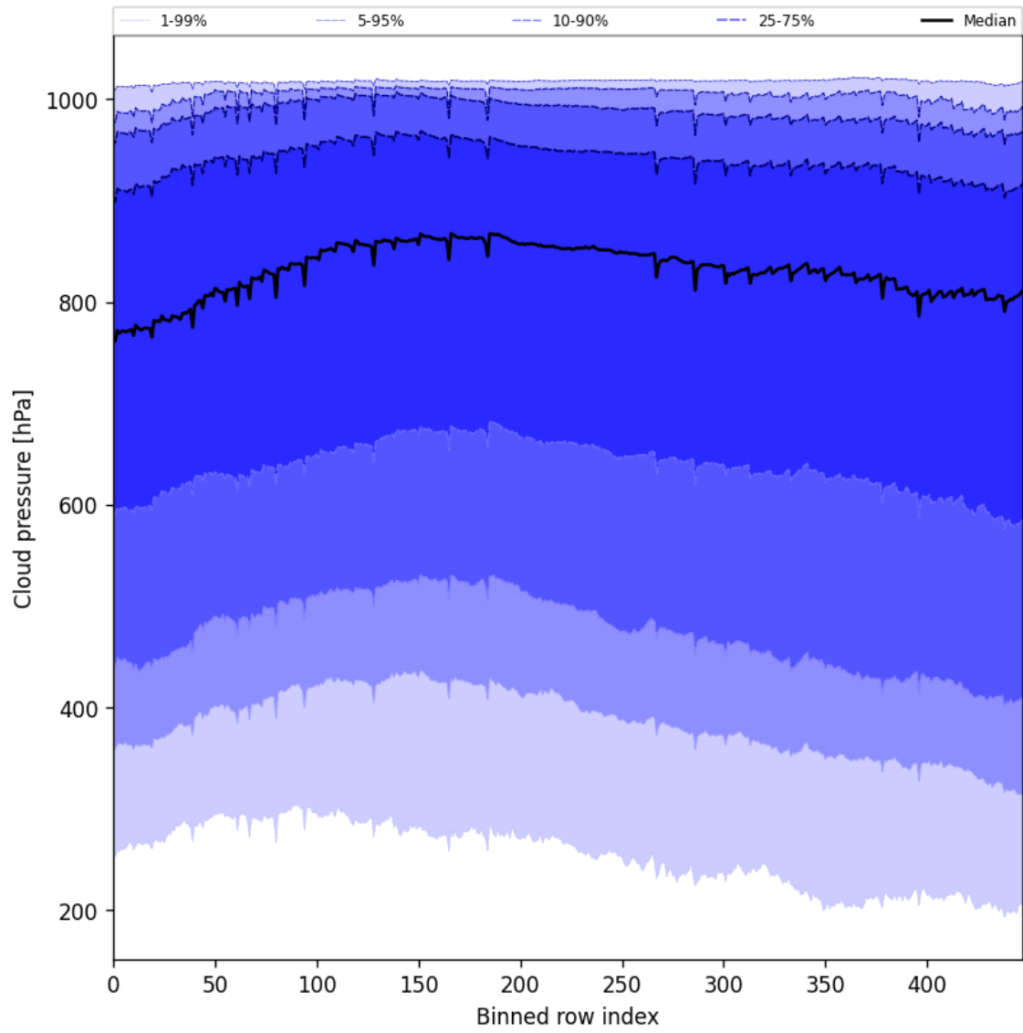
Figure 47: Along track statistics of “Cloud pressure” for 2024-11-22 to 2024-11-24
