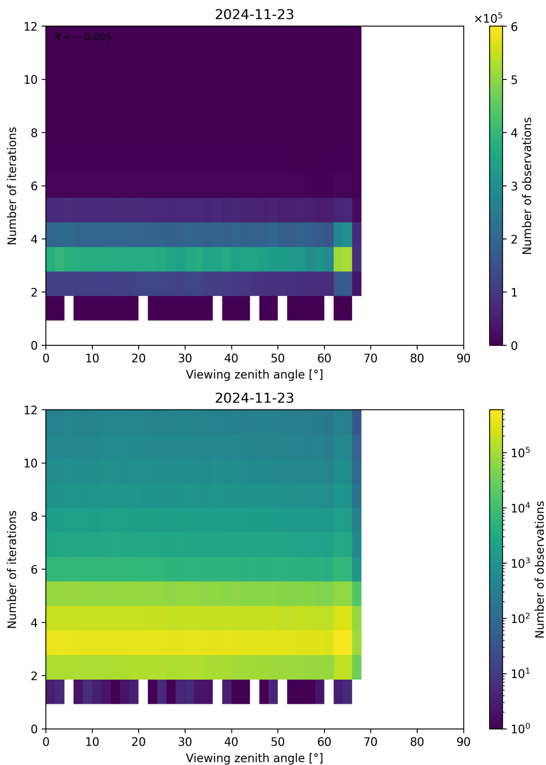
Figure 124: Scatter density plot of “Viewing zenith angle” against “Number of iterations” for 2024-11-22 to 2024-11-24.
