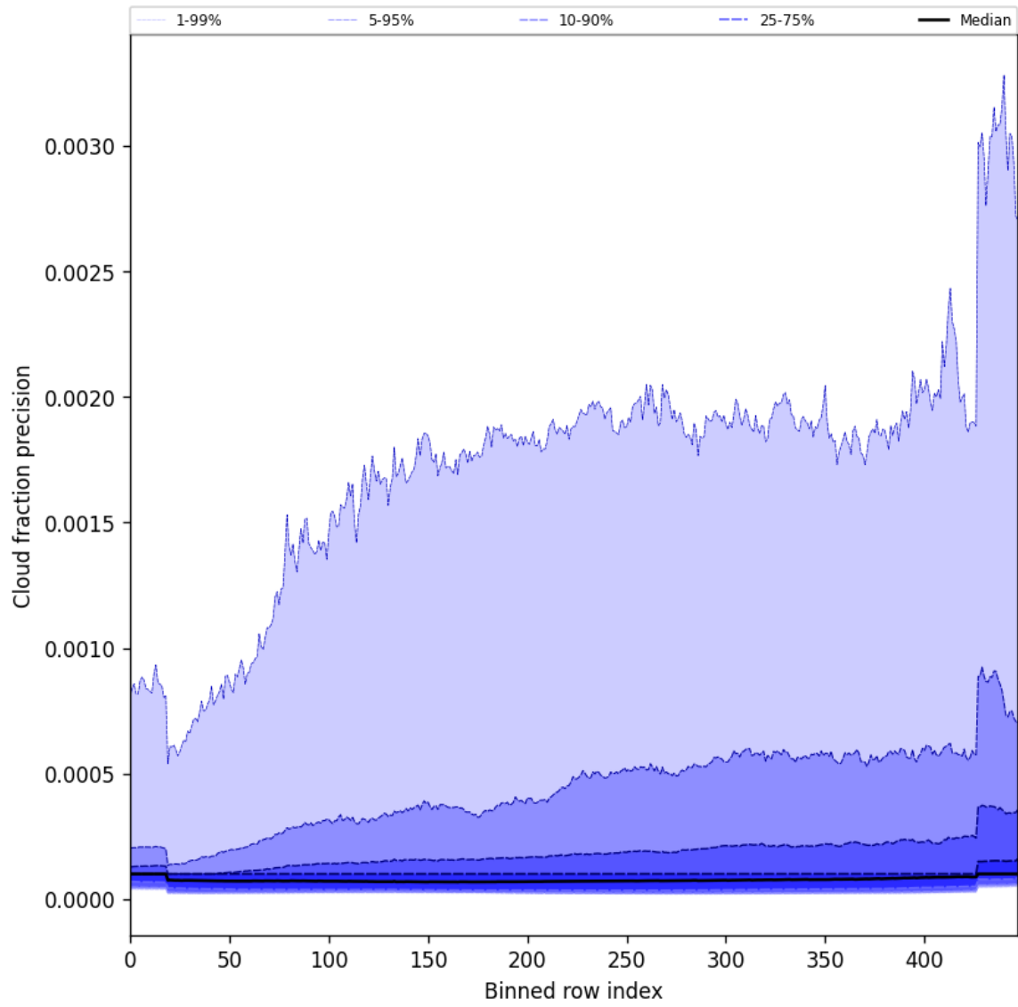
Figure 50: Along track statistics of “Cloud fraction precision” for 2024-11-22 to 2024-11-24
