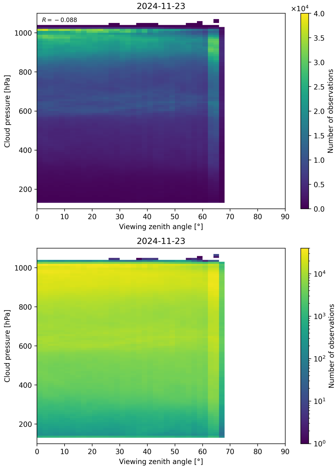
Figure 121: Scatter density plot of “Viewing zenith angle” against “Cloud pressure” for 2024-11-22 to 2024-11-24.
