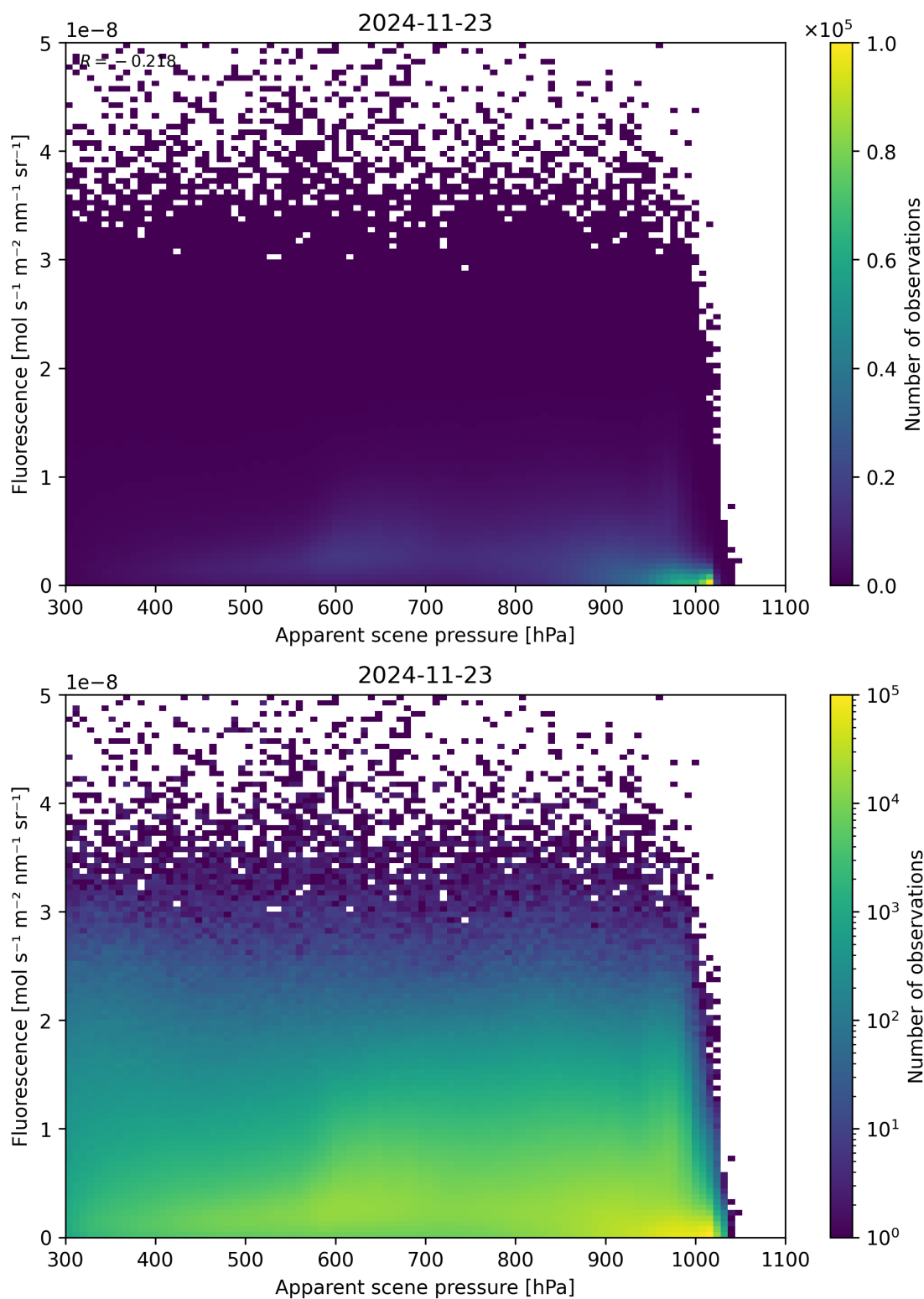
Figure 64: Scatter density plot of “Apparent scene pressure” against “Fluorescence” for 2024-11-22 to 2024-11-24.
