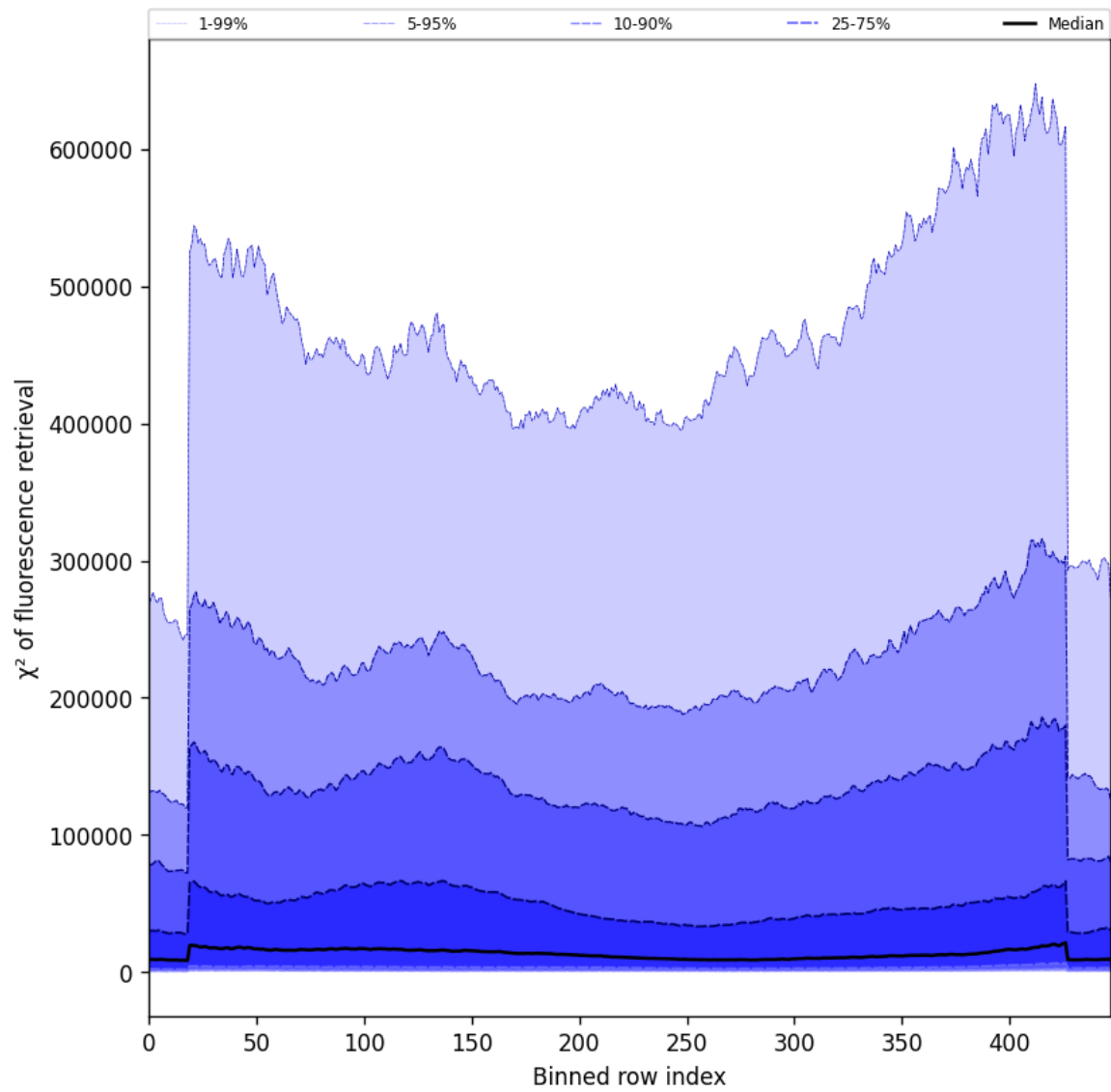
Figure 59: Along track statistics of “ \chi^2 of fluorescence retrieval” for 2024-11-22 to 2024-11-24
