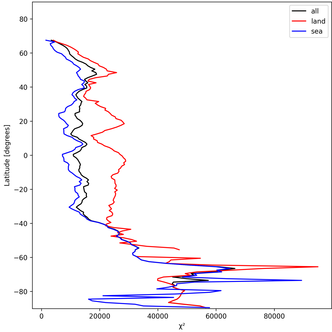
Figure 21: Zonal average of “ \chi^2 ” for 2024-11-22 to 2024-11-24.
