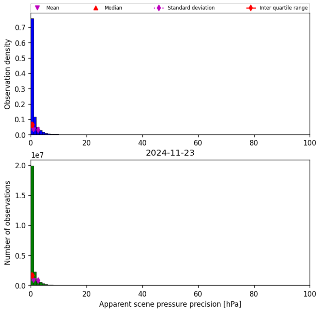
Figure 37: Histogram of “Apparent scene pressure precision” for 2024-11-22 to 2024-11-24
