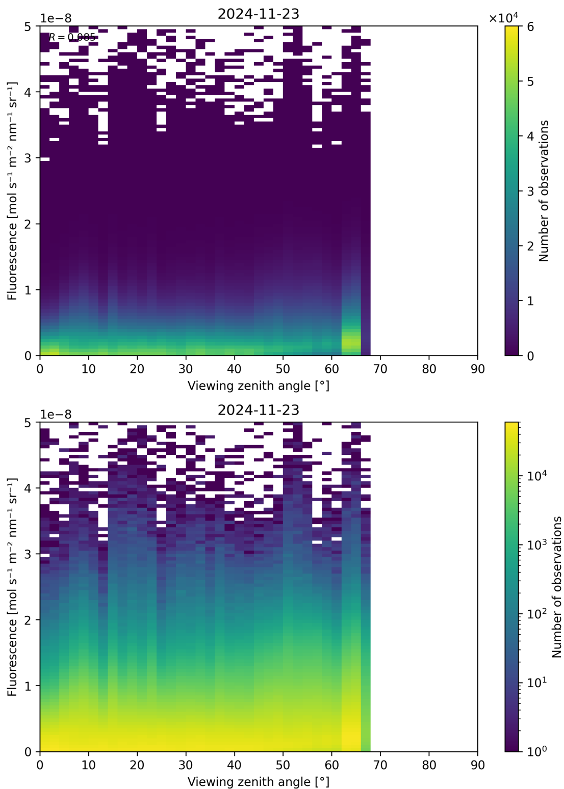
Figure 122: Scatter density plot of “Viewing zenith angle” against “Fluorescence” for 2024-11-22 to 2024-11-24.
