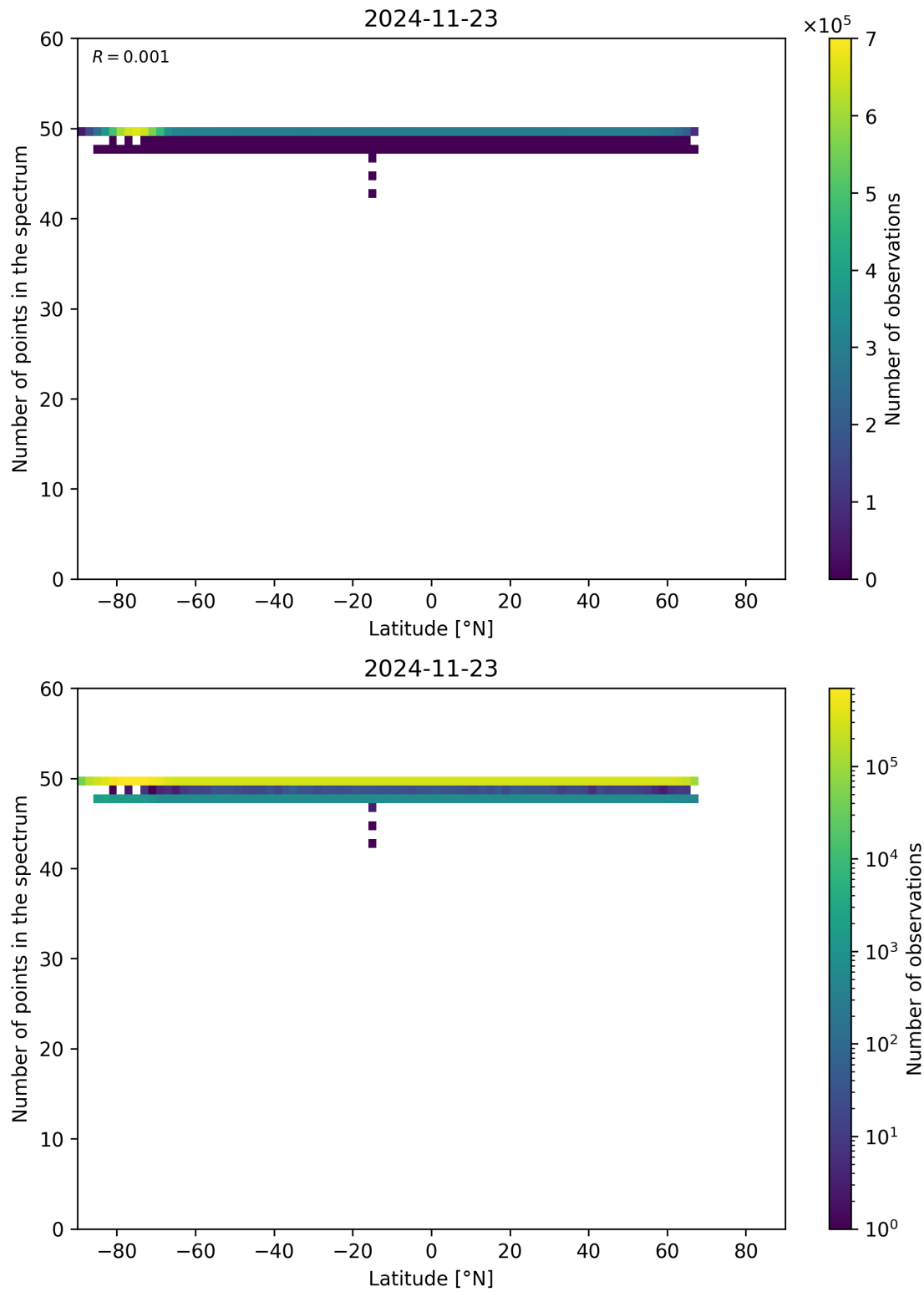
Figure 94: Scatter density plot of “Latitude” against “Number of points in the spectrum” for 2024-11-22 to 2024-11-24.
