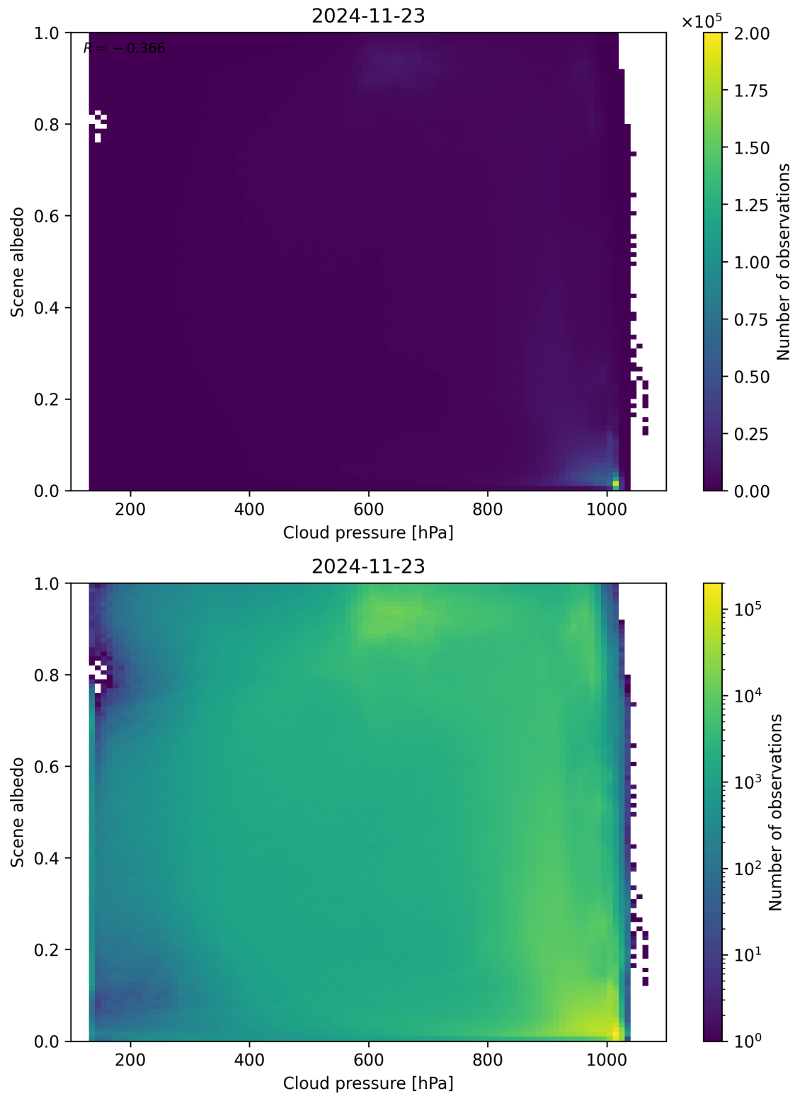
Figure 83: Scatter density plot of “Cloud pressure” against “Scene albedo” for 2024-11-22 to 2024-11-24.
