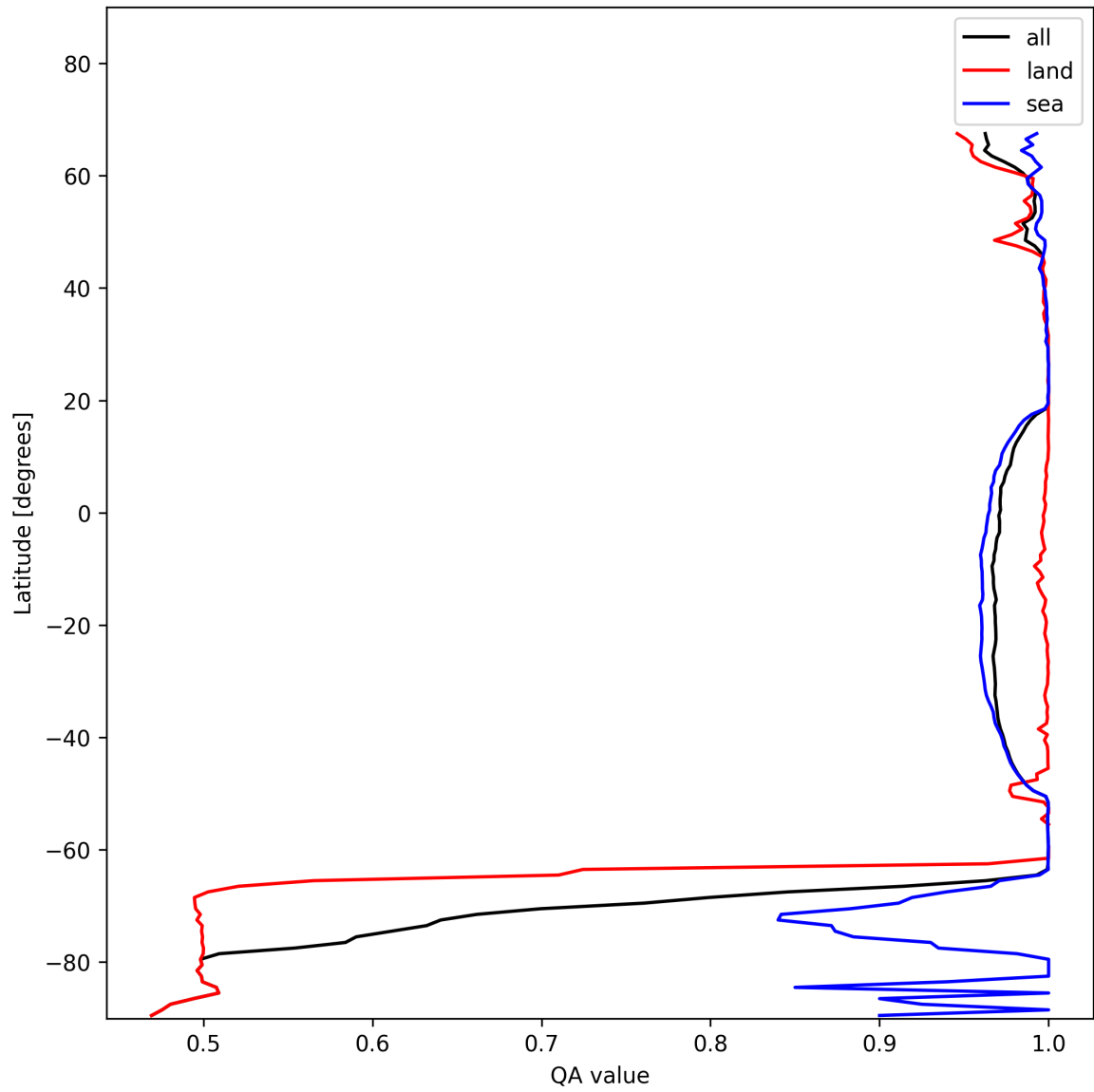
Figure 12: Zonal average of “QA value” for 2024-11-22 to 2024-11-24.
