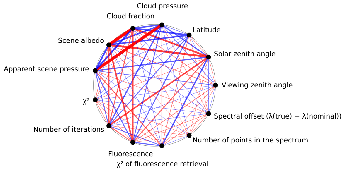
Figure 1: Map of correlation graph for 2024-11-22 to 2024-11-24.
