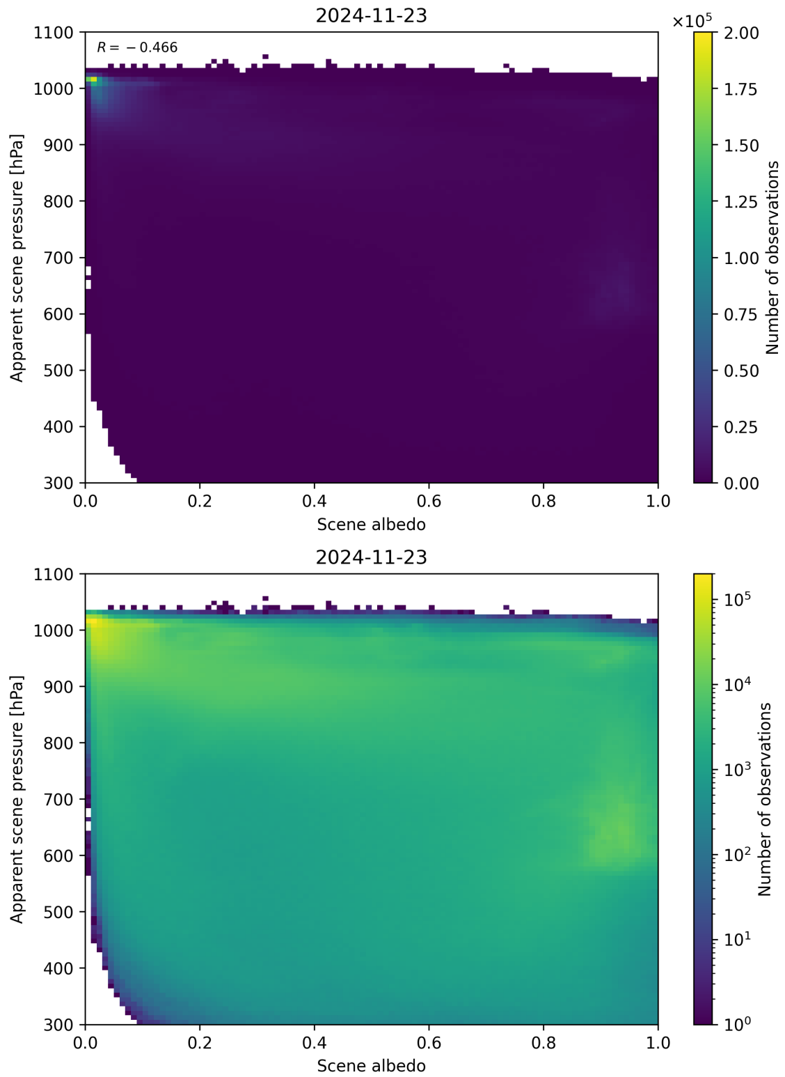
Figure 102: Scatter density plot of “Scene albedo” against “Apparent scene pressure” for 2024-11-22 to 2024-11-24.
