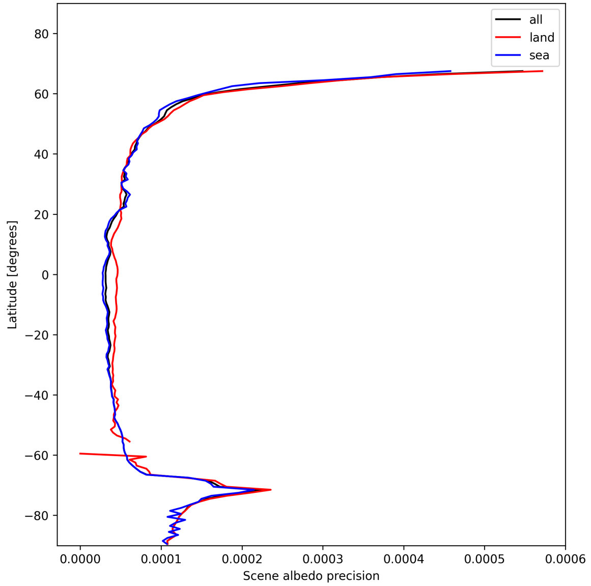
Figure 18: Zonal average of “Scene albedo precision” for 2024-11-22 to 2024-11-24.
