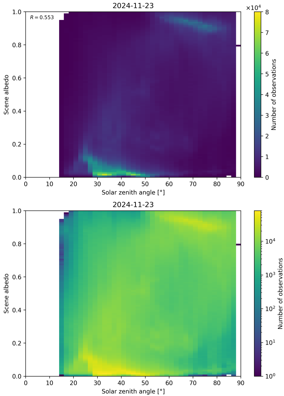
Figure 116: Scatter density plot of “Solar zenith angle” against “Scene albedo” for 2024-11-22 to 2024-11-24.
