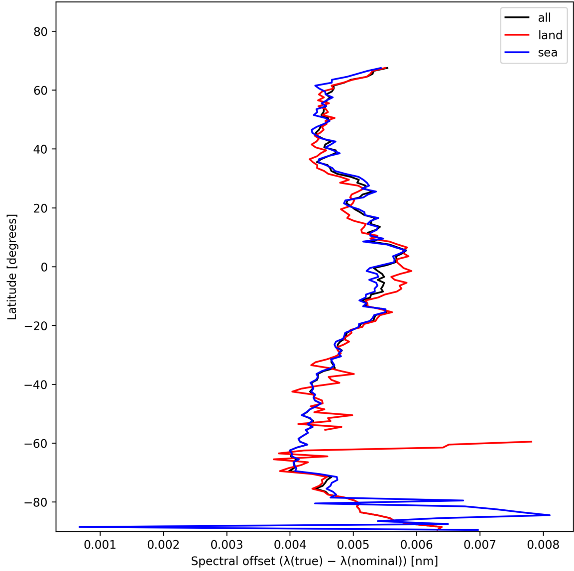
Figure 28: Zonal average of “Spectral offset ( \lambda_{\text{true}} - \lambda_{\text{nominal}} )” for 2024-11-22 to 2024-11-24.
