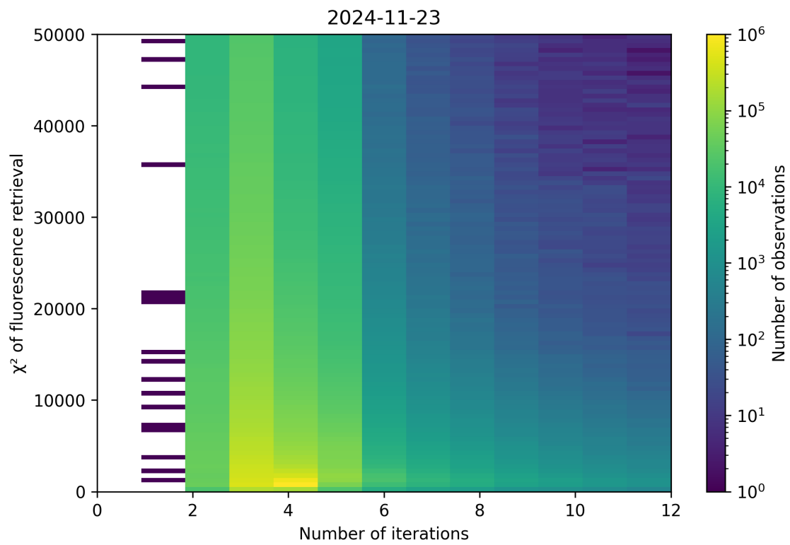
Figure 97: Scatter density plot of “Number of iterations” against “ \chi^2 of fluorescence retrieval” for 2024-11-22 to 2024-11-24.
