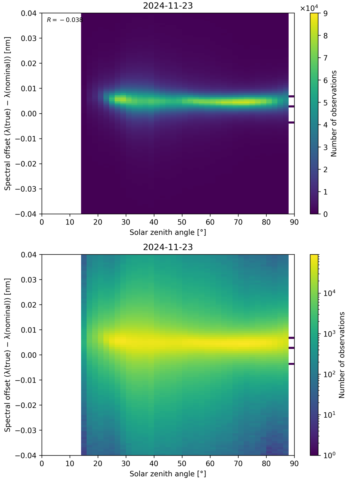
Figure 117: Scatter density plot of “Solar zenith angle” against “Spectral offset ( \lambda_{\text{true}} - \lambda_{\text{nominal}} )” for 2024-11-22 to 2024-11-24.
