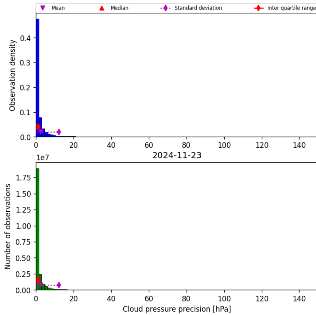
Figure 31: Histogram of “Cloud pressure precision” for 2024-11-22 to 2024-11-24
