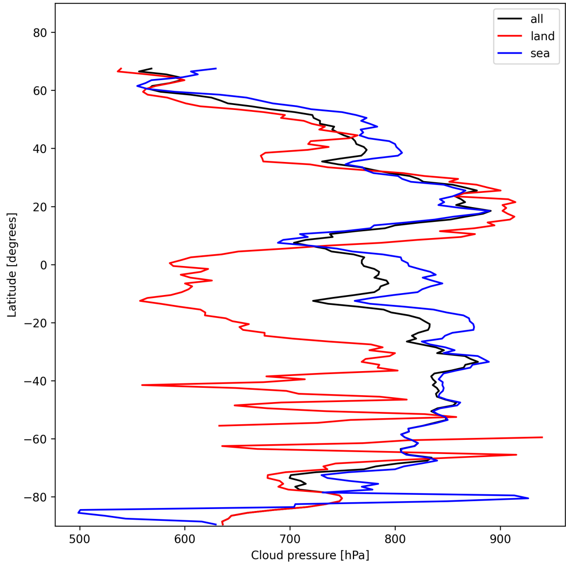
Figure 13: Zonal average of “Cloud pressure” for 2024-11-22 to 2024-11-24.
