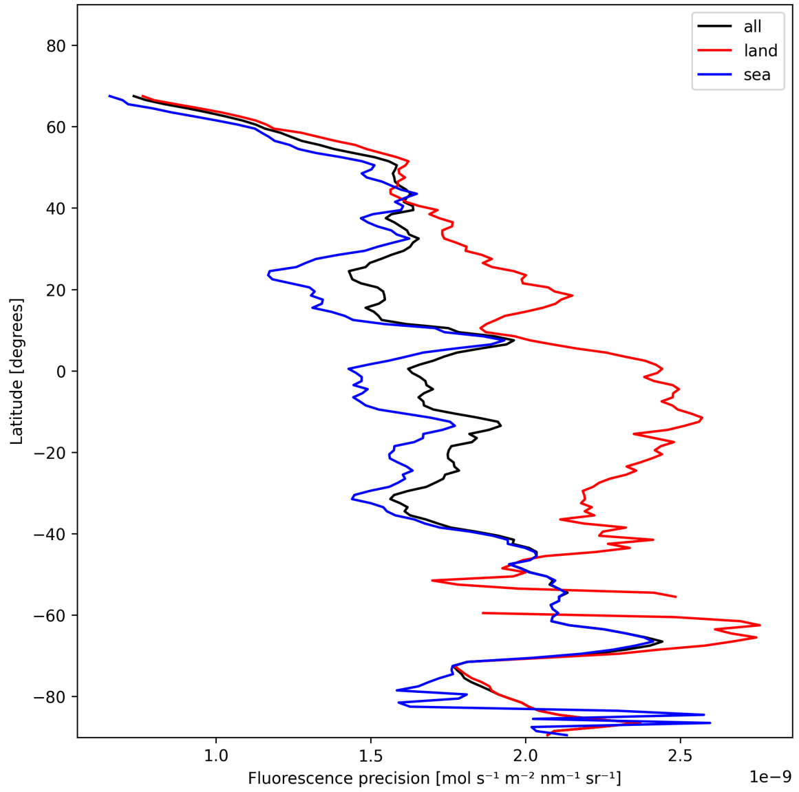
Figure 24: Zonal average of “Fluorescence precision” for 2024-11-22 to 2024-11-24.
