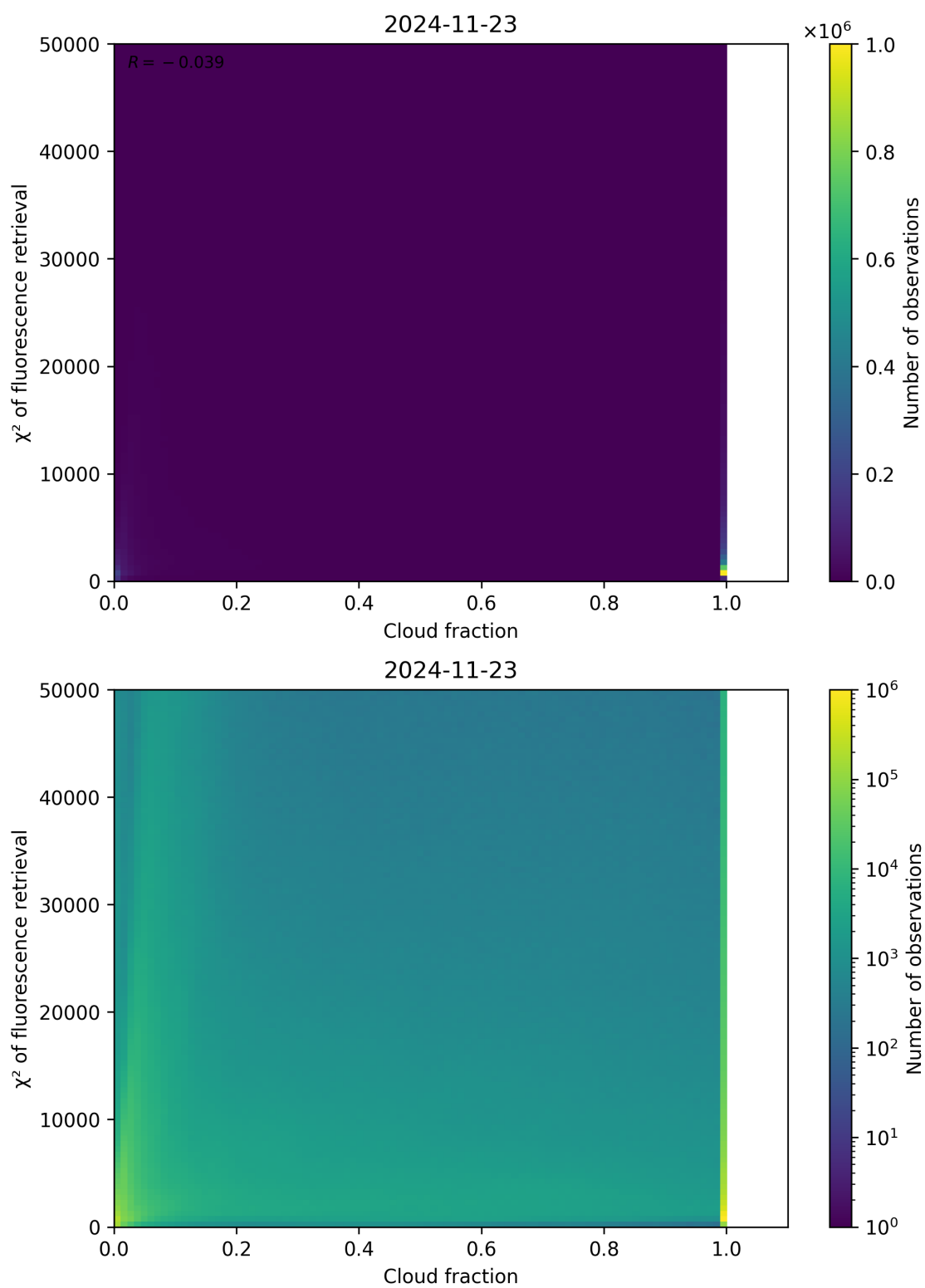
Figure 71: Scatter density plot of “Cloud fraction” against “ \chi^2 of fluorescence retrieval” for 2024-11-22 to 2024-11-24.
