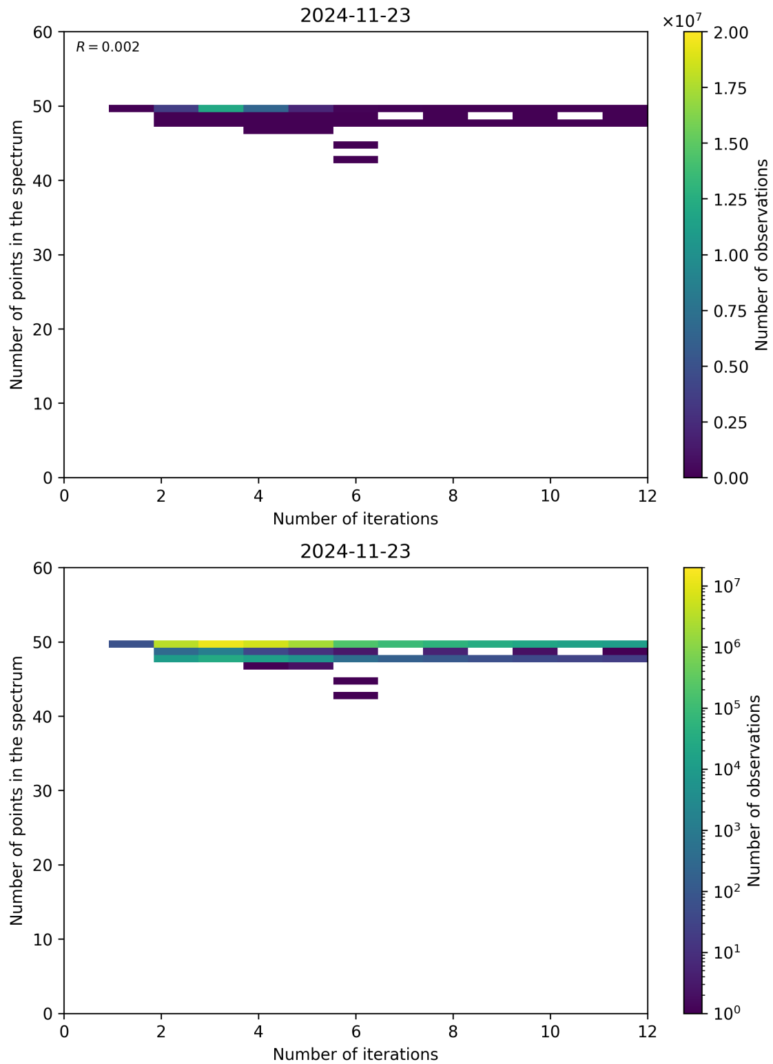
Figure 99: Scatter density plot of “Number of iterations” against “Number of points in the spectrum” for 2024-11-22 to 2024-11-24.
