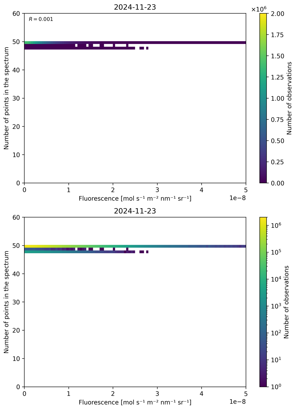
Figure 86: Scatter density plot of “Fluorescence” against “Number of points in the spectrum” for 2024-11-22 to 2024-11-24.
