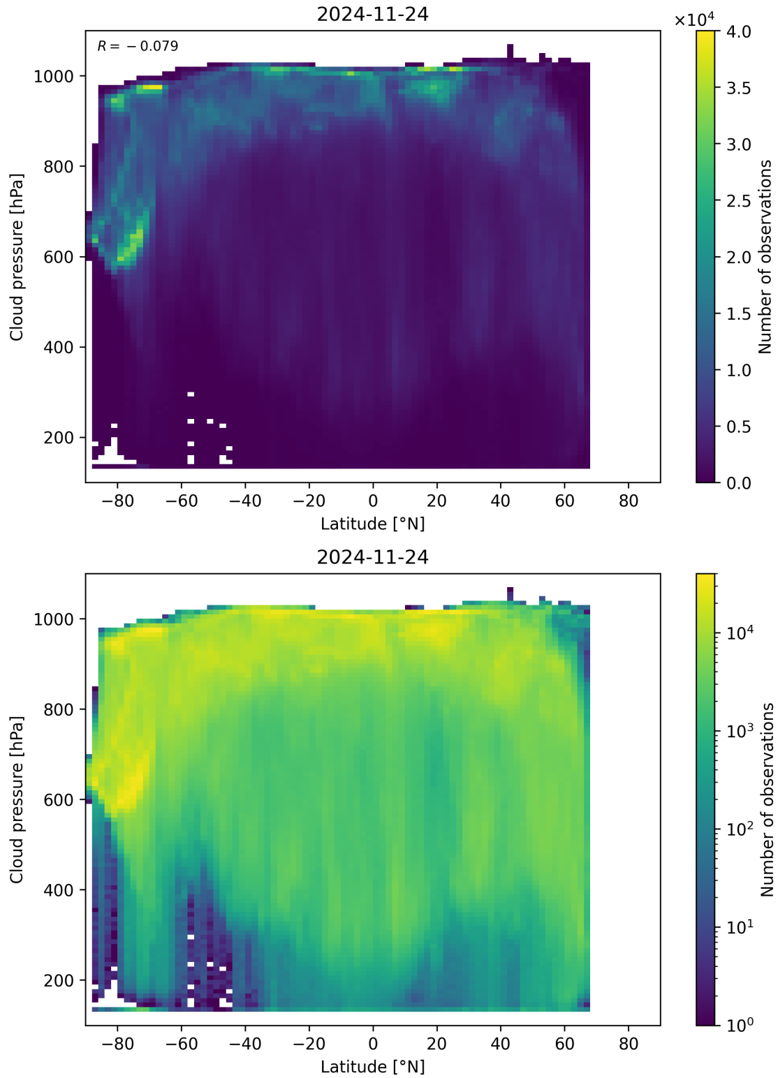
Figure 91: Scatter density plot of “Latitude” against “Cloud pressure” for 2024-11-23 to 2024-11-25.
