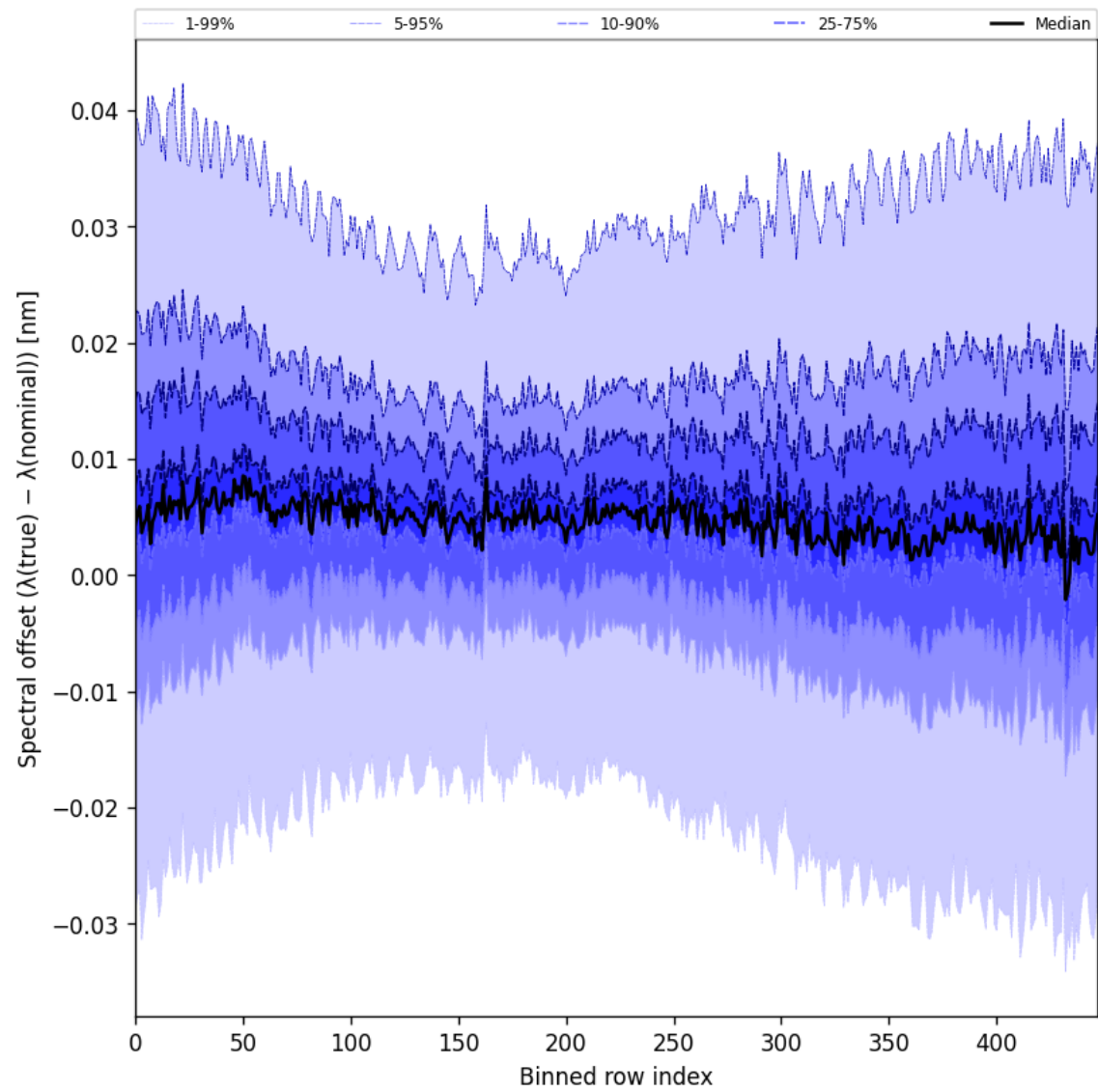
Figure 62: Along track statistics of “Spectral offset ( \lambda_{\text{true}} - \lambda_{\text{nominal}} )” for 2024-11-23 to 2024-11-25
