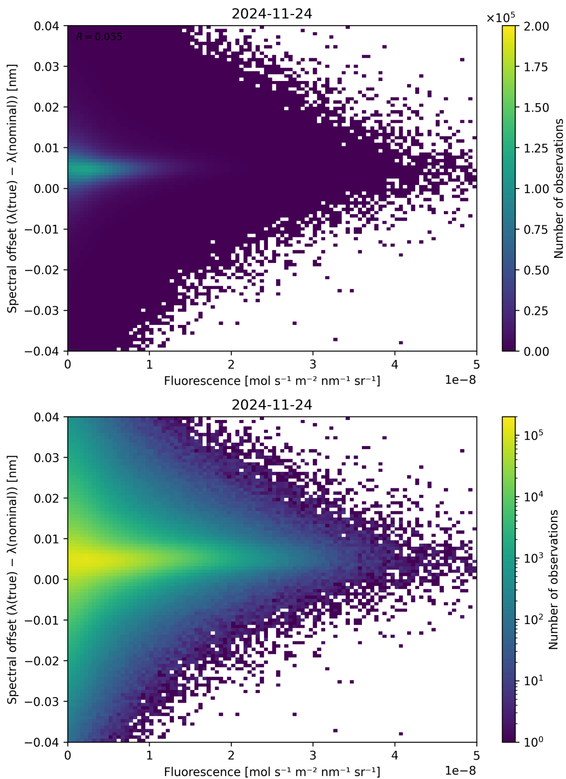
Figure 87: Scatter density plot of “Fluorescence” against “Spectral offset ( \lambda_{\text{true}} - \lambda_{\text{nominal}} )” for 2024-11-23 to 2024-11-25.
