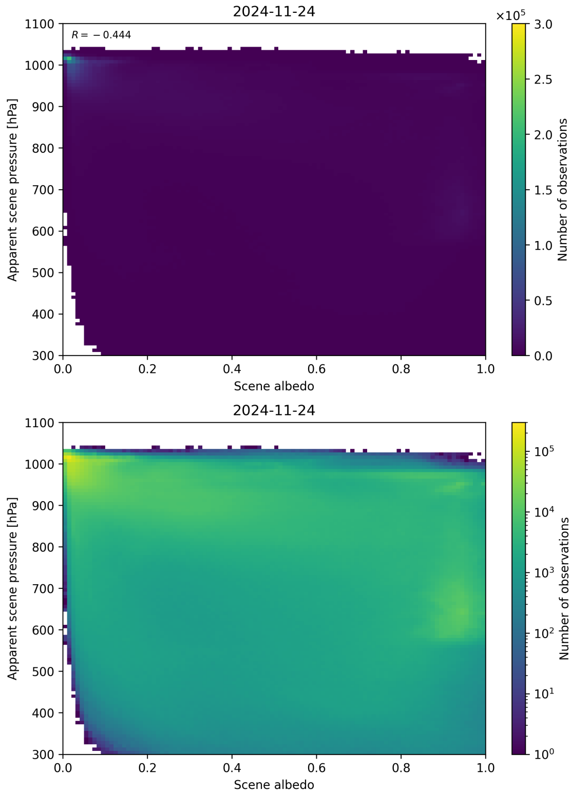
Figure 102: Scatter density plot of “Scene albedo” against “Apparent scene pressure” for 2024-11-23 to 2024-11-25.
