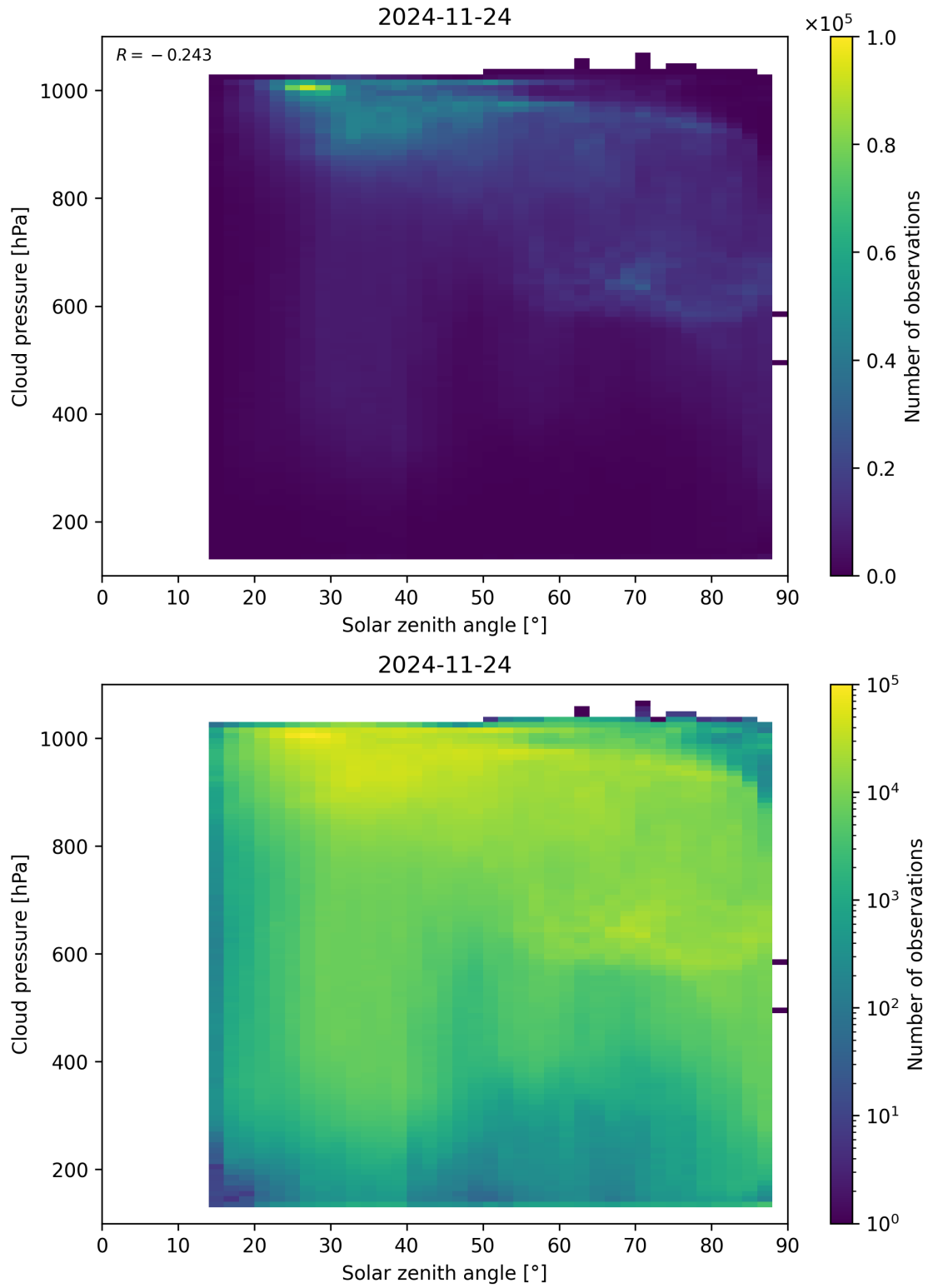
Figure 111: Scatter density plot of “Solar zenith angle” against “Cloud pressure” for 2024-11-23 to 2024-11-25.
