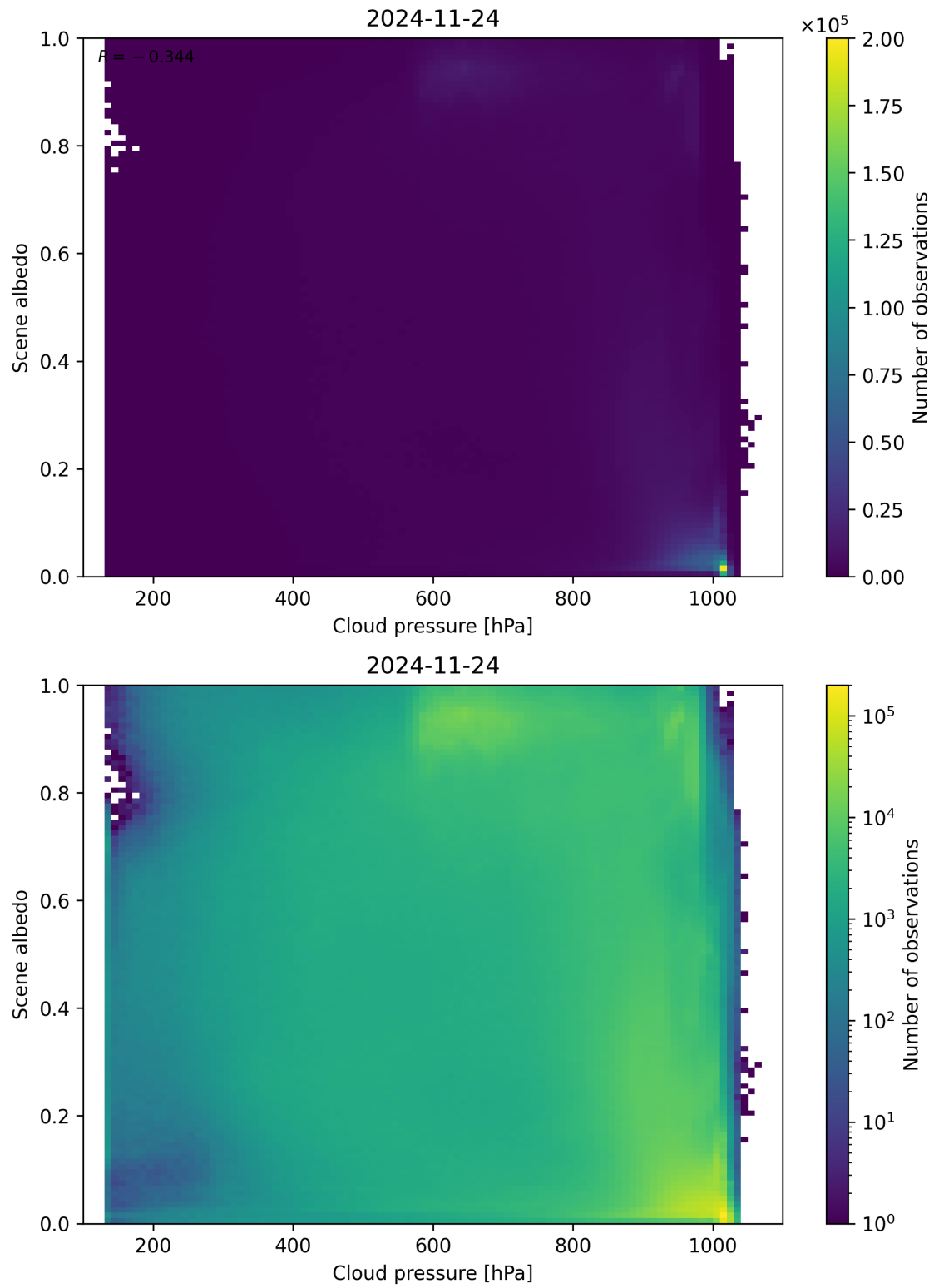
Figure 83: Scatter density plot of “Cloud pressure” against “Scene albedo” for 2024-11-23 to 2024-11-25.
