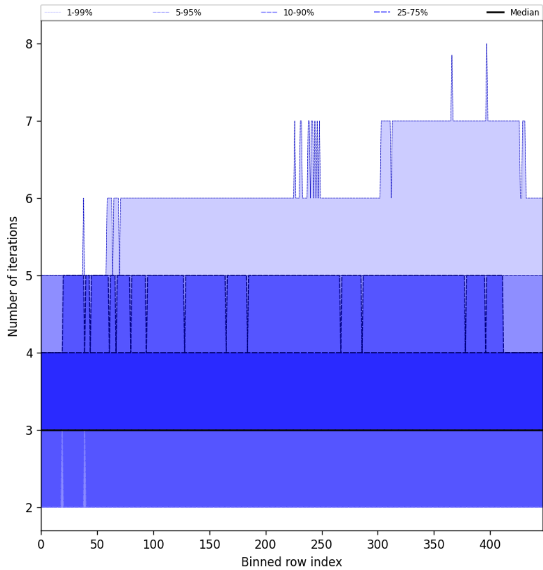
Figure 56: Along track statistics of “Number of iterations” for 2024-11-23 to 2024-11-25
