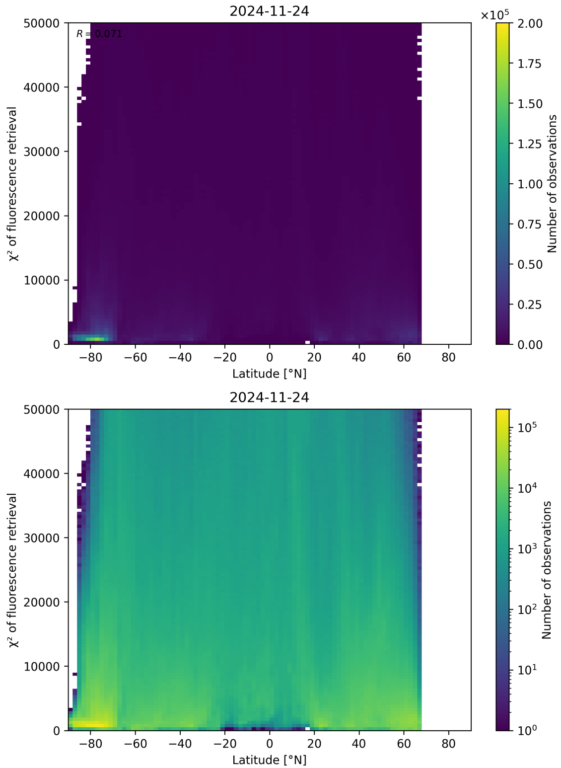
Figure 89: Scatter density plot of “Latitude” against “ \chi^2 of fluorescence retrieval” for 2024-11-23 to 2024-11-25.
