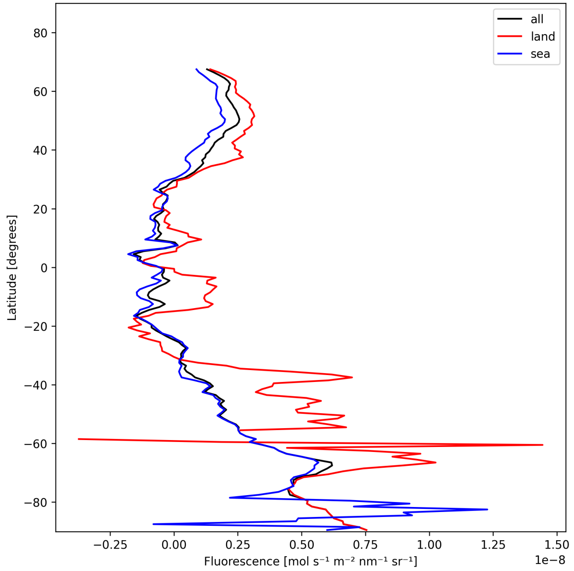
Figure 23: Zonal average of “Fluorescence” for 2024-11-23 to 2024-11-25.
