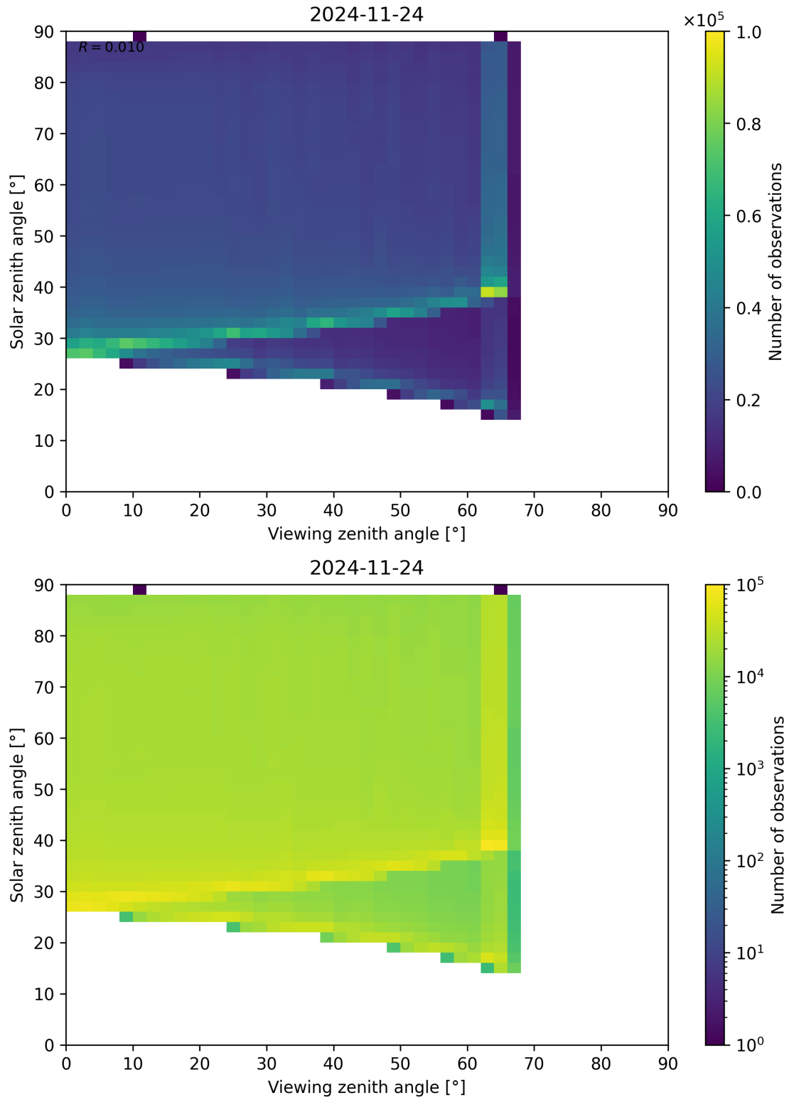
Figure 127: Scatter density plot of “Viewing zenith angle” against “Solar zenith angle” for 2024-11-23 to 2024-11-25.
