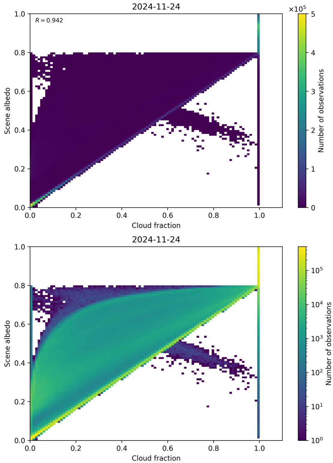
Figure 75: Scatter density plot of “Cloud fraction” against “Scene albedo” for 2024-11-23 to 2024-11-25.
