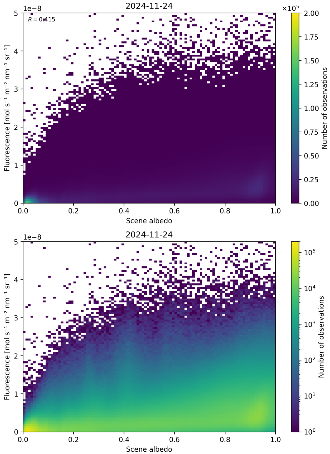
Figure 104: Scatter density plot of “Scene albedo” against “Fluorescence” for 2024-11-23 to 2024-11-25.
