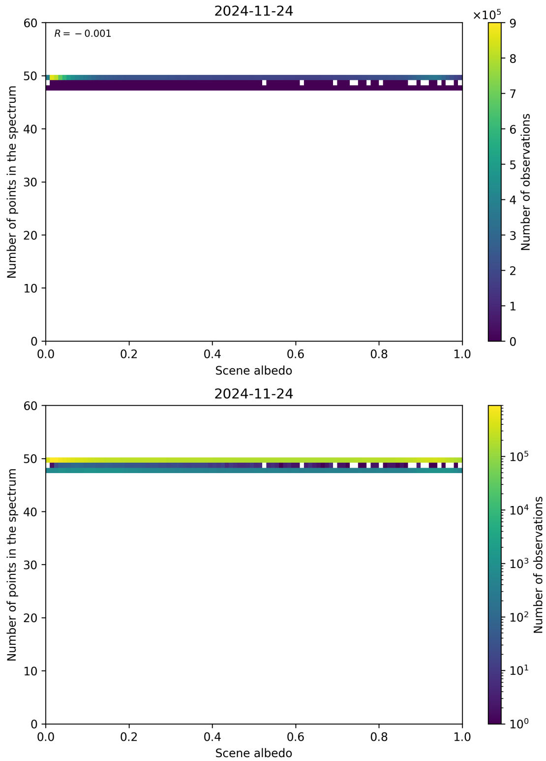
Figure 106: Scatter density plot of “Scene albedo” against “Number of points in the spectrum” for 2024-11-23 to 2024-11-25.
