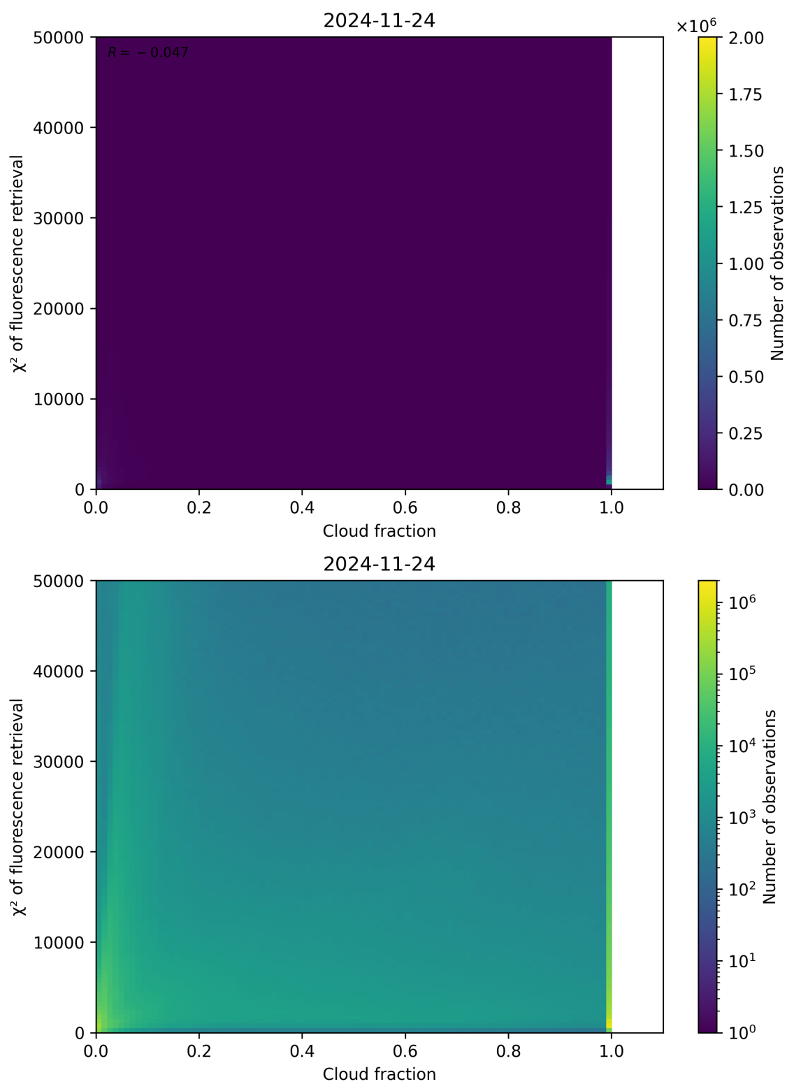
Figure 71: Scatter density plot of “Cloud fraction” against “ \chi^2 of fluorescence retrieval” for 2024-11-23 to 2024-11-25.
