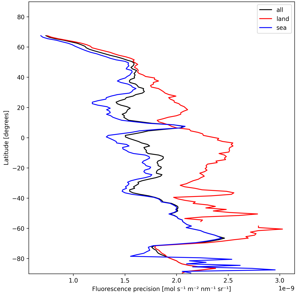
Figure 24: Zonal average of “Fluorescence precision” for 2024-11-23 to 2024-11-25.
