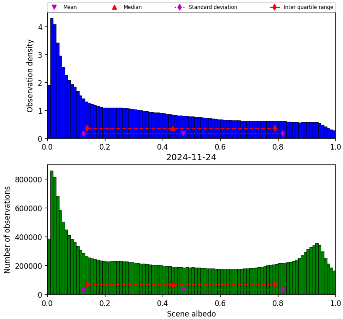
Figure 34: Histogram of “Scene albedo” for 2024-11-23 to 2024-11-25
