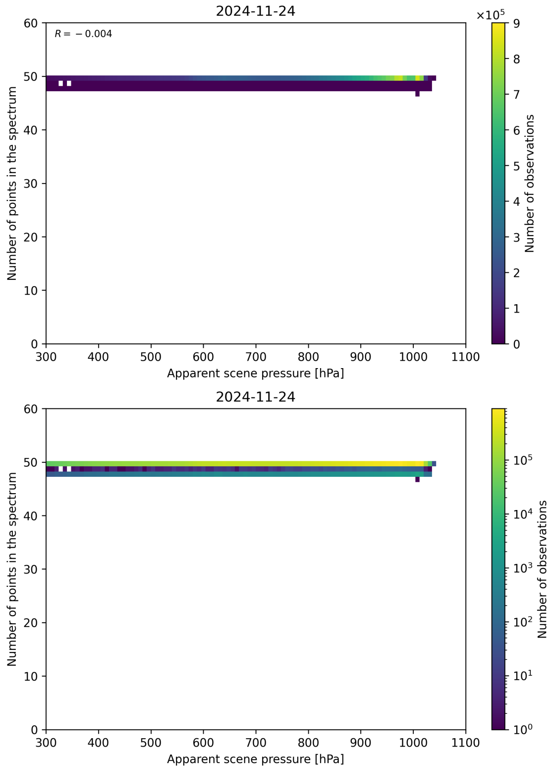
Figure 66: Scatter density plot of “Apparent scene pressure” against “Number of points in the spectrum” for 2024-11-23 to 2024-11-25.
