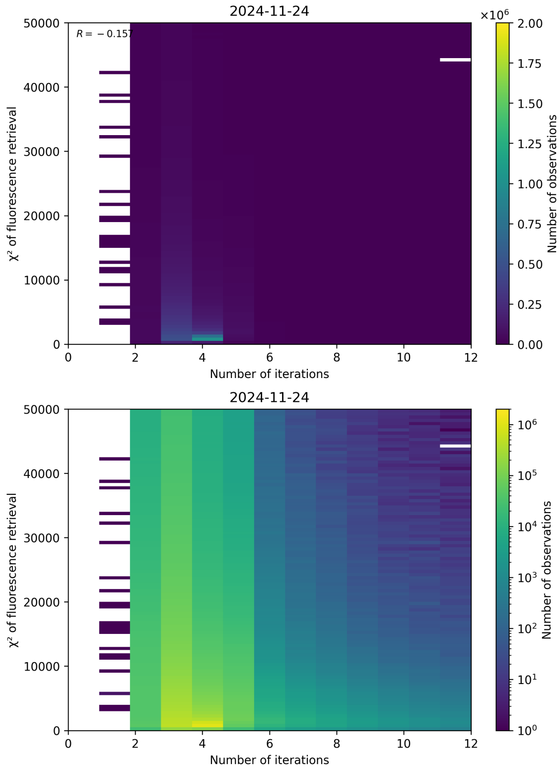
Figure 97: Scatter density plot of “Number of iterations” against “ \chi^2 of fluorescence retrieval” for 2024-11-23 to 2024-11-25.
