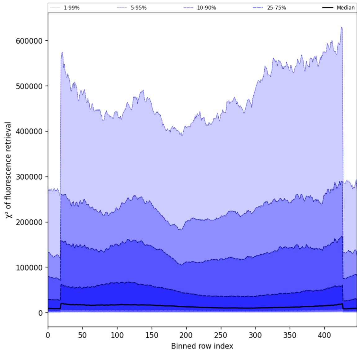
Figure 59: Along track statistics of “ \chi^2 of fluorescence retrieval” for 2024-11-23 to 2024-11-25
