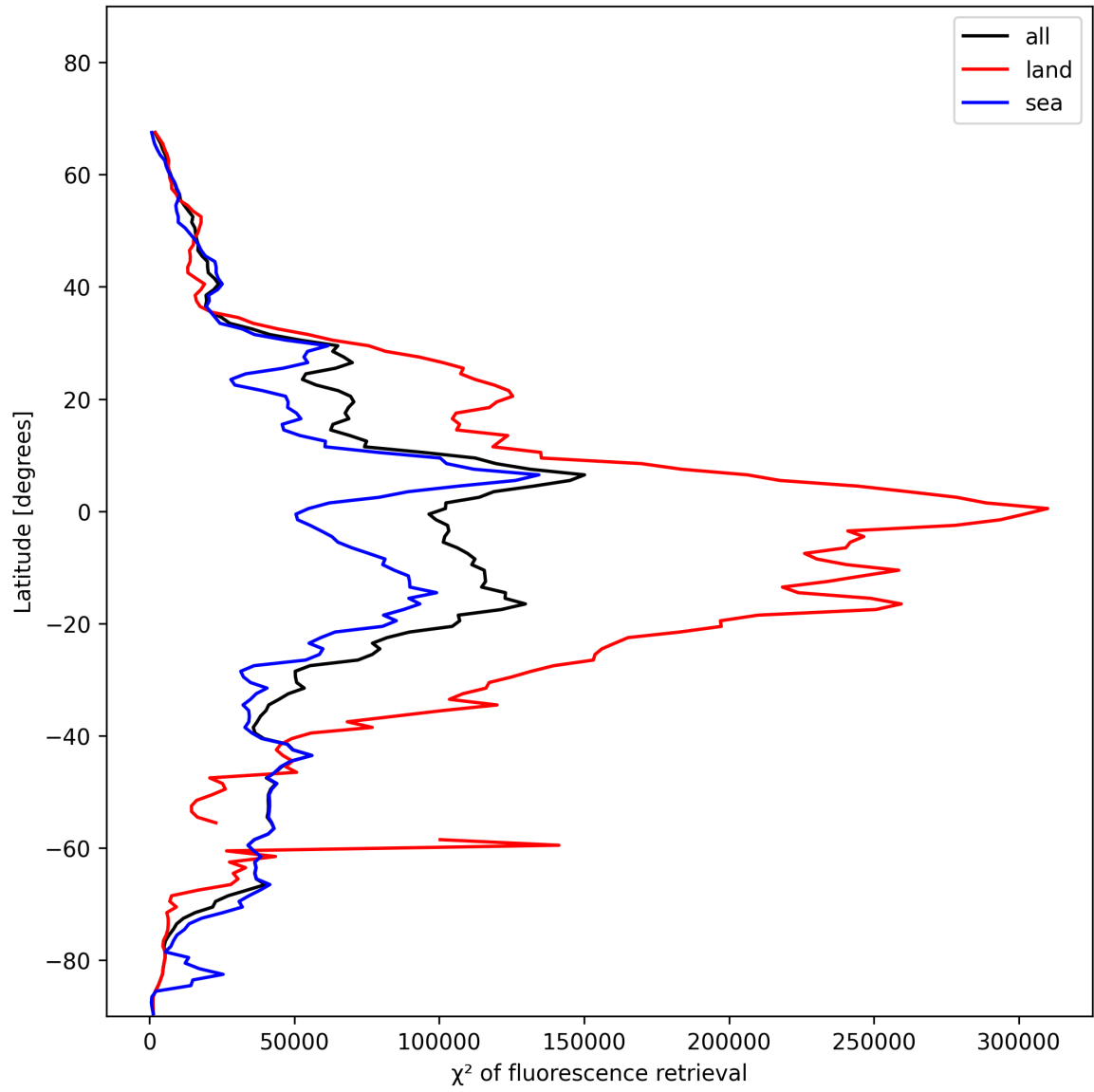
Figure 25: Zonal average of “ \chi^2 of fluorescence retrieval” for 2024-11-23 to 2024-11-25.
