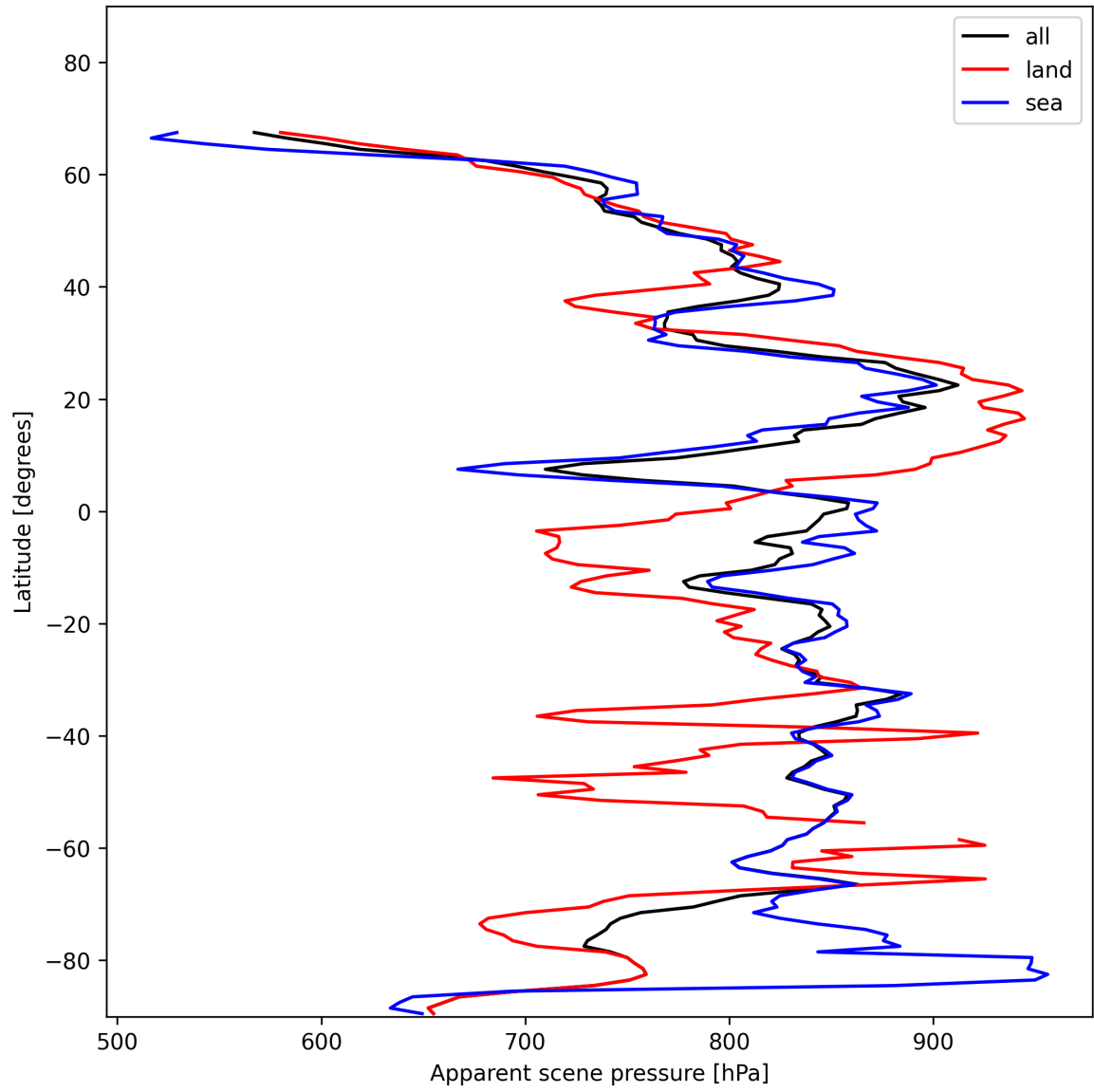
Figure 19: Zonal average of “Apparent scene pressure” for 2024-11-23 to 2024-11-25.
