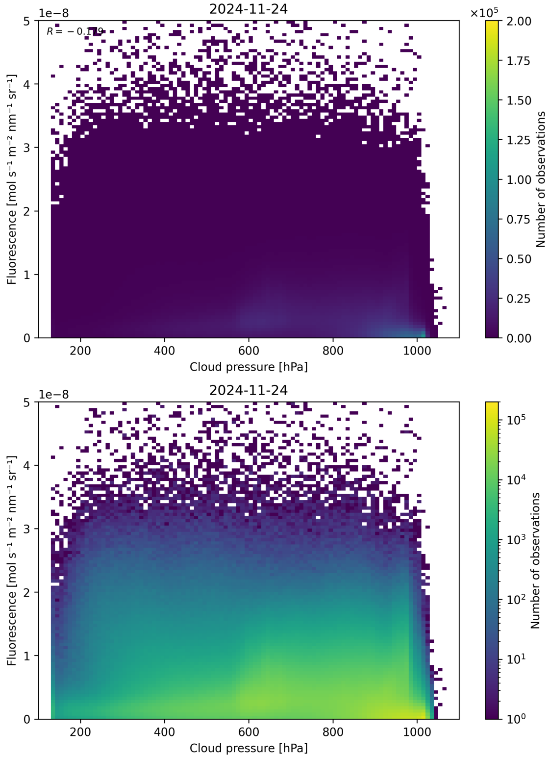
Figure 80: Scatter density plot of “Cloud pressure” against “Fluorescence” for 2024-11-23 to 2024-11-25.
