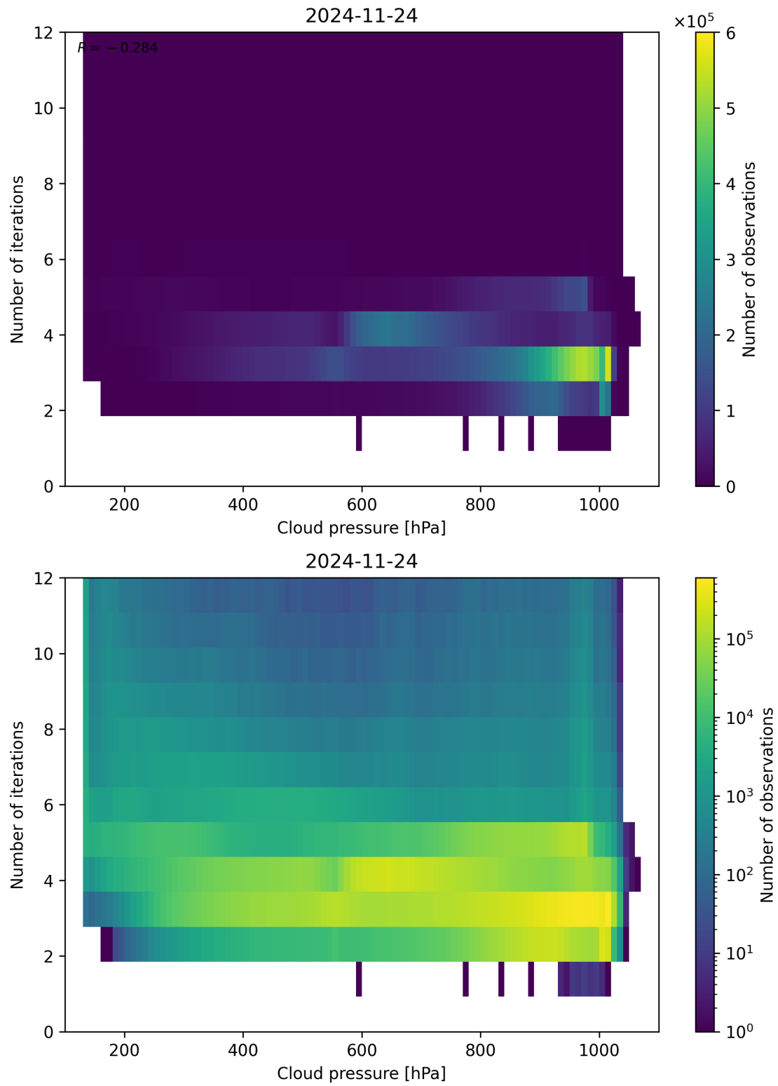
Figure 81: Scatter density plot of “Cloud pressure” against “Number of iterations” for 2024-11-23 to 2024-11-25.
