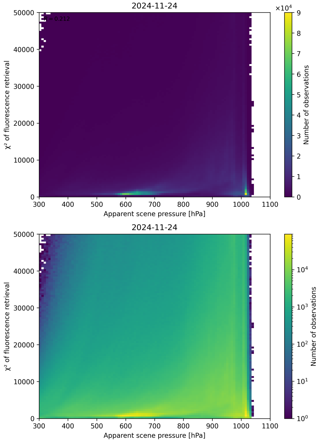
Figure 63: Scatter density plot of “Apparent scene pressure” against “ \chi^2 of fluorescence retrieval” for 2024-11-23 to 2024-11-25.
