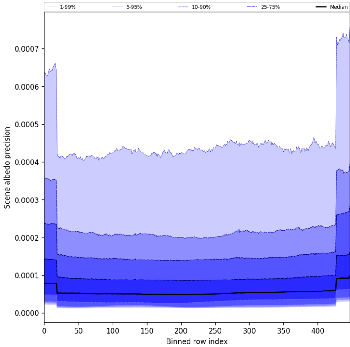
Figure 52: Along track statistics of “Scene albedo precision” for 2024-11-23 to 2024-11-25
