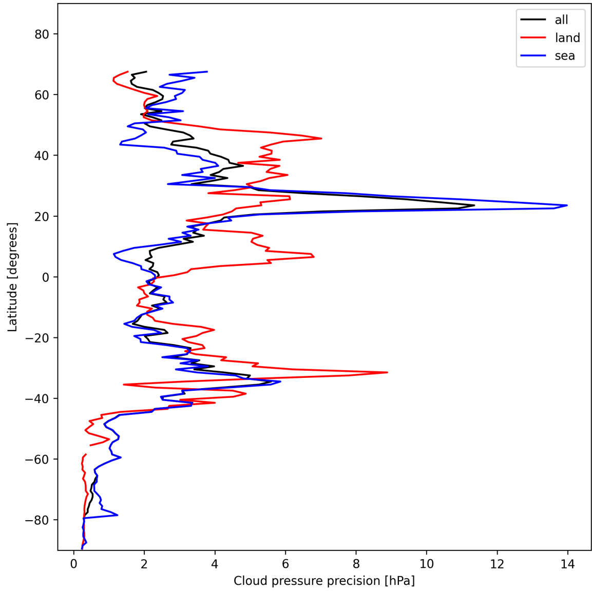
Figure 14: Zonal average of “Cloud pressure precision” for 2024-11-23 to 2024-11-25.
