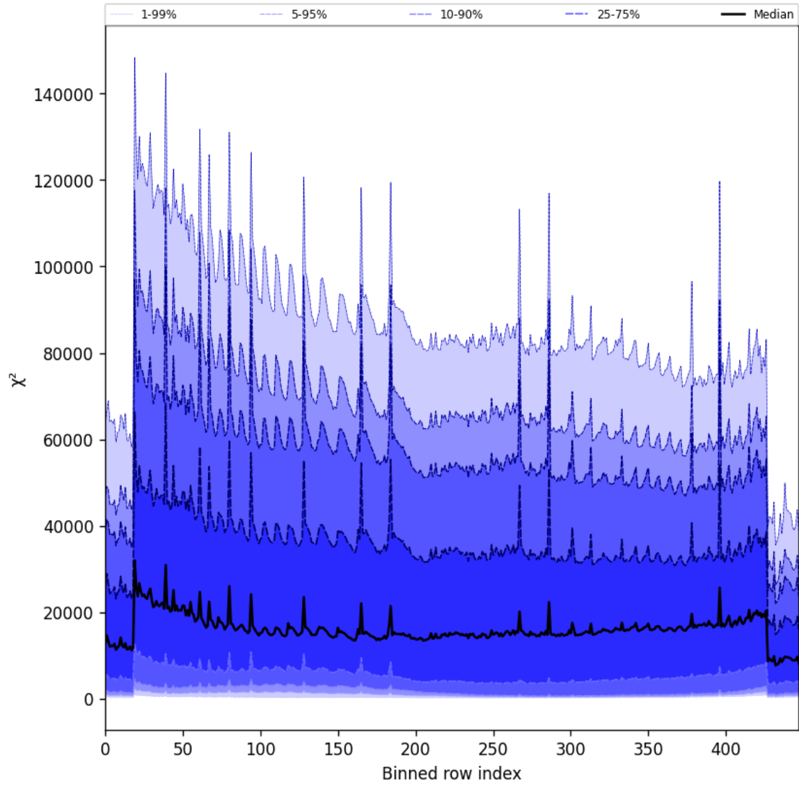
Figure 55: Along track statistics of “ \chi^2 ” for 2024-11-23 to 2024-11-25
