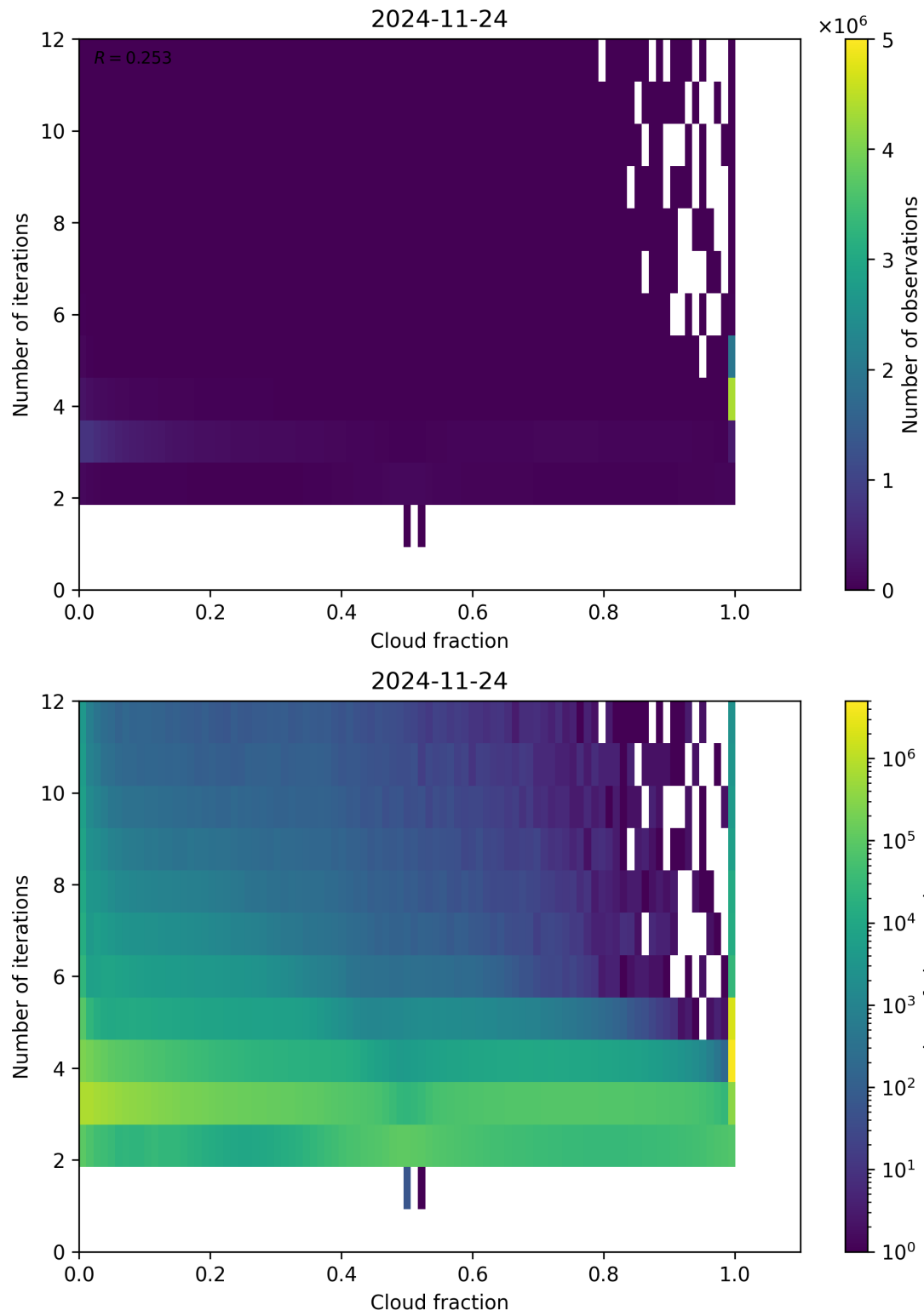
Figure 73: Scatter density plot of “Cloud fraction” against “Number of iterations” for 2024-11-23 to 2024-11-25.
