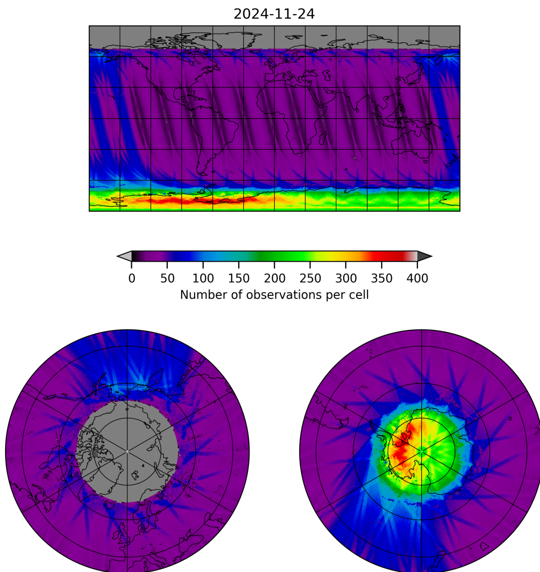
Figure 11: Map of the number of observations for 2024-11-23 to 2024-11-25
