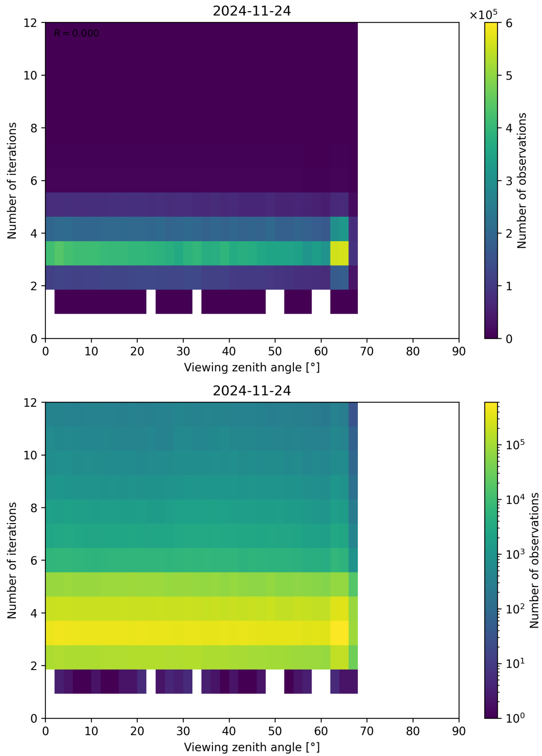
Figure 124: Scatter density plot of “Viewing zenith angle” against “Number of iterations” for 2024-11-23 to 2024-11-25.
