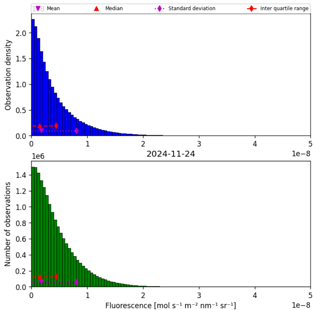
Figure 40: Histogram of “Fluorescence” for 2024-11-23 to 2024-11-25
