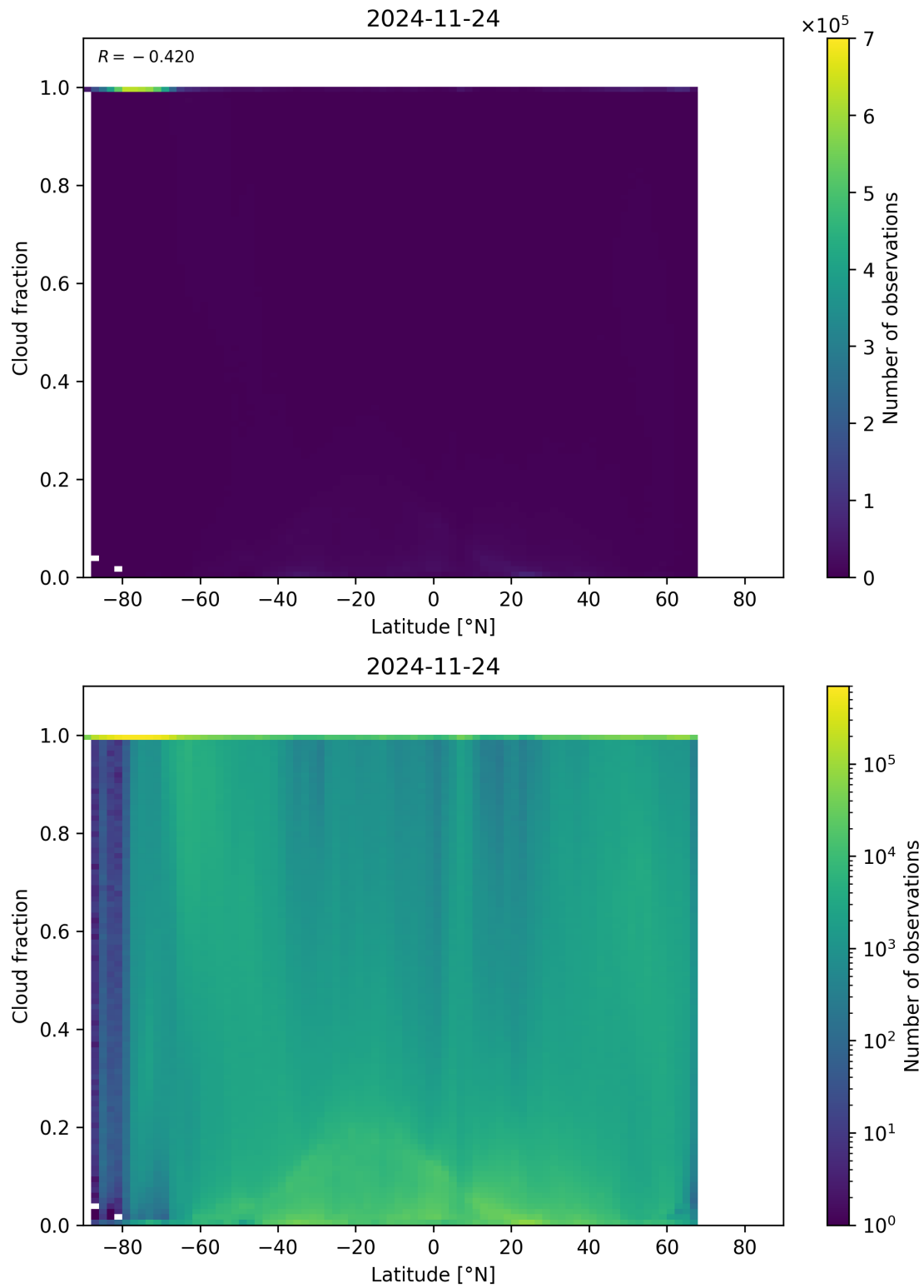
Figure 90: Scatter density plot of “Latitude” against “Cloud fraction” for 2024-11-23 to 2024-11-25.
