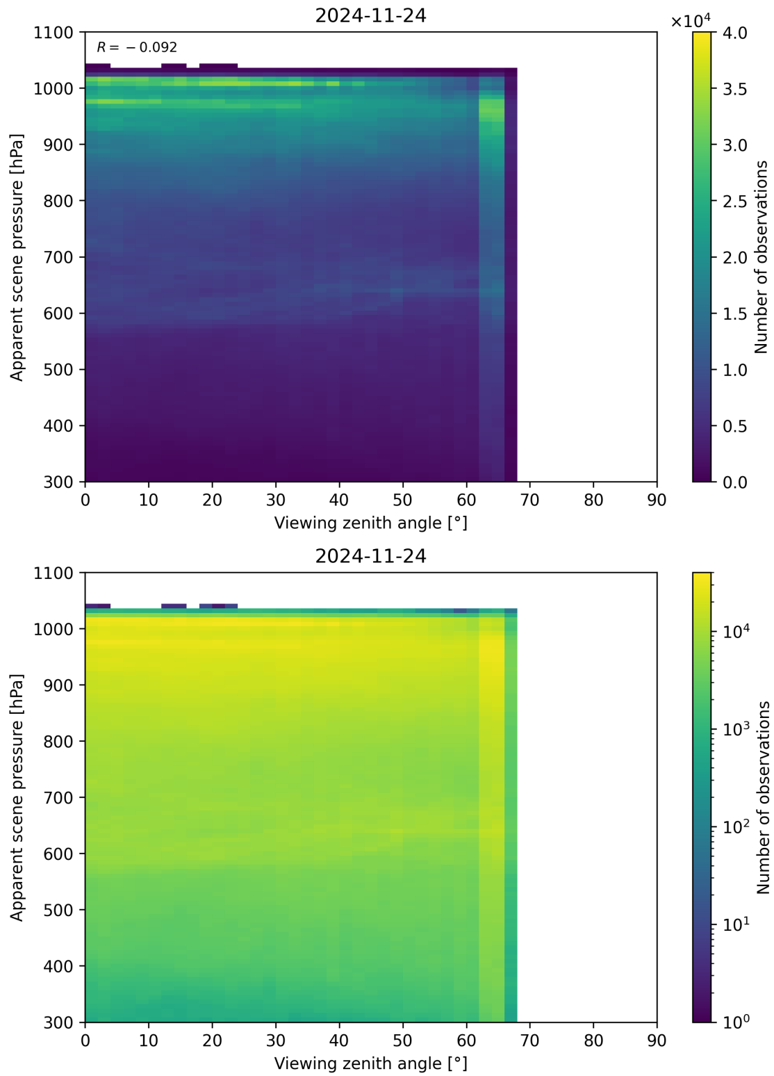
Figure 118: Scatter density plot of “Viewing zenith angle” against “Apparent scene pressure” for 2024-11-23 to 2024-11-25.
