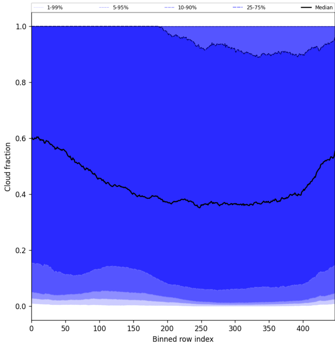
Figure 49: Along track statistics of “Cloud fraction” for 2024-11-23 to 2024-11-25
