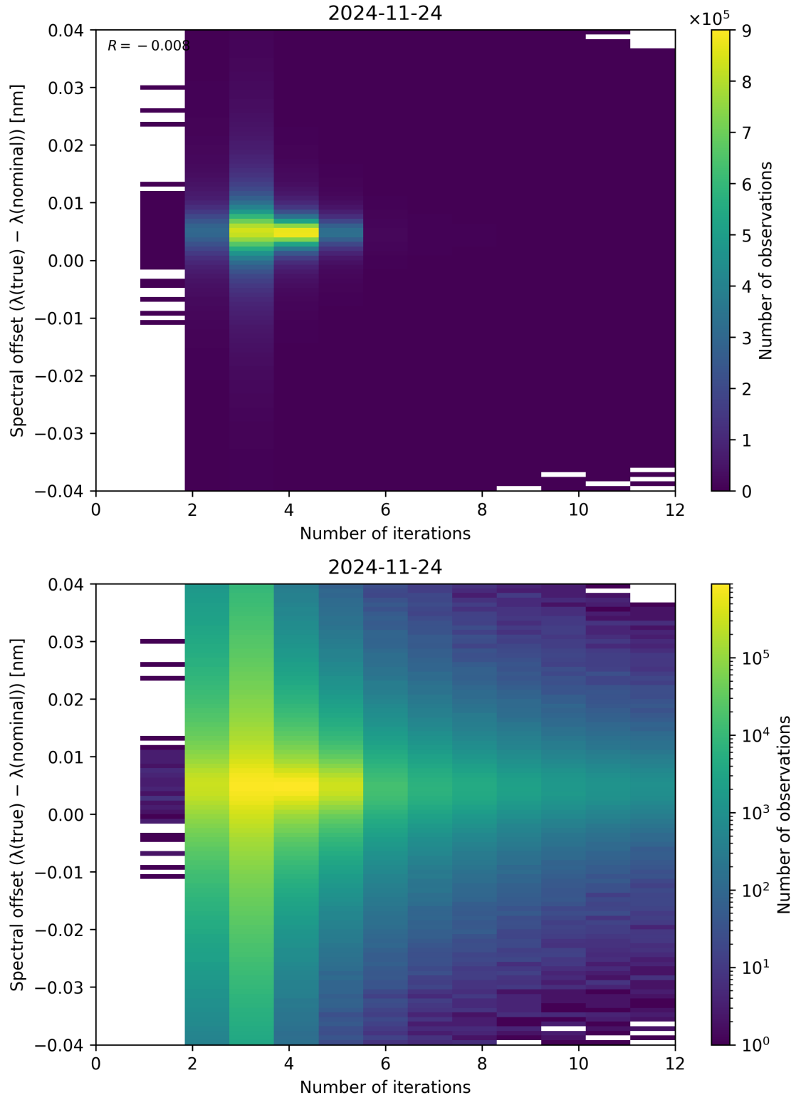
Figure 100: Scatter density plot of “Number of iterations” against “Spectral offset ( \lambda_{\text{true}} - \lambda_{\text{nominal}} )” for 2024-11-23 to 2024-11-25.
