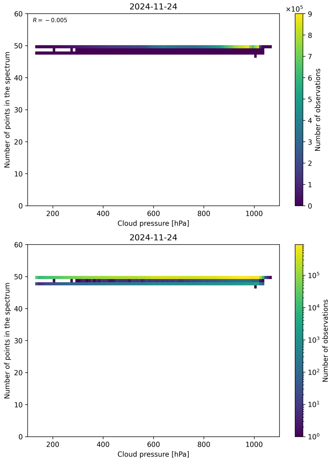
Figure 82: Scatter density plot of “Cloud pressure” against “Number of points in the spectrum” for 2024-11-23 to 2024-11-25.
