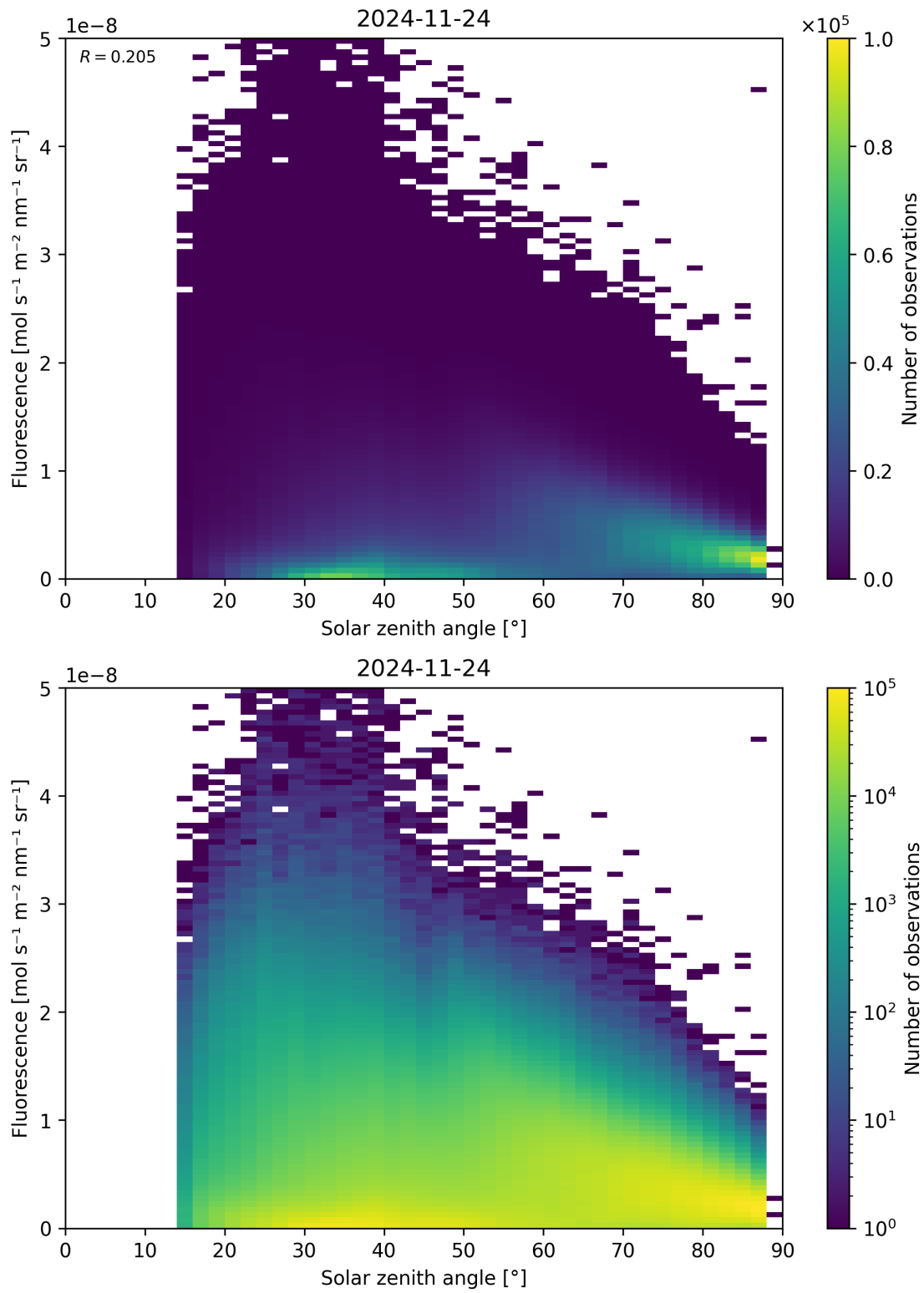
Figure 112: Scatter density plot of “Solar zenith angle” against “Fluorescence” for 2024-11-23 to 2024-11-25.
