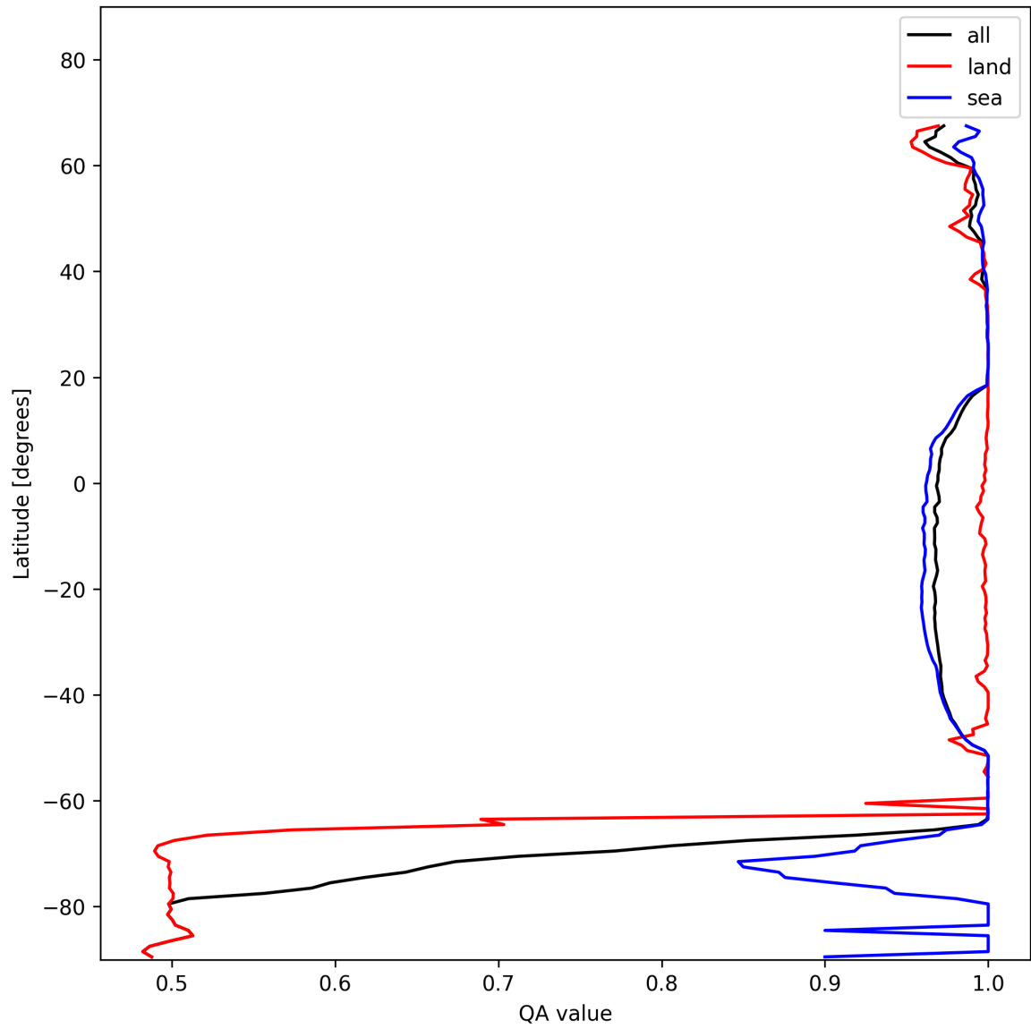
Figure 12: Zonal average of “QA value” for 2024-11-23 to 2024-11-25.
