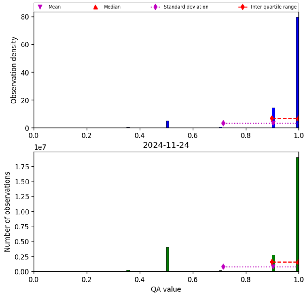
Figure 29: Histogram of “QA value” for 2024-11-23 to 2024-11-25
