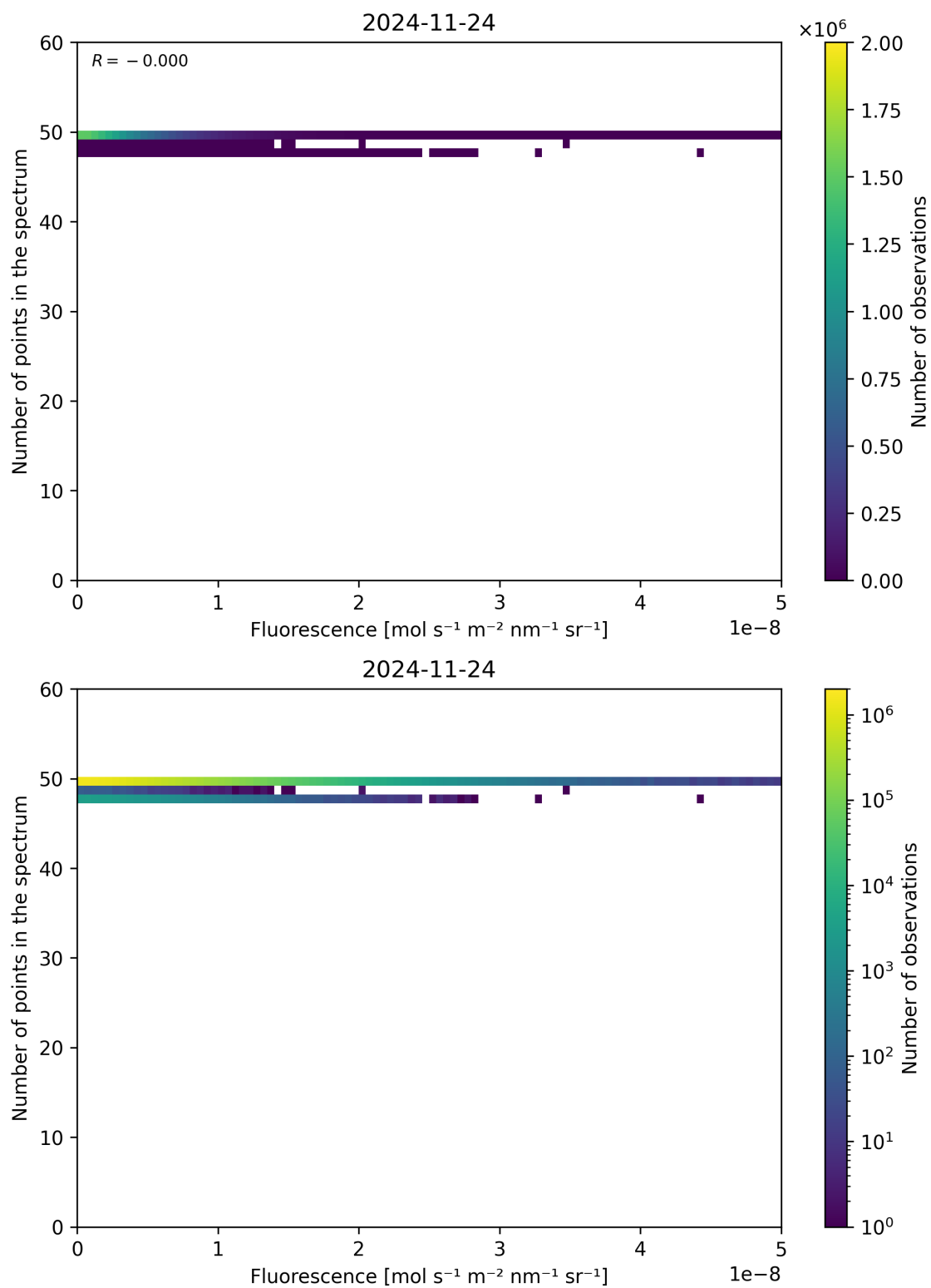
Figure 86: Scatter density plot of “Fluorescence” against “Number of points in the spectrum” for 2024-11-23 to 2024-11-25.
