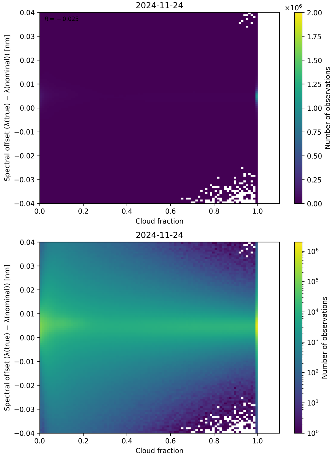
Figure 76: Scatter density plot of “Cloud fraction” against “Spectral offset ( \lambda_{\text{true}} - \lambda_{\text{nominal}} )” for 2024-11-23 to 2024-11-25.
