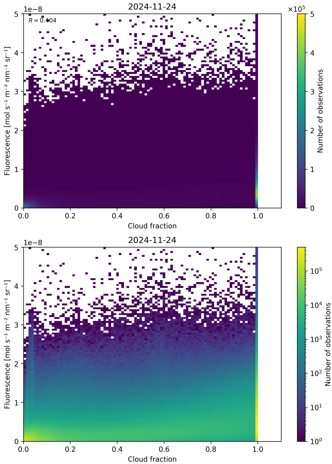
Figure 72: Scatter density plot of “Cloud fraction” against “Fluorescence” for 2024-11-23 to 2024-11-25.
