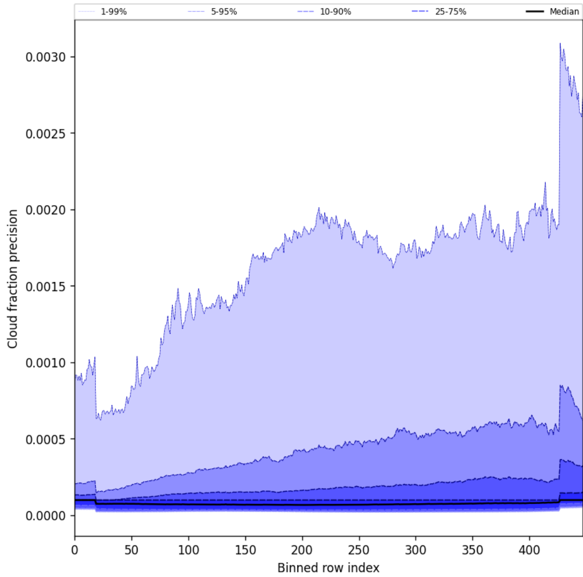
Figure 50: Along track statistics of “Cloud fraction precision” for 2024-11-23 to 2024-11-25
