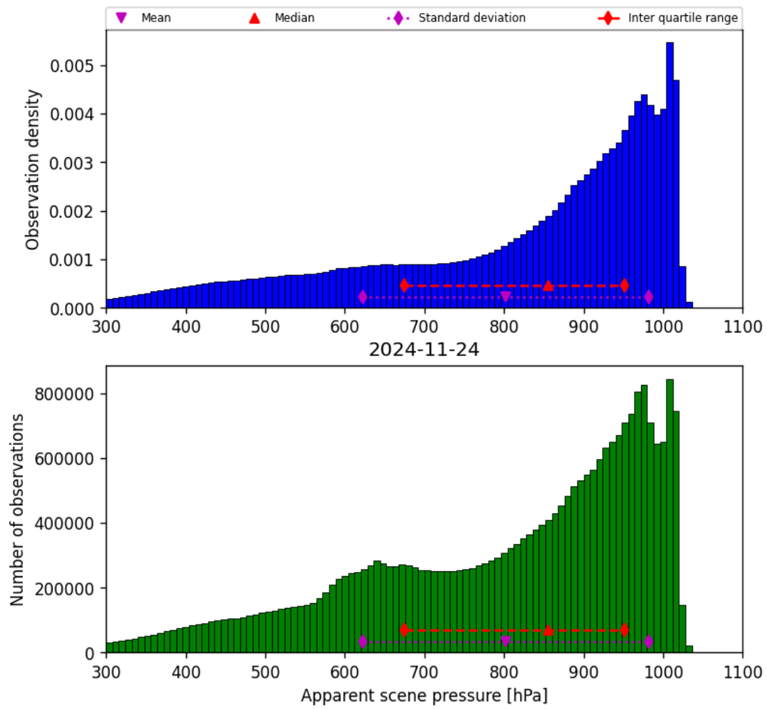
Figure 36: Histogram of “Apparent scene pressure” for 2024-11-23 to 2024-11-25
