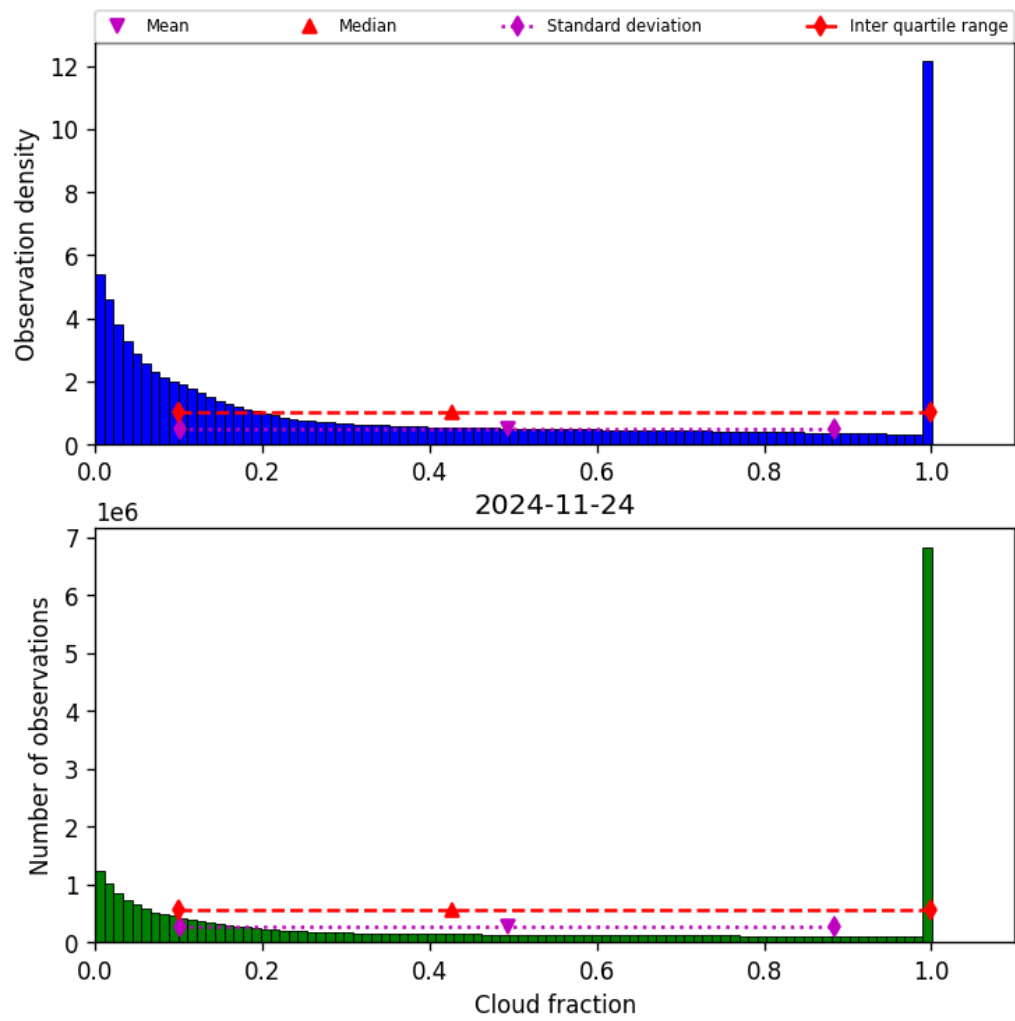
Figure 32: Histogram of “Cloud fraction” for 2024-11-23 to 2024-11-25
