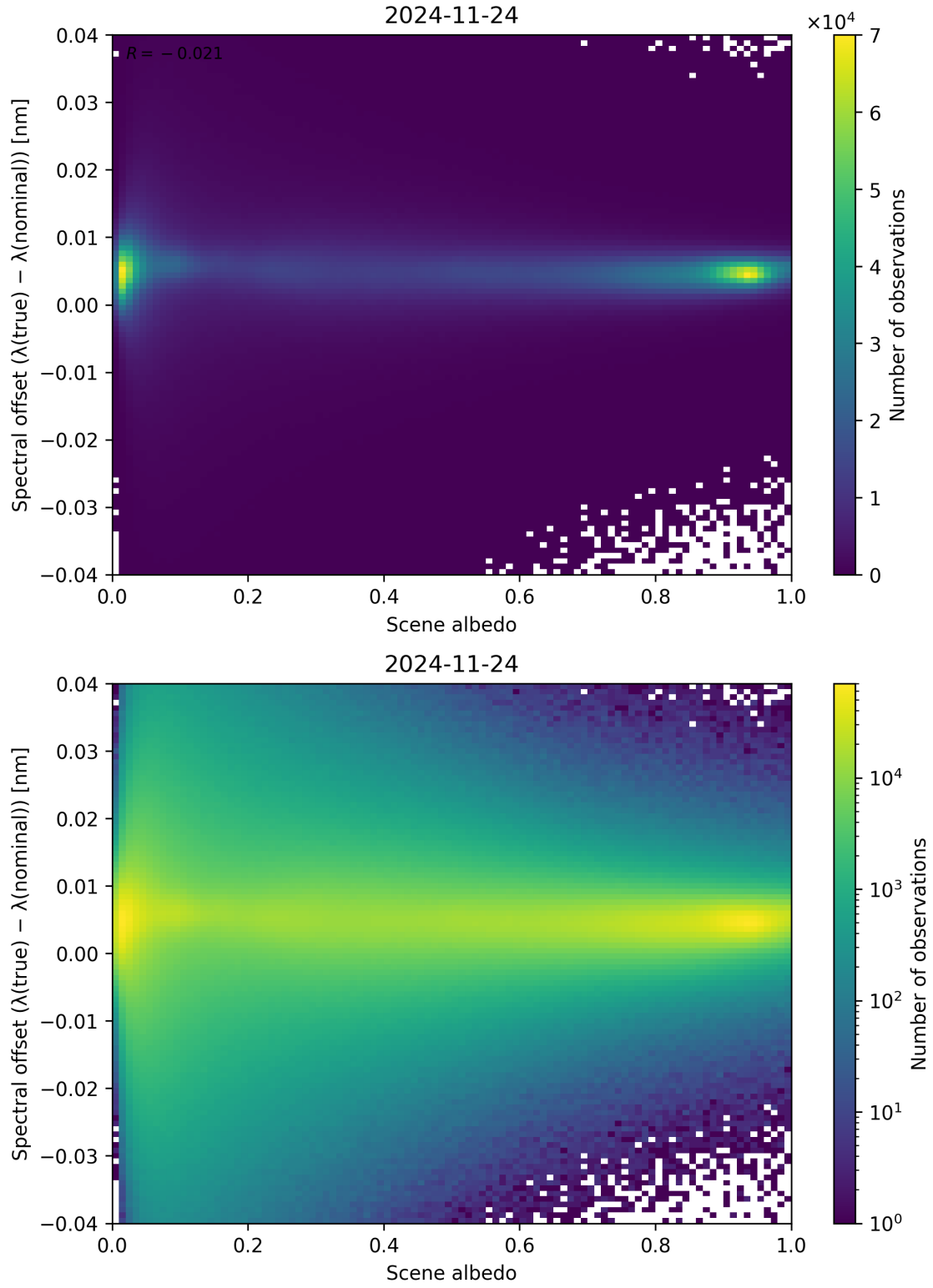
Figure 107: Scatter density plot of “Scene albedo” against “Spectral offset ( \lambda_{\text{true}} - \lambda_{\text{nominal}} )” for 2024-11-23 to 2024-11-25.
