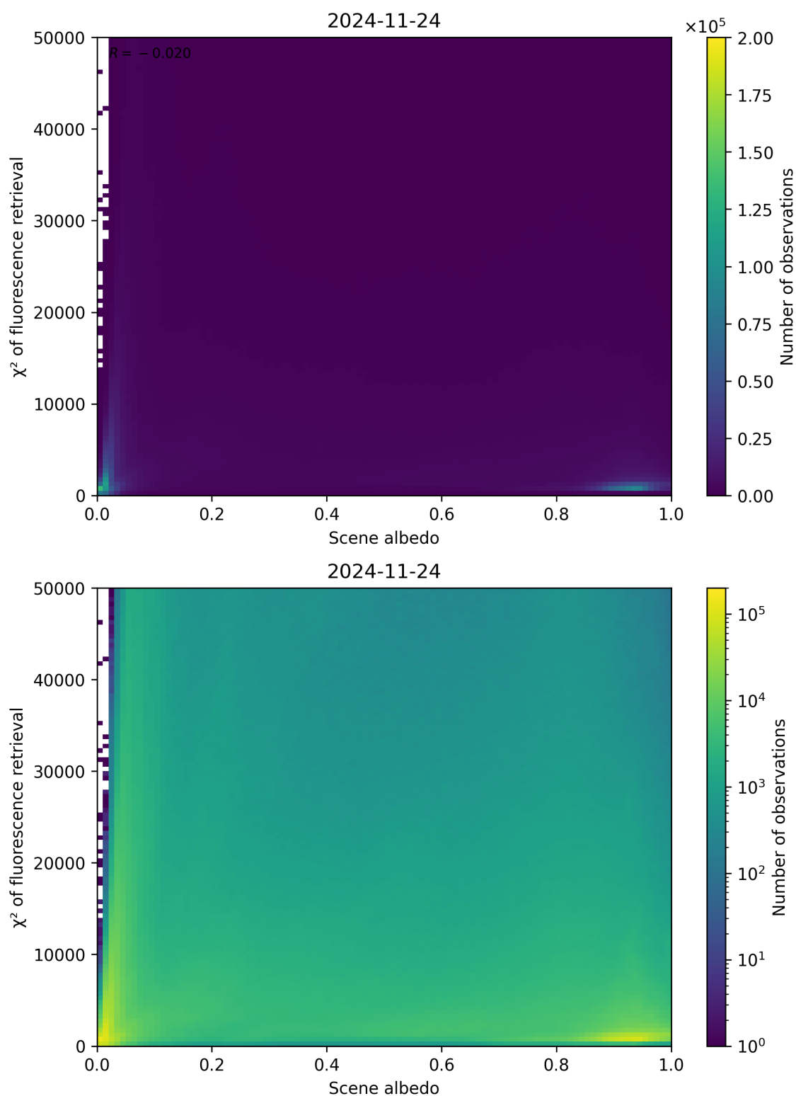
Figure 103: Scatter density plot of “Scene albedo” against “ \chi^2 of fluorescence retrieval” for 2024-11-23 to 2024-11-25.
