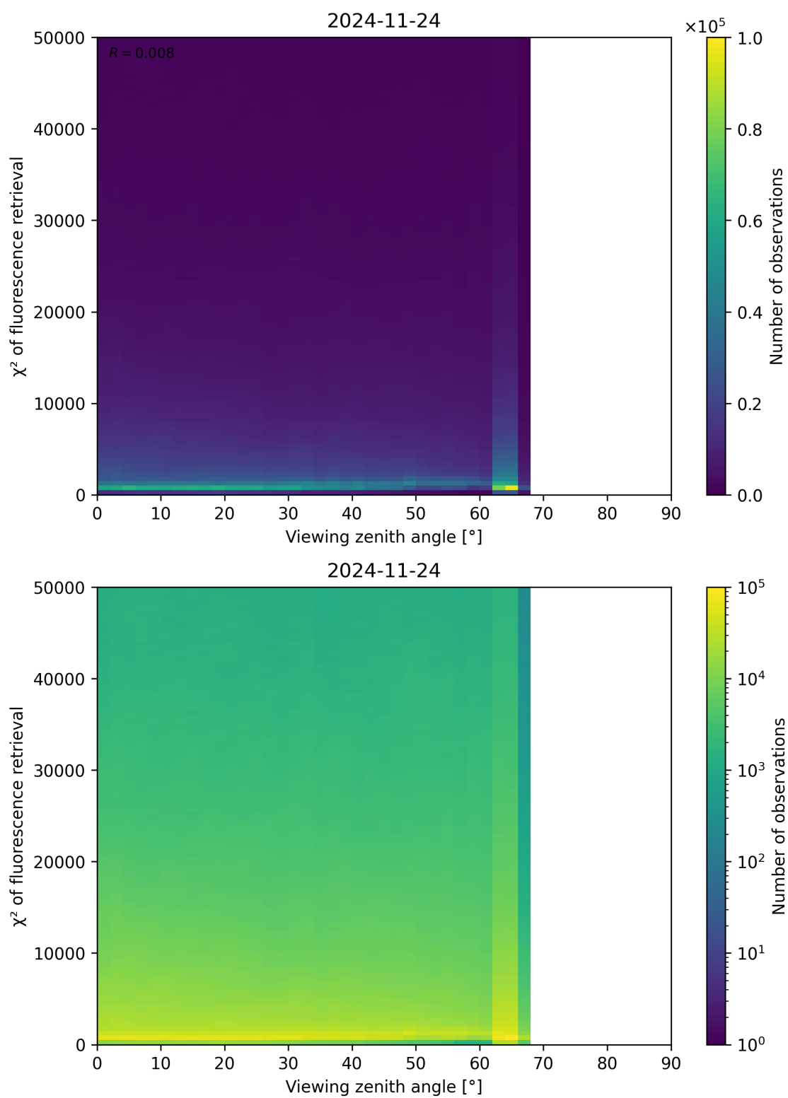
Figure 119: Scatter density plot of “Viewing zenith angle” against “ \chi^2 of fluorescence retrieval” for 2024-11-23 to 2024-11-25.
