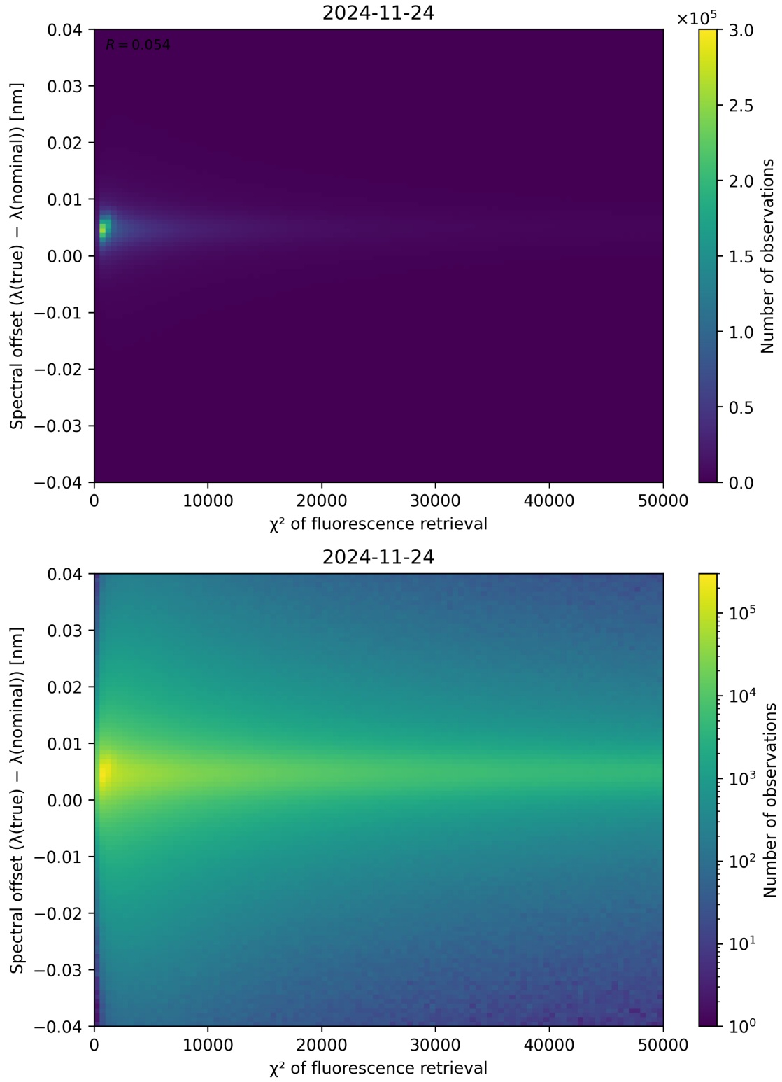
Figure 69: Scatter density plot of “ \chi^2 of fluorescence retrieval” against “Spectral offset ( \lambda_{\text{true}} - \lambda_{\text{nominal}} )” for 2024-11-23 to 2024-11-25.
