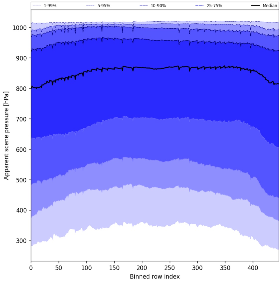
Figure 53: Along track statistics of “Apparent scene pressure” for 2024-11-23 to 2024-11-25
