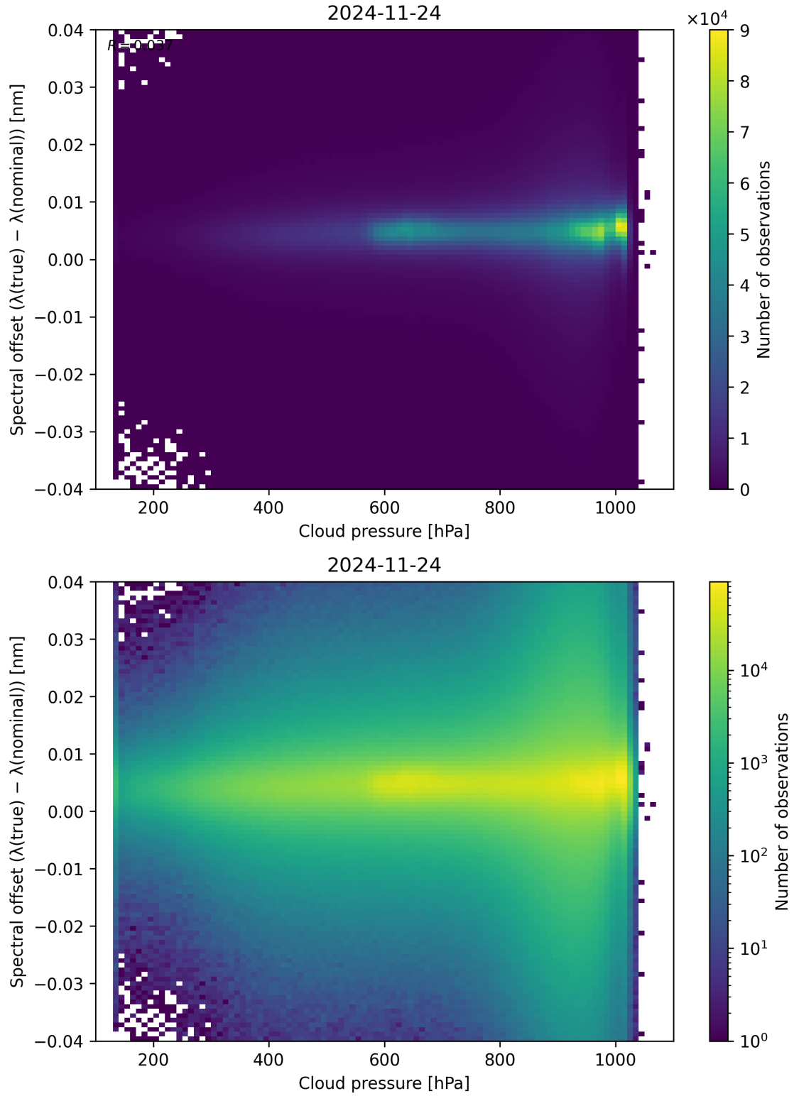
Figure 84: Scatter density plot of “Cloud pressure” against “Spectral offset ( \lambda_{\text{true}} - \lambda_{\text{nominal}} )” for 2024-11-23 to 2024-11-25.
