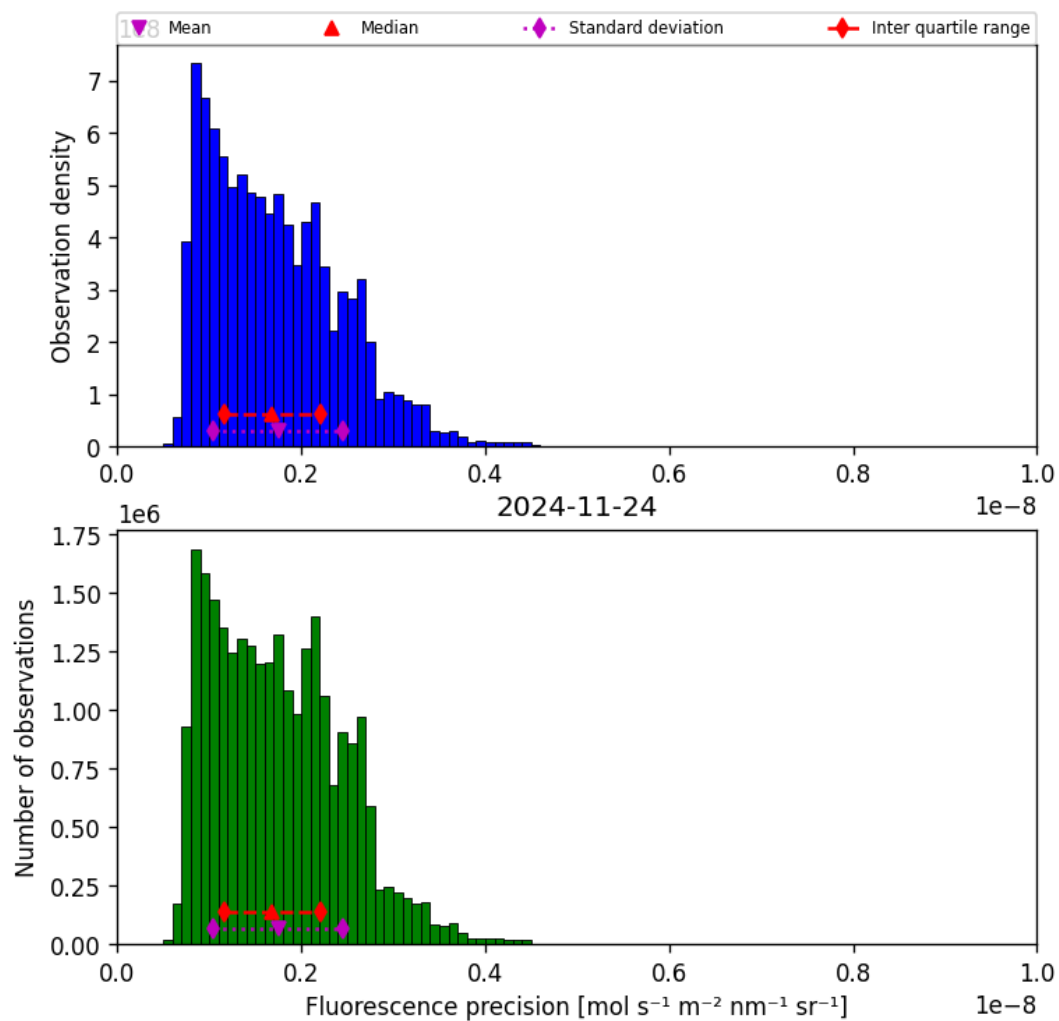
Figure 41: Histogram of “Fluorescence precision” for 2024-11-23 to 2024-11-25
