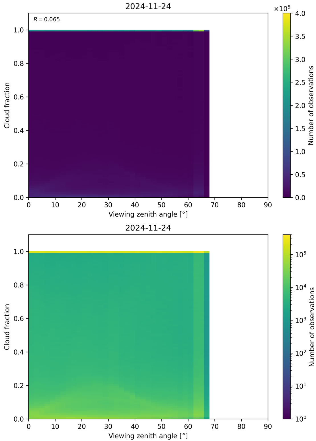
Figure 120: Scatter density plot of “Viewing zenith angle” against “Cloud fraction” for 2024-11-23 to 2024-11-25.
