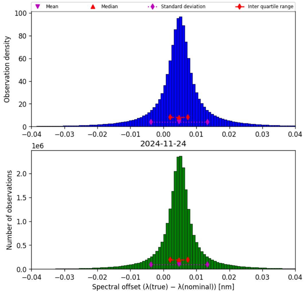
Figure 45: Histogram of “Spectral offset ( \lambda_{\text{true}} - \lambda_{\text{nominal}} )” for 2024-11-23 to 2024-11-25
