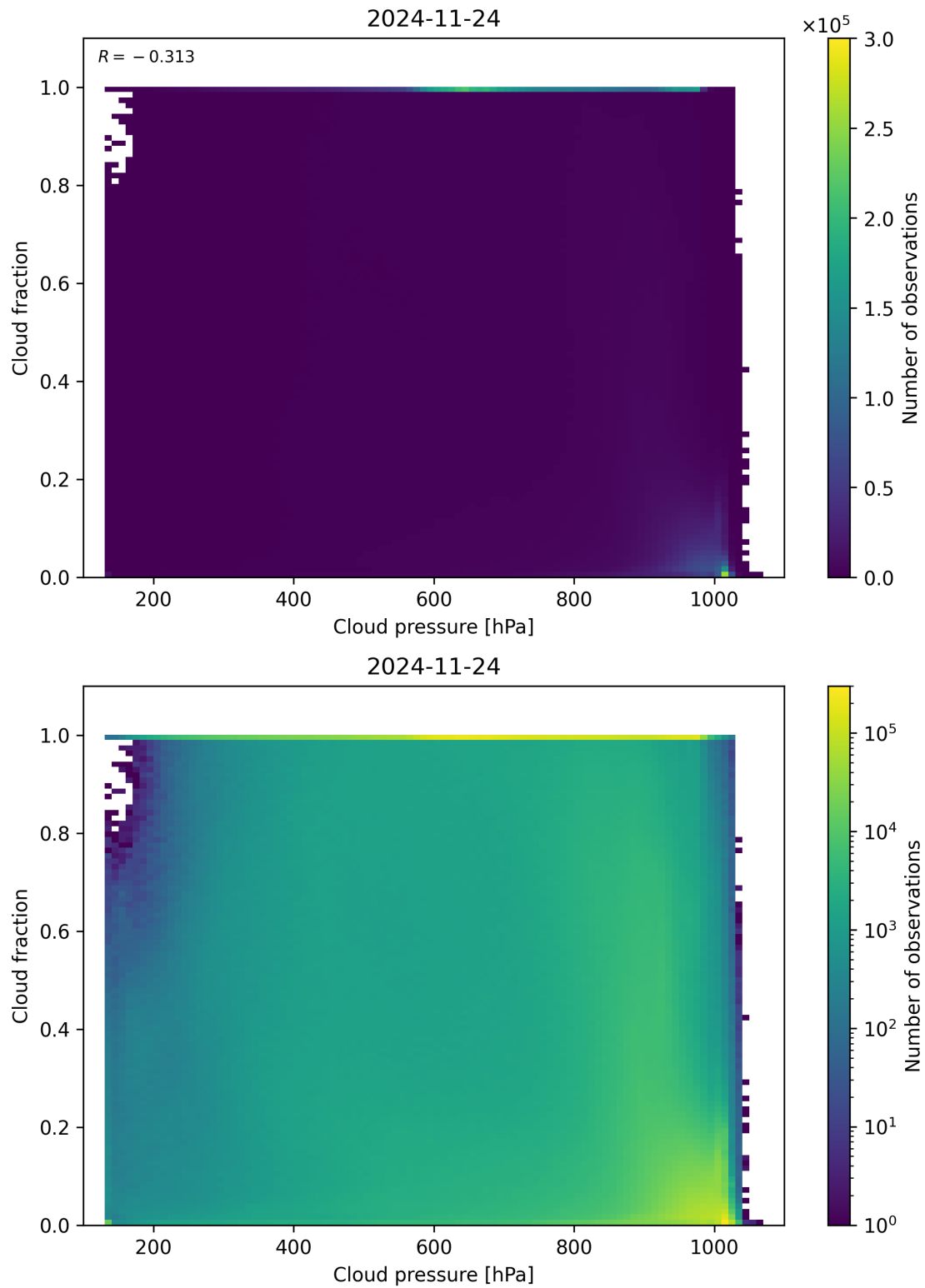
Figure 79: Scatter density plot of “Cloud pressure” against “Cloud fraction” for 2024-11-23 to 2024-11-25.
