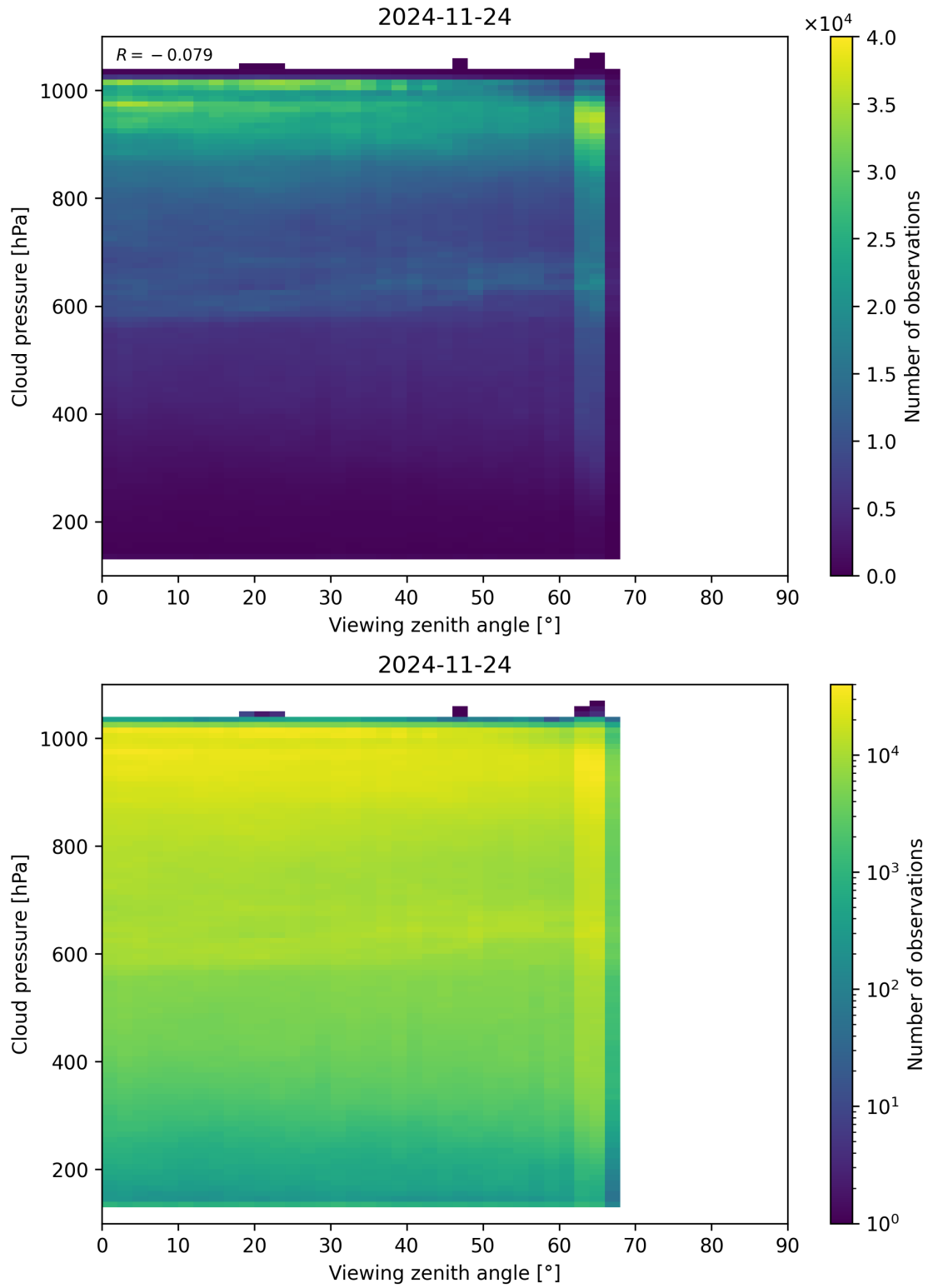
Figure 121: Scatter density plot of “Viewing zenith angle” against “Cloud pressure” for 2024-11-23 to 2024-11-25.
