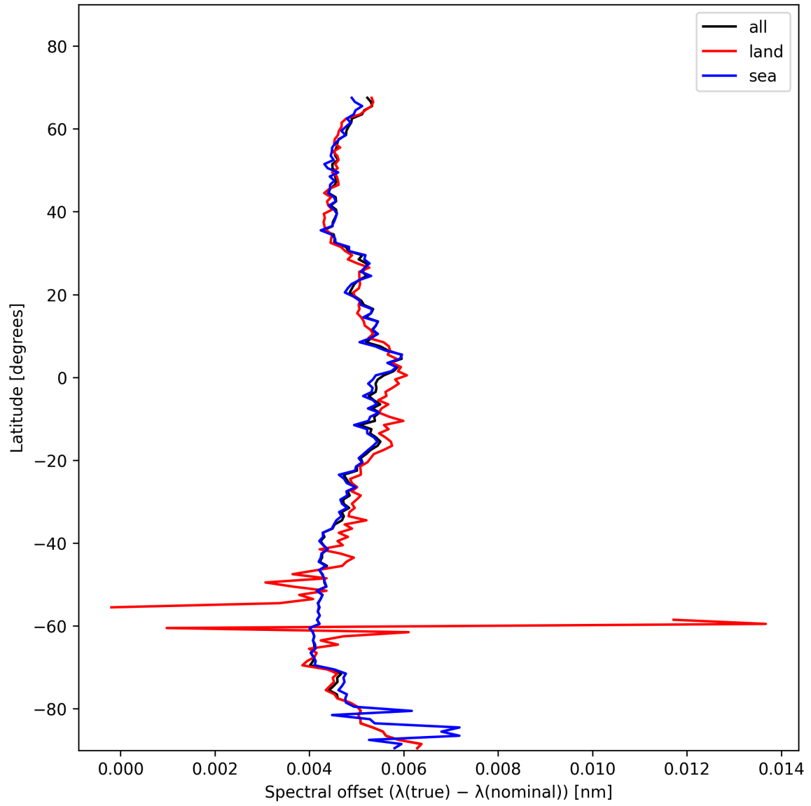
Figure 28: Zonal average of “Spectral offset ( \lambda_{\text{true}} - \lambda_{\text{nominal}} )” for 2024-11-23 to 2024-11-25.
