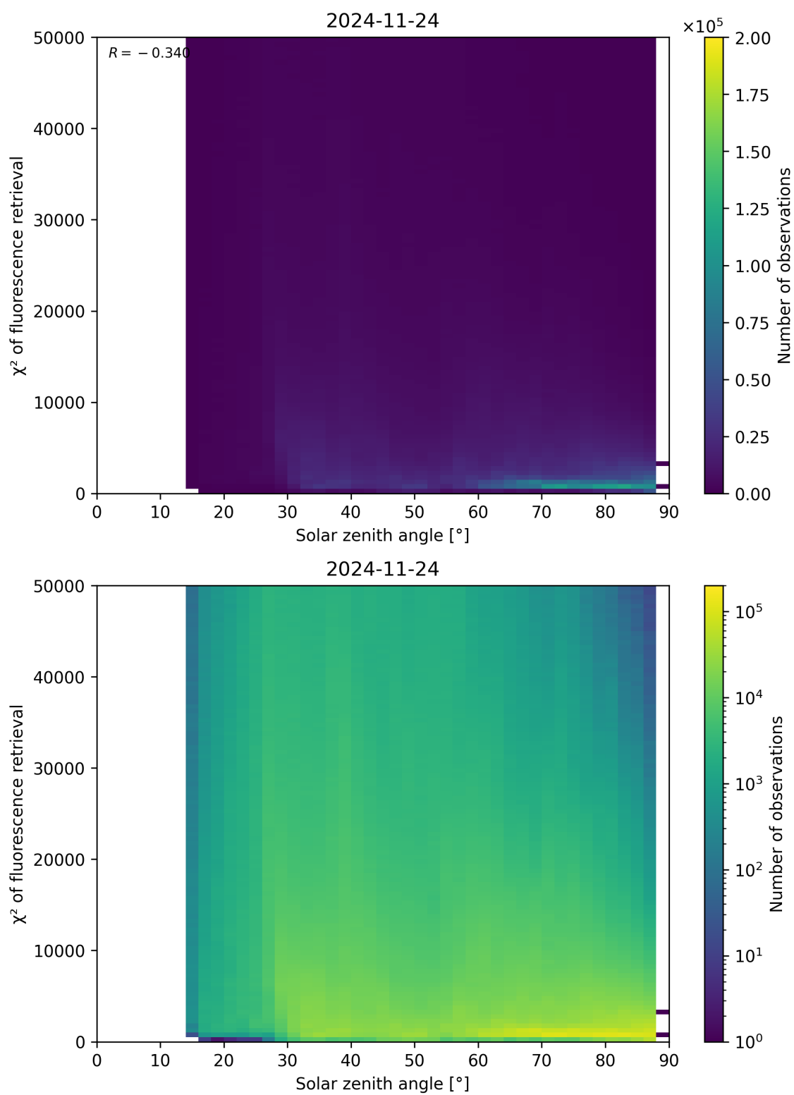
Figure 109: Scatter density plot of “Solar zenith angle” against “ \chi^2 of fluorescence retrieval” for 2024-11-23 to 2024-11-25.
