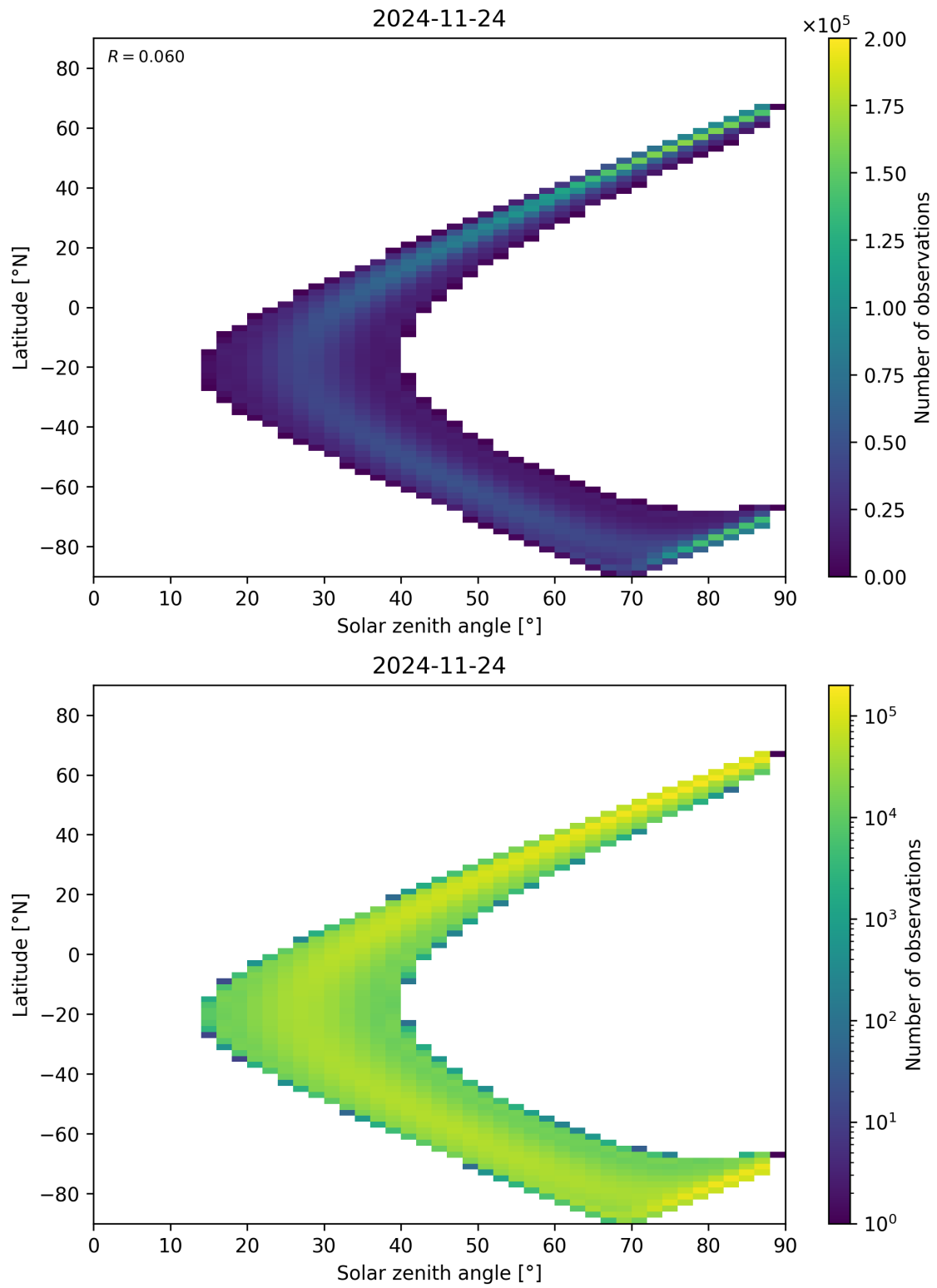
Figure 113: Scatter density plot of “Solar zenith angle” against “Latitude” for 2024-11-23 to 2024-11-25.
