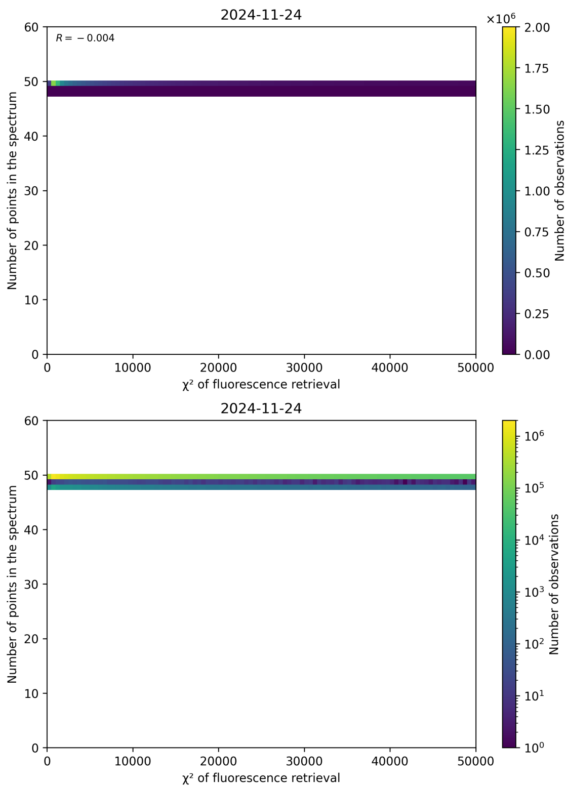
Figure 68: Scatter density plot of " \chi^2 of fluorescence retrieval" against "Number of points in the spectrum" for 2024-11-23 to 2024-11-25.
