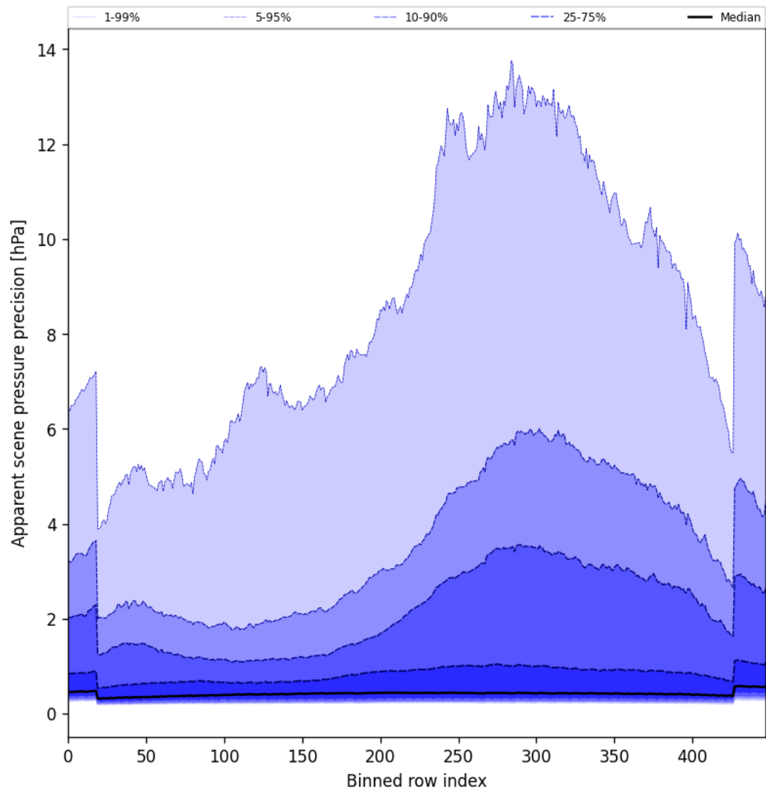
Figure 54: Along track statistics of “Apparent scene pressure precision” for 2024-11-23 to 2024-11-25
