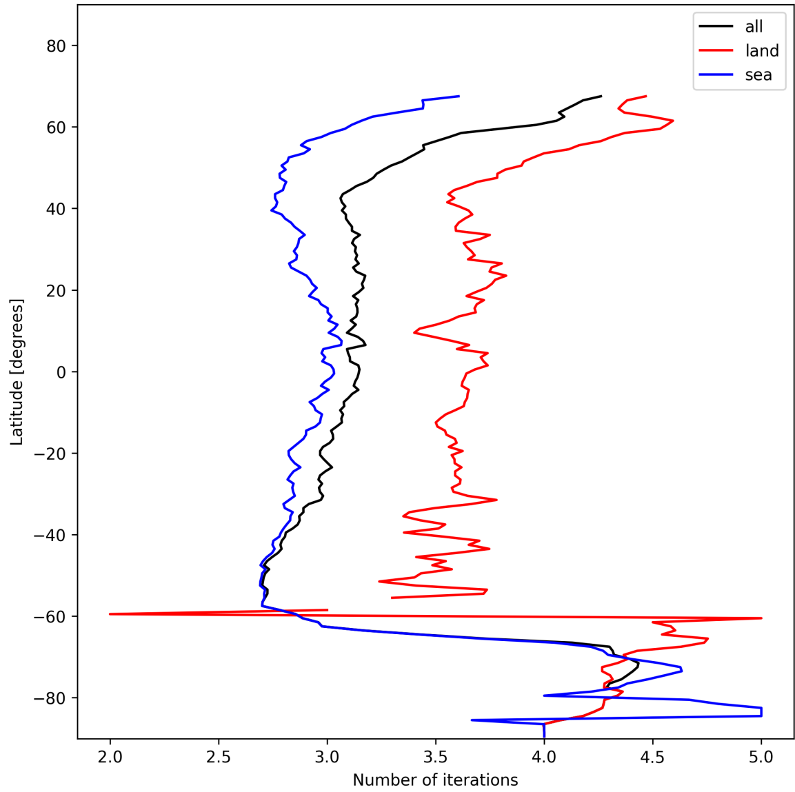
Figure 22: Zonal average of “Number of iterations” for 2024-11-23 to 2024-11-25.
