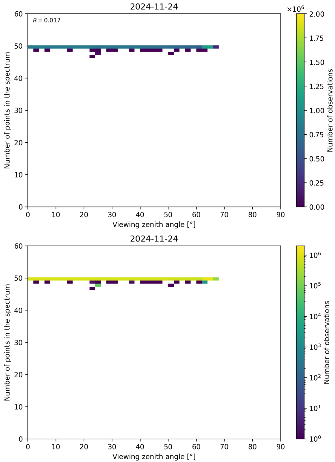
Figure 125: Scatter density plot of “Viewing zenith angle” against “Number of points in the spectrum” for 2024-11-23 to 2024-11-25.
