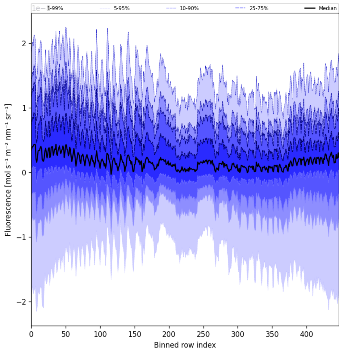
Figure 57: Along track statistics of "Fluorescence" for 2024-11-23 to 2024-11-25
