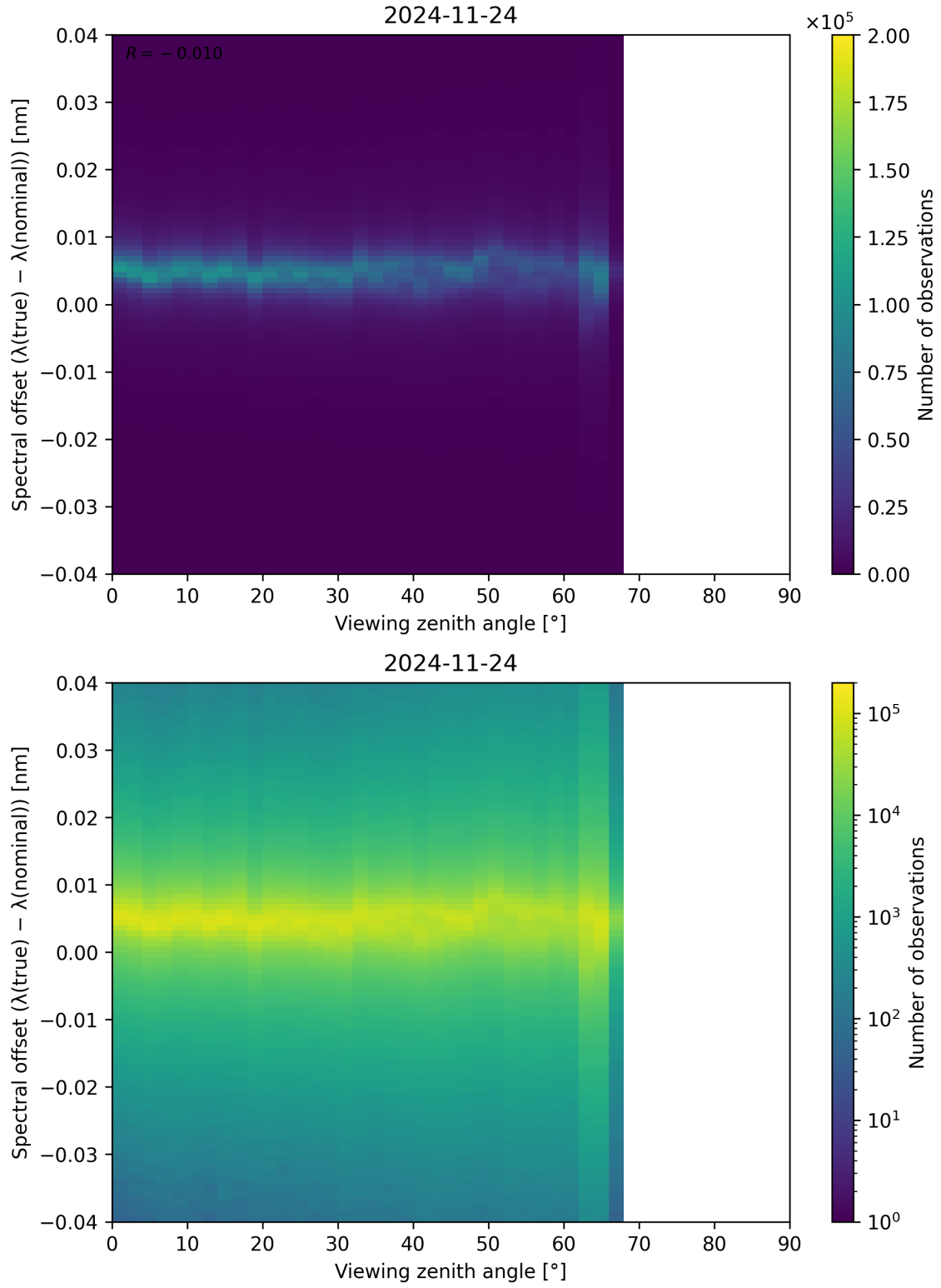
Figure 128: Scatter density plot of “Viewing zenith angle” against “Spectral offset ( \lambda_{\text{true}} - \lambda_{\text{nominal}} )” for 2024-11-23 to 2024-11-25.
