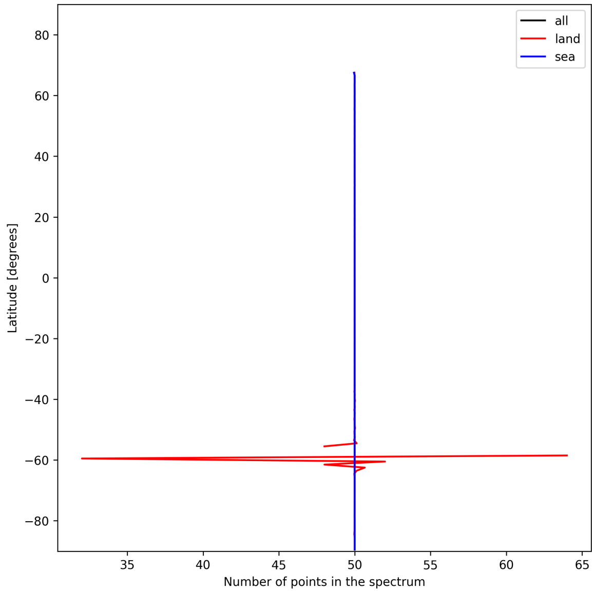
Figure 27: Zonal average of “Number of points in the spectrum” for 2024-11-23 to 2024-11-25.
