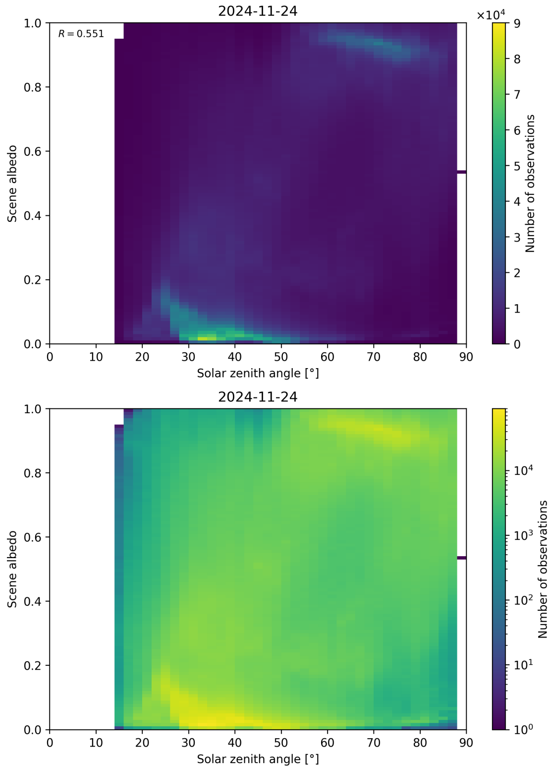
Figure 116: Scatter density plot of “Solar zenith angle” against “Scene albedo” for 2024-11-23 to 2024-11-25.
