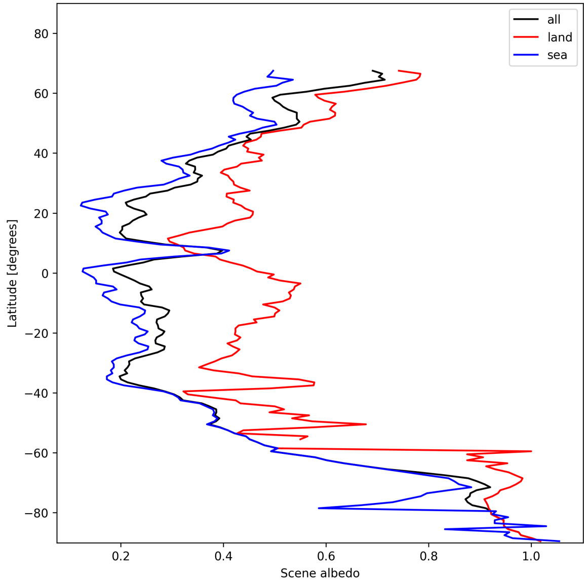
Figure 17: Zonal average of “Scene albedo” for 2024-11-23 to 2024-11-25.
