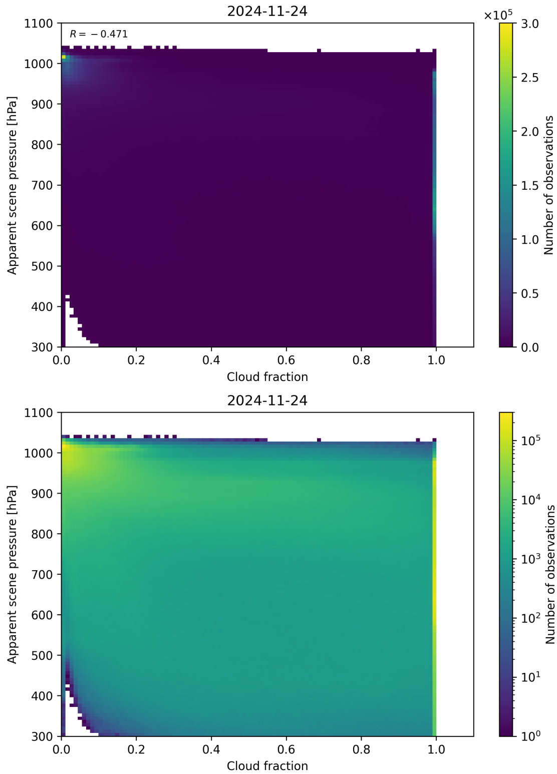
Figure 70: Scatter density plot of “Cloud fraction” against “Apparent scene pressure” for 2024-11-23 to 2024-11-25.
