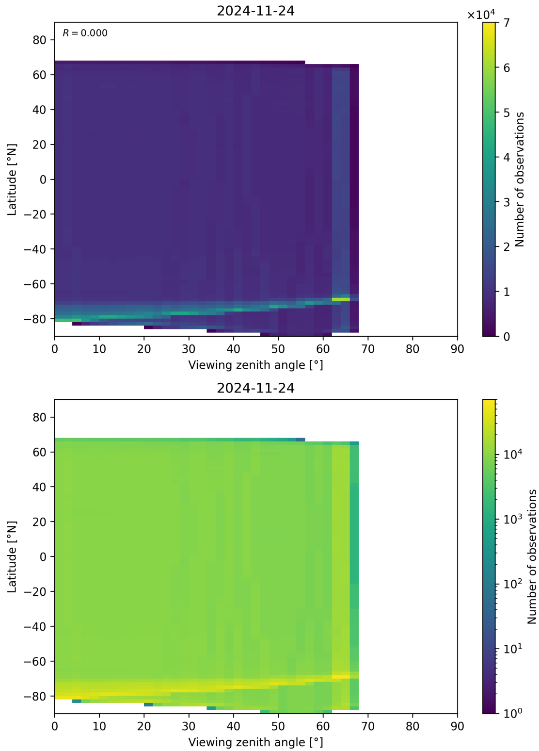
Figure 123: Scatter density plot of “Viewing zenith angle” against “Latitude” for 2024-11-23 to 2024-11-25.
