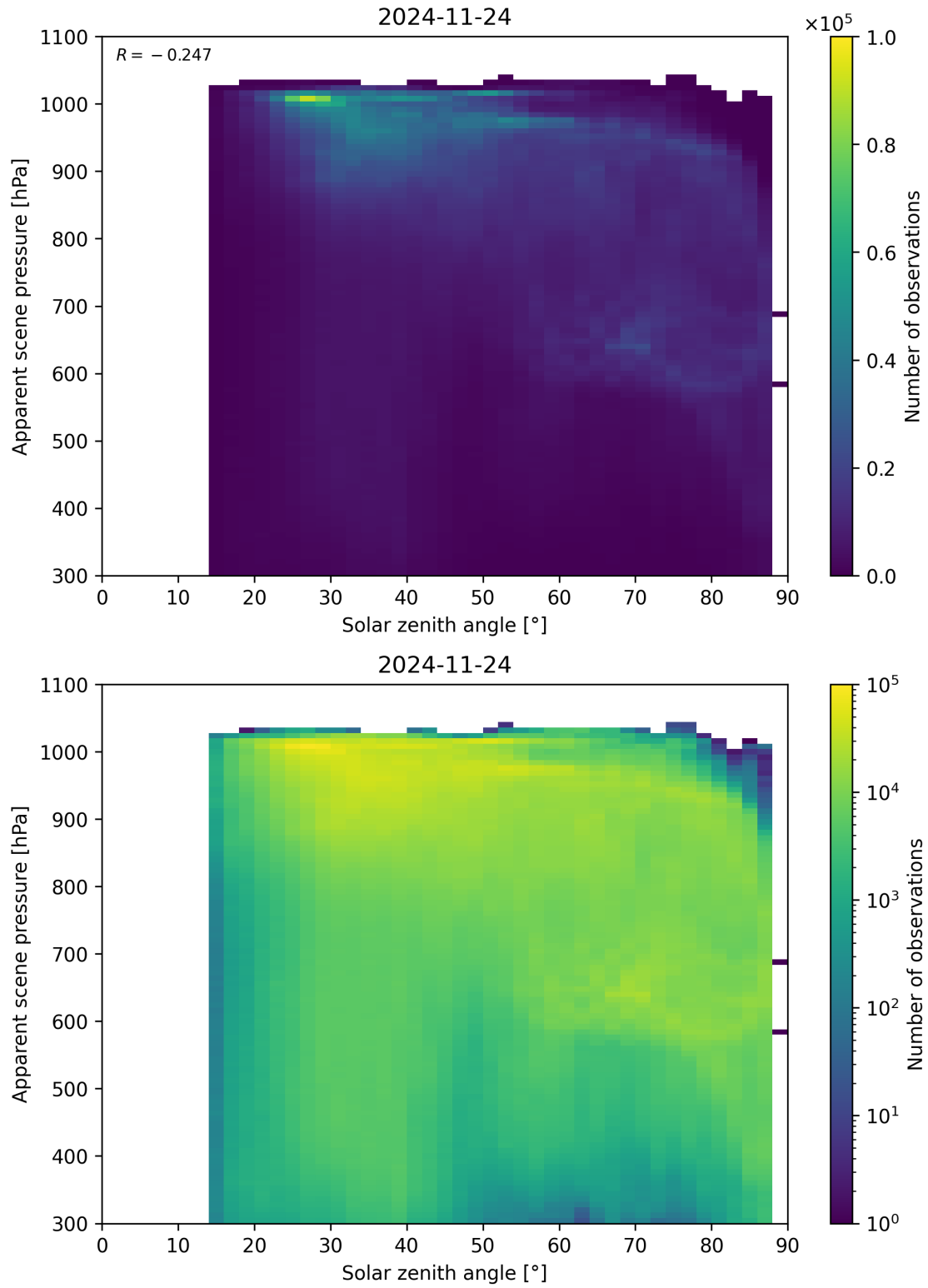
Figure 108: Scatter density plot of “Solar zenith angle” against “Apparent scene pressure” for 2024-11-23 to 2024-11-25.
