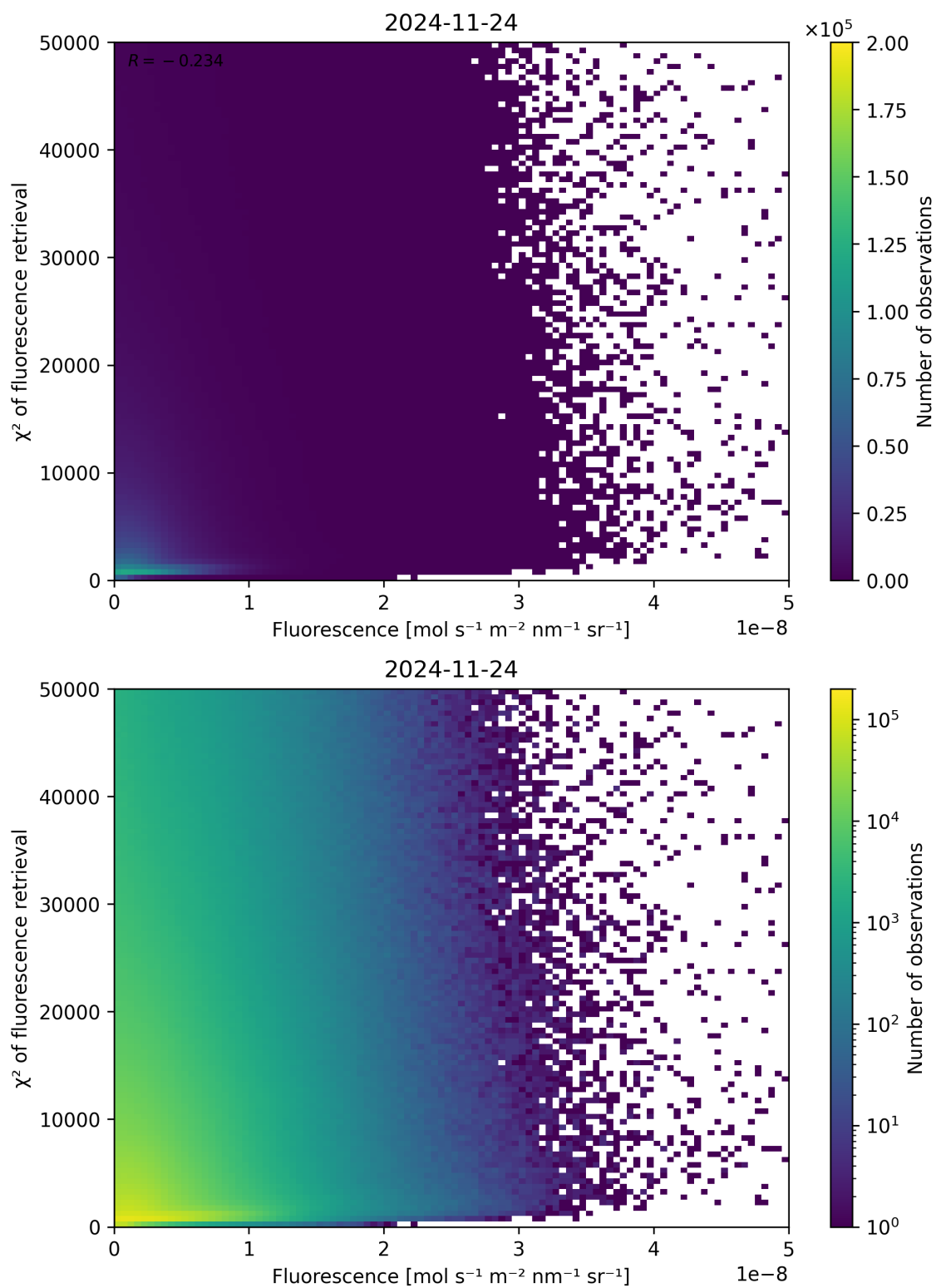
Figure 85: Scatter density plot of “Fluorescence” against “ \chi^2 of fluorescence retrieval” for 2024-11-23 to 2024-11-25.
