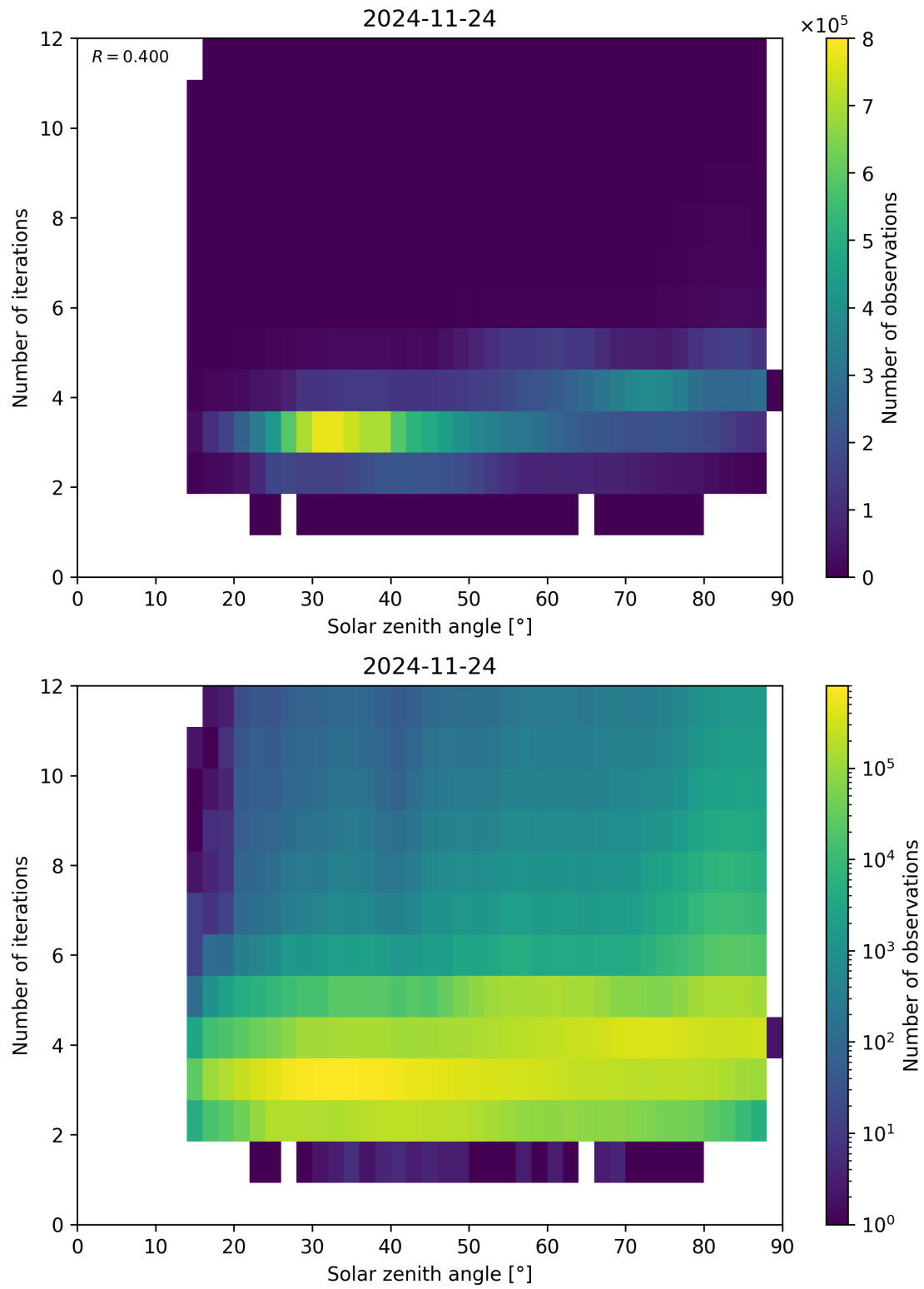
Figure 114: Scatter density plot of “Solar zenith angle” against “Number of iterations” for 2024-11-23 to 2024-11-25.
