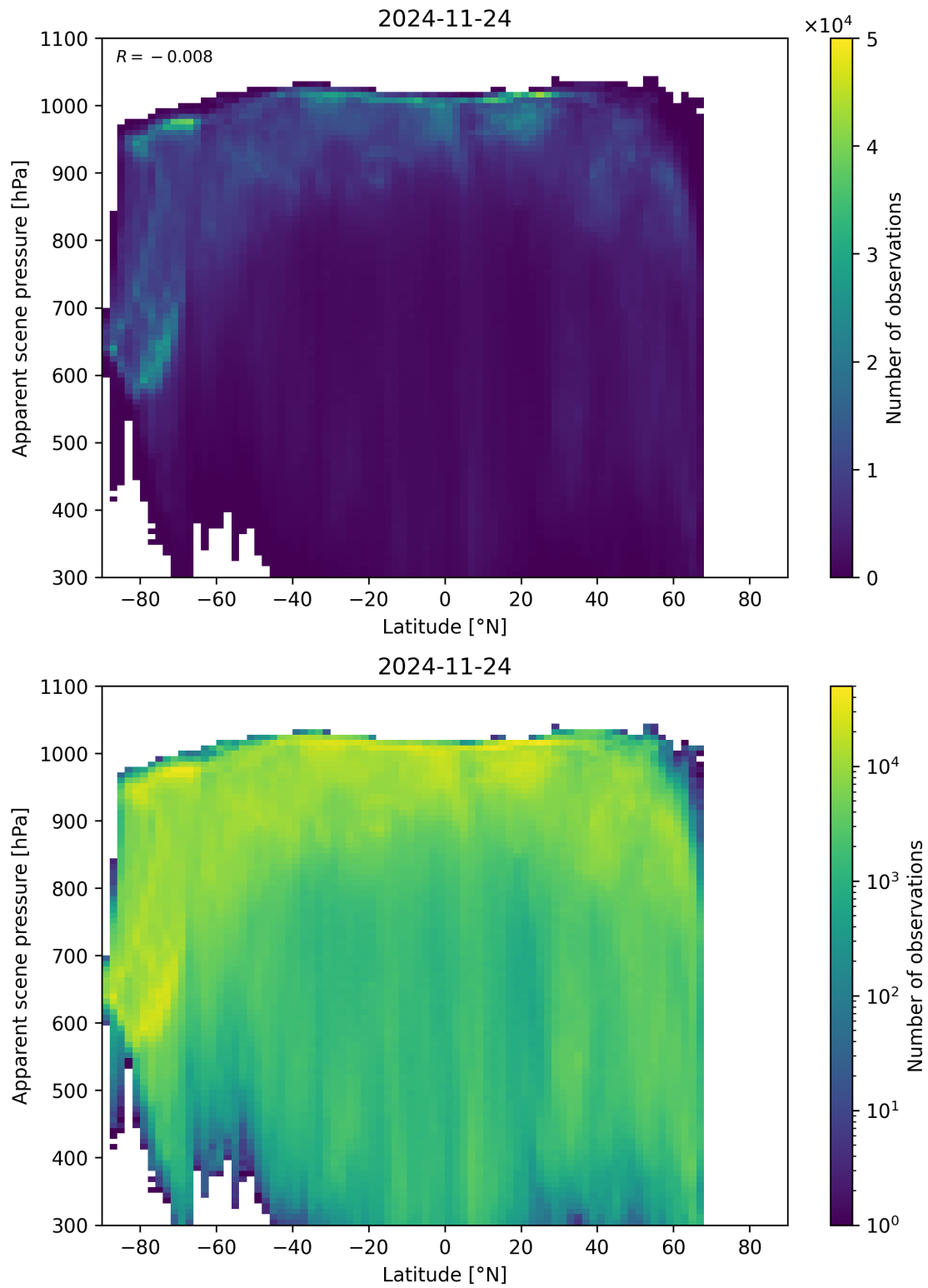
Figure 88: Scatter density plot of “Latitude” against “Apparent scene pressure” for 2024-11-23 to 2024-11-25.
