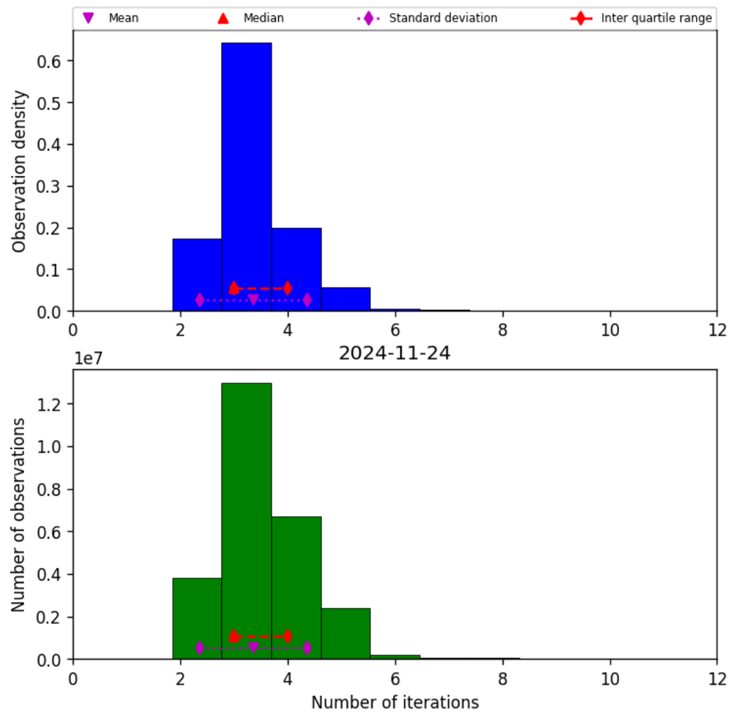
Figure 39: Histogram of “Number of iterations” for 2024-11-23 to 2024-11-25
