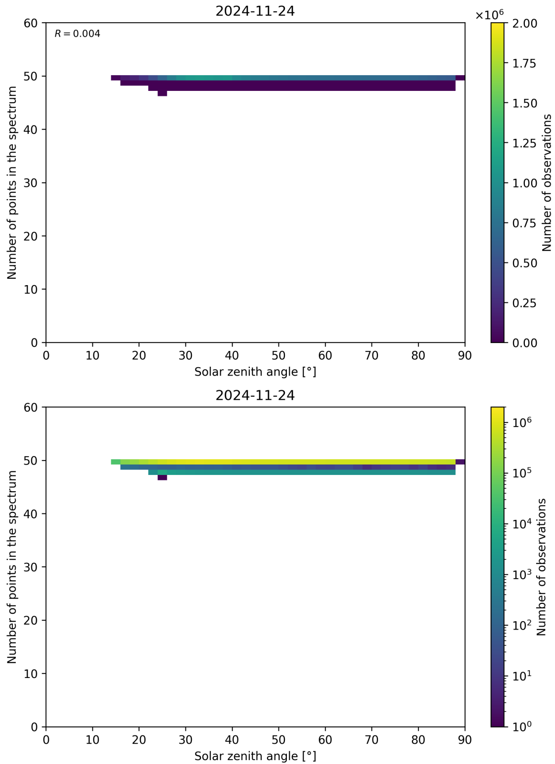
Figure 115: Scatter density plot of “Solar zenith angle” against “Number of points in the spectrum” for 2024-11-23 to 2024-11-25.
