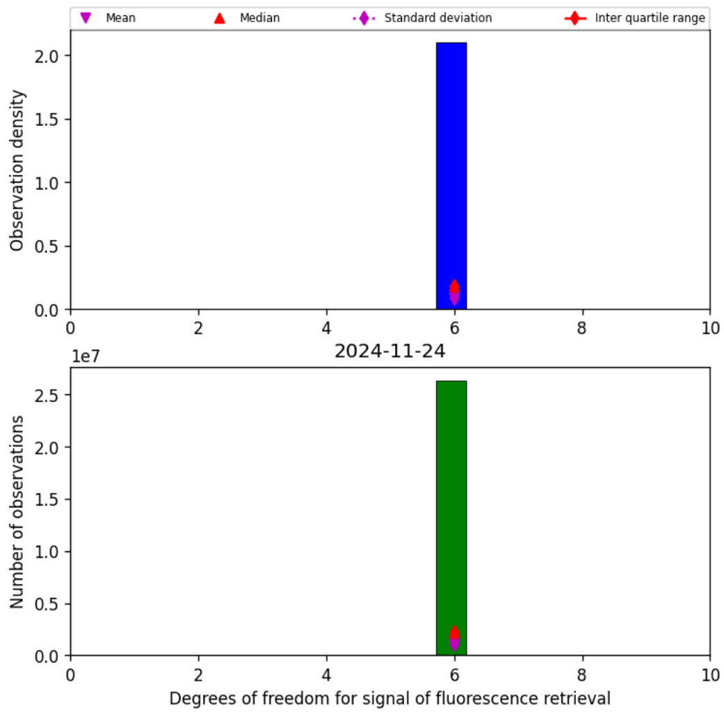
Figure 43: Histogram of “Degrees of freedom for signal of fluorescence retrieval” for 2024-11-23 to 2024-11-25
