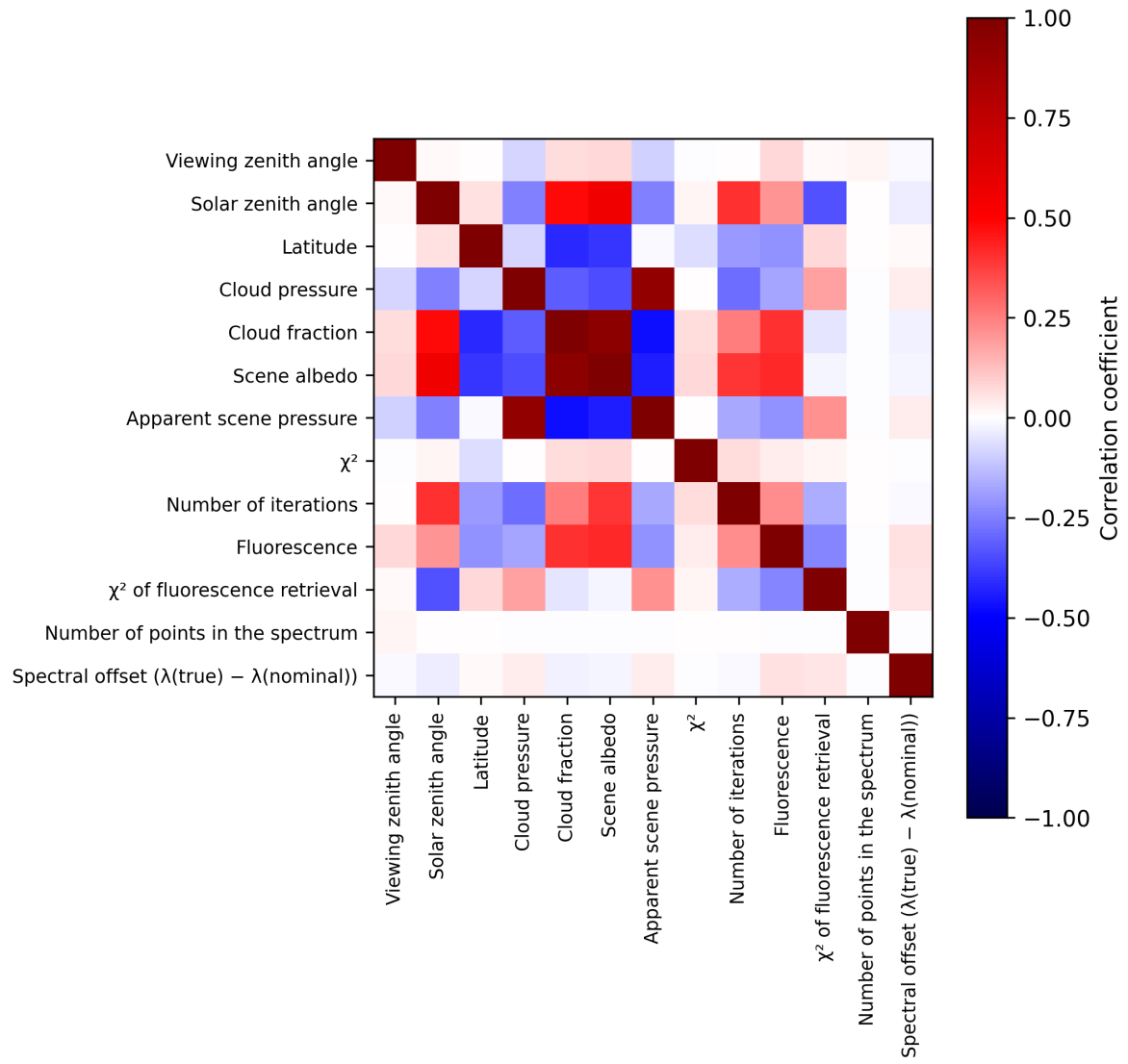
Figure 2: Map of correlation matrix for 2024-11-23 to 2024-11-25.
