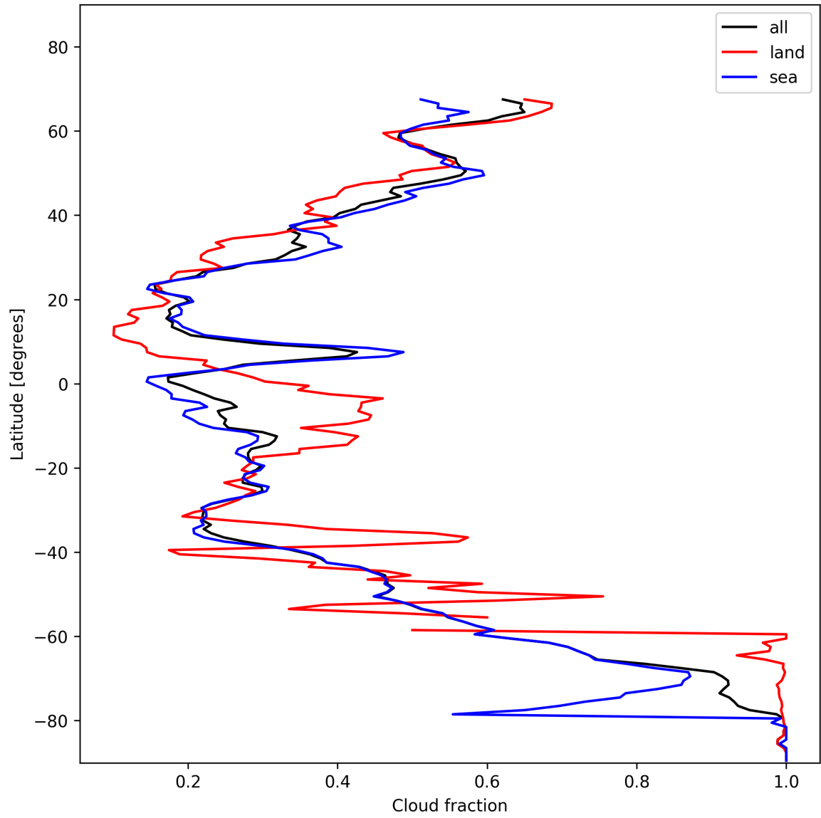
Figure 15: Zonal average of “Cloud fraction” for 2024-11-23 to 2024-11-25.
