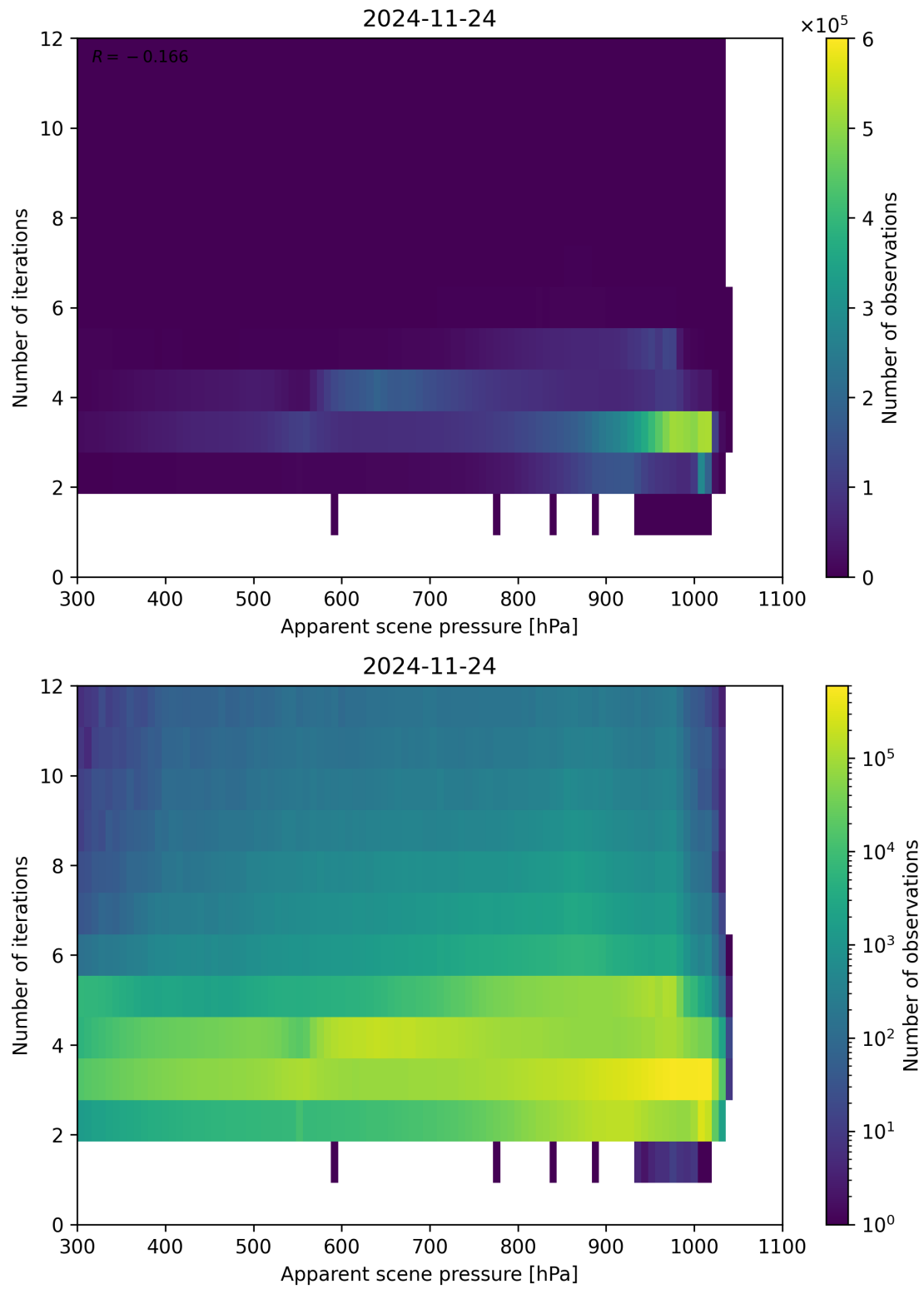
Figure 65: Scatter density plot of “Apparent scene pressure” against “Number of iterations” for 2024-11-23 to 2024-11-25.
