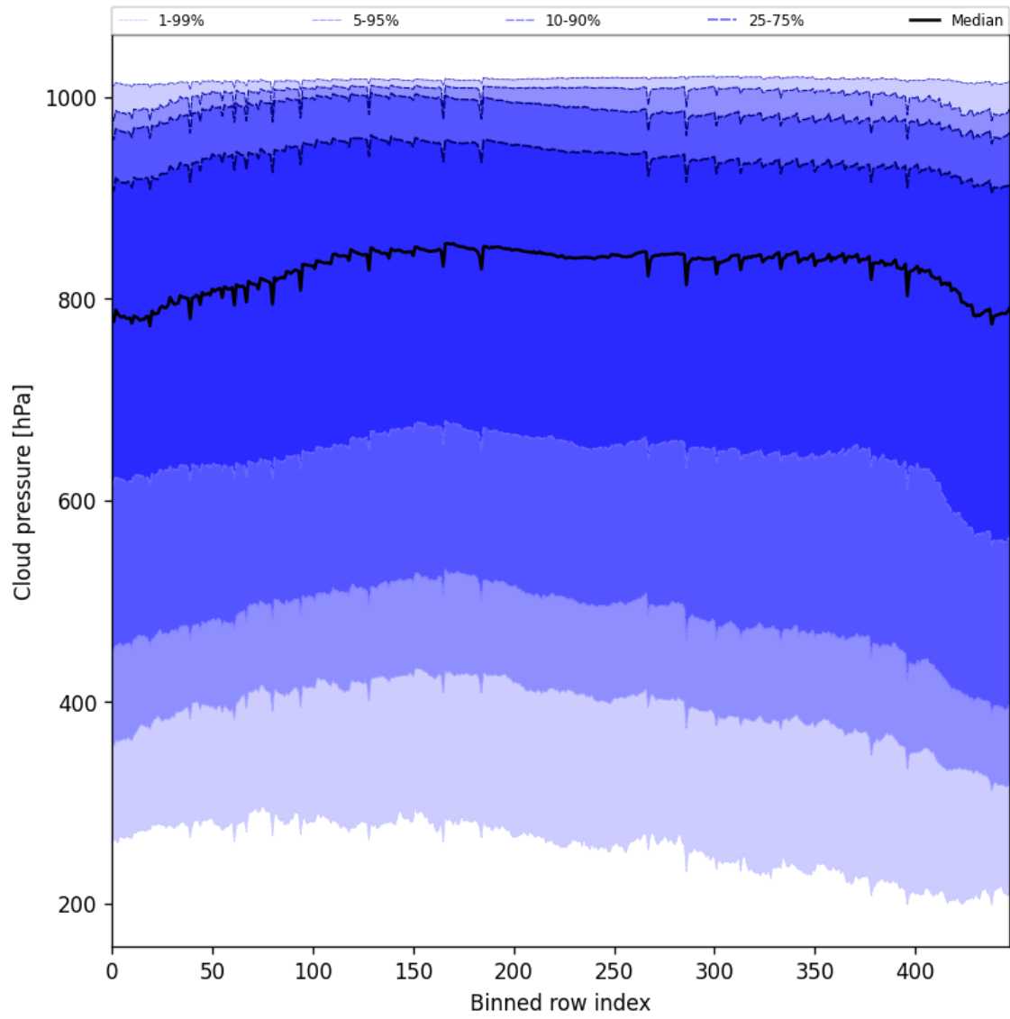
Figure 47: Along track statistics of “Cloud pressure” for 2024-11-23 to 2024-11-25
