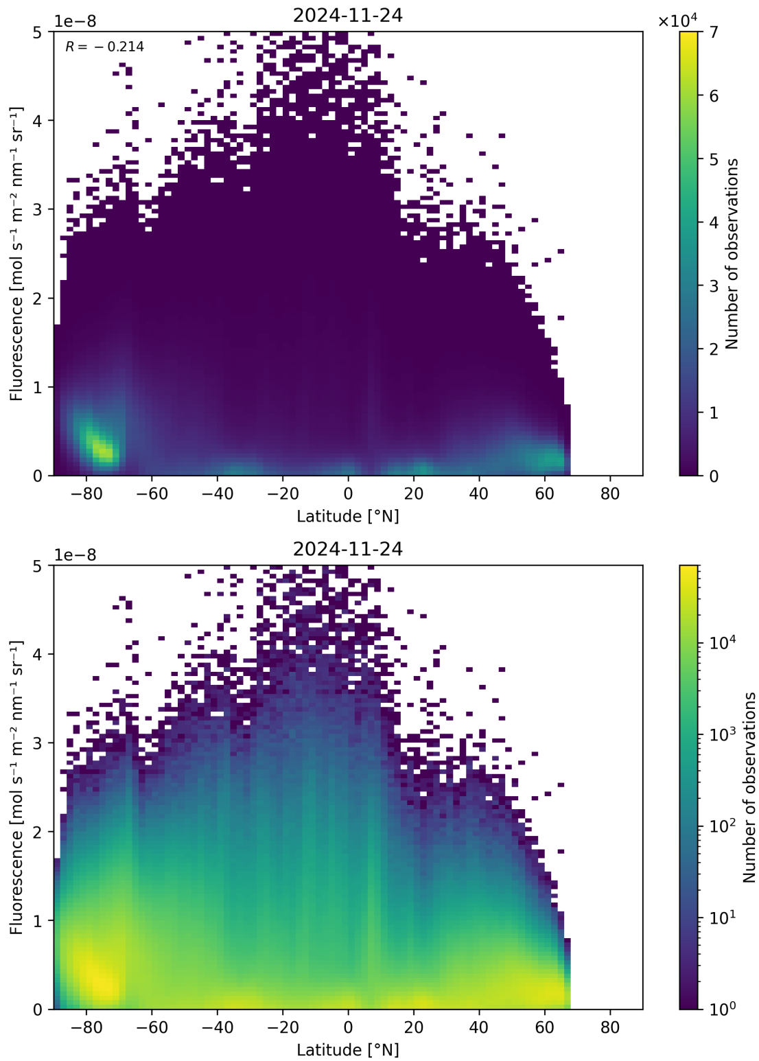
Figure 92: Scatter density plot of “Latitude” against “Fluorescence” for 2024-11-23 to 2024-11-25.
