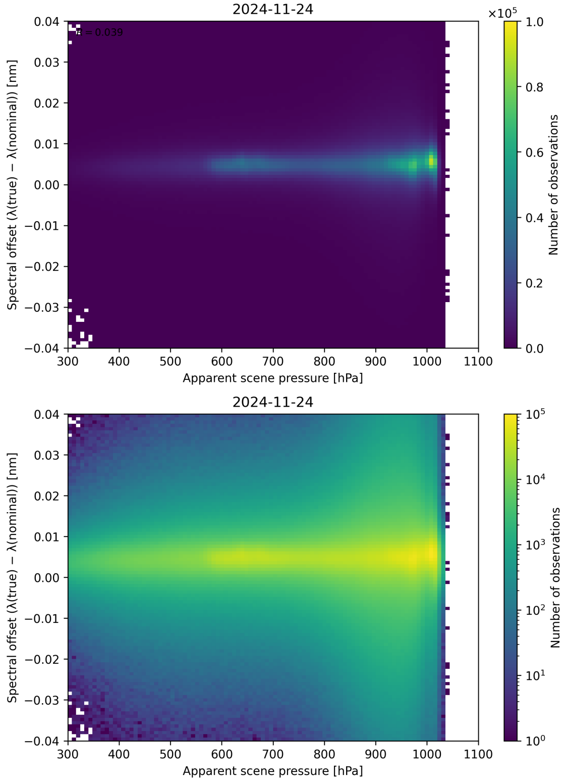
Figure 67: Scatter density plot of “Apparent scene pressure” against “Spectral offset ( \lambda_{\text{true}} - \lambda_{\text{nominal}} )” for 2024-11-23 to 2024-11-25.
