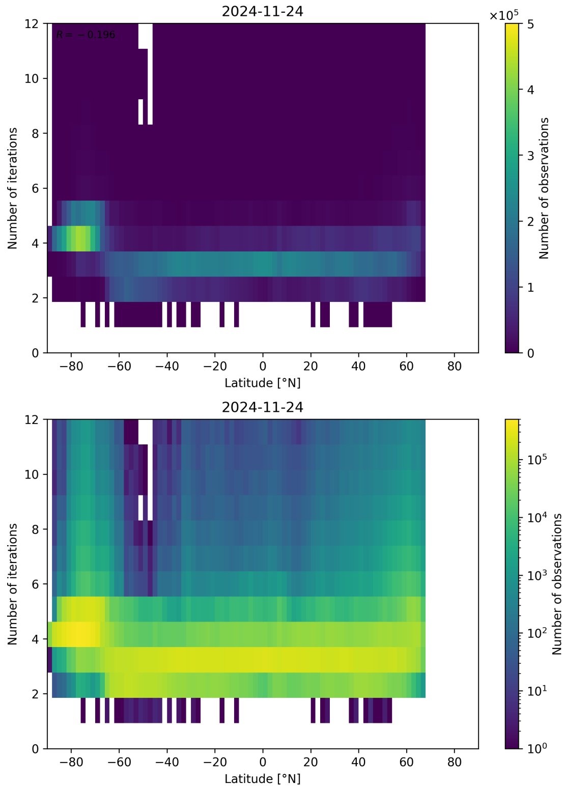
Figure 93: Scatter density plot of “Latitude” against “Number of iterations” for 2024-11-23 to 2024-11-25.
