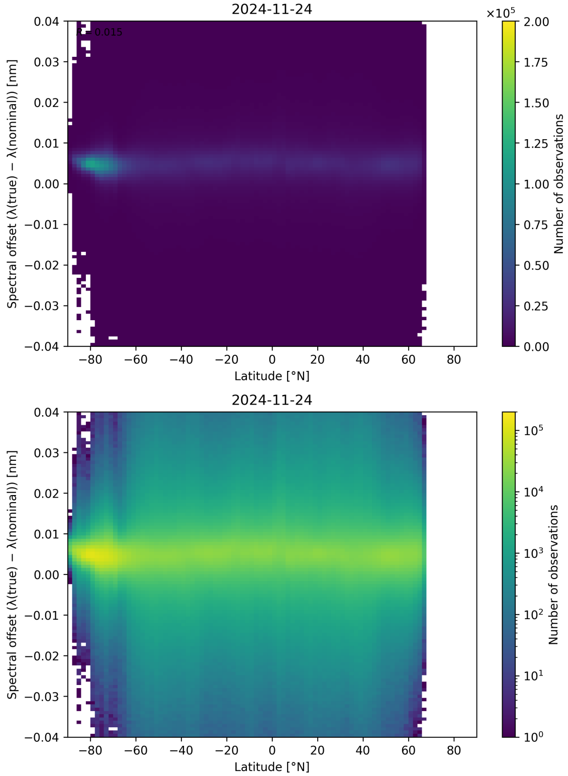
Figure 96: Scatter density plot of “Latitude” against “Spectral offset ( \lambda_{\text{true}} - \lambda_{\text{nominal}} )” for 2024-11-23 to 2024-11-25.
