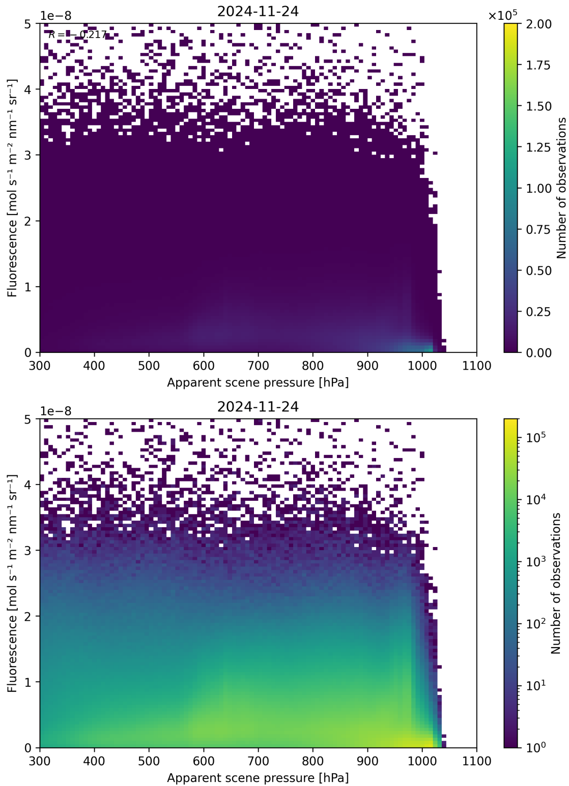
Figure 64: Scatter density plot of “Apparent scene pressure” against “Fluorescence” for 2024-11-23 to 2024-11-25.
