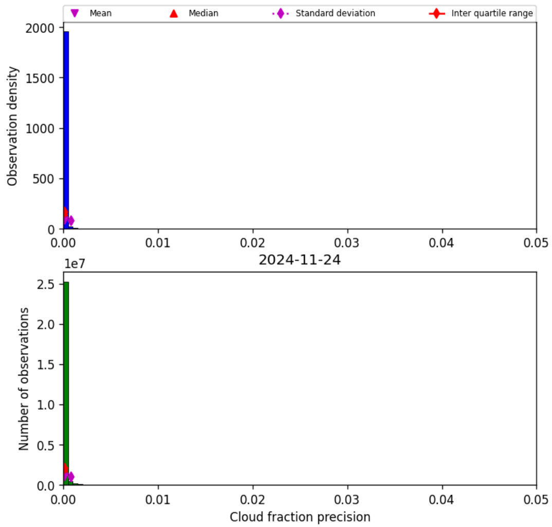
Figure 33: Histogram of “Cloud fraction precision” for 2024-11-23 to 2024-11-25
