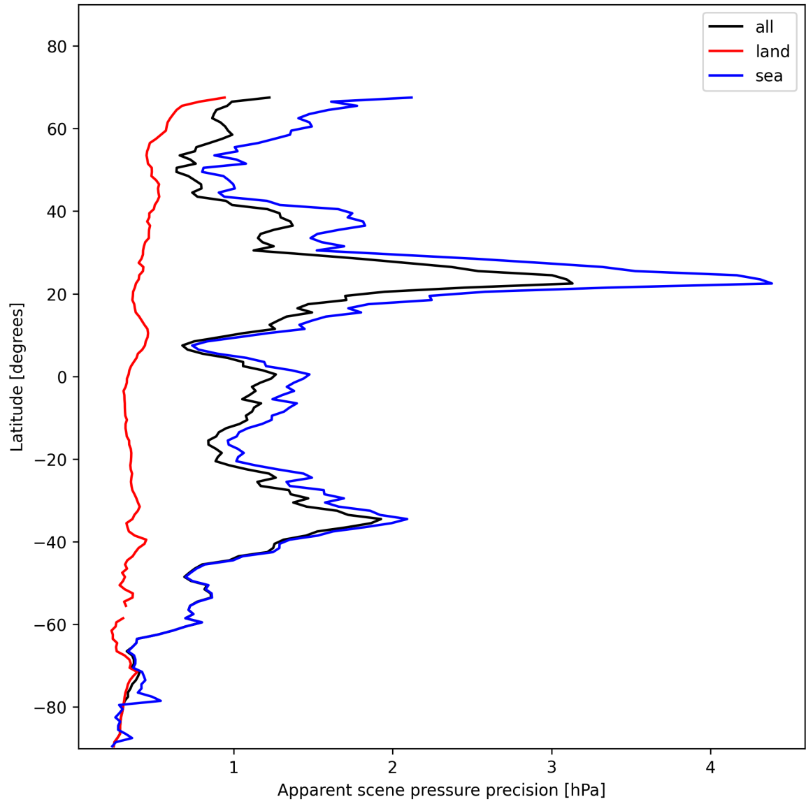
Figure 20: Zonal average of “Apparent scene pressure precision” for 2024-11-23 to 2024-11-25.
