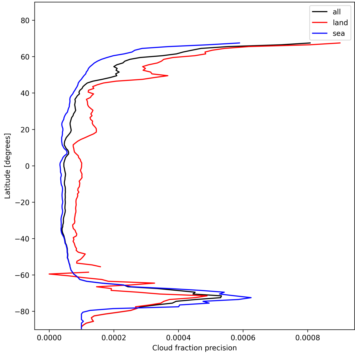
Figure 16: Zonal average of “Cloud fraction precision” for 2024-11-23 to 2024-11-25.
