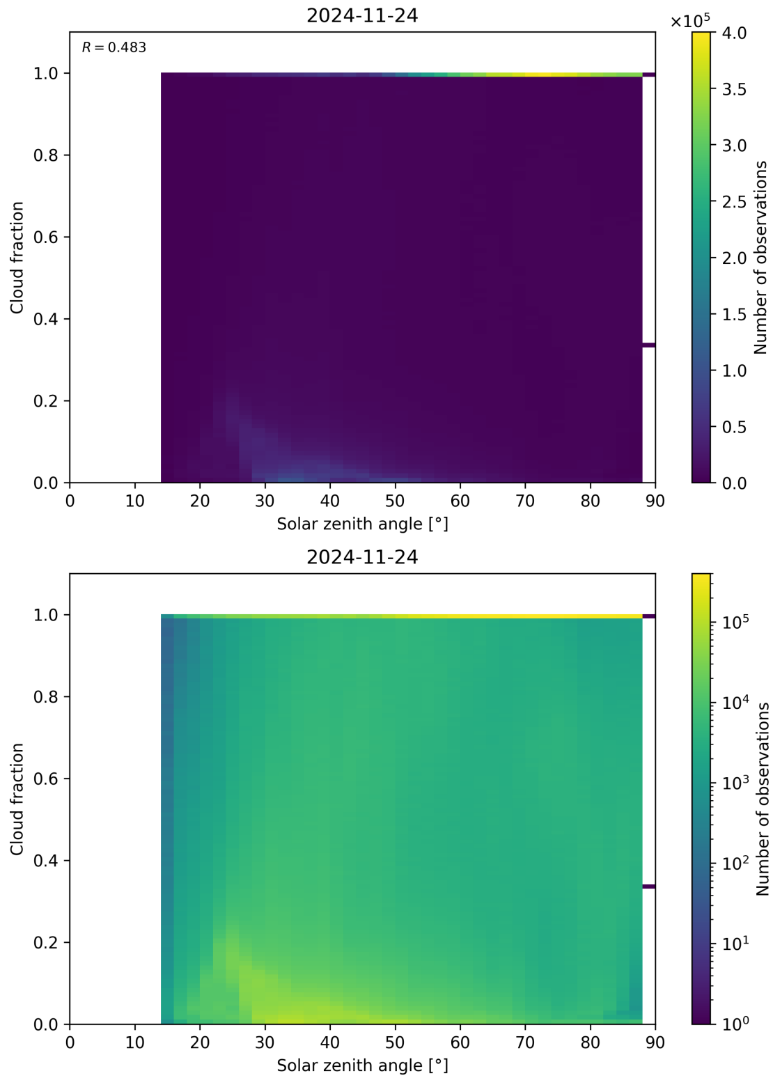
Figure 110: Scatter density plot of “Solar zenith angle” against “Cloud fraction” for 2024-11-23 to 2024-11-25.
