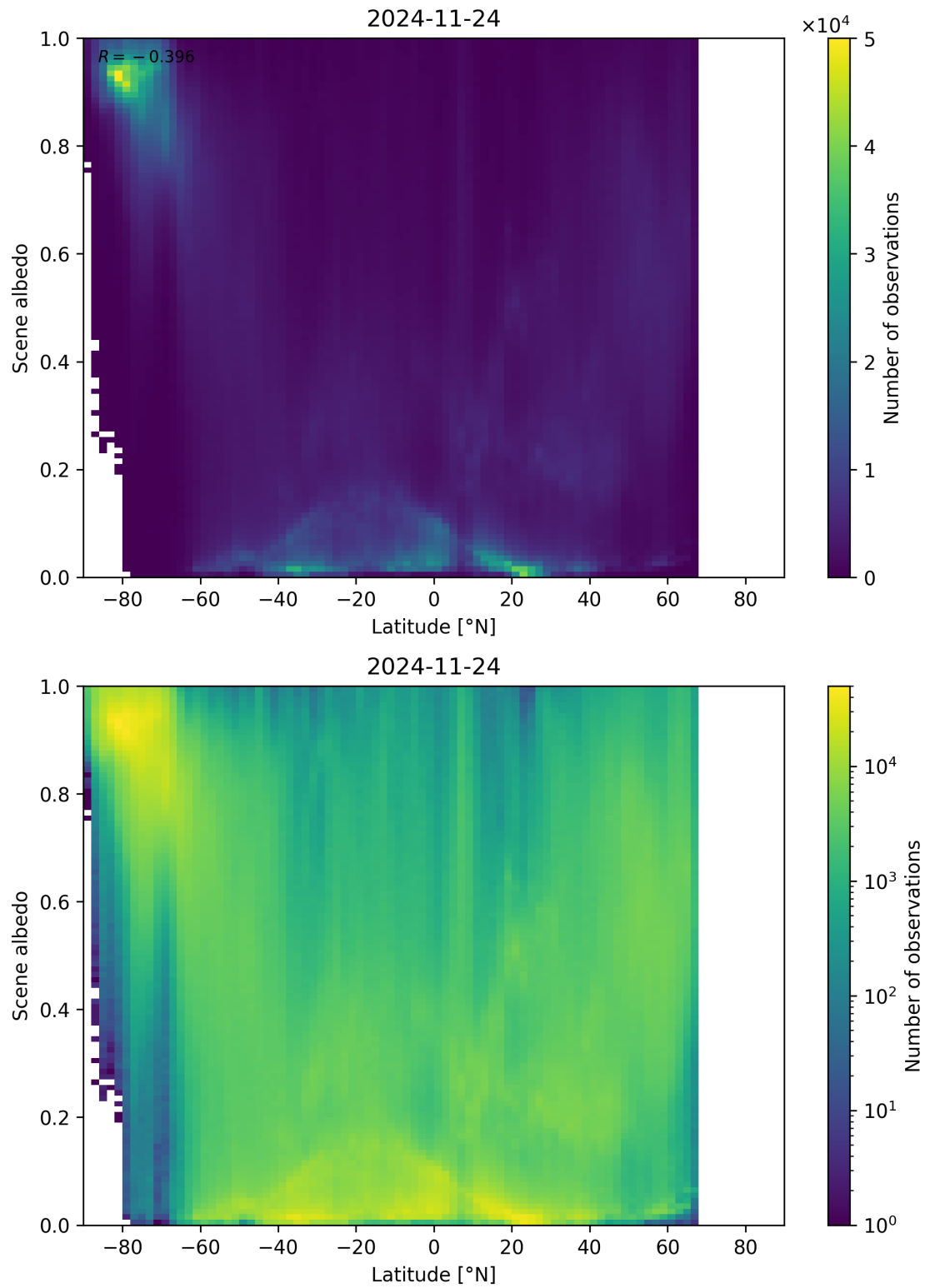
Figure 95: Scatter density plot of “Latitude” against “Scene albedo” for 2024-11-23 to 2024-11-25.
