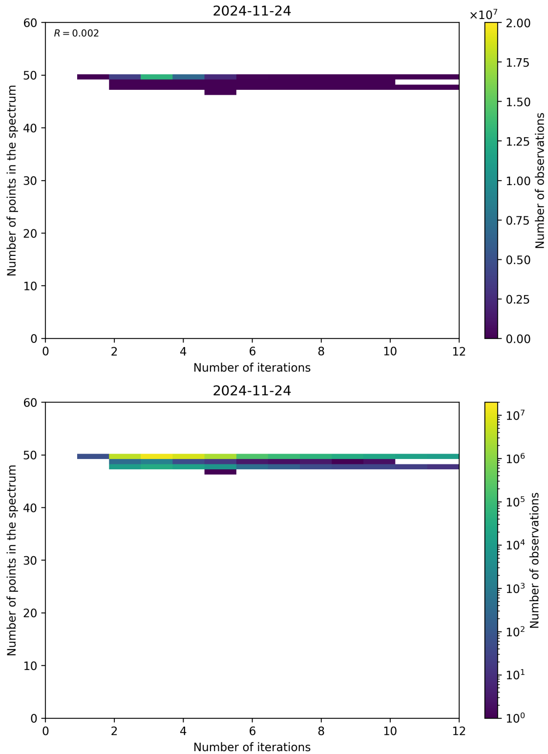
Figure 99: Scatter density plot of “Number of iterations” against “Number of points in the spectrum” for 2024-11-23 to 2024-11-25.
