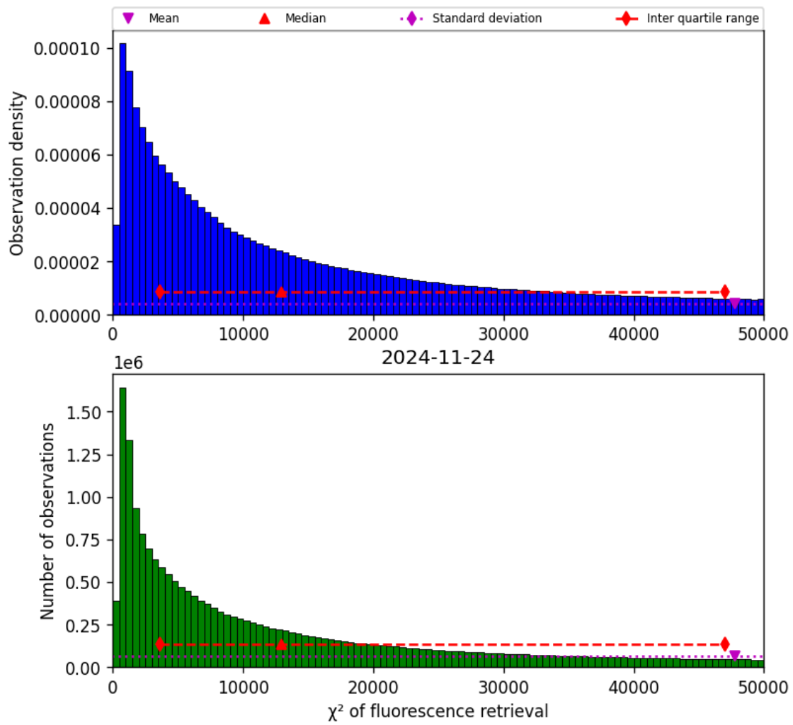
Figure 42: Histogram of “ \chi^2 of fluorescence retrieval” for 2024-11-23 to 2024-11-25
