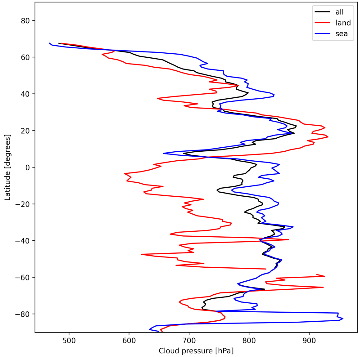
Figure 13: Zonal average of “Cloud pressure” for 2024-11-23 to 2024-11-25.
