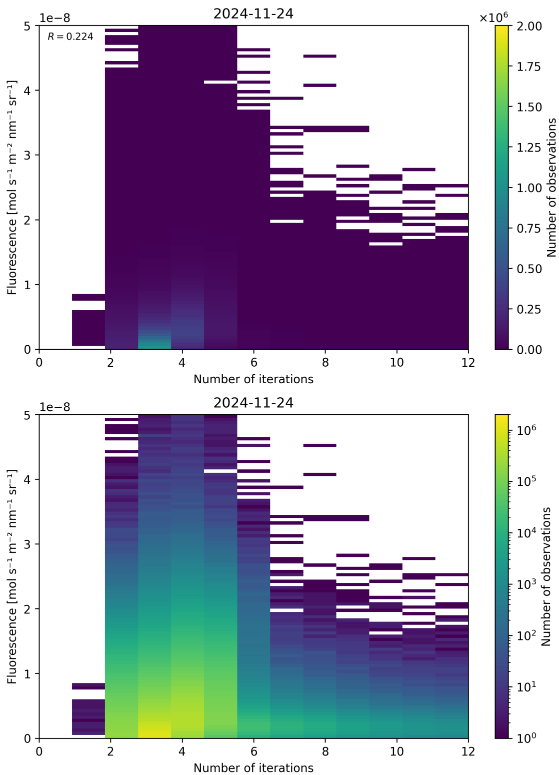
Figure 98: Scatter density plot of “Number of iterations” against “Fluorescence” for 2024-11-23 to 2024-11-25.
