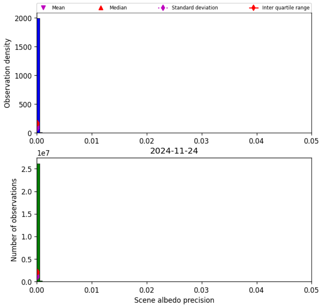
Figure 35: Histogram of “Scene albedo precision” for 2024-11-23 to 2024-11-25
