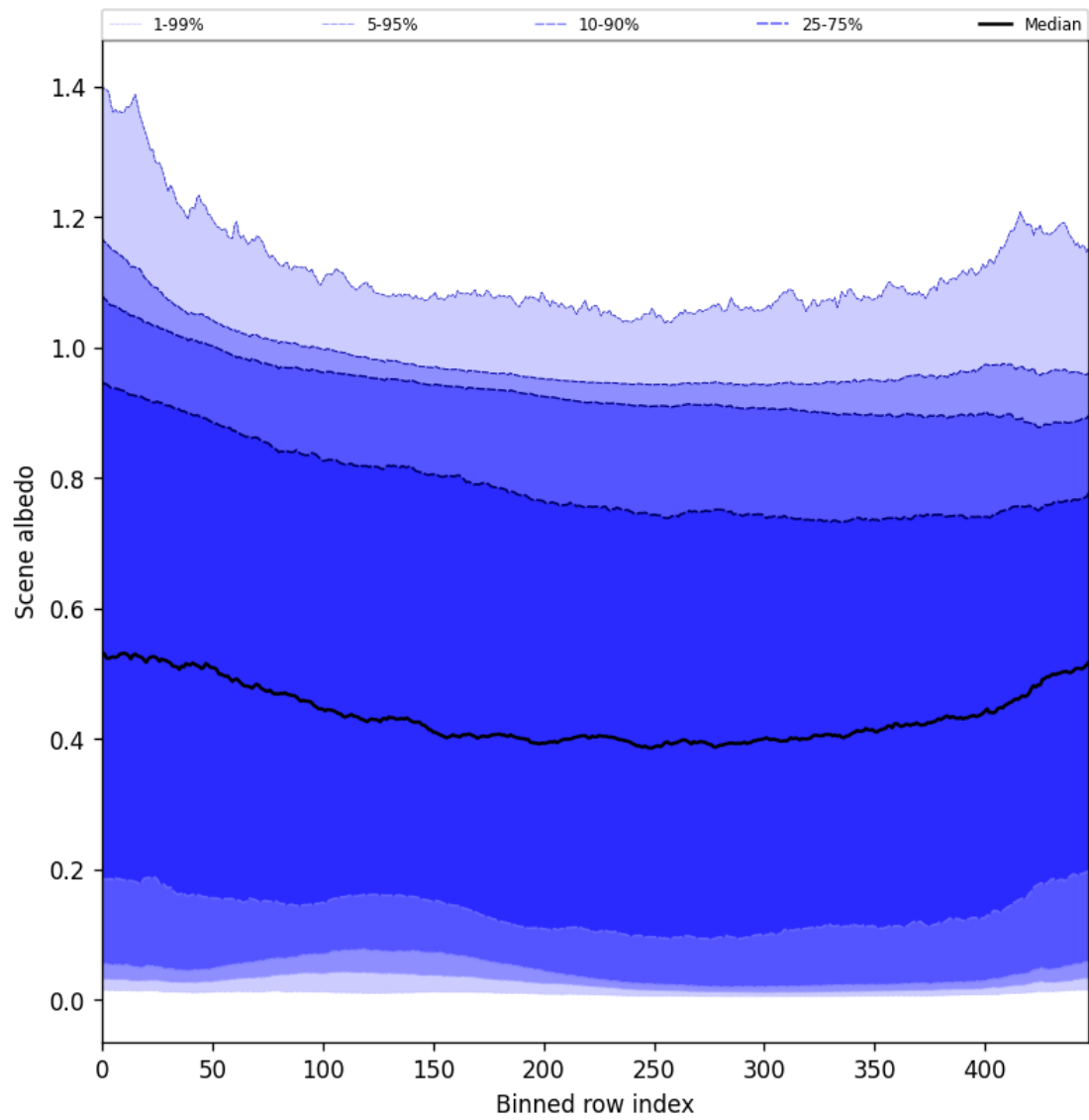
Figure 51: Along track statistics of “Scene albedo” for 2024-11-23 to 2024-11-25
