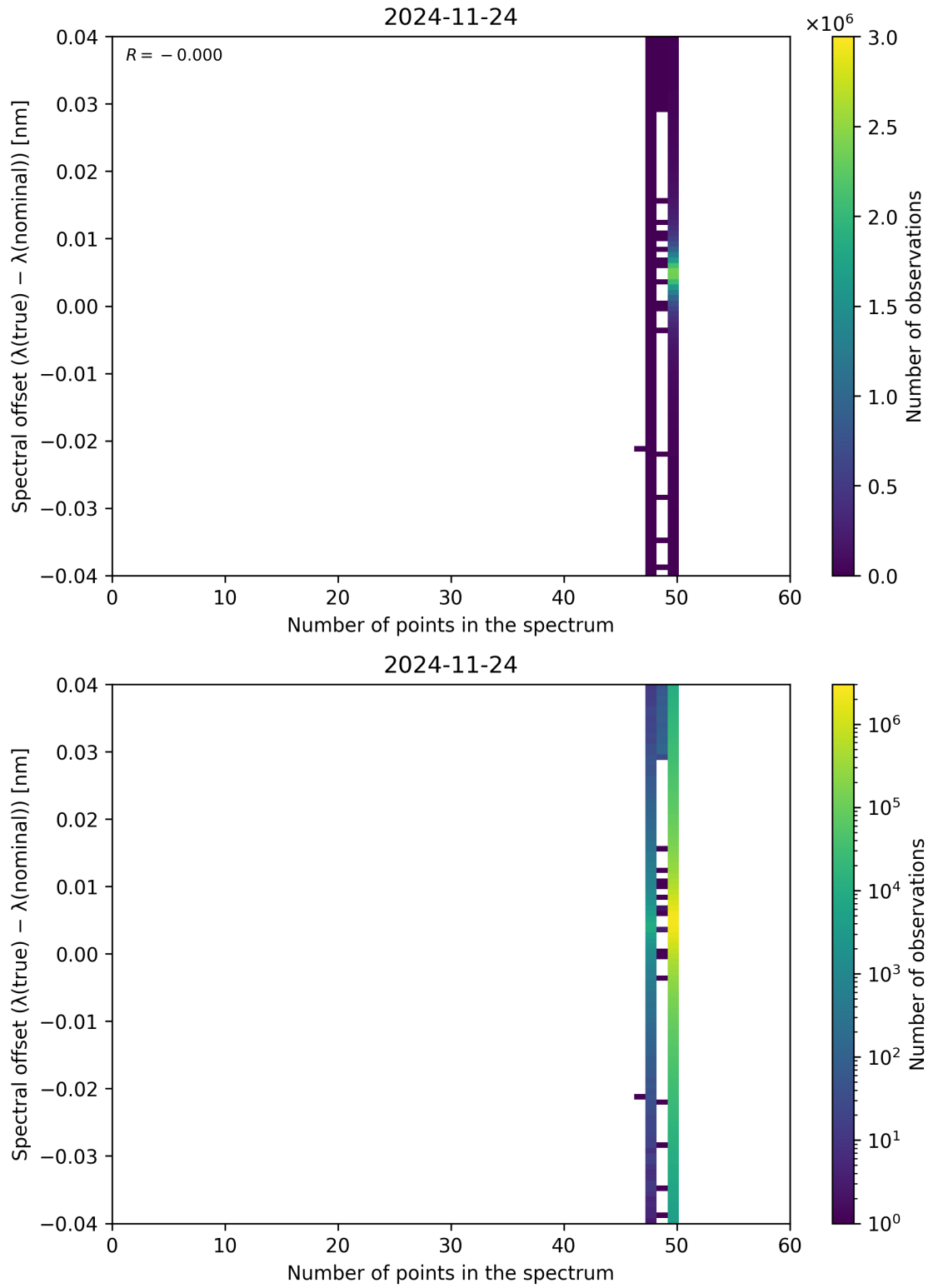
Figure 101: Scatter density plot of “Number of points in the spectrum” against “Spectral offset ( \lambda_{\text{true}} - \lambda_{\text{nominal}} )” for 2024-11-23 to 2024-11-25.
