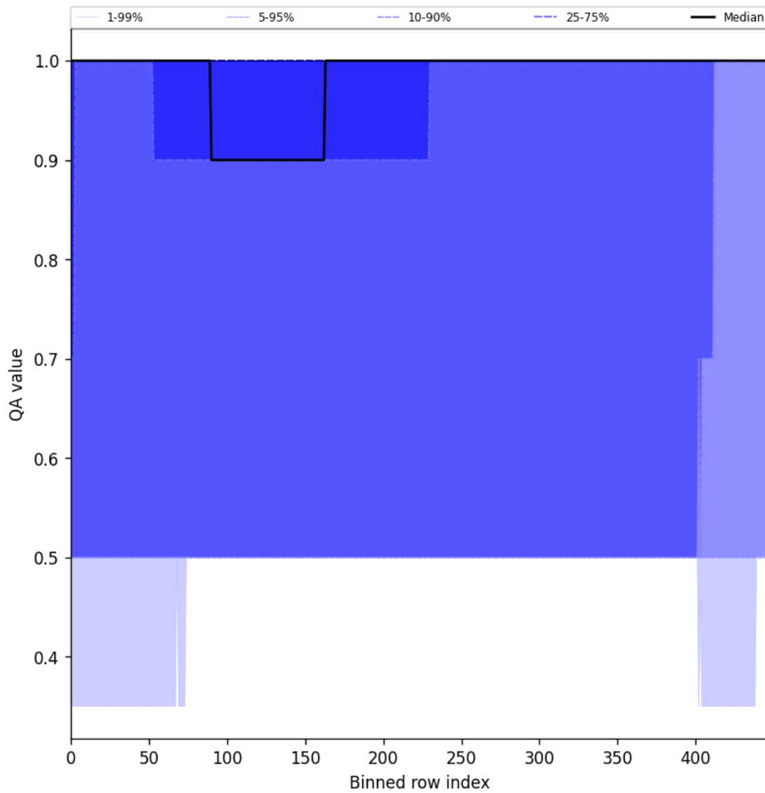
Figure 46: Along track statistics of “QA value” for 2024-11-23 to 2024-11-25
