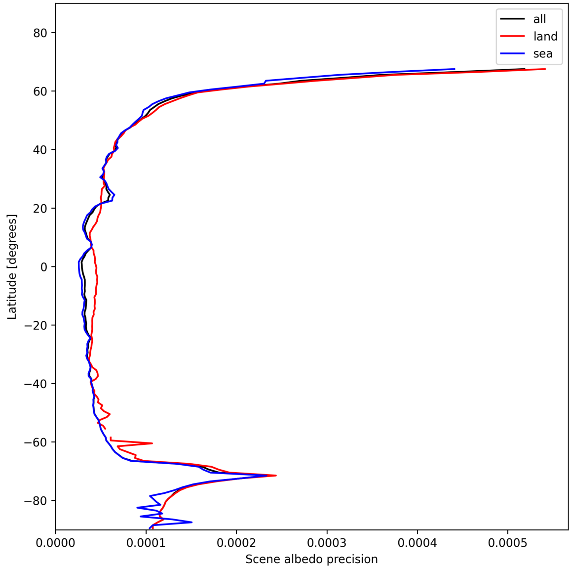
Figure 18: Zonal average of “Scene albedo precision” for 2024-11-23 to 2024-11-25.
