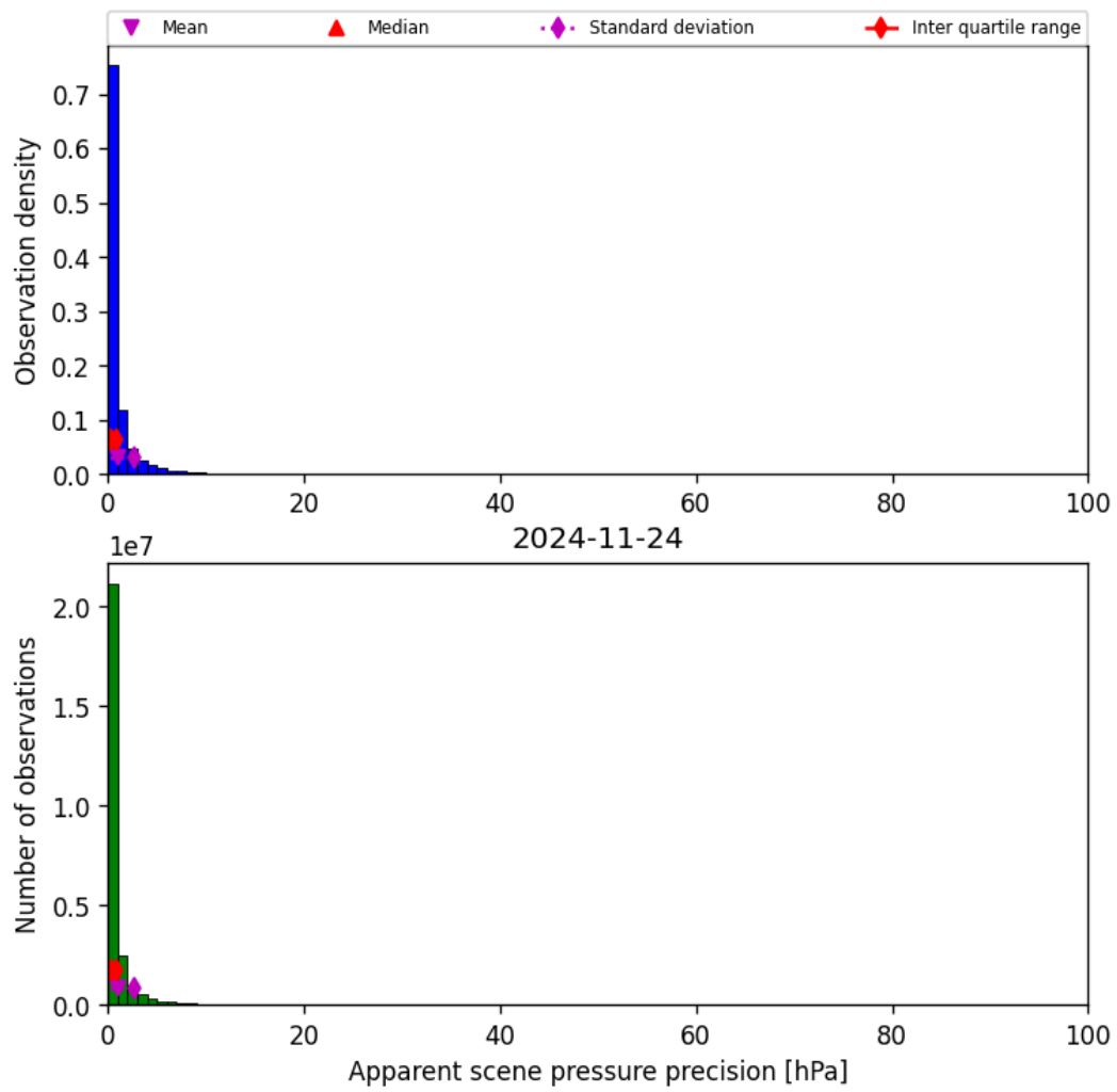
Figure 37: Histogram of “Apparent scene pressure precision” for 2024-11-23 to 2024-11-25
