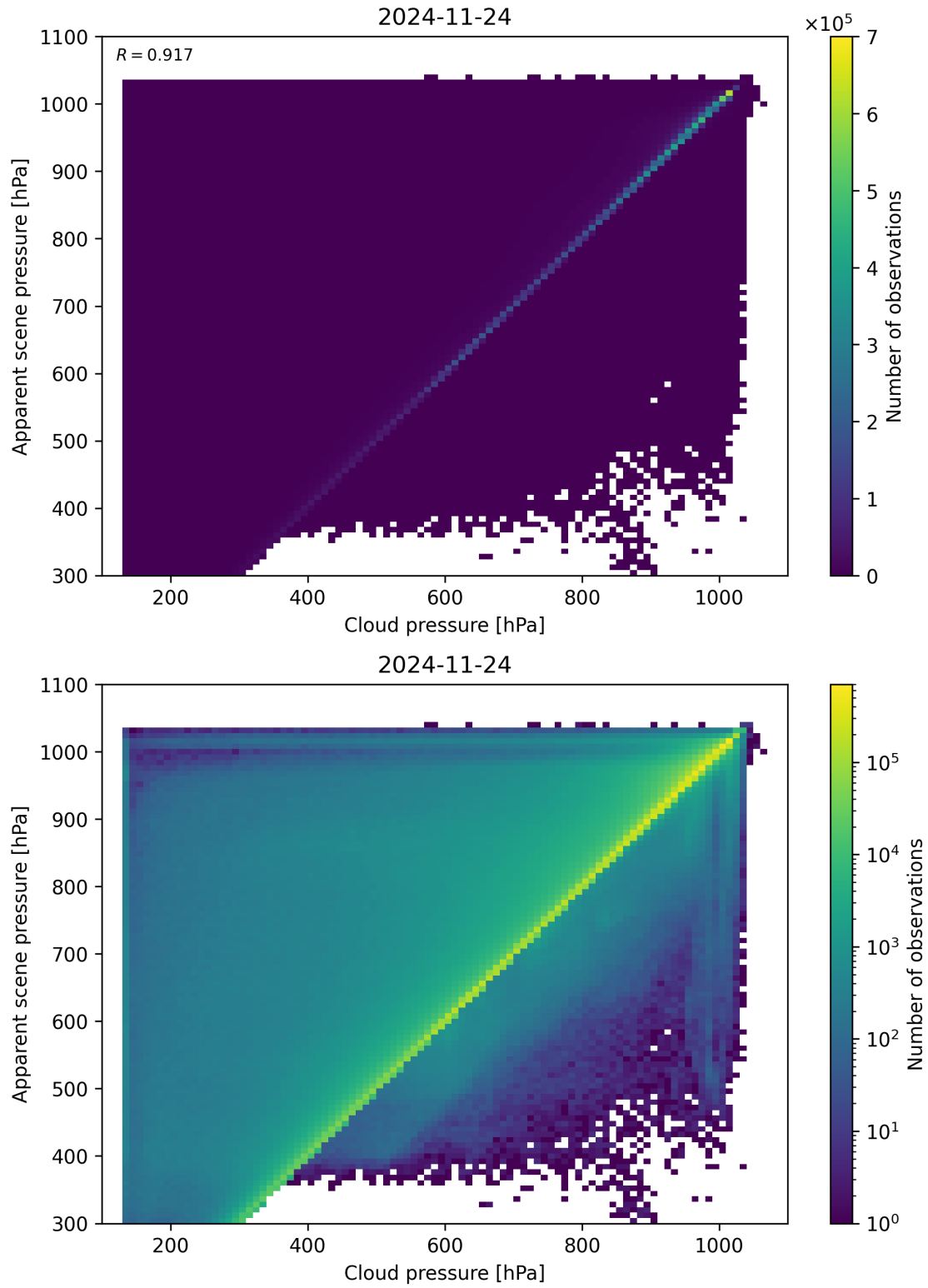
Figure 77: Scatter density plot of “Cloud pressure” against “Apparent scene pressure” for 2024-11-23 to 2024-11-25.
