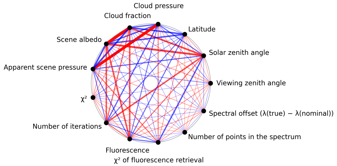
Figure 1: Map of correlation graph for 2024-11-23 to 2024-11-25.
