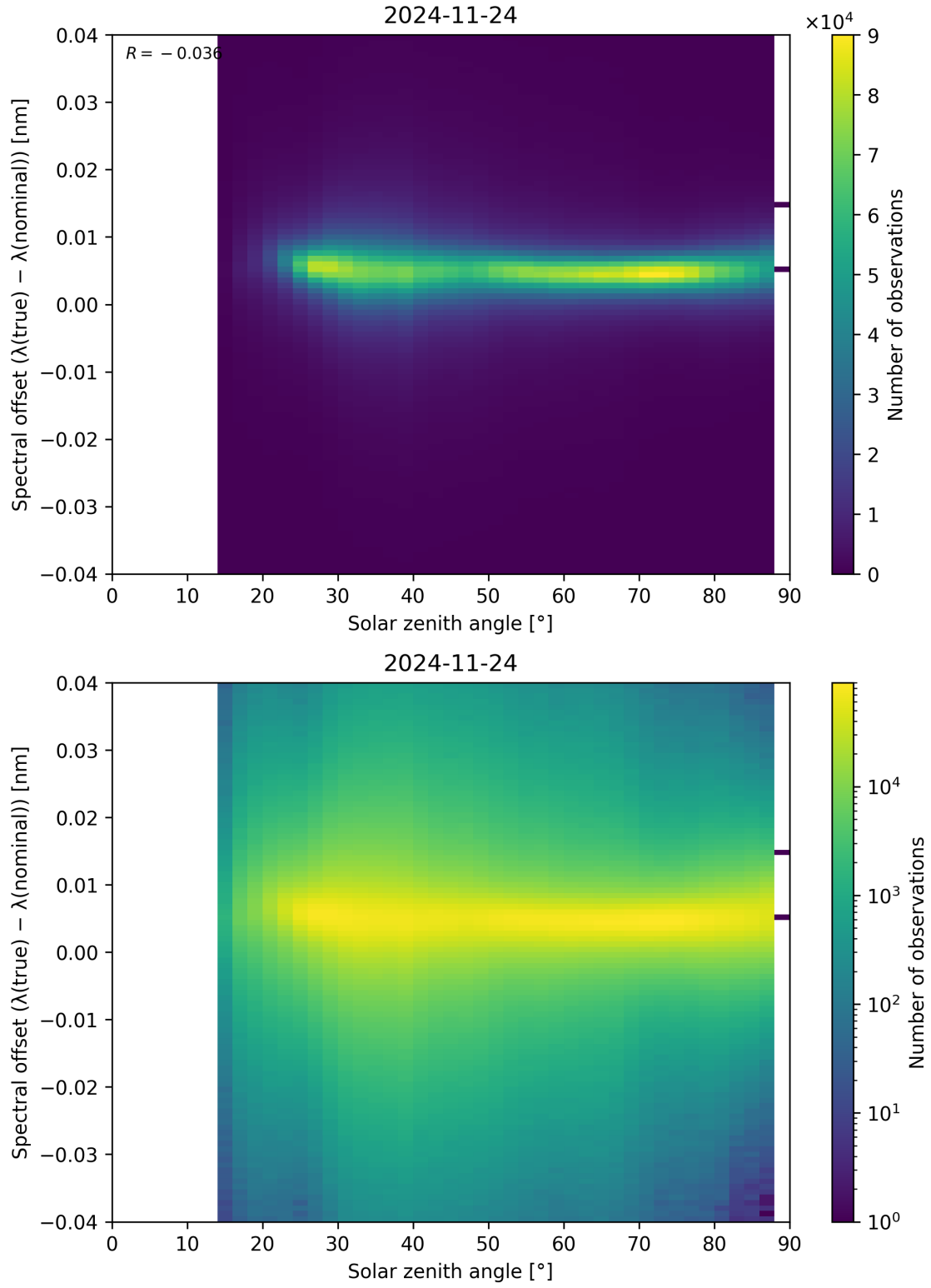
Figure 117: Scatter density plot of “Solar zenith angle” against “Spectral offset ( \lambda_{\text{true}} - \lambda_{\text{nominal}} )” for 2024-11-23 to 2024-11-25.
