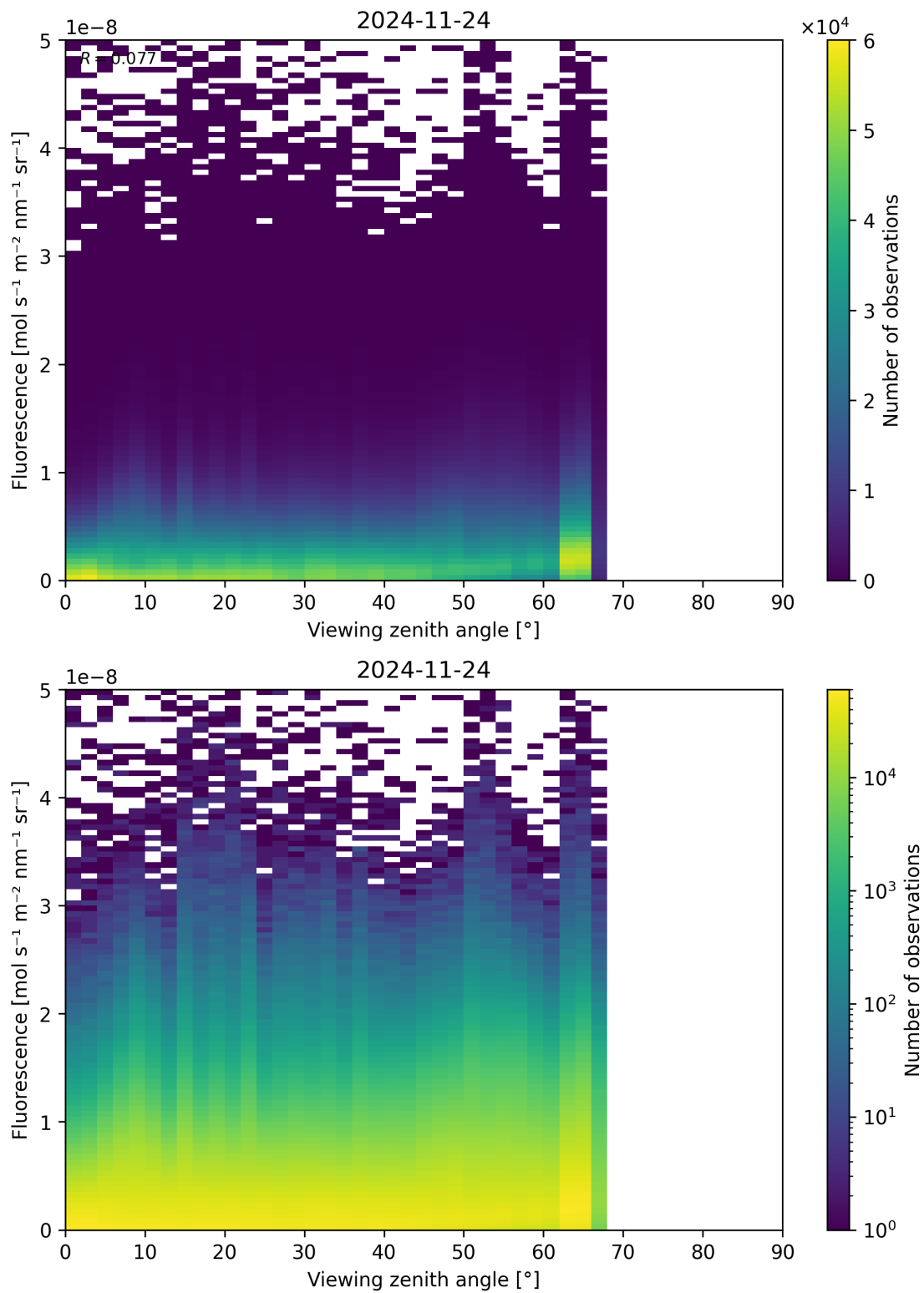
Figure 122: Scatter density plot of “Viewing zenith angle” against “Fluorescence” for 2024-11-23 to 2024-11-25.
