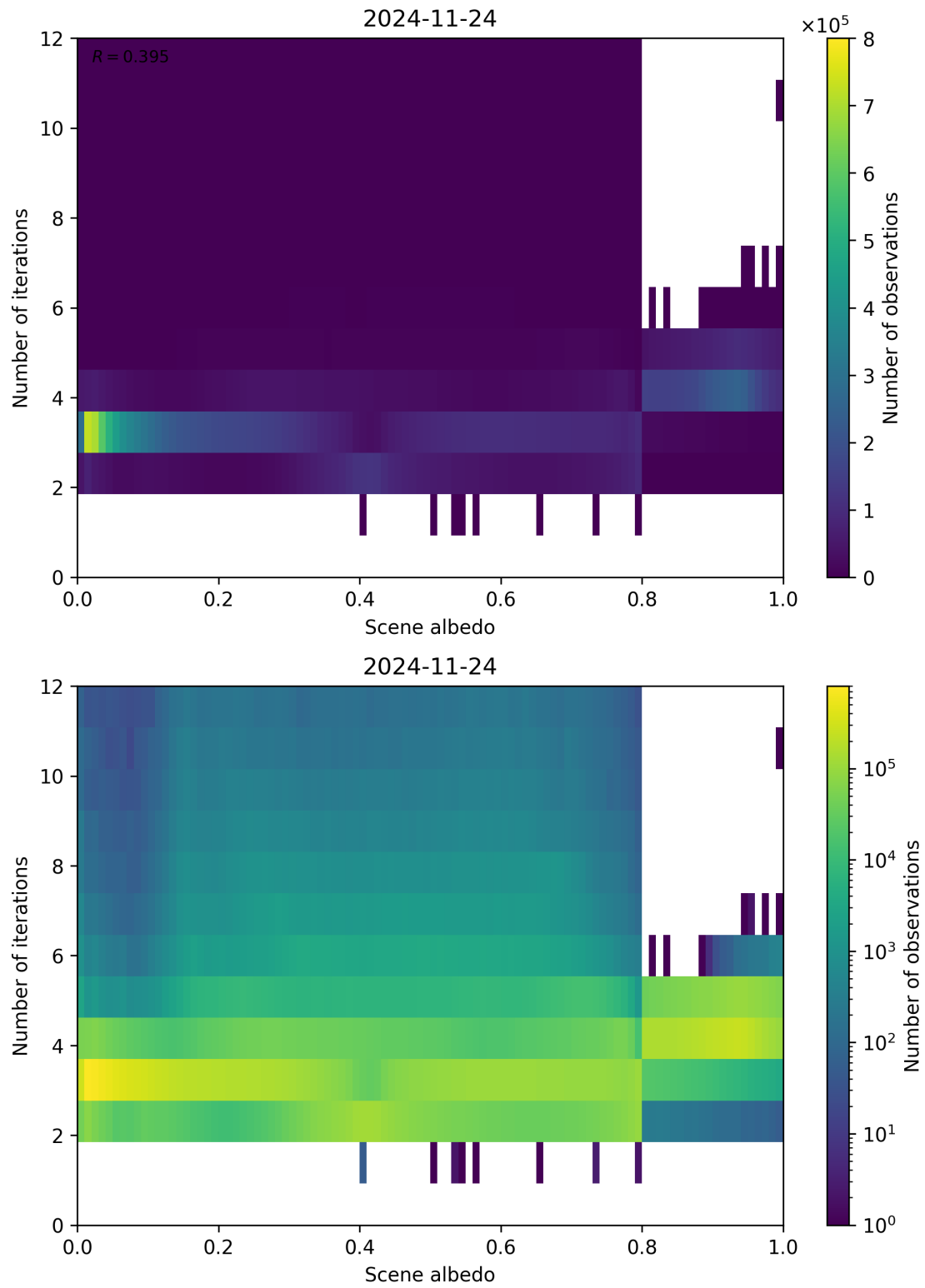
Figure 105: Scatter density plot of “Scene albedo” against “Number of iterations” for 2024-11-23 to 2024-11-25.
