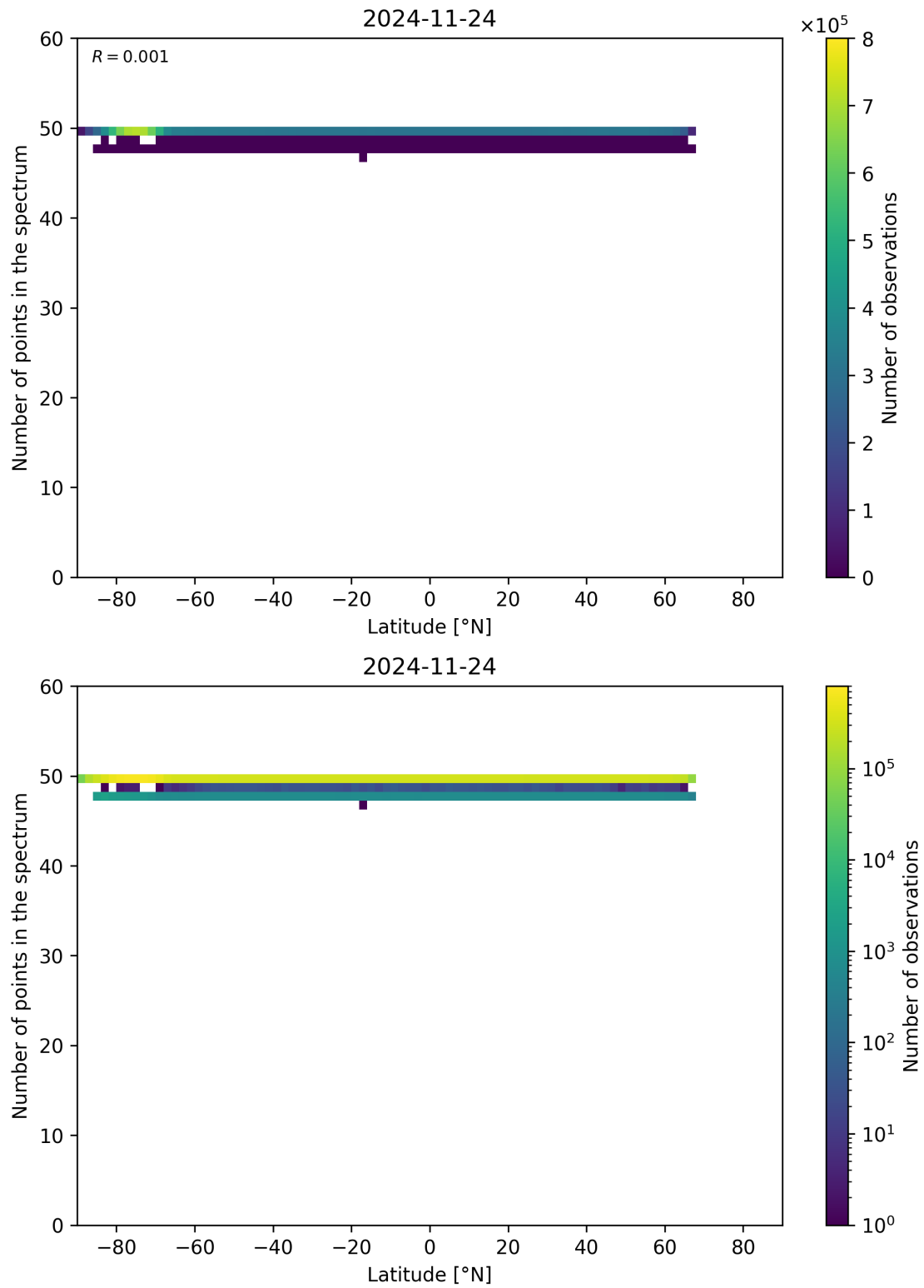
Figure 94: Scatter density plot of “Latitude” against “Number of points in the spectrum” for 2024-11-23 to 2024-11-25.
