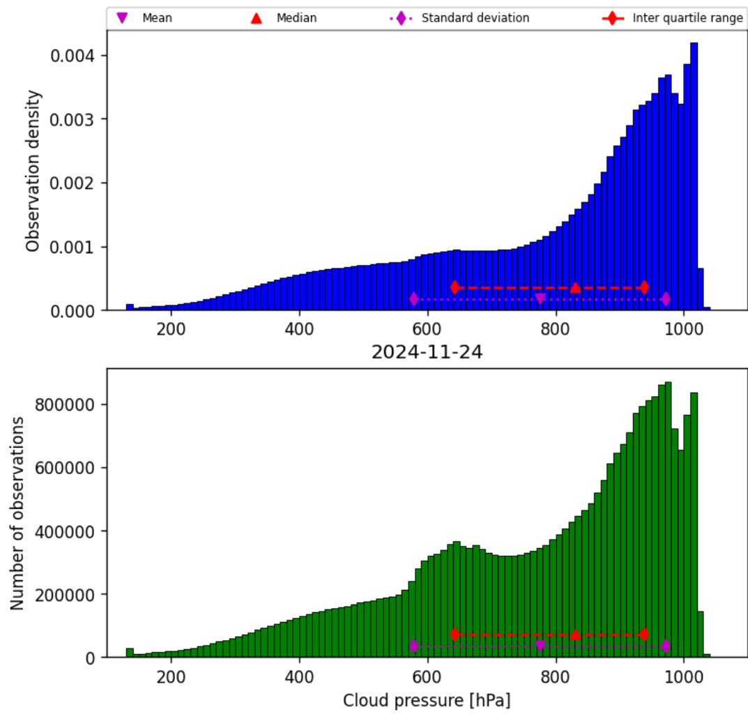
Figure 30: Histogram of “Cloud pressure” for 2024-11-23 to 2024-11-25
