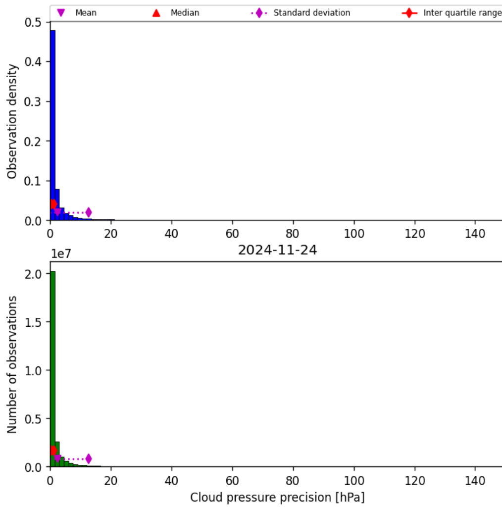
Figure 31: Histogram of “Cloud pressure precision” for 2024-11-23 to 2024-11-25
