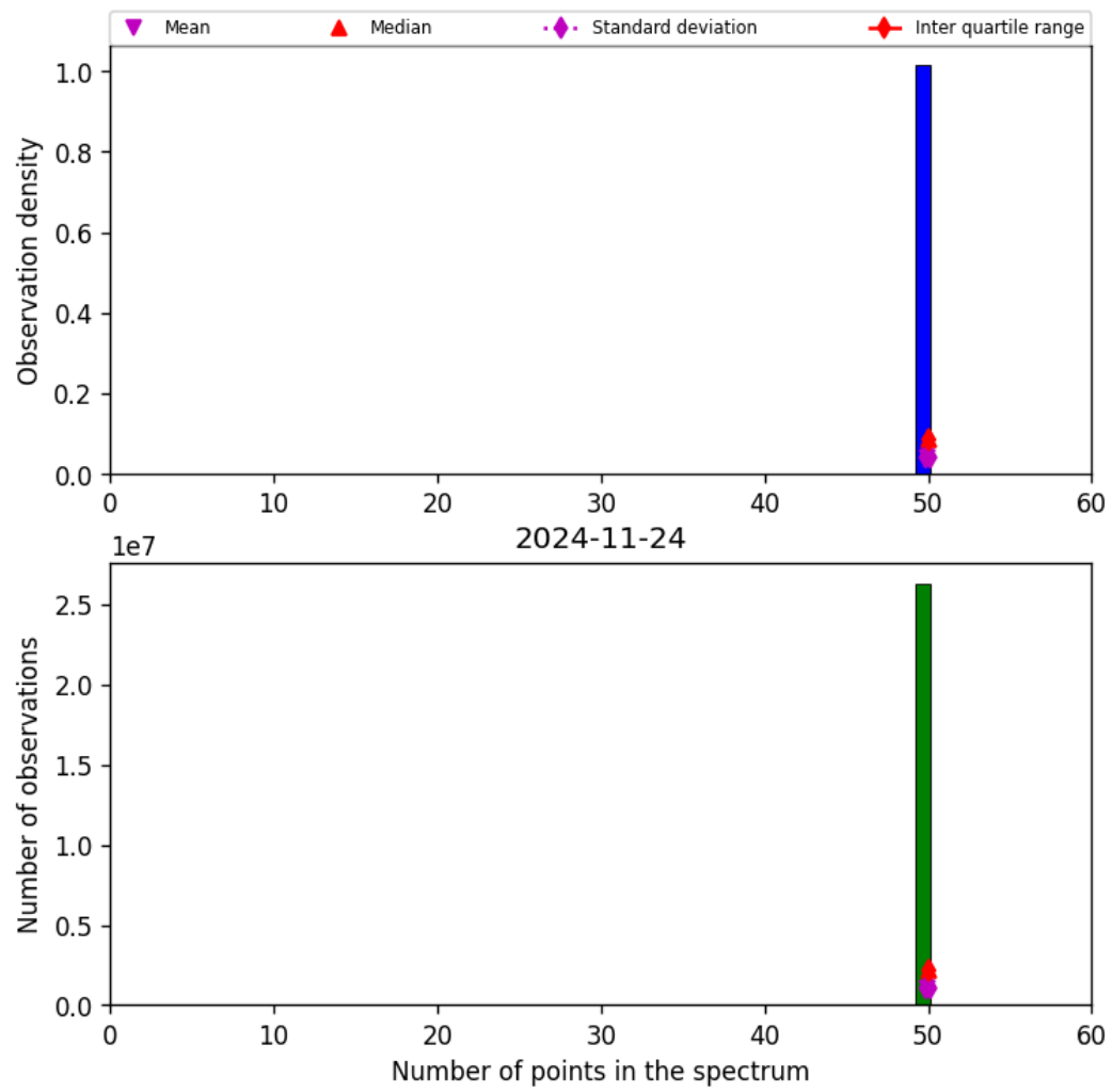
Figure 44: Histogram of "Number of points in the spectrum" for 2024-11-23 to 2024-11-25
