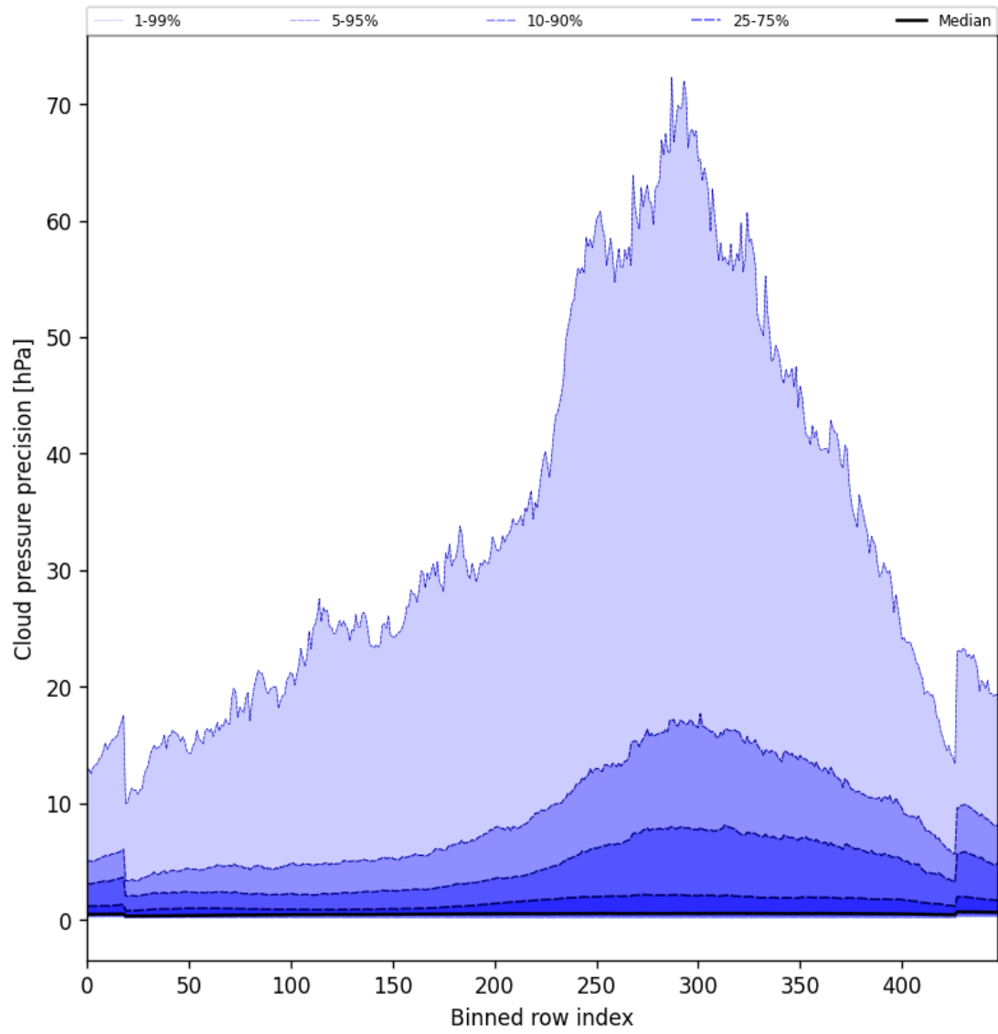
Figure 48: Along track statistics of “Cloud pressure precision” for 2024-11-23 to 2024-11-25
