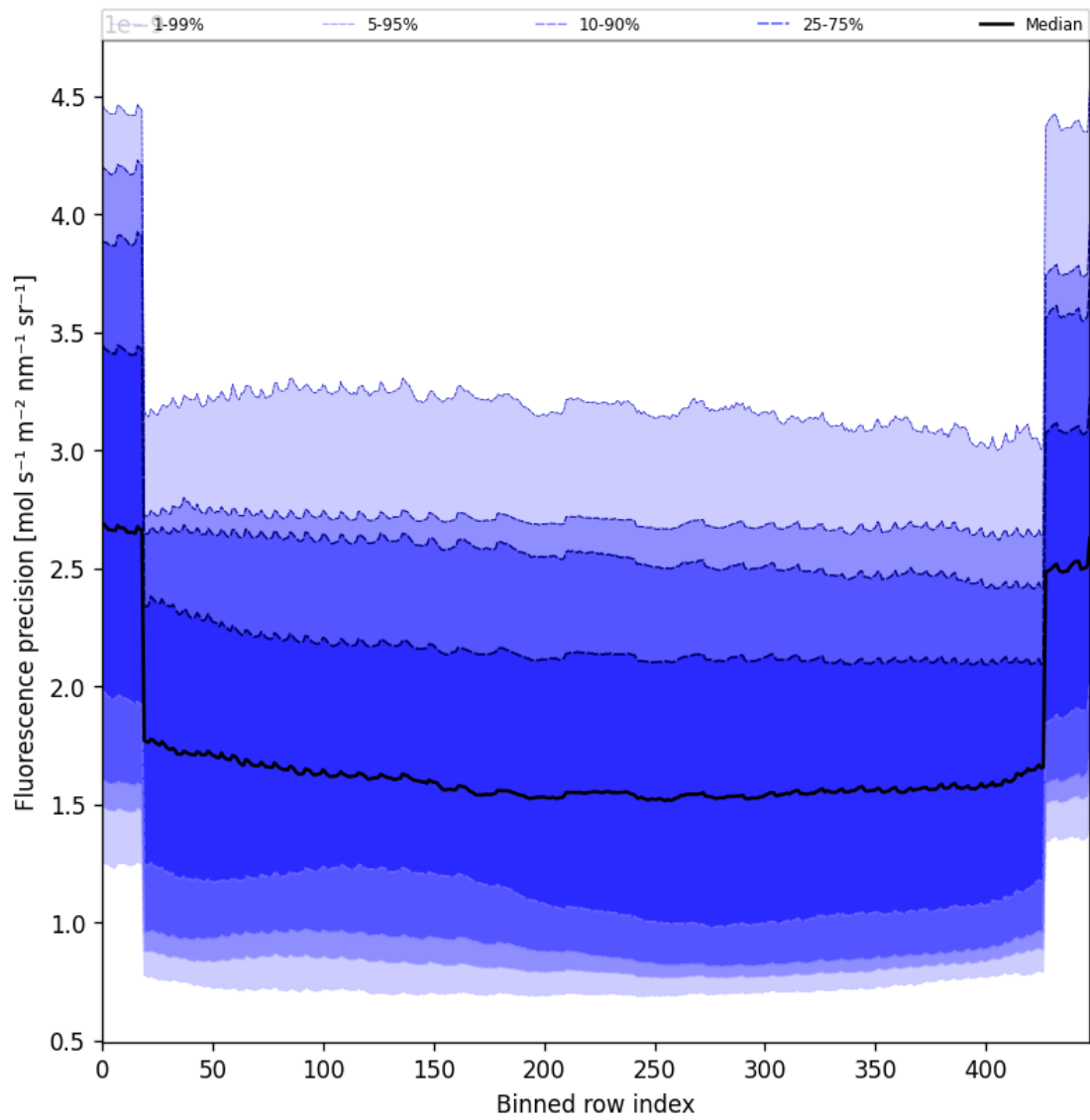
Figure 58: Along track statistics of “Fluorescence precision” for 2024-11-23 to 2024-11-25
