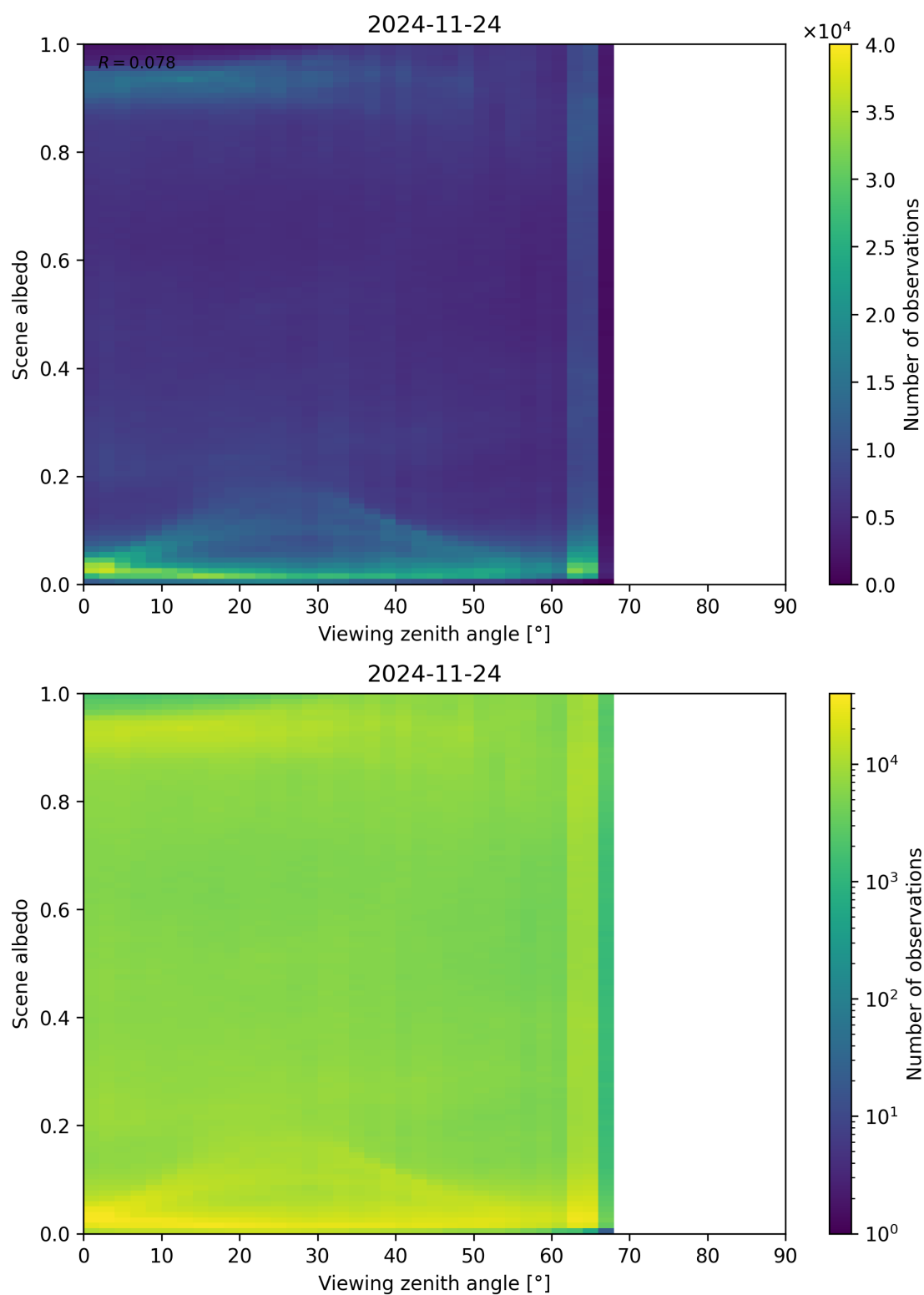
Figure 126: Scatter density plot of “Viewing zenith angle” against “Scene albedo” for 2024-11-23 to 2024-11-25.
