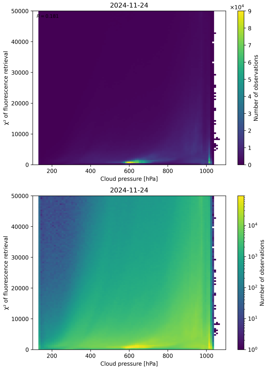
Figure 78: Scatter density plot of “Cloud pressure” against “ \chi^2 of fluorescence retrieval” for 2024-11-23 to 2024-11-25.
