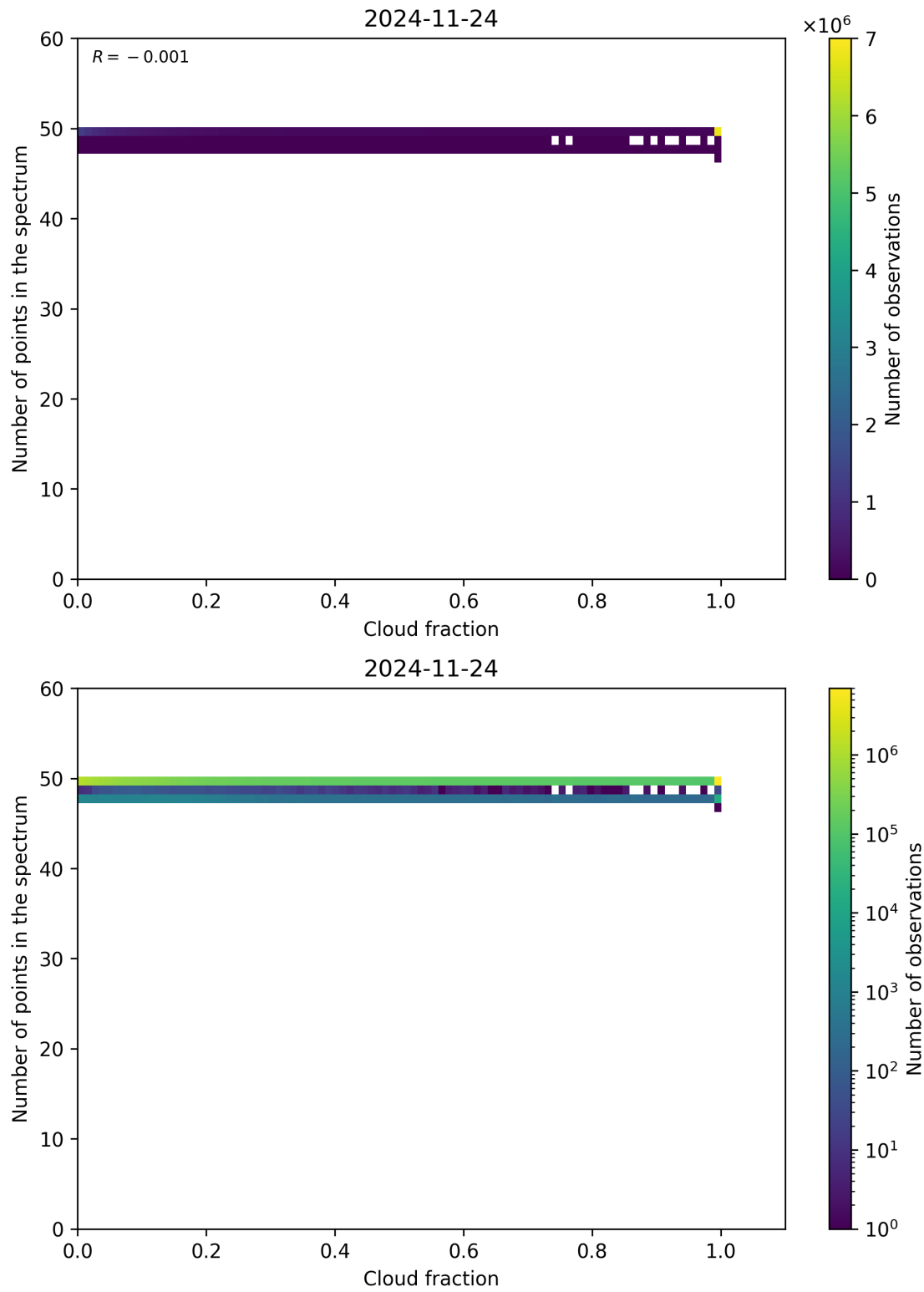
Figure 74: Scatter density plot of “Cloud fraction” against “Number of points in the spectrum” for 2024-11-23 to 2024-11-25.
