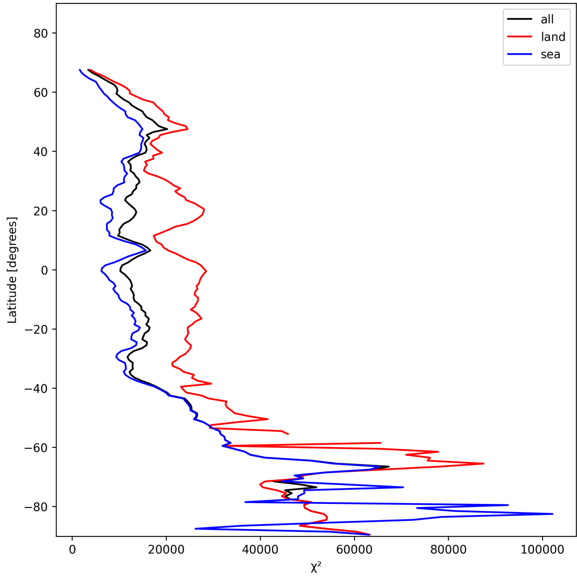
Figure 21: Zonal average of “ \chi^2 ” for 2024-11-23 to 2024-11-25.
