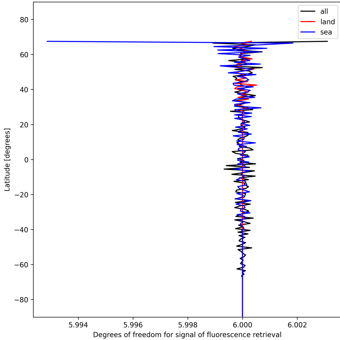
Figure 26: Zonal average of “Degrees of freedom for signal of fluorescence retrieval” for 2024-11-23 to 2024-11-25.
