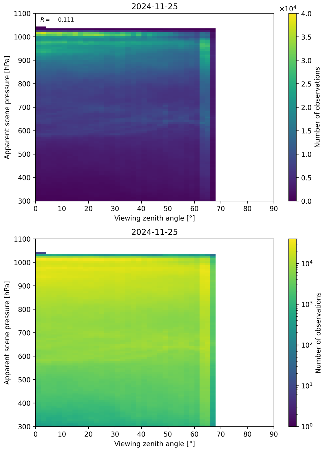
Figure 118: Scatter density plot of “Viewing zenith angle” against “Apparent scene pressure” for 2024-11-25 to 2024-11-26.
