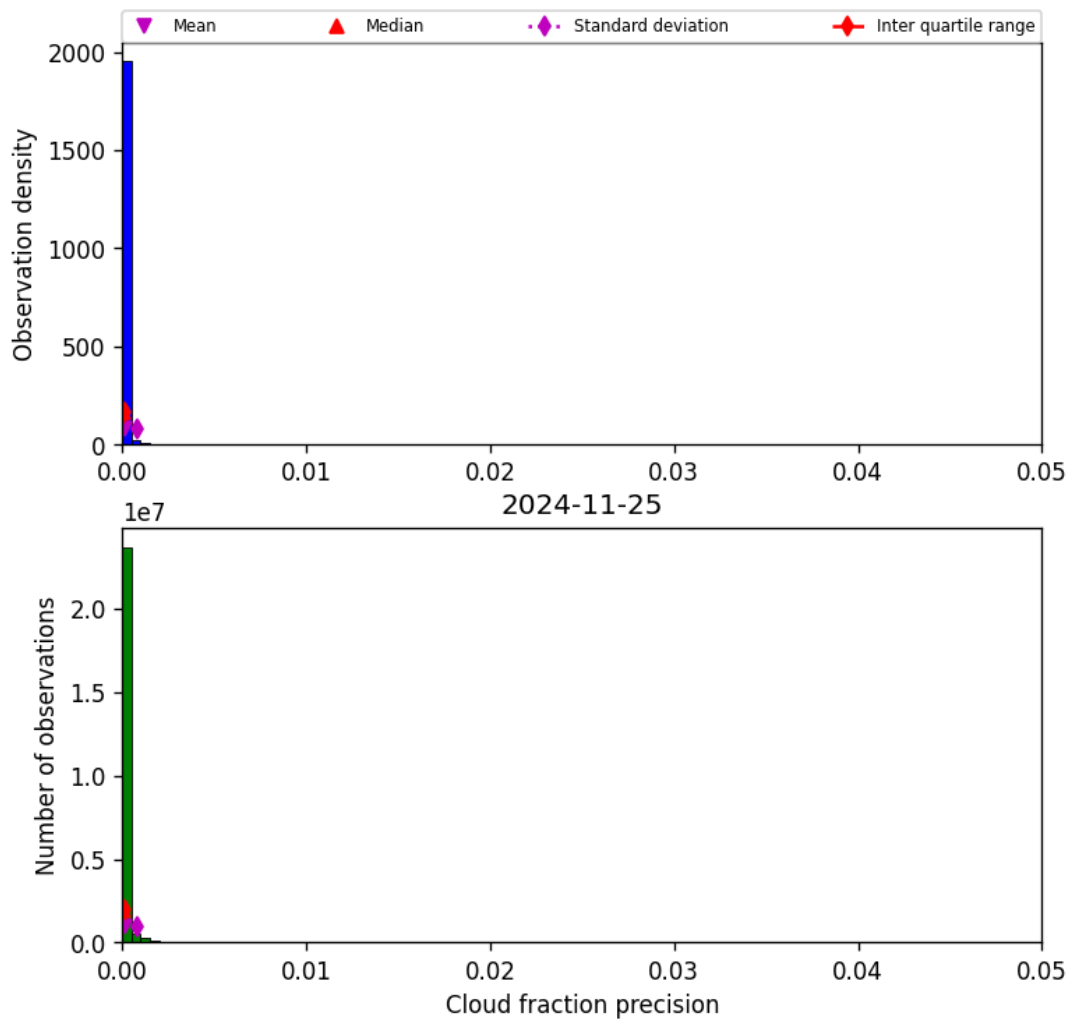
Figure 33: Histogram of “Cloud fraction precision” for 2024-11-25 to 2024-11-26
