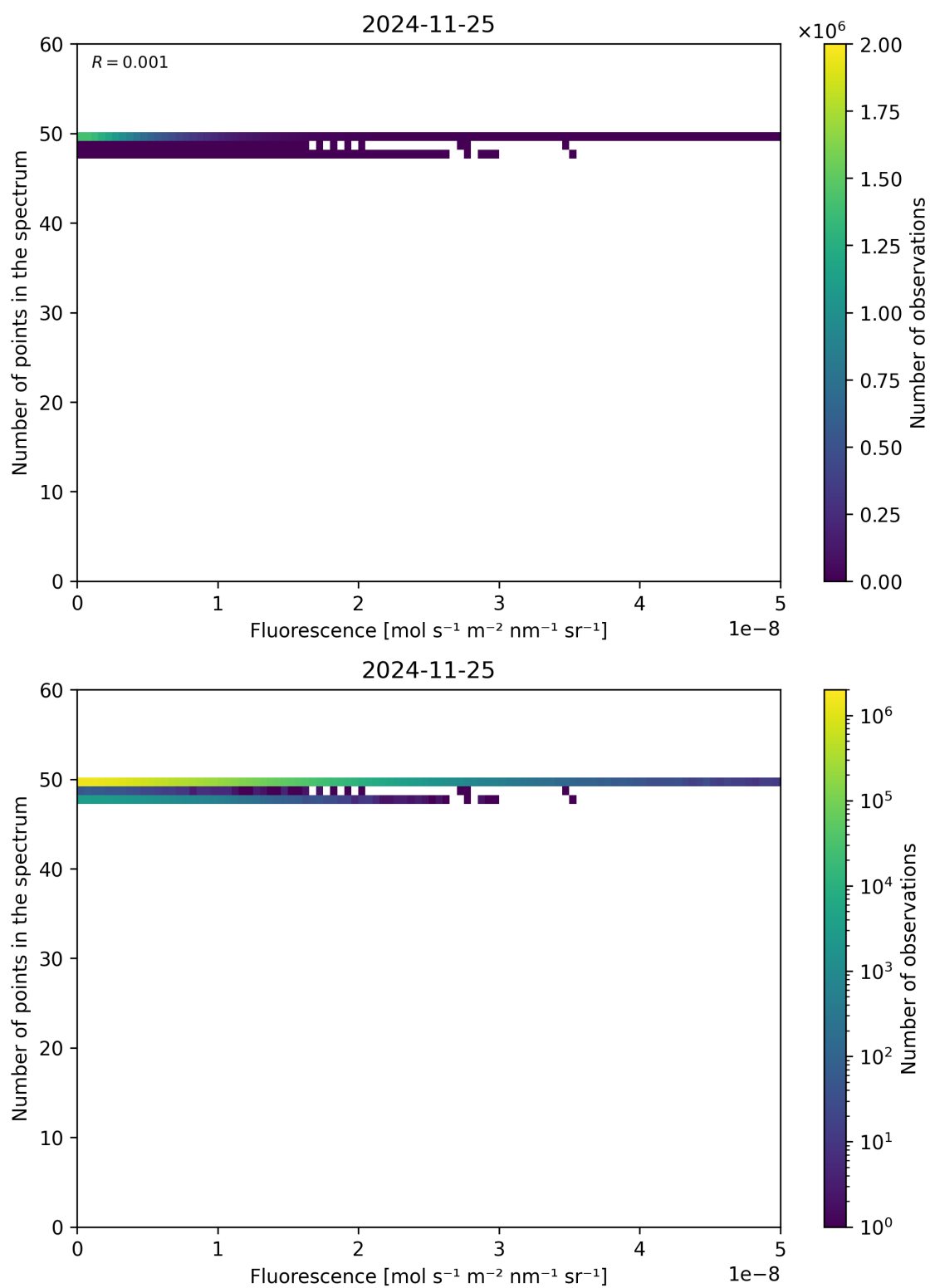
Figure 86: Scatter density plot of “Fluorescence” against “Number of points in the spectrum” for 2024-11-25 to 2024-11-26.
