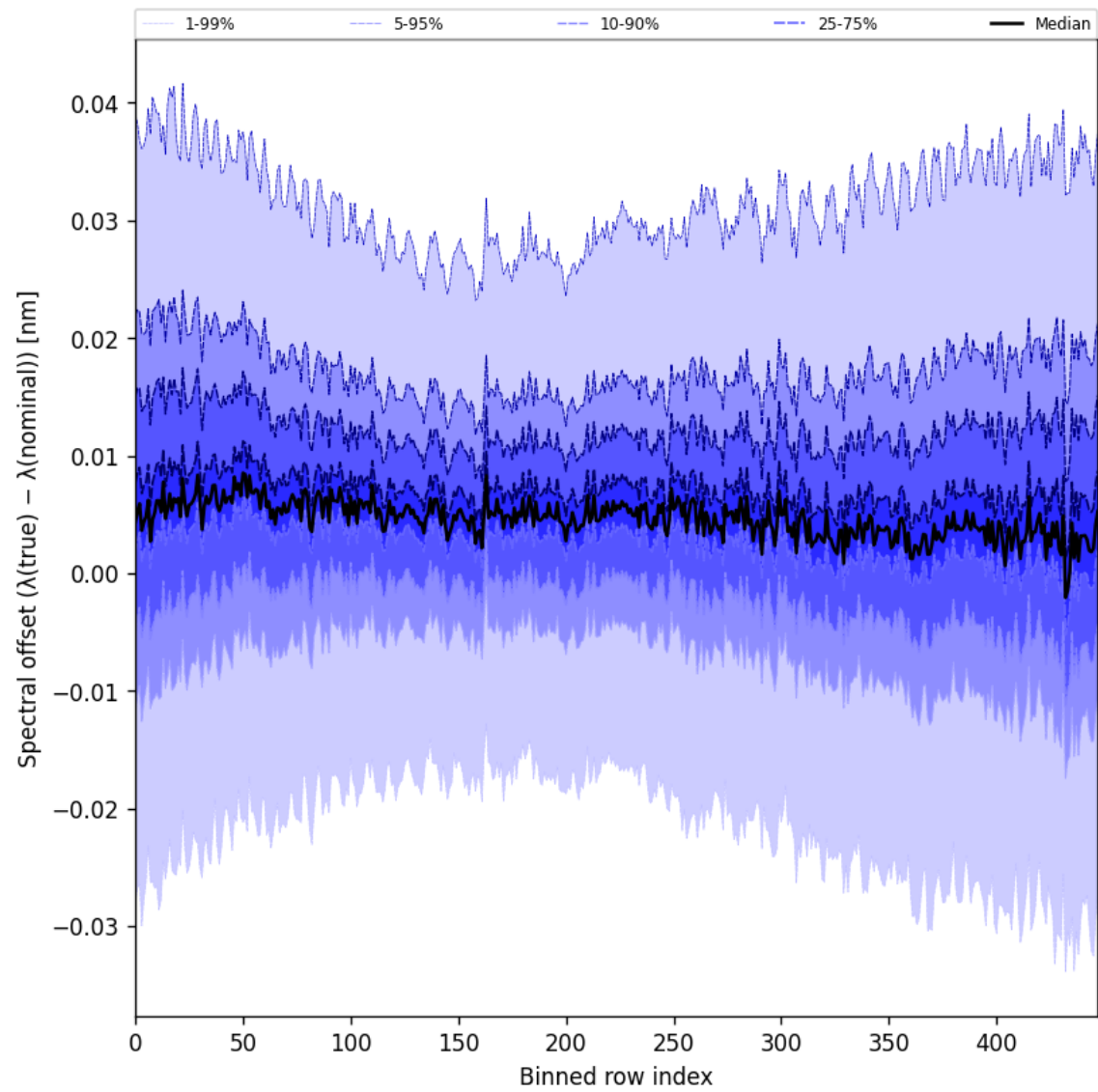
Figure 62: Along track statistics of “Spectral offset ( \lambda_{\text{true}} - \lambda_{\text{nominal}} )” for 2024-11-25 to 2024-11-26
