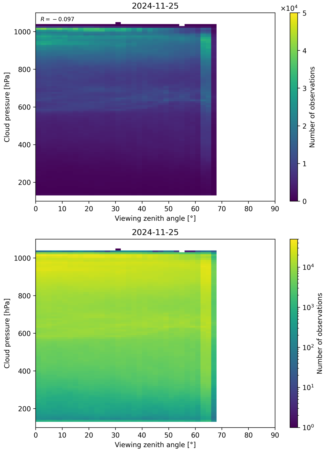
Figure 121: Scatter density plot of “Viewing zenith angle” against “Cloud pressure” for 2024-11-25 to 2024-11-26.
