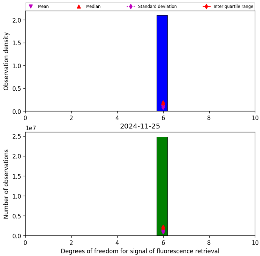
Figure 43: Histogram of “Degrees of freedom for signal of fluorescence retrieval” for 2024-11-25 to 2024-11-26
