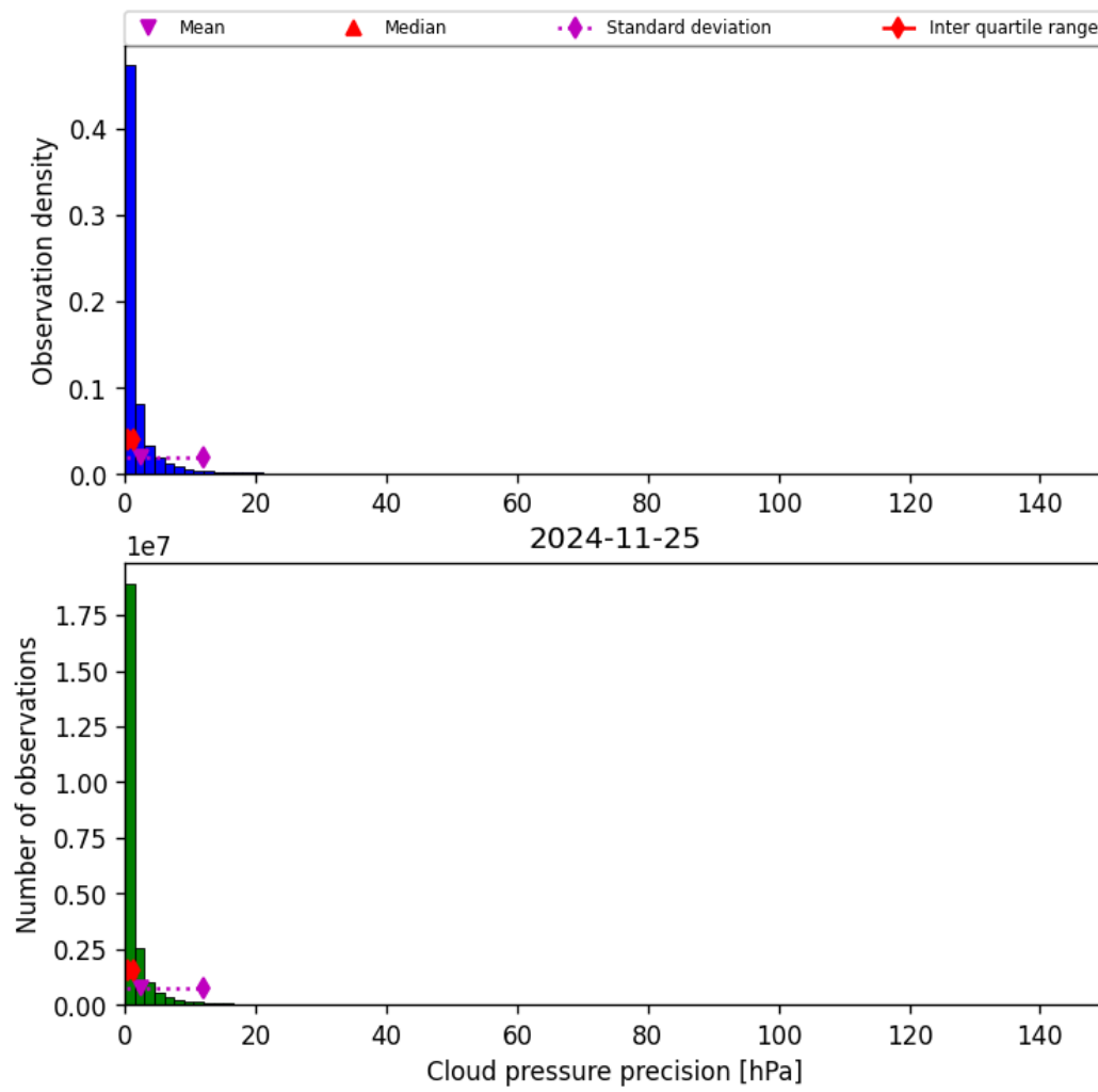
Figure 31: Histogram of “Cloud pressure precision” for 2024-11-25 to 2024-11-26
