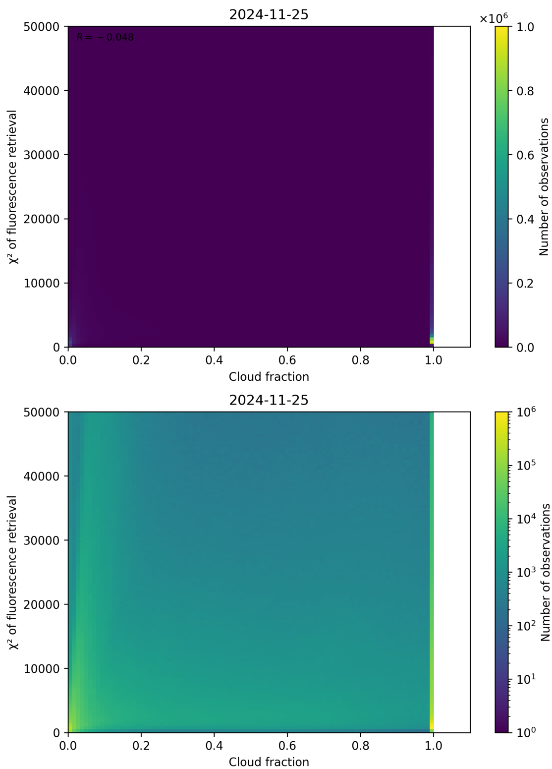
Figure 71: Scatter density plot of “Cloud fraction” against “ \chi^2 of fluorescence retrieval” for 2024-11-25 to 2024-11-26.
