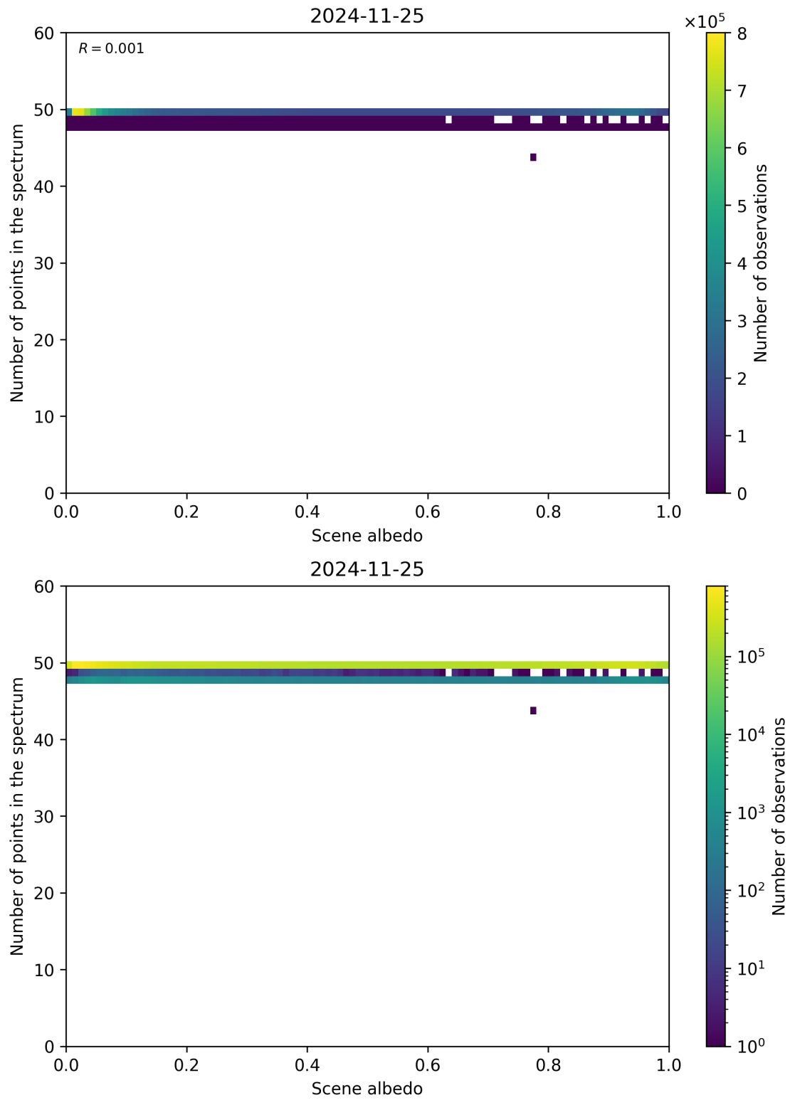
Figure 106: Scatter density plot of “Scene albedo” against “Number of points in the spectrum” for 2024-11-25 to 2024-11-26.
