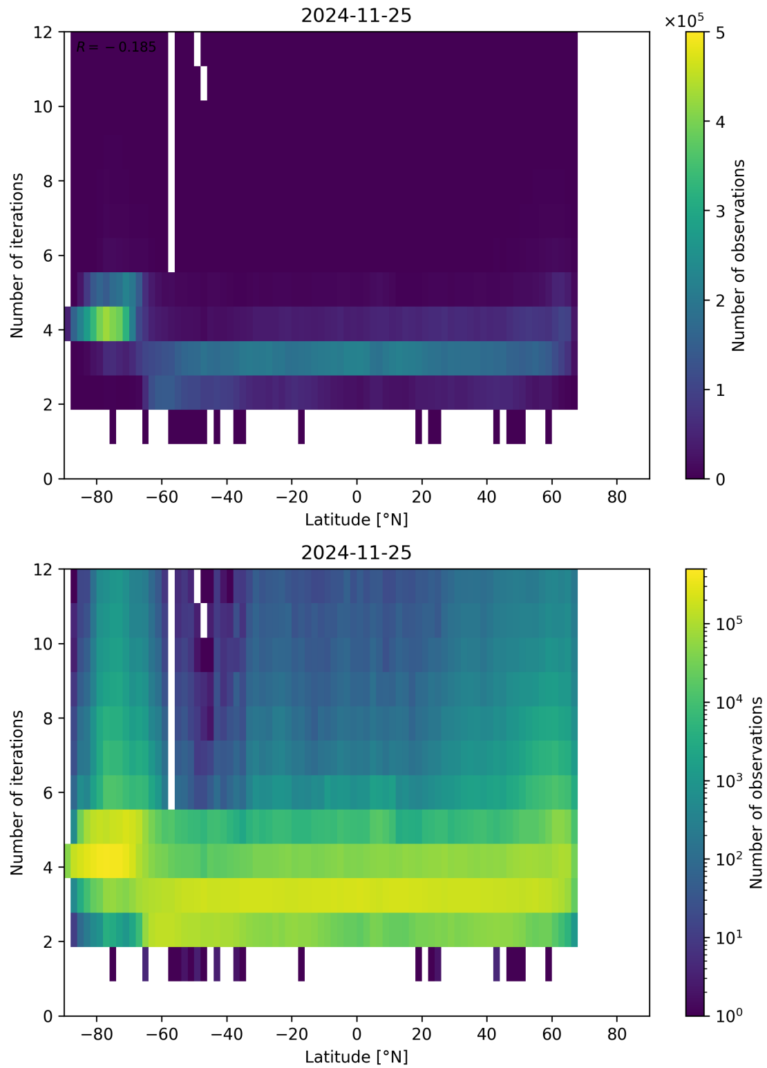
Figure 93: Scatter density plot of “Latitude” against “Number of iterations” for 2024-11-25 to 2024-11-26.
