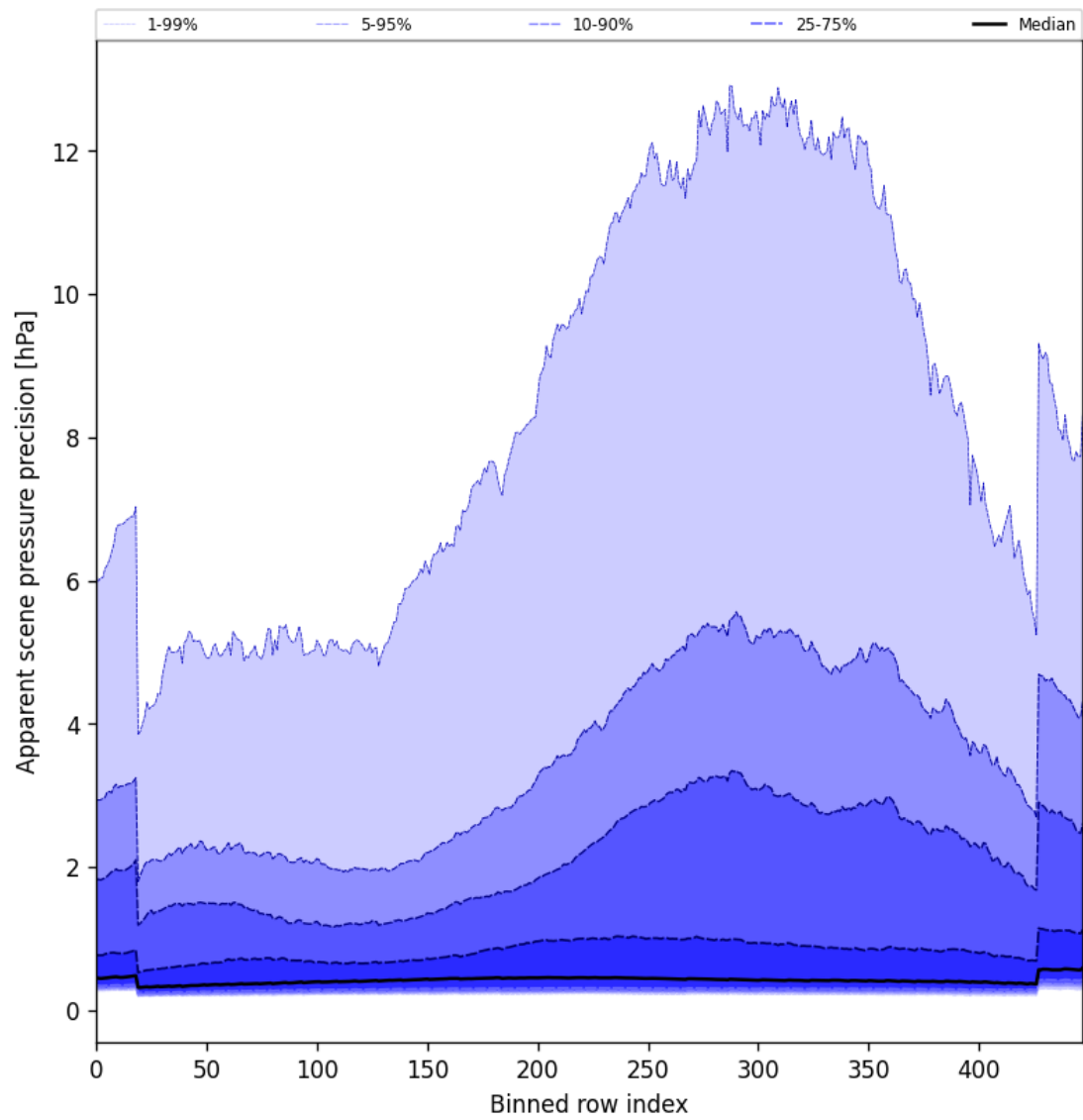
Figure 54: Along track statistics of “Apparent scene pressure precision” for 2024-11-25 to 2024-11-26
