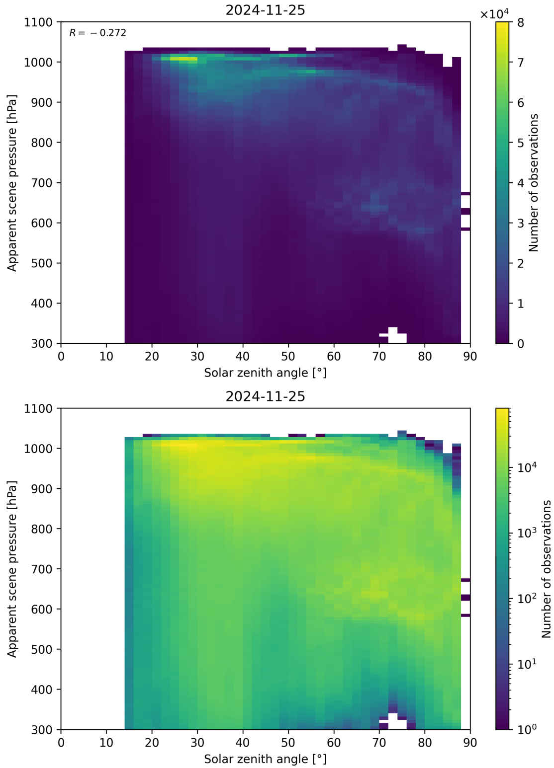
Figure 108: Scatter density plot of “Solar zenith angle” against “Apparent scene pressure” for 2024-11-25 to 2024-11-26.
