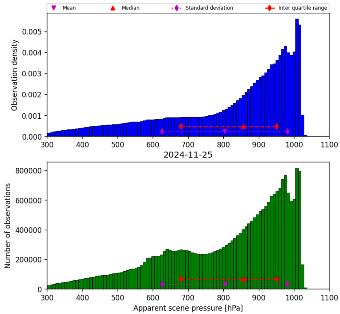
Figure 36: Histogram of “Apparent scene pressure” for 2024-11-25 to 2024-11-26
