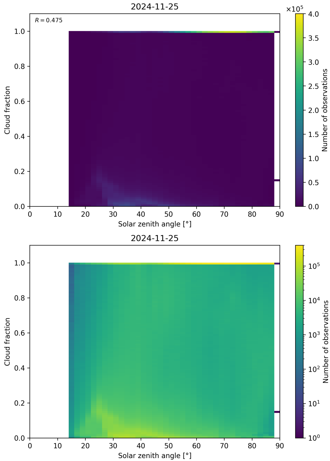
Figure 110: Scatter density plot of “Solar zenith angle” against “Cloud fraction” for 2024-11-25 to 2024-11-26.
