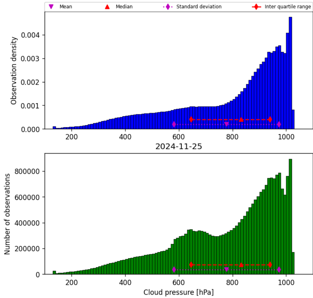
Figure 30: Histogram of “Cloud pressure” for 2024-11-25 to 2024-11-26
