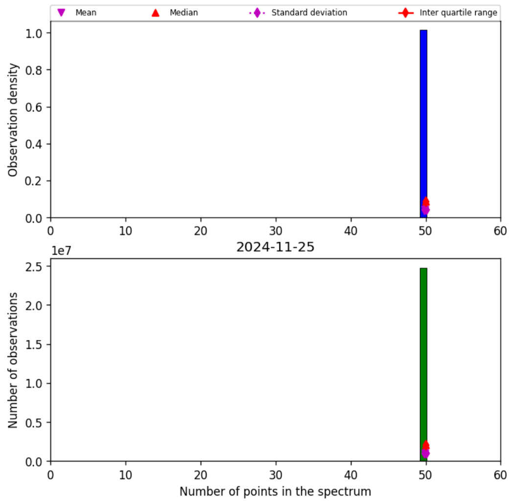
Figure 44: Histogram of "Number of points in the spectrum" for 2024-11-25 to 2024-11-26
