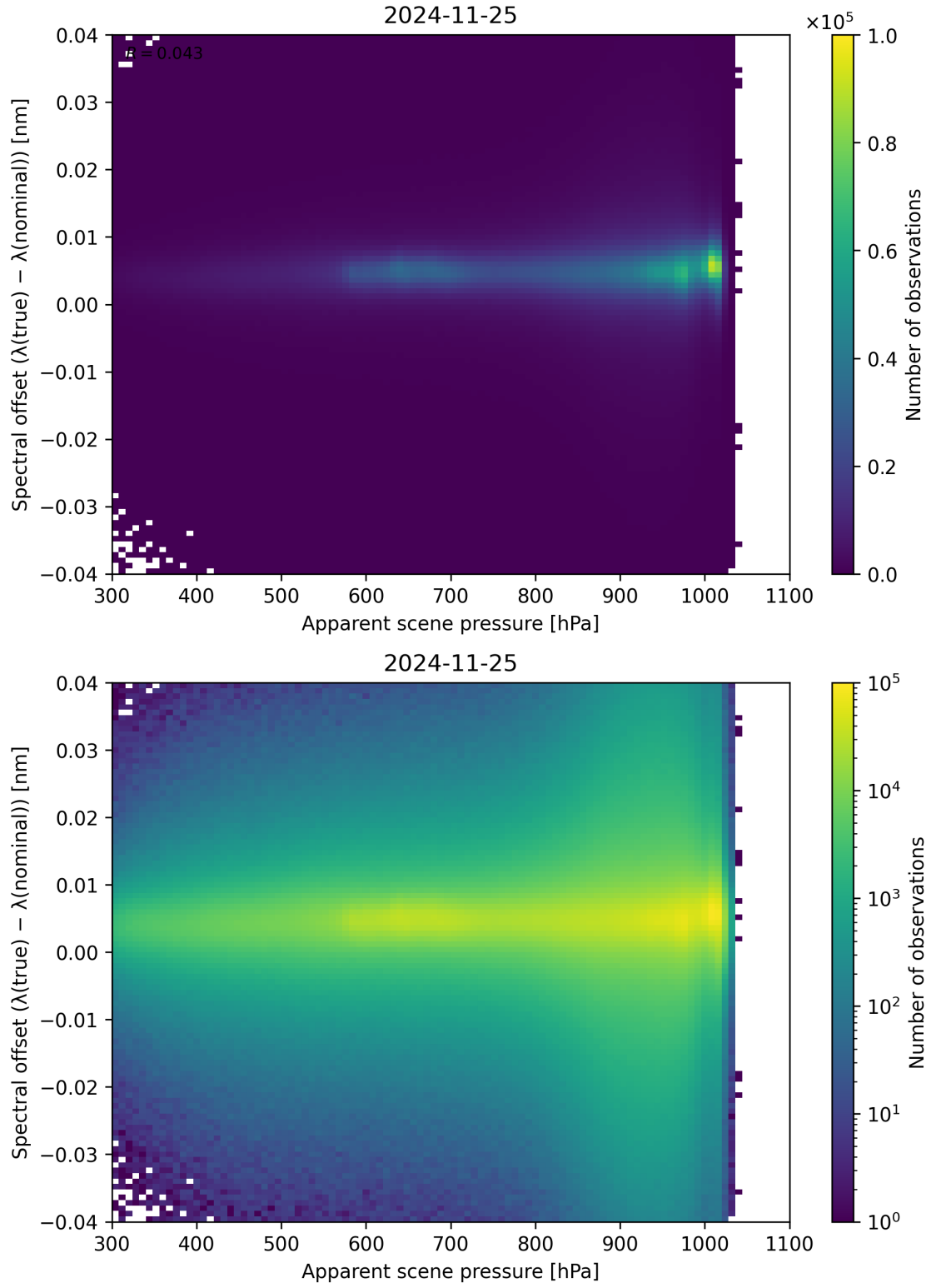
Figure 67: Scatter density plot of “Apparent scene pressure” against “Spectral offset ( \lambda_{\text{true}} - \lambda_{\text{nominal}} )” for 2024-11-25 to 2024-11-26.
