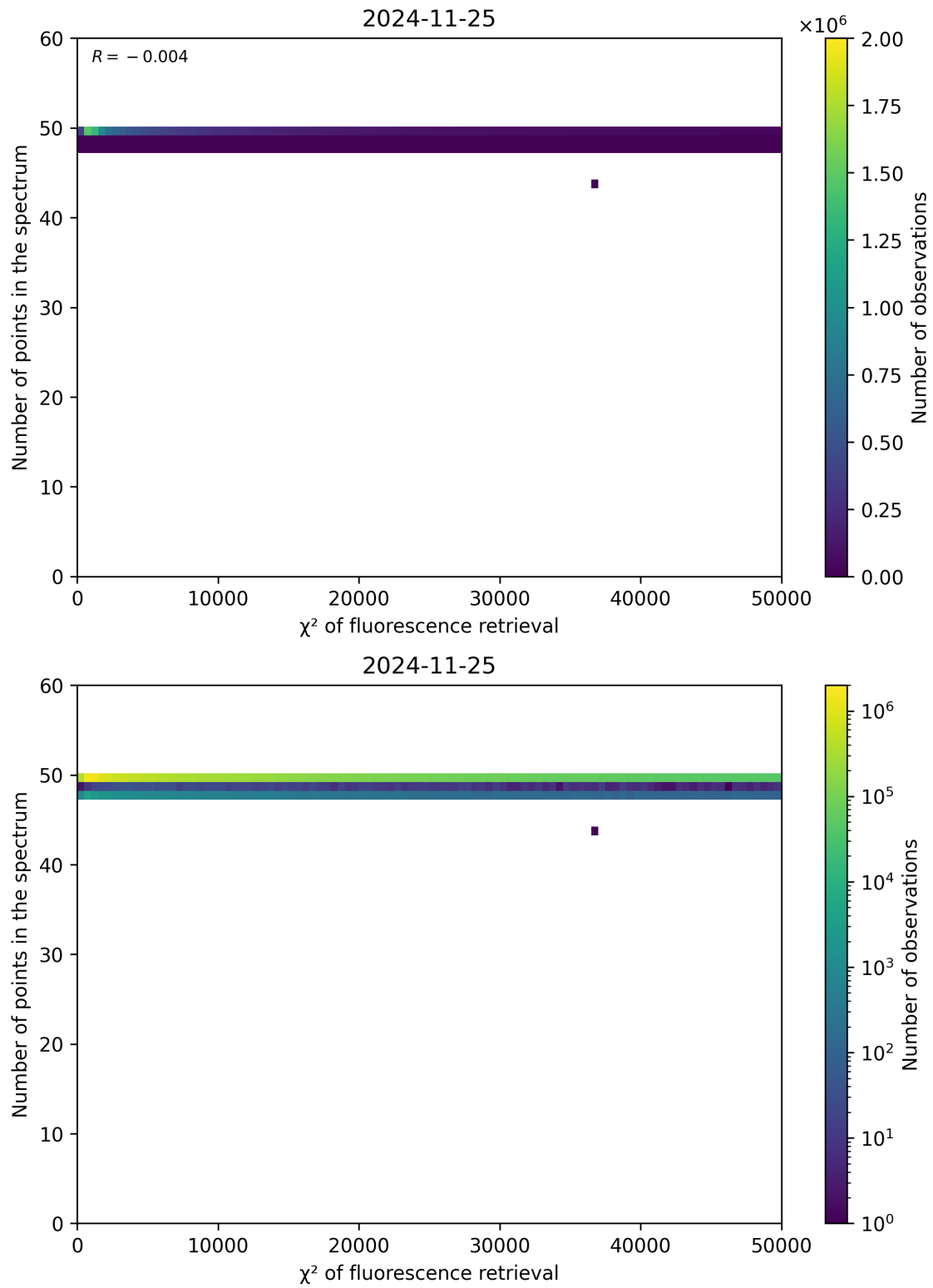
Figure 68: Scatter density plot of " \chi^2 of fluorescence retrieval" against "Number of points in the spectrum" for 2024-11-25 to 2024-11-26.
