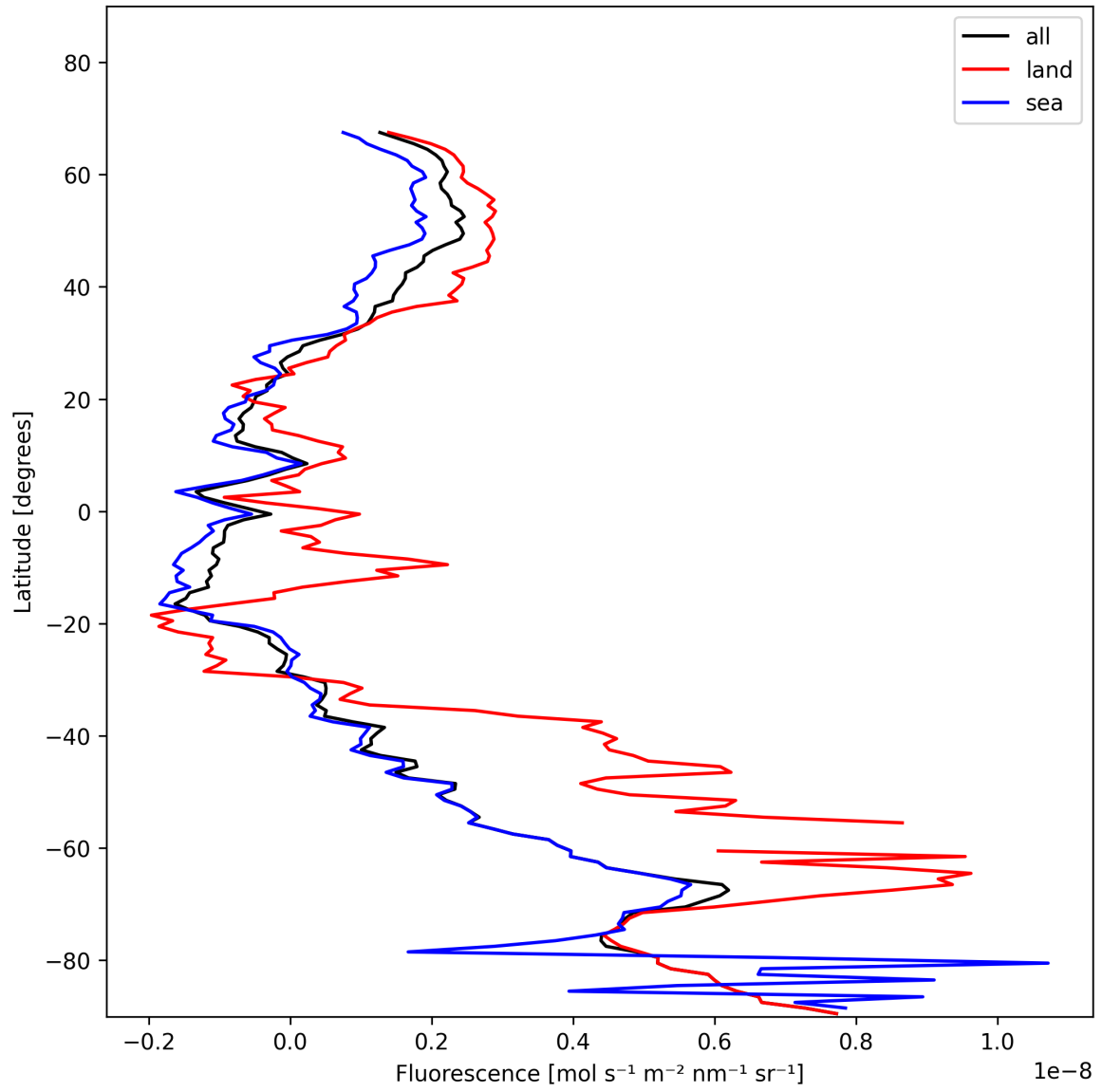
Figure 23: Zonal average of “Fluorescence” for 2024-11-25 to 2024-11-26.
