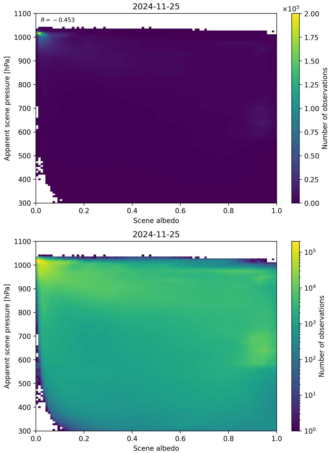
Figure 102: Scatter density plot of “Scene albedo” against “Apparent scene pressure” for 2024-11-25 to 2024-11-26.
