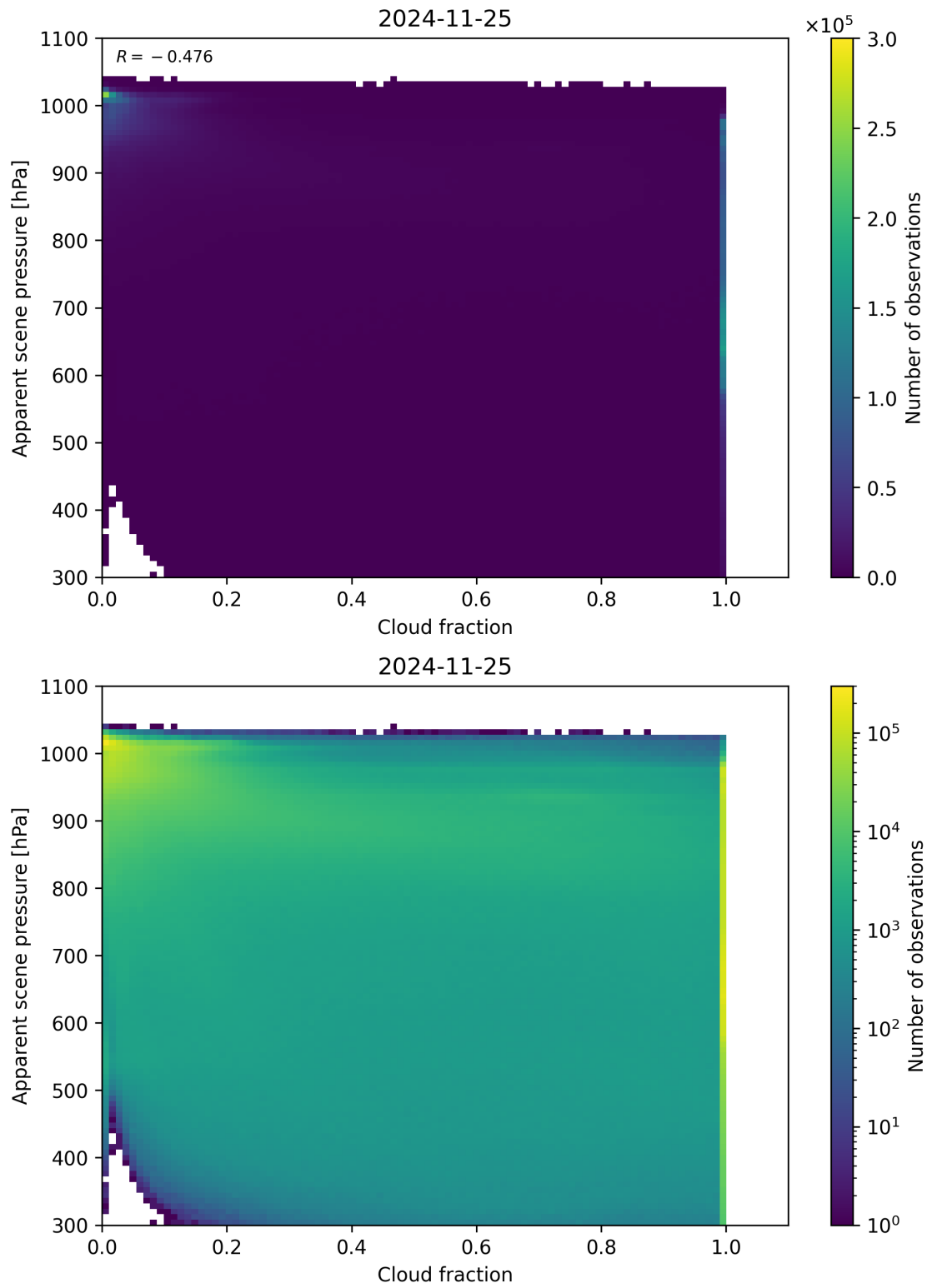
Figure 70: Scatter density plot of “Cloud fraction” against “Apparent scene pressure” for 2024-11-25 to 2024-11-26.
