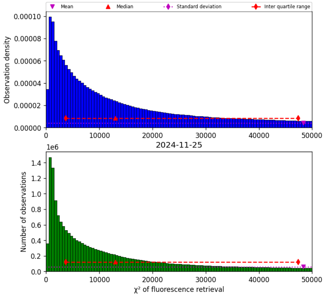
Figure 42: Histogram of “ \chi^2 of fluorescence retrieval” for 2024-11-25 to 2024-11-26
