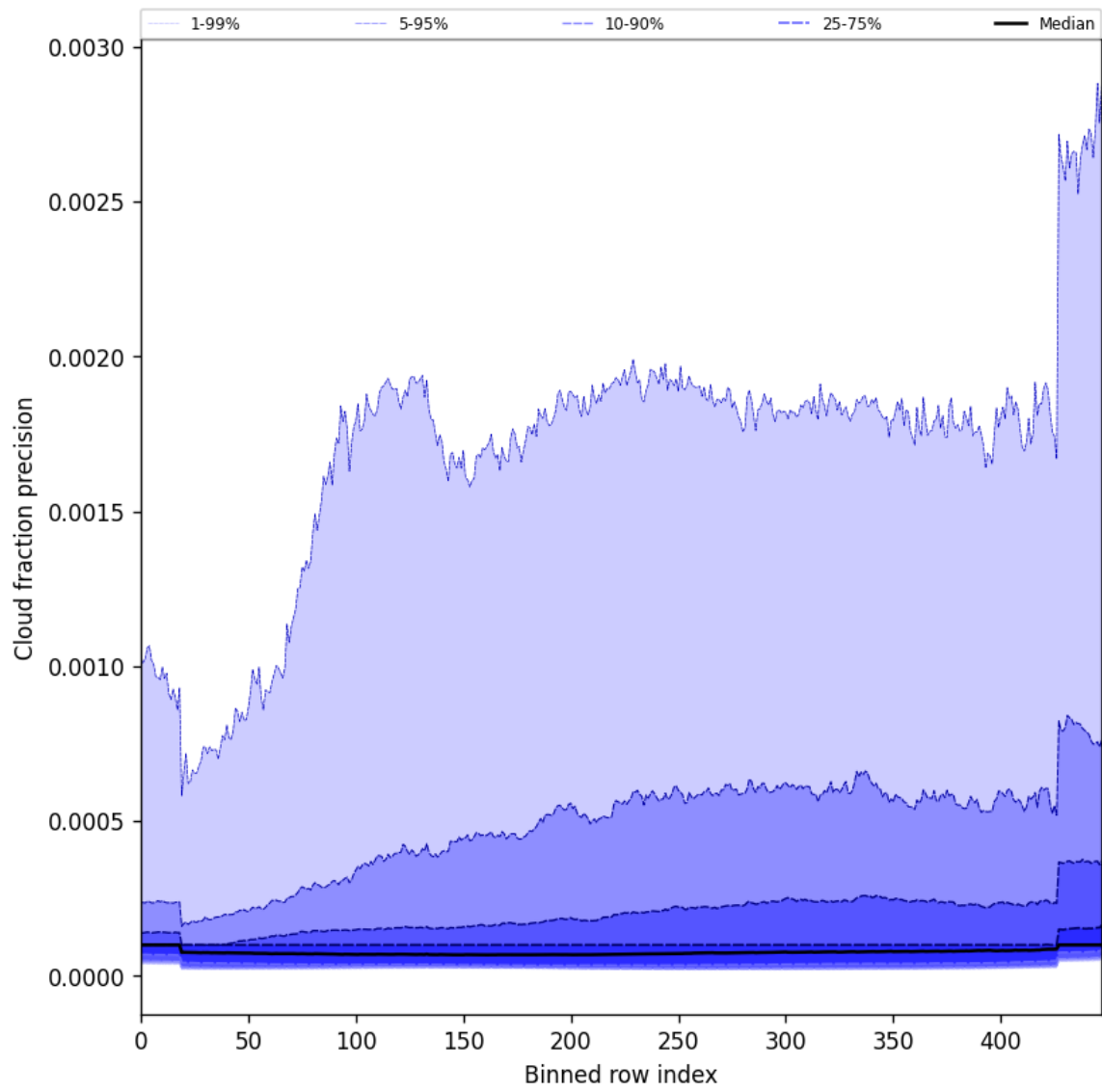
Figure 50: Along track statistics of “Cloud fraction precision” for 2024-11-25 to 2024-11-26
