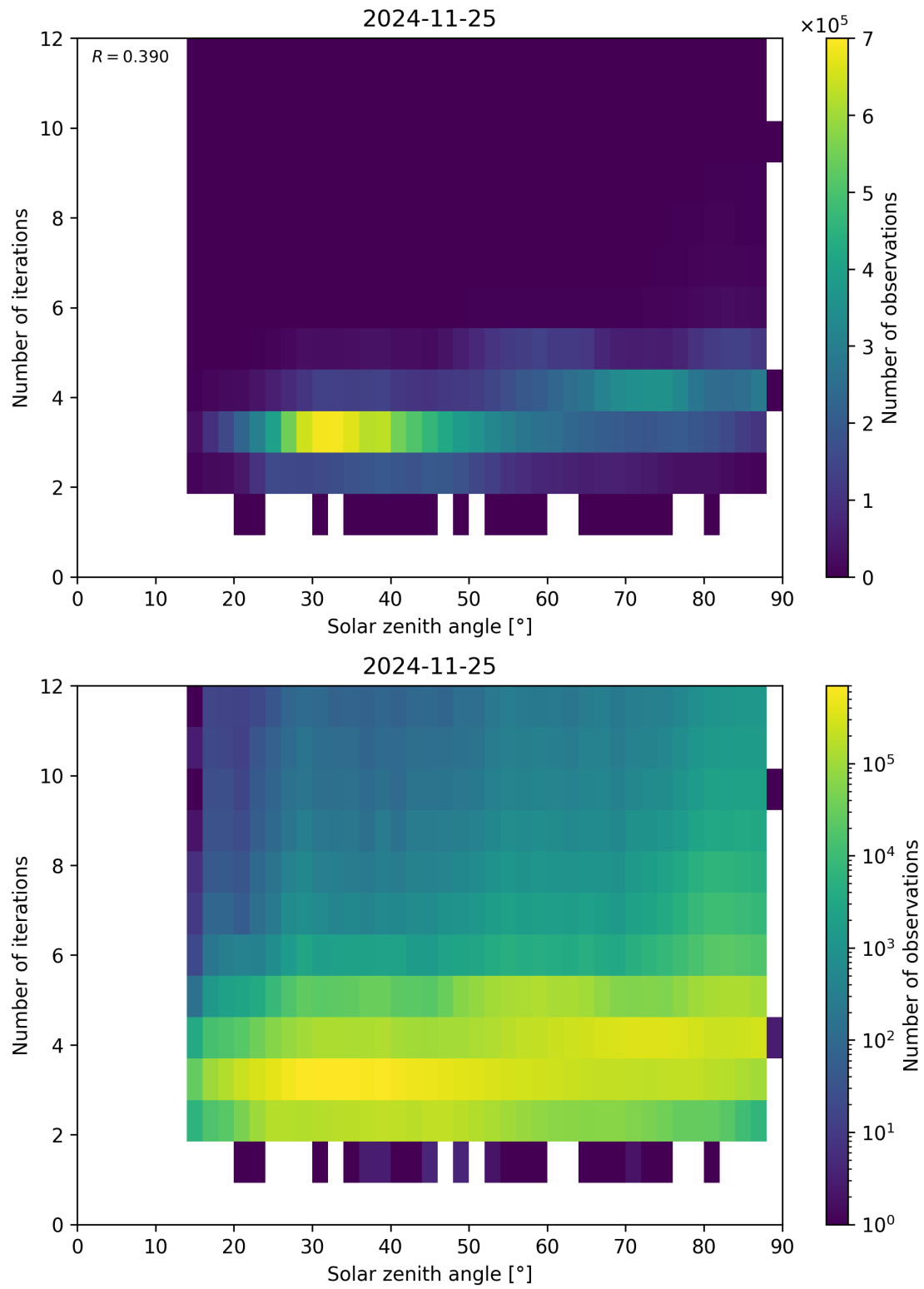
Figure 114: Scatter density plot of “Solar zenith angle” against “Number of iterations” for 2024-11-25 to 2024-11-26.
