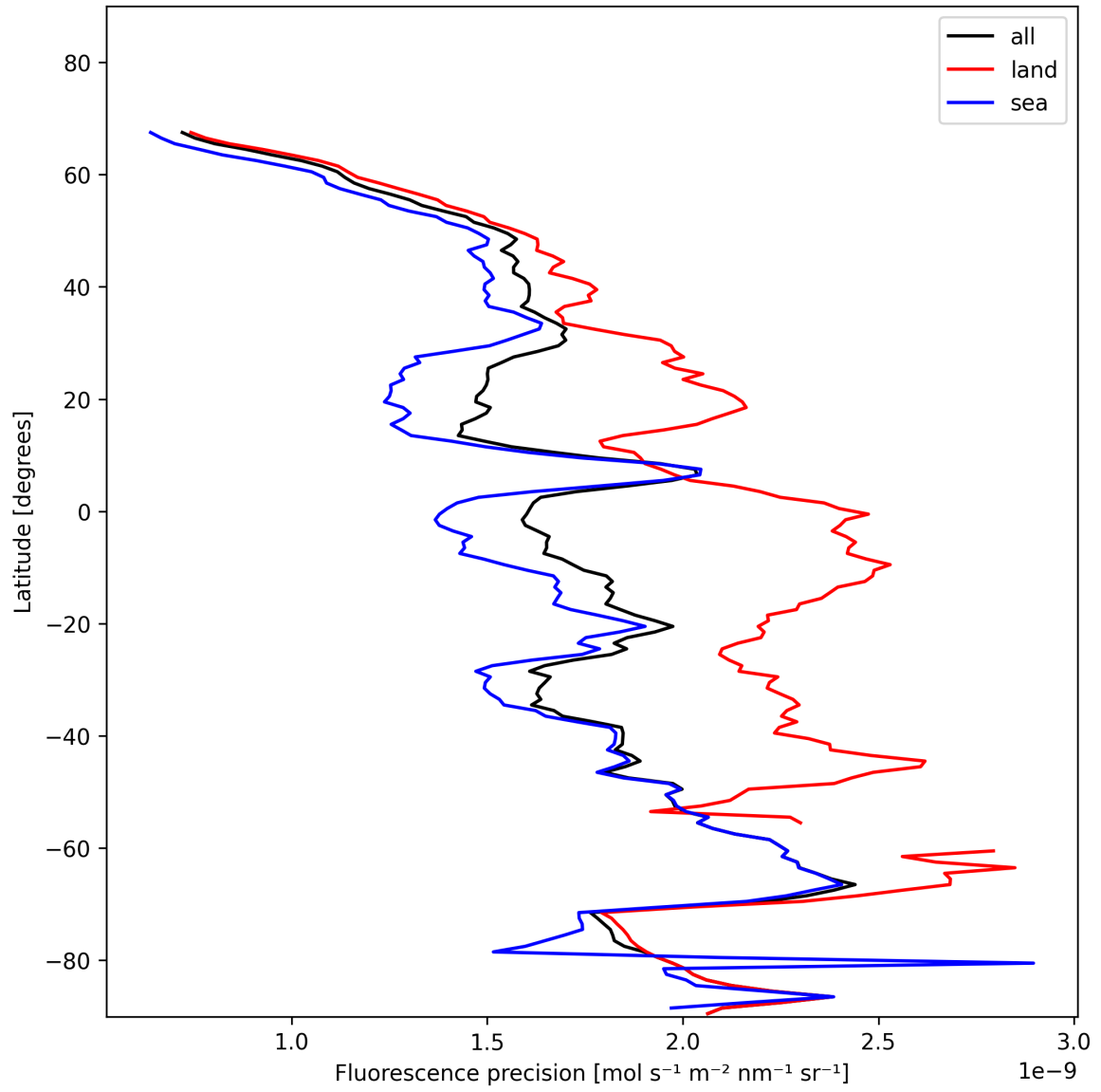
Figure 24: Zonal average of “Fluorescence precision” for 2024-11-25 to 2024-11-26.
