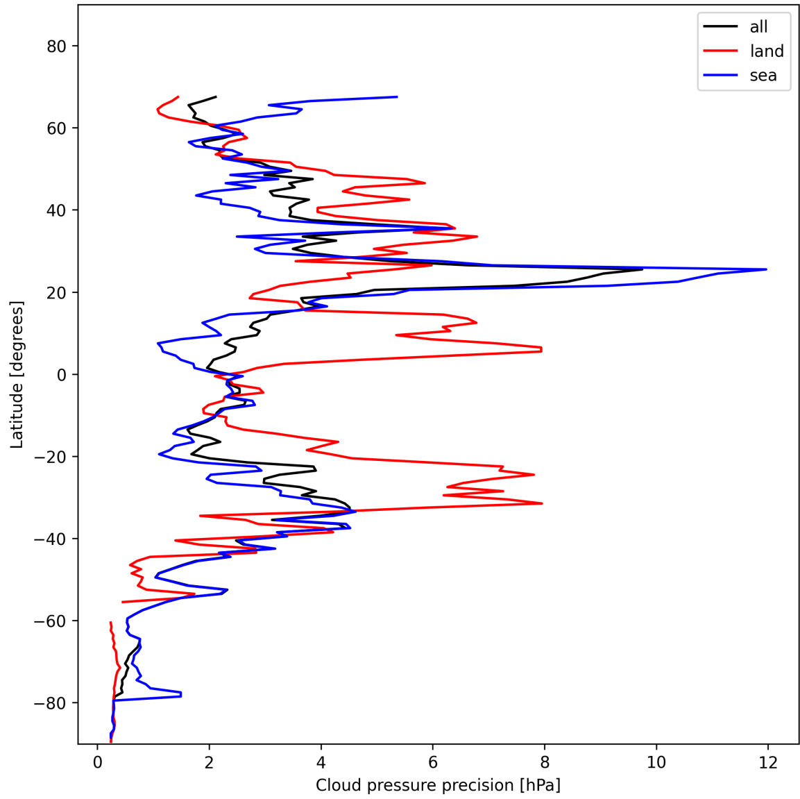
Figure 14: Zonal average of “Cloud pressure precision” for 2024-11-25 to 2024-11-26.
