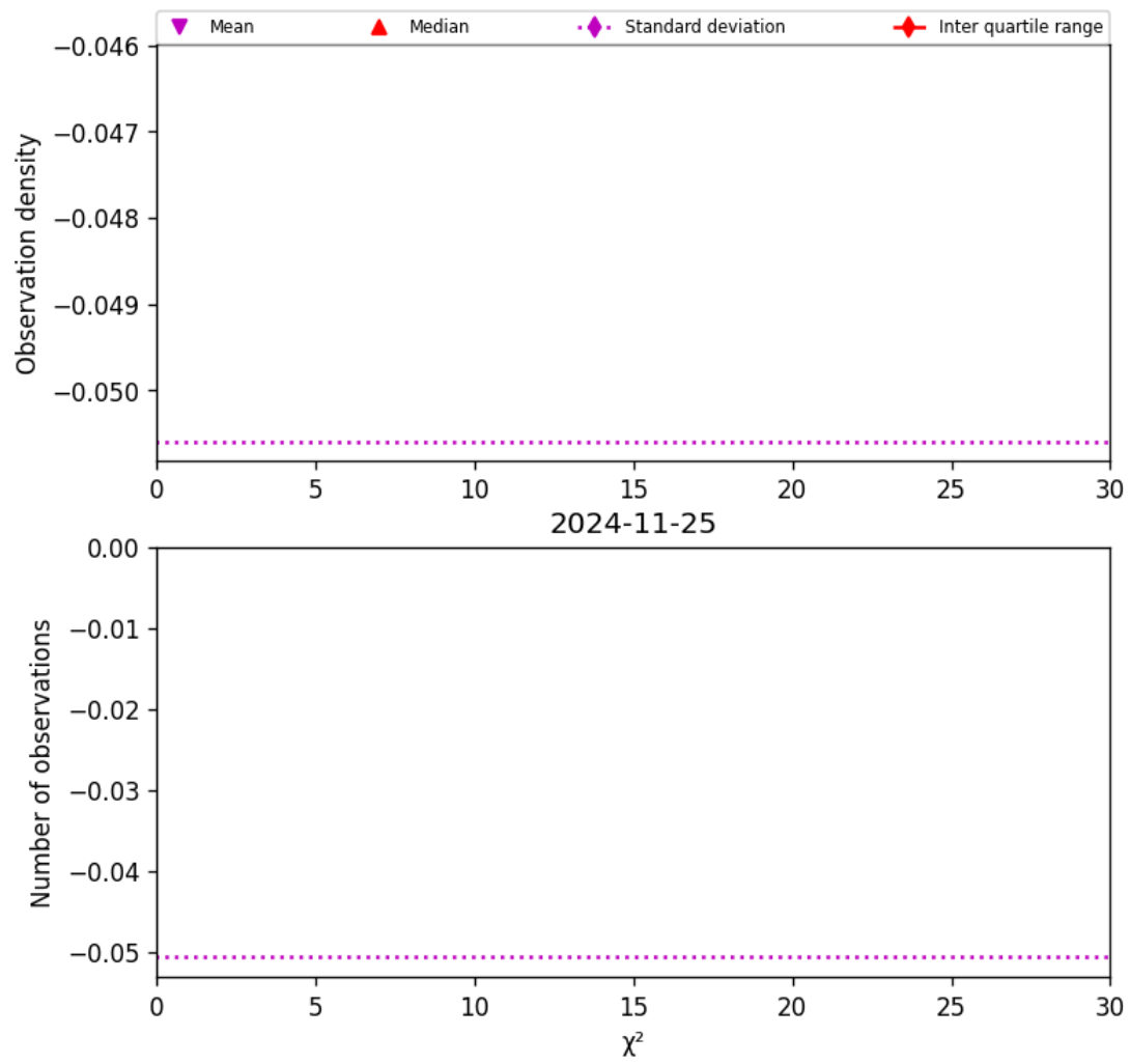
Figure 38: Histogram of " \chi^2 " for 2024-11-25 to 2024-11-26
