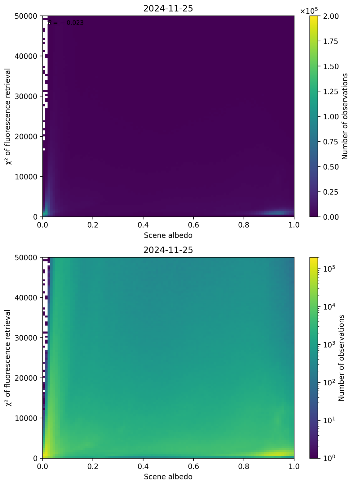
Figure 103: Scatter density plot of “Scene albedo” against “ \chi^2 of fluorescence retrieval” for 2024-11-25 to 2024-11-26.
