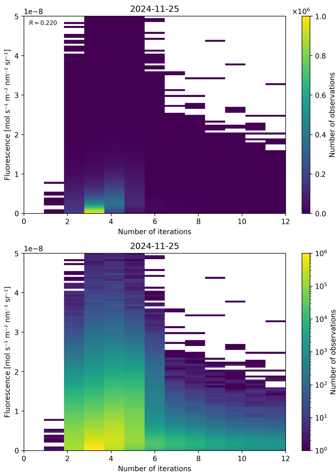
Figure 98: Scatter density plot of “Number of iterations” against “Fluorescence” for 2024-11-25 to 2024-11-26.
