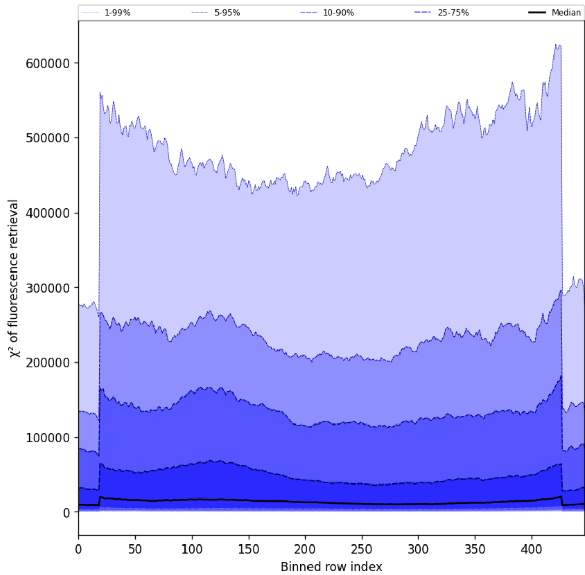
Figure 59: Along track statistics of “ \chi^2 of fluorescence retrieval” for 2024-11-25 to 2024-11-26
