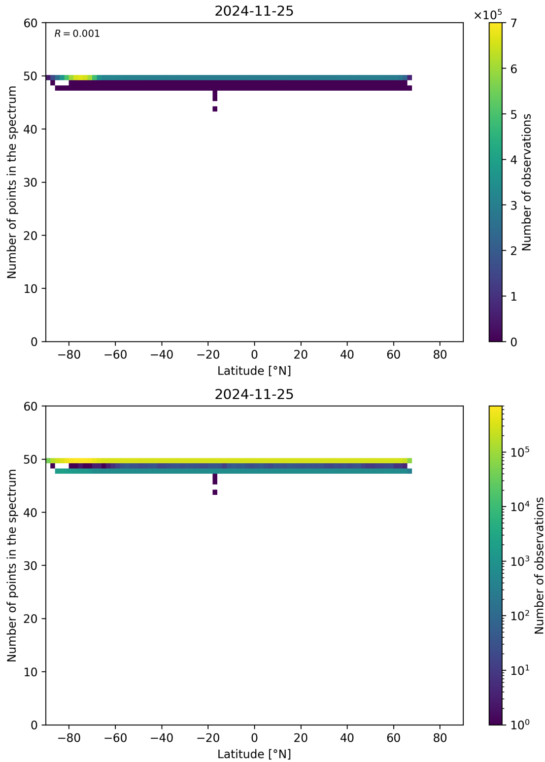
Figure 94: Scatter density plot of “Latitude” against “Number of points in the spectrum” for 2024-11-25 to 2024-11-26.
