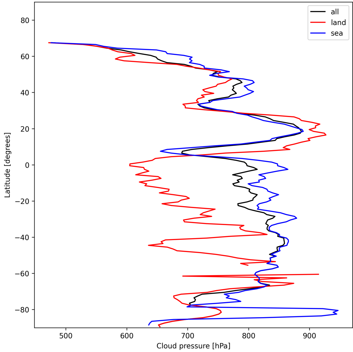
Figure 13: Zonal average of “Cloud pressure” for 2024-11-25 to 2024-11-26.
