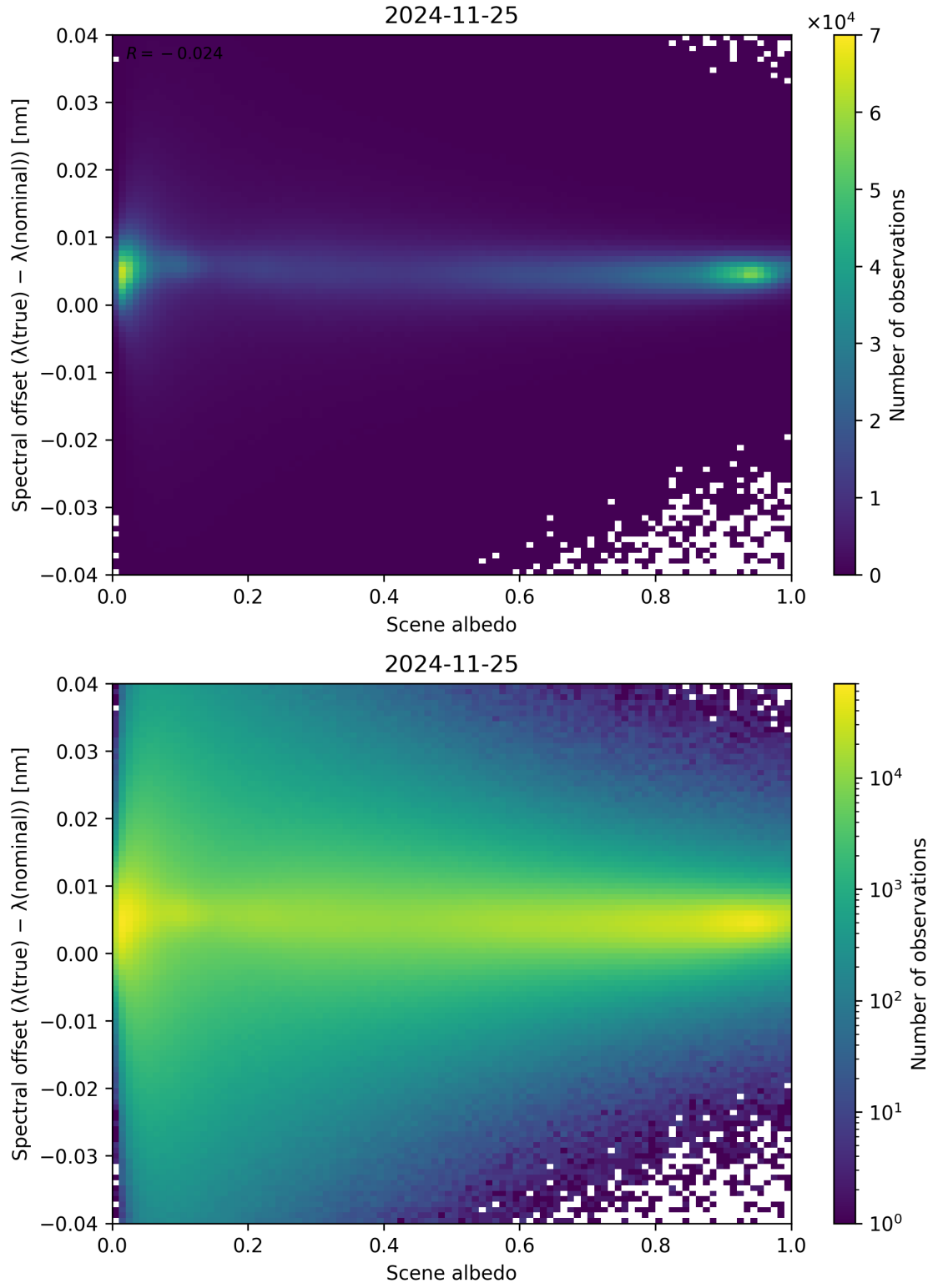
Figure 107: Scatter density plot of “Scene albedo” against “Spectral offset ( \lambda_{\text{true}} - \lambda_{\text{nominal}} )” for 2024-11-25 to 2024-11-26.
