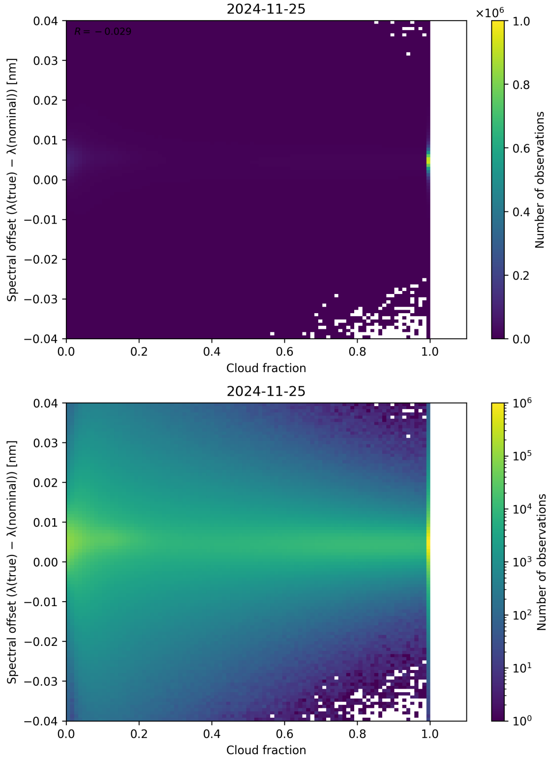
Figure 76: Scatter density plot of “Cloud fraction” against “Spectral offset ( \lambda_{\text{true}} - \lambda_{\text{nominal}} )” for 2024-11-25 to 2024-11-26.
