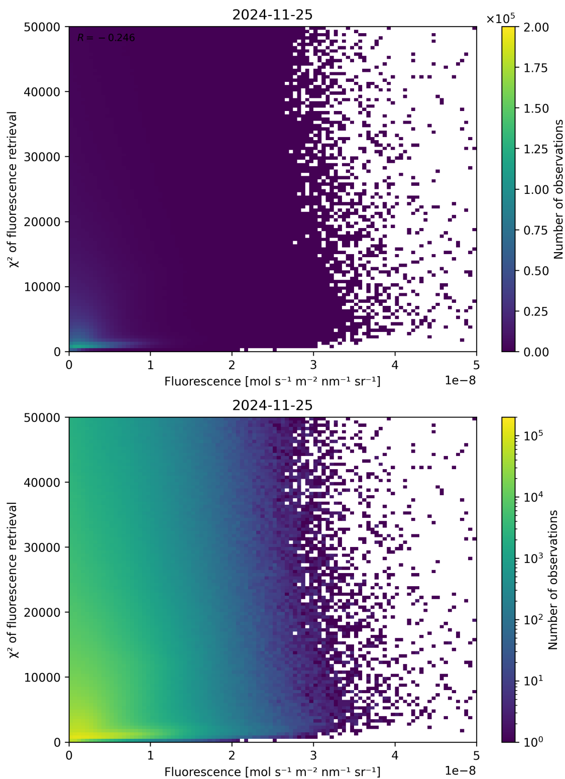
Figure 85: Scatter density plot of “Fluorescence” against “ \chi^2 of fluorescence retrieval” for 2024-11-25 to 2024-11-26.
