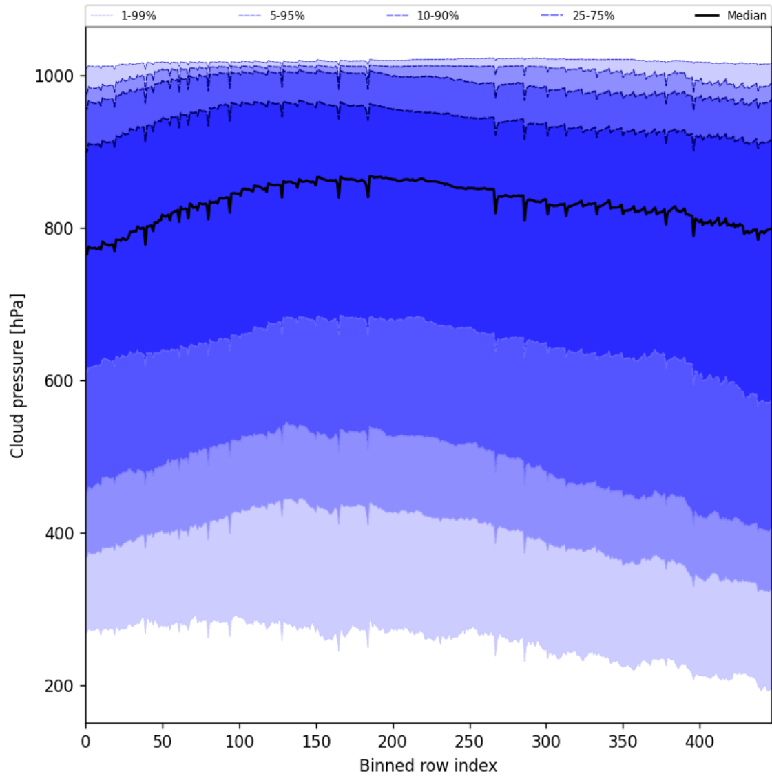
Figure 47: Along track statistics of “Cloud pressure” for 2024-11-25 to 2024-11-26
