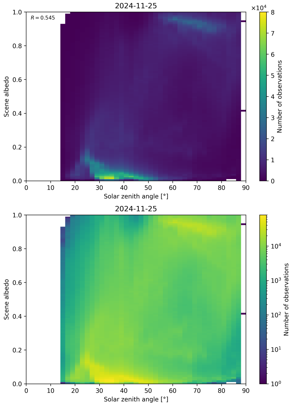
Figure 116: Scatter density plot of “Solar zenith angle” against “Scene albedo” for 2024-11-25 to 2024-11-26.
