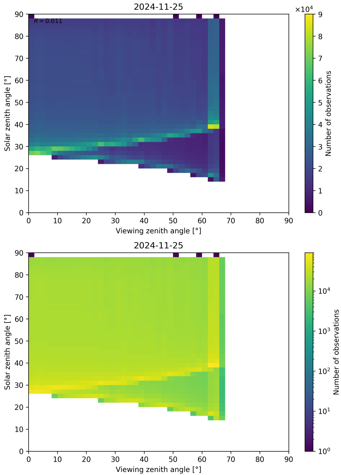
Figure 127: Scatter density plot of “Viewing zenith angle” against “Solar zenith angle” for 2024-11-25 to 2024-11-26.
