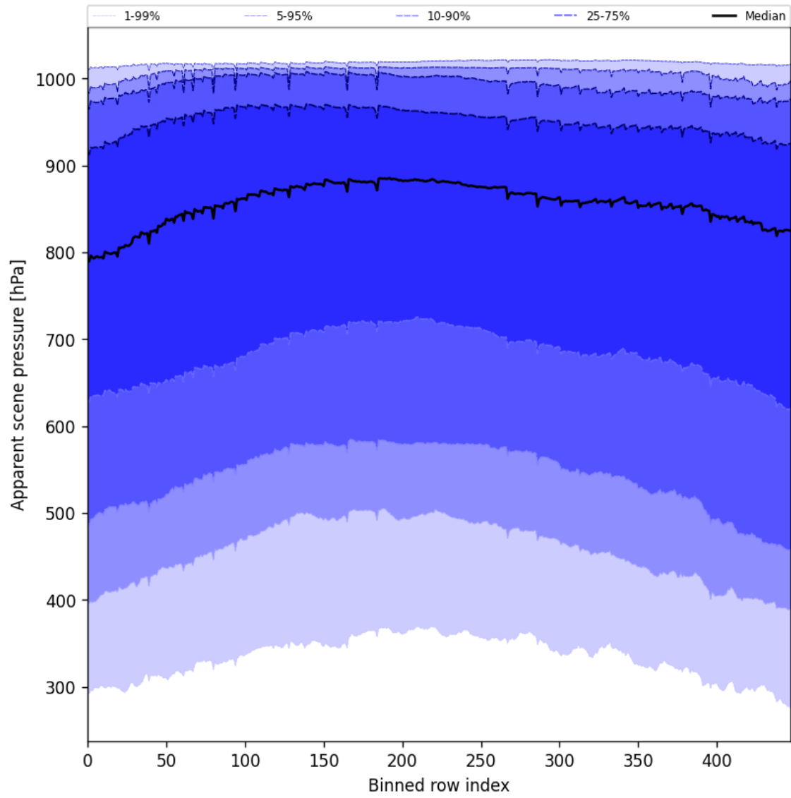
Figure 53: Along track statistics of “Apparent scene pressure” for 2024-11-25 to 2024-11-26
