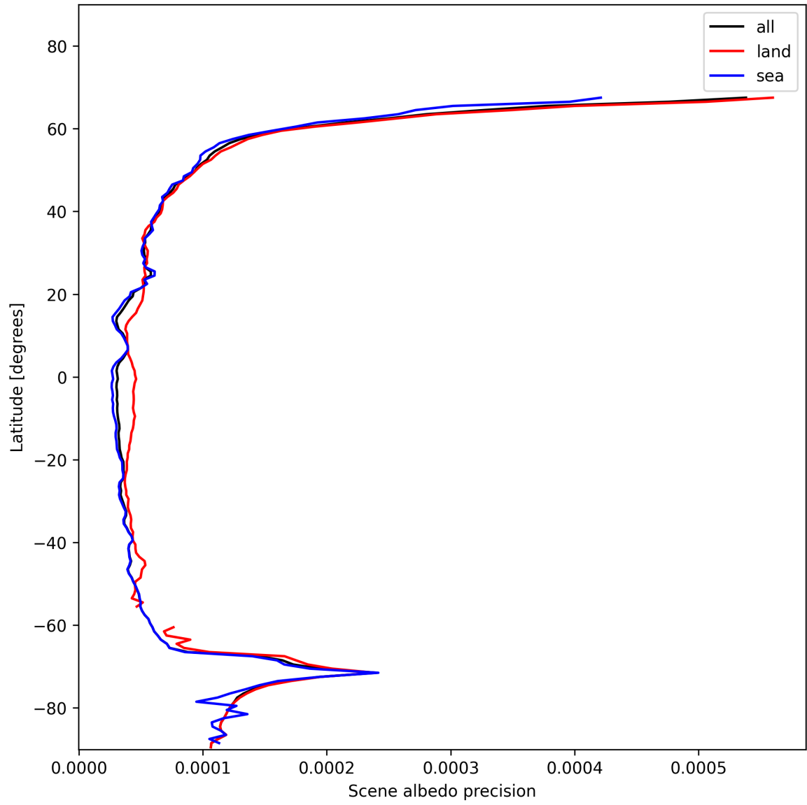
Figure 18: Zonal average of “Scene albedo precision” for 2024-11-25 to 2024-11-26.
