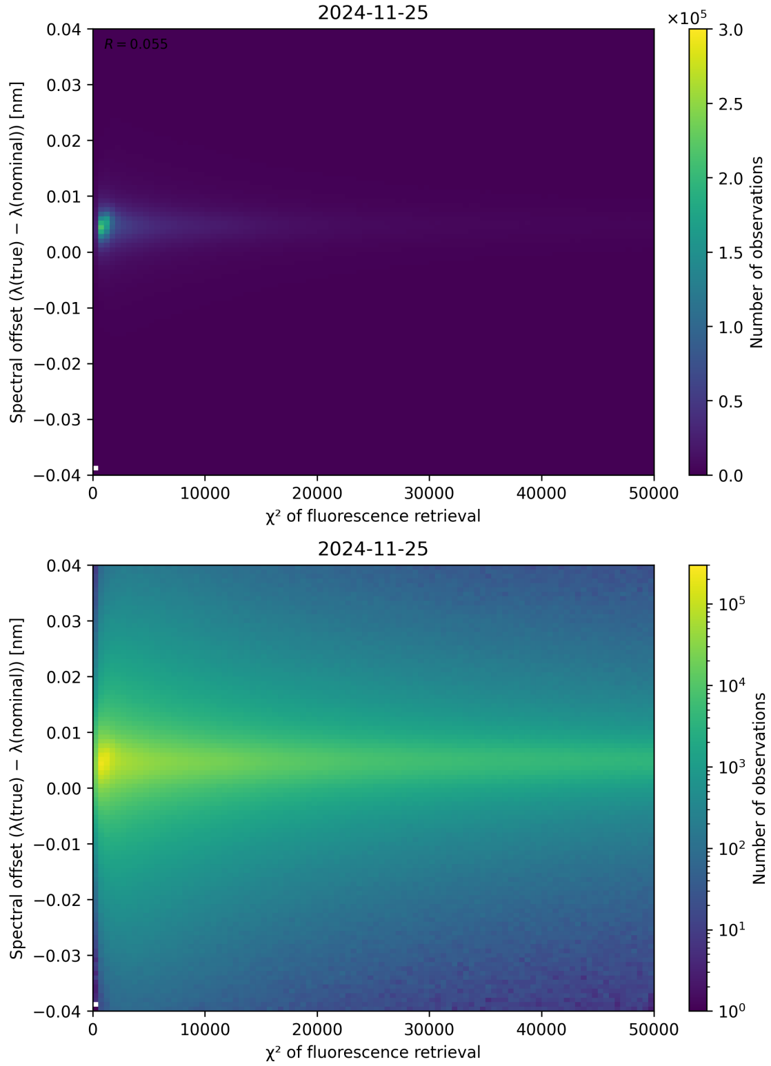
Figure 69: Scatter density plot of “ \chi^2 of fluorescence retrieval” against “Spectral offset ( \lambda_{\text{true}} - \lambda_{\text{nominal}} )” for 2024-11-25 to 2024-11-26.
