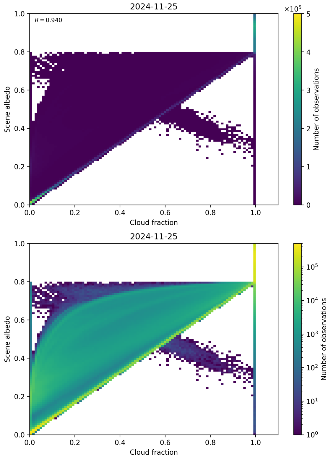
Figure 75: Scatter density plot of “Cloud fraction” against “Scene albedo” for 2024-11-25 to 2024-11-26.
