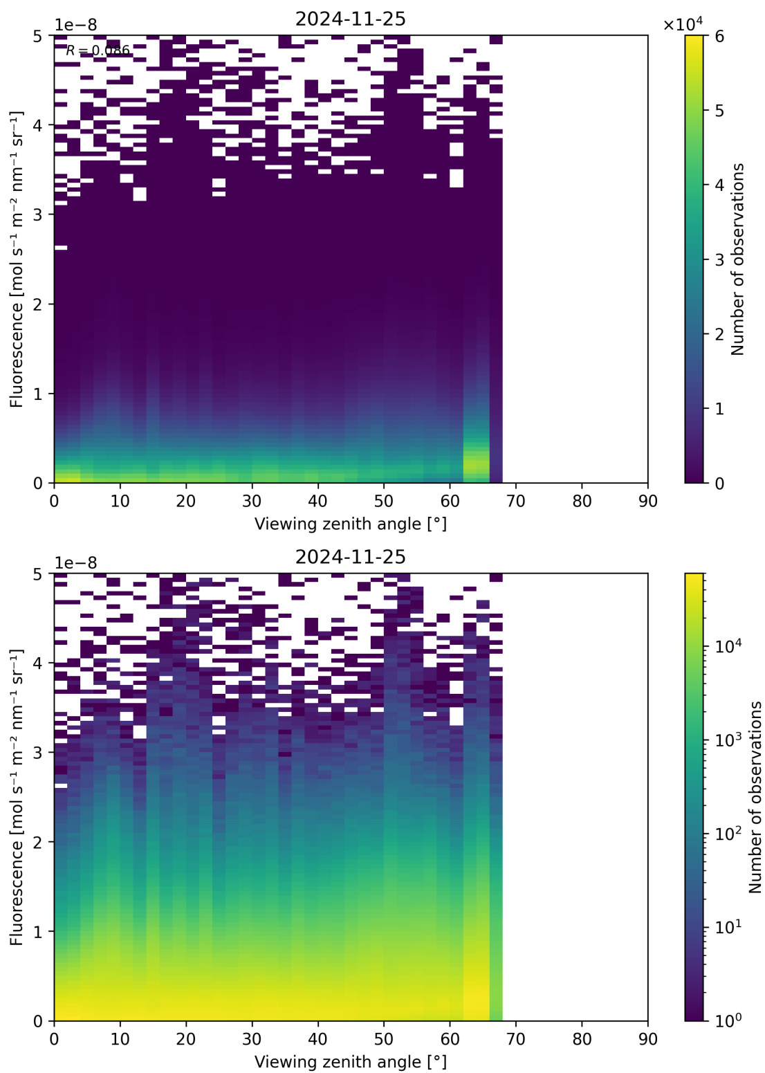
Figure 122: Scatter density plot of “Viewing zenith angle” against “Fluorescence” for 2024-11-25 to 2024-11-26.
