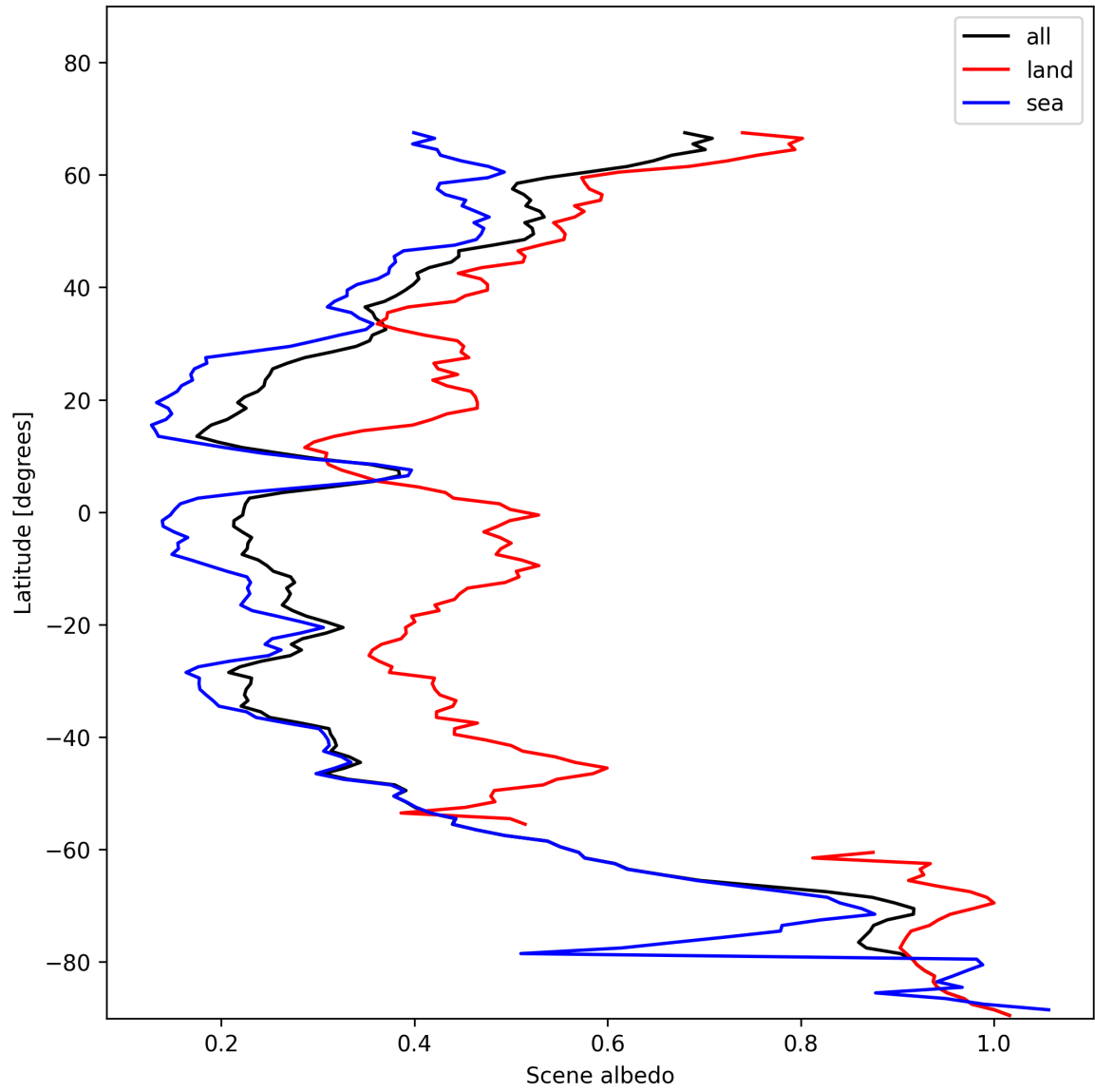
Figure 17: Zonal average of “Scene albedo” for 2024-11-25 to 2024-11-26.
