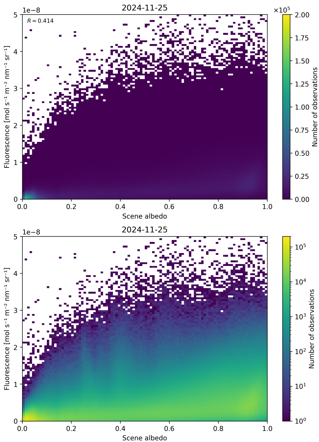
Figure 104: Scatter density plot of “Scene albedo” against “Fluorescence” for 2024-11-25 to 2024-11-26.
