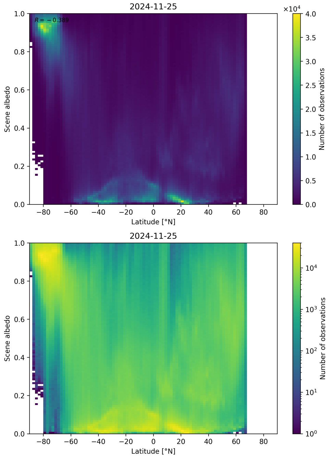
Figure 95: Scatter density plot of “Latitude” against “Scene albedo” for 2024-11-25 to 2024-11-26.
