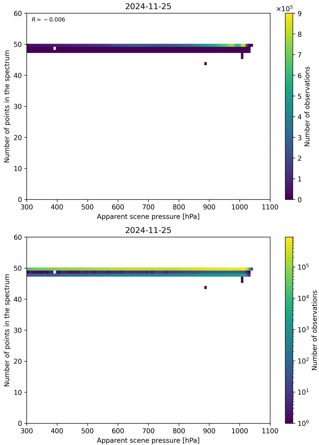
Figure 66: Scatter density plot of “Apparent scene pressure” against “Number of points in the spectrum” for 2024-11-25 to 2024-11-26.
