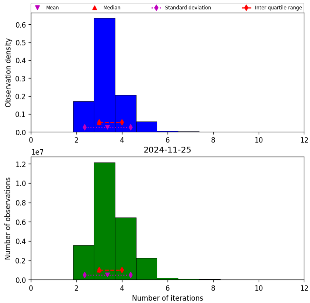
Figure 39: Histogram of “Number of iterations” for 2024-11-25 to 2024-11-26
