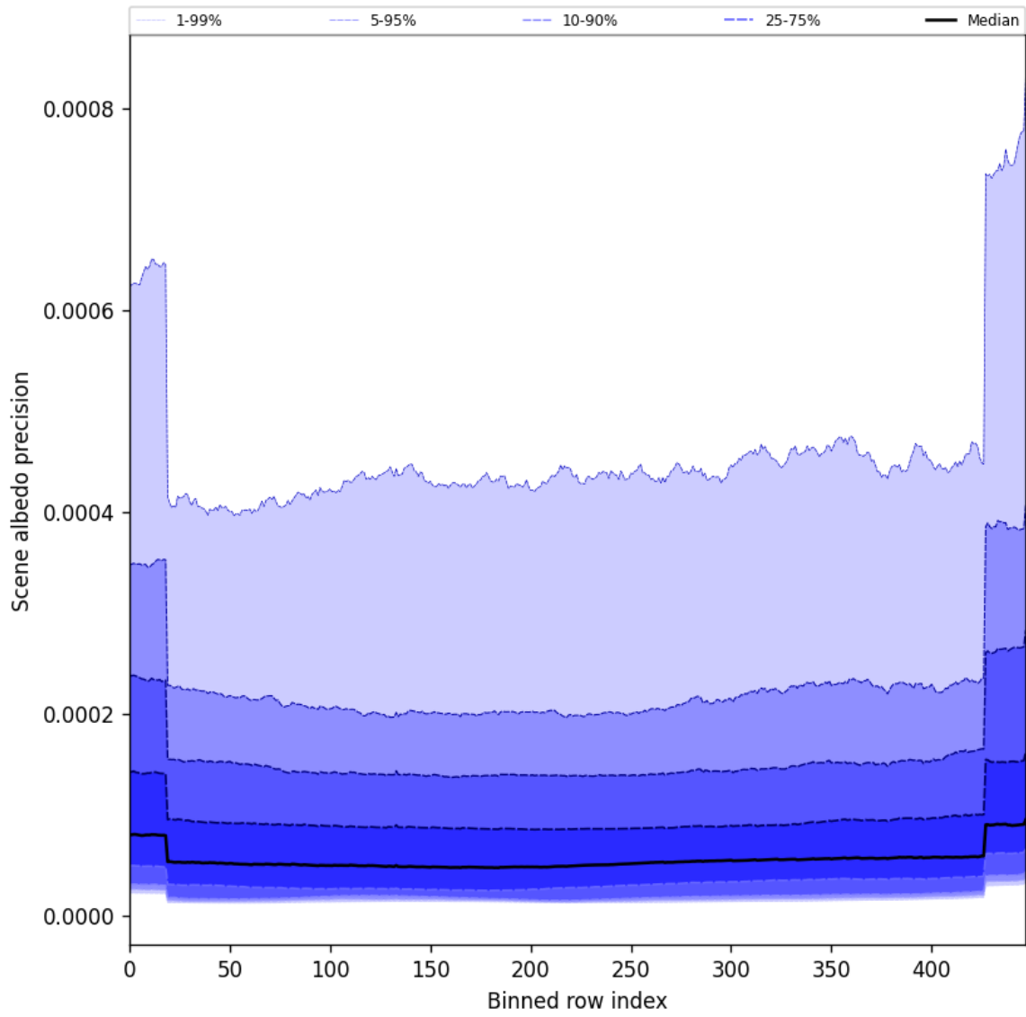
Figure 52: Along track statistics of “Scene albedo precision” for 2024-11-25 to 2024-11-26
