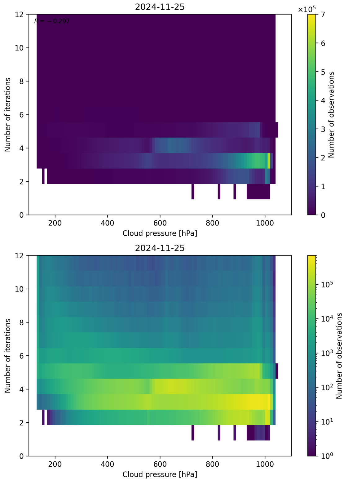
Figure 81: Scatter density plot of “Cloud pressure” against “Number of iterations” for 2024-11-25 to 2024-11-26.
