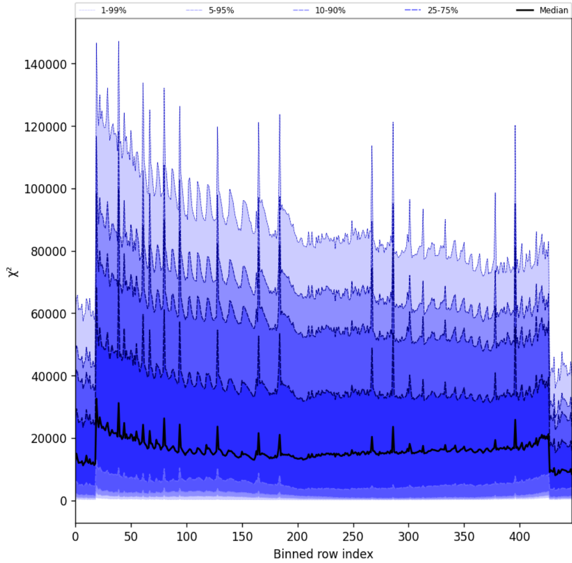
Figure 55: Along track statistics of “ \chi^2 ” for 2024-11-25 to 2024-11-26
