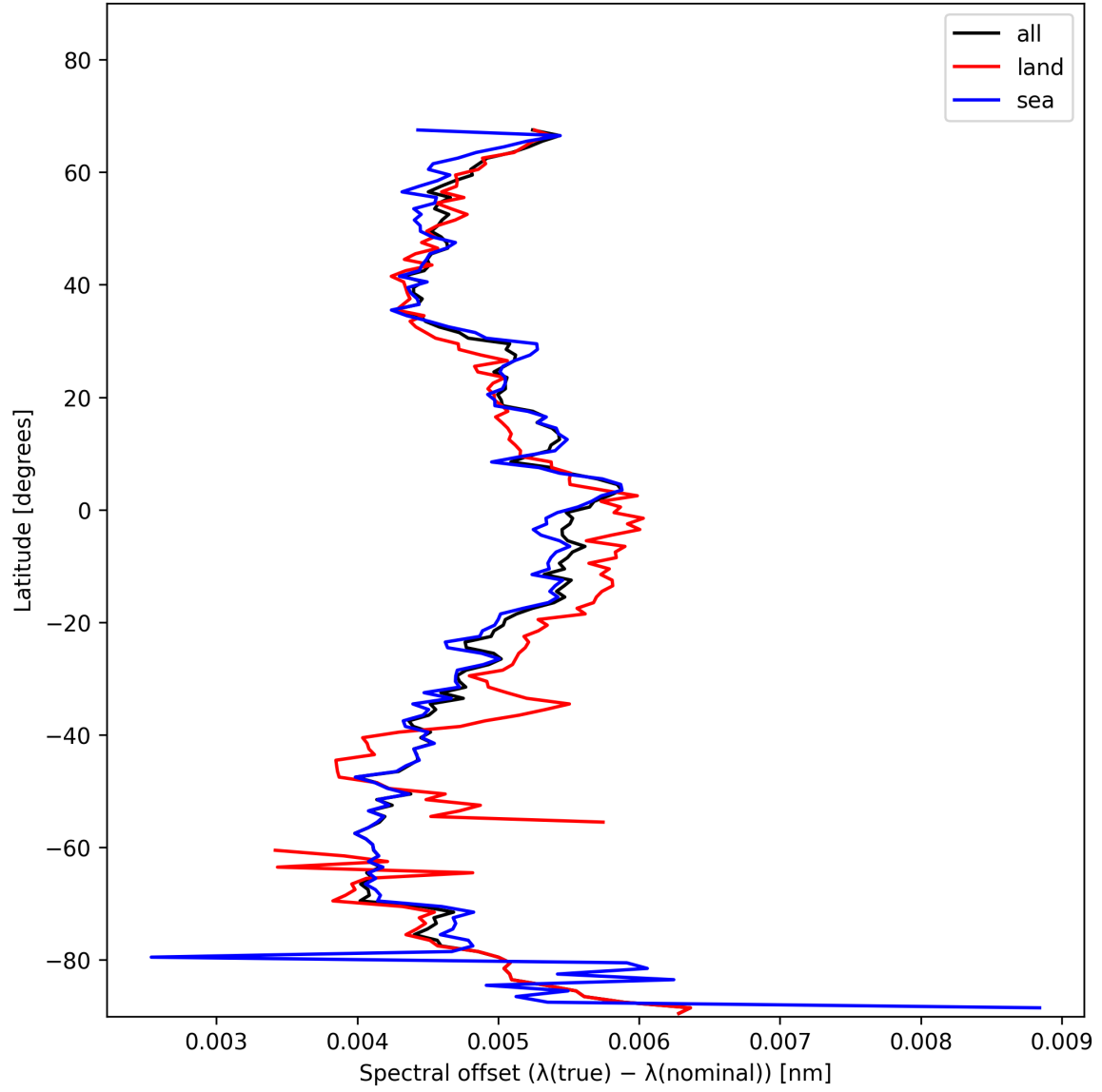
Figure 28: Zonal average of “Spectral offset ( \lambda_{\text{true}} - \lambda_{\text{nominal}} )” for 2024-11-25 to 2024-11-26.
