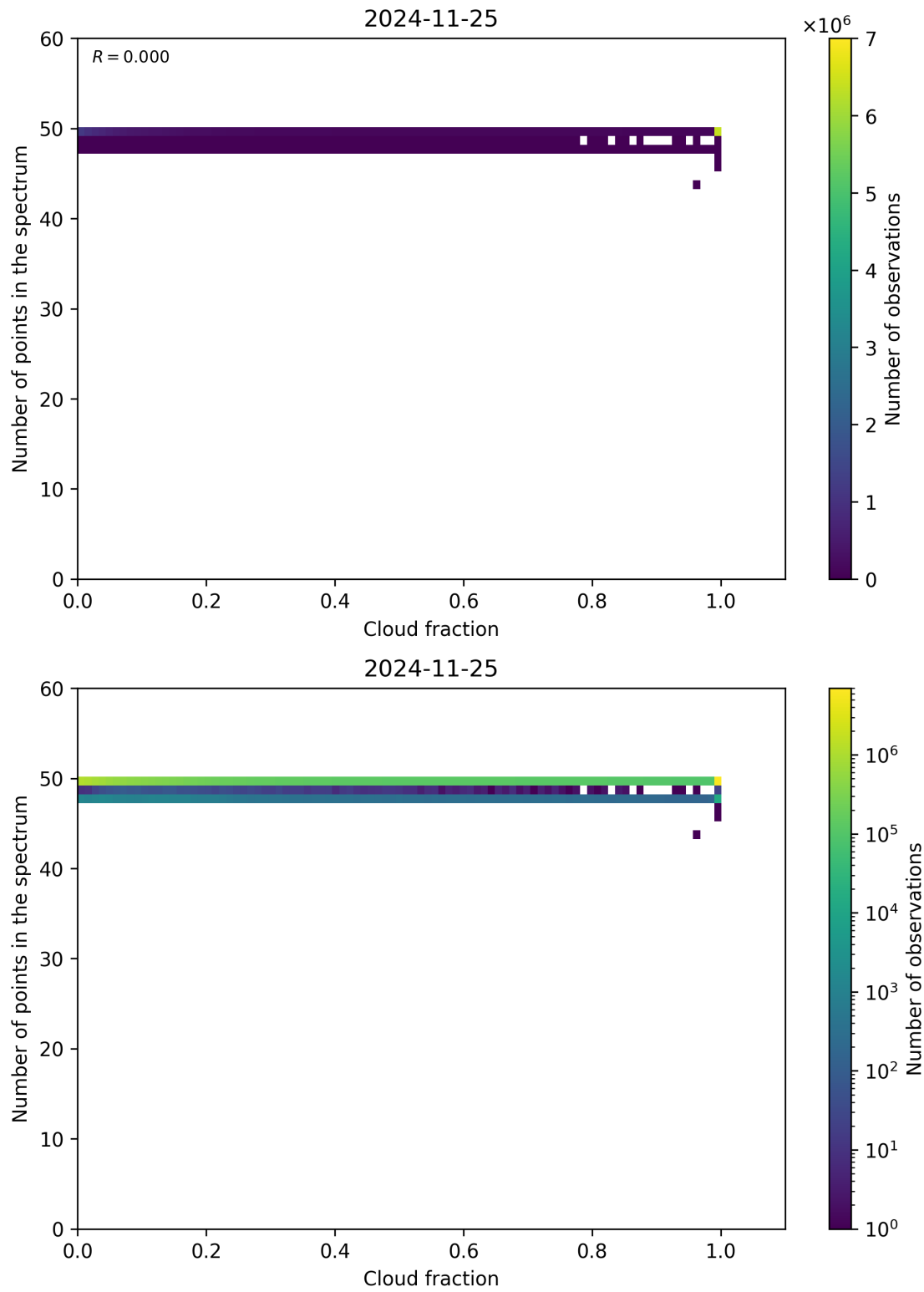
Figure 74: Scatter density plot of “Cloud fraction” against “Number of points in the spectrum” for 2024-11-25 to 2024-11-26.
