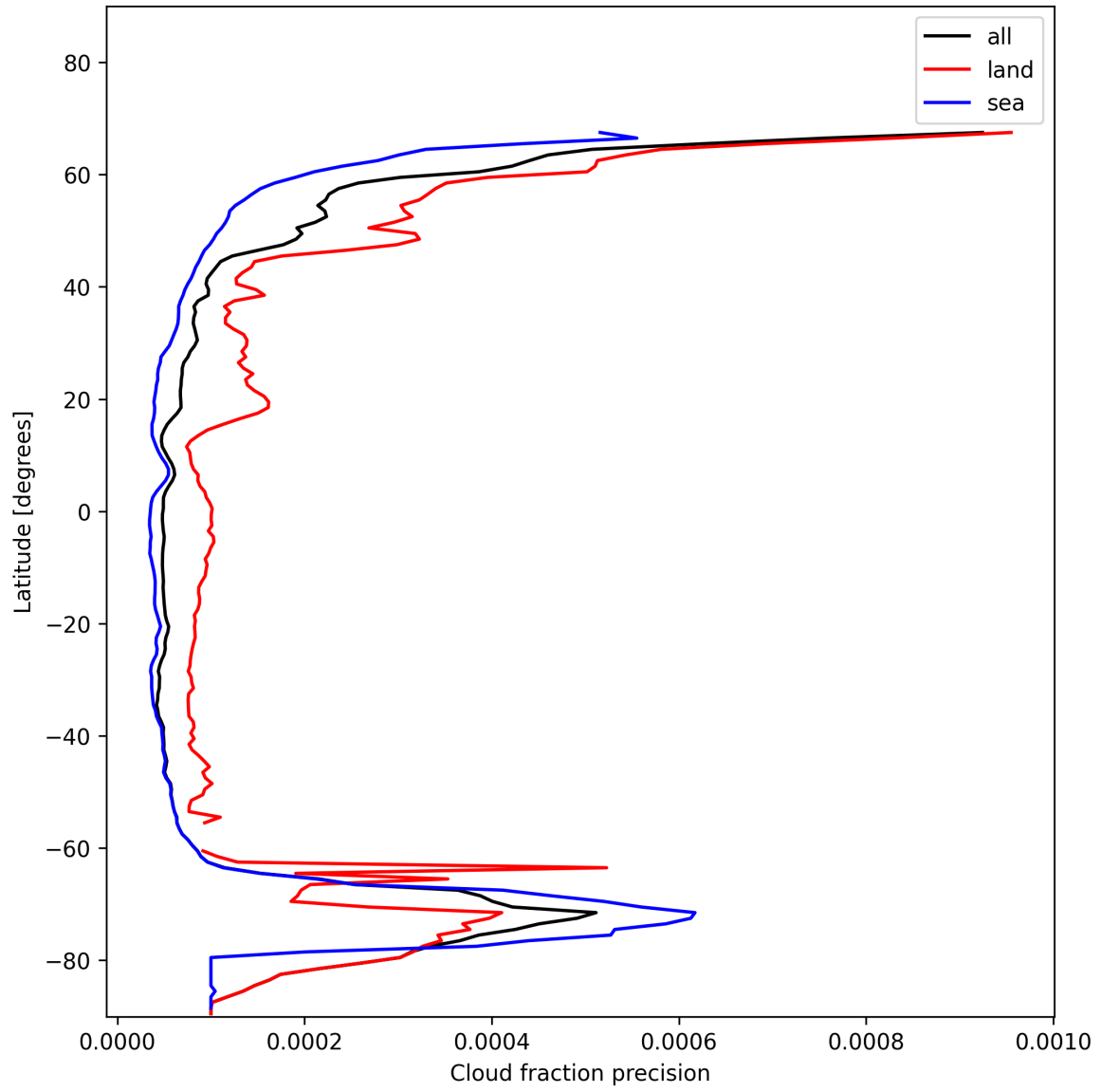
Figure 16: Zonal average of “Cloud fraction precision” for 2024-11-25 to 2024-11-26.
