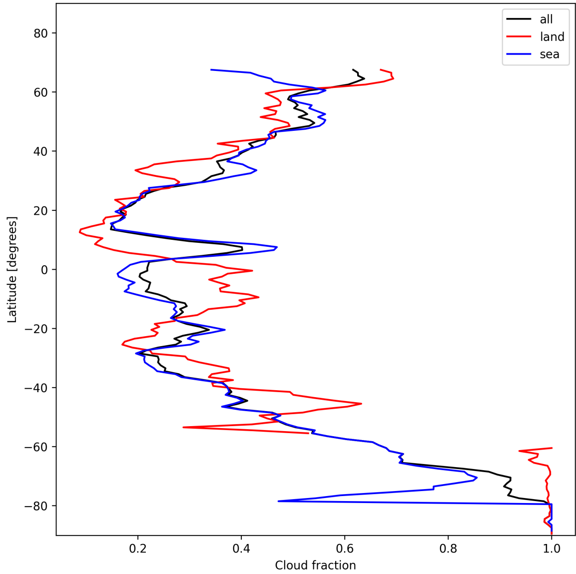
Figure 15: Zonal average of “Cloud fraction” for 2024-11-25 to 2024-11-26.
