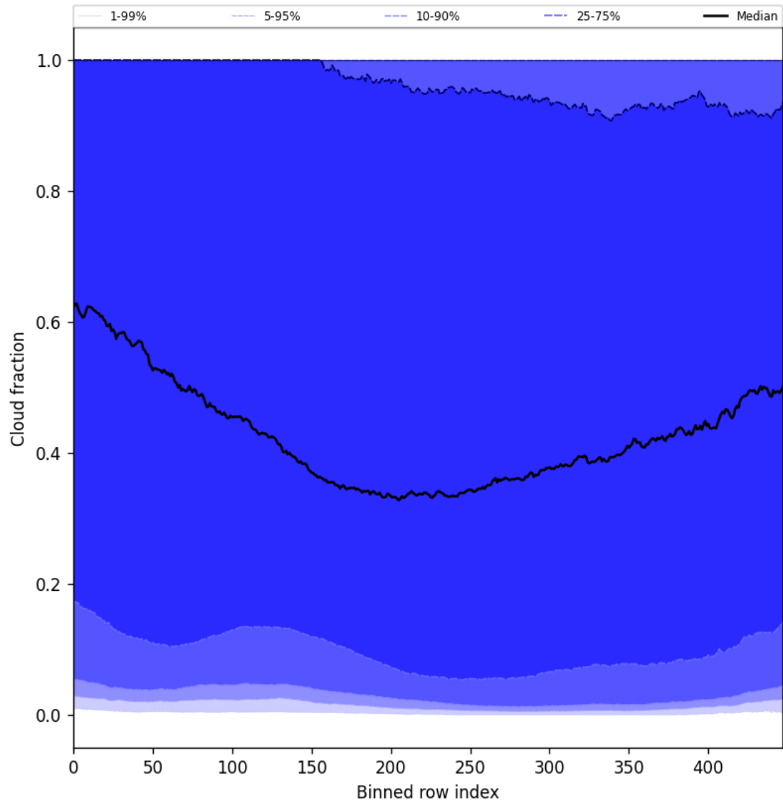
Figure 49: Along track statistics of “Cloud fraction” for 2024-11-25 to 2024-11-26
