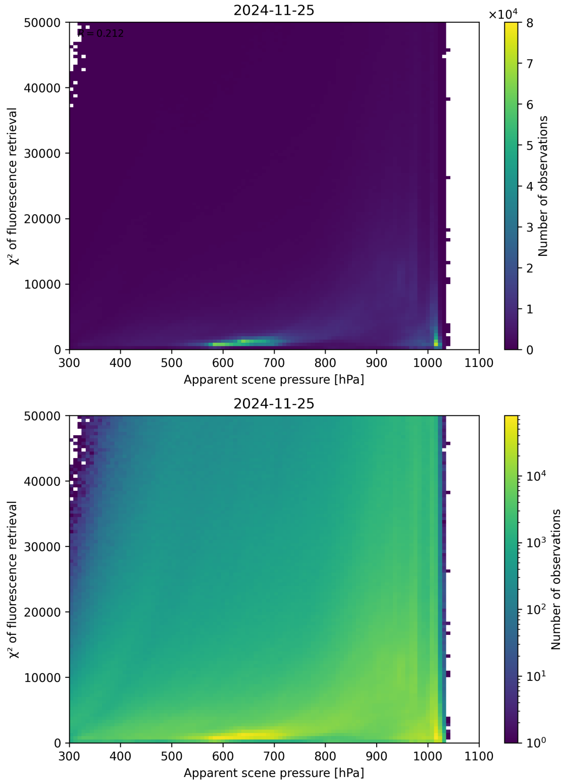
Figure 63: Scatter density plot of “Apparent scene pressure” against “ \chi^2 of fluorescence retrieval” for 2024-11-25 to 2024-11-26.
