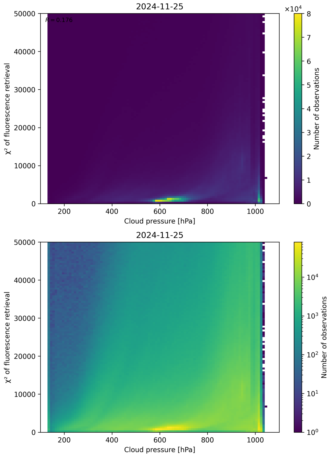
Figure 78: Scatter density plot of “Cloud pressure” against “ \chi^2 of fluorescence retrieval” for 2024-11-25 to 2024-11-26.
