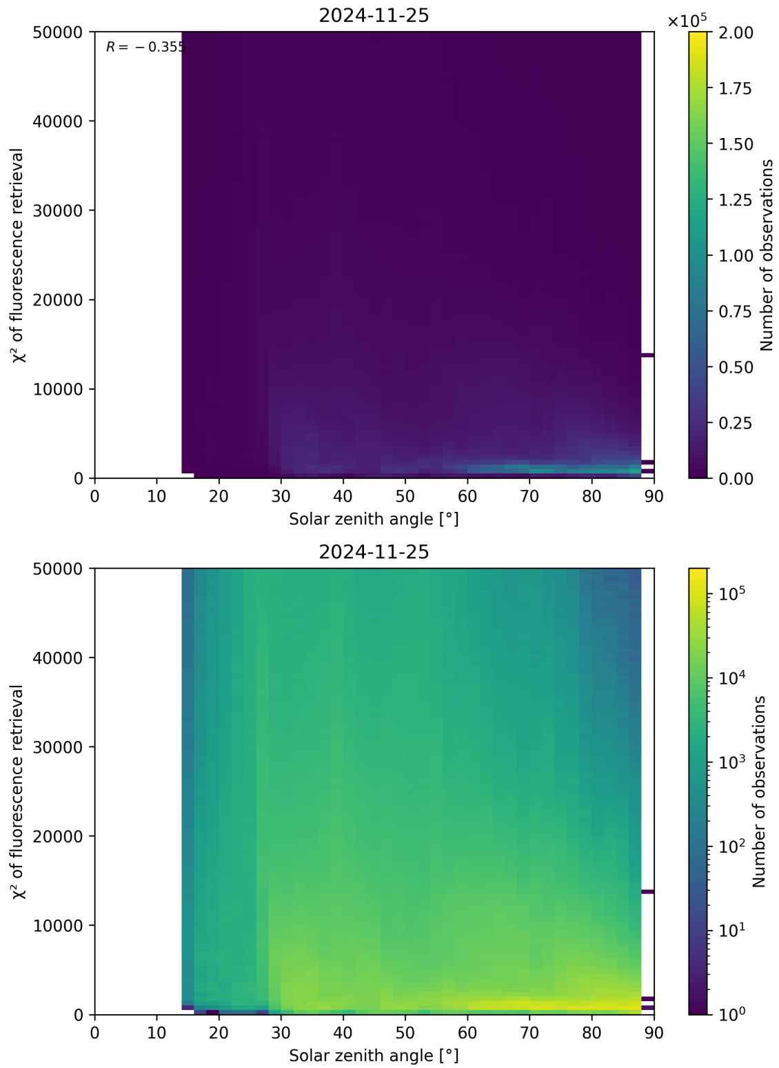
Figure 109: Scatter density plot of “Solar zenith angle” against “ \chi^2 of fluorescence retrieval” for 2024-11-25 to 2024-11-26.
