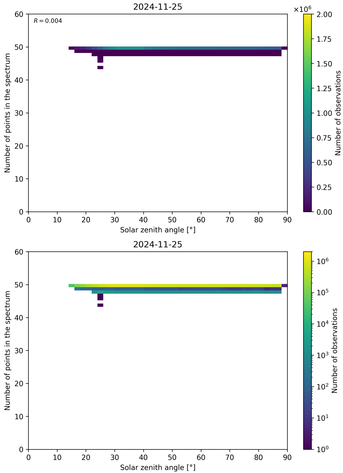
Figure 115: Scatter density plot of “Solar zenith angle” against “Number of points in the spectrum” for 2024-11-25 to 2024-11-26.
