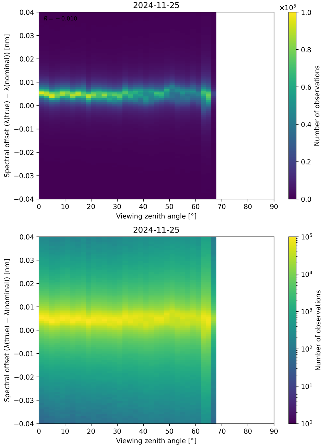
Figure 128: Scatter density plot of “Viewing zenith angle” against “Spectral offset ( \lambda_{\text{true}} - \lambda_{\text{nominal}} )” for 2024-11-25 to 2024-11-26.
