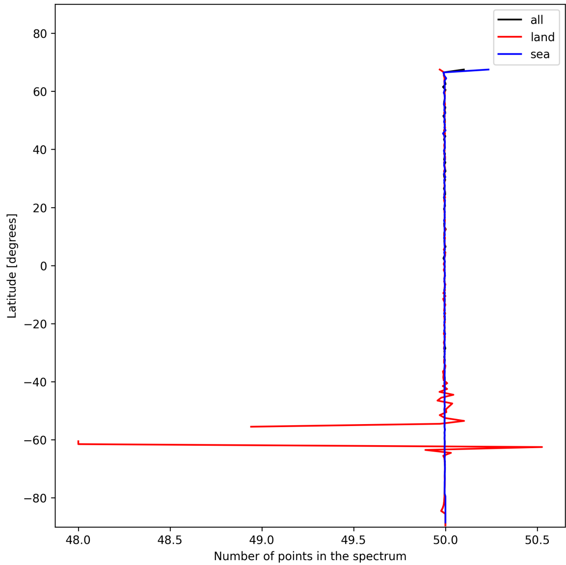
Figure 27: Zonal average of “Number of points in the spectrum” for 2024-11-25 to 2024-11-26.
