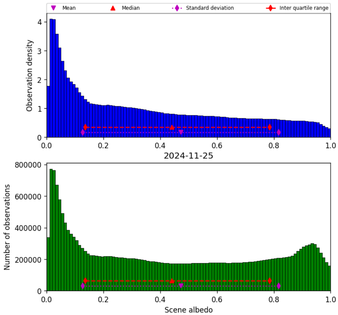
Figure 34: Histogram of “Scene albedo” for 2024-11-25 to 2024-11-26
