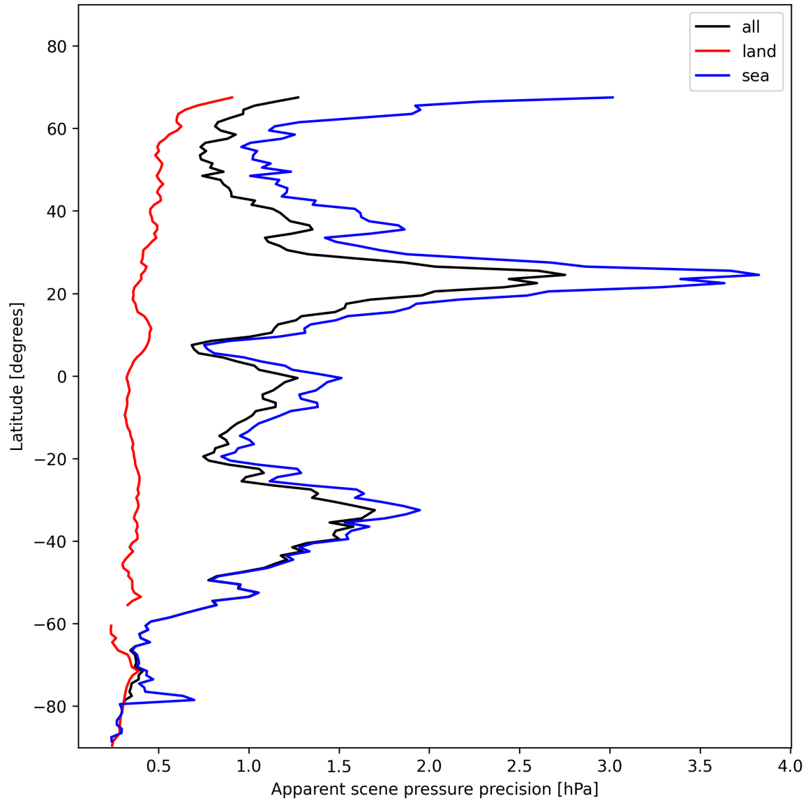
Figure 20: Zonal average of “Apparent scene pressure precision” for 2024-11-25 to 2024-11-26.
