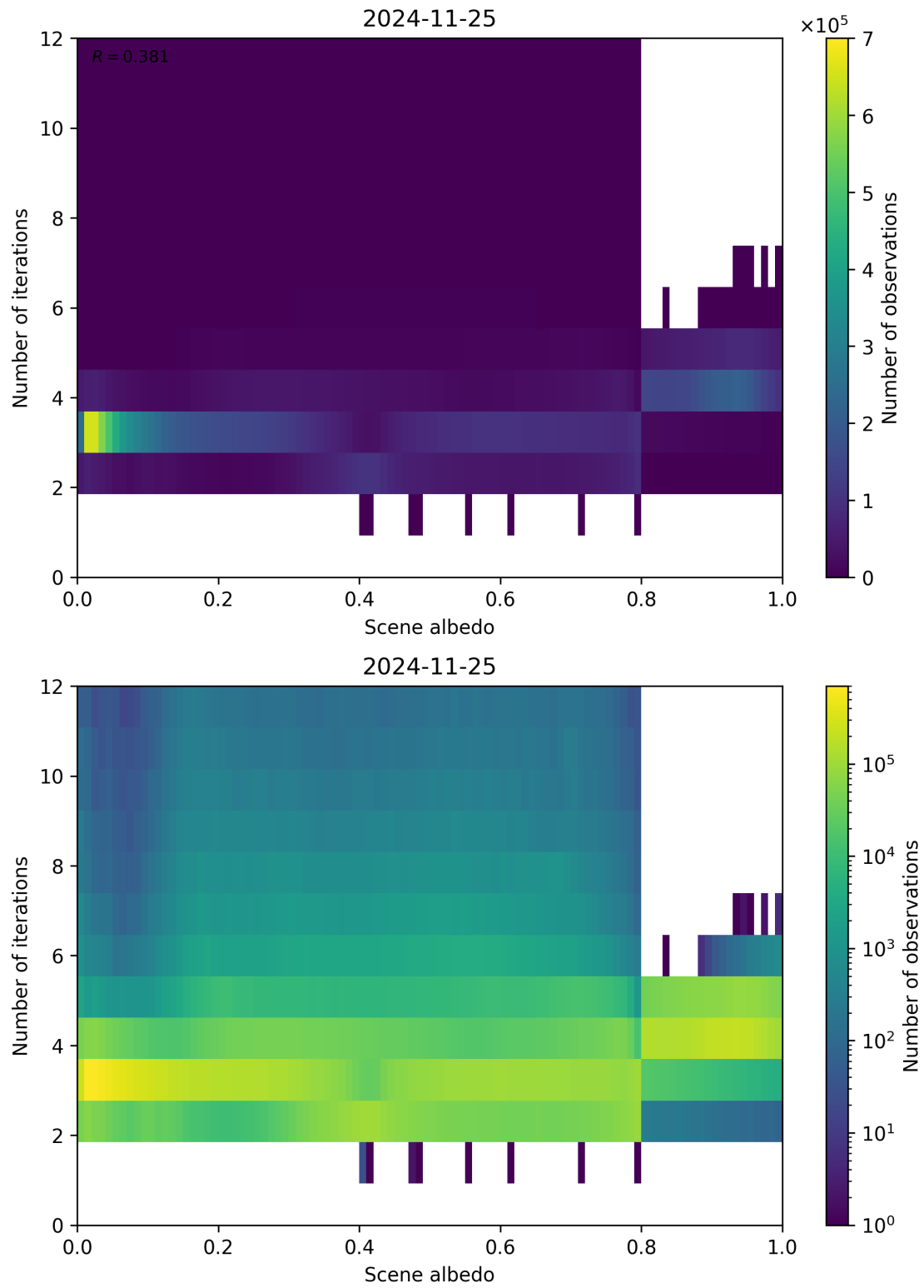
Figure 105: Scatter density plot of “Scene albedo” against “Number of iterations” for 2024-11-25 to 2024-11-26.
