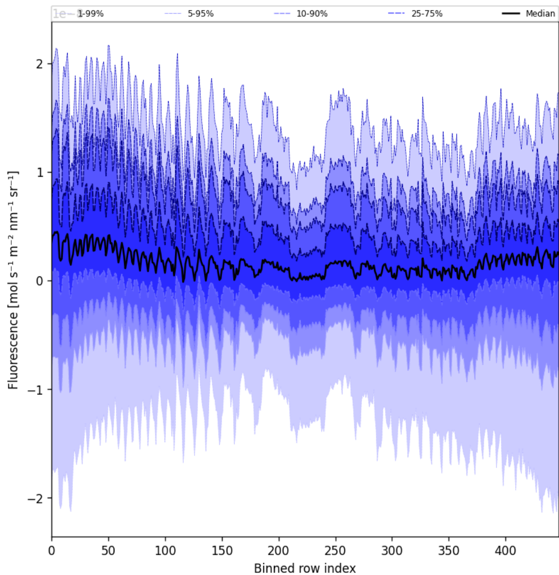
Figure 57: Along track statistics of "Fluorescence" for 2024-11-25 to 2024-11-26
