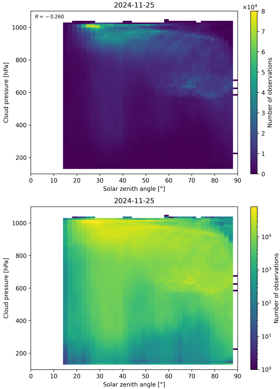
Figure 111: Scatter density plot of “Solar zenith angle” against “Cloud pressure” for 2024-11-25 to 2024-11-26.
