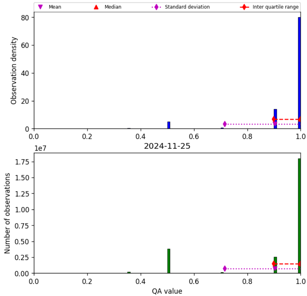
Figure 29: Histogram of “QA value” for 2024-11-25 to 2024-11-26
