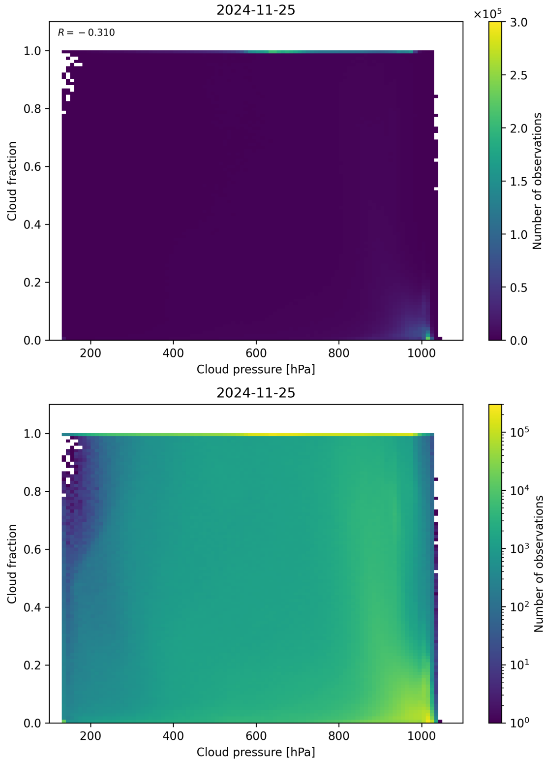
Figure 79: Scatter density plot of “Cloud pressure” against “Cloud fraction” for 2024-11-25 to 2024-11-26.
