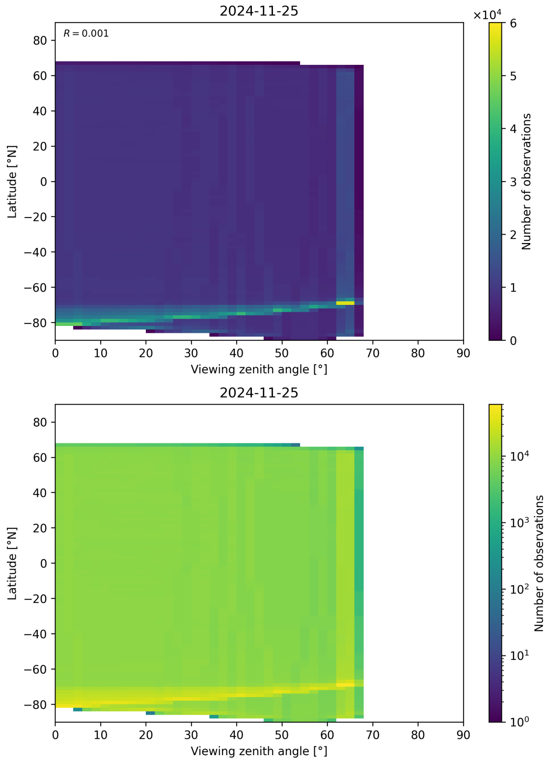
Figure 123: Scatter density plot of “Viewing zenith angle” against “Latitude” for 2024-11-25 to 2024-11-26.
