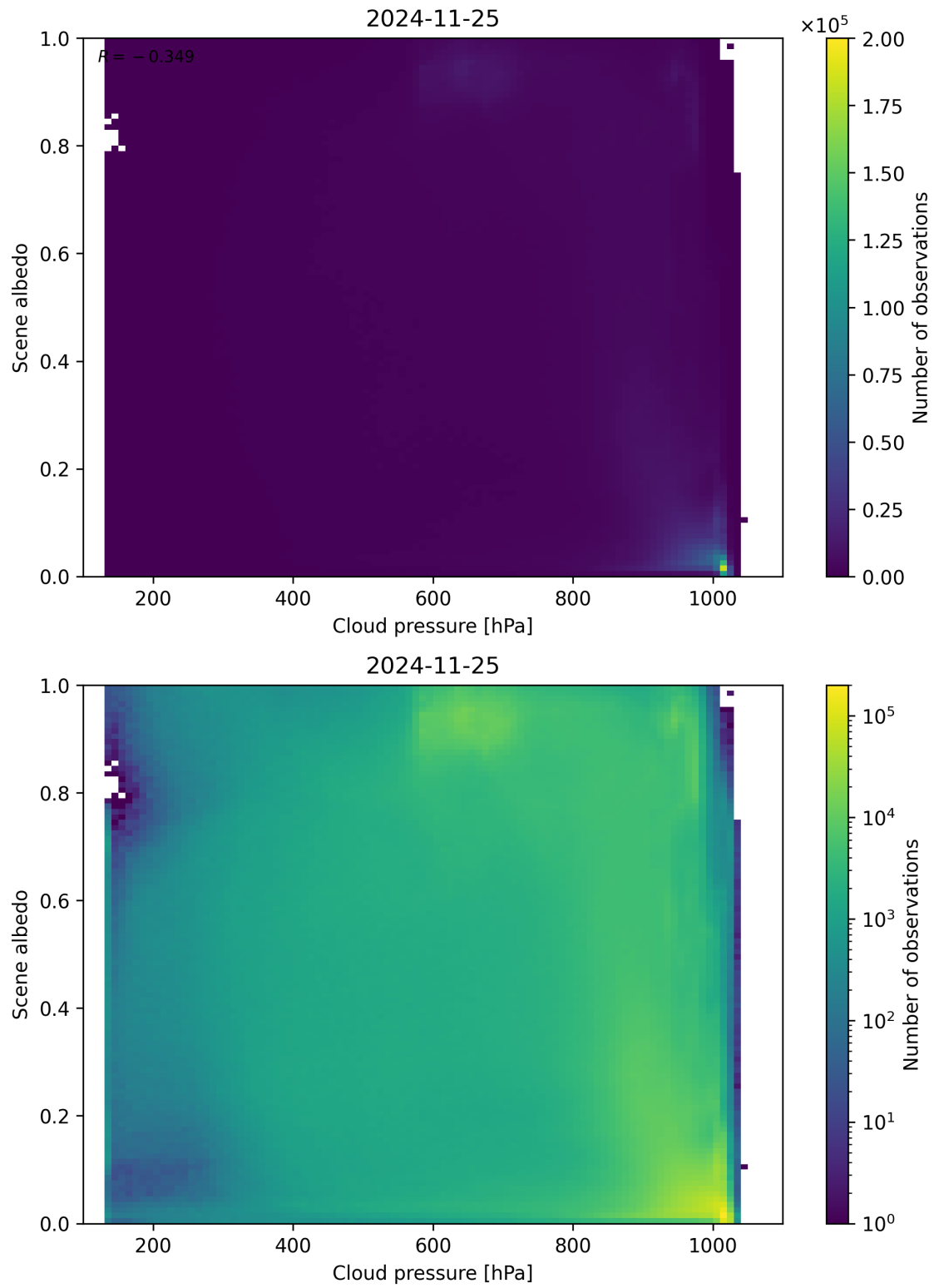
Figure 83: Scatter density plot of “Cloud pressure” against “Scene albedo” for 2024-11-25 to 2024-11-26.
