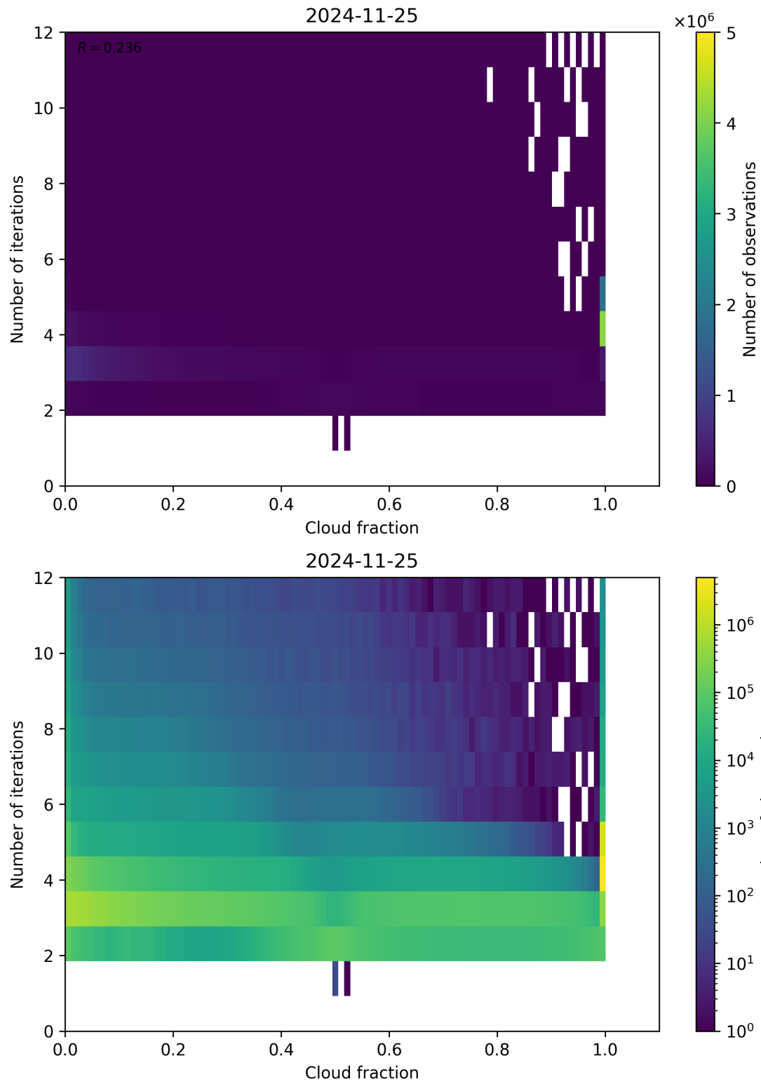
Figure 73: Scatter density plot of “Cloud fraction” against “Number of iterations” for 2024-11-25 to 2024-11-26.
