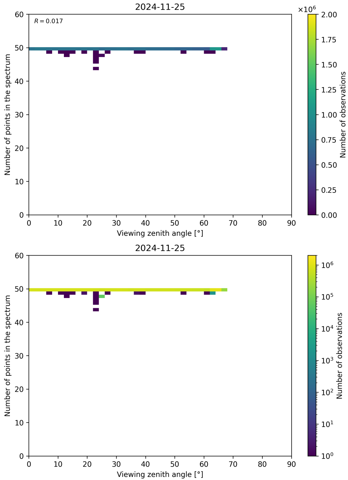
Figure 125: Scatter density plot of “Viewing zenith angle” against “Number of points in the spectrum” for 2024-11-25 to 2024-11-26.
