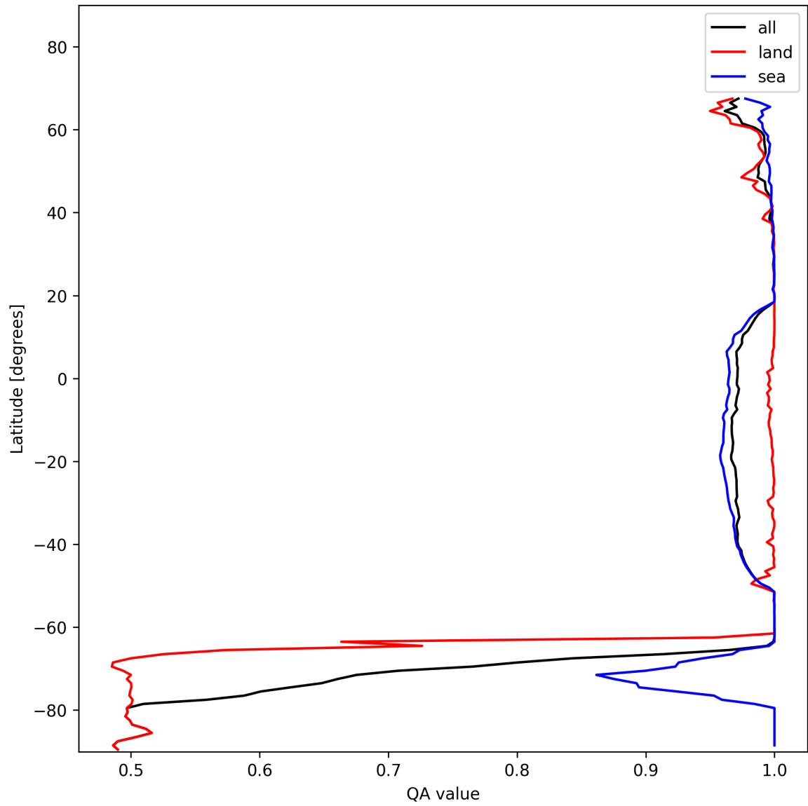
Figure 12: Zonal average of “QA value” for 2024-11-25 to 2024-11-26.
