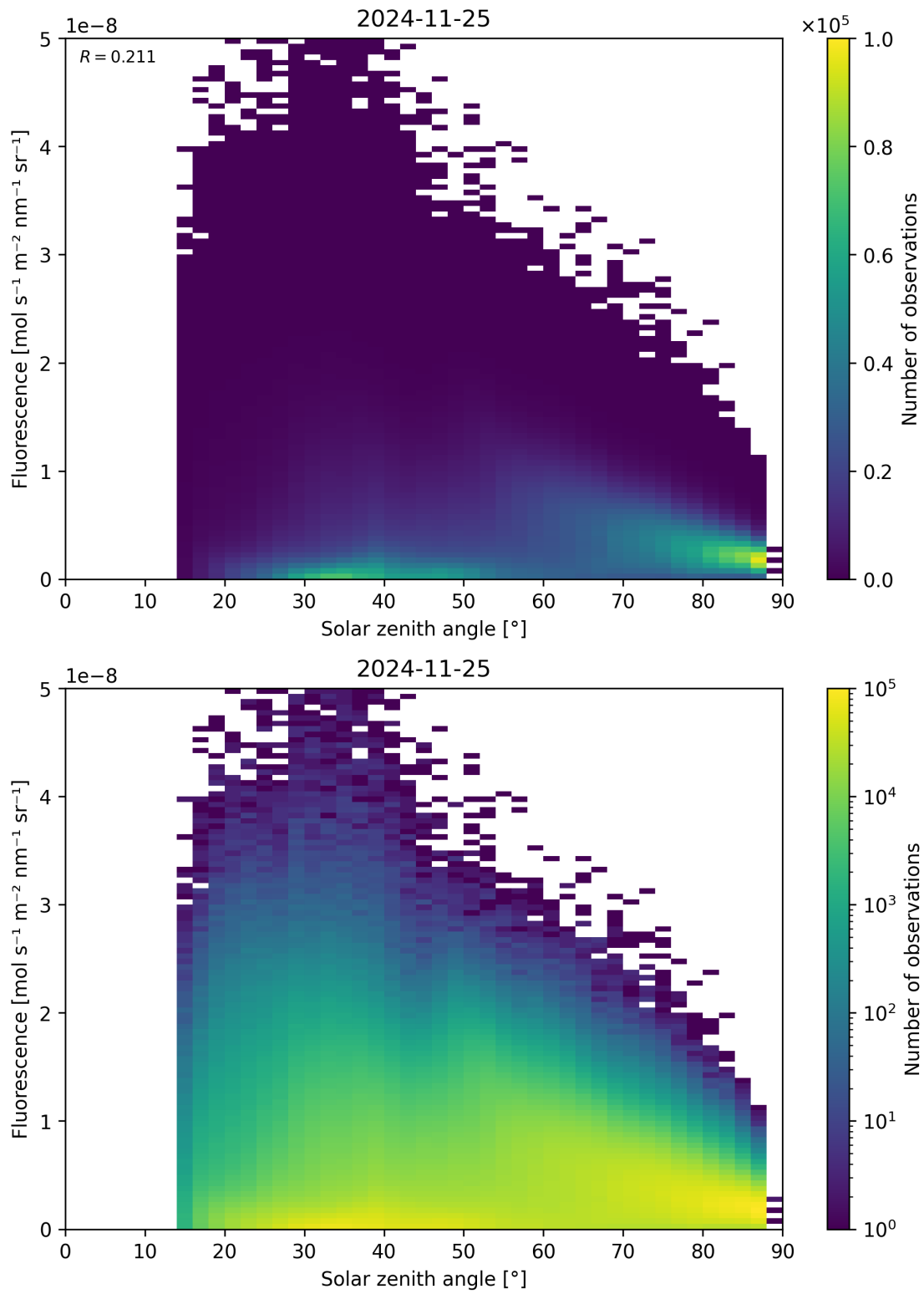
Figure 112: Scatter density plot of “Solar zenith angle” against “Fluorescence” for 2024-11-25 to 2024-11-26.
