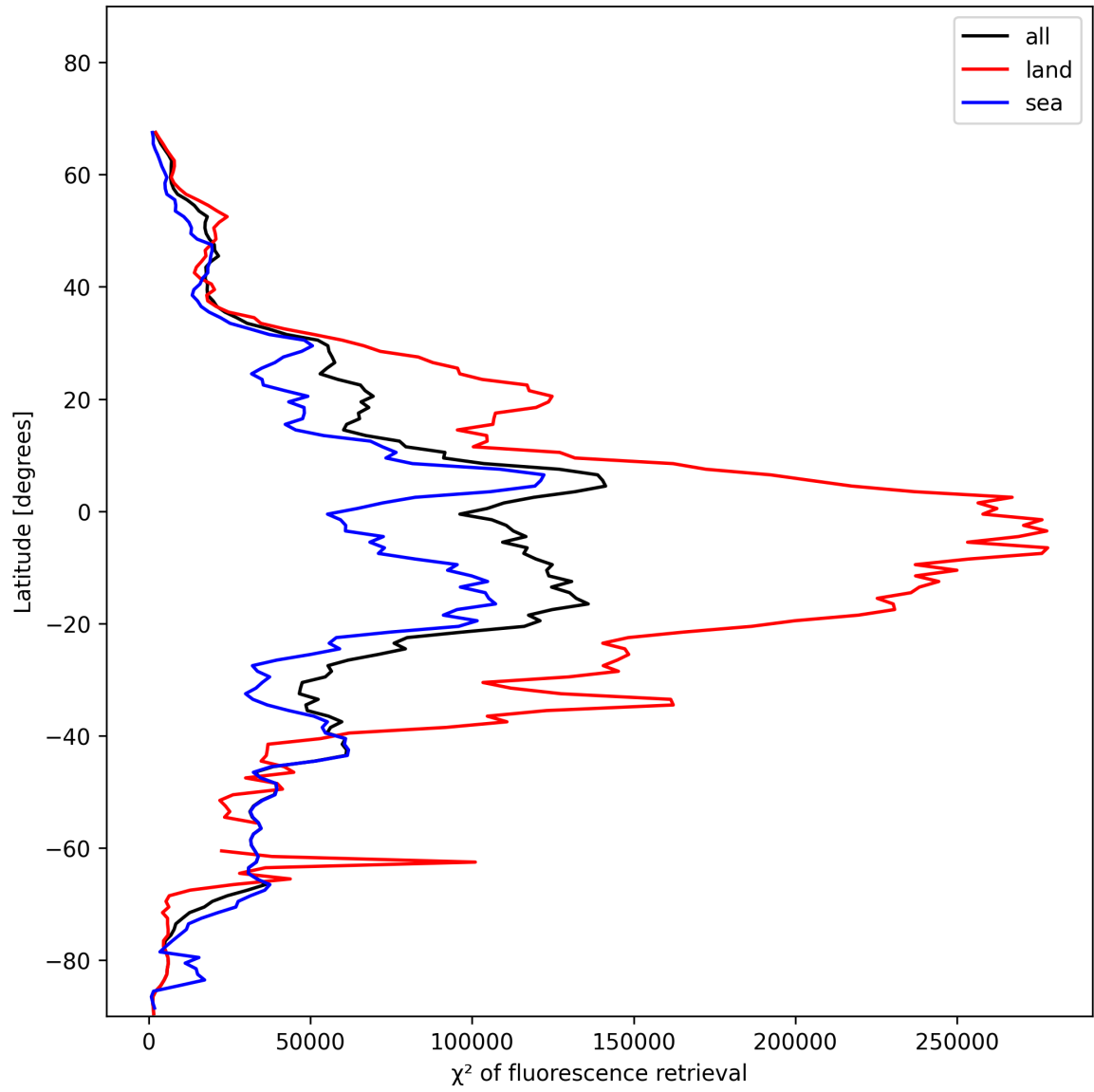
Figure 25: Zonal average of “ \chi^2 of fluorescence retrieval” for 2024-11-25 to 2024-11-26.
