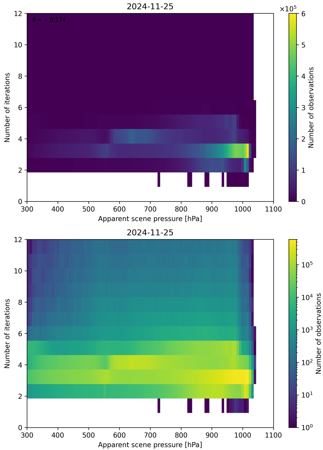
Figure 65: Scatter density plot of “Apparent scene pressure” against “Number of iterations” for 2024-11-25 to 2024-11-26.
