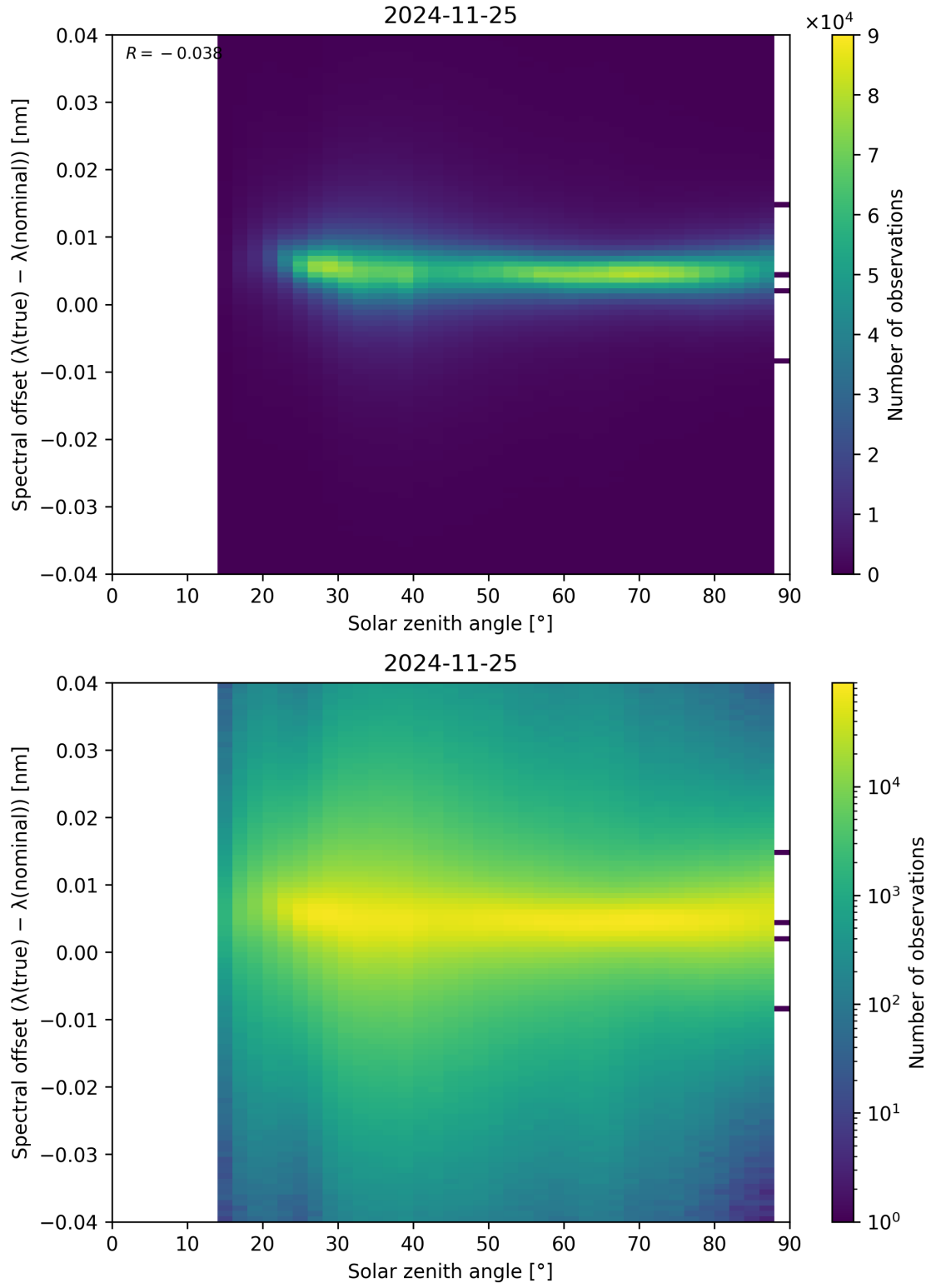
Figure 117: Scatter density plot of “Solar zenith angle” against “Spectral offset ( \lambda_{\text{true}} - \lambda_{\text{nominal}} )” for 2024-11-25 to 2024-11-26.
