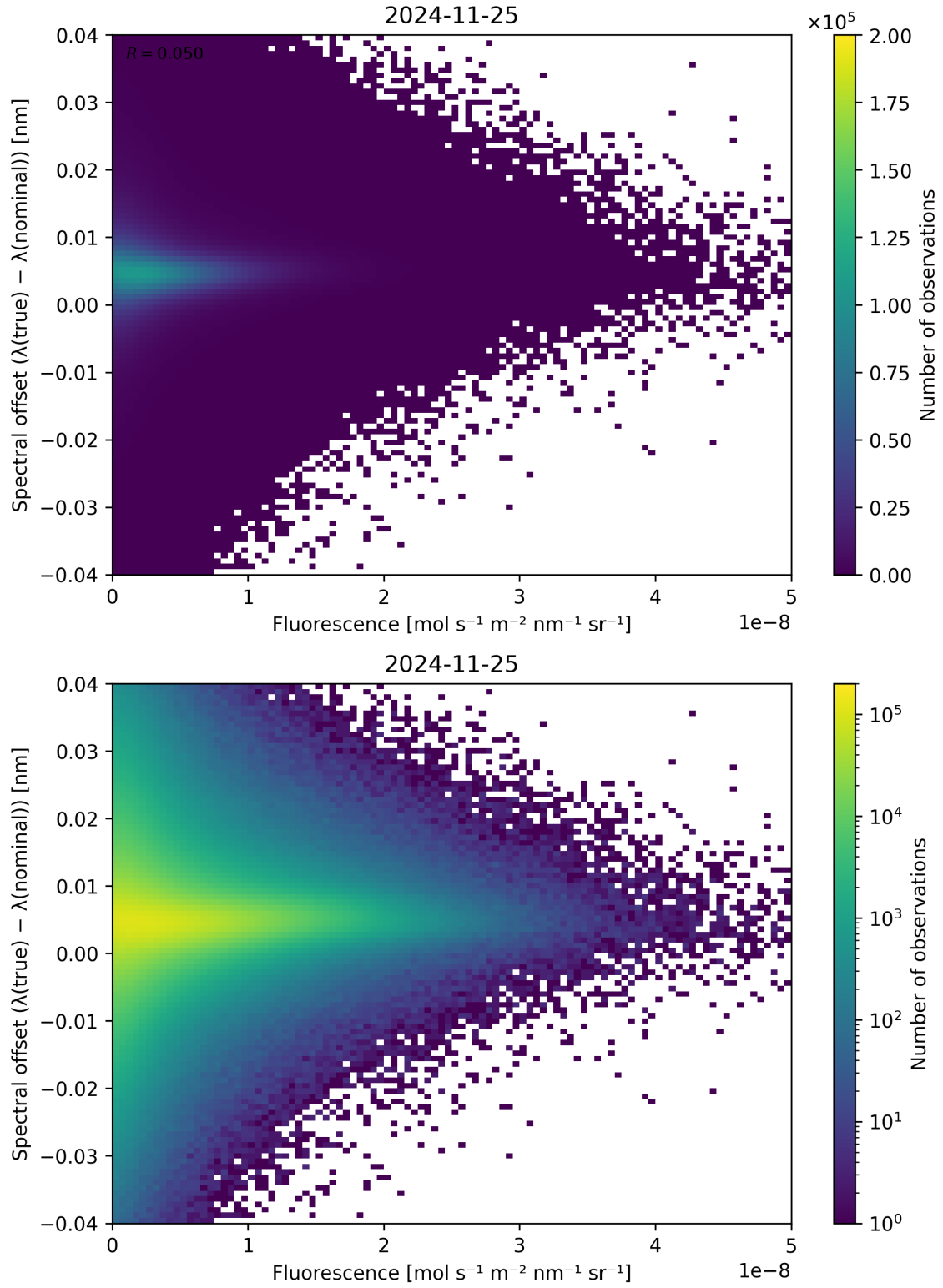
Figure 87: Scatter density plot of “Fluorescence” against “Spectral offset ( \lambda_{\text{true}} - \lambda_{\text{nominal}} )” for 2024-11-25 to 2024-11-26.
