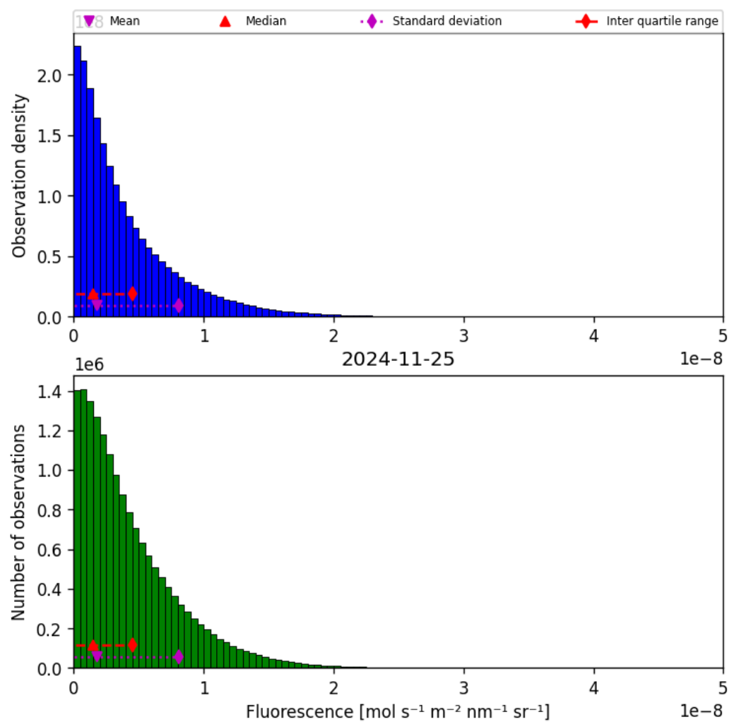
Figure 40: Histogram of “Fluorescence” for 2024-11-25 to 2024-11-26
