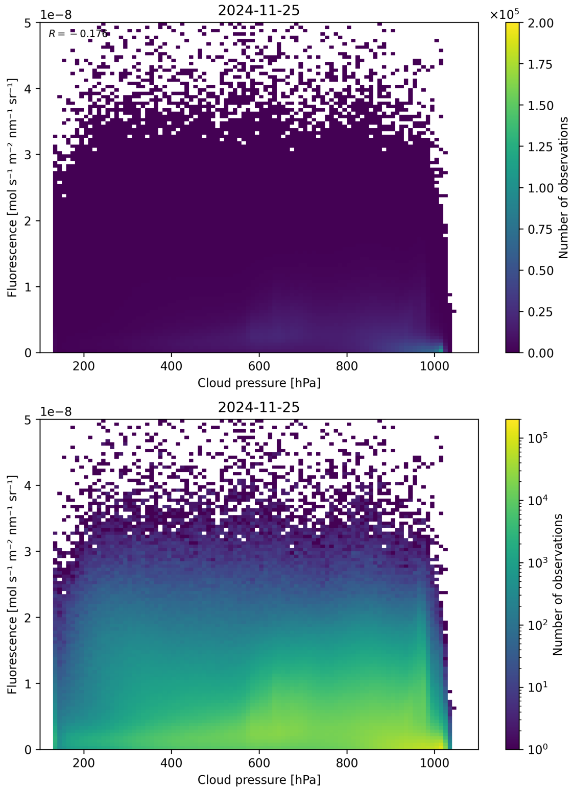
Figure 80: Scatter density plot of “Cloud pressure” against “Fluorescence” for 2024-11-25 to 2024-11-26.
