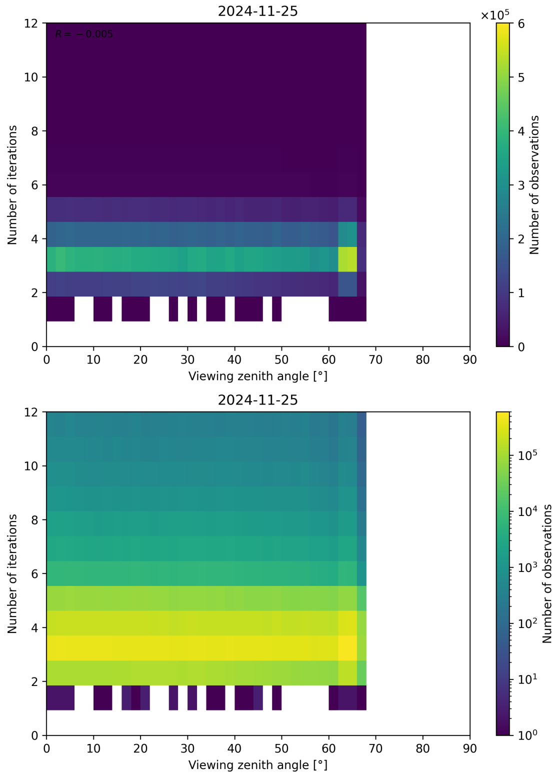
Figure 124: Scatter density plot of “Viewing zenith angle” against “Number of iterations” for 2024-11-25 to 2024-11-26.
