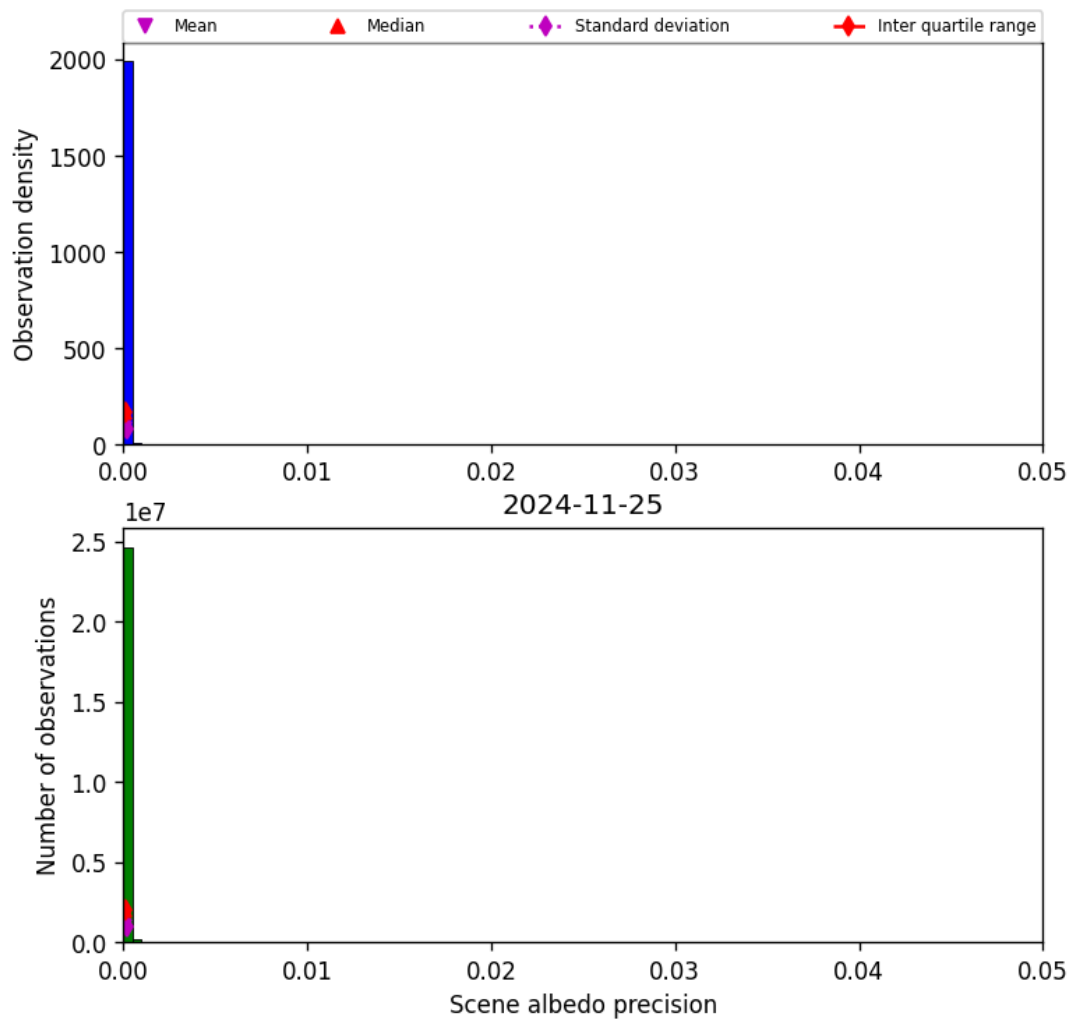
Figure 35: Histogram of “Scene albedo precision” for 2024-11-25 to 2024-11-26
