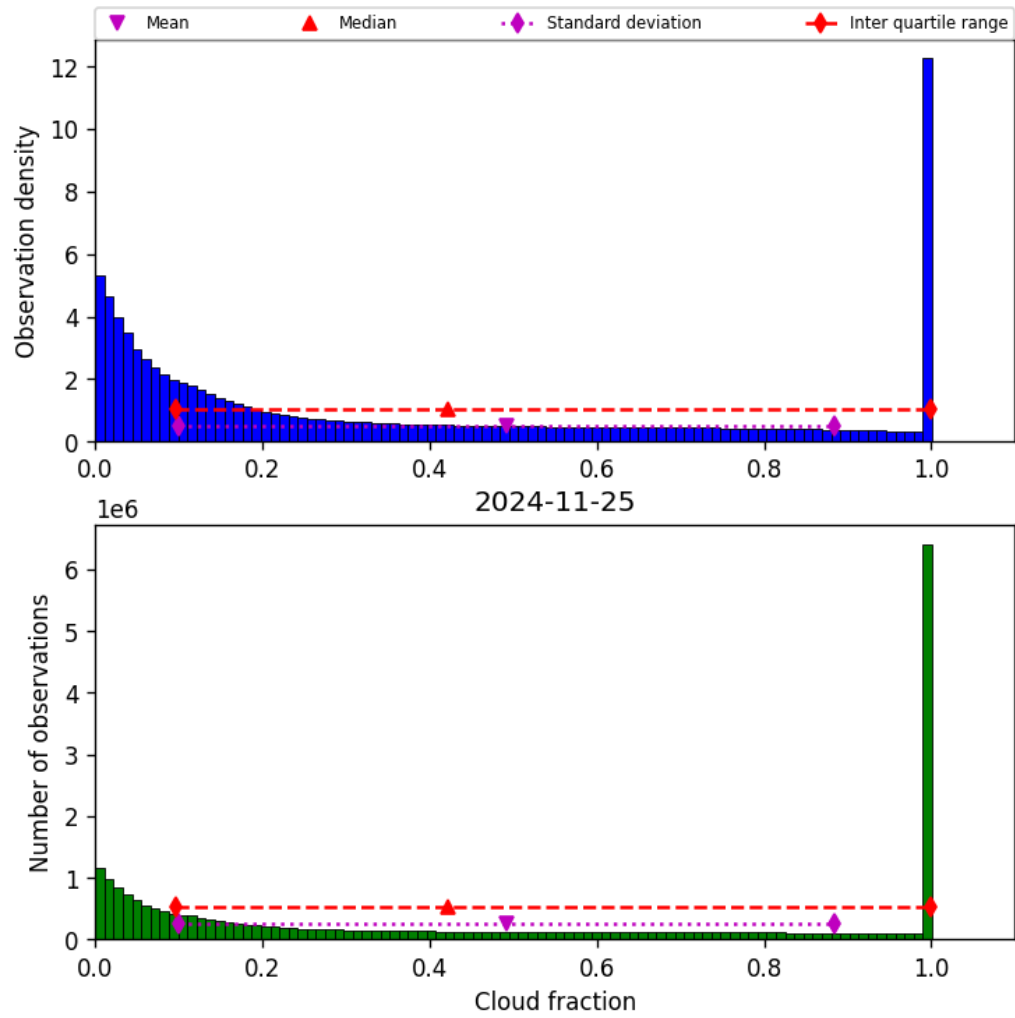
Figure 32: Histogram of “Cloud fraction” for 2024-11-25 to 2024-11-26
