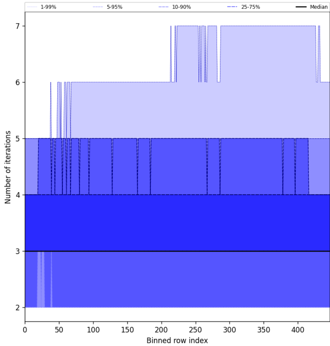
Figure 56: Along track statistics of “Number of iterations” for 2024-11-25 to 2024-11-26
