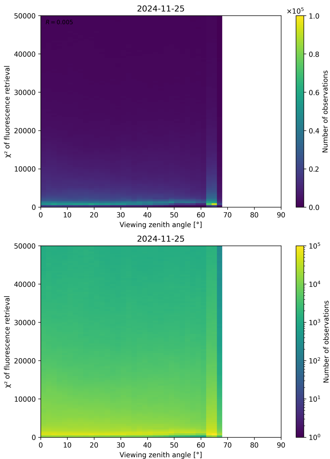
Figure 119: Scatter density plot of “Viewing zenith angle” against “ \chi^2 of fluorescence retrieval” for 2024-11-25 to 2024-11-26.
