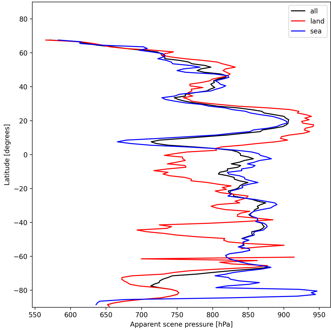
Figure 19: Zonal average of “Apparent scene pressure” for 2024-11-25 to 2024-11-26.
