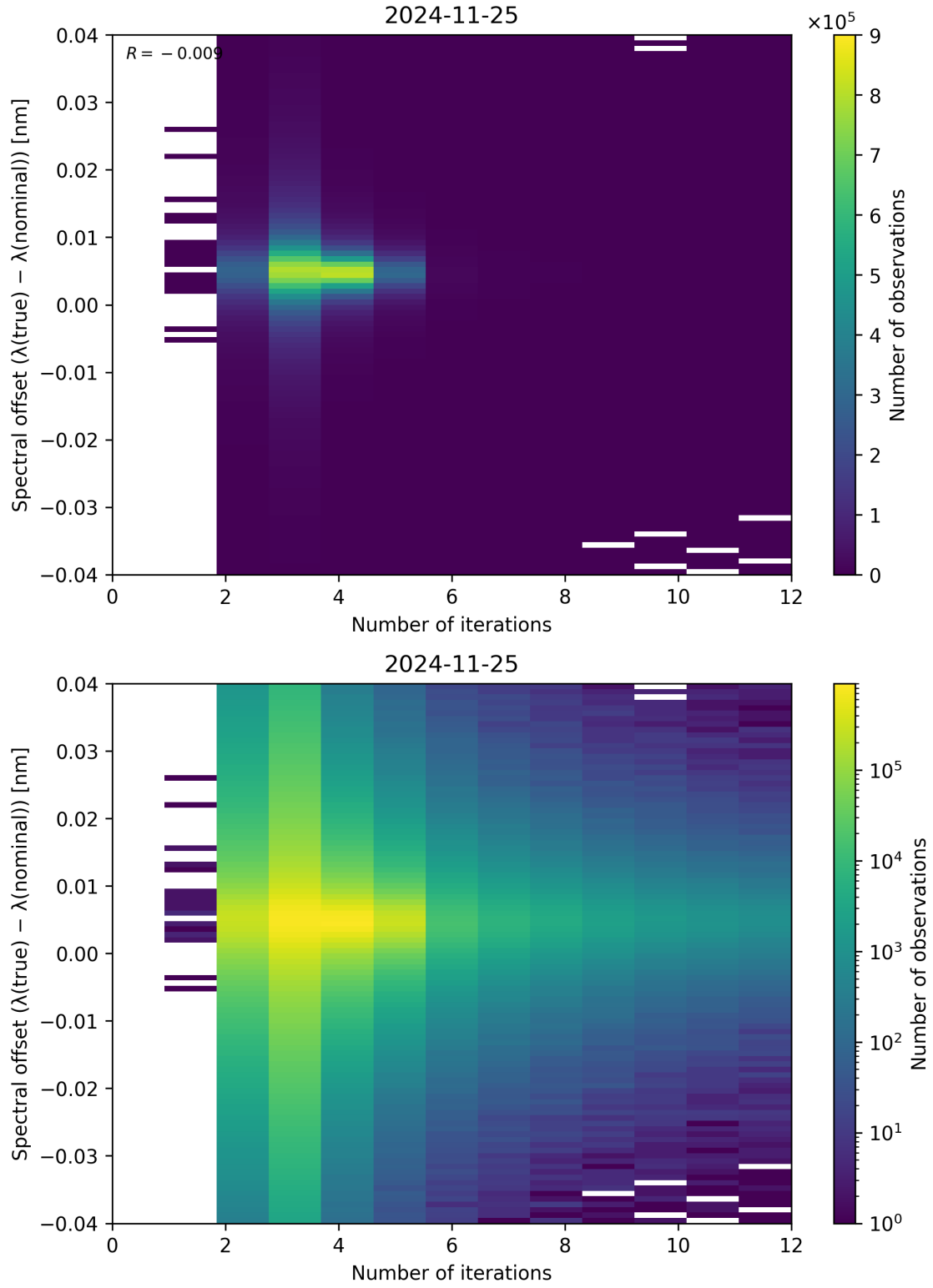
Figure 100: Scatter density plot of “Number of iterations” against “Spectral offset ( \lambda_{\text{true}} - \lambda_{\text{nominal}} )” for 2024-11-25 to 2024-11-26.
