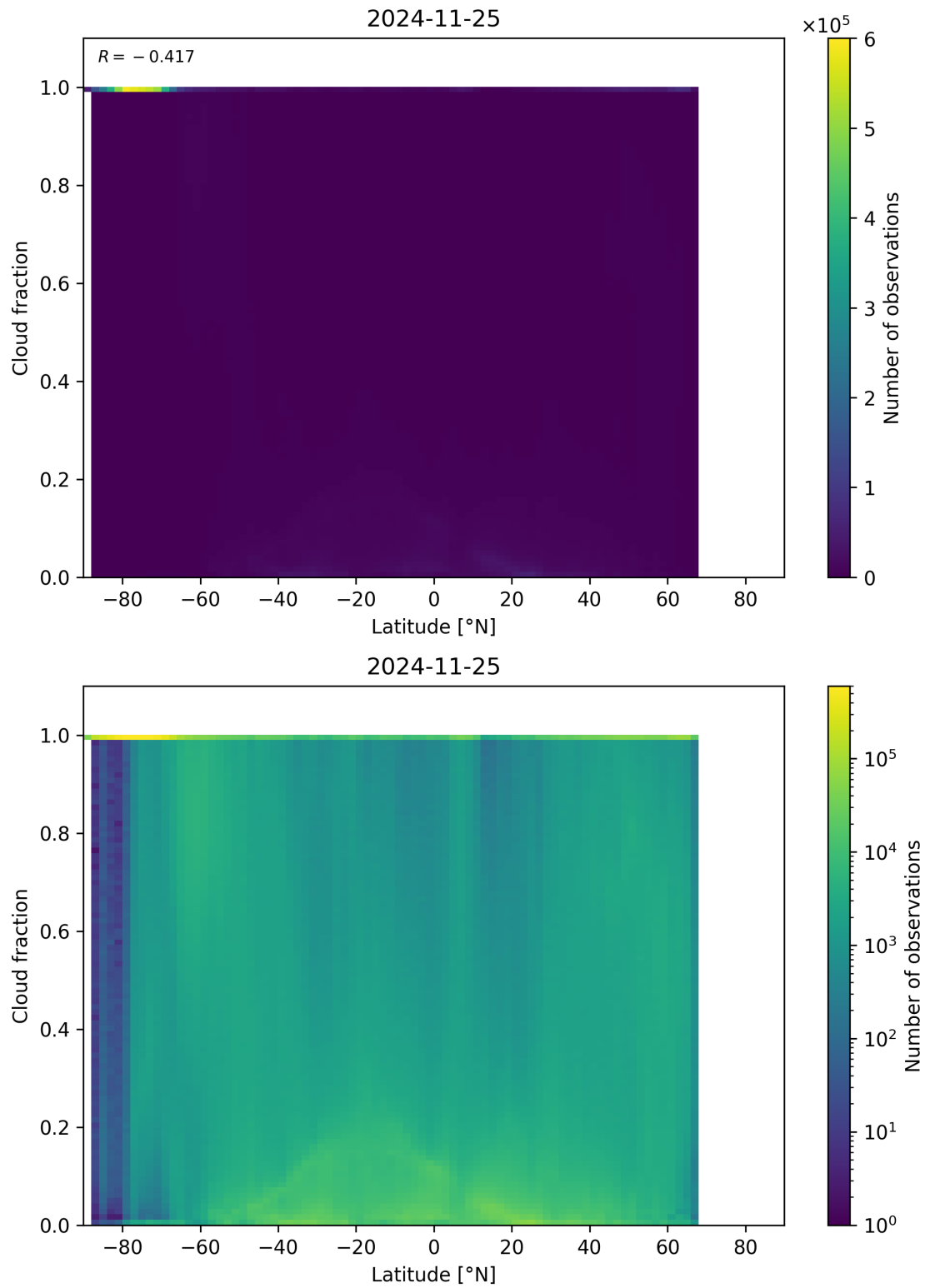
Figure 90: Scatter density plot of “Latitude” against “Cloud fraction” for 2024-11-25 to 2024-11-26.
