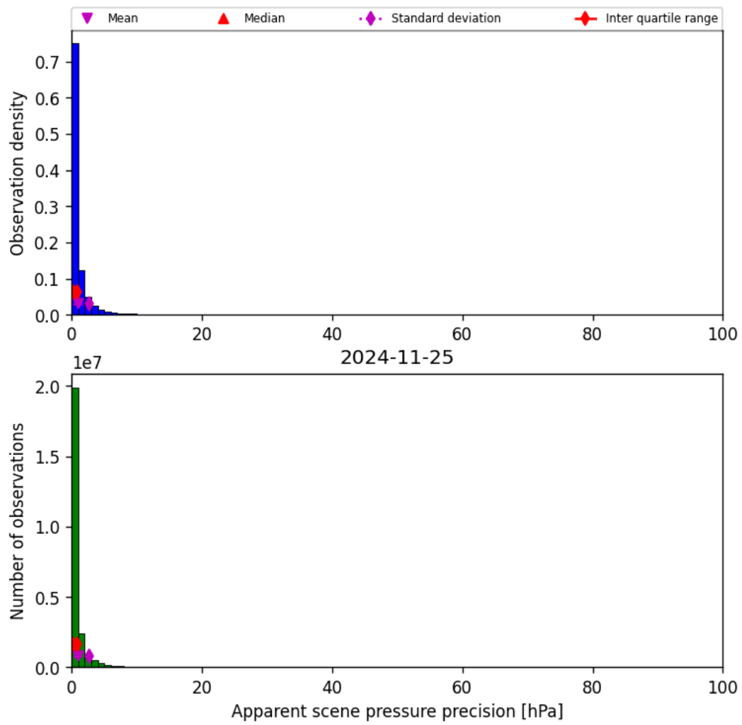
Figure 37: Histogram of “Apparent scene pressure precision” for 2024-11-25 to 2024-11-26
