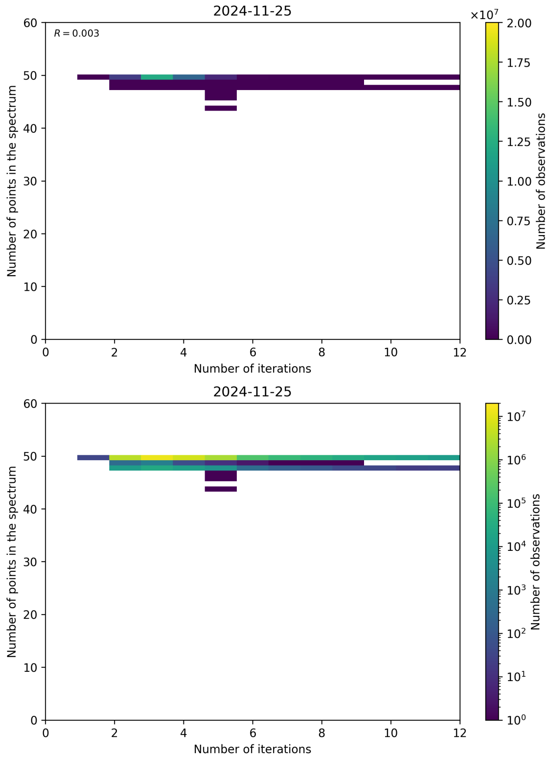
Figure 99: Scatter density plot of “Number of iterations” against “Number of points in the spectrum” for 2024-11-25 to 2024-11-26.
