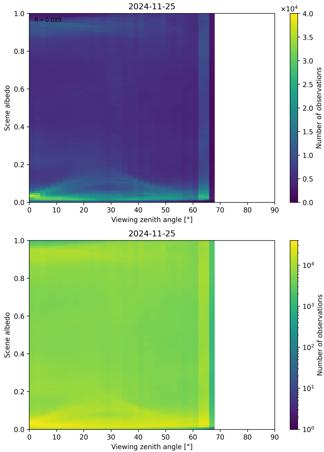
Figure 126: Scatter density plot of “Viewing zenith angle” against “Scene albedo” for 2024-11-25 to 2024-11-26.
