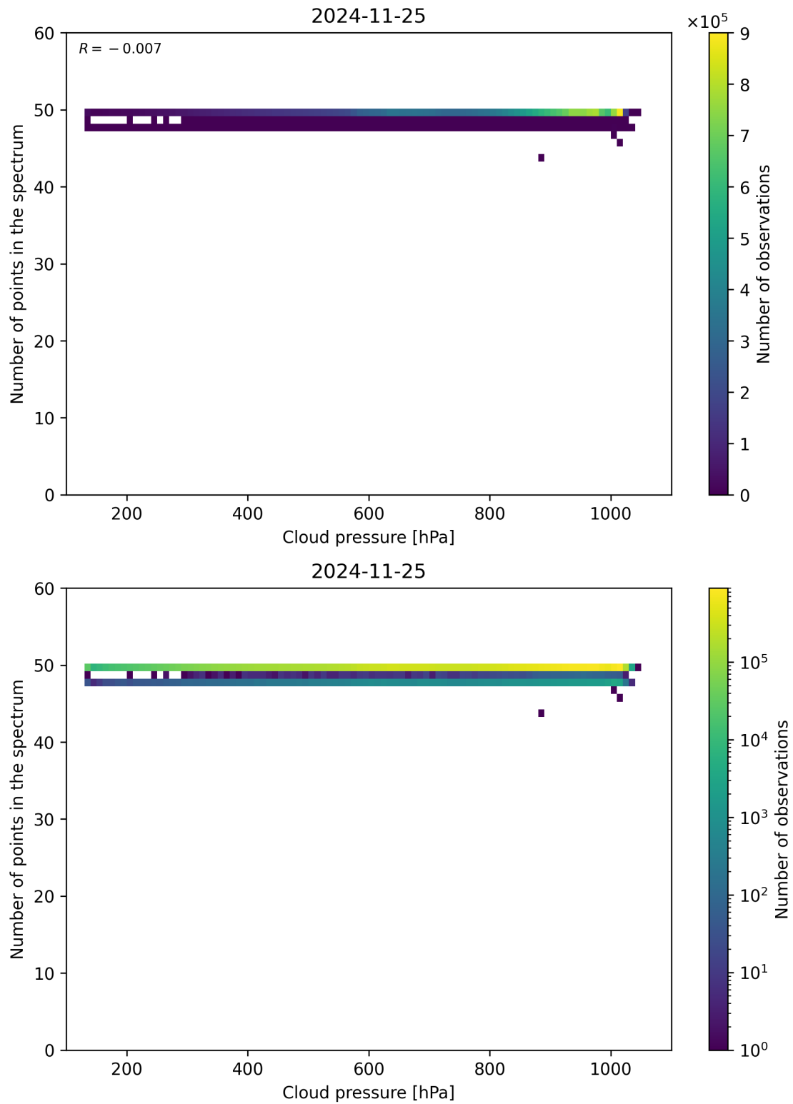
Figure 82: Scatter density plot of “Cloud pressure” against “Number of points in the spectrum” for 2024-11-25 to 2024-11-26.
