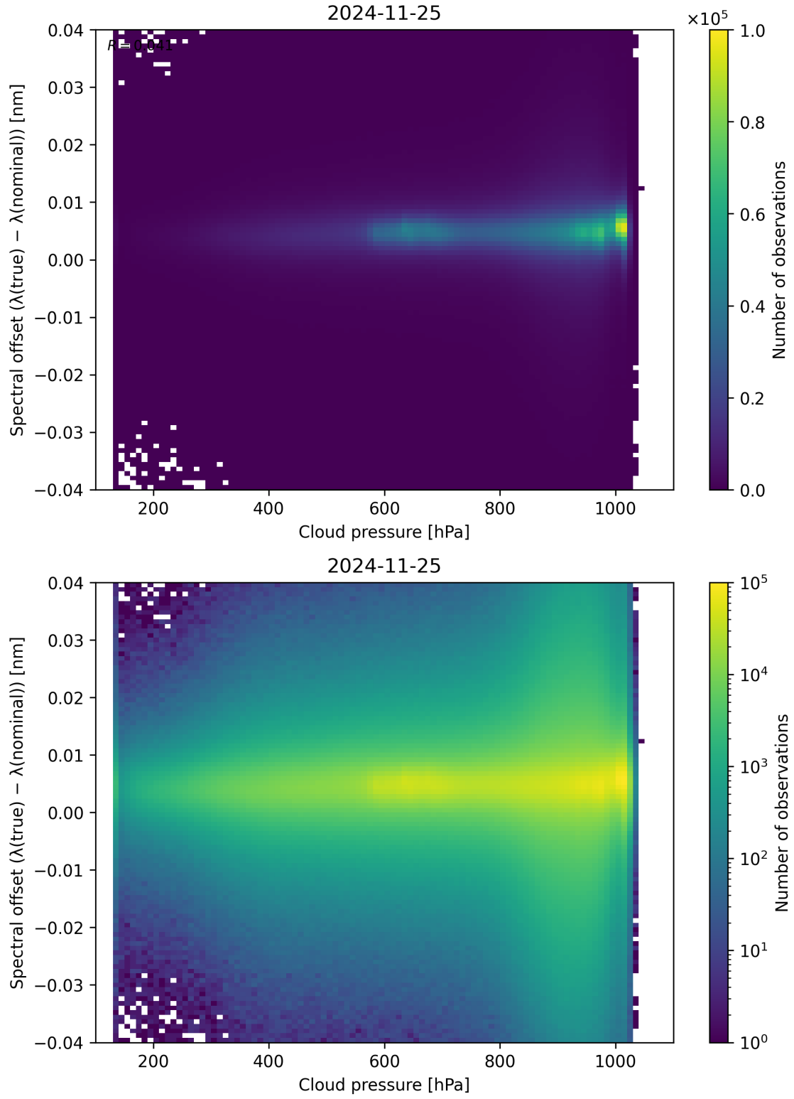
Figure 84: Scatter density plot of “Cloud pressure” against “Spectral offset ( \lambda_{\text{true}} - \lambda_{\text{nominal}} )” for 2024-11-25 to 2024-11-26.
