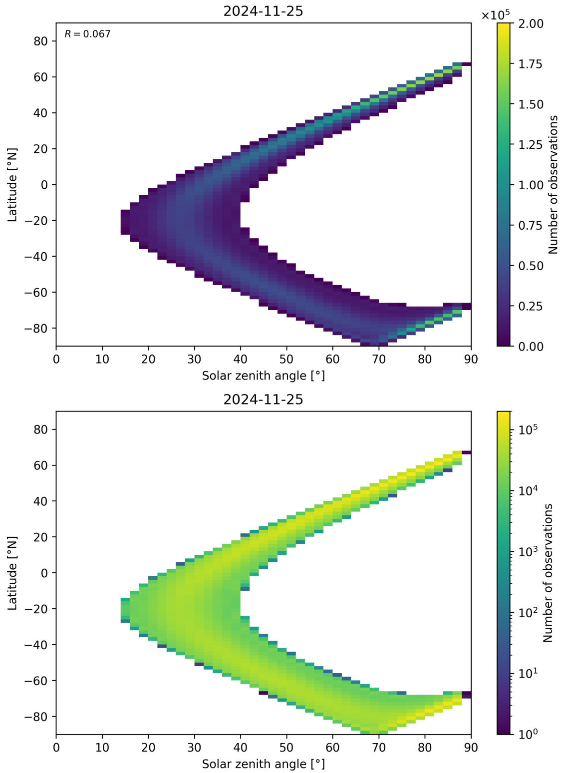
Figure 113: Scatter density plot of “Solar zenith angle” against “Latitude” for 2024-11-25 to 2024-11-26.
