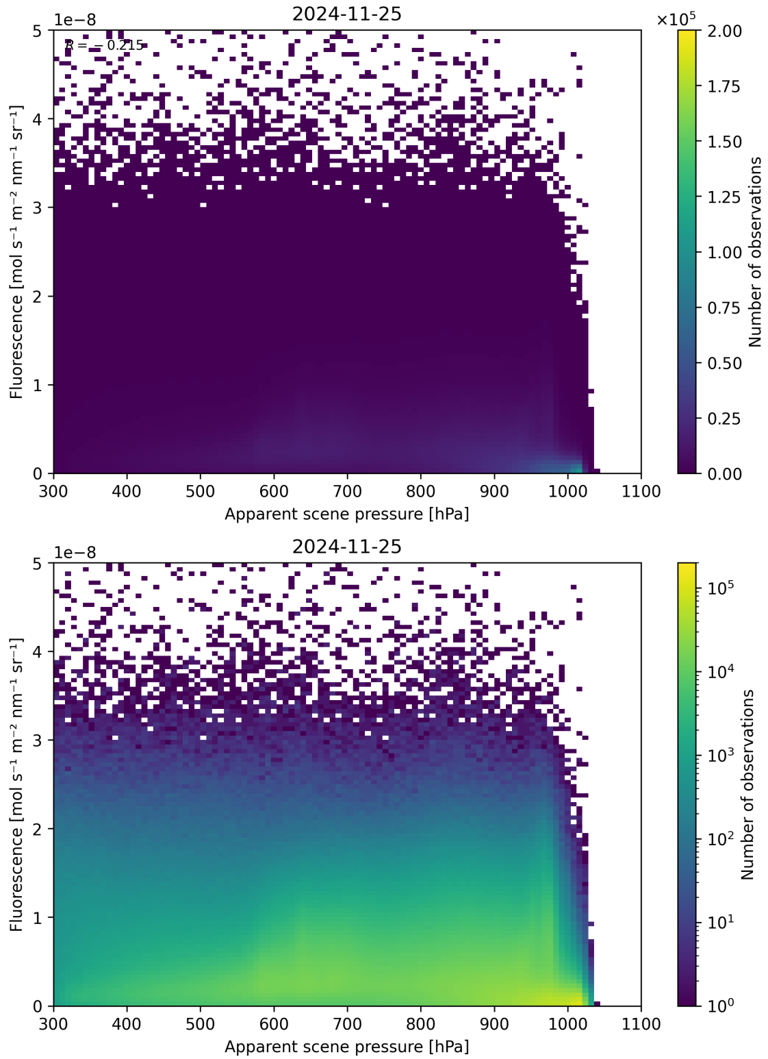
Figure 64: Scatter density plot of “Apparent scene pressure” against “Fluorescence” for 2024-11-25 to 2024-11-26.
