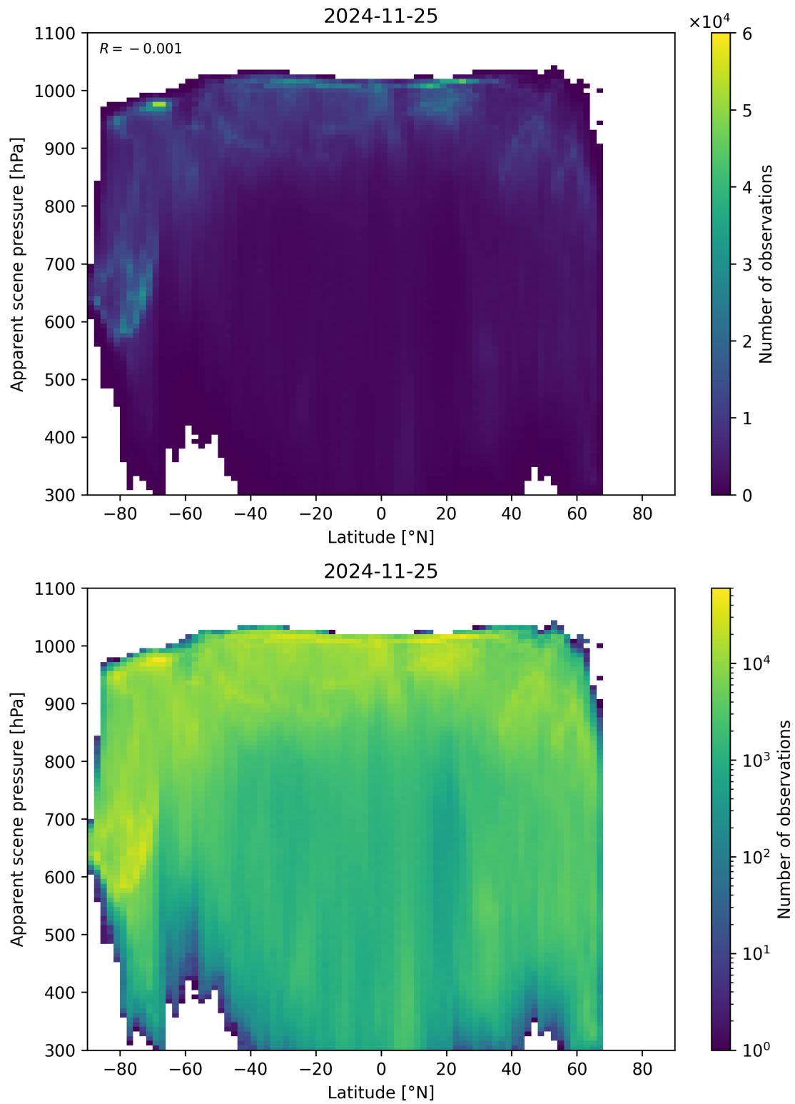
Figure 88: Scatter density plot of “Latitude” against “Apparent scene pressure” for 2024-11-25 to 2024-11-26.
