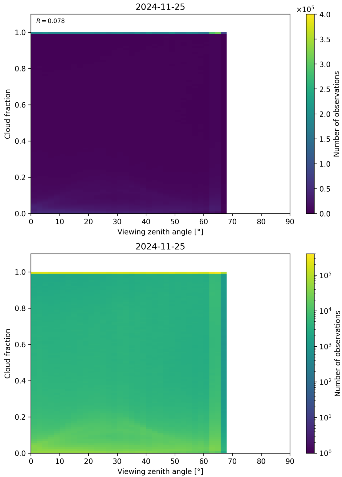
Figure 120: Scatter density plot of “Viewing zenith angle” against “Cloud fraction” for 2024-11-25 to 2024-11-26.
