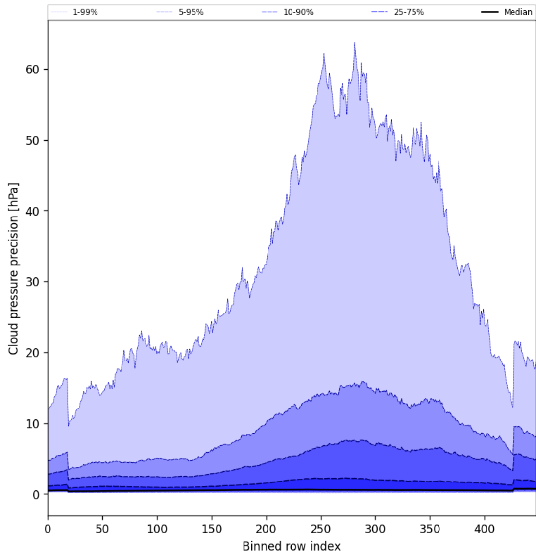
Figure 48: Along track statistics of “Cloud pressure precision” for 2024-11-25 to 2024-11-26
