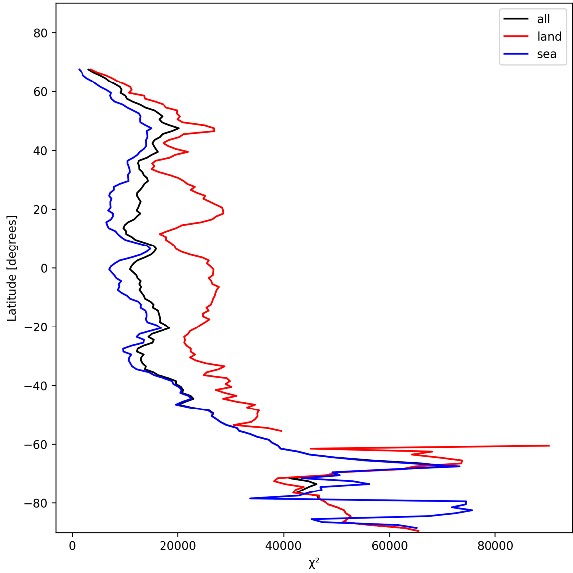
Figure 21: Zonal average of “ \chi^2 ” for 2024-11-25 to 2024-11-26.
