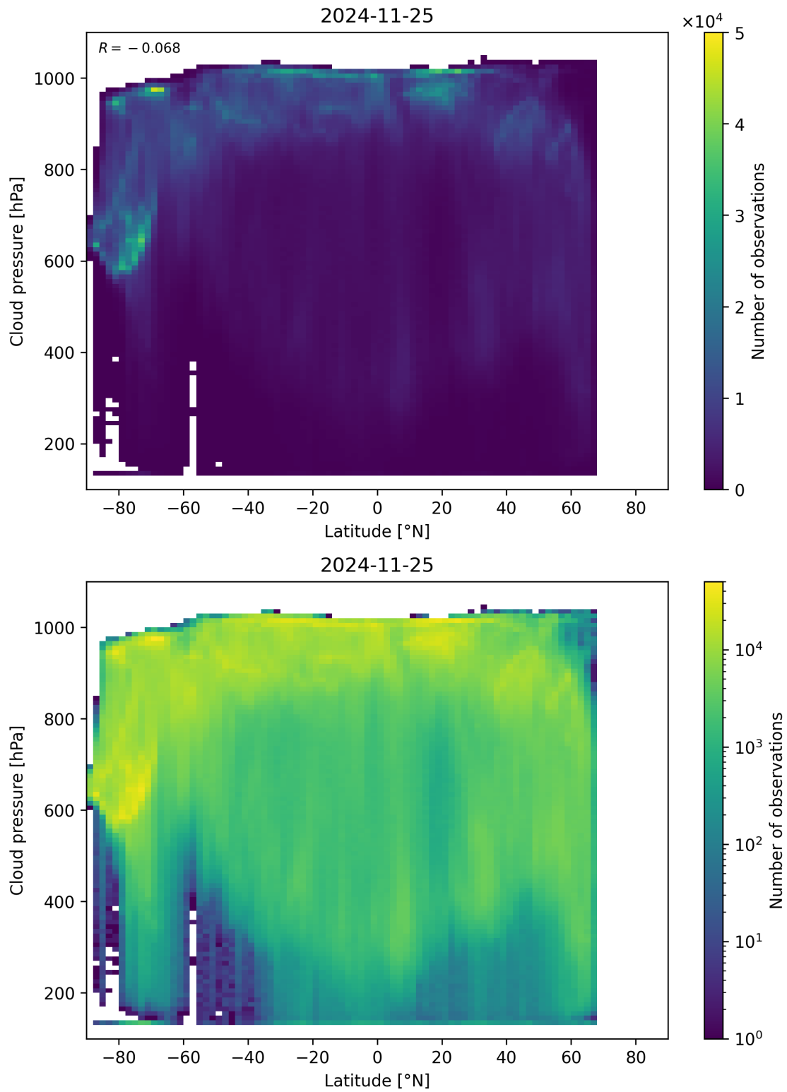
Figure 91: Scatter density plot of “Latitude” against “Cloud pressure” for 2024-11-25 to 2024-11-26.
