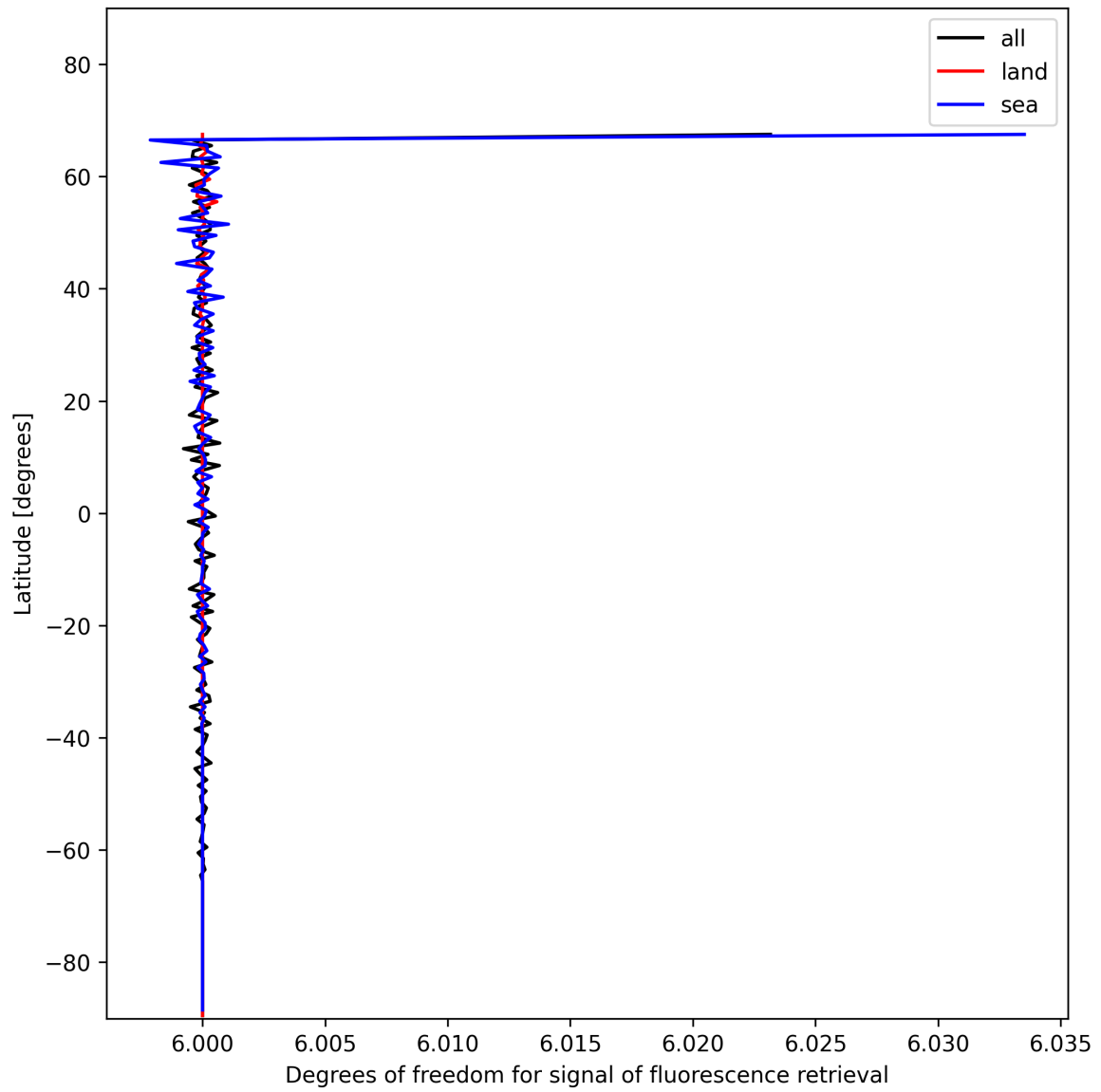
Figure 26: Zonal average of “Degrees of freedom for signal of fluorescence retrieval” for 2024-11-25 to 2024-11-26.
