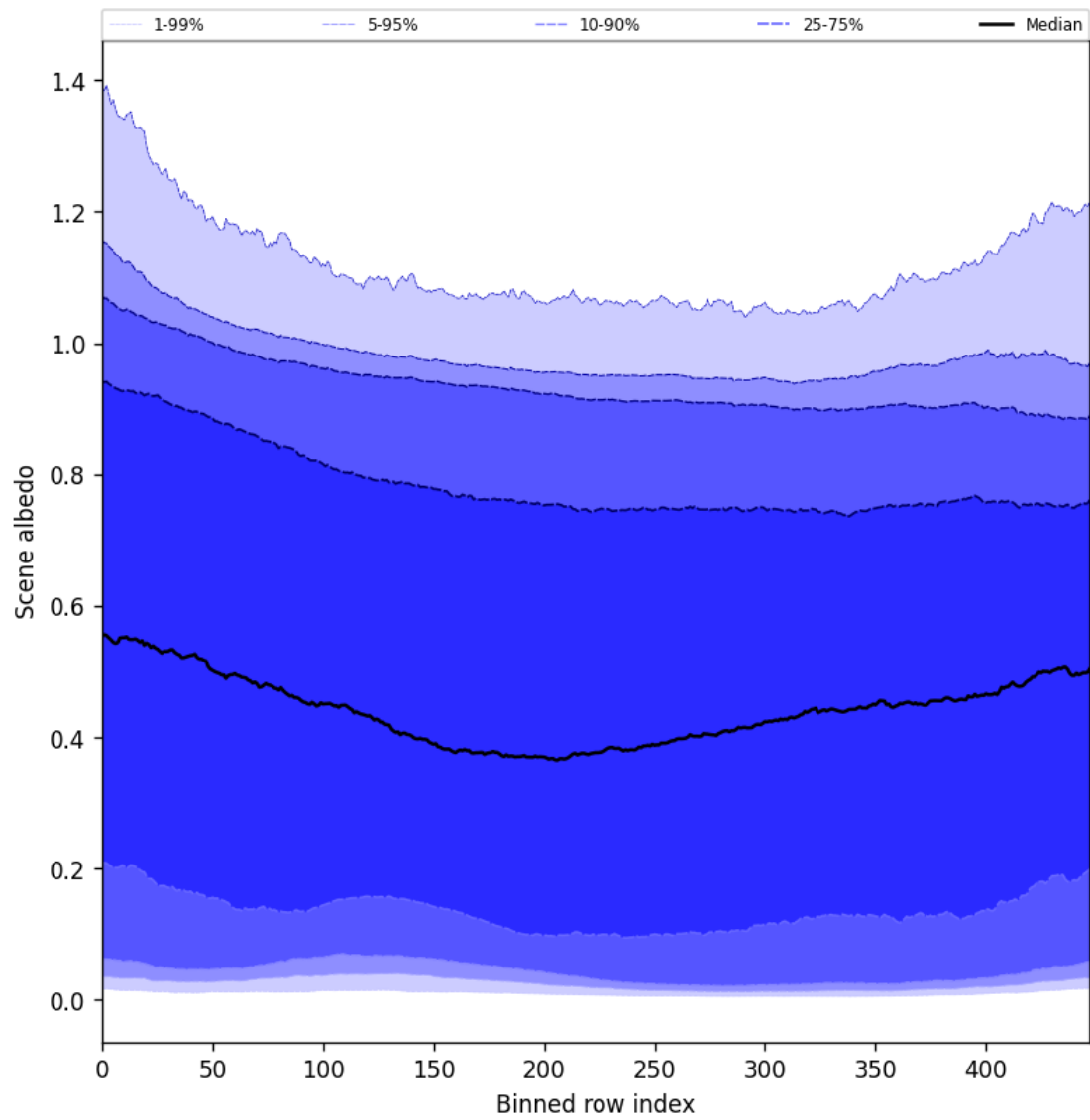
Figure 51: Along track statistics of “Scene albedo” for 2024-11-25 to 2024-11-26
