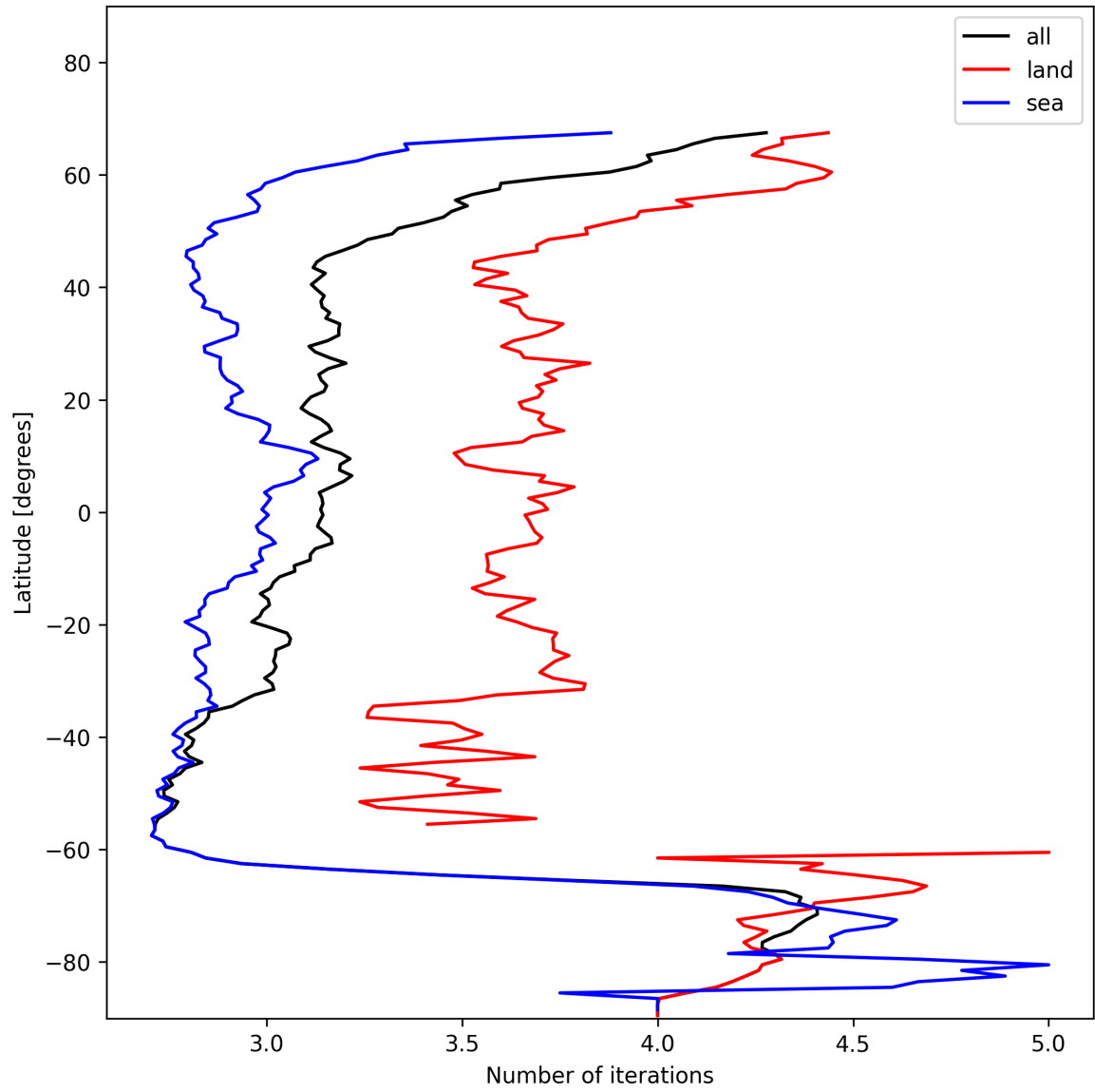
Figure 22: Zonal average of “Number of iterations” for 2024-11-25 to 2024-11-26.
