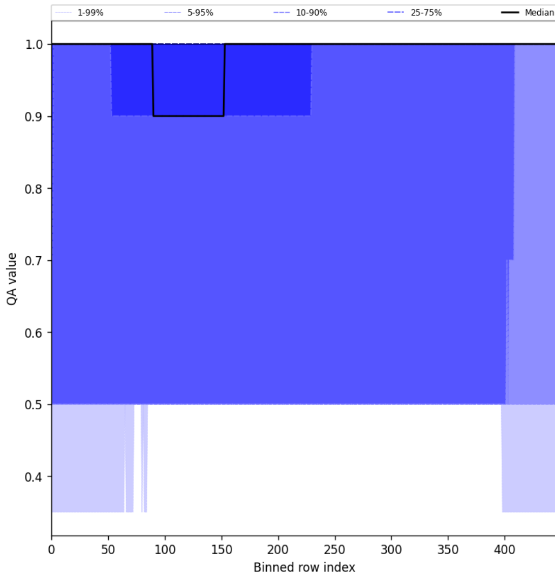
Figure 46: Along track statistics of “QA value” for 2024-11-25 to 2024-11-26
