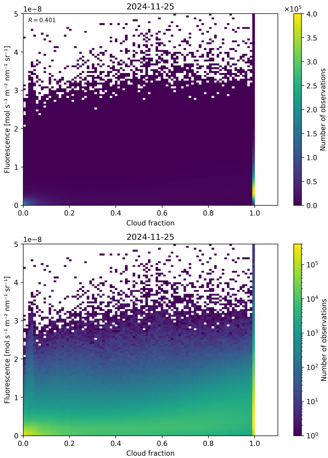
Figure 72: Scatter density plot of “Cloud fraction” against “Fluorescence” for 2024-11-25 to 2024-11-26.
