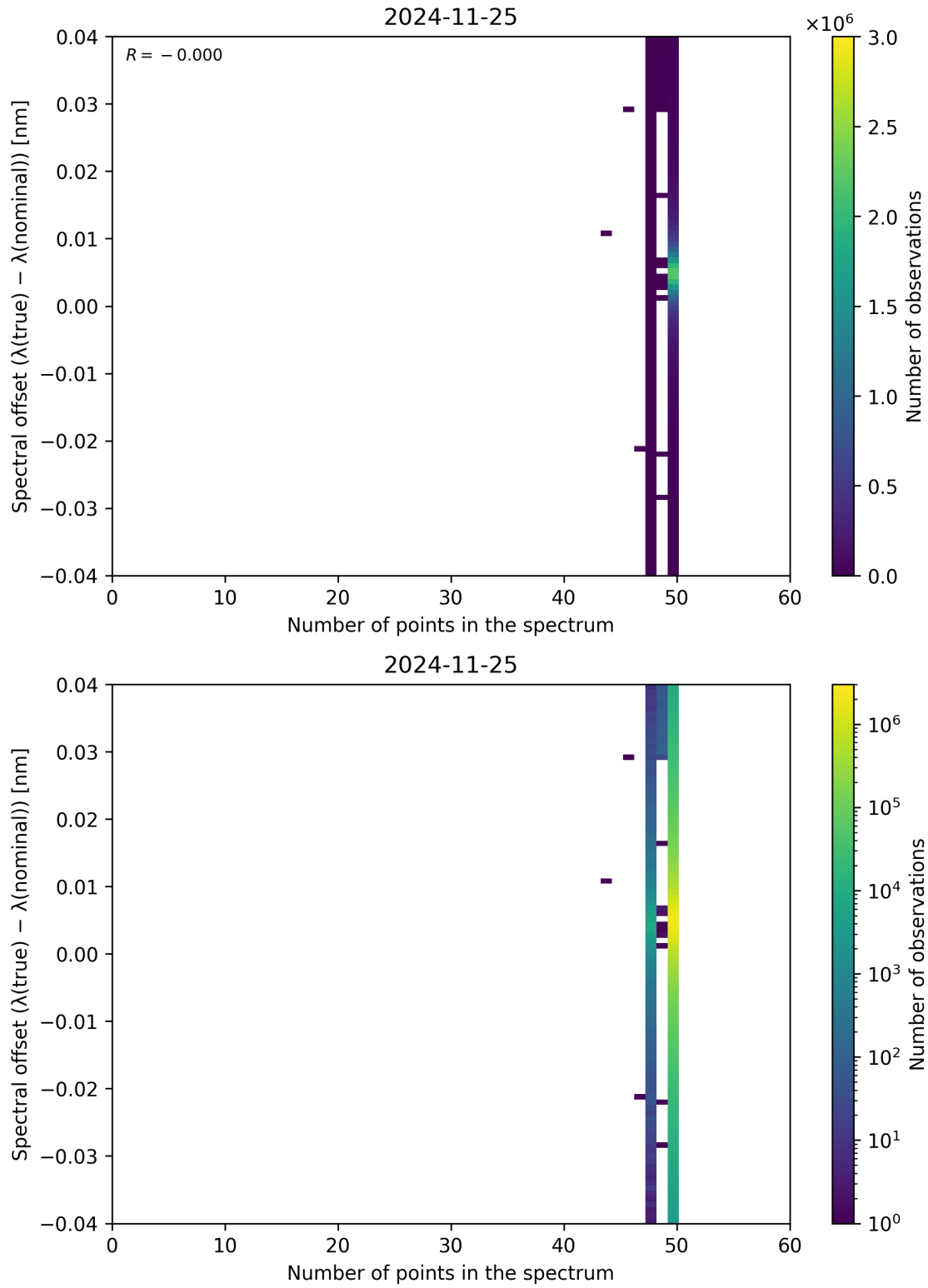
Figure 101: Scatter density plot of “Number of points in the spectrum” against “Spectral offset ( \lambda_{\text{true}} - \lambda_{\text{nominal}} )” for 2024-11-25 to 2024-11-26.
