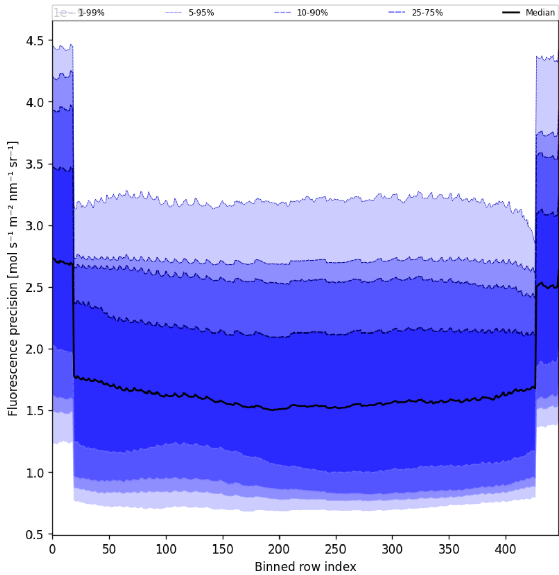
Figure 58: Along track statistics of “Fluorescence precision” for 2024-11-25 to 2024-11-26
