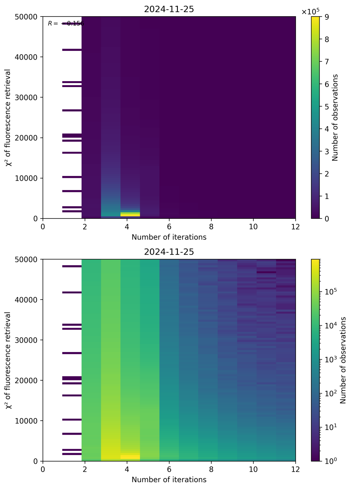
Figure 97: Scatter density plot of “Number of iterations” against “ \chi^2 of fluorescence retrieval” for 2024-11-25 to 2024-11-26.
