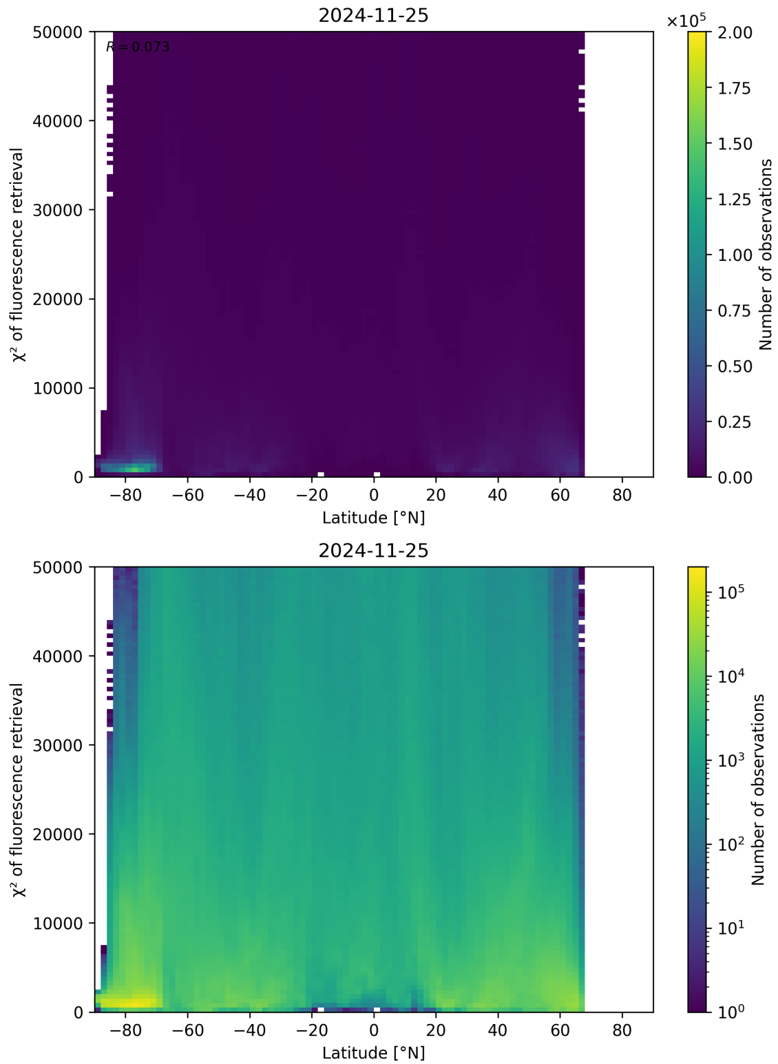
Figure 89: Scatter density plot of “Latitude” against “ \chi^2 of fluorescence retrieval” for 2024-11-25 to 2024-11-26.
