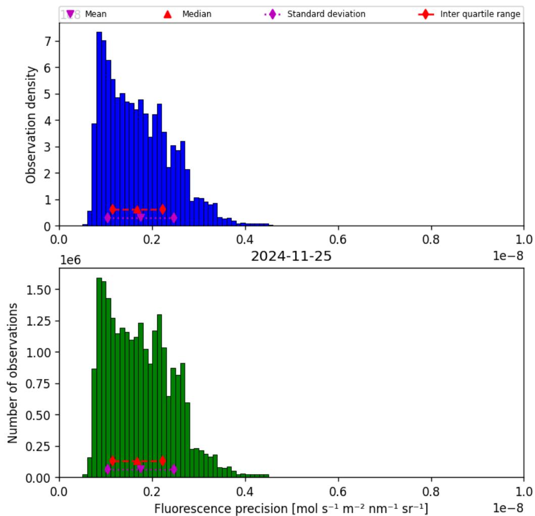
Figure 41: Histogram of “Fluorescence precision” for 2024-11-25 to 2024-11-26
