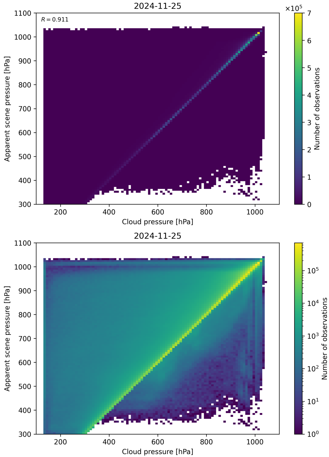
Figure 77: Scatter density plot of “Cloud pressure” against “Apparent scene pressure” for 2024-11-25 to 2024-11-26.
