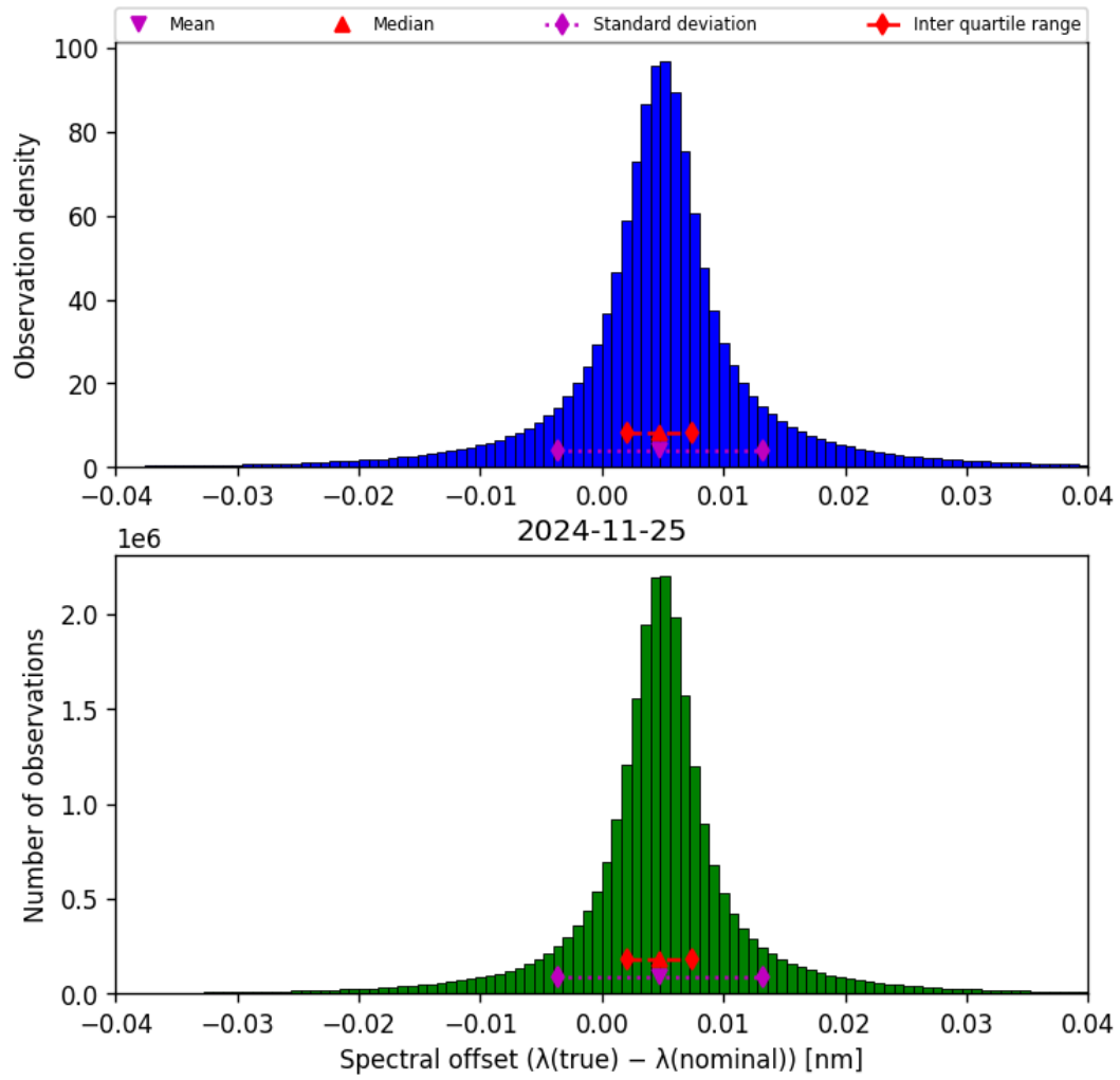
Figure 45: Histogram of “Spectral offset ( \lambda_{\text{true}} - \lambda_{\text{nominal}} )” for 2024-11-25 to 2024-11-26
