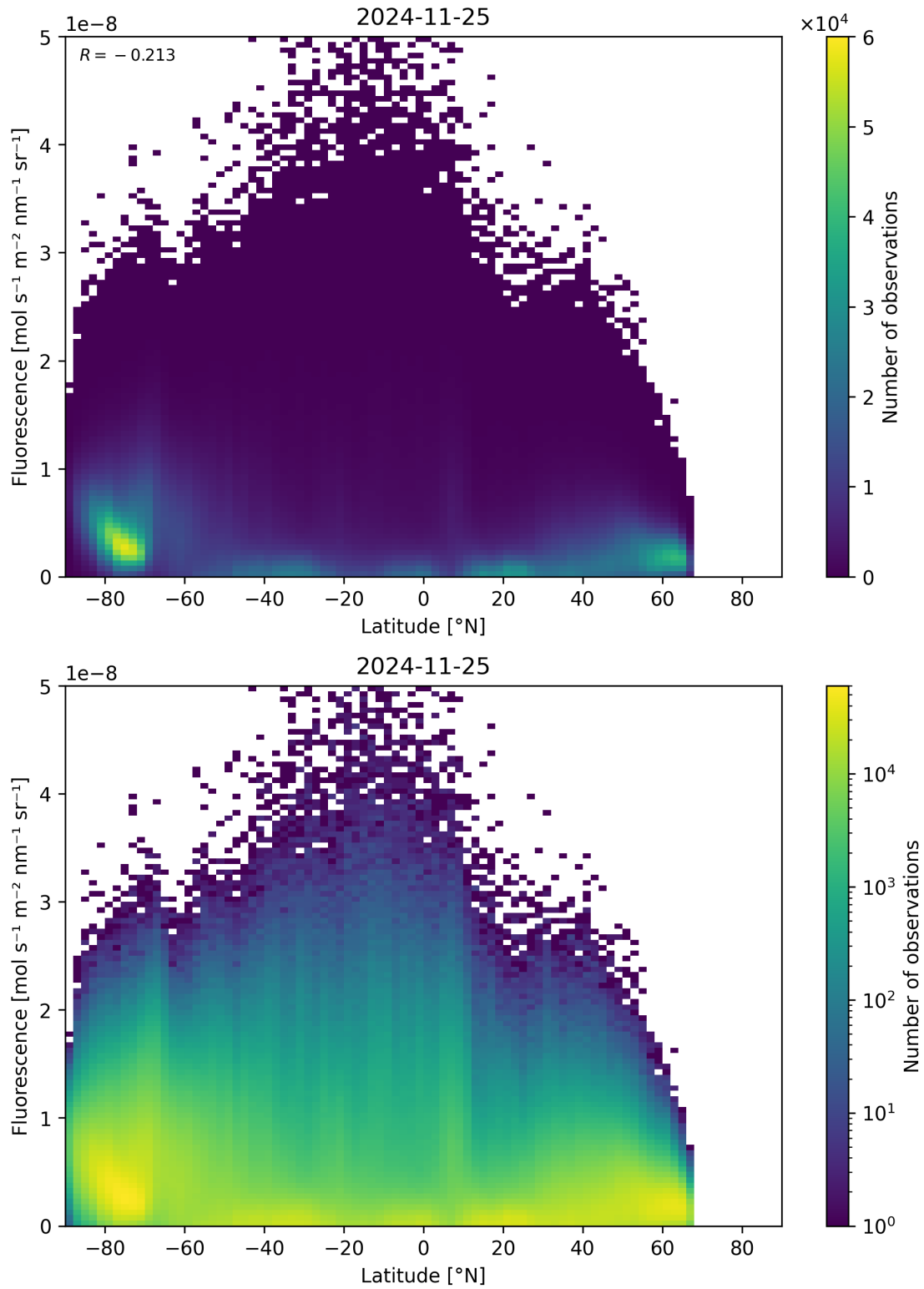
Figure 92: Scatter density plot of “Latitude” against “Fluorescence” for 2024-11-25 to 2024-11-26.
