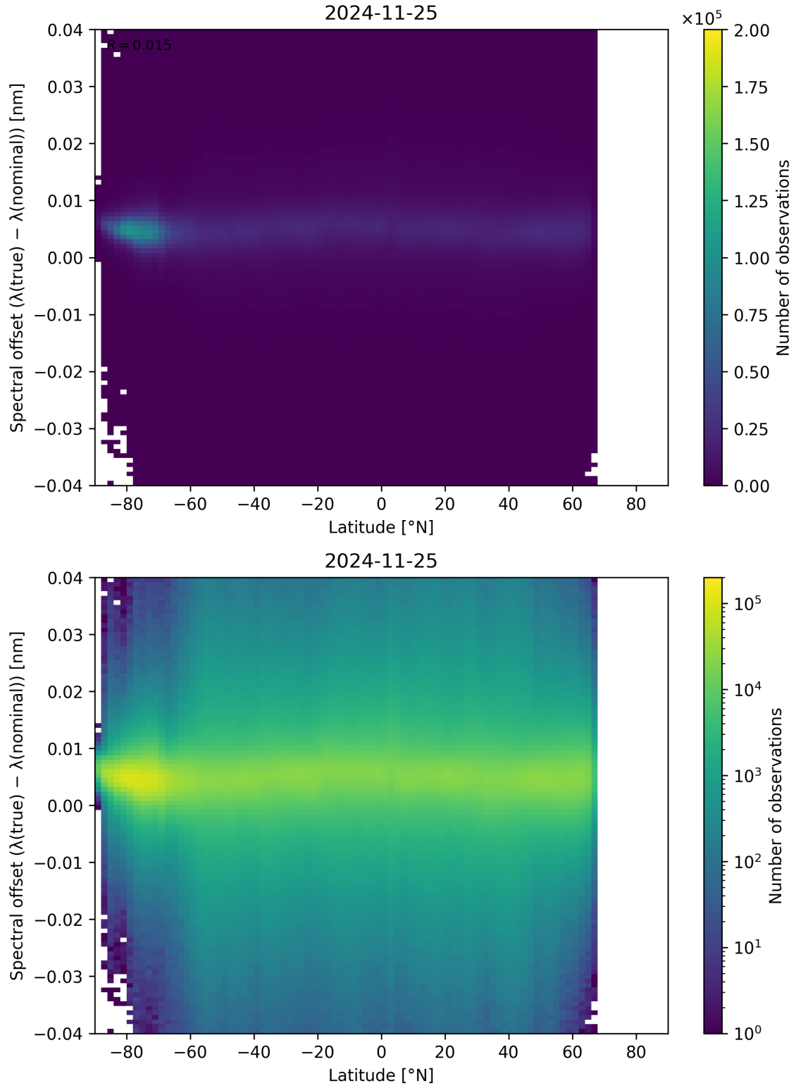
Figure 96: Scatter density plot of “Latitude” against “Spectral offset ( \lambda_{\text{true}} - \lambda_{\text{nominal}} )” for 2024-11-25 to 2024-11-26.
