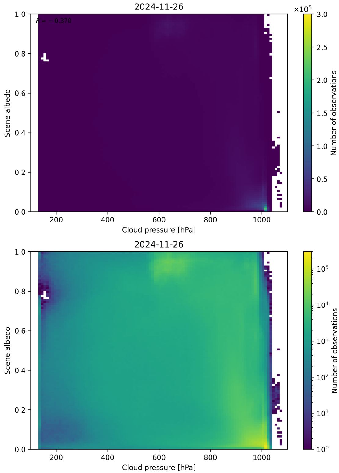
Figure 83: Scatter density plot of “Cloud pressure” against “Scene albedo” for 2024-11-25 to 2024-11-27.
