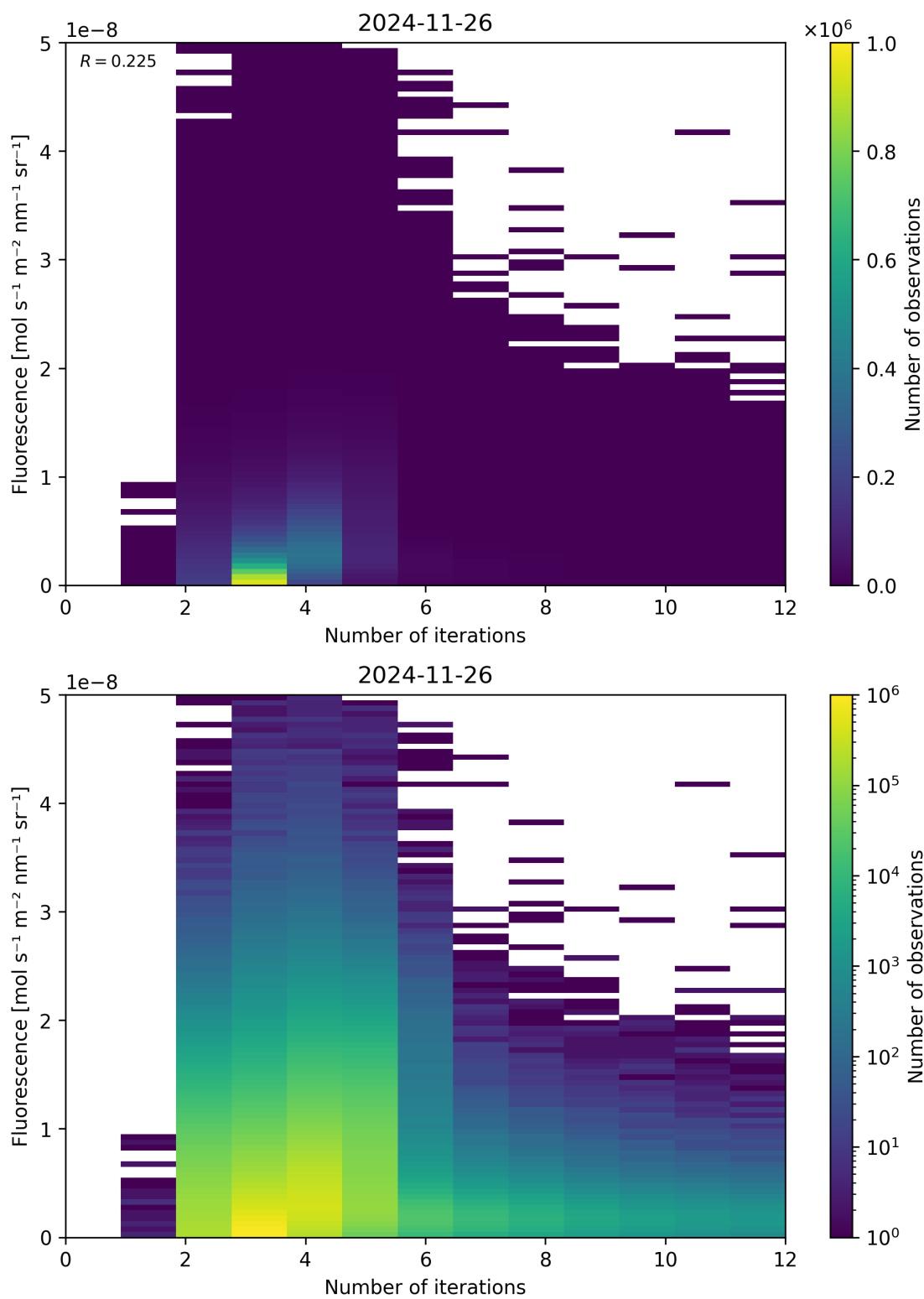
Figure 98: Scatter density plot of “Number of iterations” against “Fluorescence” for 2024-11-25 to 2024-11-27.
