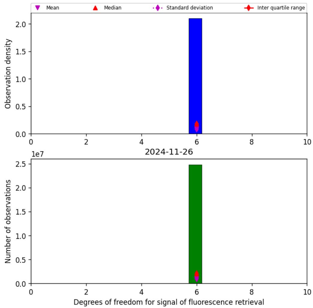
Figure 43: Histogram of “Degrees of freedom for signal of fluorescence retrieval” for 2024-11-25 to 2024-11-27
