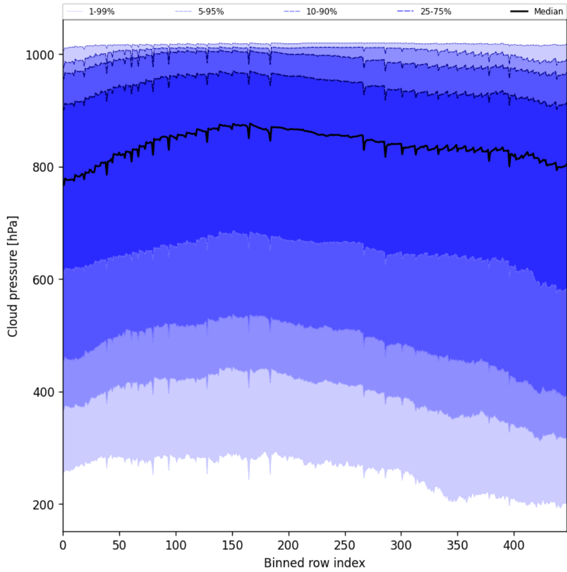
Figure 47: Along track statistics of “Cloud pressure” for 2024-11-25 to 2024-11-27
