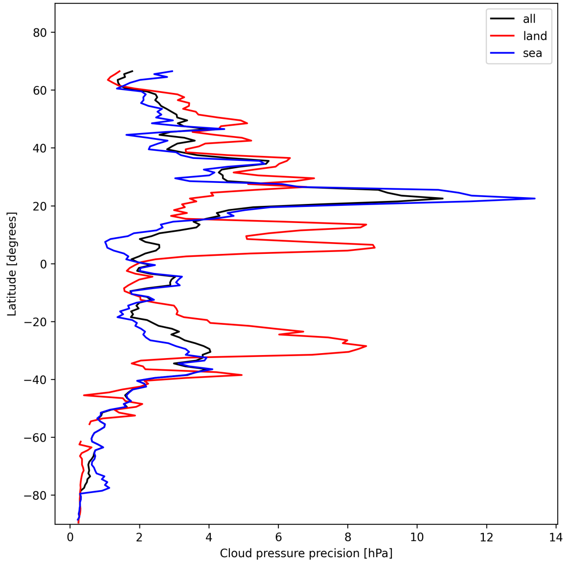
Figure 14: Zonal average of “Cloud pressure precision” for 2024-11-25 to 2024-11-27.
