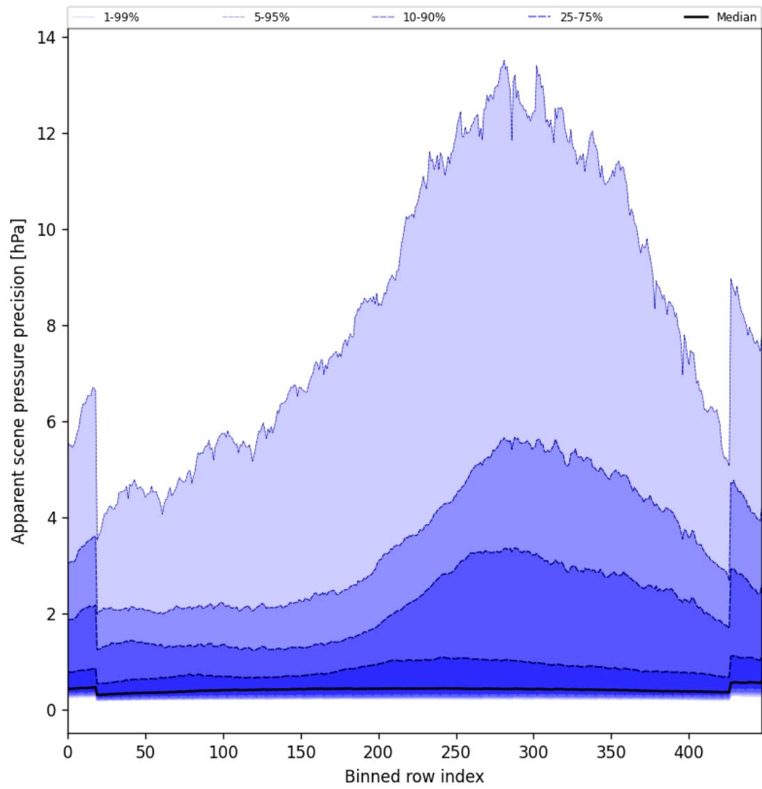
Figure 54: Along track statistics of “Apparent scene pressure precision” for 2024-11-25 to 2024-11-27
