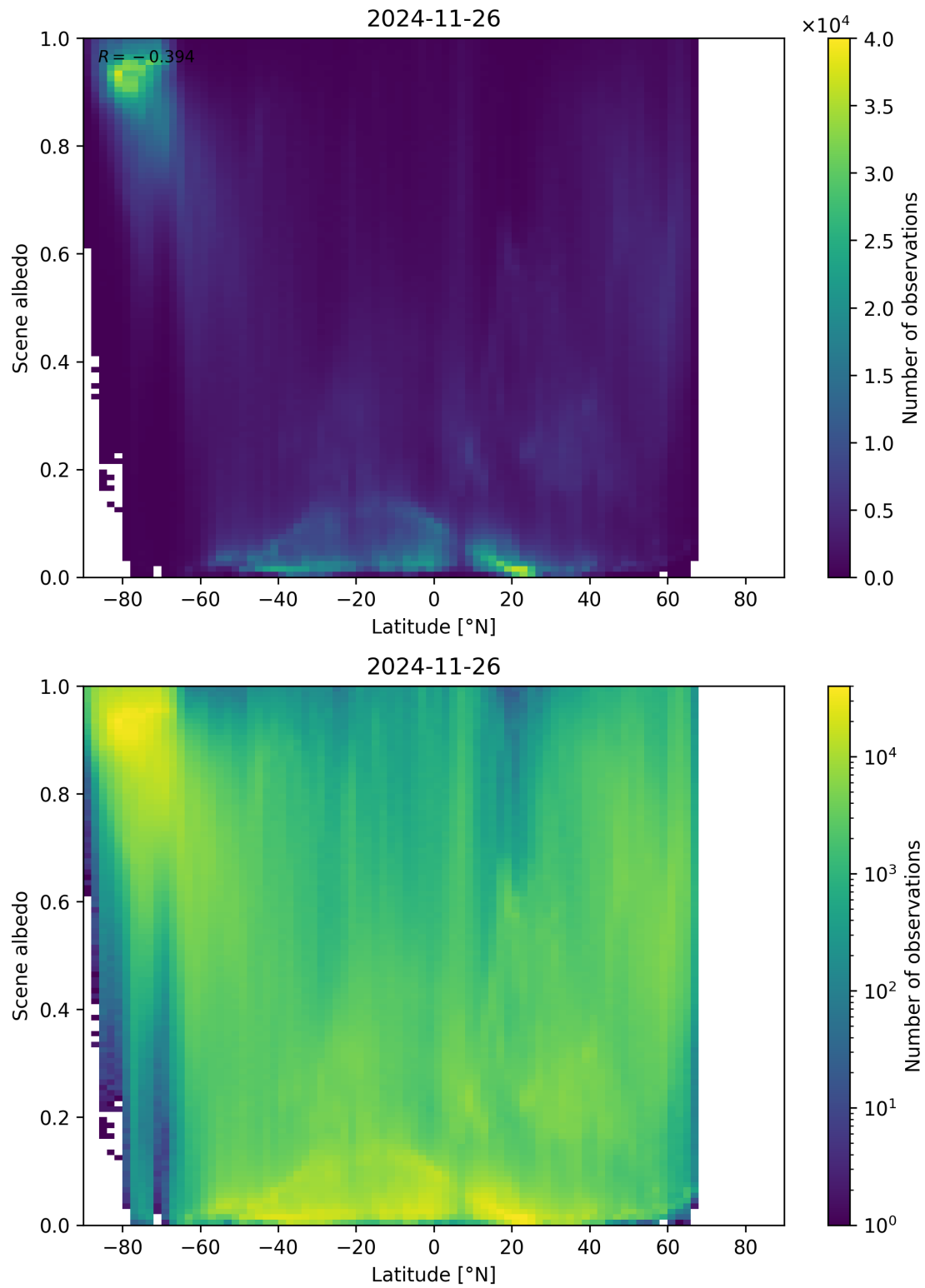
Figure 95: Scatter density plot of “Latitude” against “Scene albedo” for 2024-11-25 to 2024-11-27.
