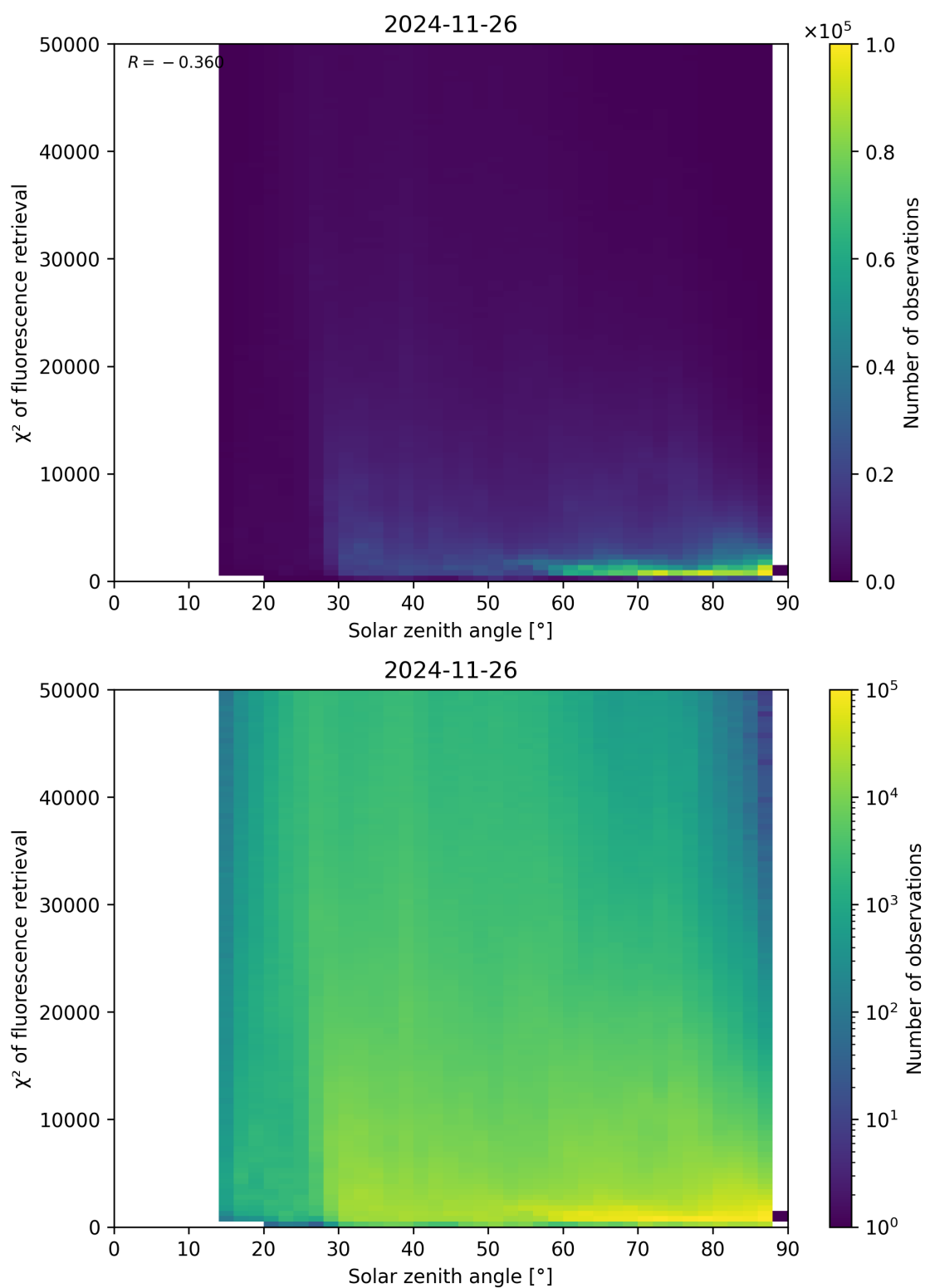
Figure 109: Scatter density plot of “Solar zenith angle” against “ \chi^2 of fluorescence retrieval” for 2024-11-25 to 2024-11-27.
