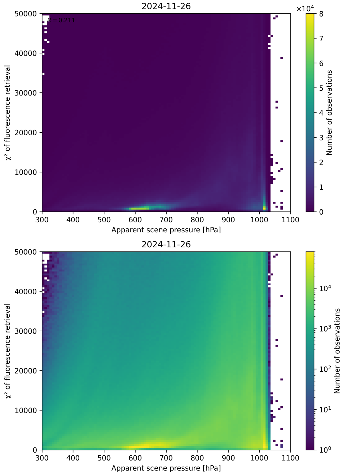
Figure 63: Scatter density plot of “Apparent scene pressure” against “ \chi^2 of fluorescence retrieval” for 2024-11-25 to 2024-11-27.
