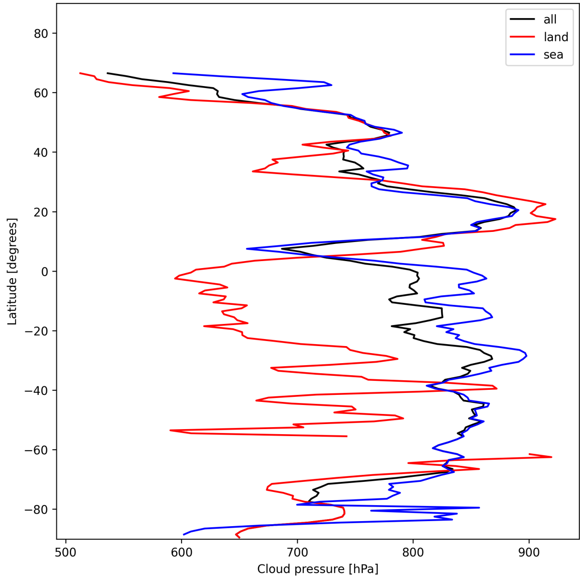
Figure 13: Zonal average of “Cloud pressure” for 2024-11-25 to 2024-11-27.
