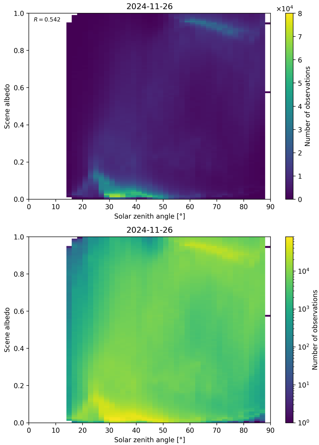
Figure 116: Scatter density plot of “Solar zenith angle” against “Scene albedo” for 2024-11-25 to 2024-11-27.
