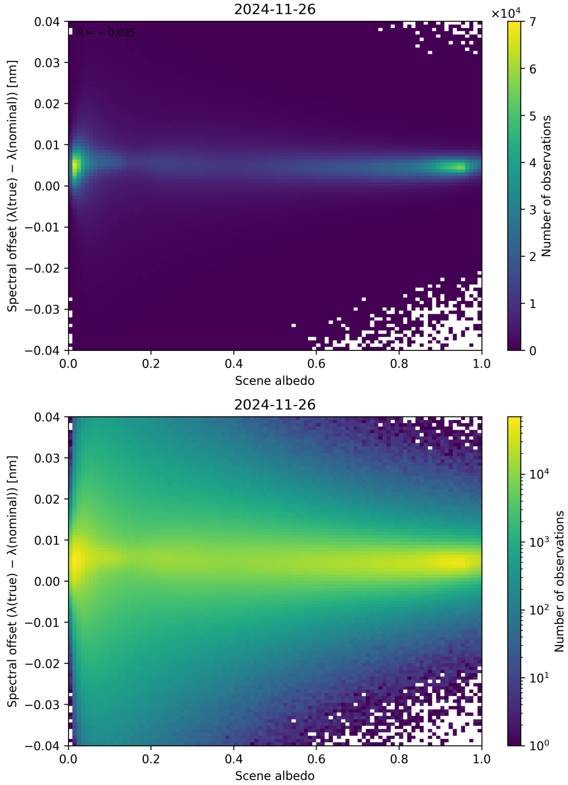
Figure 107: Scatter density plot of “Scene albedo” against “Spectral offset ( \lambda_{\text{true}} - \lambda_{\text{nominal}} )” for 2024-11-25 to 2024-11-27.
