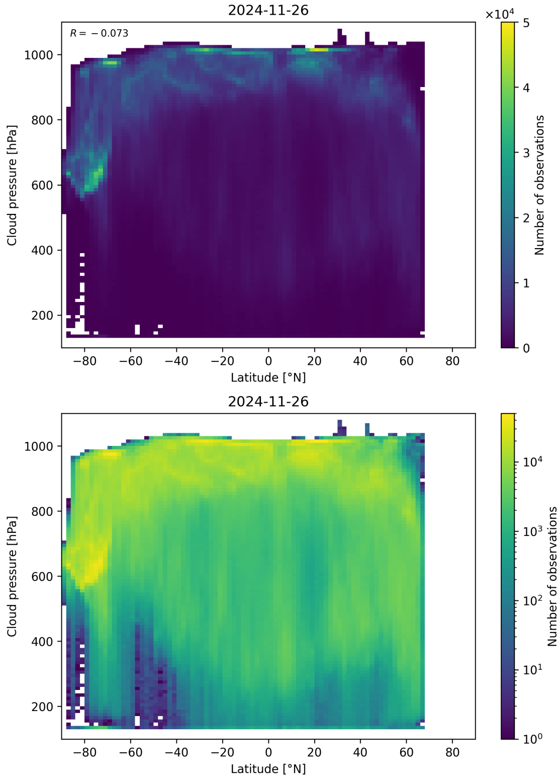
Figure 91: Scatter density plot of “Latitude” against “Cloud pressure” for 2024-11-25 to 2024-11-27.
