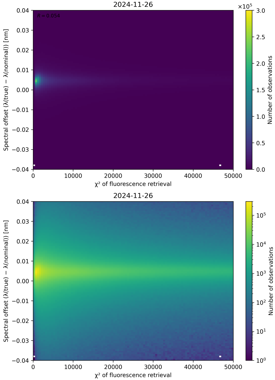
Figure 69: Scatter density plot of “ \chi^2 of fluorescence retrieval” against “Spectral offset ( \lambda_{\text{true}} - \lambda_{\text{nominal}} )” for 2024-11-25 to 2024-11-27.
