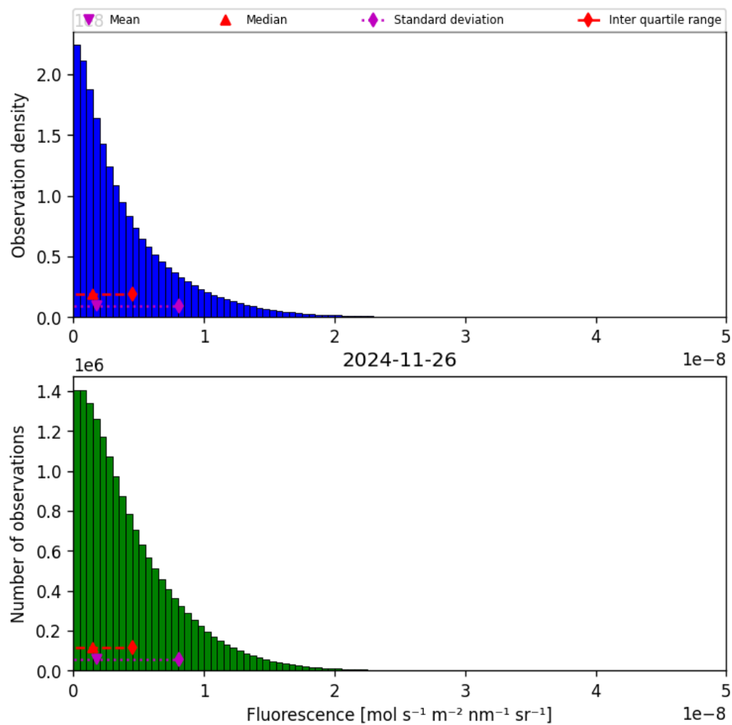
Figure 40: Histogram of “Fluorescence” for 2024-11-25 to 2024-11-27
