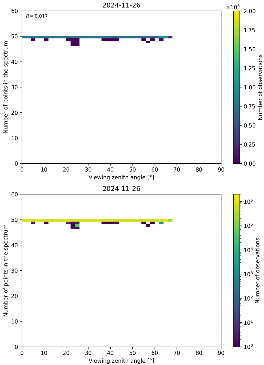
Figure 125: Scatter density plot of “Viewing zenith angle” against “Number of points in the spectrum” for 2024-11-25 to 2024-11-27.
