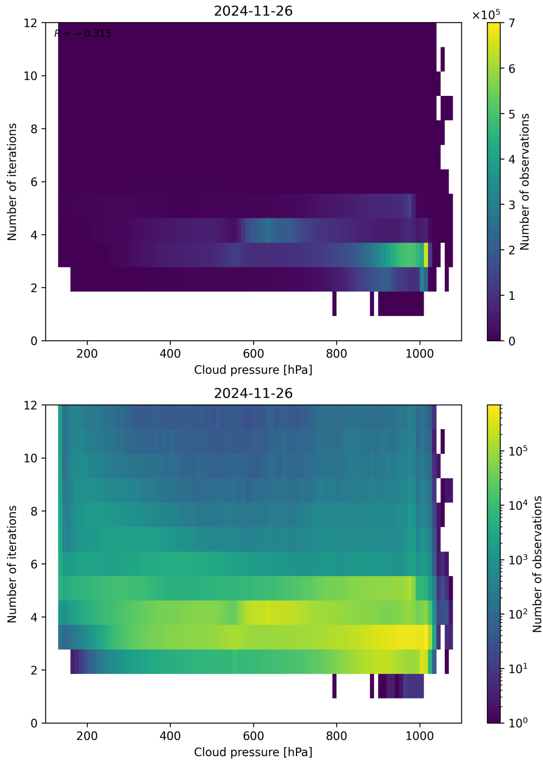
Figure 81: Scatter density plot of “Cloud pressure” against “Number of iterations” for 2024-11-25 to 2024-11-27.
