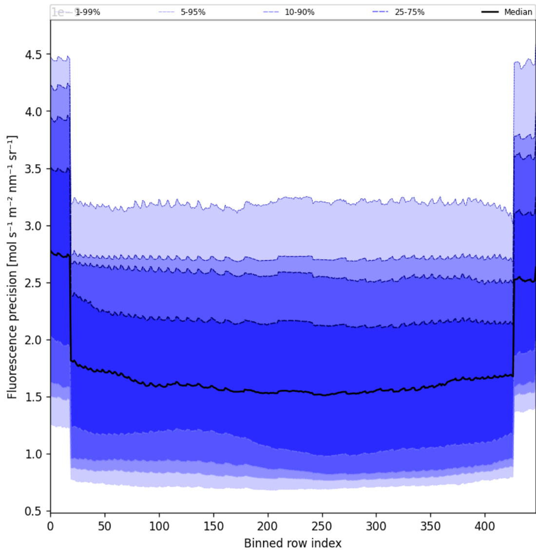
Figure 58: Along track statistics of “Fluorescence precision” for 2024-11-25 to 2024-11-27
