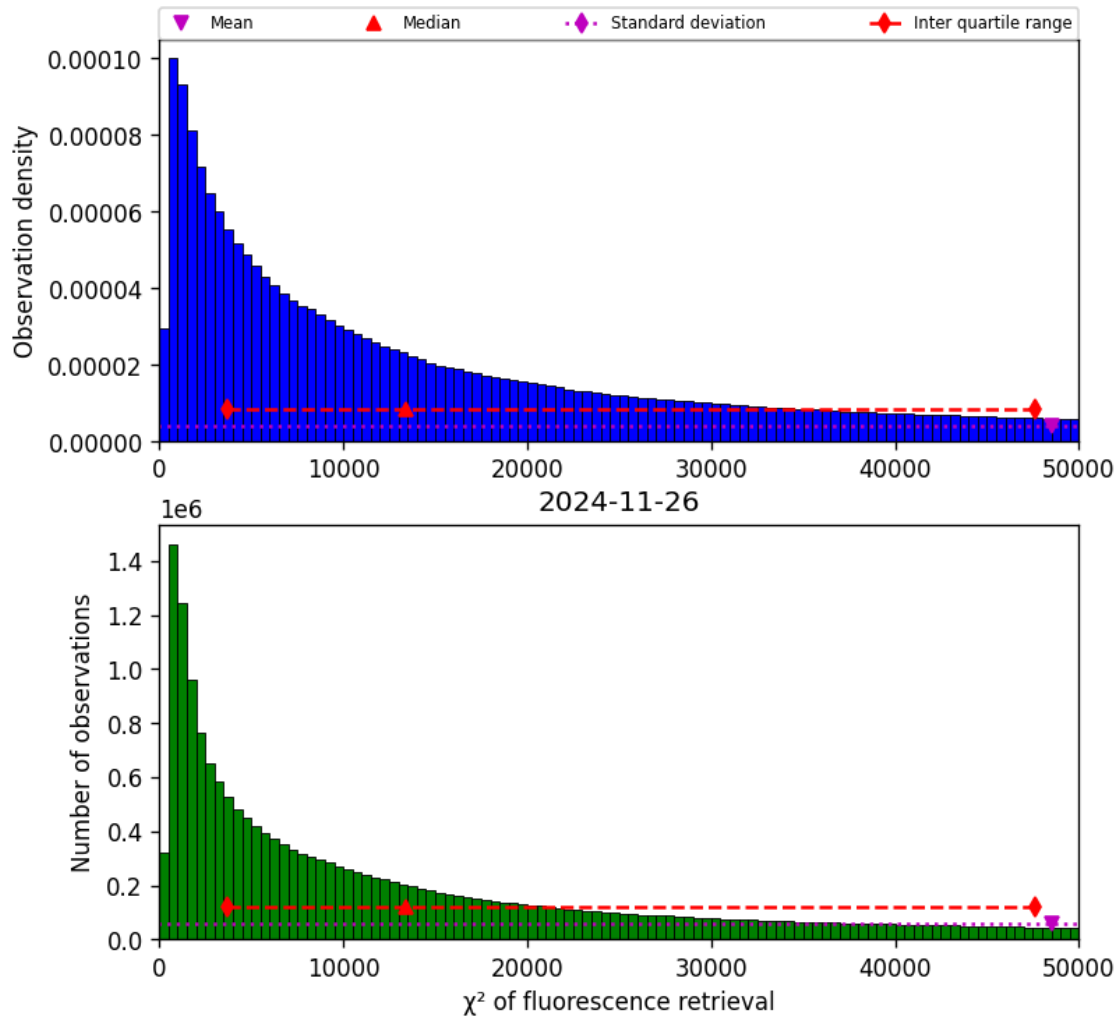
Figure 42: Histogram of “ \chi^2 of fluorescence retrieval” for 2024-11-25 to 2024-11-27
