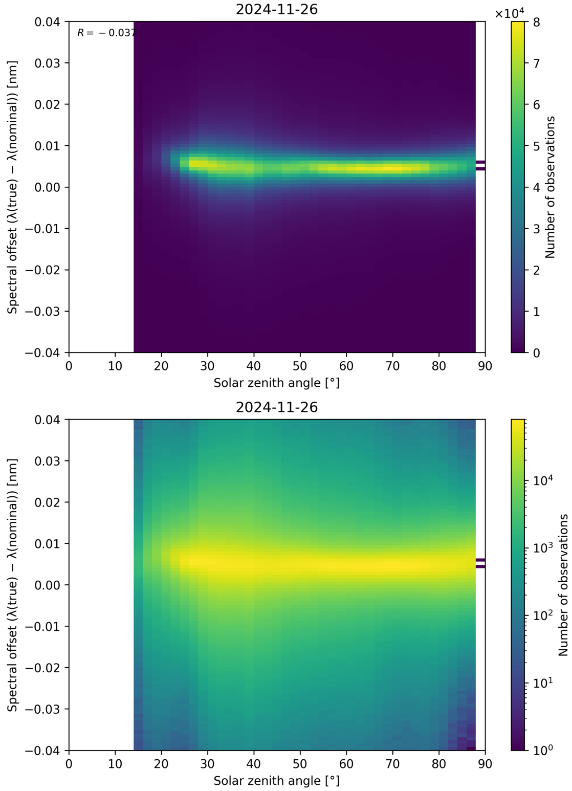
Figure 117: Scatter density plot of “Solar zenith angle” against “Spectral offset ( \lambda_{\text{true}} - \lambda_{\text{nominal}} )” for 2024-11-25 to 2024-11-27.
