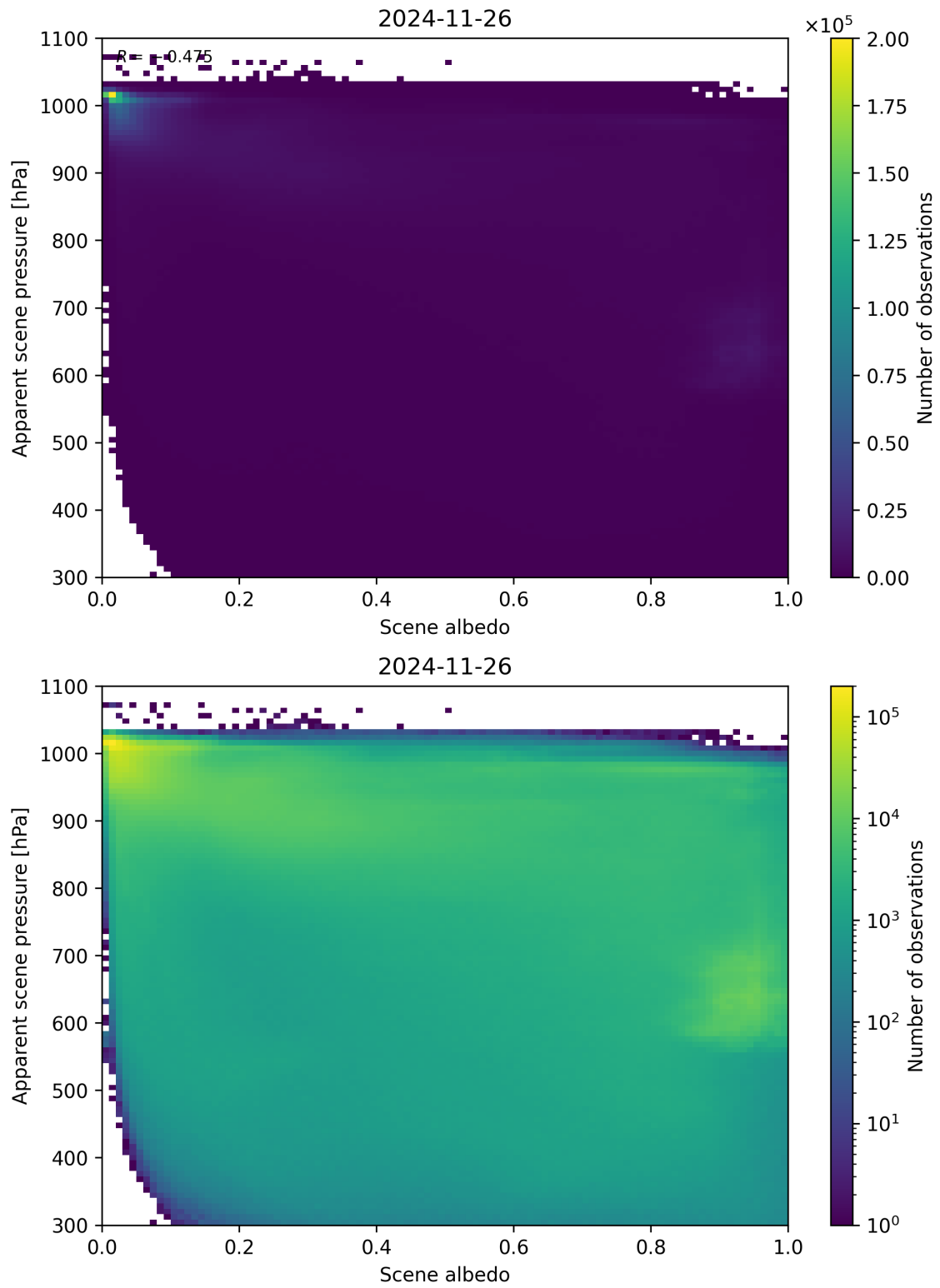
Figure 102: Scatter density plot of “Scene albedo” against “Apparent scene pressure” for 2024-11-25 to 2024-11-27.
