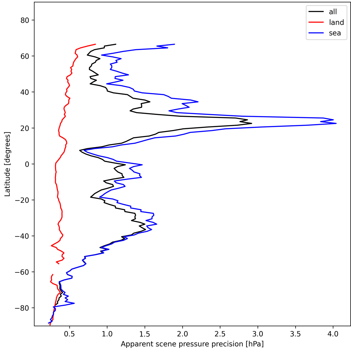
Figure 20: Zonal average of “Apparent scene pressure precision” for 2024-11-25 to 2024-11-27.
