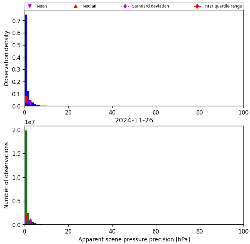
Figure 37: Histogram of “Apparent scene pressure precision” for 2024-11-25 to 2024-11-27
