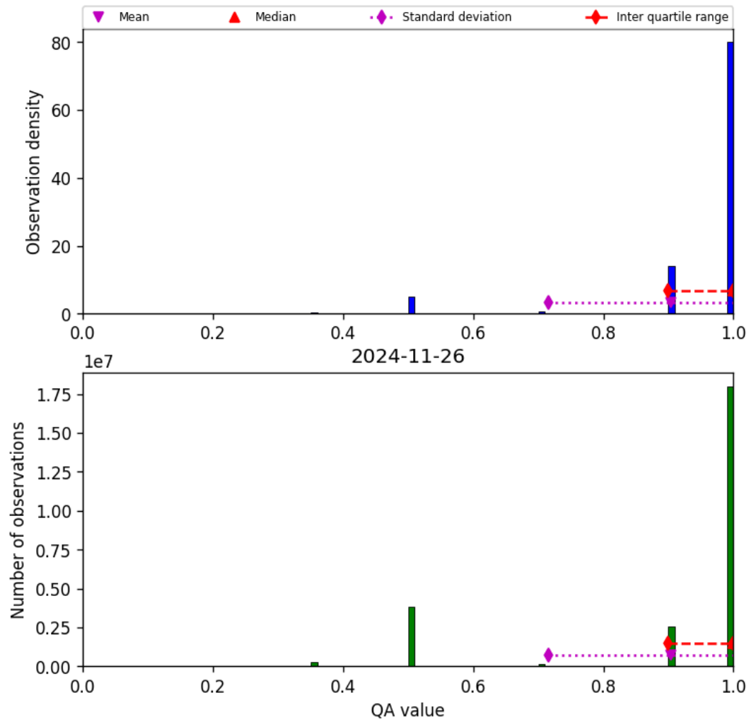
Figure 29: Histogram of “QA value” for 2024-11-25 to 2024-11-27
