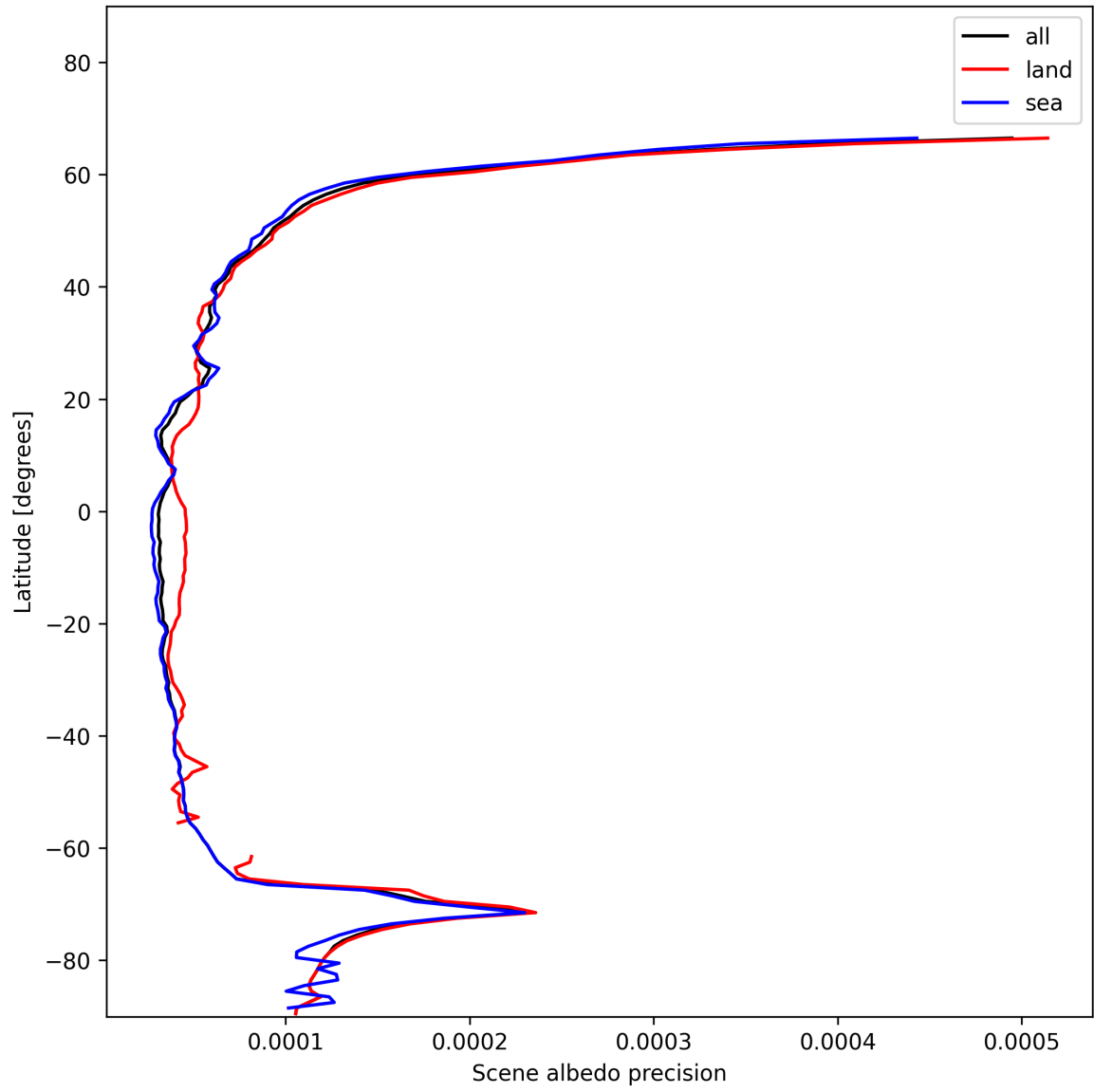
Figure 18: Zonal average of “Scene albedo precision” for 2024-11-25 to 2024-11-27.
