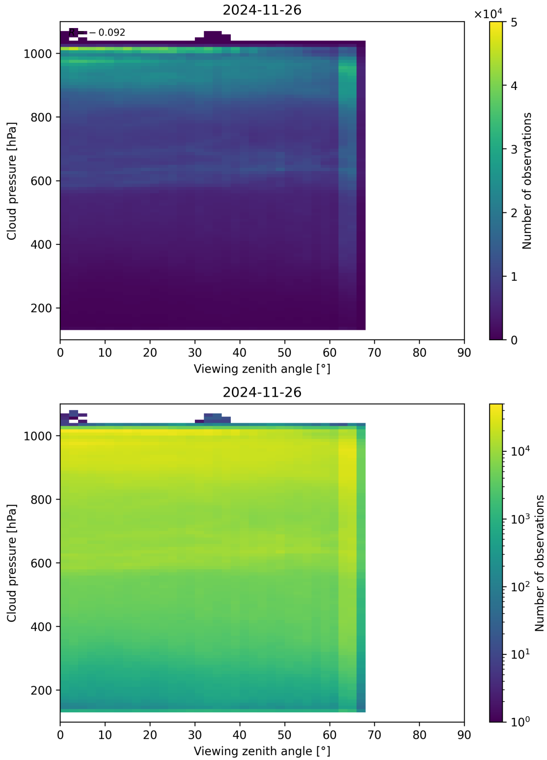
Figure 121: Scatter density plot of “Viewing zenith angle” against “Cloud pressure” for 2024-11-25 to 2024-11-27.
