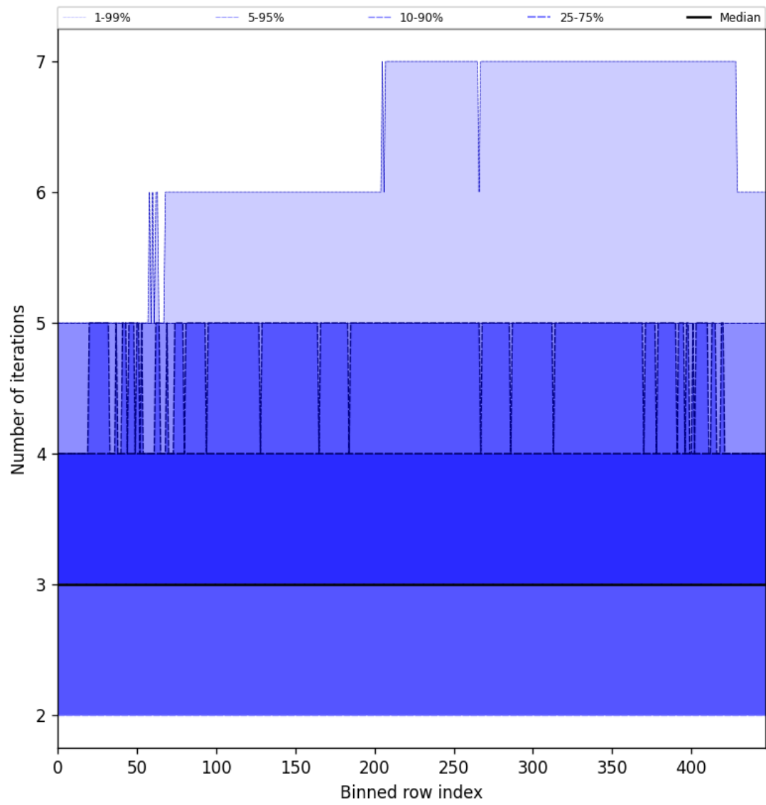
Figure 56: Along track statistics of “Number of iterations” for 2024-11-25 to 2024-11-27
