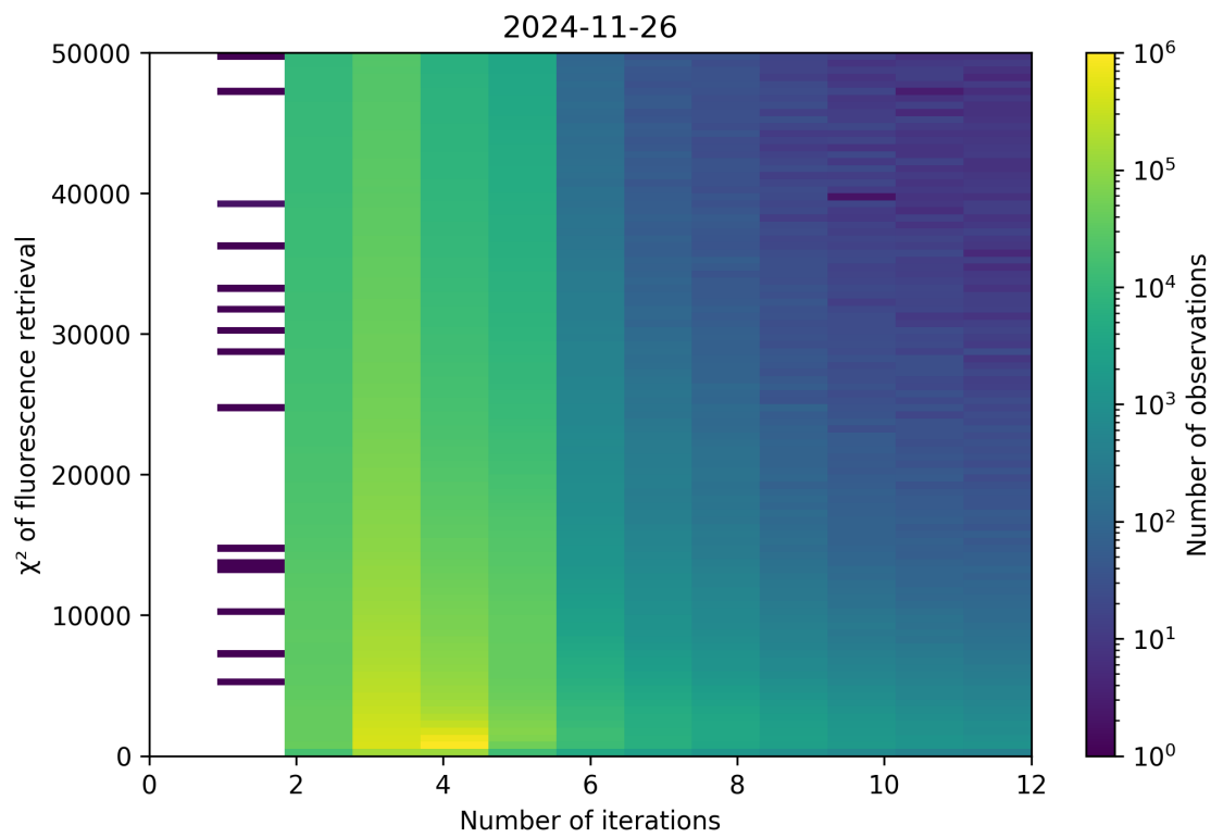
Figure 97: Scatter density plot of “Number of iterations” against “ \chi^2 of fluorescence retrieval” for 2024-11-25 to 2024-11-27.
