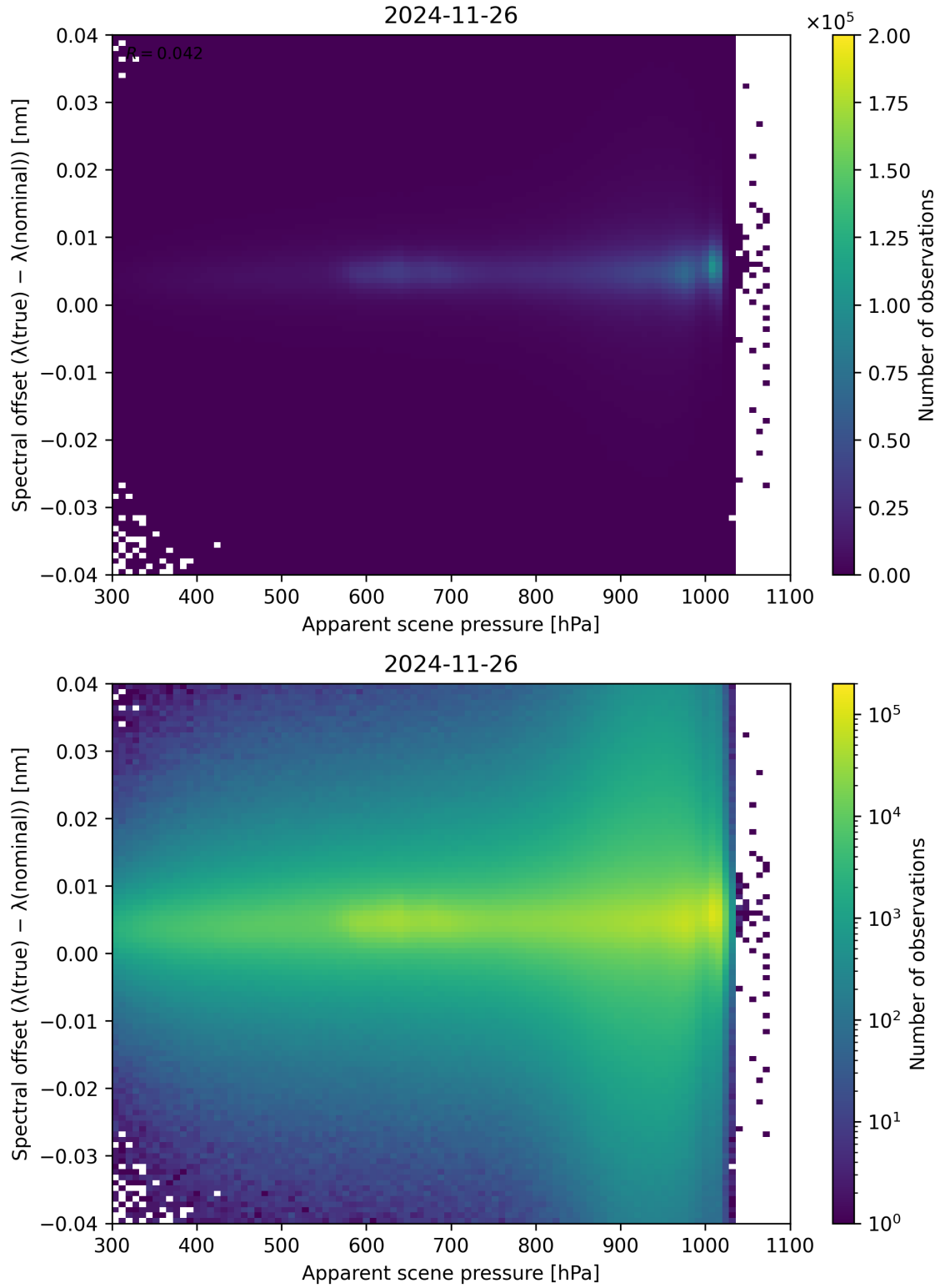
Figure 67: Scatter density plot of “Apparent scene pressure” against “Spectral offset ( \lambda_{\text{true}} - \lambda_{\text{nominal}} )” for 2024-11-25 to 2024-11-27.
