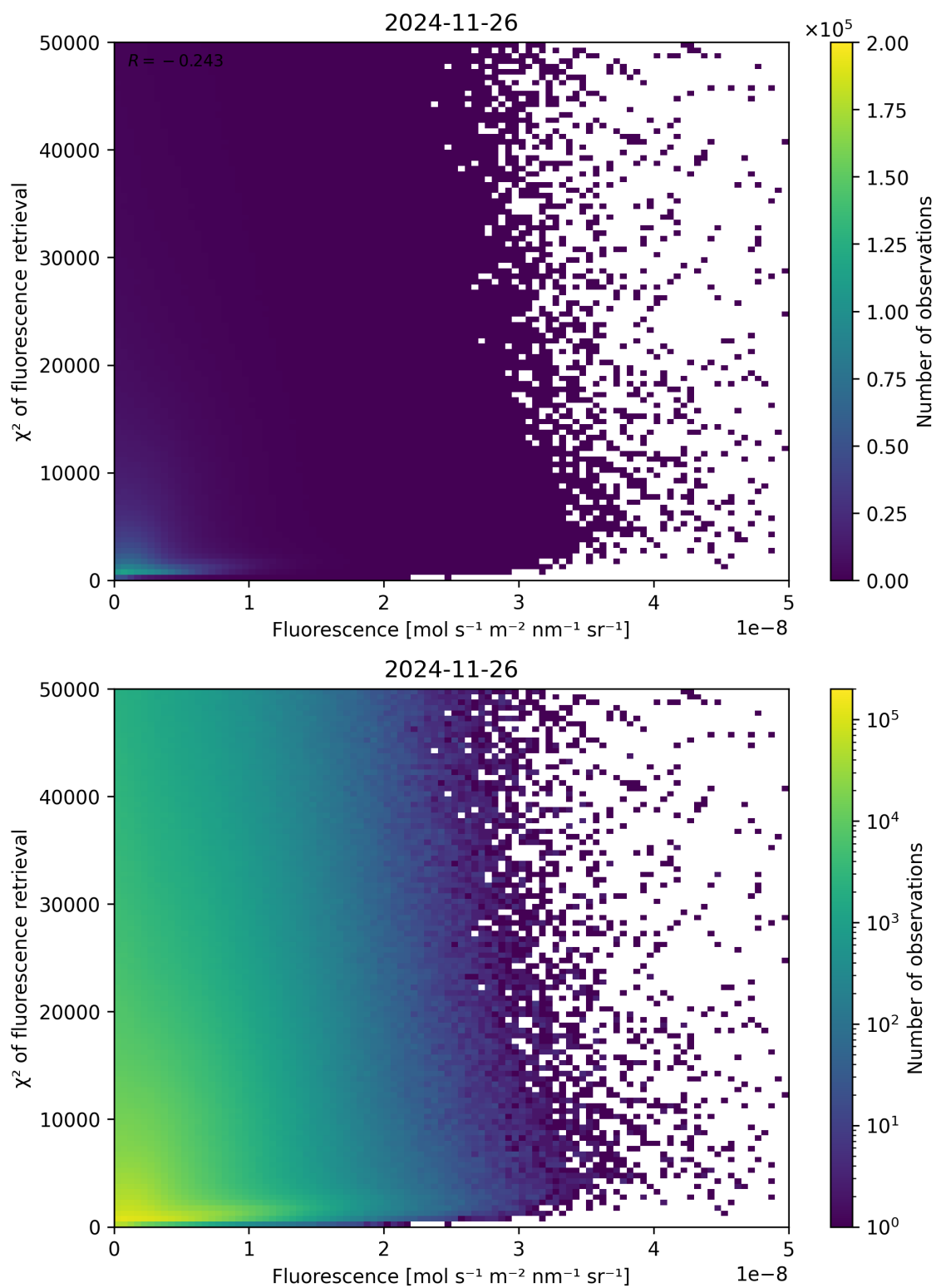
Figure 85: Scatter density plot of “Fluorescence” against “ \chi^2 of fluorescence retrieval” for 2024-11-25 to 2024-11-27.
