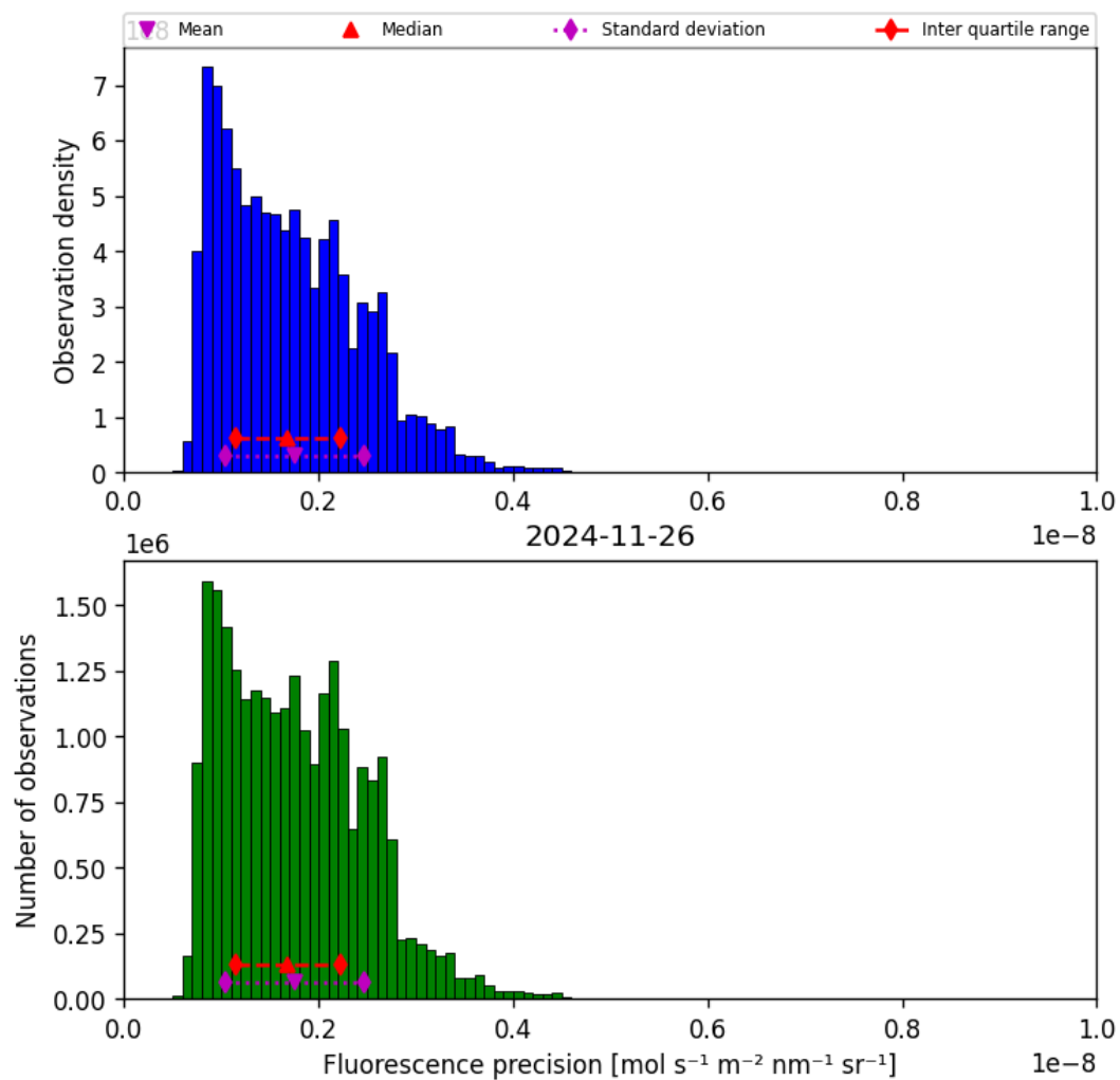
Figure 41: Histogram of “Fluorescence precision” for 2024-11-25 to 2024-11-27
