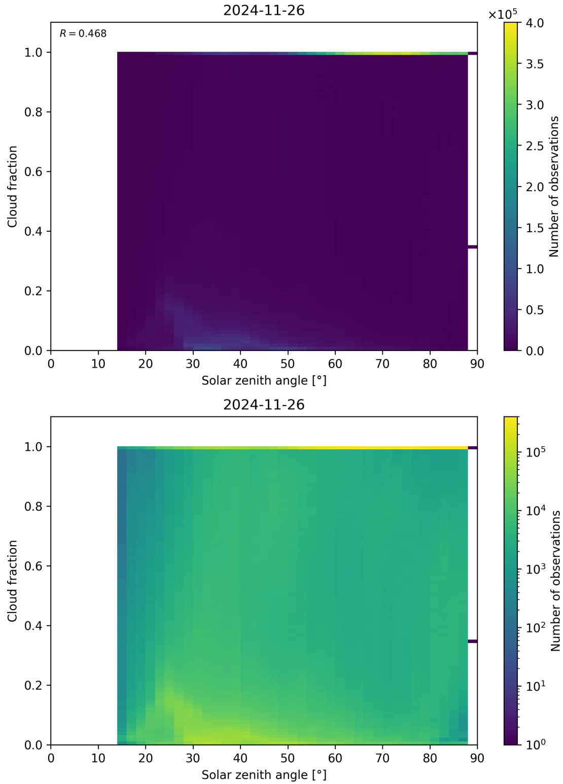
Figure 110: Scatter density plot of “Solar zenith angle” against “Cloud fraction” for 2024-11-25 to 2024-11-27.
