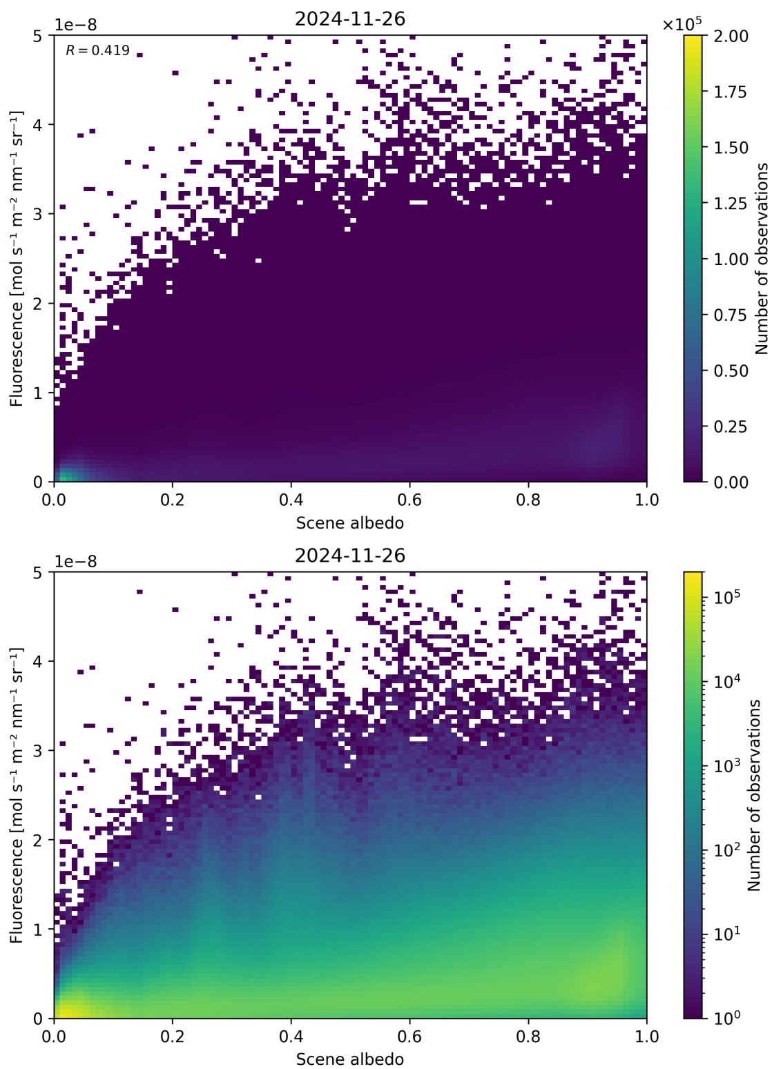
Figure 104: Scatter density plot of “Scene albedo” against “Fluorescence” for 2024-11-25 to 2024-11-27.
