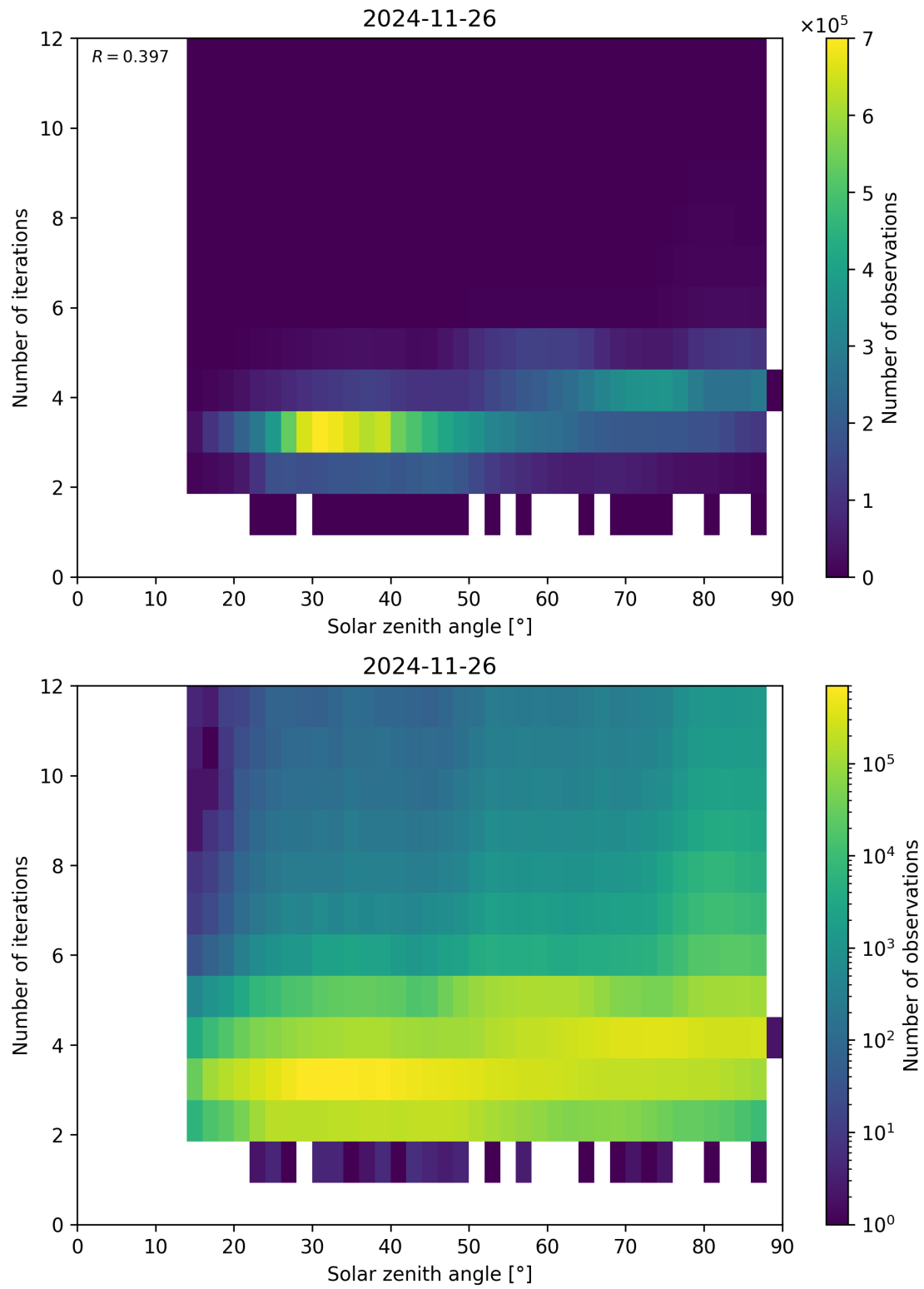
Figure 114: Scatter density plot of “Solar zenith angle” against “Number of iterations” for 2024-11-25 to 2024-11-27.
