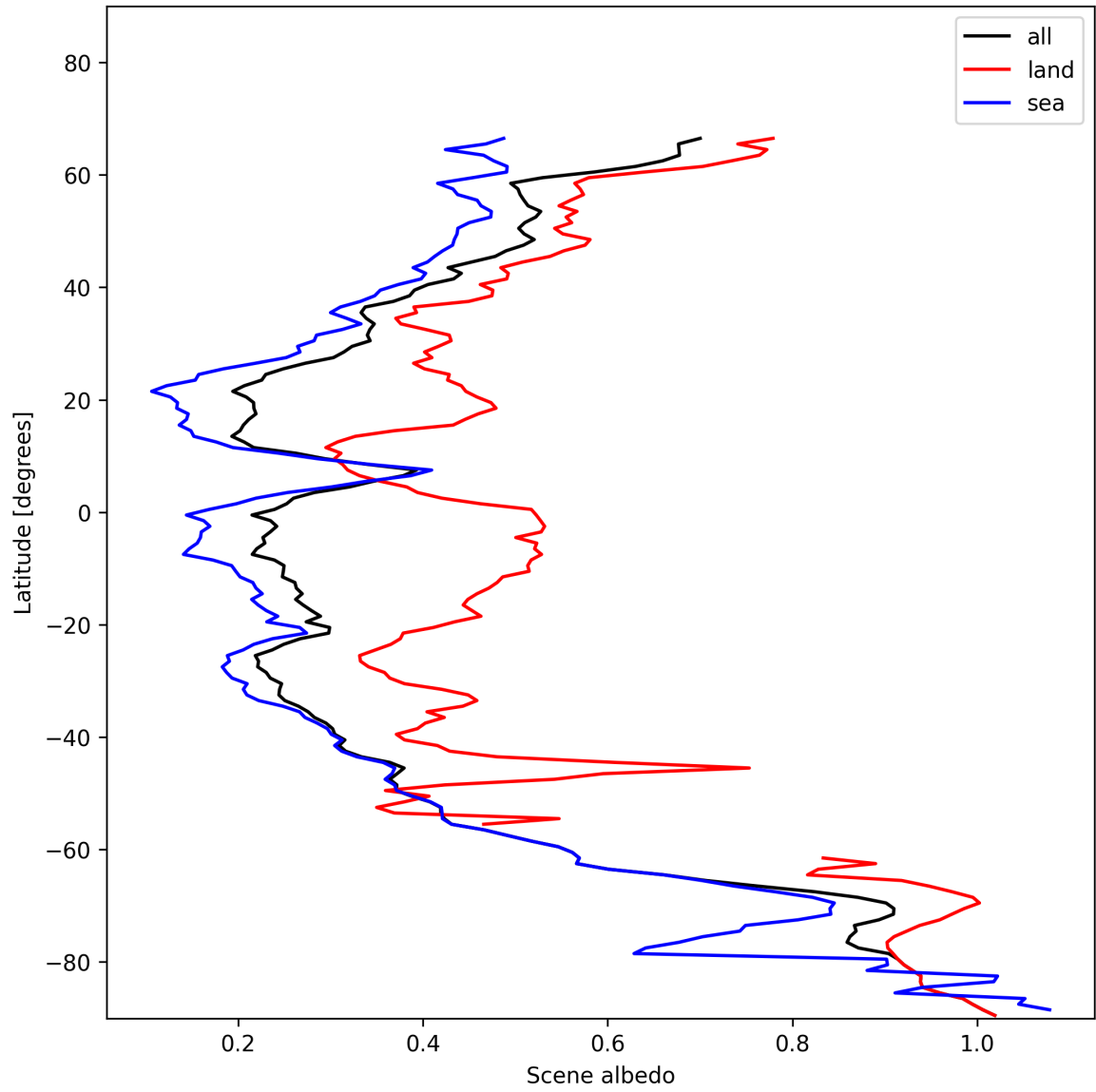
Figure 17: Zonal average of “Scene albedo” for 2024-11-25 to 2024-11-27.
