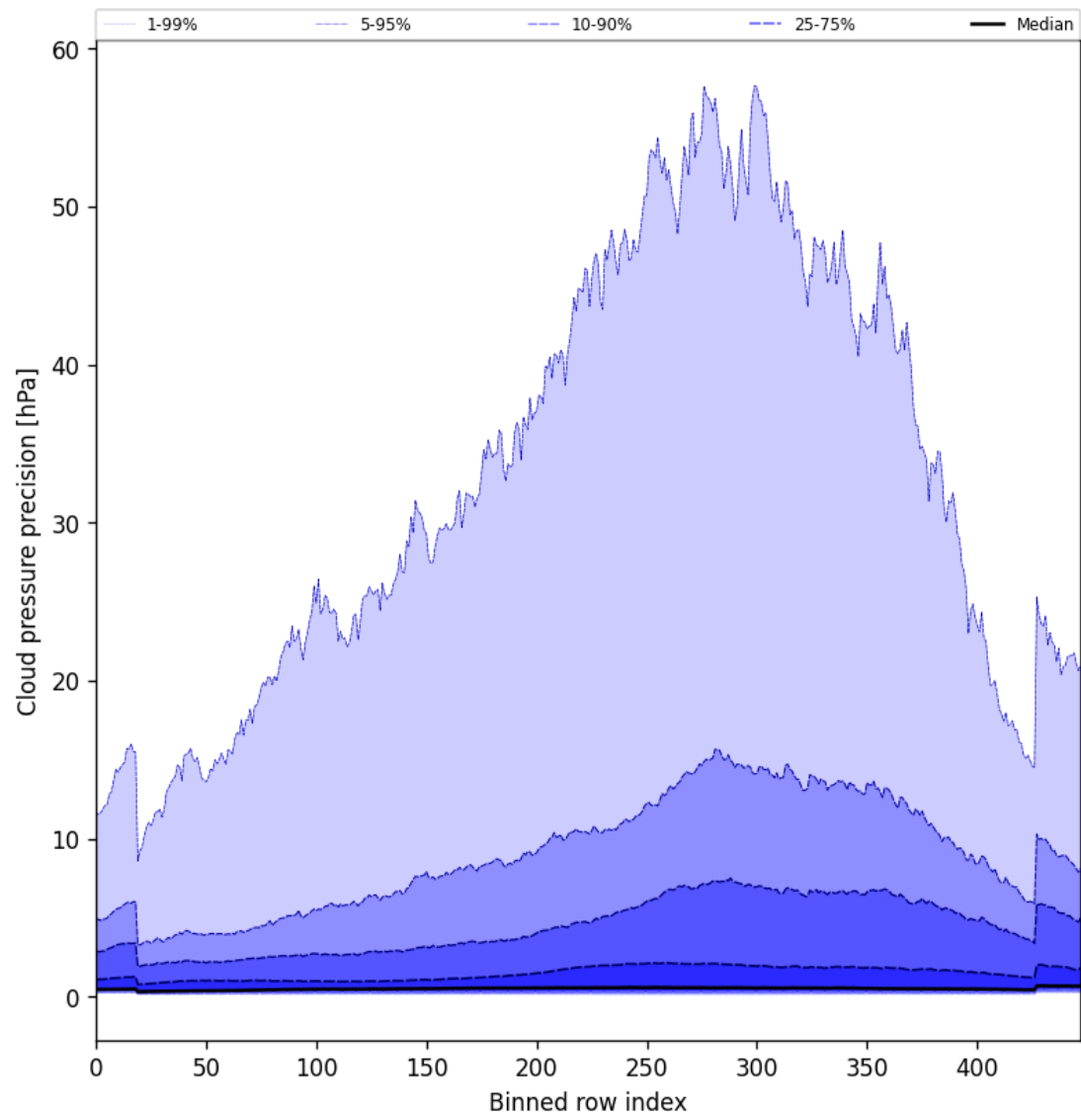
Figure 48: Along track statistics of “Cloud pressure precision” for 2024-11-25 to 2024-11-27
