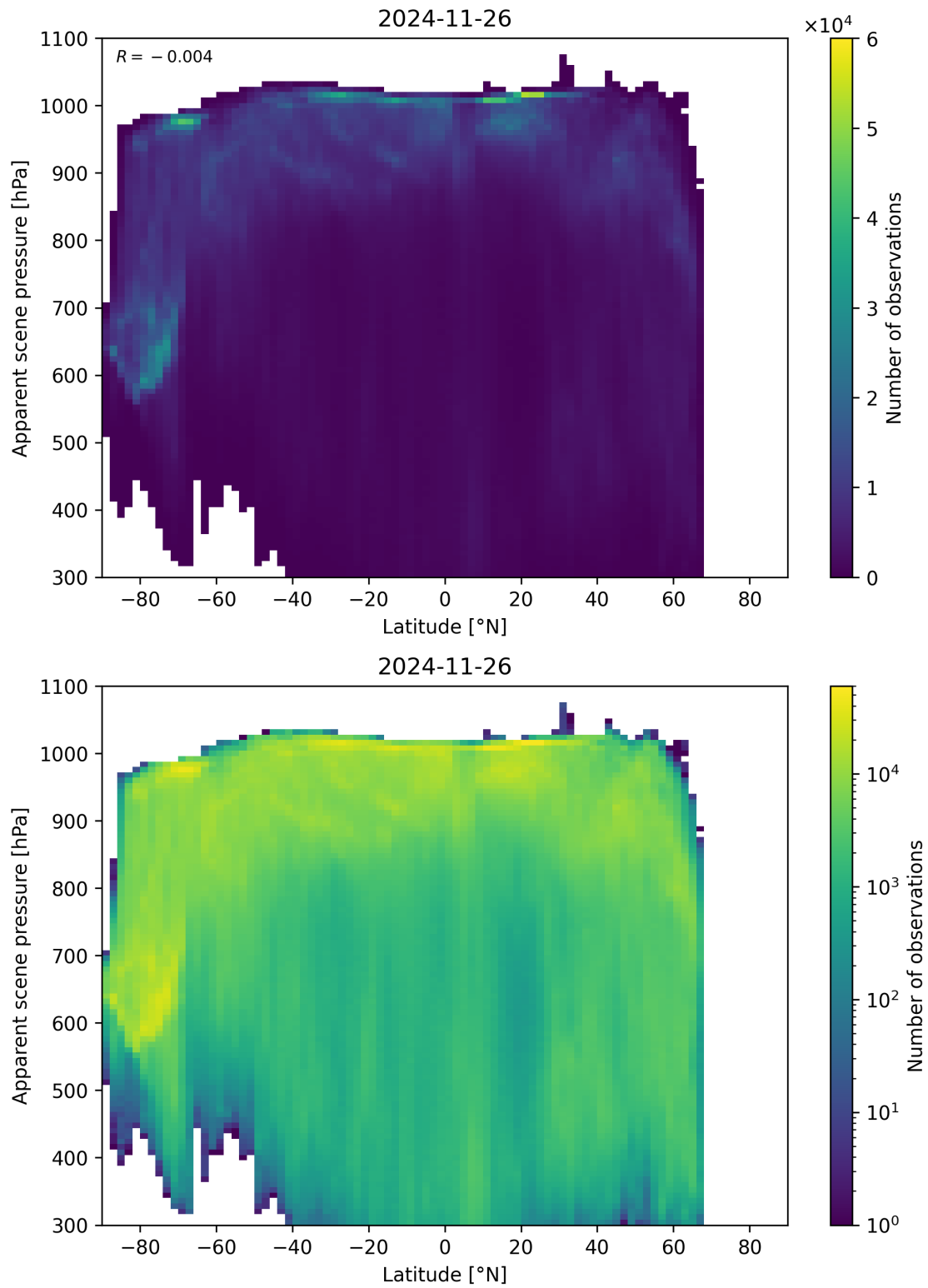
Figure 88: Scatter density plot of “Latitude” against “Apparent scene pressure” for 2024-11-25 to 2024-11-27.
