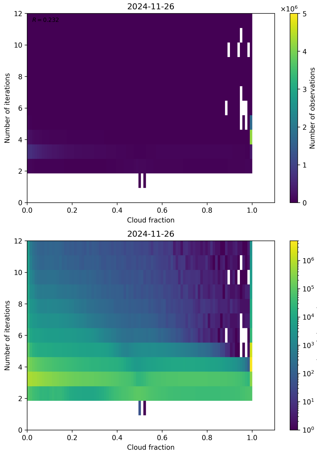
Figure 73: Scatter density plot of “Cloud fraction” against “Number of iterations” for 2024-11-25 to 2024-11-27.
