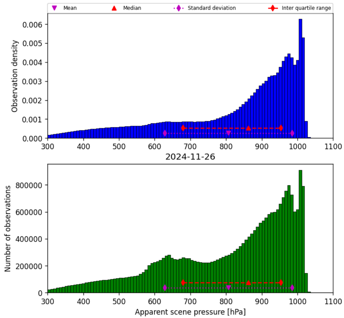
Figure 36: Histogram of “Apparent scene pressure” for 2024-11-25 to 2024-11-27
