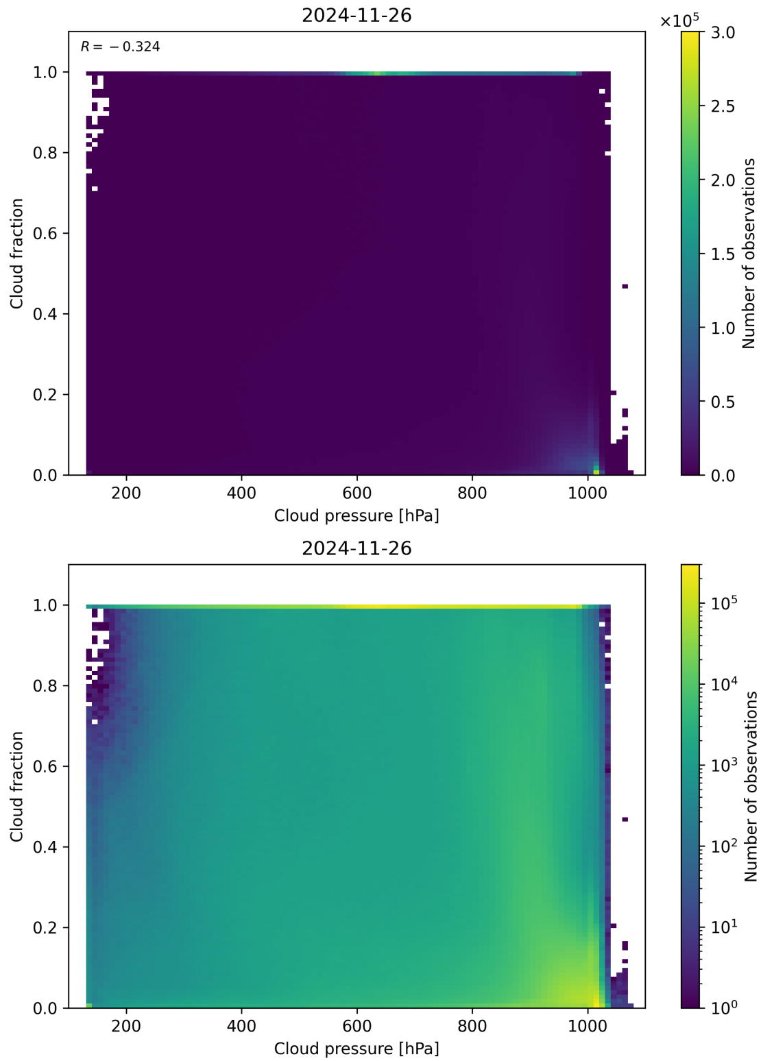
Figure 79: Scatter density plot of “Cloud pressure” against “Cloud fraction” for 2024-11-25 to 2024-11-27.
