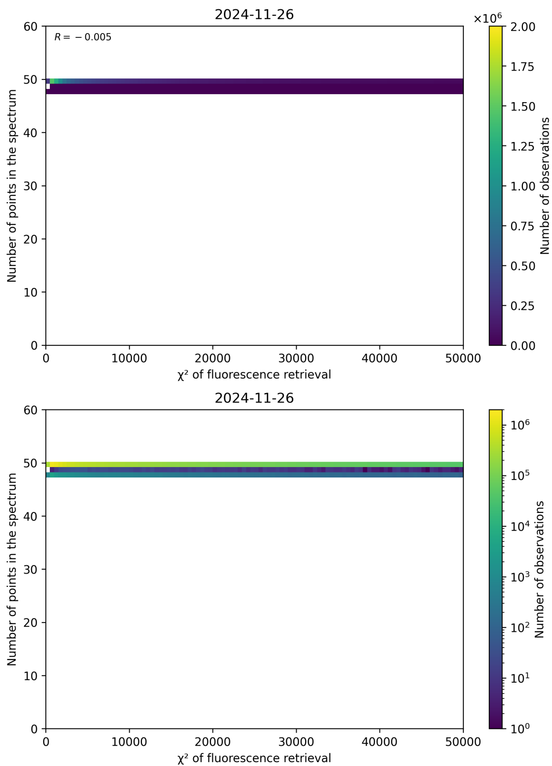
Figure 68: Scatter density plot of “ \chi^2 of fluorescence retrieval” against “Number of points in the spectrum” for 2024-11-25 to 2024-11-27.
