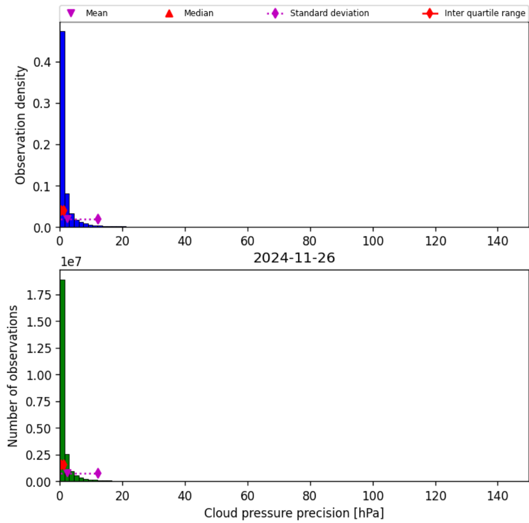
Figure 31: Histogram of “Cloud pressure precision” for 2024-11-25 to 2024-11-27
