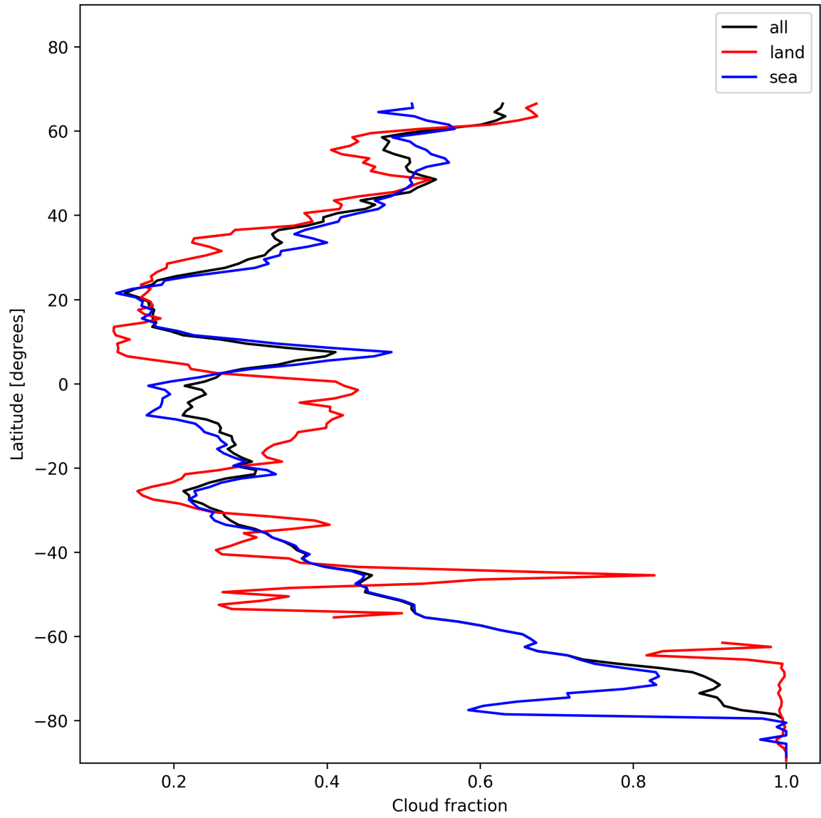
Figure 15: Zonal average of “Cloud fraction” for 2024-11-25 to 2024-11-27.
