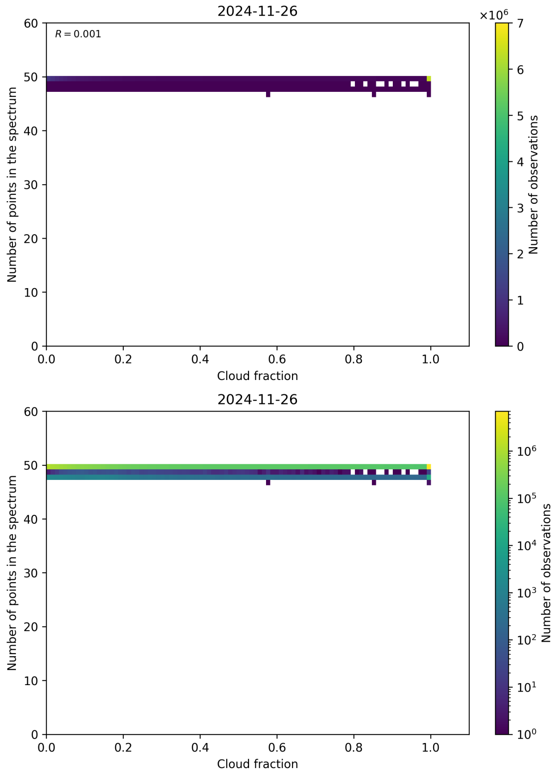
Figure 74: Scatter density plot of “Cloud fraction” against “Number of points in the spectrum” for 2024-11-25 to 2024-11-27.
