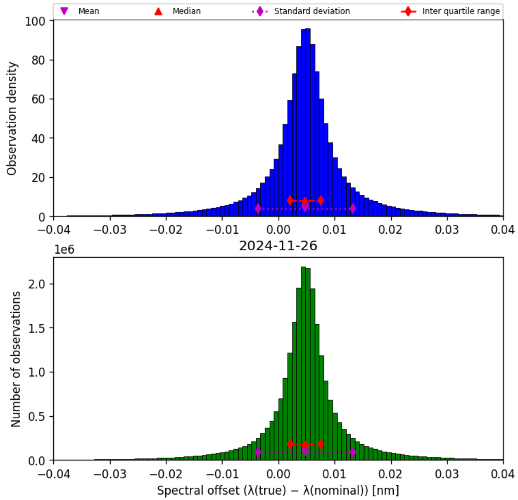
Figure 45: Histogram of “Spectral offset ( \lambda_{\text{true}} - \lambda_{\text{nominal}} )” for 2024-11-25 to 2024-11-27
