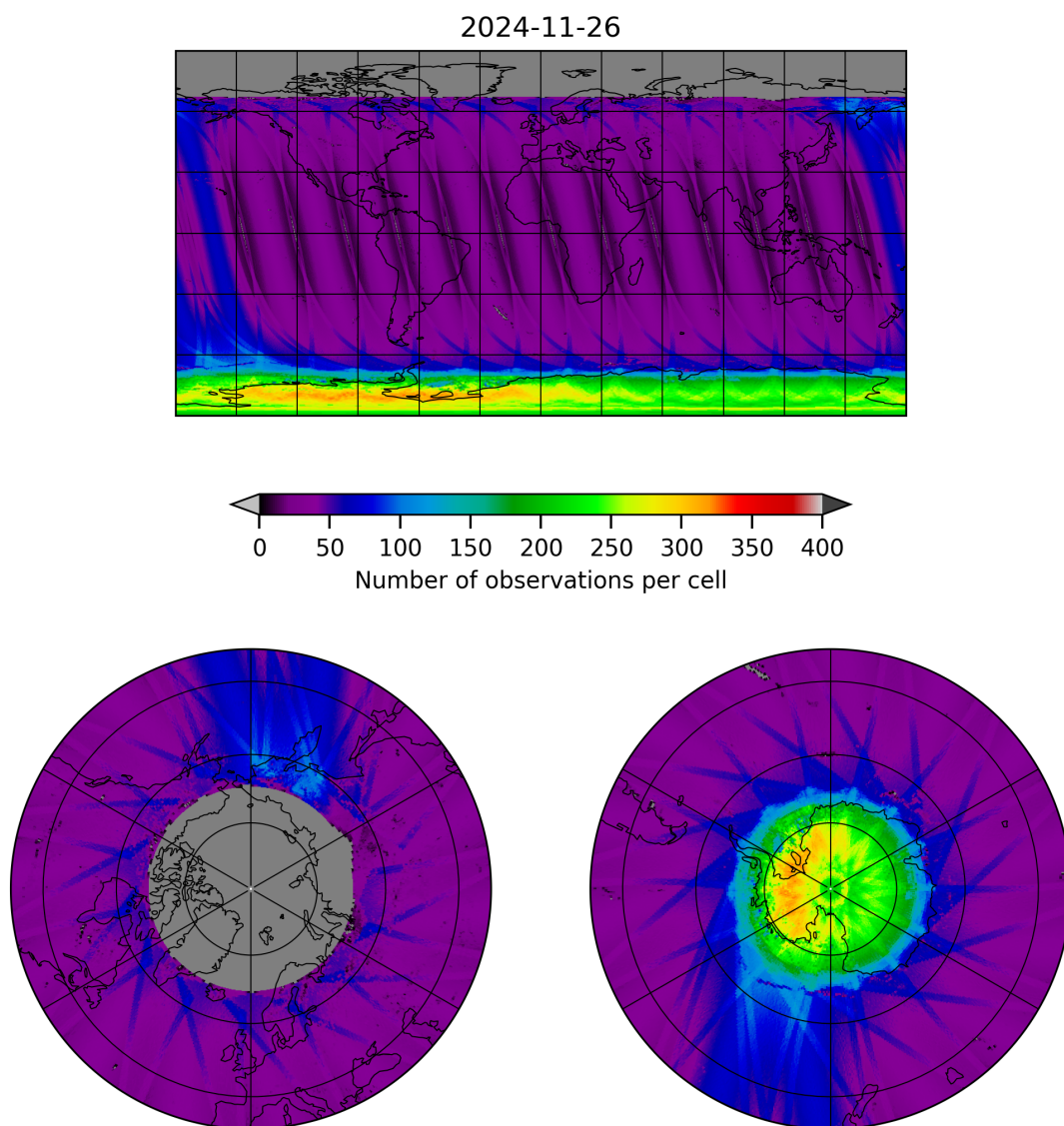
Figure 11: Map of the number of observations for 2024-11-25 to 2024-11-27
