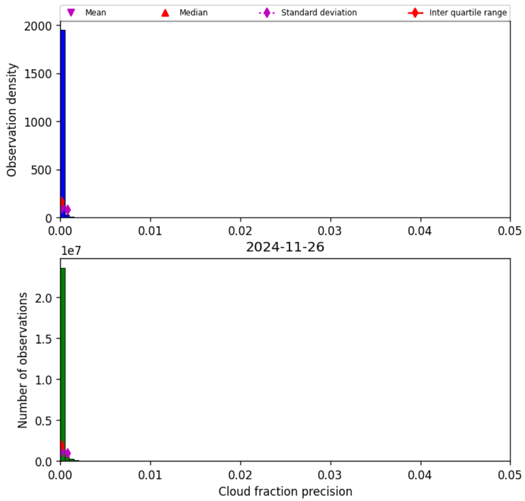
Figure 33: Histogram of “Cloud fraction precision” for 2024-11-25 to 2024-11-27
