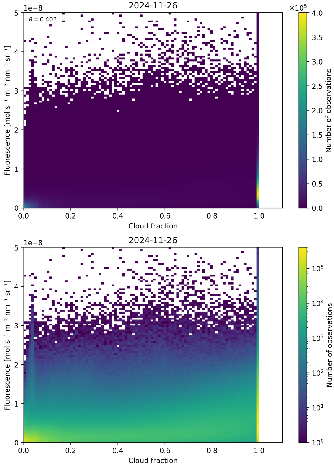
Figure 72: Scatter density plot of “Cloud fraction” against “Fluorescence” for 2024-11-25 to 2024-11-27.
