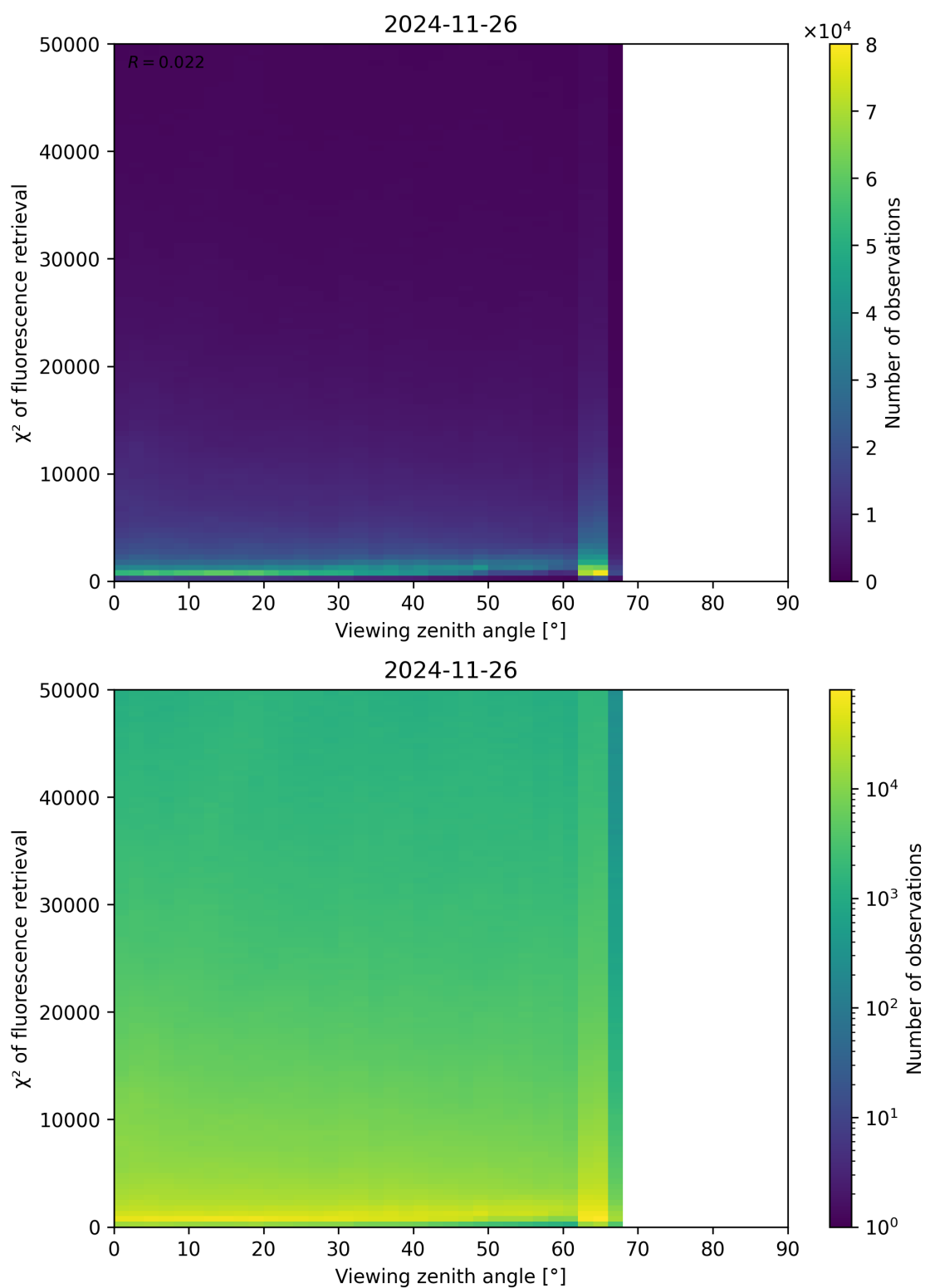
Figure 119: Scatter density plot of “Viewing zenith angle” against “ \chi^2 of fluorescence retrieval” for 2024-11-25 to 2024-11-27.
