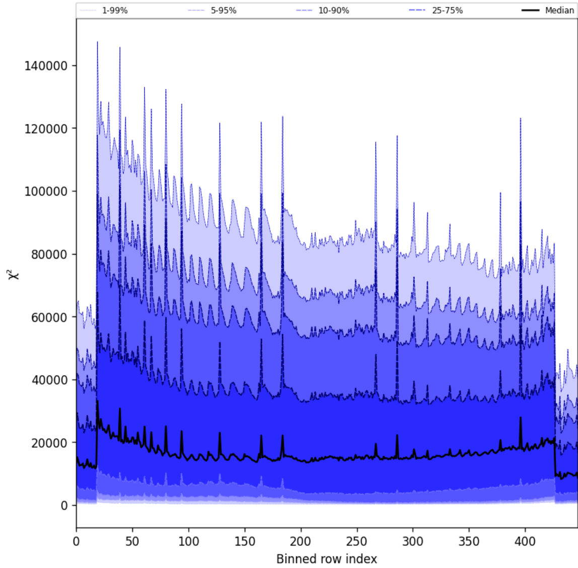
Figure 55: Along track statistics of “ \chi^2 ” for 2024-11-25 to 2024-11-27
