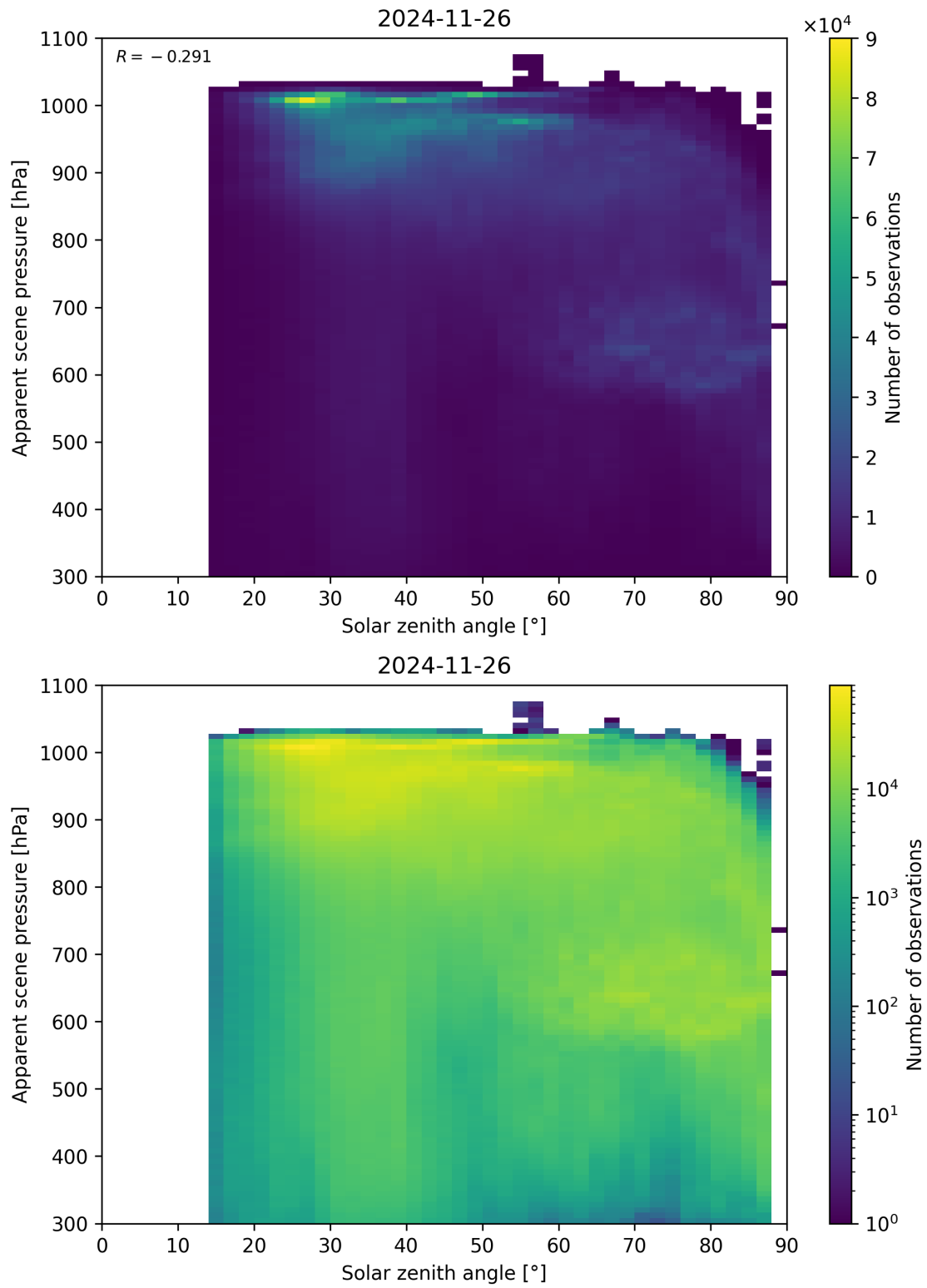
Figure 108: Scatter density plot of “Solar zenith angle” against “Apparent scene pressure” for 2024-11-25 to 2024-11-27.
