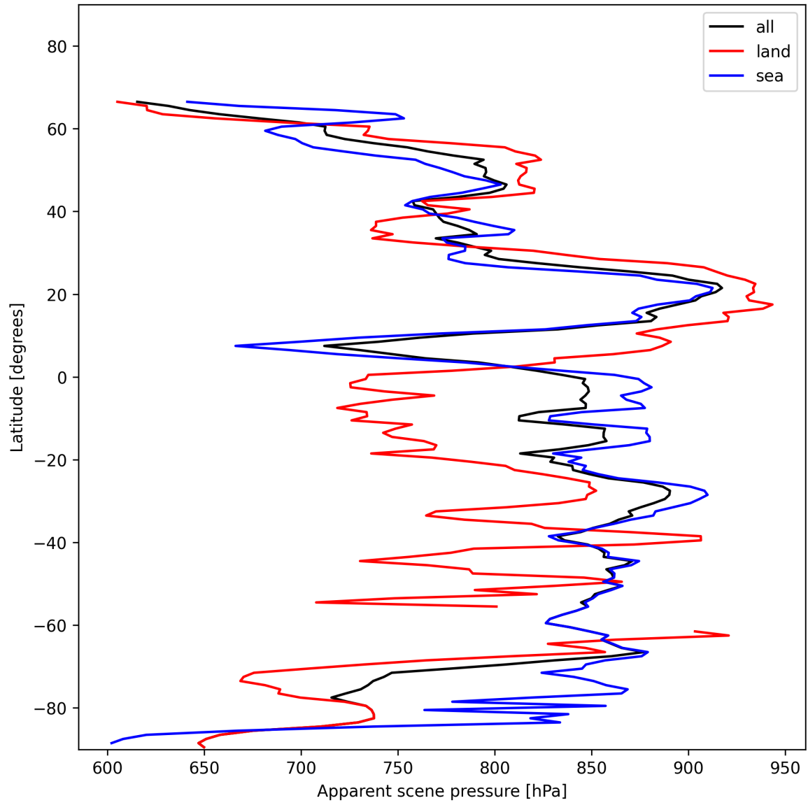
Figure 19: Zonal average of “Apparent scene pressure” for 2024-11-25 to 2024-11-27.
