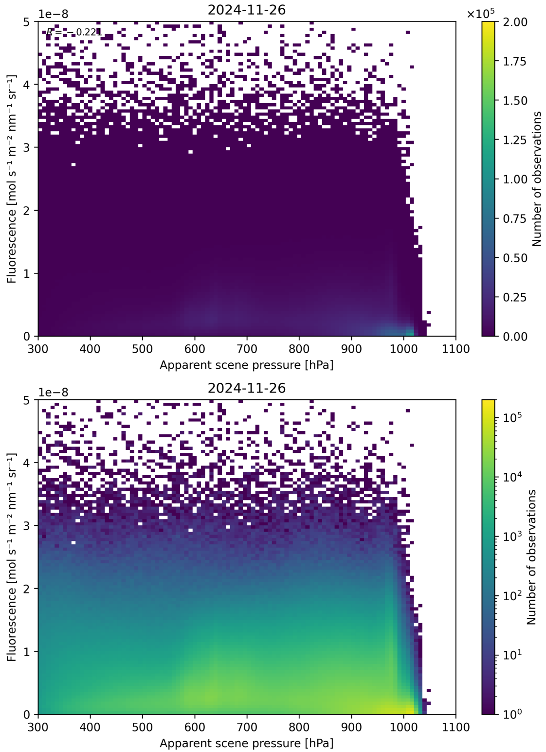
Figure 64: Scatter density plot of “Apparent scene pressure” against “Fluorescence” for 2024-11-25 to 2024-11-27.
