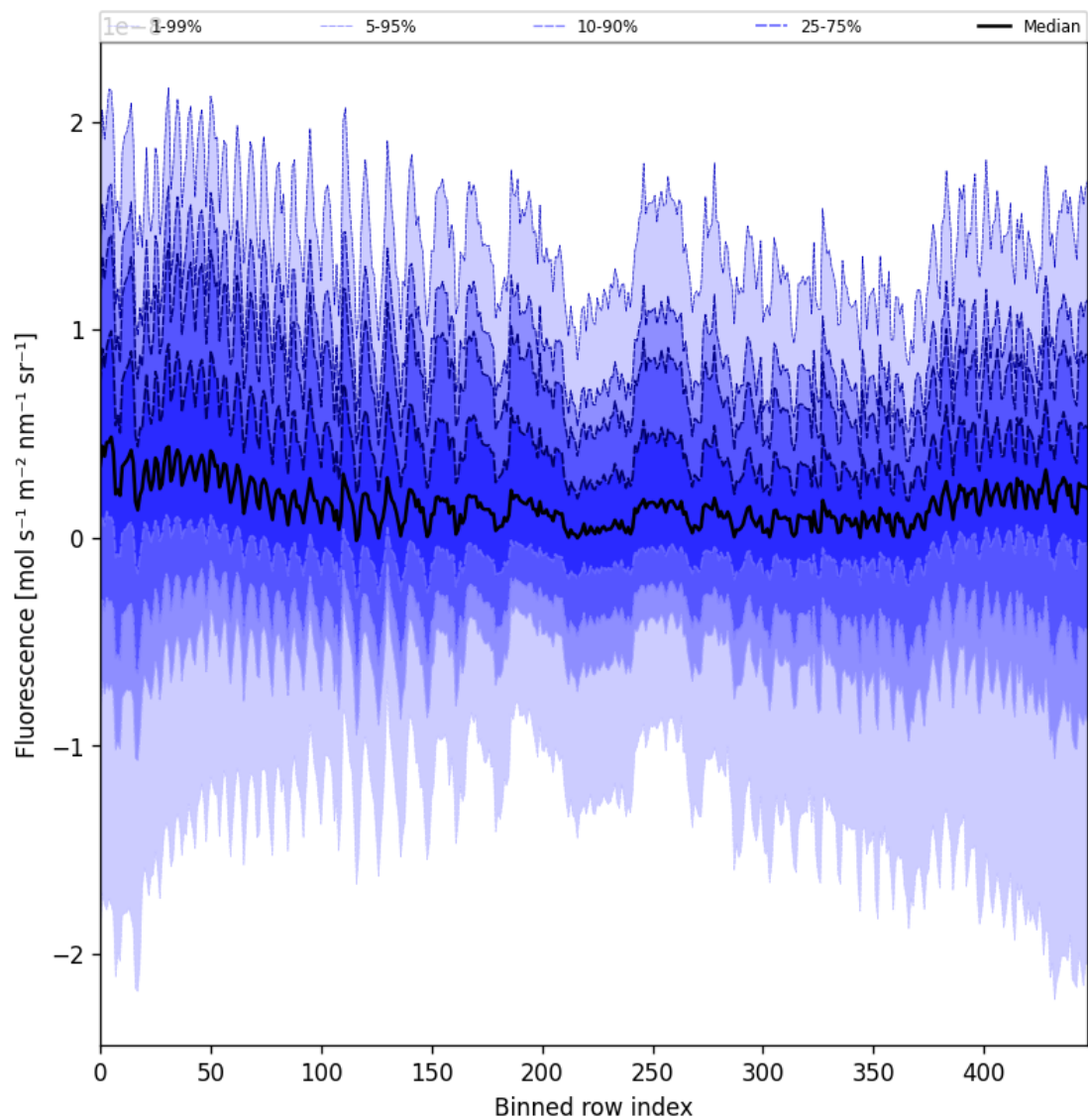
Figure 57: Along track statistics of “Fluorescence” for 2024-11-25 to 2024-11-27
