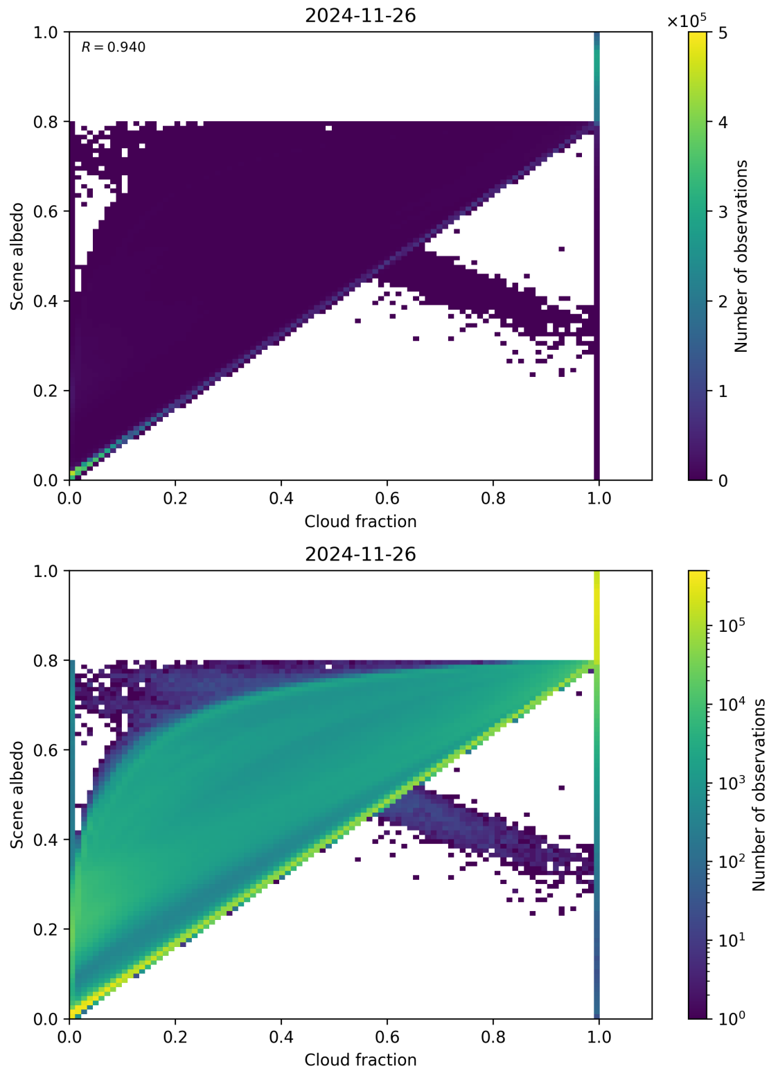
Figure 75: Scatter density plot of “Cloud fraction” against “Scene albedo” for 2024-11-25 to 2024-11-27.
