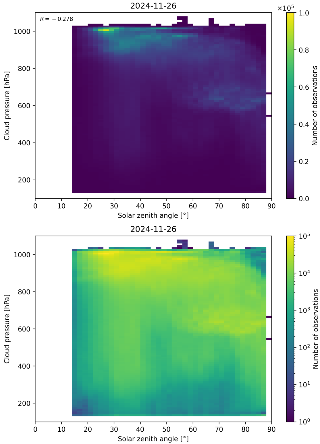
Figure 111: Scatter density plot of “Solar zenith angle” against “Cloud pressure” for 2024-11-25 to 2024-11-27.
