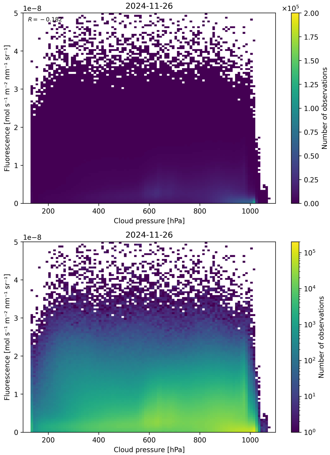
Figure 80: Scatter density plot of “Cloud pressure” against “Fluorescence” for 2024-11-25 to 2024-11-27.
