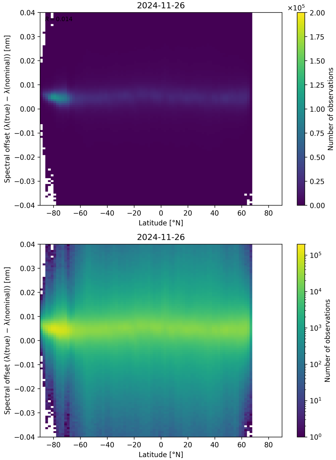
Figure 96: Scatter density plot of “Latitude” against “Spectral offset ( \lambda_{\text{true}} - \lambda_{\text{nominal}} )” for 2024-11-25 to 2024-11-27.
