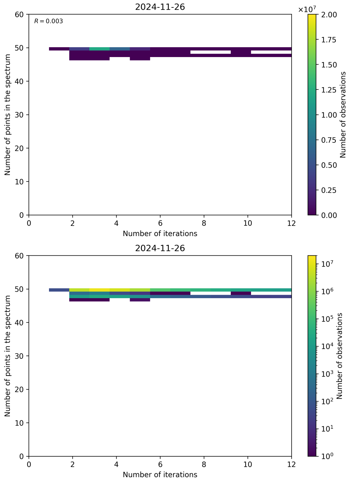
Figure 99: Scatter density plot of “Number of iterations” against “Number of points in the spectrum” for 2024-11-25 to 2024-11-27.
