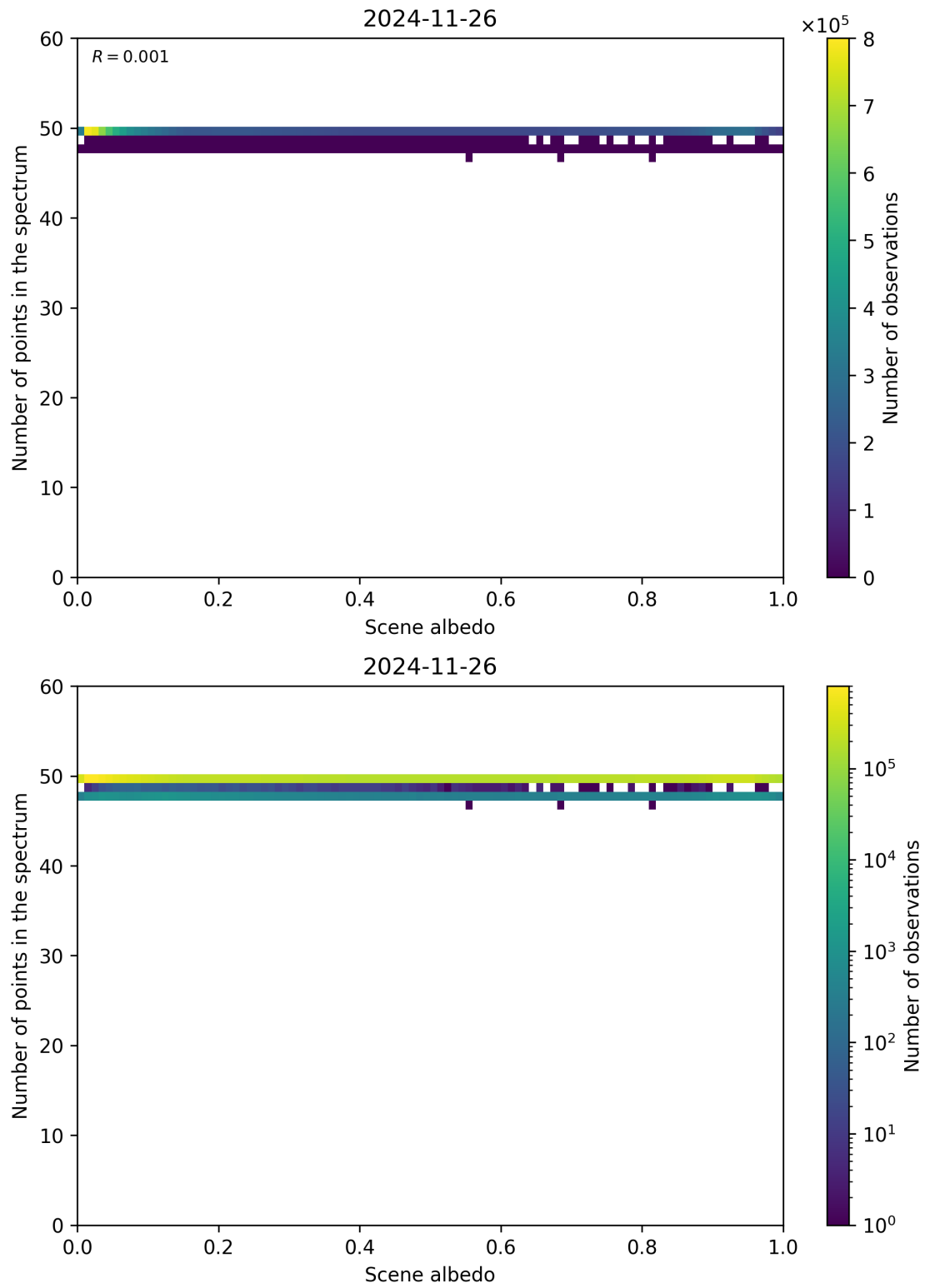
Figure 106: Scatter density plot of “Scene albedo” against “Number of points in the spectrum” for 2024-11-25 to 2024-11-27.
