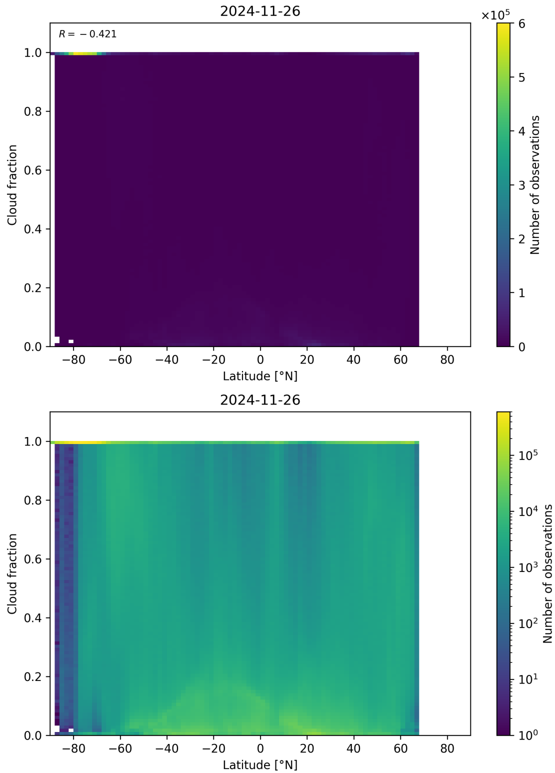
Figure 90: Scatter density plot of “Latitude” against “Cloud fraction” for 2024-11-25 to 2024-11-27.
