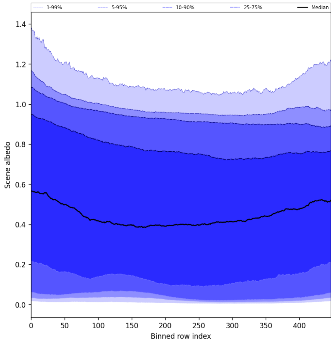
Figure 51: Along track statistics of “Scene albedo” for 2024-11-25 to 2024-11-27
