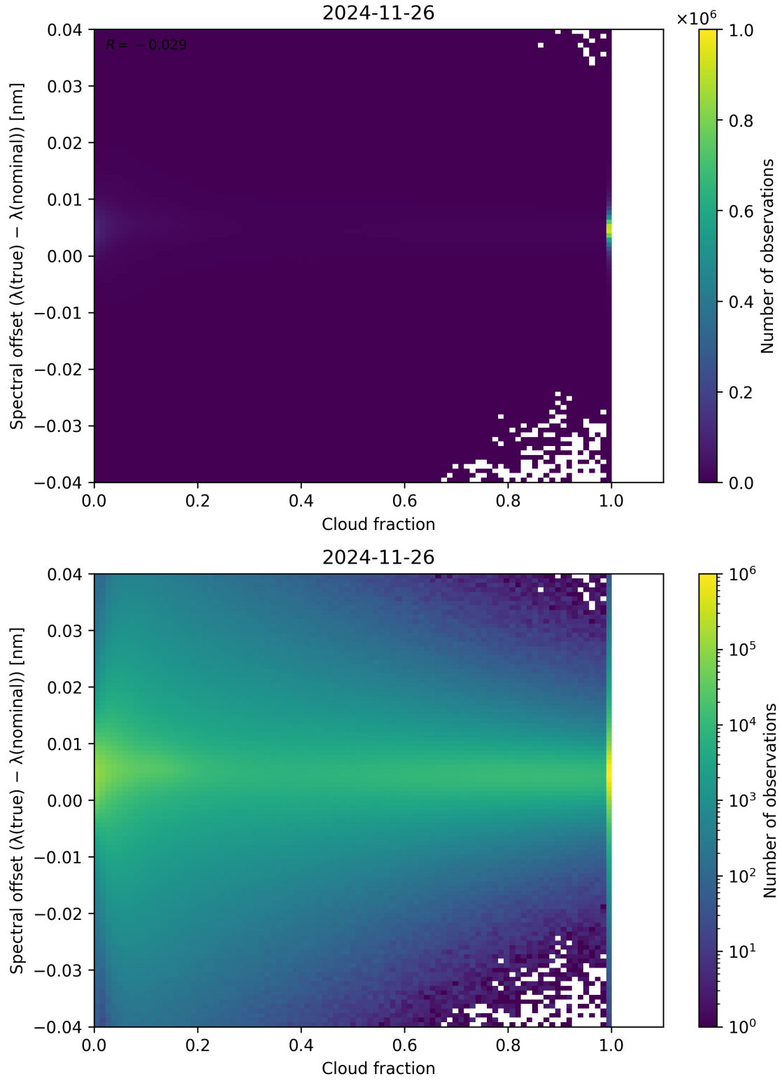
Figure 76: Scatter density plot of “Cloud fraction” against “Spectral offset ( \lambda_{\text{true}} - \lambda_{\text{nominal}} )” for 2024-11-25 to 2024-11-27.
