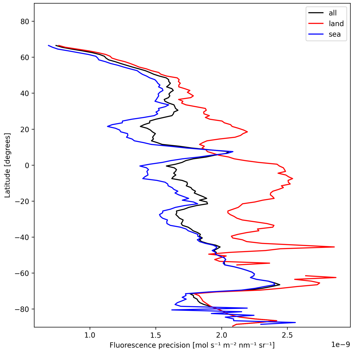
Figure 24: Zonal average of “Fluorescence precision” for 2024-11-25 to 2024-11-27.
