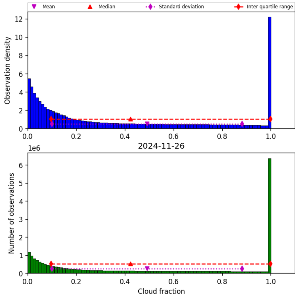
Figure 32: Histogram of “Cloud fraction” for 2024-11-25 to 2024-11-27
