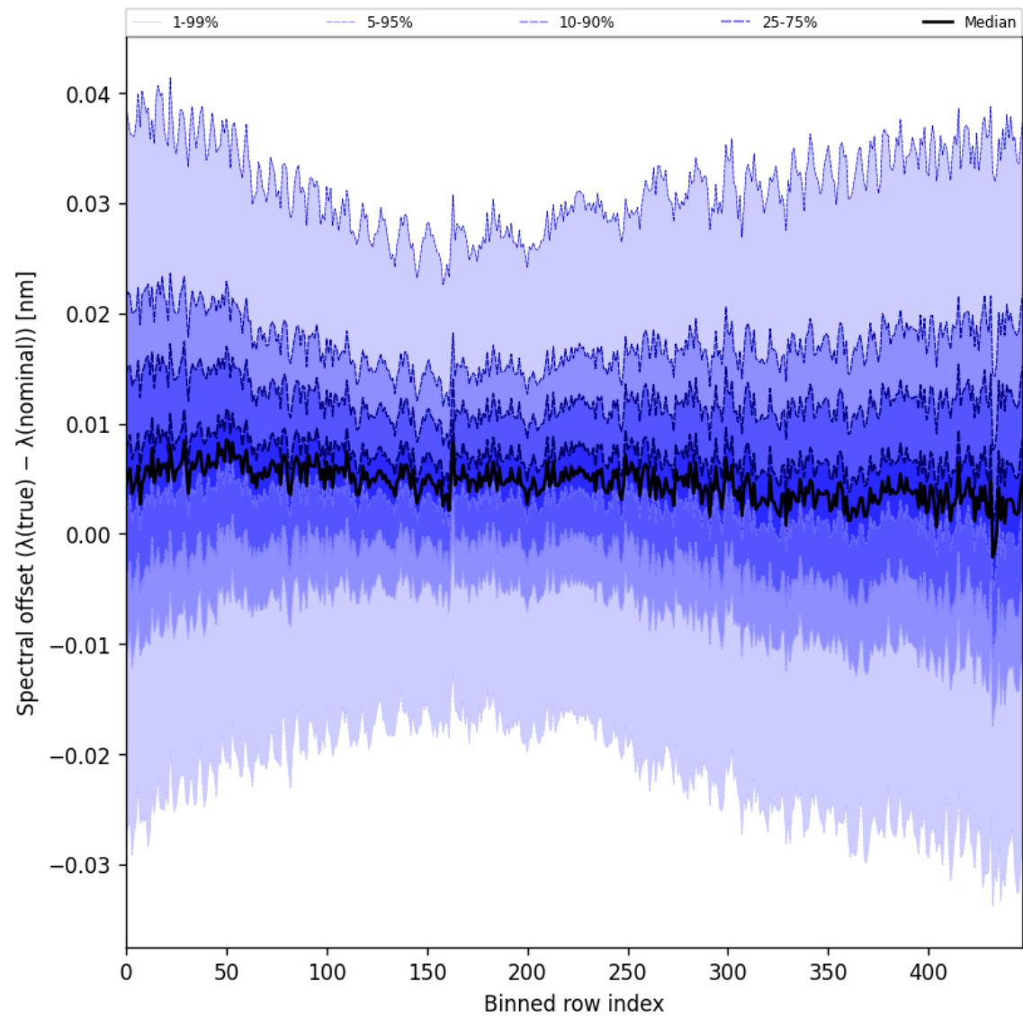
Figure 62: Along track statistics of “Spectral offset ( \lambda_{\text{true}} - \lambda_{\text{nominal}} )” for 2024-11-25 to 2024-11-27
