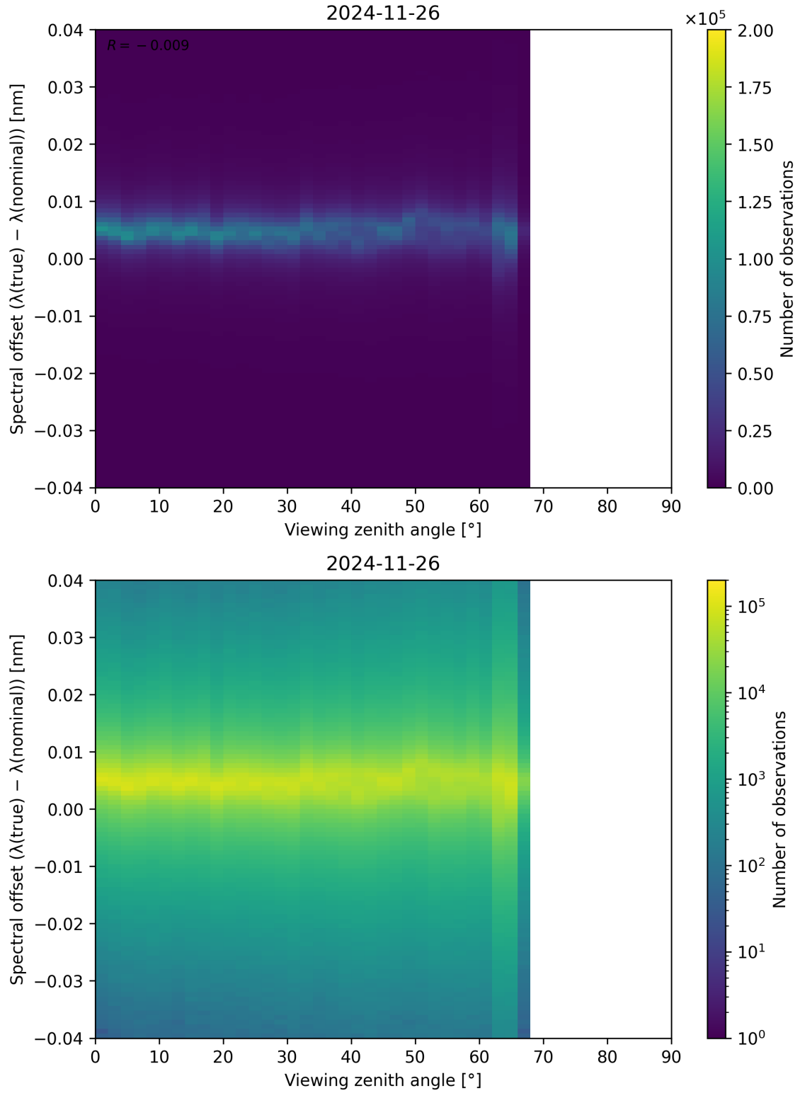
Figure 128: Scatter density plot of “Viewing zenith angle” against “Spectral offset ( \lambda_{\text{true}} - \lambda_{\text{nominal}} )” for 2024-11-25 to 2024-11-27.
