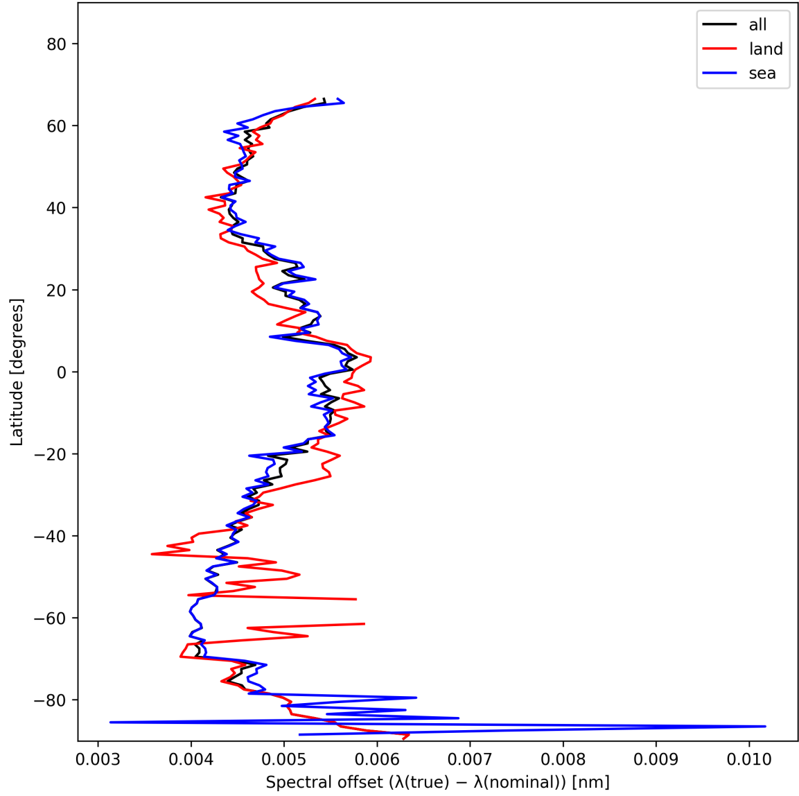
Figure 28: Zonal average of “Spectral offset ( \lambda_{\text{true}} - \lambda_{\text{nominal}} )” for 2024-11-25 to 2024-11-27.
