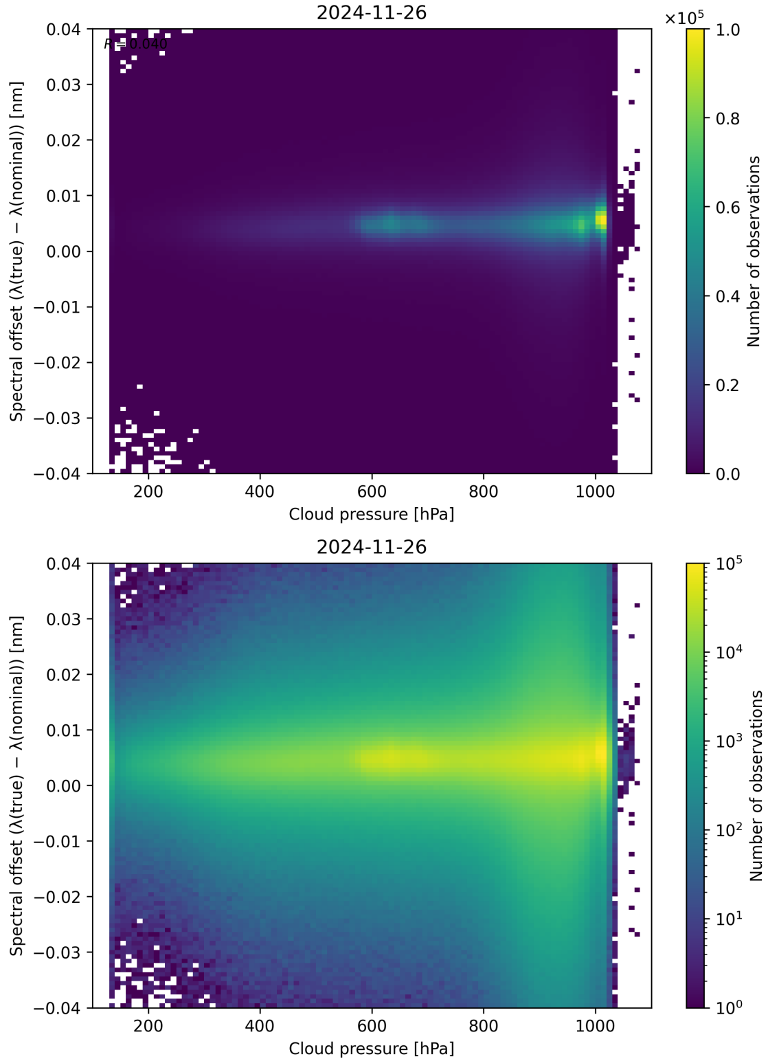
Figure 84: Scatter density plot of “Cloud pressure” against “Spectral offset ( \lambda_{\text{true}} - \lambda_{\text{nominal}} )” for 2024-11-25 to 2024-11-27.
