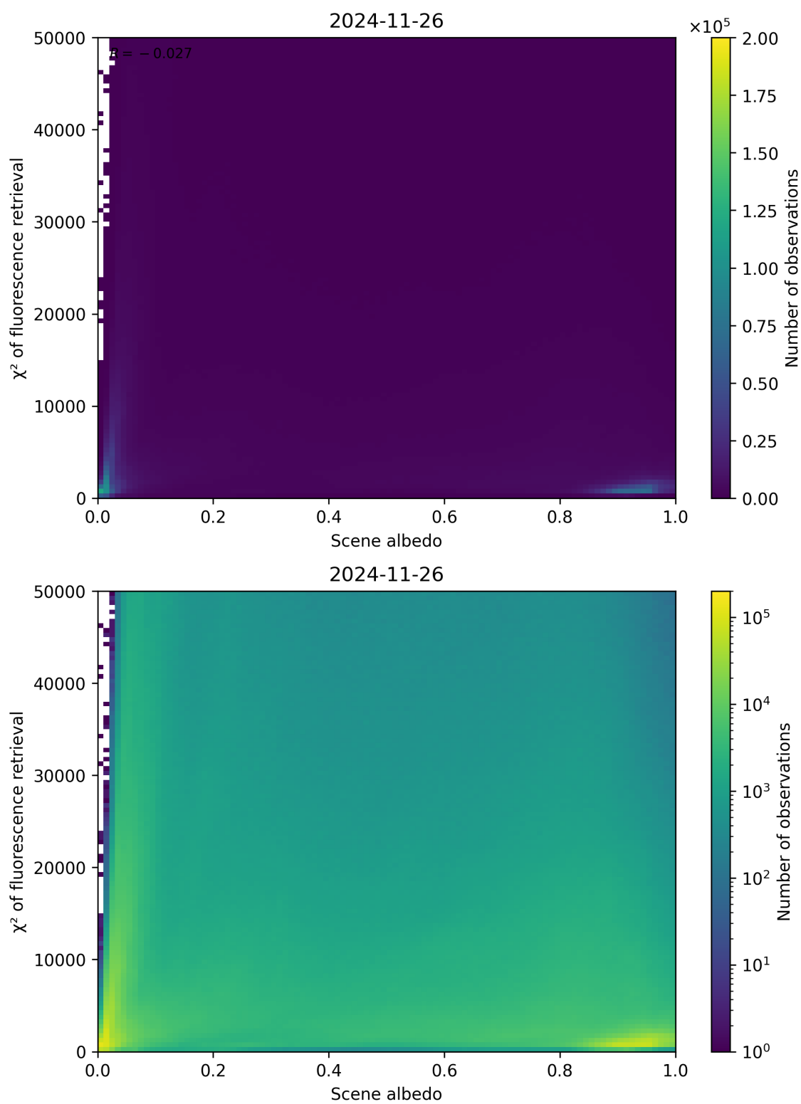
Figure 103: Scatter density plot of “Scene albedo” against “ \chi^2 of fluorescence retrieval” for 2024-11-25 to 2024-11-27.
