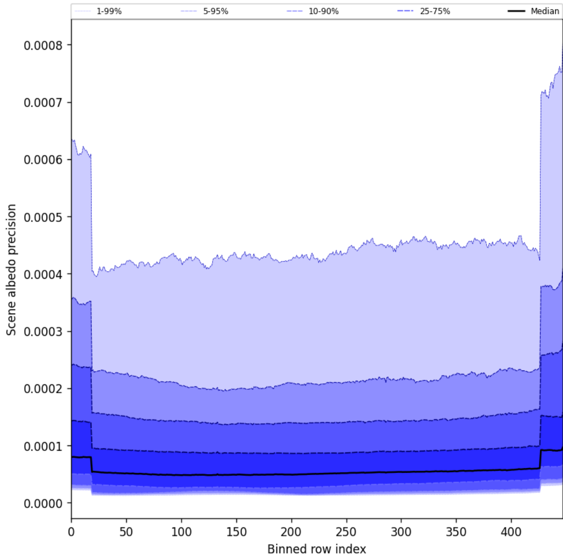
Figure 52: Along track statistics of “Scene albedo precision” for 2024-11-25 to 2024-11-27
