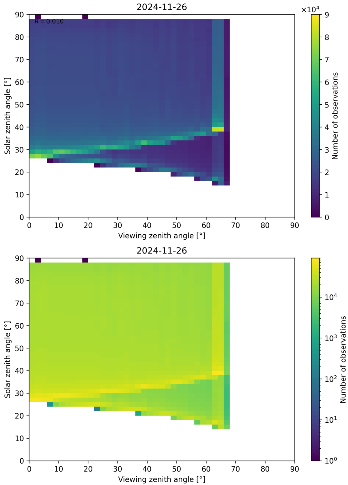
Figure 127: Scatter density plot of “Viewing zenith angle” against “Solar zenith angle” for 2024-11-25 to 2024-11-27.
