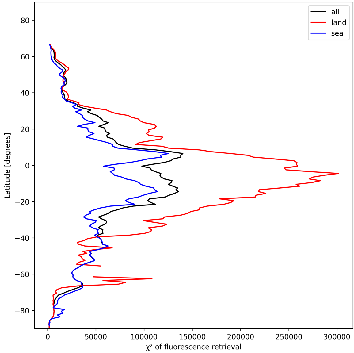
Figure 25: Zonal average of “ \chi^2 of fluorescence retrieval” for 2024-11-25 to 2024-11-27.
