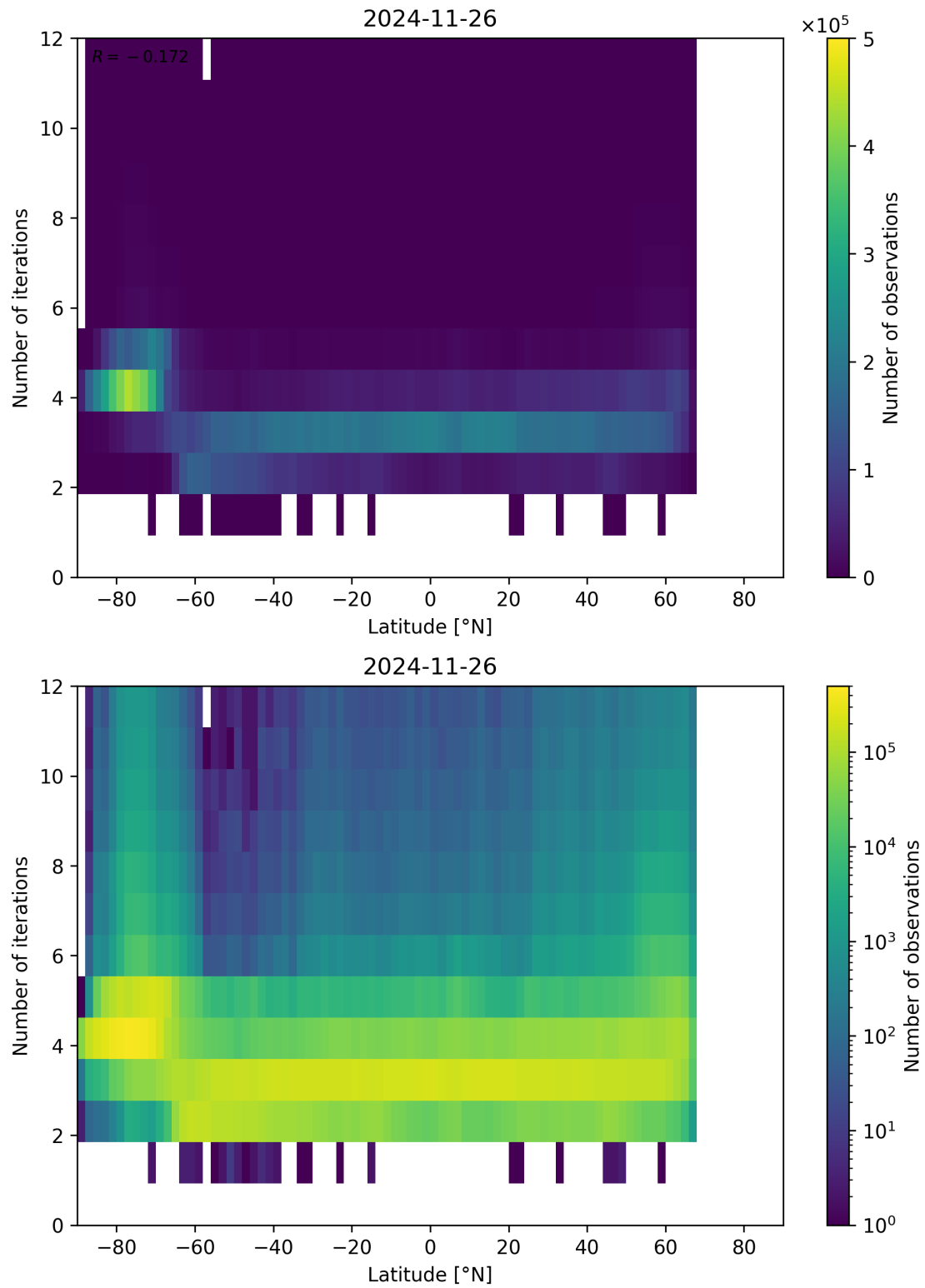
Figure 93: Scatter density plot of “Latitude” against “Number of iterations” for 2024-11-25 to 2024-11-27.
