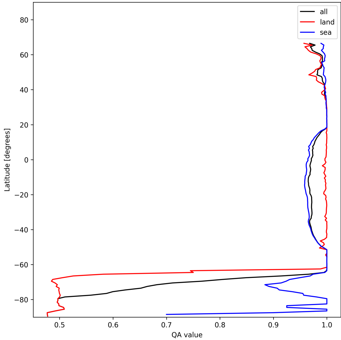
Figure 12: Zonal average of “QA value” for 2024-11-25 to 2024-11-27.
