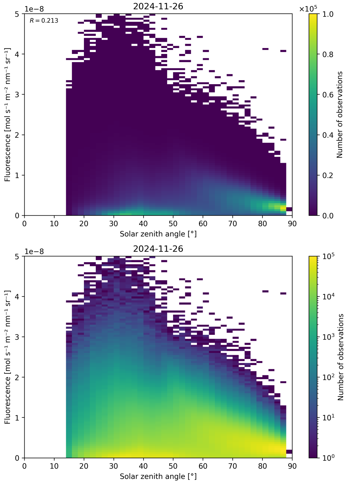
Figure 112: Scatter density plot of “Solar zenith angle” against “Fluorescence” for 2024-11-25 to 2024-11-27.
