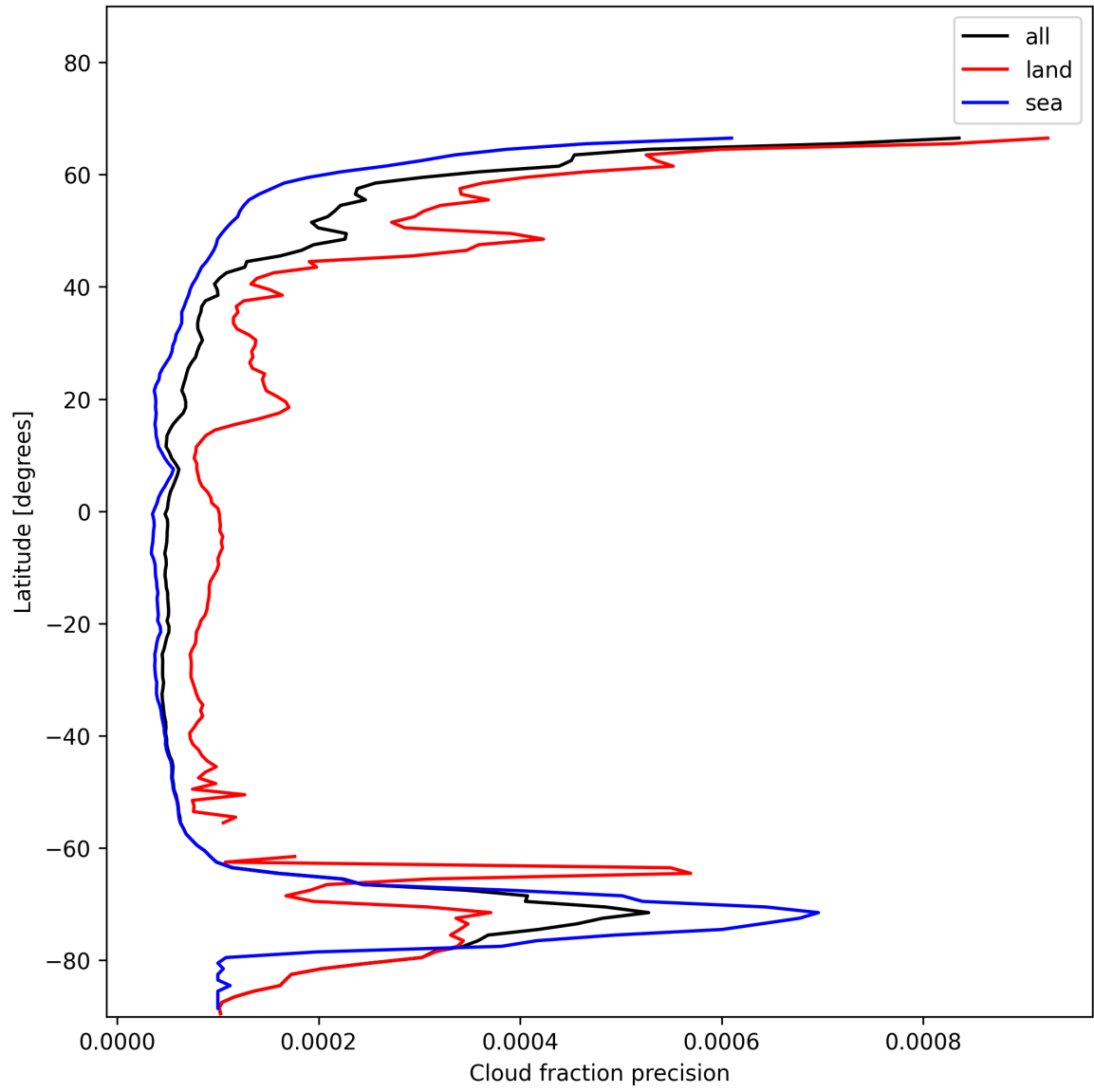
Figure 16: Zonal average of “Cloud fraction precision” for 2024-11-25 to 2024-11-27.
