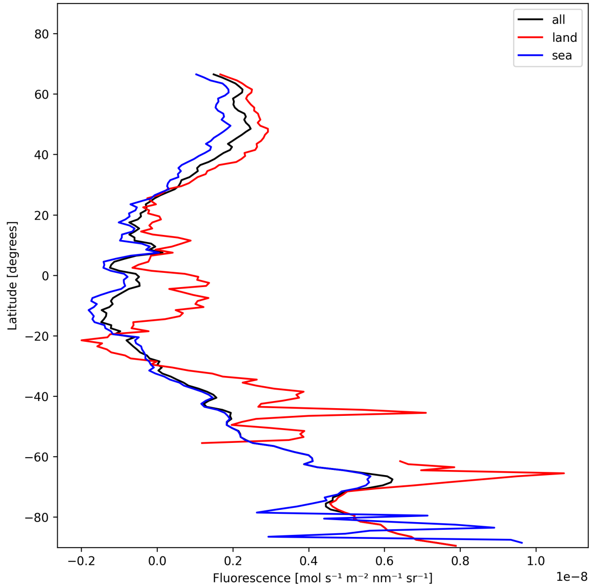
Figure 23: Zonal average of “Fluorescence” for 2024-11-25 to 2024-11-27.
