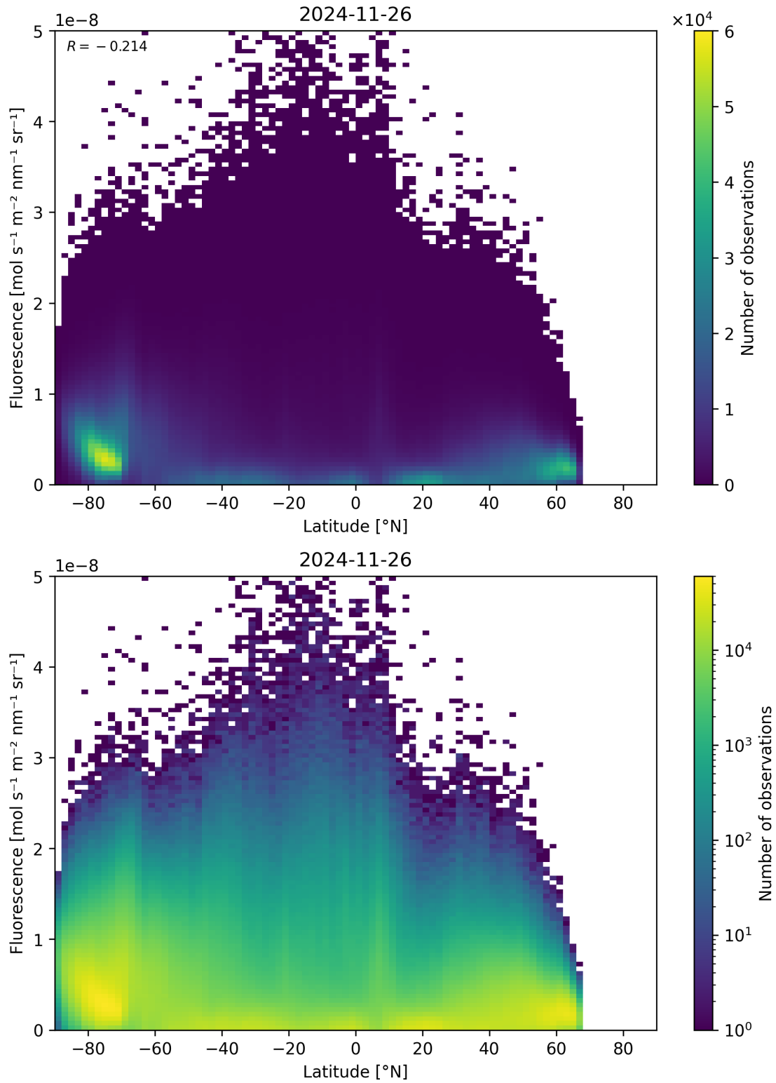
Figure 92: Scatter density plot of “Latitude” against “Fluorescence” for 2024-11-25 to 2024-11-27.
