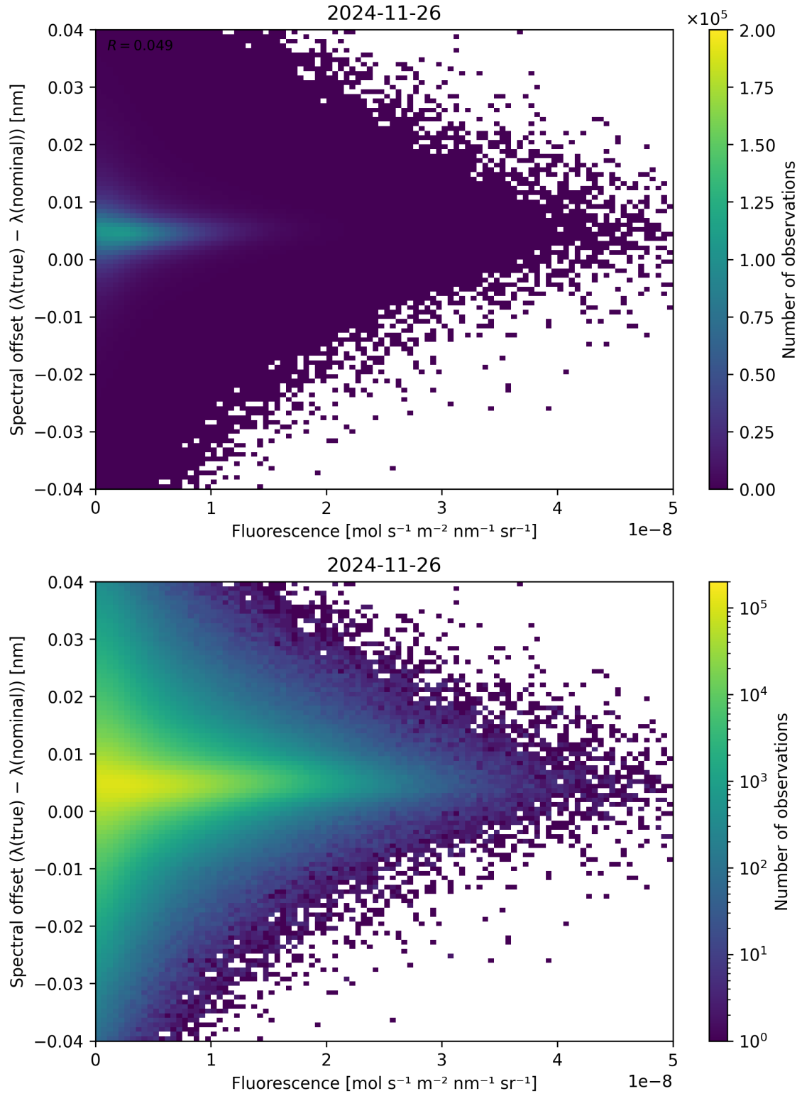
Figure 87: Scatter density plot of “Fluorescence” against “Spectral offset ( \lambda_{\text{true}} - \lambda_{\text{nominal}} )” for 2024-11-25 to 2024-11-27.
