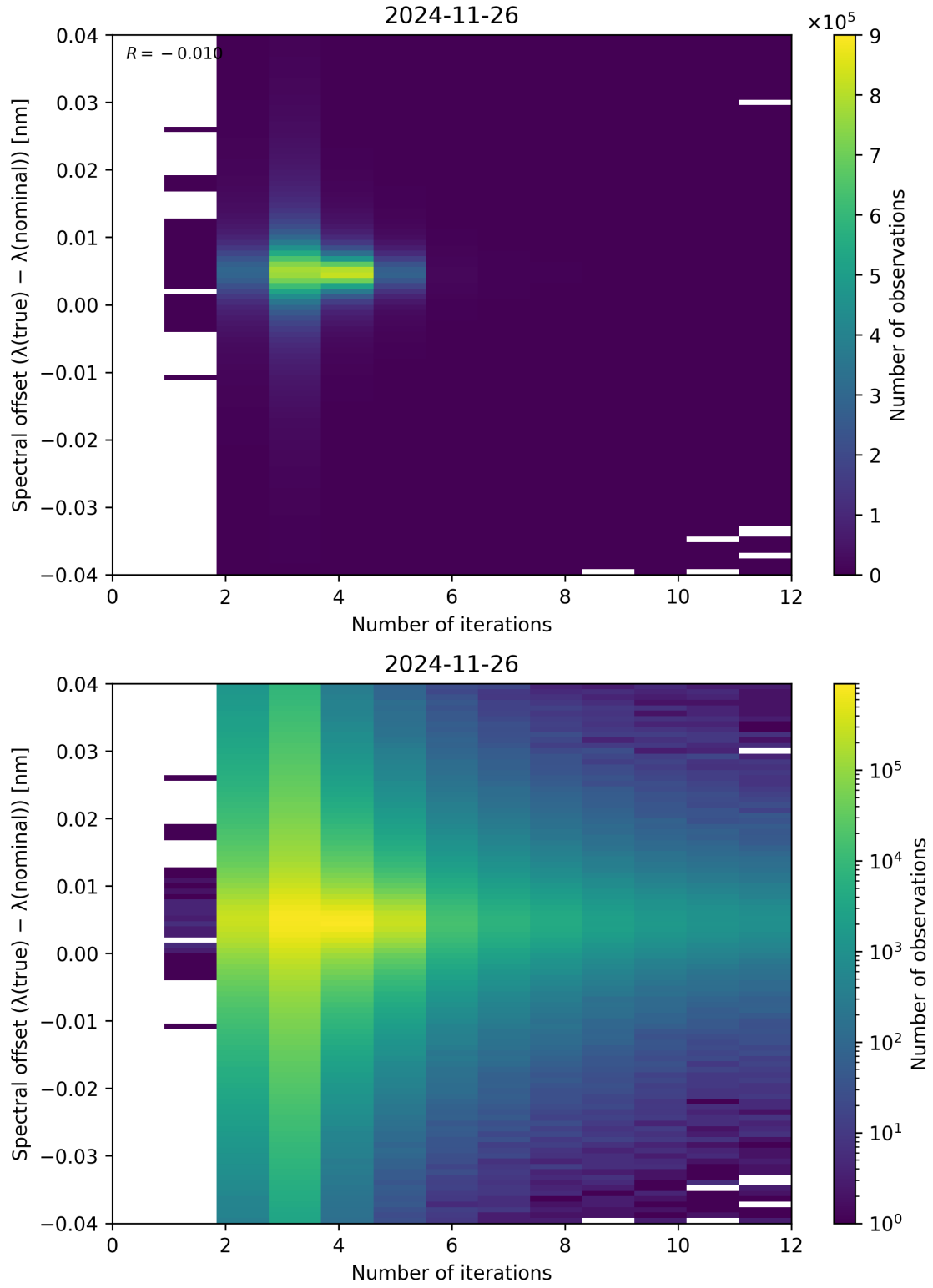
Figure 100: Scatter density plot of “Number of iterations” against “Spectral offset ( \lambda_{\text{true}} - \lambda_{\text{nominal}} )” for 2024-11-25 to 2024-11-27.
