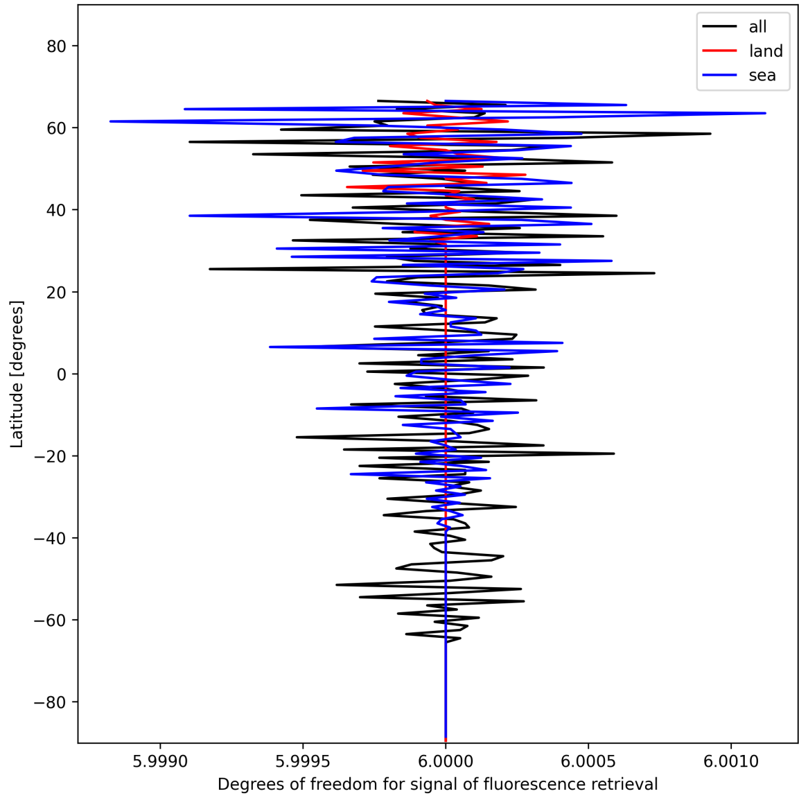
Figure 26: Zonal average of “Degrees of freedom for signal of fluorescence retrieval” for 2024-11-25 to 2024-11-27.
