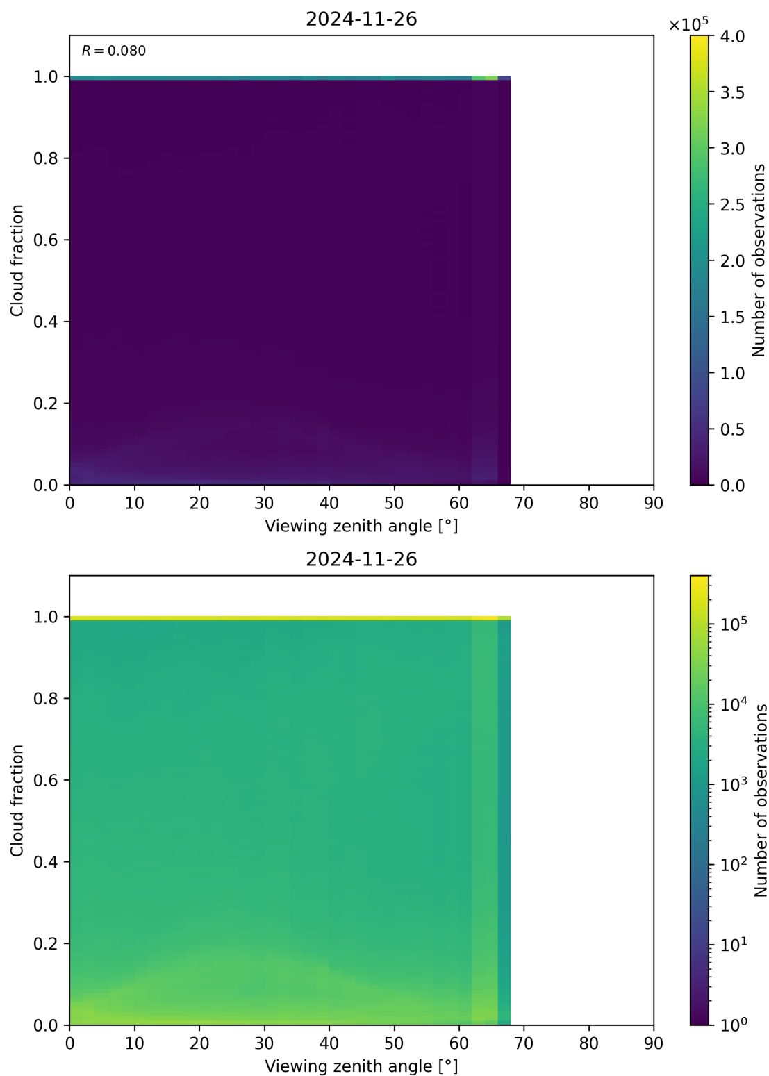
Figure 120: Scatter density plot of “Viewing zenith angle” against “Cloud fraction” for 2024-11-25 to 2024-11-27.
