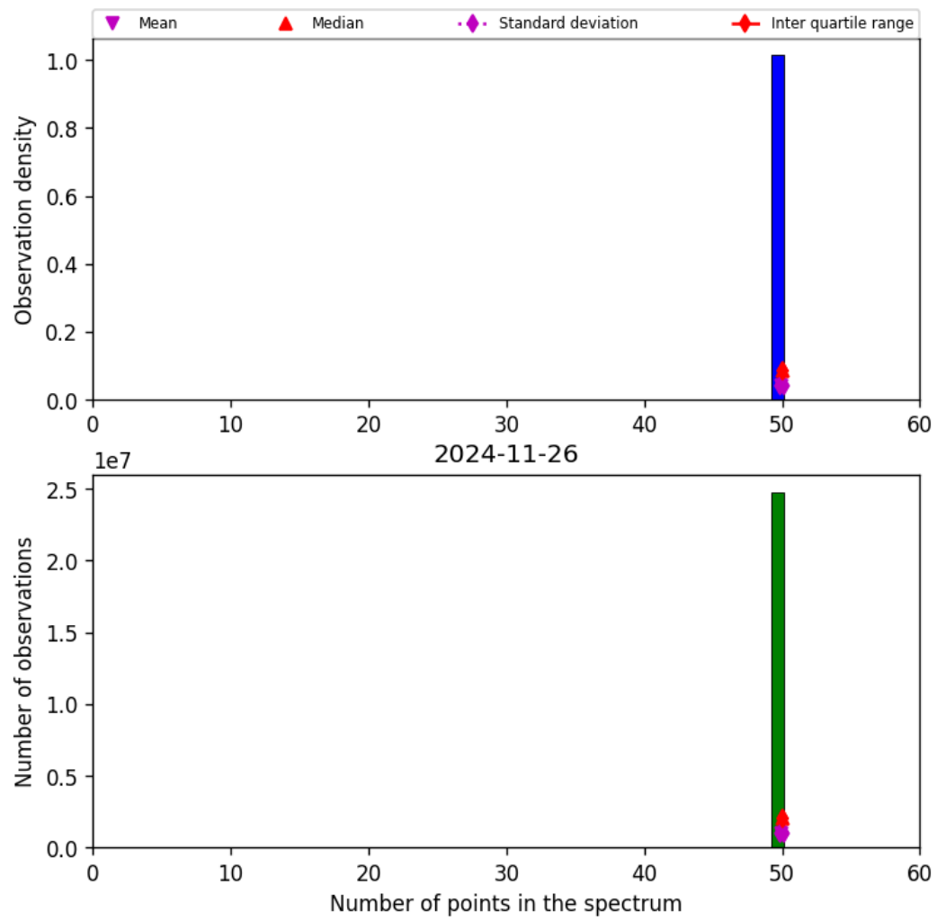
Figure 44: Histogram of “Number of points in the spectrum” for 2024-11-25 to 2024-11-27
