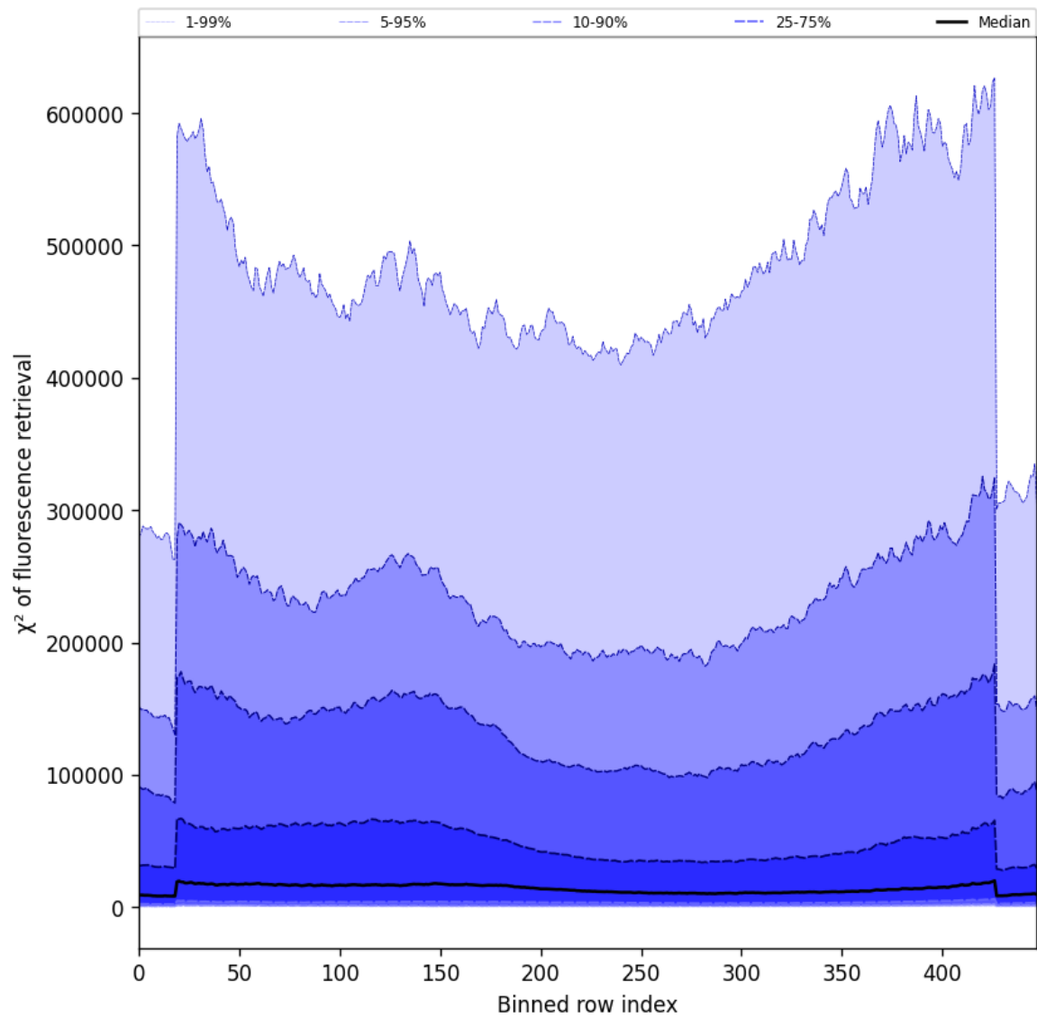
Figure 59: Along track statistics of “ \chi^2 of fluorescence retrieval” for 2024-11-25 to 2024-11-27
