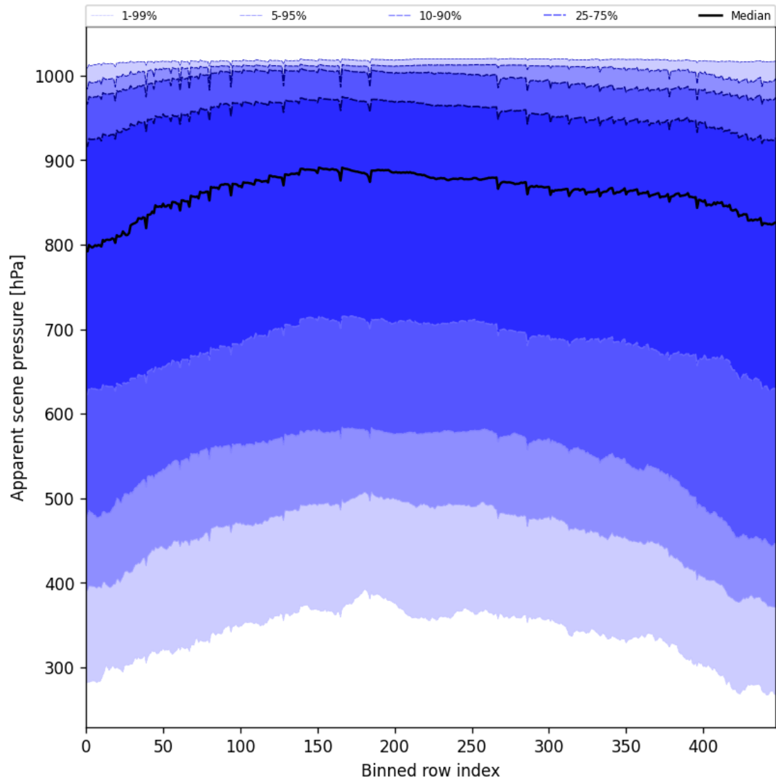
Figure 53: Along track statistics of “Apparent scene pressure” for 2024-11-25 to 2024-11-27
