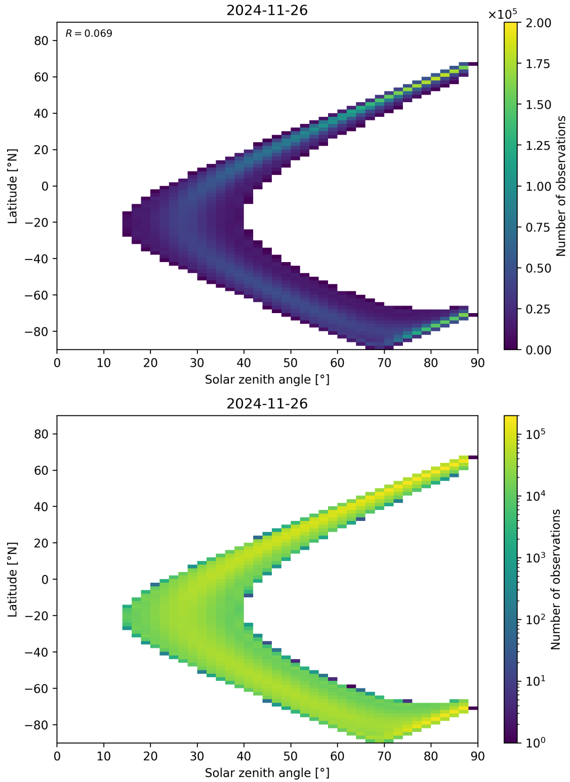
Figure 113: Scatter density plot of “Solar zenith angle” against “Latitude” for 2024-11-25 to 2024-11-27.
