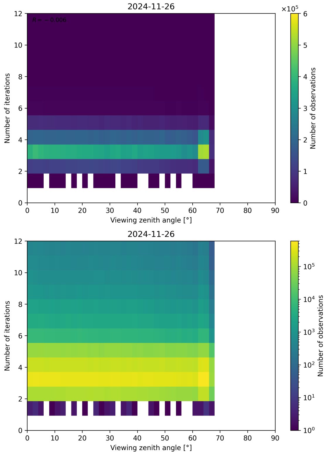
Figure 124: Scatter density plot of “Viewing zenith angle” against “Number of iterations” for 2024-11-25 to 2024-11-27.
