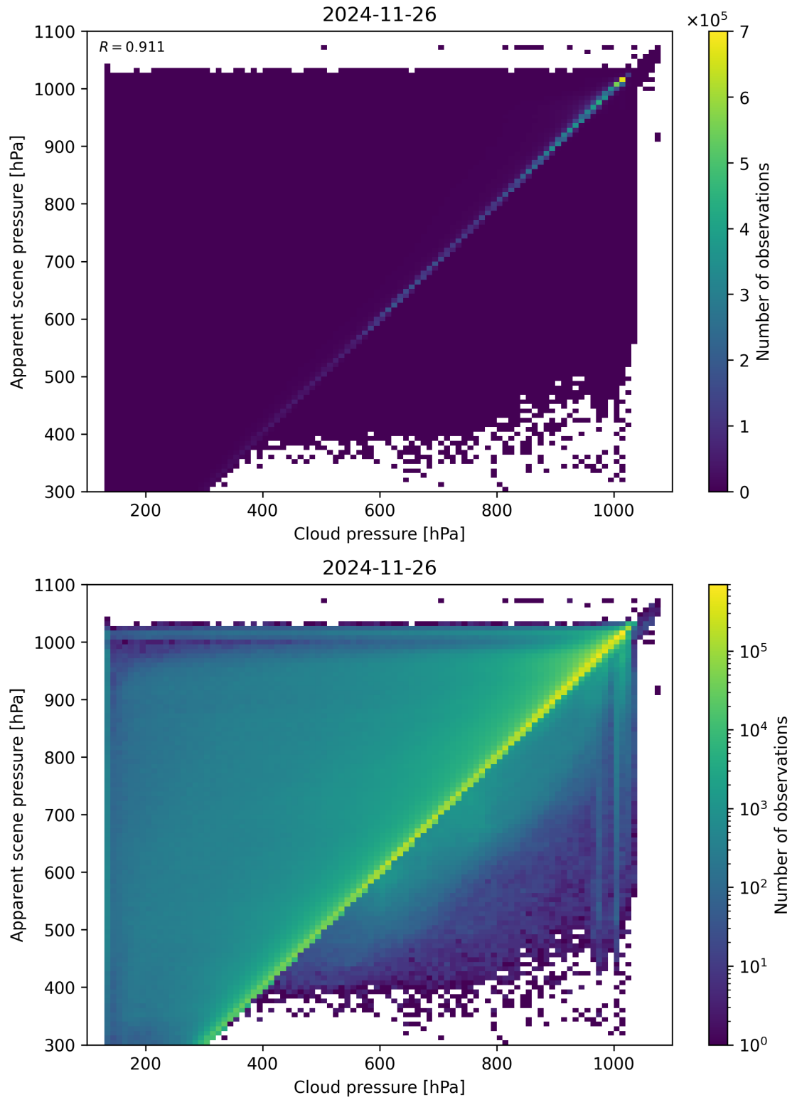
Figure 77: Scatter density plot of “Cloud pressure” against “Apparent scene pressure” for 2024-11-25 to 2024-11-27.
