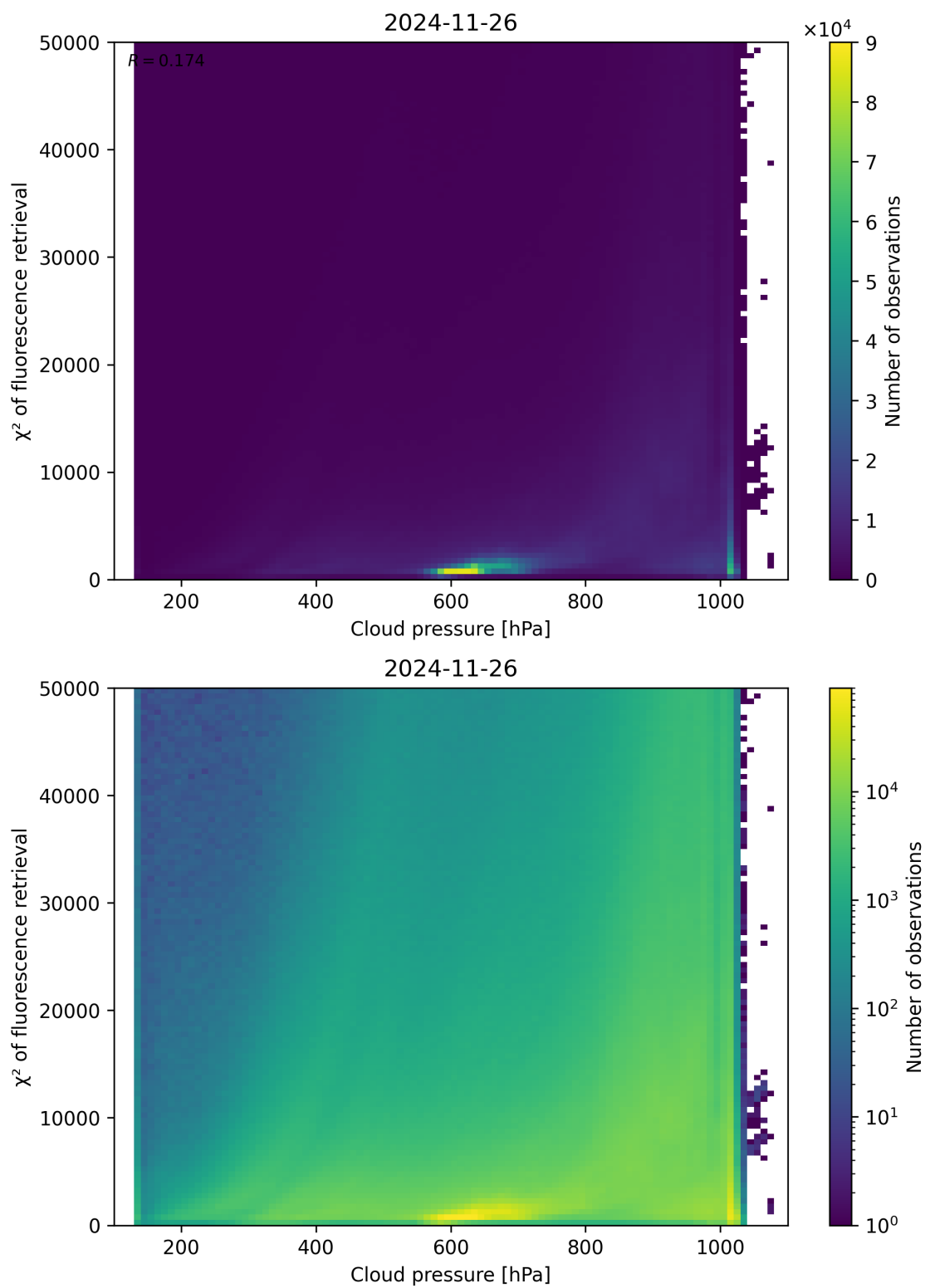
Figure 78: Scatter density plot of “Cloud pressure” against “ \chi^2 of fluorescence retrieval” for 2024-11-25 to 2024-11-27.
