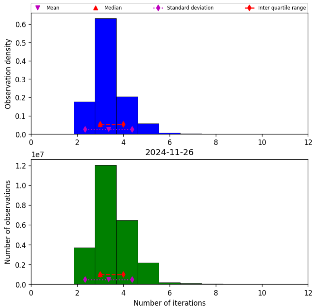
Figure 39: Histogram of “Number of iterations” for 2024-11-25 to 2024-11-27
