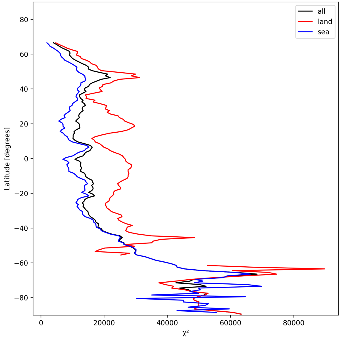
Figure 21: Zonal average of “ \chi^2 ” for 2024-11-25 to 2024-11-27.
