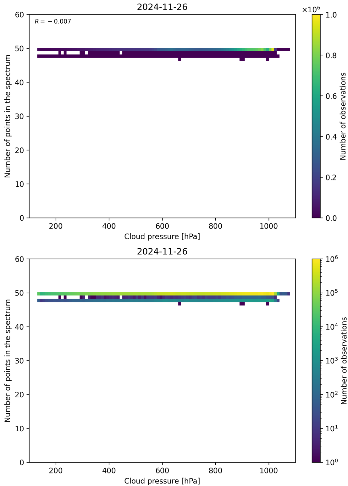
Figure 82: Scatter density plot of “Cloud pressure” against “Number of points in the spectrum” for 2024-11-25 to 2024-11-27.
