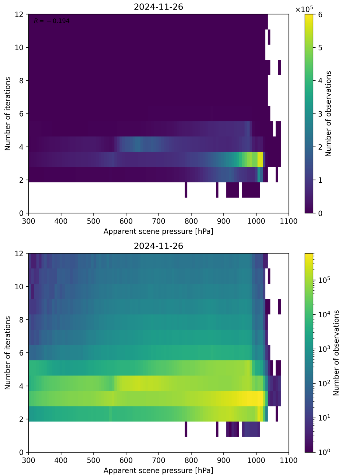
Figure 65: Scatter density plot of “Apparent scene pressure” against “Number of iterations” for 2024-11-25 to 2024-11-27.
