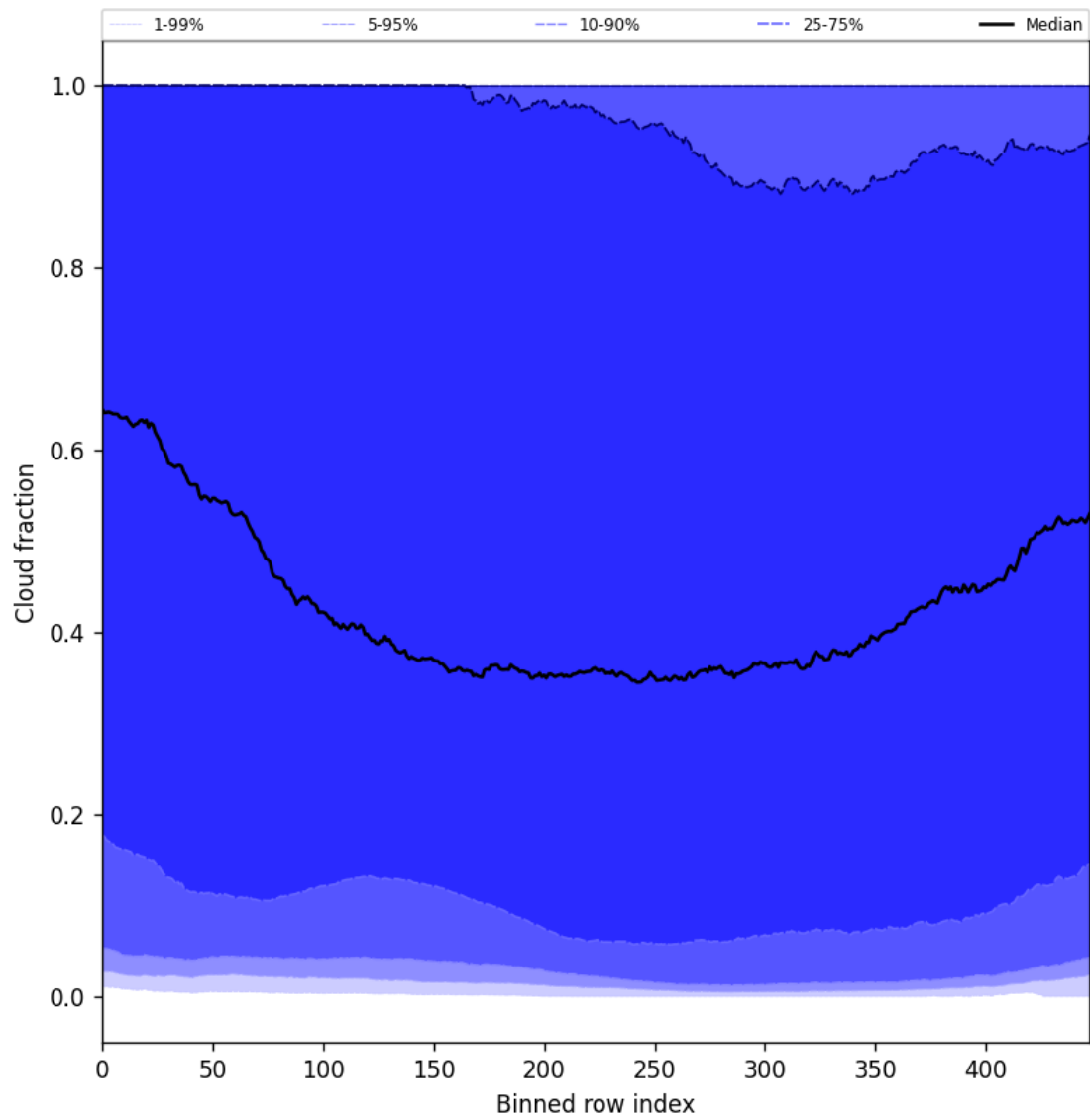
Figure 49: Along track statistics of “Cloud fraction” for 2024-11-25 to 2024-11-27
