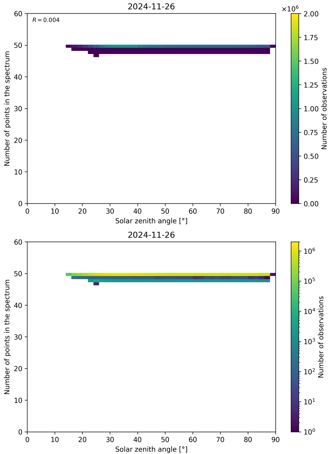
Figure 115: Scatter density plot of “Solar zenith angle” against “Number of points in the spectrum” for 2024-11-25 to 2024-11-27.
