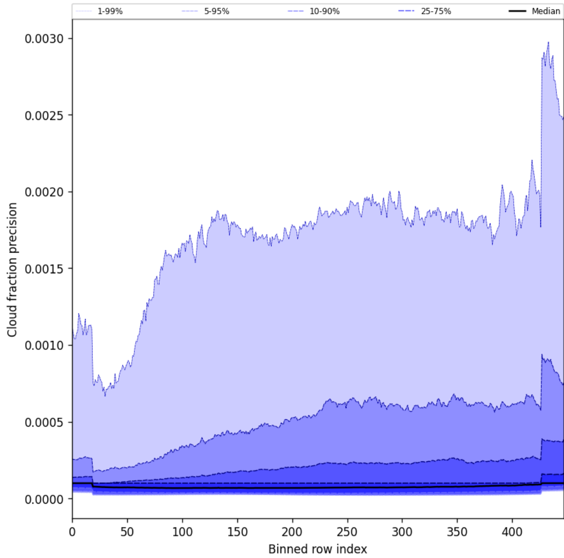
Figure 50: Along track statistics of “Cloud fraction precision” for 2024-11-25 to 2024-11-27
