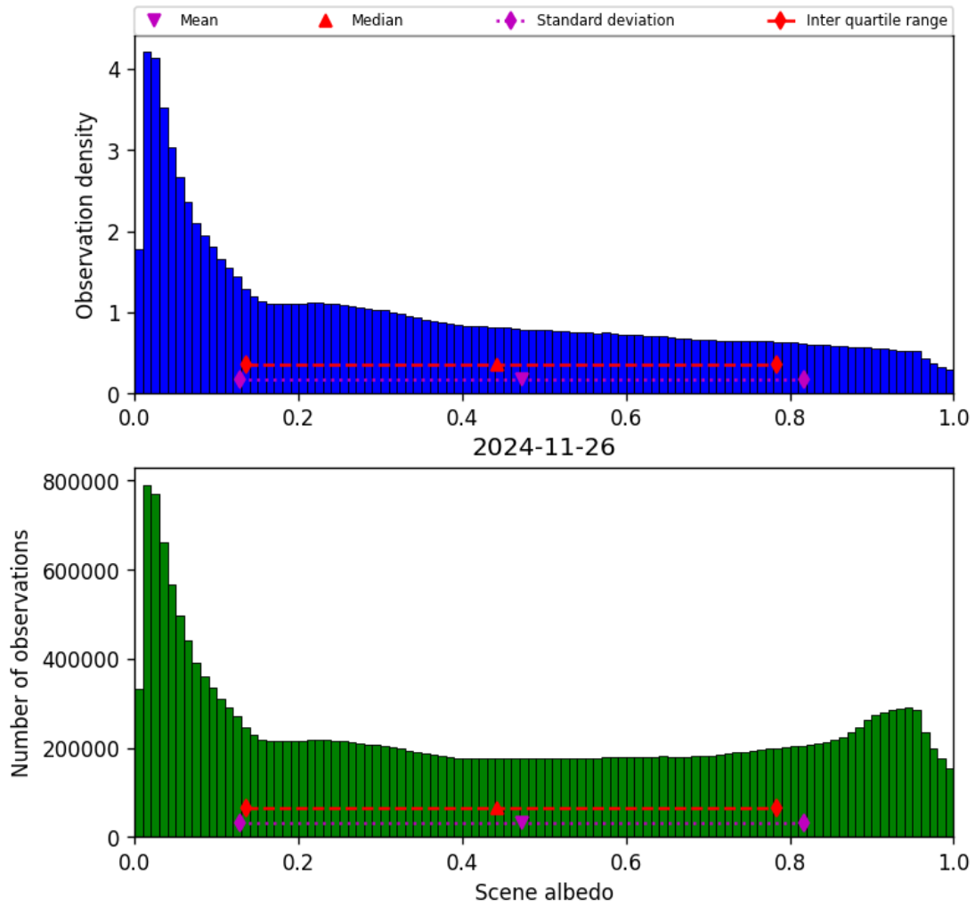
Figure 34: Histogram of “Scene albedo” for 2024-11-25 to 2024-11-27
