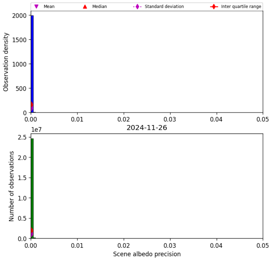
Figure 35: Histogram of “Scene albedo precision” for 2024-11-25 to 2024-11-27
