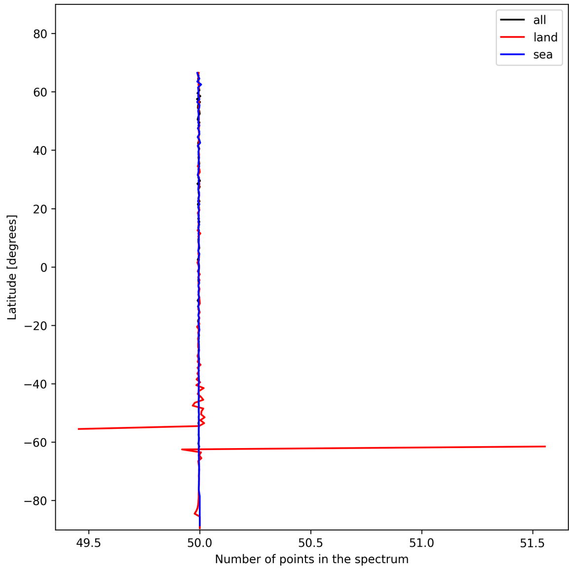
Figure 27: Zonal average of “Number of points in the spectrum” for 2024-11-25 to 2024-11-27.
