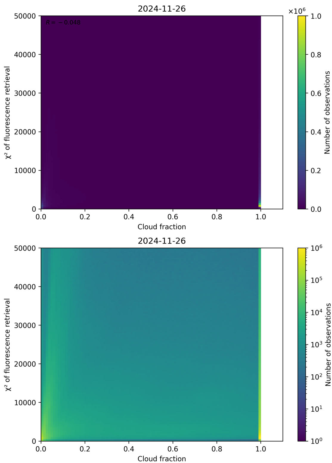
Figure 71: Scatter density plot of “Cloud fraction” against “ \chi^2 of fluorescence retrieval” for 2024-11-25 to 2024-11-27.
