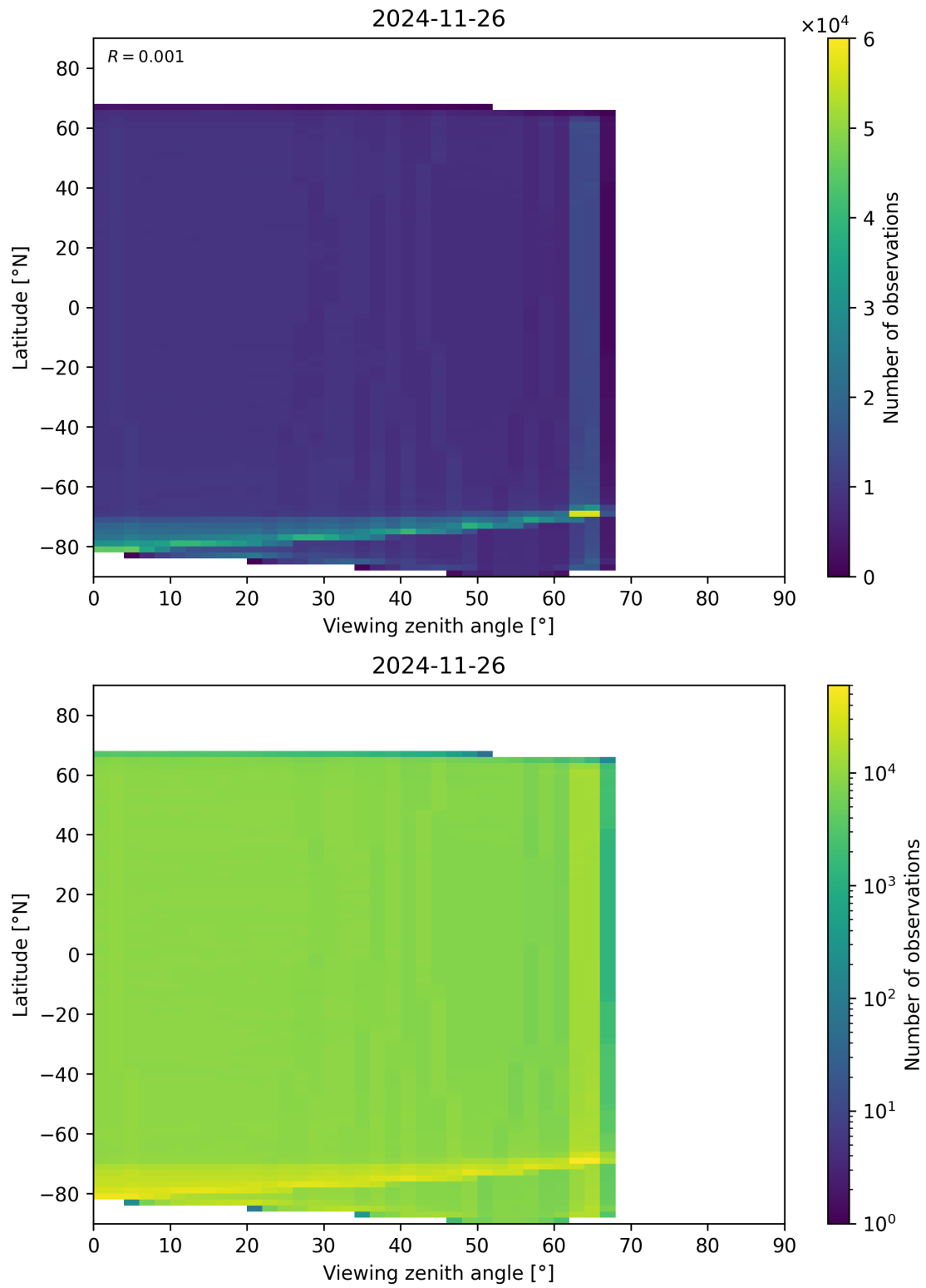
Figure 123: Scatter density plot of “Viewing zenith angle” against “Latitude” for 2024-11-25 to 2024-11-27.
