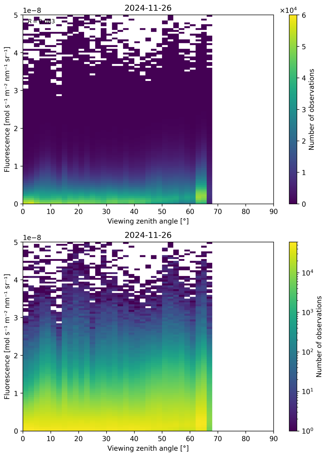
Figure 122: Scatter density plot of “Viewing zenith angle” against “Fluorescence” for 2024-11-25 to 2024-11-27.
