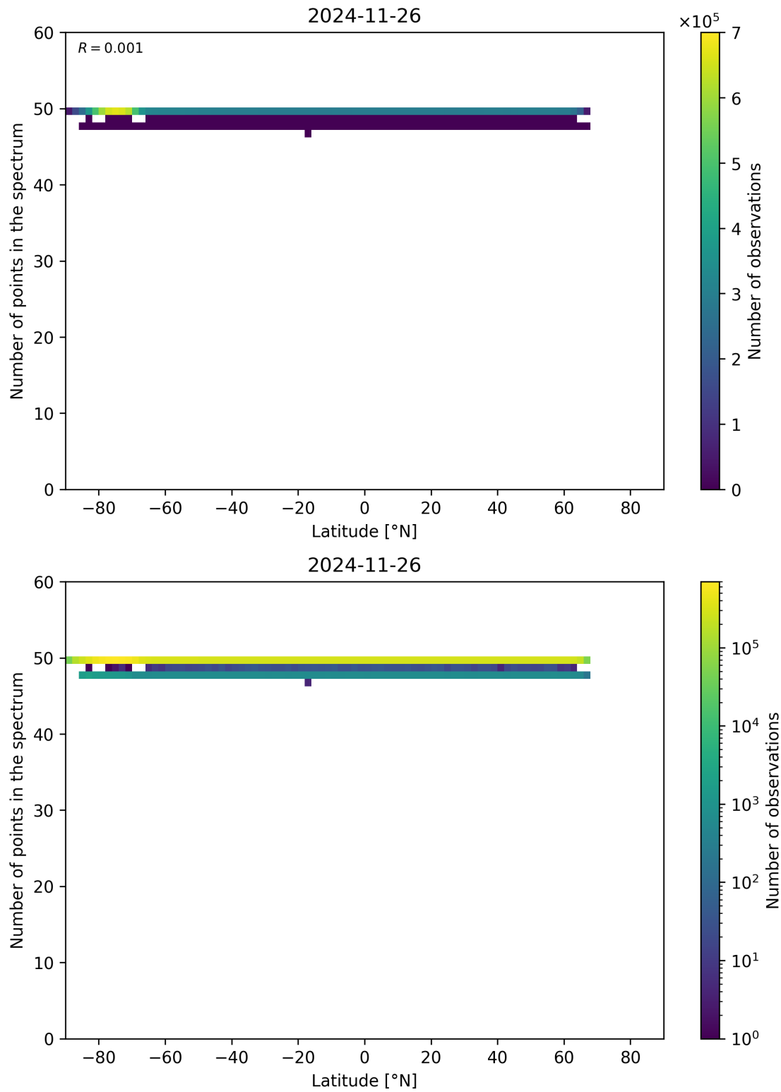
Figure 94: Scatter density plot of “Latitude” against “Number of points in the spectrum” for 2024-11-25 to 2024-11-27.
