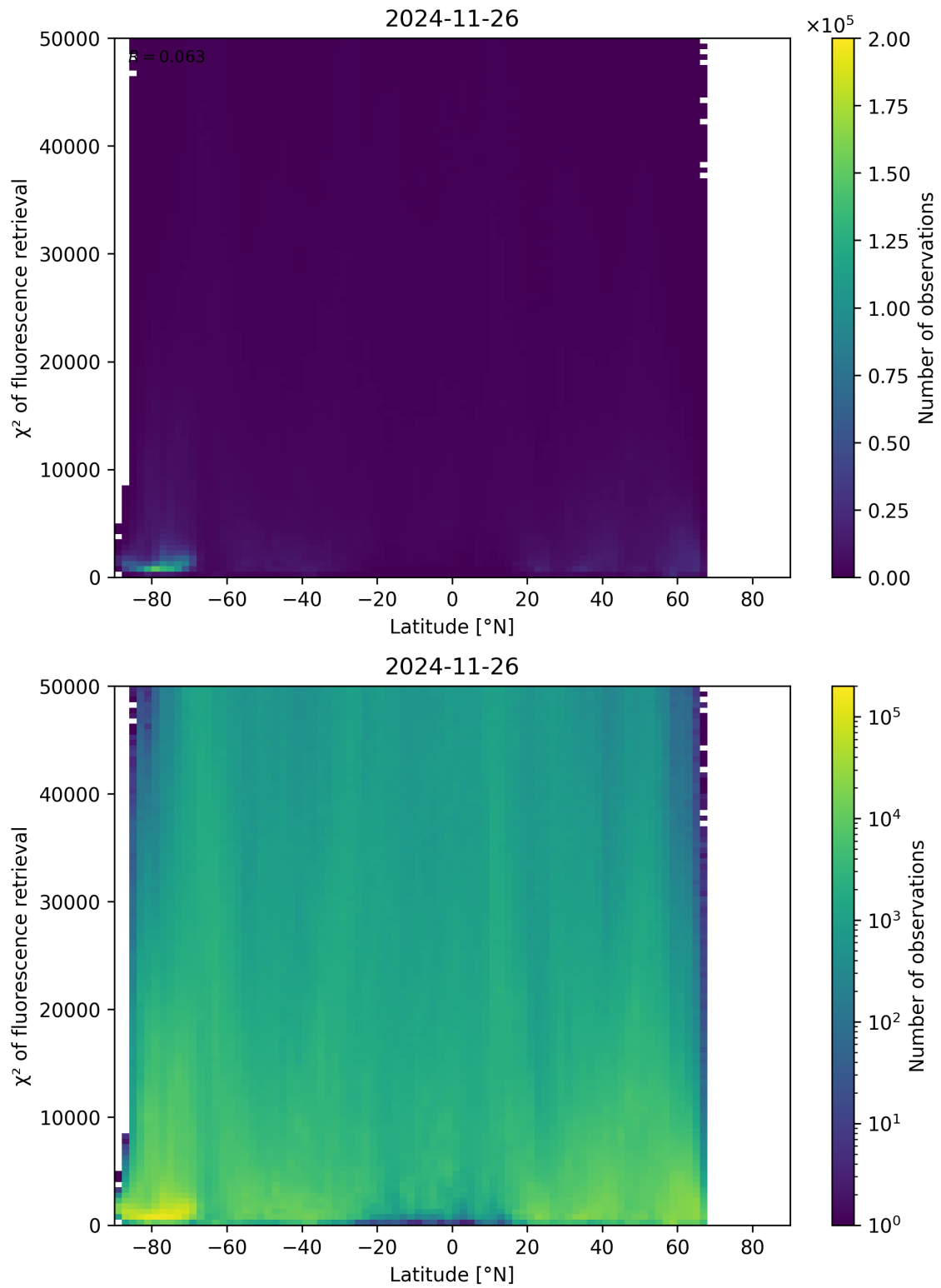
Figure 89: Scatter density plot of “Latitude” against “ \chi^2 of fluorescence retrieval” for 2024-11-25 to 2024-11-27.
