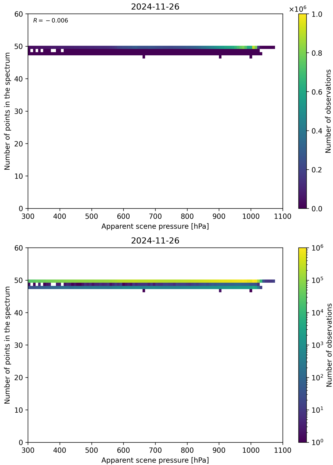
Figure 66: Scatter density plot of “Apparent scene pressure” against “Number of points in the spectrum” for 2024-11-25 to 2024-11-27.
