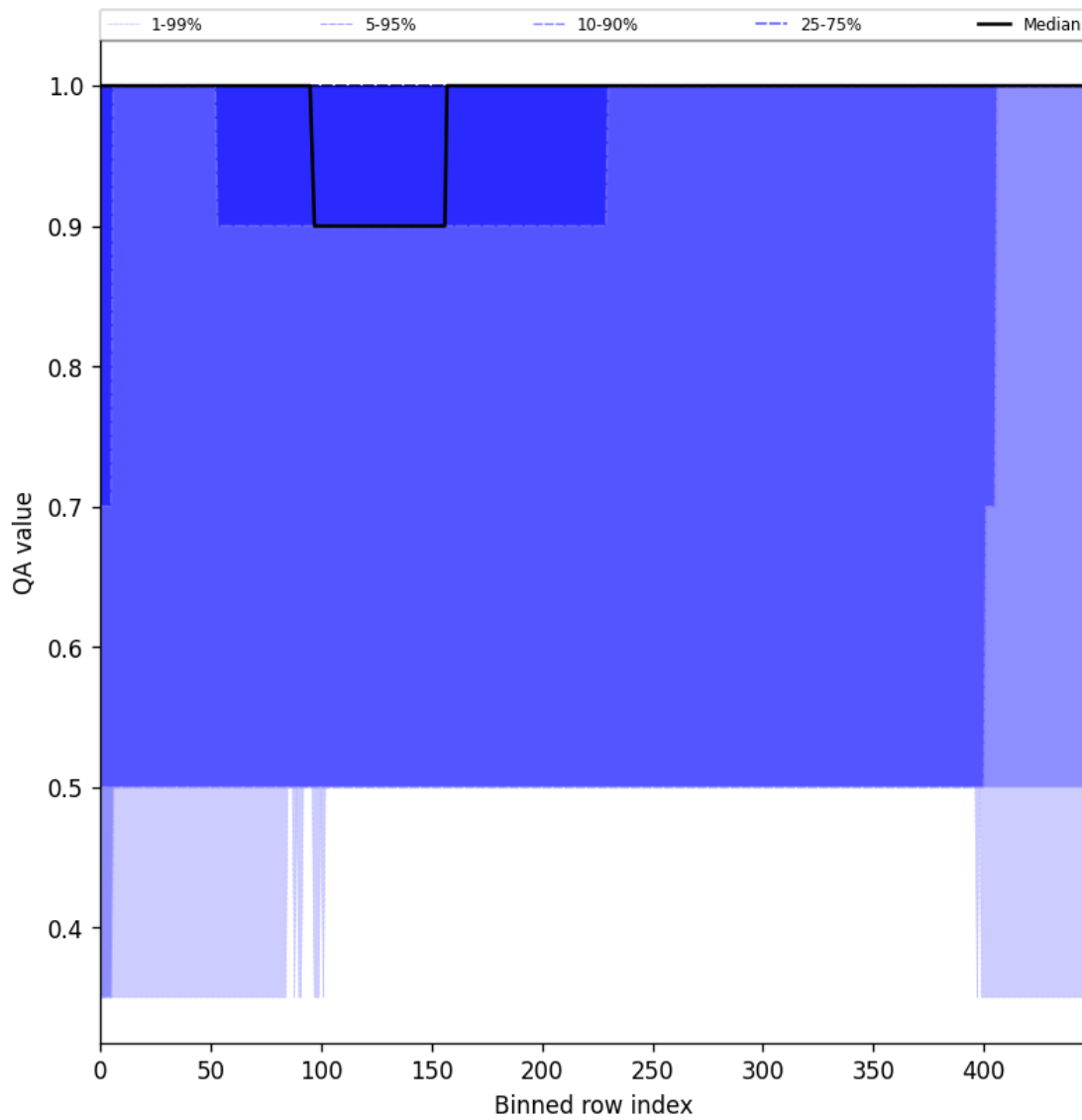
Figure 46: Along track statistics of “QA value” for 2024-11-25 to 2024-11-27
