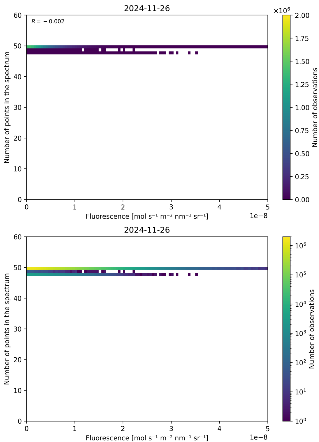
Figure 86: Scatter density plot of “Fluorescence” against “Number of points in the spectrum” for 2024-11-25 to 2024-11-27.
