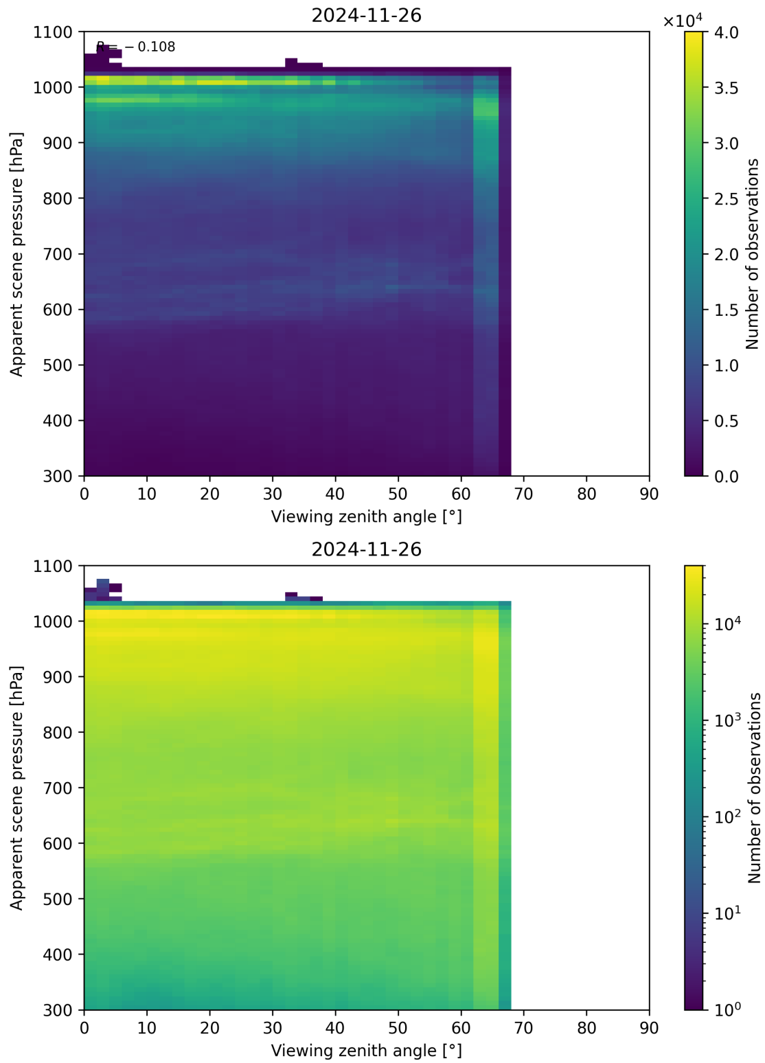
Figure 118: Scatter density plot of “Viewing zenith angle” against “Apparent scene pressure” for 2024-11-25 to 2024-11-27.
