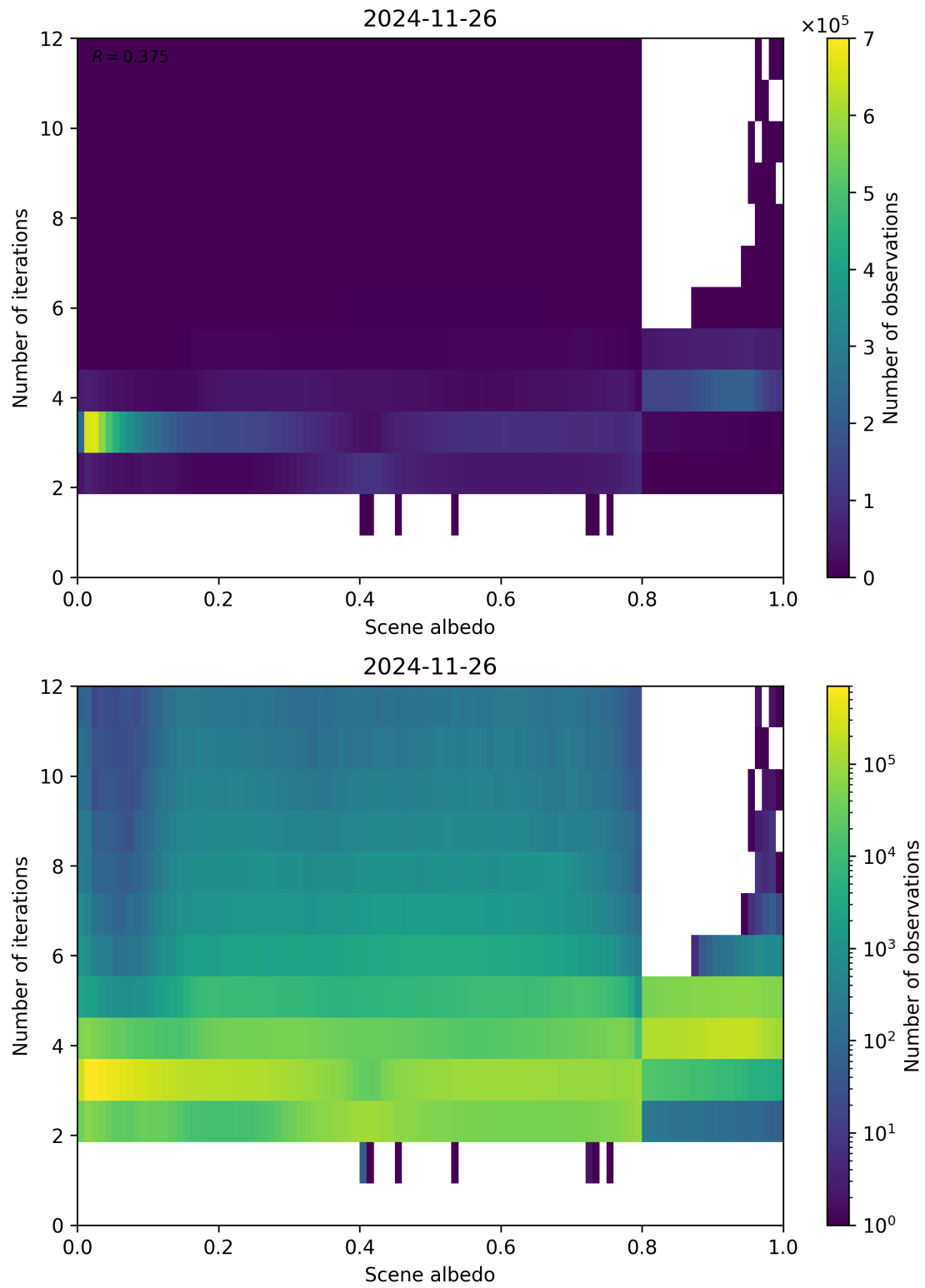
Figure 105: Scatter density plot of “Scene albedo” against “Number of iterations” for 2024-11-25 to 2024-11-27.
