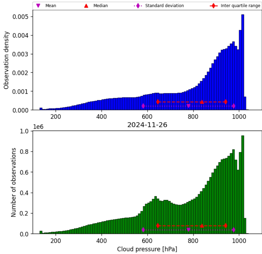
Figure 30: Histogram of “Cloud pressure” for 2024-11-25 to 2024-11-27
