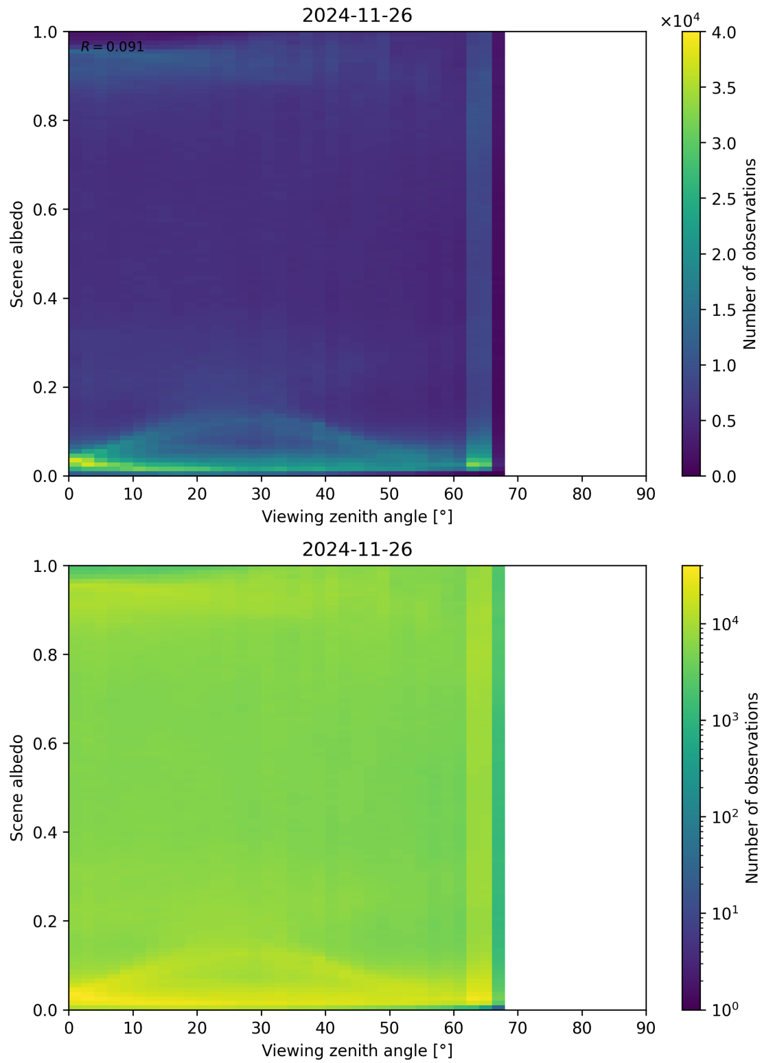
Figure 126: Scatter density plot of “Viewing zenith angle” against “Scene albedo” for 2024-11-25 to 2024-11-27.
