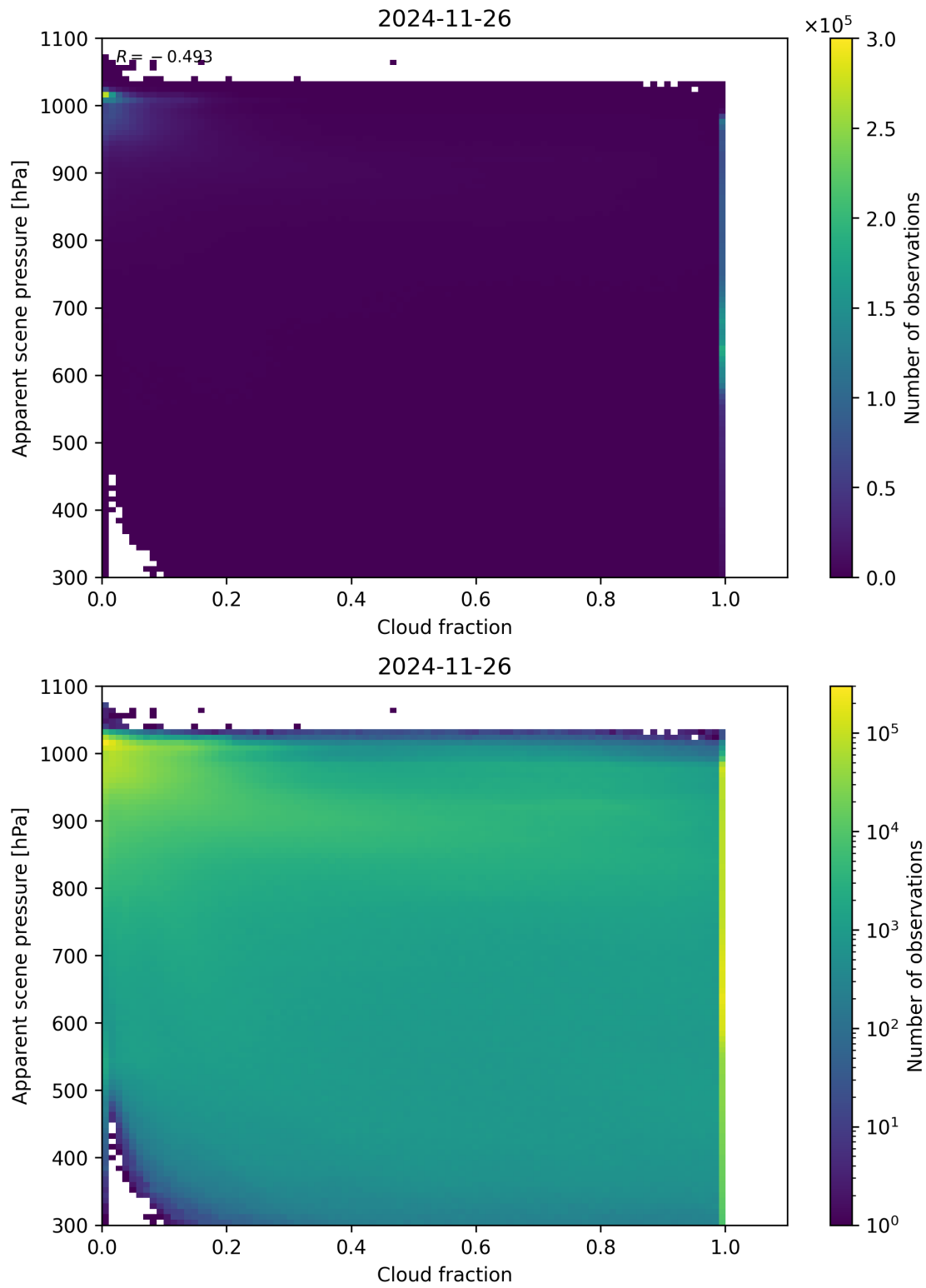
Figure 70: Scatter density plot of “Cloud fraction” against “Apparent scene pressure” for 2024-11-25 to 2024-11-27.
