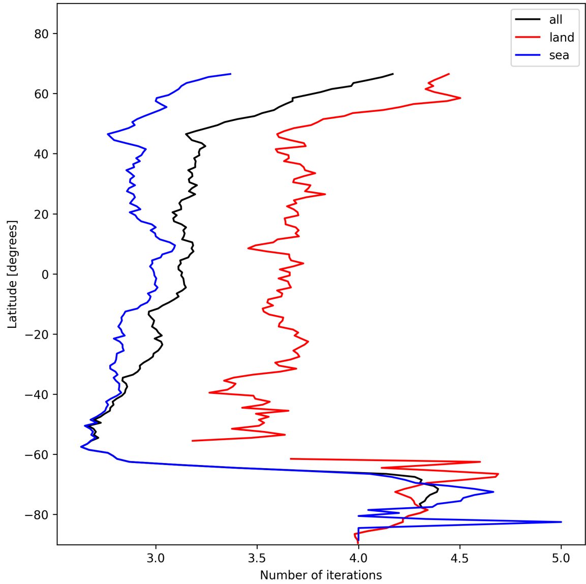
Figure 22: Zonal average of “Number of iterations” for 2024-11-25 to 2024-11-27.
