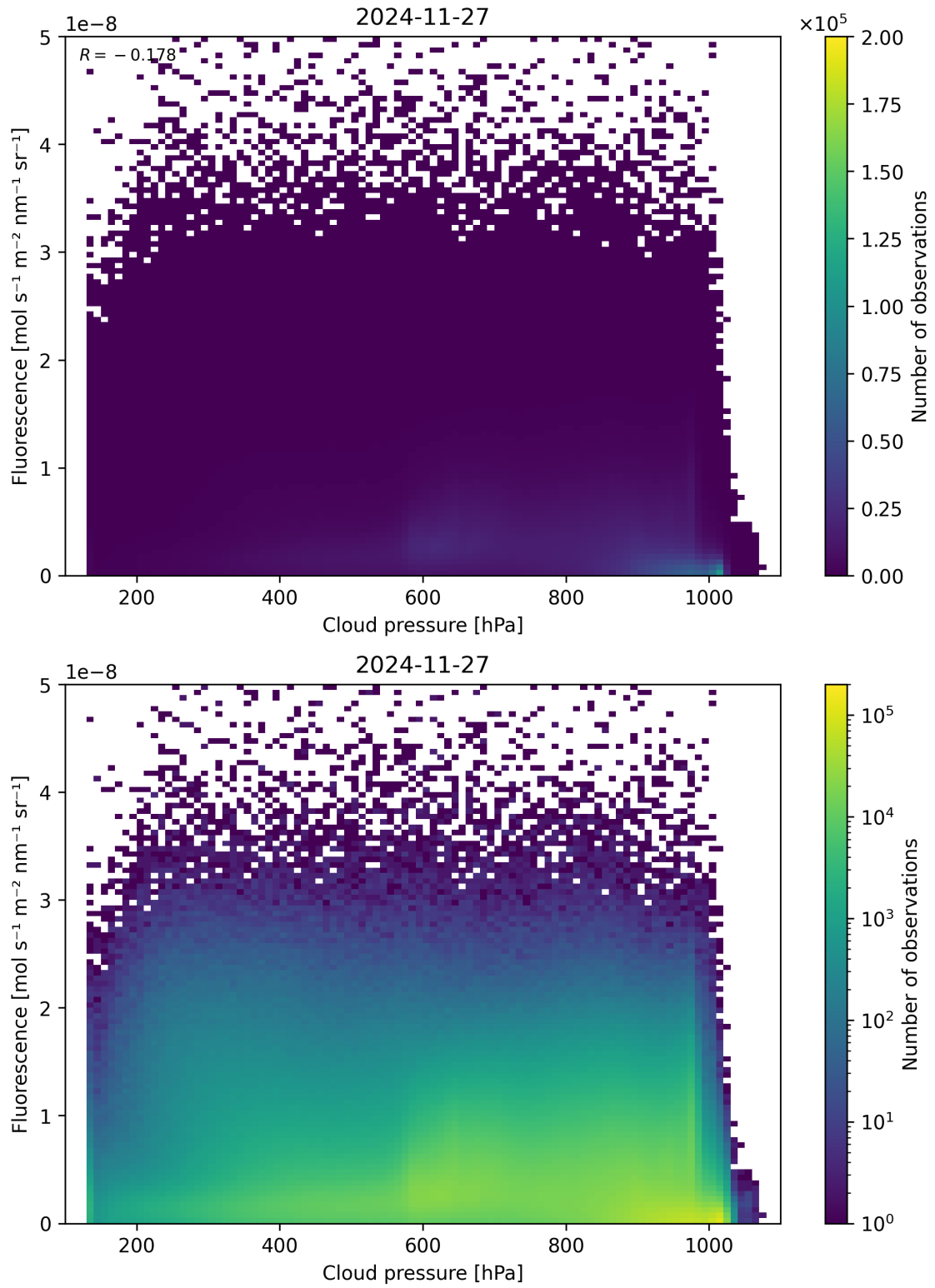
Figure 80: Scatter density plot of “Cloud pressure” against “Fluorescence” for 2024-11-26 to 2024-11-28.
