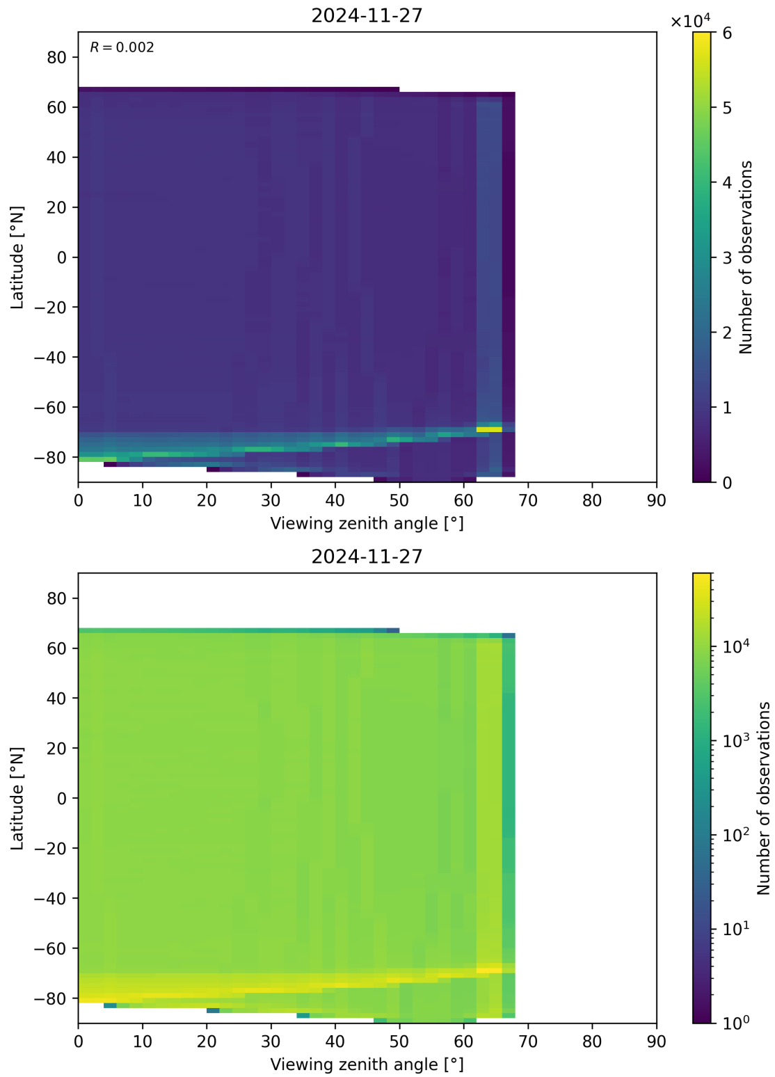
Figure 123: Scatter density plot of “Viewing zenith angle” against “Latitude” for 2024-11-26 to 2024-11-28.
