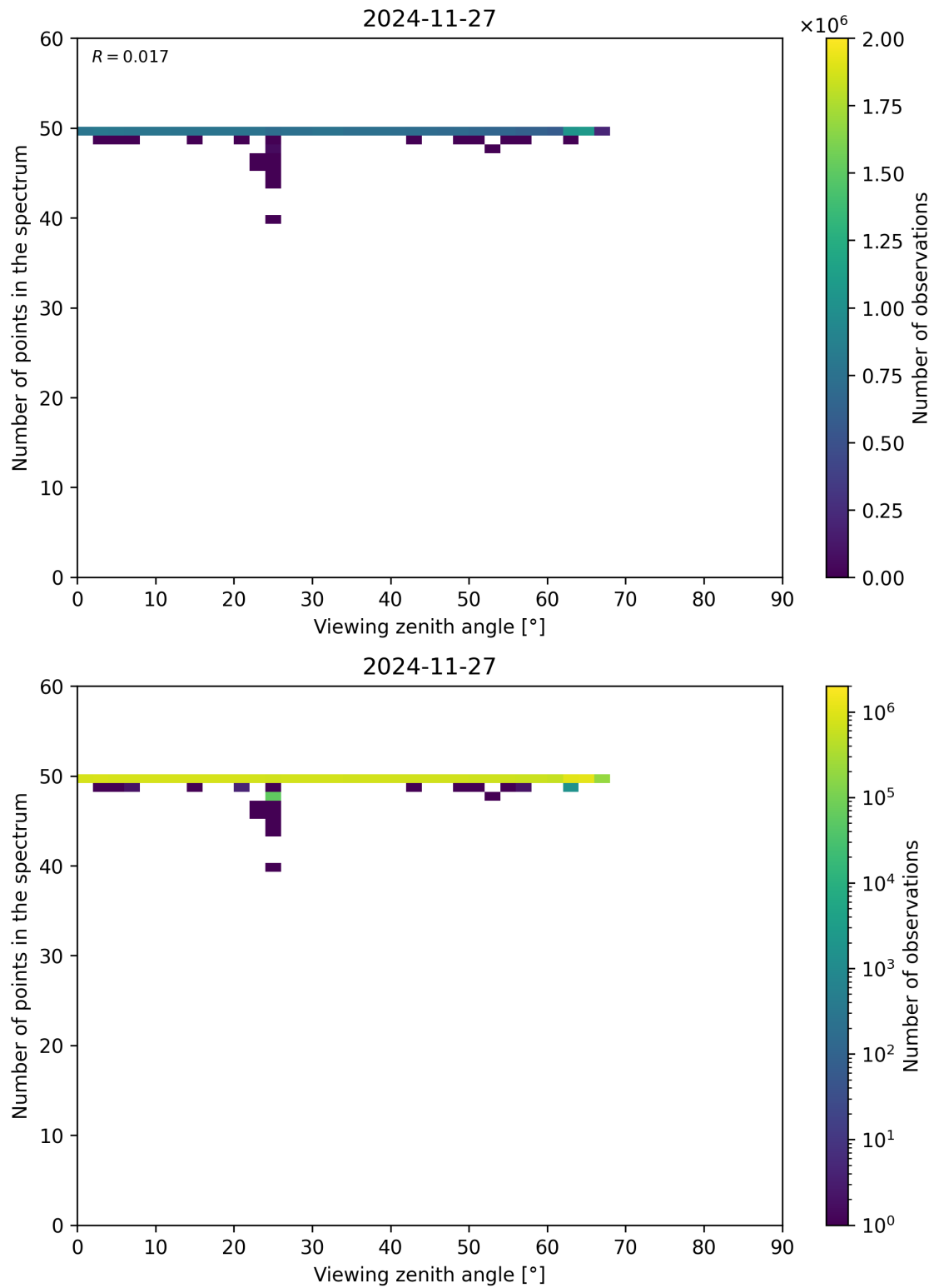
Figure 125: Scatter density plot of “Viewing zenith angle” against “Number of points in the spectrum” for 2024-11-26 to 2024-11-28.
