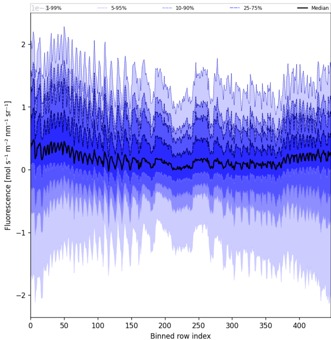
Figure 57: Along track statistics of “Fluorescence” for 2024-11-26 to 2024-11-28
