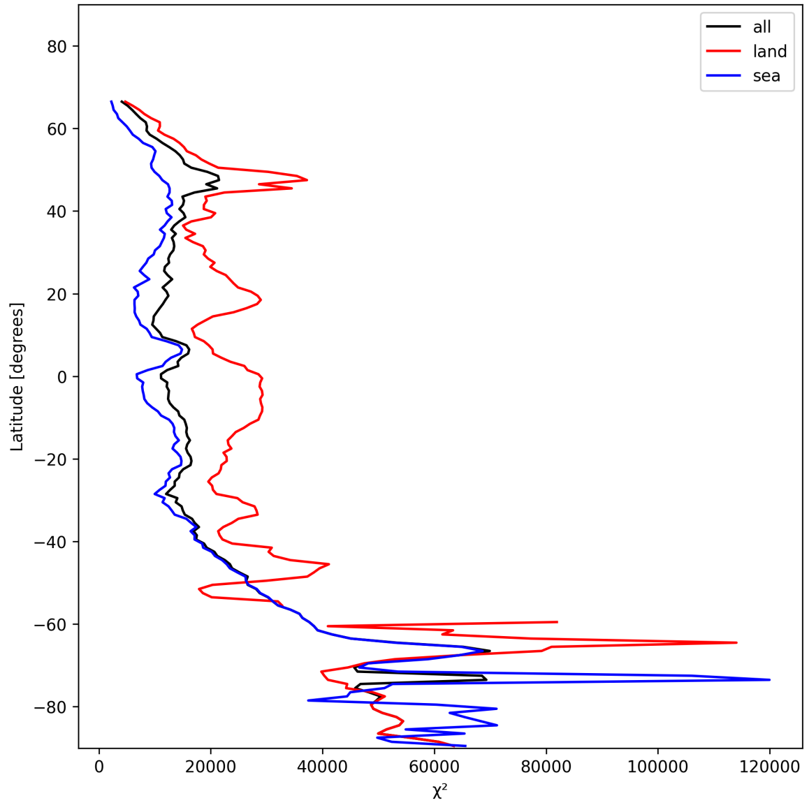
Figure 21: Zonal average of “ \chi^2 ” for 2024-11-26 to 2024-11-28.
