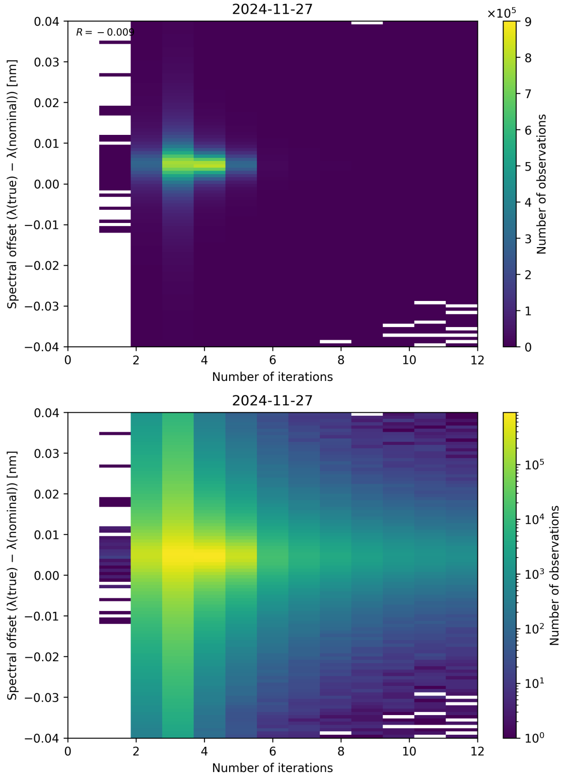
Figure 100: Scatter density plot of “Number of iterations” against “Spectral offset ( \lambda_{\text{true}} - \lambda_{\text{nominal}} )” for 2024-11-26 to 2024-11-28.
