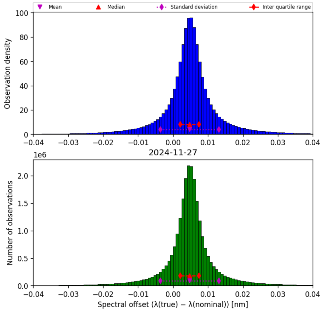
Figure 45: Histogram of “Spectral offset ( \lambda_{\text{true}} - \lambda_{\text{nominal}} )” for 2024-11-26 to 2024-11-28
