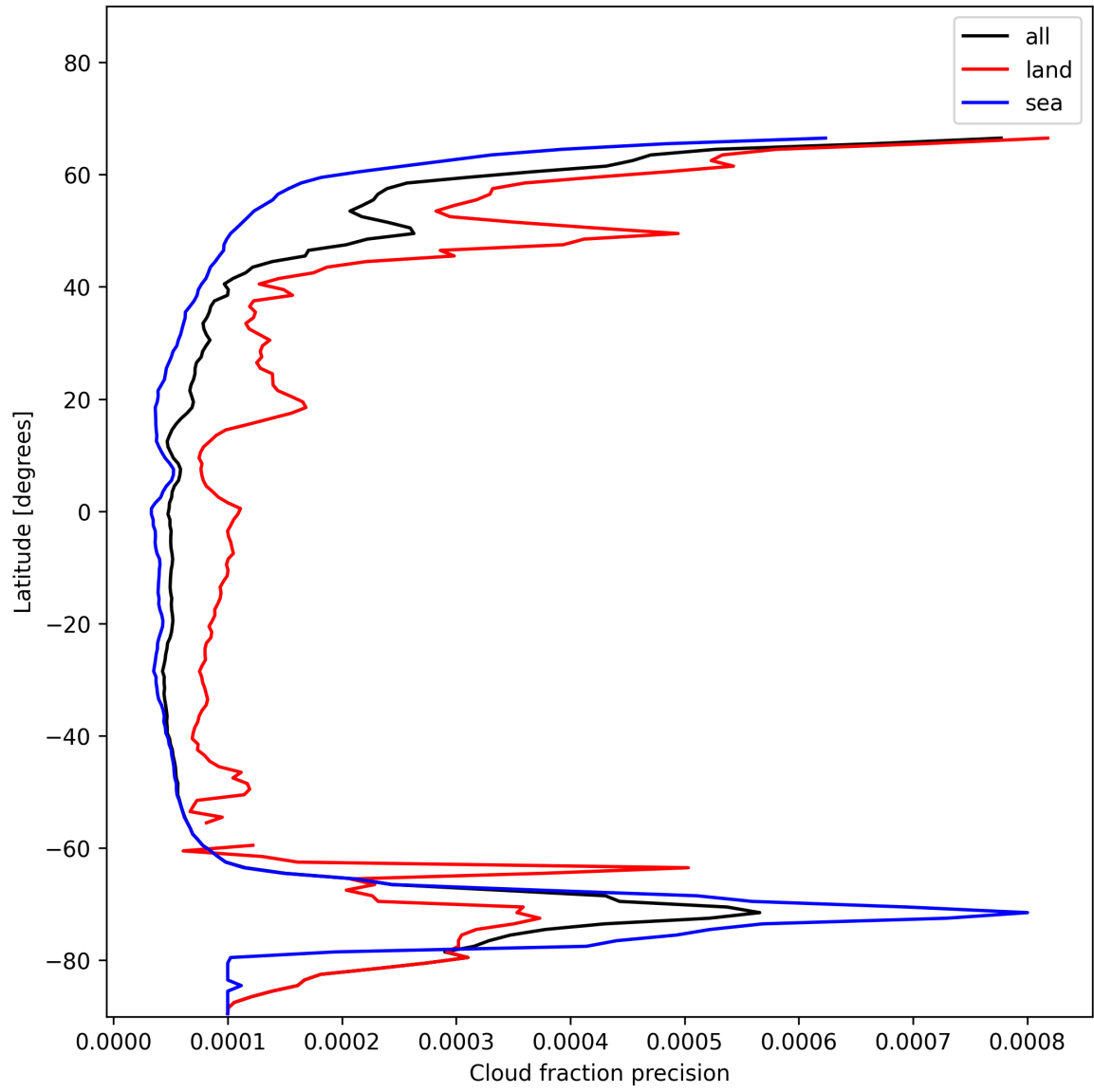
Figure 16: Zonal average of “Cloud fraction precision” for 2024-11-26 to 2024-11-28.
