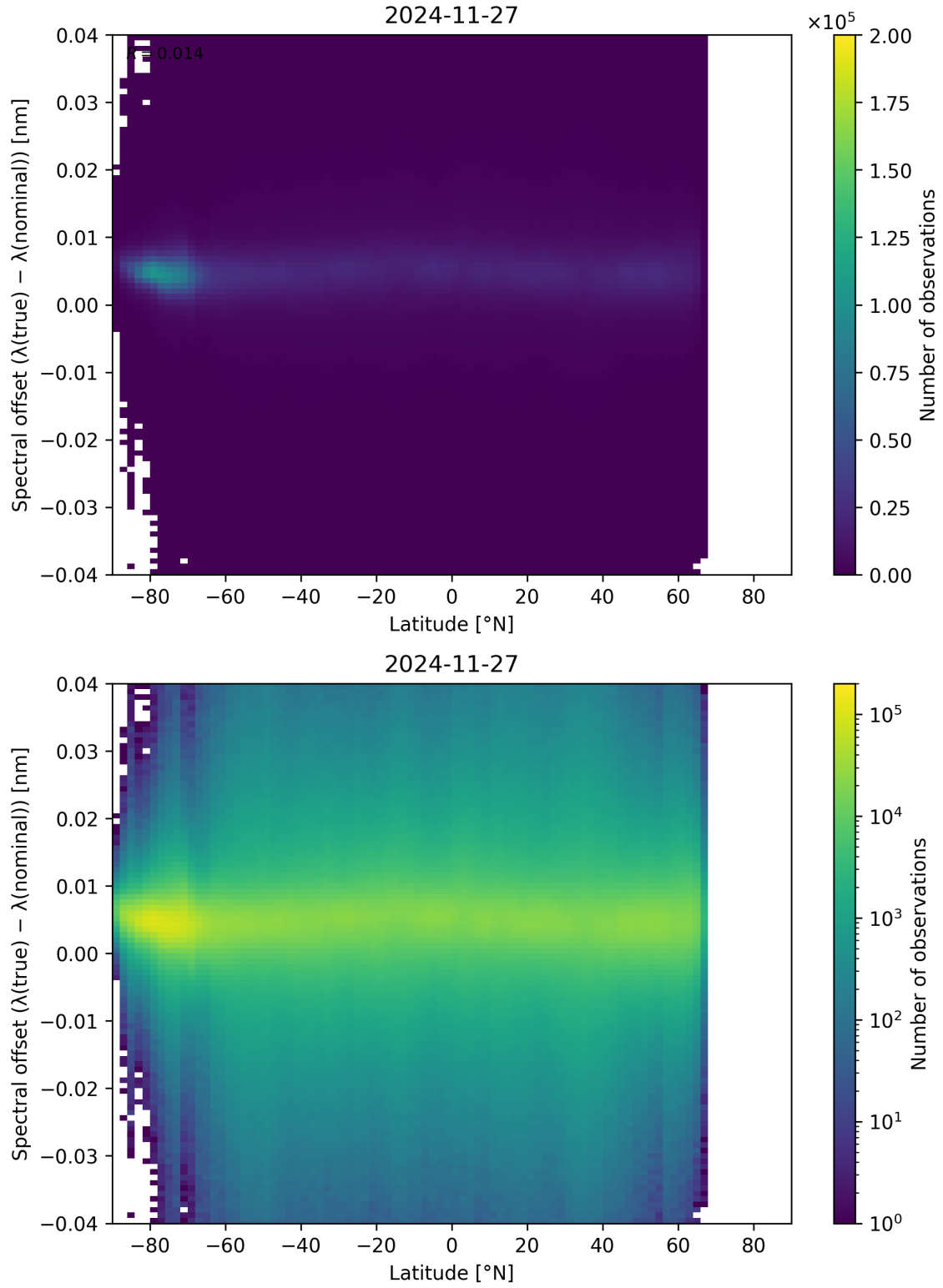
Figure 96: Scatter density plot of “Latitude” against “Spectral offset ( \lambda_{\text{true}} - \lambda_{\text{nominal}} )” for 2024-11-26 to 2024-11-28.
