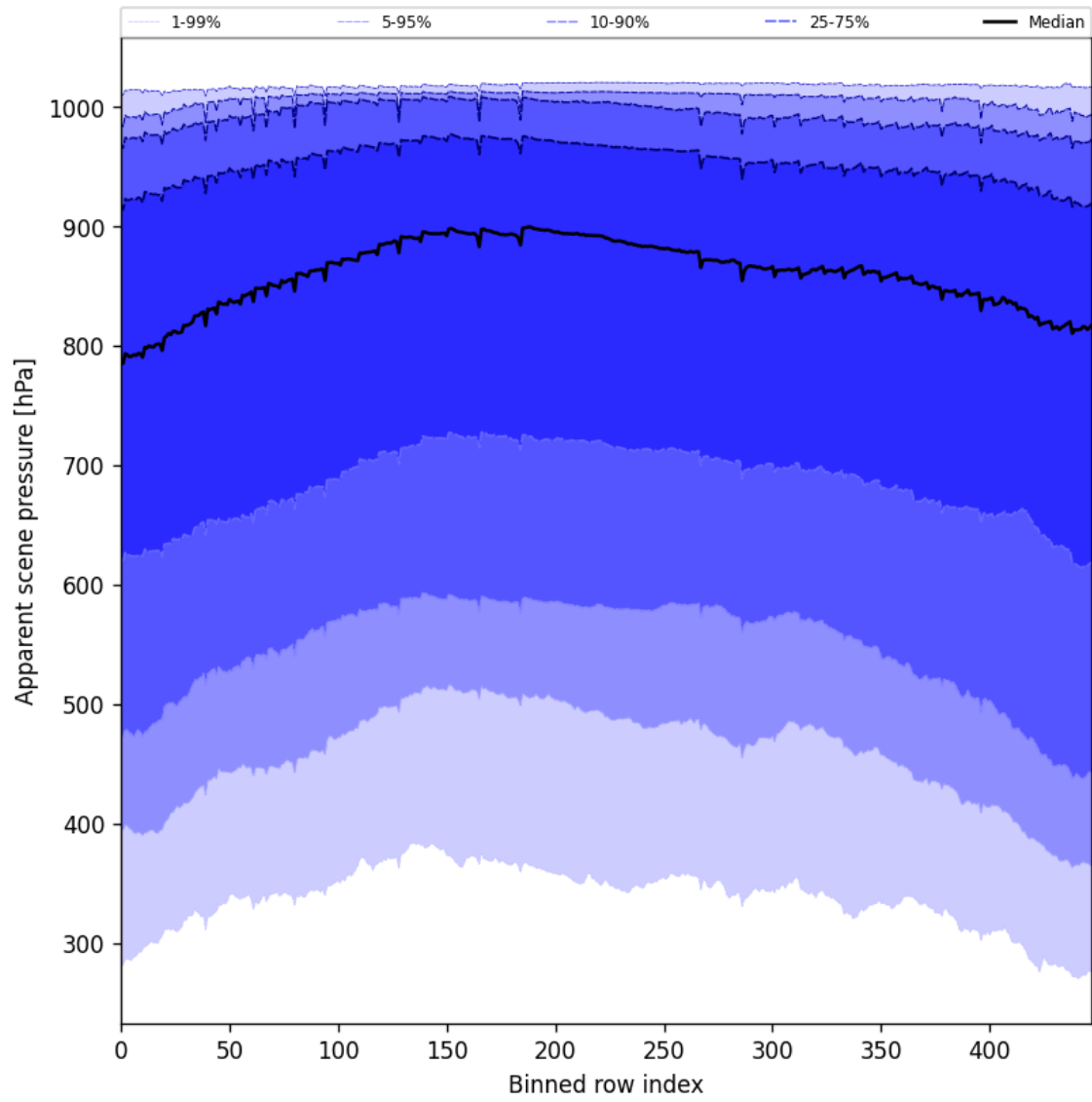
Figure 53: Along track statistics of “Apparent scene pressure” for 2024-11-26 to 2024-11-28
