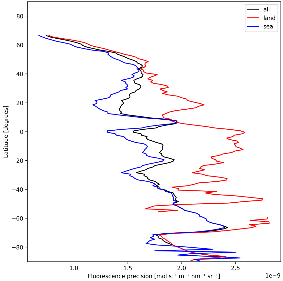
Figure 24: Zonal average of “Fluorescence precision” for 2024-11-26 to 2024-11-28.
