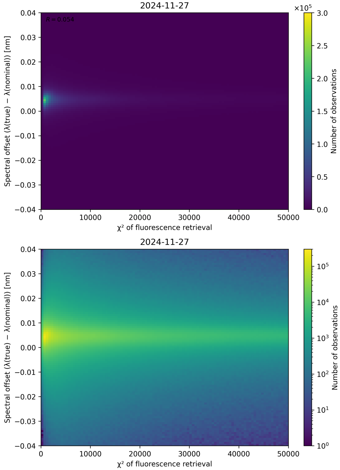
Figure 69: Scatter density plot of “ \chi^2 of fluorescence retrieval” against “Spectral offset ( \lambda_{\text{true}} - \lambda_{\text{nominal}} )” for 2024-11-26 to 2024-11-28.
