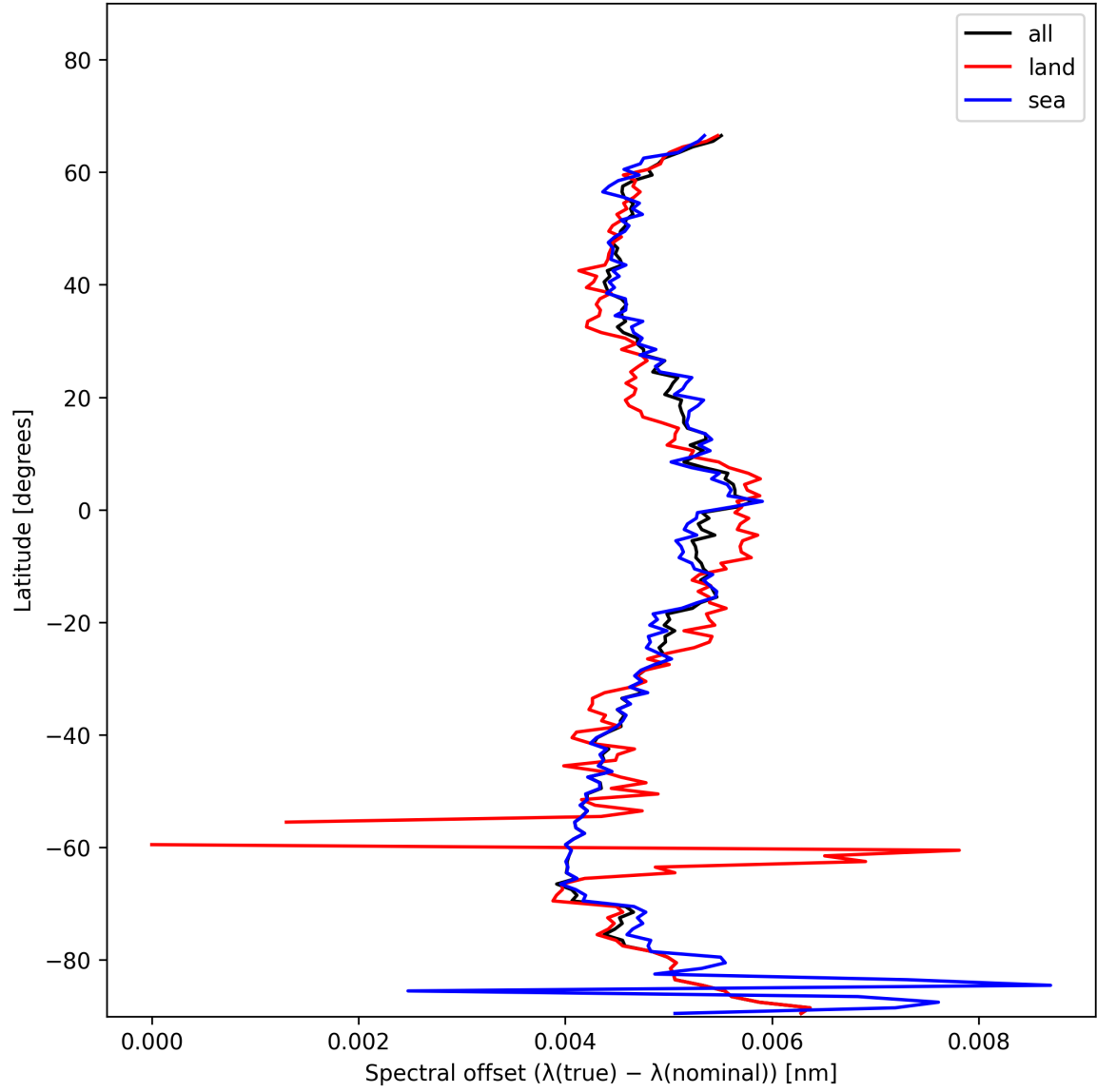
Figure 28: Zonal average of “Spectral offset ( \lambda_{\text{true}} - \lambda_{\text{nominal}} )” for 2024-11-26 to 2024-11-28.
