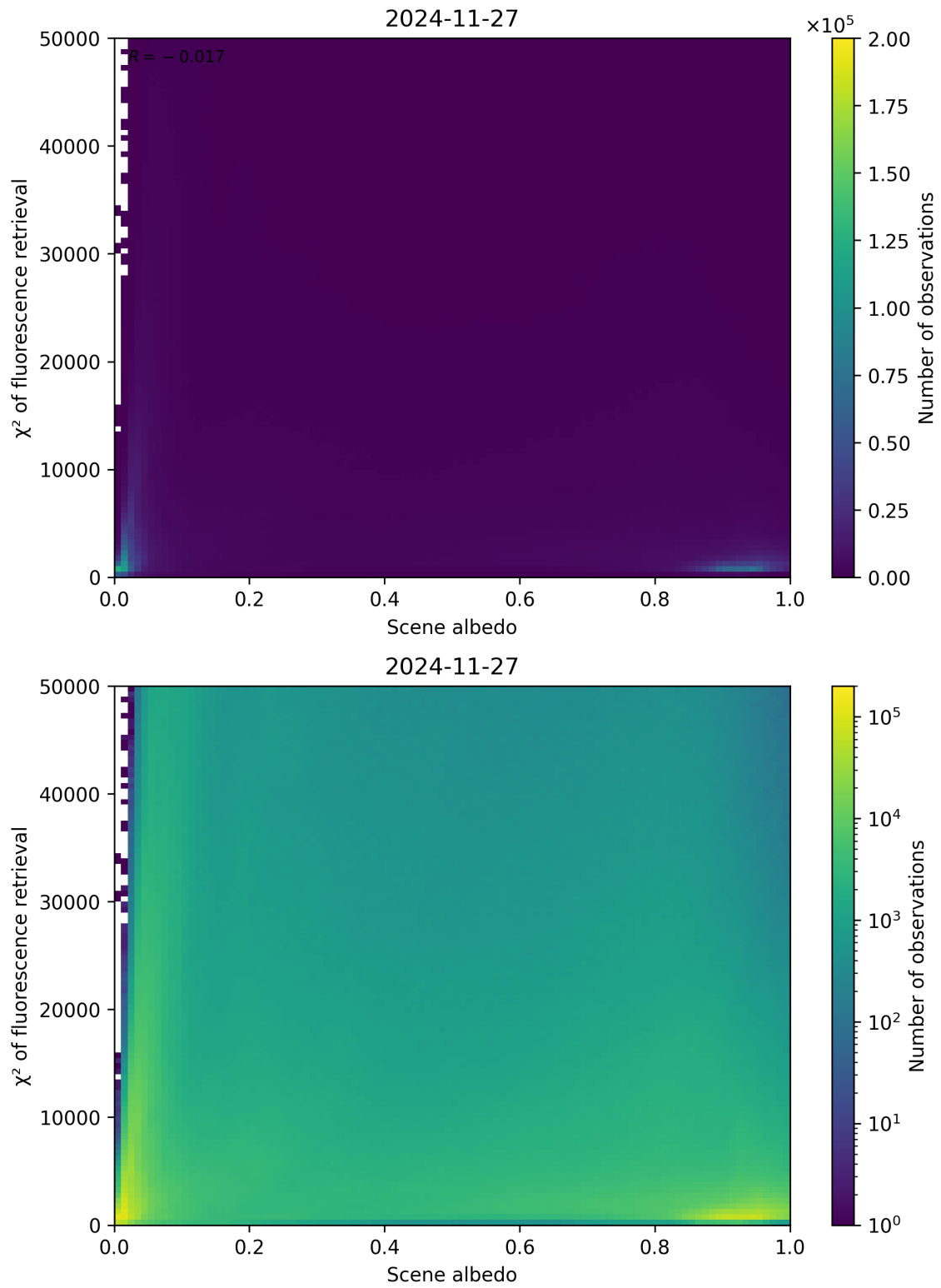
Figure 103: Scatter density plot of “Scene albedo” against “ \chi^2 of fluorescence retrieval” for 2024-11-26 to 2024-11-28.
