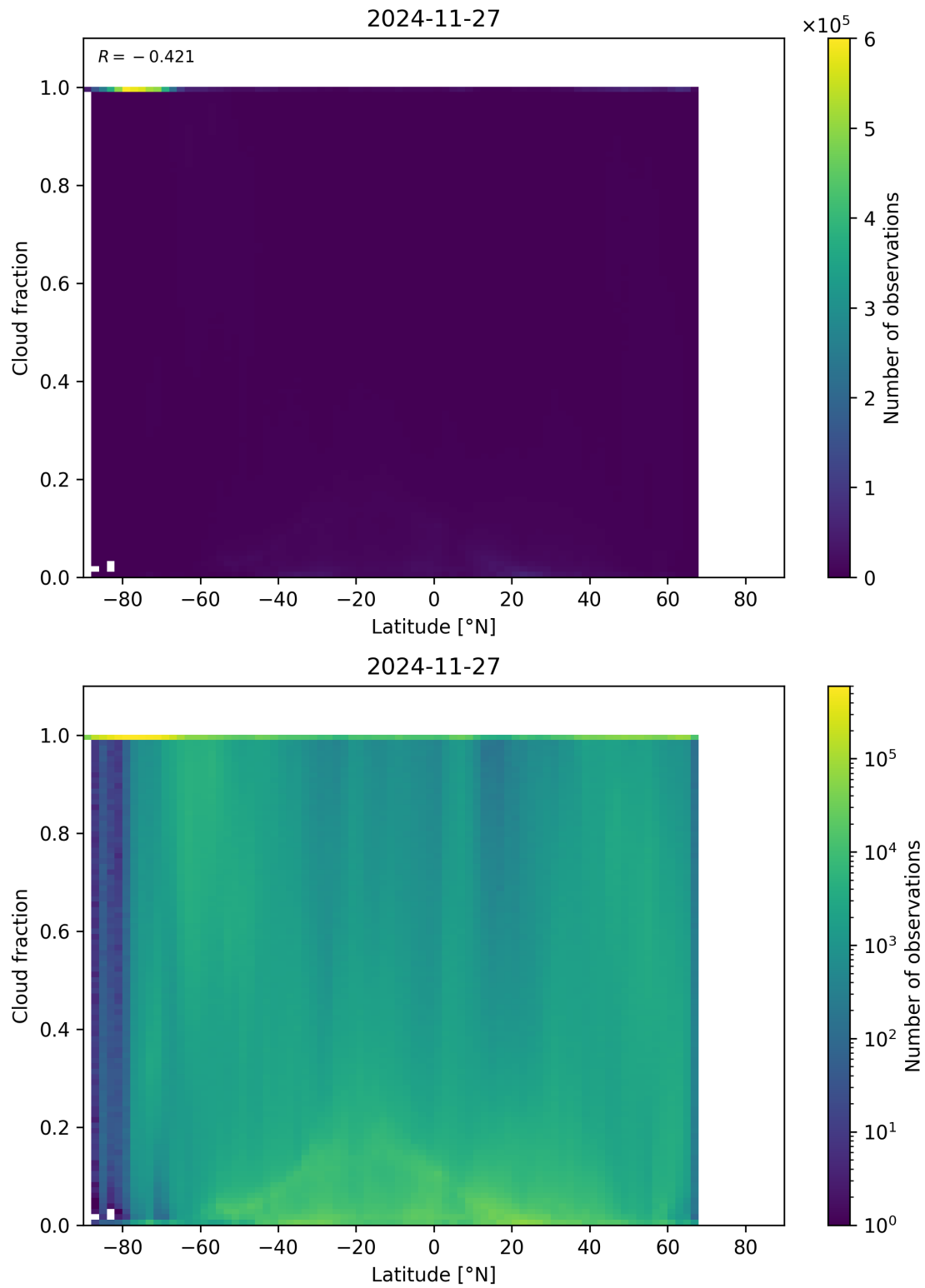
Figure 90: Scatter density plot of “Latitude” against “Cloud fraction” for 2024-11-26 to 2024-11-28.
