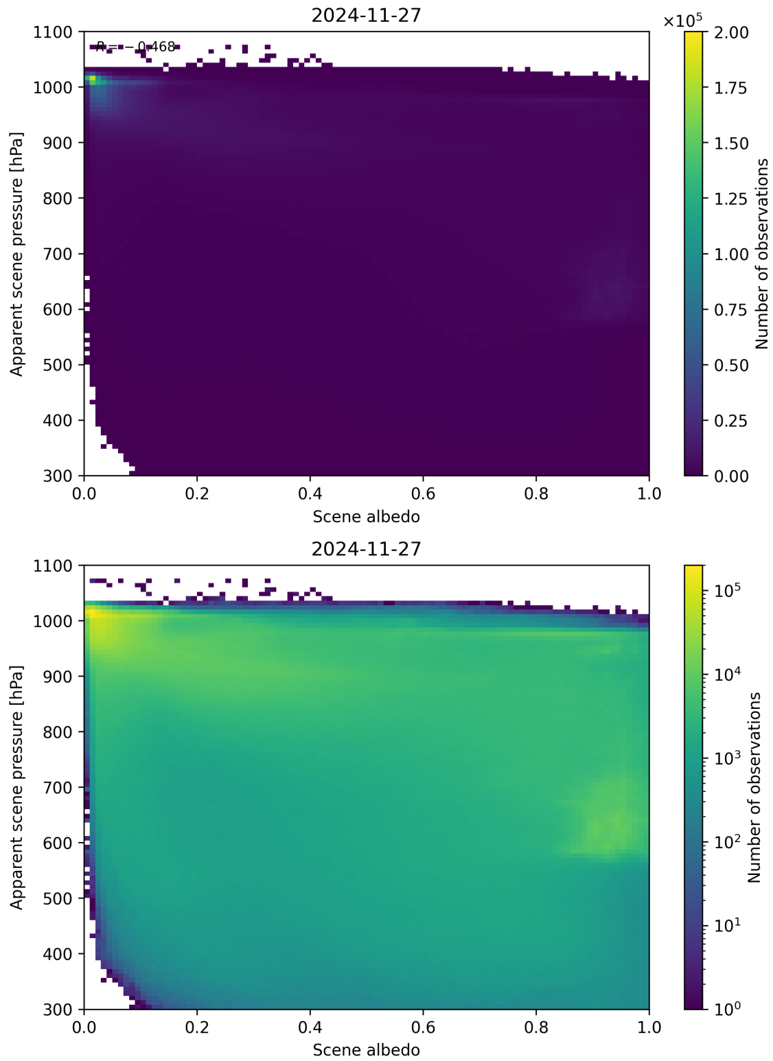
Figure 102: Scatter density plot of “Scene albedo” against “Apparent scene pressure” for 2024-11-26 to 2024-11-28.
