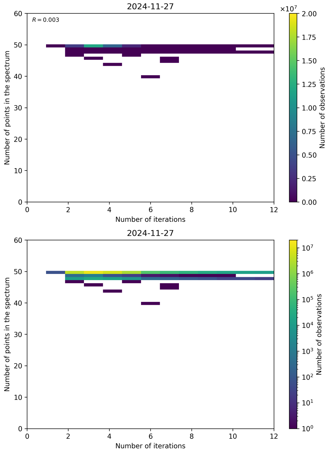
Figure 99: Scatter density plot of “Number of iterations” against “Number of points in the spectrum” for 2024-11-26 to 2024-11-28.
