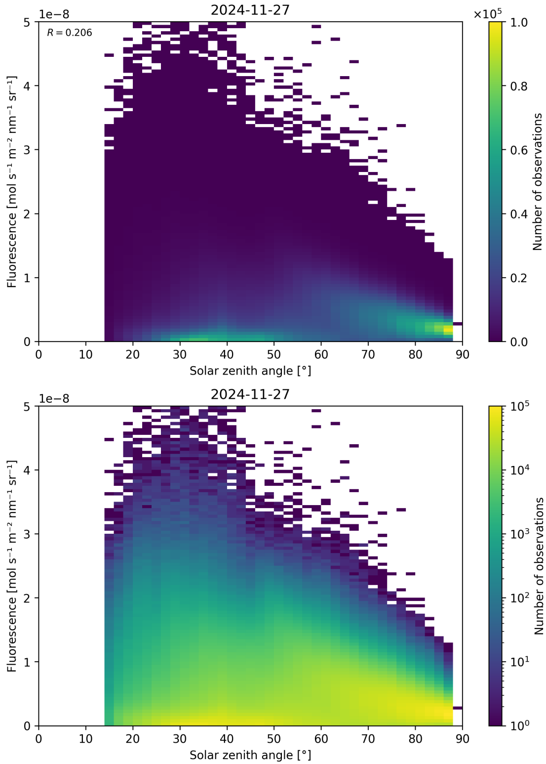
Figure 112: Scatter density plot of “Solar zenith angle” against “Fluorescence” for 2024-11-26 to 2024-11-28.
