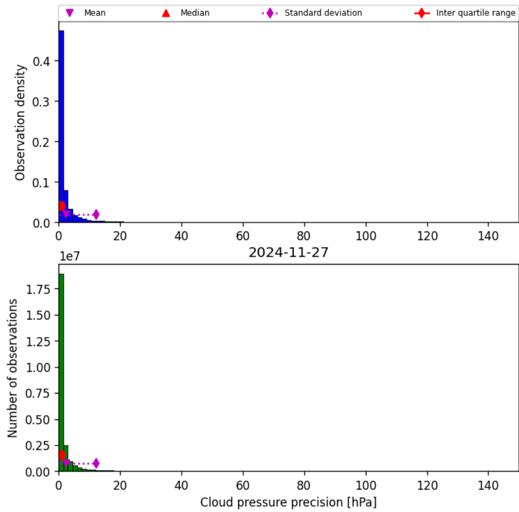
Figure 31: Histogram of “Cloud pressure precision” for 2024-11-26 to 2024-11-28
