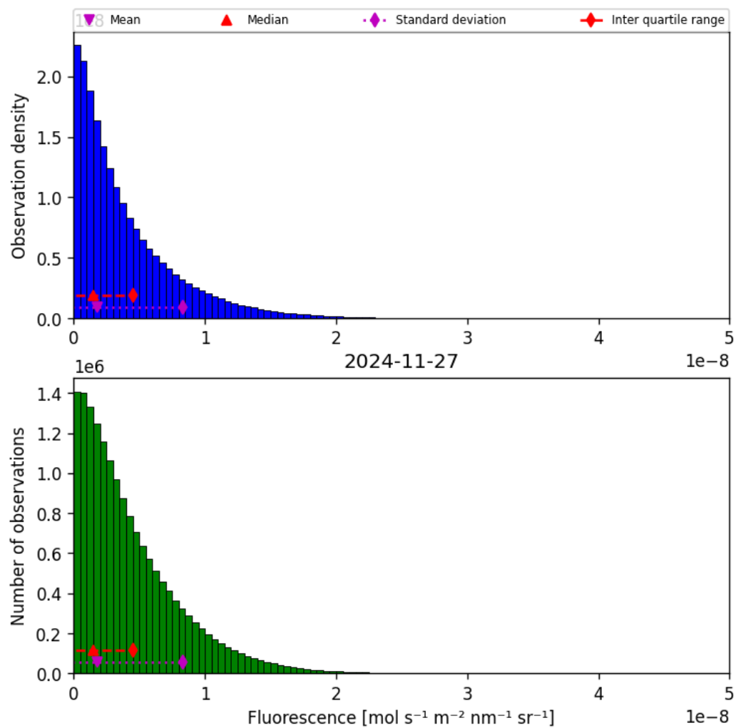
Figure 40: Histogram of “Fluorescence” for 2024-11-26 to 2024-11-28
