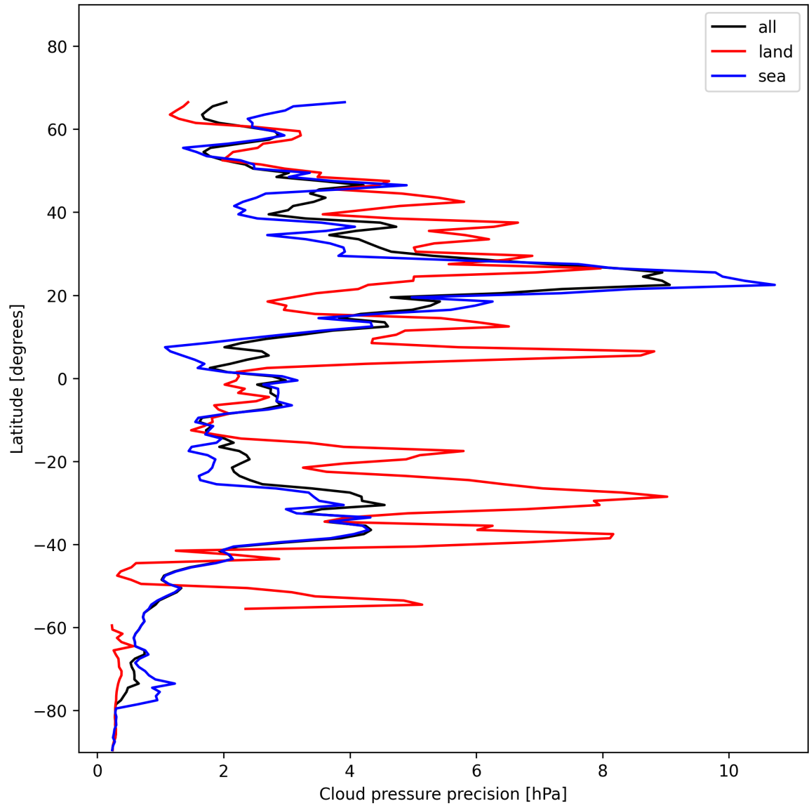
Figure 14: Zonal average of “Cloud pressure precision” for 2024-11-26 to 2024-11-28.
