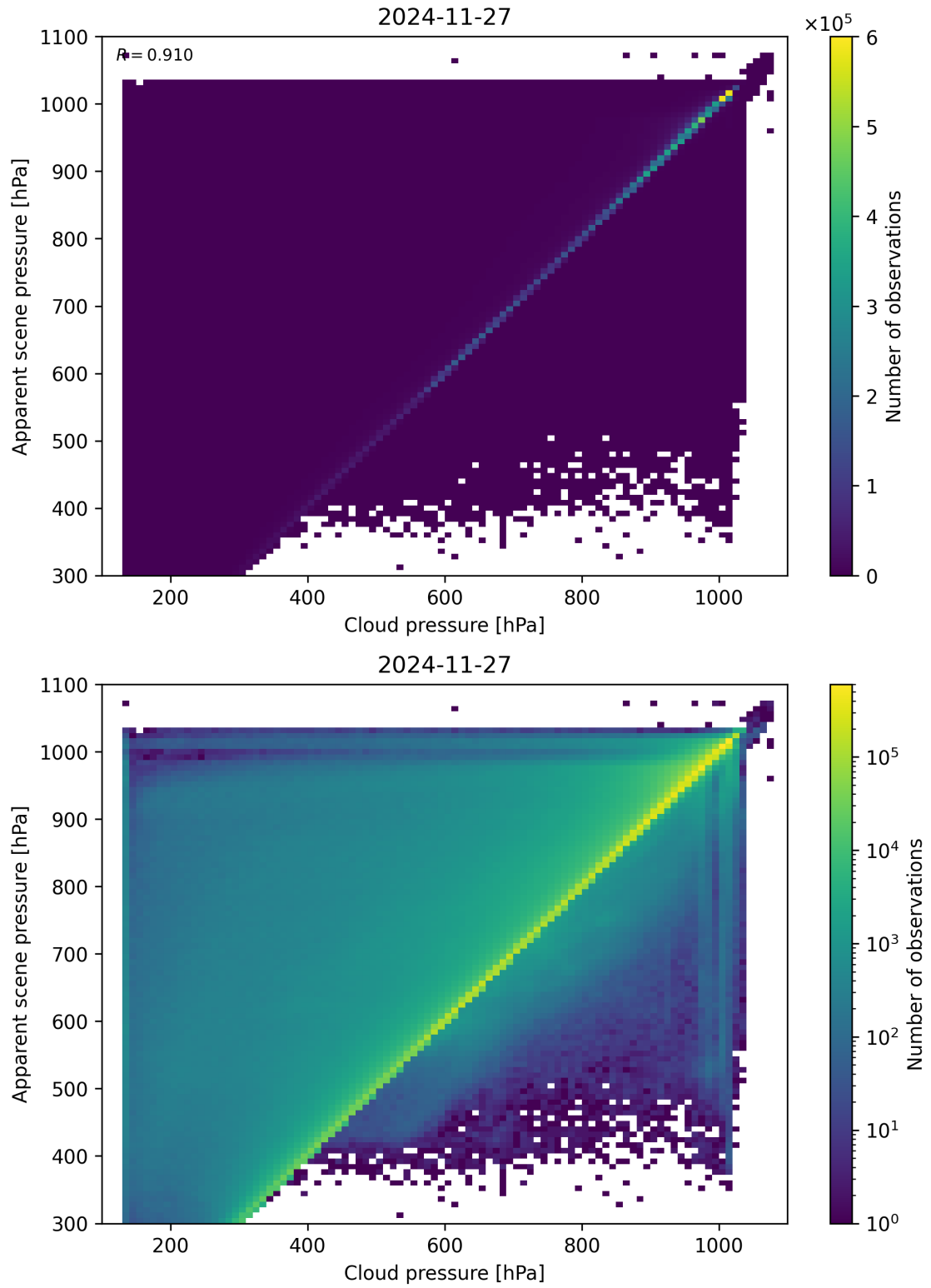
Figure 77: Scatter density plot of “Cloud pressure” against “Apparent scene pressure” for 2024-11-26 to 2024-11-28.
