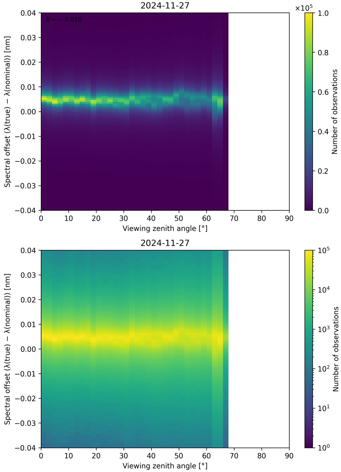
Figure 128: Scatter density plot of “Viewing zenith angle” against “Spectral offset ( \lambda_{\text{true}} - \lambda_{\text{nominal}} )” for 2024-11-26 to 2024-11-28.
