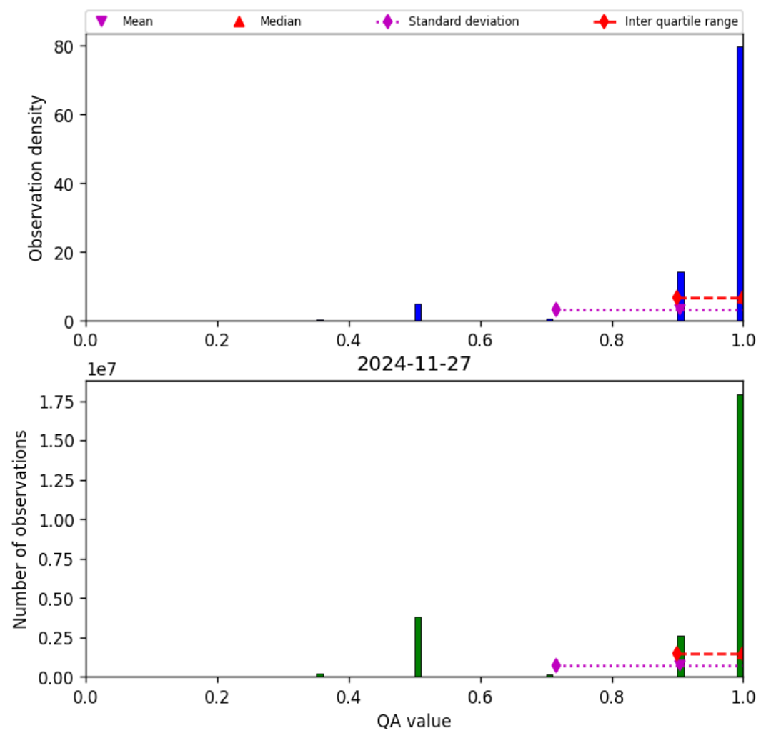
Figure 29: Histogram of “QA value” for 2024-11-26 to 2024-11-28
