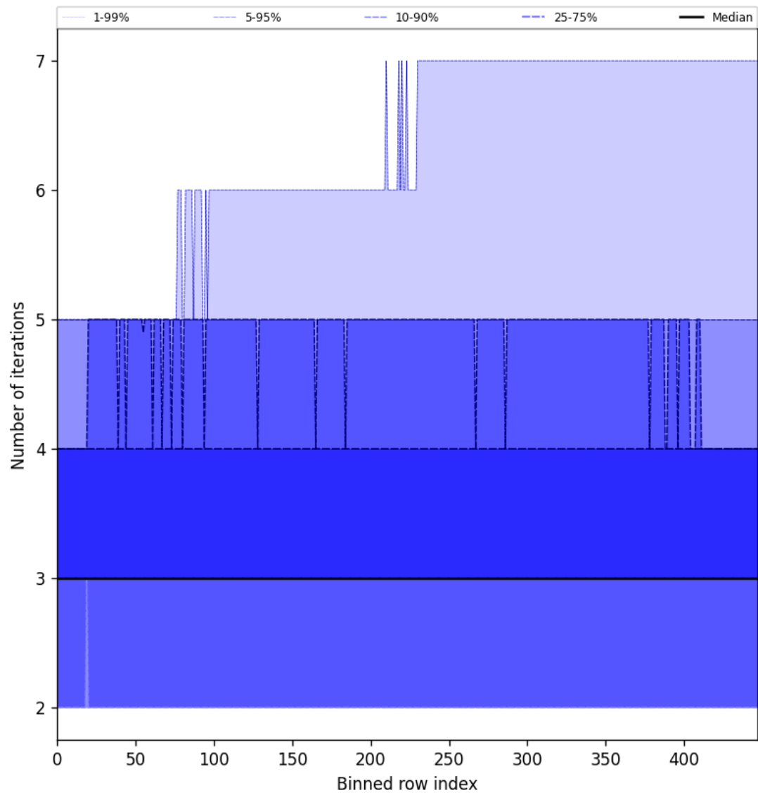
Figure 56: Along track statistics of “Number of iterations” for 2024-11-26 to 2024-11-28
