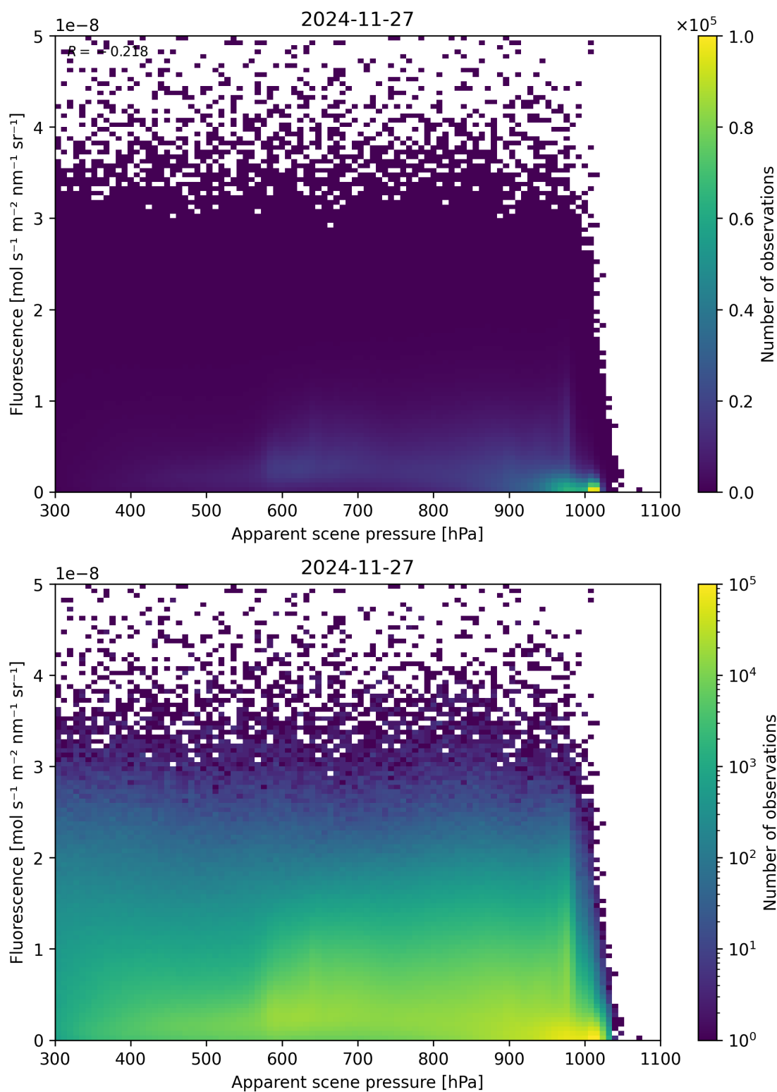
Figure 64: Scatter density plot of “Apparent scene pressure” against “Fluorescence” for 2024-11-26 to 2024-11-28.
