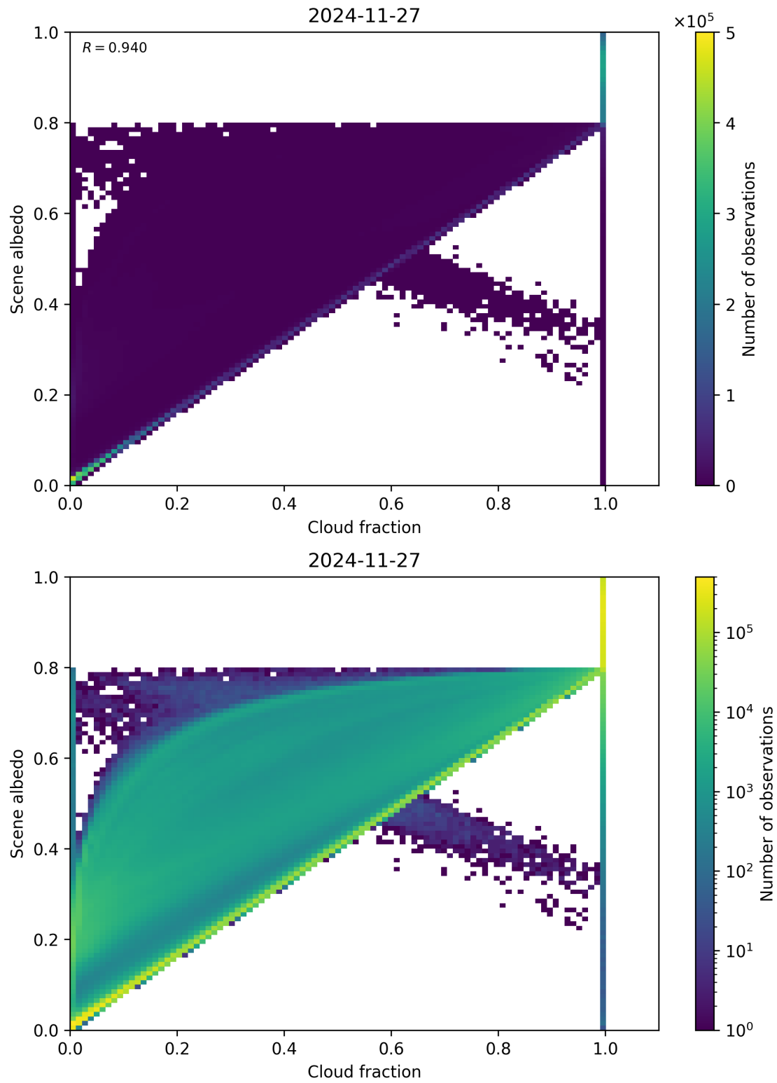
Figure 75: Scatter density plot of “Cloud fraction” against “Scene albedo” for 2024-11-26 to 2024-11-28.
