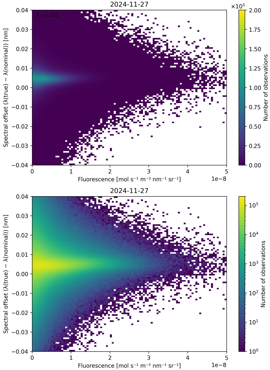
Figure 87: Scatter density plot of “Fluorescence” against “Spectral offset ( \lambda_{\text{true}} - \lambda_{\text{nominal}} )” for 2024-11-26 to 2024-11-28.
