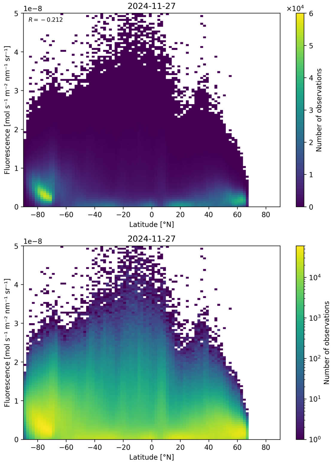
Figure 92: Scatter density plot of “Latitude” against “Fluorescence” for 2024-11-26 to 2024-11-28.
