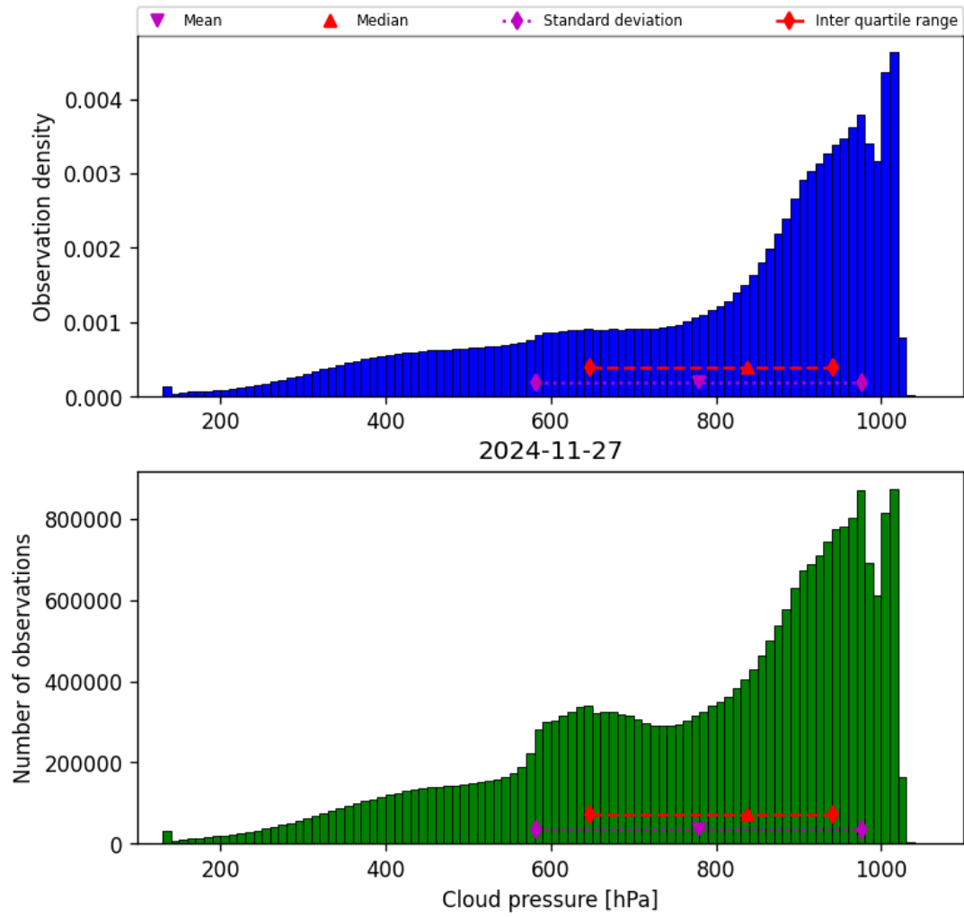
Figure 30: Histogram of “Cloud pressure” for 2024-11-26 to 2024-11-28
