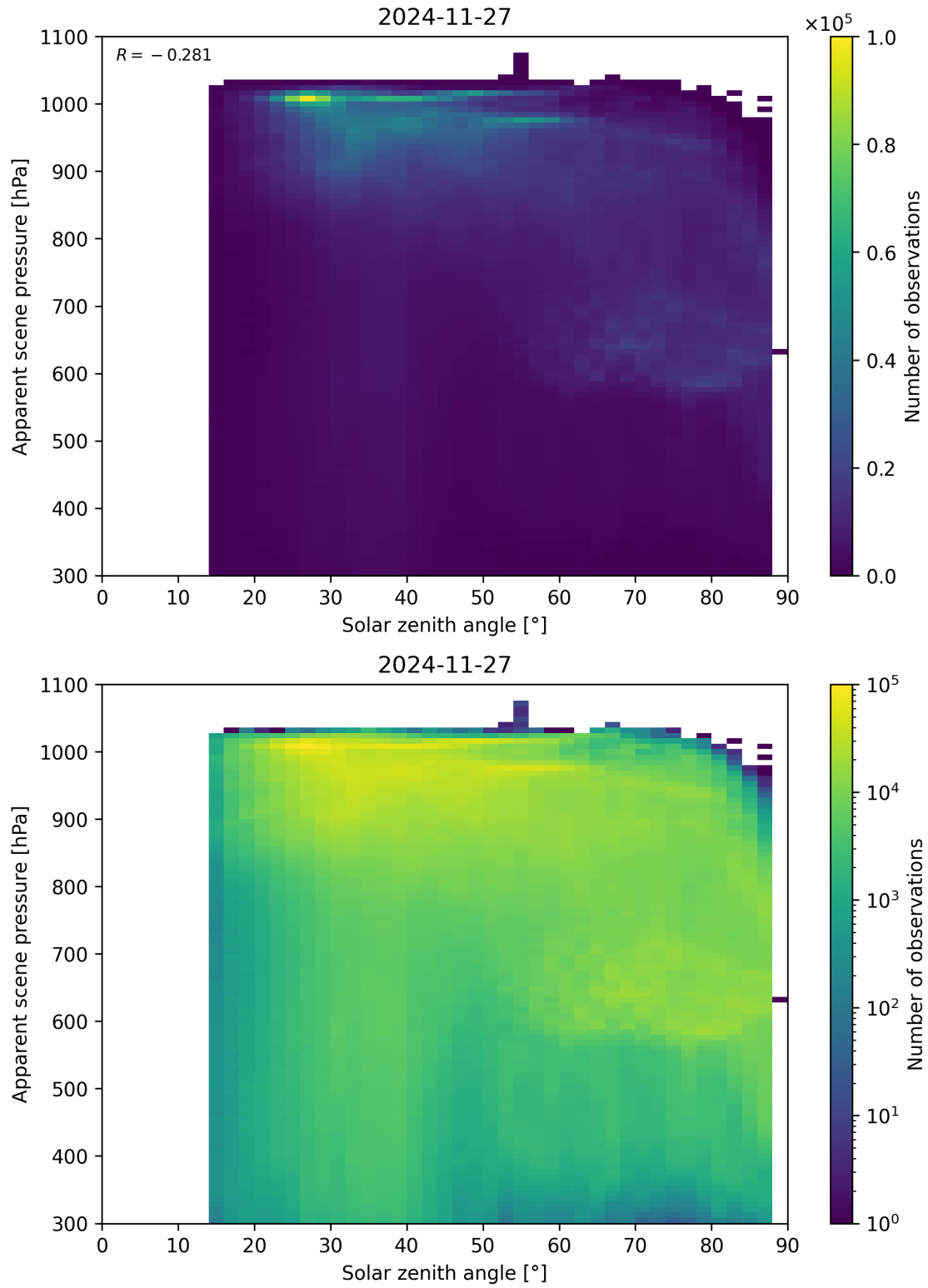
Figure 108: Scatter density plot of “Solar zenith angle” against “Apparent scene pressure” for 2024-11-26 to 2024-11-28.
