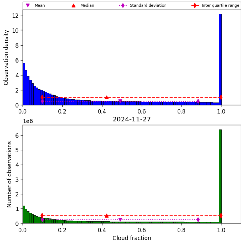
Figure 32: Histogram of “Cloud fraction” for 2024-11-26 to 2024-11-28
