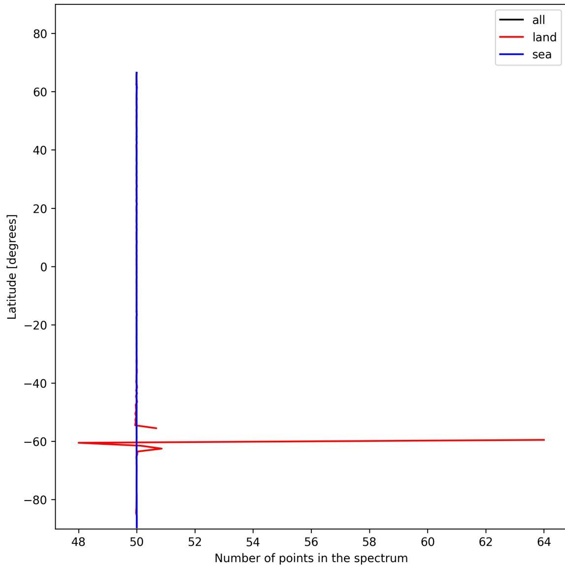
Figure 27: Zonal average of “Number of points in the spectrum” for 2024-11-26 to 2024-11-28.
