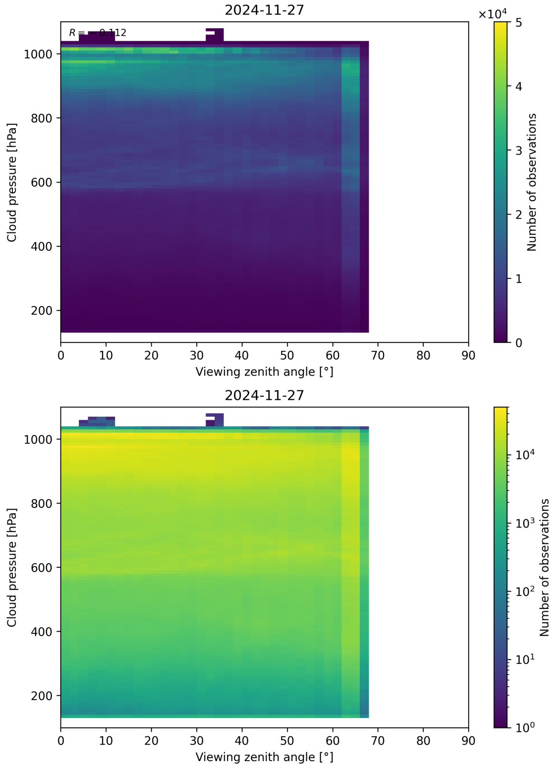
Figure 121: Scatter density plot of “Viewing zenith angle” against “Cloud pressure” for 2024-11-26 to 2024-11-28.
