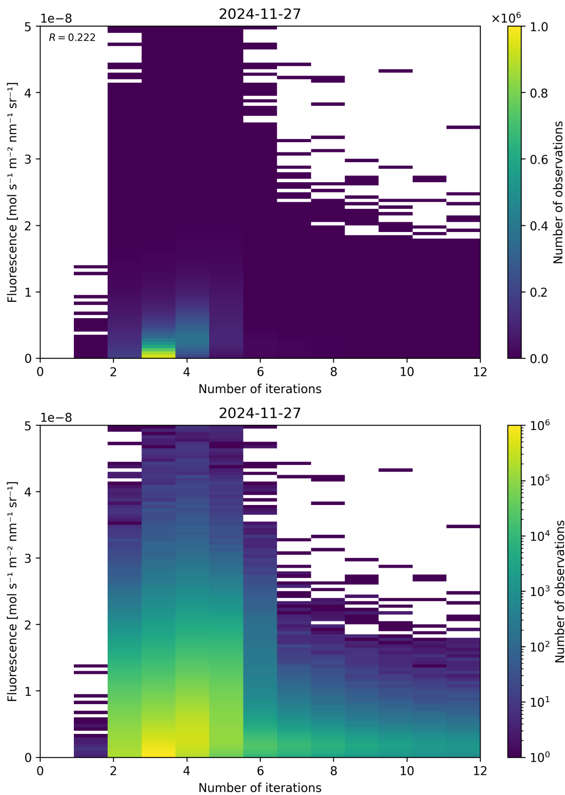
Figure 98: Scatter density plot of “Number of iterations” against “Fluorescence” for 2024-11-26 to 2024-11-28.
