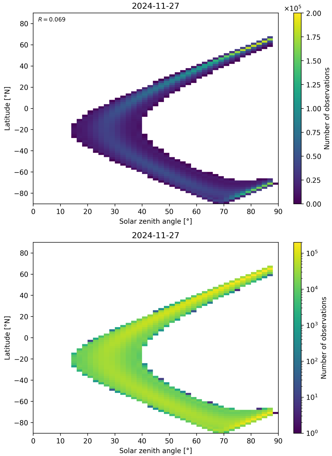
Figure 113: Scatter density plot of “Solar zenith angle” against “Latitude” for 2024-11-26 to 2024-11-28.
