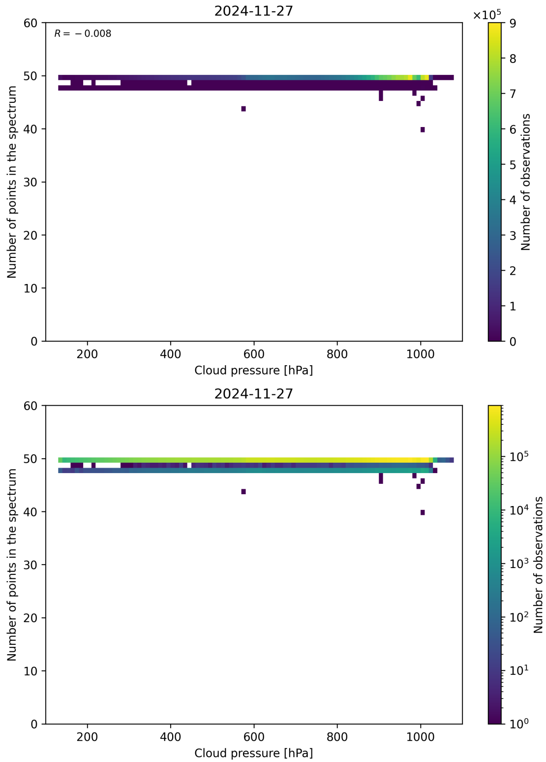
Figure 82: Scatter density plot of “Cloud pressure” against “Number of points in the spectrum” for 2024-11-26 to 2024-11-28.
