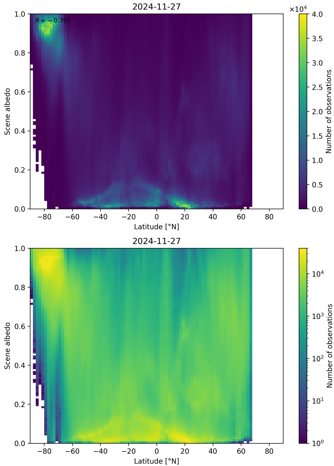
Figure 95: Scatter density plot of “Latitude” against “Scene albedo” for 2024-11-26 to 2024-11-28.
