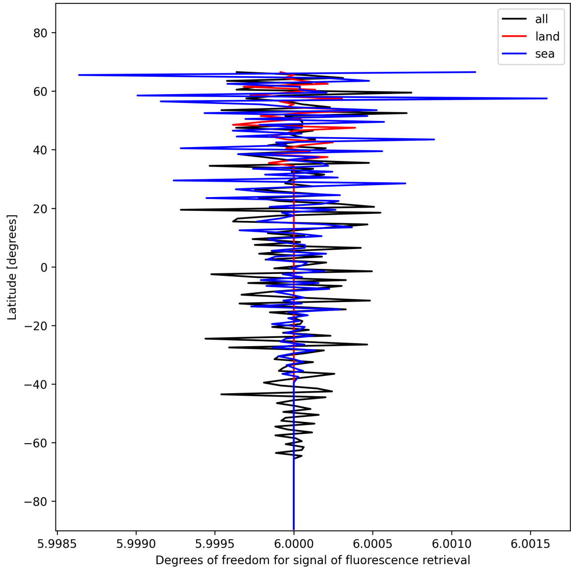
Figure 26: Zonal average of “Degrees of freedom for signal of fluorescence retrieval” for 2024-11-26 to 2024-11-28.
