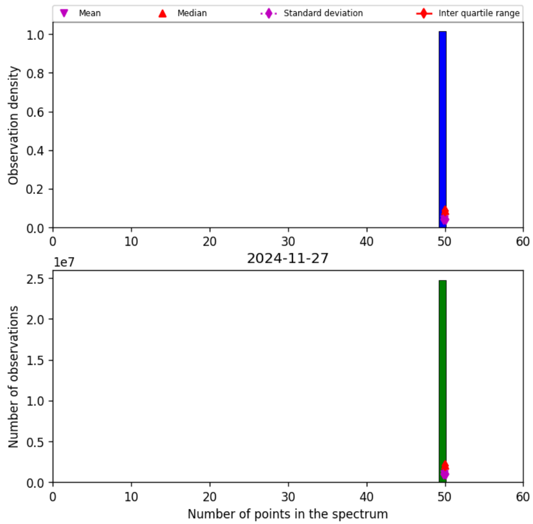
Figure 44: Histogram of “Number of points in the spectrum” for 2024-11-26 to 2024-11-28
