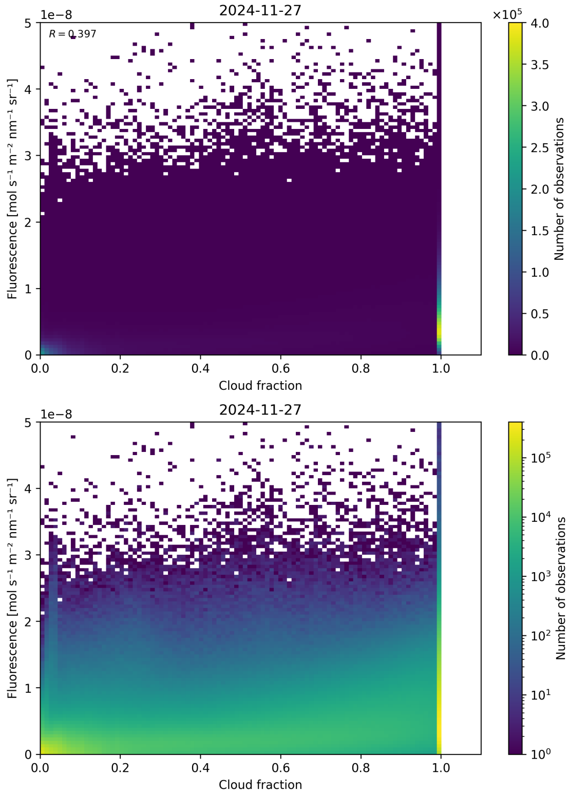
Figure 72: Scatter density plot of “Cloud fraction” against “Fluorescence” for 2024-11-26 to 2024-11-28.
