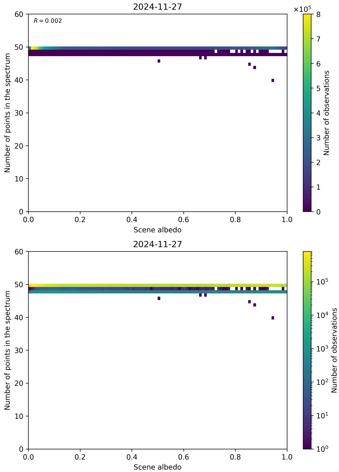
Figure 106: Scatter density plot of “Scene albedo” against “Number of points in the spectrum” for 2024-11-26 to 2024-11-28.
