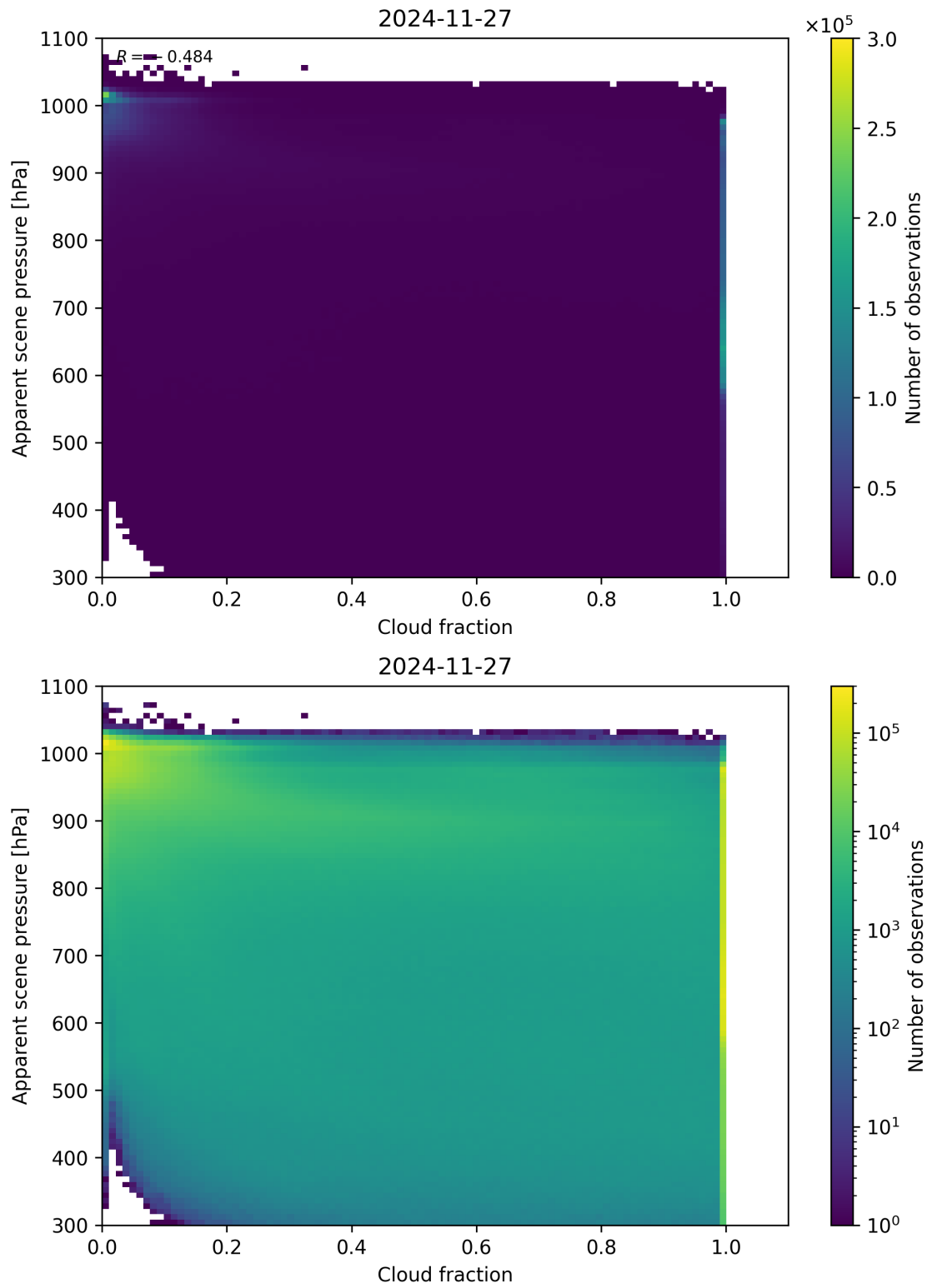
Figure 70: Scatter density plot of “Cloud fraction” against “Apparent scene pressure” for 2024-11-26 to 2024-11-28.
