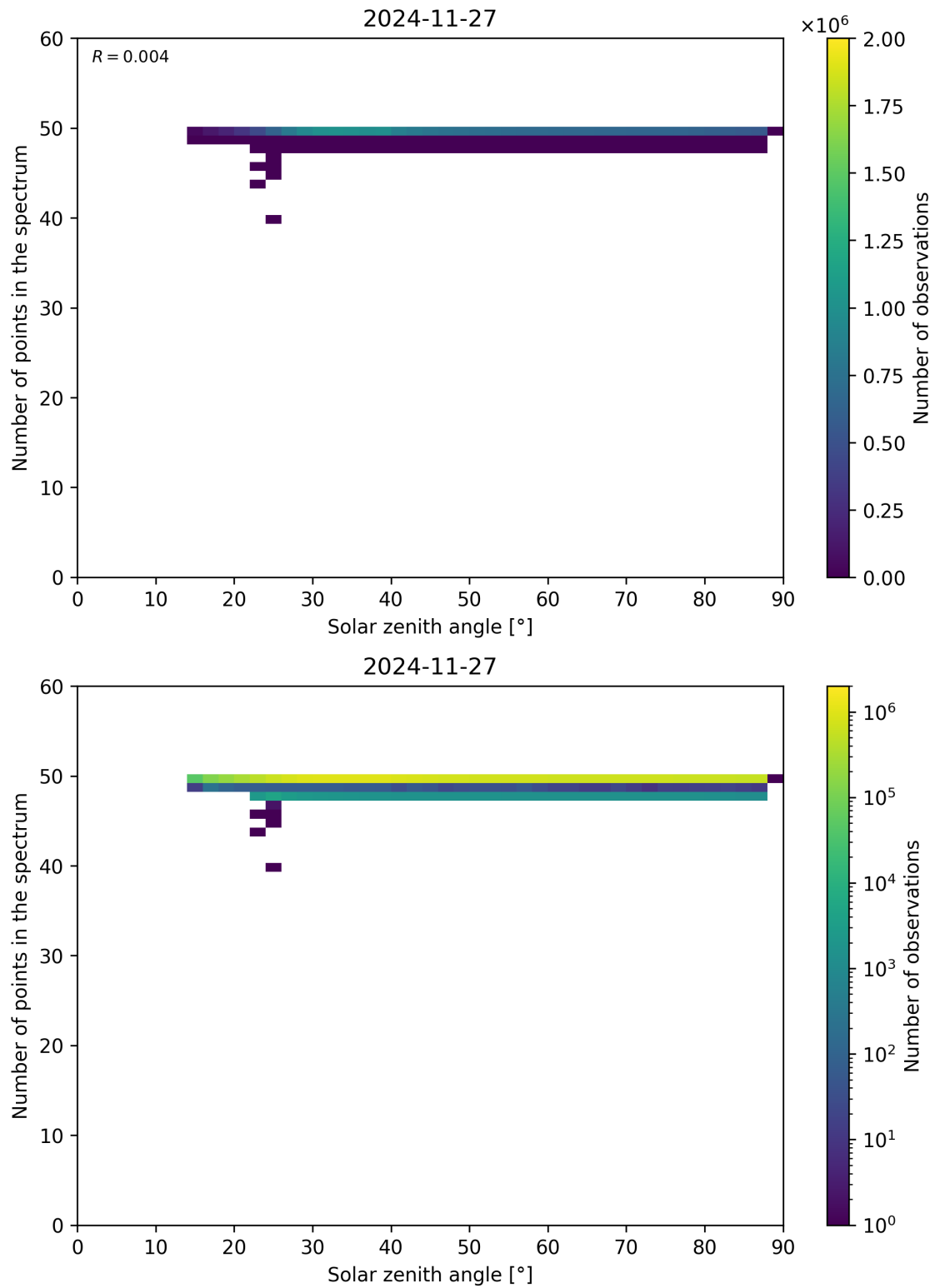
Figure 115: Scatter density plot of “Solar zenith angle” against “Number of points in the spectrum” for 2024-11-26 to 2024-11-28.
