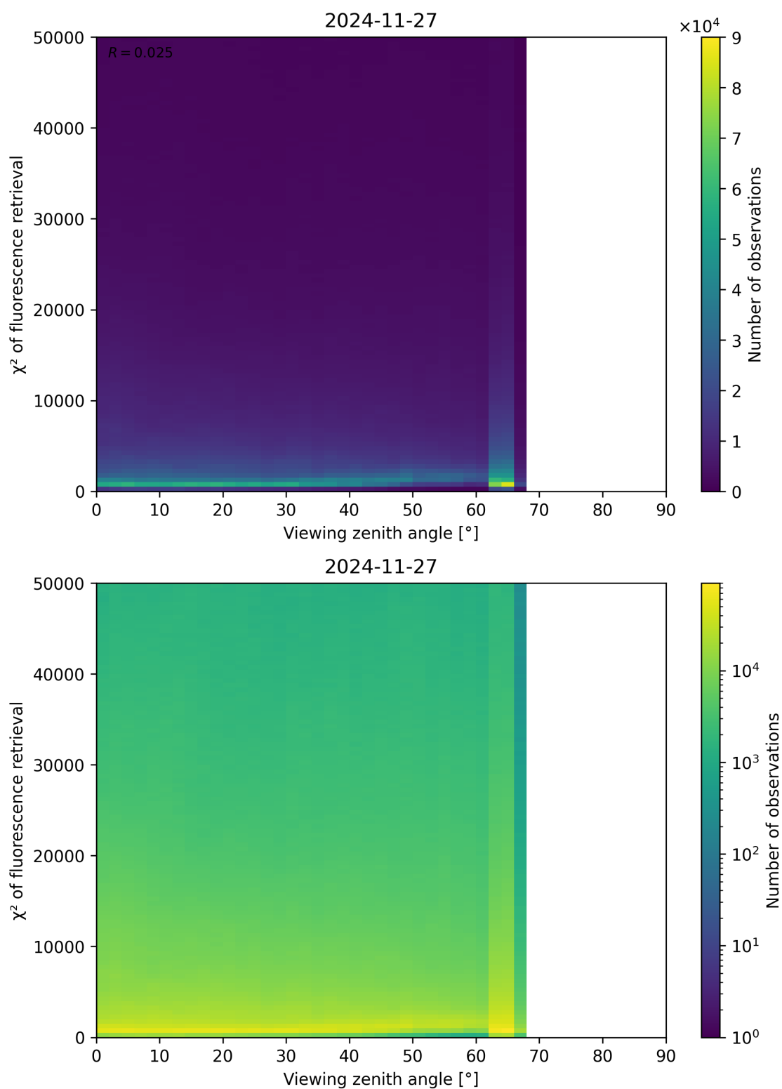
Figure 119: Scatter density plot of “Viewing zenith angle” against “ \chi^2 of fluorescence retrieval” for 2024-11-26 to 2024-11-28.
