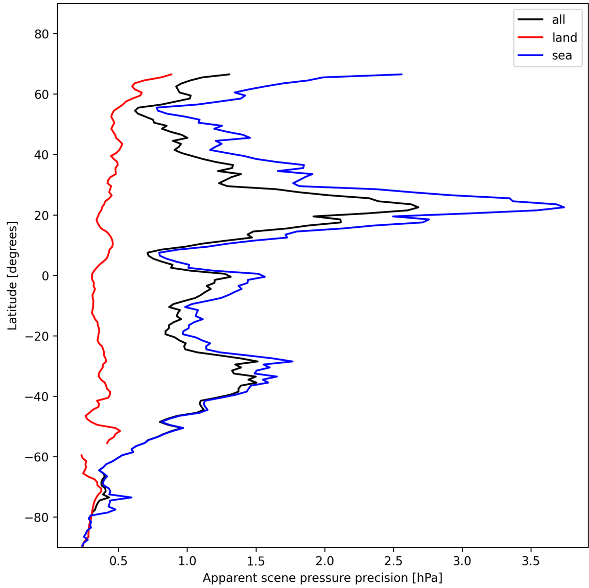
Figure 20: Zonal average of “Apparent scene pressure precision” for 2024-11-26 to 2024-11-28.
