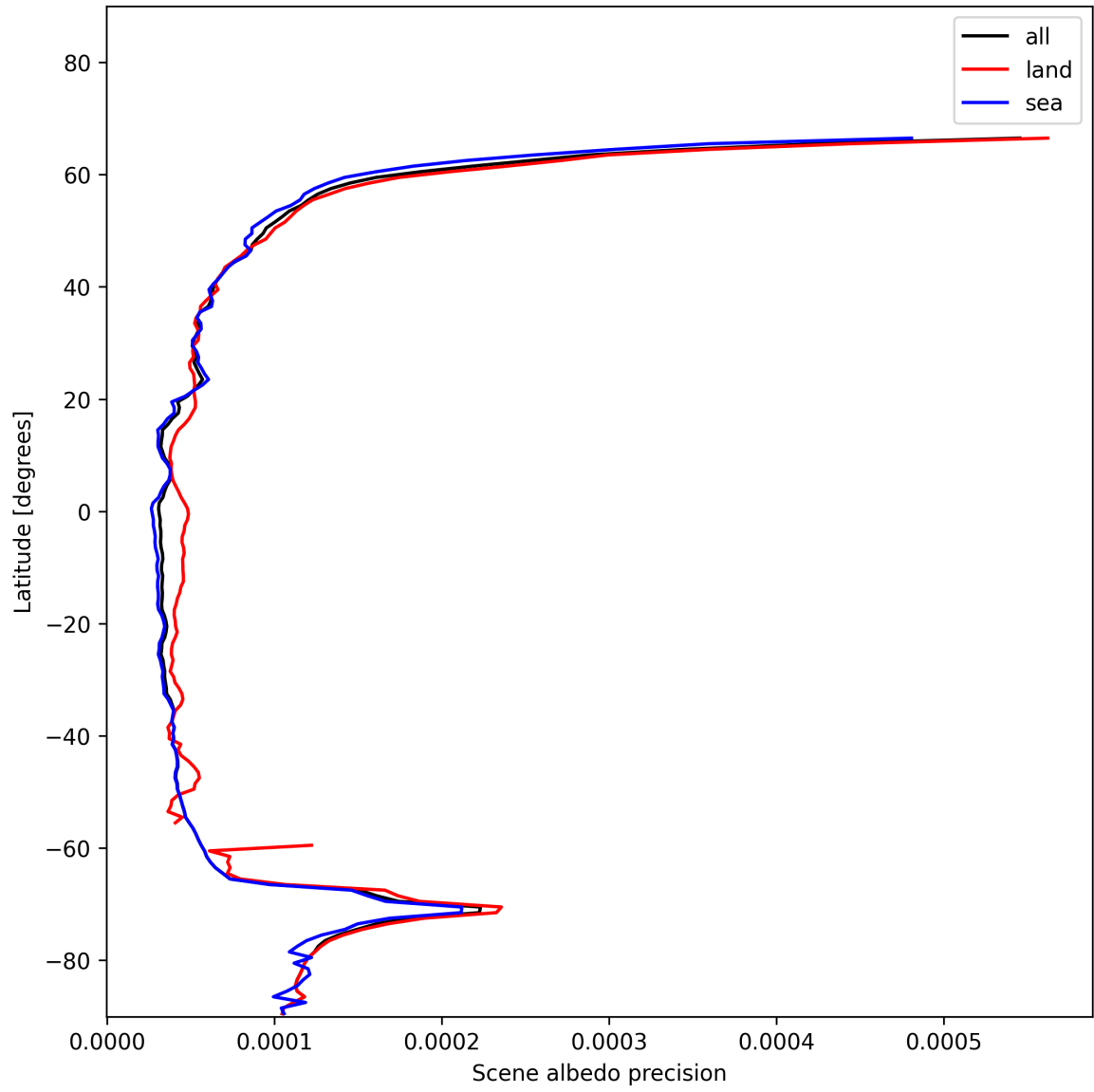
Figure 18: Zonal average of “Scene albedo precision” for 2024-11-26 to 2024-11-28.
