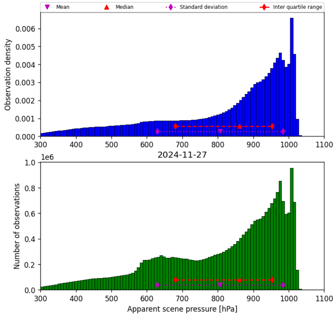
Figure 36: Histogram of “Apparent scene pressure” for 2024-11-26 to 2024-11-28
