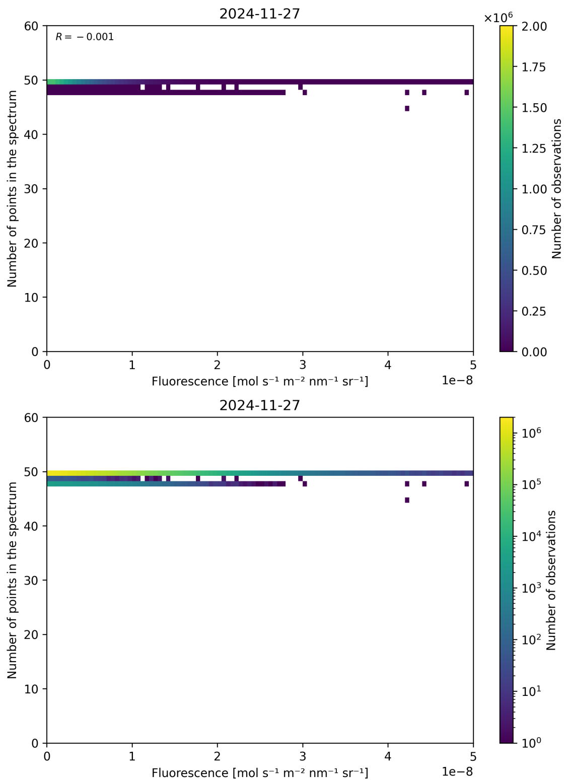
Figure 86: Scatter density plot of “Fluorescence” against “Number of points in the spectrum” for 2024-11-26 to 2024-11-28.
