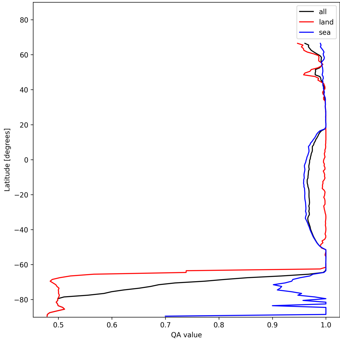
Figure 12: Zonal average of “QA value” for 2024-11-26 to 2024-11-28.
