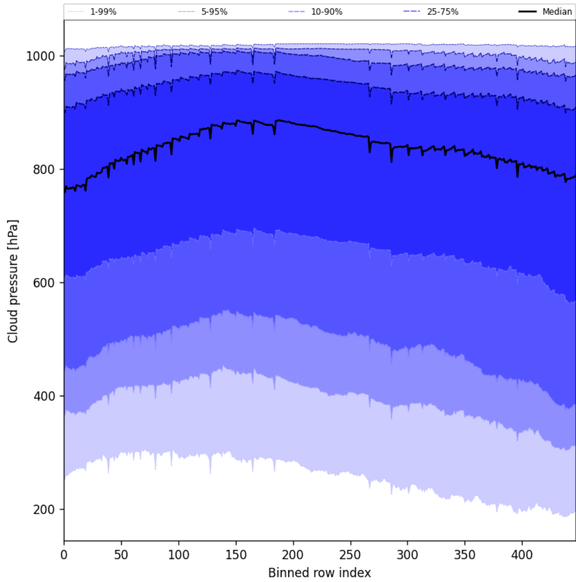
Figure 47: Along track statistics of “Cloud pressure” for 2024-11-26 to 2024-11-28
