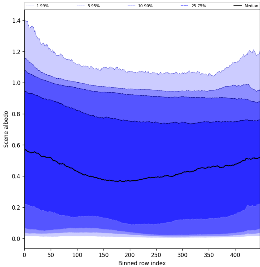
Figure 51: Along track statistics of “Scene albedo” for 2024-11-26 to 2024-11-28
