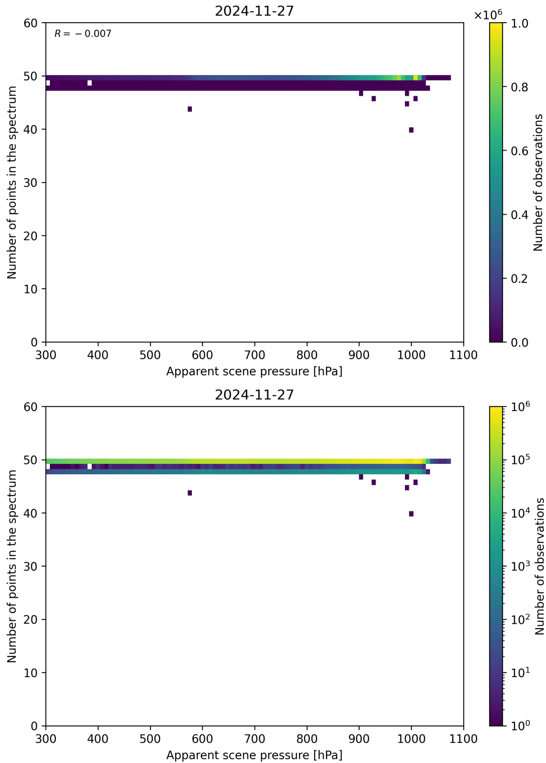
Figure 66: Scatter density plot of “Apparent scene pressure” against “Number of points in the spectrum” for 2024-11-26 to 2024-11-28.
