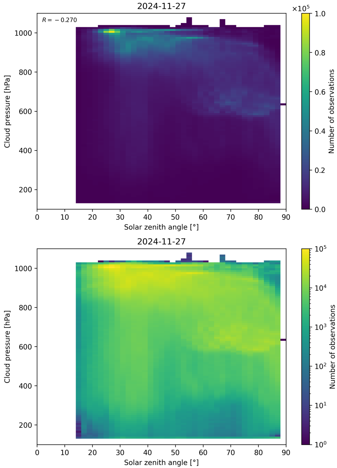
Figure 111: Scatter density plot of “Solar zenith angle” against “Cloud pressure” for 2024-11-26 to 2024-11-28.
