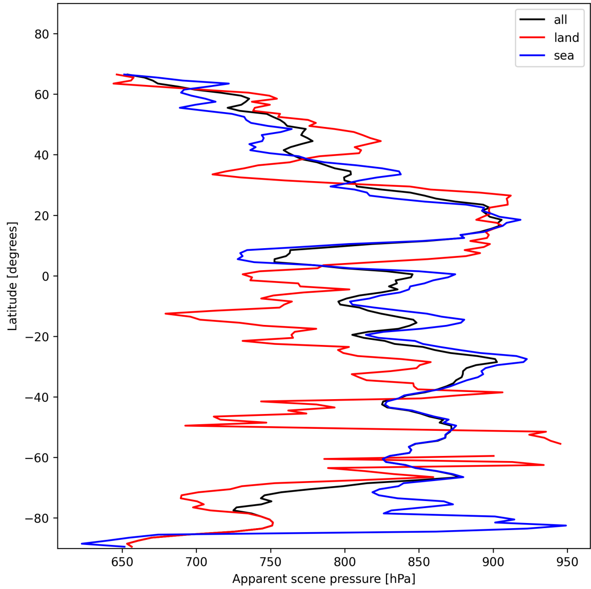
Figure 19: Zonal average of “Apparent scene pressure” for 2024-11-26 to 2024-11-28.
