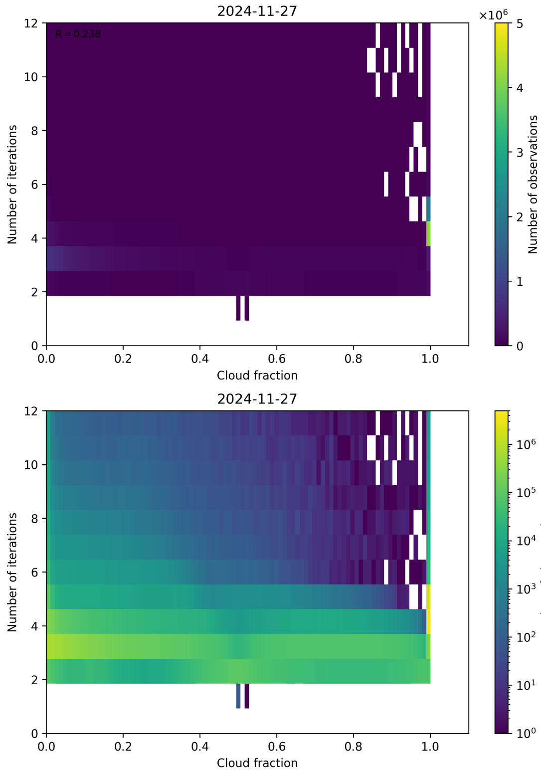
Figure 73: Scatter density plot of “Cloud fraction” against “Number of iterations” for 2024-11-26 to 2024-11-28.
