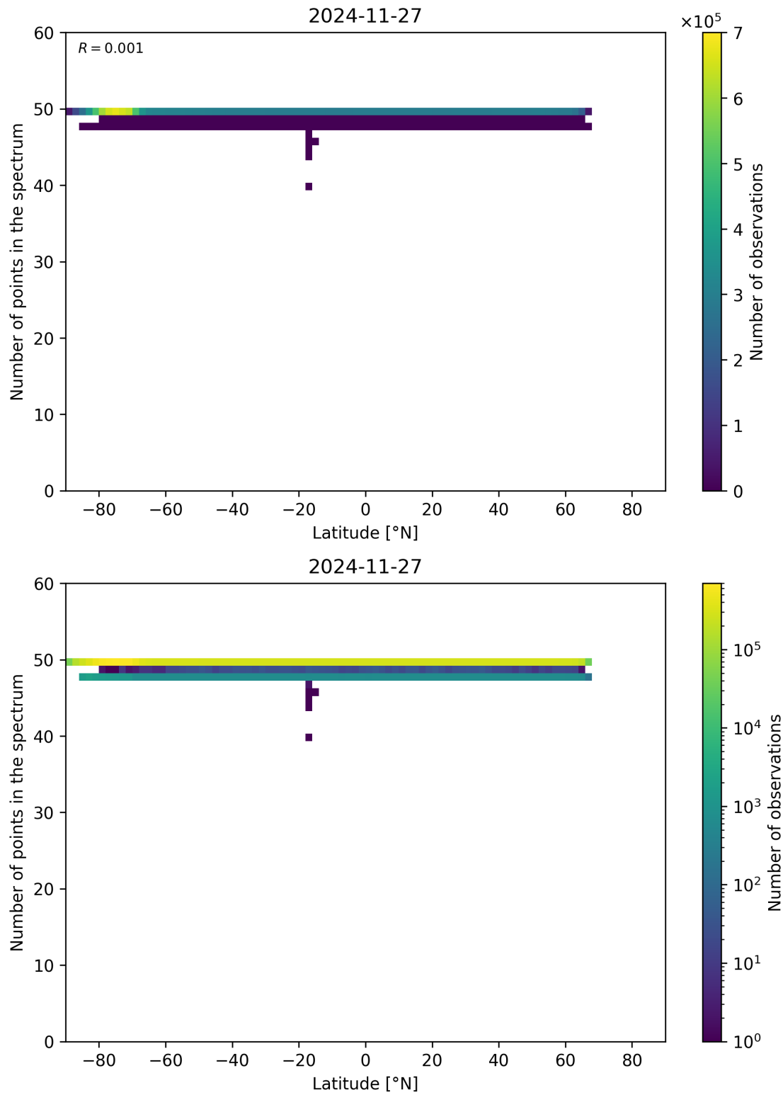
Figure 94: Scatter density plot of “Latitude” against “Number of points in the spectrum” for 2024-11-26 to 2024-11-28.
