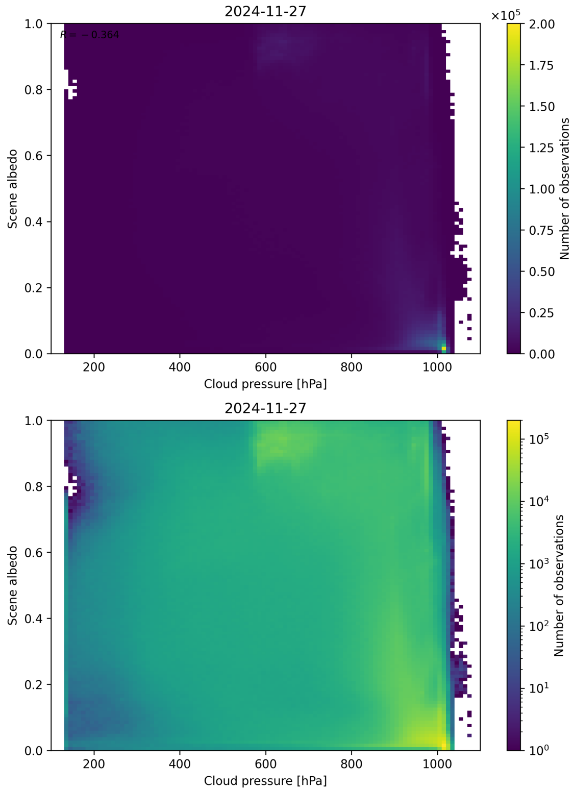
Figure 83: Scatter density plot of “Cloud pressure” against “Scene albedo” for 2024-11-26 to 2024-11-28.
