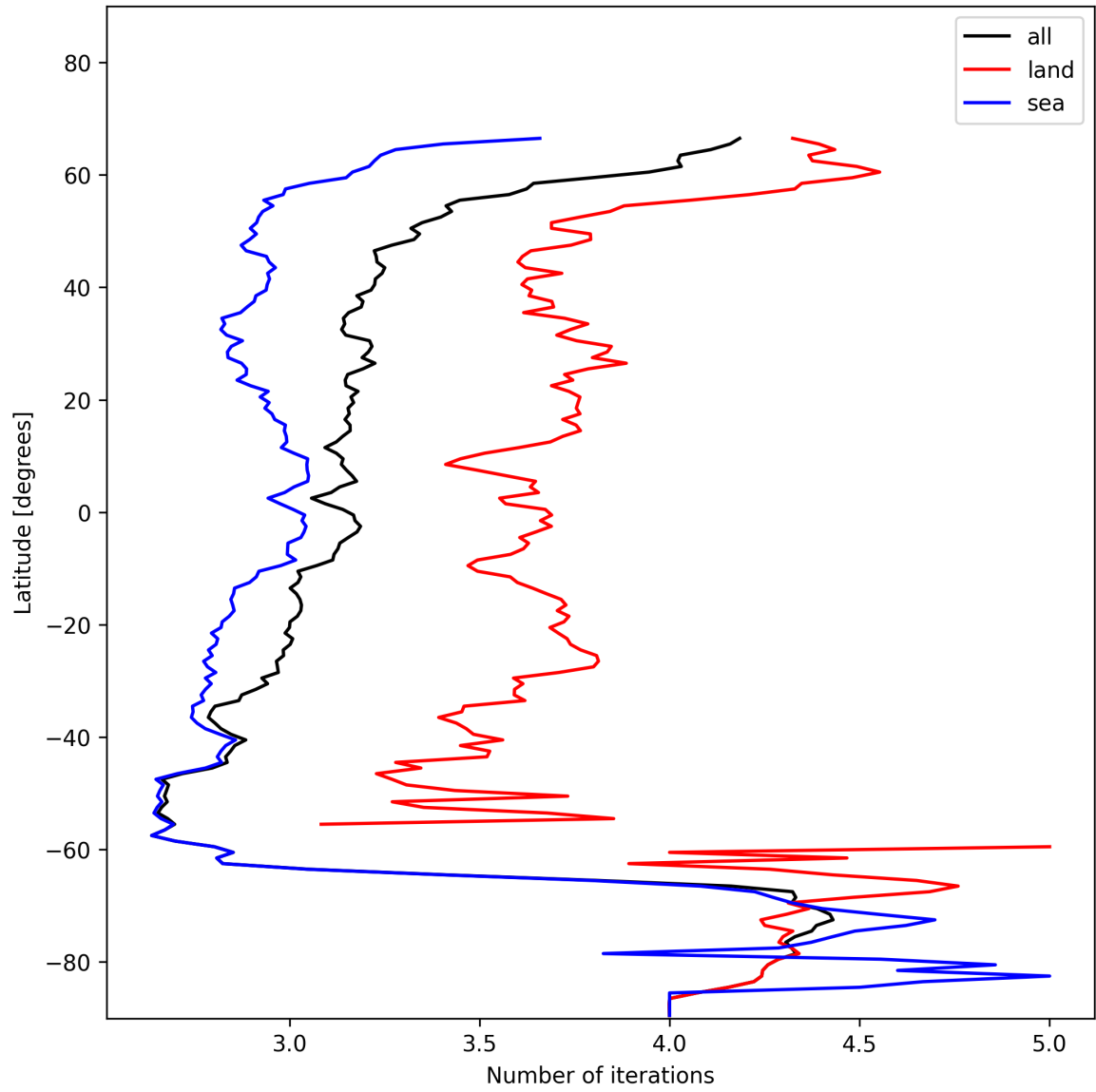
Figure 22: Zonal average of “Number of iterations” for 2024-11-26 to 2024-11-28.
