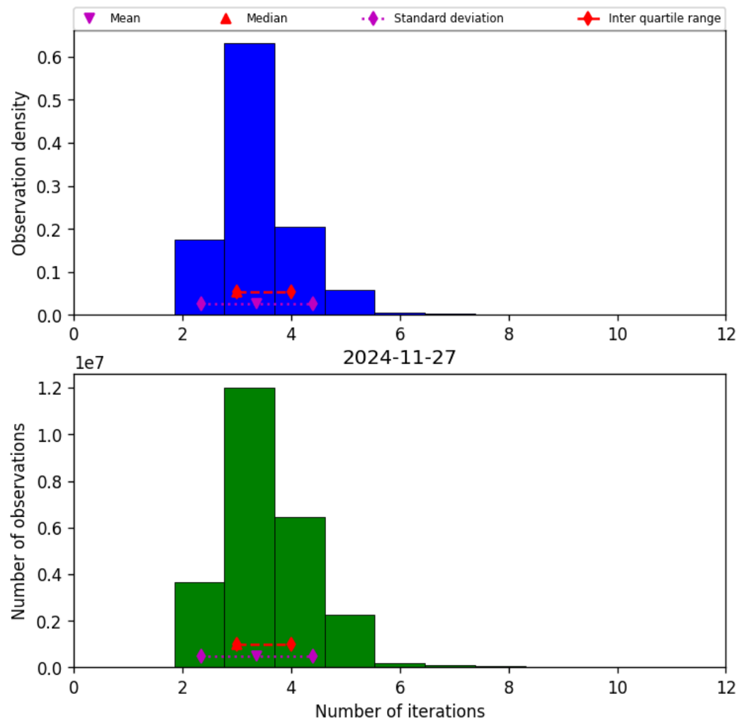
Figure 39: Histogram of “Number of iterations” for 2024-11-26 to 2024-11-28
