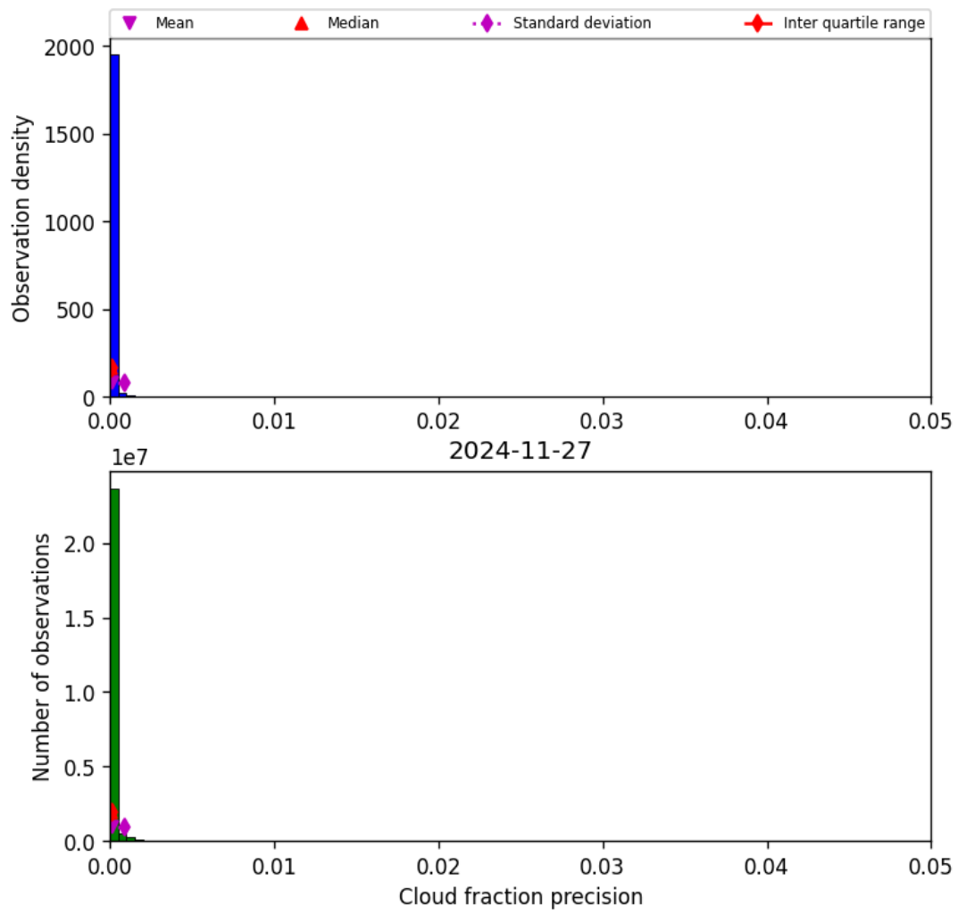
Figure 33: Histogram of “Cloud fraction precision” for 2024-11-26 to 2024-11-28
