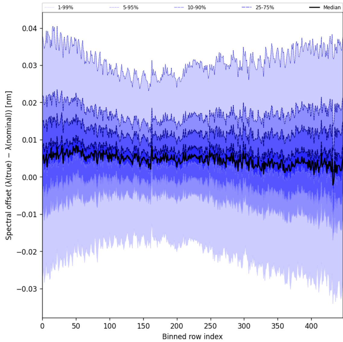
Figure 62: Along track statistics of “Spectral offset ( \lambda_{\text{true}} - \lambda_{\text{nominal}} )” for 2024-11-26 to 2024-11-28
