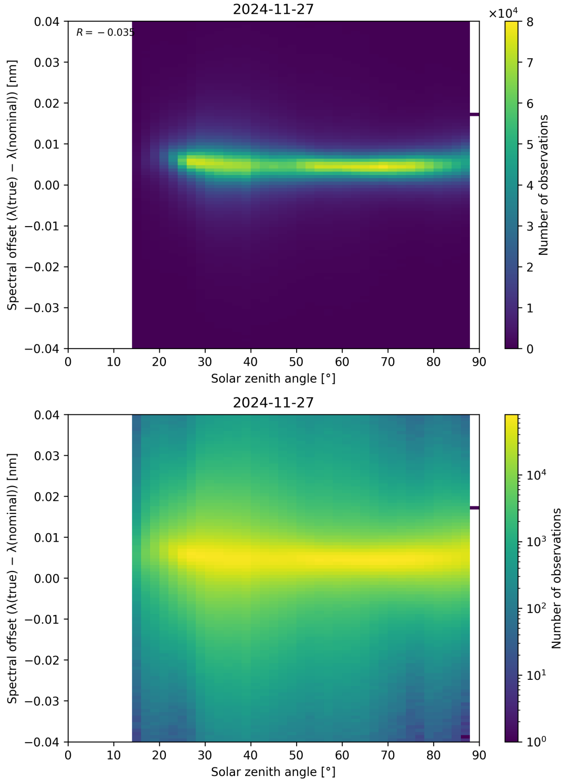
Figure 117: Scatter density plot of “Solar zenith angle” against “Spectral offset ( \lambda_{\text{true}} - \lambda_{\text{nominal}} )” for 2024-11-26 to 2024-11-28.
