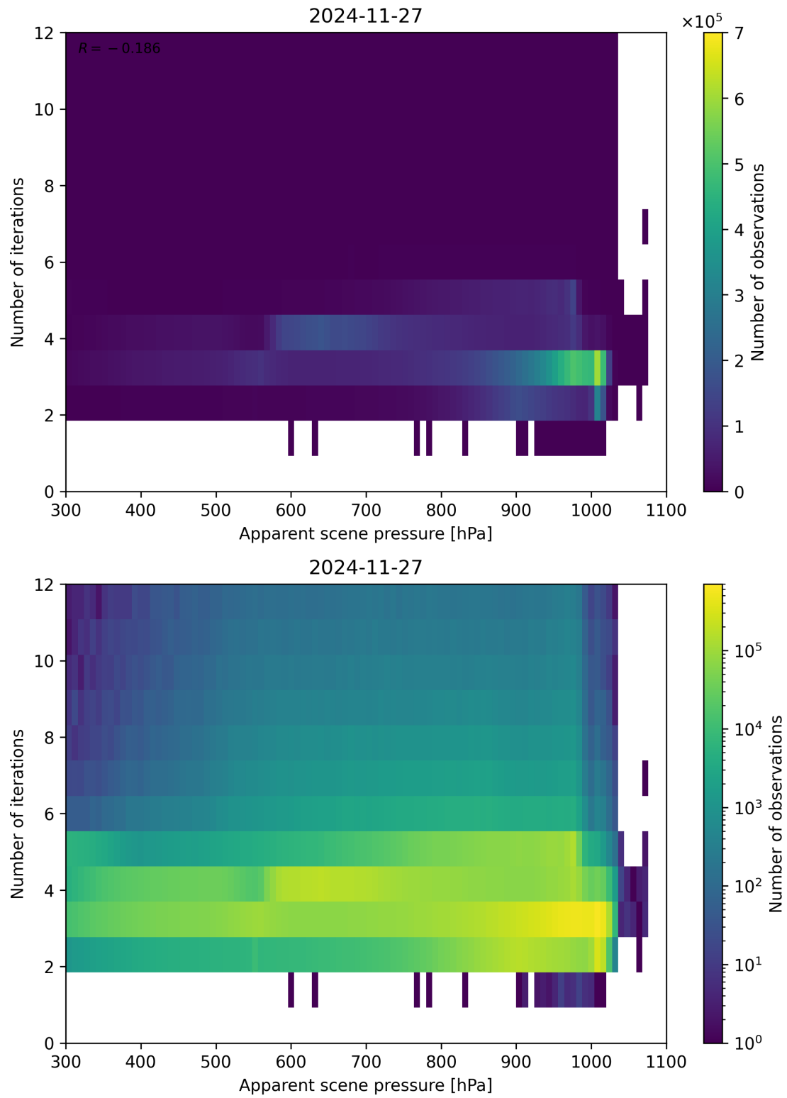
Figure 65: Scatter density plot of “Apparent scene pressure” against “Number of iterations” for 2024-11-26 to 2024-11-28.
