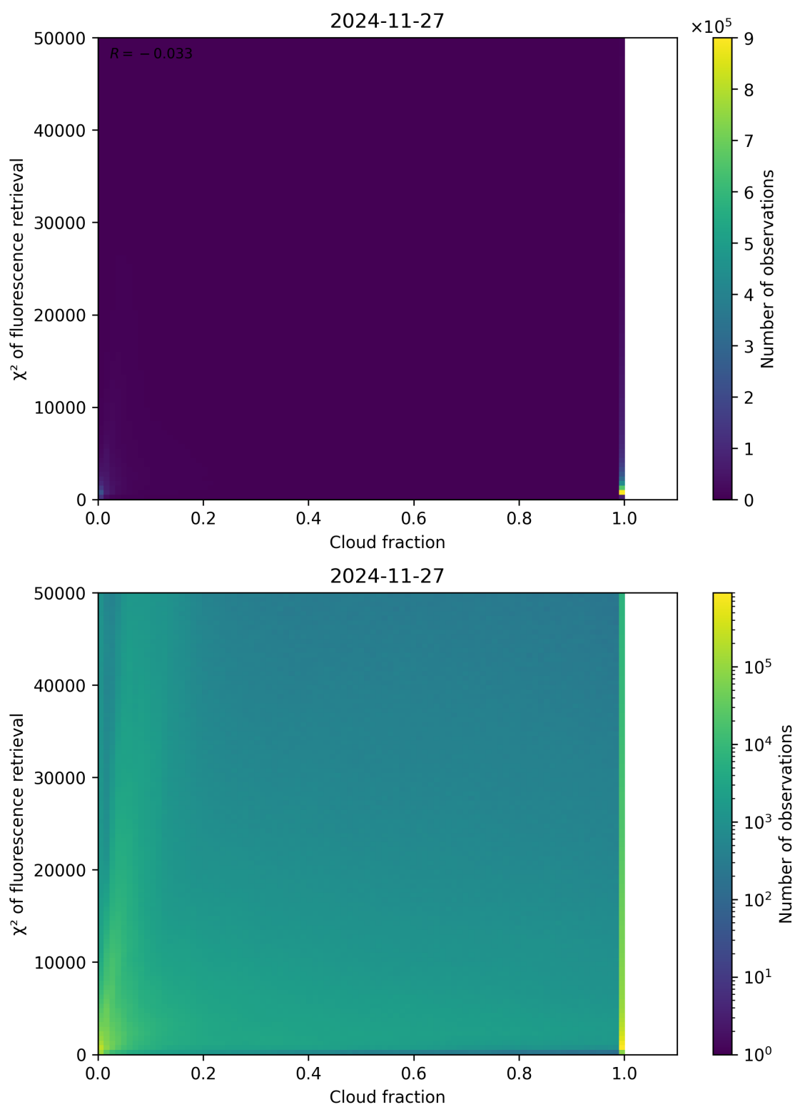
Figure 71: Scatter density plot of “Cloud fraction” against “ \chi^2 of fluorescence retrieval” for 2024-11-26 to 2024-11-28.
