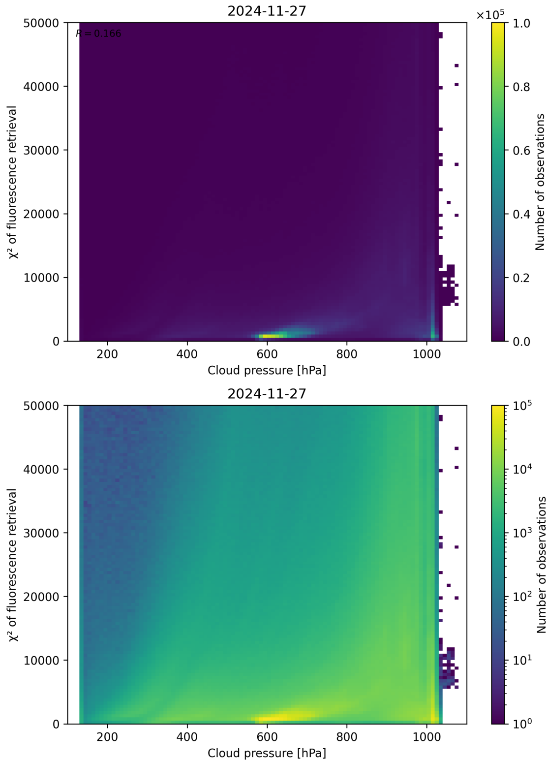
Figure 78: Scatter density plot of “Cloud pressure” against “ \chi^2 of fluorescence retrieval” for 2024-11-26 to 2024-11-28.
