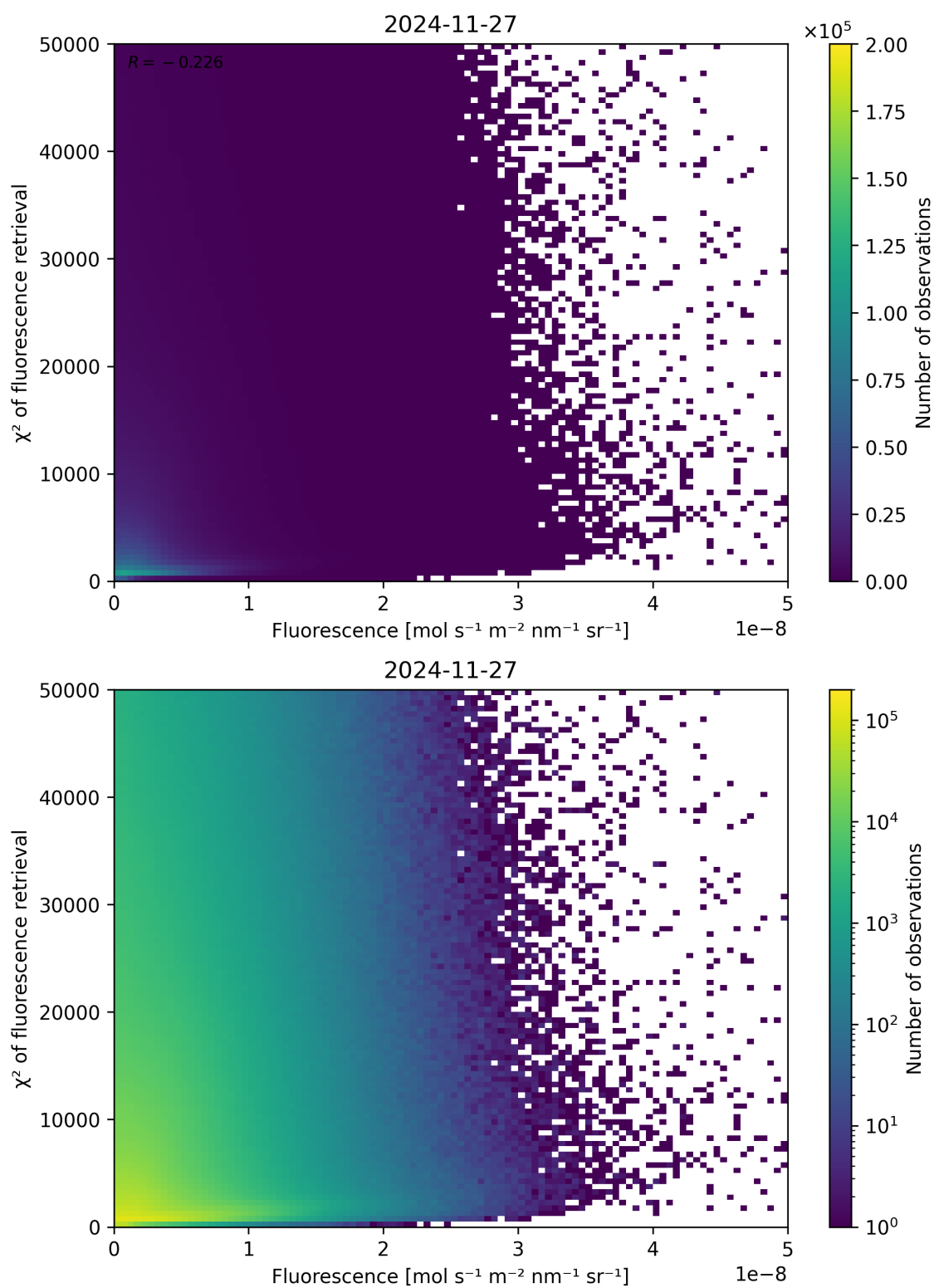
Figure 85: Scatter density plot of “Fluorescence” against “ \chi^2 of fluorescence retrieval” for 2024-11-26 to 2024-11-28.
