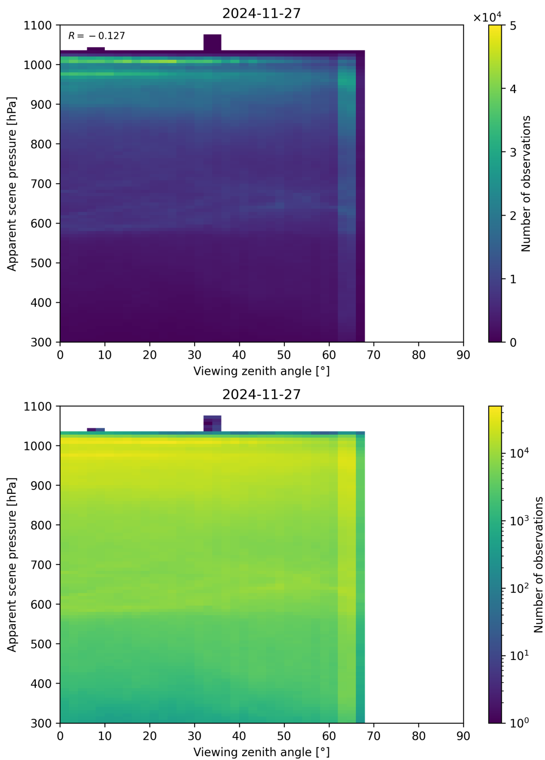
Figure 118: Scatter density plot of “Viewing zenith angle” against “Apparent scene pressure” for 2024-11-26 to 2024-11-28.
