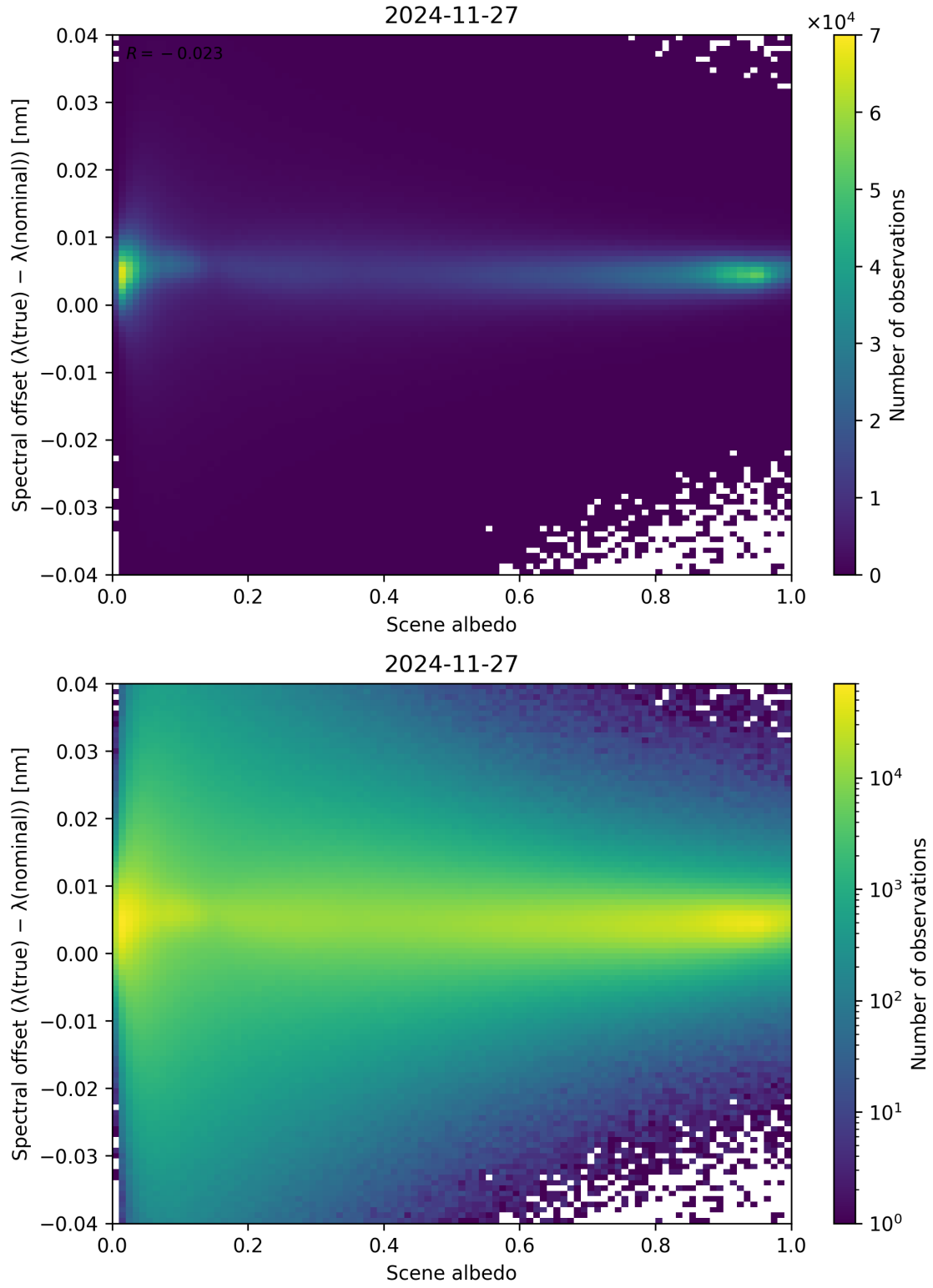
Figure 107: Scatter density plot of “Scene albedo” against “Spectral offset ( \lambda_{\text{true}} - \lambda_{\text{nominal}} )” for 2024-11-26 to 2024-11-28.
