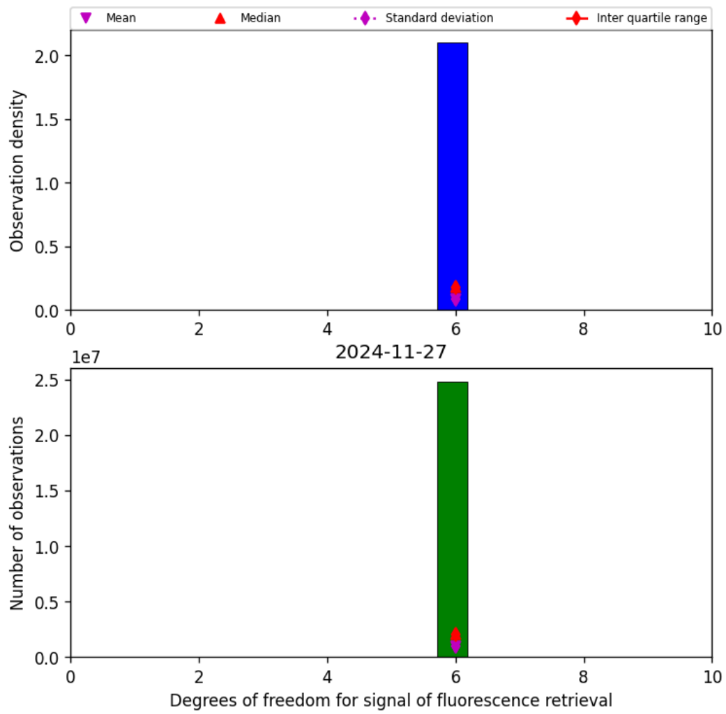
Figure 43: Histogram of "Degrees of freedom for signal of fluorescence retrieval" for 2024-11-26 to 2024-11-28
