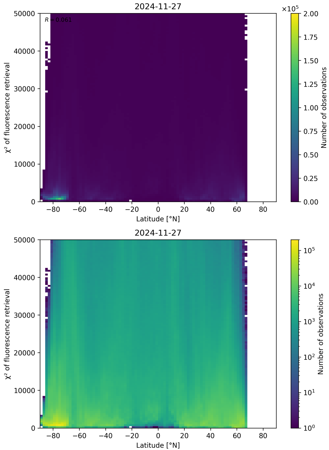
Figure 89: Scatter density plot of “Latitude” against “ \chi^2 of fluorescence retrieval” for 2024-11-26 to 2024-11-28.
