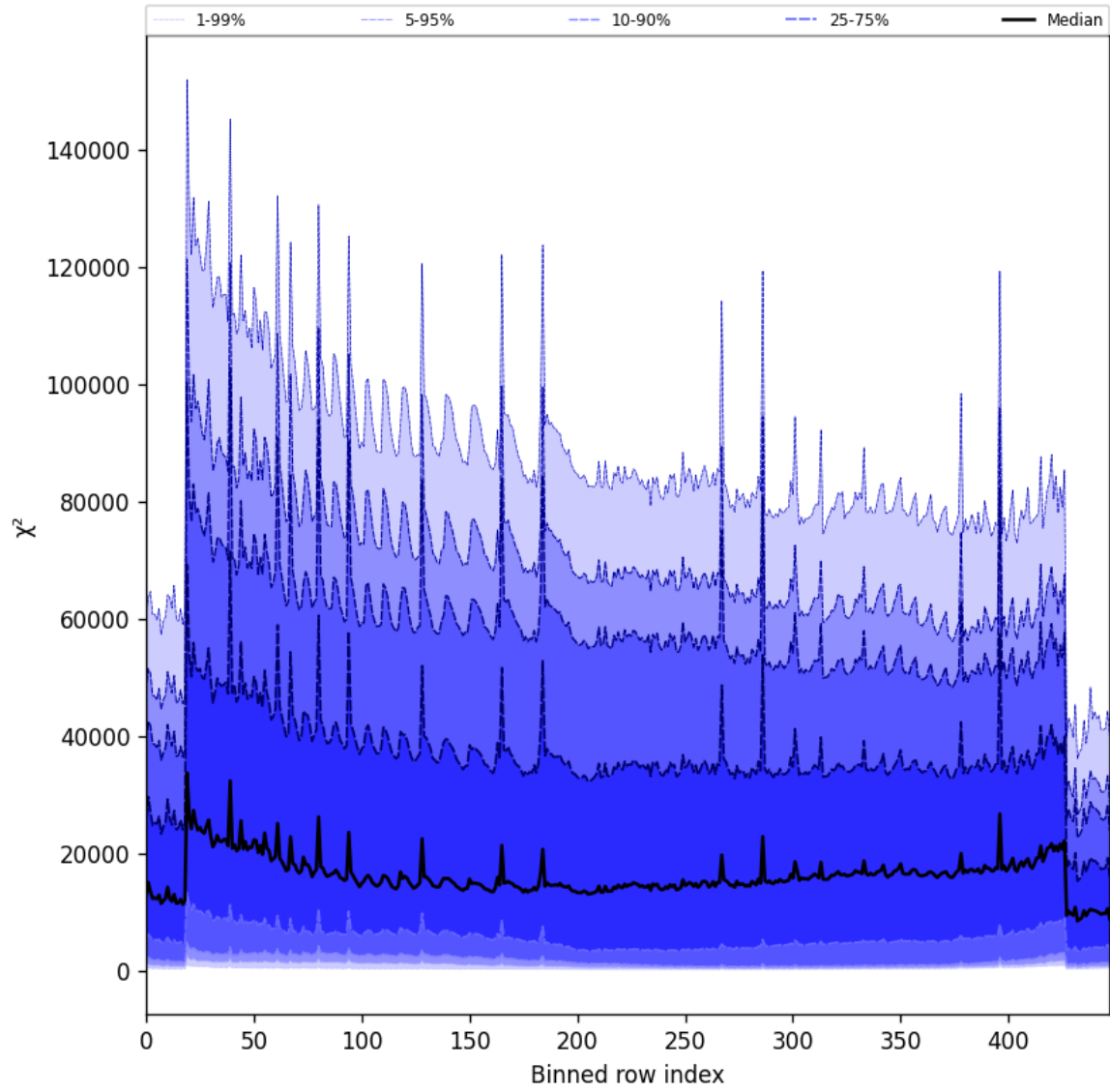
Figure 55: Along track statistics of “ \chi^2 ” for 2024-11-26 to 2024-11-28
