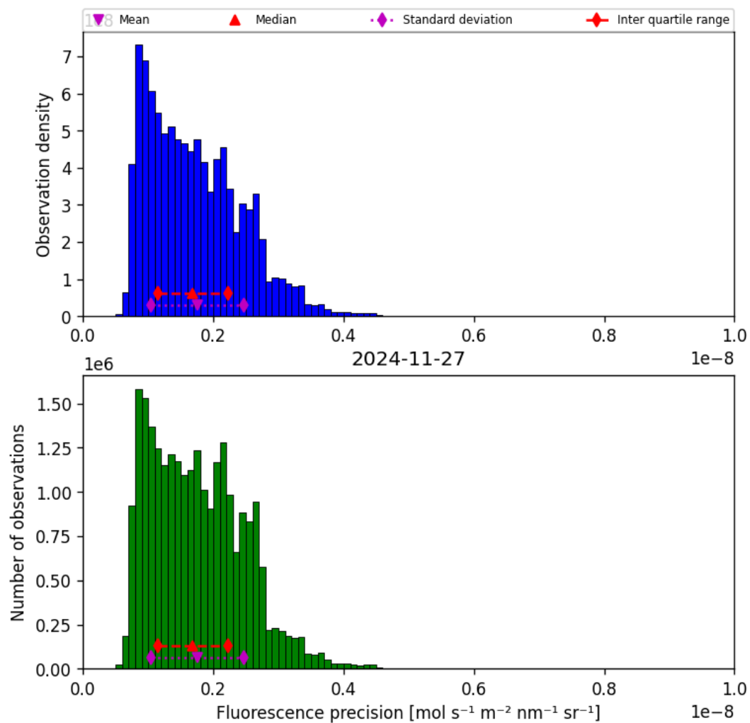
Figure 41: Histogram of “Fluorescence precision” for 2024-11-26 to 2024-11-28
