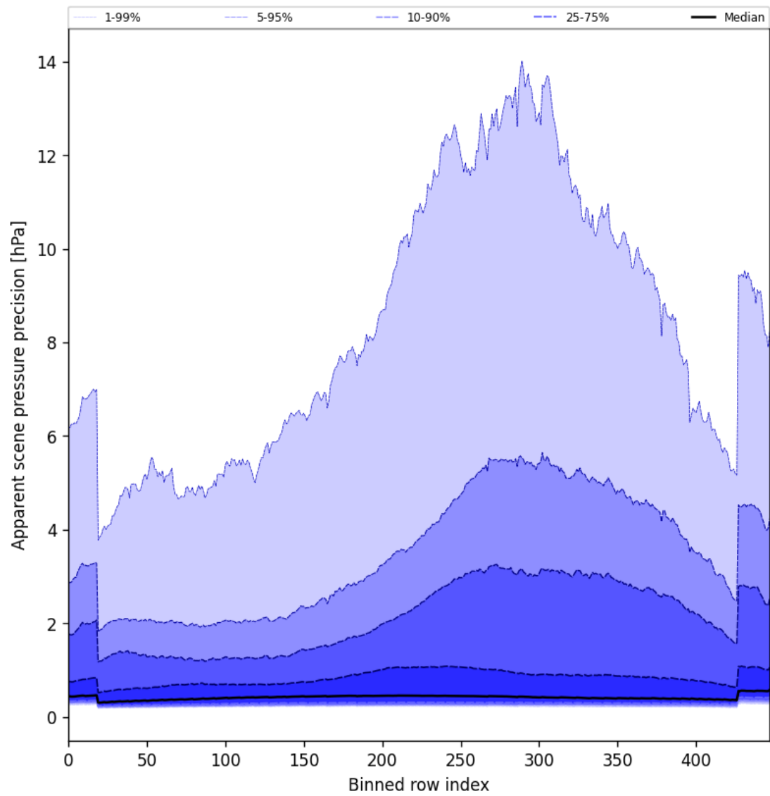
Figure 54: Along track statistics of “Apparent scene pressure precision” for 2024-11-26 to 2024-11-28
