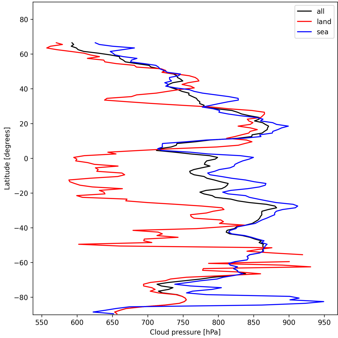
Figure 13: Zonal average of “Cloud pressure” for 2024-11-26 to 2024-11-28.
