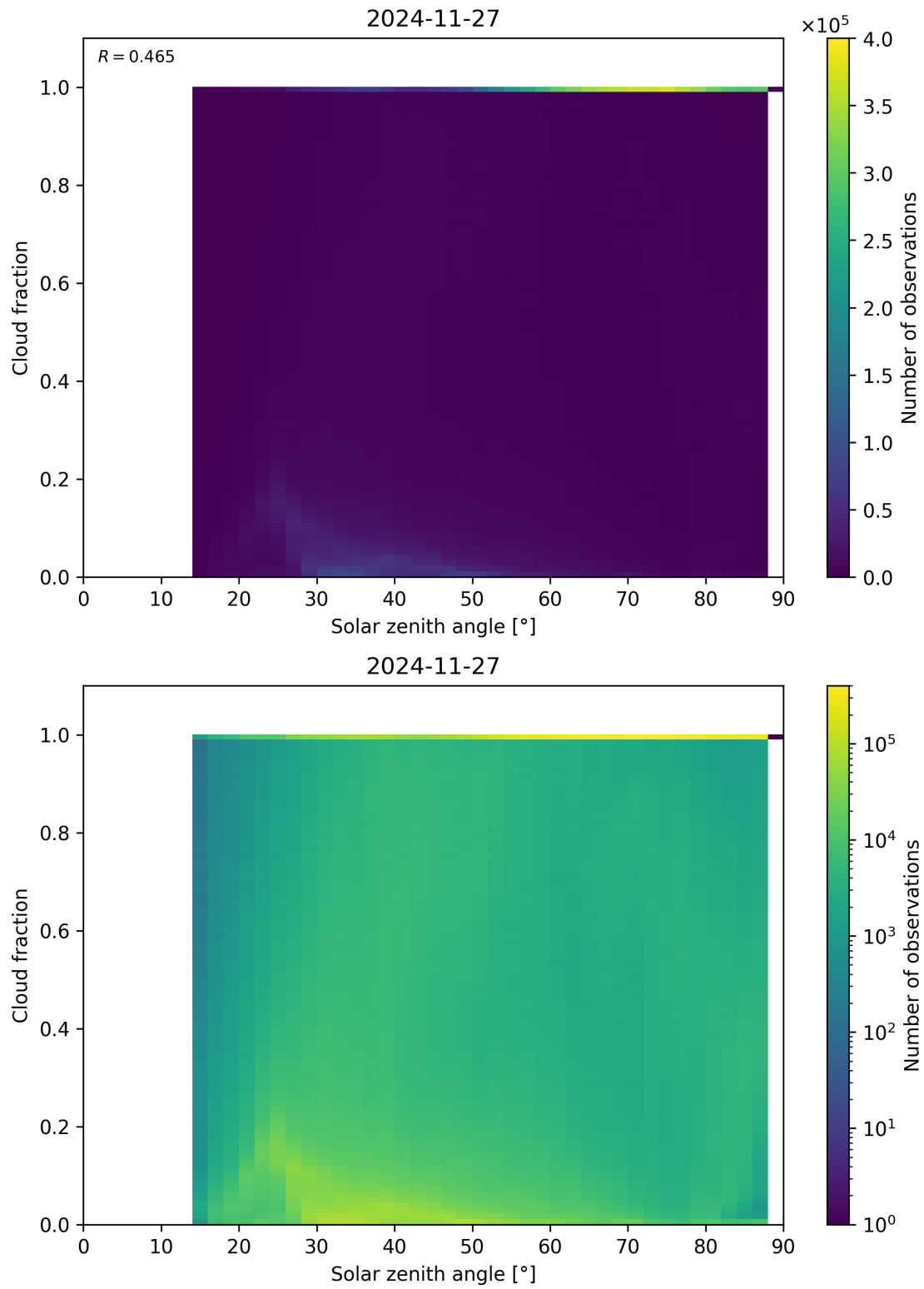
Figure 110: Scatter density plot of “Solar zenith angle” against “Cloud fraction” for 2024-11-26 to 2024-11-28.
