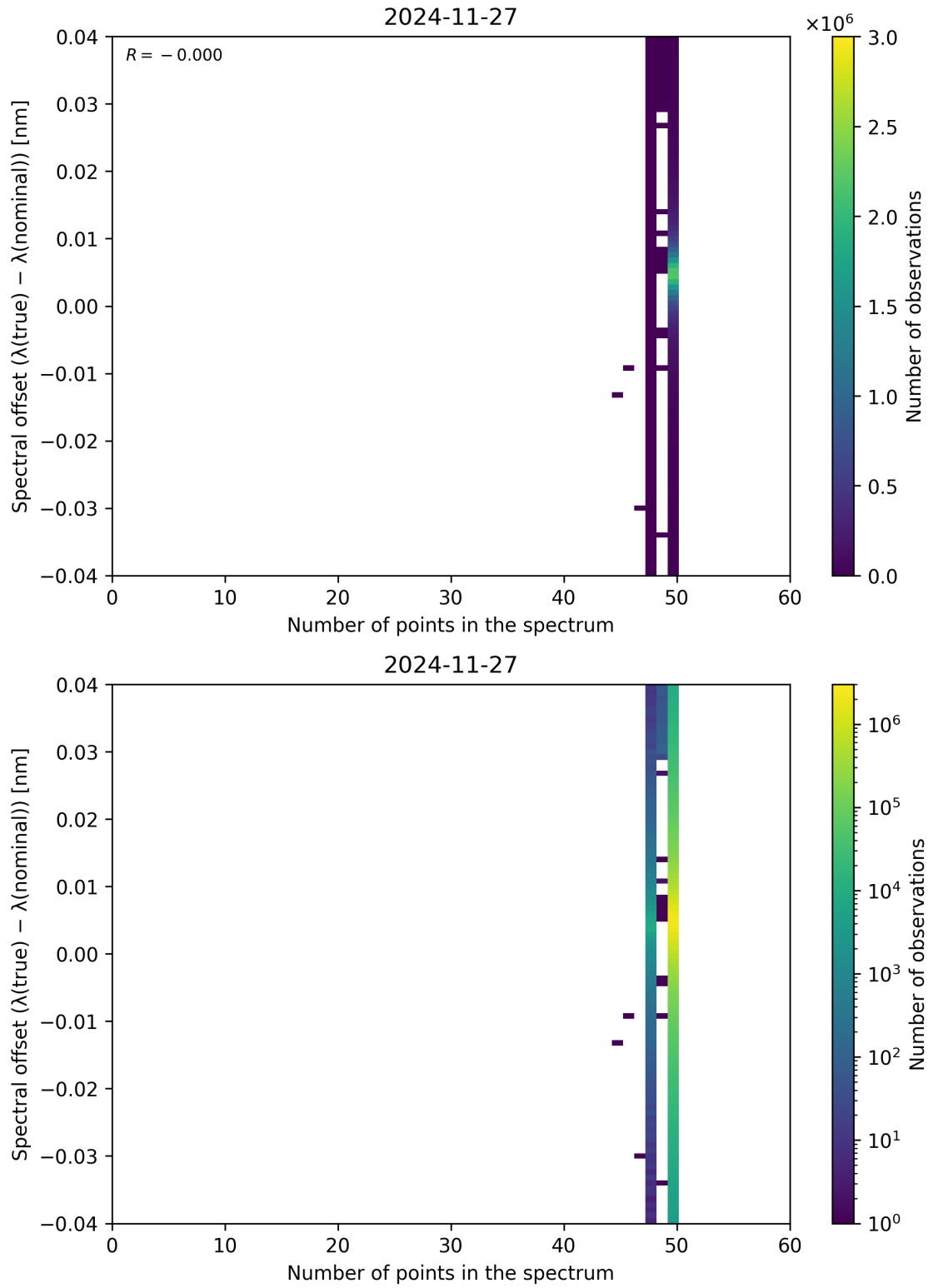
Figure 101: Scatter density plot of “Number of points in the spectrum” against “Spectral offset ( \lambda_{\text{true}} - \lambda_{\text{nominal}} )” for 2024-11-26 to 2024-11-28.
