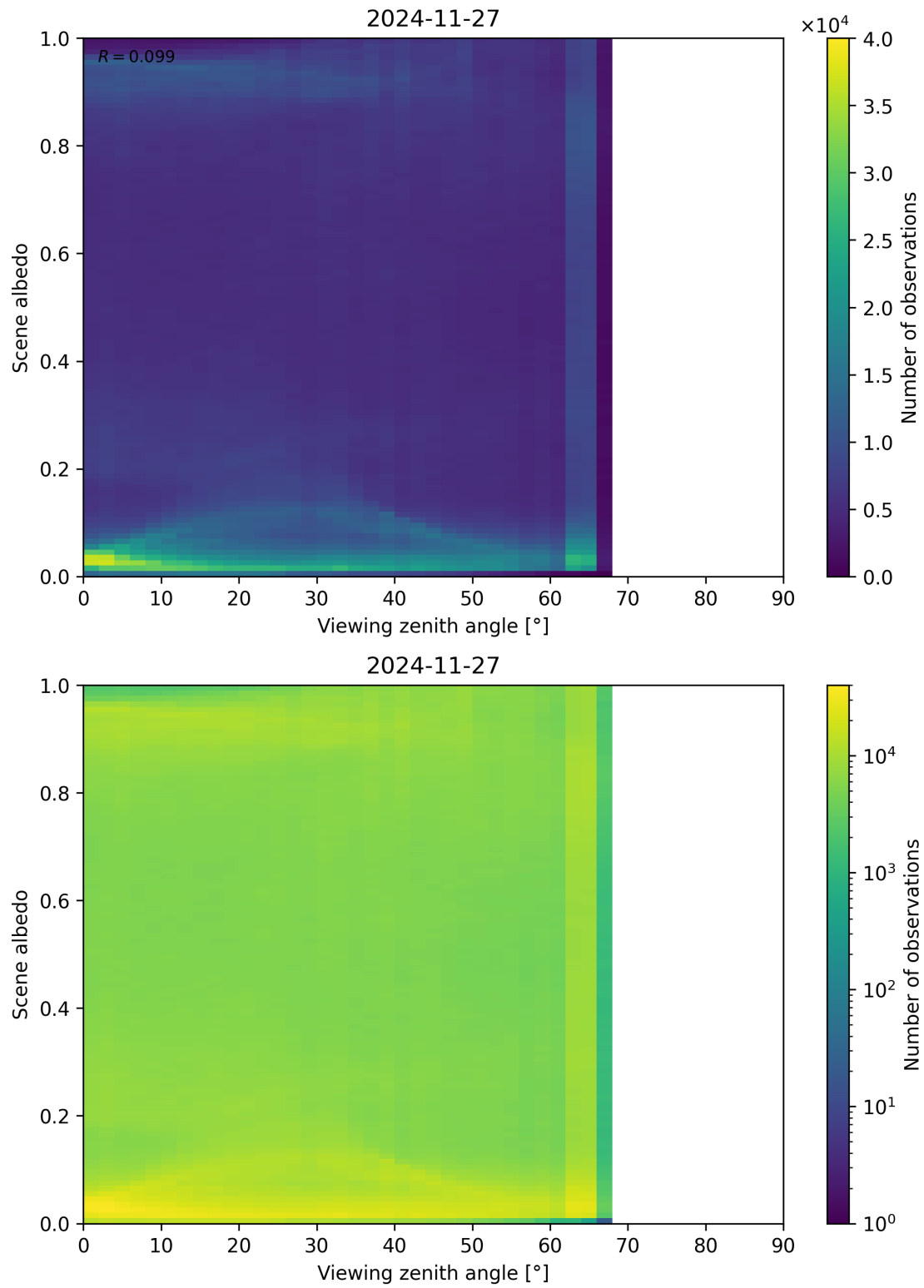
Figure 126: Scatter density plot of “Viewing zenith angle” against “Scene albedo” for 2024-11-26 to 2024-11-28.
