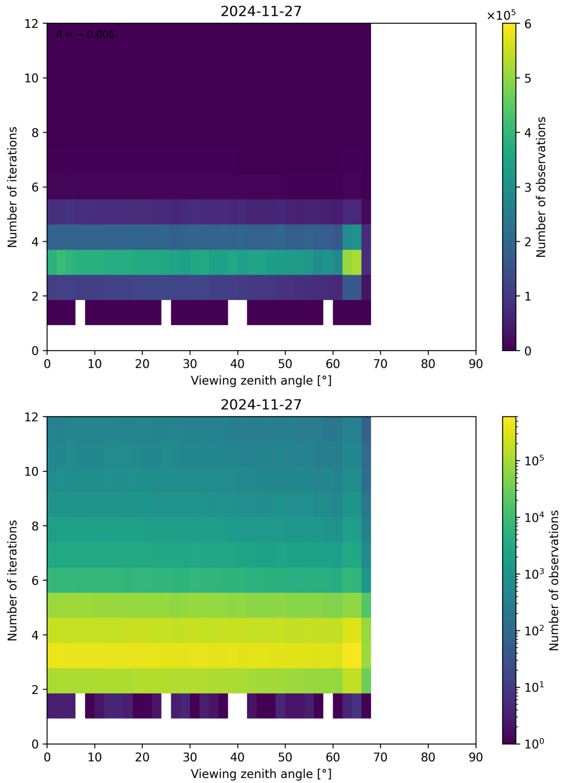
Figure 124: Scatter density plot of “Viewing zenith angle” against “Number of iterations” for 2024-11-26 to 2024-11-28.
