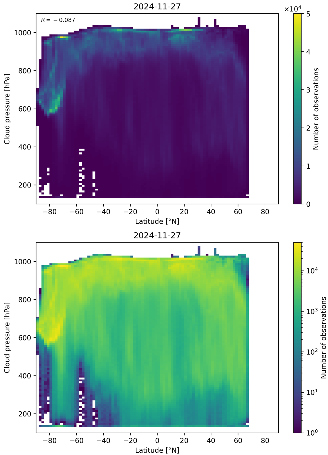
Figure 91: Scatter density plot of “Latitude” against “Cloud pressure” for 2024-11-26 to 2024-11-28.
