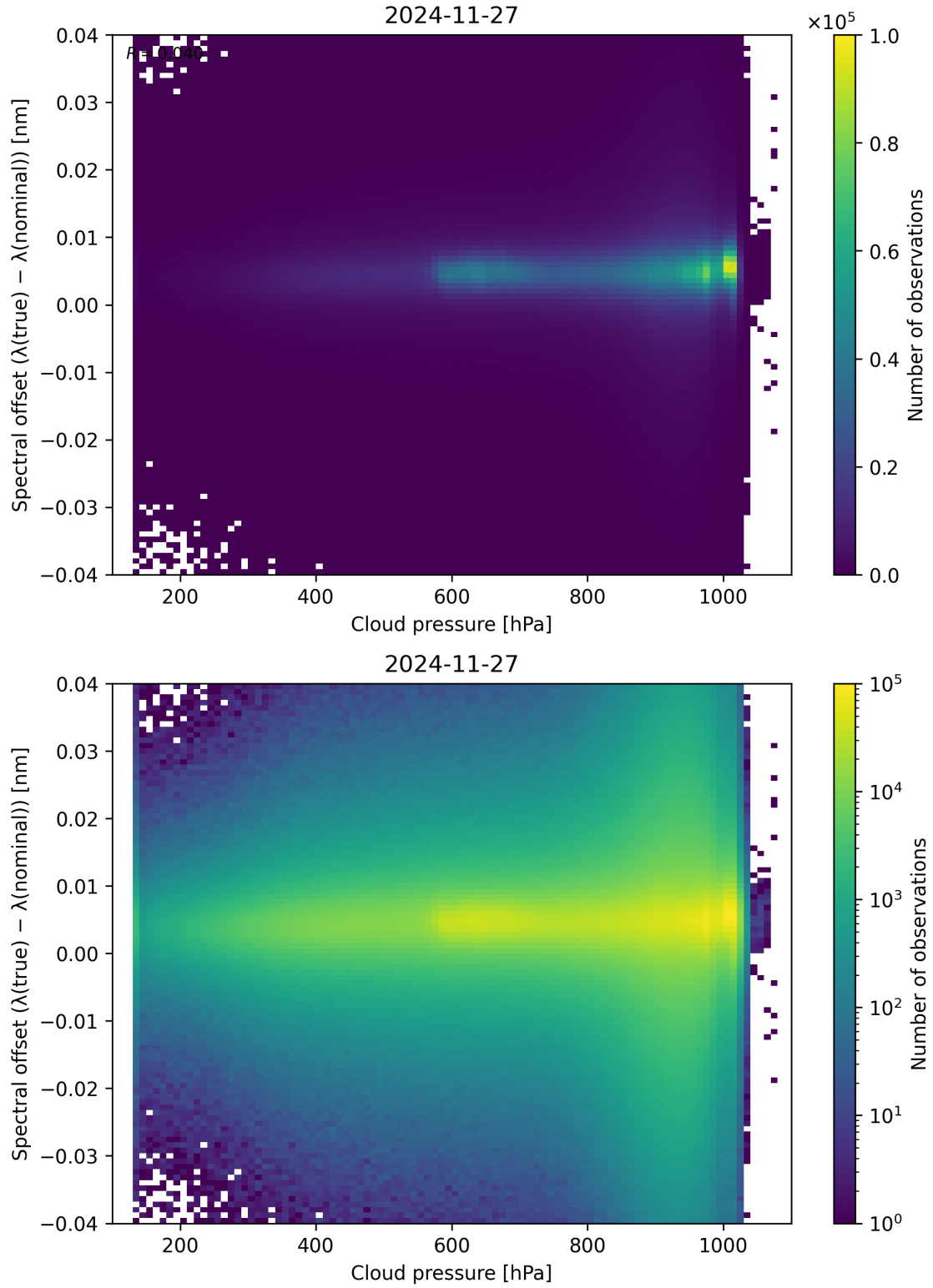
Figure 84: Scatter density plot of “Cloud pressure” against “Spectral offset ( \lambda_{\text{true}} - \lambda_{\text{nominal}} )” for 2024-11-26 to 2024-11-28.
