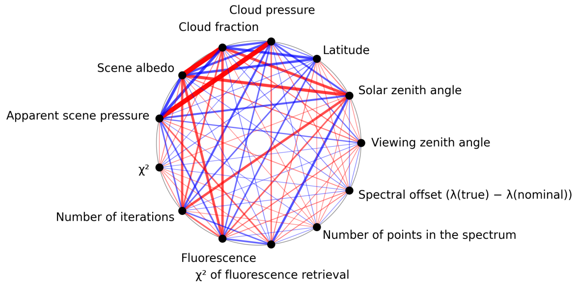
Figure 1: Map of correlation graph for 2024-11-26 to 2024-11-28.
