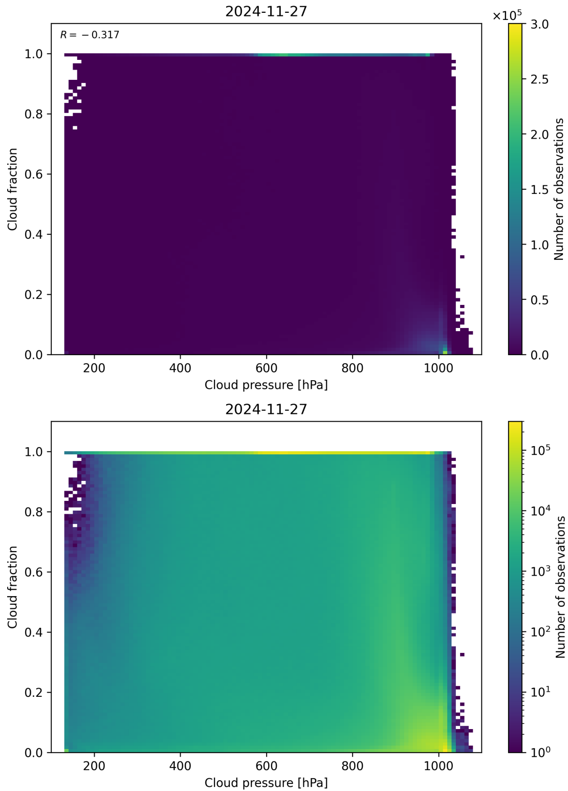
Figure 79: Scatter density plot of “Cloud pressure” against “Cloud fraction” for 2024-11-26 to 2024-11-28.
