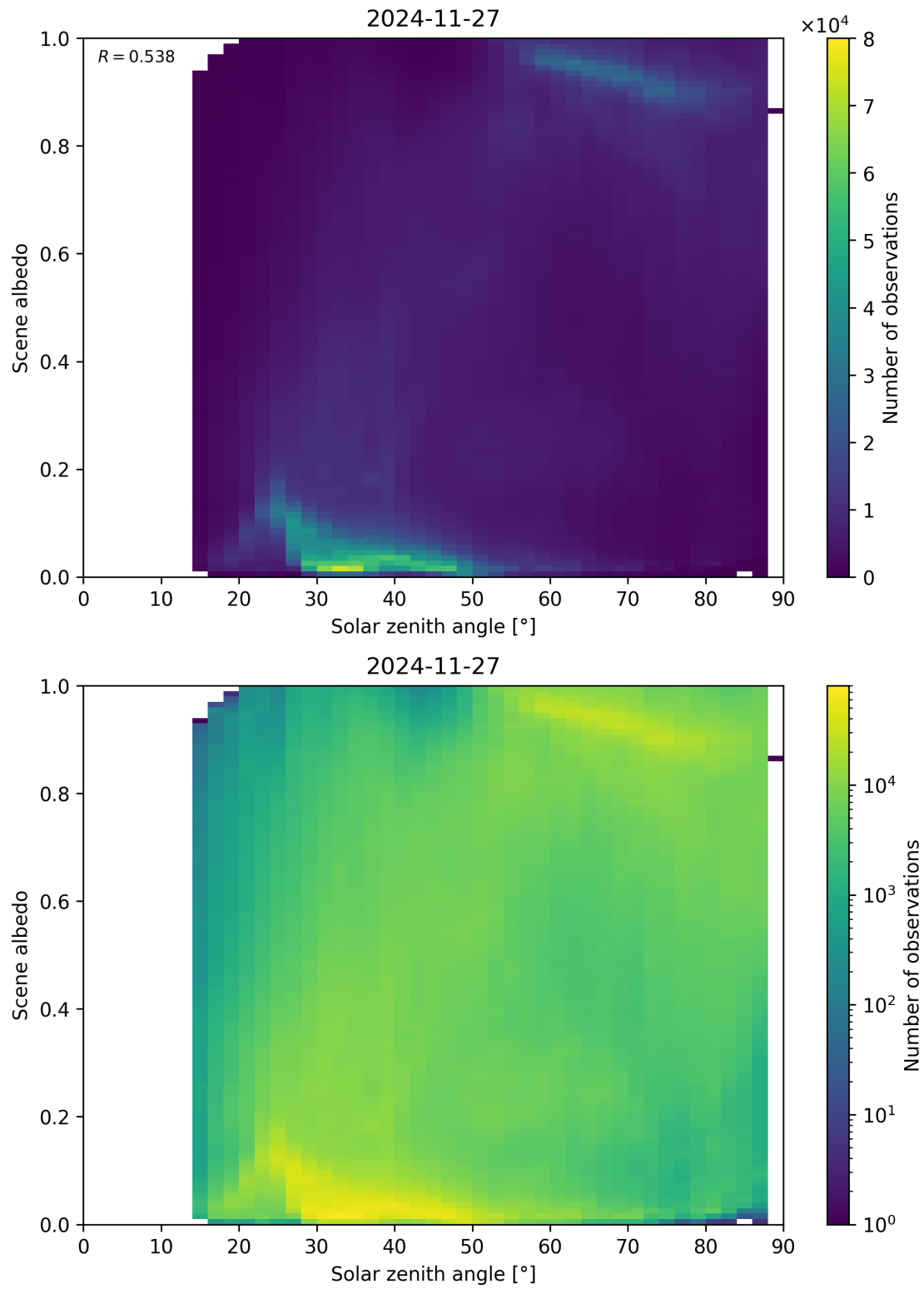
Figure 116: Scatter density plot of “Solar zenith angle” against “Scene albedo” for 2024-11-26 to 2024-11-28.
