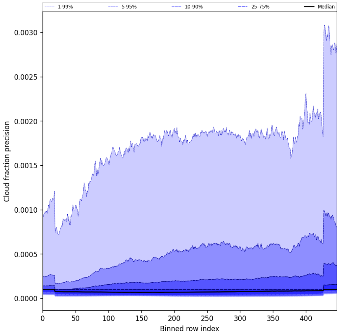
Figure 50: Along track statistics of “Cloud fraction precision” for 2024-11-26 to 2024-11-28
