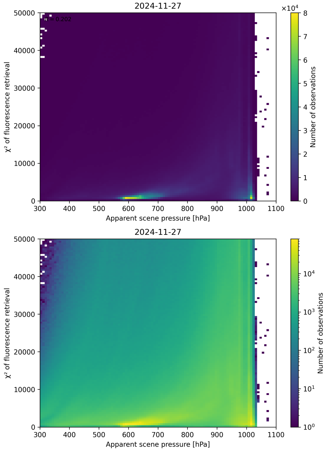
Figure 63: Scatter density plot of “Apparent scene pressure” against “ \chi^2 of fluorescence retrieval” for 2024-11-26 to 2024-11-28.
