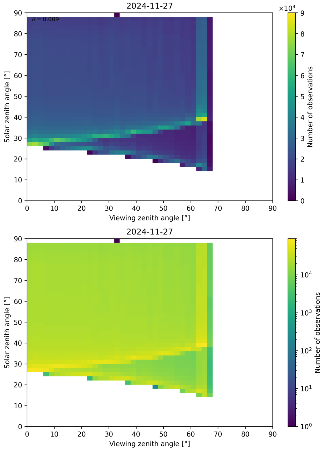
Figure 127: Scatter density plot of “Viewing zenith angle” against “Solar zenith angle” for 2024-11-26 to 2024-11-28.
