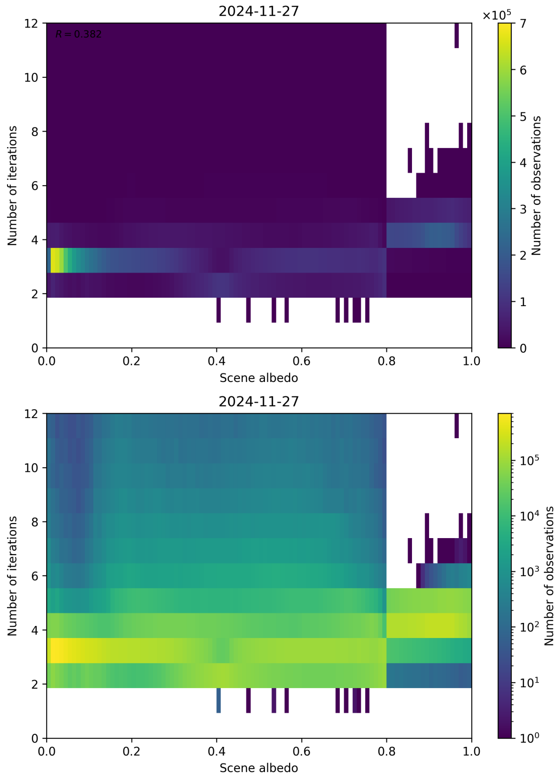
Figure 105: Scatter density plot of “Scene albedo” against “Number of iterations” for 2024-11-26 to 2024-11-28.
