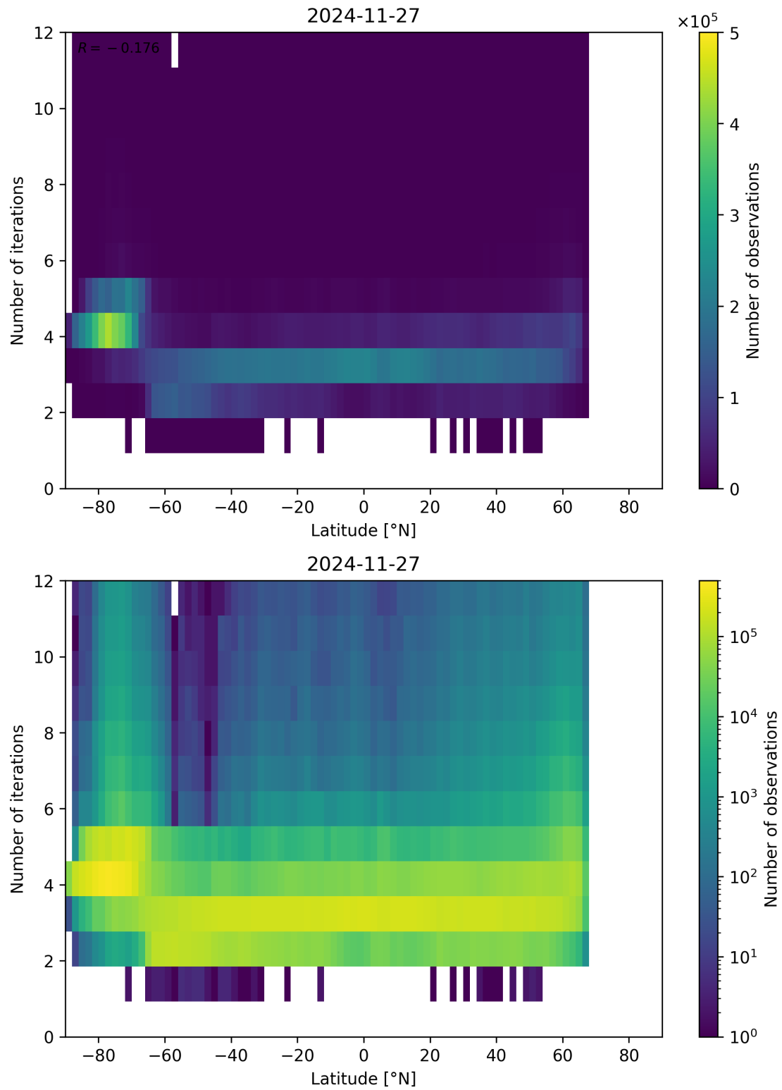
Figure 93: Scatter density plot of “Latitude” against “Number of iterations” for 2024-11-26 to 2024-11-28.
