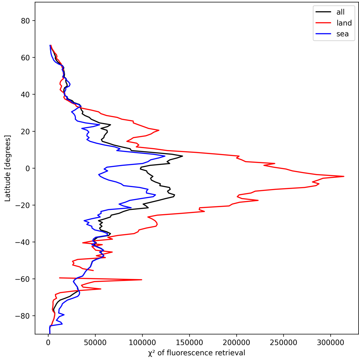
Figure 25: Zonal average of “ \chi^2 of fluorescence retrieval” for 2024-11-26 to 2024-11-28.
