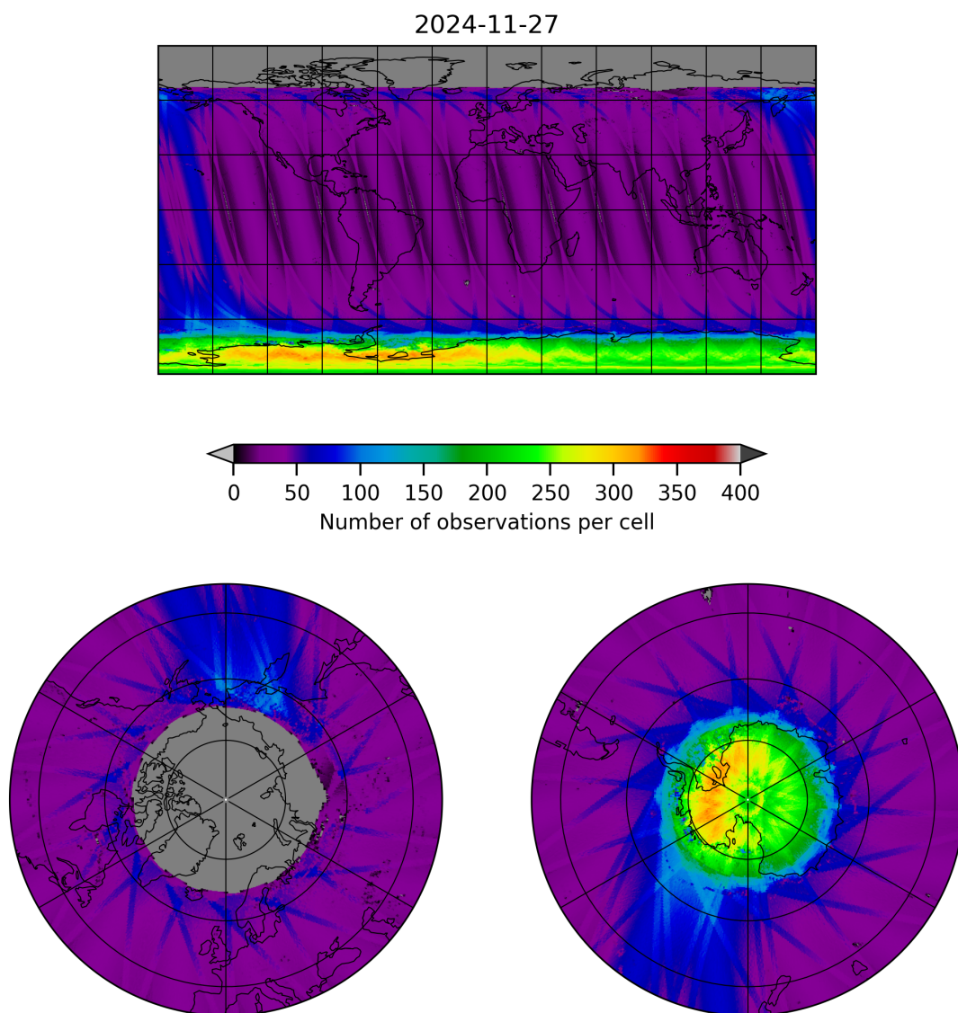
Figure 11: Map of the number of observations for 2024-11-26 to 2024-11-28
