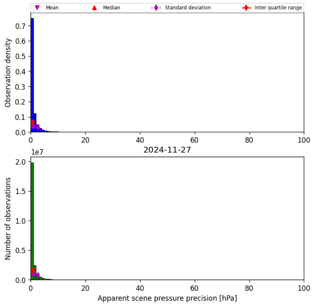
Figure 37: Histogram of “Apparent scene pressure precision” for 2024-11-26 to 2024-11-28
