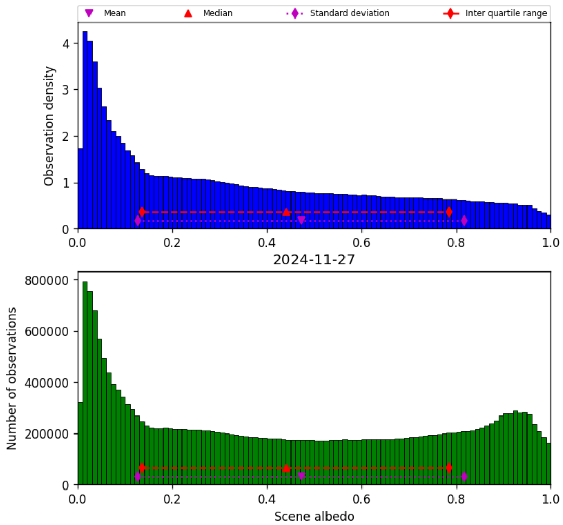
Figure 34: Histogram of “Scene albedo” for 2024-11-26 to 2024-11-28
