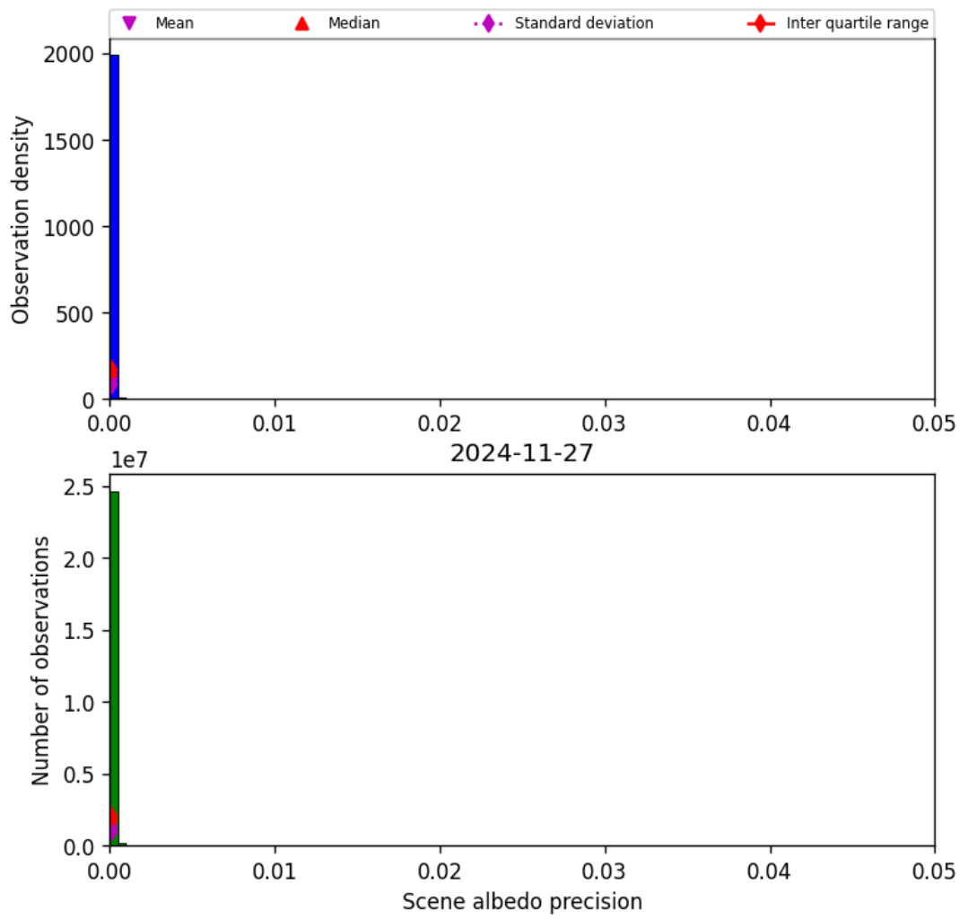
Figure 35: Histogram of “Scene albedo precision” for 2024-11-26 to 2024-11-28
