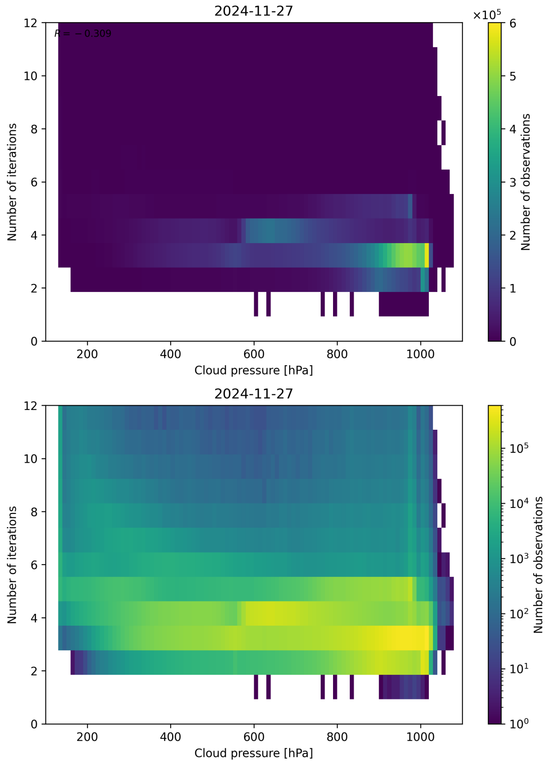
Figure 81: Scatter density plot of “Cloud pressure” against “Number of iterations” for 2024-11-26 to 2024-11-28.
