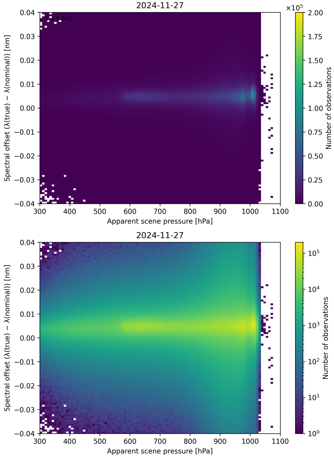
Figure 67: Scatter density plot of “Apparent scene pressure” against “Spectral offset ( \lambda_{\text{true}} - \lambda_{\text{nominal}} )” for 2024-11-26 to 2024-11-28.
