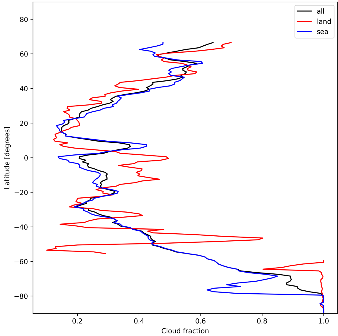
Figure 15: Zonal average of “Cloud fraction” for 2024-11-26 to 2024-11-28.
