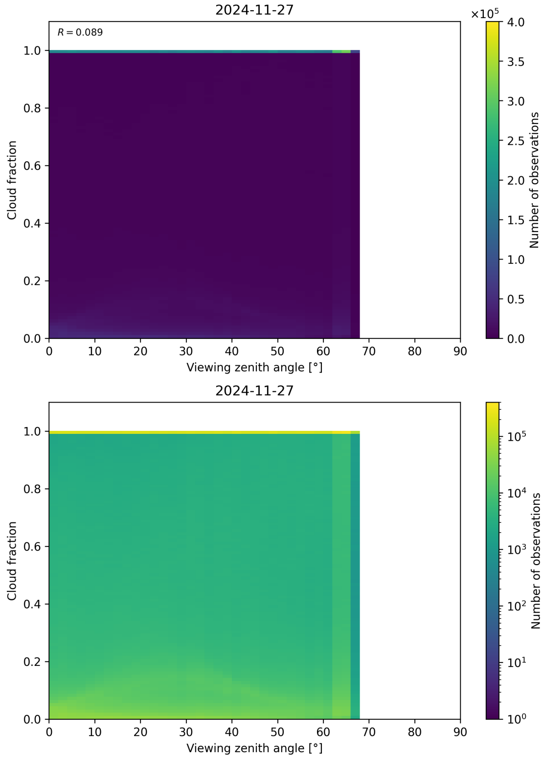
Figure 120: Scatter density plot of “Viewing zenith angle” against “Cloud fraction” for 2024-11-26 to 2024-11-28.
