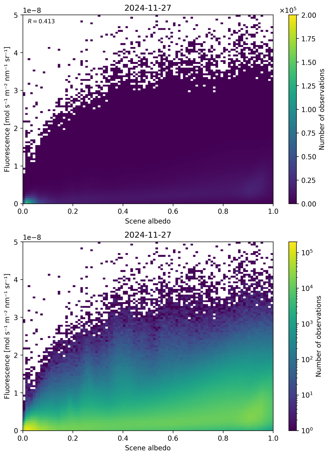
Figure 104: Scatter density plot of “Scene albedo” against “Fluorescence” for 2024-11-26 to 2024-11-28.
