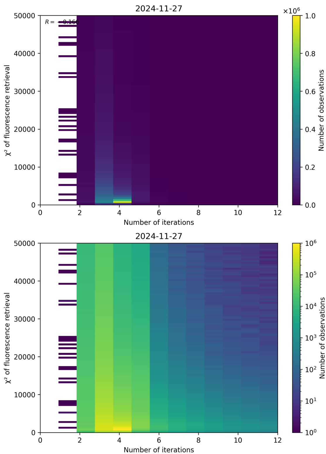
Figure 97: Scatter density plot of “Number of iterations” against “ \chi^2 of fluorescence retrieval” for 2024-11-26 to 2024-11-28.
