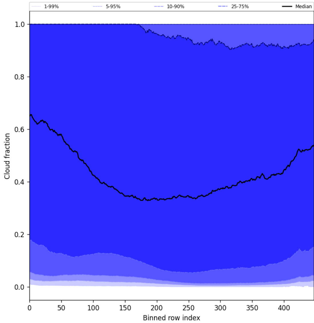
Figure 49: Along track statistics of “Cloud fraction” for 2024-11-26 to 2024-11-28
