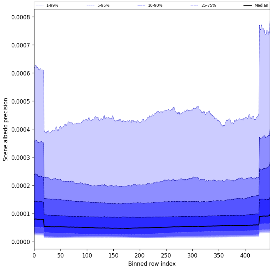
Figure 52: Along track statistics of “Scene albedo precision” for 2024-11-26 to 2024-11-28
