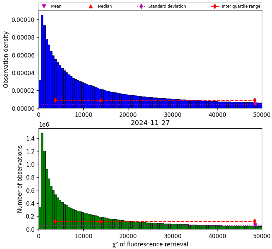
Figure 42: Histogram of “ \chi^2 of fluorescence retrieval” for 2024-11-26 to 2024-11-28
