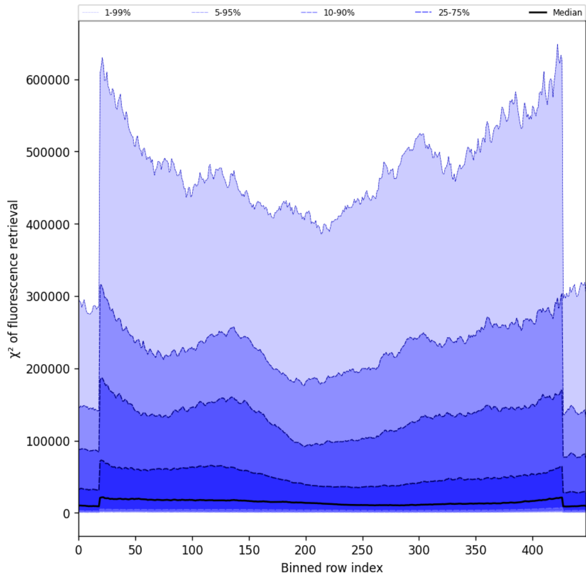
Figure 59: Along track statistics of “ \chi^2 of fluorescence retrieval” for 2024-11-26 to 2024-11-28
