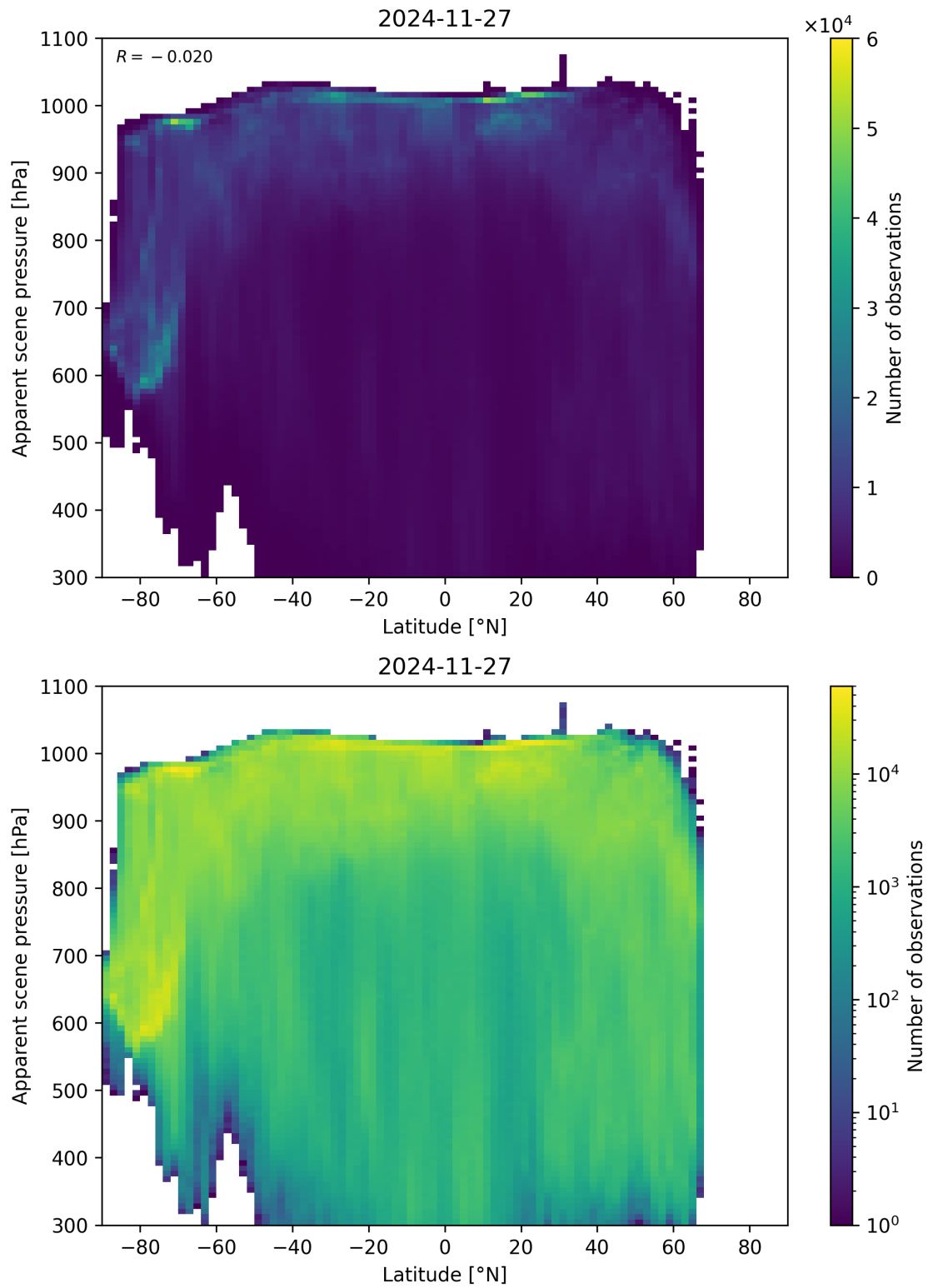
Figure 88: Scatter density plot of “Latitude” against “Apparent scene pressure” for 2024-11-26 to 2024-11-28.
