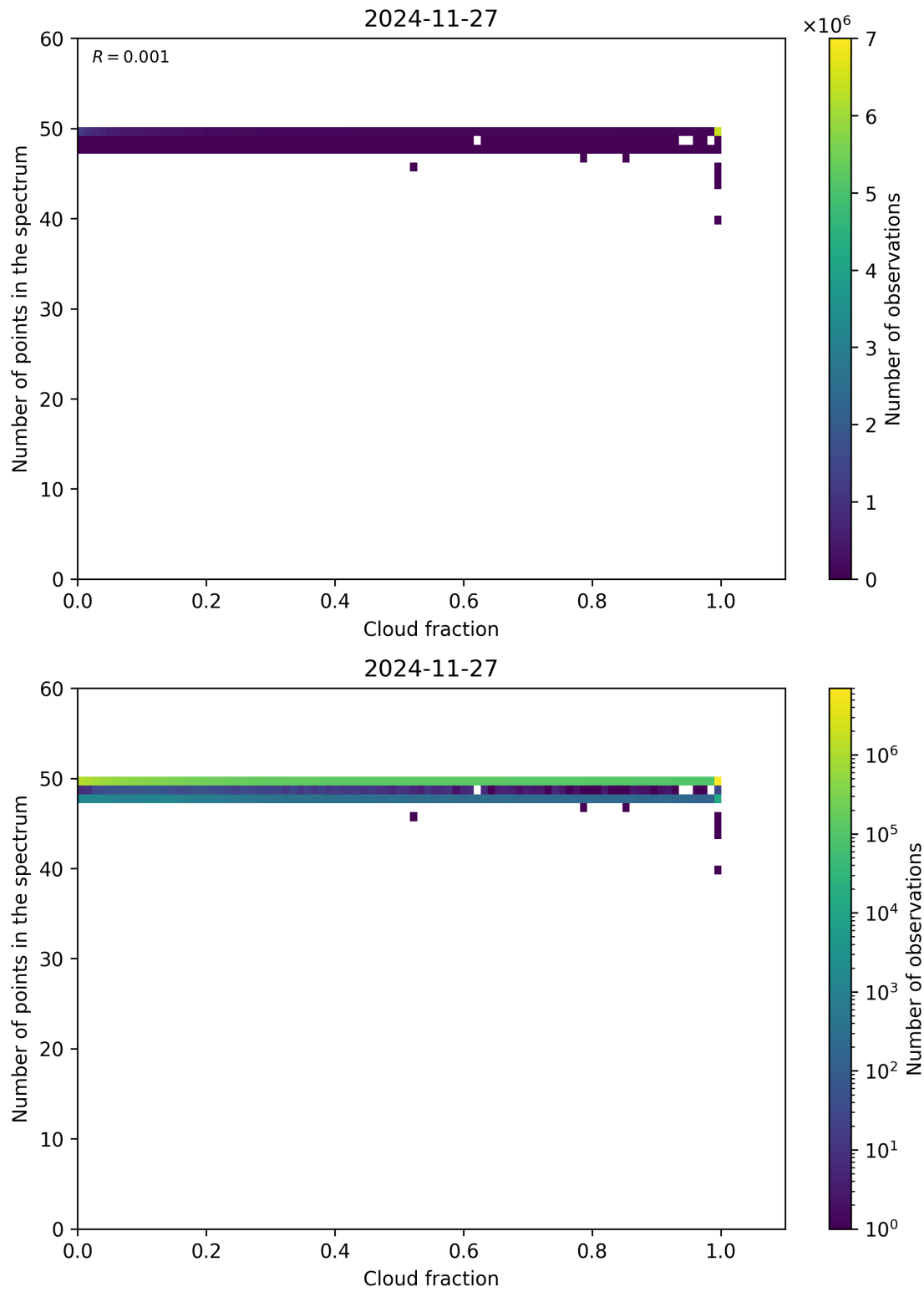
Figure 74: Scatter density plot of “Cloud fraction” against “Number of points in the spectrum” for 2024-11-26 to 2024-11-28.
