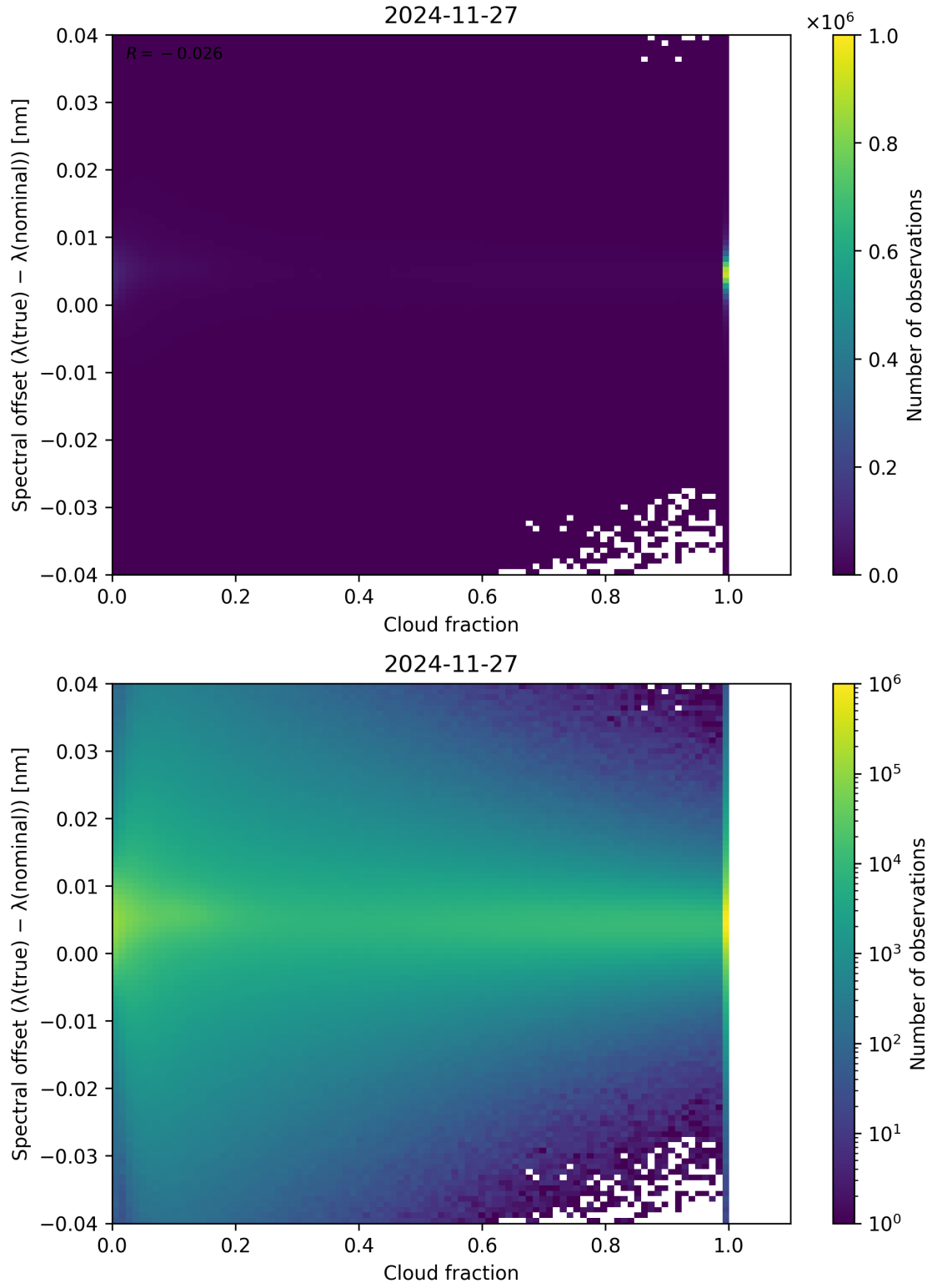
Figure 76: Scatter density plot of “Cloud fraction” against “Spectral offset ( \lambda_{\text{true}} - \lambda_{\text{nominal}} )” for 2024-11-26 to 2024-11-28.
