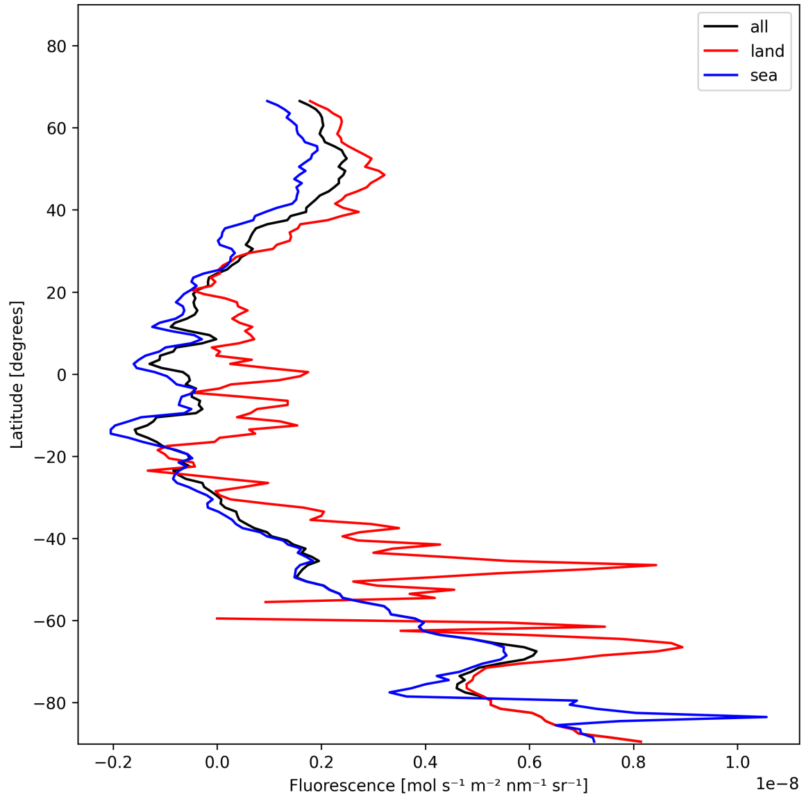
Figure 23: Zonal average of “Fluorescence” for 2024-11-26 to 2024-11-28.
