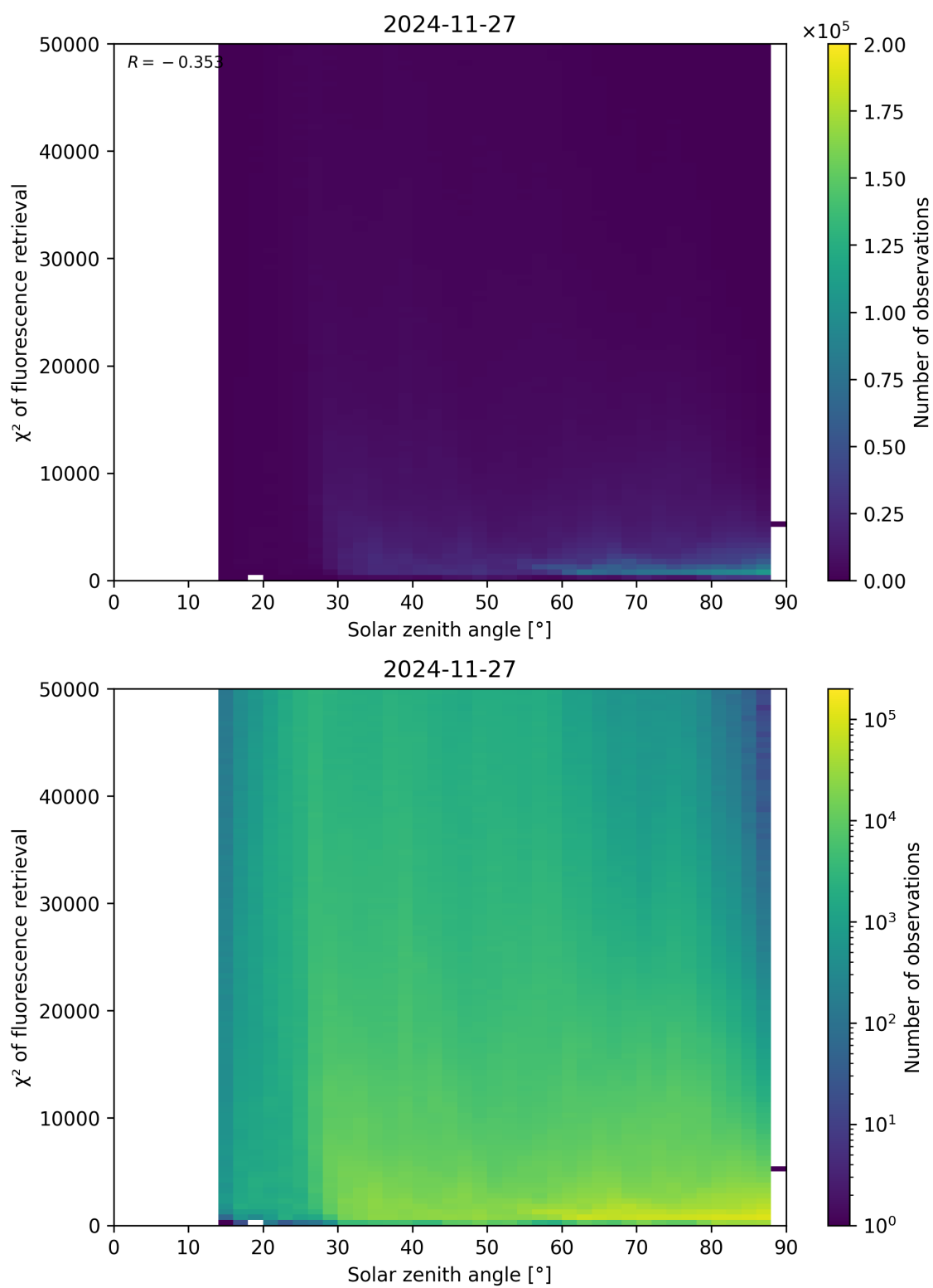
Figure 109: Scatter density plot of “Solar zenith angle” against “ \chi^2 of fluorescence retrieval” for 2024-11-26 to 2024-11-28.
