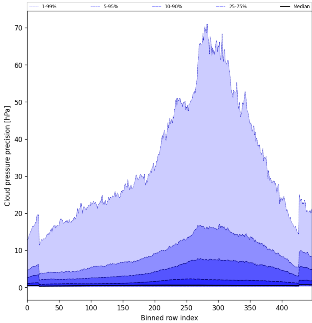
Figure 48: Along track statistics of “Cloud pressure precision” for 2024-11-26 to 2024-11-28
