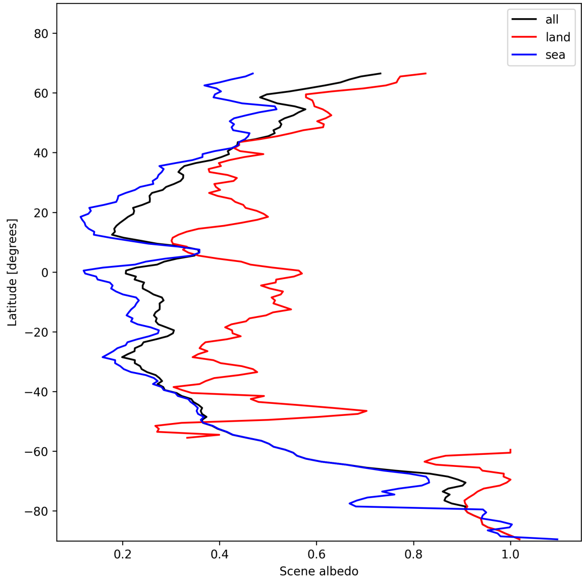
Figure 17: Zonal average of “Scene albedo” for 2024-11-26 to 2024-11-28.
