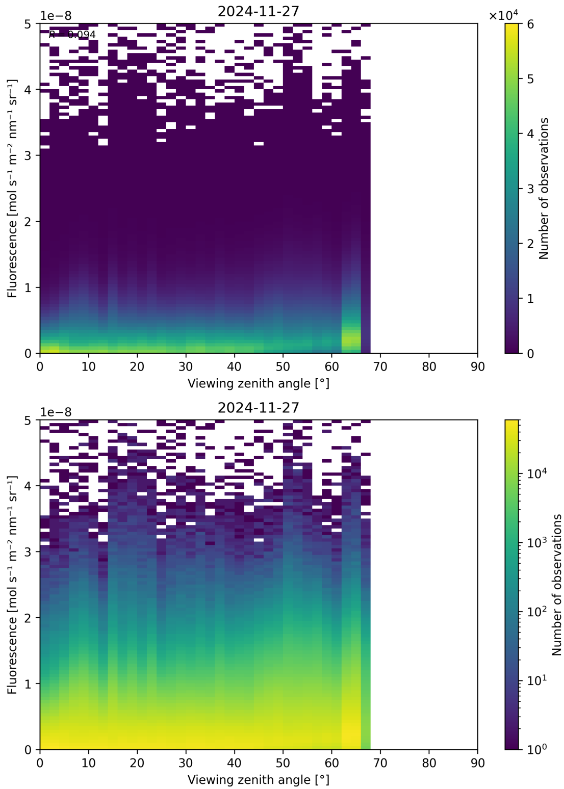
Figure 122: Scatter density plot of “Viewing zenith angle” against “Fluorescence” for 2024-11-26 to 2024-11-28.
