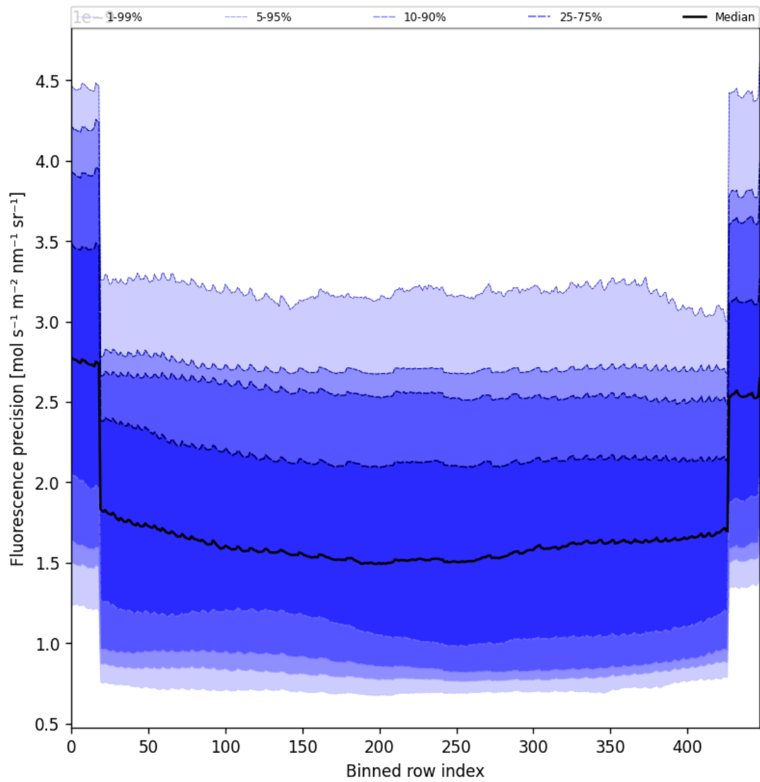
Figure 58: Along track statistics of “Fluorescence precision” for 2024-11-26 to 2024-11-28
