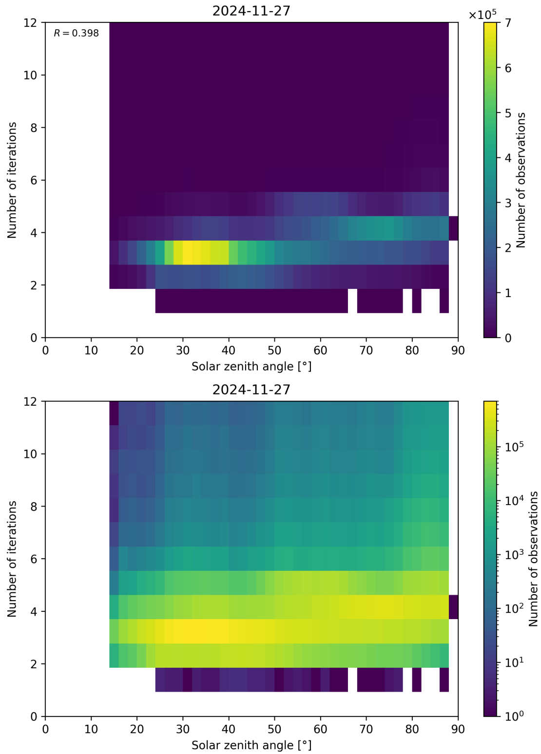
Figure 114: Scatter density plot of “Solar zenith angle” against “Number of iterations” for 2024-11-26 to 2024-11-28.
