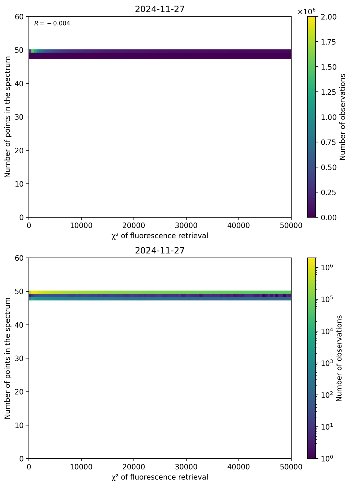
Figure 68: Scatter density plot of " \chi^2 of fluorescence retrieval" against "Number of points in the spectrum" for 2024-11-26 to 2024-11-28.
