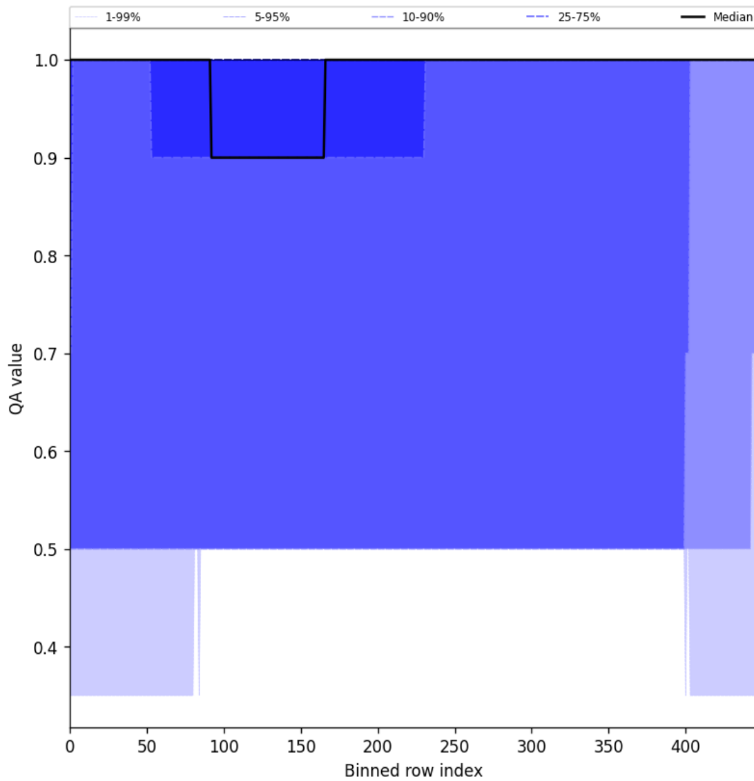
Figure 46: Along track statistics of “QA value” for 2024-11-26 to 2024-11-28
