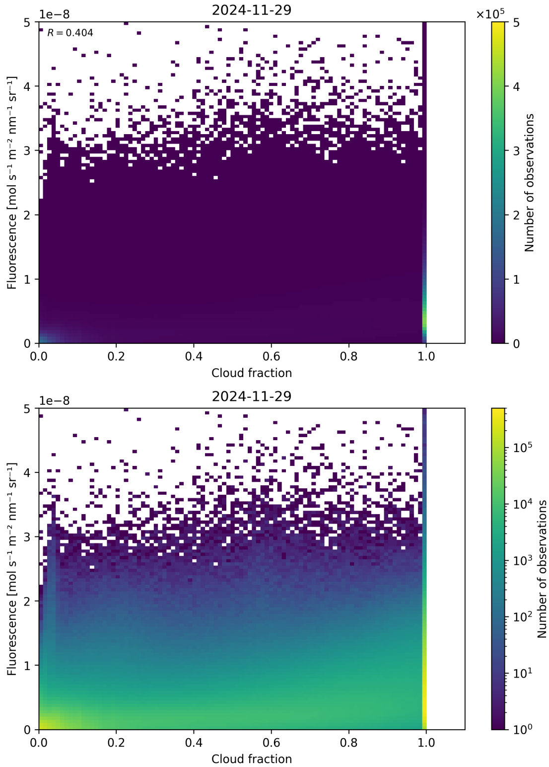
Figure 72: Scatter density plot of “Cloud fraction” against “Fluorescence” for 2024-11-28 to 2024-11-30.
