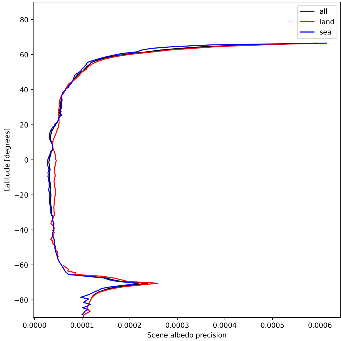
Figure 18: Zonal average of “Scene albedo precision” for 2024-11-28 to 2024-11-30.
