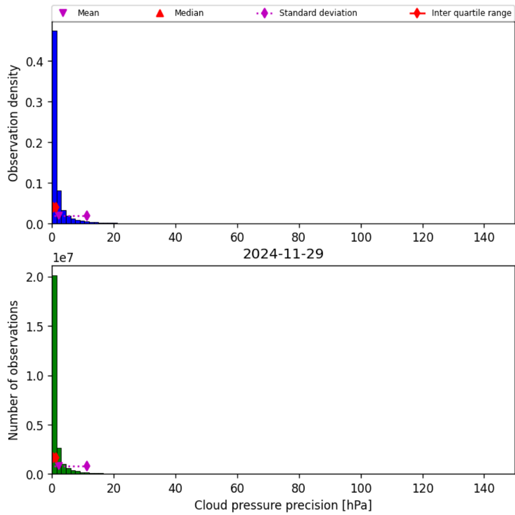
Figure 31: Histogram of “Cloud pressure precision” for 2024-11-28 to 2024-11-30
