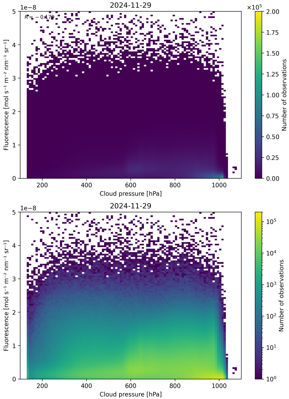
Figure 80: Scatter density plot of “Cloud pressure” against “Fluorescence” for 2024-11-28 to 2024-11-30.
