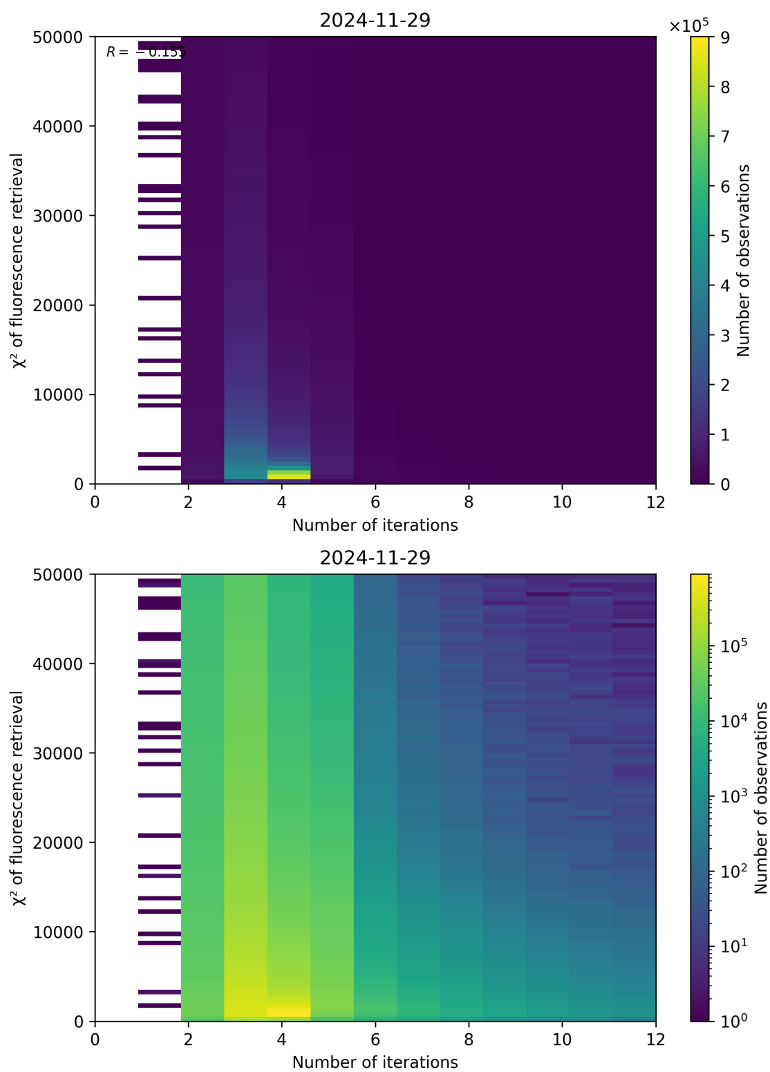
Figure 97: Scatter density plot of “Number of iterations” against “ \chi^2 of fluorescence retrieval” for 2024-11-28 to 2024-11-30.
