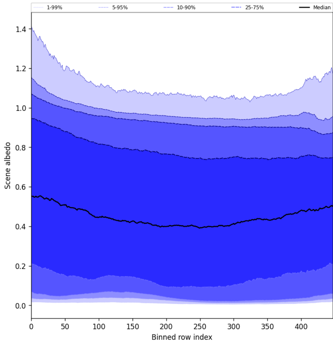
Figure 51: Along track statistics of “Scene albedo” for 2024-11-28 to 2024-11-30
