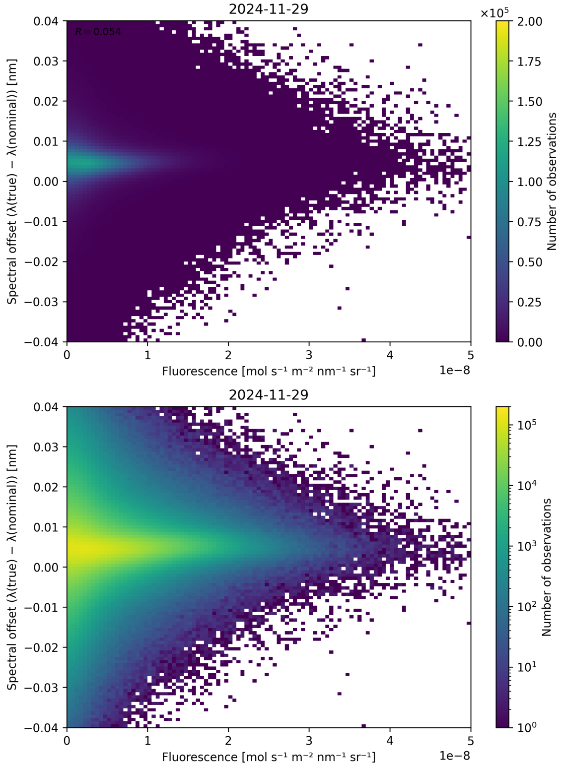
Figure 87: Scatter density plot of “Fluorescence” against “Spectral offset ( \lambda_{\text{true}} - \lambda_{\text{nominal}} )” for 2024-11-28 to 2024-11-30.
