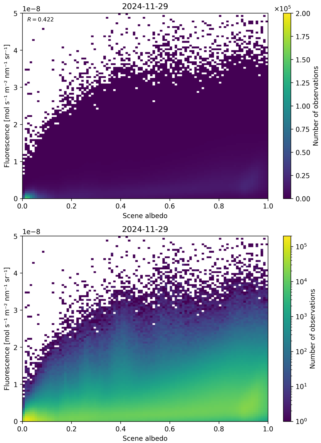
Figure 104: Scatter density plot of “Scene albedo” against “Fluorescence” for 2024-11-28 to 2024-11-30.
