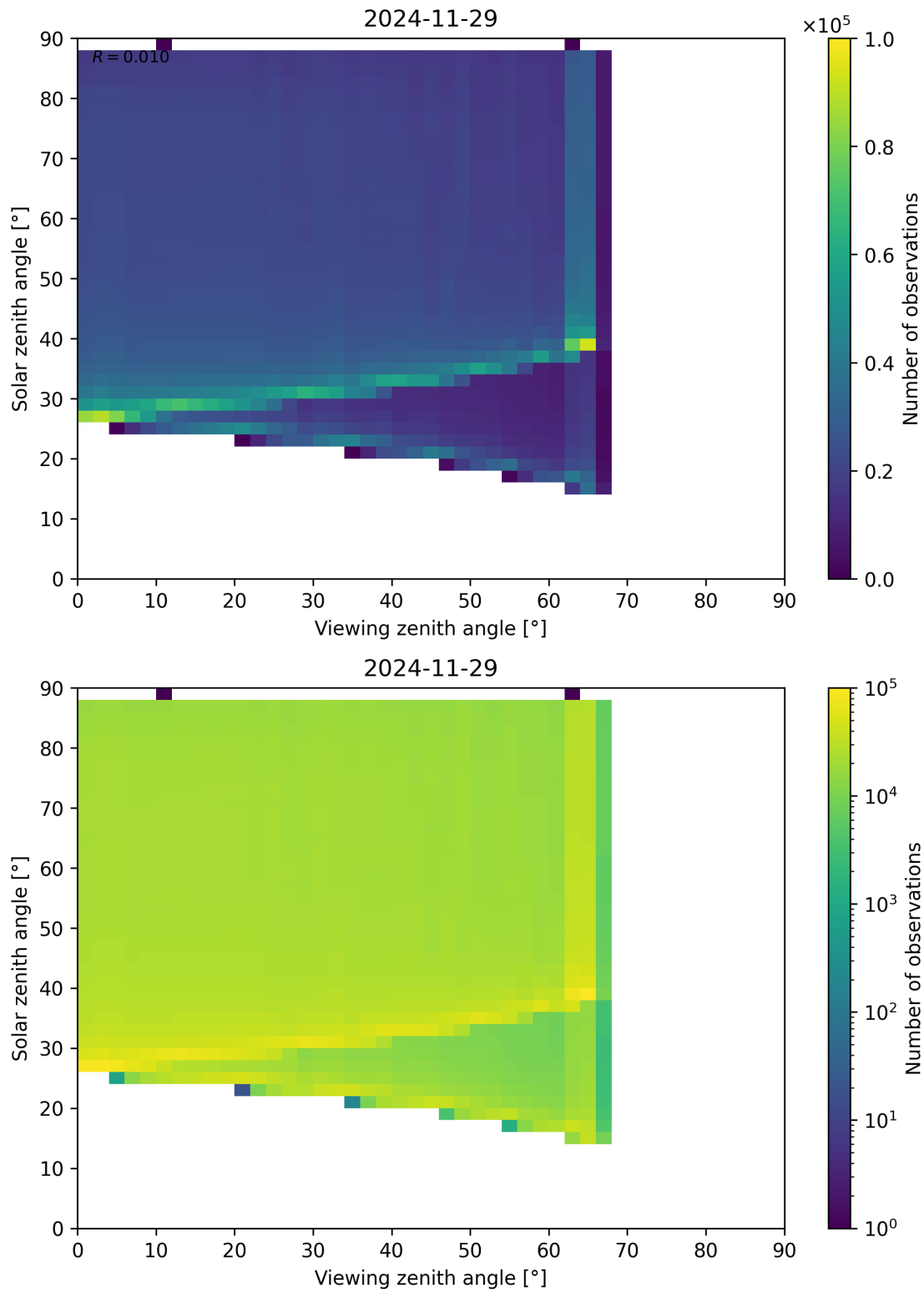
Figure 127: Scatter density plot of “Viewing zenith angle” against “Solar zenith angle” for 2024-11-28 to 2024-11-30.
