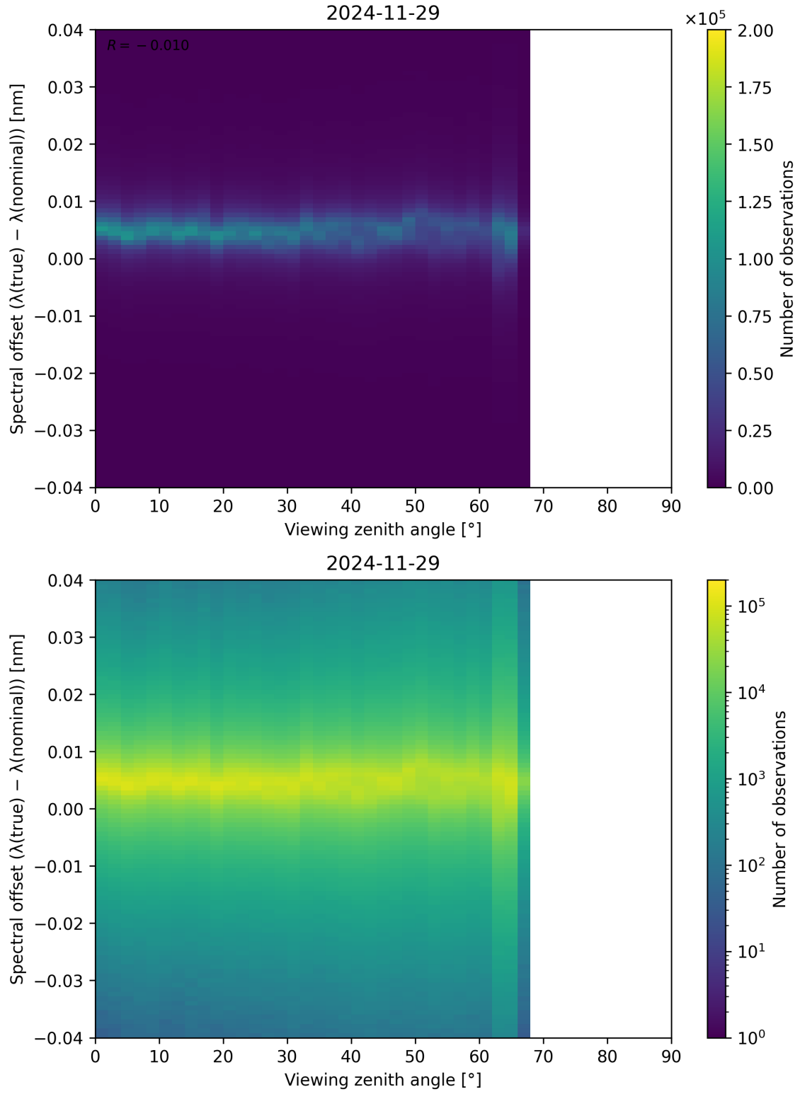
Figure 128: Scatter density plot of “Viewing zenith angle” against “Spectral offset ( \lambda_{\text{true}} - \lambda_{\text{nominal}} )” for 2024-11-28 to 2024-11-30.
