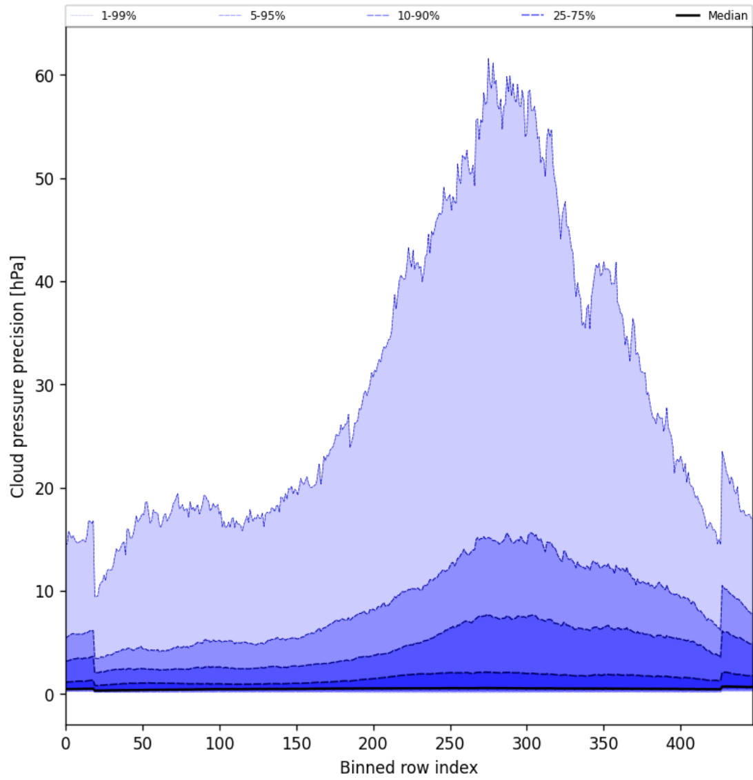
Figure 48: Along track statistics of “Cloud pressure precision” for 2024-11-28 to 2024-11-30
