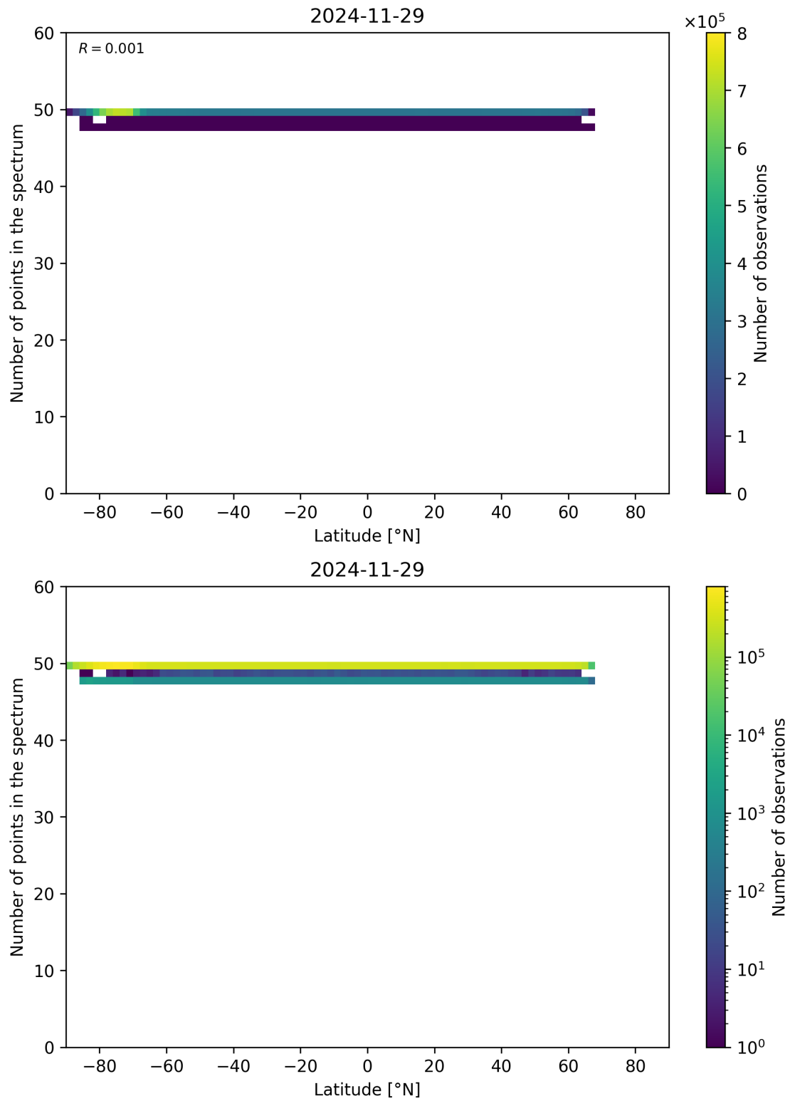
Figure 94: Scatter density plot of “Latitude” against “Number of points in the spectrum” for 2024-11-28 to 2024-11-30.
