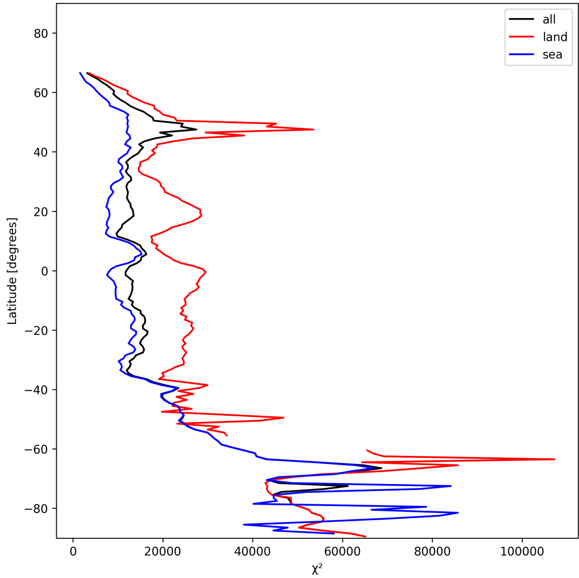
Figure 21: Zonal average of “ \chi^2 ” for 2024-11-28 to 2024-11-30.
