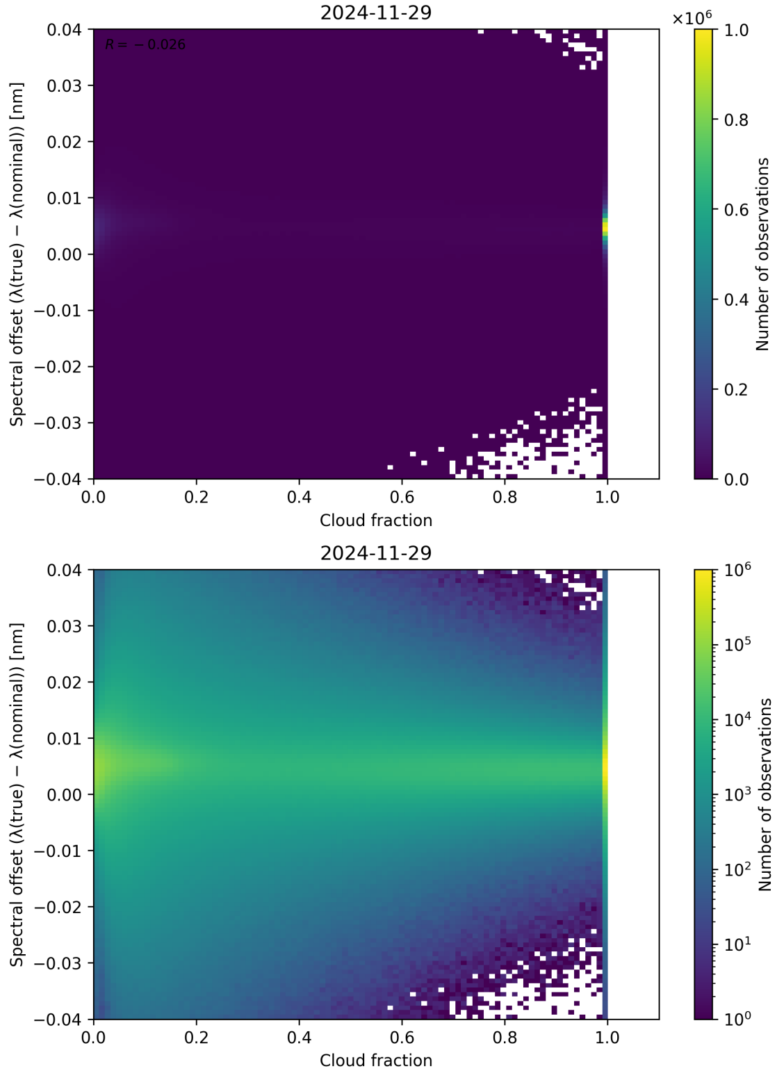
Figure 76: Scatter density plot of “Cloud fraction” against “Spectral offset ( \lambda_{\text{true}} - \lambda_{\text{nominal}} )” for 2024-11-28 to 2024-11-30.
