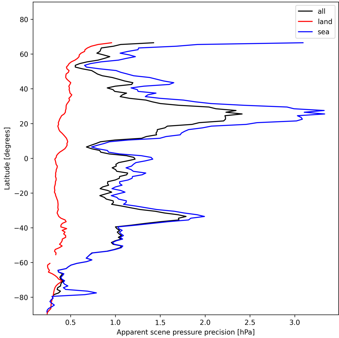
Figure 20: Zonal average of “Apparent scene pressure precision” for 2024-11-28 to 2024-11-30.
