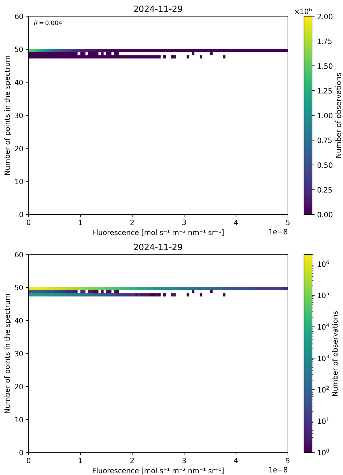
Figure 86: Scatter density plot of “Fluorescence” against “Number of points in the spectrum” for 2024-11-28 to 2024-11-30.
