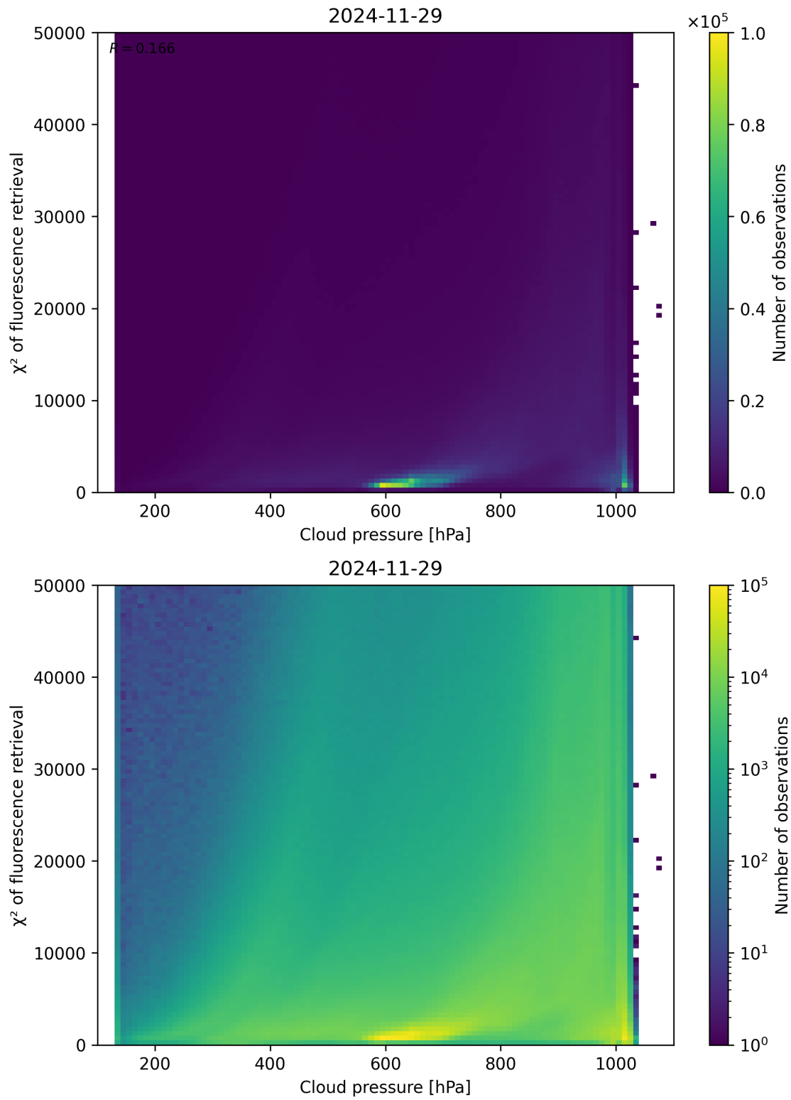
Figure 78: Scatter density plot of “Cloud pressure” against “ \chi^2 of fluorescence retrieval” for 2024-11-28 to 2024-11-30.
