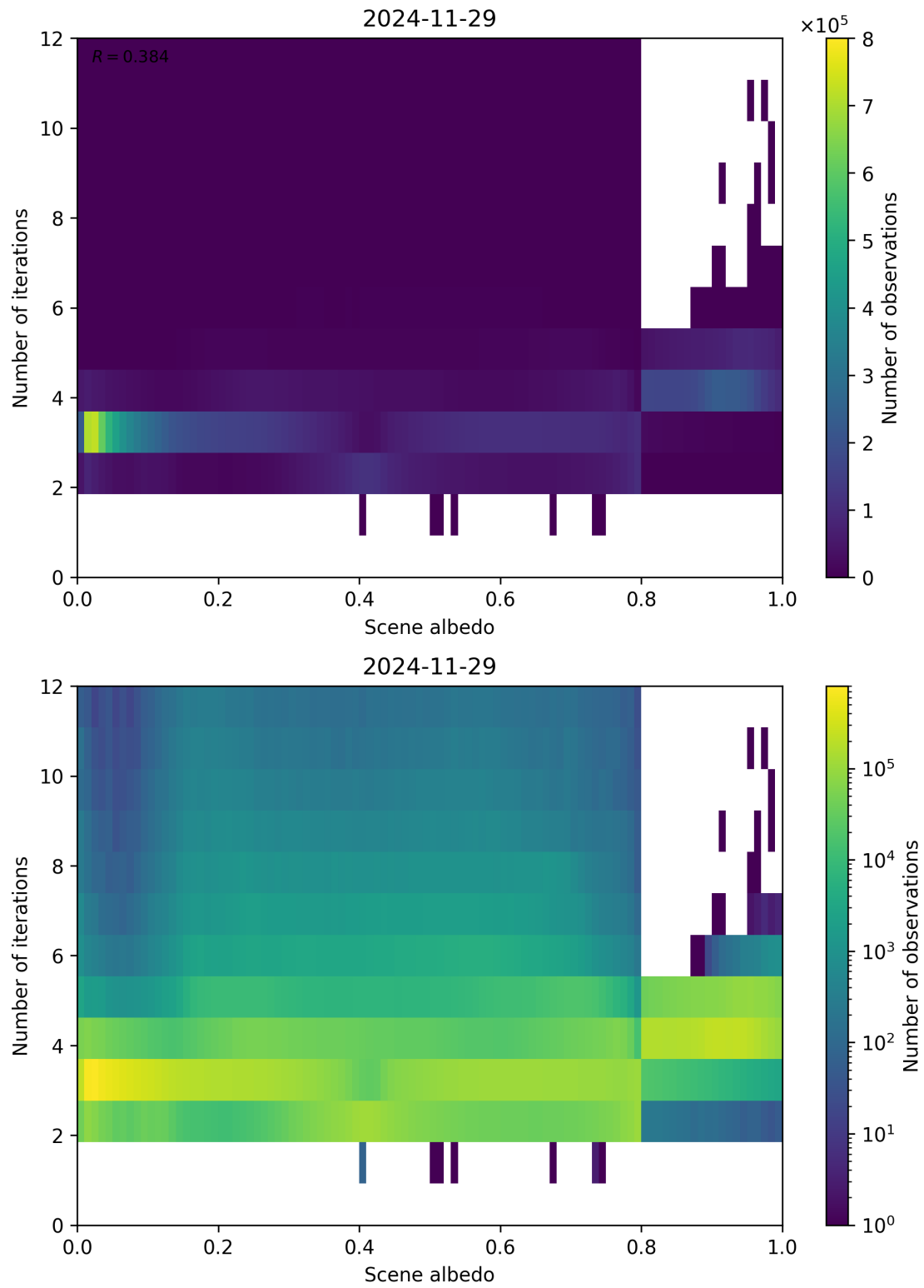
Figure 105: Scatter density plot of “Scene albedo” against “Number of iterations” for 2024-11-28 to 2024-11-30.
