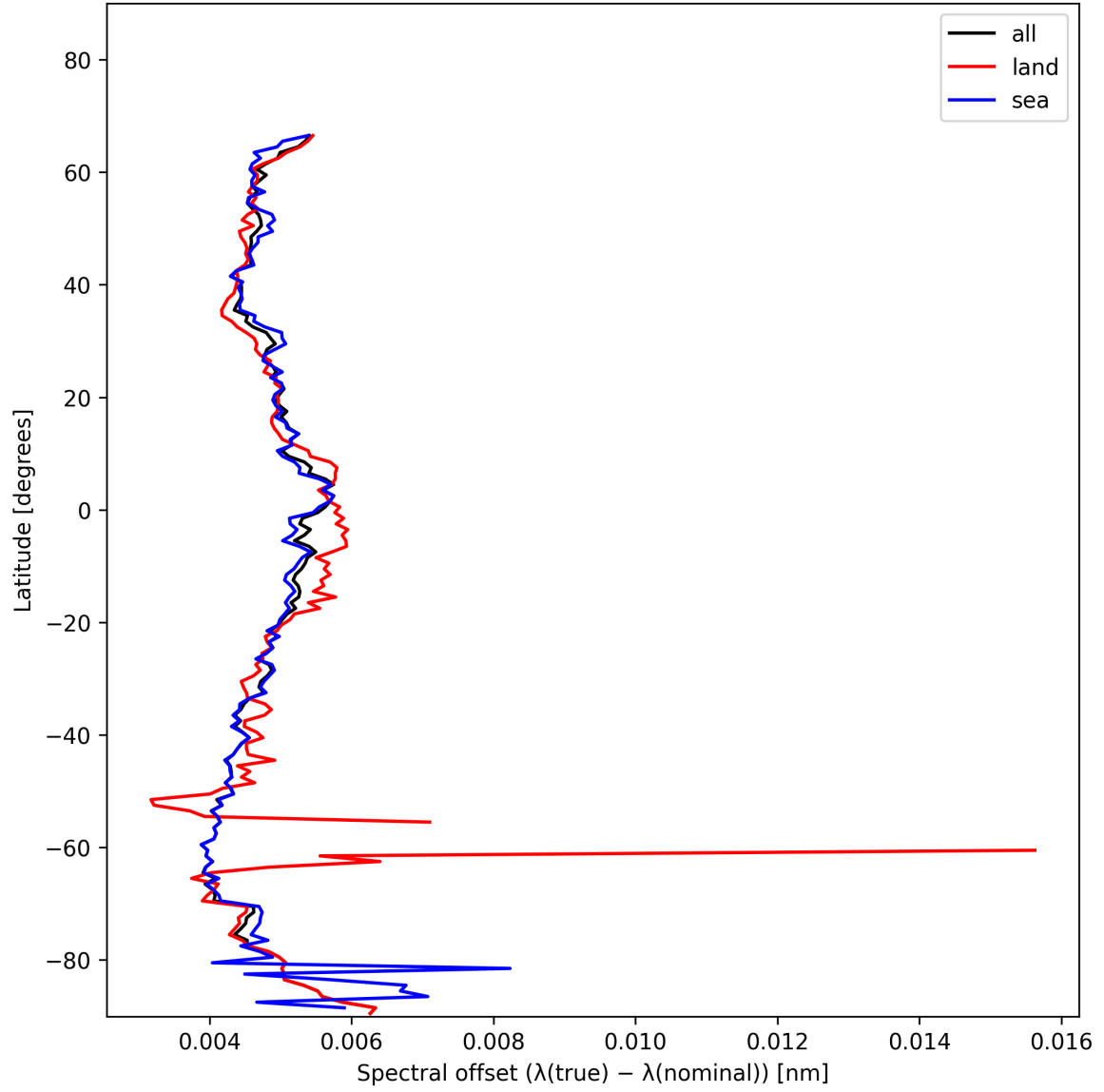
Figure 28: Zonal average of “Spectral offset ( \lambda_{\text{true}} - \lambda_{\text{nominal}} )” for 2024-11-28 to 2024-11-30.
