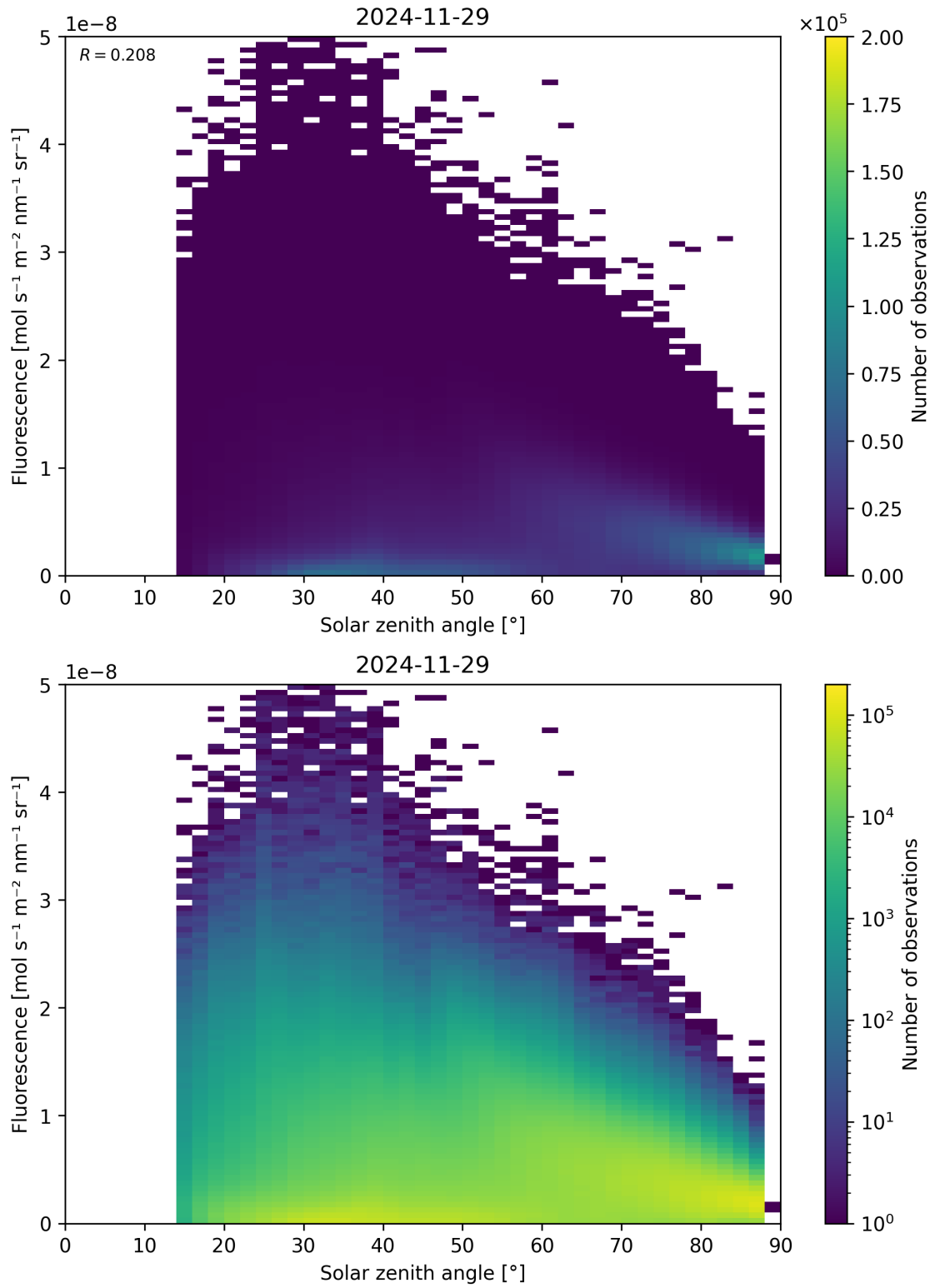
Figure 112: Scatter density plot of “Solar zenith angle” against “Fluorescence” for 2024-11-28 to 2024-11-30.
