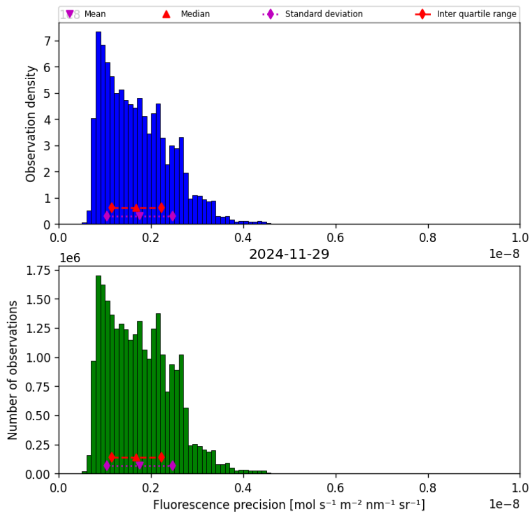
Figure 41: Histogram of “Fluorescence precision” for 2024-11-28 to 2024-11-30
