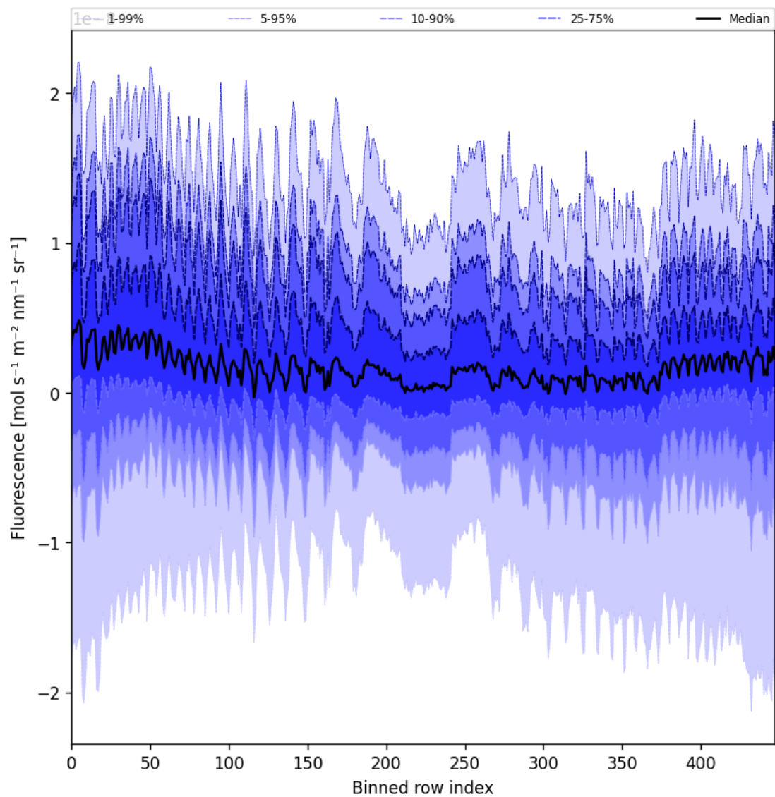
Figure 57: Along track statistics of “Fluorescence” for 2024-11-28 to 2024-11-30
