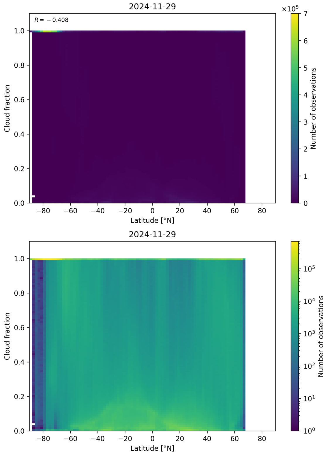
Figure 90: Scatter density plot of “Latitude” against “Cloud fraction” for 2024-11-28 to 2024-11-30.
