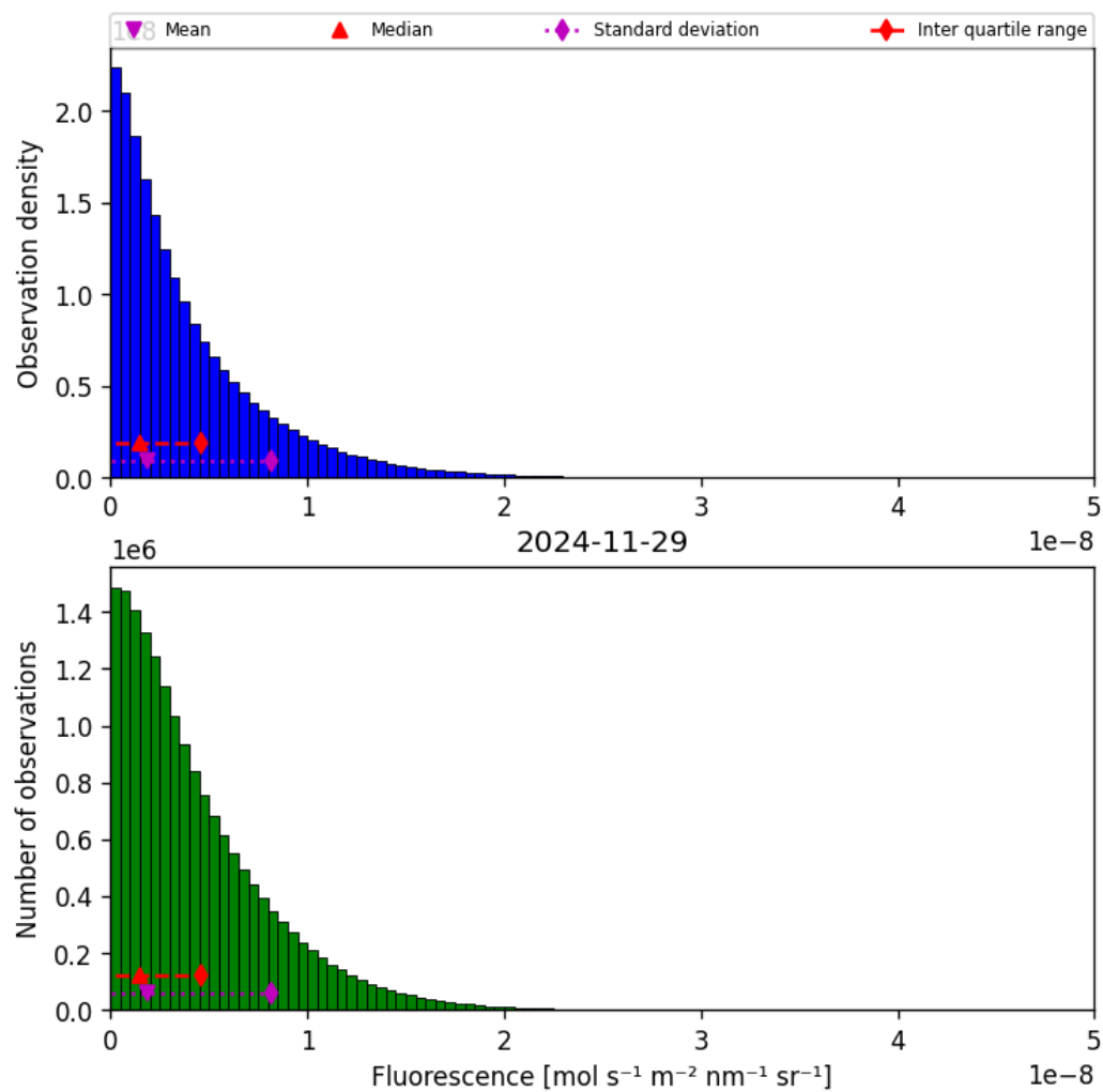
Figure 40: Histogram of “Fluorescence” for 2024-11-28 to 2024-11-30
