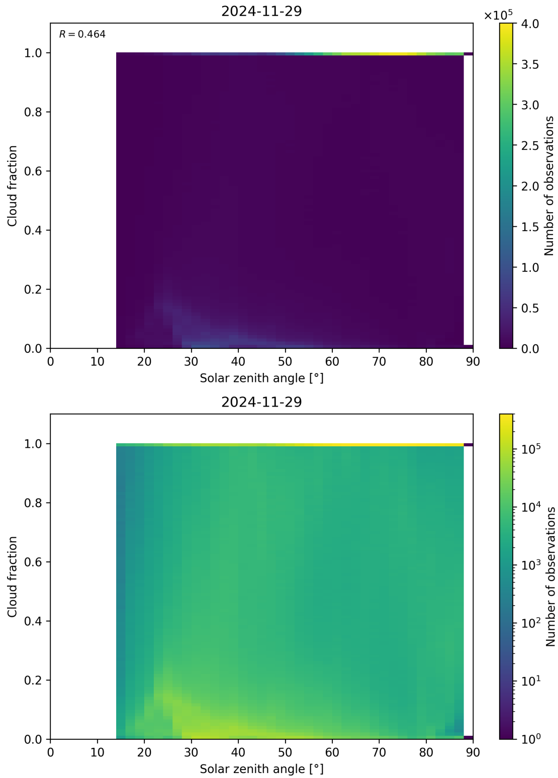
Figure 110: Scatter density plot of “Solar zenith angle” against “Cloud fraction” for 2024-11-28 to 2024-11-30.
