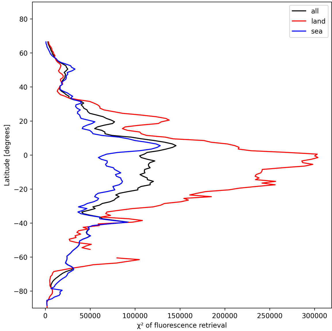
Figure 25: Zonal average of “ \chi^2 of fluorescence retrieval” for 2024-11-28 to 2024-11-30.
