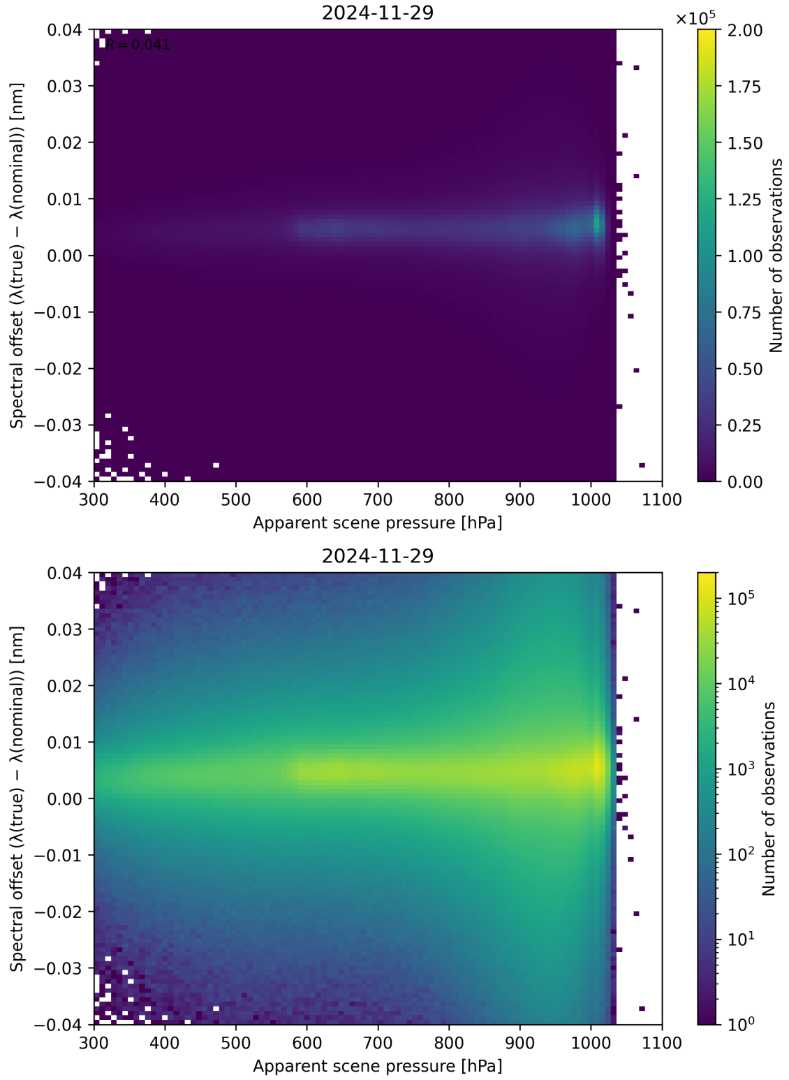
Figure 67: Scatter density plot of “Apparent scene pressure” against “Spectral offset ( \lambda_{\text{true}} - \lambda_{\text{nominal}} )” for 2024-11-28 to 2024-11-30.
