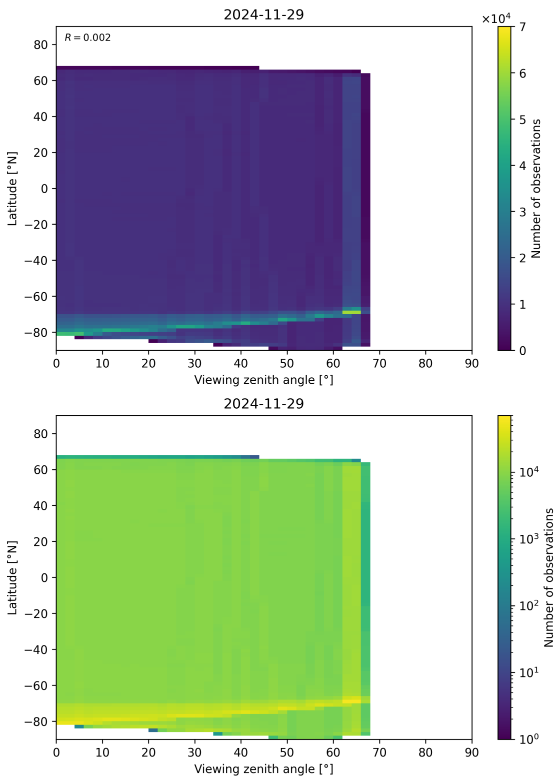
Figure 123: Scatter density plot of “Viewing zenith angle” against “Latitude” for 2024-11-28 to 2024-11-30.
