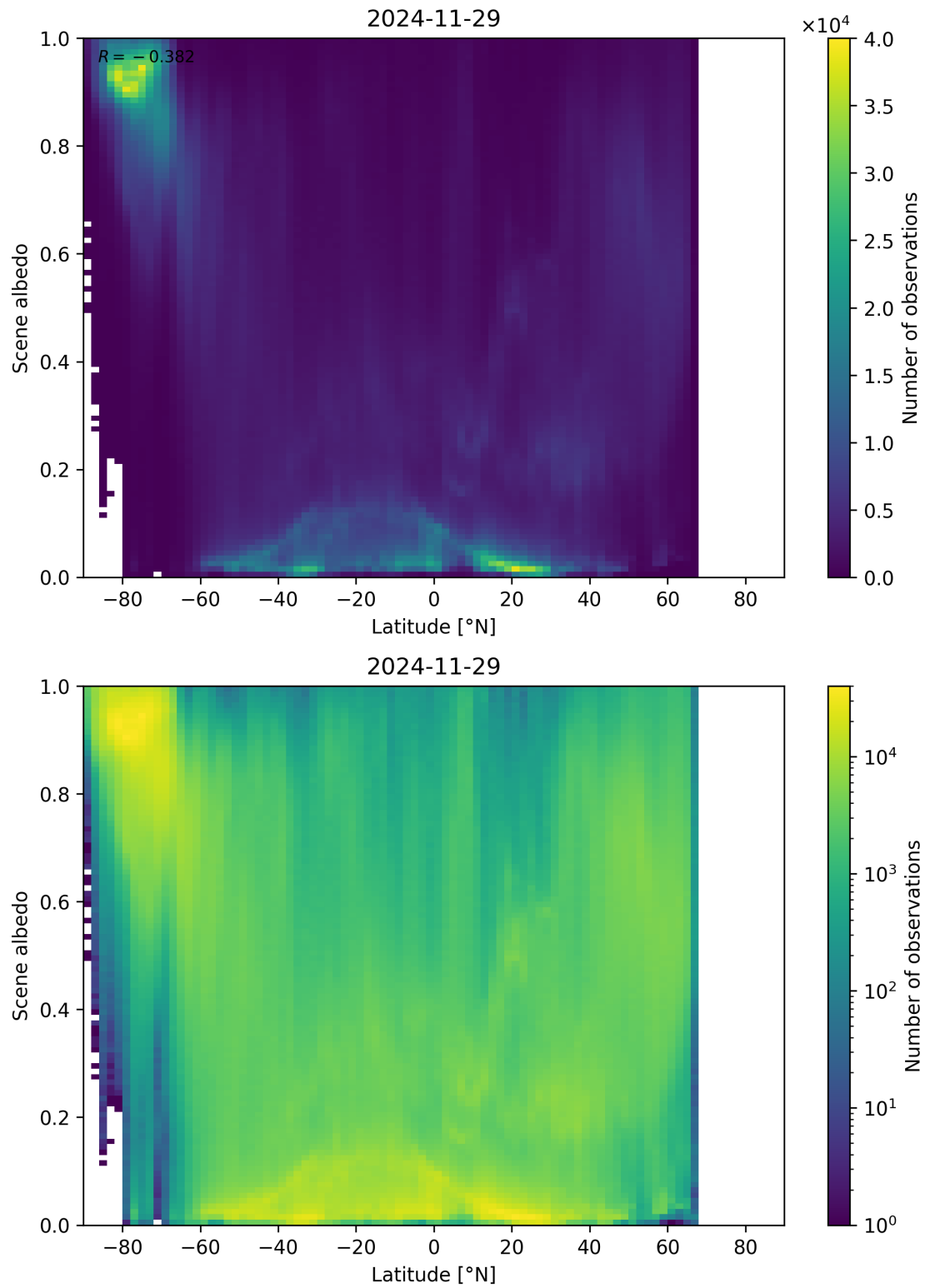
Figure 95: Scatter density plot of “Latitude” against “Scene albedo” for 2024-11-28 to 2024-11-30.
