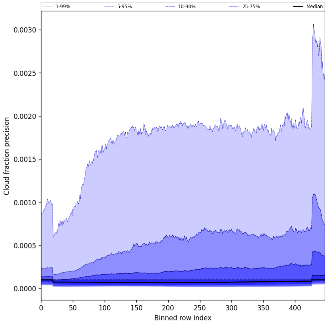
Figure 50: Along track statistics of “Cloud fraction precision” for 2024-11-28 to 2024-11-30
