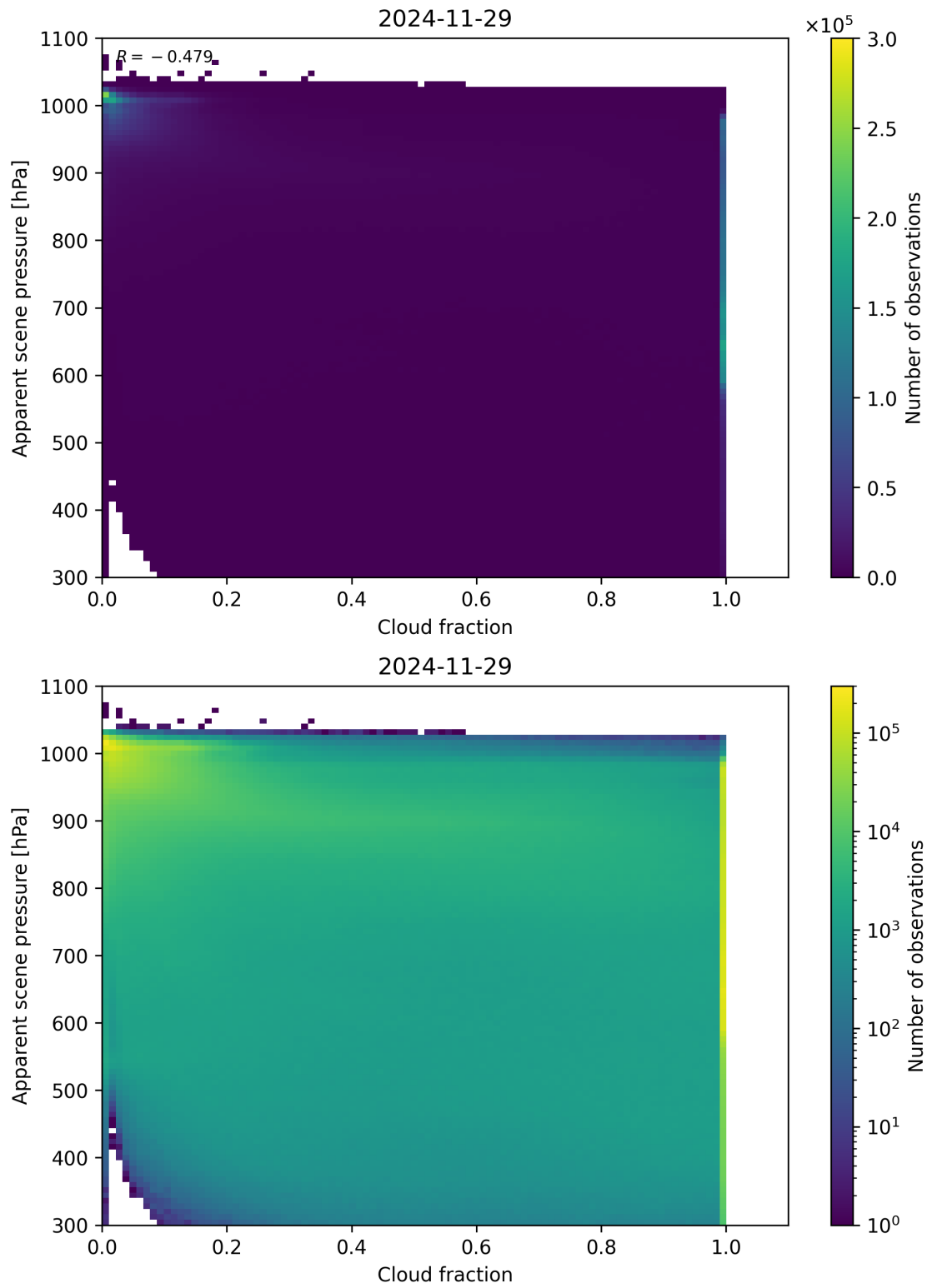
Figure 70: Scatter density plot of “Cloud fraction” against “Apparent scene pressure” for 2024-11-28 to 2024-11-30.
