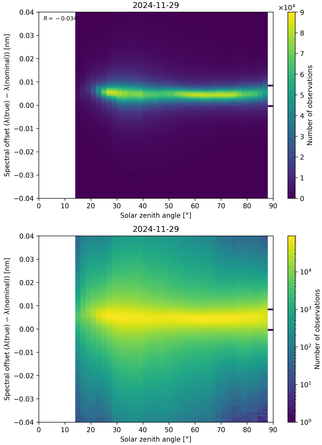
Figure 117: Scatter density plot of “Solar zenith angle” against “Spectral offset ( \lambda_{\text{true}} - \lambda_{\text{nominal}} )” for 2024-11-28 to 2024-11-30.
