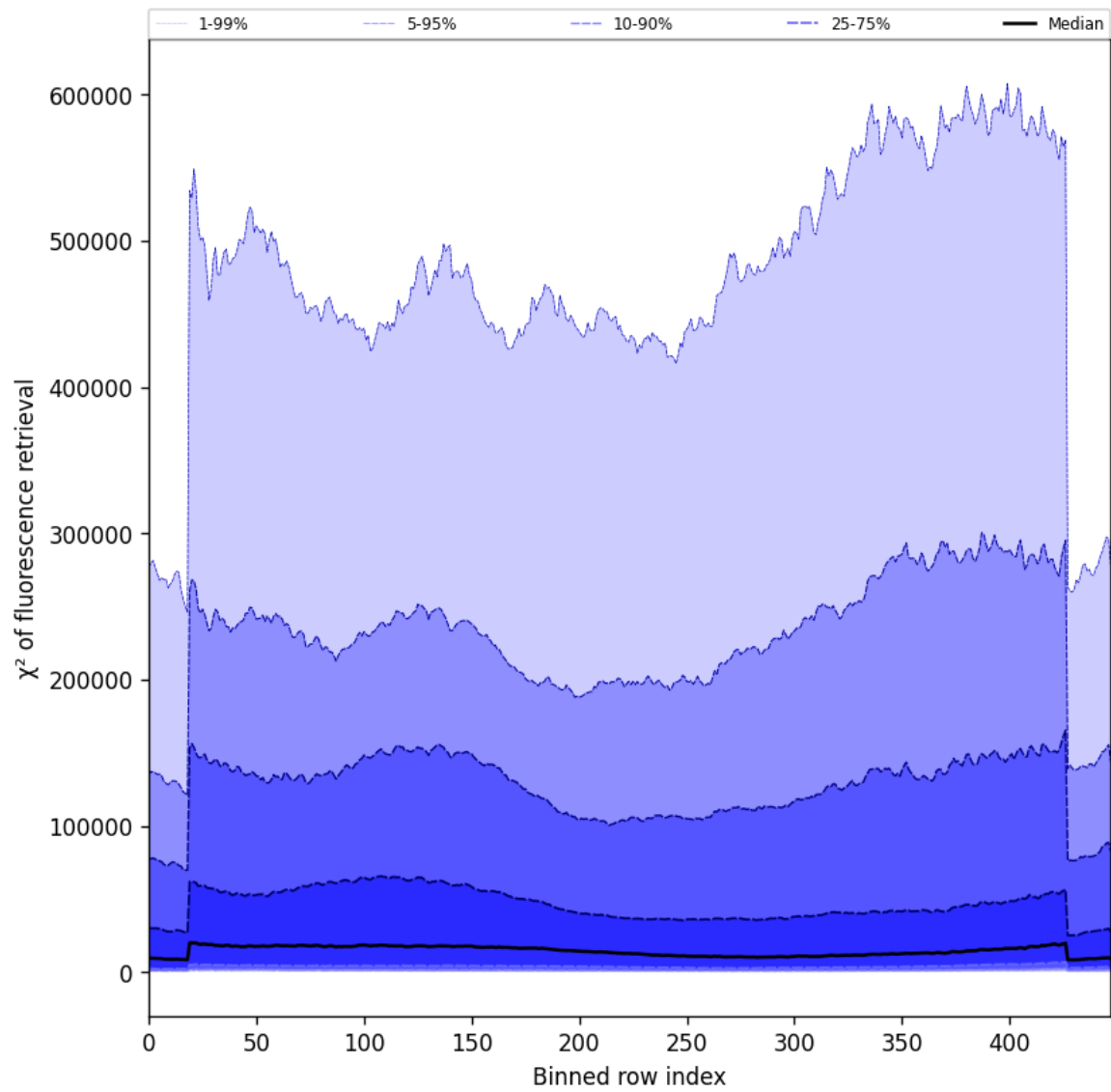
Figure 59: Along track statistics of “ \chi^2 of fluorescence retrieval” for 2024-11-28 to 2024-11-30
