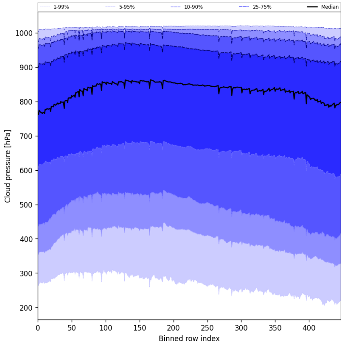
Figure 47: Along track statistics of “Cloud pressure” for 2024-11-28 to 2024-11-30
