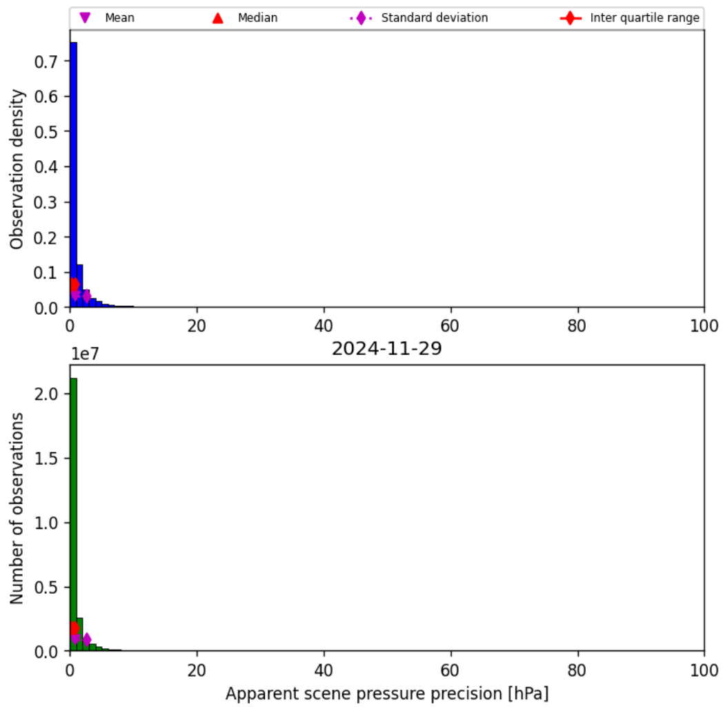
Figure 37: Histogram of “Apparent scene pressure precision” for 2024-11-28 to 2024-11-30
