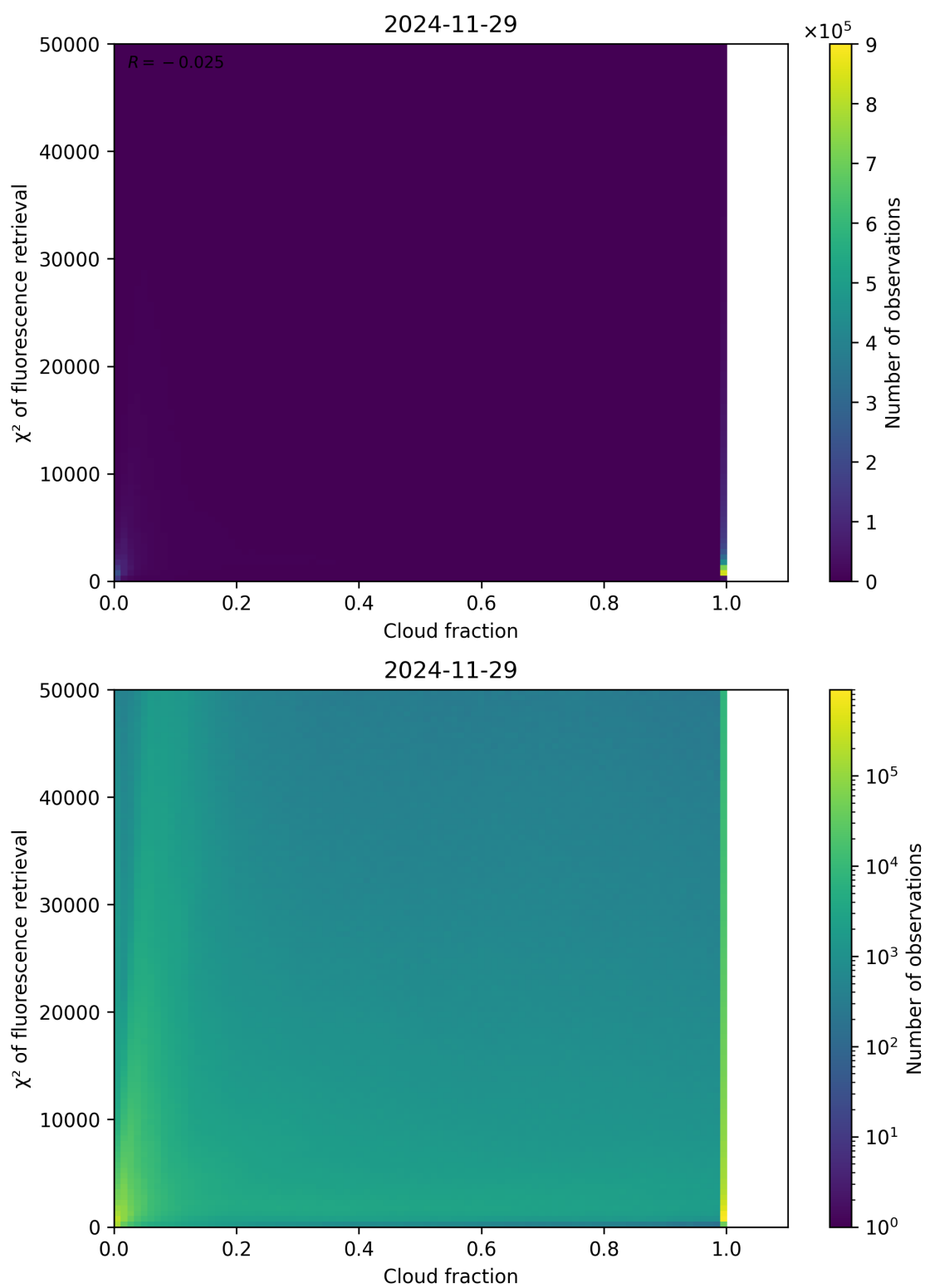
Figure 71: Scatter density plot of “Cloud fraction” against “ \chi^2 of fluorescence retrieval” for 2024-11-28 to 2024-11-30.
