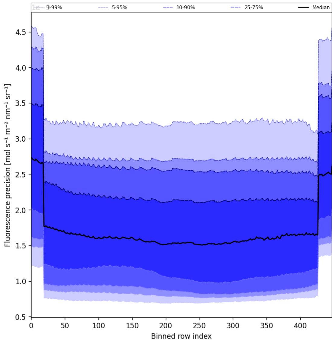
Figure 58: Along track statistics of “Fluorescence precision” for 2024-11-28 to 2024-11-30
