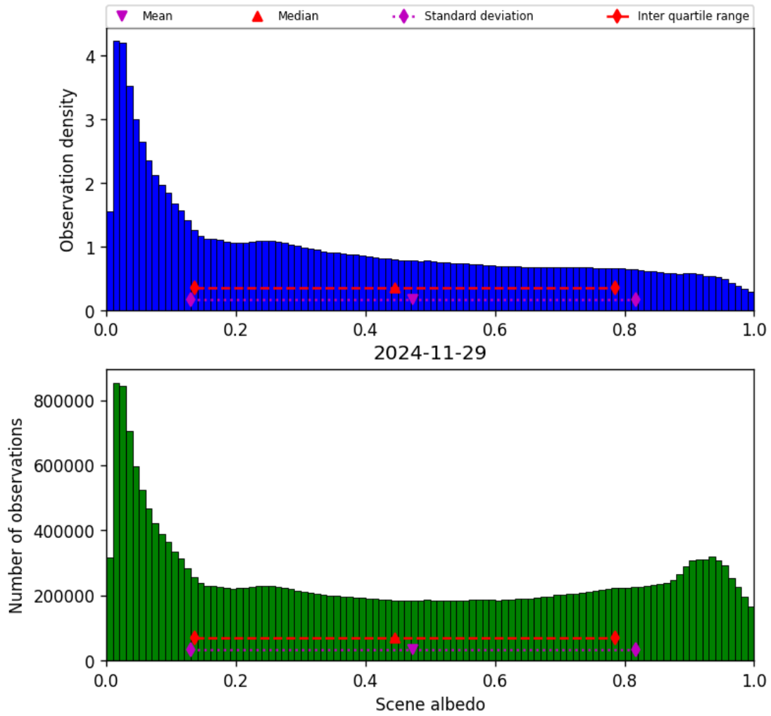
Figure 34: Histogram of “Scene albedo” for 2024-11-28 to 2024-11-30
