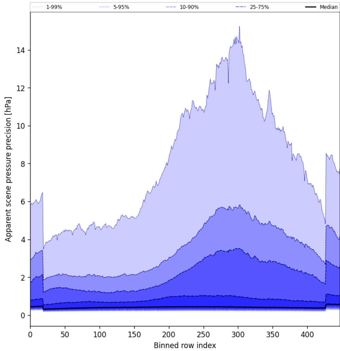
Figure 54: Along track statistics of “Apparent scene pressure precision” for 2024-11-28 to 2024-11-30
