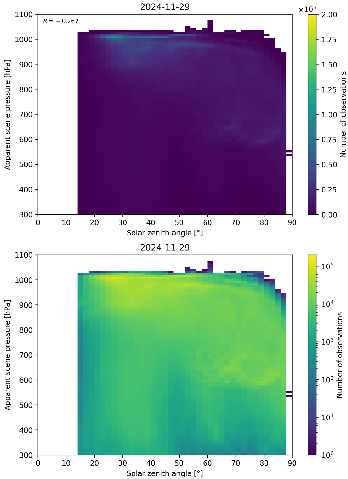
Figure 108: Scatter density plot of “Solar zenith angle” against “Apparent scene pressure” for 2024-11-28 to 2024-11-30.
