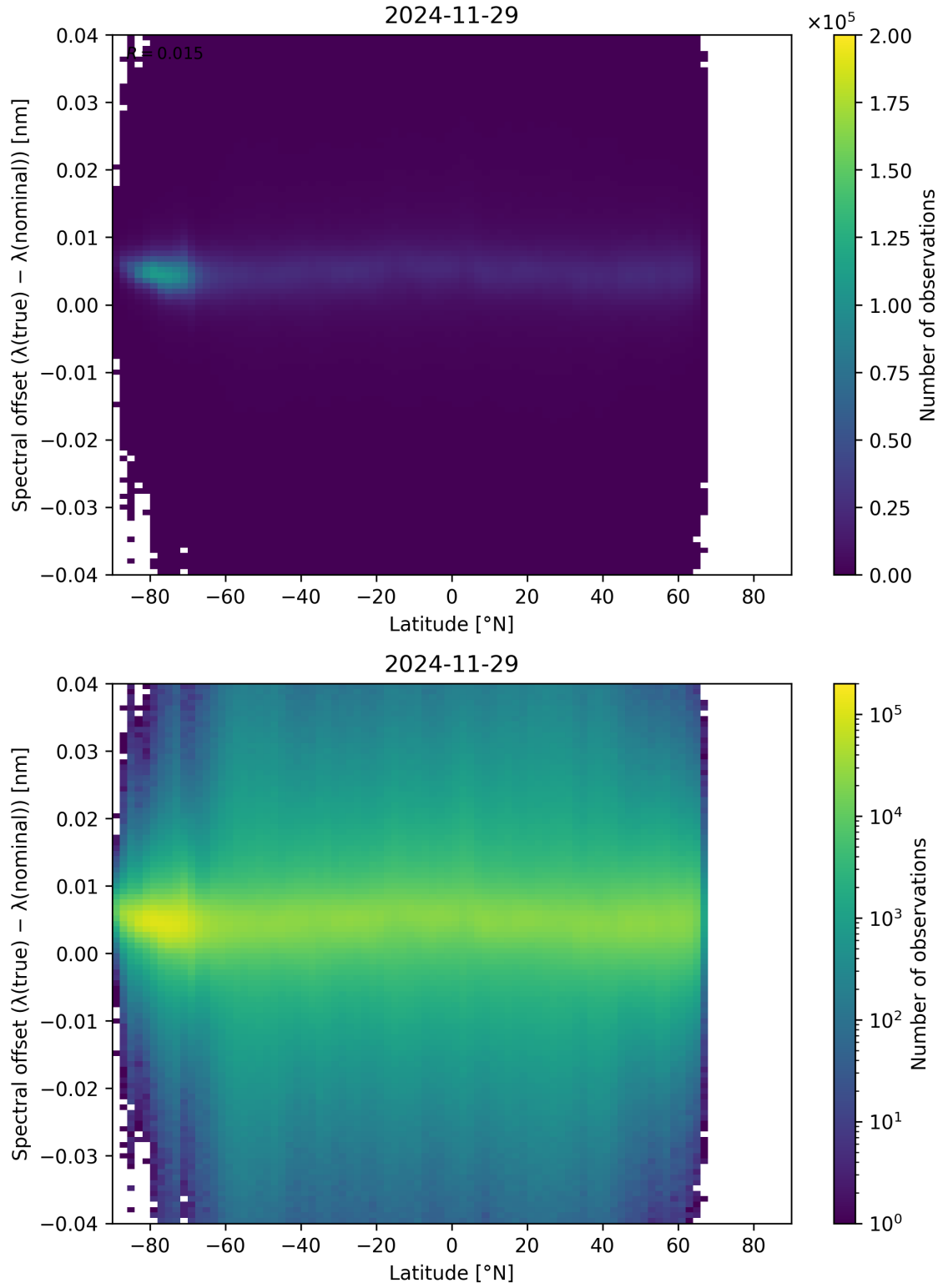
Figure 96: Scatter density plot of “Latitude” against “Spectral offset ( \lambda_{\text{true}} - \lambda_{\text{nominal}} )” for 2024-11-28 to 2024-11-30.
