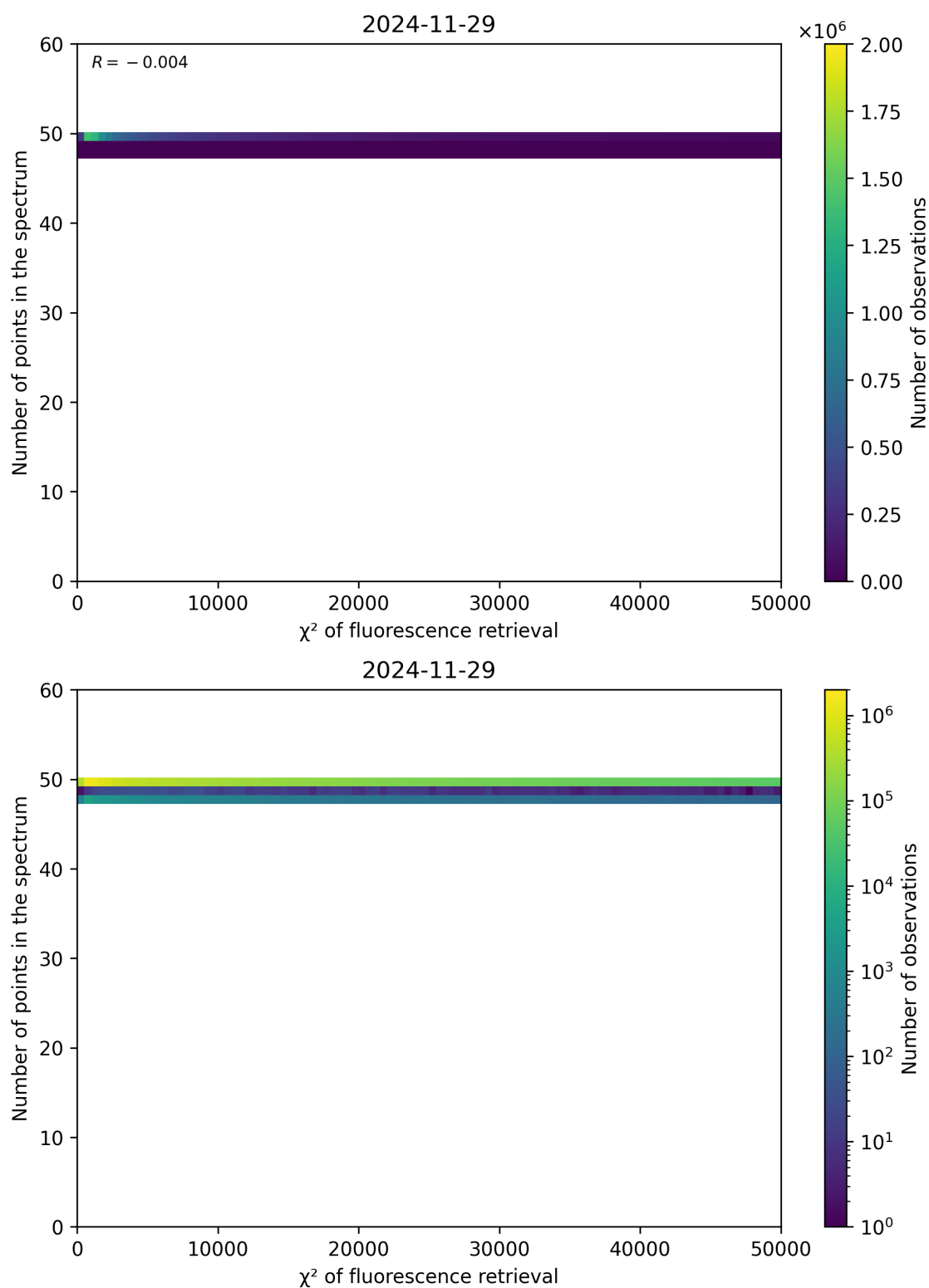
Figure 68: Scatter density plot of “ \chi^2 of fluorescence retrieval” against “Number of points in the spectrum” for 2024-11-28 to 2024-11-30.
