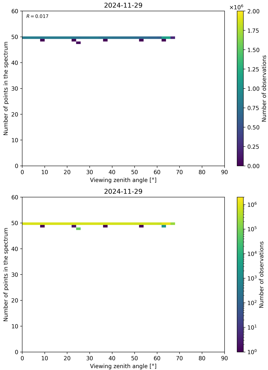
Figure 125: Scatter density plot of “Viewing zenith angle” against “Number of points in the spectrum” for 2024-11-28 to 2024-11-30.
