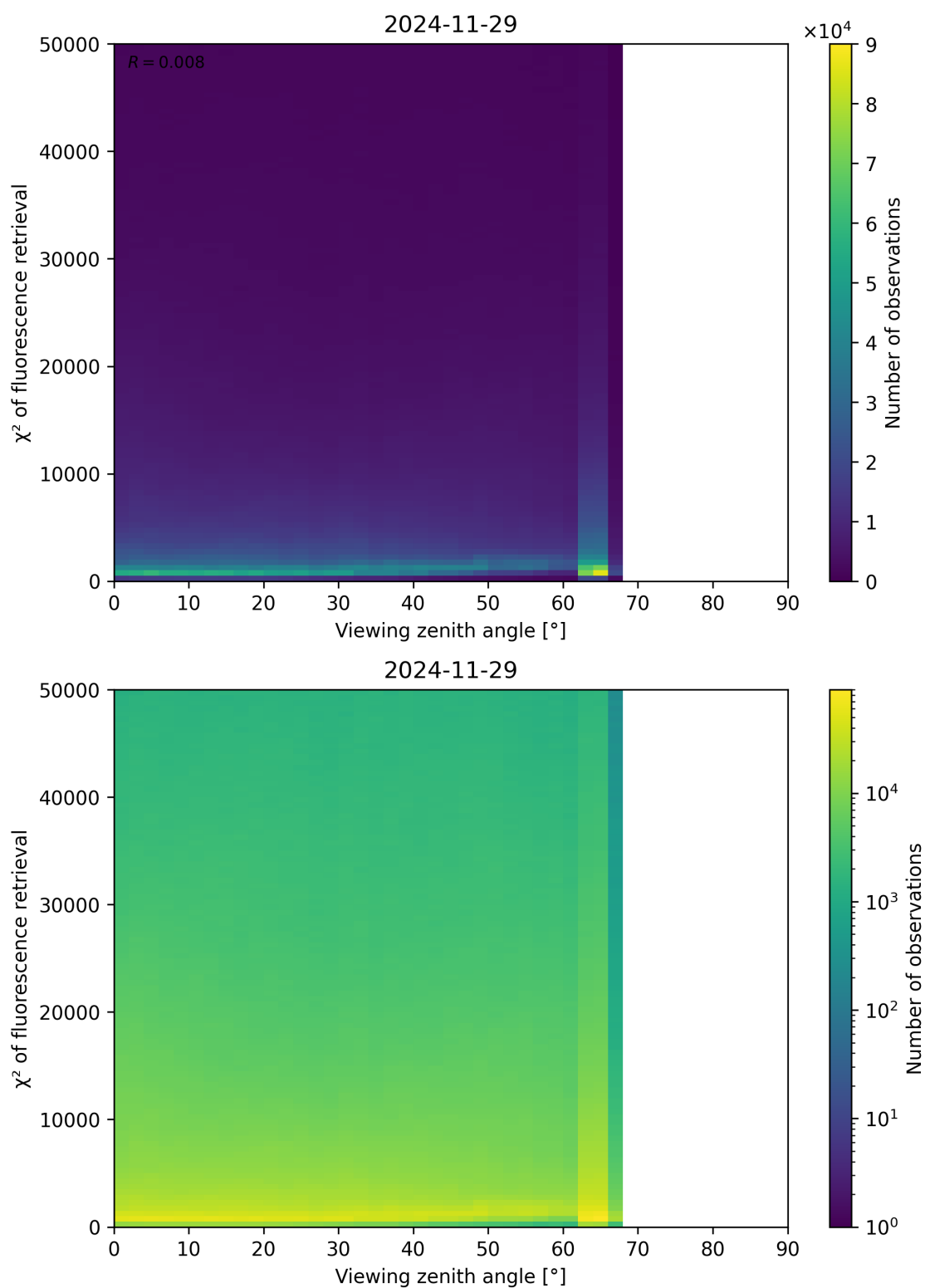
Figure 119: Scatter density plot of “Viewing zenith angle” against “ \chi^2 of fluorescence retrieval” for 2024-11-28 to 2024-11-30.
