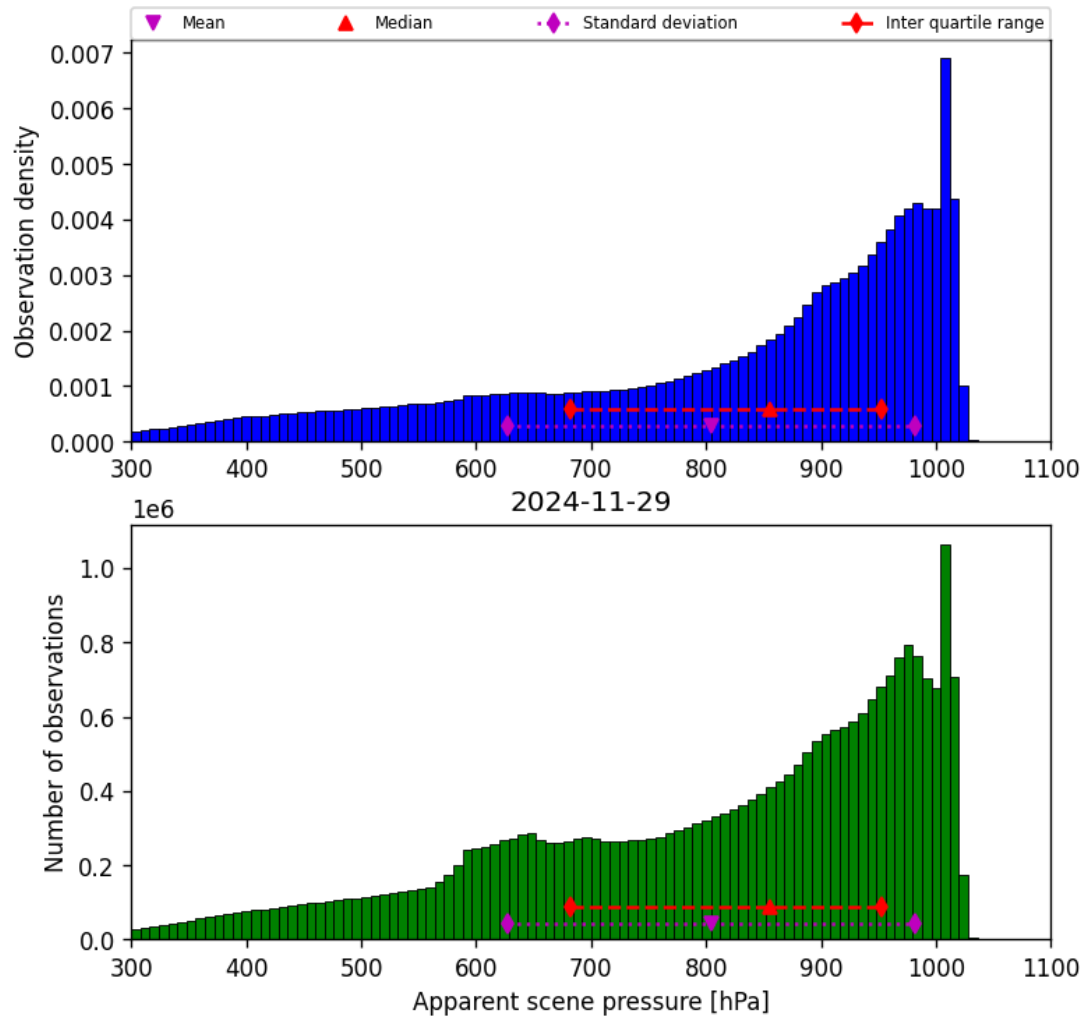
Figure 36: Histogram of “Apparent scene pressure” for 2024-11-28 to 2024-11-30
