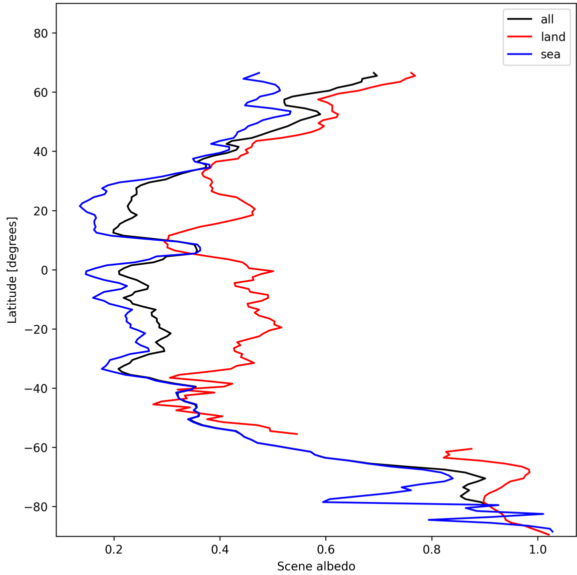
Figure 17: Zonal average of “Scene albedo” for 2024-11-28 to 2024-11-30.
