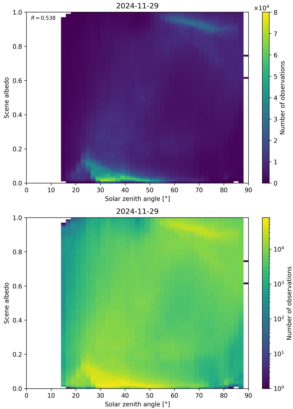
Figure 116: Scatter density plot of “Solar zenith angle” against “Scene albedo” for 2024-11-28 to 2024-11-30.
