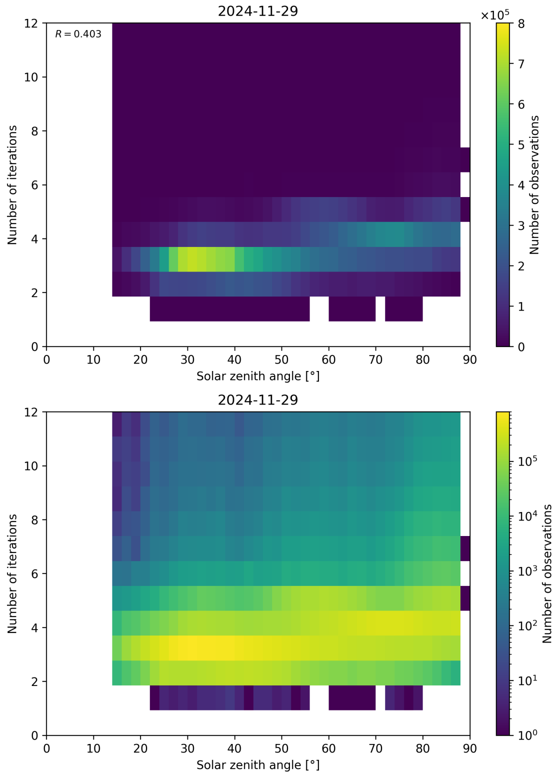
Figure 114: Scatter density plot of “Solar zenith angle” against “Number of iterations” for 2024-11-28 to 2024-11-30.
