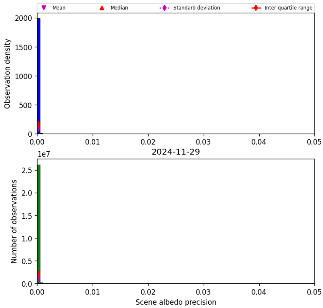
Figure 35: Histogram of “Scene albedo precision” for 2024-11-28 to 2024-11-30
