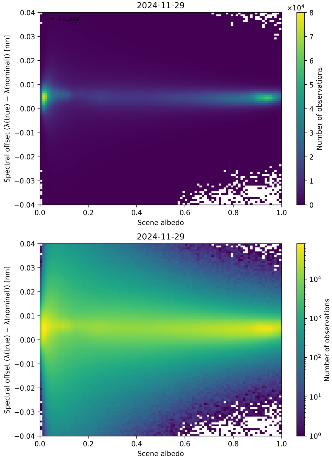
Figure 107: Scatter density plot of “Scene albedo” against “Spectral offset ( \lambda_{\text{true}} - \lambda_{\text{nominal}} )” for 2024-11-28 to 2024-11-30.
