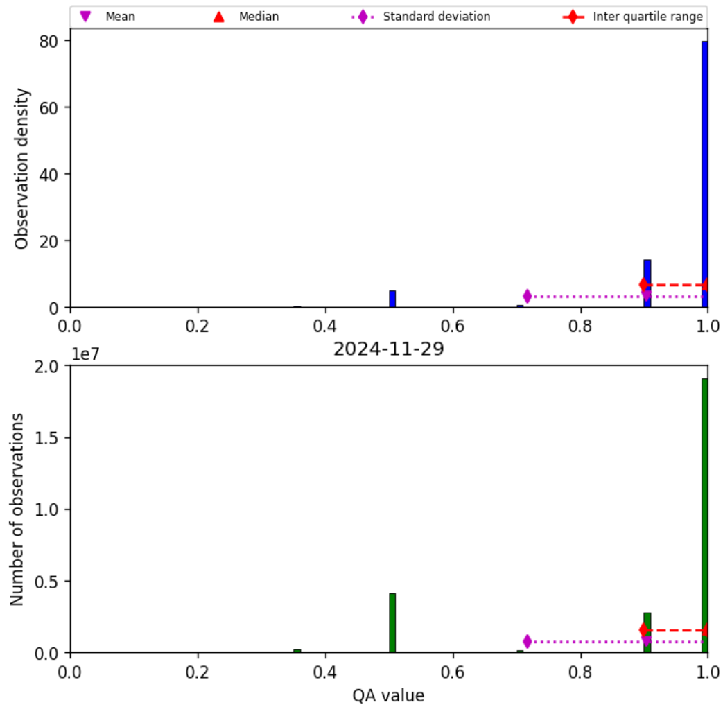
Figure 29: Histogram of “QA value” for 2024-11-28 to 2024-11-30
