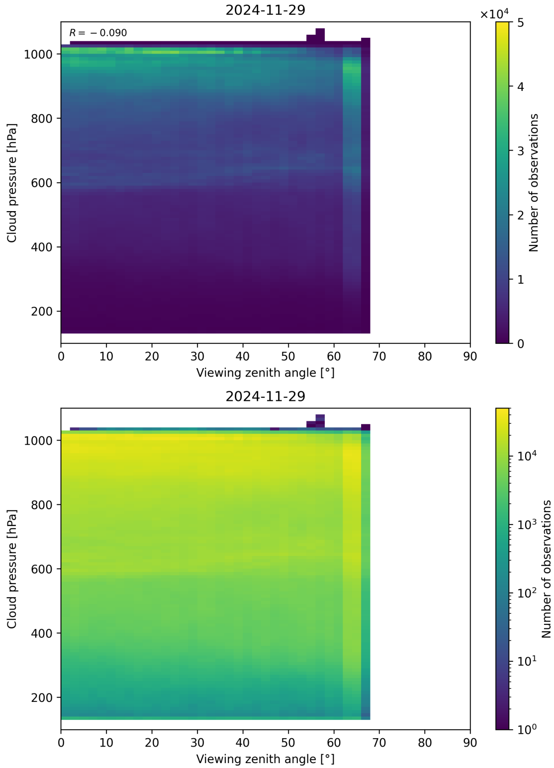
Figure 121: Scatter density plot of “Viewing zenith angle” against “Cloud pressure” for 2024-11-28 to 2024-11-30.
