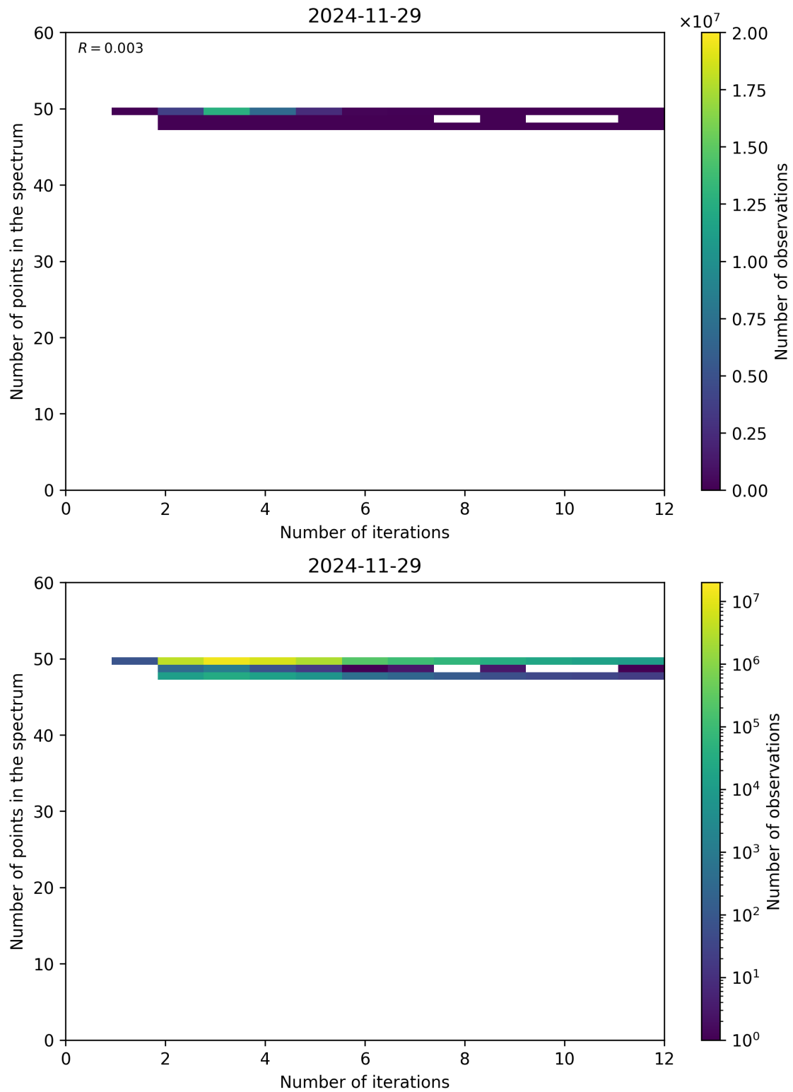
Figure 99: Scatter density plot of “Number of iterations” against “Number of points in the spectrum” for 2024-11-28 to 2024-11-30.
