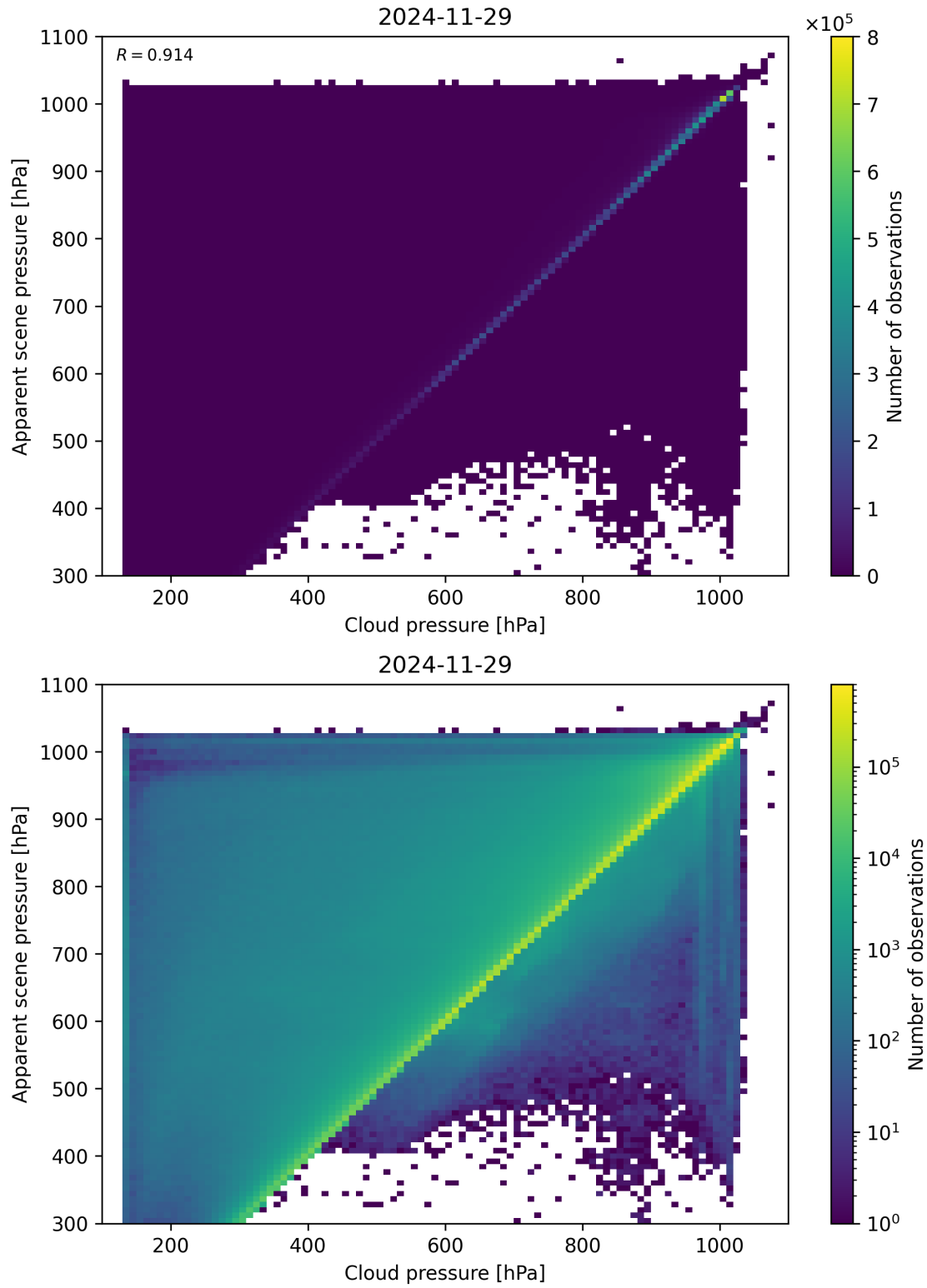
Figure 77: Scatter density plot of “Cloud pressure” against “Apparent scene pressure” for 2024-11-28 to 2024-11-30.
