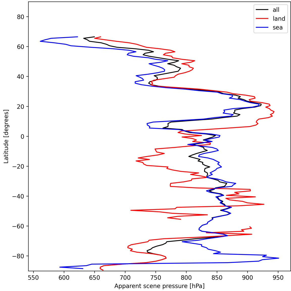
Figure 19: Zonal average of “Apparent scene pressure” for 2024-11-28 to 2024-11-30.
