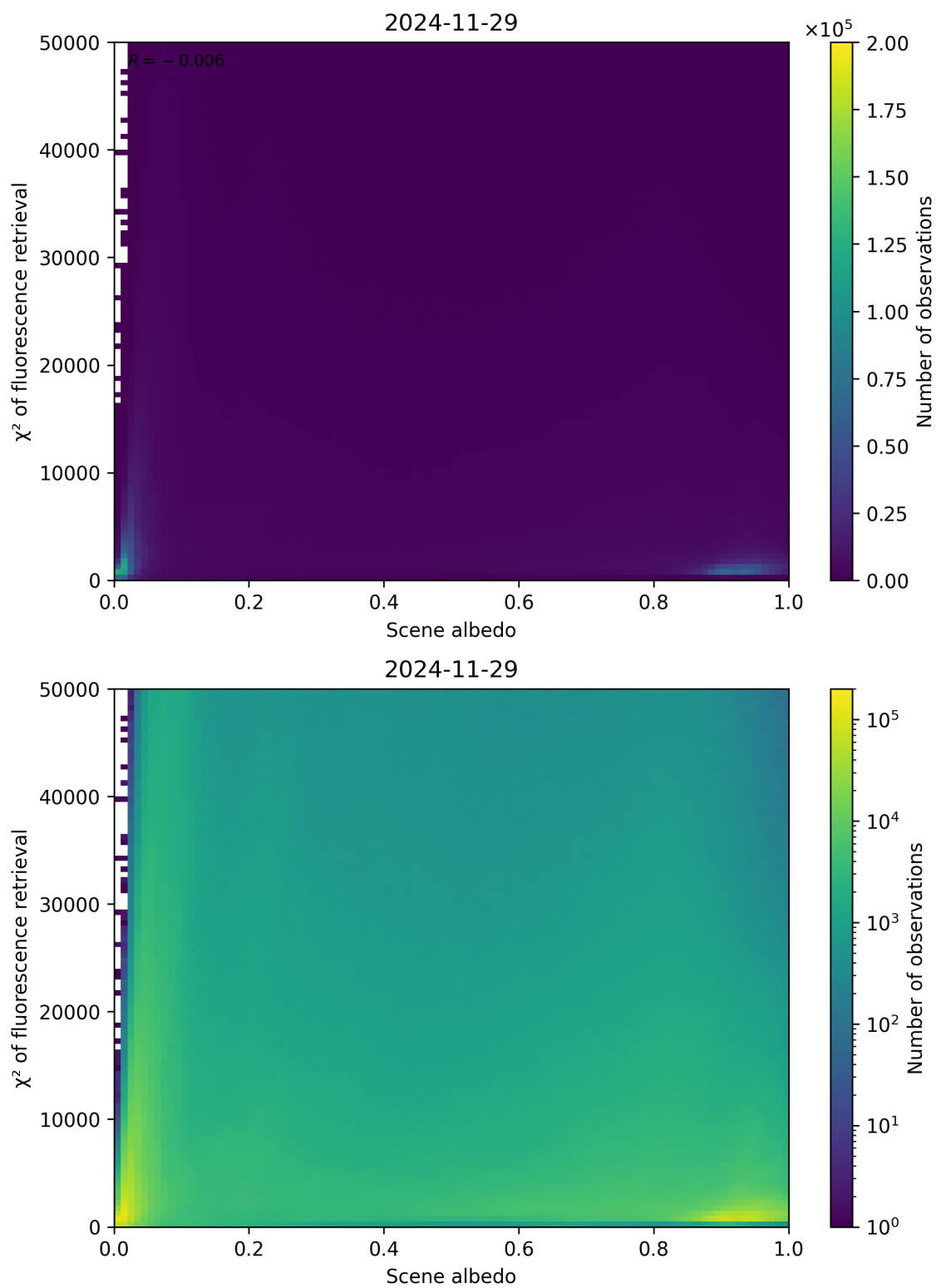
Figure 103: Scatter density plot of “Scene albedo” against “ \chi^2 of fluorescence retrieval” for 2024-11-28 to 2024-11-30.
