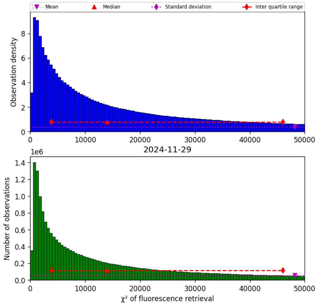
Figure 42: Histogram of “ \chi^2 of fluorescence retrieval” for 2024-11-28 to 2024-11-30
