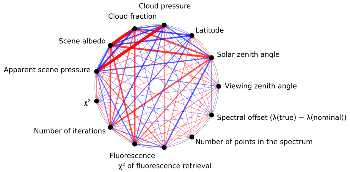
Figure 1: Map of correlation graph for 2024-11-28 to 2024-11-30.
