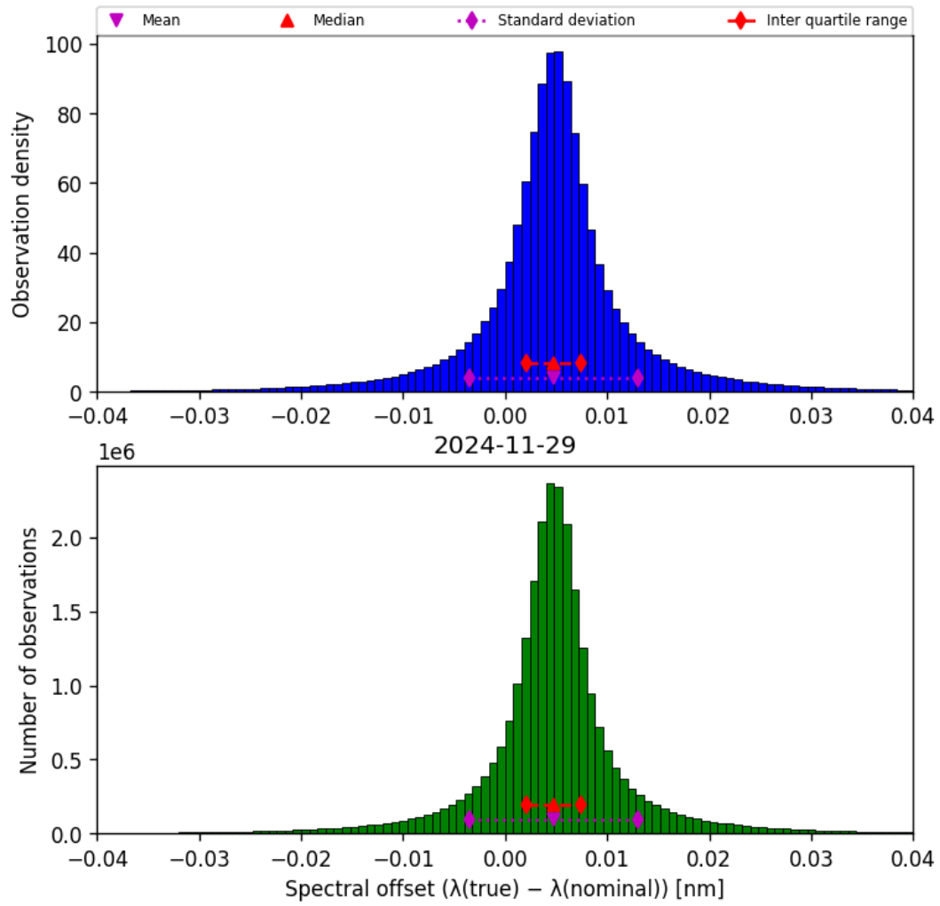
Figure 45: Histogram of “Spectral offset ( \lambda_{\text{true}} - \lambda_{\text{nominal}} )” for 2024-11-28 to 2024-11-30
