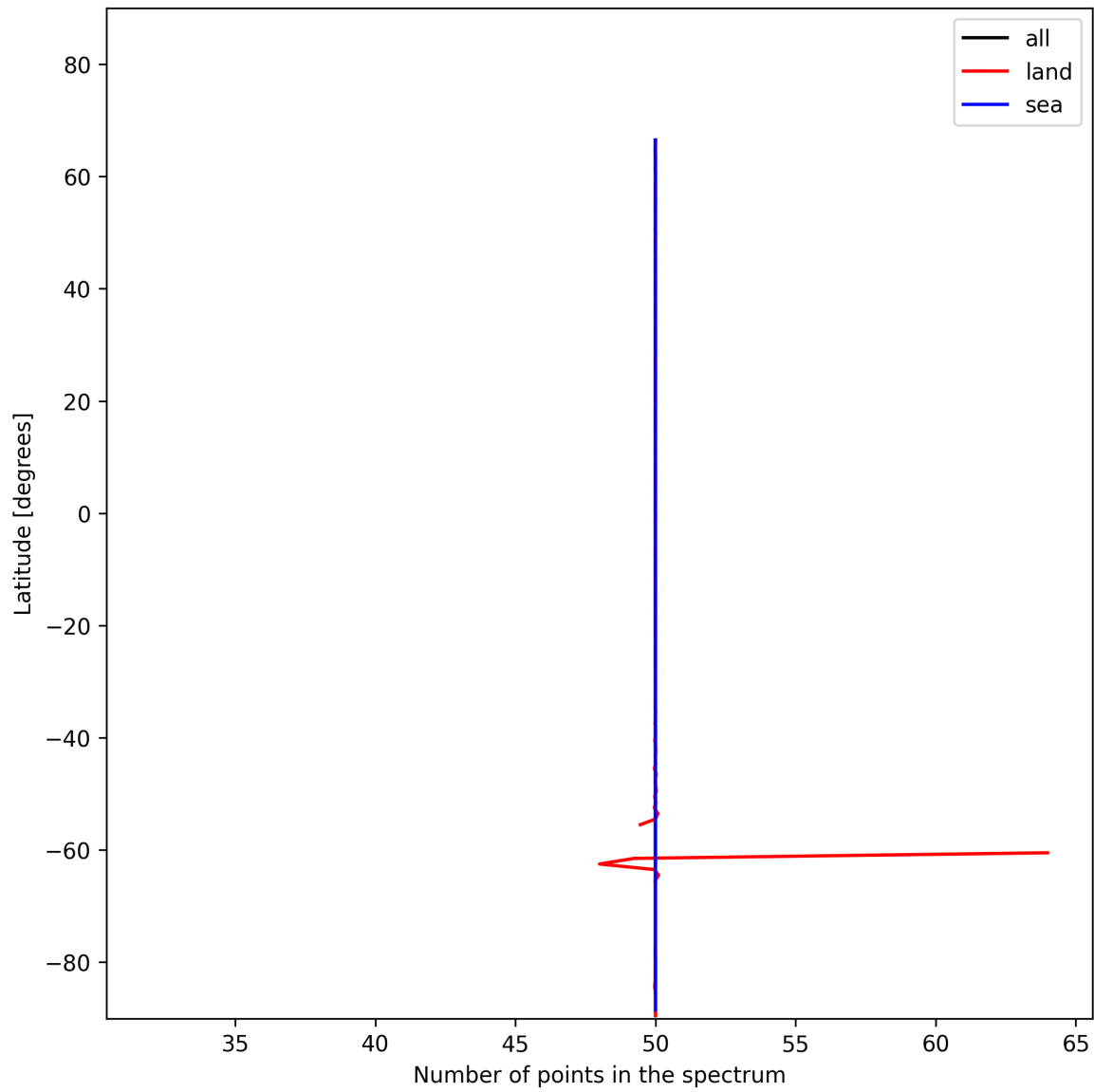
Figure 27: Zonal average of “Number of points in the spectrum” for 2024-11-28 to 2024-11-30.
