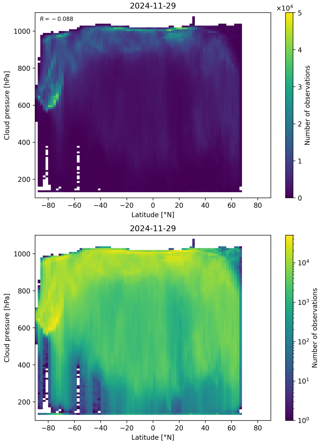
Figure 91: Scatter density plot of “Latitude” against “Cloud pressure” for 2024-11-28 to 2024-11-30.
