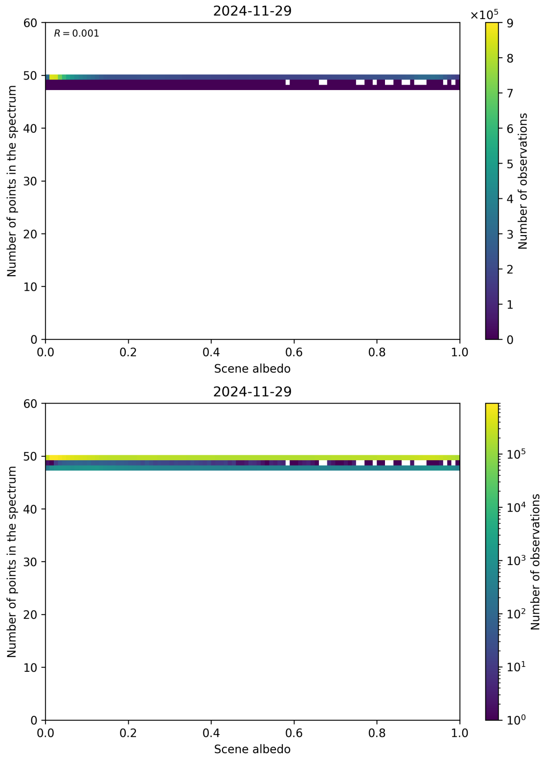
Figure 106: Scatter density plot of “Scene albedo” against “Number of points in the spectrum” for 2024-11-28 to 2024-11-30.
