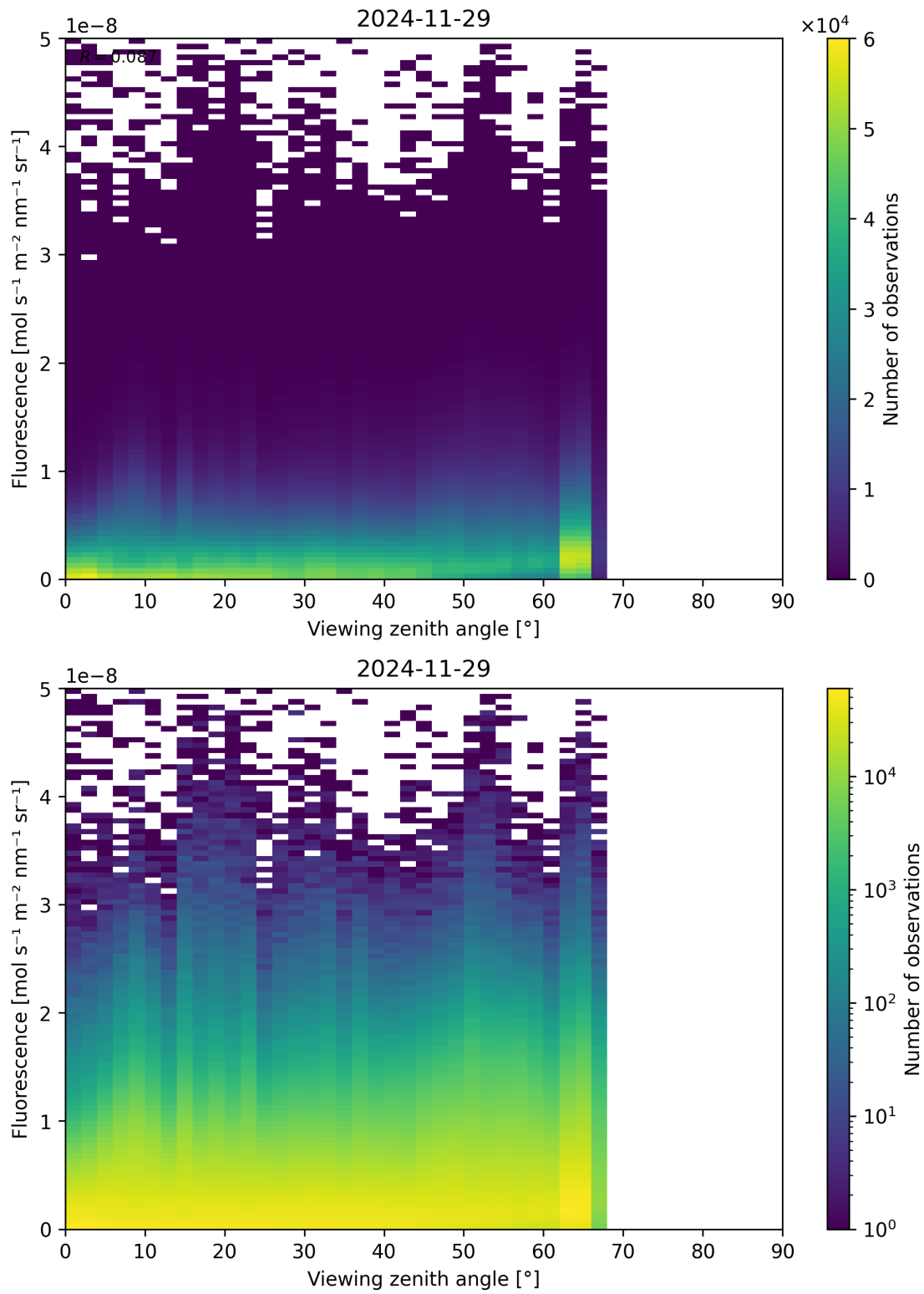
Figure 122: Scatter density plot of “Viewing zenith angle” against “Fluorescence” for 2024-11-28 to 2024-11-30.
