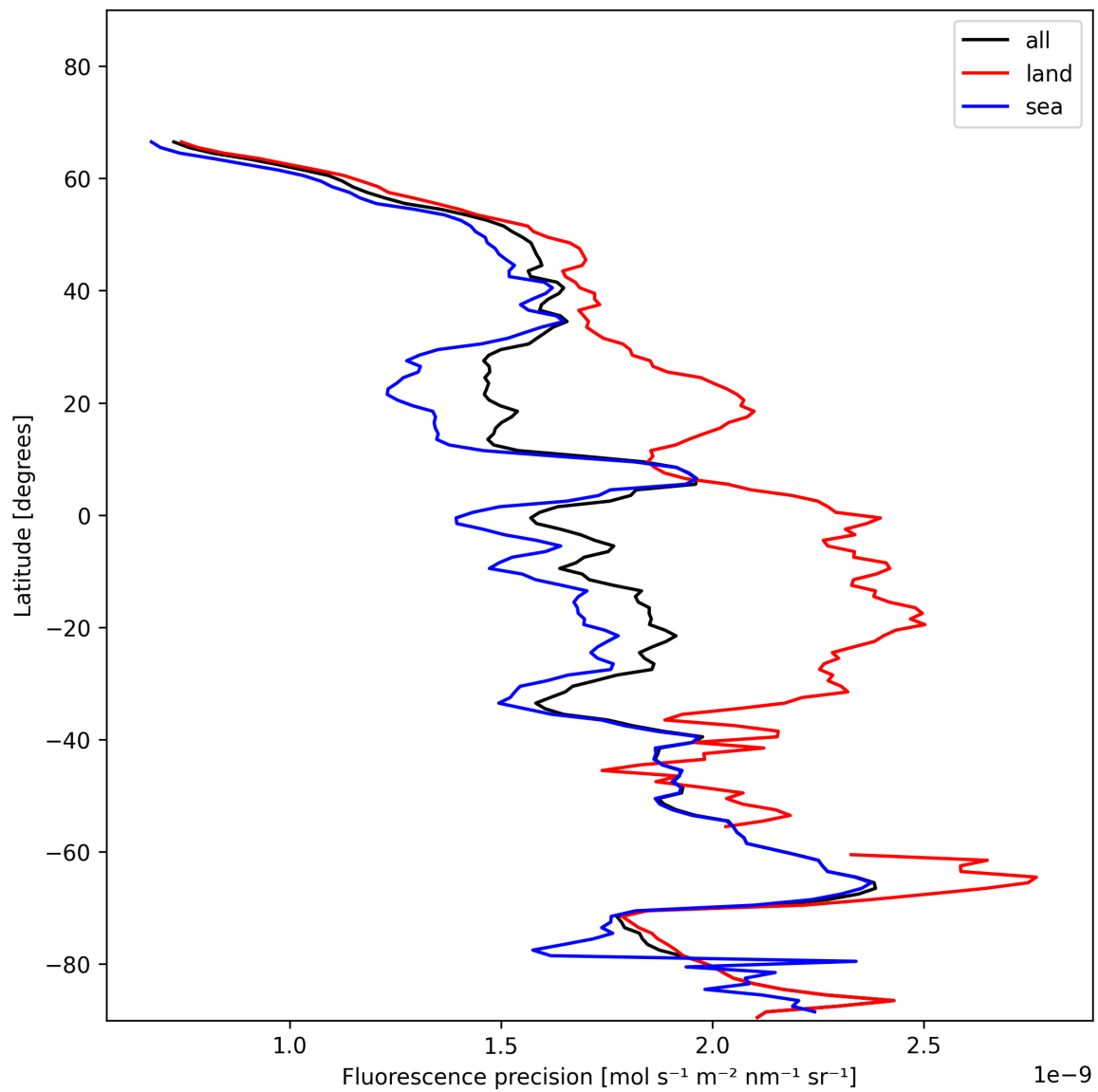
Figure 24: Zonal average of “Fluorescence precision” for 2024-11-28 to 2024-11-30.
