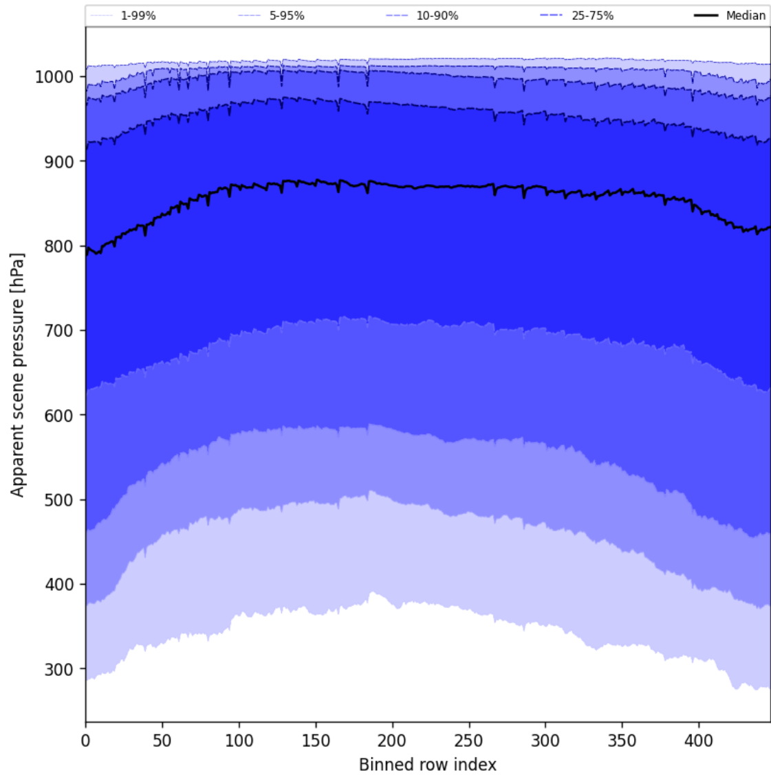
Figure 53: Along track statistics of “Apparent scene pressure” for 2024-11-28 to 2024-11-30
