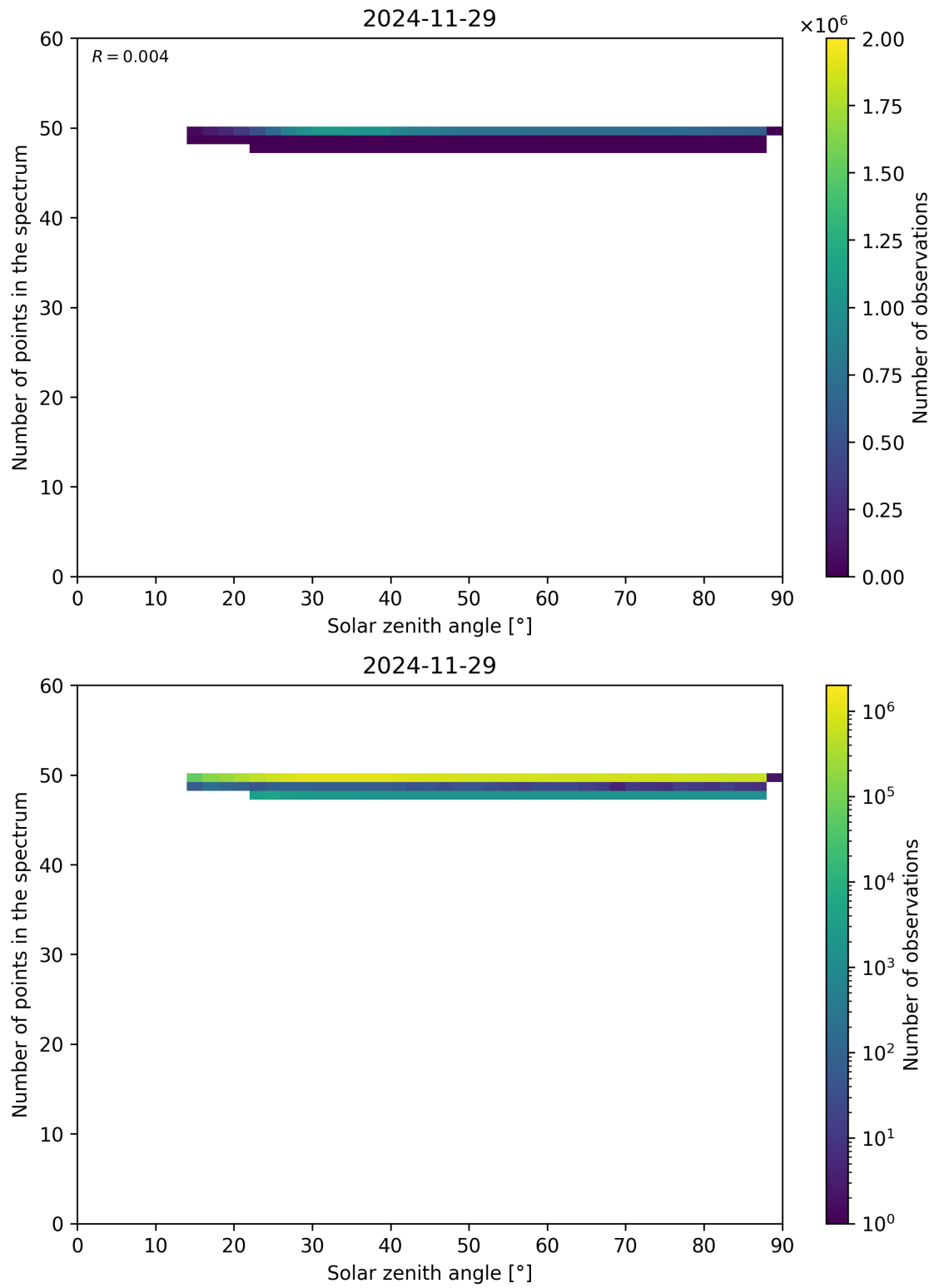
Figure 115: Scatter density plot of “Solar zenith angle” against “Number of points in the spectrum” for 2024-11-28 to 2024-11-30.
