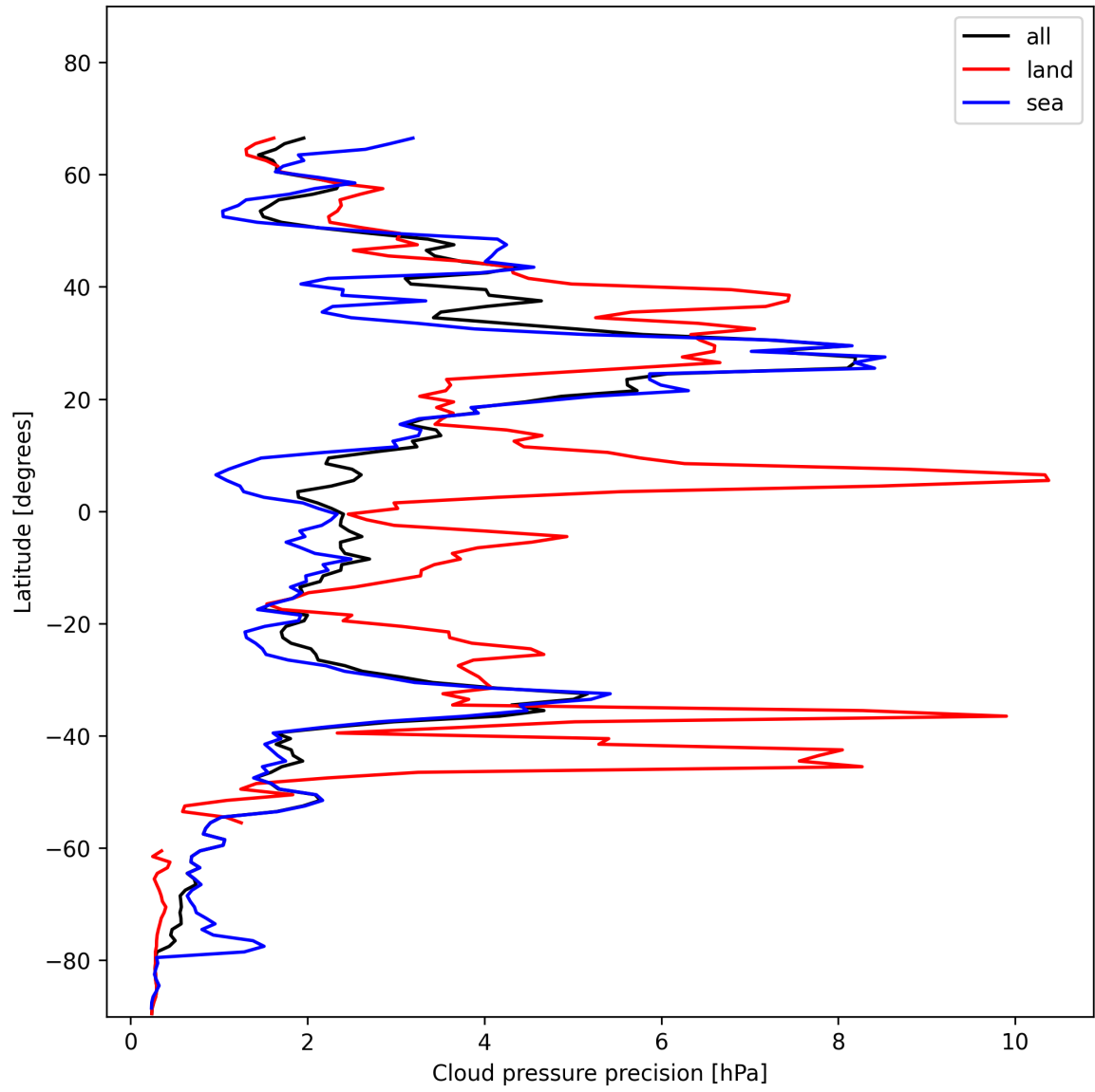
Figure 14: Zonal average of “Cloud pressure precision” for 2024-11-28 to 2024-11-30.
