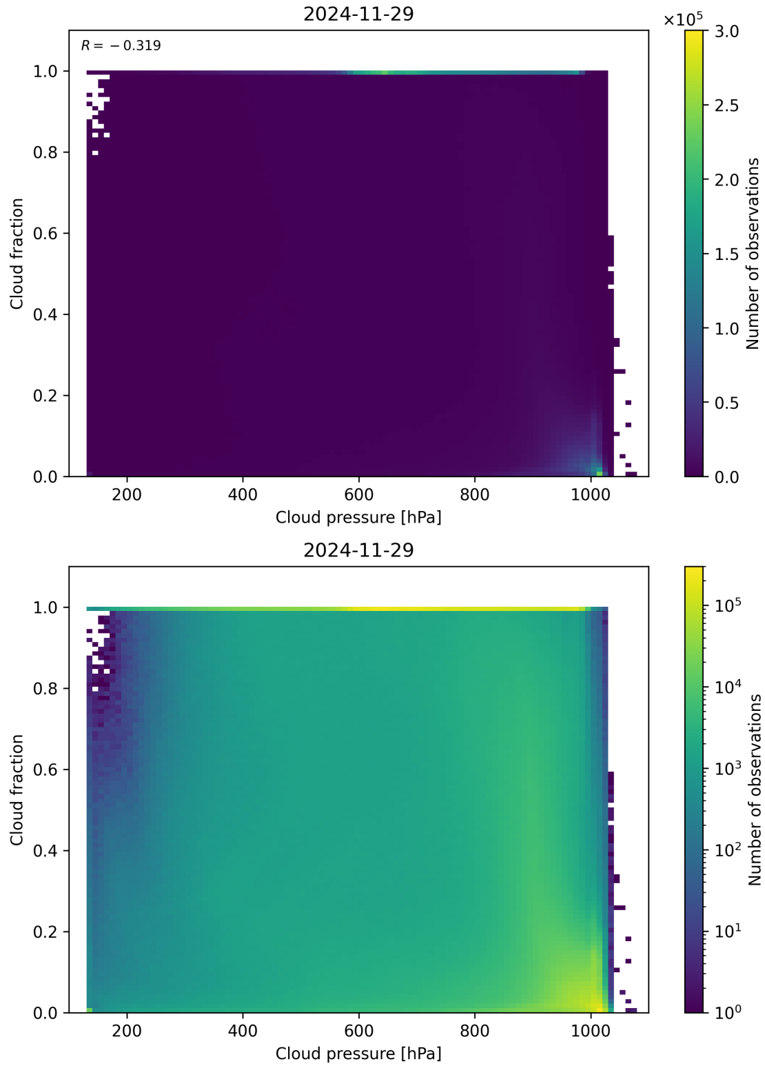
Figure 79: Scatter density plot of “Cloud pressure” against “Cloud fraction” for 2024-11-28 to 2024-11-30.
