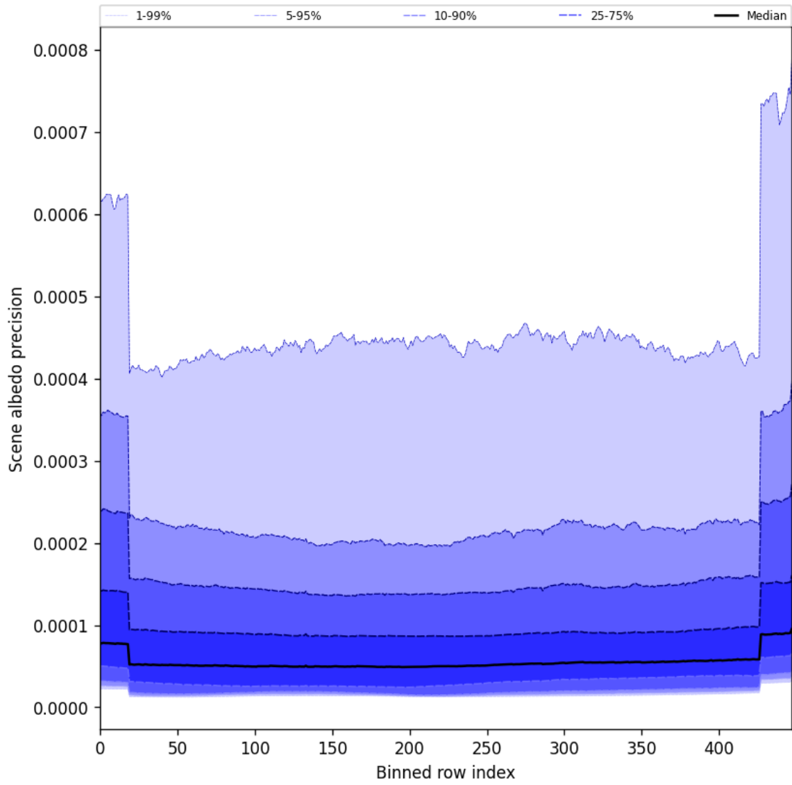
Figure 52: Along track statistics of “Scene albedo precision” for 2024-11-28 to 2024-11-30
