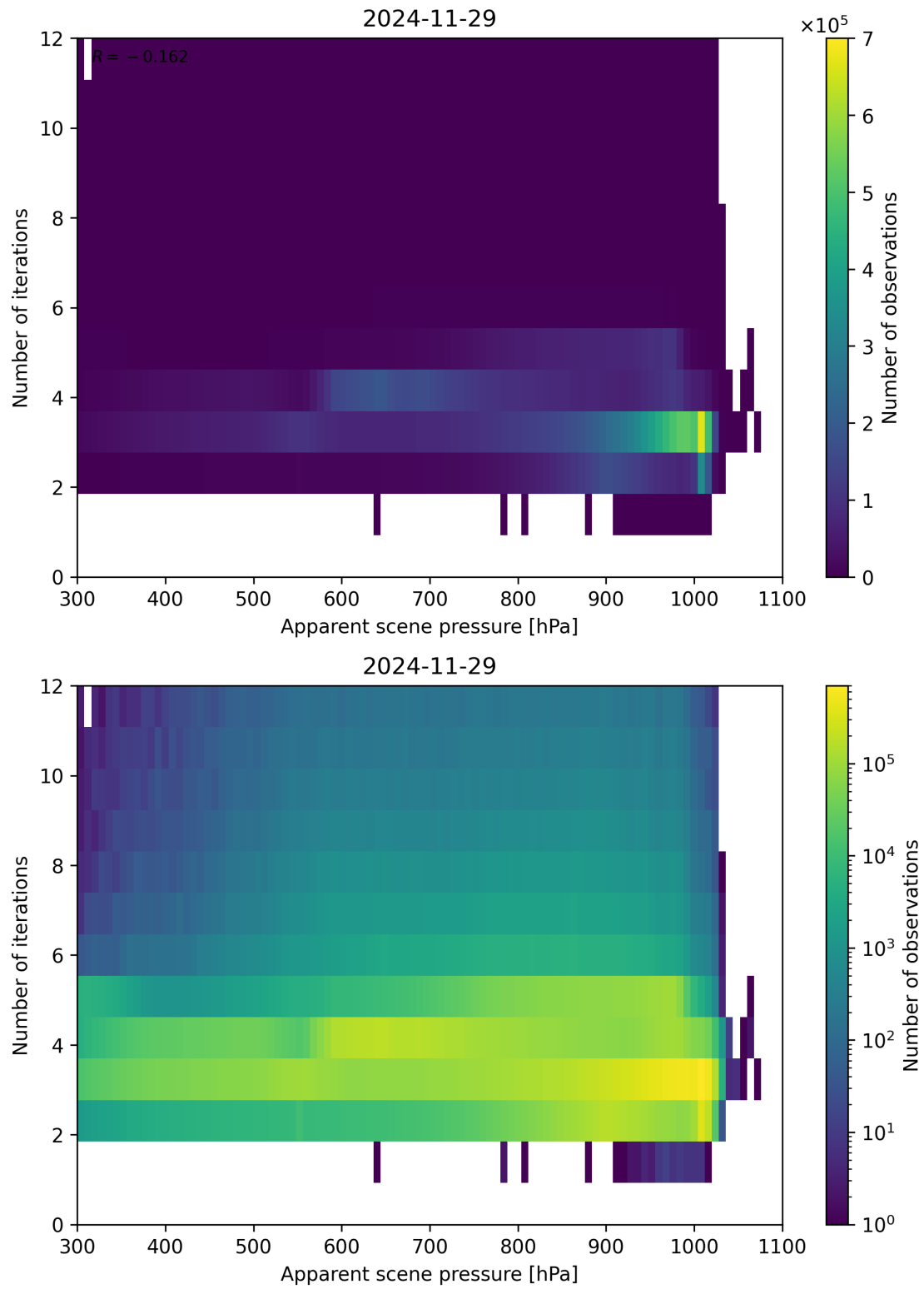
Figure 65: Scatter density plot of “Apparent scene pressure” against “Number of iterations” for 2024-11-28 to 2024-11-30.
