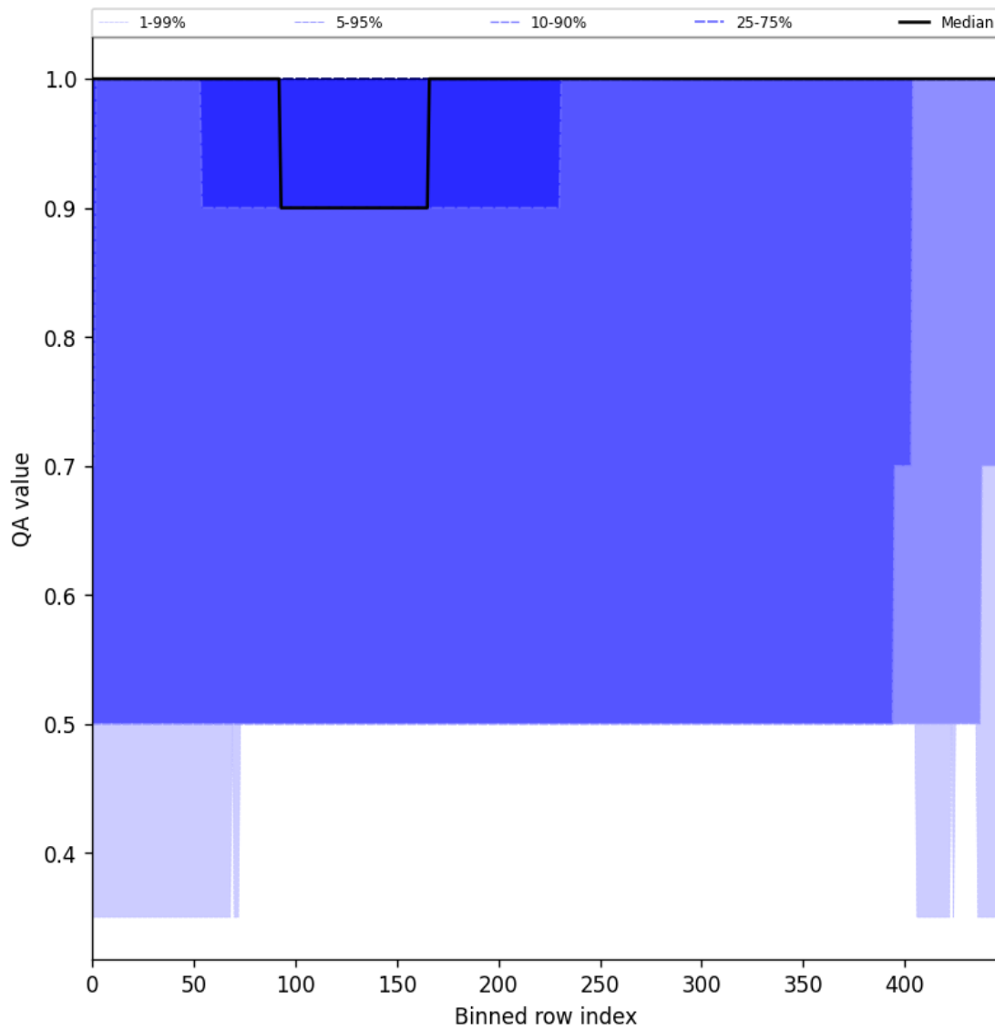
Figure 46: Along track statistics of “QA value” for 2024-11-28 to 2024-11-30
