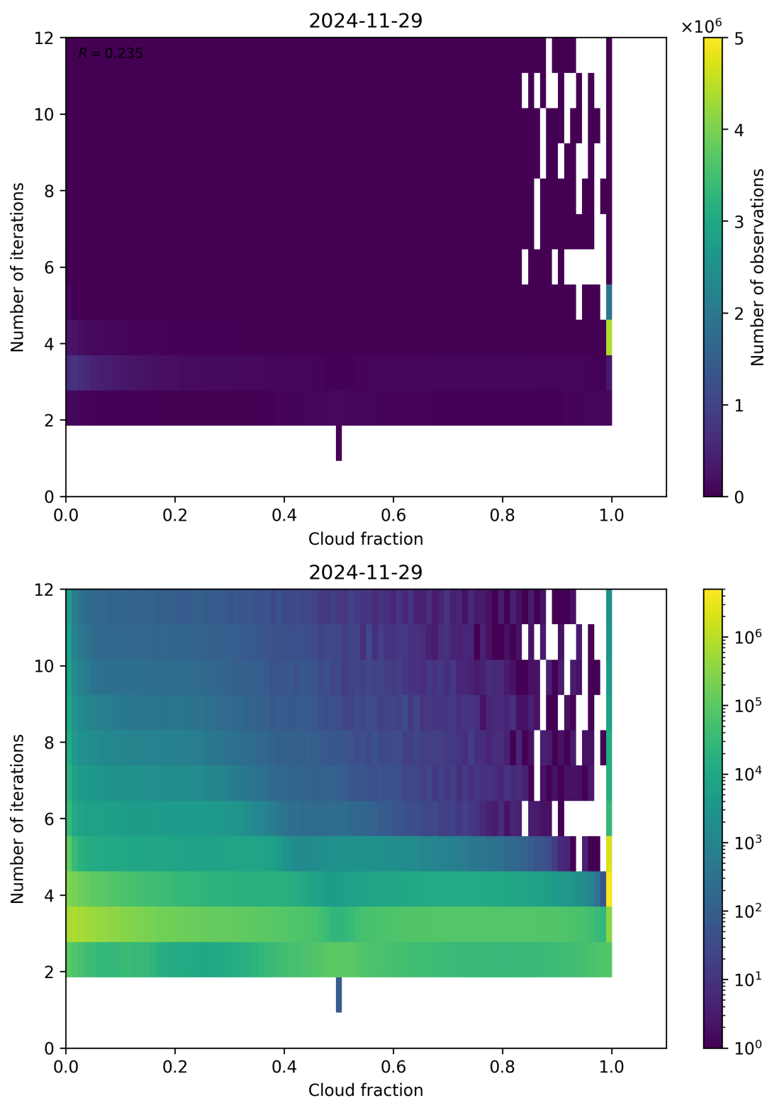
Figure 73: Scatter density plot of “Cloud fraction” against “Number of iterations” for 2024-11-28 to 2024-11-30.
