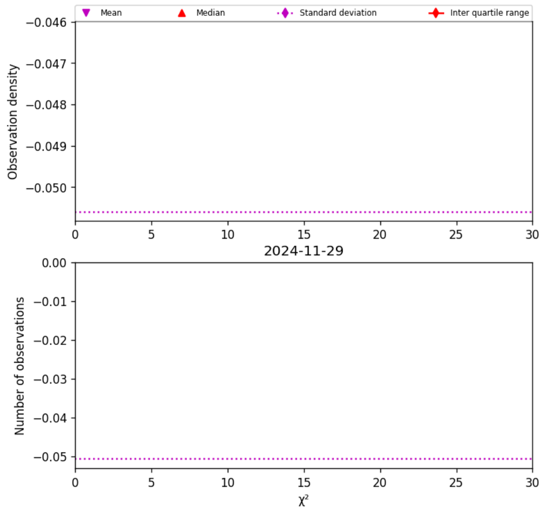
Figure 38: Histogram of “ \chi^2 ” for 2024-11-28 to 2024-11-30
