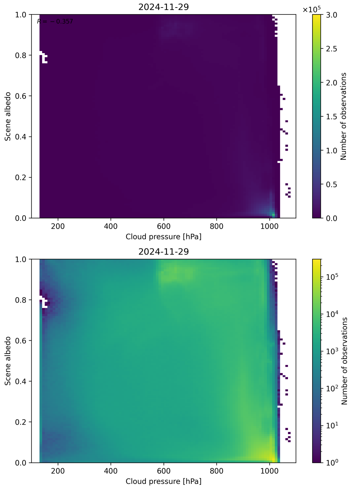
Figure 83: Scatter density plot of “Cloud pressure” against “Scene albedo” for 2024-11-28 to 2024-11-30.
