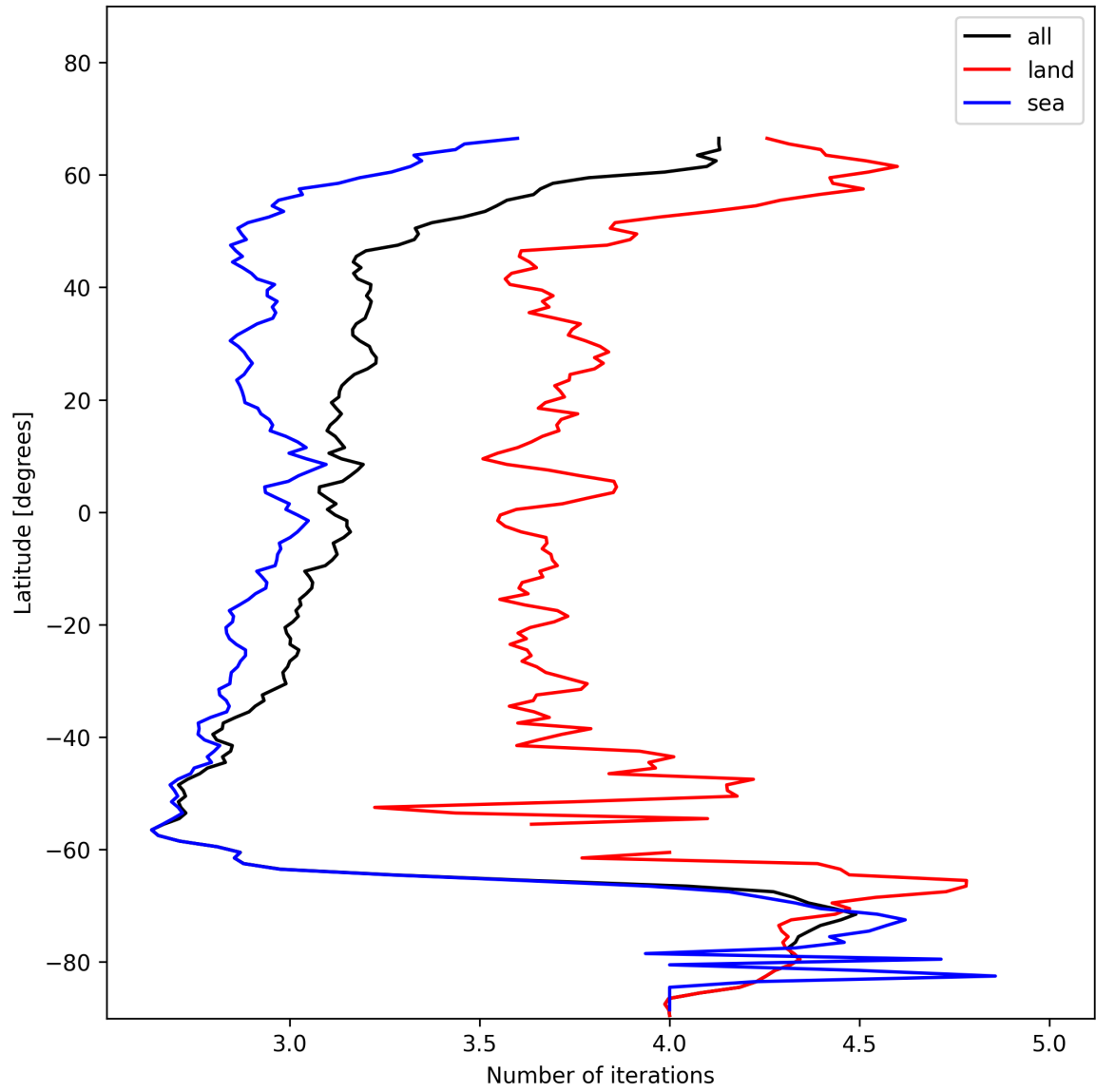
Figure 22: Zonal average of “Number of iterations” for 2024-11-28 to 2024-11-30.
