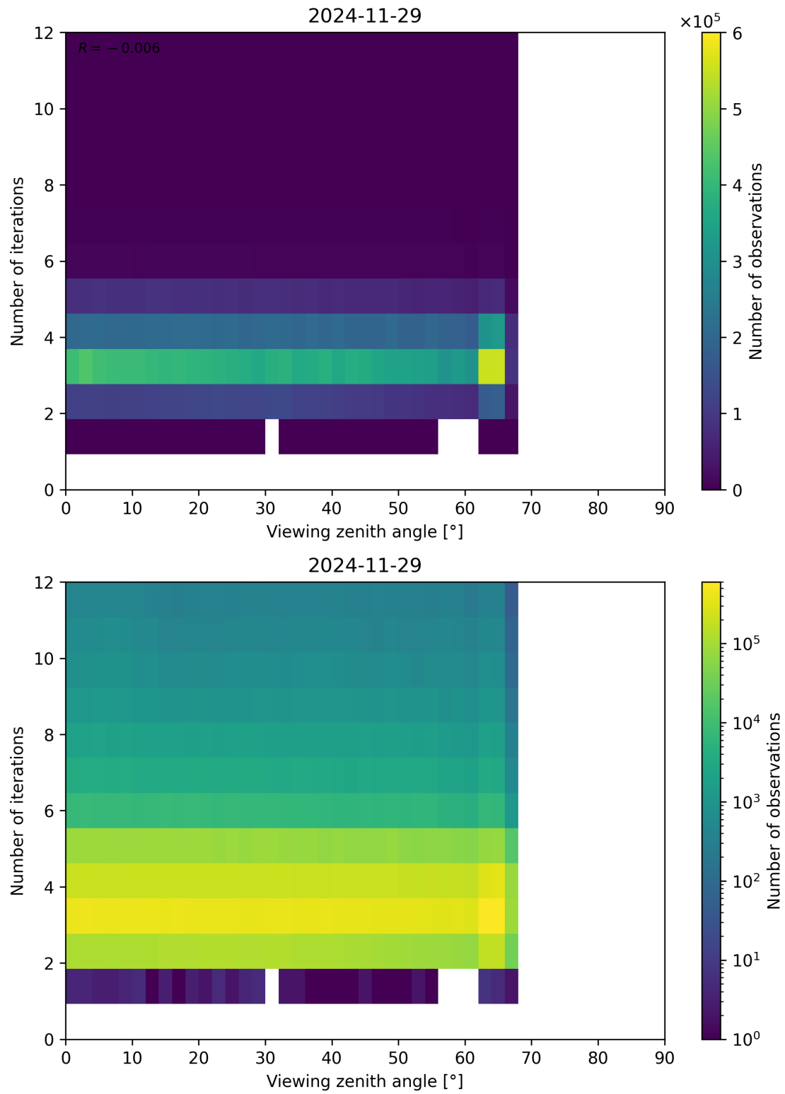
Figure 124: Scatter density plot of “Viewing zenith angle” against “Number of iterations” for 2024-11-28 to 2024-11-30.
