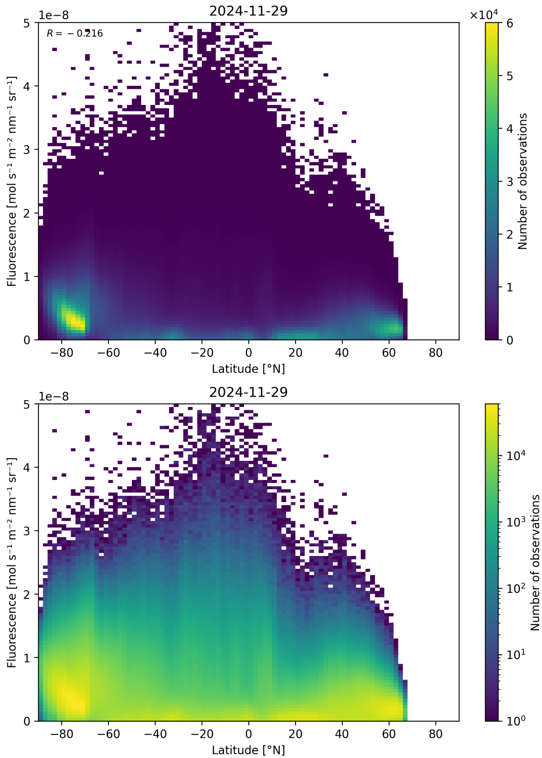
Figure 92: Scatter density plot of “Latitude” against “Fluorescence” for 2024-11-28 to 2024-11-30.
