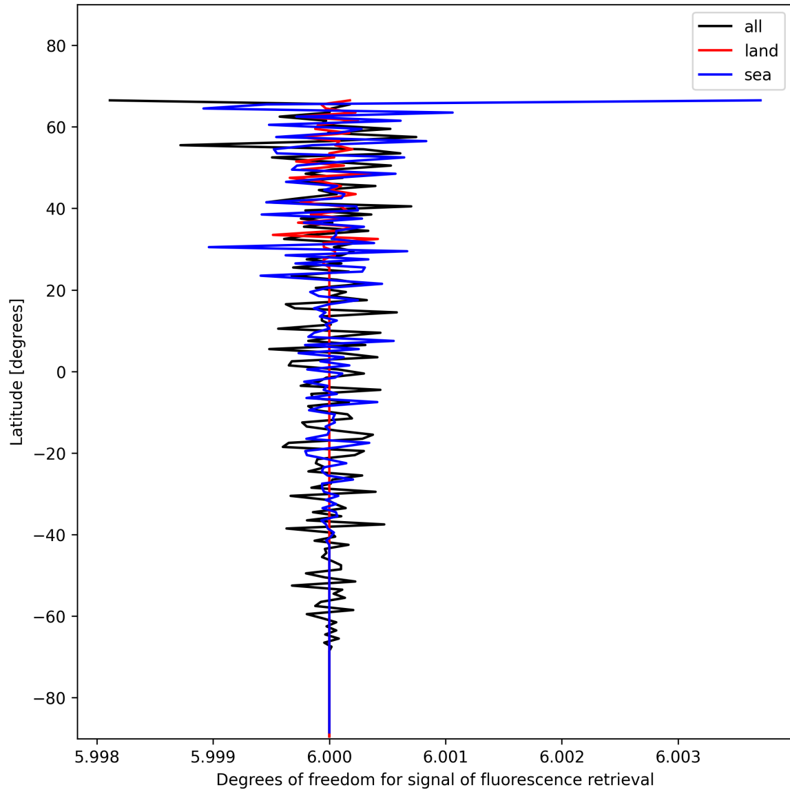
Figure 26: Zonal average of “Degrees of freedom for signal of fluorescence retrieval” for 2024-11-28 to 2024-11-30.
