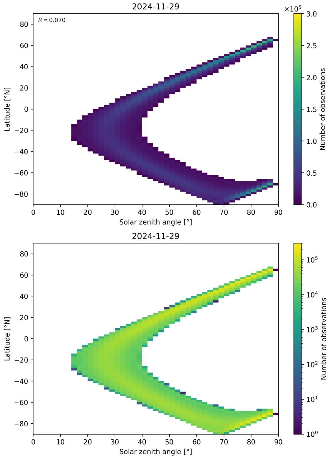
Figure 113: Scatter density plot of “Solar zenith angle” against “Latitude” for 2024-11-28 to 2024-11-30.
