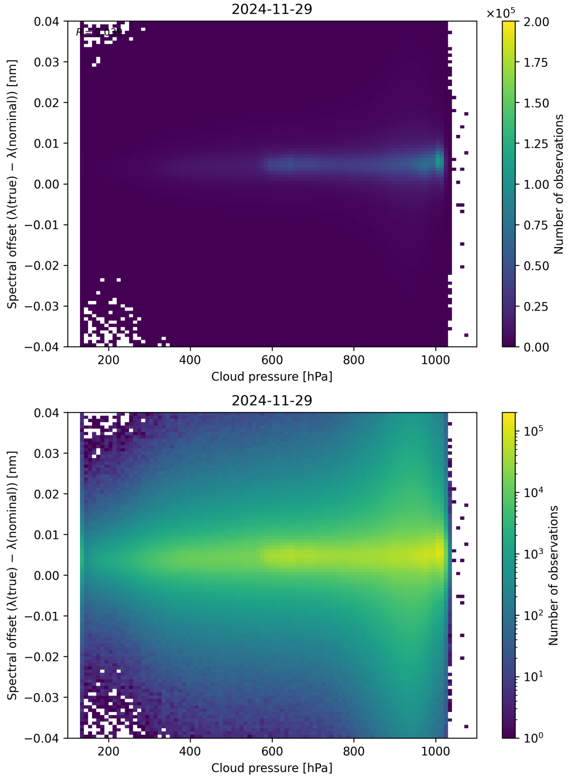
Figure 84: Scatter density plot of “Cloud pressure” against “Spectral offset ( \lambda_{\text{true}} - \lambda_{\text{nominal}} )” for 2024-11-28 to 2024-11-30.
