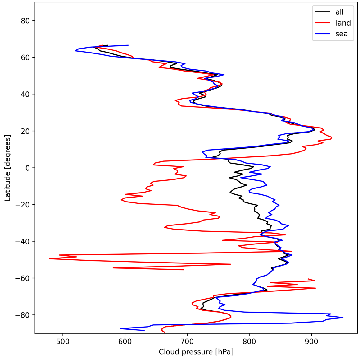
Figure 13: Zonal average of “Cloud pressure” for 2024-11-28 to 2024-11-30.
