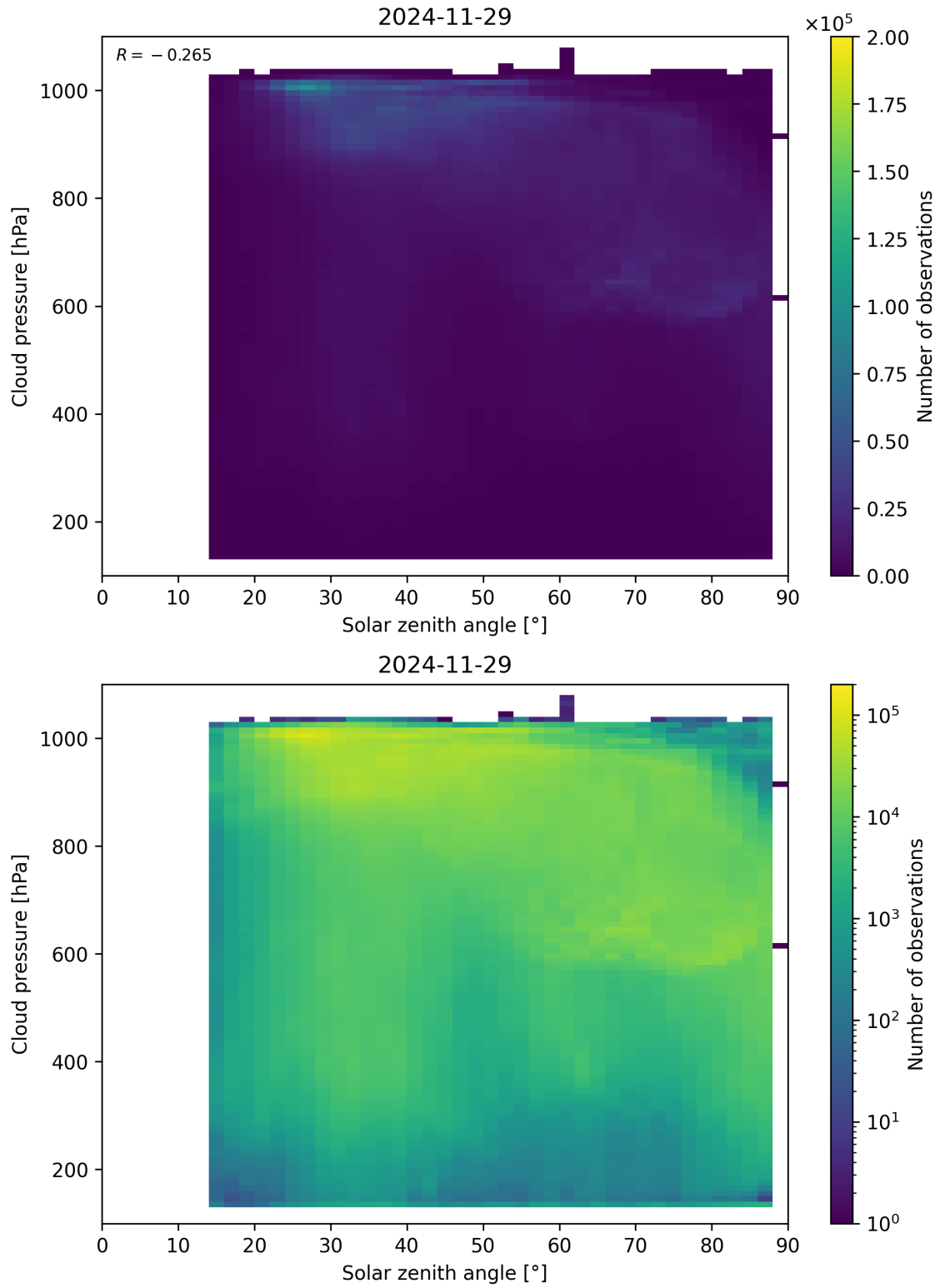
Figure 111: Scatter density plot of “Solar zenith angle” against “Cloud pressure” for 2024-11-28 to 2024-11-30.
