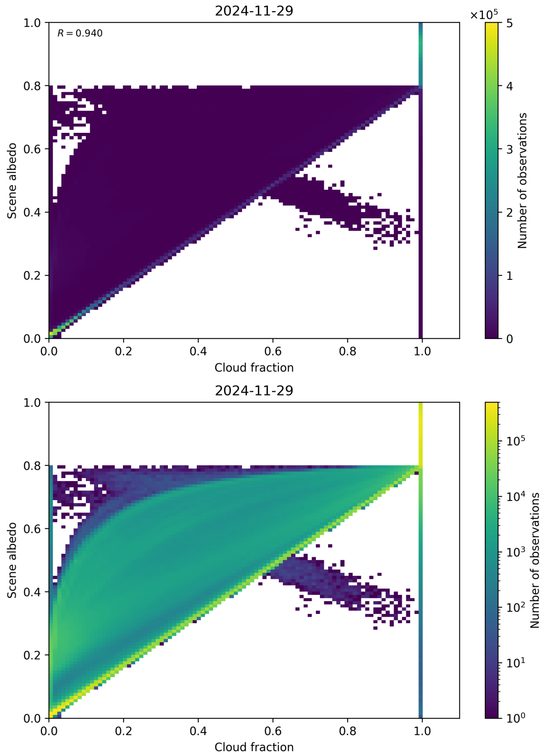
Figure 75: Scatter density plot of “Cloud fraction” against “Scene albedo” for 2024-11-28 to 2024-11-30.
