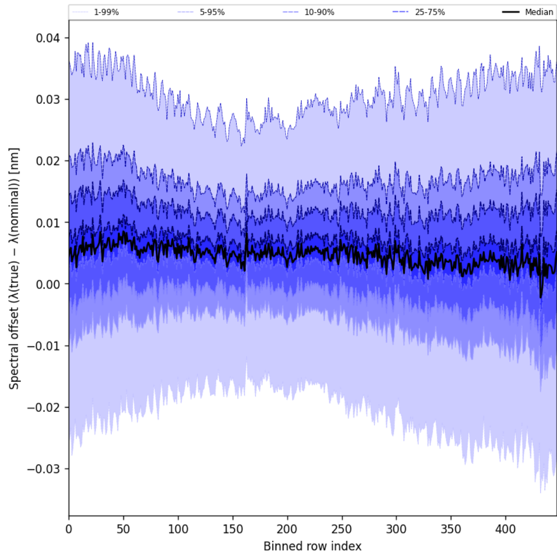
Figure 62: Along track statistics of “Spectral offset ( \lambda_{\text{true}} - \lambda_{\text{nominal}} )” for 2024-11-28 to 2024-11-30
