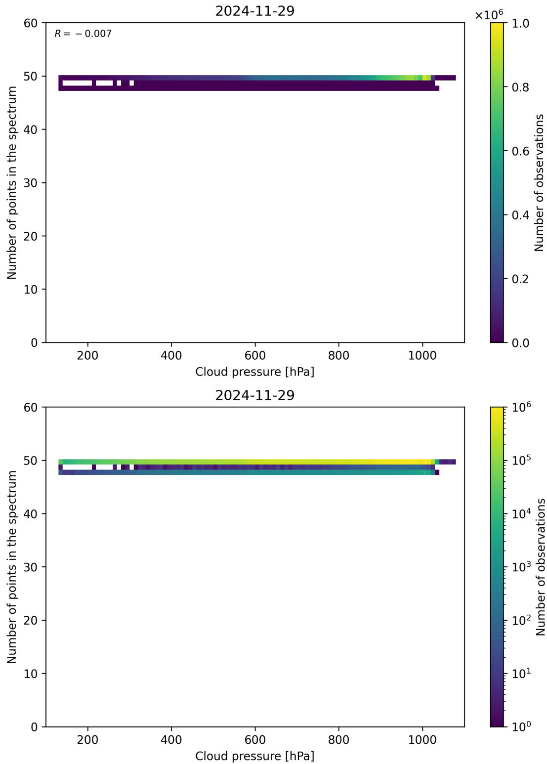
Figure 82: Scatter density plot of “Cloud pressure” against “Number of points in the spectrum” for 2024-11-28 to 2024-11-30.
