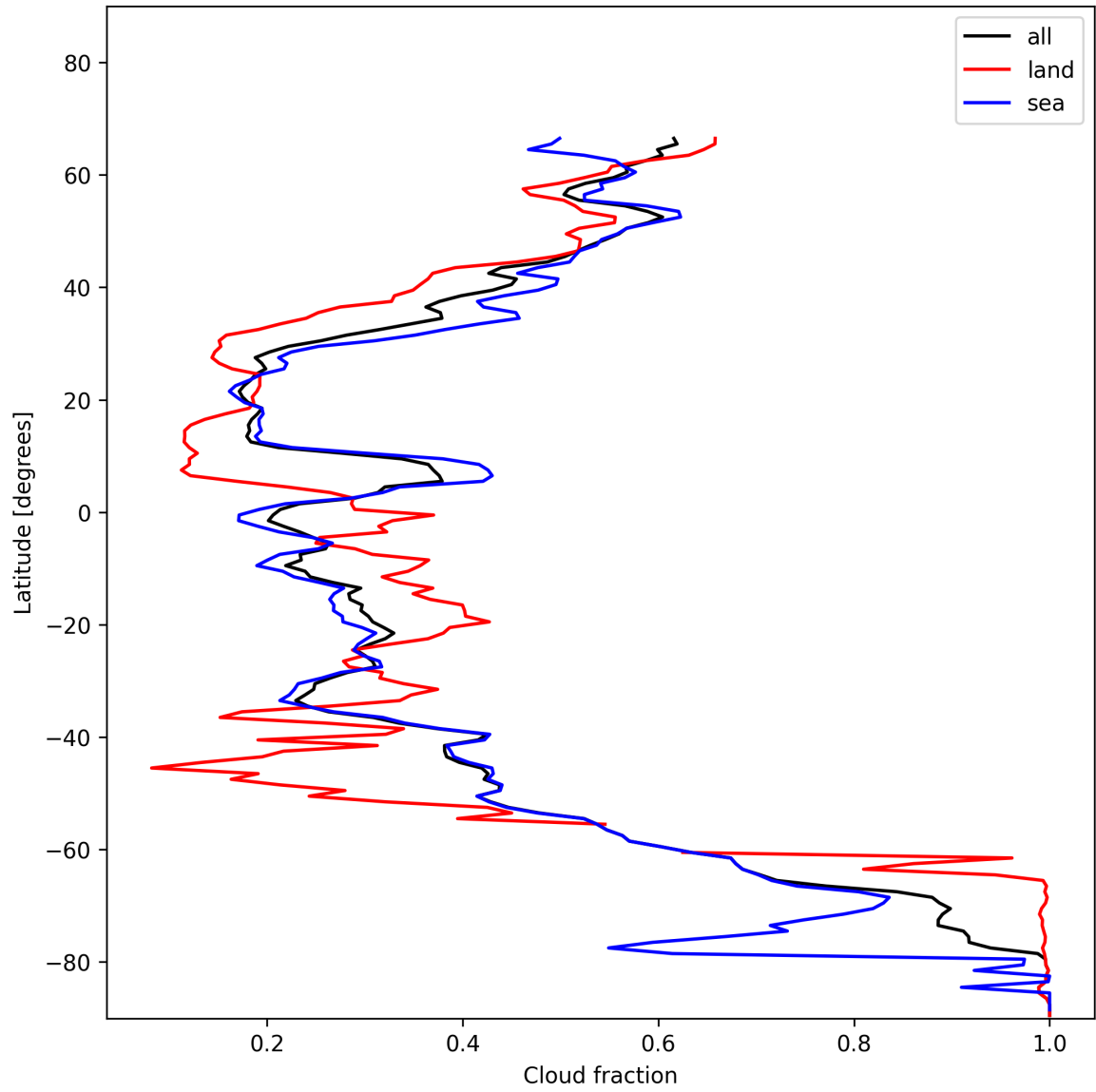
Figure 15: Zonal average of “Cloud fraction” for 2024-11-28 to 2024-11-30.
