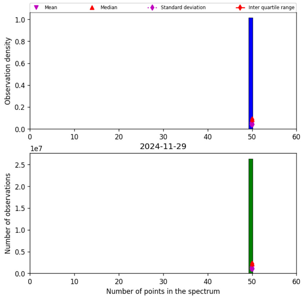
Figure 44: Histogram of “Number of points in the spectrum” for 2024-11-28 to 2024-11-30
