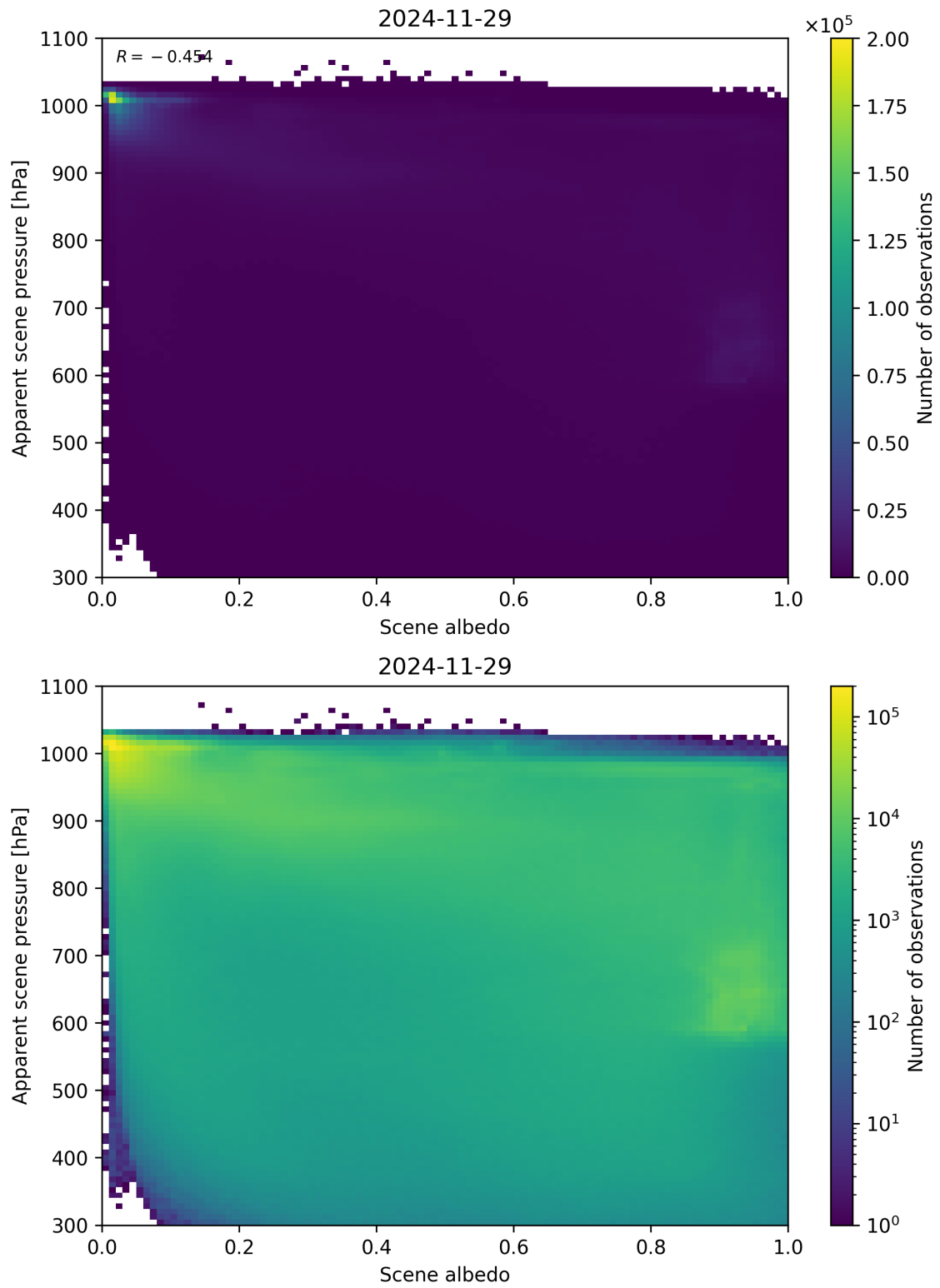
Figure 102: Scatter density plot of “Scene albedo” against “Apparent scene pressure” for 2024-11-28 to 2024-11-30.
