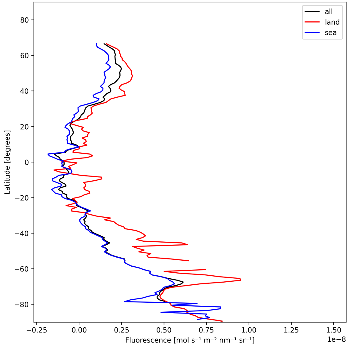
Figure 23: Zonal average of “Fluorescence” for 2024-11-28 to 2024-11-30.
