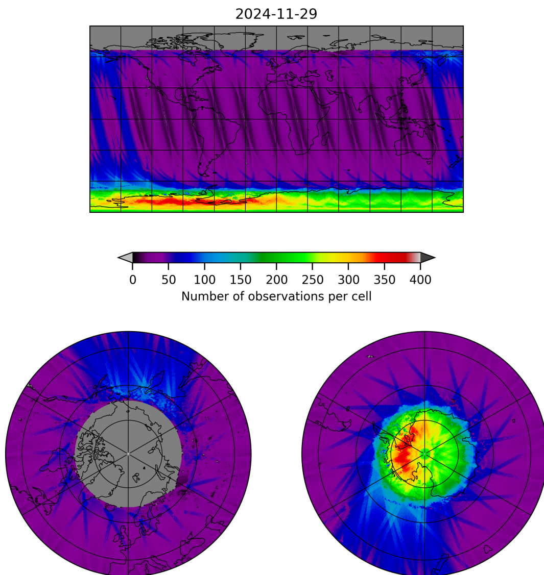
Figure 11: Map of the number of observations for 2024-11-28 to 2024-11-30
