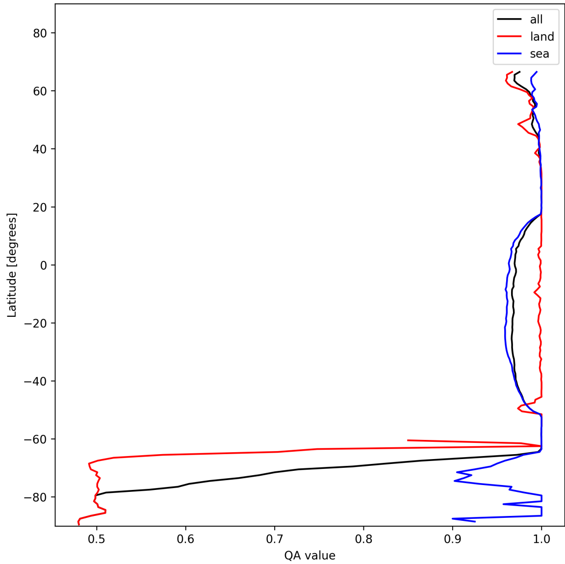
Figure 12: Zonal average of “QA value” for 2024-11-28 to 2024-11-30.
