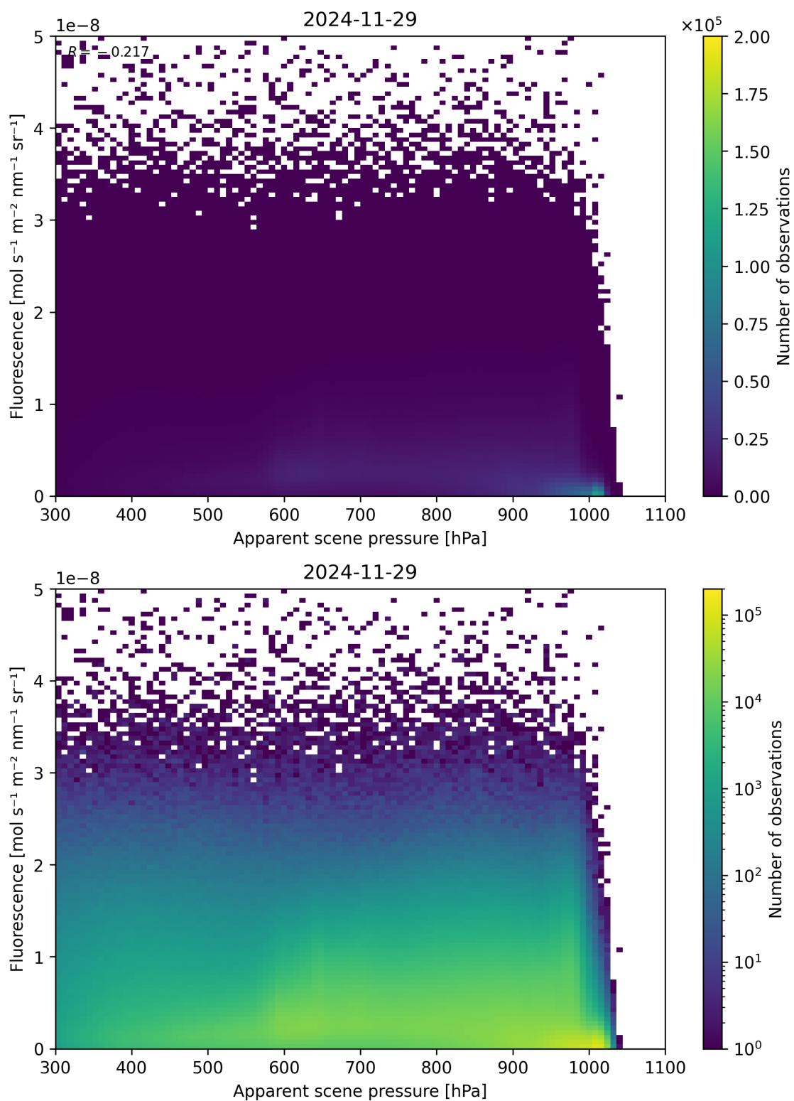
Figure 64: Scatter density plot of “Apparent scene pressure” against “Fluorescence” for 2024-11-28 to 2024-11-30.
