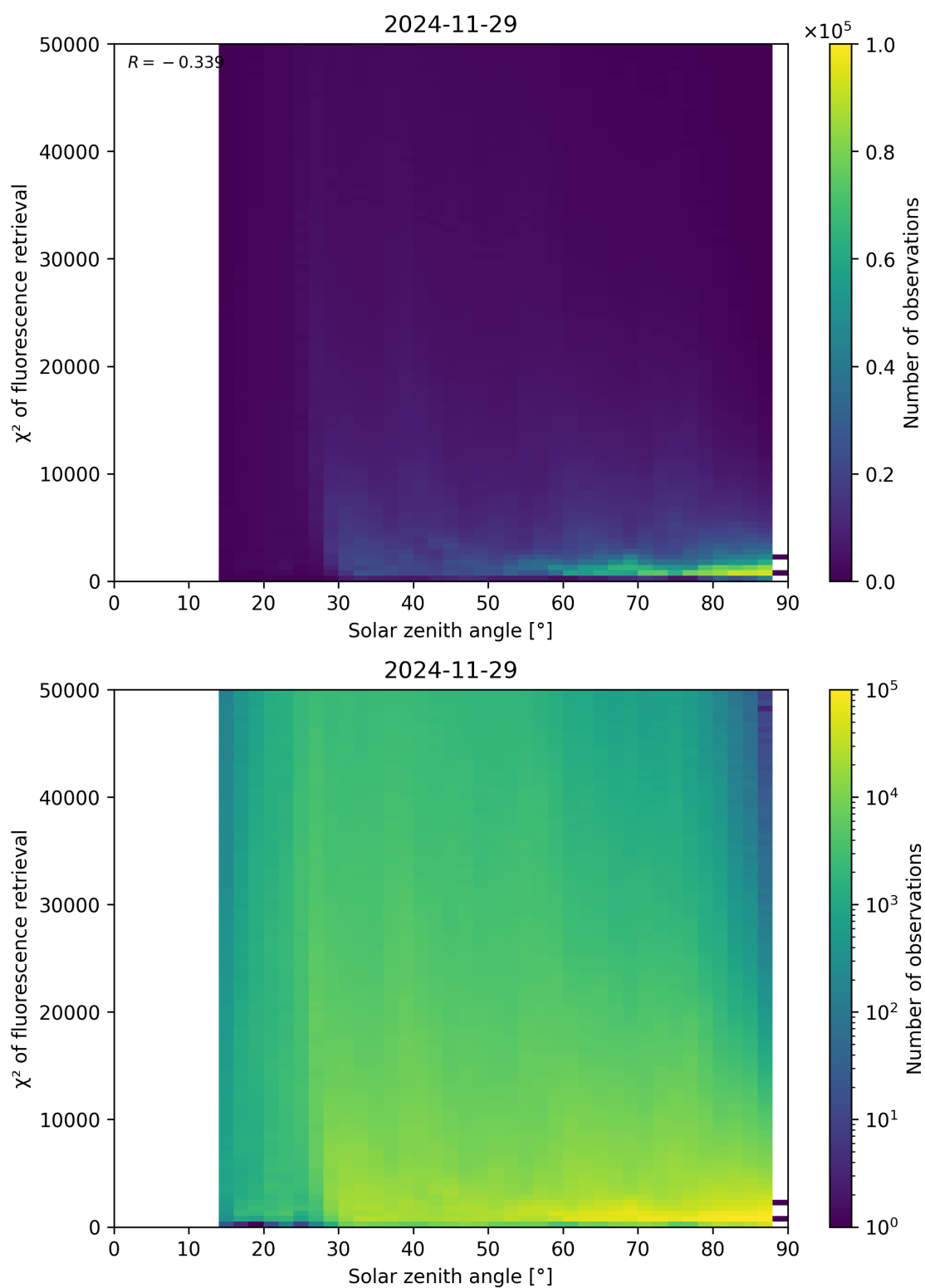
Figure 109: Scatter density plot of “Solar zenith angle” against “ \chi^2 of fluorescence retrieval” for 2024-11-28 to 2024-11-30.
