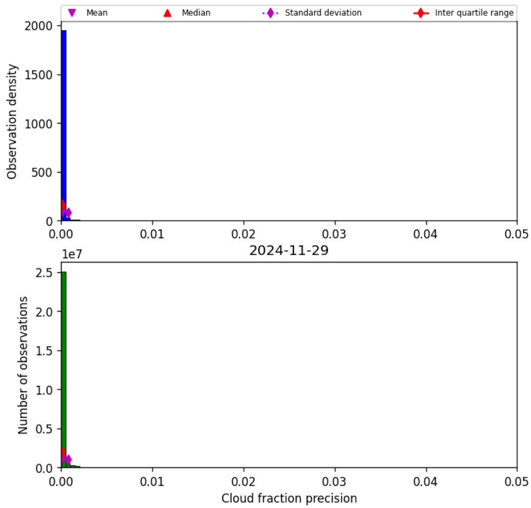
Figure 33: Histogram of “Cloud fraction precision” for 2024-11-28 to 2024-11-30
