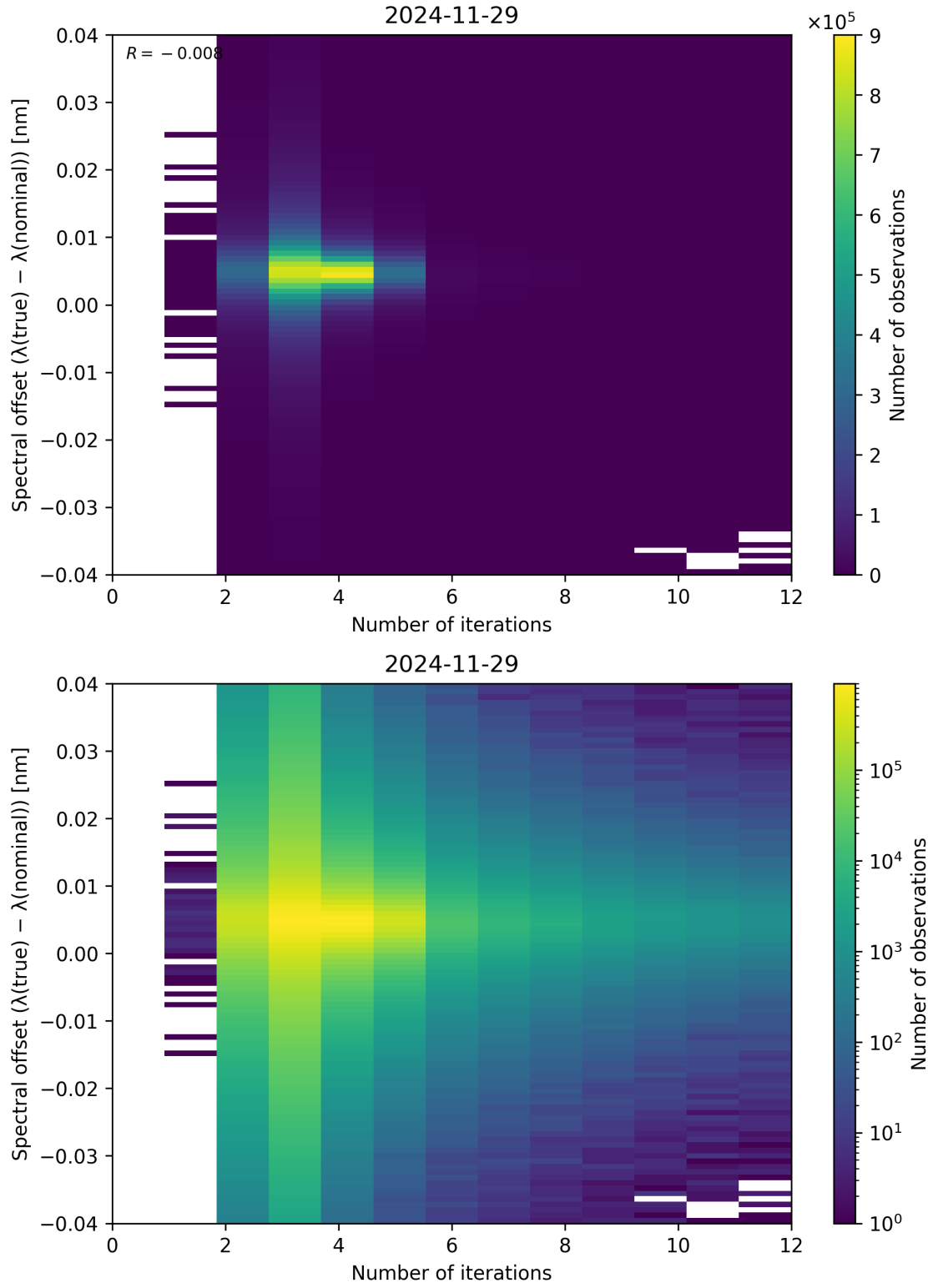
Figure 100: Scatter density plot of “Number of iterations” against “Spectral offset ( \lambda_{\text{true}} - \lambda_{\text{nominal}} )” for 2024-11-28 to 2024-11-30.
