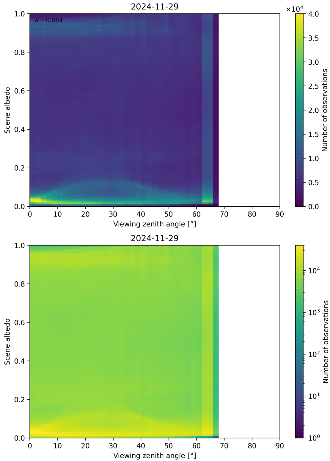
Figure 126: Scatter density plot of “Viewing zenith angle” against “Scene albedo” for 2024-11-28 to 2024-11-30.
