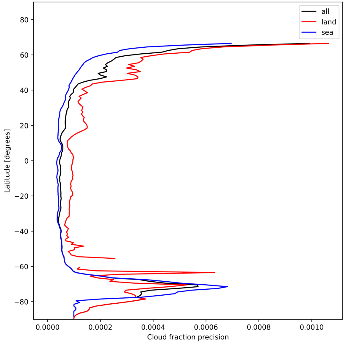
Figure 16: Zonal average of “Cloud fraction precision” for 2024-11-28 to 2024-11-30.
