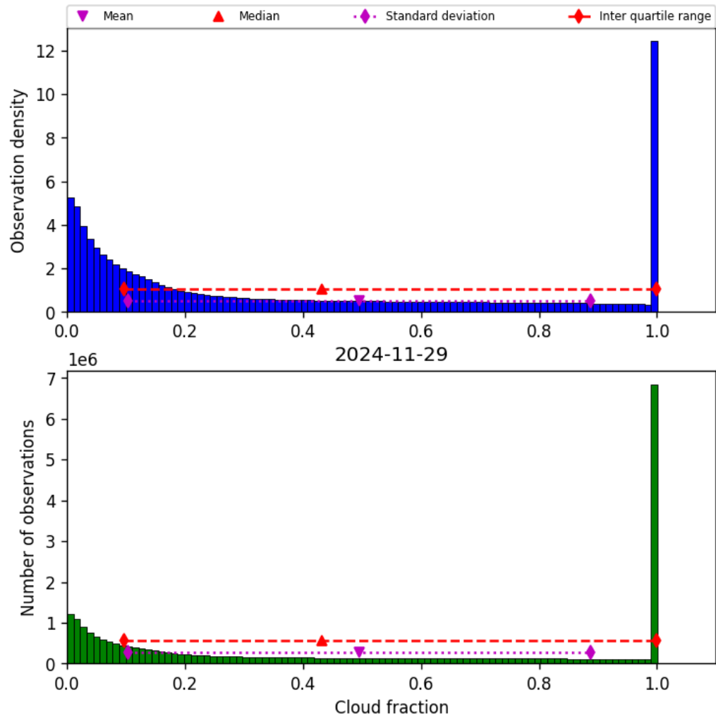
Figure 32: Histogram of “Cloud fraction” for 2024-11-28 to 2024-11-30
