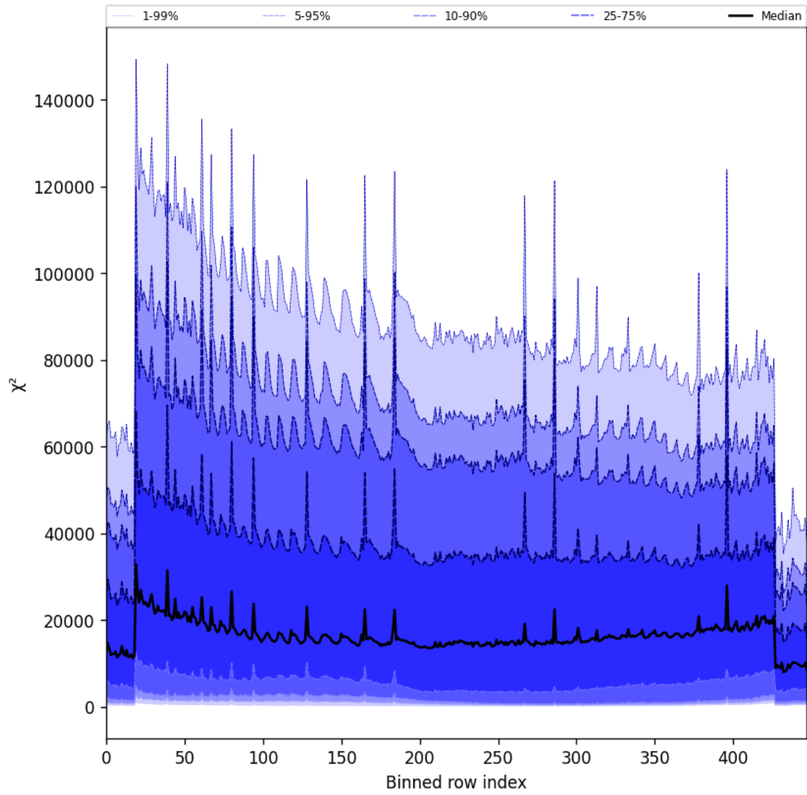
Figure 55: Along track statistics of “ \chi^2 ” for 2024-11-28 to 2024-11-30
