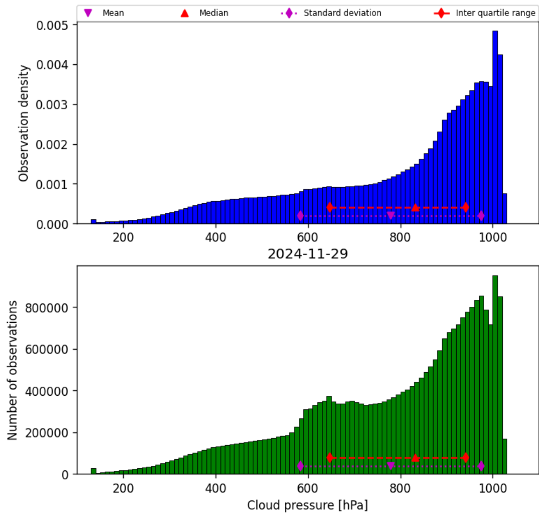
Figure 30: Histogram of “Cloud pressure” for 2024-11-28 to 2024-11-30
