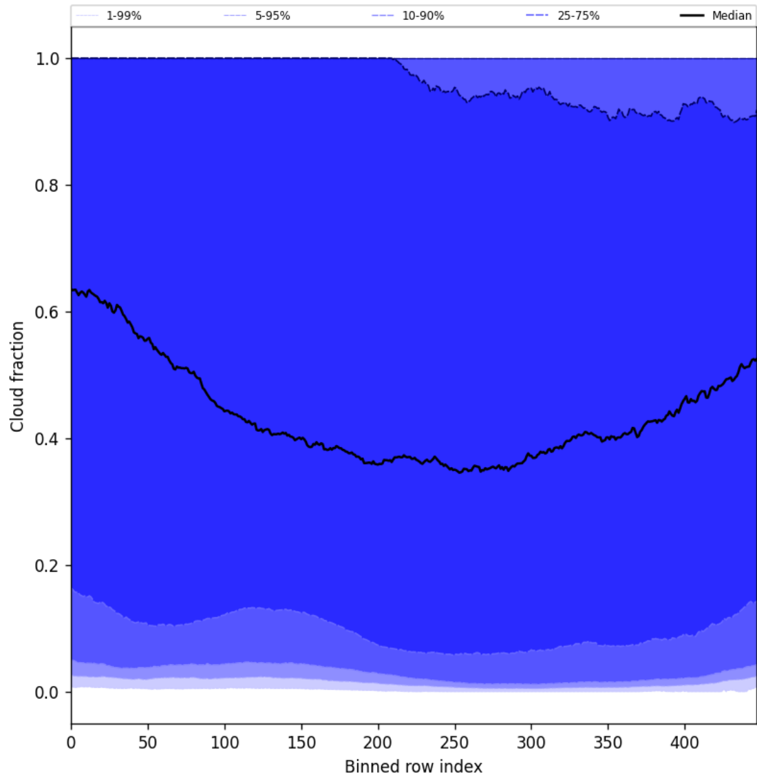
Figure 49: Along track statistics of “Cloud fraction” for 2024-11-28 to 2024-11-30
