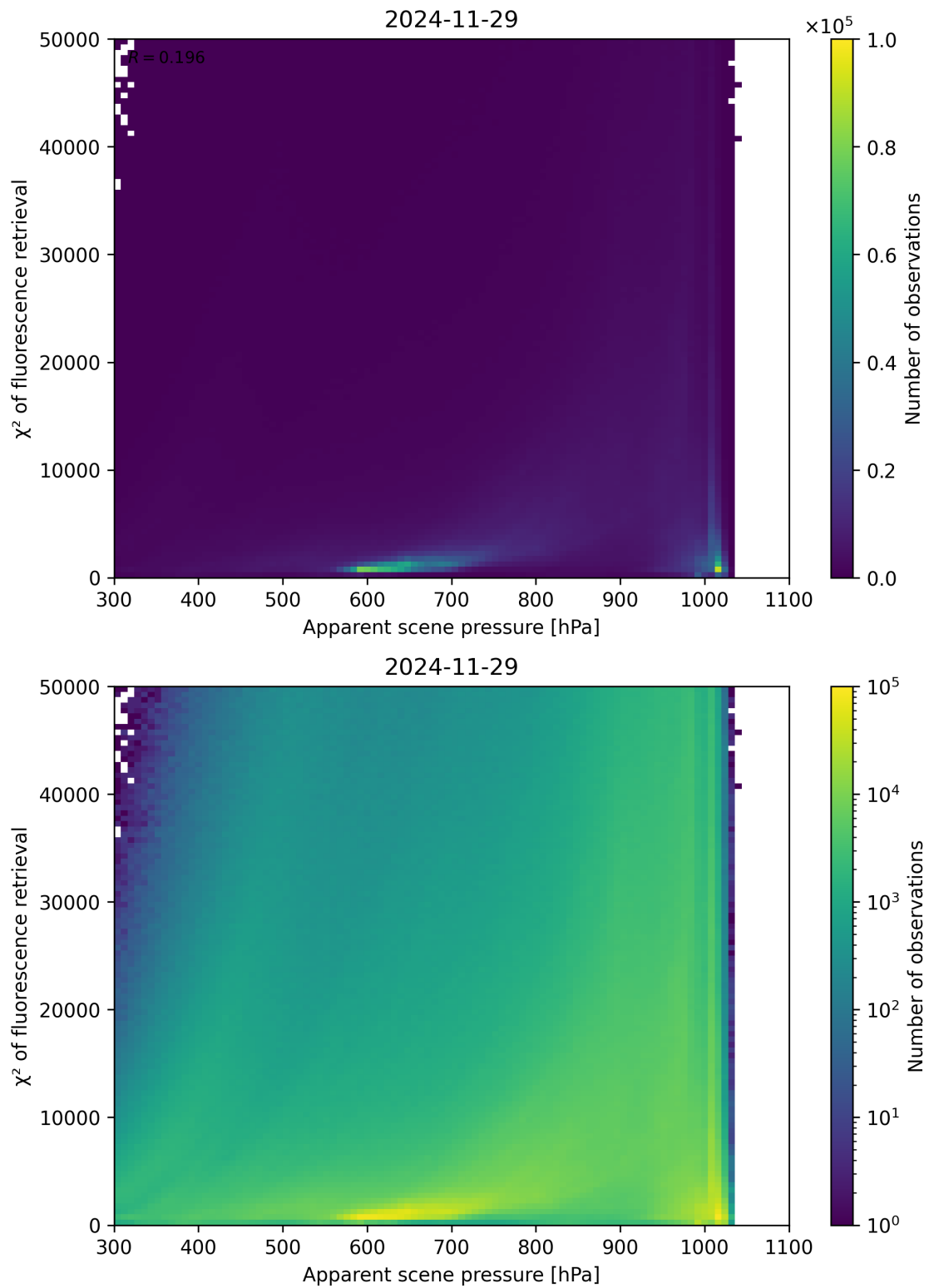
Figure 63: Scatter density plot of “Apparent scene pressure” against “ \chi^2 of fluorescence retrieval” for 2024-11-28 to 2024-11-30.
