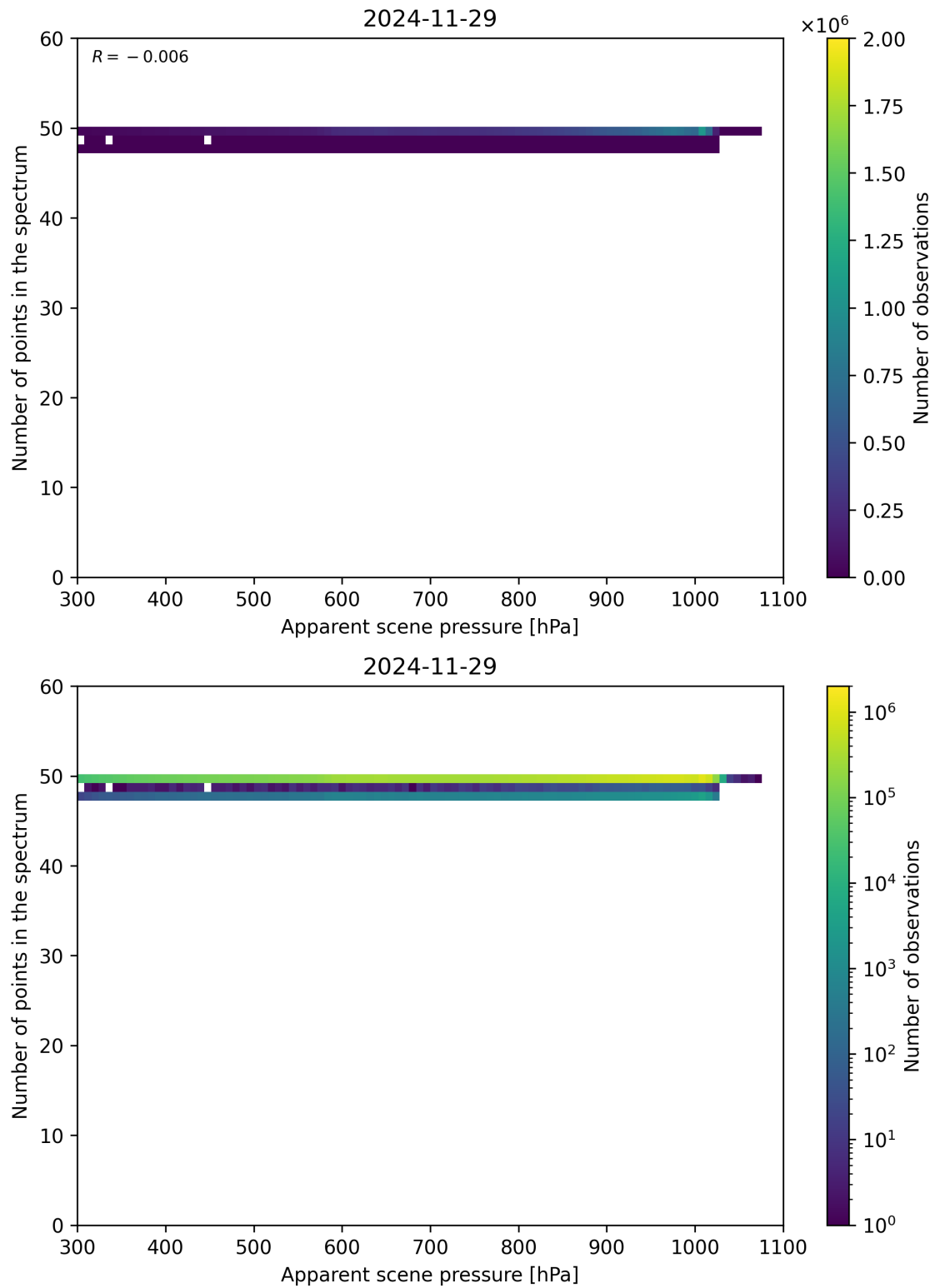
Figure 66: Scatter density plot of “Apparent scene pressure” against “Number of points in the spectrum” for 2024-11-28 to 2024-11-30.
