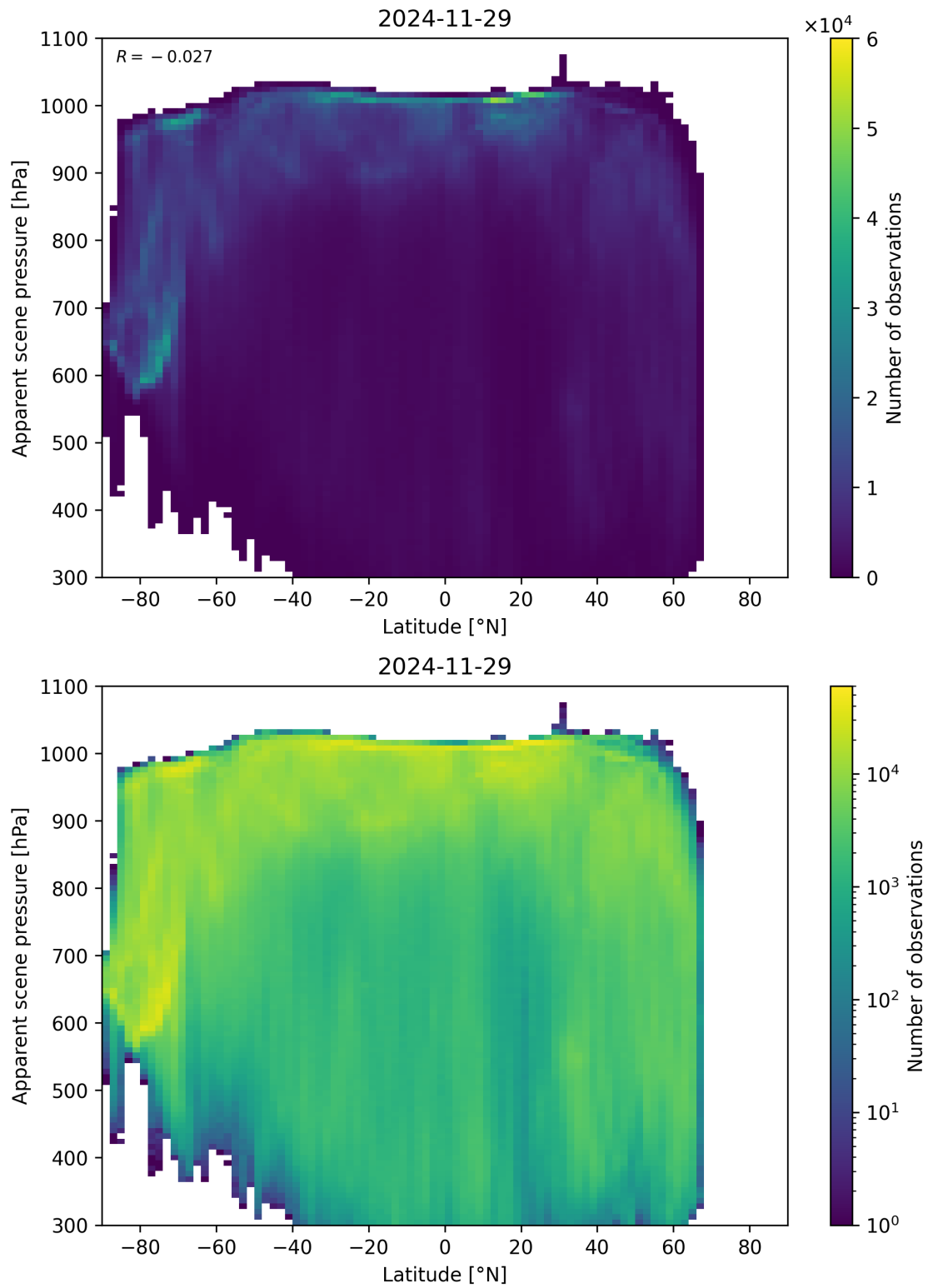
Figure 88: Scatter density plot of “Latitude” against “Apparent scene pressure” for 2024-11-28 to 2024-11-30.
