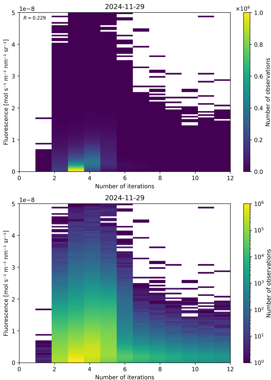
Figure 98: Scatter density plot of “Number of iterations” against “Fluorescence” for 2024-11-28 to 2024-11-30.
