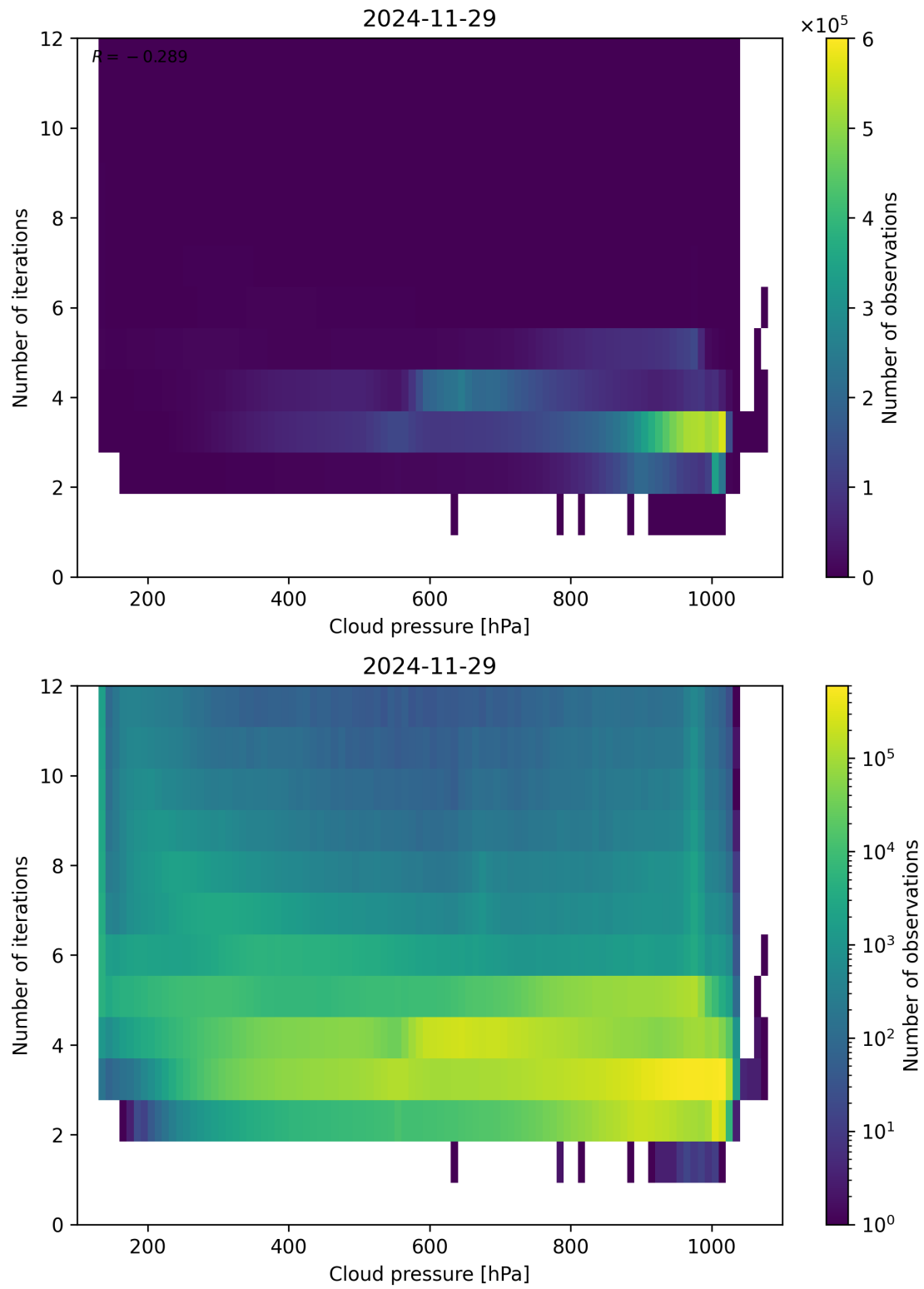
Figure 81: Scatter density plot of “Cloud pressure” against “Number of iterations” for 2024-11-28 to 2024-11-30.
