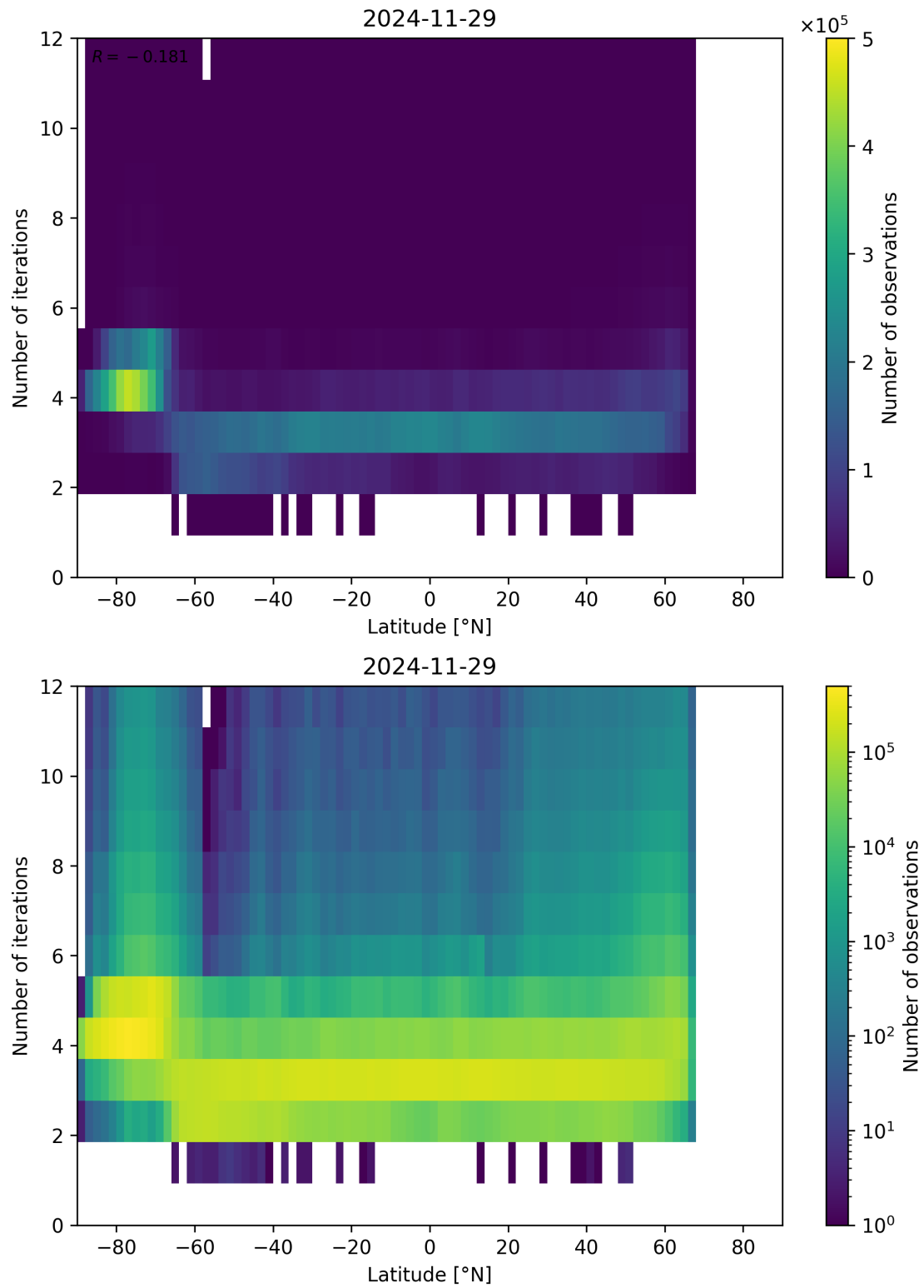
Figure 93: Scatter density plot of “Latitude” against “Number of iterations” for 2024-11-28 to 2024-11-30.
