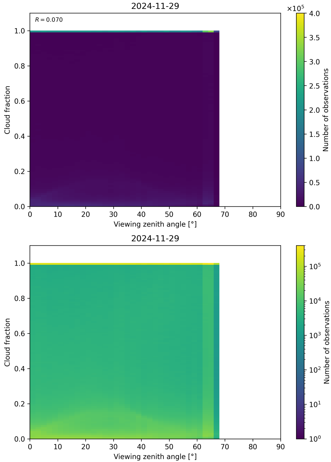
Figure 120: Scatter density plot of “Viewing zenith angle” against “Cloud fraction” for 2024-11-28 to 2024-11-30.
