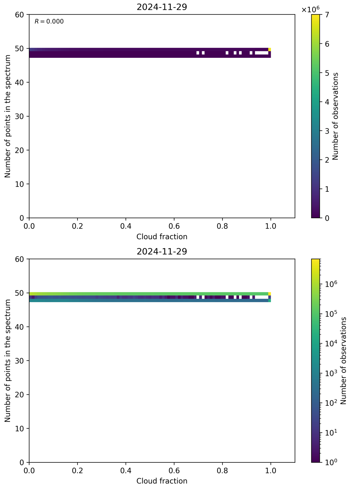
Figure 74: Scatter density plot of “Cloud fraction” against “Number of points in the spectrum” for 2024-11-28 to 2024-11-30.
