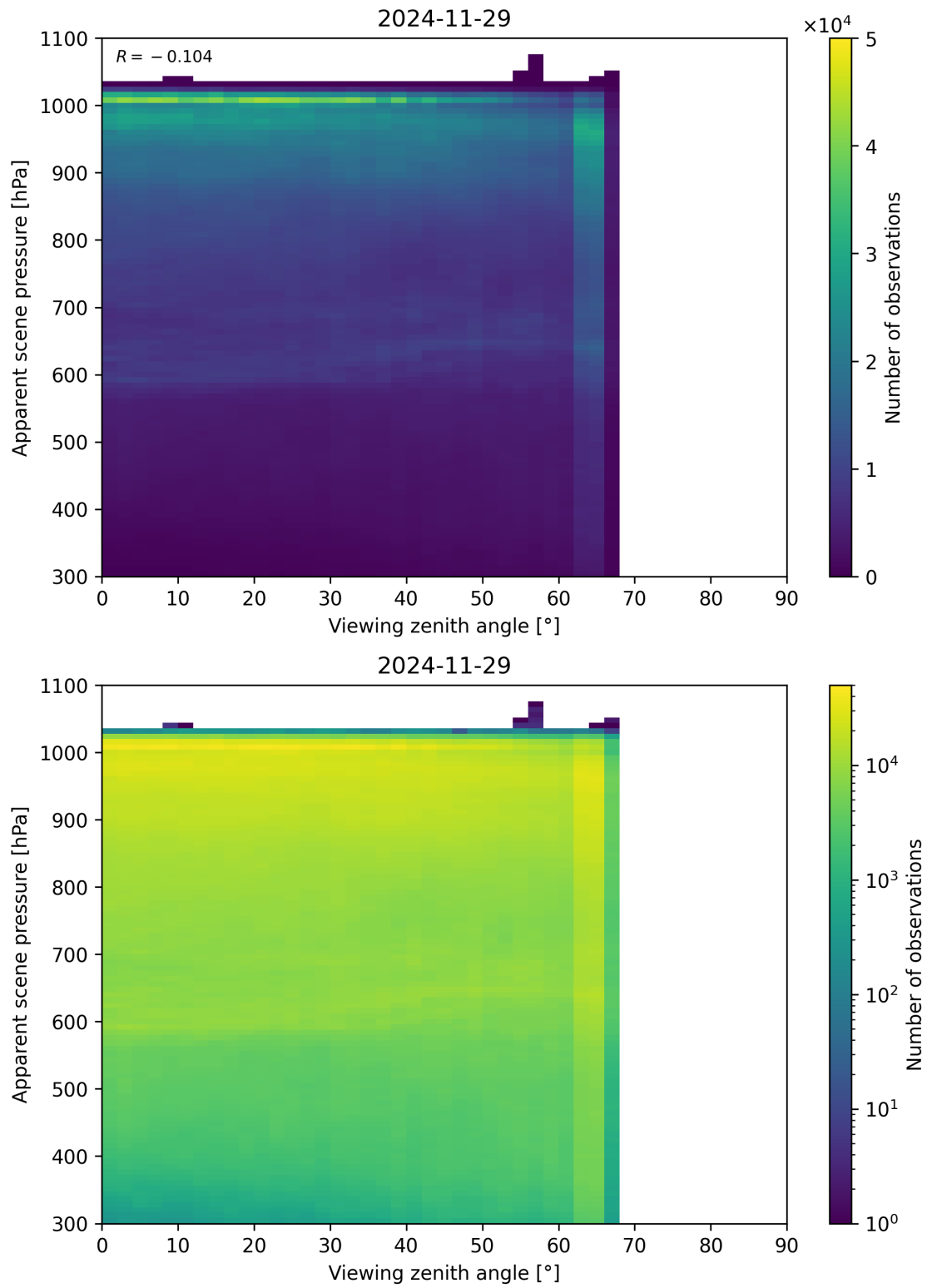
Figure 118: Scatter density plot of “Viewing zenith angle” against “Apparent scene pressure” for 2024-11-28 to 2024-11-30.
