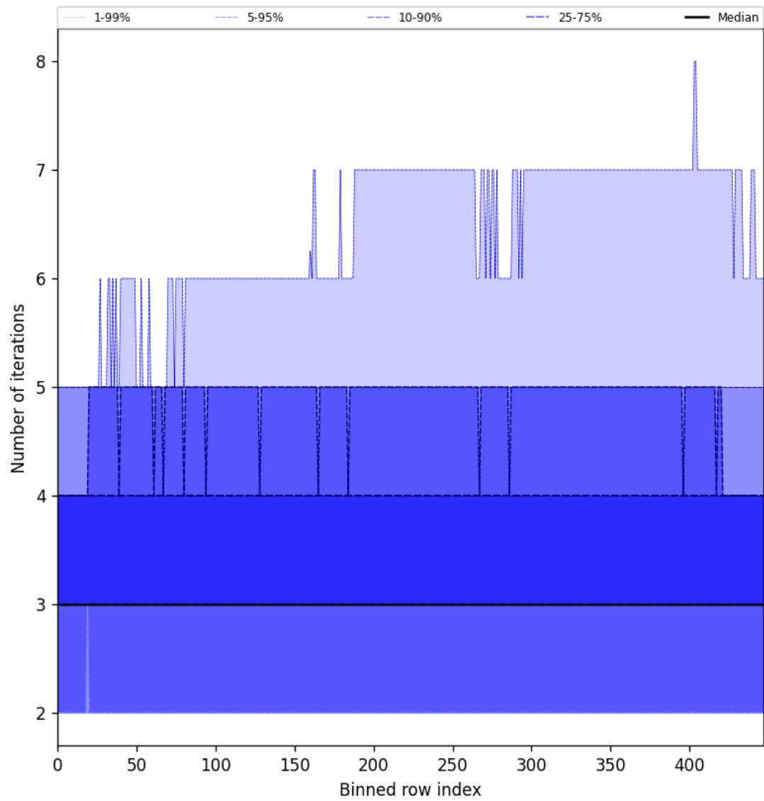
Figure 56: Along track statistics of “Number of iterations” for 2024-11-28 to 2024-11-30
