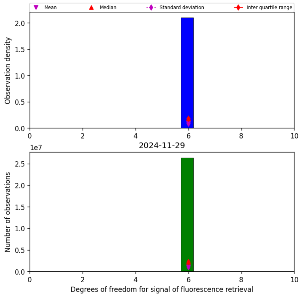
Figure 43: Histogram of “Degrees of freedom for signal of fluorescence retrieval” for 2024-11-28 to 2024-11-30
