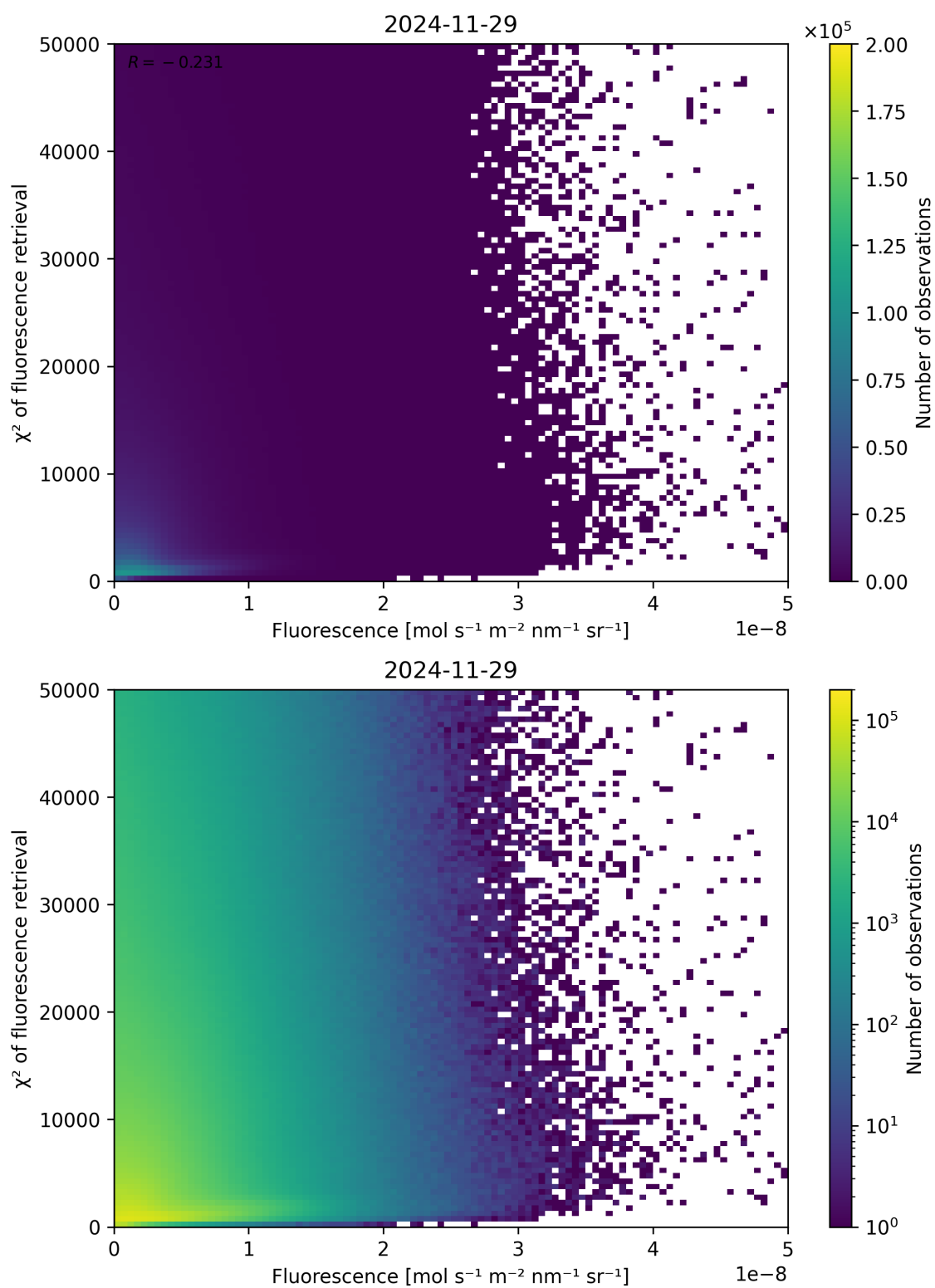
Figure 85: Scatter density plot of “Fluorescence” against “ \chi^2 of fluorescence retrieval” for 2024-11-28 to 2024-11-30.
