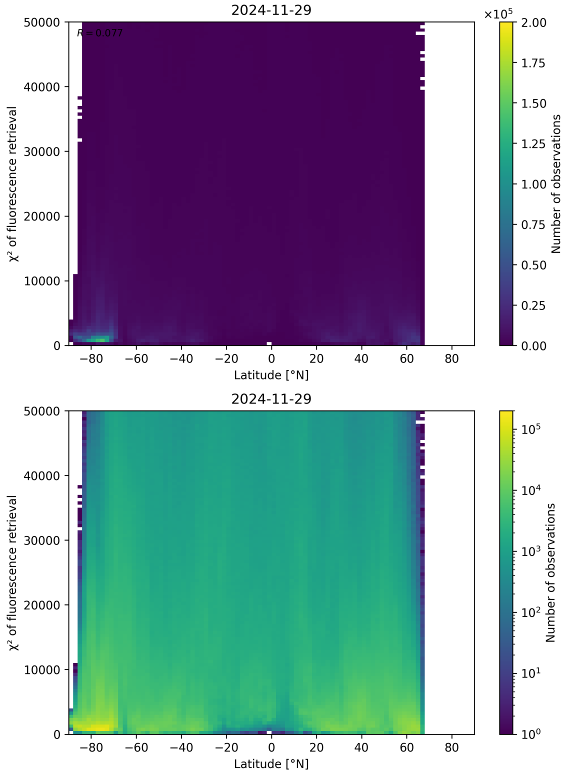
Figure 89: Scatter density plot of “Latitude” against “ \chi^2 of fluorescence retrieval” for 2024-11-28 to 2024-11-30.
