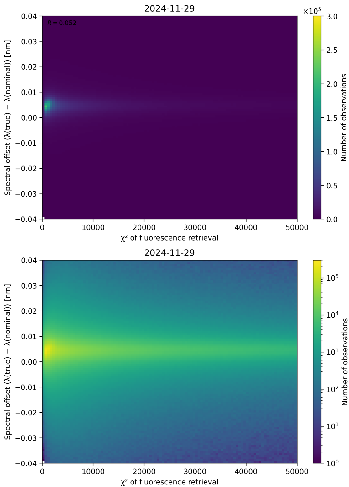
Figure 69: Scatter density plot of “ \chi^2 of fluorescence retrieval” against “Spectral offset ( \lambda_{\text{true}} - \lambda_{\text{nominal}} )” for 2024-11-28 to 2024-11-30.
