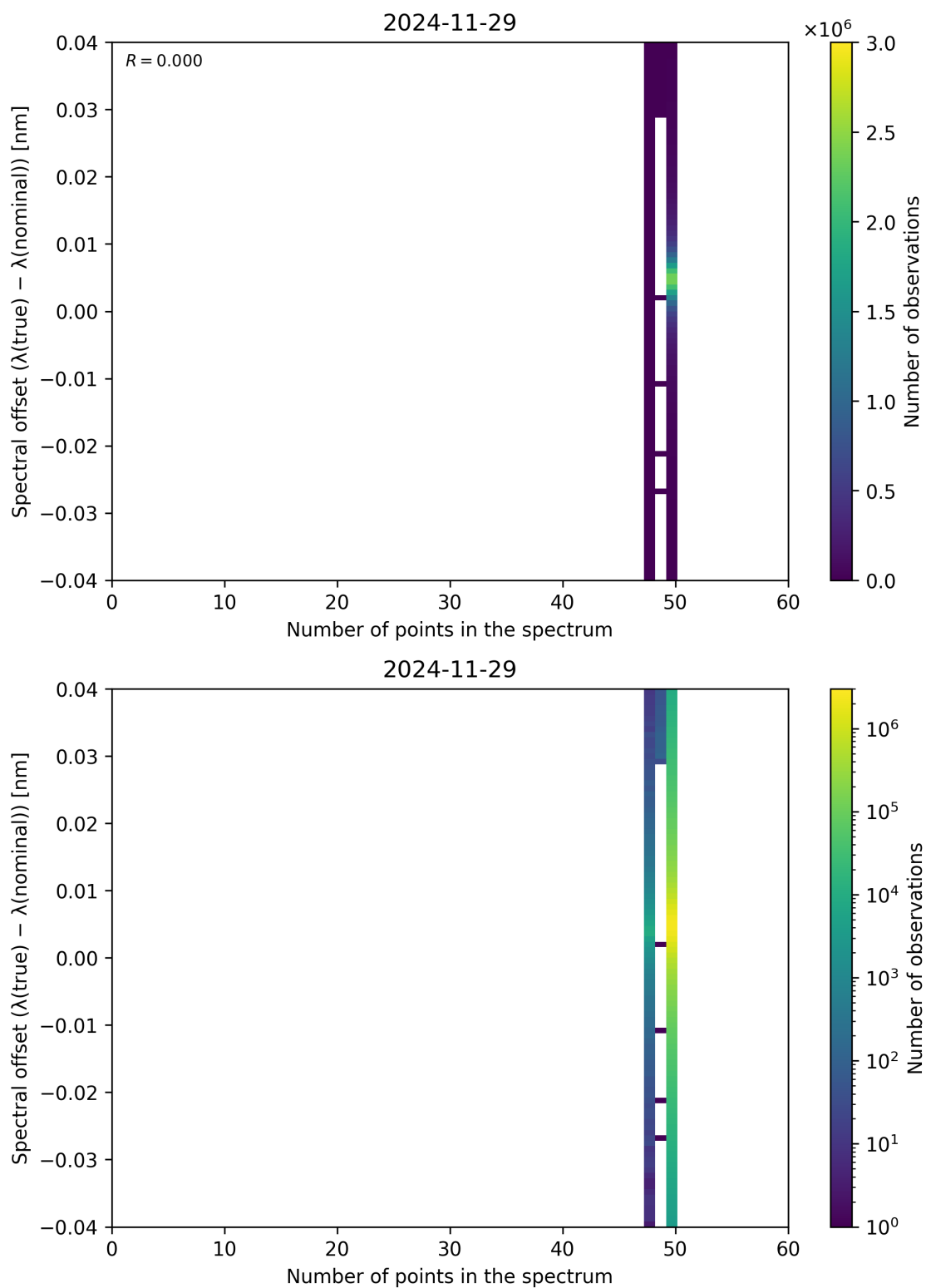
Figure 101: Scatter density plot of “Number of points in the spectrum” against “Spectral offset ( \lambda_{\text{true}} - \lambda_{\text{nominal}} )” for 2024-11-28 to 2024-11-30.
