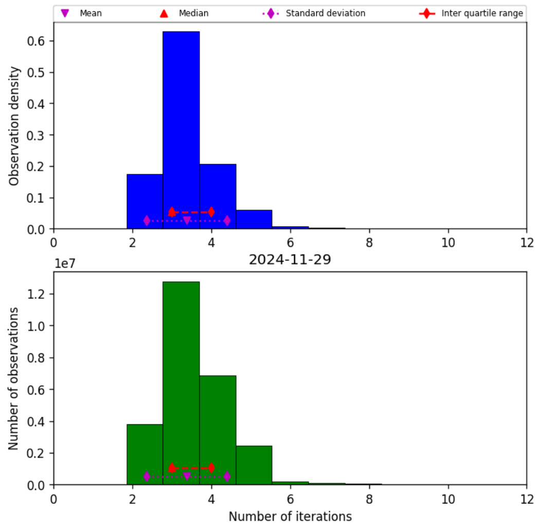
Figure 39: Histogram of “Number of iterations” for 2024-11-28 to 2024-11-30
