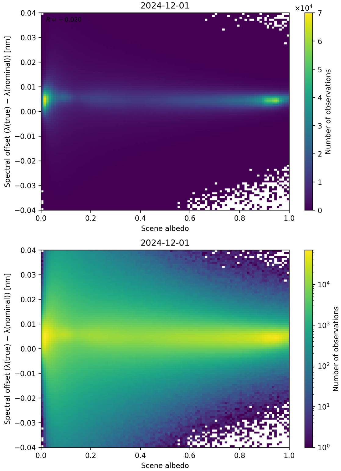
Figure 107: Scatter density plot of “Scene albedo” against “Spectral offset ( \lambda_{\text{true}} - \lambda_{\text{nominal}} )” for 2024-11-30 to 2024-12-02.
