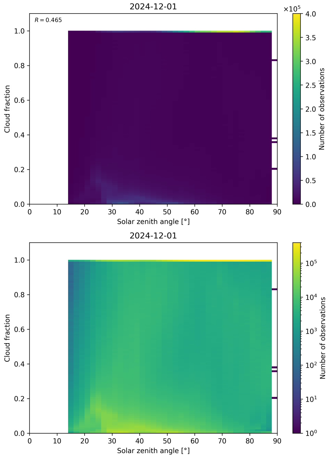
Figure 110: Scatter density plot of “Solar zenith angle” against “Cloud fraction” for 2024-11-30 to 2024-12-02.
