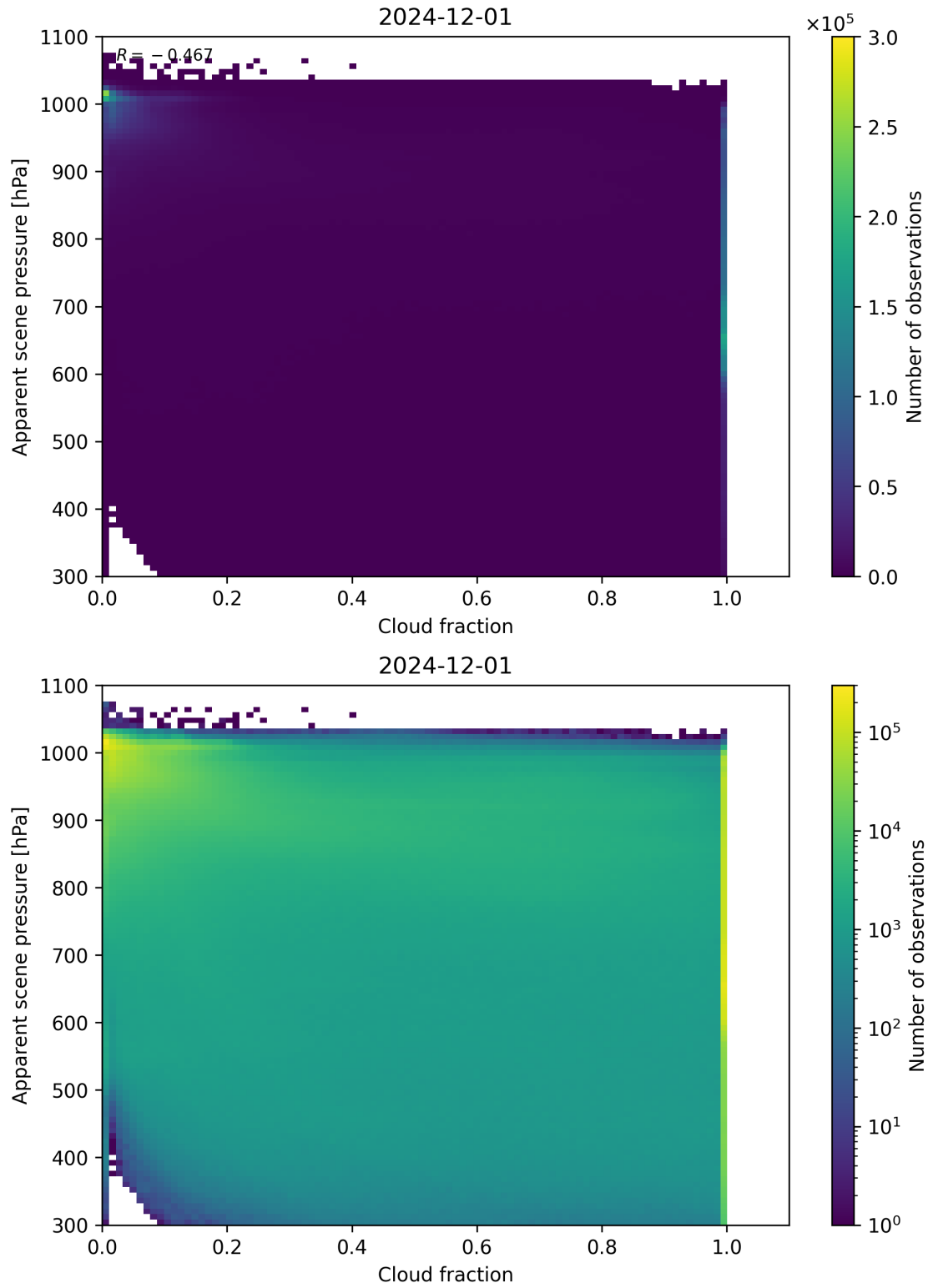
Figure 70: Scatter density plot of “Cloud fraction” against “Apparent scene pressure” for 2024-11-30 to 2024-12-02.
