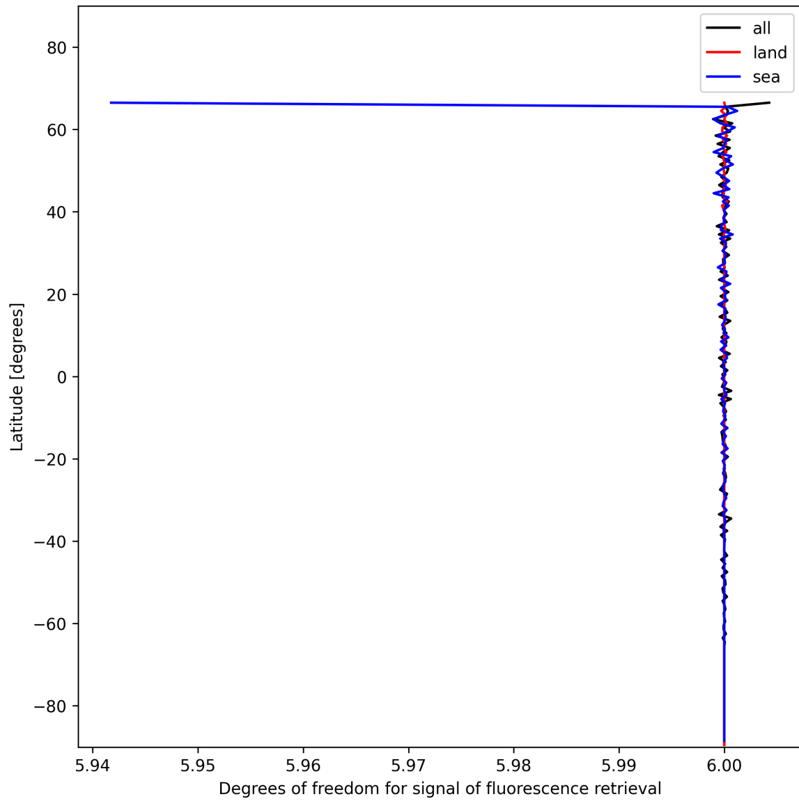
Figure 26: Zonal average of “Degrees of freedom for signal of fluorescence retrieval” for 2024-11-30 to 2024-12-02.
