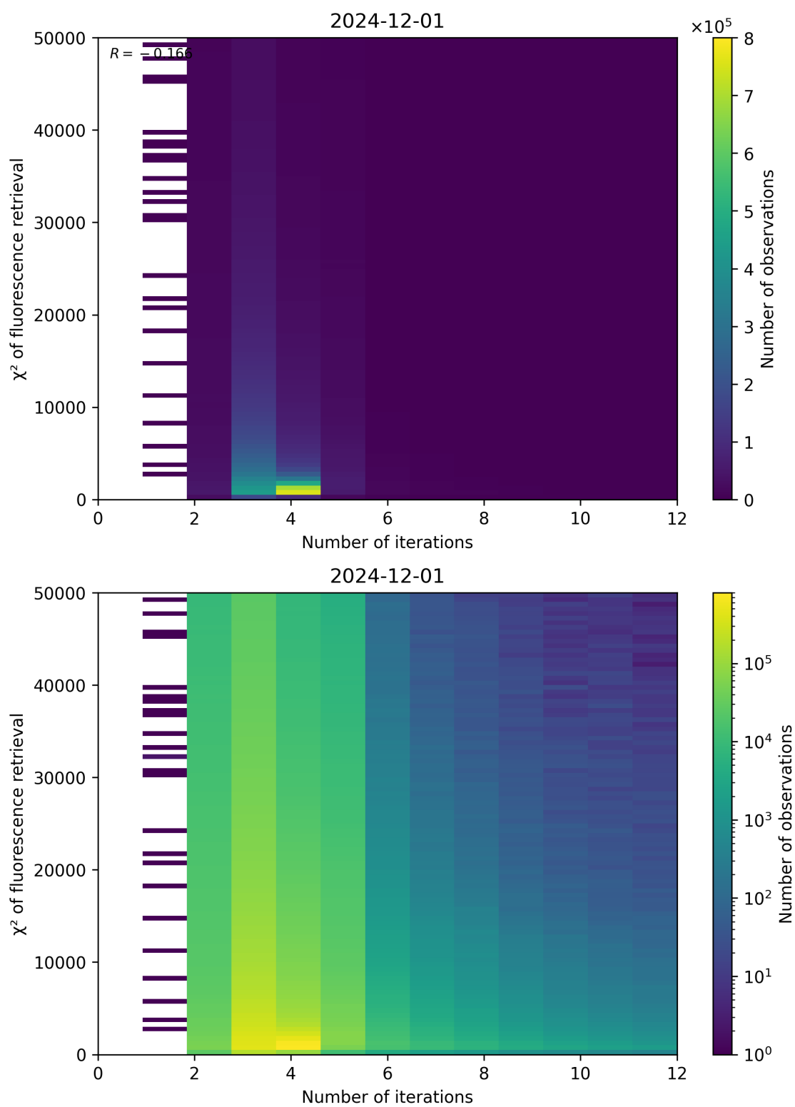
Figure 97: Scatter density plot of “Number of iterations” against “ \chi^2 of fluorescence retrieval” for 2024-11-30 to 2024-12-02.
