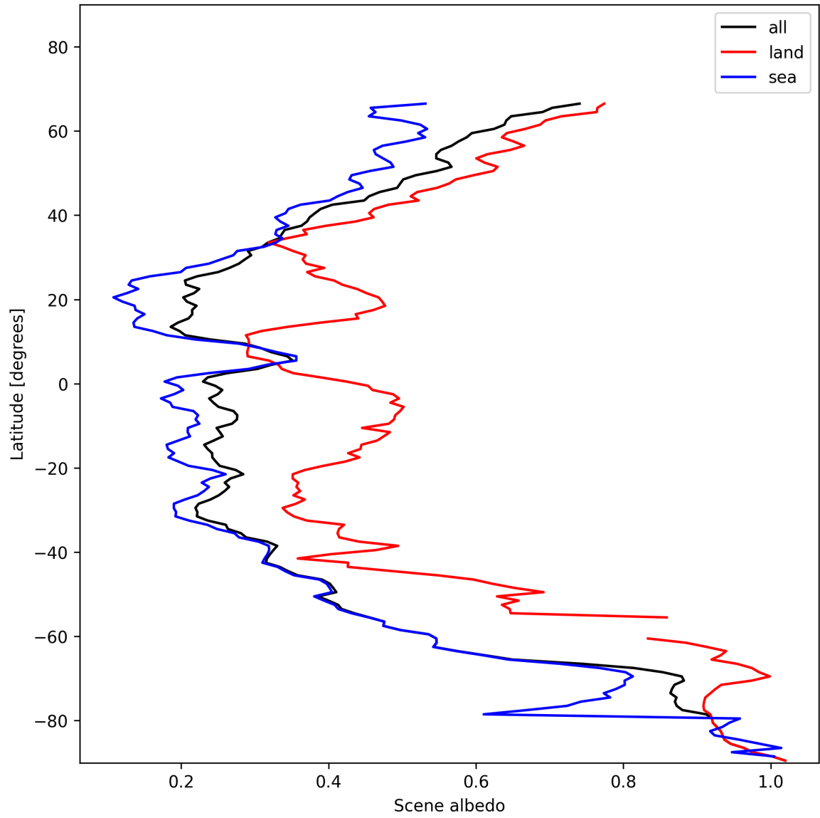
Figure 17: Zonal average of “Scene albedo” for 2024-11-30 to 2024-12-02.
