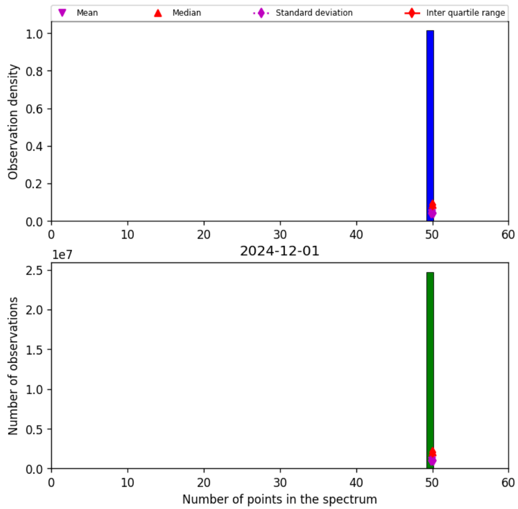
Figure 44: Histogram of “Number of points in the spectrum” for 2024-11-30 to 2024-12-02
