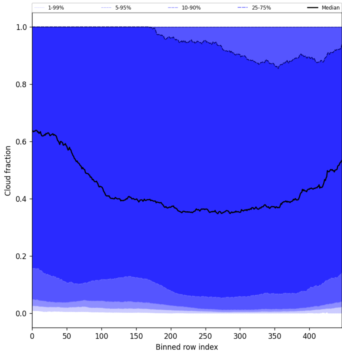
Figure 49: Along track statistics of “Cloud fraction” for 2024-11-30 to 2024-12-02
