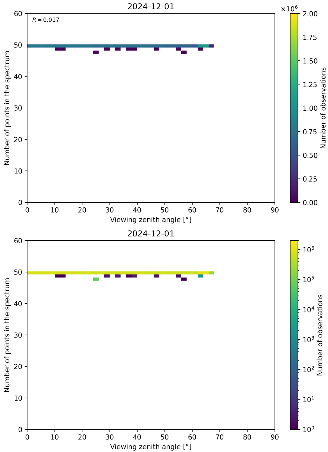
Figure 125: Scatter density plot of “Viewing zenith angle” against “Number of points in the spectrum” for 2024-11-30 to 2024-12-02.
