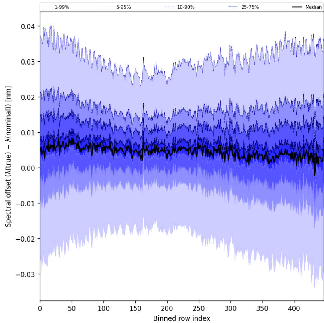
Figure 62: Along track statistics of “Spectral offset ( \lambda_{\text{true}} - \lambda_{\text{nominal}} )” for 2024-11-30 to 2024-12-02
