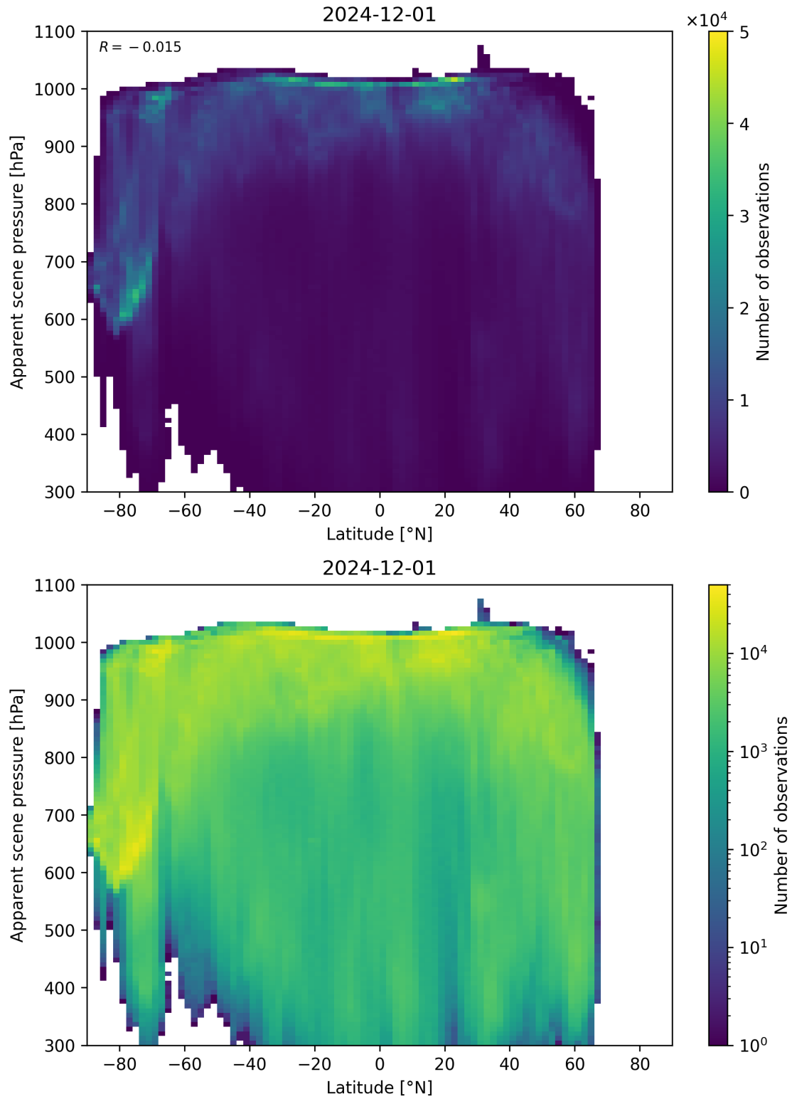
Figure 88: Scatter density plot of “Latitude” against “Apparent scene pressure” for 2024-11-30 to 2024-12-02.
