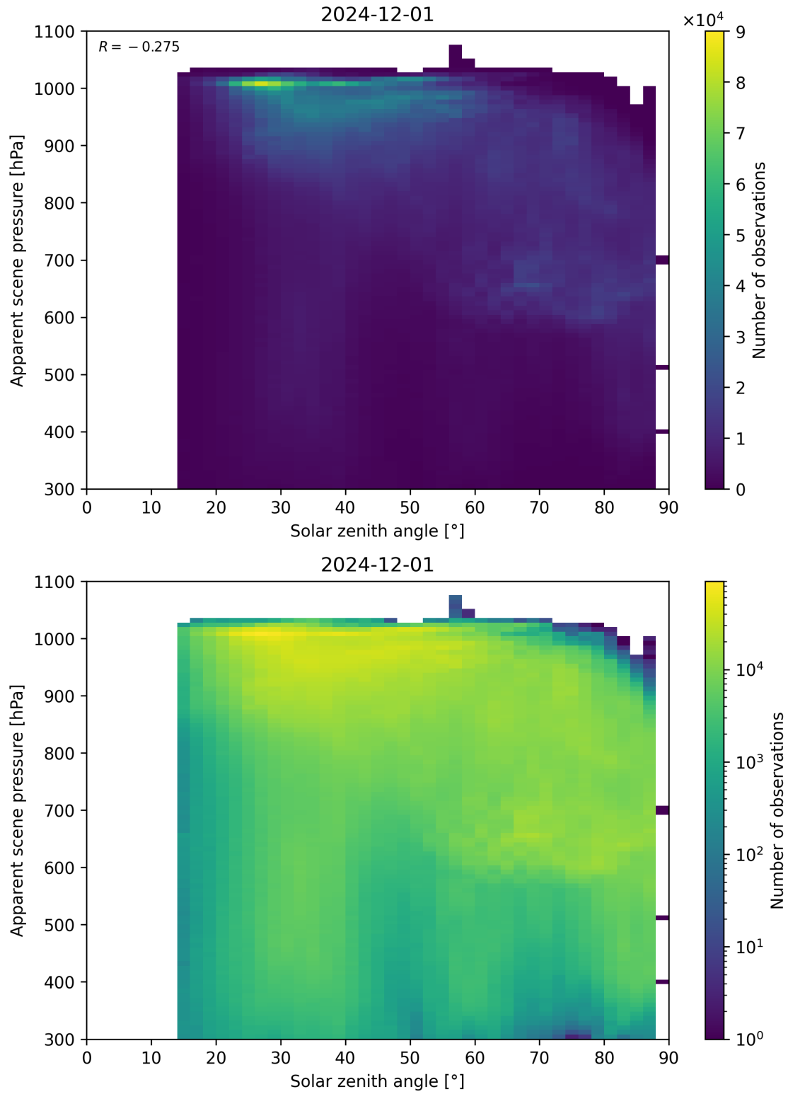
Figure 108: Scatter density plot of “Solar zenith angle” against “Apparent scene pressure” for 2024-11-30 to 2024-12-02.
