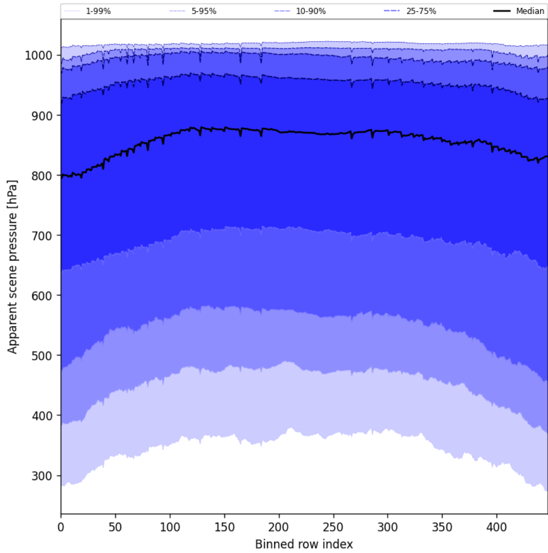
Figure 53: Along track statistics of “Apparent scene pressure” for 2024-11-30 to 2024-12-02
