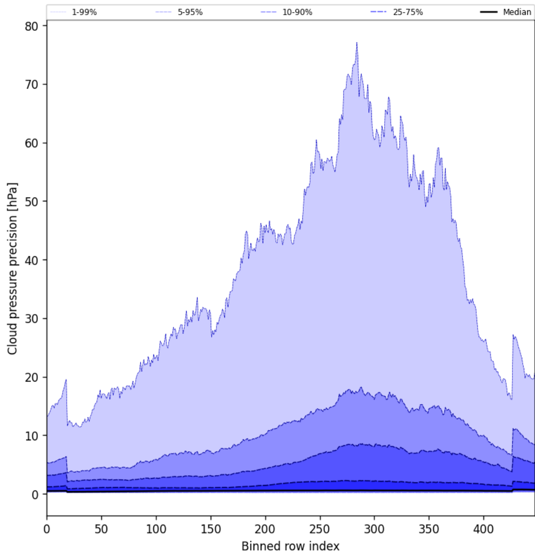
Figure 48: Along track statistics of “Cloud pressure precision” for 2024-11-30 to 2024-12-02
