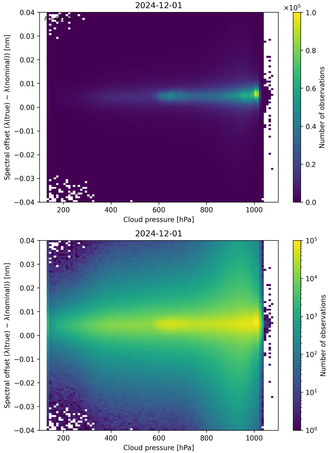
Figure 84: Scatter density plot of “Cloud pressure” against “Spectral offset ( \lambda_{\text{true}} - \lambda_{\text{nominal}} )” for 2024-11-30 to 2024-12-02.
