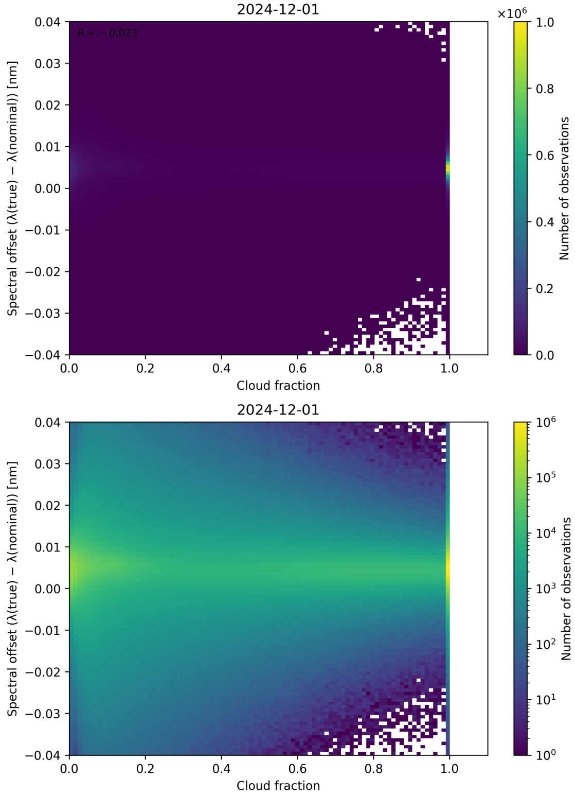
Figure 76: Scatter density plot of “Cloud fraction” against “Spectral offset ( \lambda_{\text{true}} - \lambda_{\text{nominal}} )” for 2024-11-30 to 2024-12-02.
