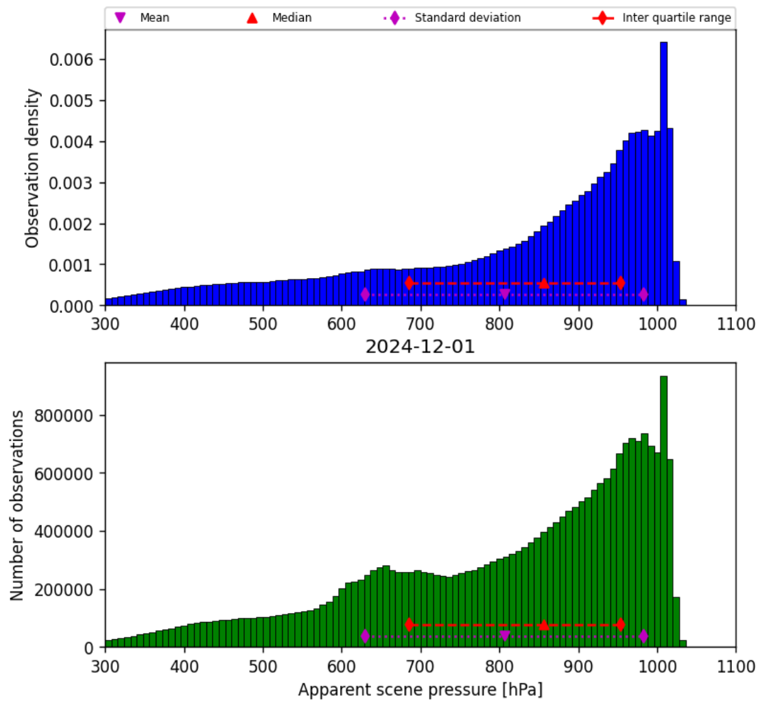
Figure 36: Histogram of “Apparent scene pressure” for 2024-11-30 to 2024-12-02
