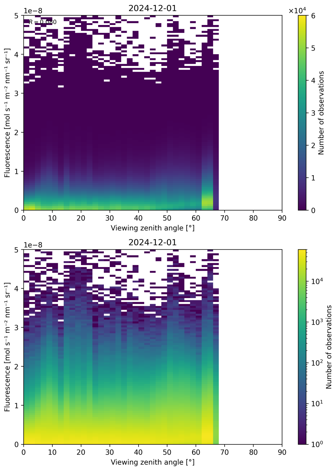
Figure 122: Scatter density plot of “Viewing zenith angle” against “Fluorescence” for 2024-11-30 to 2024-12-02.
