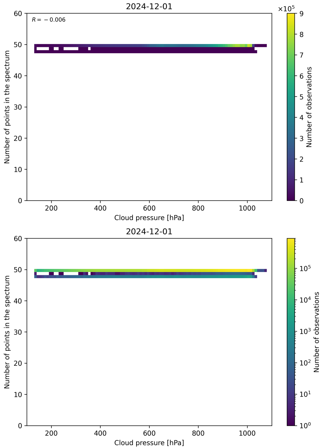
Figure 82: Scatter density plot of “Cloud pressure” against “Number of points in the spectrum” for 2024-11-30 to 2024-12-02.
