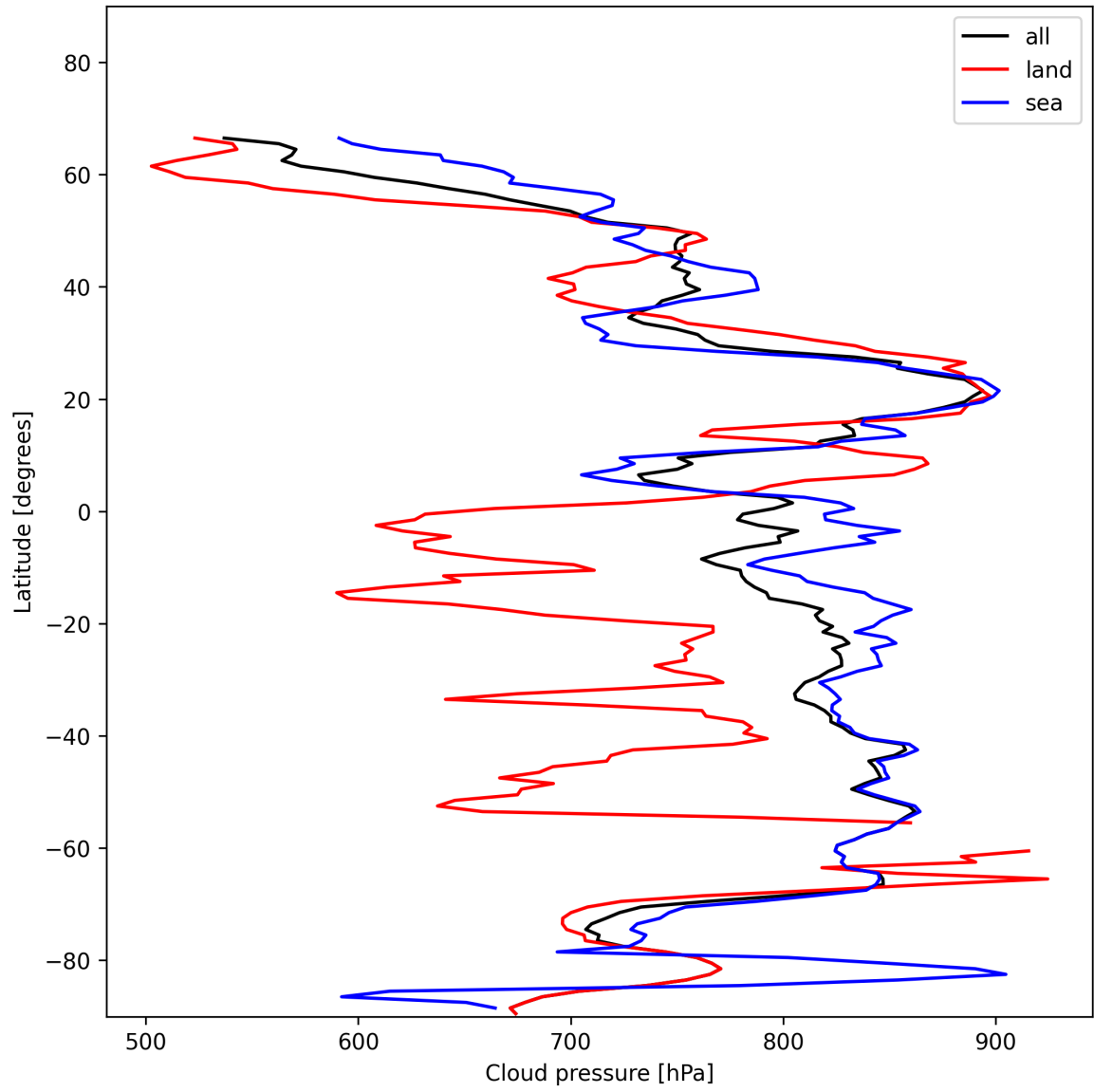
Figure 13: Zonal average of “Cloud pressure” for 2024-11-30 to 2024-12-02.
