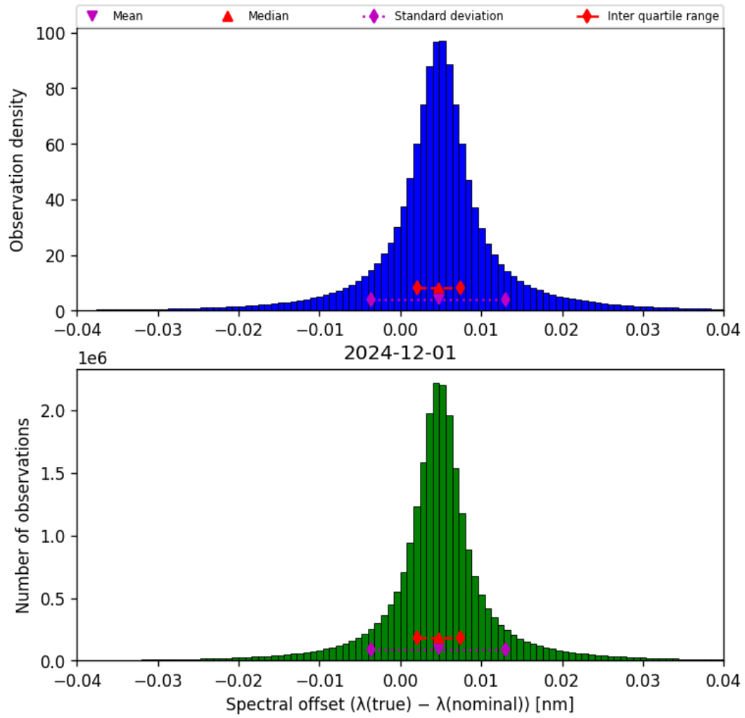
Figure 45: Histogram of “Spectral offset ( \lambda_{\text{true}} - \lambda_{\text{nominal}} )” for 2024-11-30 to 2024-12-02
