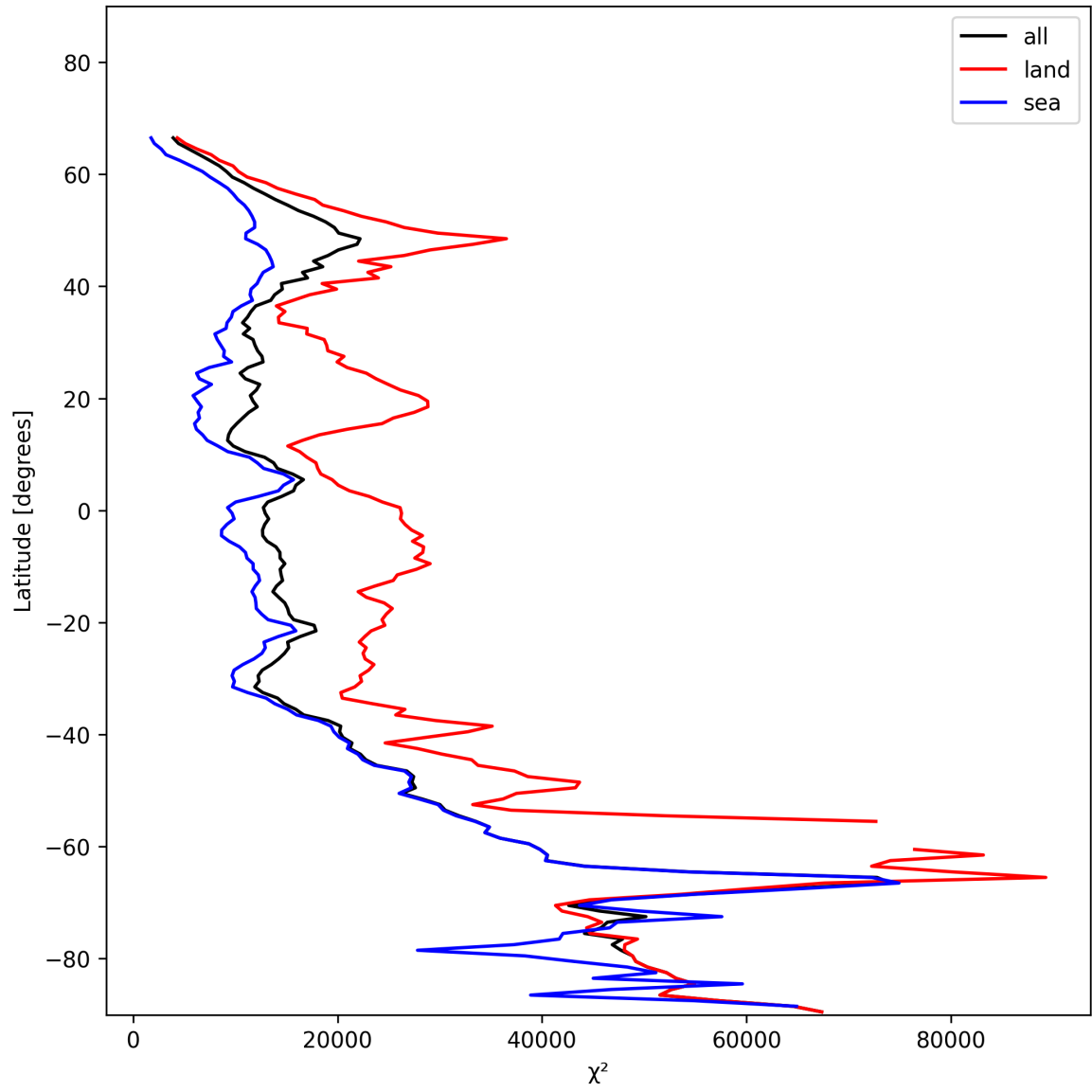
Figure 21: Zonal average of “ \chi^2 ” for 2024-11-30 to 2024-12-02.
