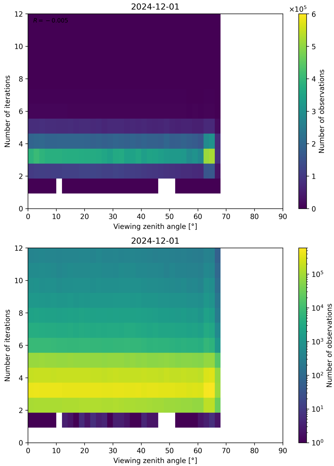
Figure 124: Scatter density plot of “Viewing zenith angle” against “Number of iterations” for 2024-11-30 to 2024-12-02.
