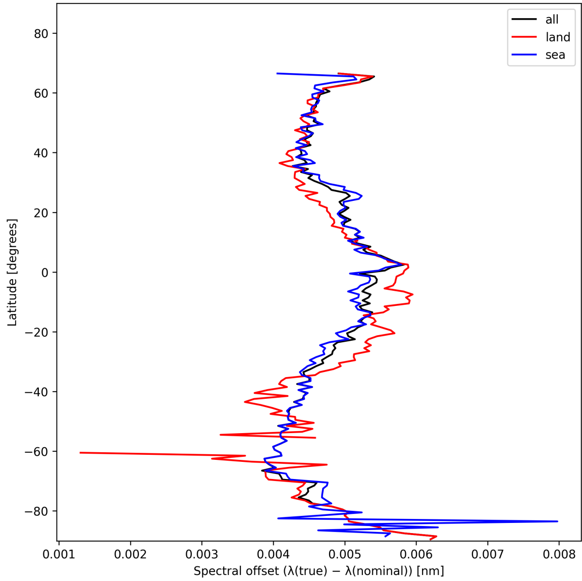
Figure 28: Zonal average of “Spectral offset ( \lambda_{\text{true}} - \lambda_{\text{nominal}} )” for 2024-11-30 to 2024-12-02.
