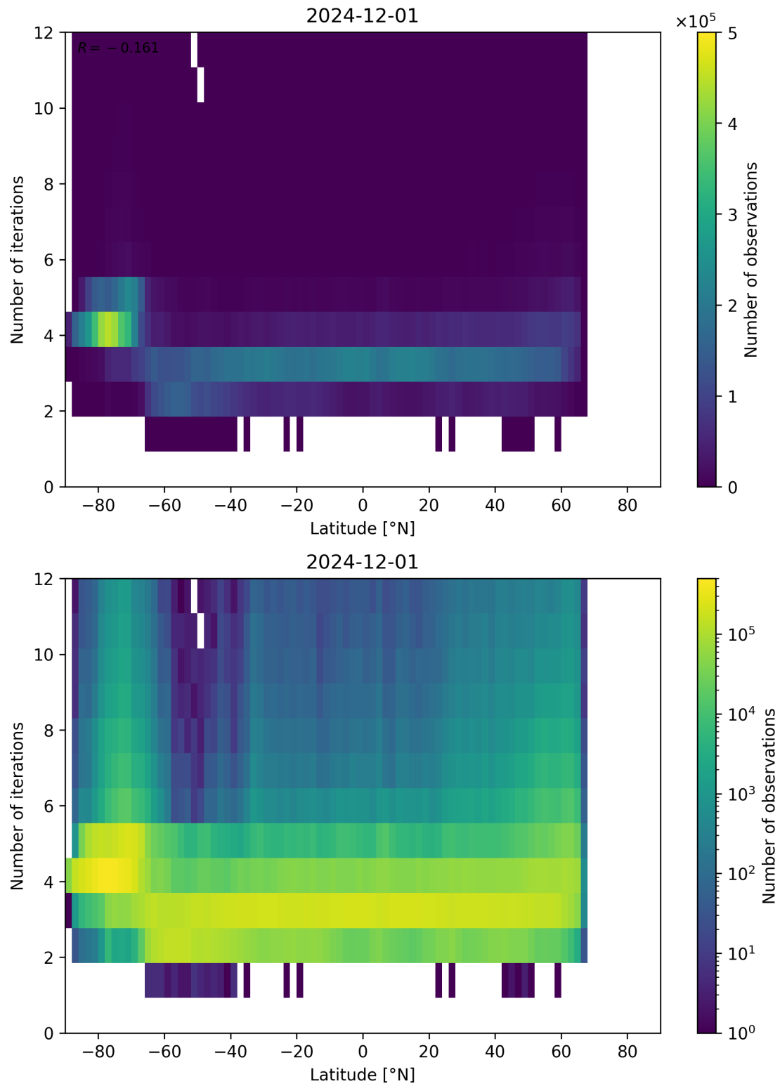
Figure 93: Scatter density plot of “Latitude” against “Number of iterations” for 2024-11-30 to 2024-12-02.
