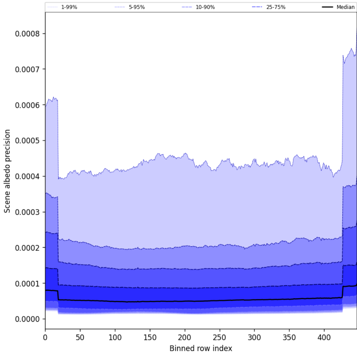
Figure 52: Along track statistics of “Scene albedo precision” for 2024-11-30 to 2024-12-02
