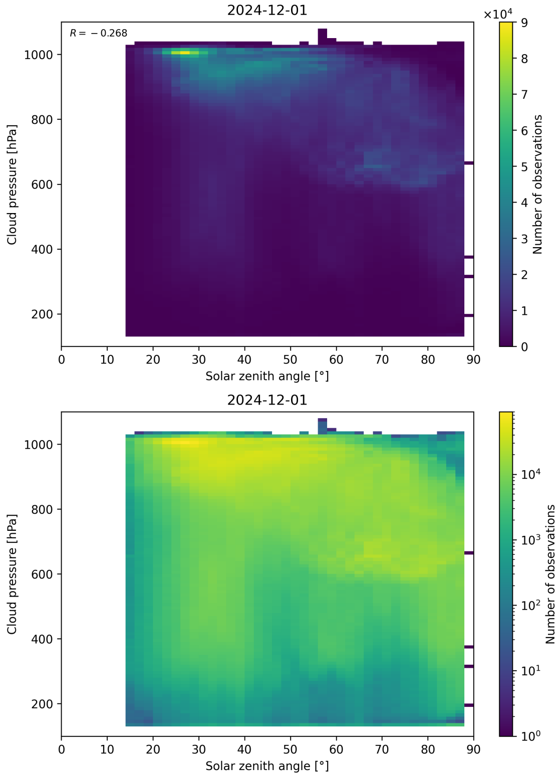
Figure 111: Scatter density plot of “Solar zenith angle” against “Cloud pressure” for 2024-11-30 to 2024-12-02.
