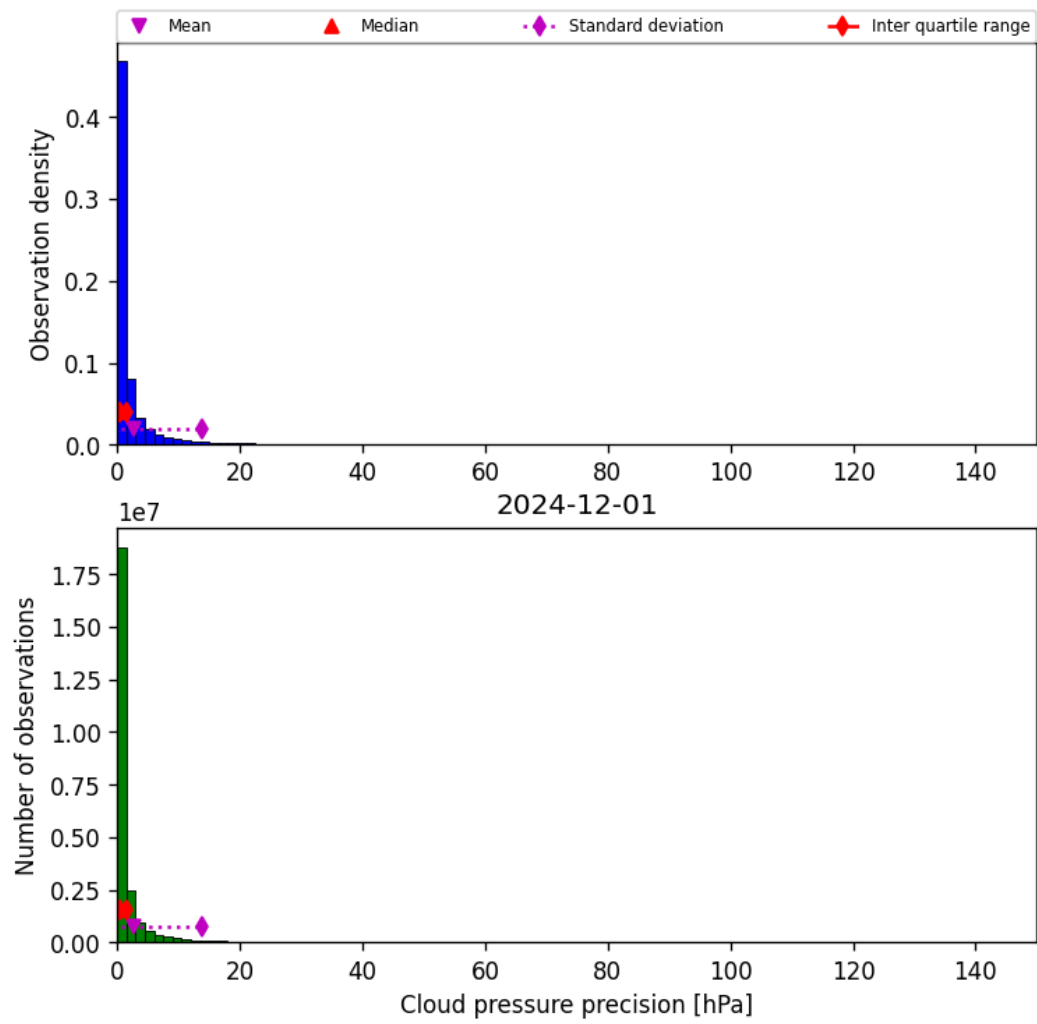
Figure 31: Histogram of “Cloud pressure precision” for 2024-11-30 to 2024-12-02
