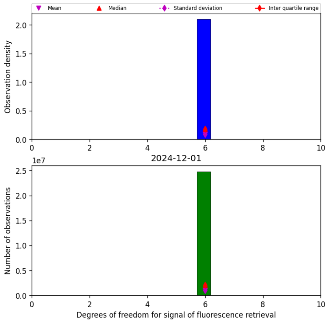
Figure 43: Histogram of “Degrees of freedom for signal of fluorescence retrieval” for 2024-11-30 to 2024-12-02
