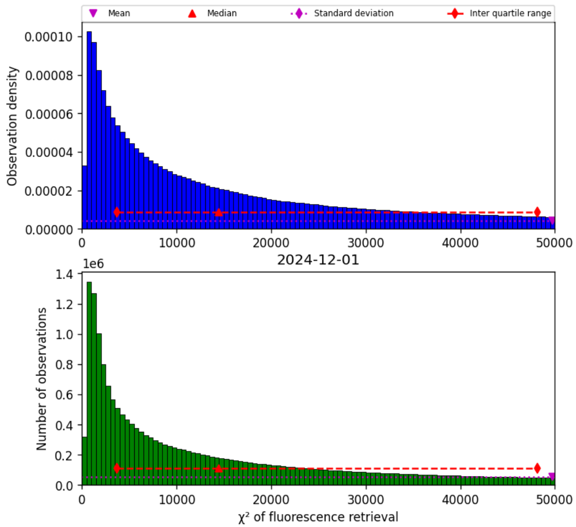
Figure 42: Histogram of “ \chi^2 of fluorescence retrieval” for 2024-11-30 to 2024-12-02
