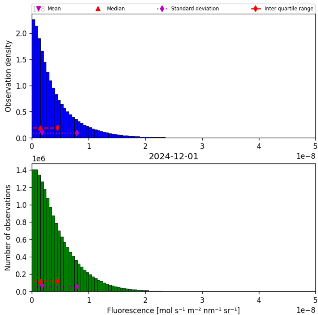
Figure 40: Histogram of “Fluorescence” for 2024-11-30 to 2024-12-02
