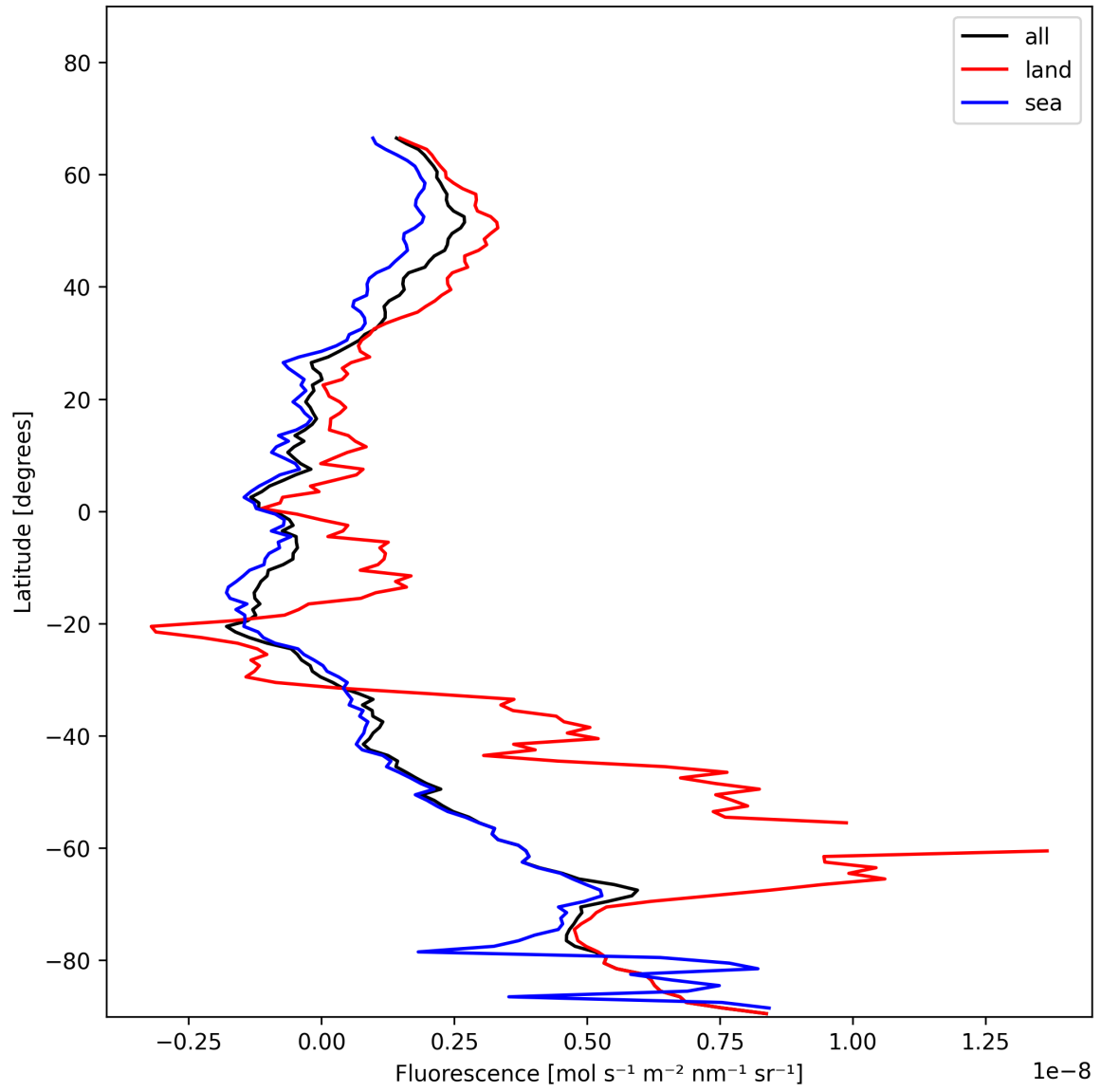
Figure 23: Zonal average of “Fluorescence” for 2024-11-30 to 2024-12-02.
