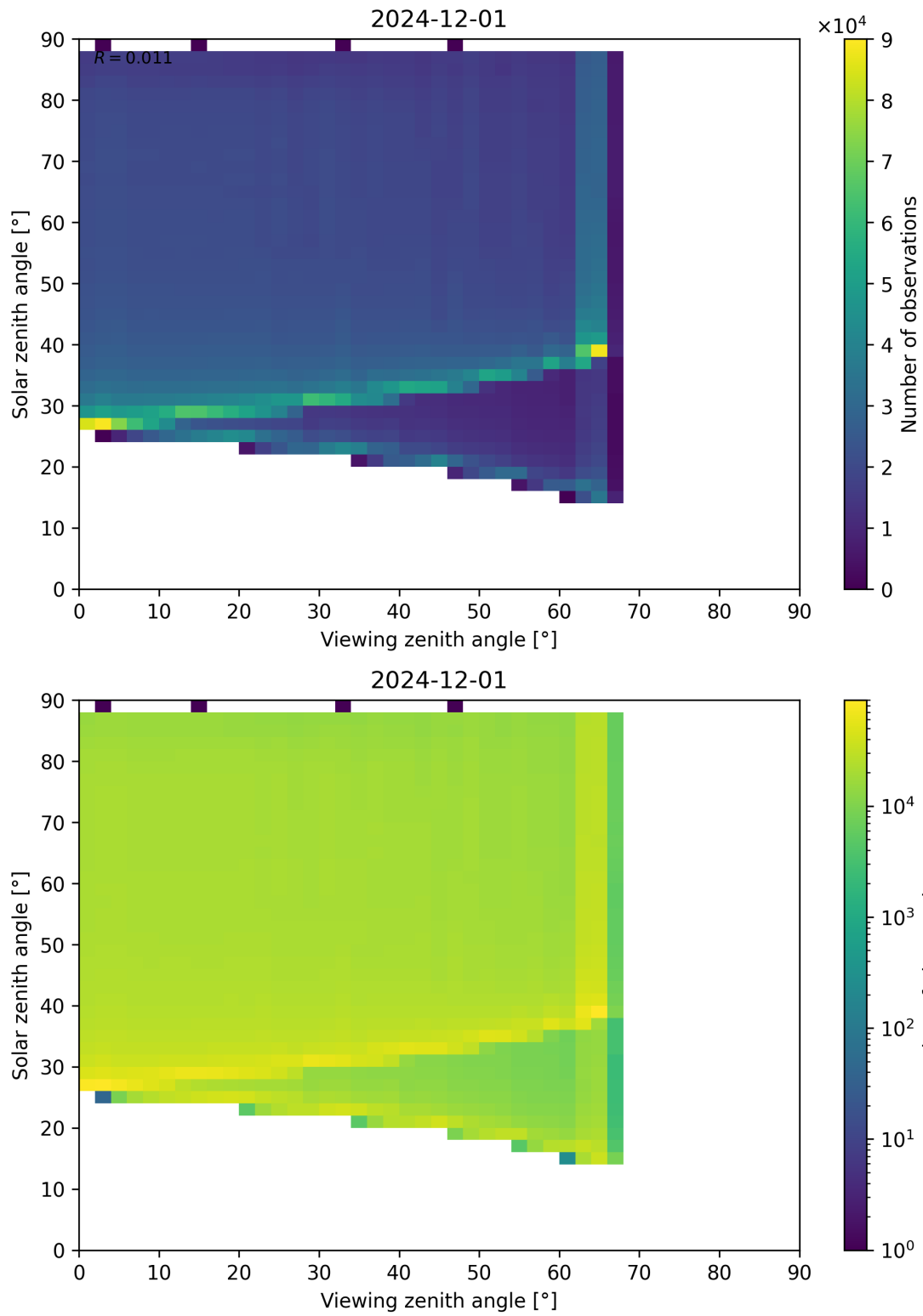
Figure 127: Scatter density plot of “Viewing zenith angle” against “Solar zenith angle” for 2024-11-30 to 2024-12-02.
