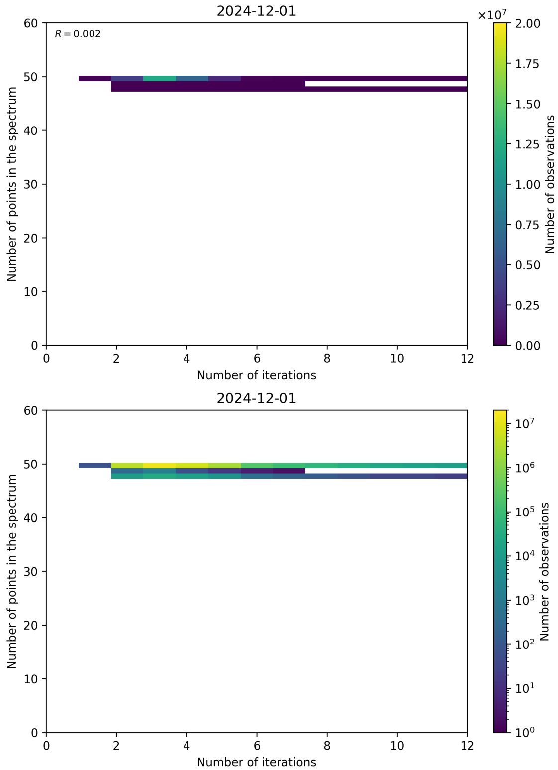
Figure 99: Scatter density plot of “Number of iterations” against “Number of points in the spectrum” for 2024-11-30 to 2024-12-02.
