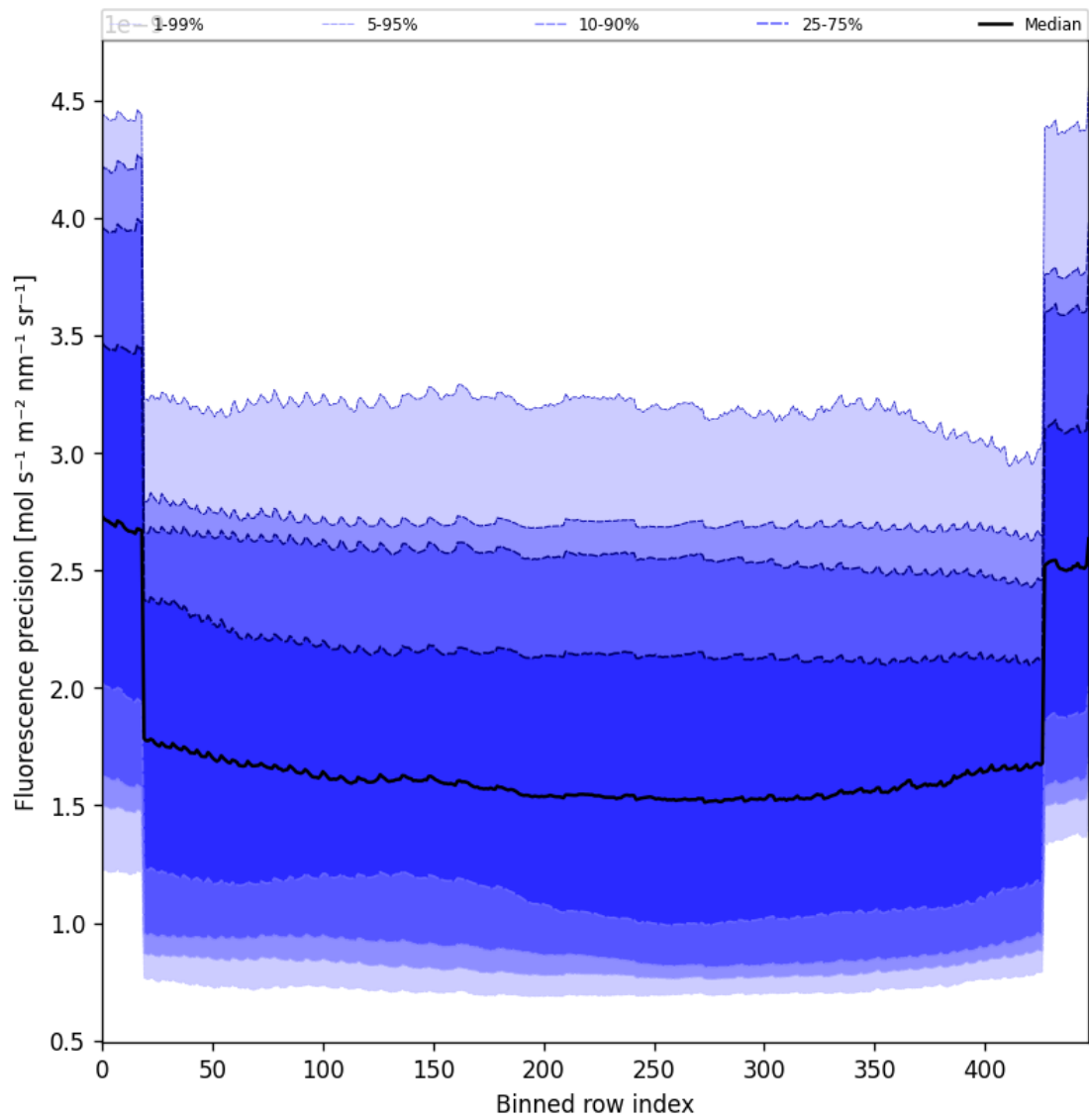
Figure 58: Along track statistics of “Fluorescence precision” for 2024-11-30 to 2024-12-02
