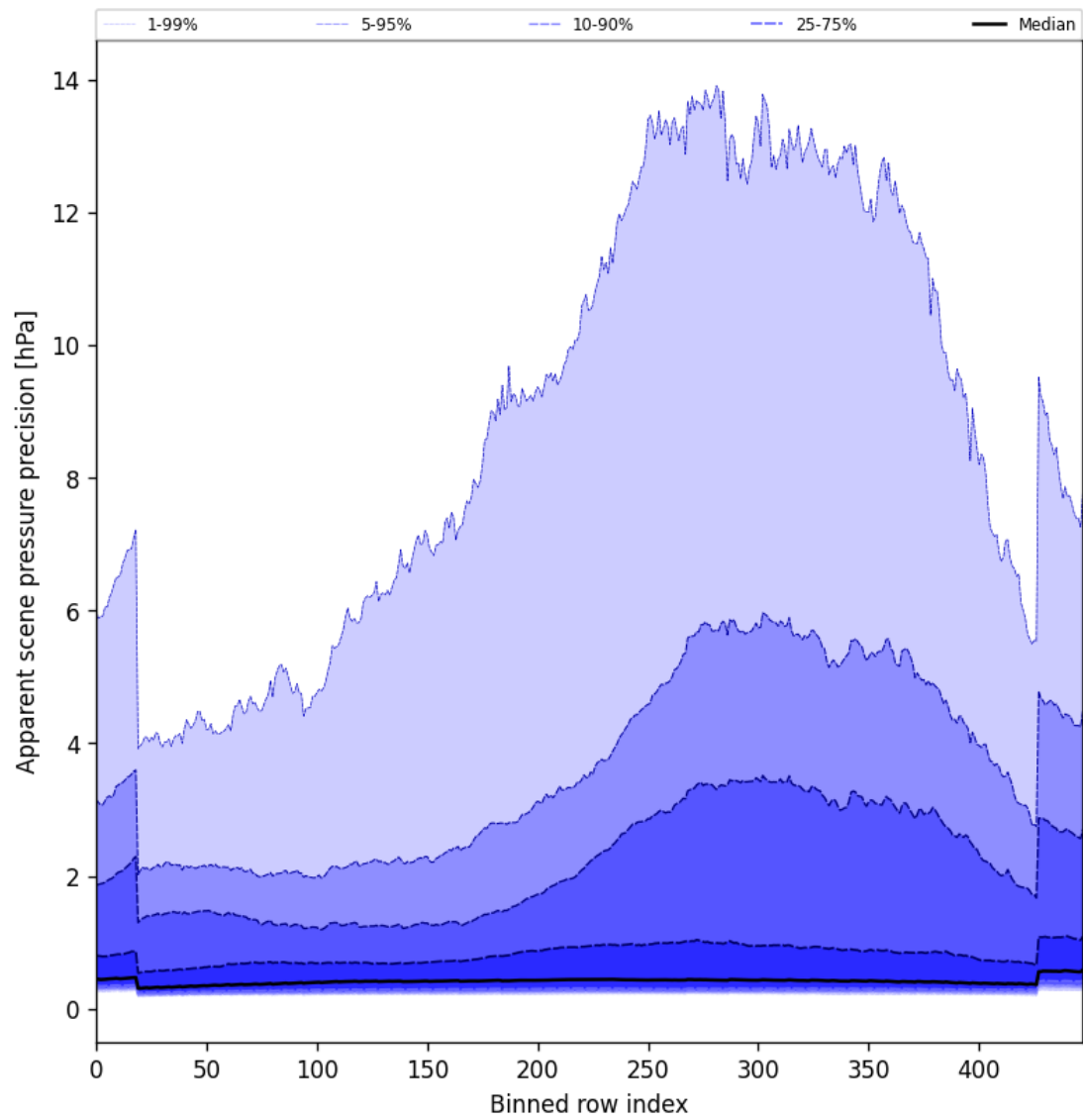
Figure 54: Along track statistics of “Apparent scene pressure precision” for 2024-11-30 to 2024-12-02
