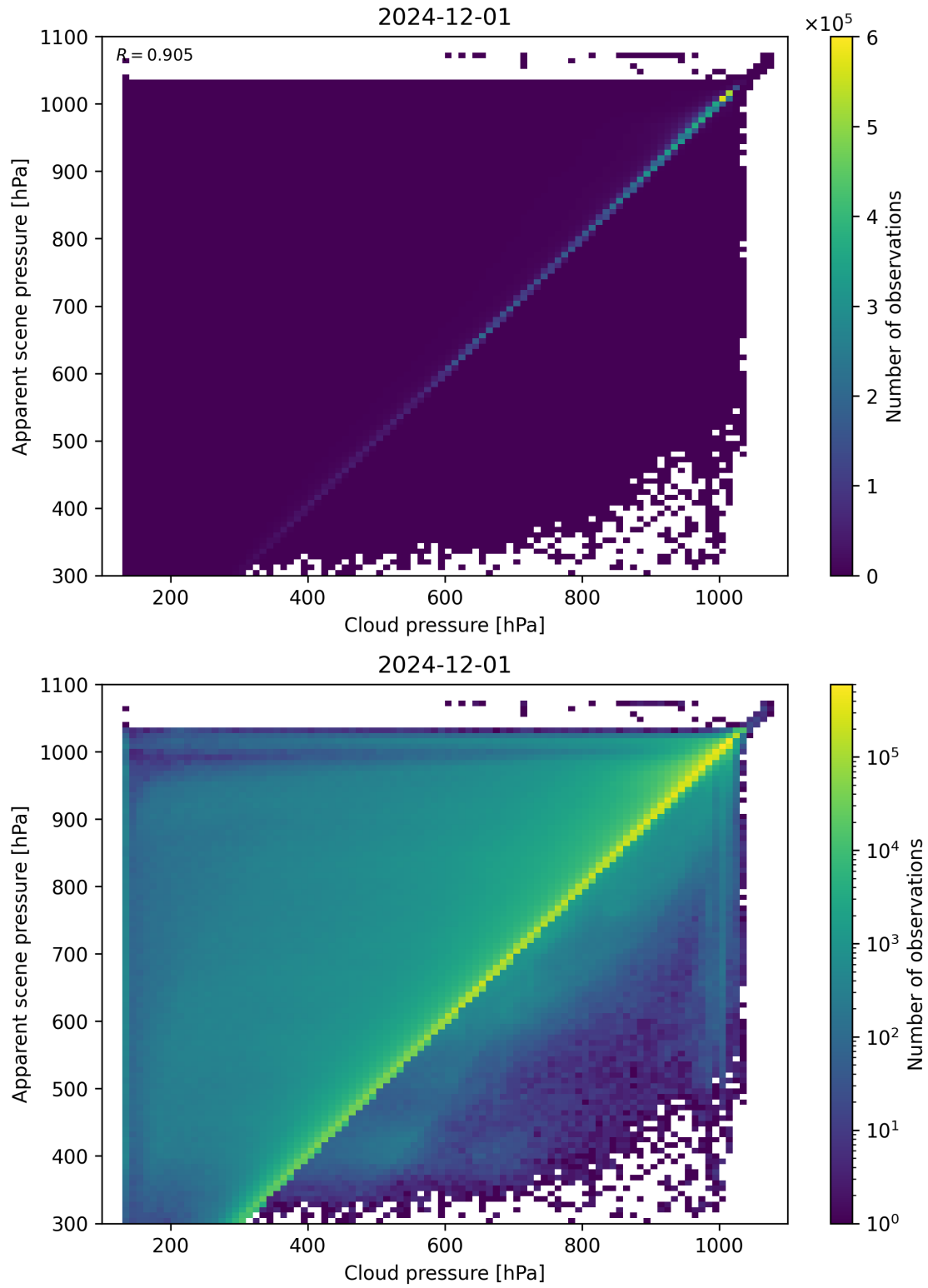
Figure 77: Scatter density plot of “Cloud pressure” against “Apparent scene pressure” for 2024-11-30 to 2024-12-02.
