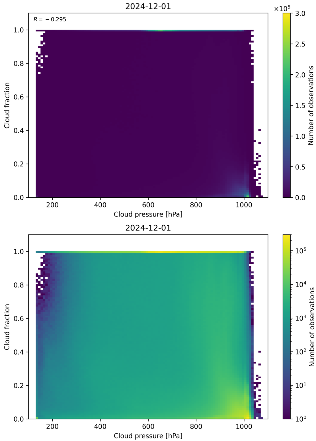
Figure 79: Scatter density plot of “Cloud pressure” against “Cloud fraction” for 2024-11-30 to 2024-12-02.
