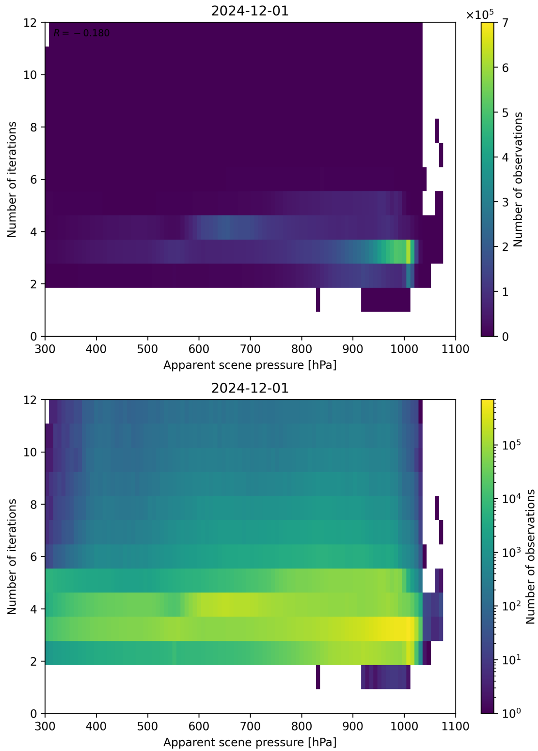
Figure 65: Scatter density plot of “Apparent scene pressure” against “Number of iterations” for 2024-11-30 to 2024-12-02.
