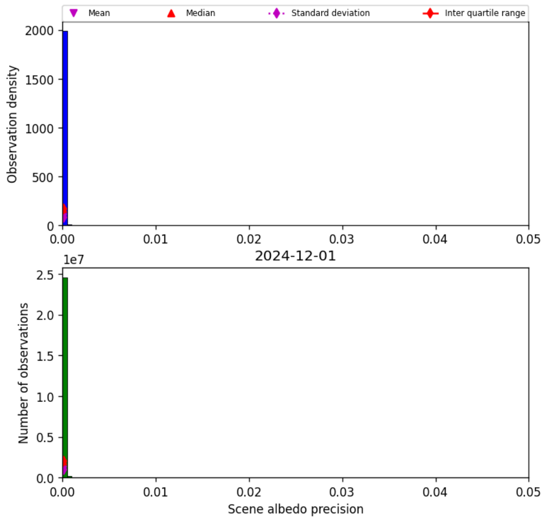
Figure 35: Histogram of “Scene albedo precision” for 2024-11-30 to 2024-12-02
