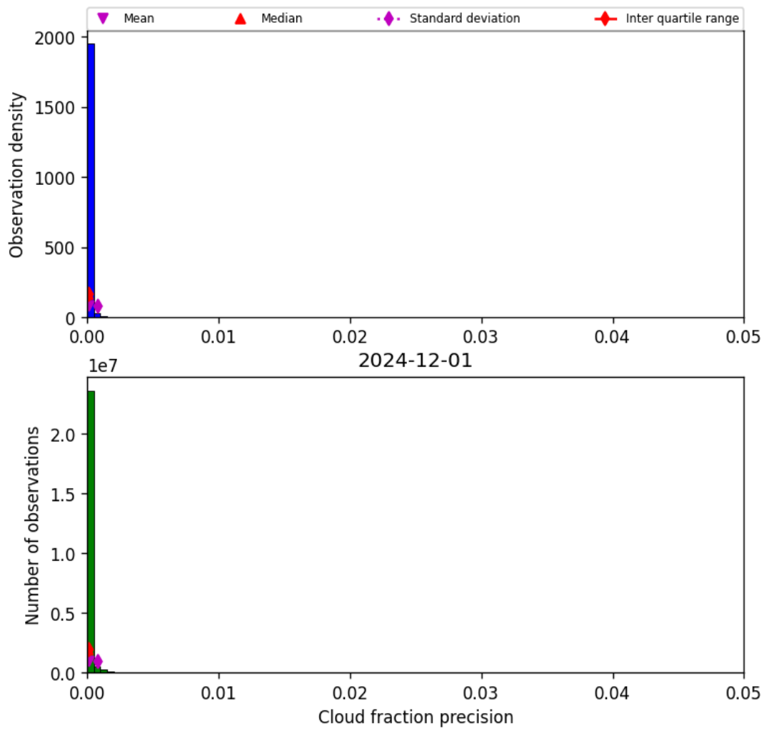
Figure 33: Histogram of “Cloud fraction precision” for 2024-11-30 to 2024-12-02
