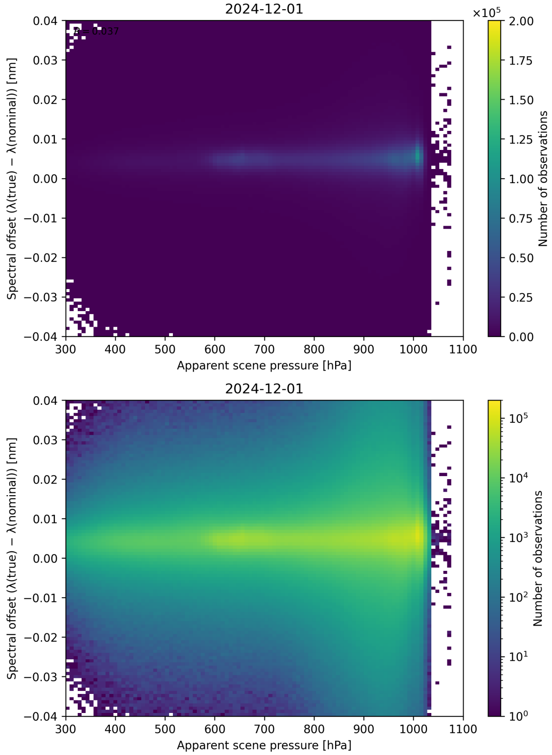
Figure 67: Scatter density plot of “Apparent scene pressure” against “Spectral offset ( \lambda_{\text{true}} - \lambda_{\text{nominal}} )” for 2024-11-30 to 2024-12-02.
