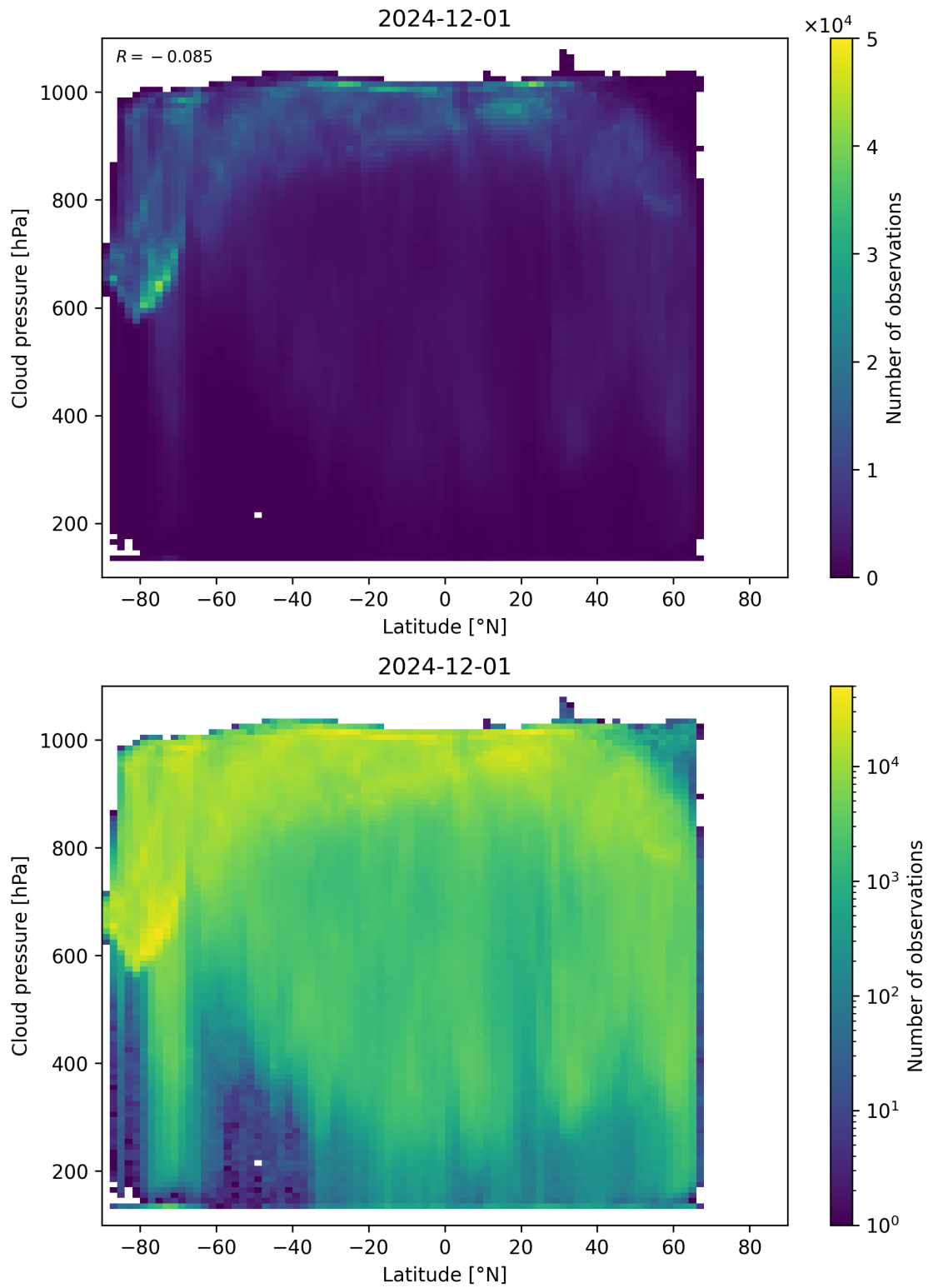
Figure 91: Scatter density plot of “Latitude” against “Cloud pressure” for 2024-11-30 to 2024-12-02.
