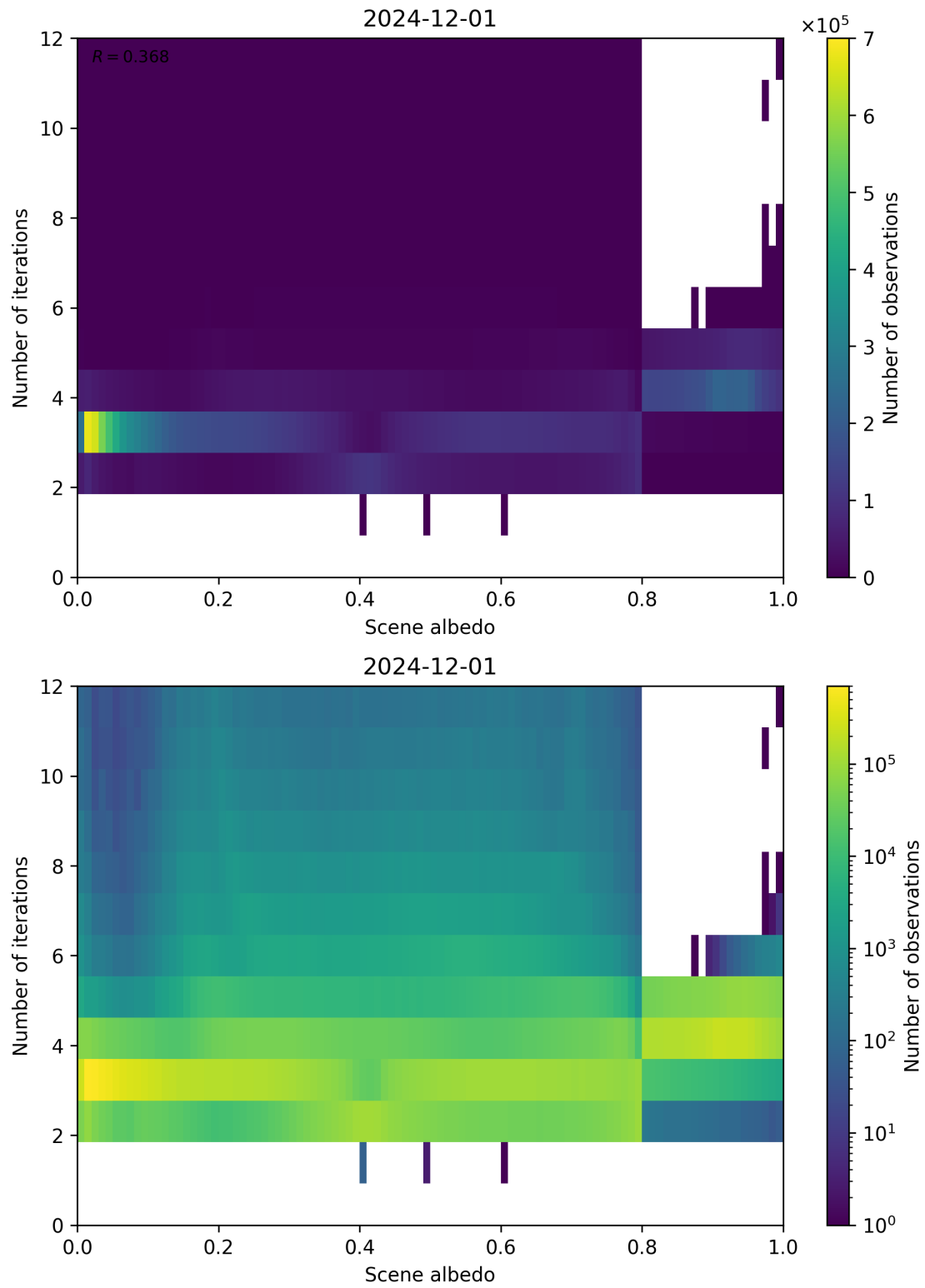
Figure 105: Scatter density plot of “Scene albedo” against “Number of iterations” for 2024-11-30 to 2024-12-02.
