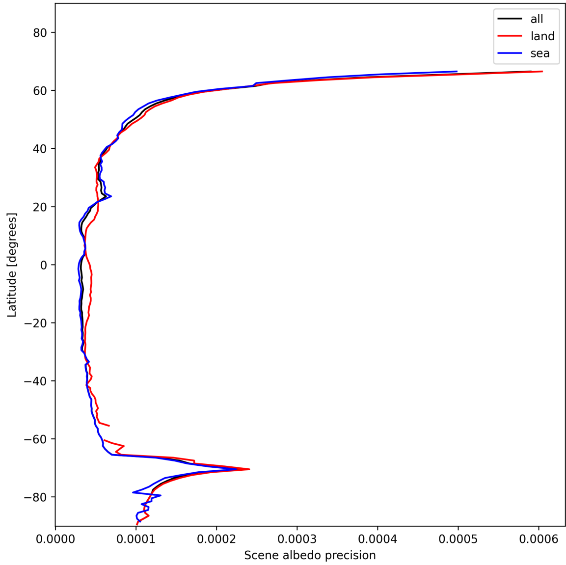
Figure 18: Zonal average of “Scene albedo precision” for 2024-11-30 to 2024-12-02.
