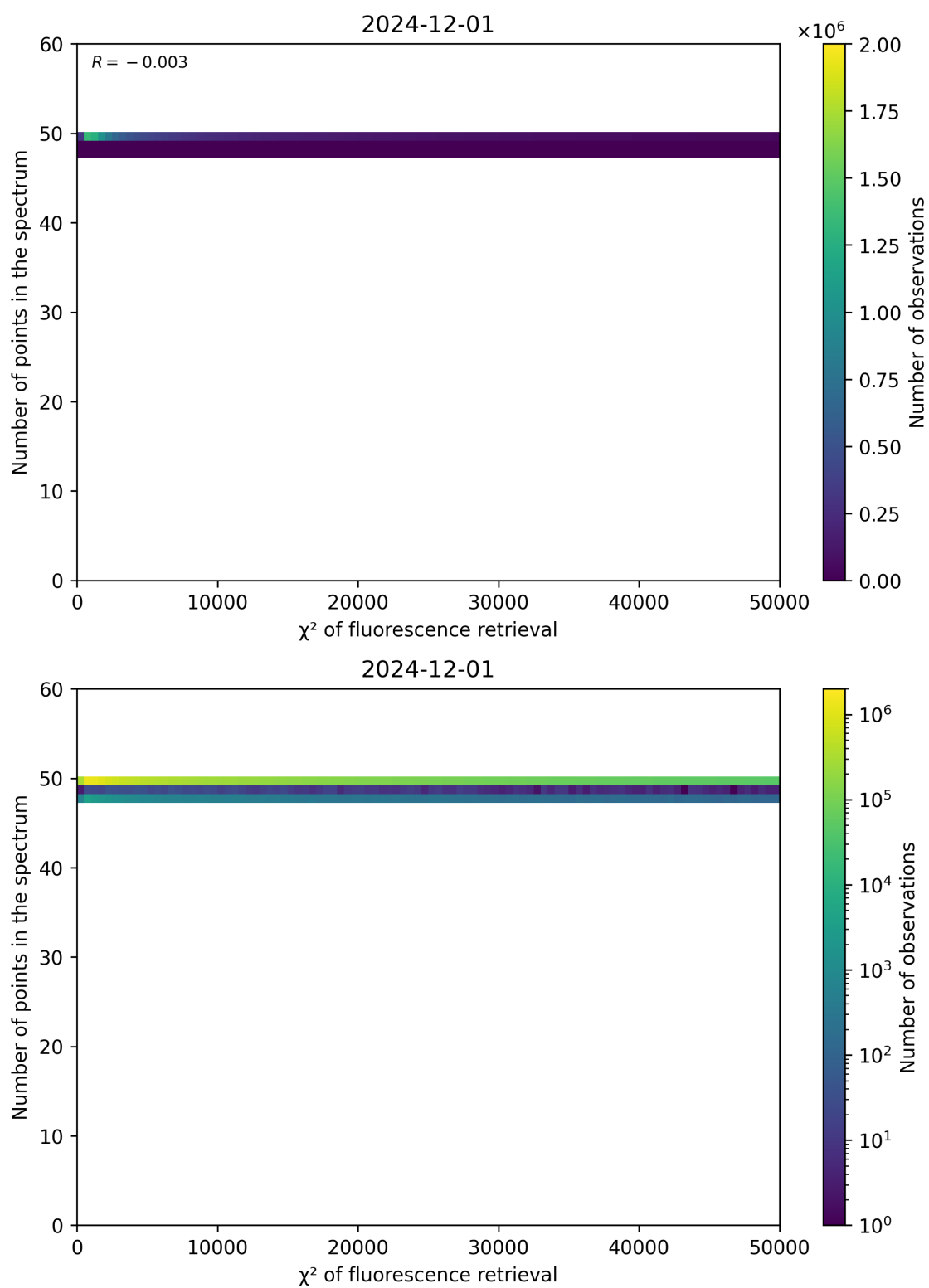
Figure 68: Scatter density plot of “ \chi^2 of fluorescence retrieval” against “Number of points in the spectrum” for 2024-11-30 to 2024-12-02.
