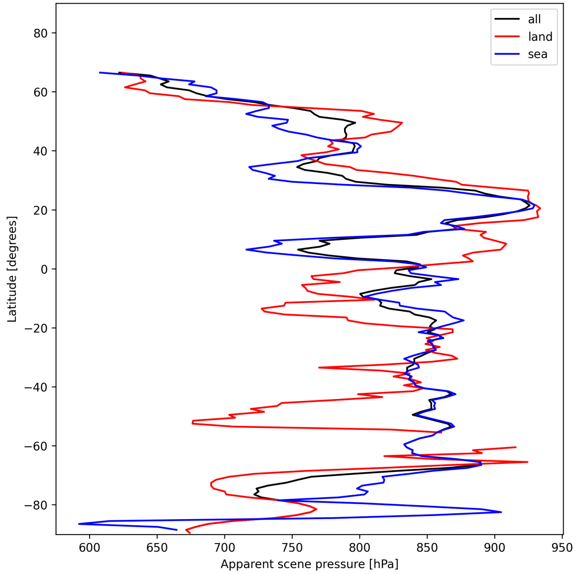
Figure 19: Zonal average of “Apparent scene pressure” for 2024-11-30 to 2024-12-02.
