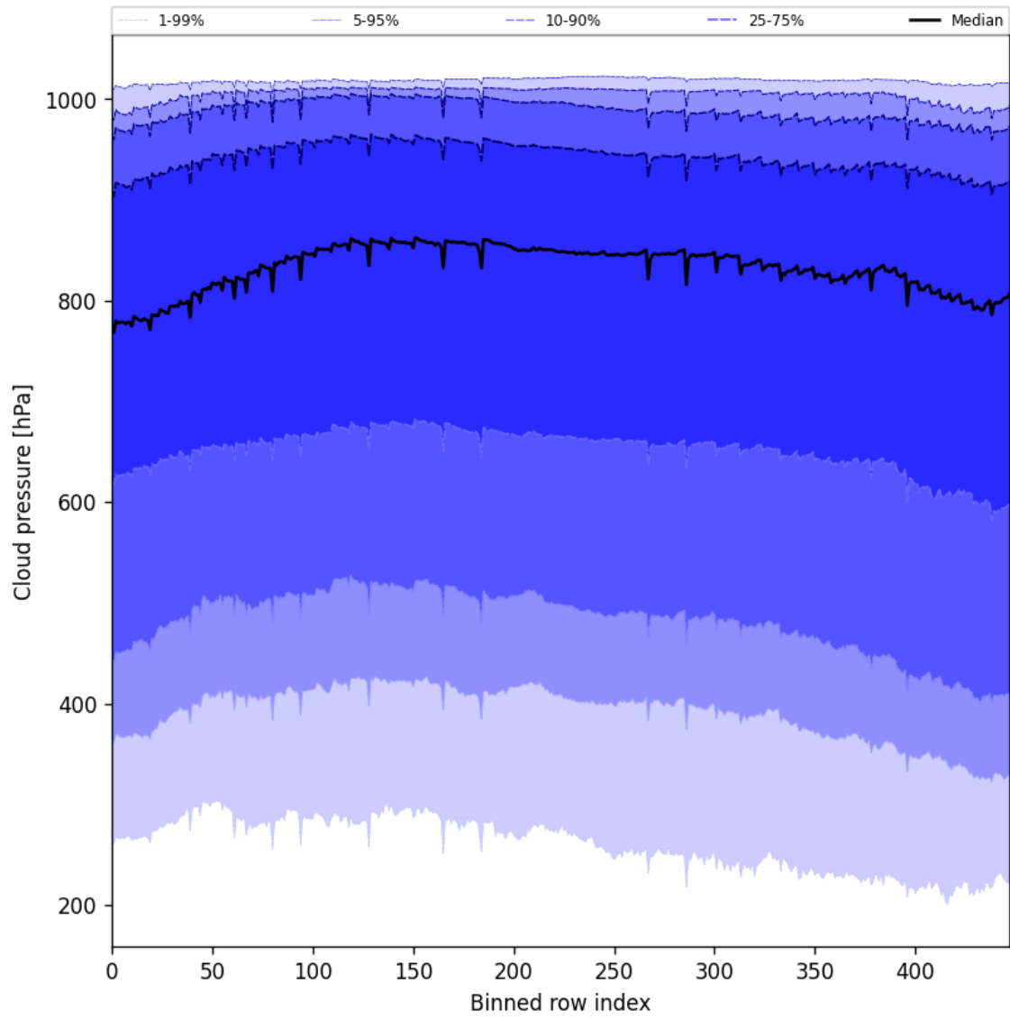
Figure 47: Along track statistics of “Cloud pressure” for 2024-11-30 to 2024-12-02
