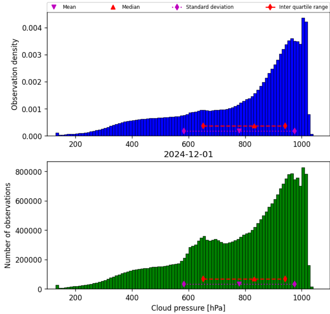
Figure 30: Histogram of “Cloud pressure” for 2024-11-30 to 2024-12-02
