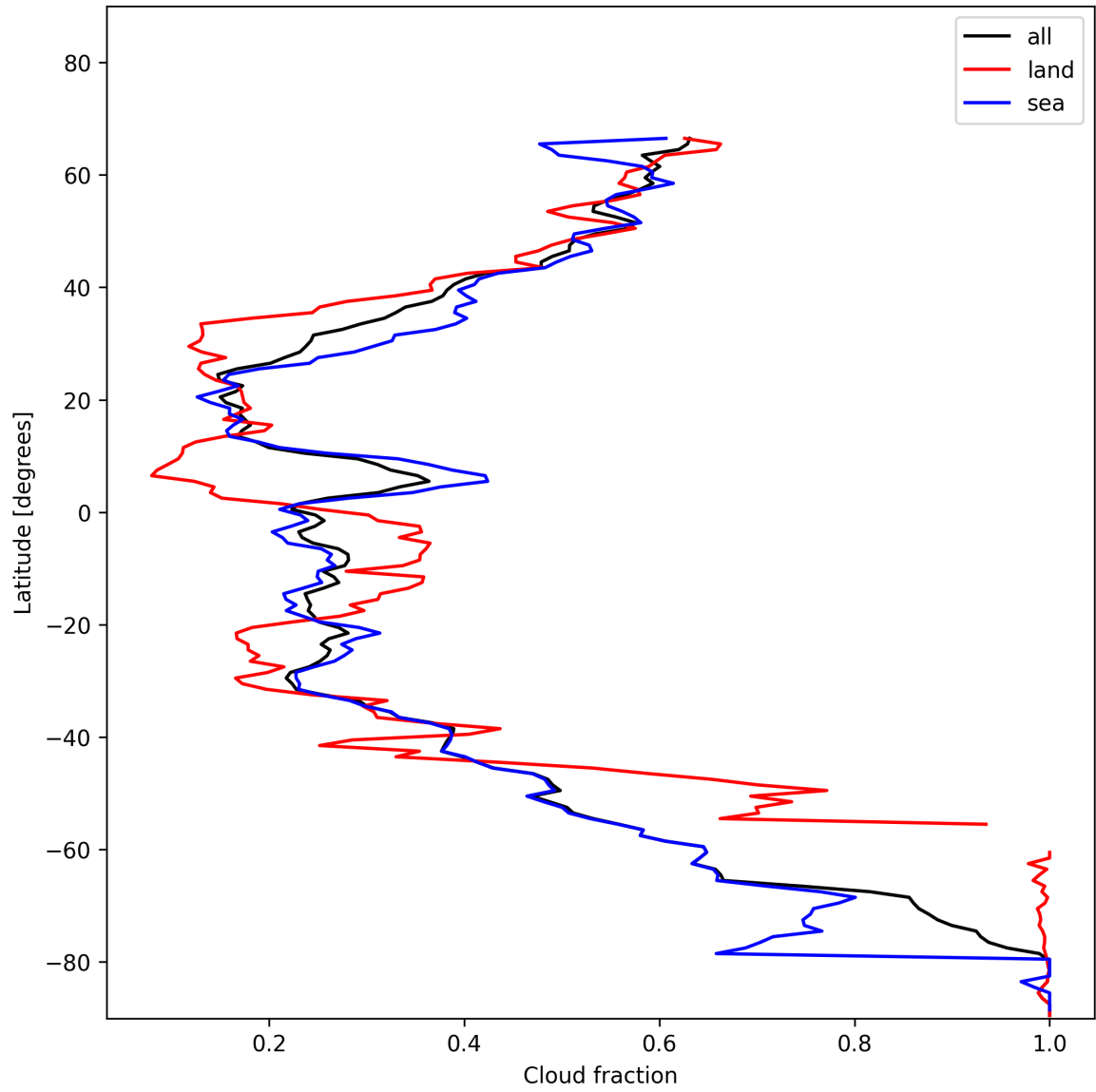
Figure 15: Zonal average of “Cloud fraction” for 2024-11-30 to 2024-12-02.
