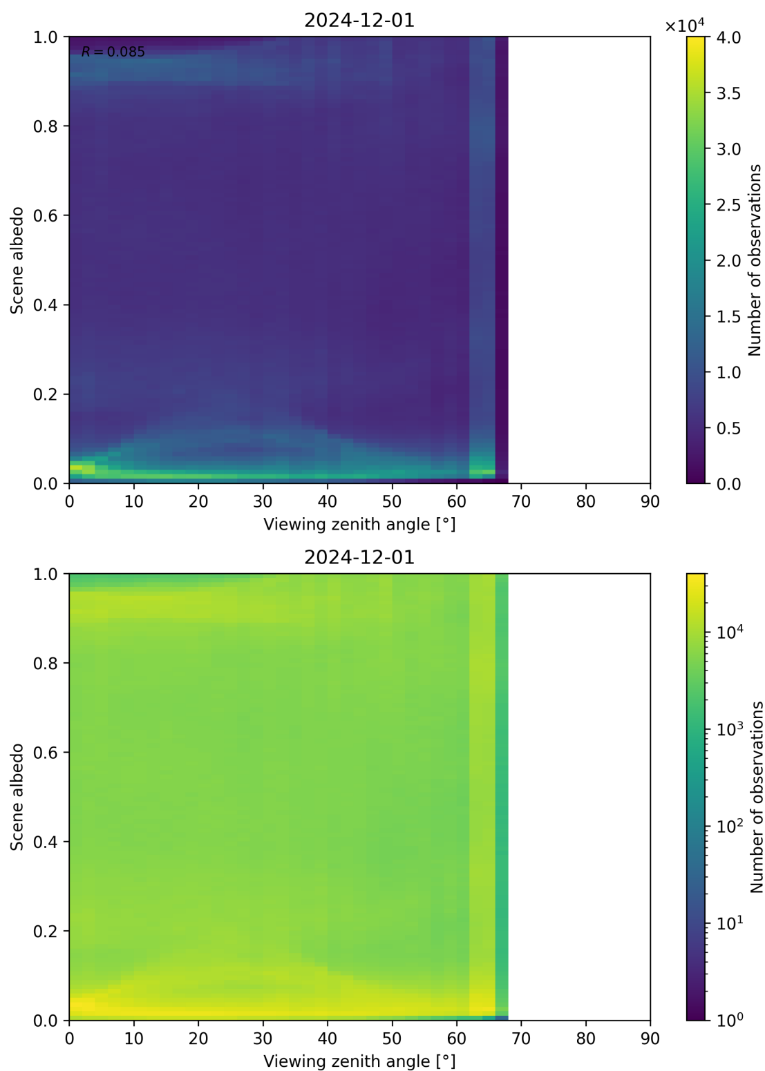
Figure 126: Scatter density plot of “Viewing zenith angle” against “Scene albedo” for 2024-11-30 to 2024-12-02.
