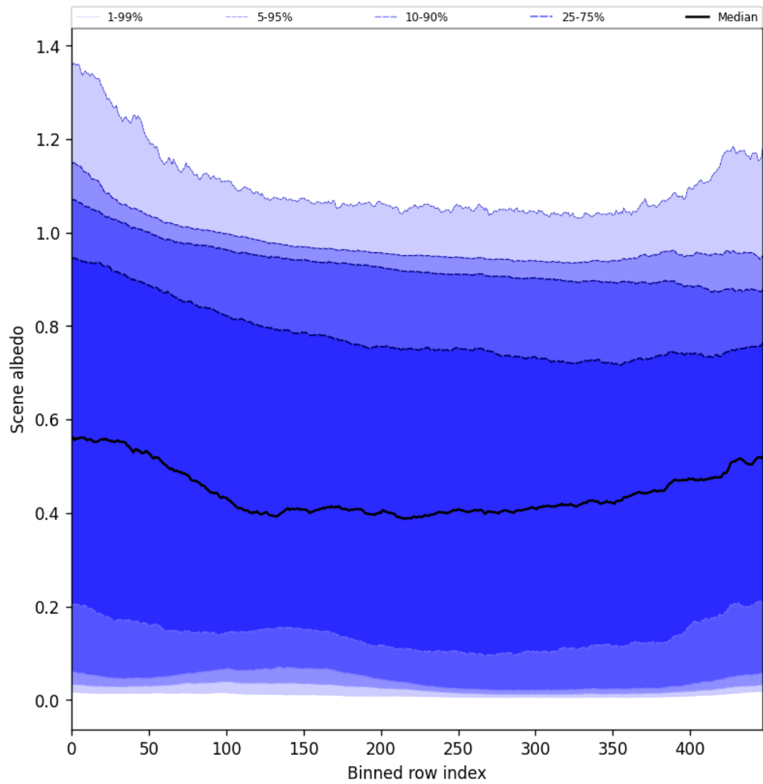
Figure 51: Along track statistics of “Scene albedo” for 2024-11-30 to 2024-12-02
