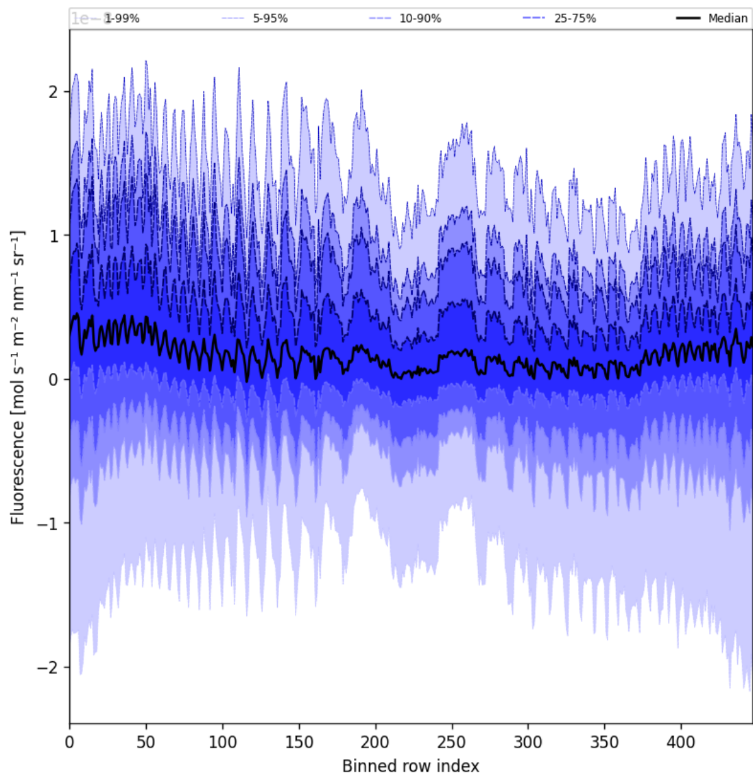
Figure 57: Along track statistics of “Fluorescence” for 2024-11-30 to 2024-12-02
