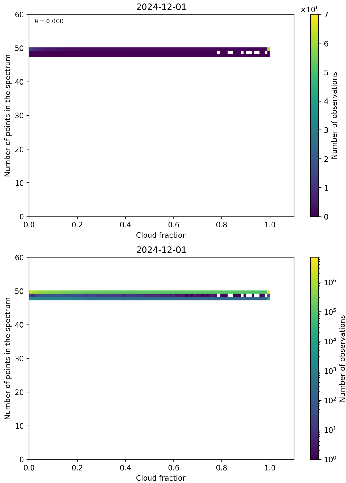
Figure 74: Scatter density plot of “Cloud fraction” against “Number of points in the spectrum” for 2024-11-30 to 2024-12-02.
