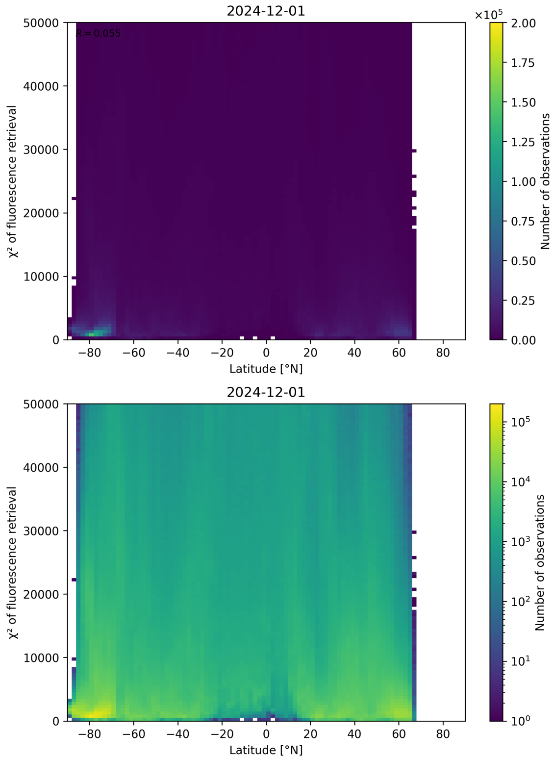
Figure 89: Scatter density plot of “Latitude” against “ \chi^2 of fluorescence retrieval” for 2024-11-30 to 2024-12-02.
