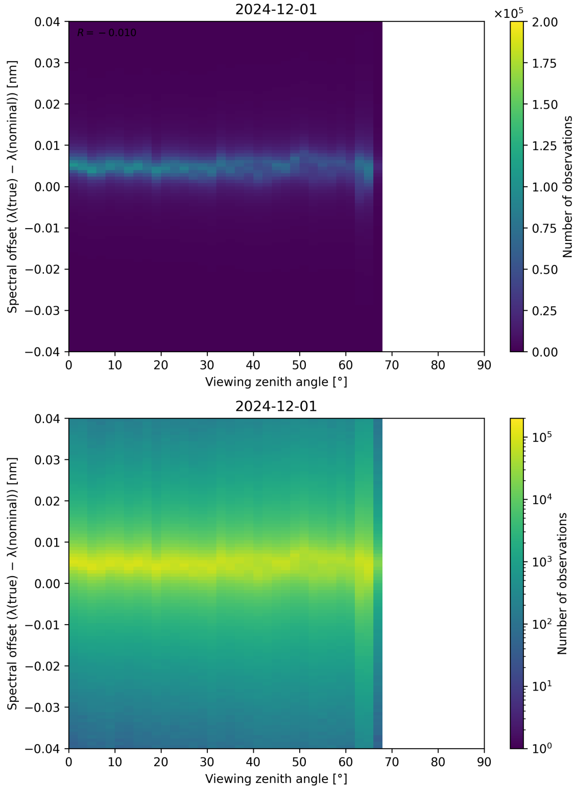
Figure 128: Scatter density plot of “Viewing zenith angle” against “Spectral offset ( \lambda_{\text{true}} - \lambda_{\text{nominal}} )” for 2024-11-30 to 2024-12-02.
