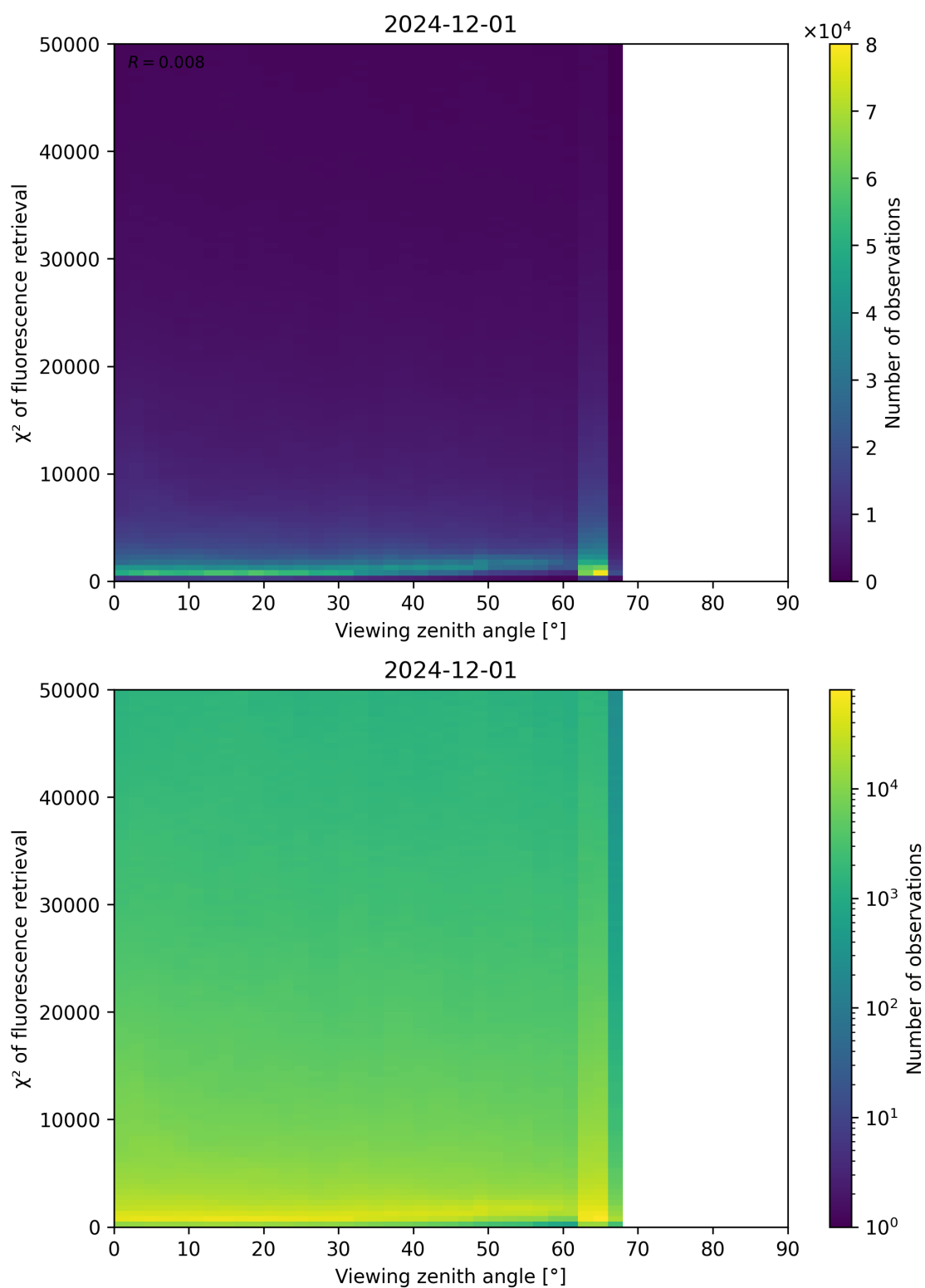
Figure 119: Scatter density plot of “Viewing zenith angle” against “ \chi^2 of fluorescence retrieval” for 2024-11-30 to 2024-12-02.
