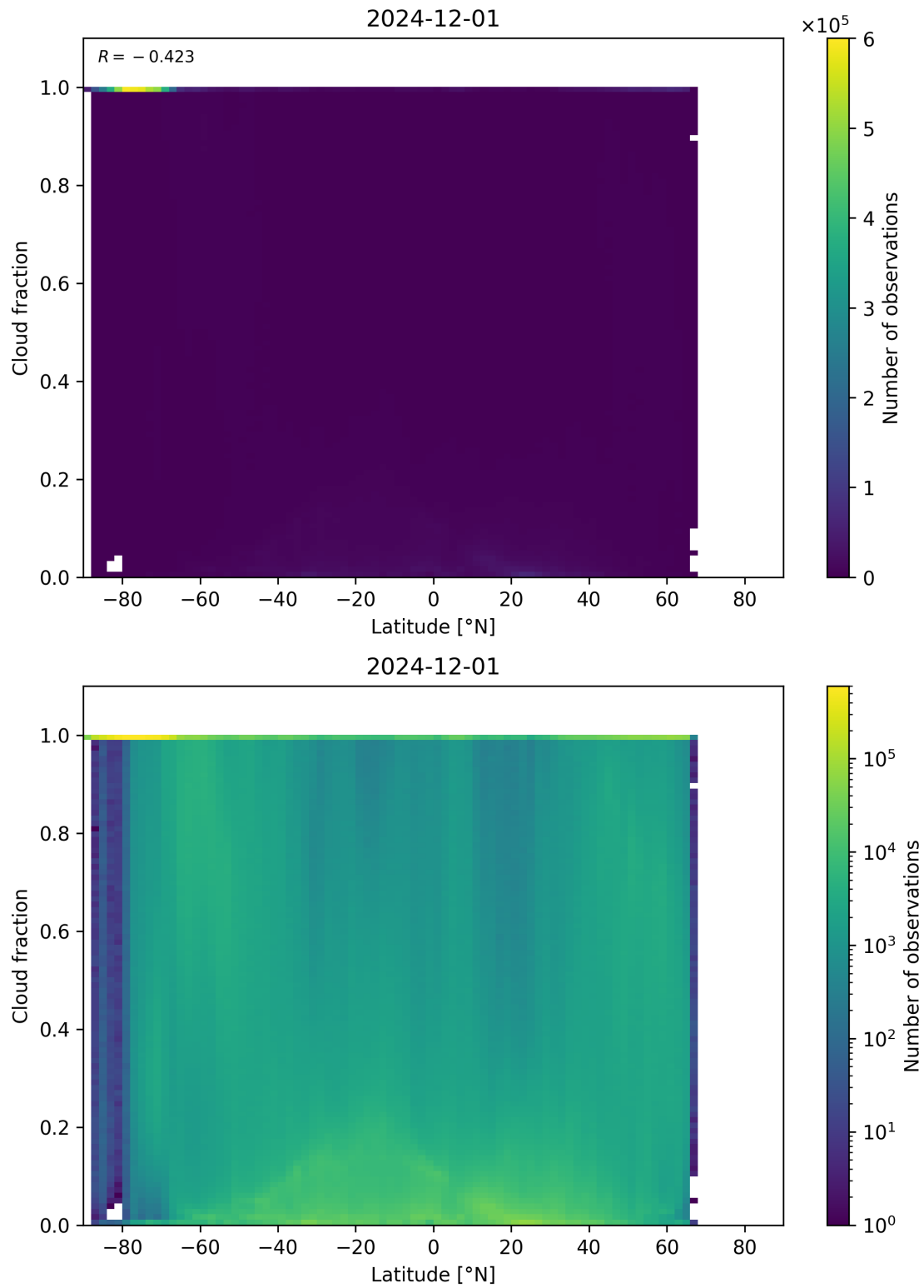
Figure 90: Scatter density plot of “Latitude” against “Cloud fraction” for 2024-11-30 to 2024-12-02.
