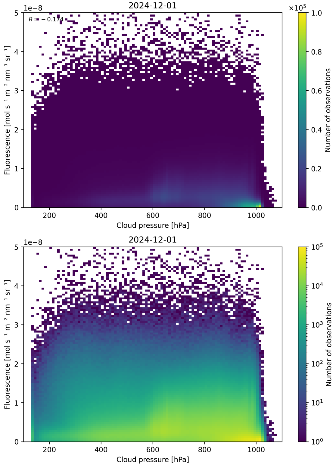
Figure 80: Scatter density plot of “Cloud pressure” against “Fluorescence” for 2024-11-30 to 2024-12-02.
