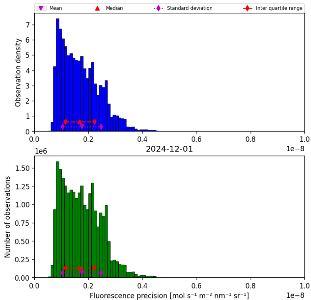
Figure 41: Histogram of “Fluorescence precision” for 2024-11-30 to 2024-12-02
