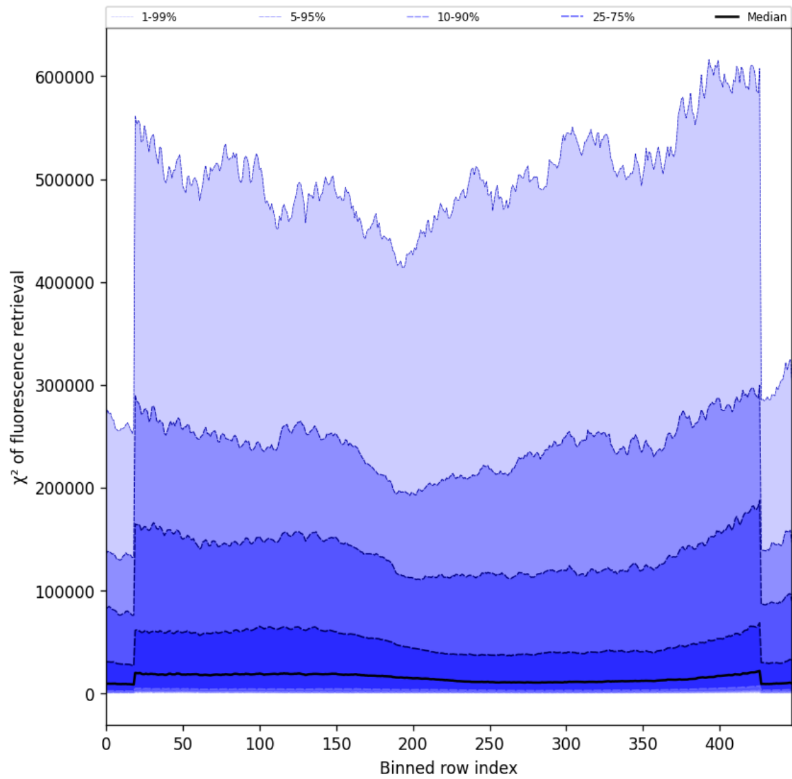
Figure 59: Along track statistics of “ \chi^2 of fluorescence retrieval” for 2024-11-30 to 2024-12-02
