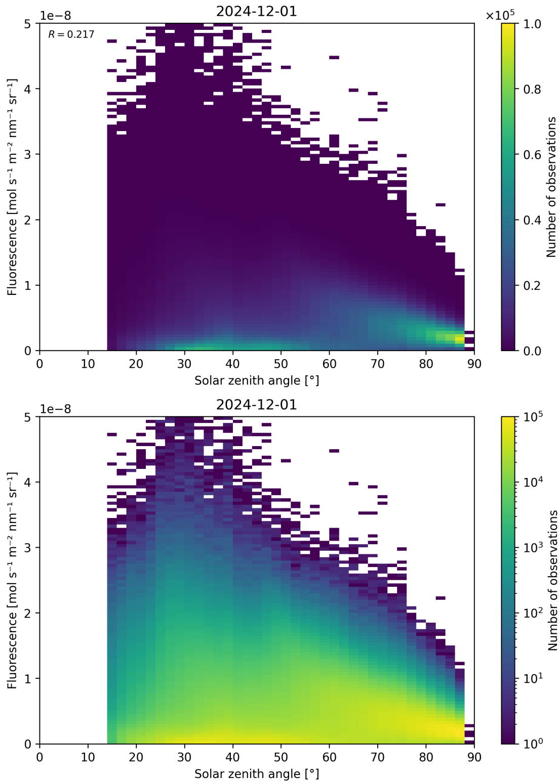
Figure 112: Scatter density plot of “Solar zenith angle” against “Fluorescence” for 2024-11-30 to 2024-12-02.
