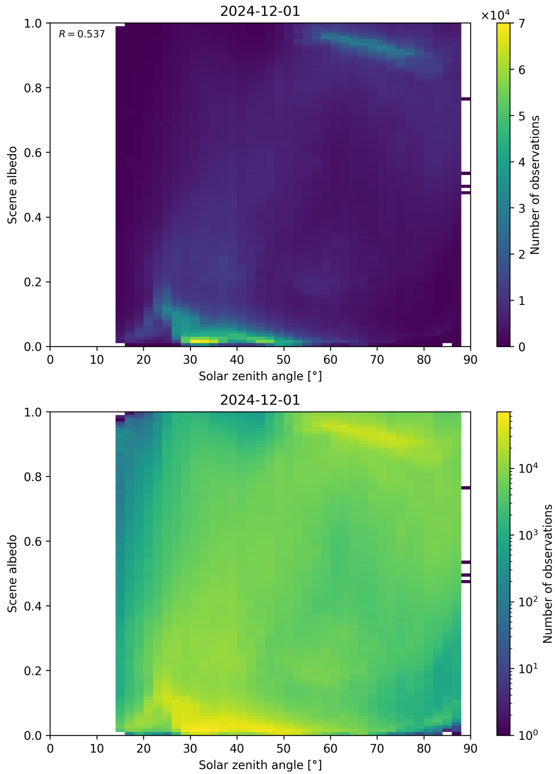
Figure 116: Scatter density plot of “Solar zenith angle” against “Scene albedo” for 2024-11-30 to 2024-12-02.
