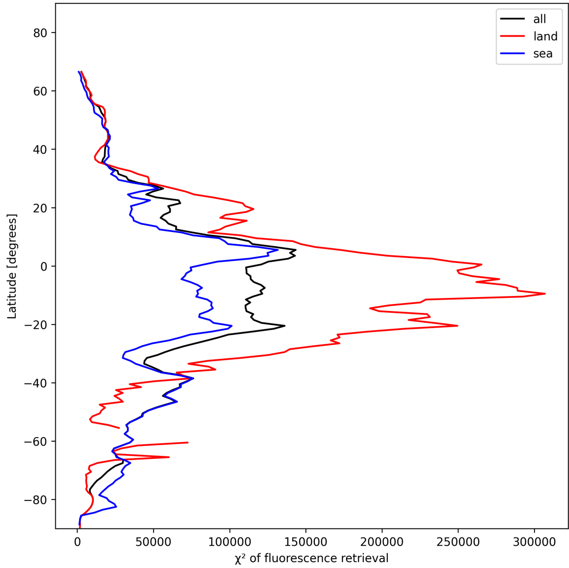
Figure 25: Zonal average of “ \chi^2 of fluorescence retrieval” for 2024-11-30 to 2024-12-02.
