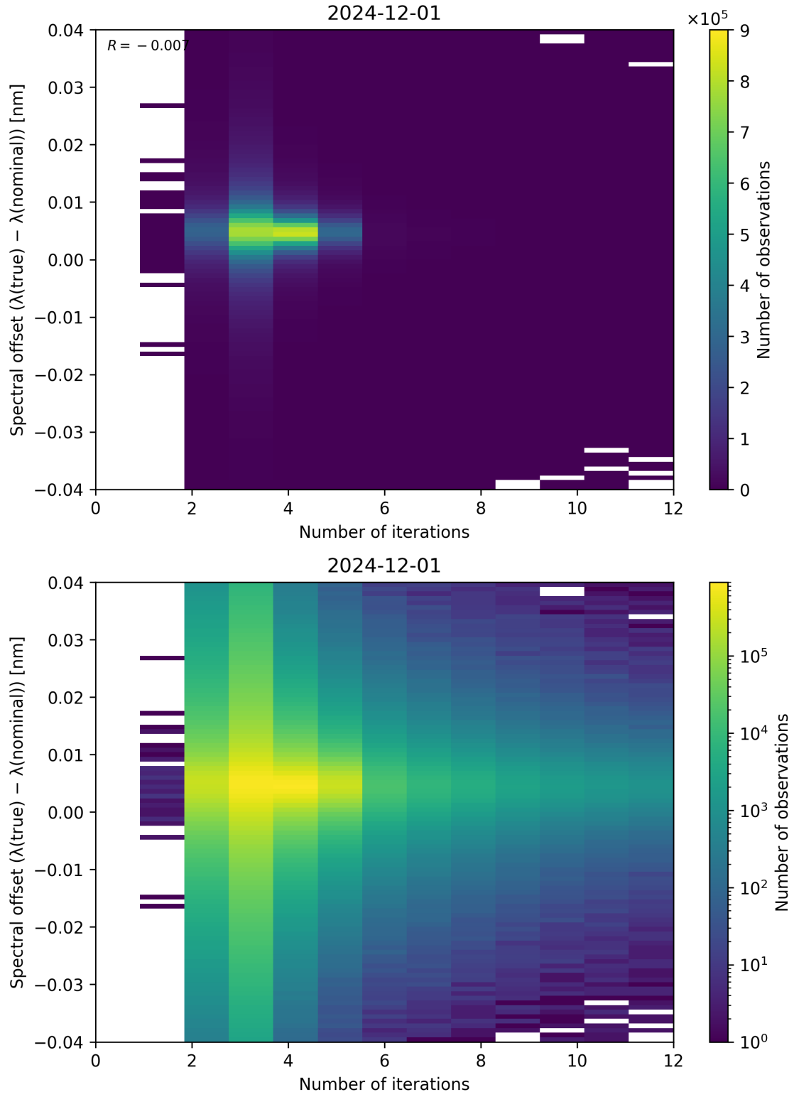
Figure 100: Scatter density plot of “Number of iterations” against “Spectral offset ( \lambda_{\text{true}} - \lambda_{\text{nominal}} )” for 2024-11-30 to 2024-12-02.
