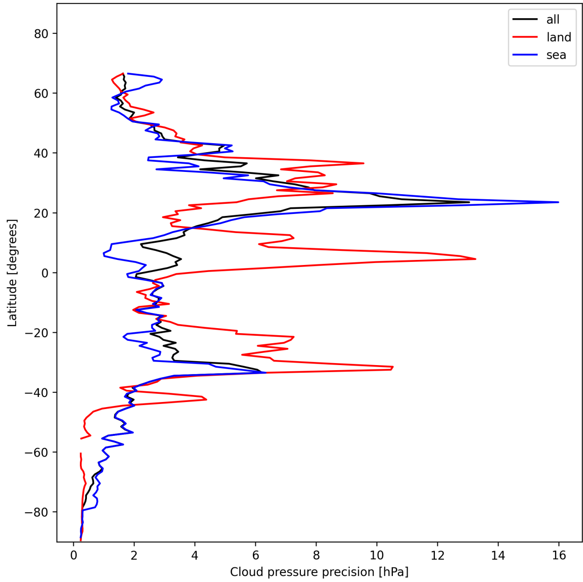
Figure 14: Zonal average of “Cloud pressure precision” for 2024-11-30 to 2024-12-02.
