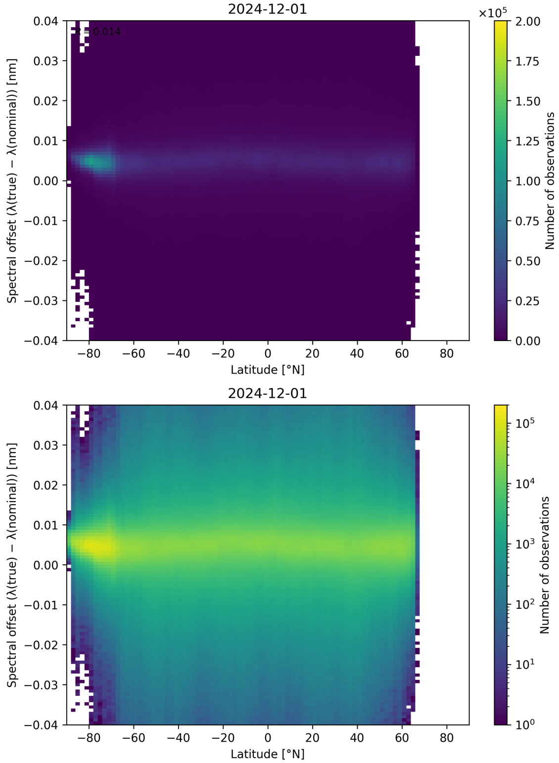
Figure 96: Scatter density plot of “Latitude” against “Spectral offset ( \lambda_{\text{true}} - \lambda_{\text{nominal}} )” for 2024-11-30 to 2024-12-02.
