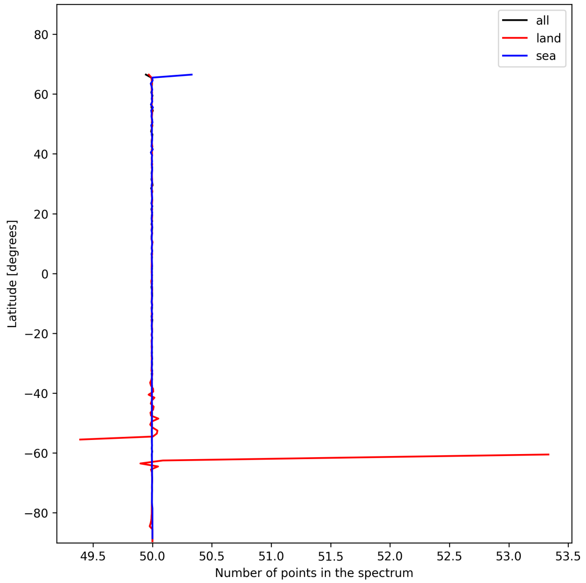
Figure 27: Zonal average of “Number of points in the spectrum” for 2024-11-30 to 2024-12-02.
