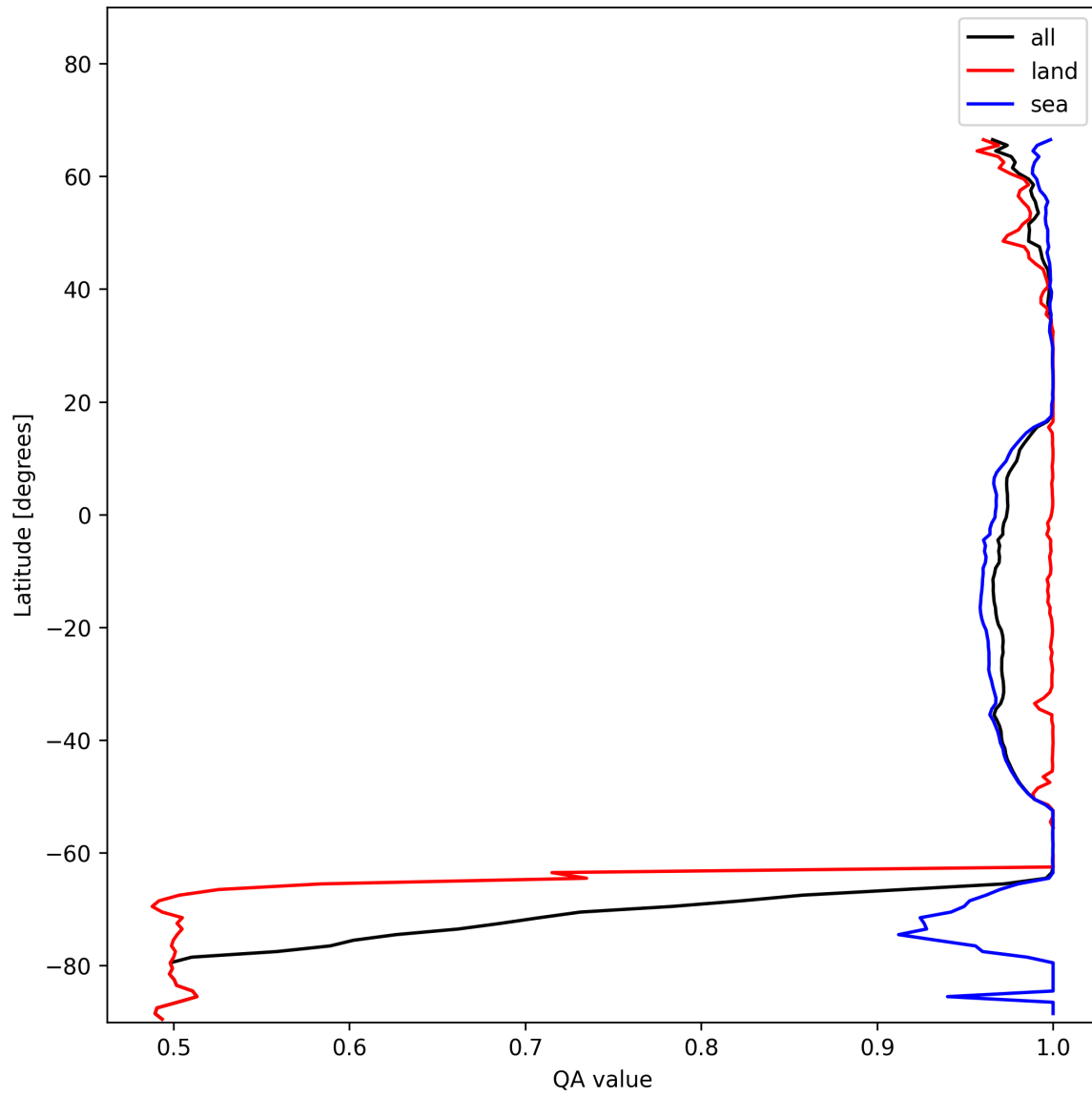
Figure 12: Zonal average of “QA value” for 2024-11-30 to 2024-12-02.
