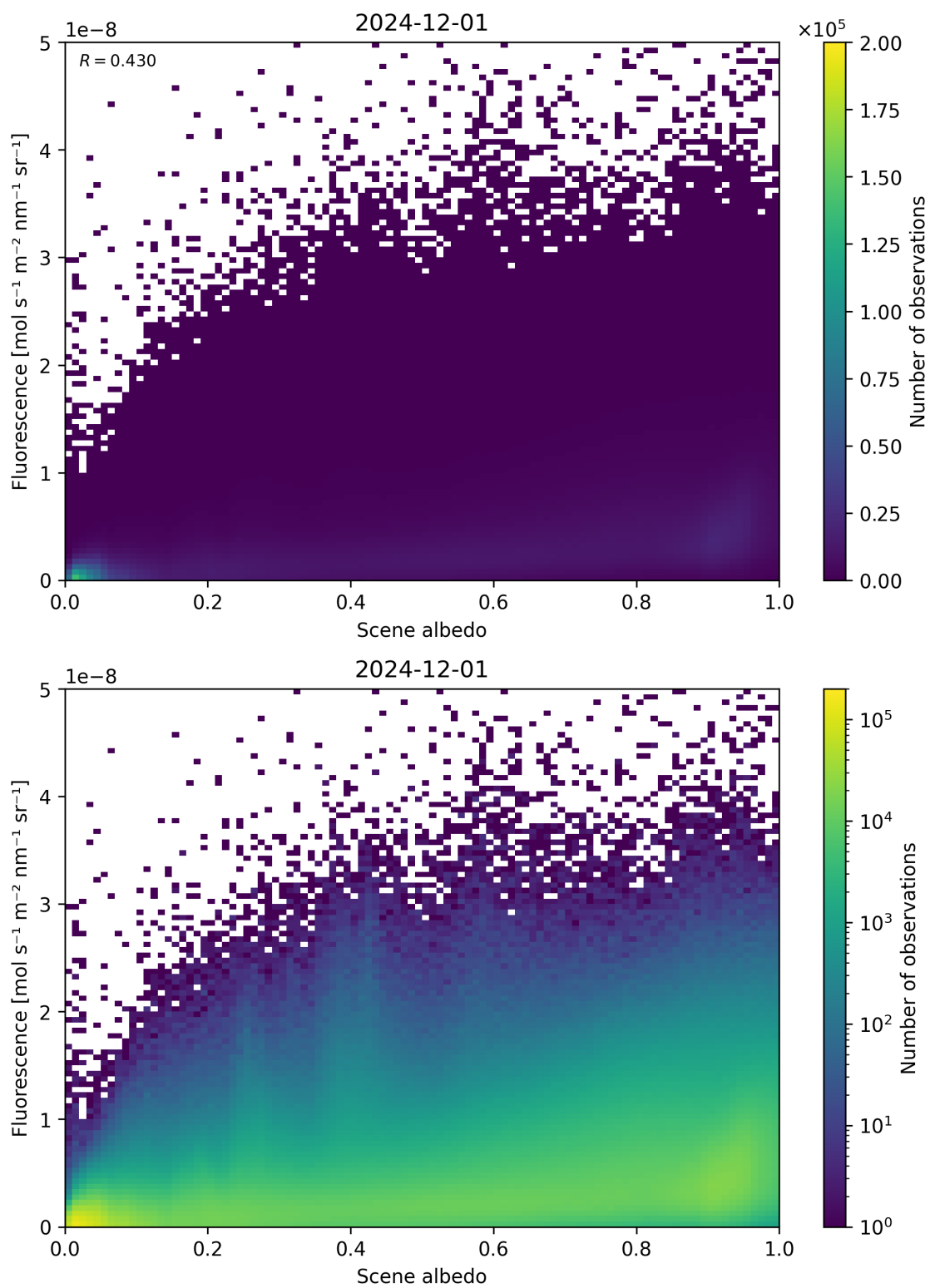
Figure 104: Scatter density plot of “Scene albedo” against “Fluorescence” for 2024-11-30 to 2024-12-02.
