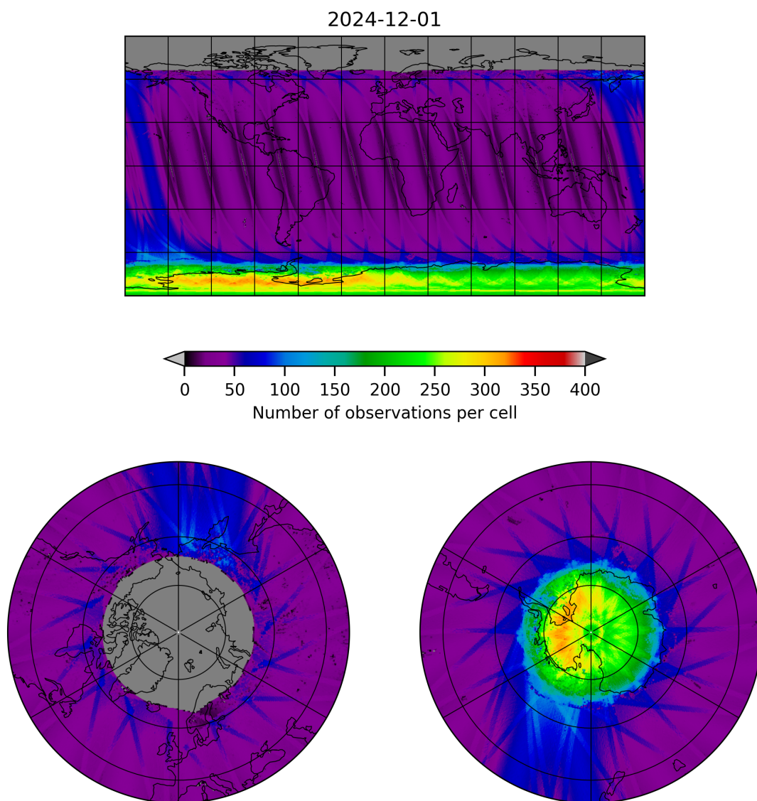
Figure 11: Map of the number of observations for 2024-11-30 to 2024-12-02
