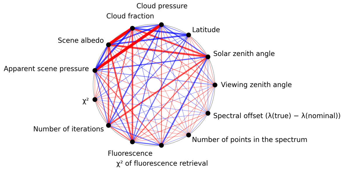
Figure 1: Map of correlation graph for 2024-11-30 to 2024-12-02.
