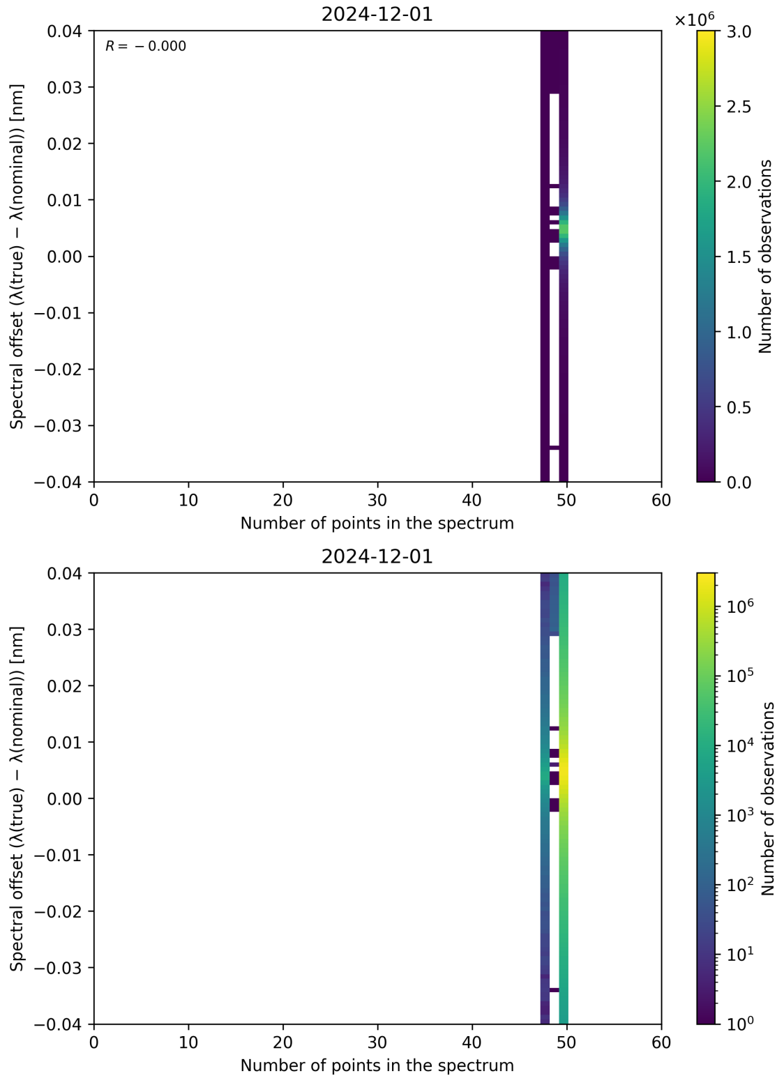
Figure 101: Scatter density plot of “Number of points in the spectrum” against “Spectral offset ( \lambda_{\text{true}} - \lambda_{\text{nominal}} )” for 2024-11-30 to 2024-12-02.
