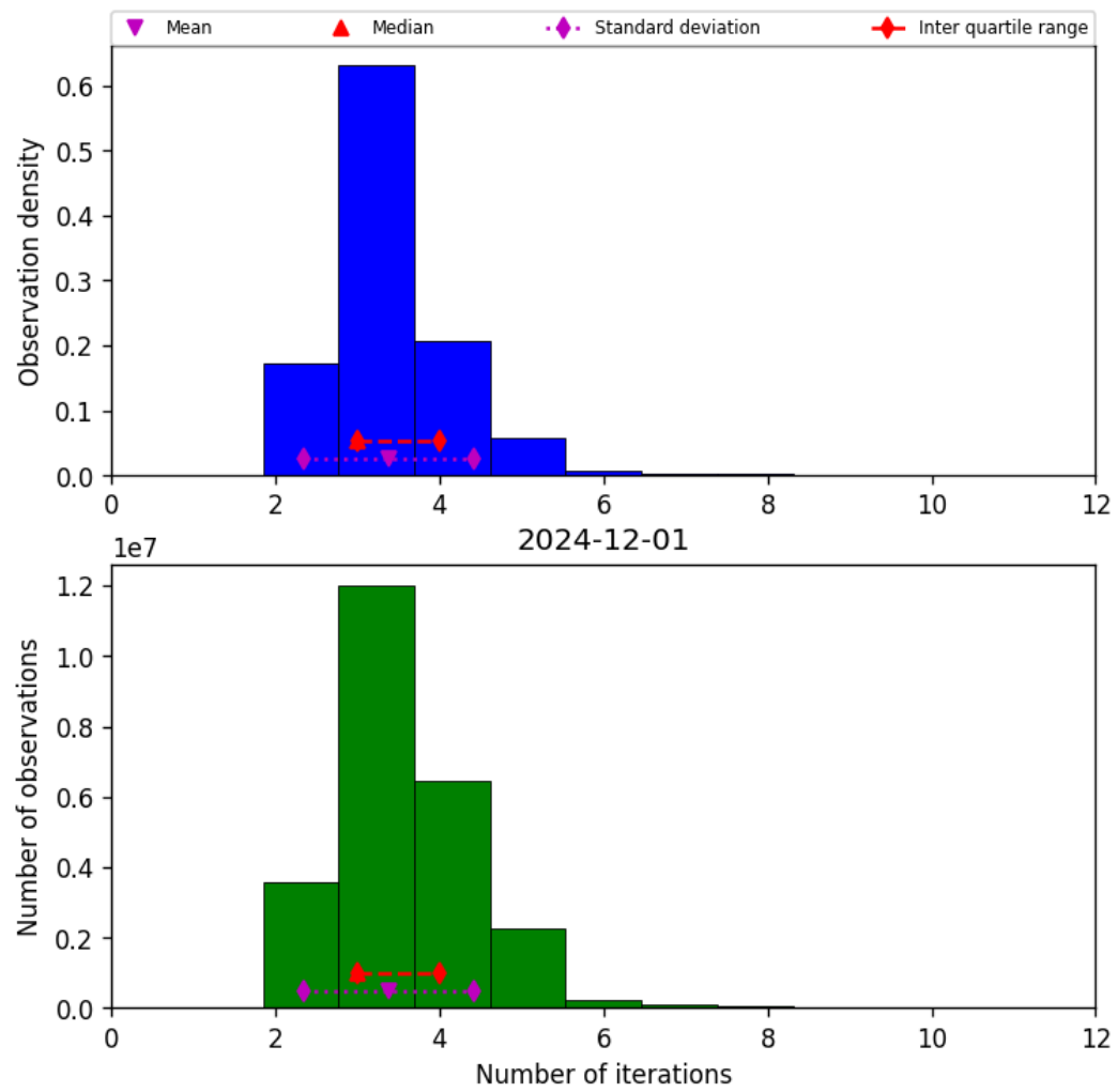
Figure 39: Histogram of “Number of iterations” for 2024-11-30 to 2024-12-02
