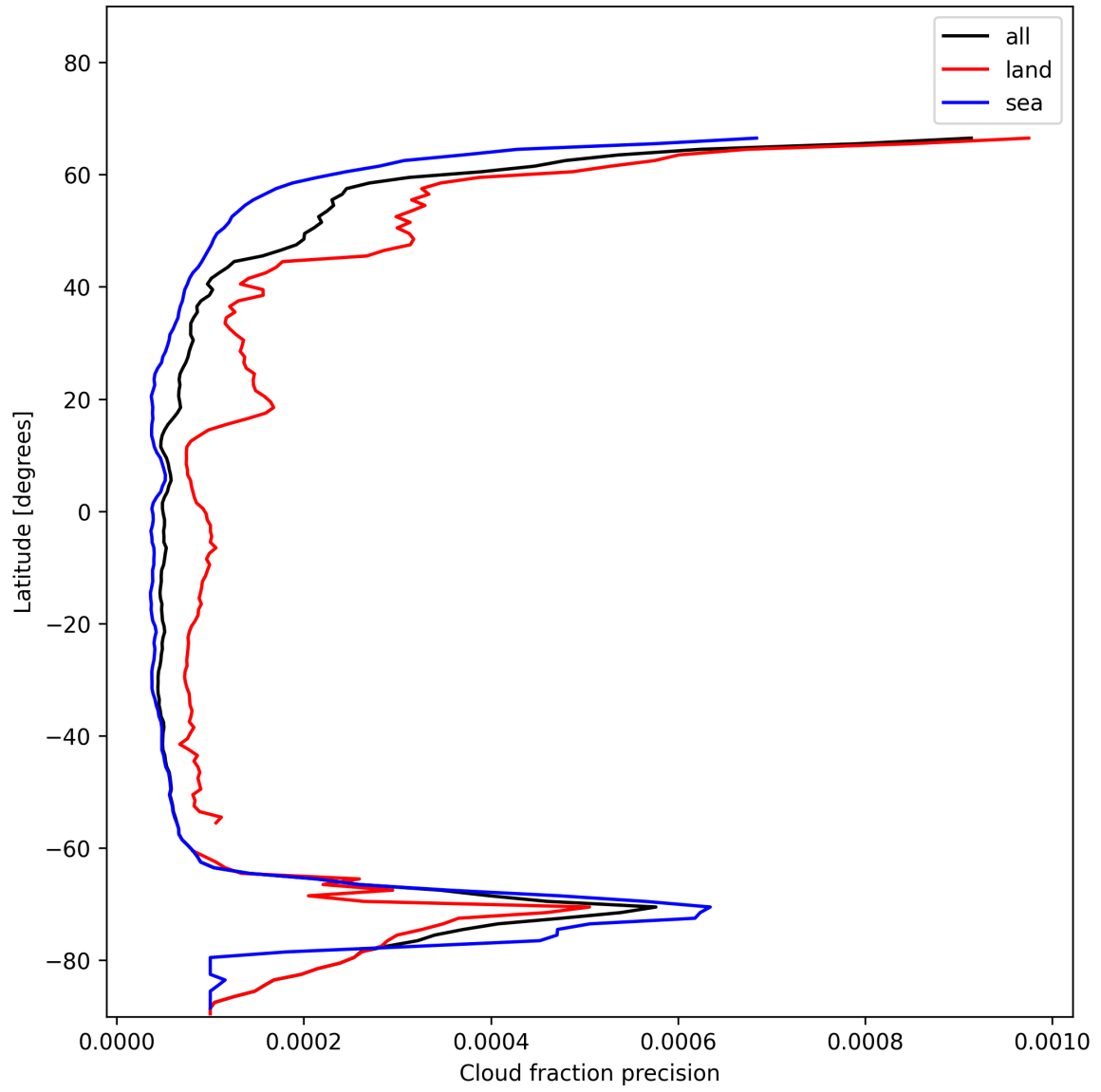
Figure 16: Zonal average of “Cloud fraction precision” for 2024-11-30 to 2024-12-02.
