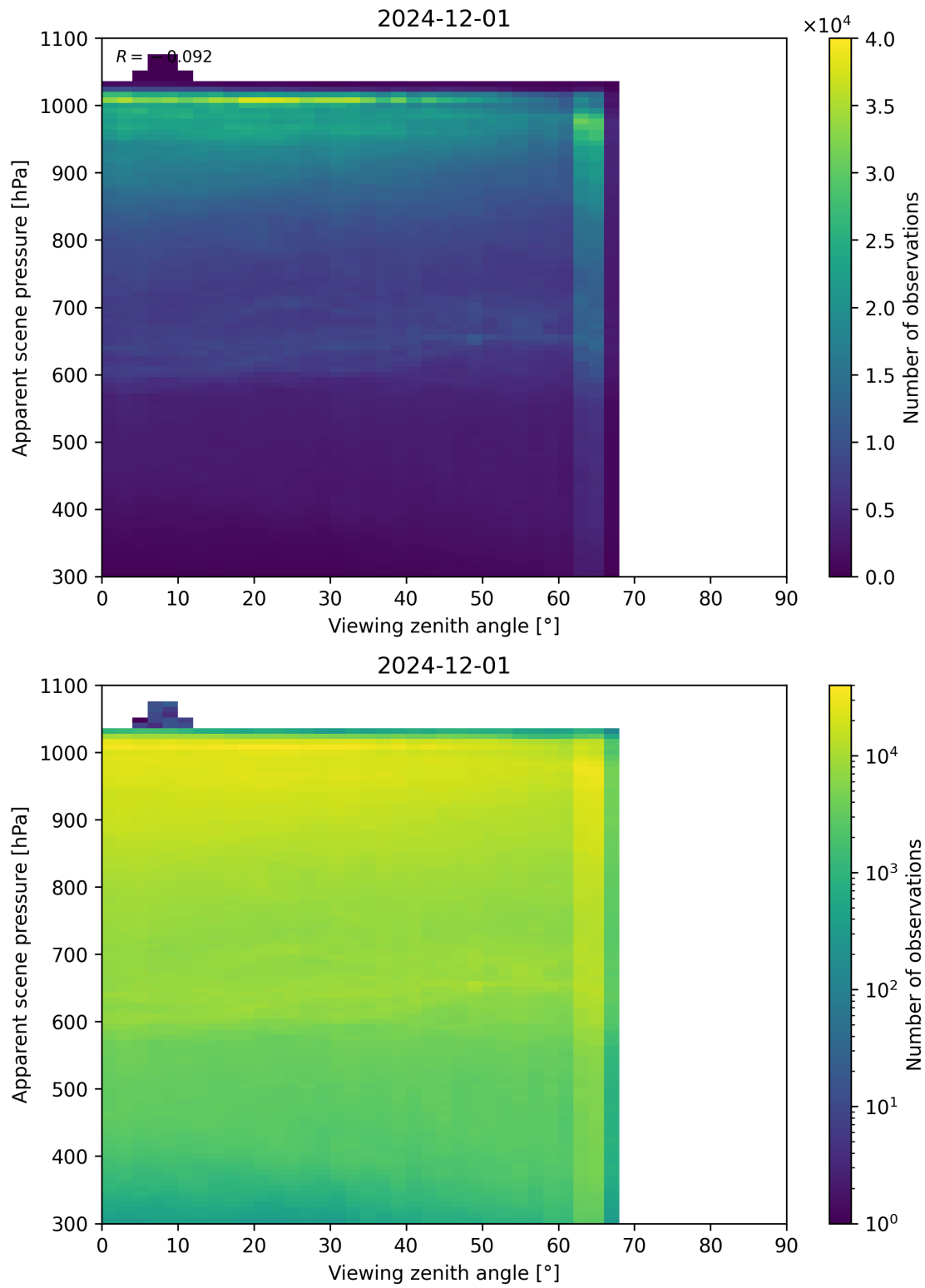
Figure 118: Scatter density plot of “Viewing zenith angle” against “Apparent scene pressure” for 2024-11-30 to 2024-12-02.
