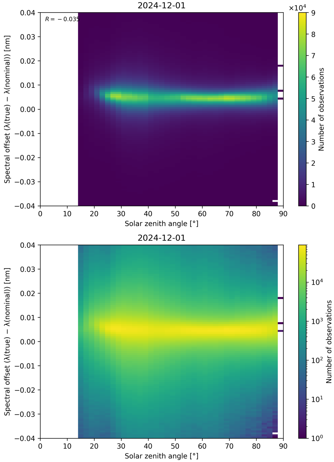
Figure 117: Scatter density plot of “Solar zenith angle” against “Spectral offset ( \lambda_{\text{true}} - \lambda_{\text{nominal}} )” for 2024-11-30 to 2024-12-02.
