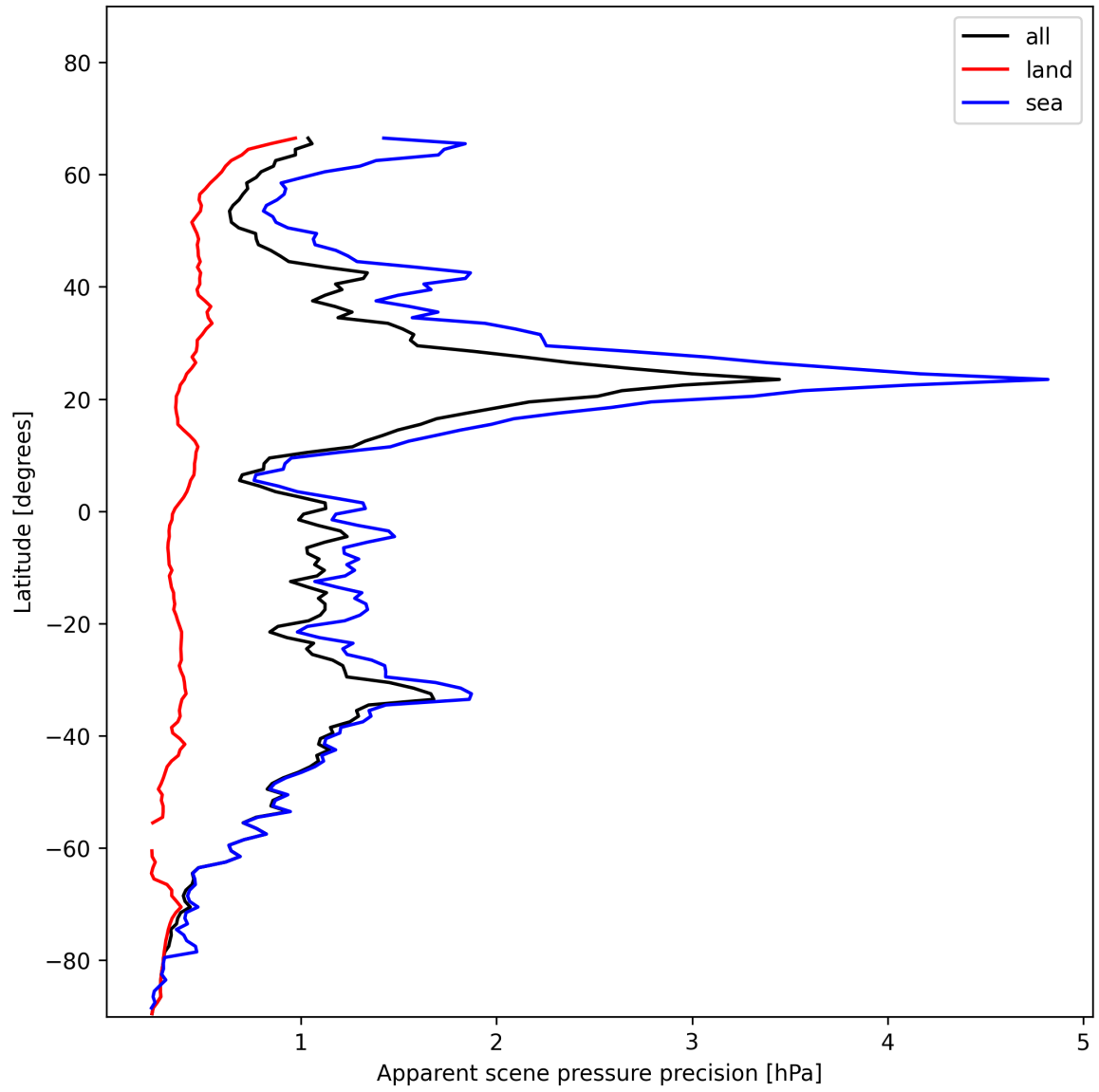
Figure 20: Zonal average of “Apparent scene pressure precision” for 2024-11-30 to 2024-12-02.
