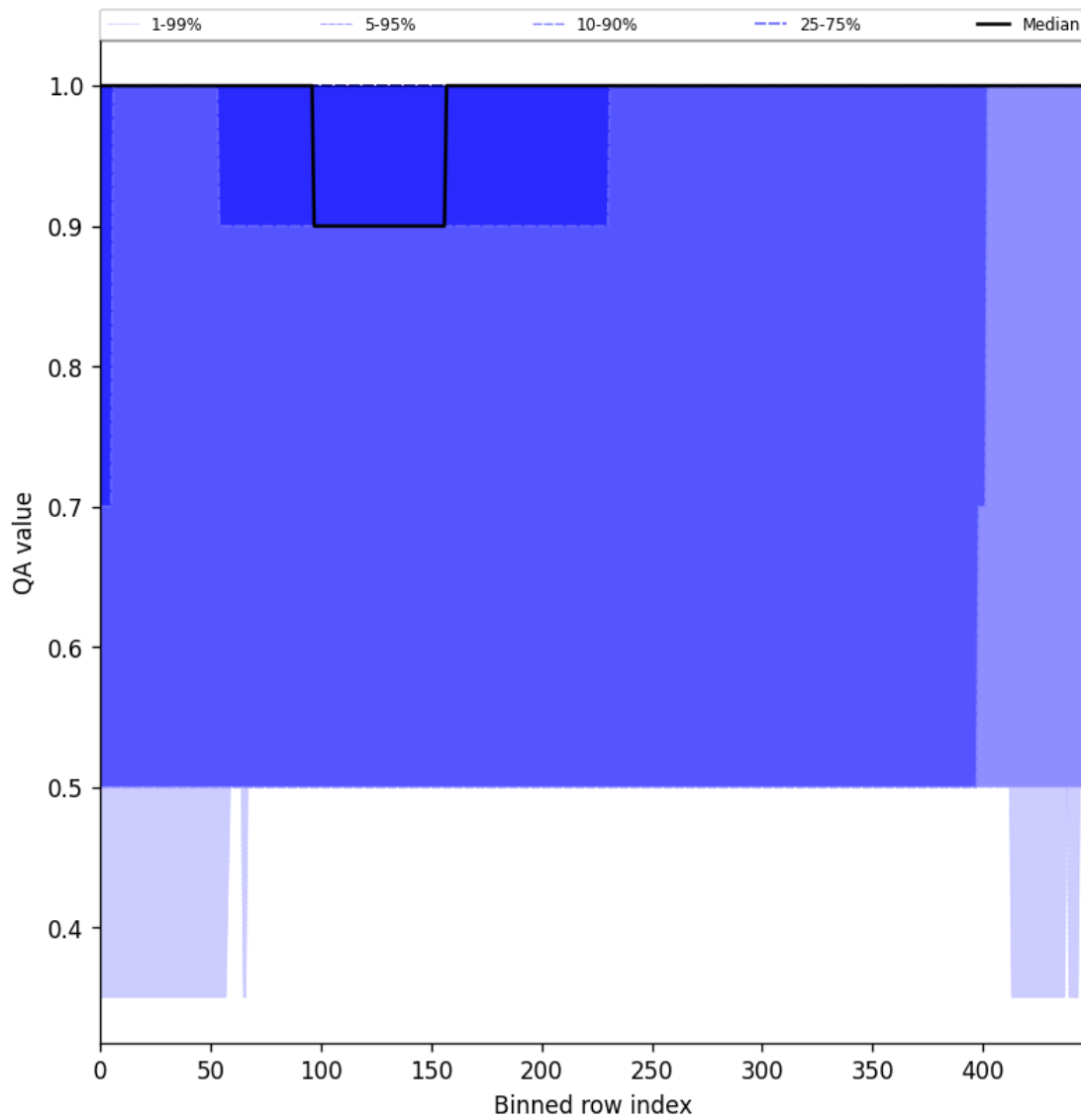
Figure 46: Along track statistics of “QA value” for 2024-11-30 to 2024-12-02
