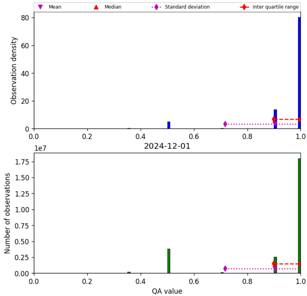
Figure 29: Histogram of “QA value” for 2024-11-30 to 2024-12-02
