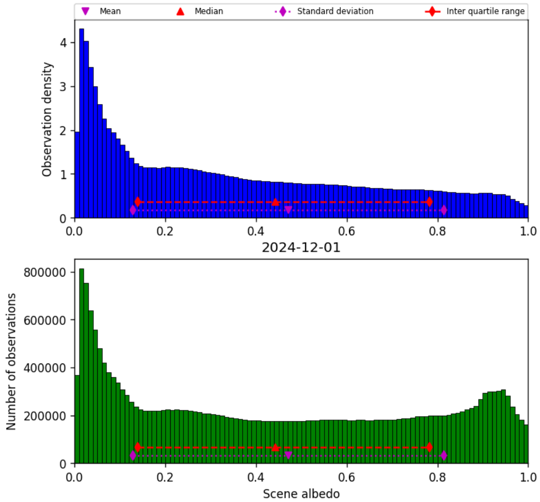
Figure 34: Histogram of “Scene albedo” for 2024-11-30 to 2024-12-02
