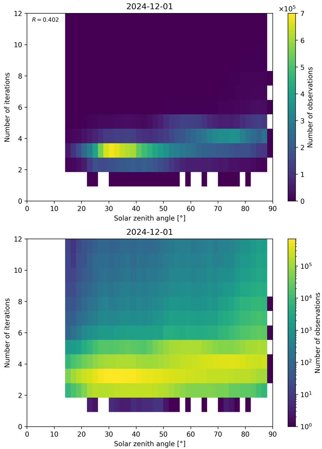
Figure 114: Scatter density plot of “Solar zenith angle” against “Number of iterations” for 2024-11-30 to 2024-12-02.
