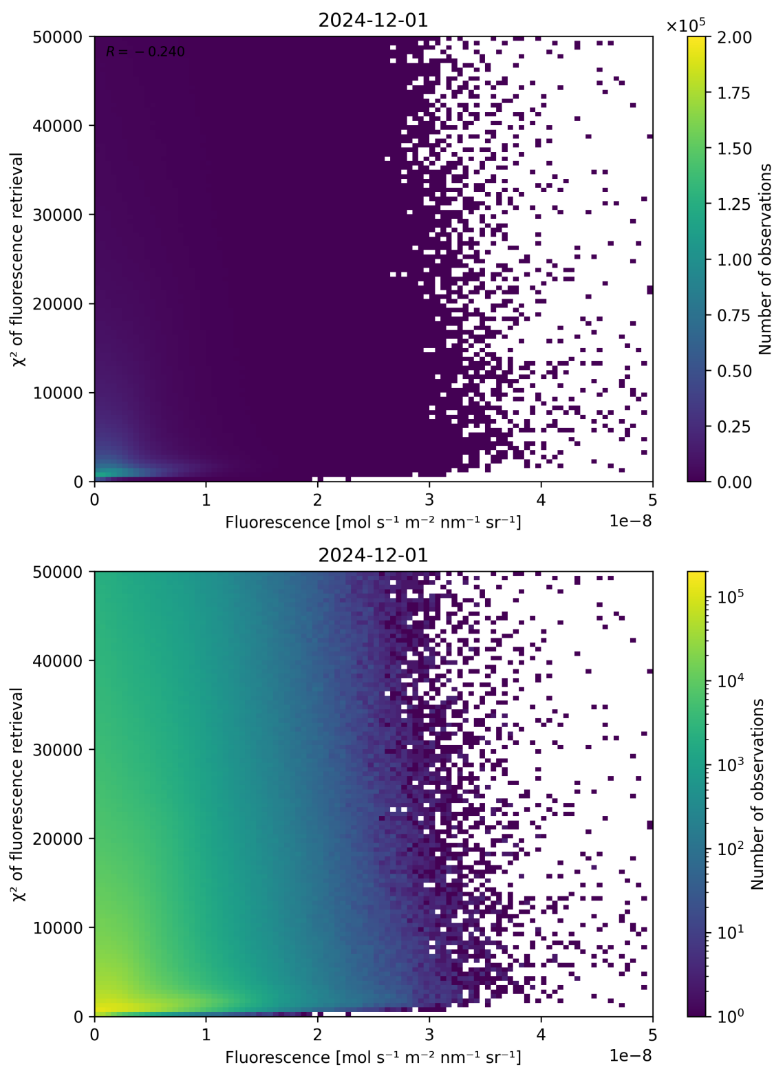
Figure 85: Scatter density plot of “Fluorescence” against “ \chi^2 of fluorescence retrieval” for 2024-11-30 to 2024-12-02.
