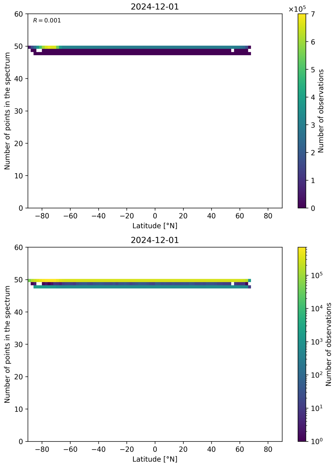
Figure 94: Scatter density plot of “Latitude” against “Number of points in the spectrum” for 2024-11-30 to 2024-12-02.
