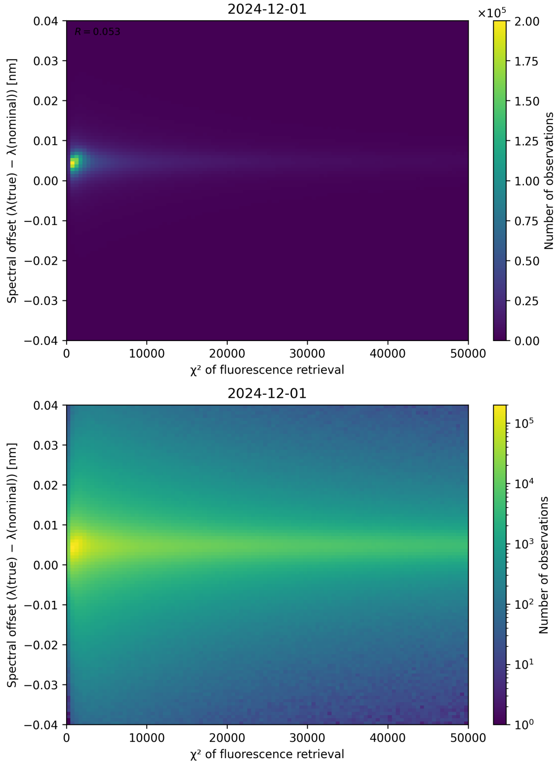
Figure 69: Scatter density plot of “ \chi^2 of fluorescence retrieval” against “Spectral offset ( \lambda_{\text{true}} - \lambda_{\text{nominal}} )” for 2024-11-30 to 2024-12-02.
