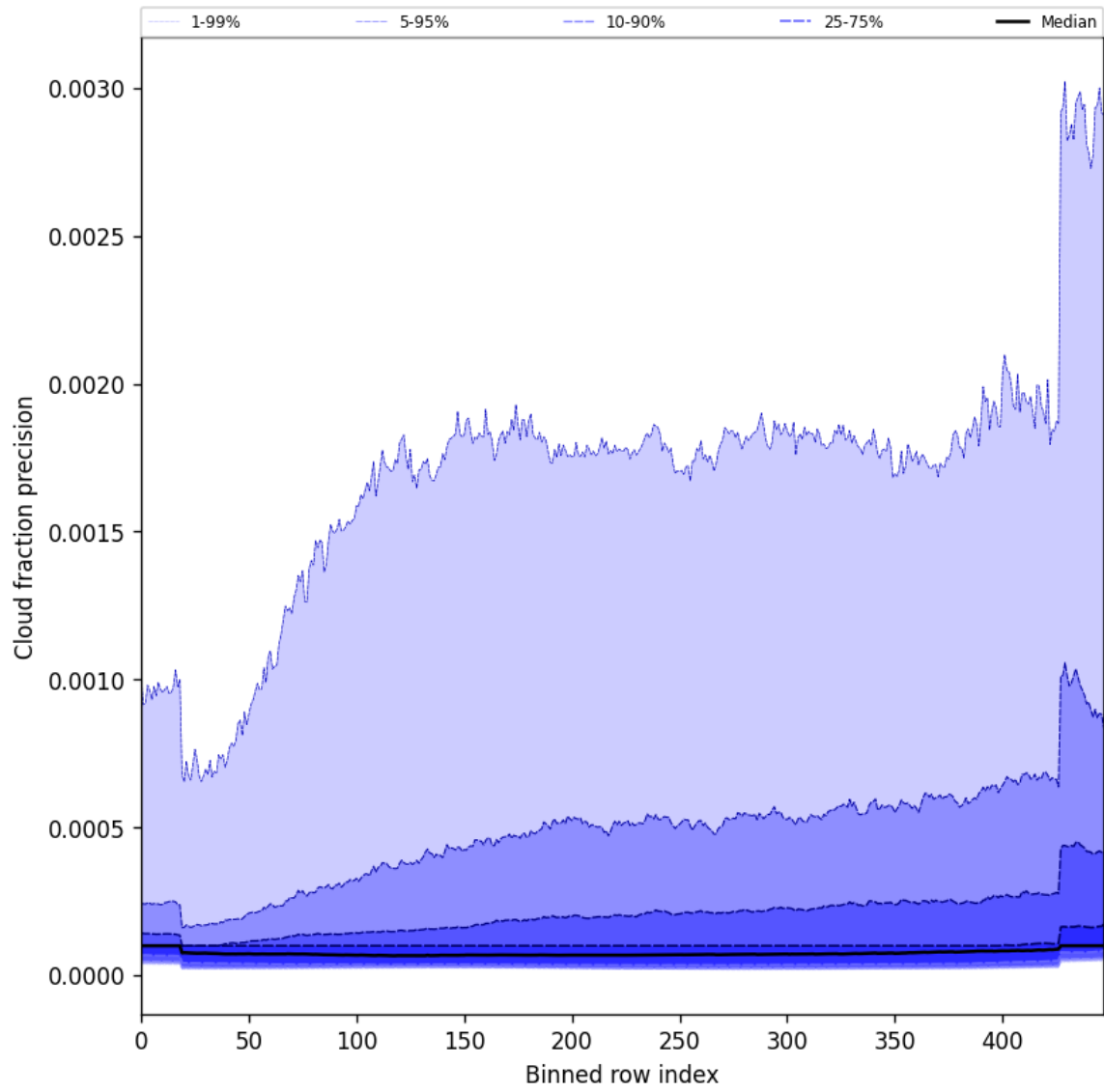
Figure 50: Along track statistics of “Cloud fraction precision” for 2024-11-30 to 2024-12-02
