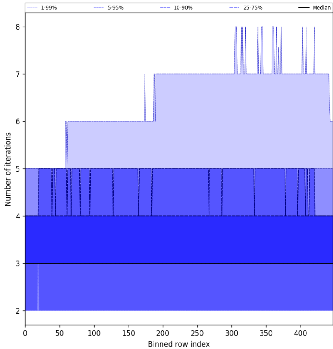
Figure 56: Along track statistics of “Number of iterations” for 2024-11-30 to 2024-12-02
