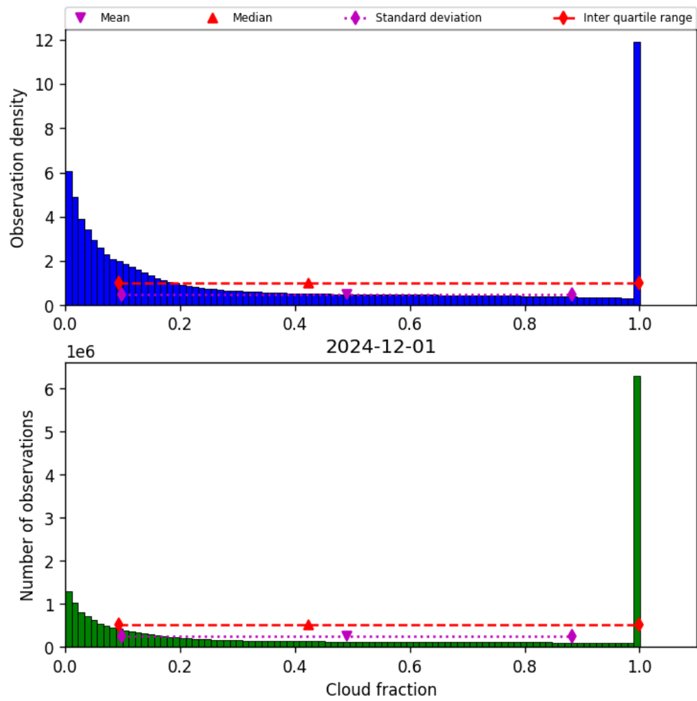
Figure 32: Histogram of “Cloud fraction” for 2024-11-30 to 2024-12-02
