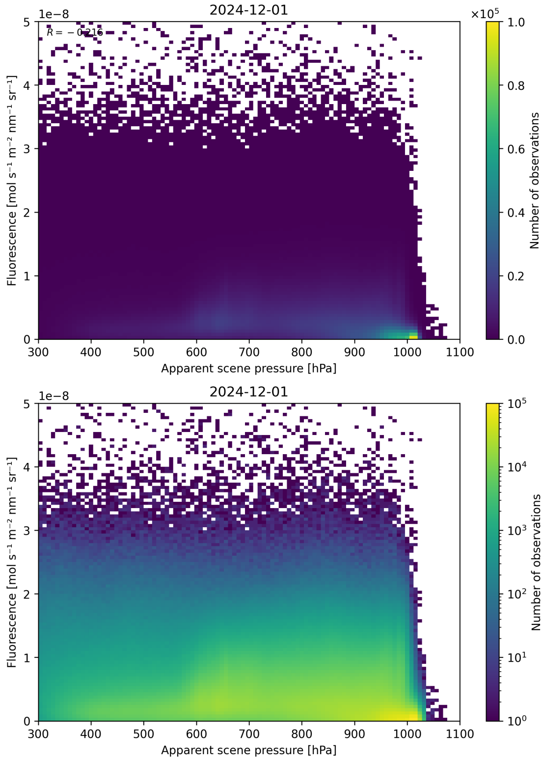
Figure 64: Scatter density plot of “Apparent scene pressure” against “Fluorescence” for 2024-11-30 to 2024-12-02.
