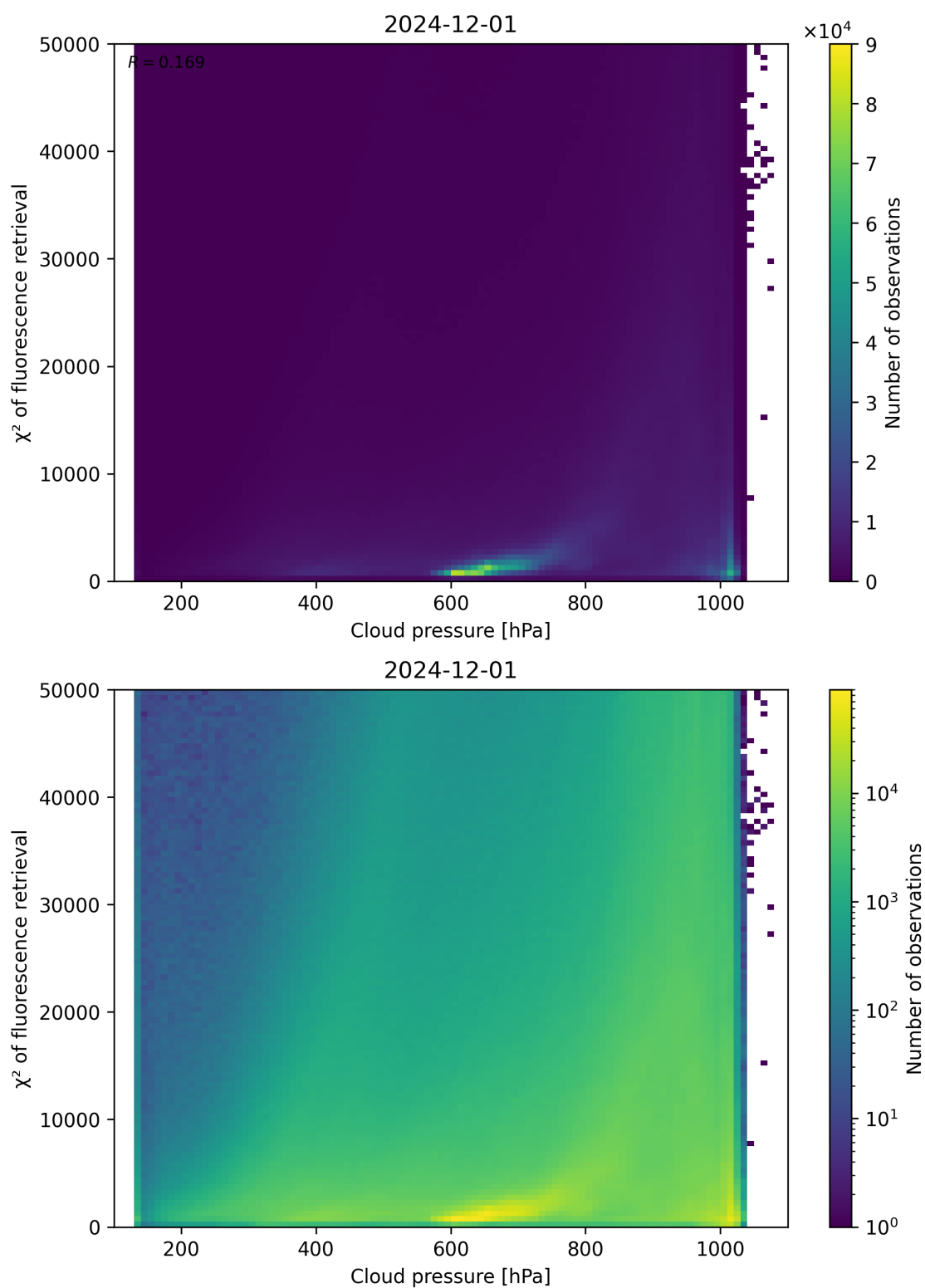
Figure 78: Scatter density plot of “Cloud pressure” against “ \chi^2 of fluorescence retrieval” for 2024-11-30 to 2024-12-02.
