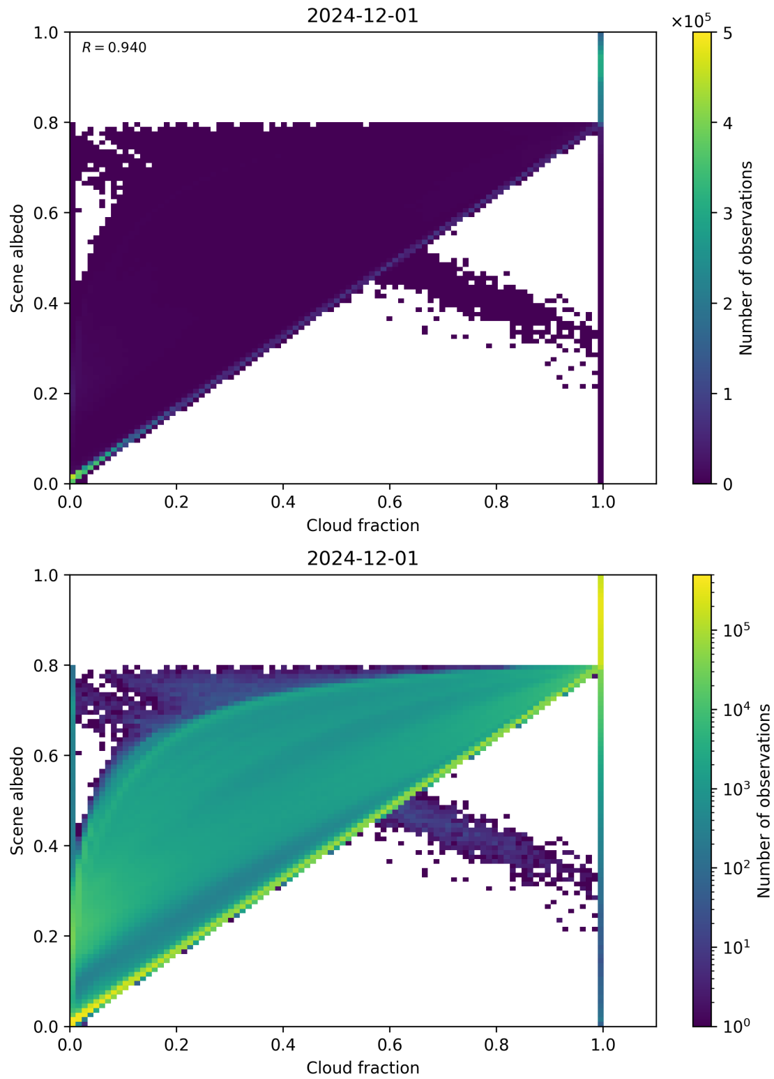
Figure 75: Scatter density plot of “Cloud fraction” against “Scene albedo” for 2024-11-30 to 2024-12-02.
