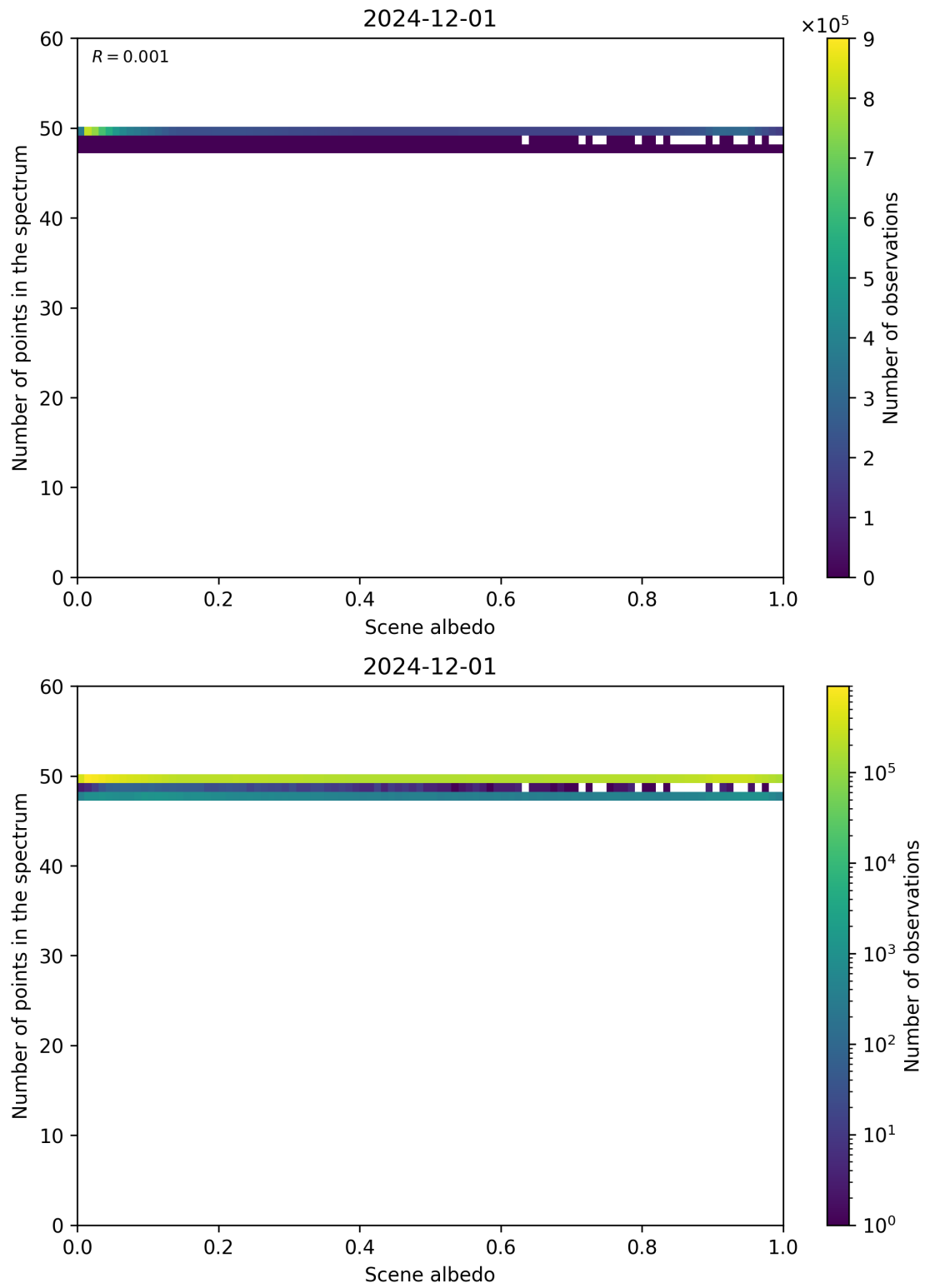
Figure 106: Scatter density plot of “Scene albedo” against “Number of points in the spectrum” for 2024-11-30 to 2024-12-02.
