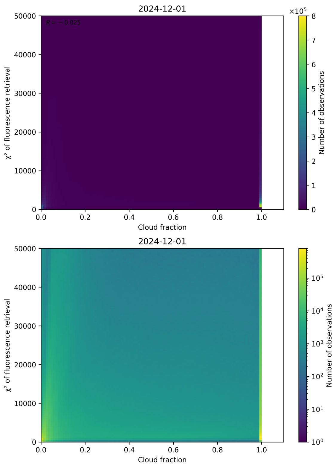
Figure 71: Scatter density plot of “Cloud fraction” against “ \chi^2 of fluorescence retrieval” for 2024-11-30 to 2024-12-02.
