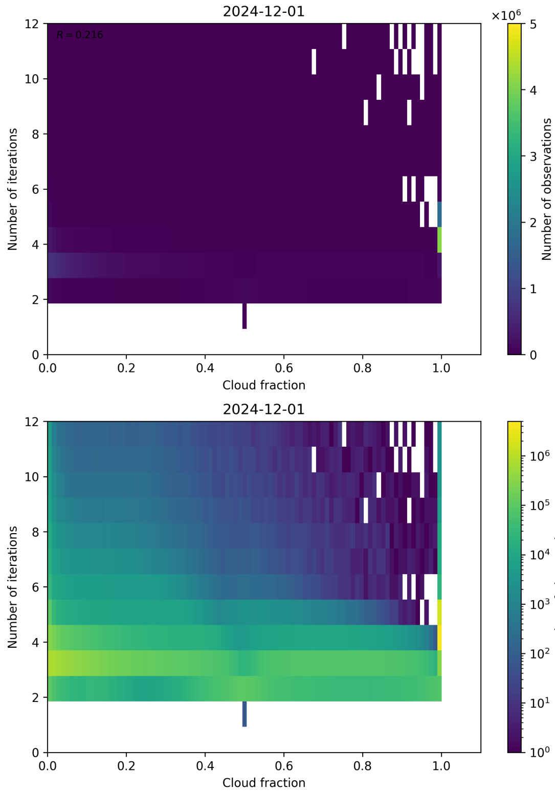
Figure 73: Scatter density plot of “Cloud fraction” against “Number of iterations” for 2024-11-30 to 2024-12-02.
