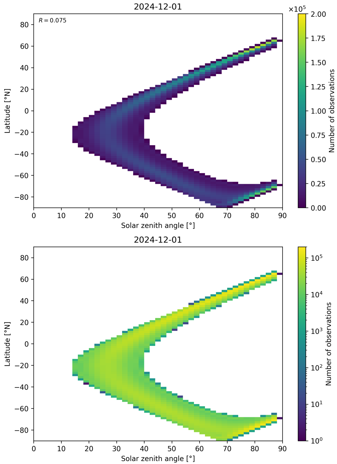
Figure 113: Scatter density plot of “Solar zenith angle” against “Latitude” for 2024-11-30 to 2024-12-02.
