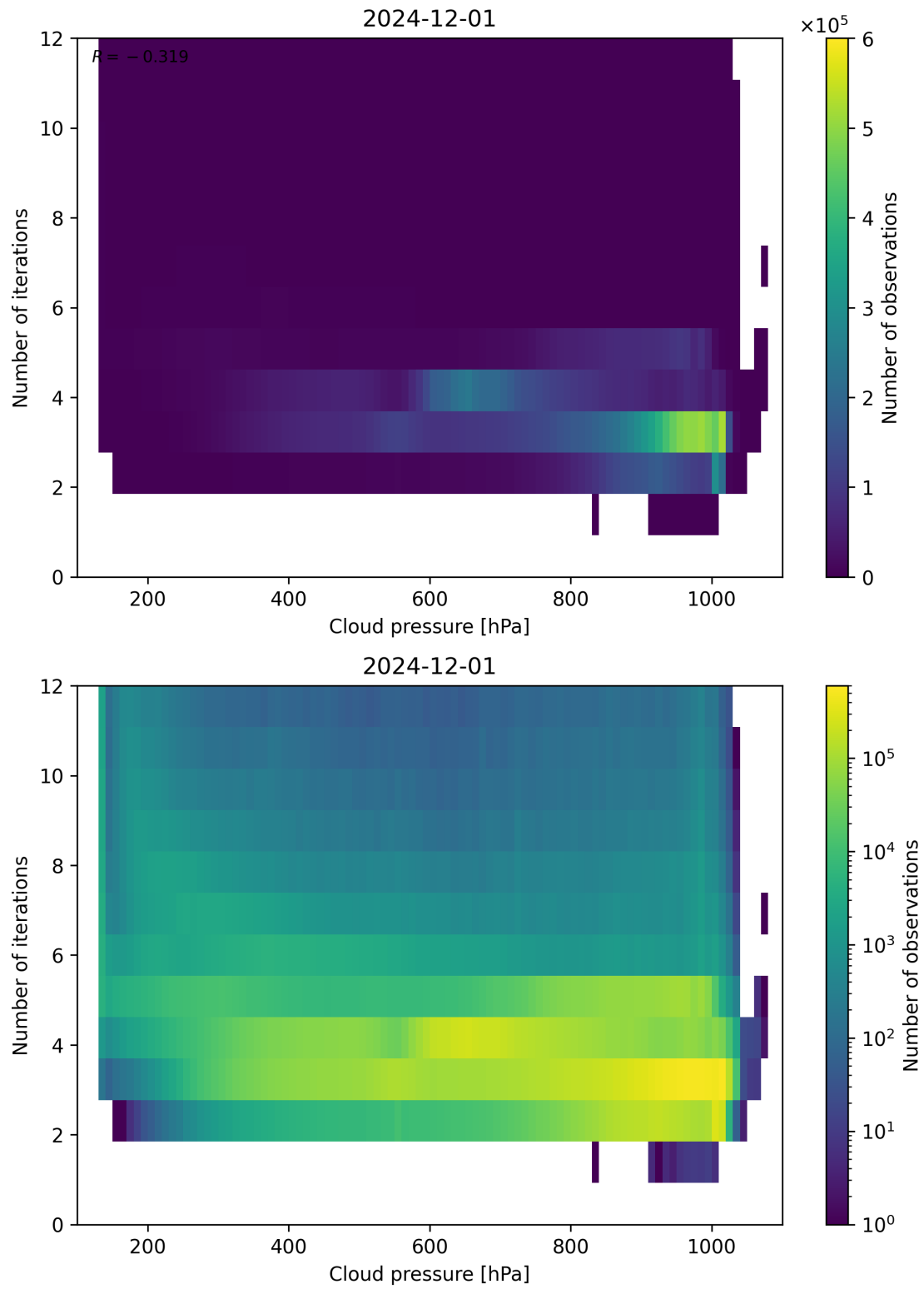
Figure 81: Scatter density plot of “Cloud pressure” against “Number of iterations” for 2024-11-30 to 2024-12-02.
