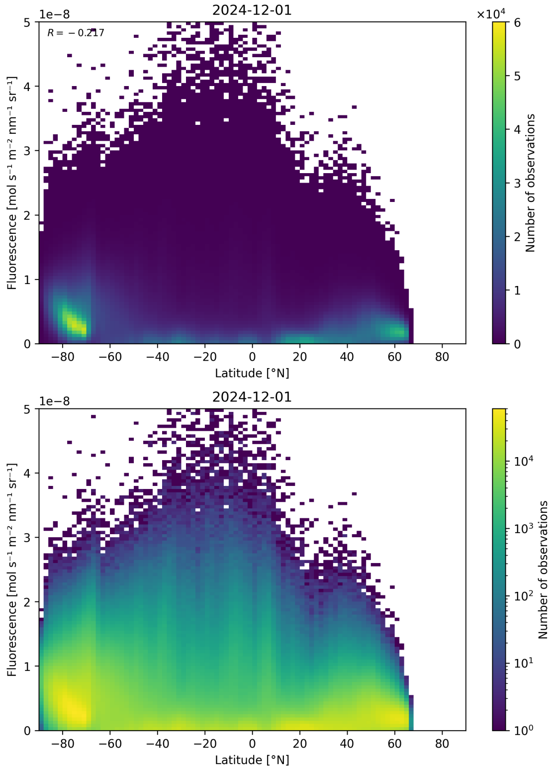
Figure 92: Scatter density plot of “Latitude” against “Fluorescence” for 2024-11-30 to 2024-12-02.
