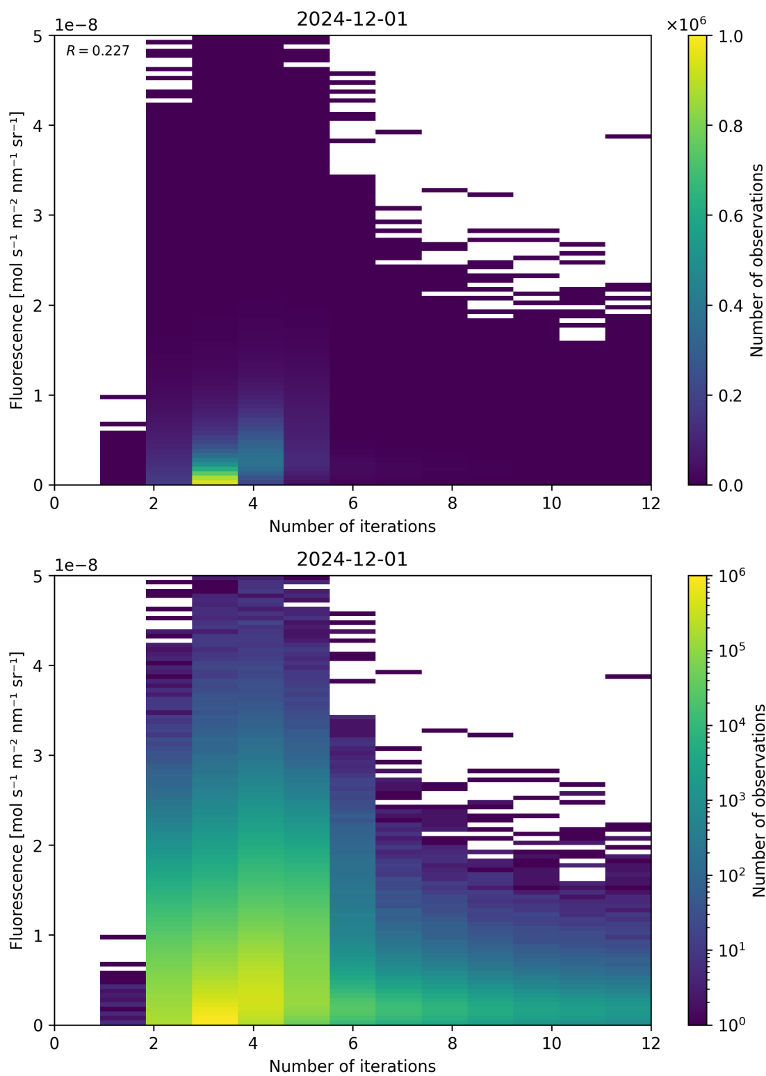
Figure 98: Scatter density plot of “Number of iterations” against “Fluorescence” for 2024-11-30 to 2024-12-02.
