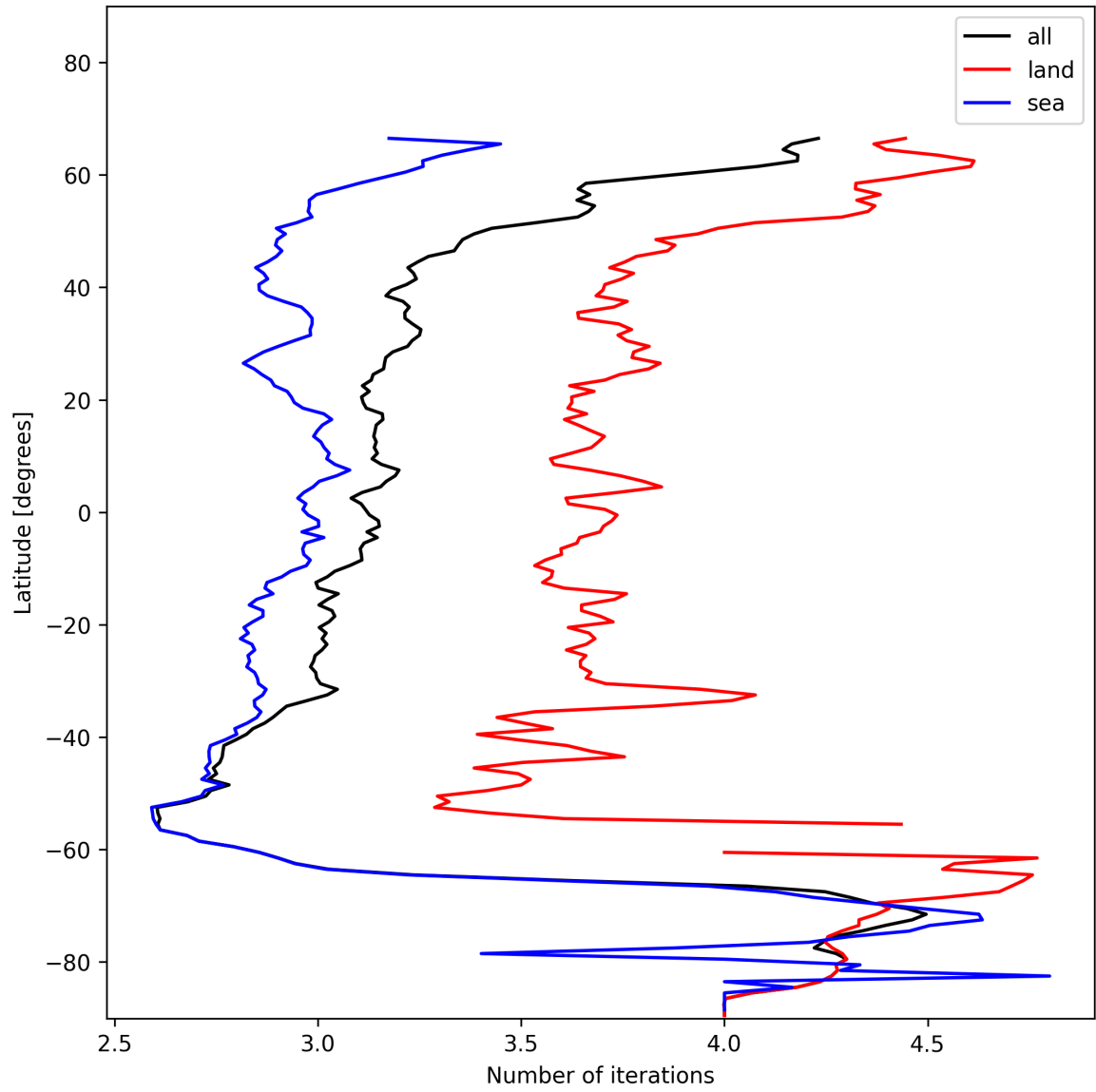
Figure 22: Zonal average of “Number of iterations” for 2024-11-30 to 2024-12-02.
