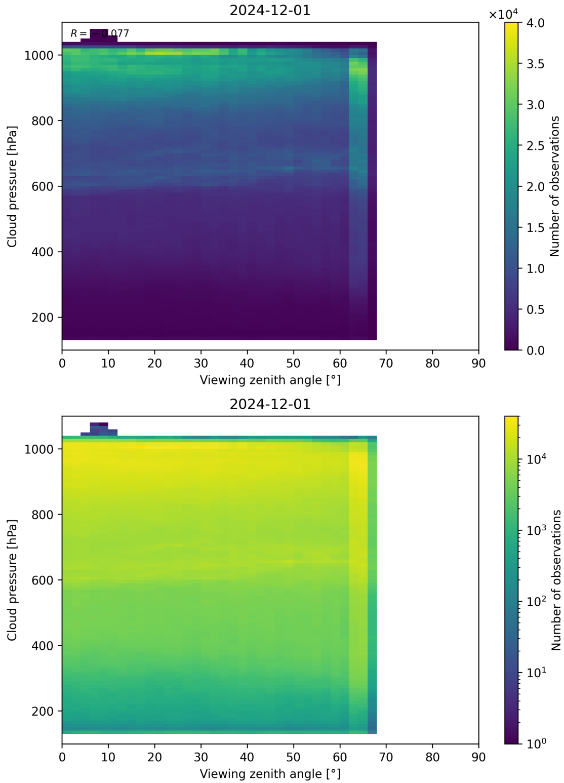
Figure 121: Scatter density plot of “Viewing zenith angle” against “Cloud pressure” for 2024-11-30 to 2024-12-02.
