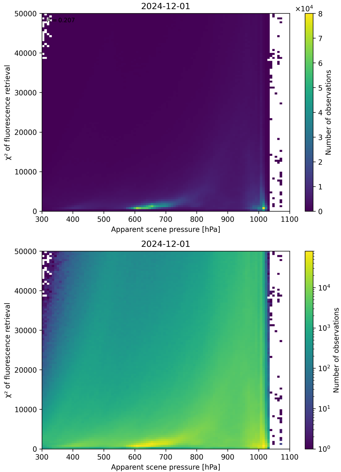
Figure 63: Scatter density plot of “Apparent scene pressure” against “ \chi^2 of fluorescence retrieval” for 2024-11-30 to 2024-12-02.
