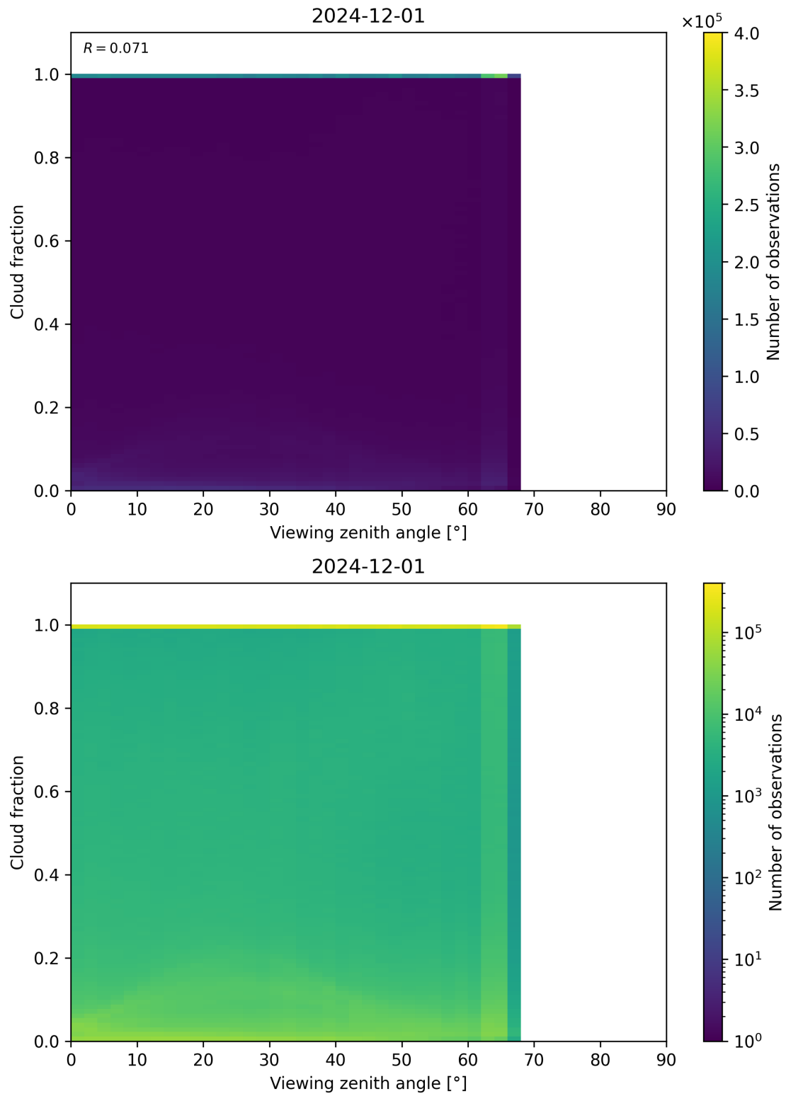
Figure 120: Scatter density plot of “Viewing zenith angle” against “Cloud fraction” for 2024-11-30 to 2024-12-02.
