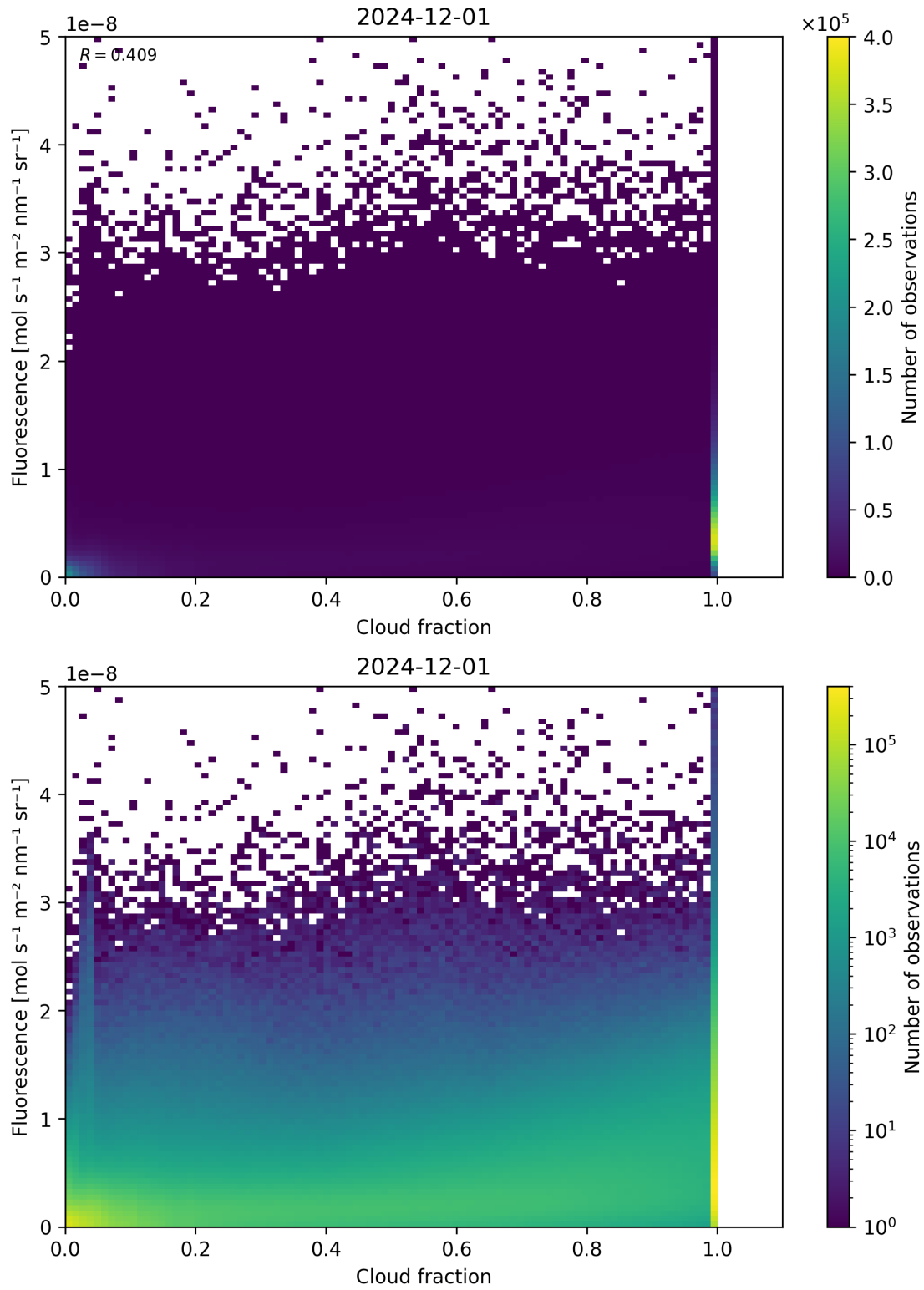
Figure 72: Scatter density plot of “Cloud fraction” against “Fluorescence” for 2024-11-30 to 2024-12-02.
