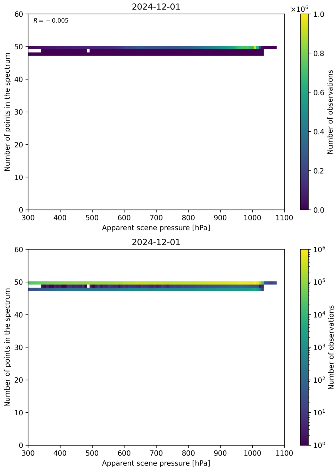
Figure 66: Scatter density plot of “Apparent scene pressure” against “Number of points in the spectrum” for 2024-11-30 to 2024-12-02.
