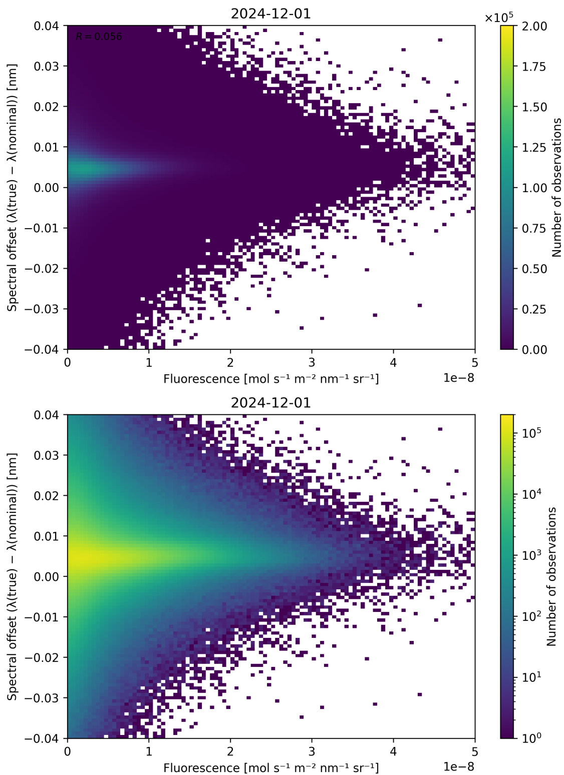
Figure 87: Scatter density plot of “Fluorescence” against “Spectral offset ( \lambda_{\text{true}} - \lambda_{\text{nominal}} )” for 2024-11-30 to 2024-12-02.
