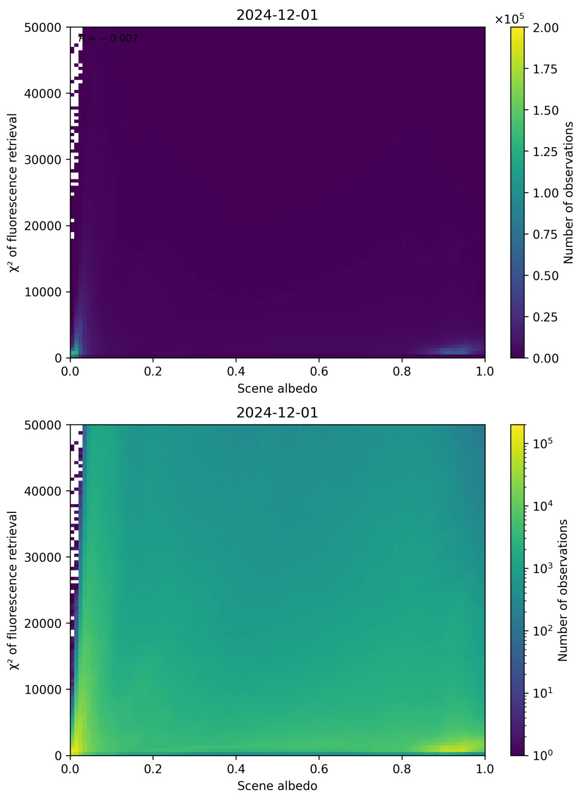
Figure 103: Scatter density plot of “Scene albedo” against “ \chi^2 of fluorescence retrieval” for 2024-11-30 to 2024-12-02.
