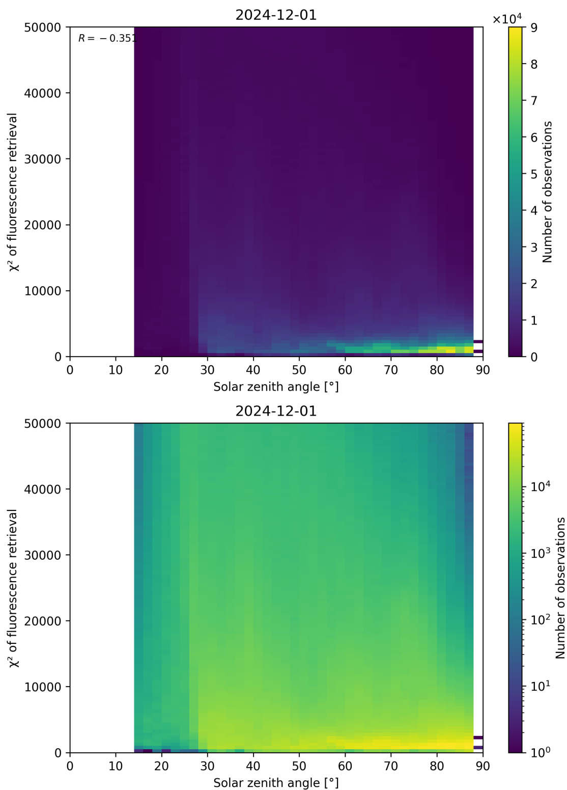
Figure 109: Scatter density plot of “Solar zenith angle” against “ \chi^2 of fluorescence retrieval” for 2024-11-30 to 2024-12-02.
