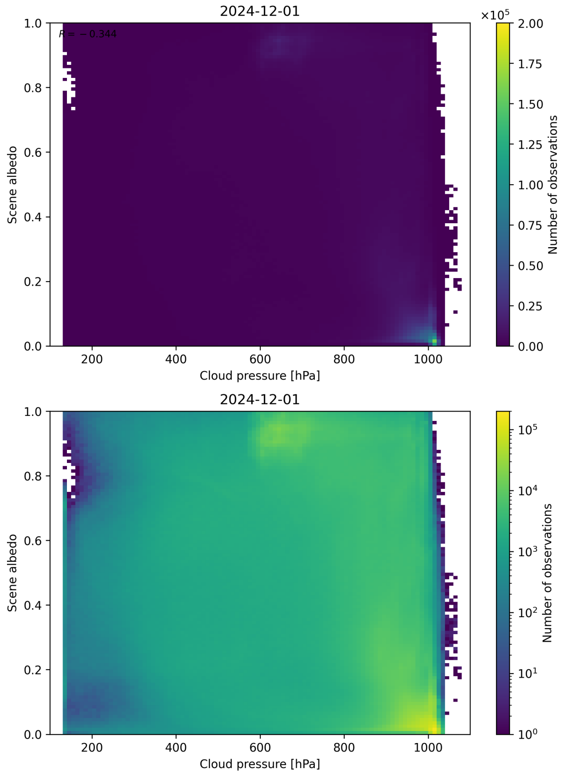
Figure 83: Scatter density plot of “Cloud pressure” against “Scene albedo” for 2024-11-30 to 2024-12-02.
