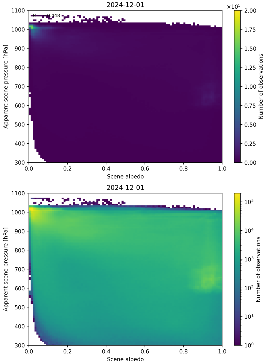
Figure 102: Scatter density plot of “Scene albedo” against “Apparent scene pressure” for 2024-11-30 to 2024-12-02.
