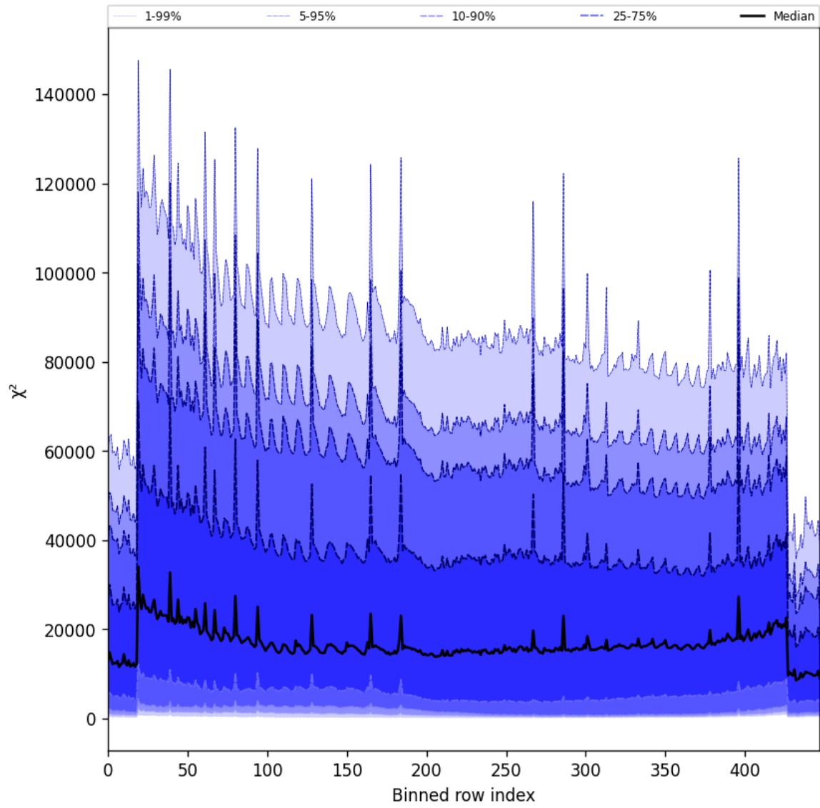
Figure 55: Along track statistics of “ \chi^2 ” for 2024-11-30 to 2024-12-02
