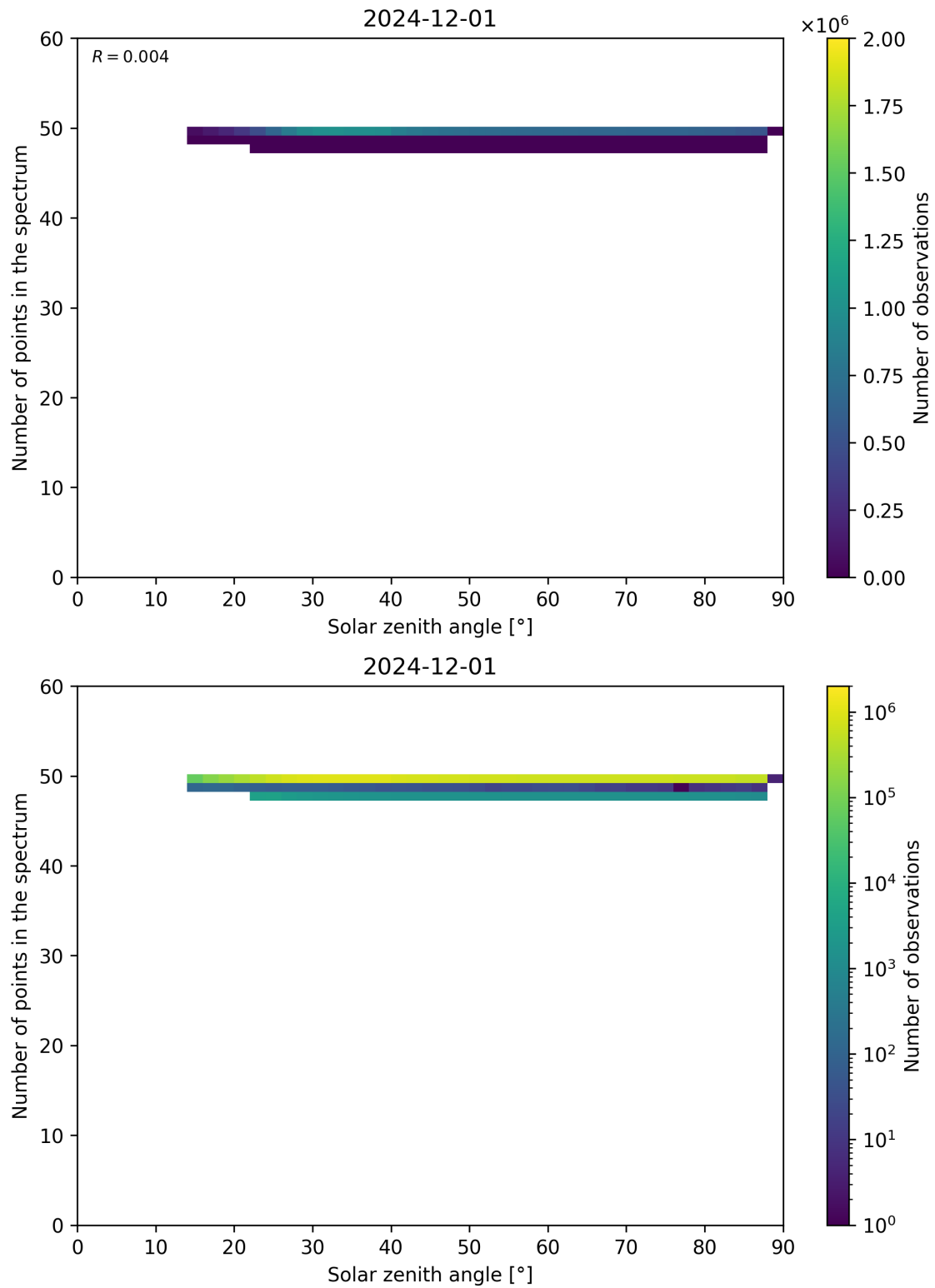
Figure 115: Scatter density plot of “Solar zenith angle” against “Number of points in the spectrum” for 2024-11-30 to 2024-12-02.
