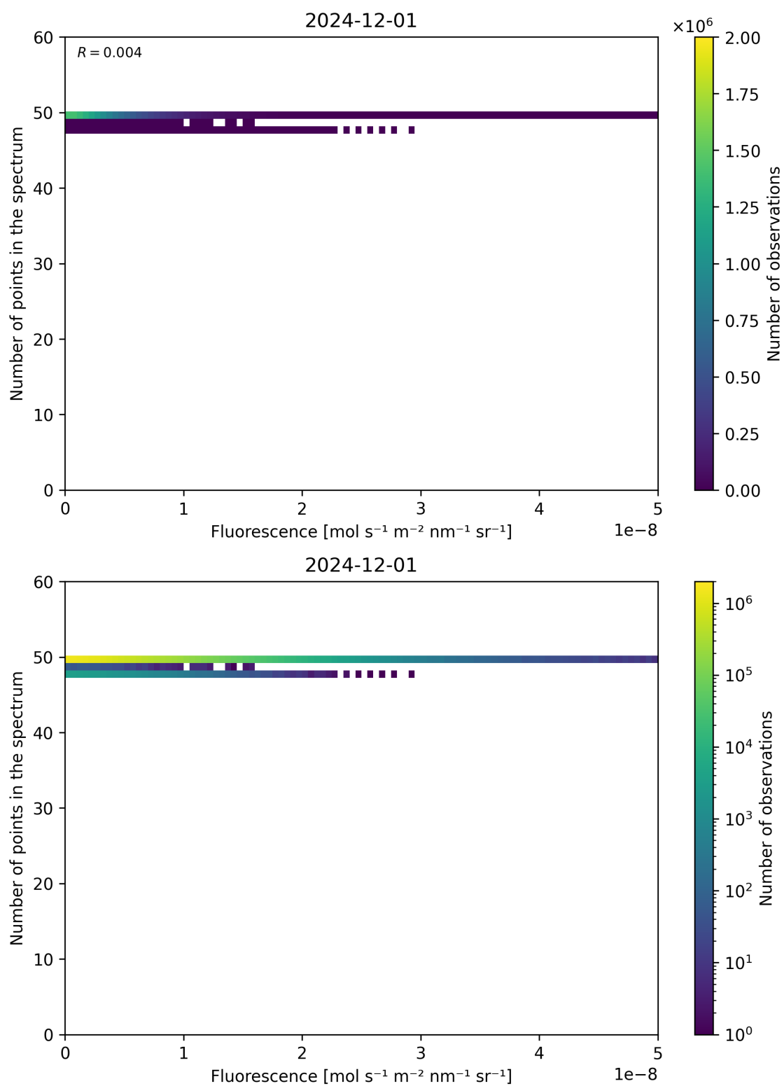
Figure 86: Scatter density plot of “Fluorescence” against “Number of points in the spectrum” for 2024-11-30 to 2024-12-02.
