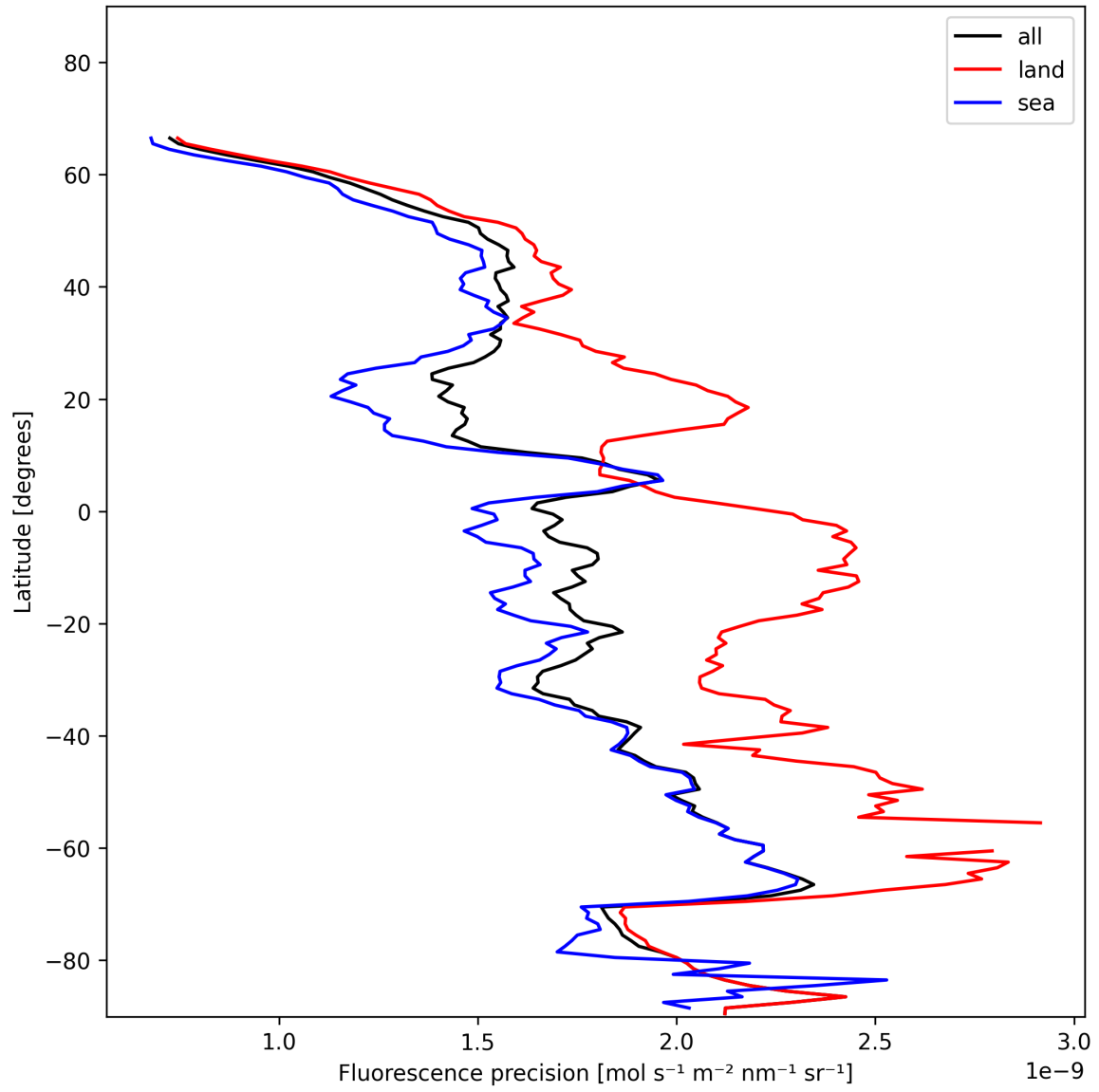
Figure 24: Zonal average of “Fluorescence precision” for 2024-11-30 to 2024-12-02.
