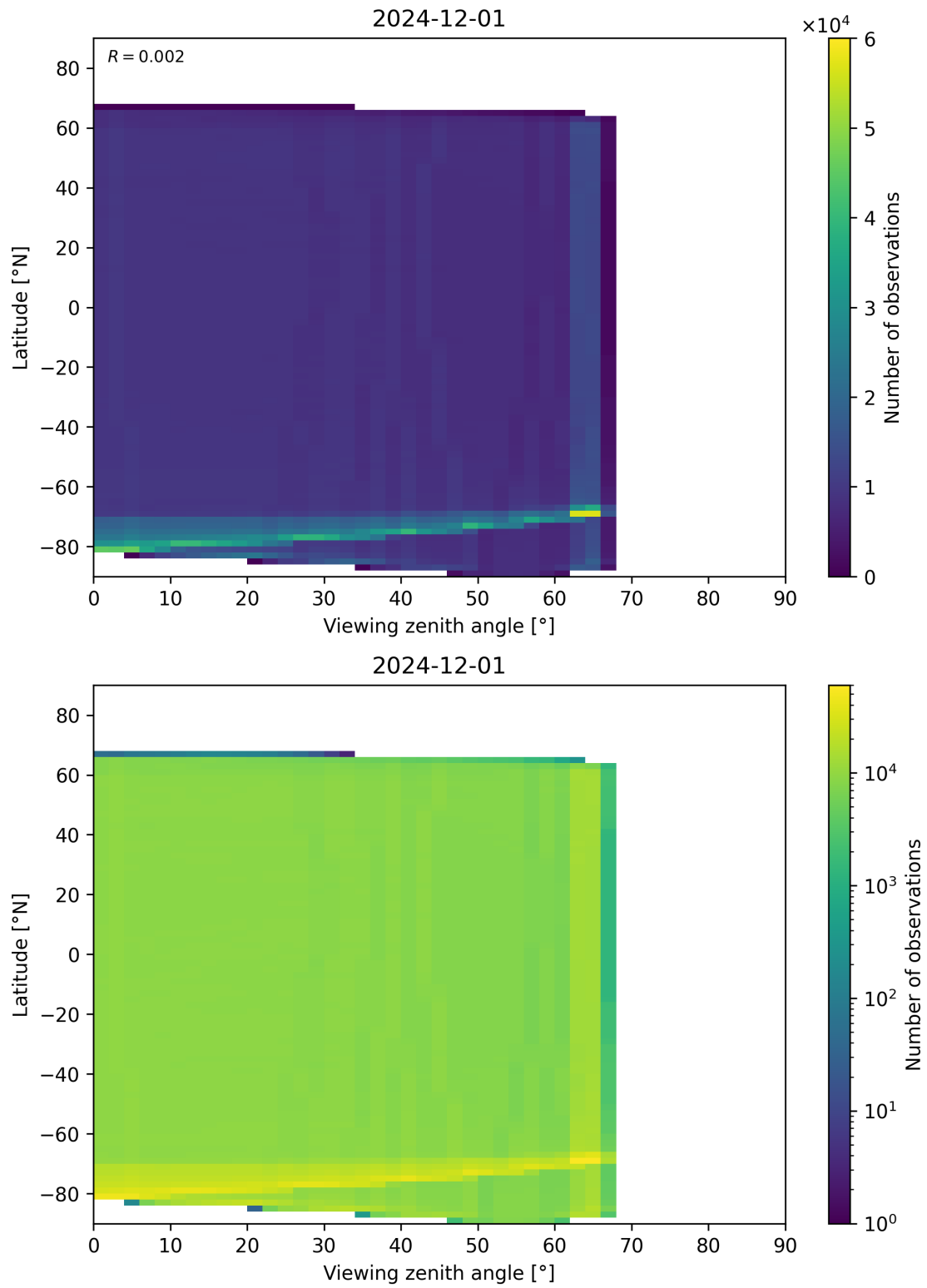
Figure 123: Scatter density plot of “Viewing zenith angle” against “Latitude” for 2024-11-30 to 2024-12-02.
