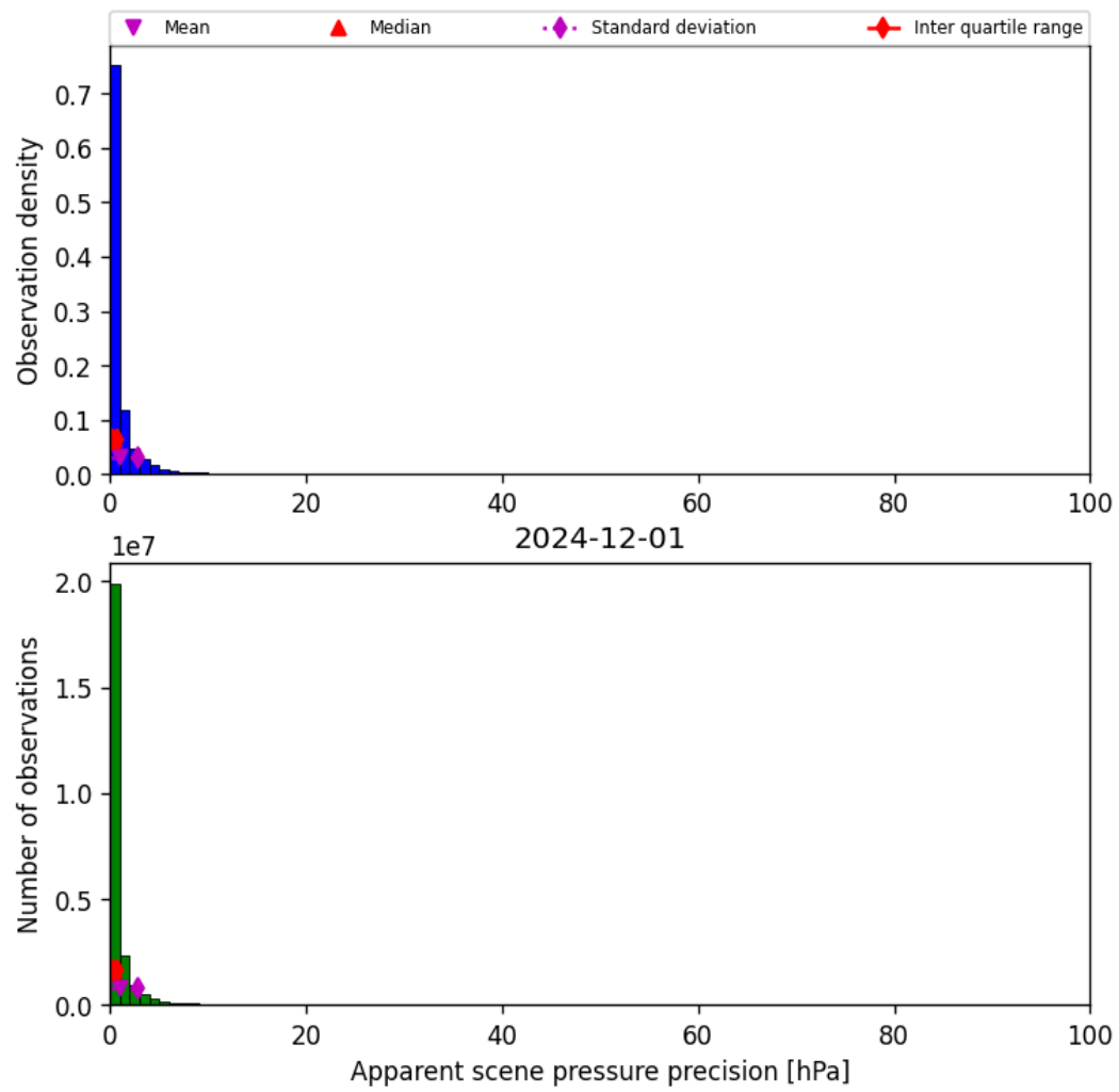
Figure 37: Histogram of “Apparent scene pressure precision” for 2024-11-30 to 2024-12-02
