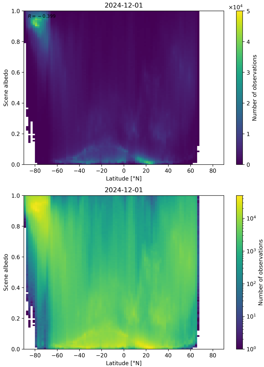
Figure 95: Scatter density plot of “Latitude” against “Scene albedo” for 2024-11-30 to 2024-12-02.
