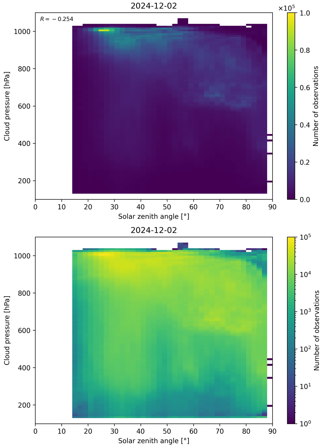
Figure 111: Scatter density plot of “Solar zenith angle” against “Cloud pressure” for 2024-12-01 to 2024-12-03.
