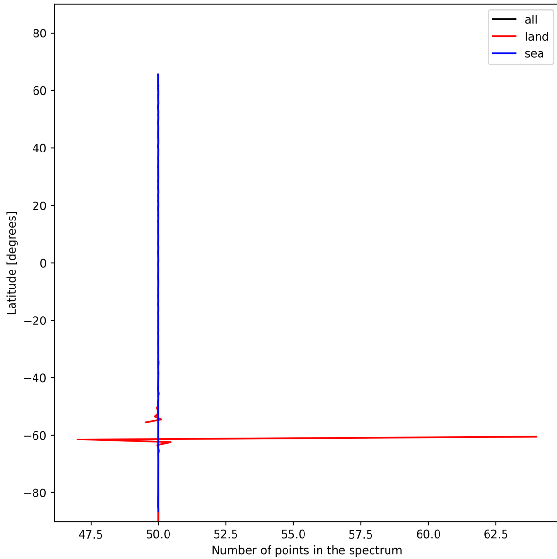
Figure 27: Zonal average of “Number of points in the spectrum” for 2024-12-01 to 2024-12-03.
