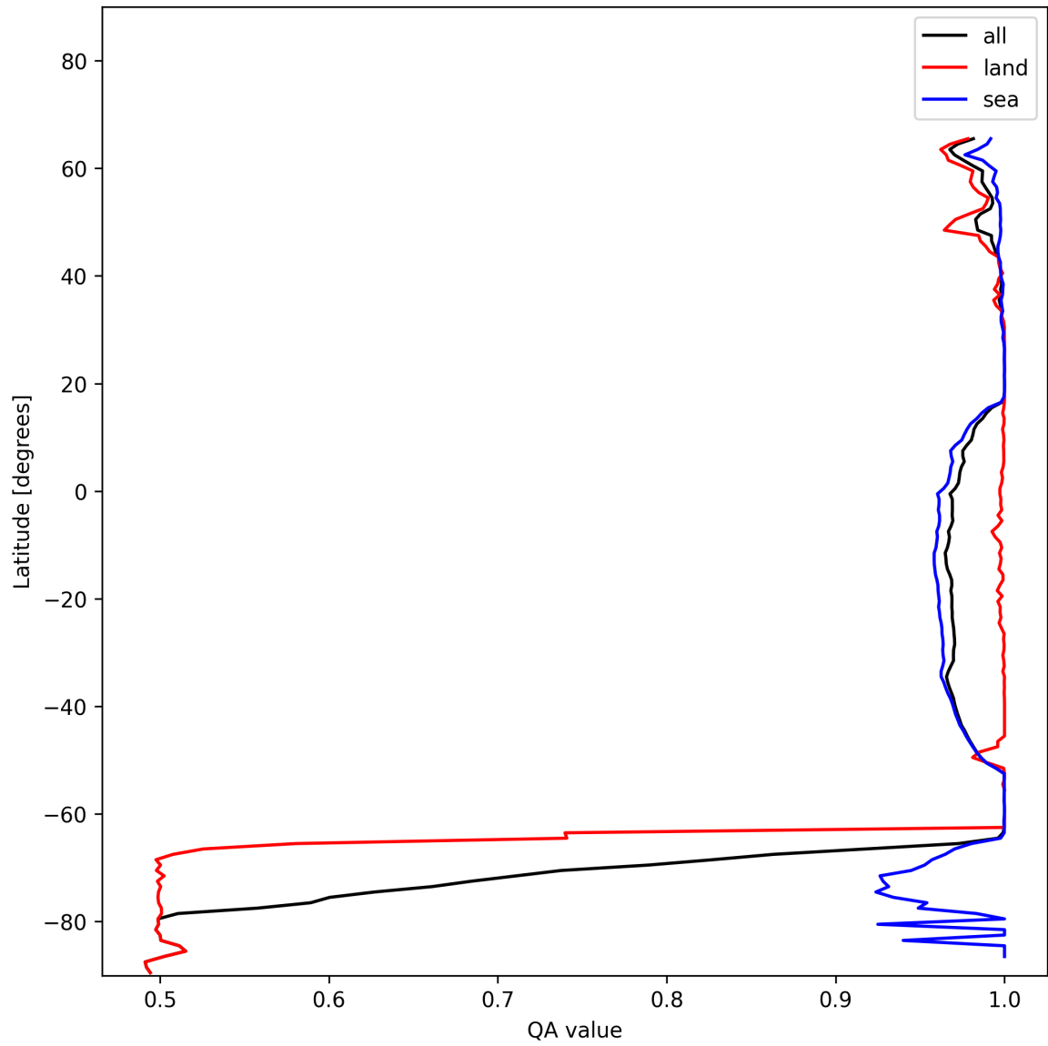
Figure 12: Zonal average of “QA value” for 2024-12-01 to 2024-12-03.
