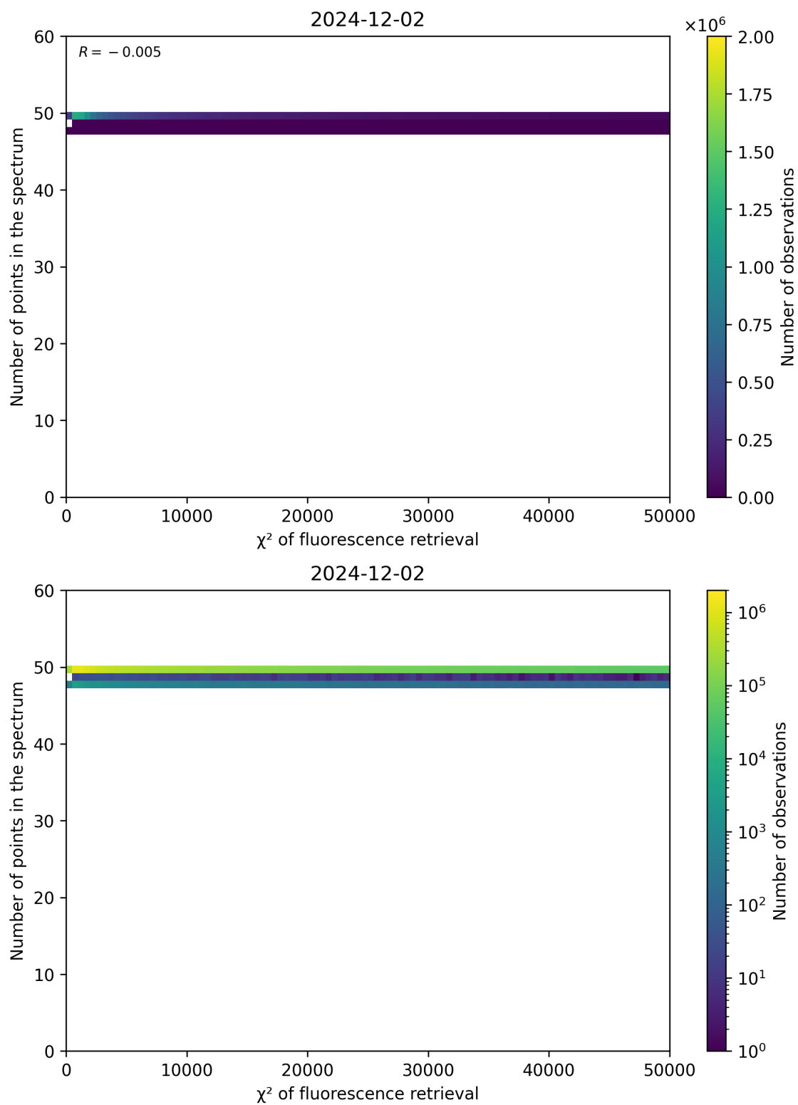
Figure 68: Scatter density plot of " \chi^2 of fluorescence retrieval" against "Number of points in the spectrum" for 2024-12-01 to 2024-12-03.
