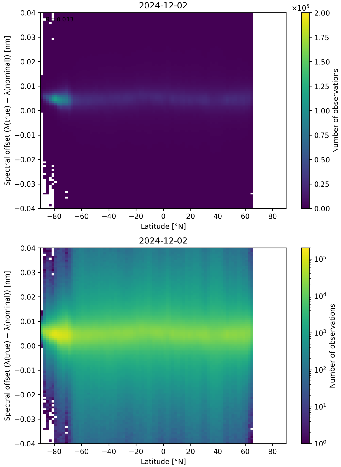
Figure 96: Scatter density plot of “Latitude” against “Spectral offset ( \lambda_{\text{true}} - \lambda_{\text{nominal}} )” for 2024-12-01 to 2024-12-03.
