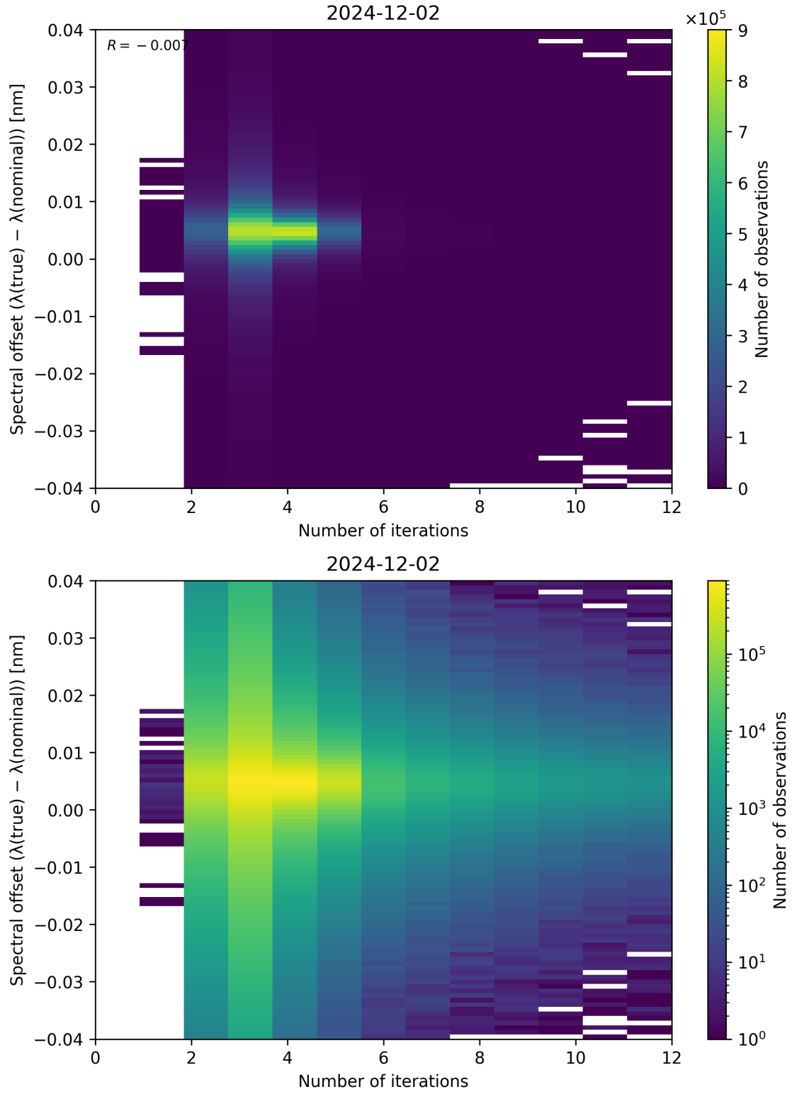
Figure 100: Scatter density plot of “Number of iterations” against “Spectral offset ( \lambda_{\text{true}} - \lambda_{\text{nominal}} )” for 2024-12-01 to 2024-12-03.
