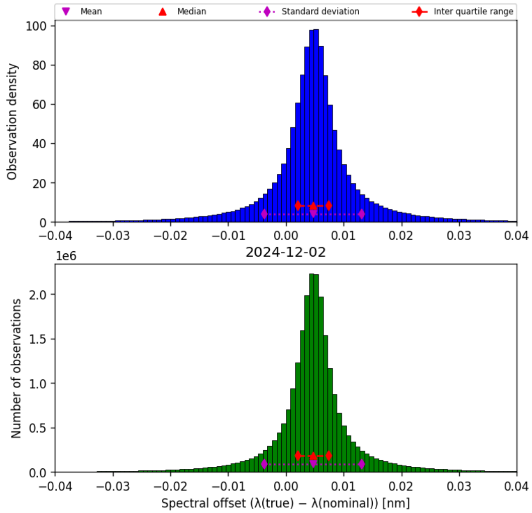
Figure 45: Histogram of “Spectral offset ( \lambda_{\text{true}} - \lambda_{\text{nominal}} )” for 2024-12-01 to 2024-12-03
