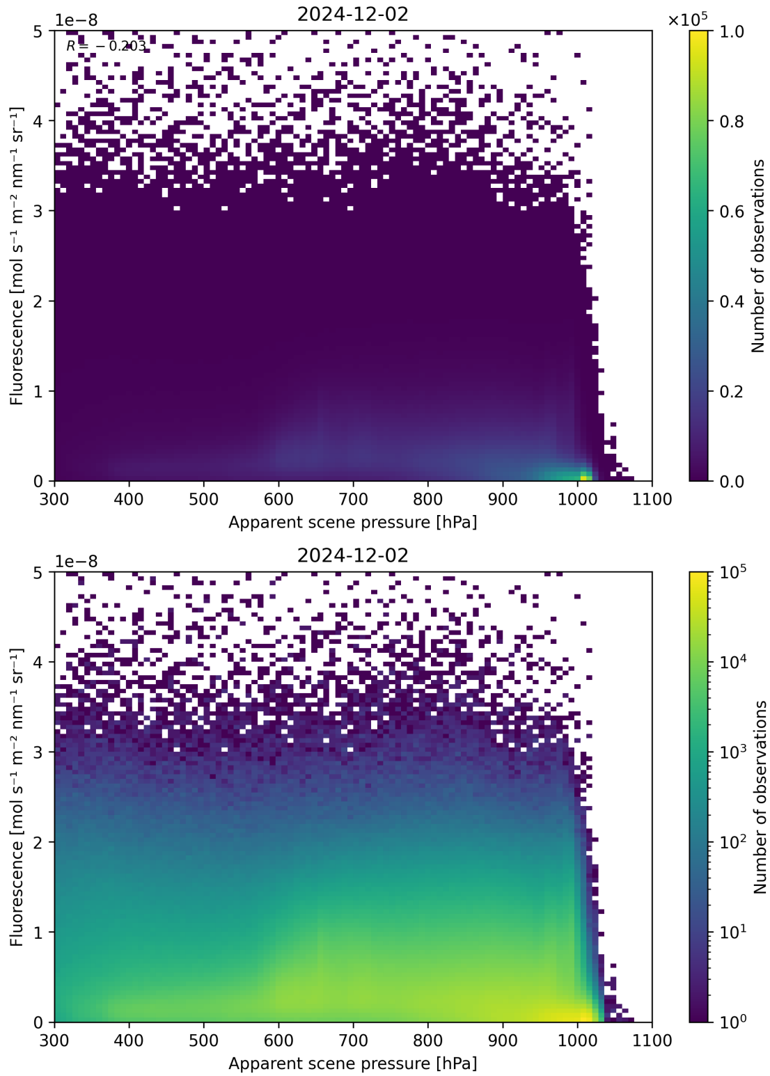
Figure 64: Scatter density plot of “Apparent scene pressure” against “Fluorescence” for 2024-12-01 to 2024-12-03.
