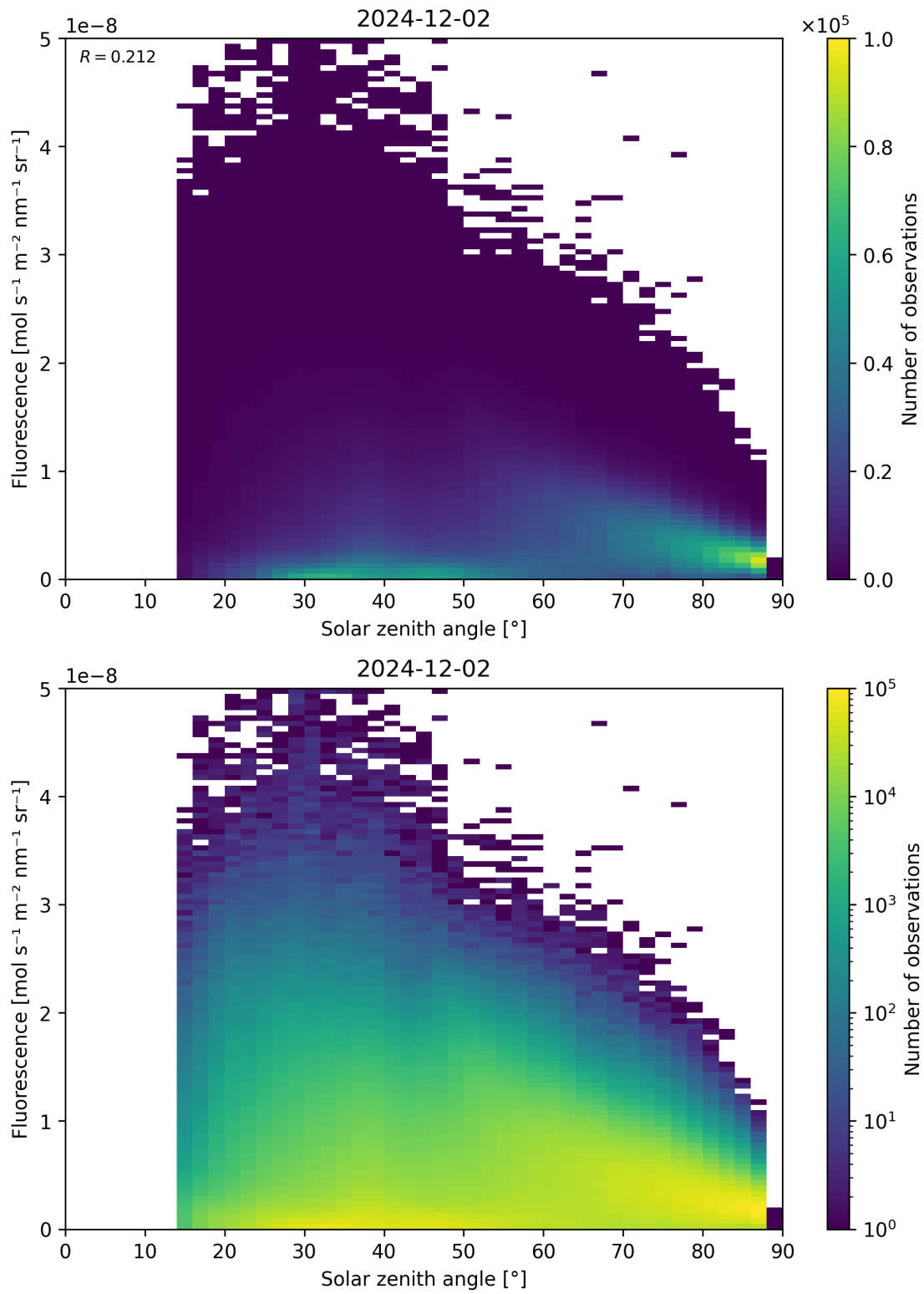
Figure 112: Scatter density plot of “Solar zenith angle” against “Fluorescence” for 2024-12-01 to 2024-12-03.
