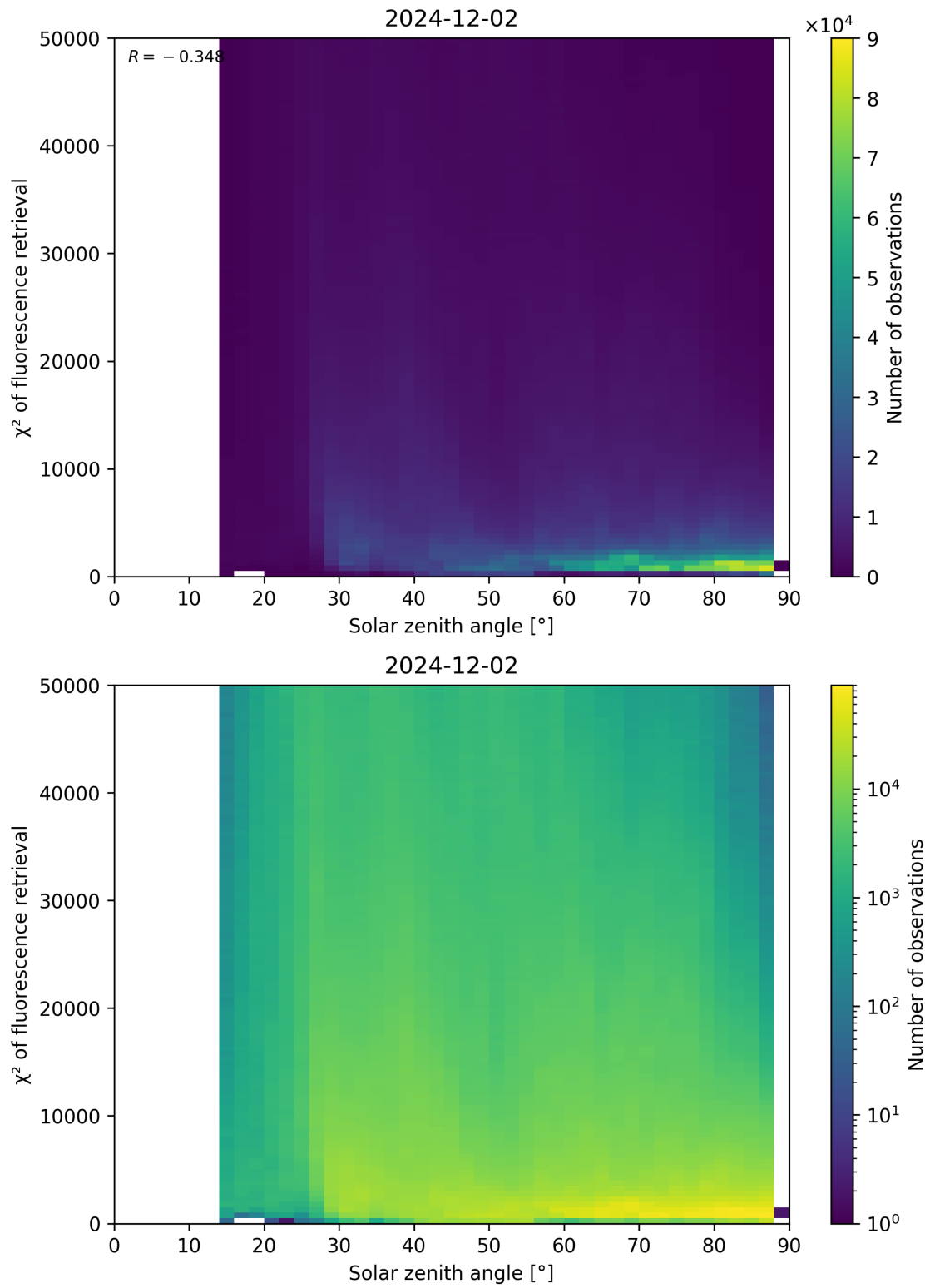
Figure 109: Scatter density plot of “Solar zenith angle” against “ \chi^2 of fluorescence retrieval” for 2024-12-01 to 2024-12-03.
