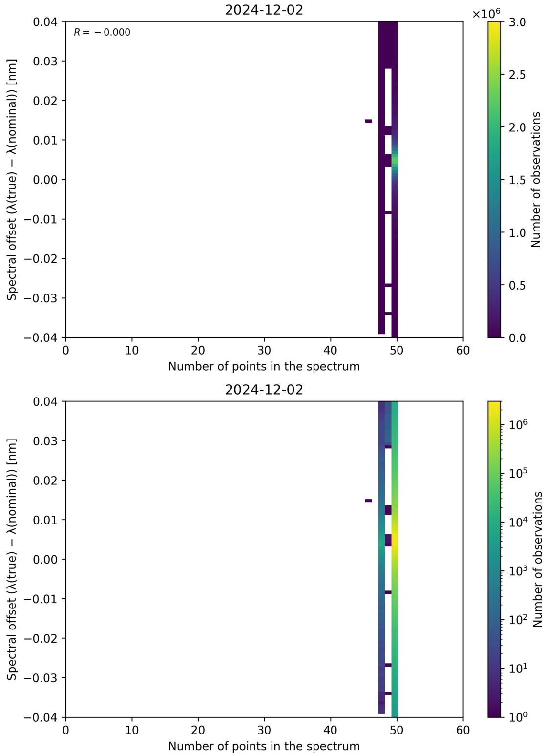
Figure 101: Scatter density plot of “Number of points in the spectrum” against “Spectral offset ( \lambda_{\text{true}} - \lambda_{\text{nominal}} )” for 2024-12-01 to 2024-12-03.
