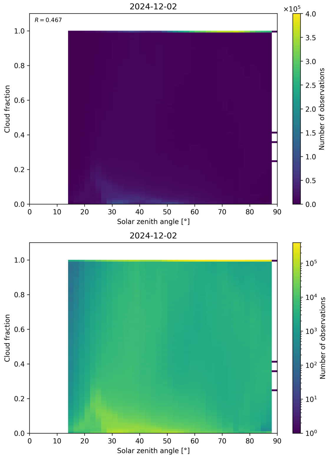
Figure 110: Scatter density plot of “Solar zenith angle” against “Cloud fraction” for 2024-12-01 to 2024-12-03.
