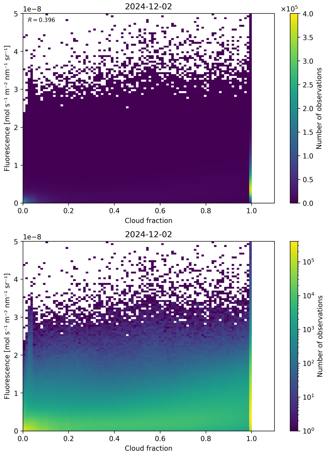
Figure 72: Scatter density plot of “Cloud fraction” against “Fluorescence” for 2024-12-01 to 2024-12-03.
