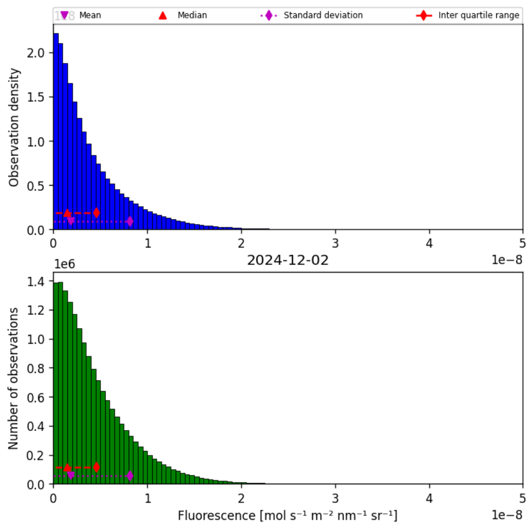
Figure 40: Histogram of “Fluorescence” for 2024-12-01 to 2024-12-03
