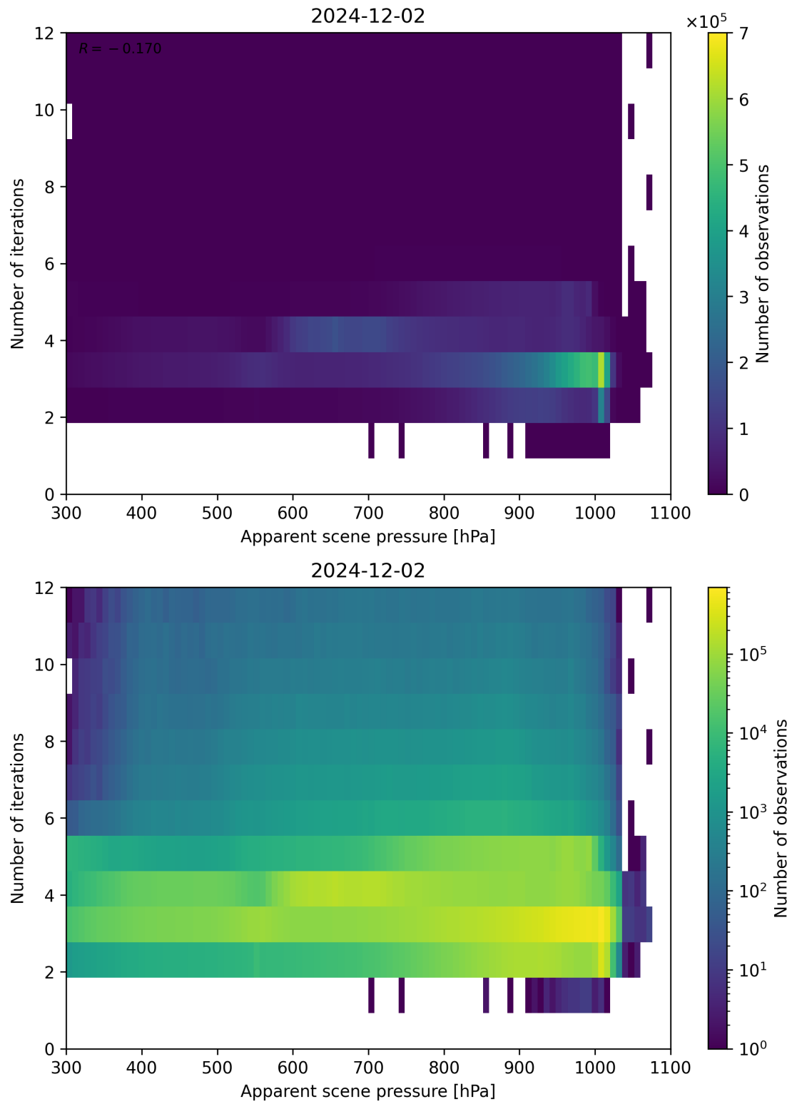
Figure 65: Scatter density plot of “Apparent scene pressure” against “Number of iterations” for 2024-12-01 to 2024-12-03.
