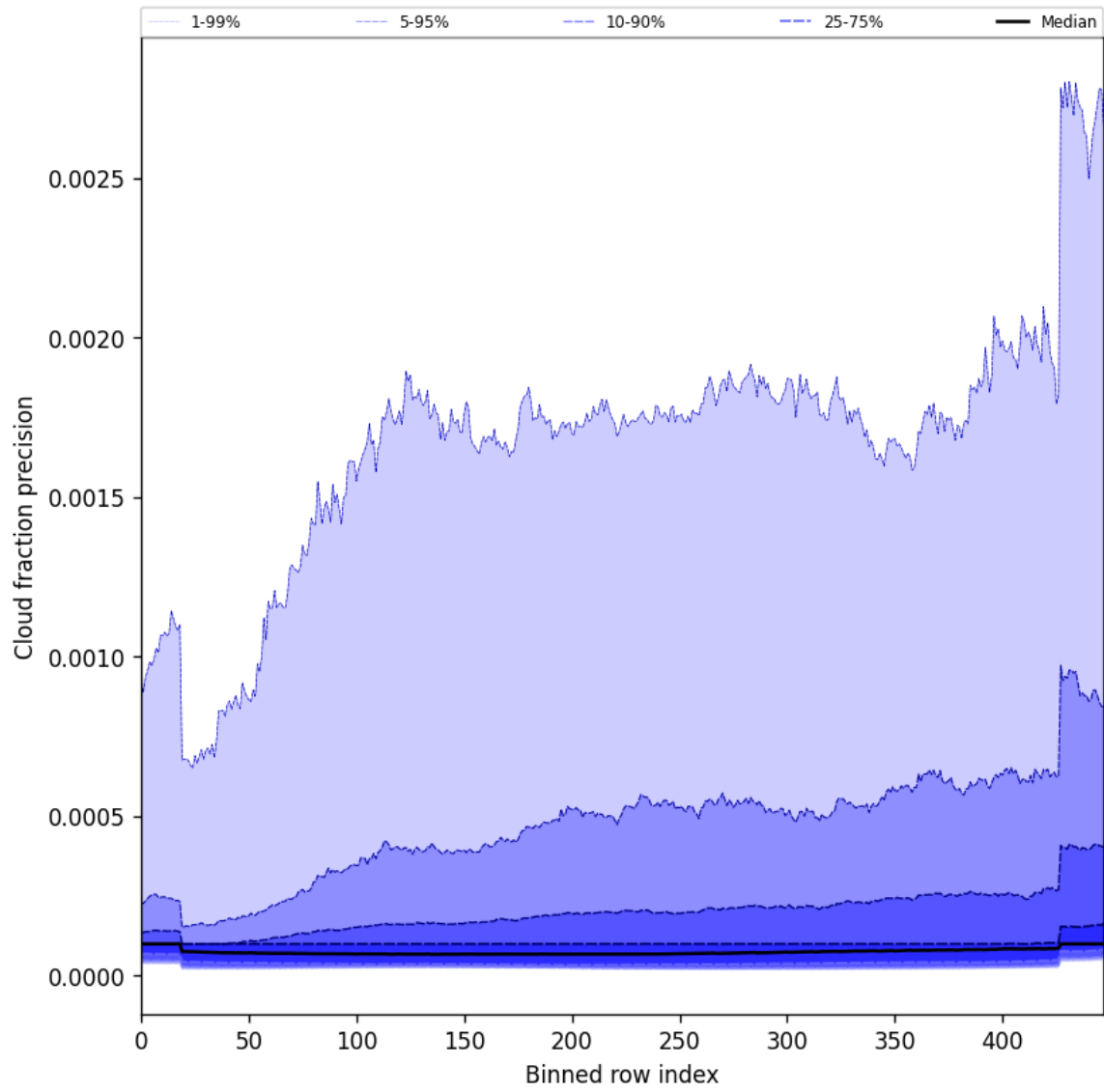
Figure 50: Along track statistics of “Cloud fraction precision” for 2024-12-01 to 2024-12-03
