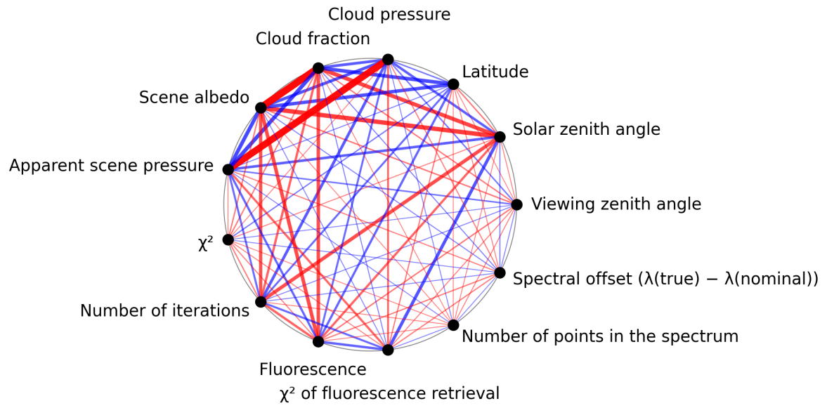
Figure 1: Map of correlation graph for 2024-12-01 to 2024-12-03.
