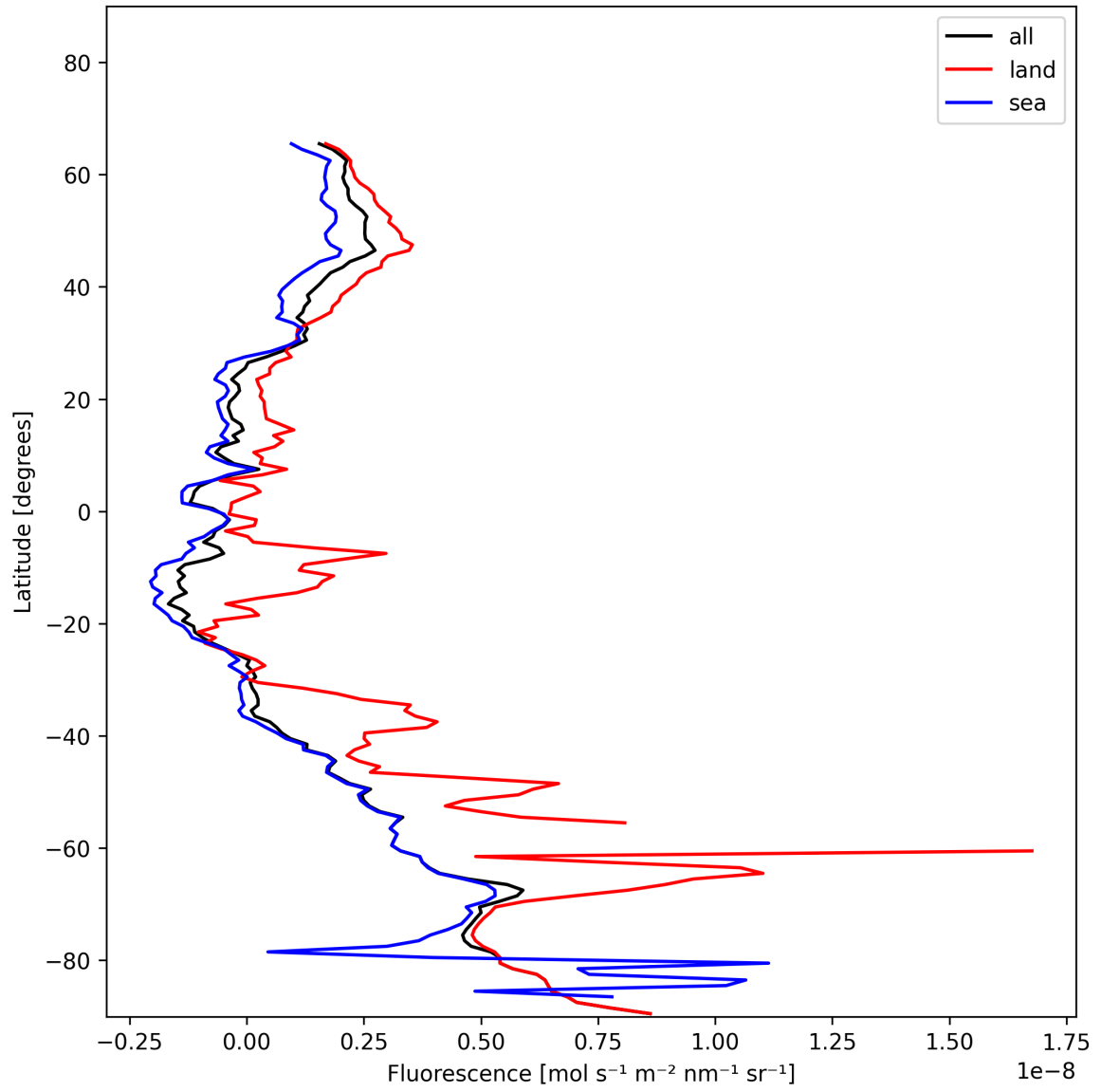
Figure 23: Zonal average of “Fluorescence” for 2024-12-01 to 2024-12-03.
