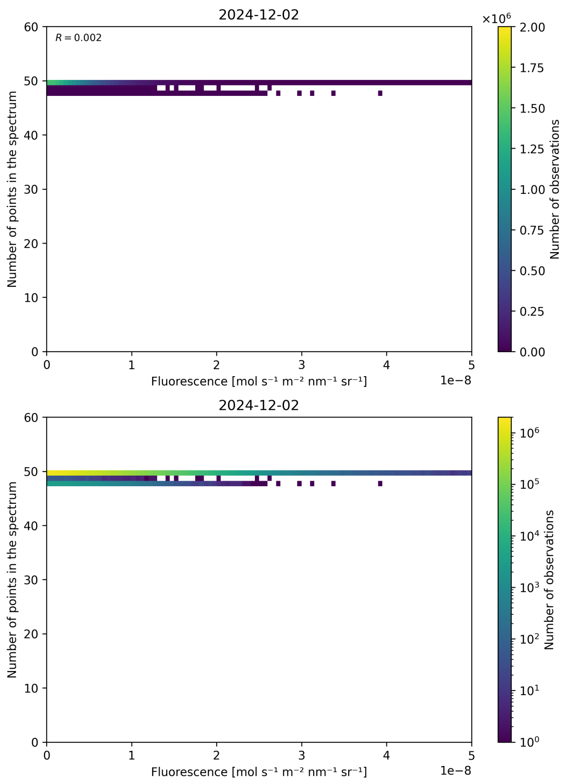
Figure 86: Scatter density plot of “Fluorescence” against “Number of points in the spectrum” for 2024-12-01 to 2024-12-03.
