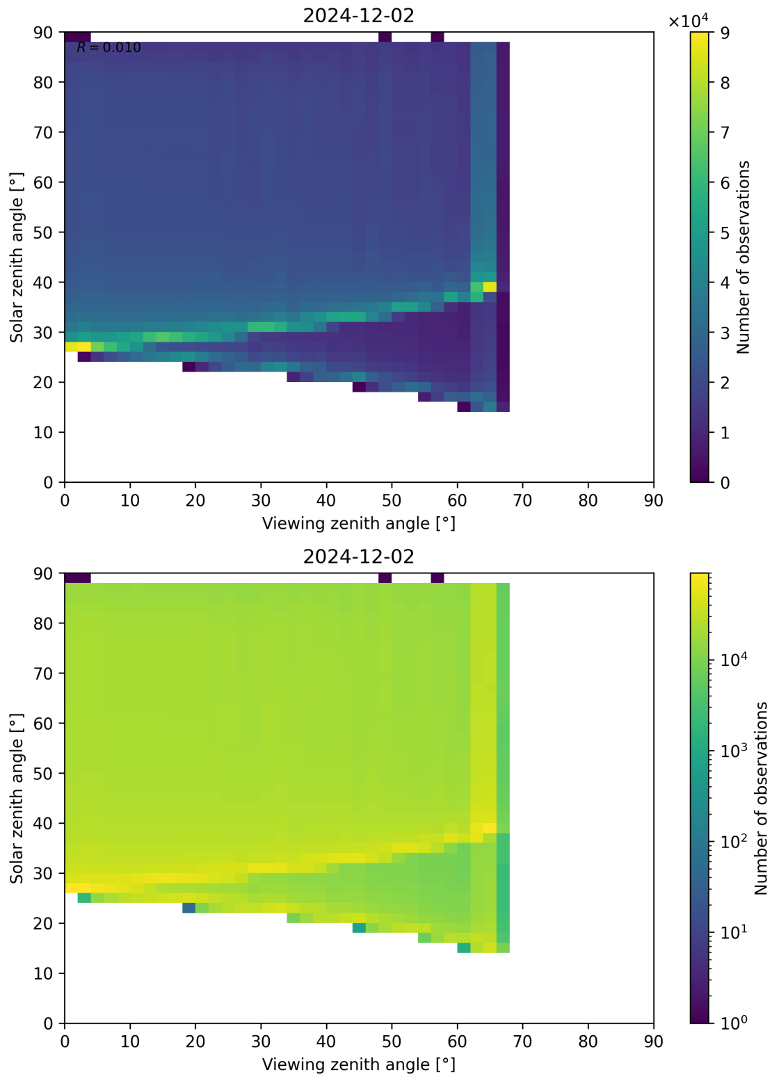
Figure 127: Scatter density plot of “Viewing zenith angle” against “Solar zenith angle” for 2024-12-01 to 2024-12-03.
