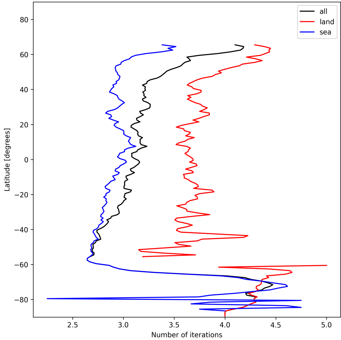
Figure 22: Zonal average of “Number of iterations” for 2024-12-01 to 2024-12-03.
