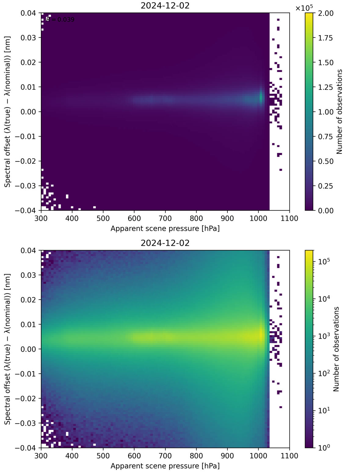
Figure 67: Scatter density plot of “Apparent scene pressure” against “Spectral offset ( \lambda_{\text{true}} - \lambda_{\text{nominal}} )” for 2024-12-01 to 2024-12-03.
