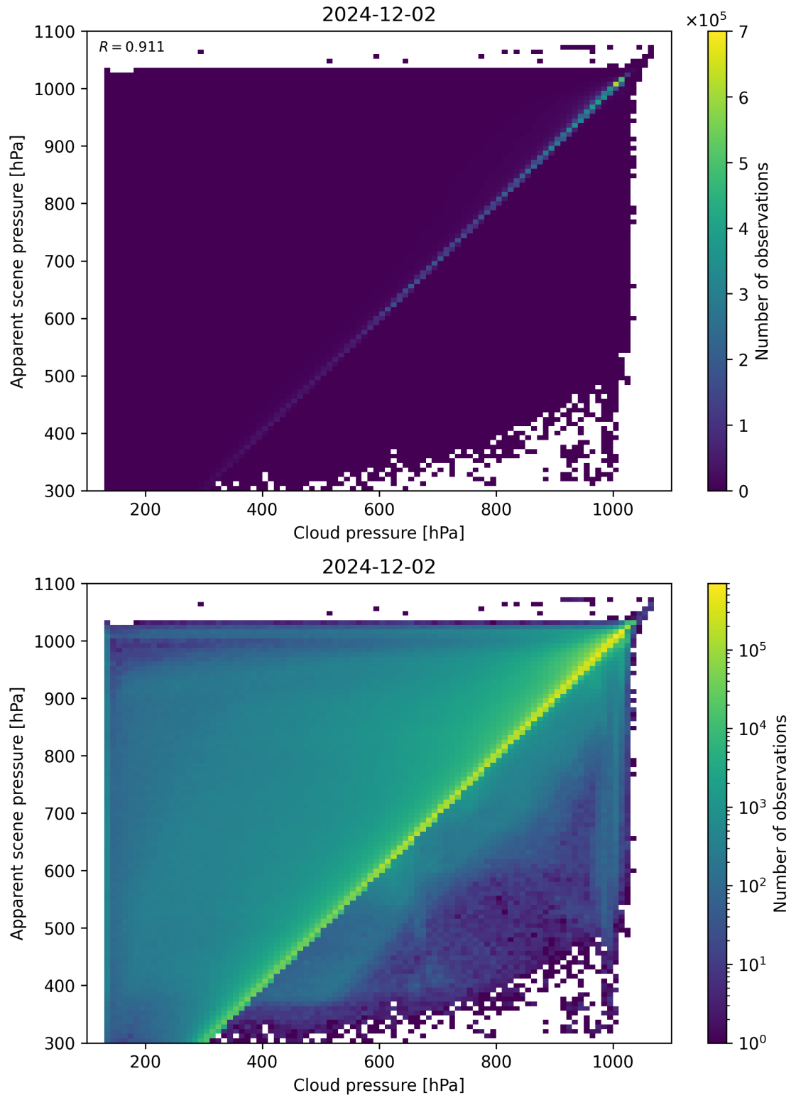
Figure 77: Scatter density plot of “Cloud pressure” against “Apparent scene pressure” for 2024-12-01 to 2024-12-03.
