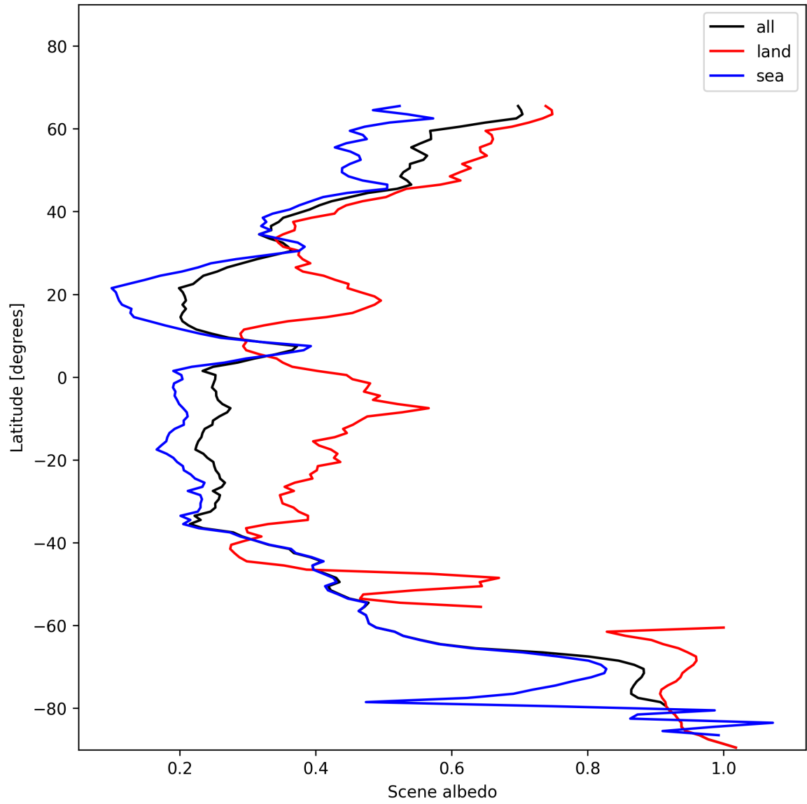
Figure 17: Zonal average of “Scene albedo” for 2024-12-01 to 2024-12-03.
