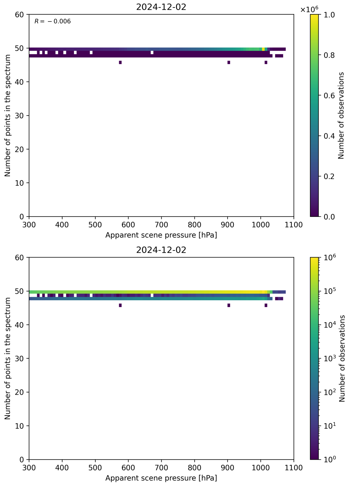
Figure 66: Scatter density plot of “Apparent scene pressure” against “Number of points in the spectrum” for 2024-12-01 to 2024-12-03.
