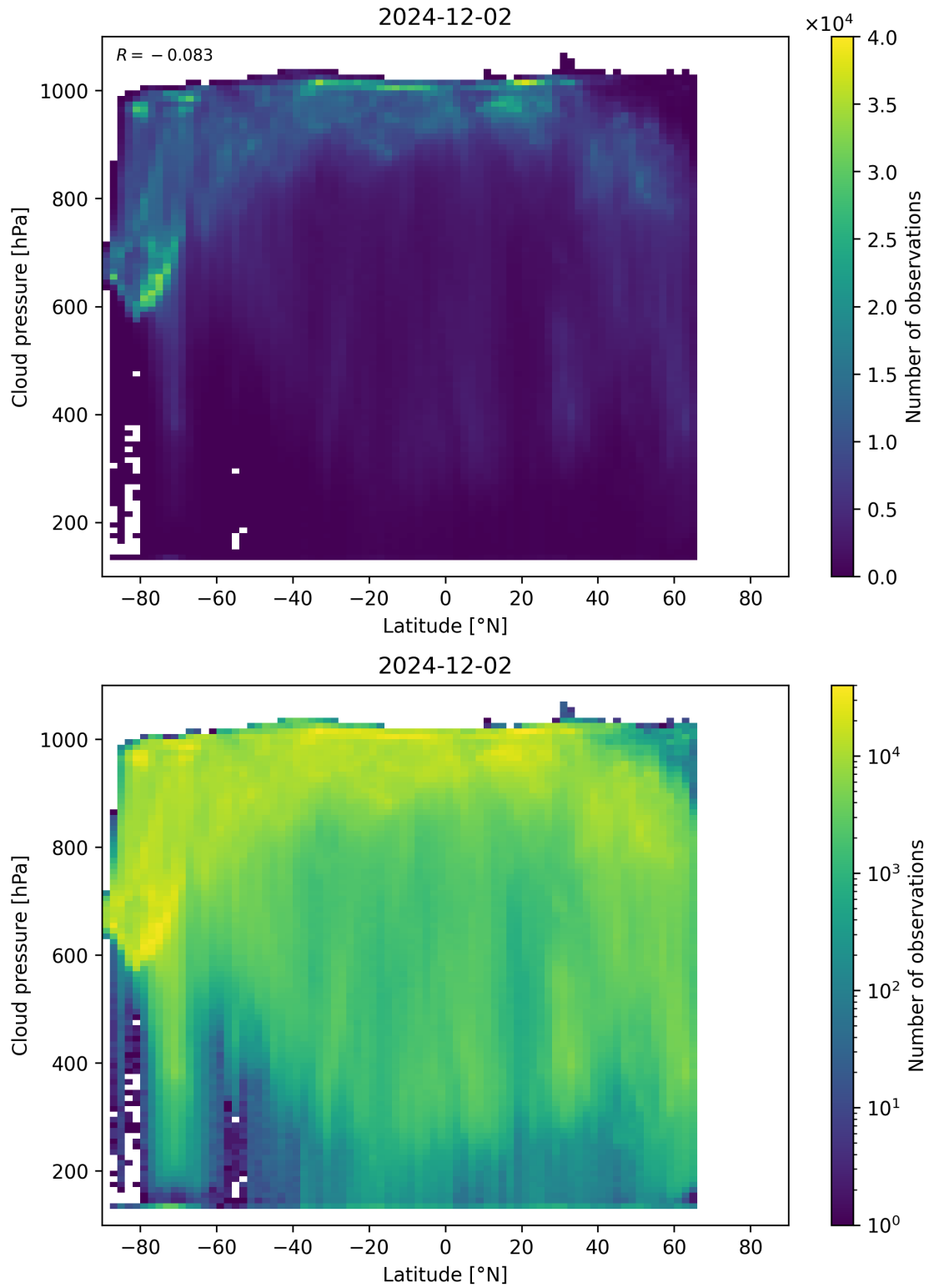
Figure 91: Scatter density plot of “Latitude” against “Cloud pressure” for 2024-12-01 to 2024-12-03.
