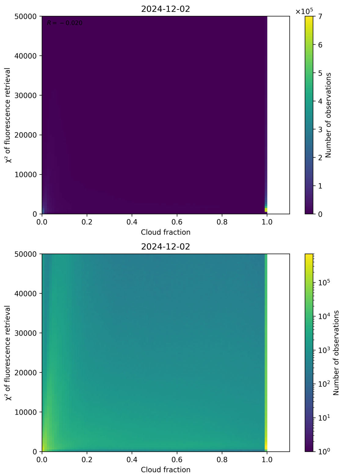
Figure 71: Scatter density plot of “Cloud fraction” against “ \chi^2 of fluorescence retrieval” for 2024-12-01 to 2024-12-03.
