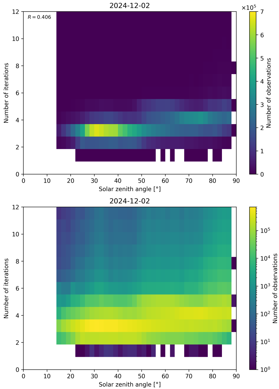
Figure 114: Scatter density plot of “Solar zenith angle” against “Number of iterations” for 2024-12-01 to 2024-12-03.
