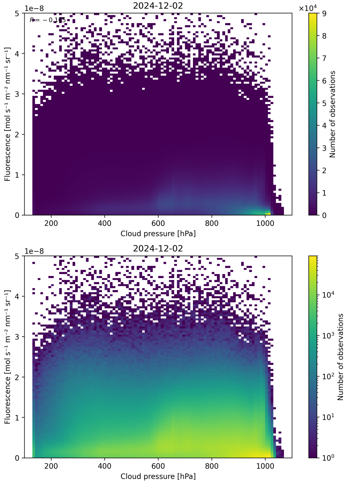
Figure 80: Scatter density plot of “Cloud pressure” against “Fluorescence” for 2024-12-01 to 2024-12-03.
