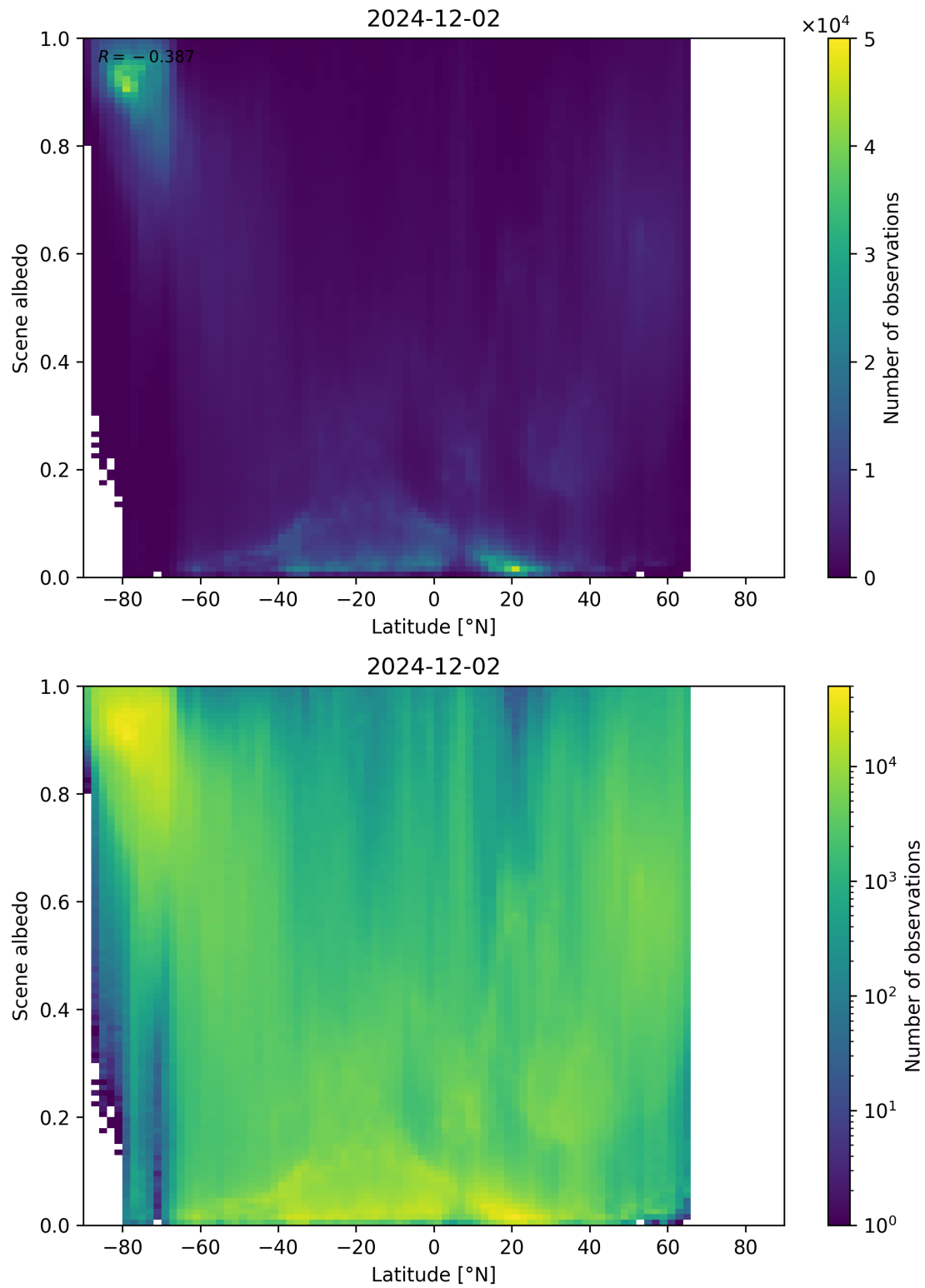
Figure 95: Scatter density plot of “Latitude” against “Scene albedo” for 2024-12-01 to 2024-12-03.
