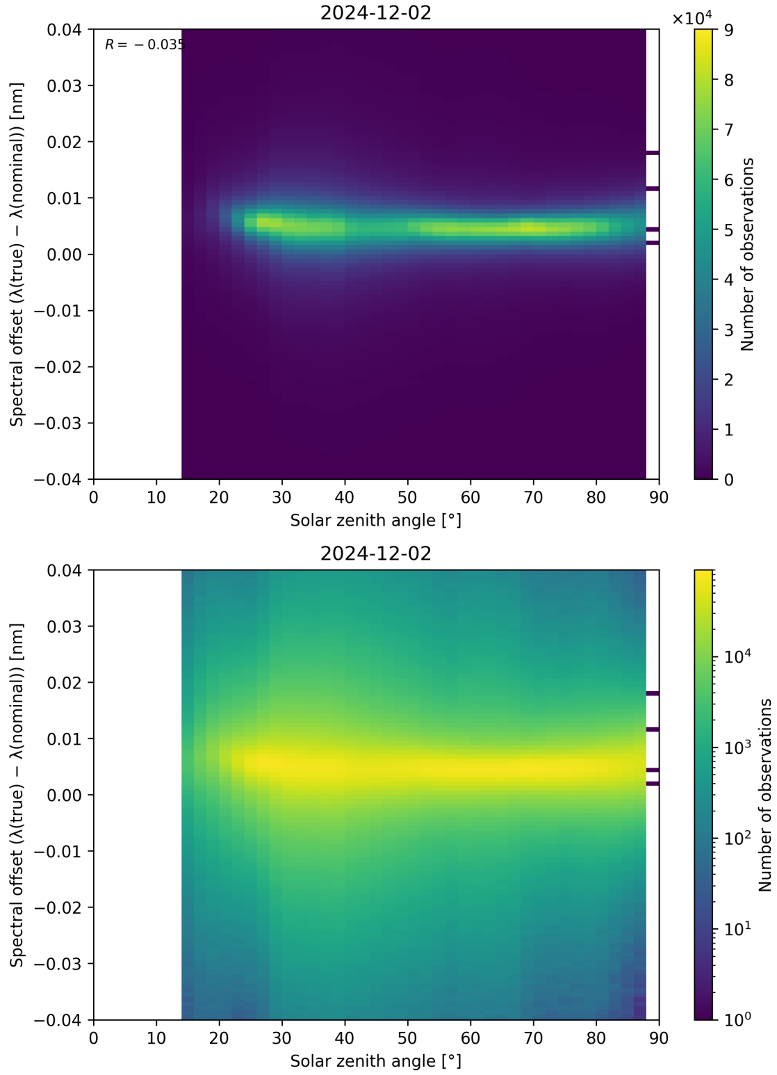
Figure 117: Scatter density plot of “Solar zenith angle” against “Spectral offset ( \lambda_{\text{true}} - \lambda_{\text{nominal}} )” for 2024-12-01 to 2024-12-03.
