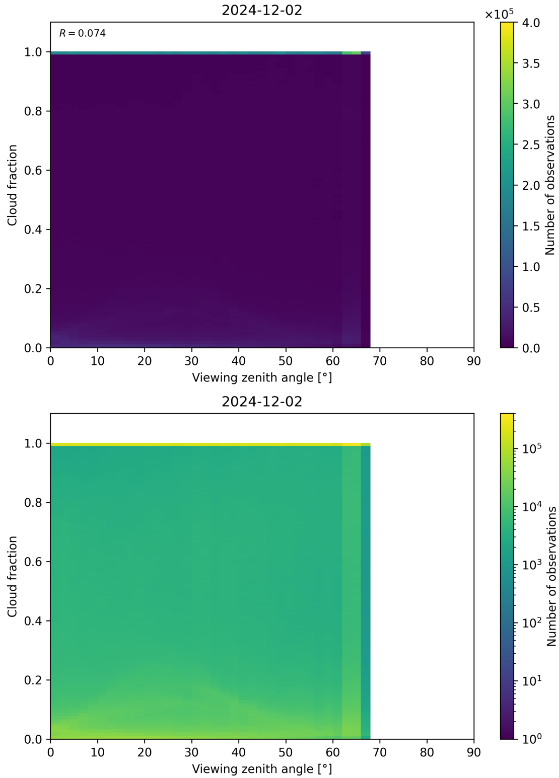
Figure 120: Scatter density plot of “Viewing zenith angle” against “Cloud fraction” for 2024-12-01 to 2024-12-03.
