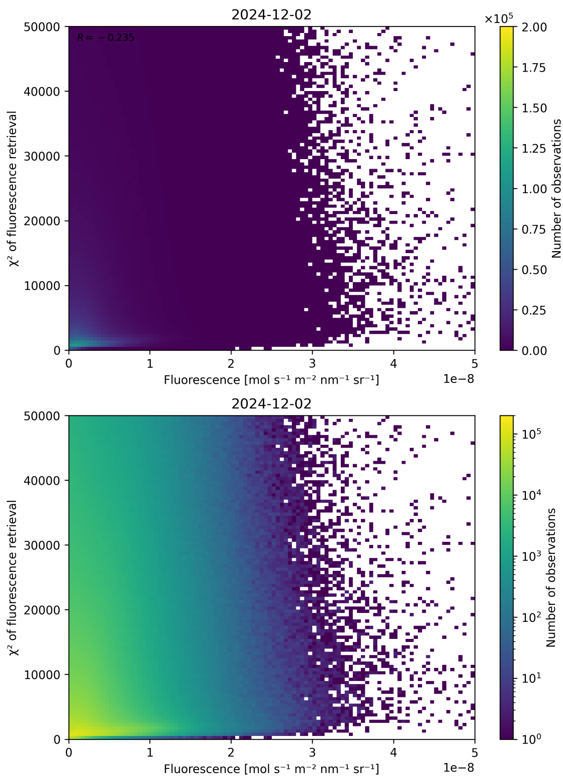
Figure 85: Scatter density plot of “Fluorescence” against “ \chi^2 of fluorescence retrieval” for 2024-12-01 to 2024-12-03.
