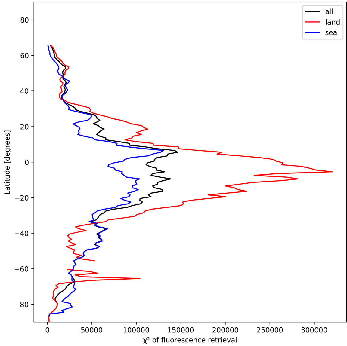
Figure 25: Zonal average of “ \chi^2 of fluorescence retrieval” for 2024-12-01 to 2024-12-03.
