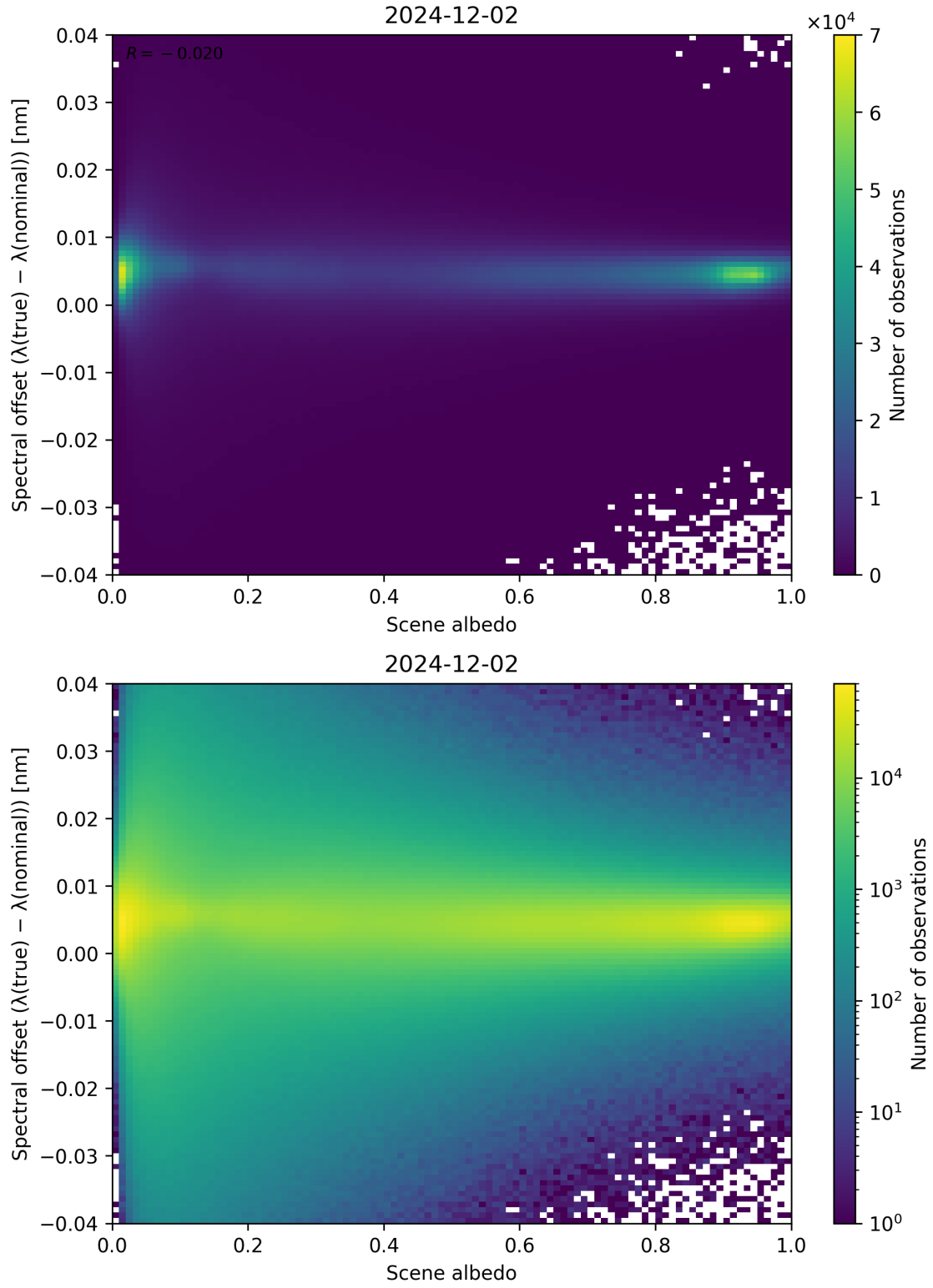
Figure 107: Scatter density plot of “Scene albedo” against “Spectral offset ( \lambda_{\text{true}} - \lambda_{\text{nominal}} )” for 2024-12-01 to 2024-12-03.
