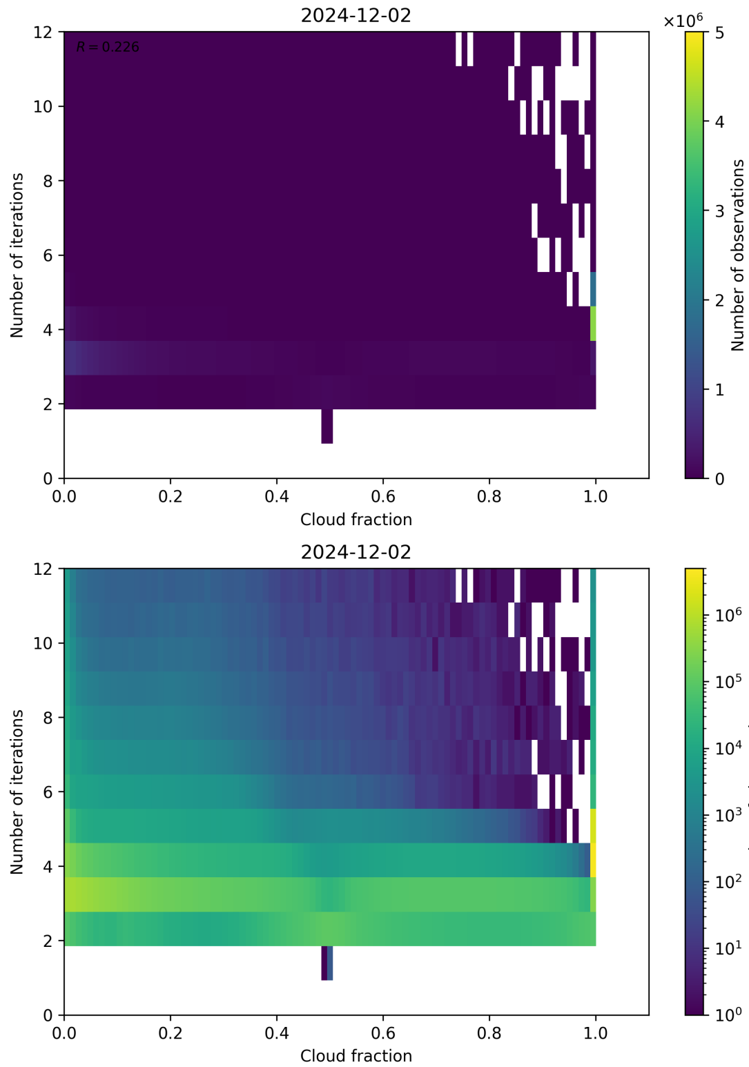
Figure 73: Scatter density plot of “Cloud fraction” against “Number of iterations” for 2024-12-01 to 2024-12-03.
