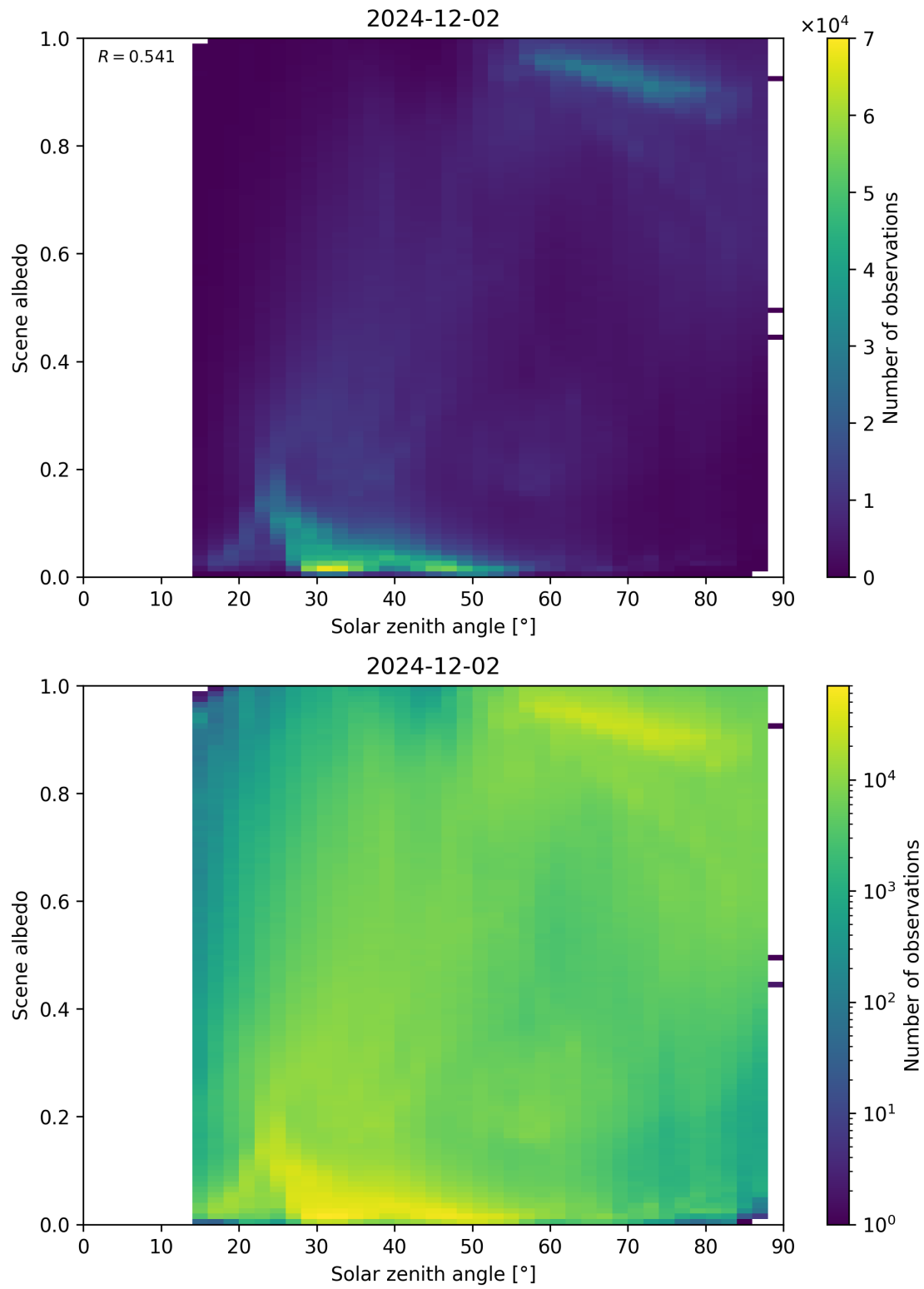
Figure 116: Scatter density plot of “Solar zenith angle” against “Scene albedo” for 2024-12-01 to 2024-12-03.
