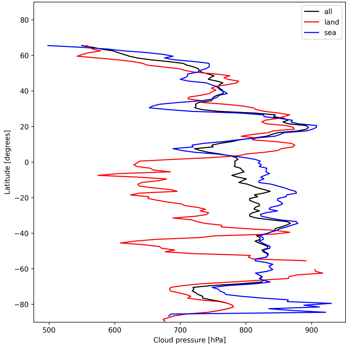
Figure 13: Zonal average of “Cloud pressure” for 2024-12-01 to 2024-12-03.
