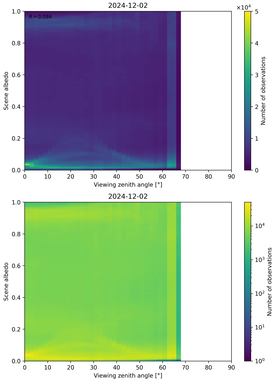
Figure 126: Scatter density plot of “Viewing zenith angle” against “Scene albedo” for 2024-12-01 to 2024-12-03.
