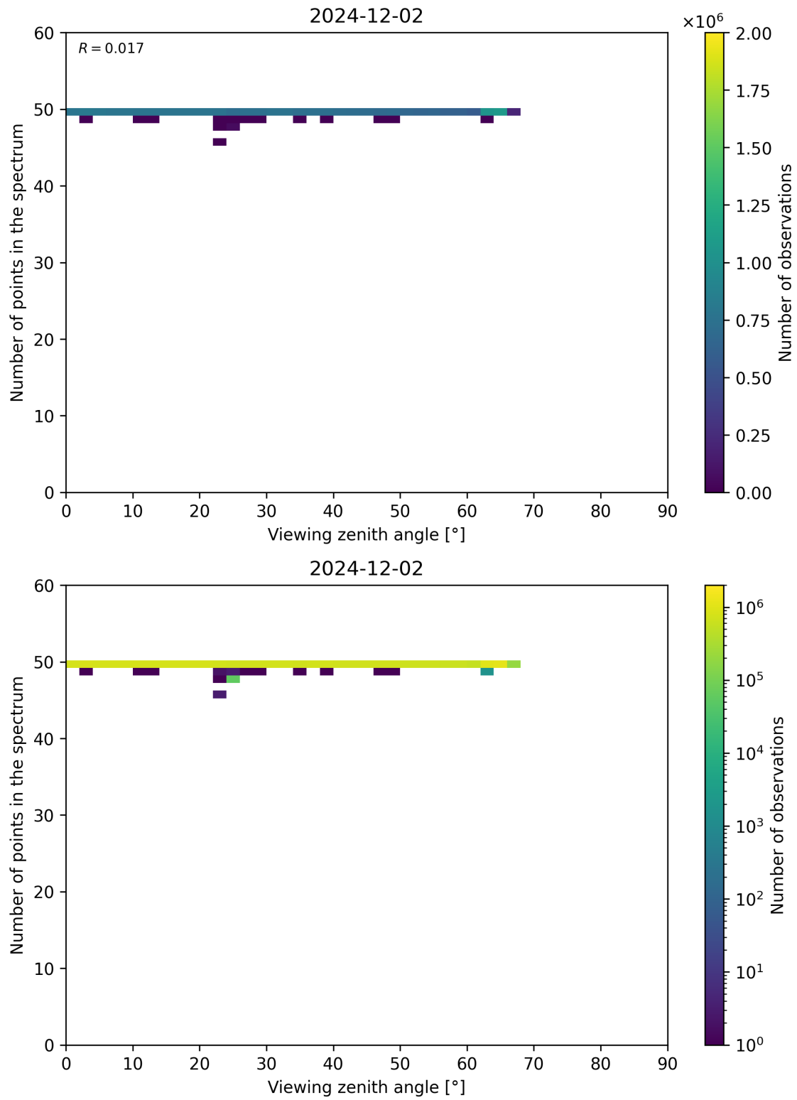
Figure 125: Scatter density plot of “Viewing zenith angle” against “Number of points in the spectrum” for 2024-12-01 to 2024-12-03.
