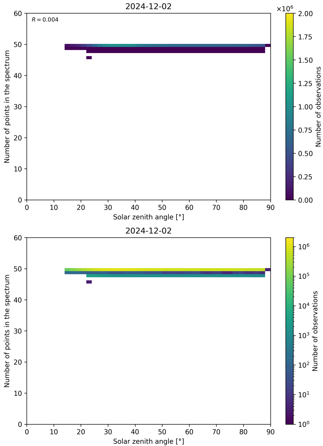
Figure 115: Scatter density plot of “Solar zenith angle” against “Number of points in the spectrum” for 2024-12-01 to 2024-12-03.
