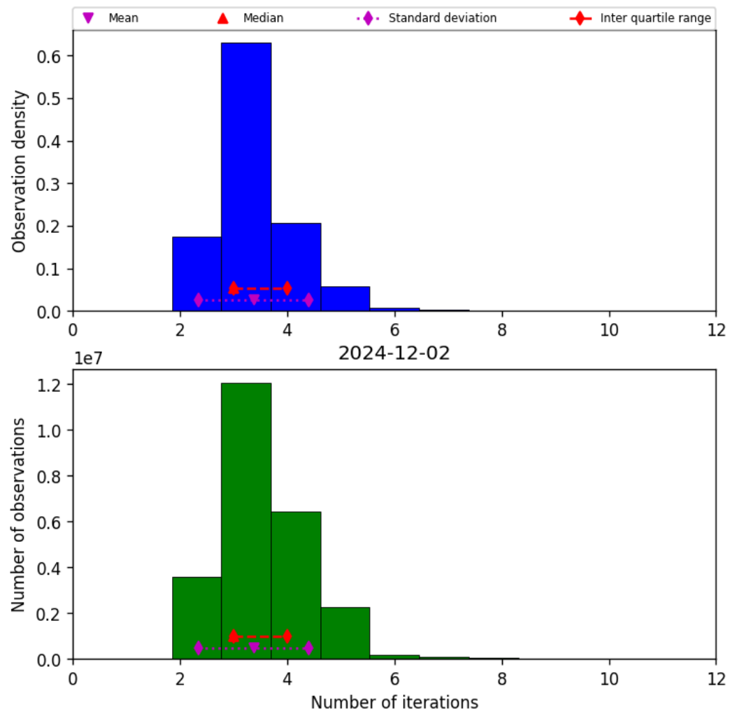
Figure 39: Histogram of “Number of iterations” for 2024-12-01 to 2024-12-03
