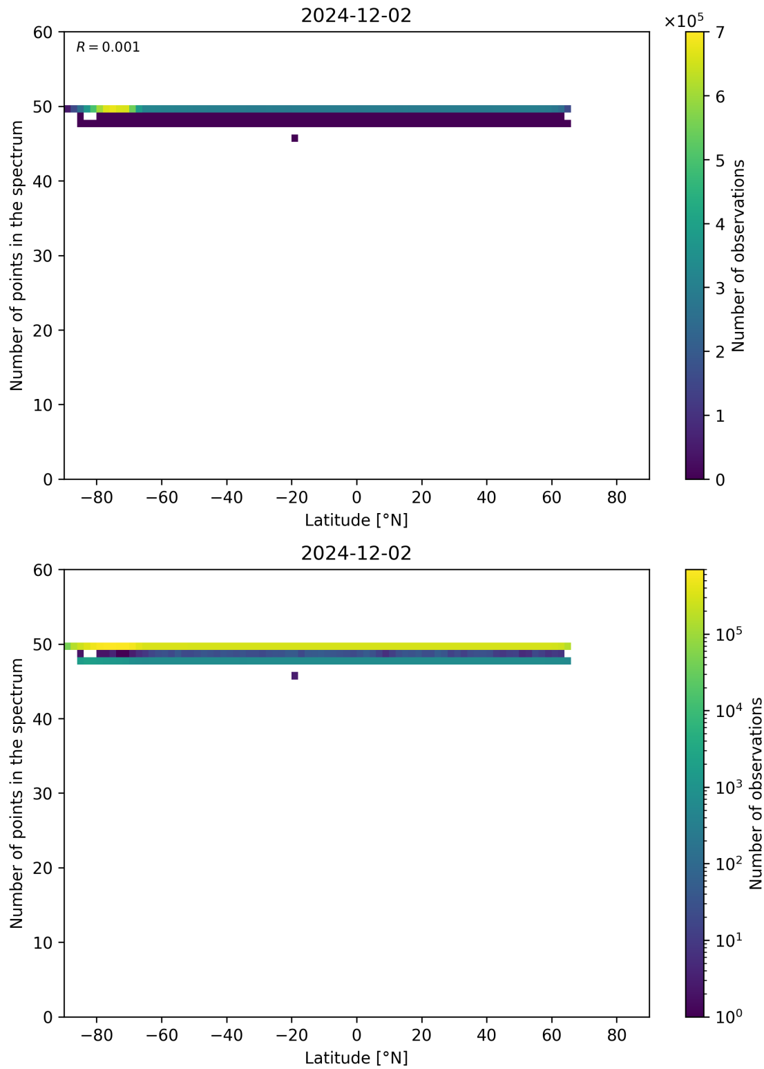
Figure 94: Scatter density plot of “Latitude” against “Number of points in the spectrum” for 2024-12-01 to 2024-12-03.
