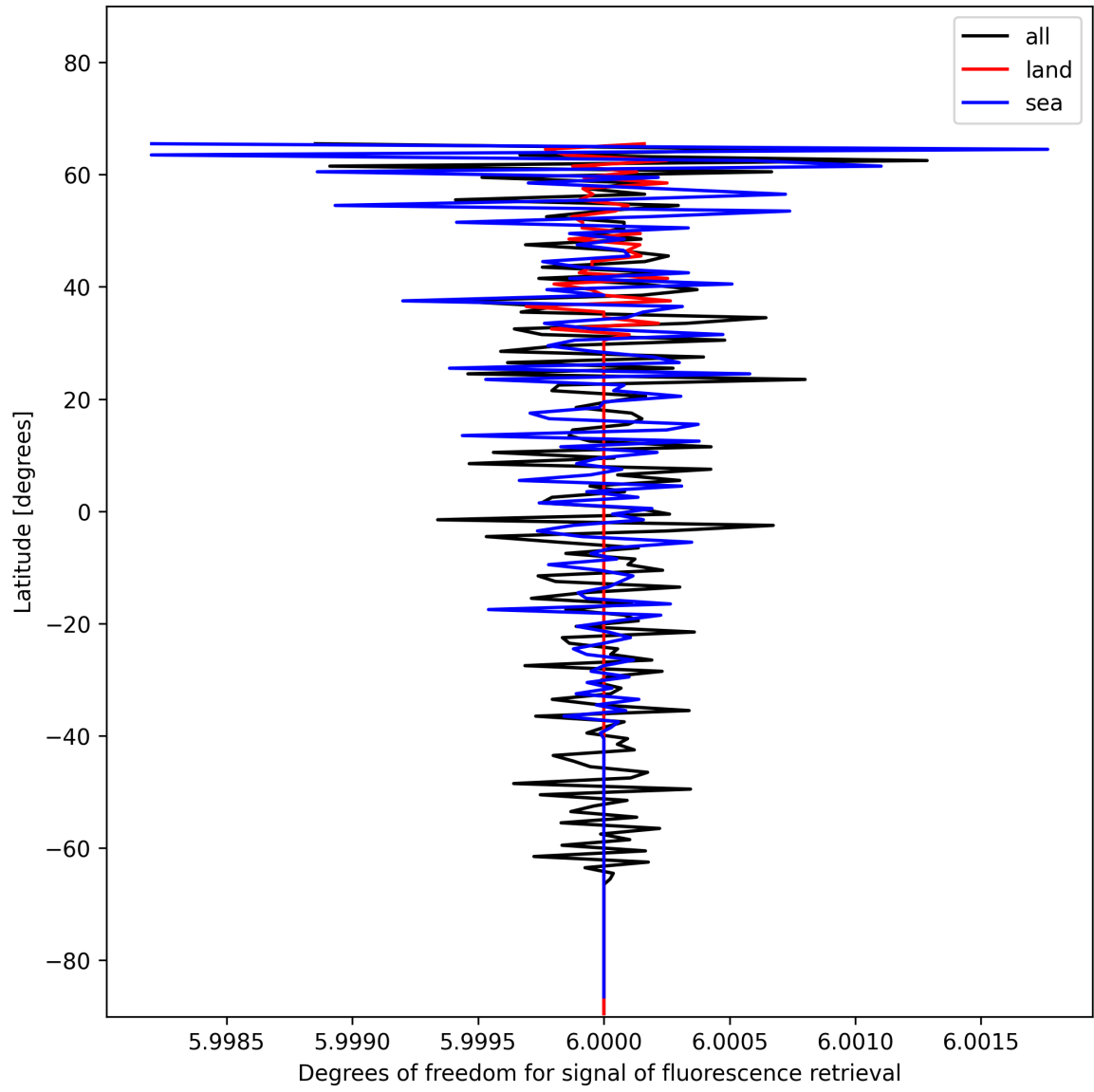
Figure 26: Zonal average of “Degrees of freedom for signal of fluorescence retrieval” for 2024-12-01 to 2024-12-03.
