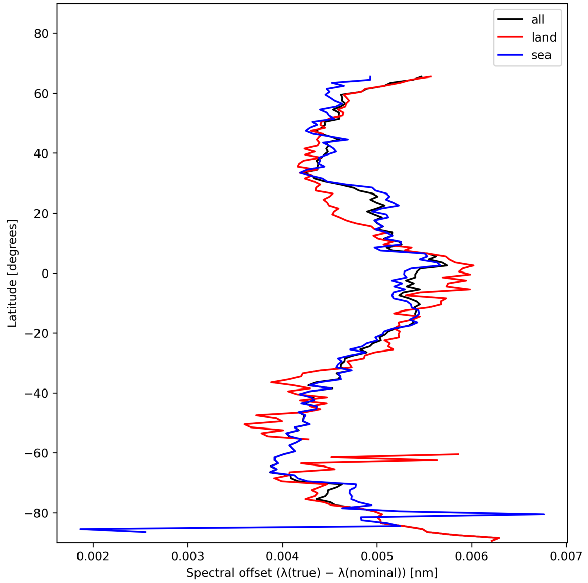
Figure 28: Zonal average of “Spectral offset ( \lambda_{\text{true}} - \lambda_{\text{nominal}} )” for 2024-12-01 to 2024-12-03.
