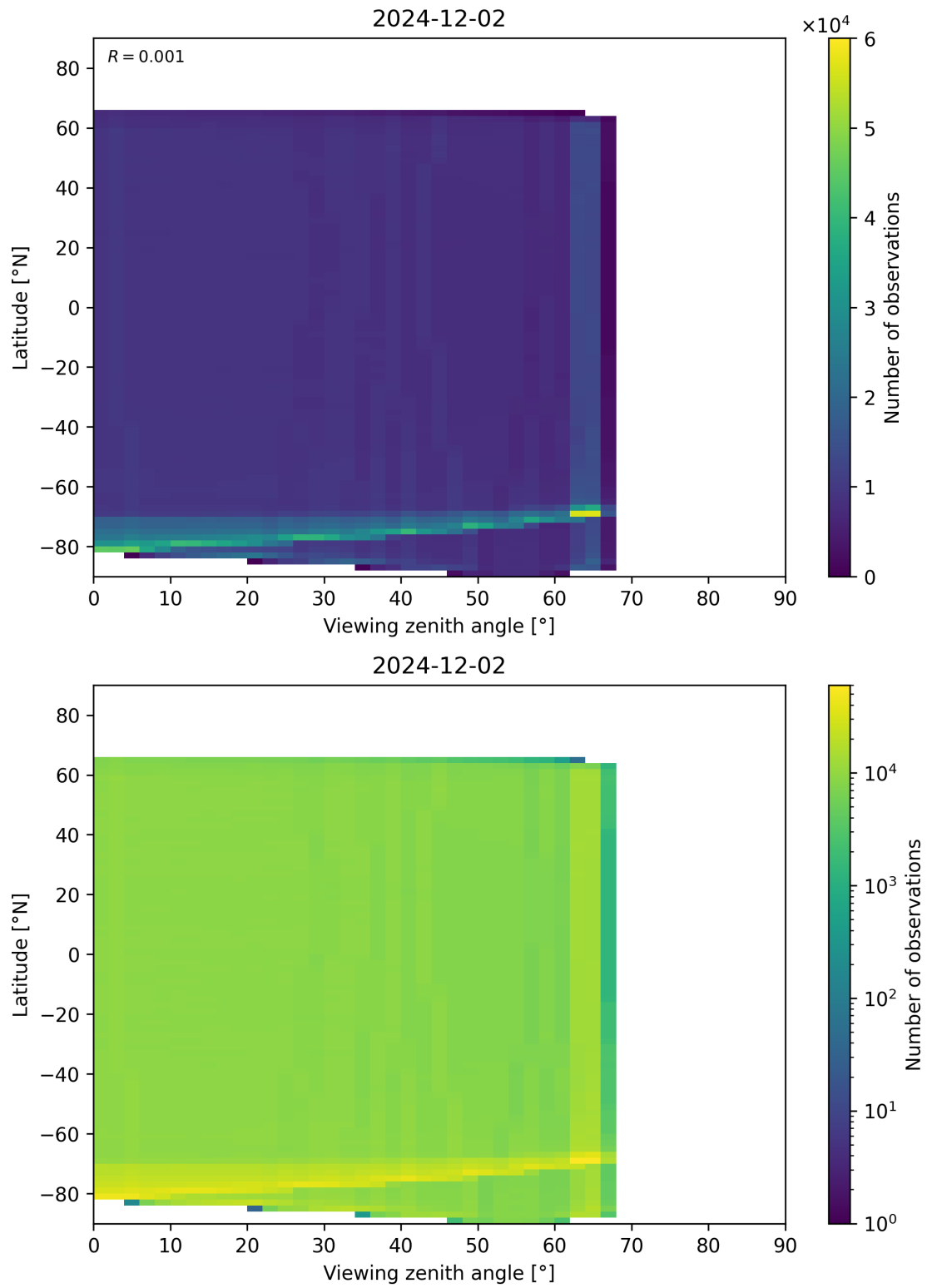
Figure 123: Scatter density plot of “Viewing zenith angle” against “Latitude” for 2024-12-01 to 2024-12-03.
