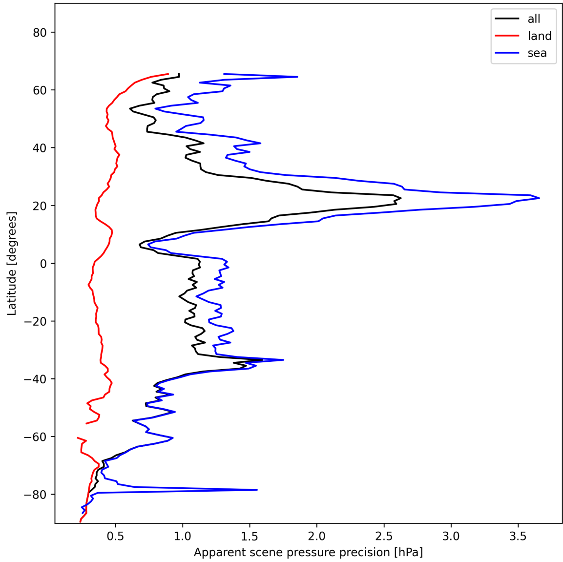
Figure 20: Zonal average of “Apparent scene pressure precision” for 2024-12-01 to 2024-12-03.
