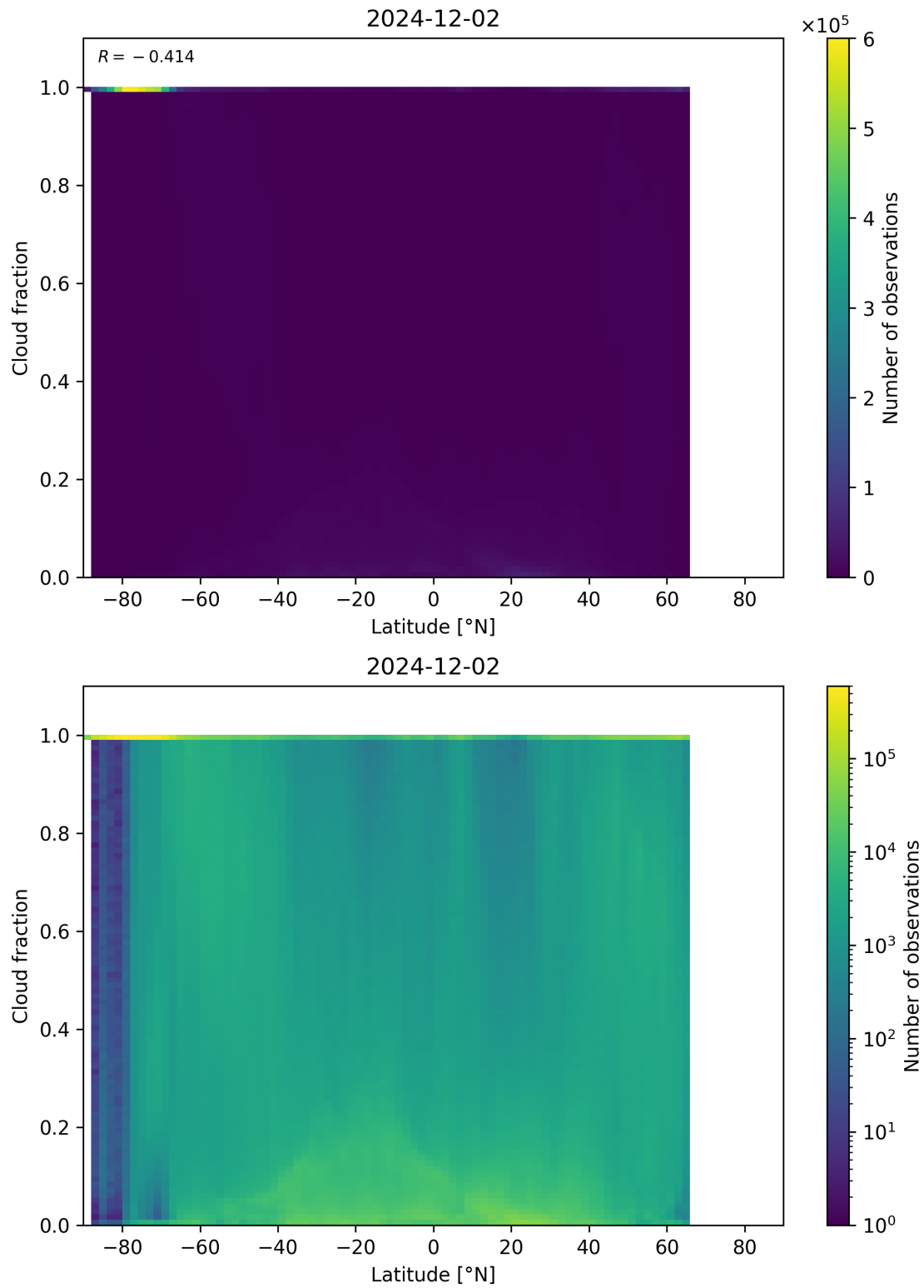
Figure 90: Scatter density plot of “Latitude” against “Cloud fraction” for 2024-12-01 to 2024-12-03.
