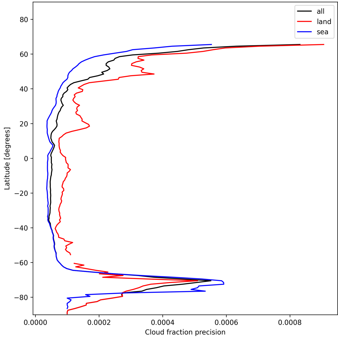
Figure 16: Zonal average of “Cloud fraction precision” for 2024-12-01 to 2024-12-03.
