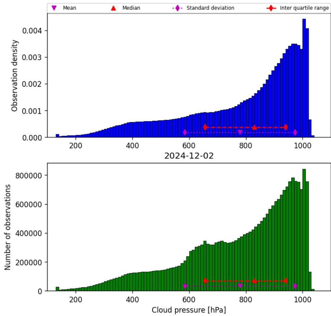
Figure 30: Histogram of “Cloud pressure” for 2024-12-01 to 2024-12-03
