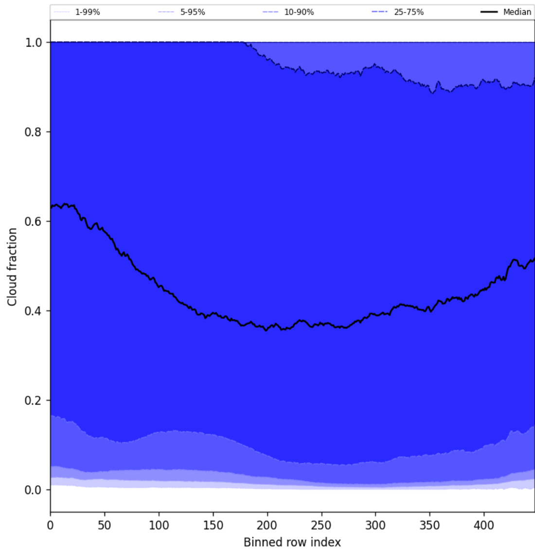
Figure 49: Along track statistics of “Cloud fraction” for 2024-12-01 to 2024-12-03
