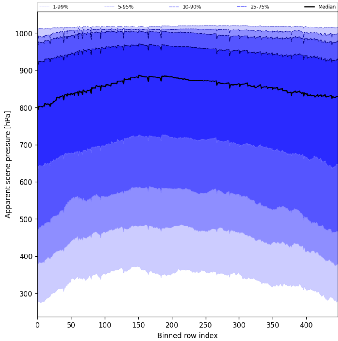
Figure 53: Along track statistics of “Apparent scene pressure” for 2024-12-01 to 2024-12-03
