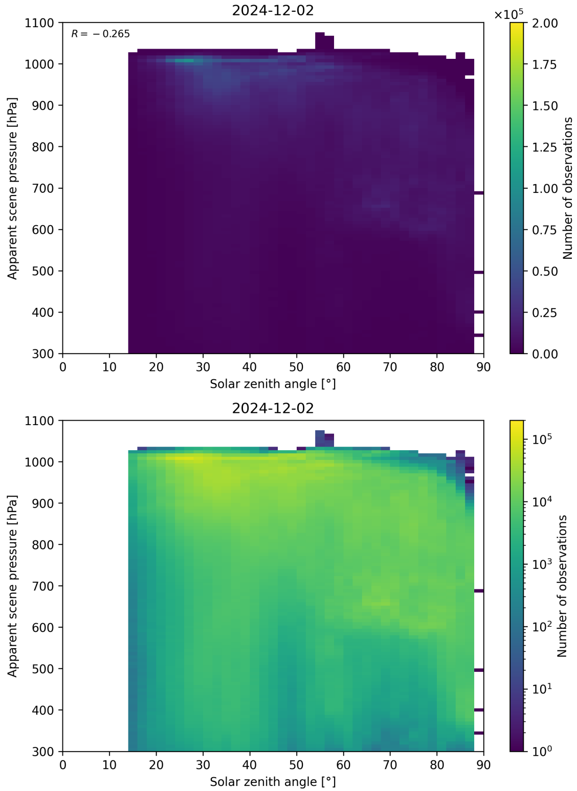
Figure 108: Scatter density plot of “Solar zenith angle” against “Apparent scene pressure” for 2024-12-01 to 2024-12-03.
