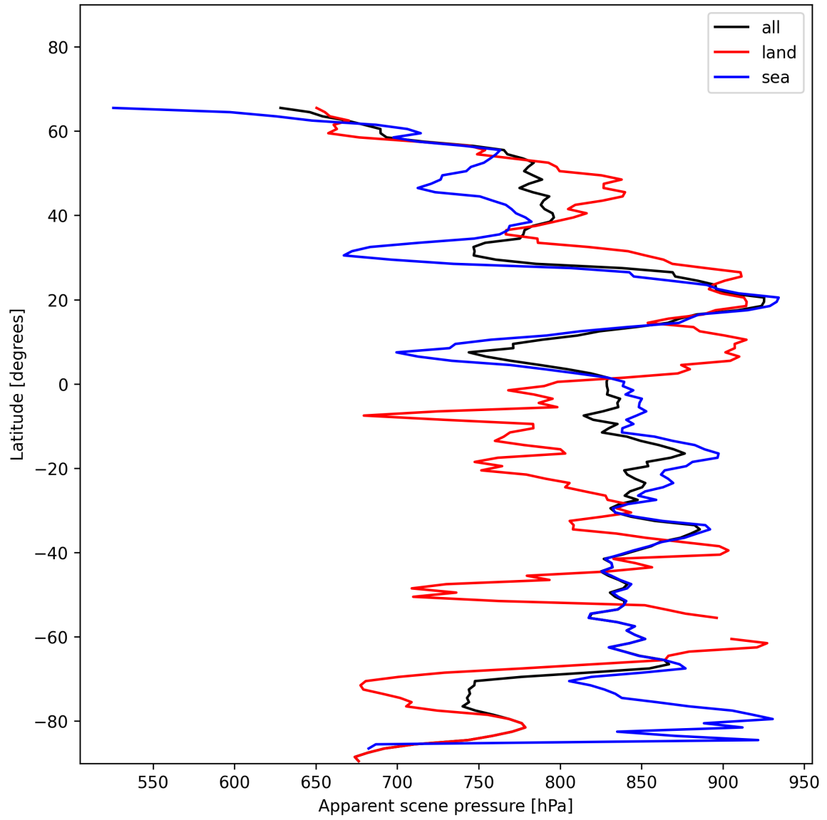
Figure 19: Zonal average of “Apparent scene pressure” for 2024-12-01 to 2024-12-03.
