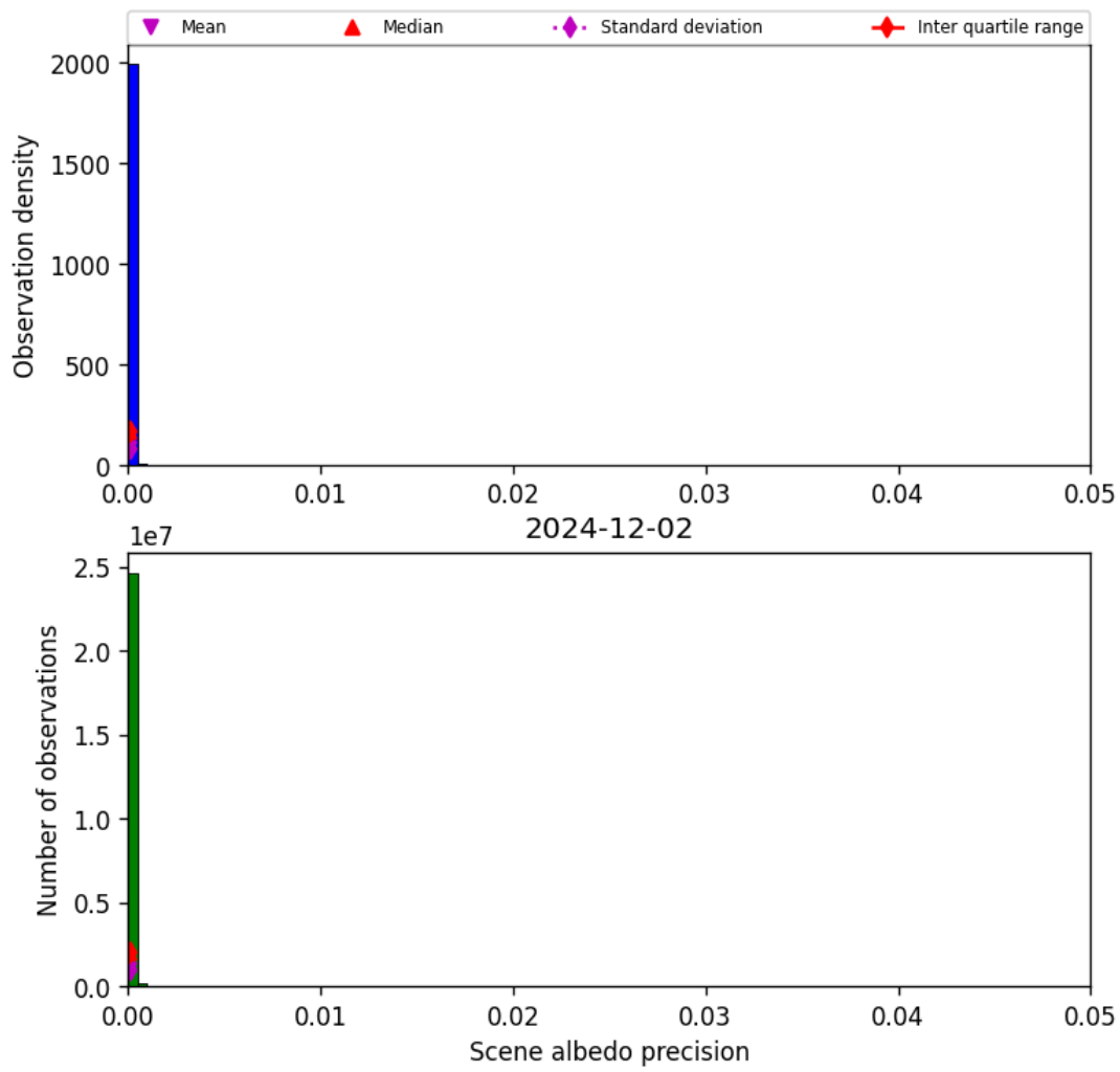
Figure 35: Histogram of “Scene albedo precision” for 2024-12-01 to 2024-12-03
