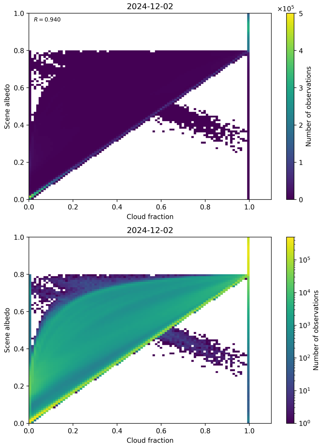
Figure 75: Scatter density plot of “Cloud fraction” against “Scene albedo” for 2024-12-01 to 2024-12-03.
