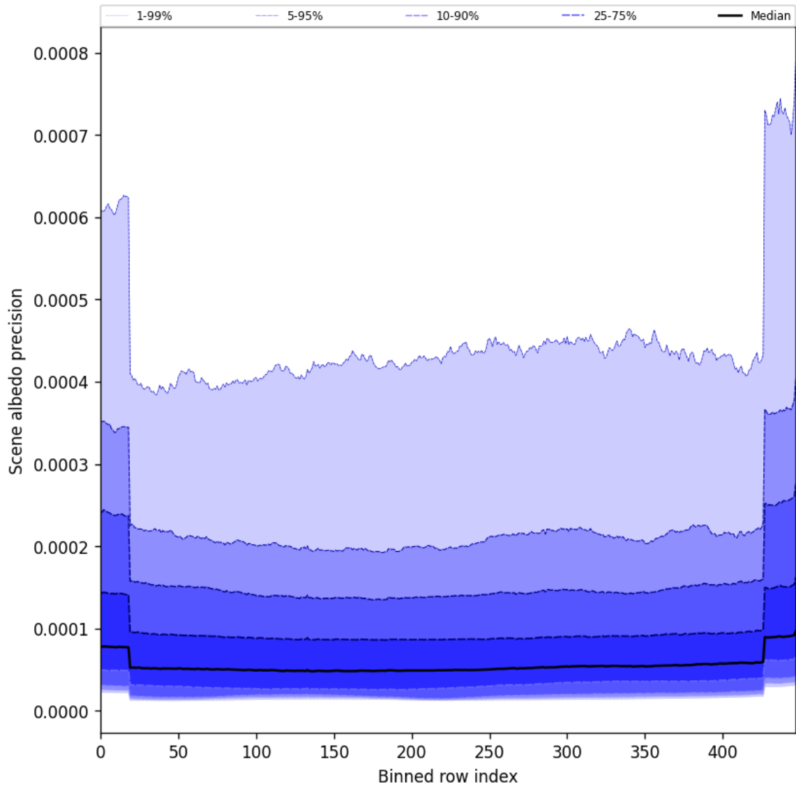
Figure 52: Along track statistics of “Scene albedo precision” for 2024-12-01 to 2024-12-03
