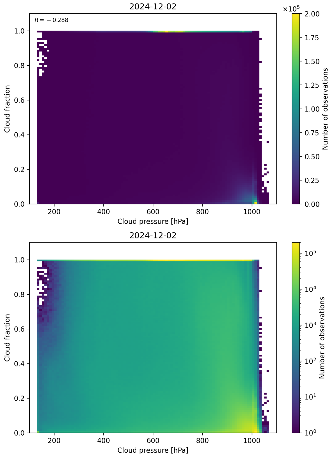
Figure 79: Scatter density plot of “Cloud pressure” against “Cloud fraction” for 2024-12-01 to 2024-12-03.
