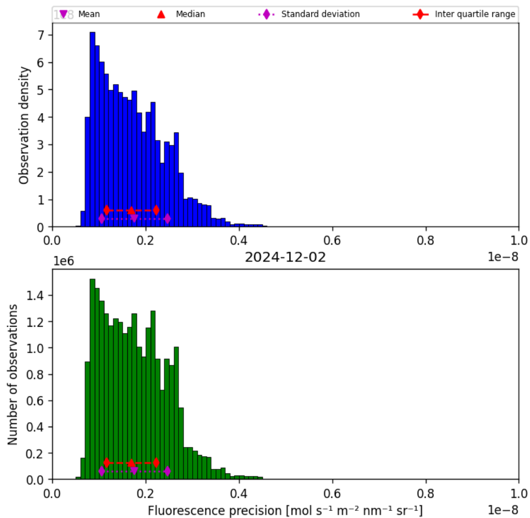
Figure 41: Histogram of “Fluorescence precision” for 2024-12-01 to 2024-12-03
