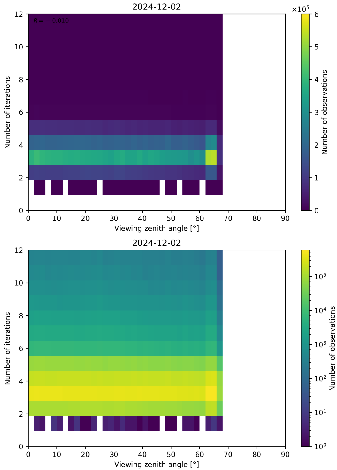
Figure 124: Scatter density plot of “Viewing zenith angle” against “Number of iterations” for 2024-12-01 to 2024-12-03.
