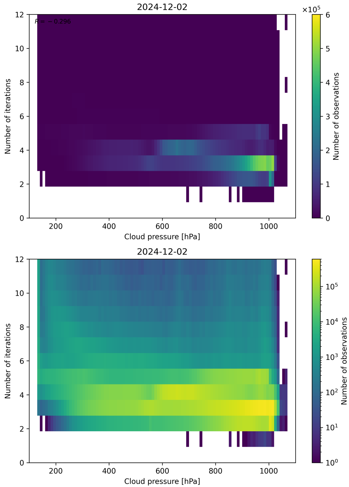
Figure 81: Scatter density plot of “Cloud pressure” against “Number of iterations” for 2024-12-01 to 2024-12-03.
