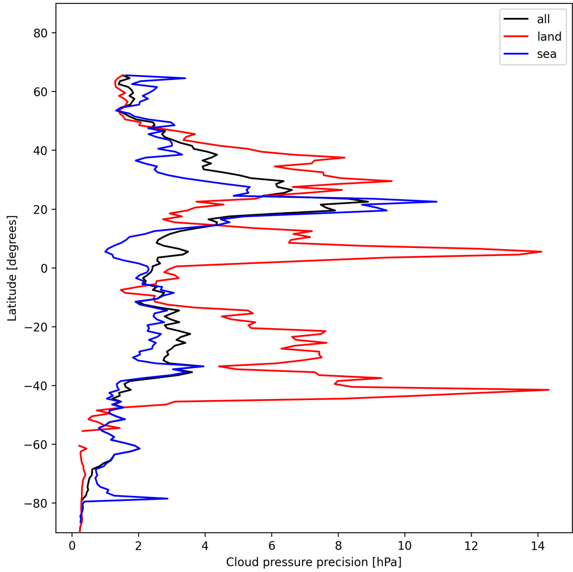
Figure 14: Zonal average of "Cloud pressure precision" for 2024-12-01 to 2024-12-03.
