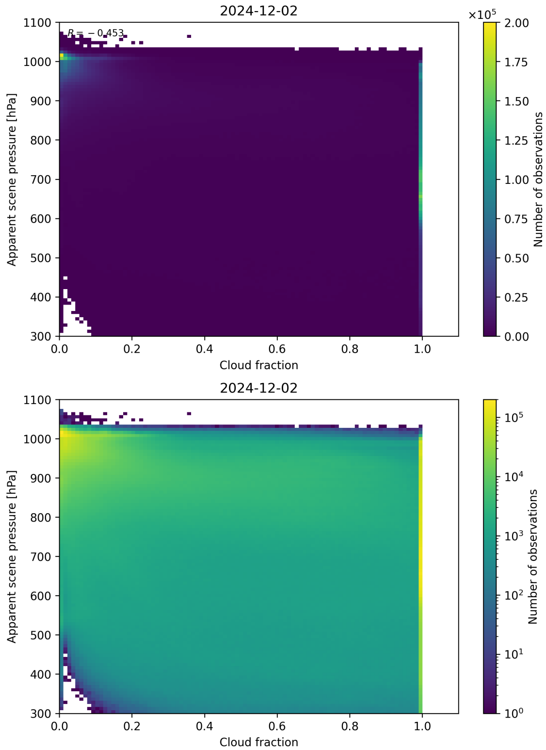
Figure 70: Scatter density plot of “Cloud fraction” against “Apparent scene pressure” for 2024-12-01 to 2024-12-03.
