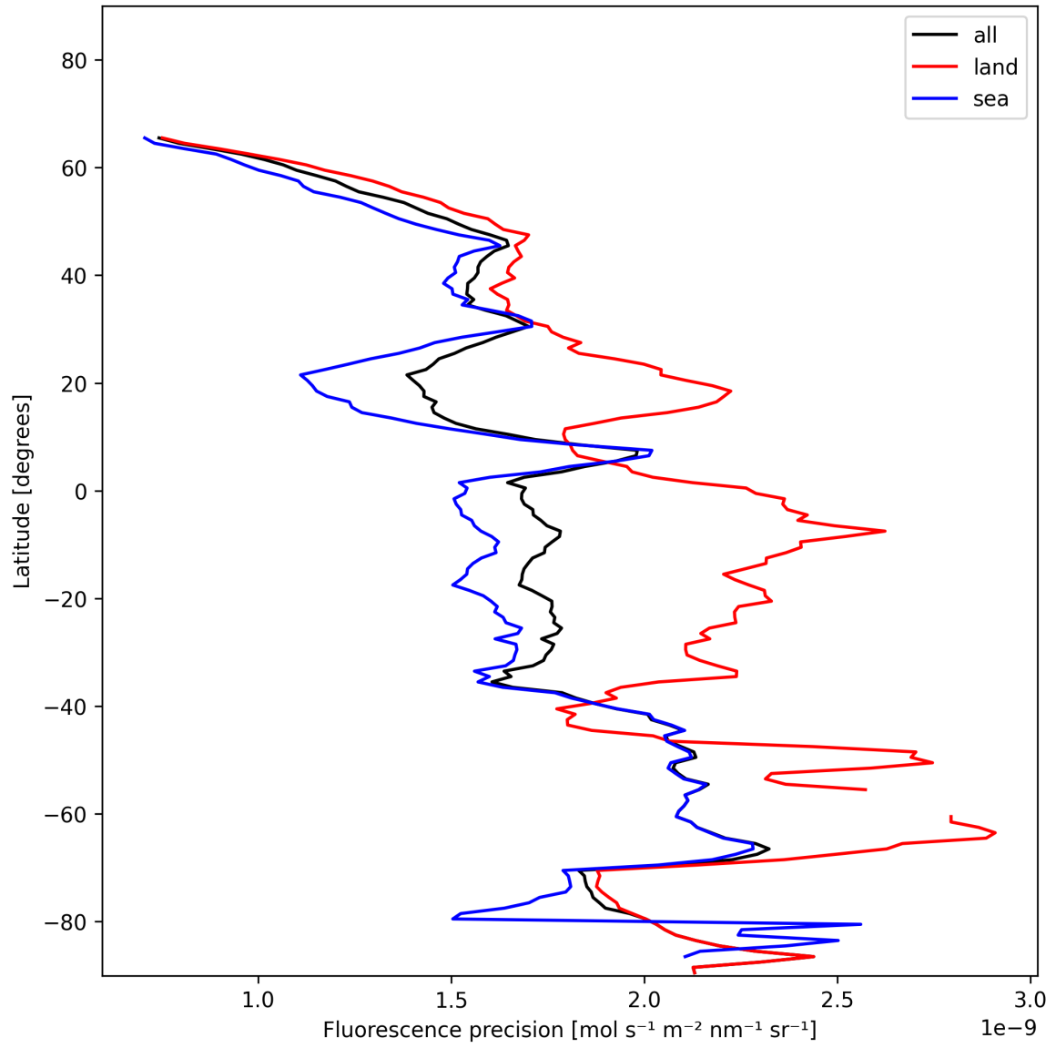
Figure 24: Zonal average of “Fluorescence precision” for 2024-12-01 to 2024-12-03.
