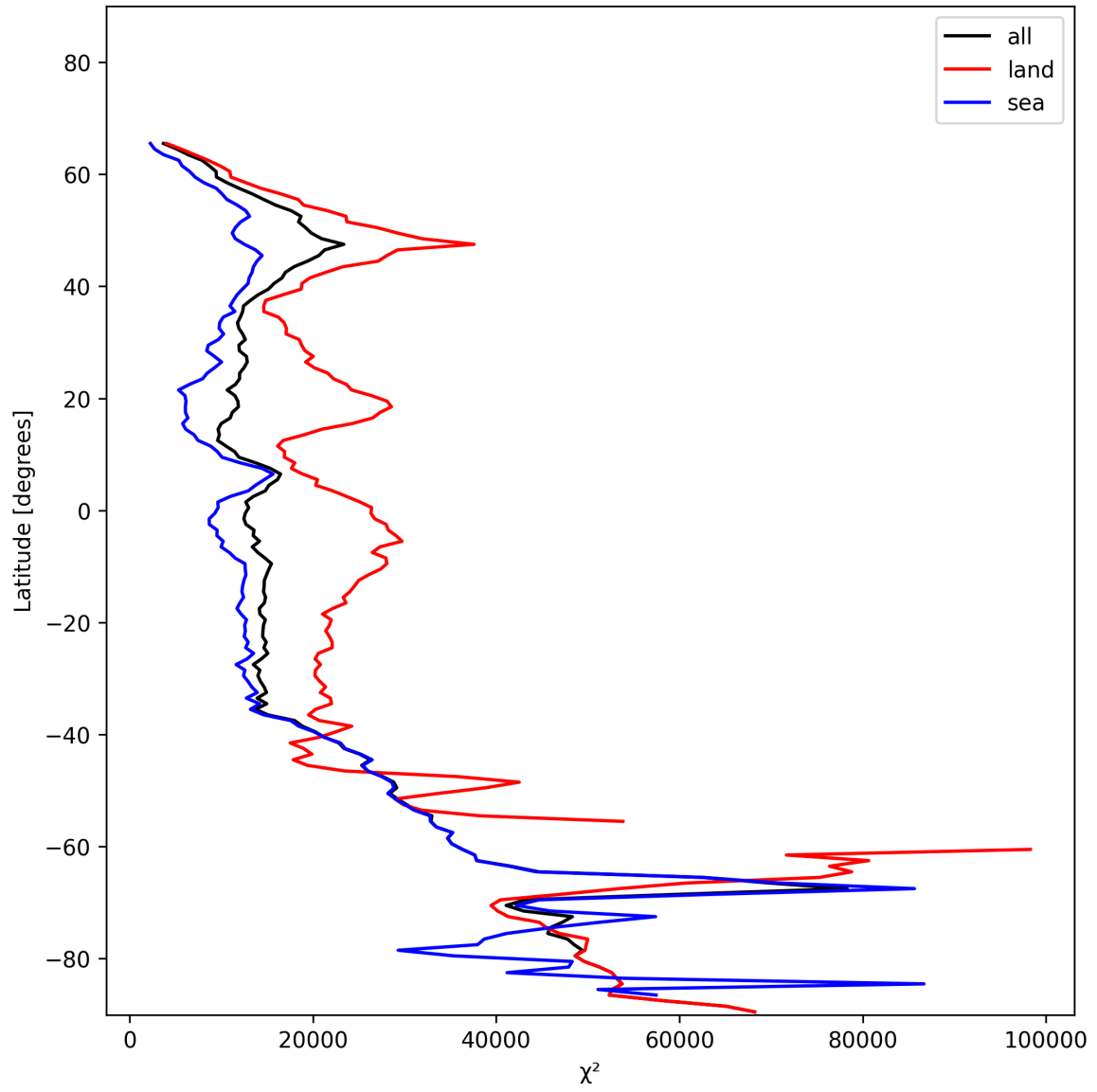
Figure 21: Zonal average of “ \chi^2 ” for 2024-12-01 to 2024-12-03.
