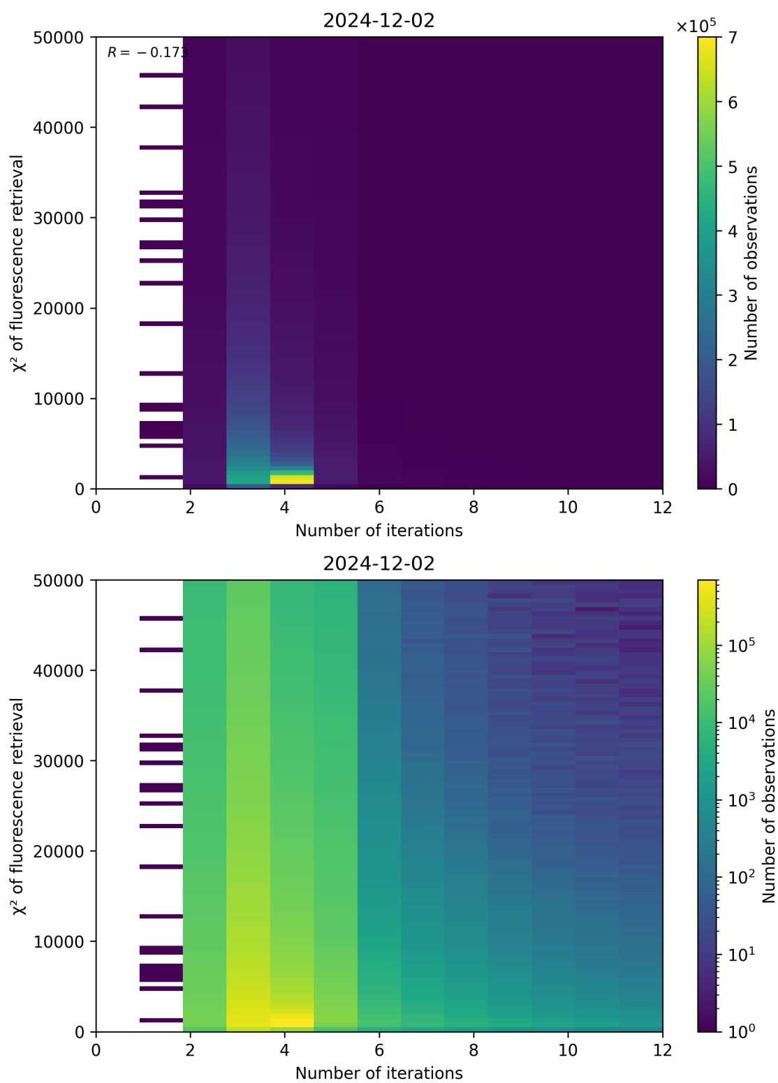
Figure 97: Scatter density plot of “Number of iterations” against “ \chi^2 of fluorescence retrieval” for 2024-12-01 to 2024-12-03.
