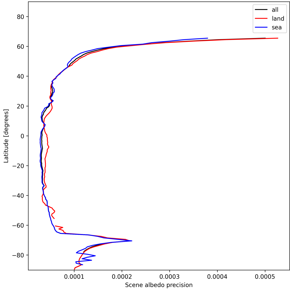
Figure 18: Zonal average of “Scene albedo precision” for 2024-12-01 to 2024-12-03.
