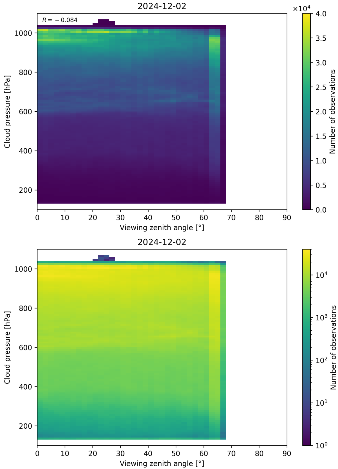
Figure 121: Scatter density plot of “Viewing zenith angle” against “Cloud pressure” for 2024-12-01 to 2024-12-03.
