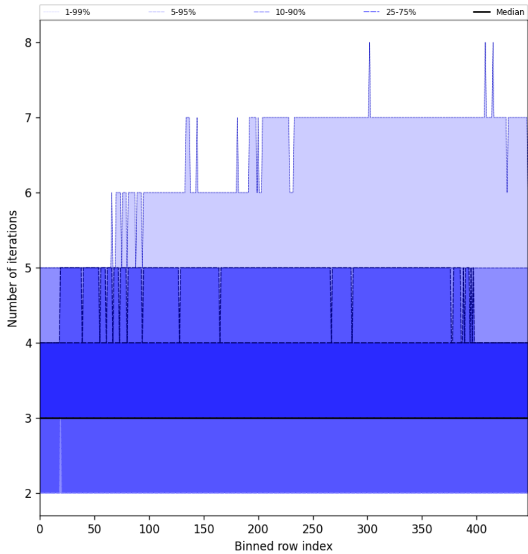
Figure 56: Along track statistics of “Number of iterations” for 2024-12-01 to 2024-12-03
