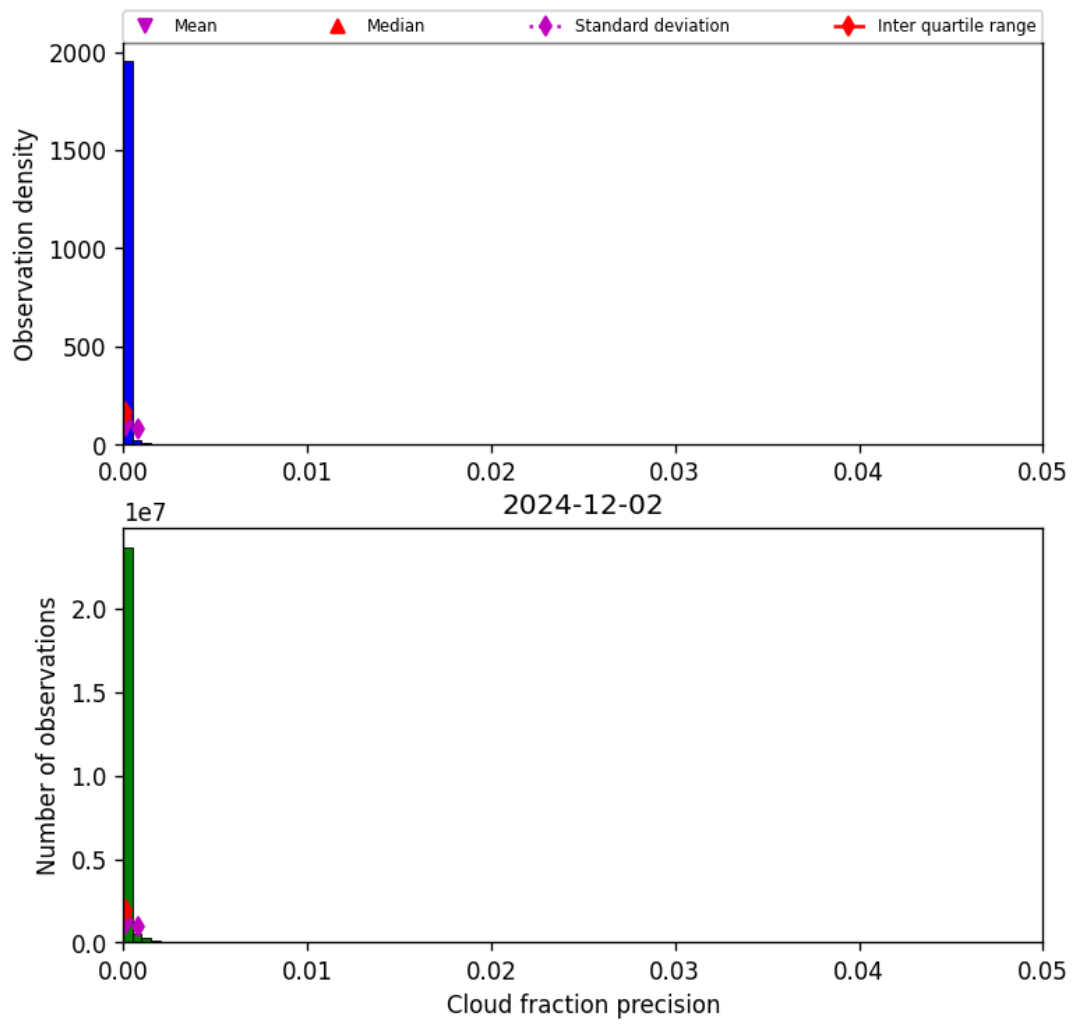
Figure 33: Histogram of “Cloud fraction precision” for 2024-12-01 to 2024-12-03
