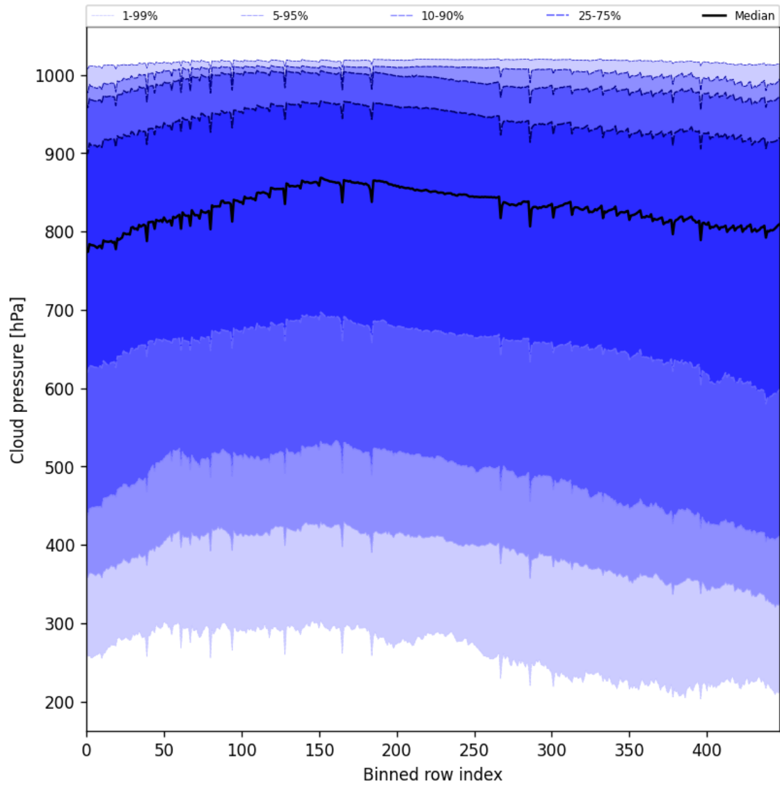
Figure 47: Along track statistics of “Cloud pressure” for 2024-12-01 to 2024-12-03
