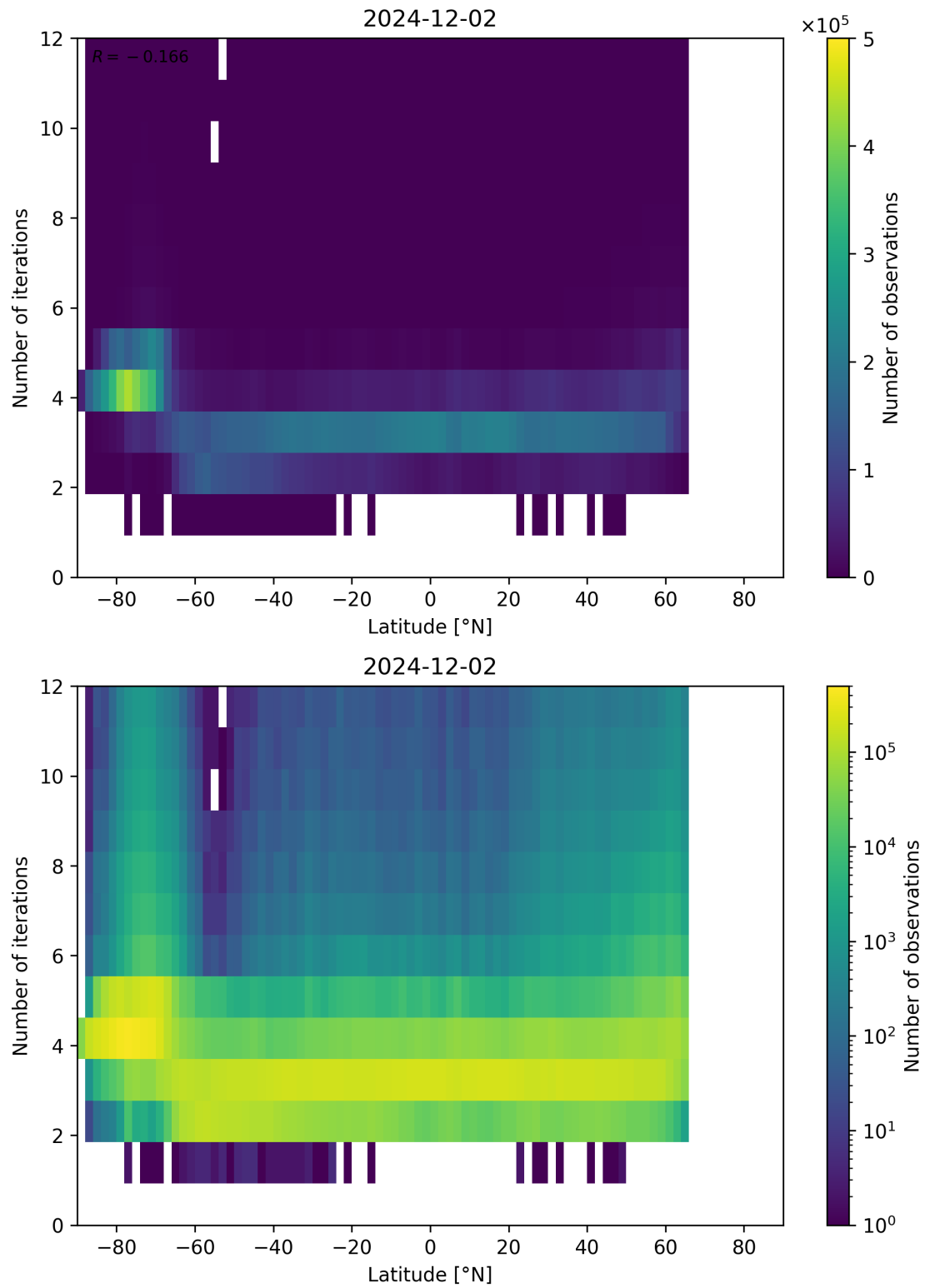
Figure 93: Scatter density plot of “Latitude” against “Number of iterations” for 2024-12-01 to 2024-12-03.
