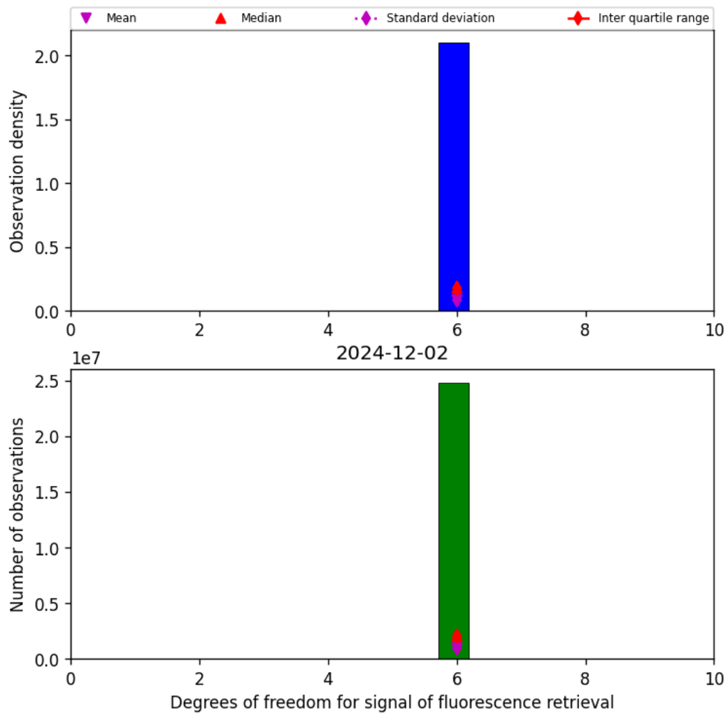
Figure 43: Histogram of "Degrees of freedom for signal of fluorescence retrieval" for 2024-12-01 to 2024-12-03
