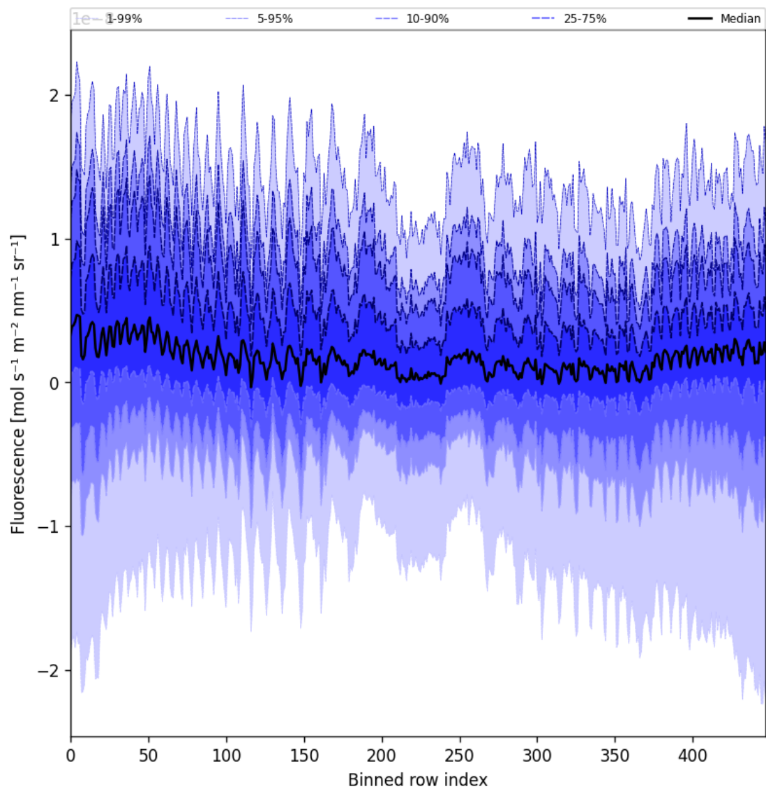
Figure 57: Along track statistics of “Fluorescence” for 2024-12-01 to 2024-12-03
