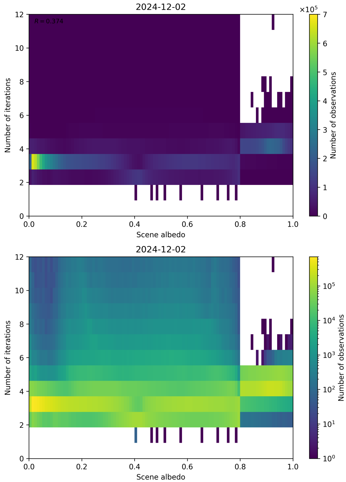
Figure 105: Scatter density plot of “Scene albedo” against “Number of iterations” for 2024-12-01 to 2024-12-03.
