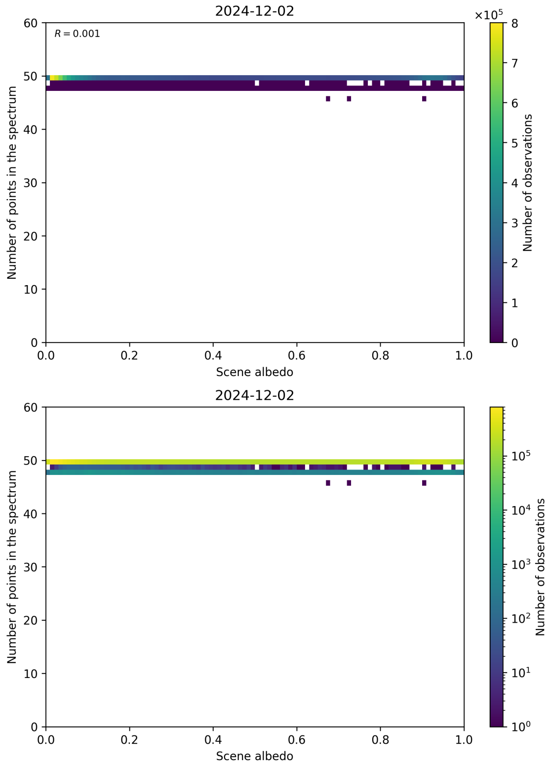
Figure 106: Scatter density plot of “Scene albedo” against “Number of points in the spectrum” for 2024-12-01 to 2024-12-03.
