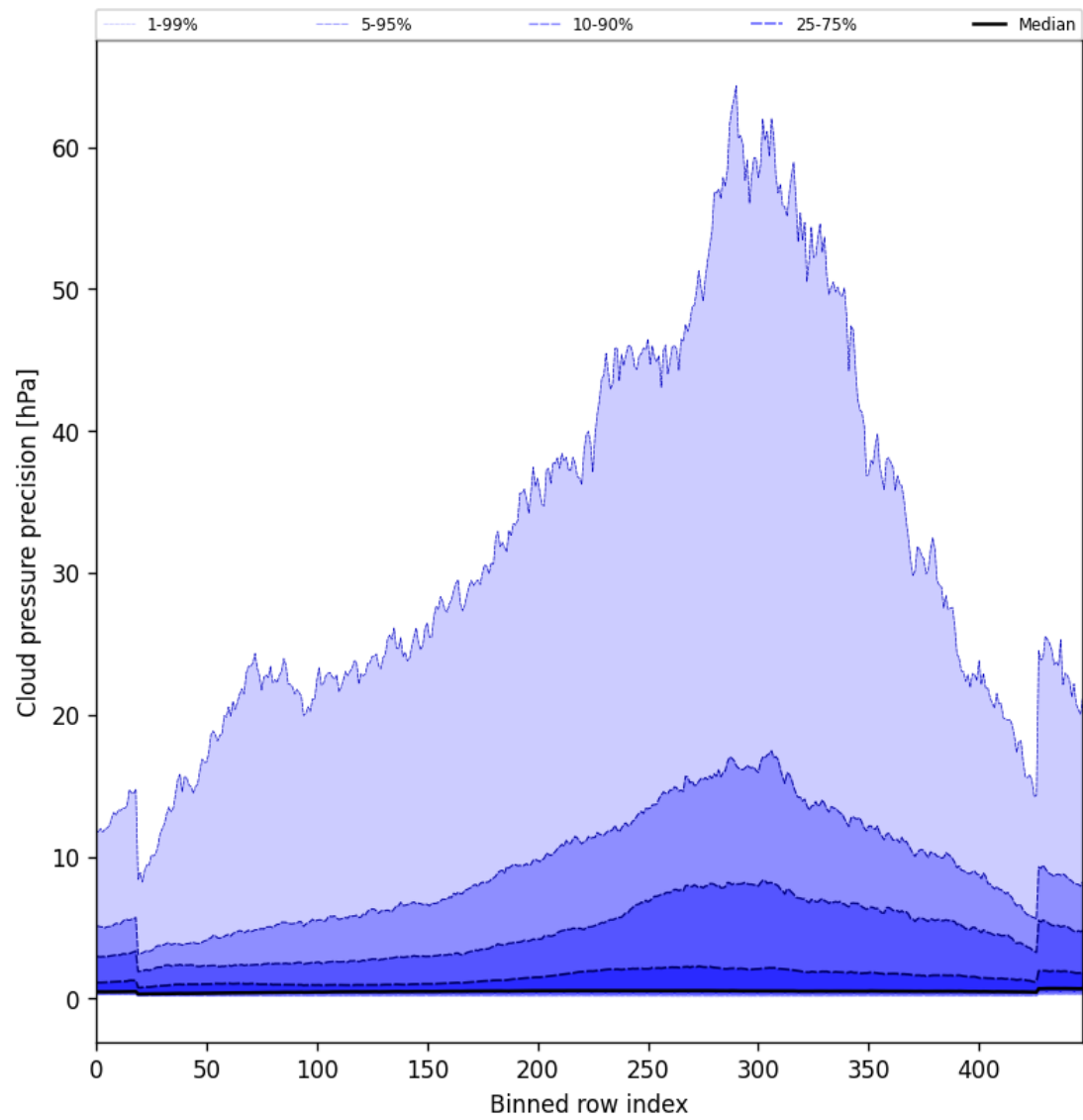
Figure 48: Along track statistics of “Cloud pressure precision” for 2024-12-01 to 2024-12-03
