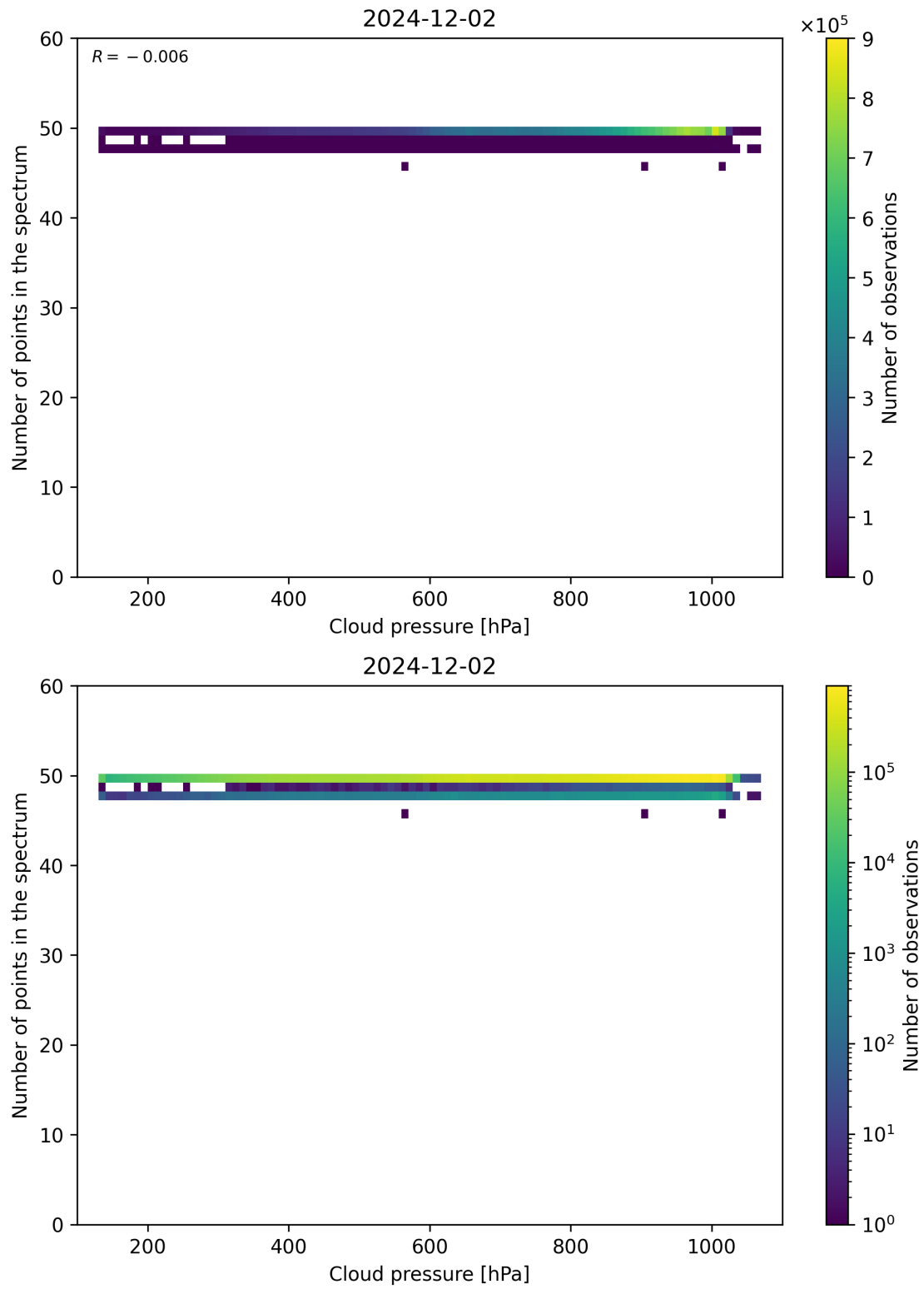
Figure 82: Scatter density plot of “Cloud pressure” against “Number of points in the spectrum” for 2024-12-01 to 2024-12-03.
