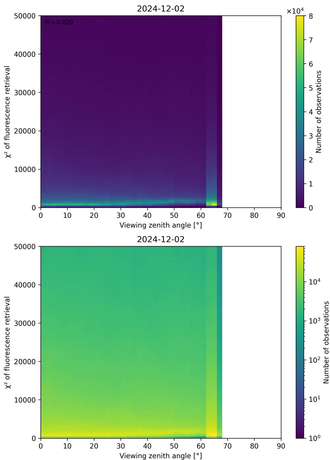
Figure 119: Scatter density plot of “Viewing zenith angle” against “ \chi^2 of fluorescence retrieval” for 2024-12-01 to 2024-12-03.
