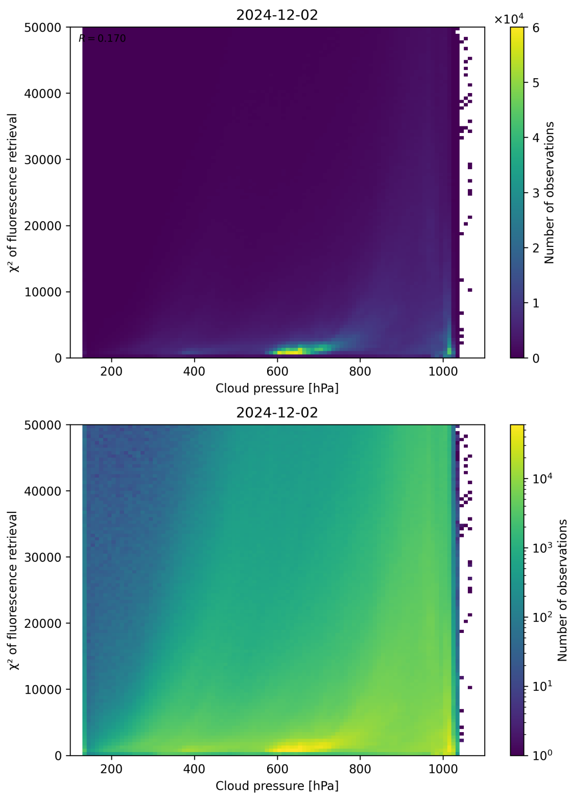
Figure 78: Scatter density plot of “Cloud pressure” against “ \chi^2 of fluorescence retrieval” for 2024-12-01 to 2024-12-03.
