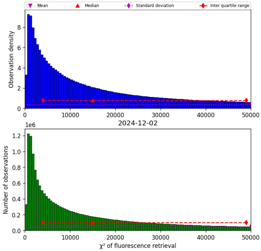
Figure 42: Histogram of “ \chi^2 of fluorescence retrieval” for 2024-12-01 to 2024-12-03
