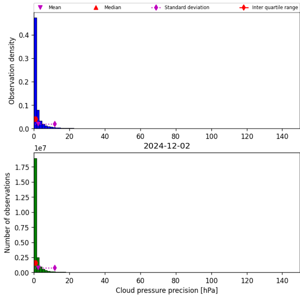
Figure 31: Histogram of “Cloud pressure precision” for 2024-12-01 to 2024-12-03
