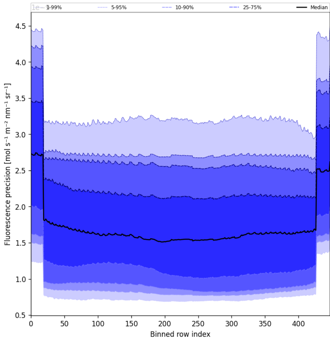
Figure 58: Along track statistics of “Fluorescence precision” for 2024-12-01 to 2024-12-03
