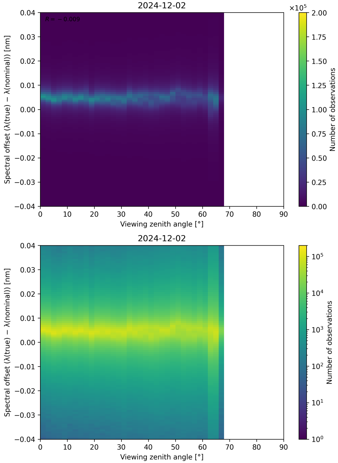
Figure 128: Scatter density plot of “Viewing zenith angle” against “Spectral offset ( \lambda_{\text{true}} - \lambda_{\text{nominal}} )” for 2024-12-01 to 2024-12-03.
