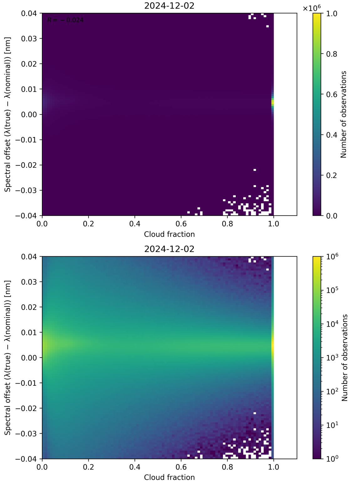
Figure 76: Scatter density plot of “Cloud fraction” against “Spectral offset ( \lambda_{\text{true}} - \lambda_{\text{nominal}} )” for 2024-12-01 to 2024-12-03.
