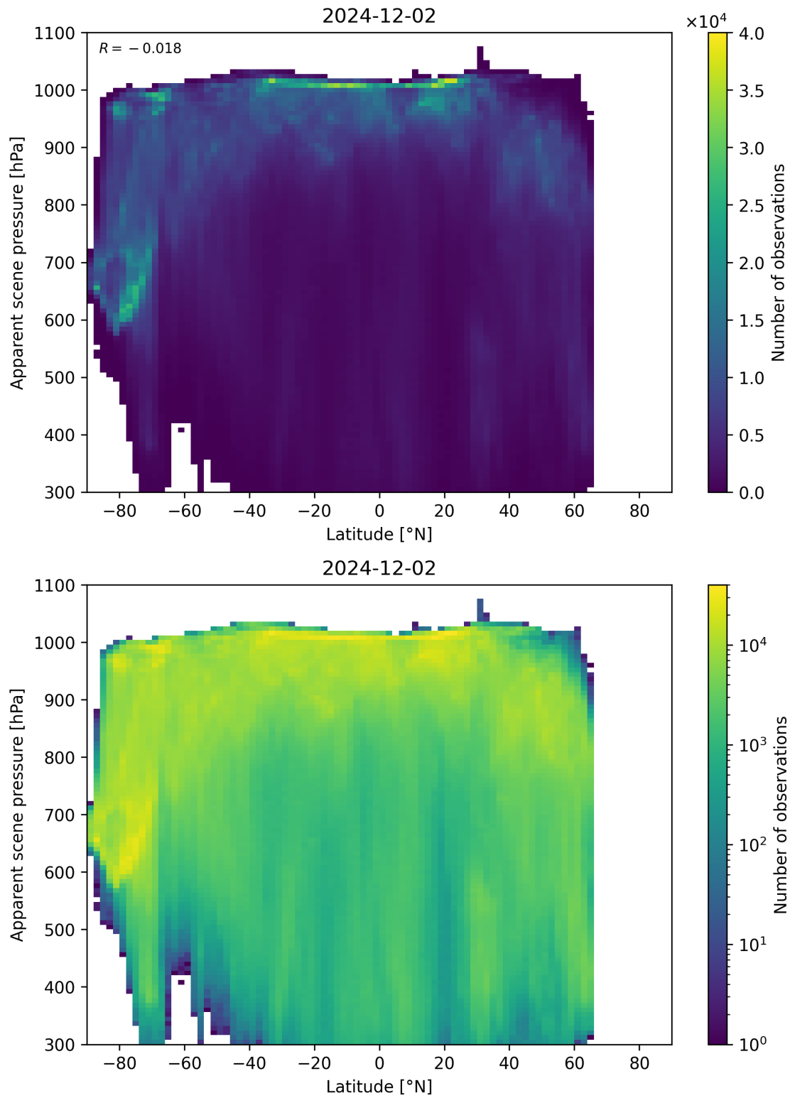
Figure 88: Scatter density plot of “Latitude” against “Apparent scene pressure” for 2024-12-01 to 2024-12-03.
