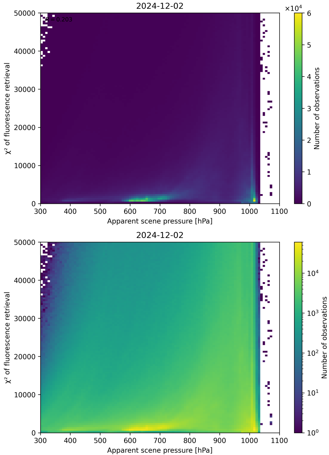
Figure 63: Scatter density plot of “Apparent scene pressure” against “ \chi^2 of fluorescence retrieval” for 2024-12-01 to 2024-12-03.
