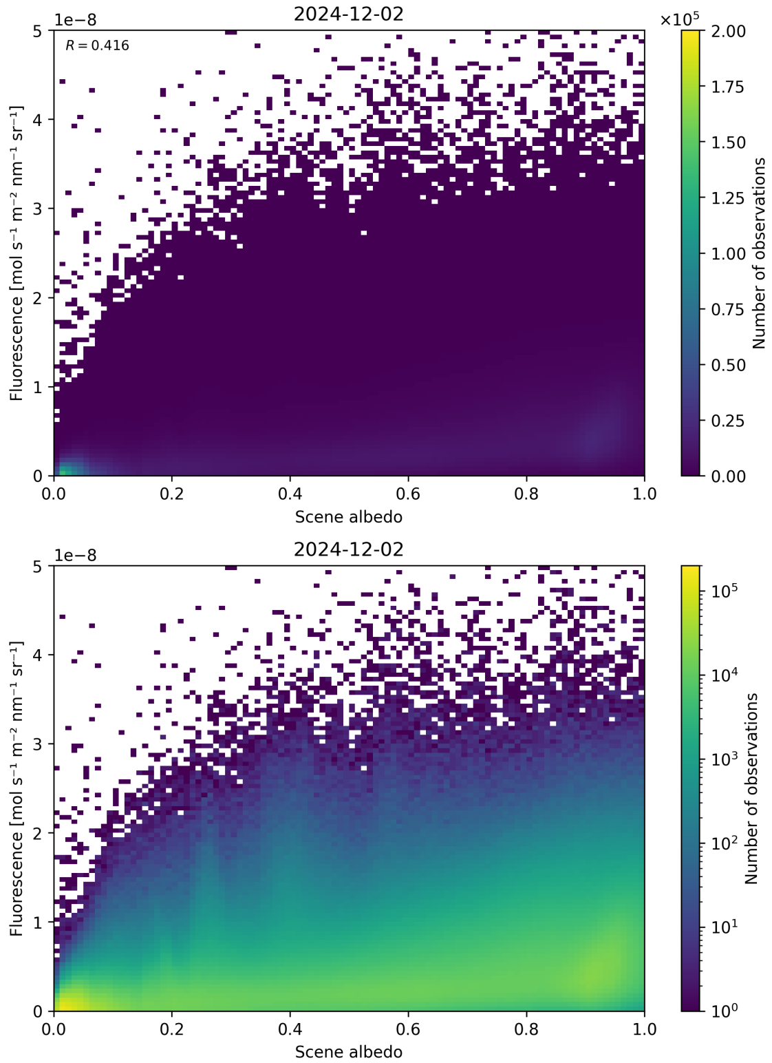
Figure 104: Scatter density plot of “Scene albedo” against “Fluorescence” for 2024-12-01 to 2024-12-03.
