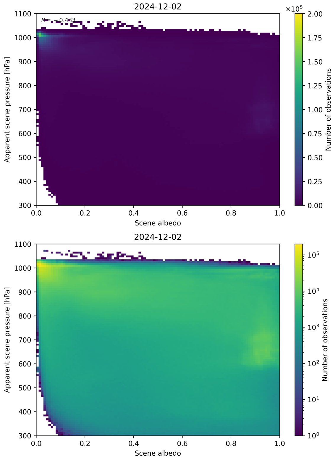
Figure 102: Scatter density plot of “Scene albedo” against “Apparent scene pressure” for 2024-12-01 to 2024-12-03.
