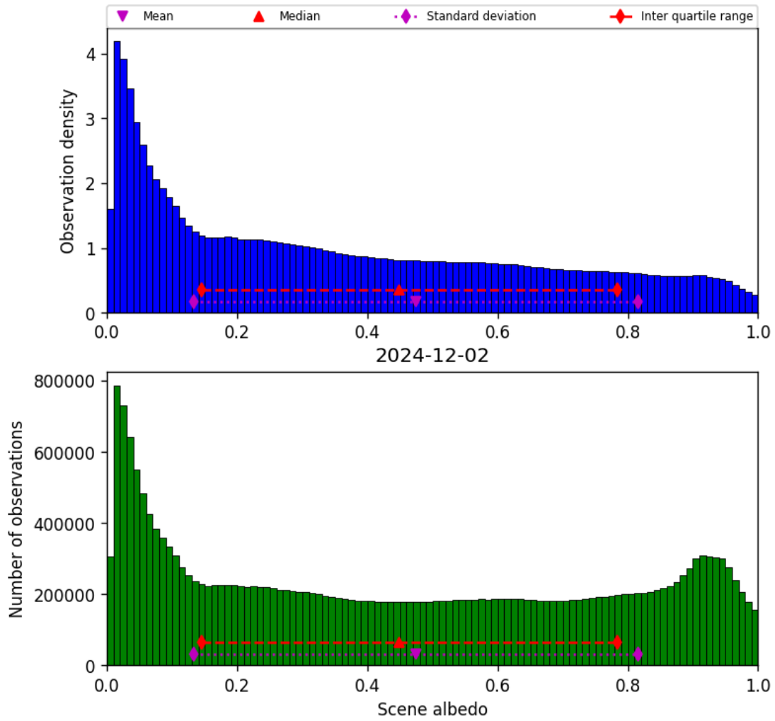
Figure 34: Histogram of “Scene albedo” for 2024-12-01 to 2024-12-03
