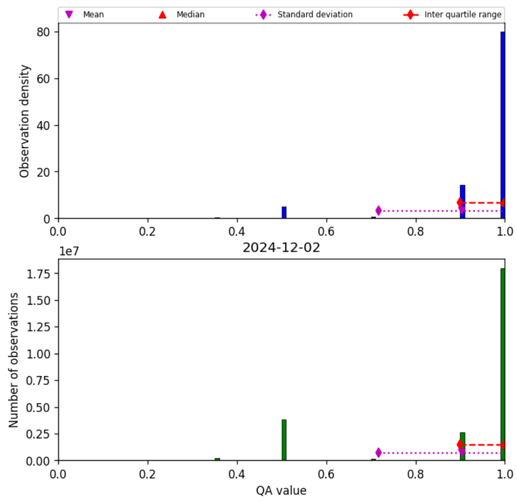
Figure 29: Histogram of “QA value” for 2024-12-01 to 2024-12-03
