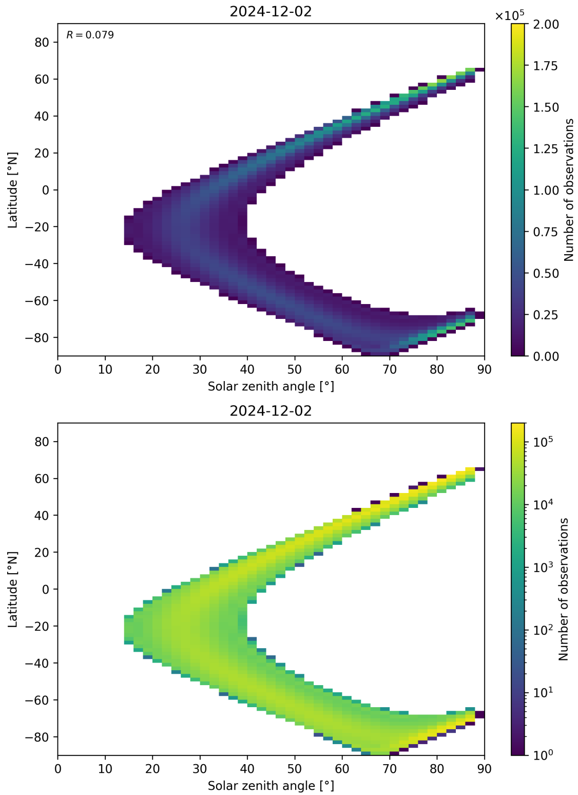
Figure 113: Scatter density plot of “Solar zenith angle” against “Latitude” for 2024-12-01 to 2024-12-03.
