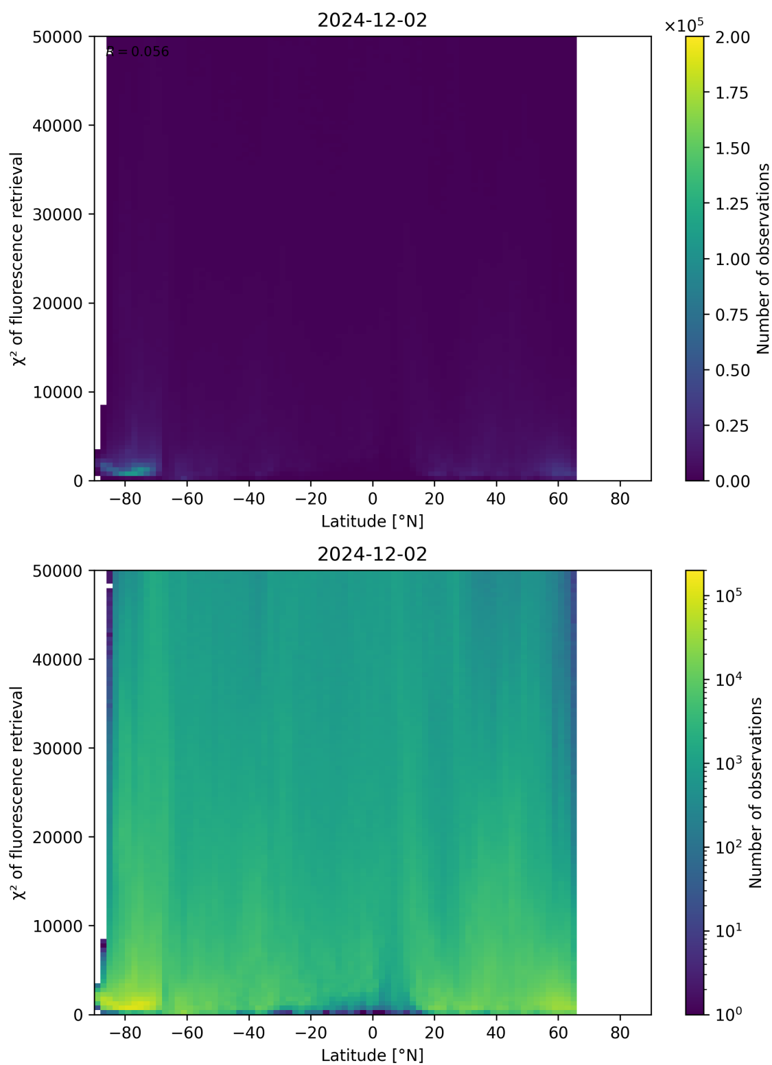
Figure 89: Scatter density plot of “Latitude” against “ \chi^2 of fluorescence retrieval” for 2024-12-01 to 2024-12-03.
