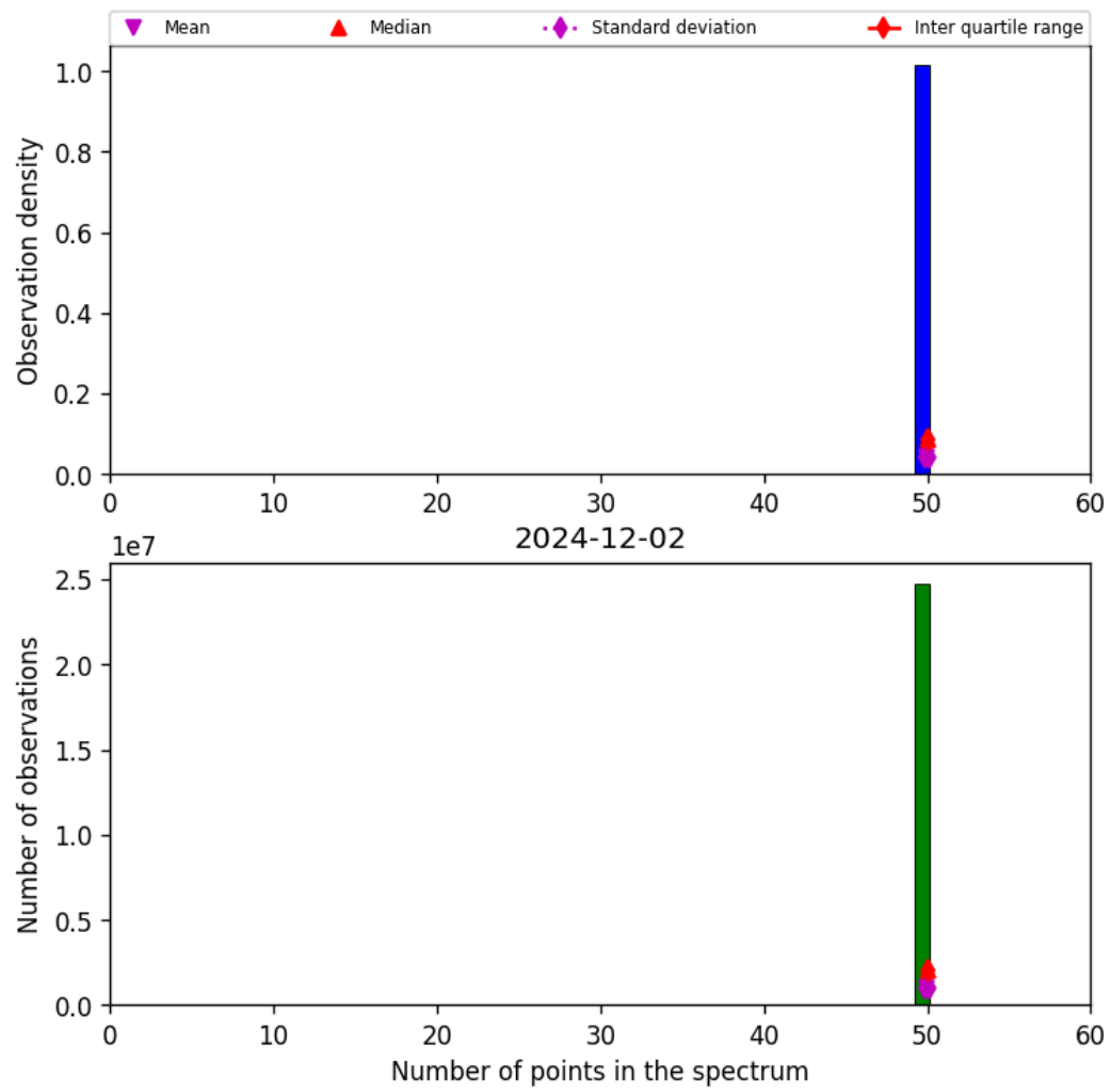
Figure 44: Histogram of “Number of points in the spectrum” for 2024-12-01 to 2024-12-03
