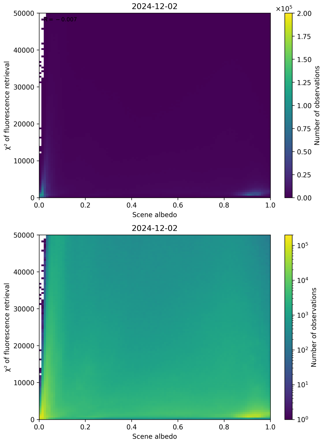
Figure 103: Scatter density plot of “Scene albedo” against “ \chi^2 of fluorescence retrieval” for 2024-12-01 to 2024-12-03.
