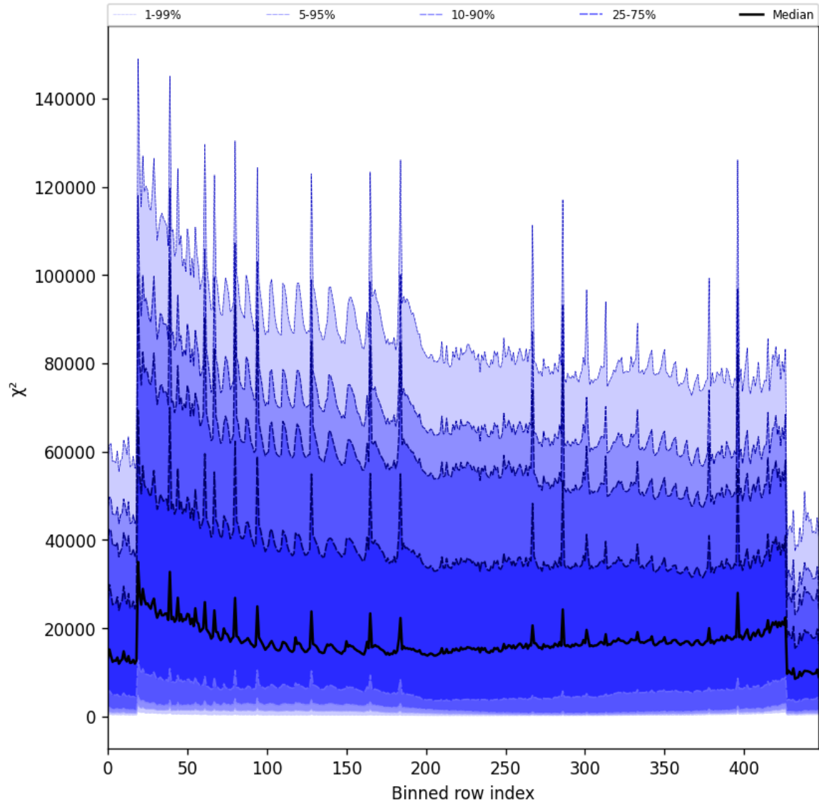
Figure 55: Along track statistics of “ \chi^2 ” for 2024-12-01 to 2024-12-03
