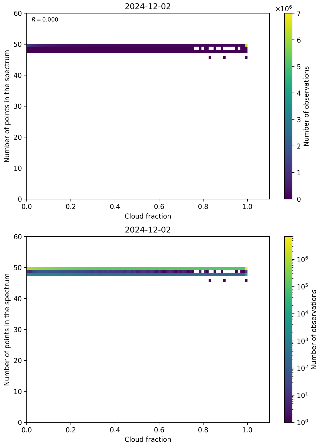
Figure 74: Scatter density plot of “Cloud fraction” against “Number of points in the spectrum” for 2024-12-01 to 2024-12-03.
