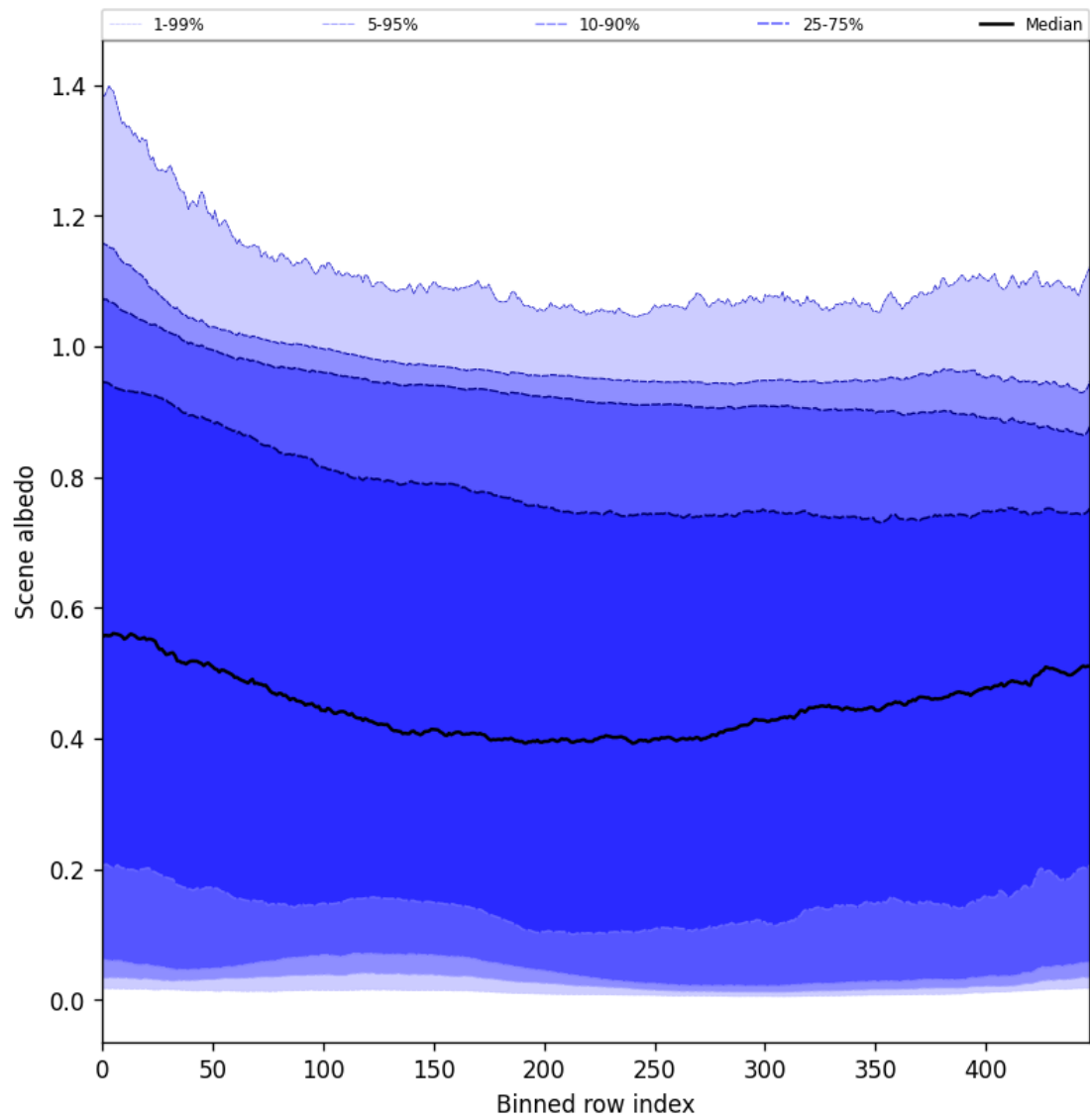
Figure 51: Along track statistics of “Scene albedo” for 2024-12-01 to 2024-12-03
