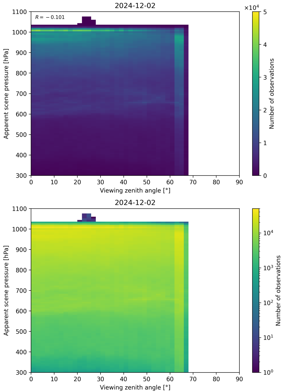
Figure 118: Scatter density plot of “Viewing zenith angle” against “Apparent scene pressure” for 2024-12-01 to 2024-12-03.
