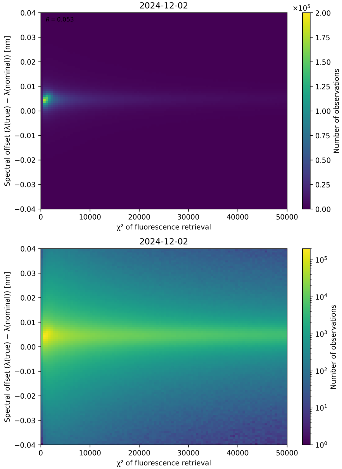
Figure 69: Scatter density plot of “ \chi^2 of fluorescence retrieval” against “Spectral offset ( \lambda_{\text{true}} - \lambda_{\text{nominal}} )” for 2024-12-01 to 2024-12-03.
