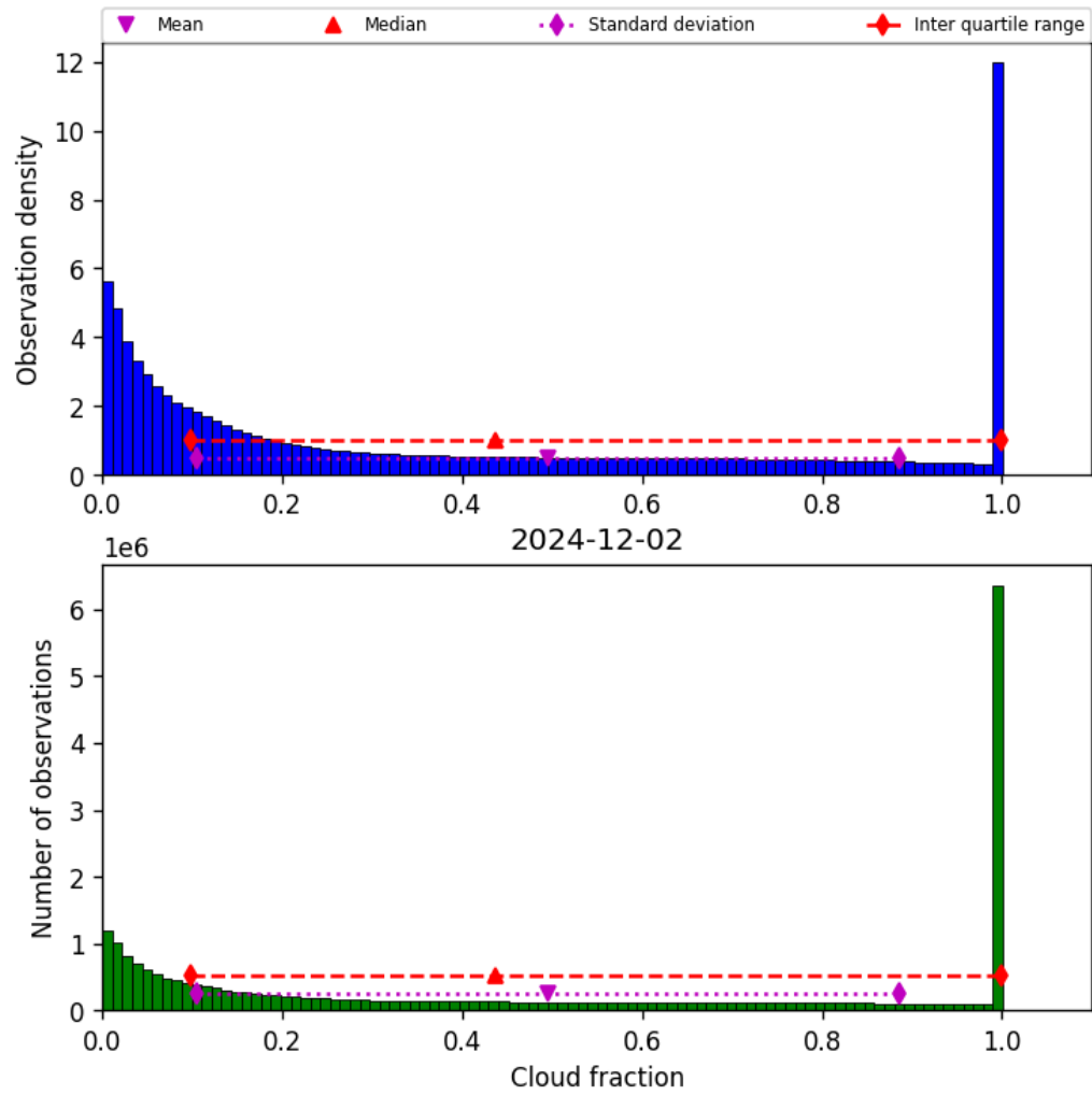
Figure 32: Histogram of “Cloud fraction” for 2024-12-01 to 2024-12-03
