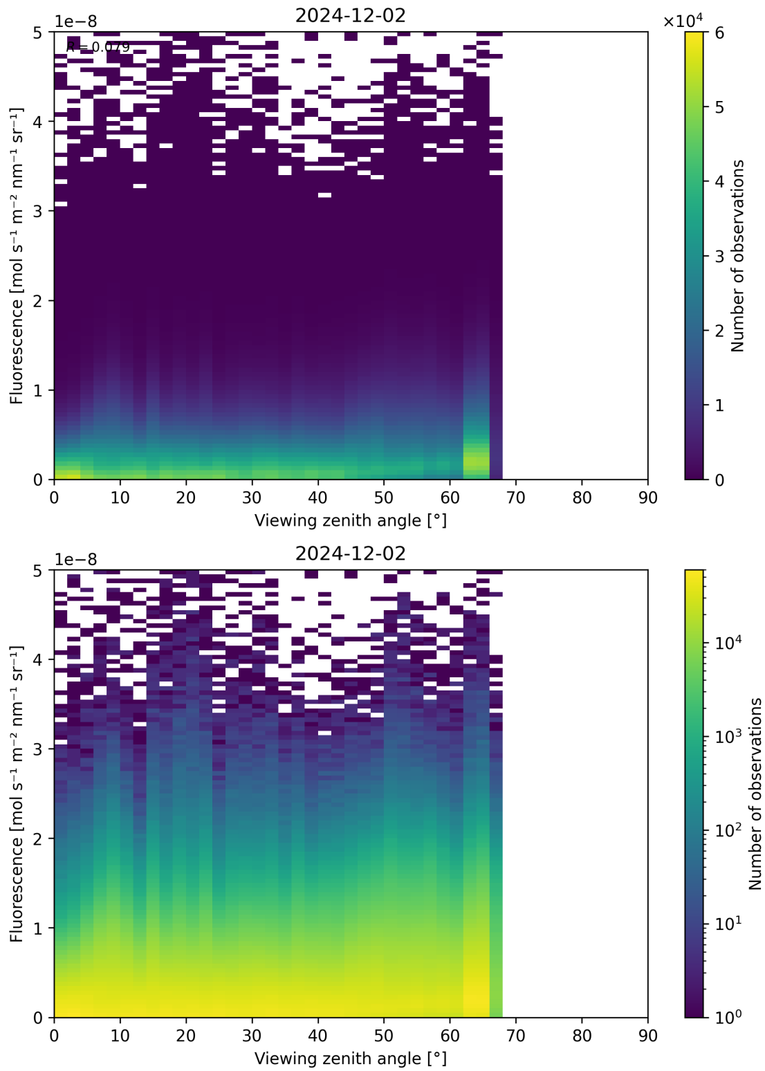
Figure 122: Scatter density plot of “Viewing zenith angle” against “Fluorescence” for 2024-12-01 to 2024-12-03.
