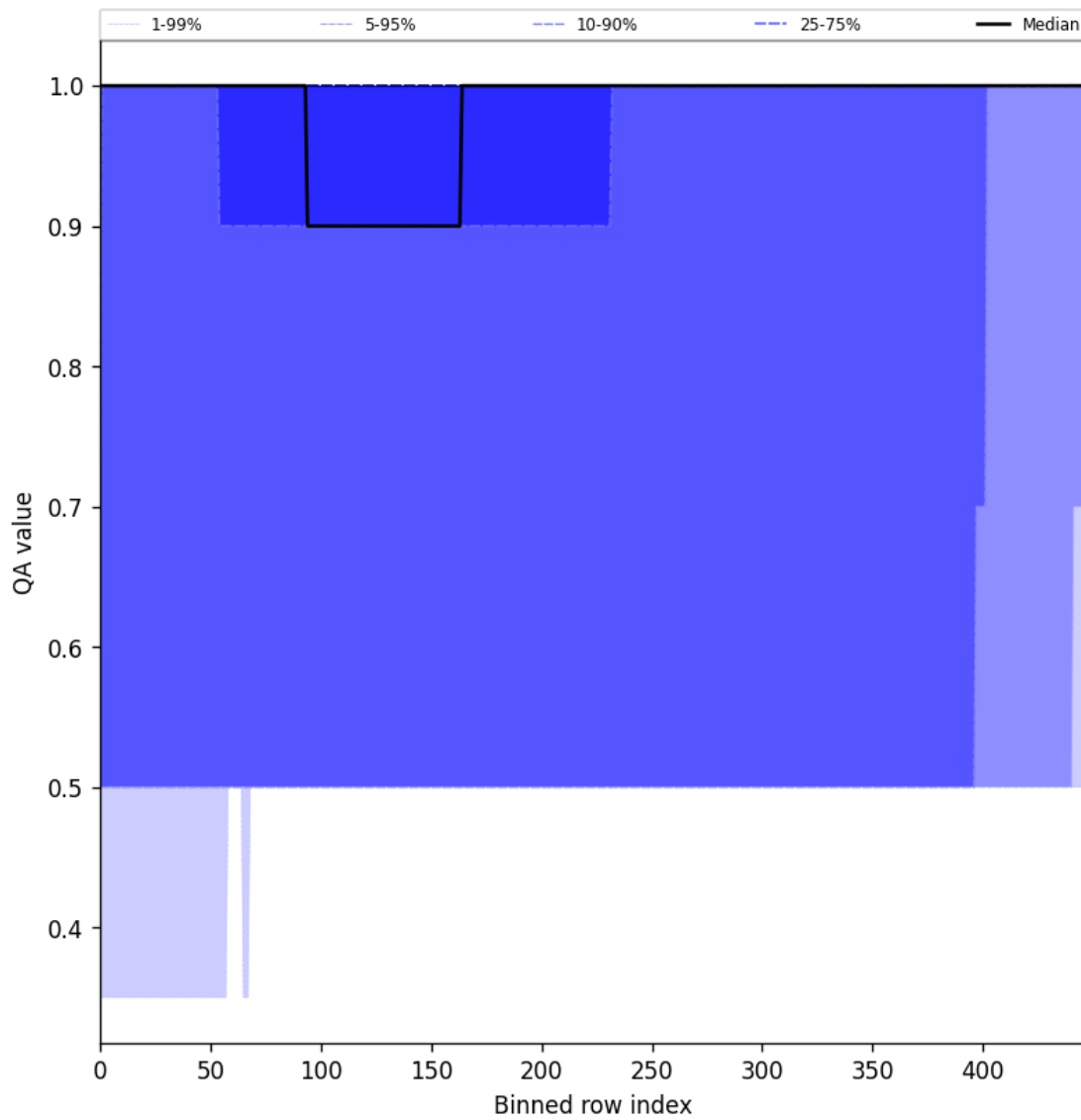
Figure 46: Along track statistics of “QA value” for 2024-12-01 to 2024-12-03
