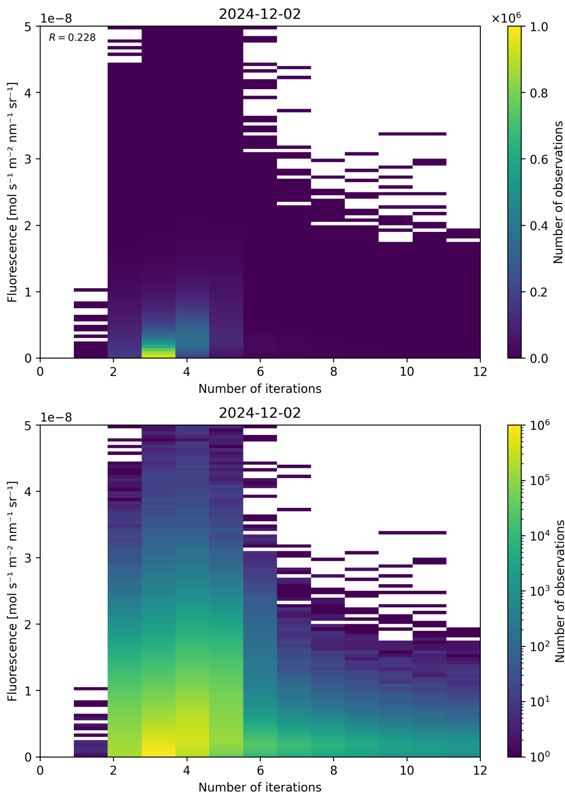
Figure 98: Scatter density plot of “Number of iterations” against “Fluorescence” for 2024-12-01 to 2024-12-03.
