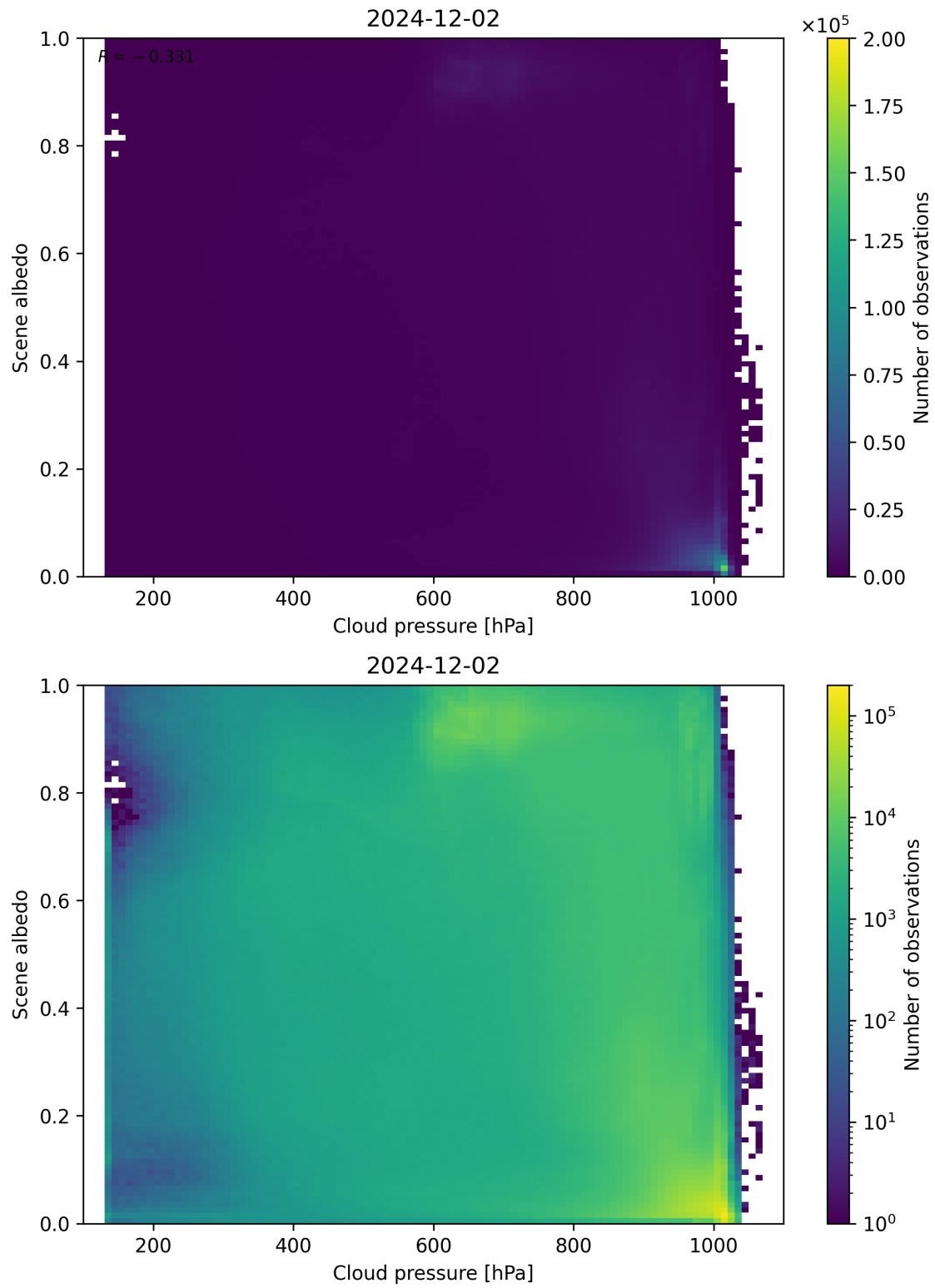
Figure 83: Scatter density plot of “Cloud pressure” against “Scene albedo” for 2024-12-01 to 2024-12-03.
