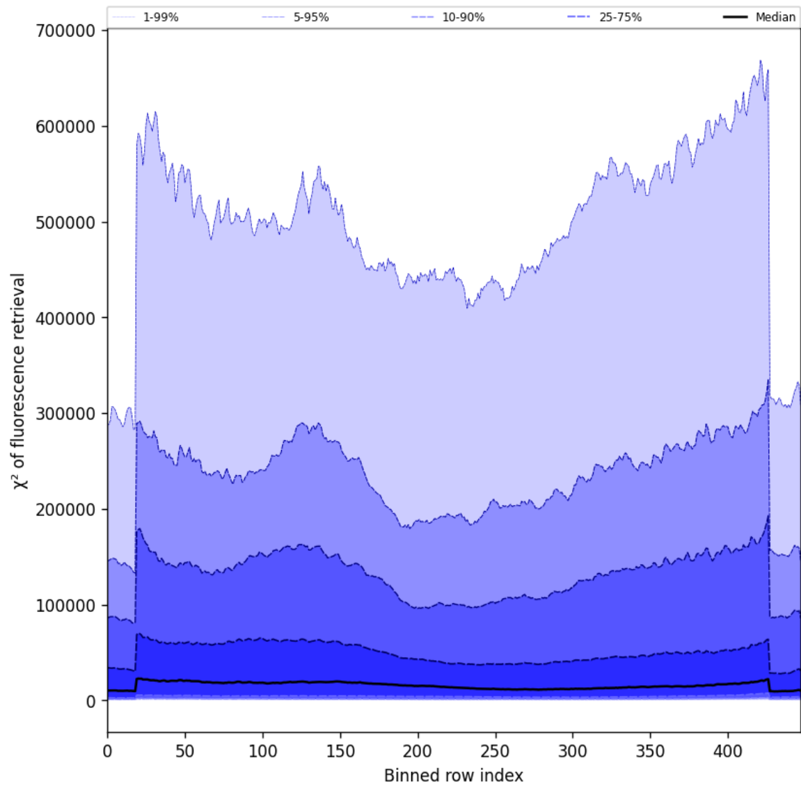
Figure 59: Along track statistics of “ \chi^2 of fluorescence retrieval” for 2024-12-01 to 2024-12-03
