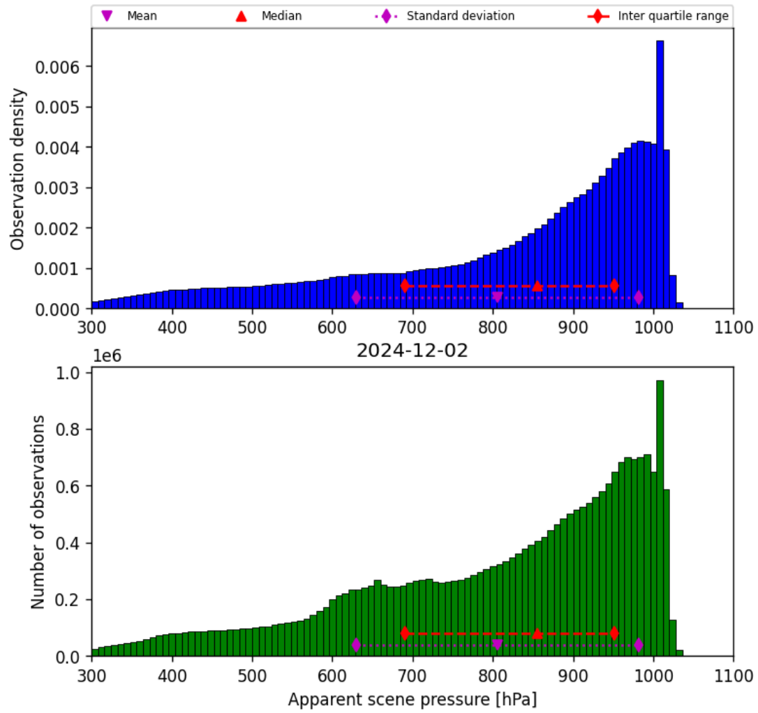
Figure 36: Histogram of “Apparent scene pressure” for 2024-12-01 to 2024-12-03
