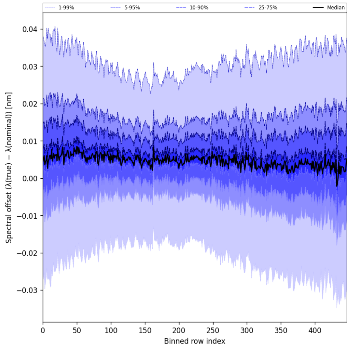
Figure 62: Along track statistics of “Spectral offset ( \lambda_{\text{true}} - \lambda_{\text{nominal}} )” for 2024-12-01 to 2024-12-03
