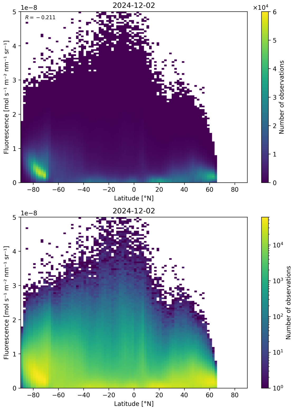
Figure 92: Scatter density plot of “Latitude” against “Fluorescence” for 2024-12-01 to 2024-12-03.
