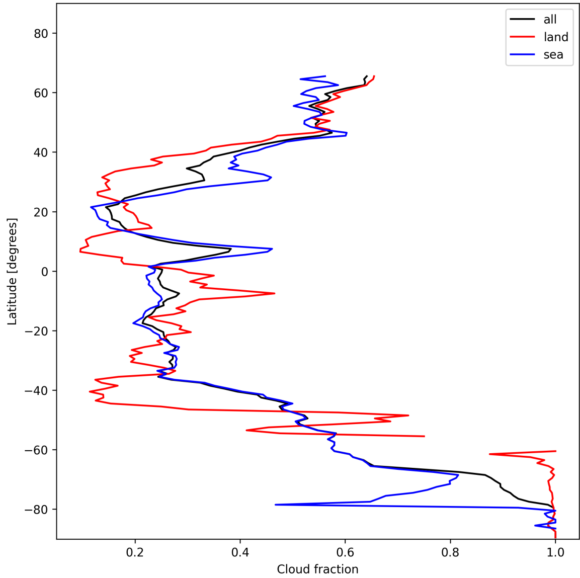
Figure 15: Zonal average of “Cloud fraction” for 2024-12-01 to 2024-12-03.
