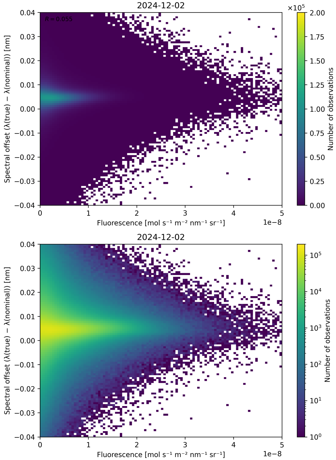
Figure 87: Scatter density plot of “Fluorescence” against “Spectral offset ( \lambda_{\text{true}} - \lambda_{\text{nominal}} )” for 2024-12-01 to 2024-12-03.
