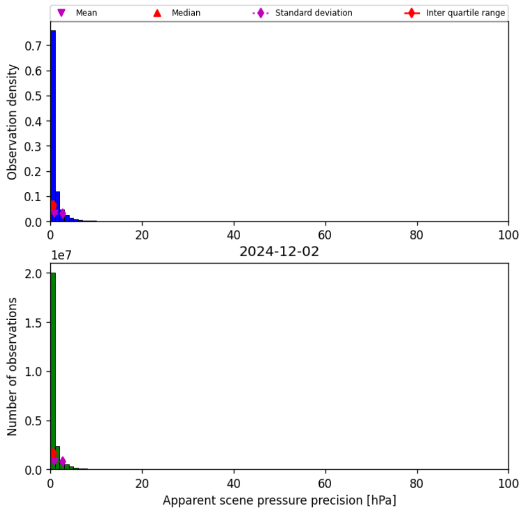
Figure 37: Histogram of “Apparent scene pressure precision” for 2024-12-01 to 2024-12-03
