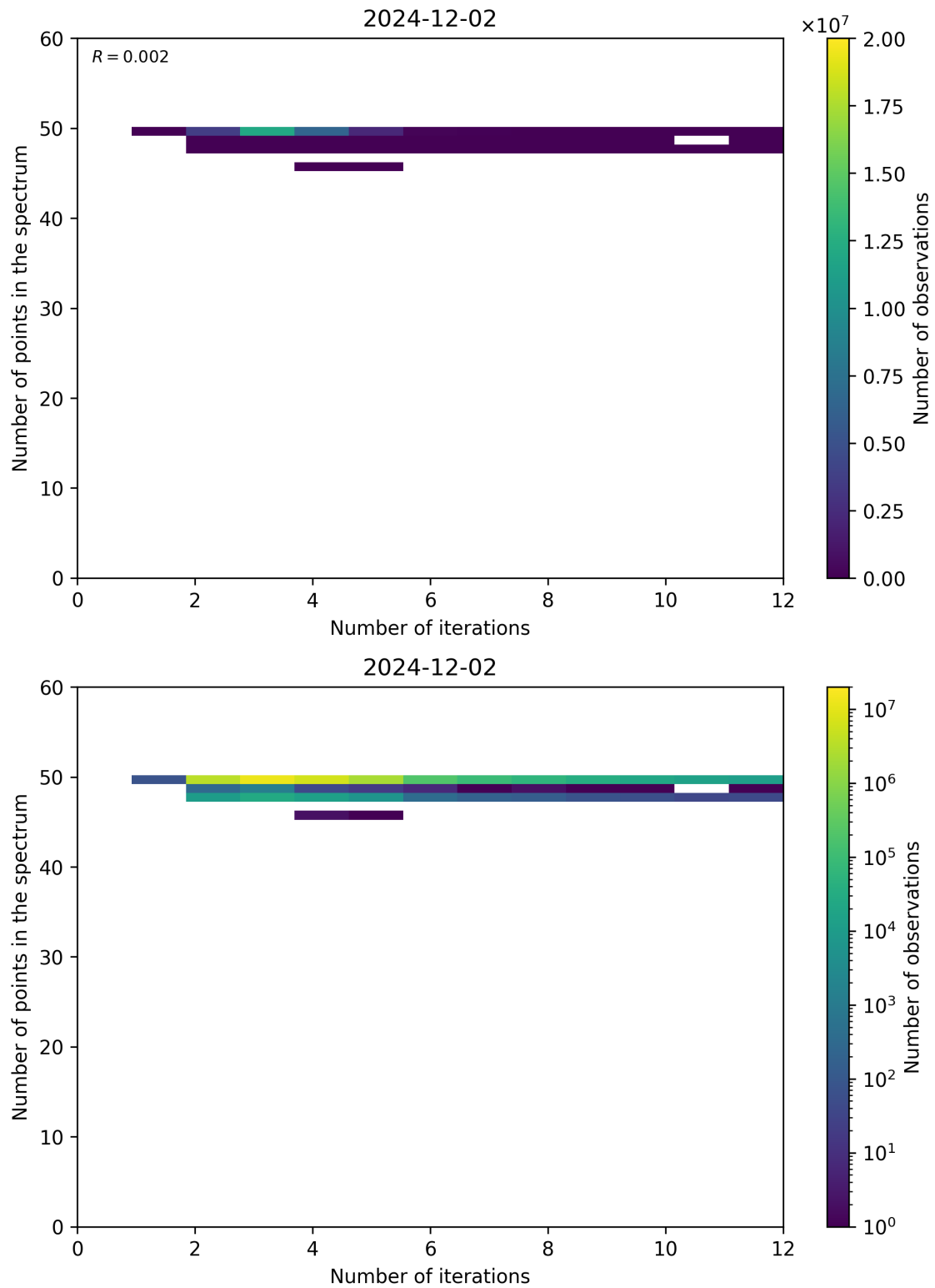
Figure 99: Scatter density plot of “Number of iterations” against “Number of points in the spectrum” for 2024-12-01 to 2024-12-03.
