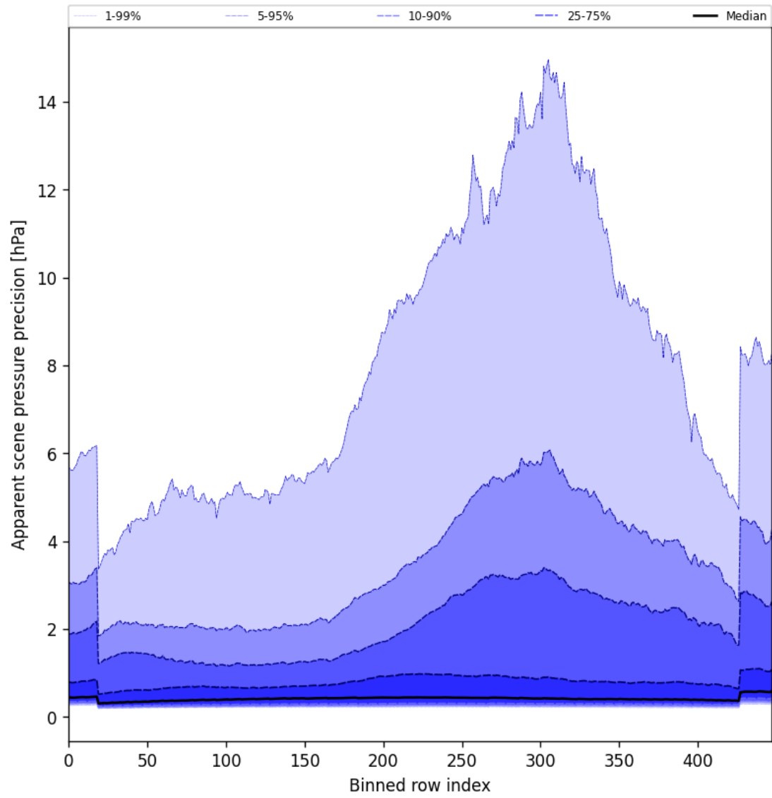
Figure 54: Along track statistics of “Apparent scene pressure precision” for 2024-12-01 to 2024-12-03
