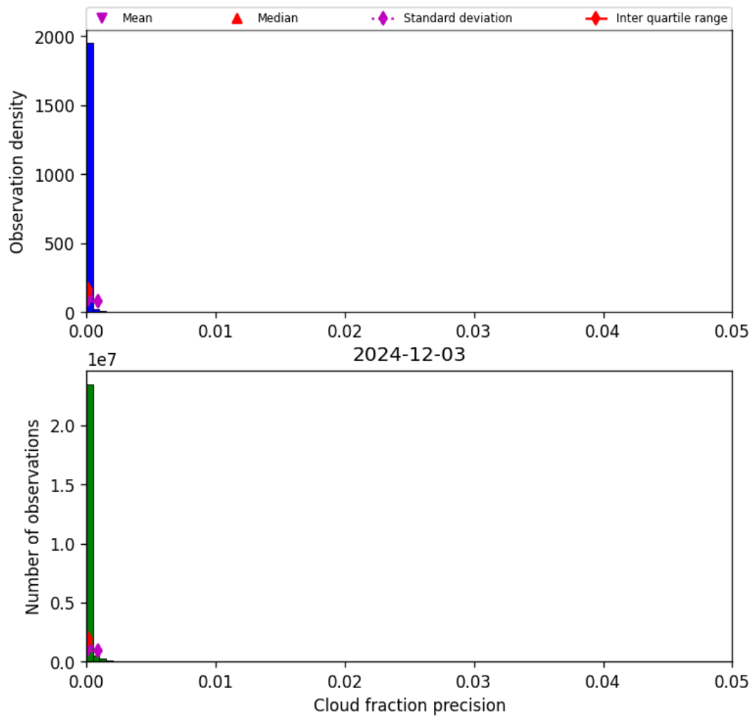
Figure 33: Histogram of “Cloud fraction precision” for 2024-12-02 to 2024-12-04
