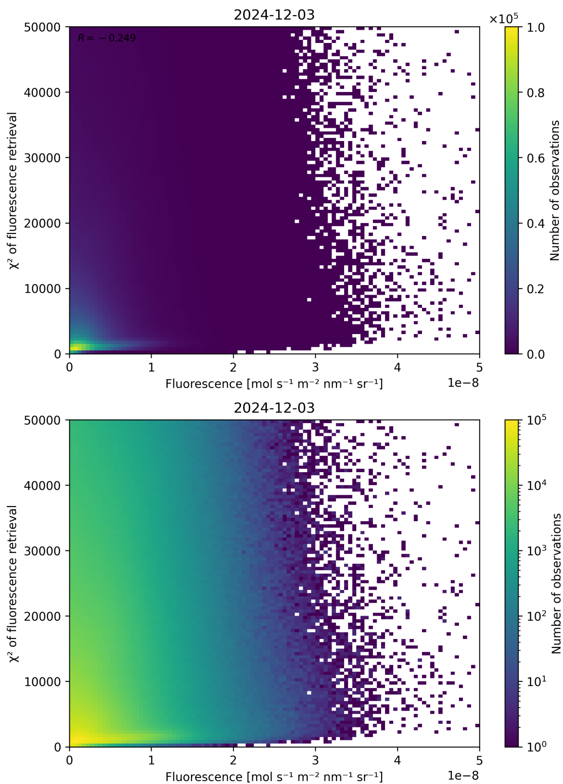
Figure 85: Scatter density plot of “Fluorescence” against “ \chi^2 of fluorescence retrieval” for 2024-12-02 to 2024-12-04.
