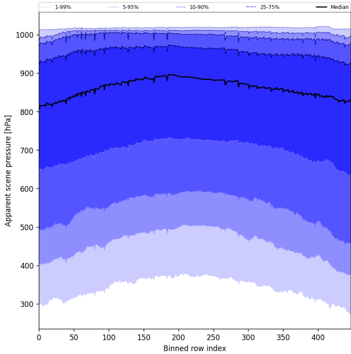
Figure 53: Along track statistics of “Apparent scene pressure” for 2024-12-02 to 2024-12-04
