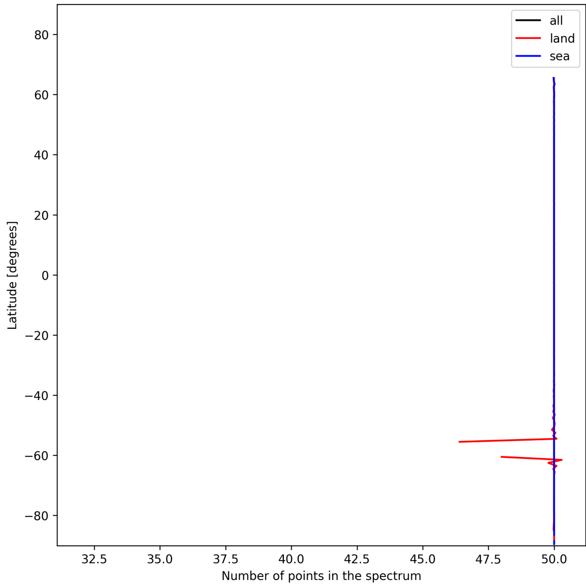
Figure 27: Zonal average of “Number of points in the spectrum” for 2024-12-02 to 2024-12-04.
