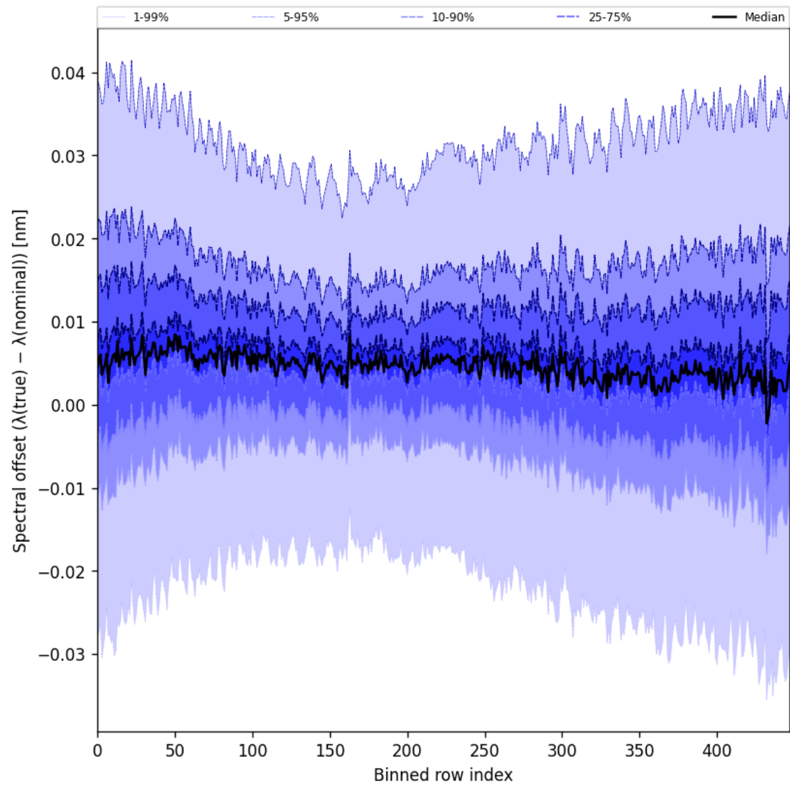
Figure 62: Along track statistics of “Spectral offset ( \lambda_{\text{true}} - \lambda_{\text{nominal}} )” for 2024-12-02 to 2024-12-04
