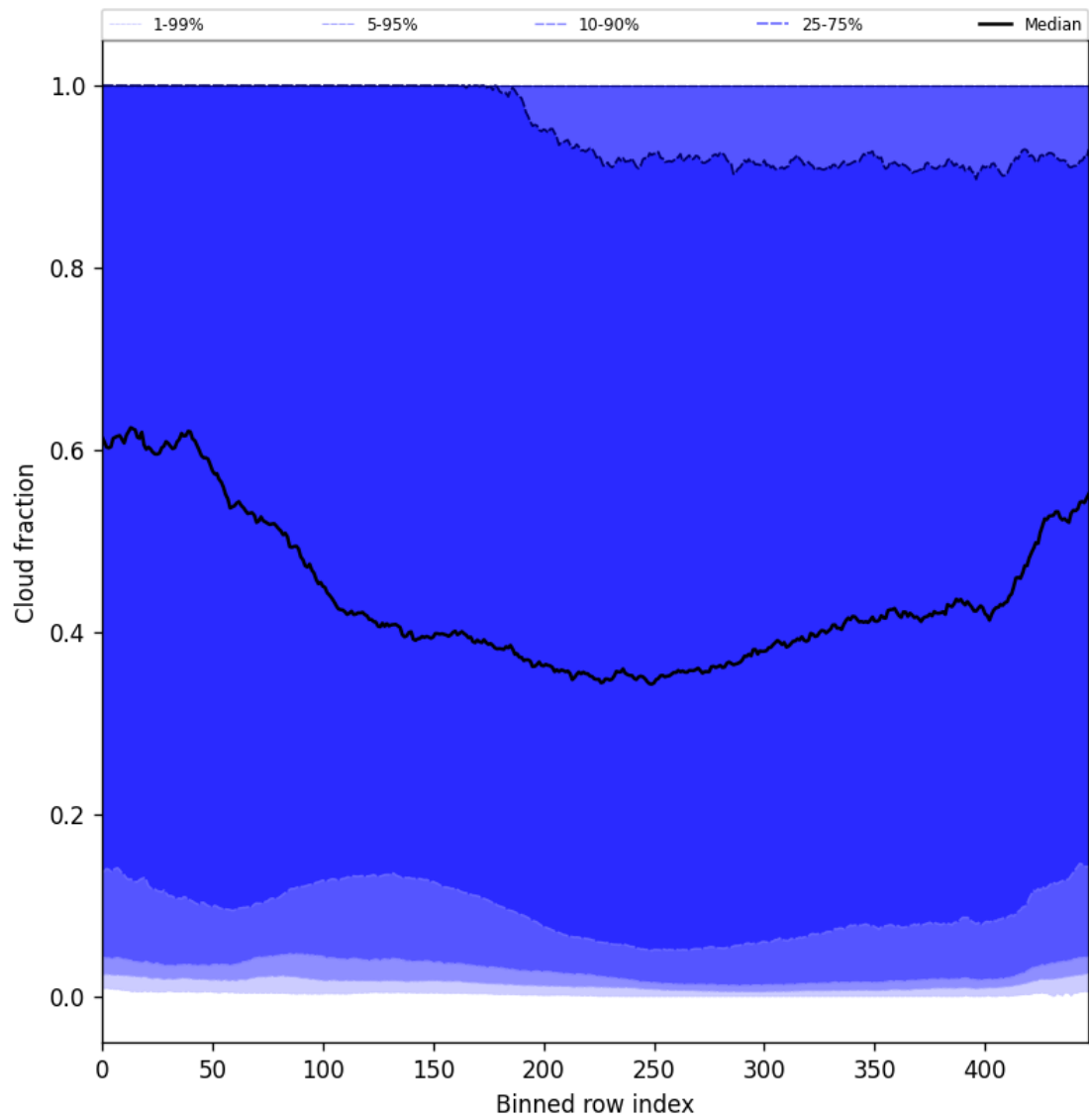
Figure 49: Along track statistics of “Cloud fraction” for 2024-12-02 to 2024-12-04
