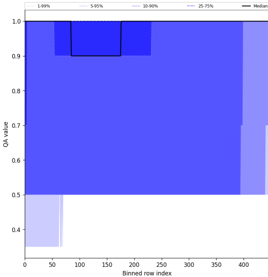
Figure 46: Along track statistics of “QA value” for 2024-12-02 to 2024-12-04
