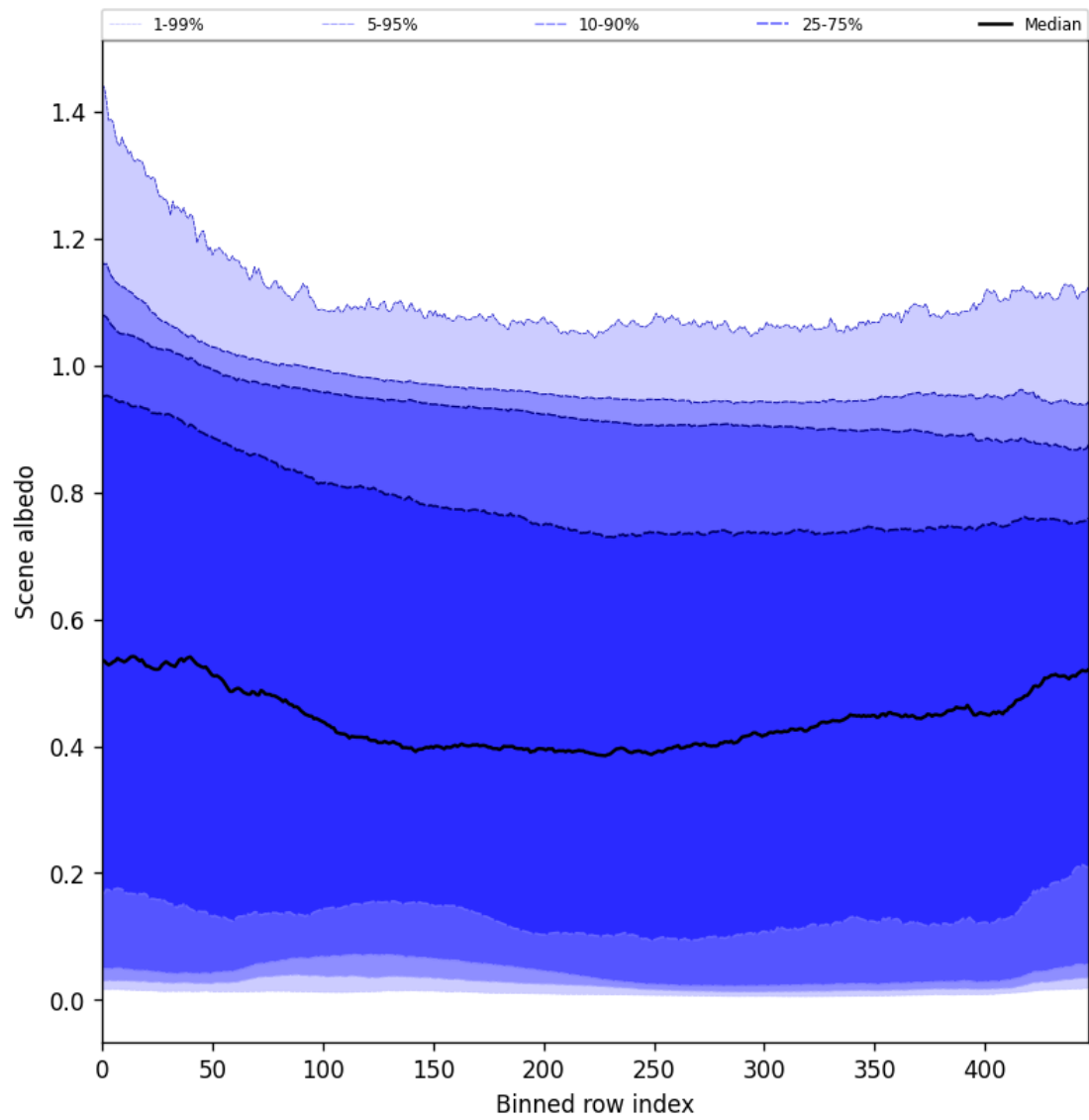
Figure 51: Along track statistics of “Scene albedo” for 2024-12-02 to 2024-12-04
