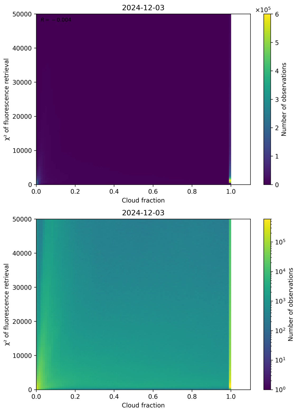
Figure 71: Scatter density plot of “Cloud fraction” against “ \chi^2 of fluorescence retrieval” for 2024-12-02 to 2024-12-04.
