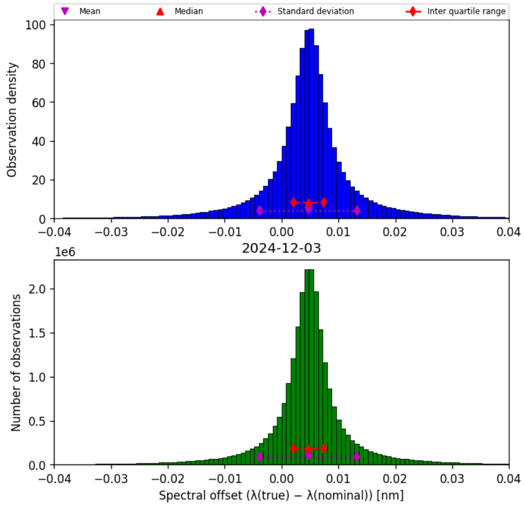
Figure 45: Histogram of “Spectral offset ( \lambda_{\text{true}} - \lambda_{\text{nominal}} )” for 2024-12-02 to 2024-12-04
