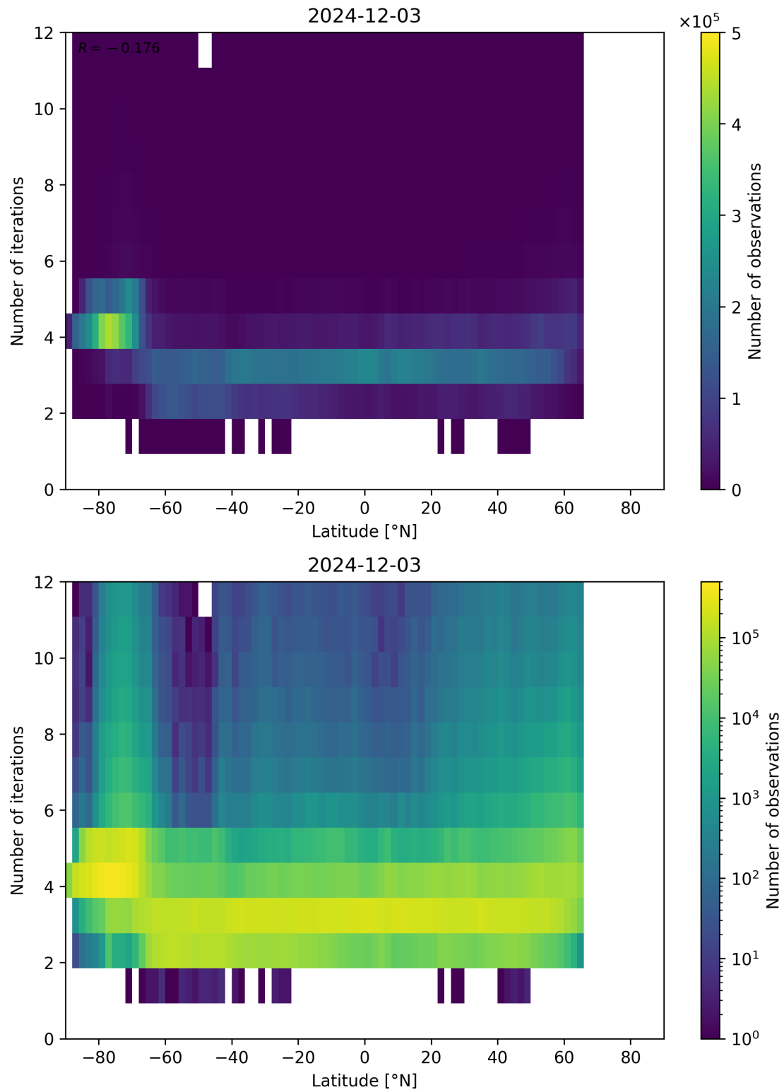
Figure 93: Scatter density plot of “Latitude” against “Number of iterations” for 2024-12-02 to 2024-12-04.
