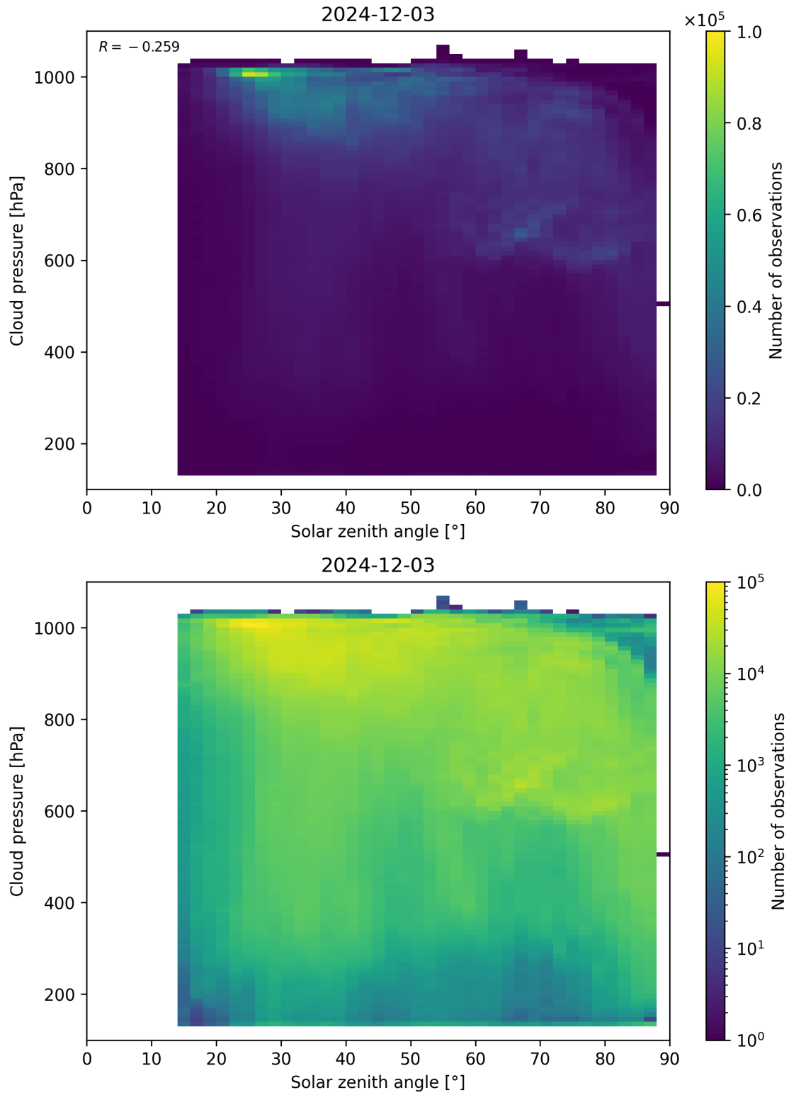
Figure 111: Scatter density plot of “Solar zenith angle” against “Cloud pressure” for 2024-12-02 to 2024-12-04.
