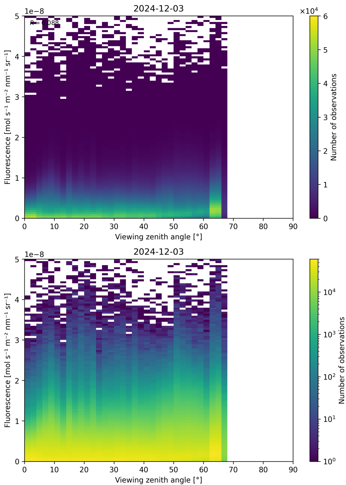
Figure 122: Scatter density plot of “Viewing zenith angle” against “Fluorescence” for 2024-12-02 to 2024-12-04.
