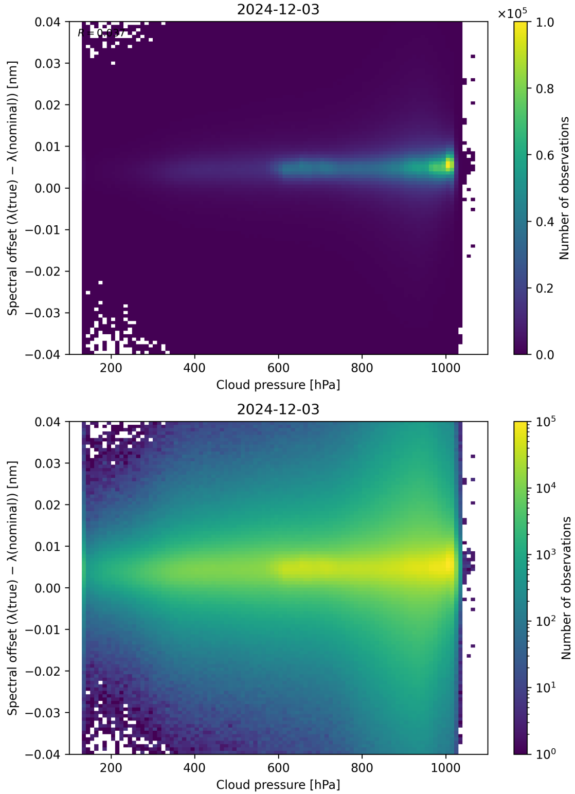
Figure 84: Scatter density plot of “Cloud pressure” against “Spectral offset ( \lambda_{\text{true}} - \lambda_{\text{nominal}} )” for 2024-12-02 to 2024-12-04.
