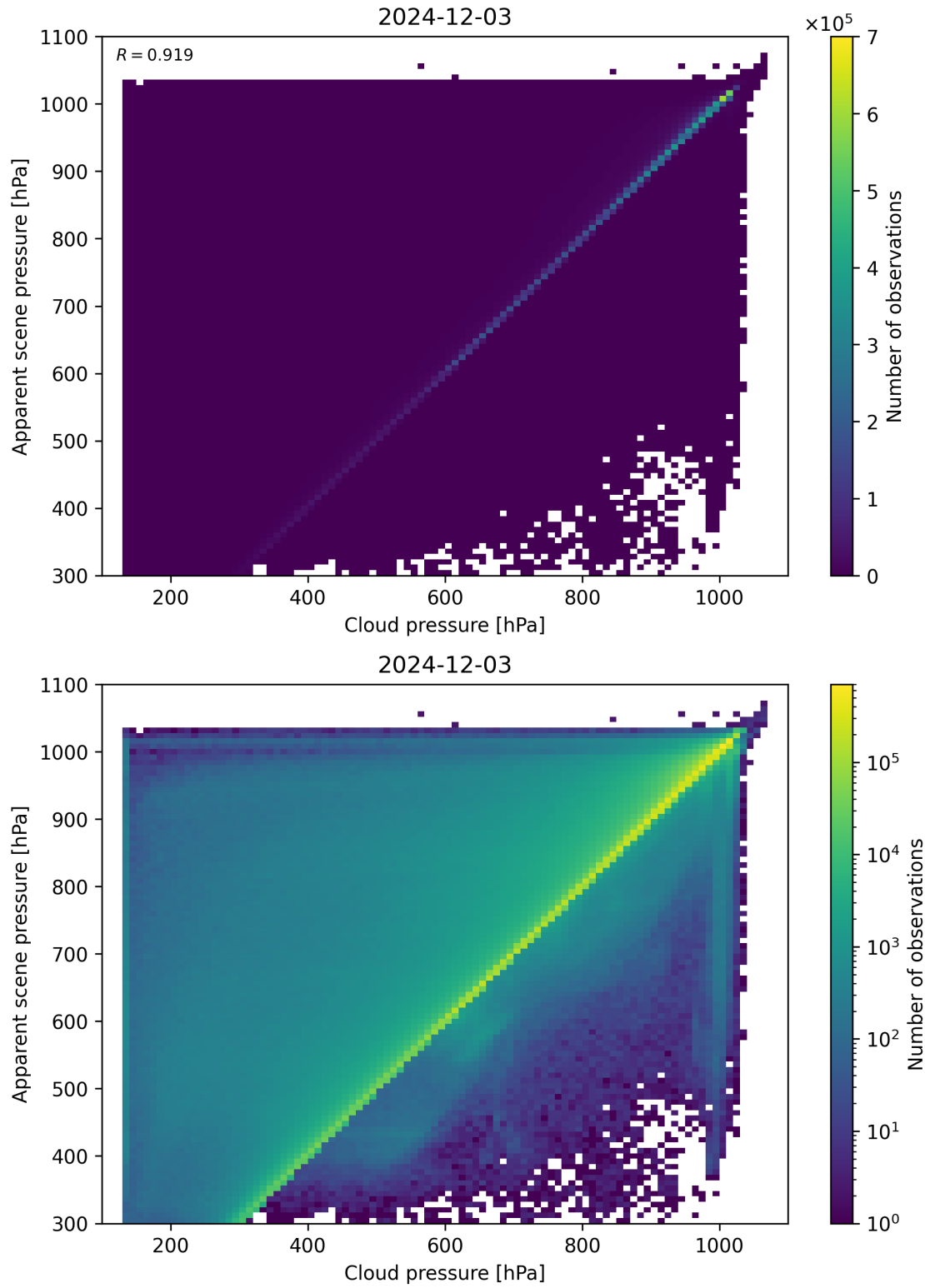
Figure 77: Scatter density plot of “Cloud pressure” against “Apparent scene pressure” for 2024-12-02 to 2024-12-04.
