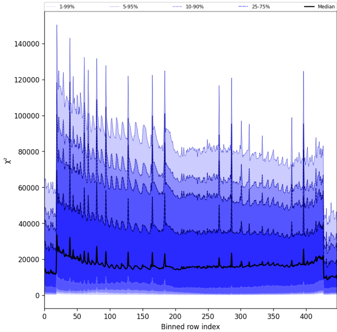
Figure 55: Along track statistics of “ \chi^2 ” for 2024-12-02 to 2024-12-04
