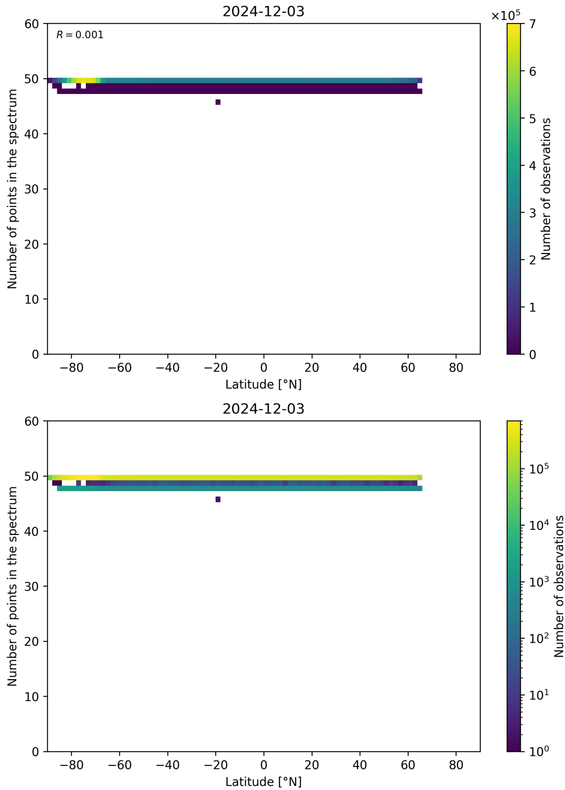
Figure 94: Scatter density plot of “Latitude” against “Number of points in the spectrum” for 2024-12-02 to 2024-12-04.
