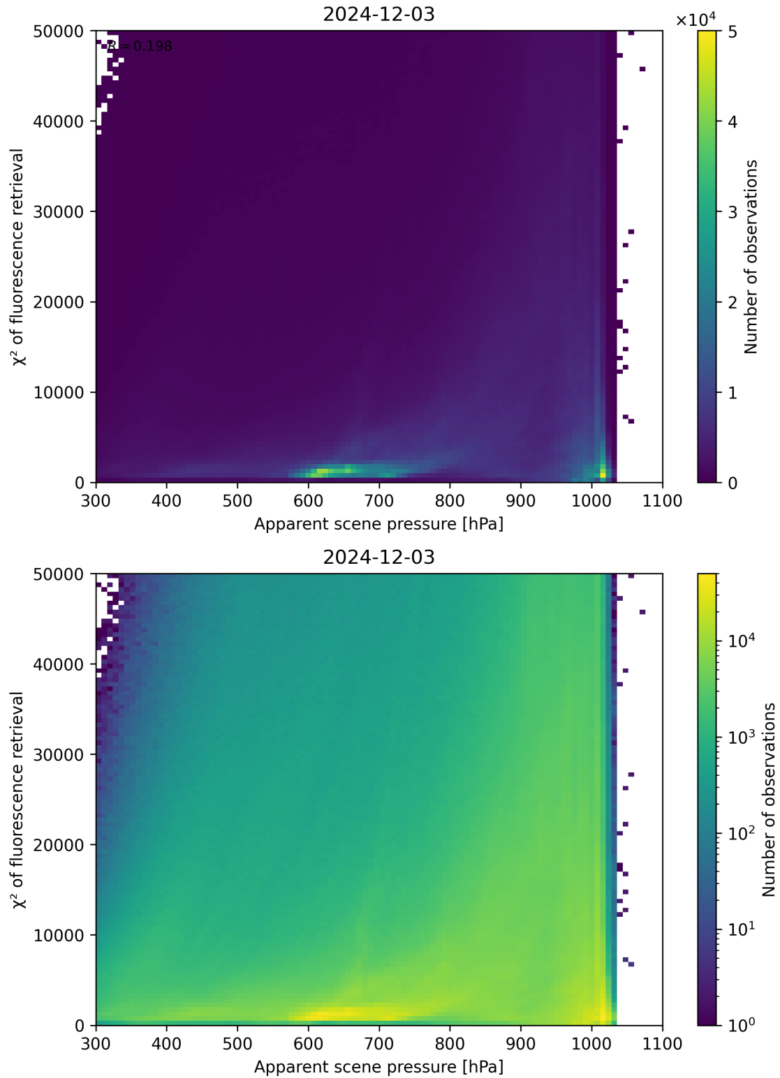
Figure 63: Scatter density plot of “Apparent scene pressure” against “ \chi^2 of fluorescence retrieval” for 2024-12-02 to 2024-12-04.
