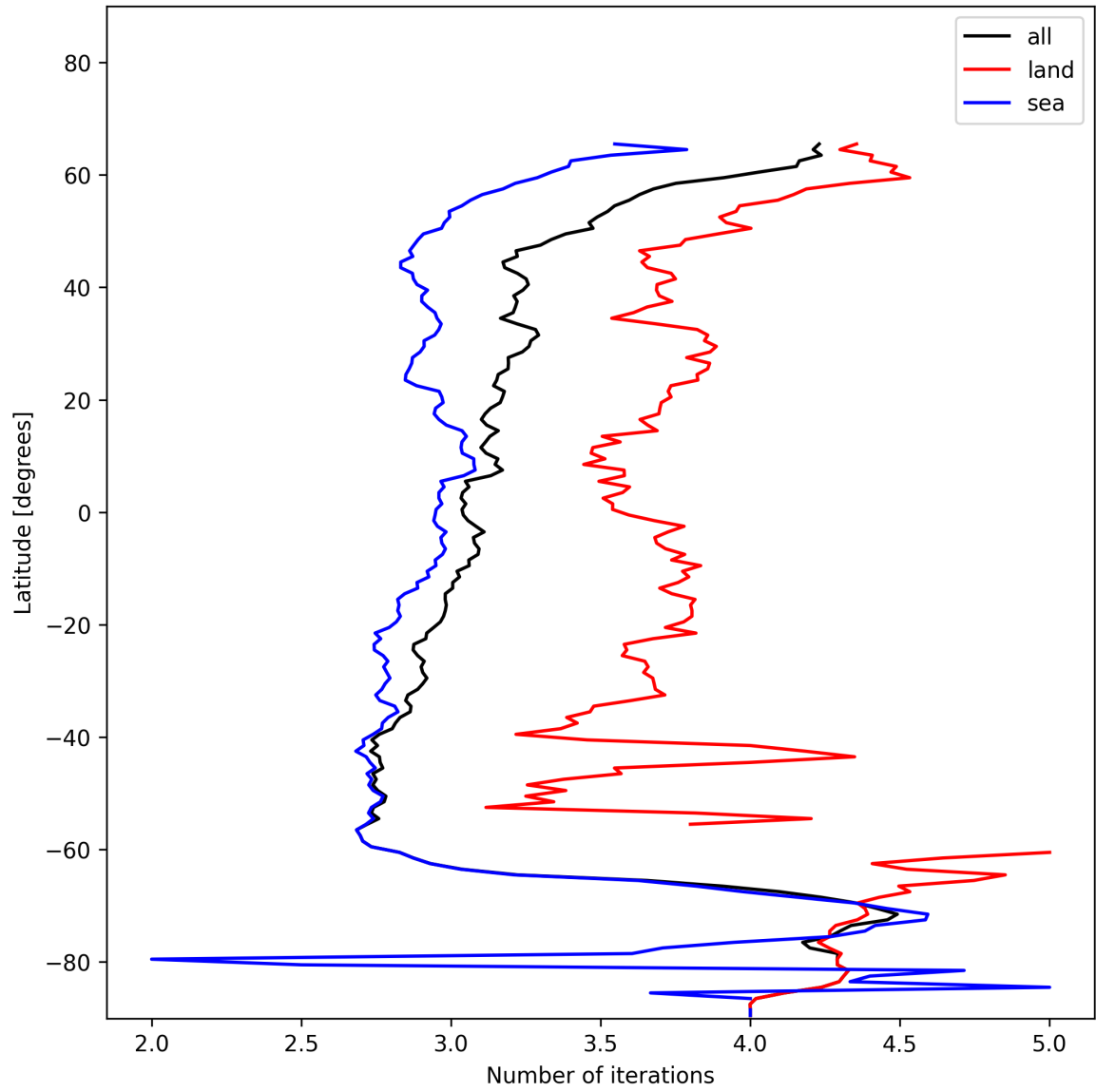
Figure 22: Zonal average of “Number of iterations” for 2024-12-02 to 2024-12-04.
