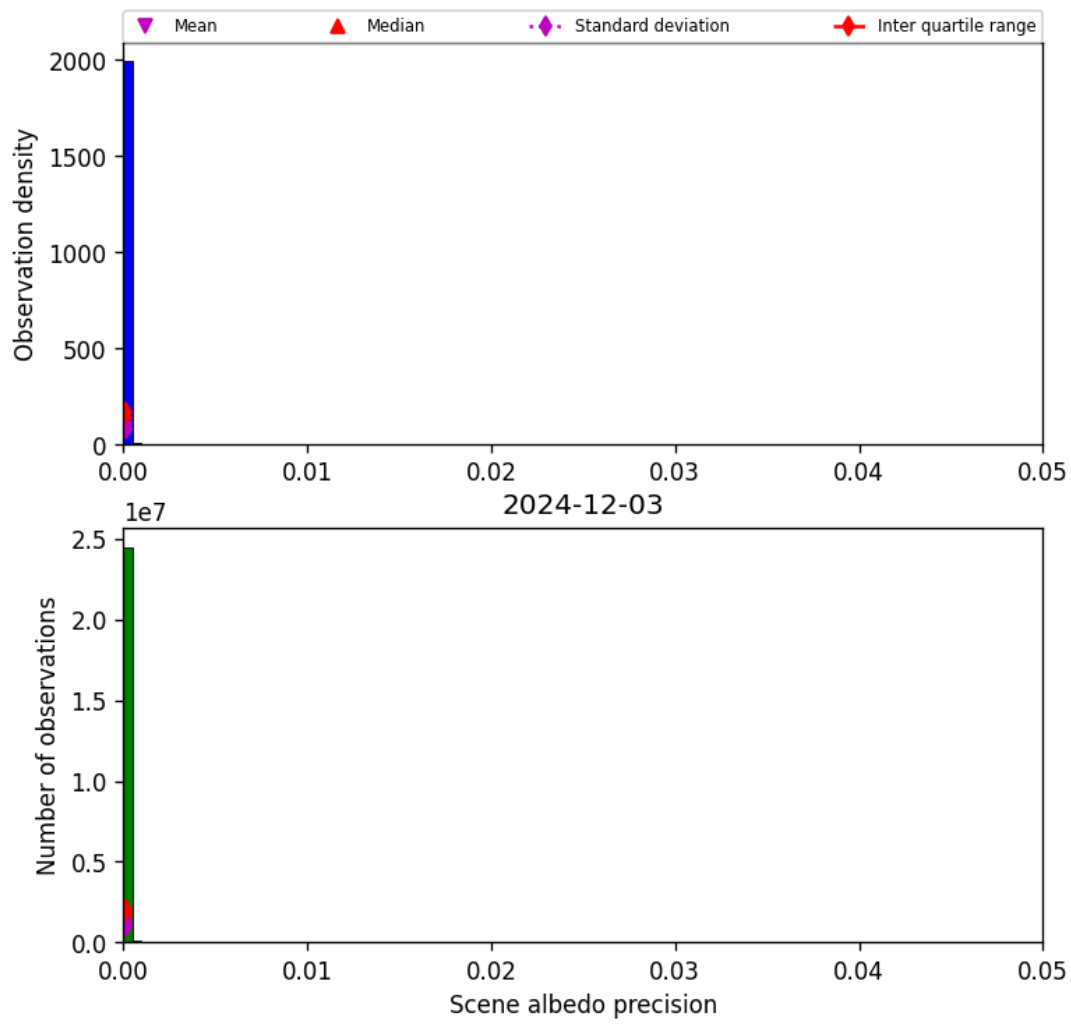
Figure 35: Histogram of “Scene albedo precision” for 2024-12-02 to 2024-12-04
