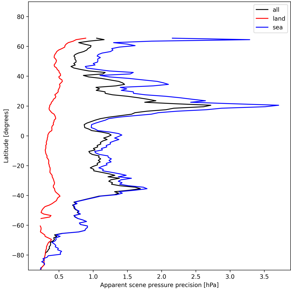
Figure 20: Zonal average of “Apparent scene pressure precision” for 2024-12-02 to 2024-12-04.
