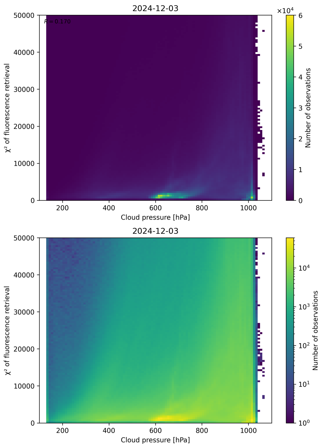
Figure 78: Scatter density plot of “Cloud pressure” against “ \chi^2 of fluorescence retrieval” for 2024-12-02 to 2024-12-04.
