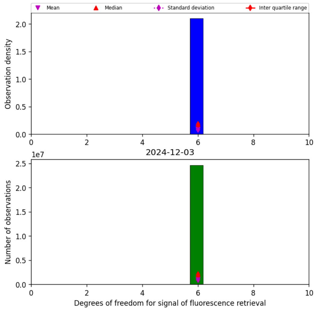
Figure 43: Histogram of “Degrees of freedom for signal of fluorescence retrieval” for 2024-12-02 to 2024-12-04
