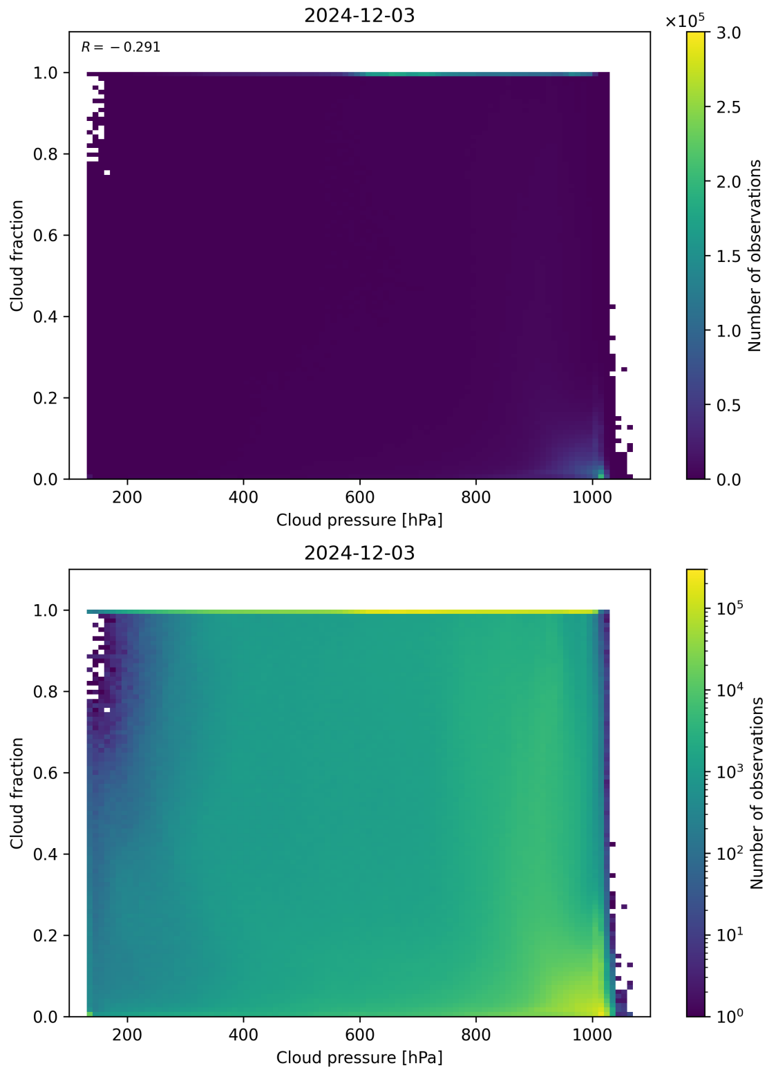
Figure 79: Scatter density plot of “Cloud pressure” against “Cloud fraction” for 2024-12-02 to 2024-12-04.
