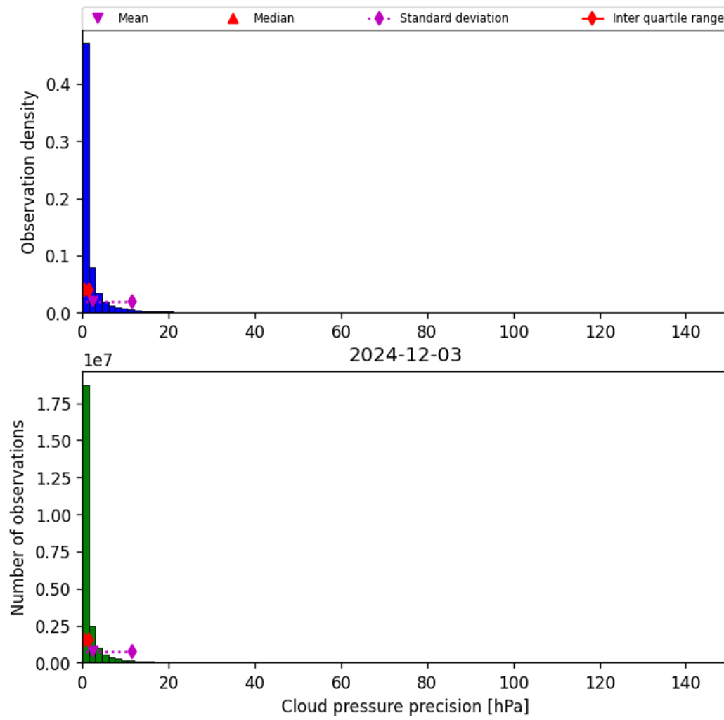
Figure 31: Histogram of “Cloud pressure precision” for 2024-12-02 to 2024-12-04
