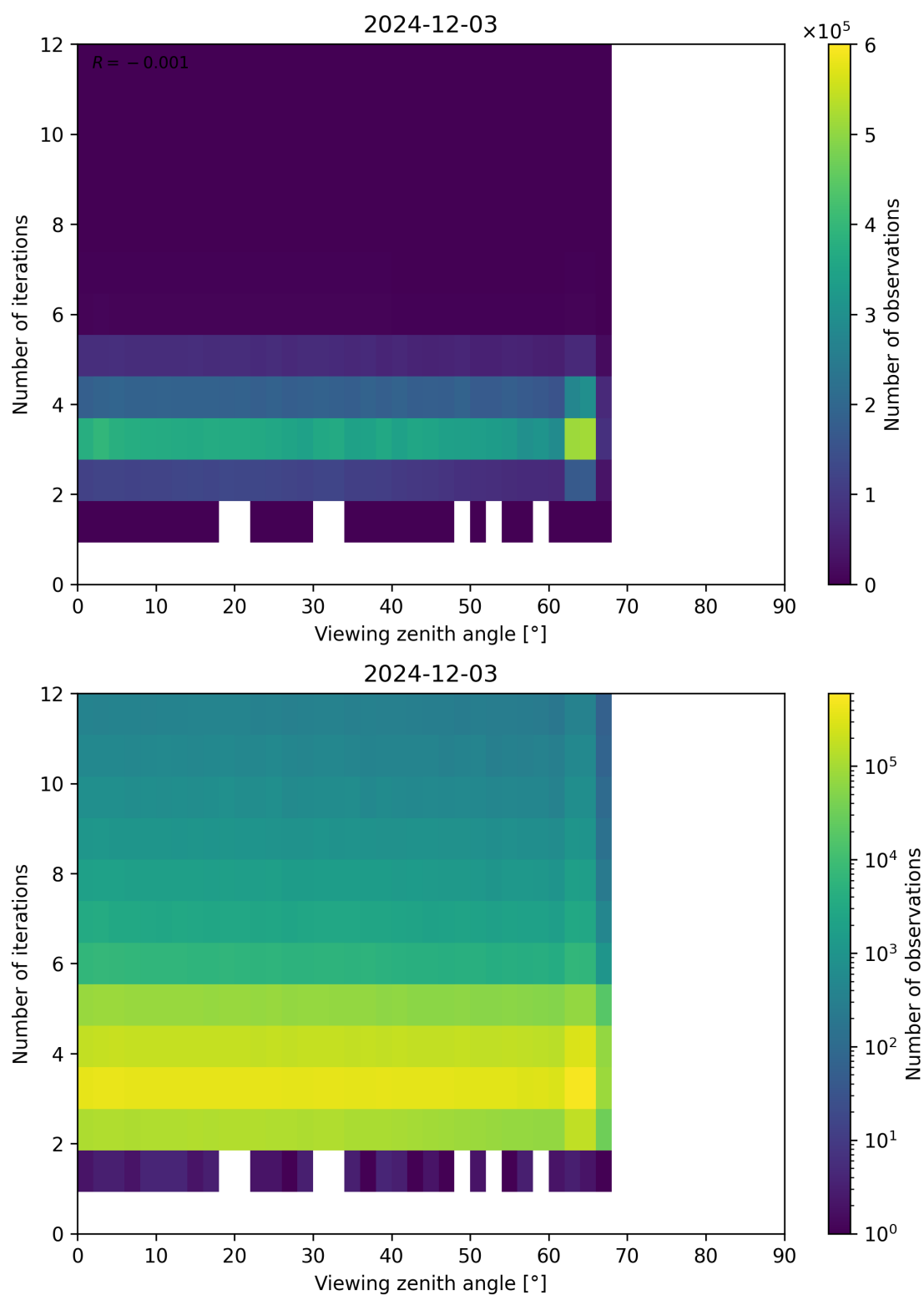
Figure 124: Scatter density plot of “Viewing zenith angle” against “Number of iterations” for 2024-12-02 to 2024-12-04.
