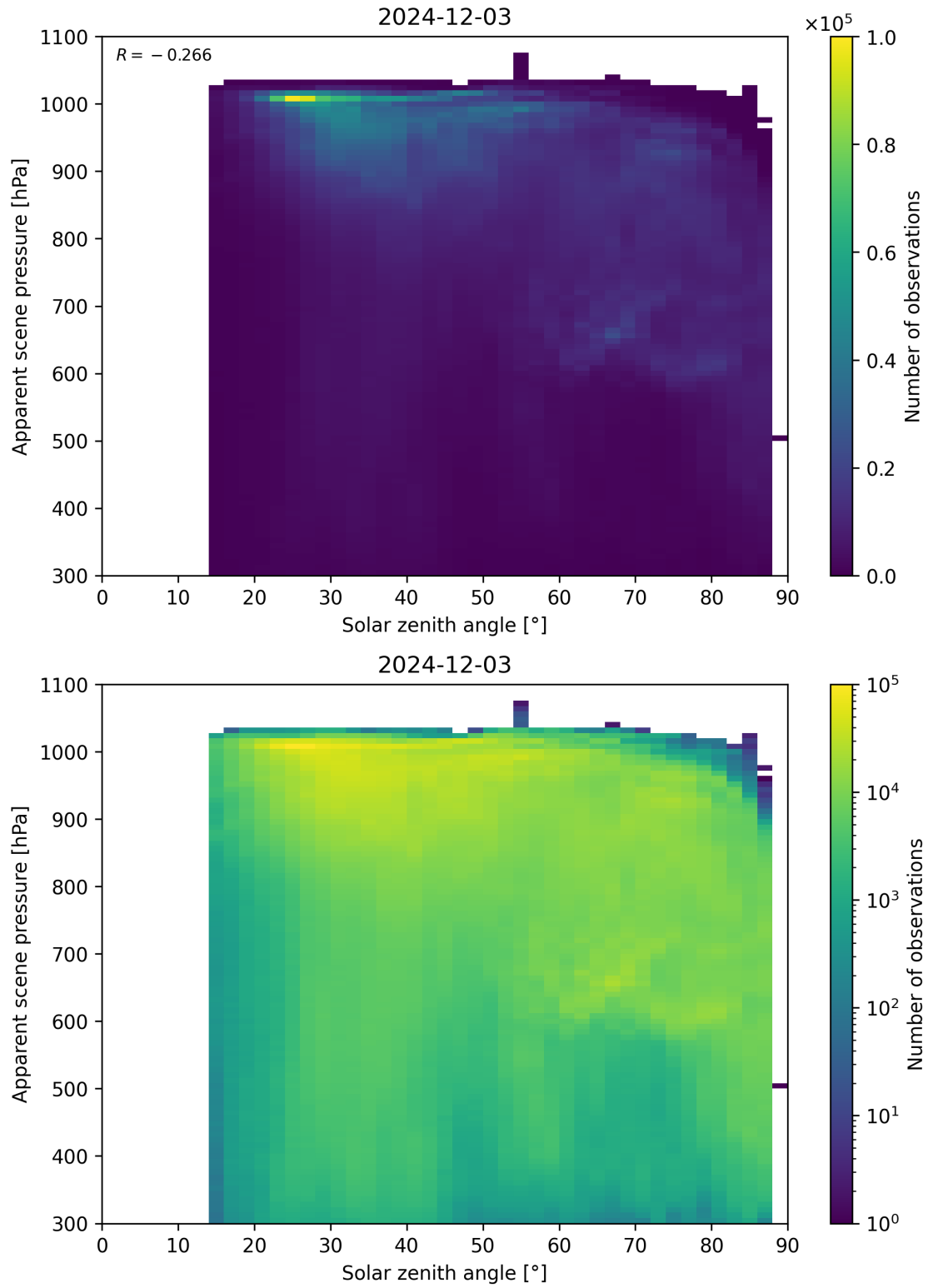
Figure 108: Scatter density plot of “Solar zenith angle” against “Apparent scene pressure” for 2024-12-02 to 2024-12-04.
