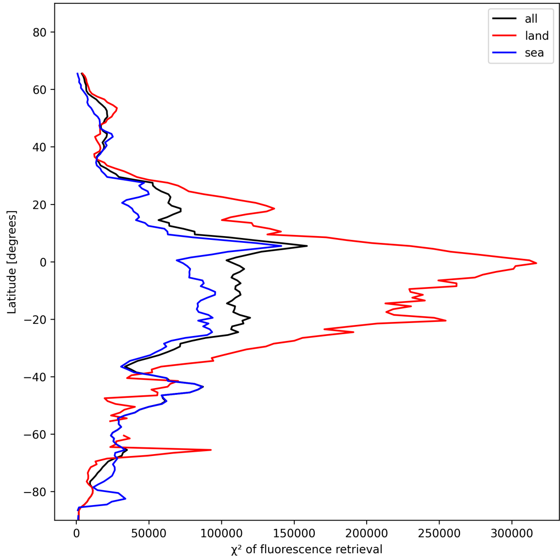
Figure 25: Zonal average of “ \chi^2 of fluorescence retrieval” for 2024-12-02 to 2024-12-04.
