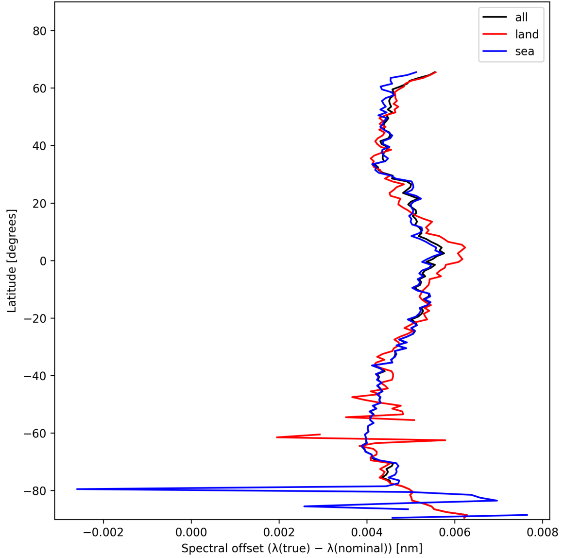
Figure 28: Zonal average of “Spectral offset ( \lambda_{\text{true}} - \lambda_{\text{nominal}} )” for 2024-12-02 to 2024-12-04.
