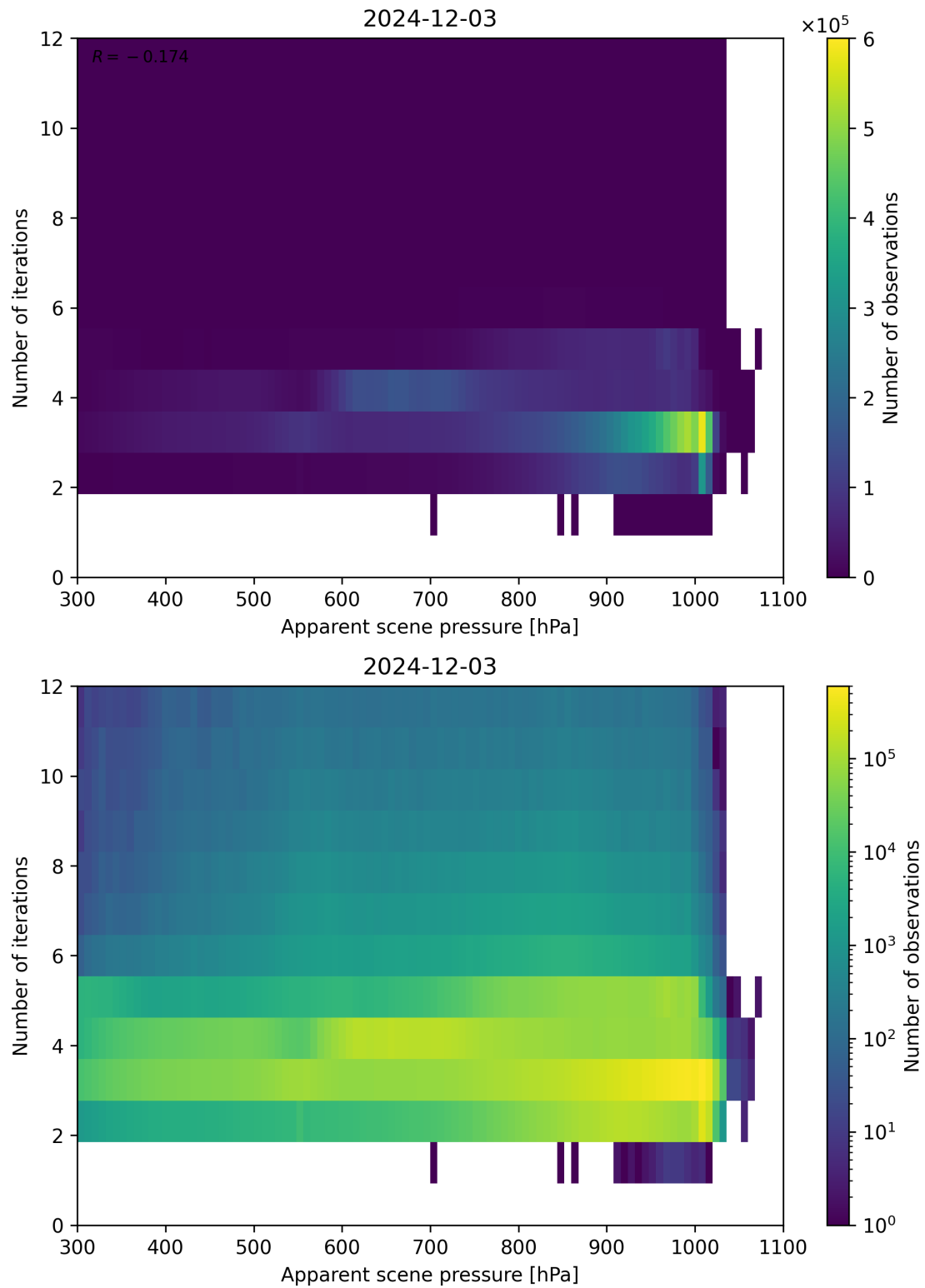
Figure 65: Scatter density plot of “Apparent scene pressure” against “Number of iterations” for 2024-12-02 to 2024-12-04.
