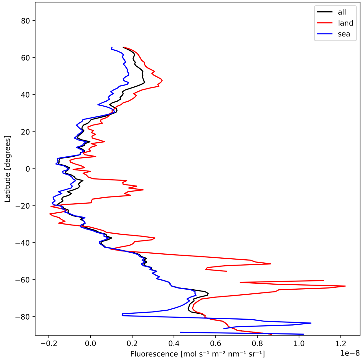
Figure 23: Zonal average of “Fluorescence” for 2024-12-02 to 2024-12-04.
