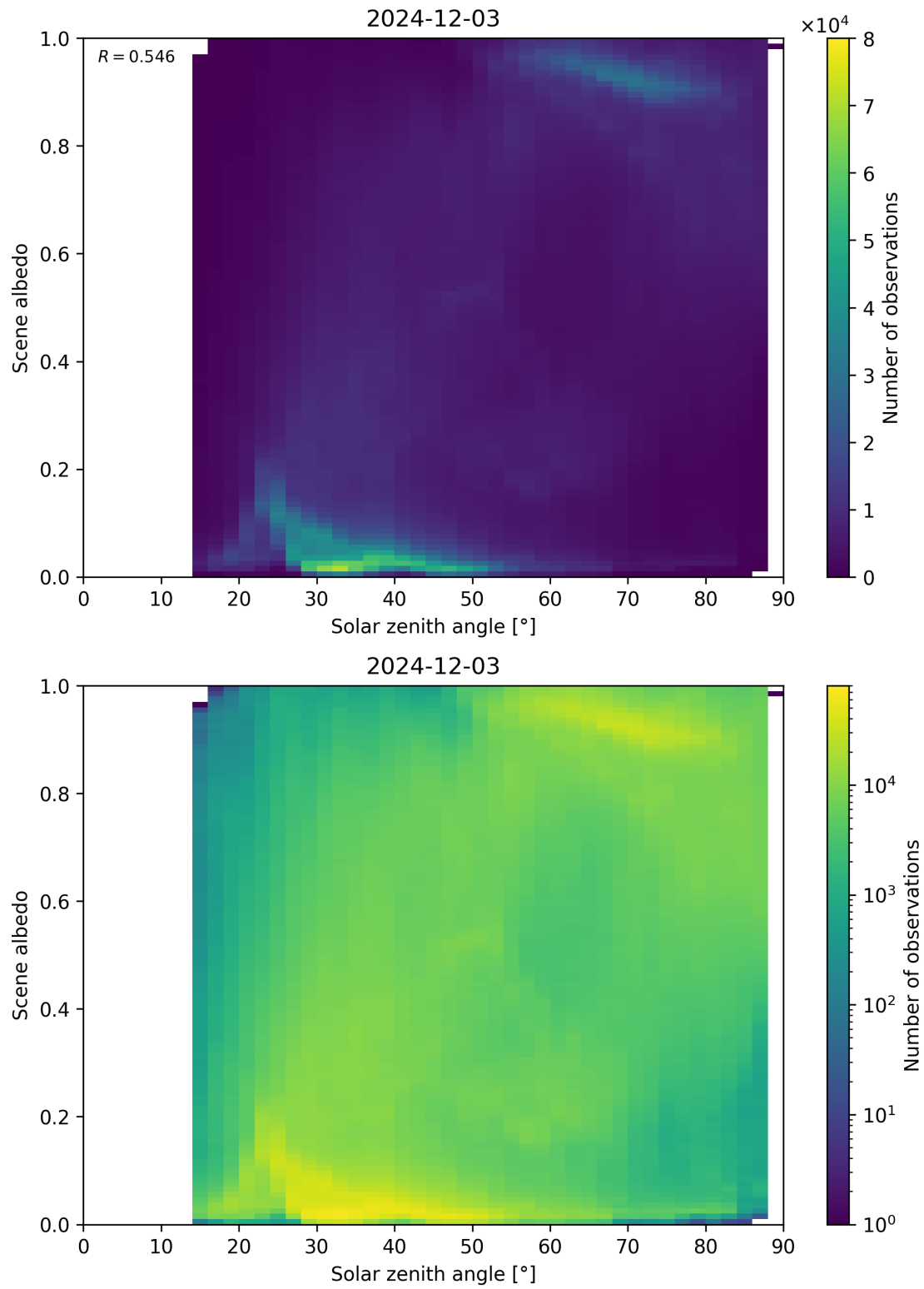
Figure 116: Scatter density plot of “Solar zenith angle” against “Scene albedo” for 2024-12-02 to 2024-12-04.
