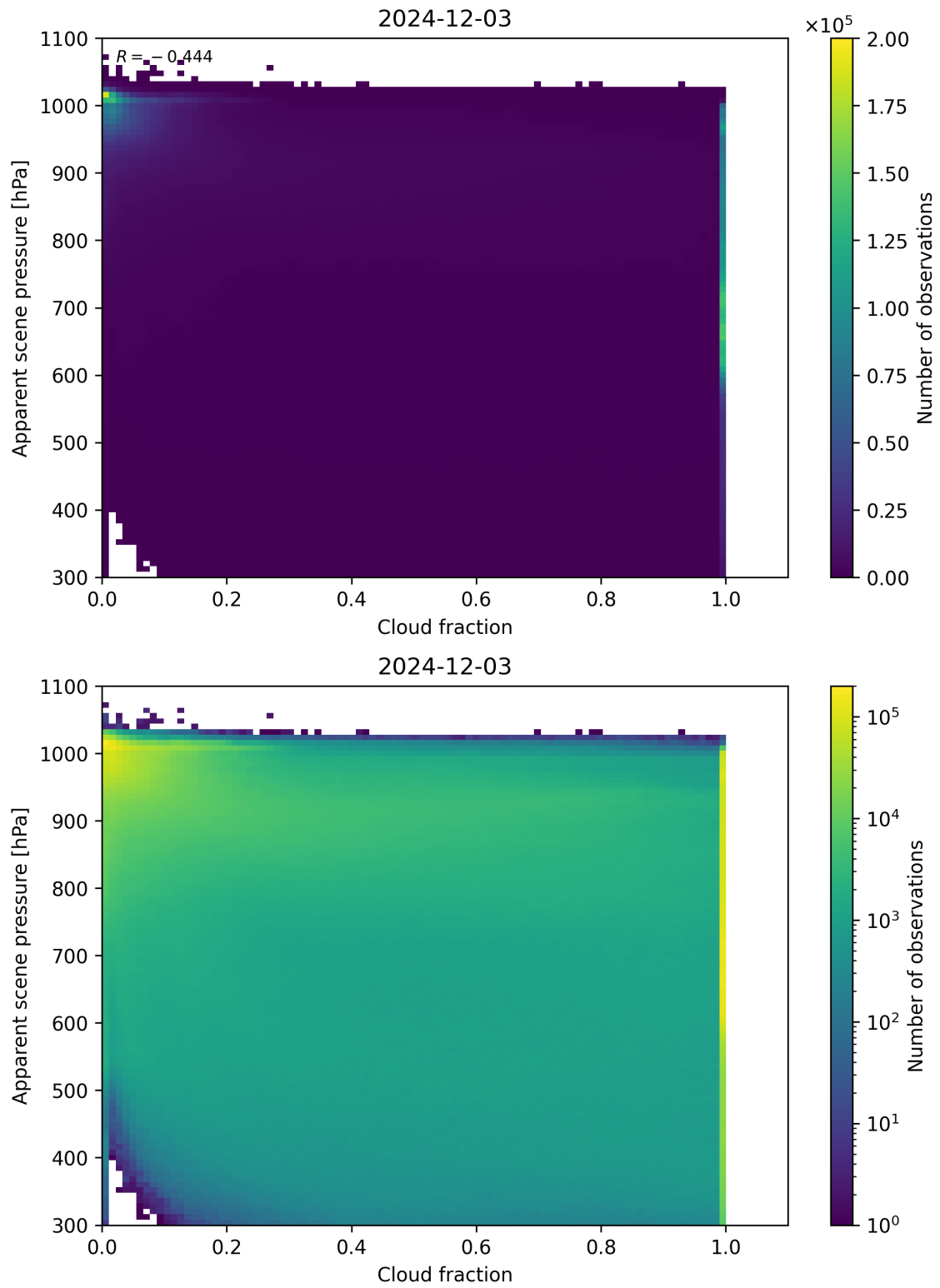
Figure 70: Scatter density plot of “Cloud fraction” against “Apparent scene pressure” for 2024-12-02 to 2024-12-04.
