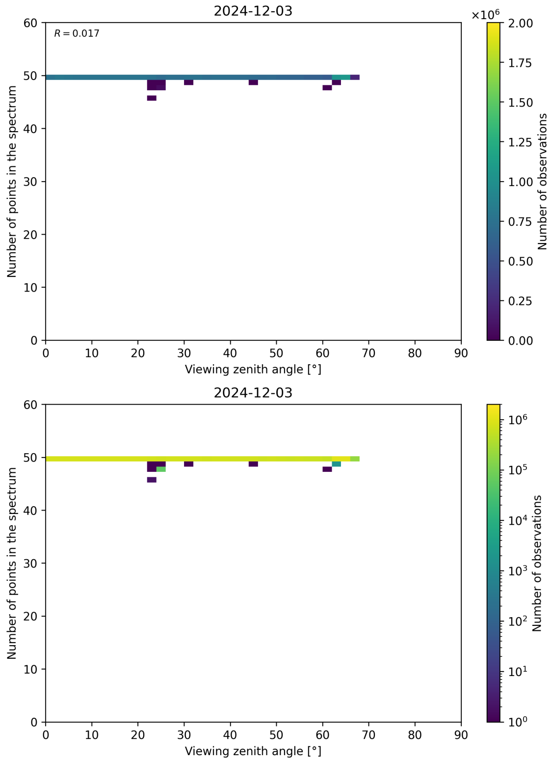
Figure 125: Scatter density plot of “Viewing zenith angle” against “Number of points in the spectrum” for 2024-12-02 to 2024-12-04.
