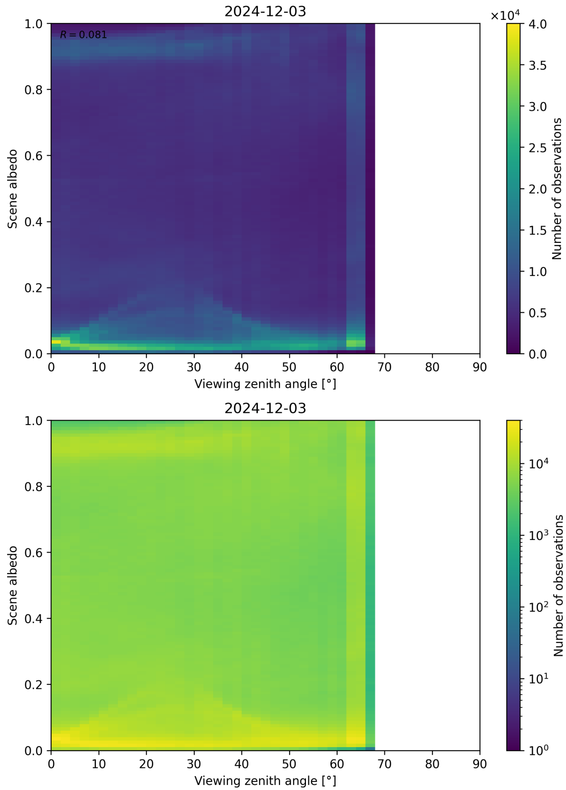
Figure 126: Scatter density plot of “Viewing zenith angle” against “Scene albedo” for 2024-12-02 to 2024-12-04.
