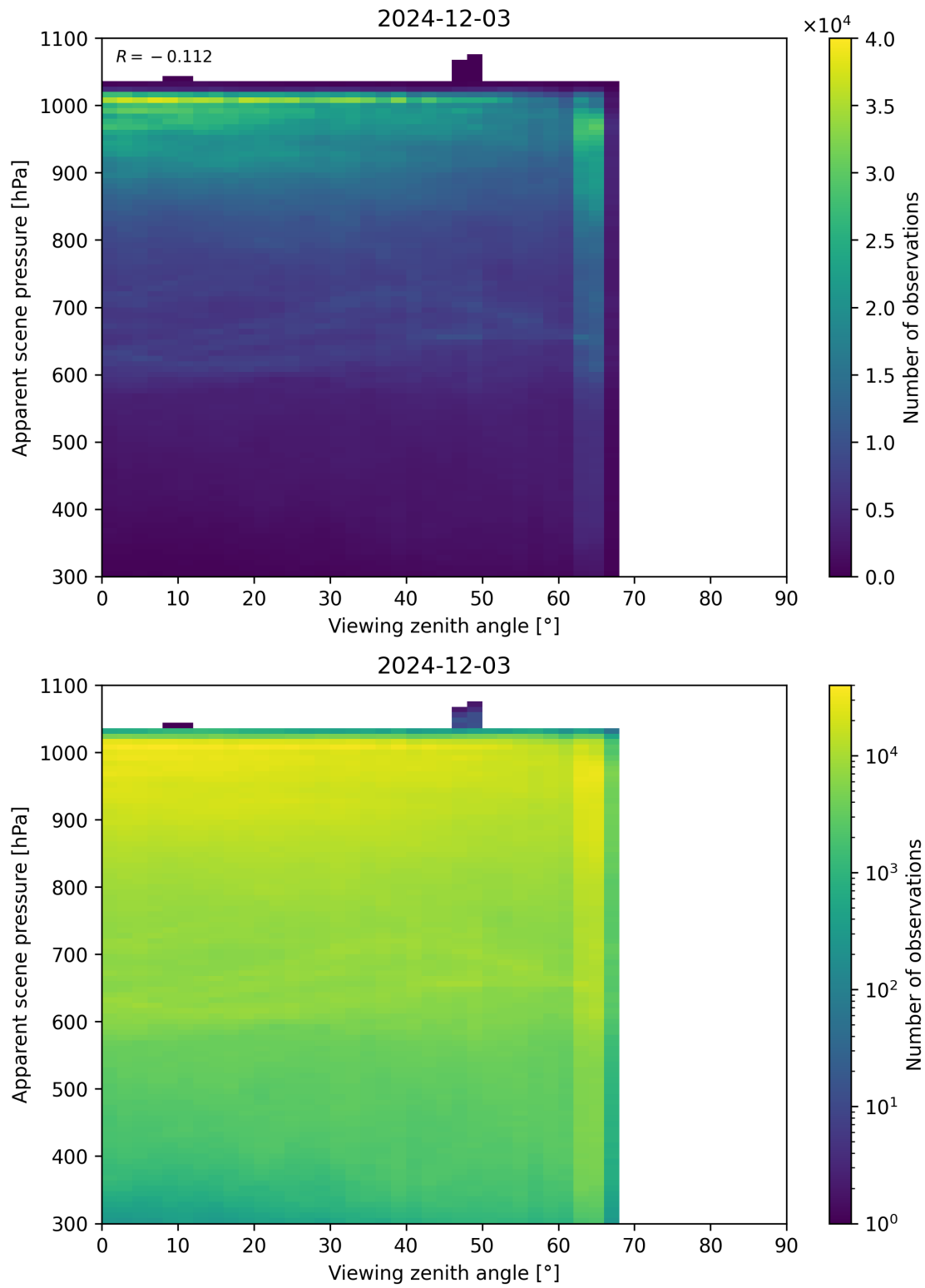
Figure 118: Scatter density plot of “Viewing zenith angle” against “Apparent scene pressure” for 2024-12-02 to 2024-12-04.
