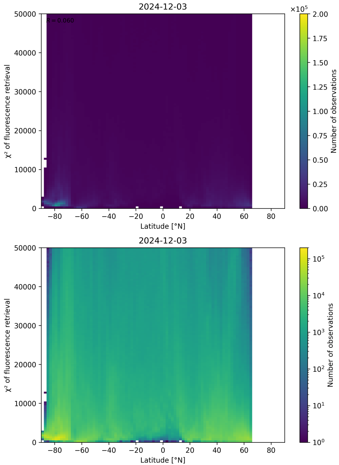
Figure 89: Scatter density plot of “Latitude” against “ \chi^2 of fluorescence retrieval” for 2024-12-02 to 2024-12-04.
