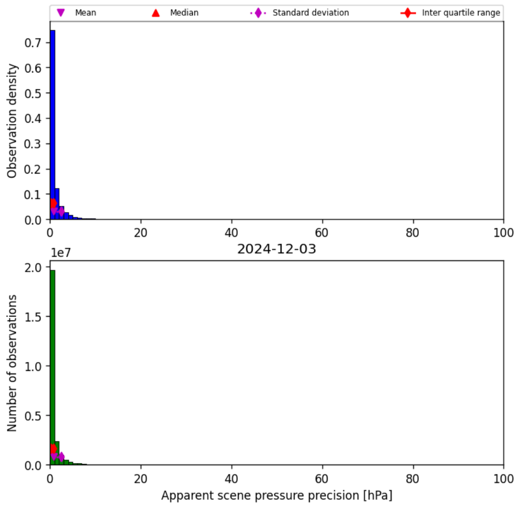
Figure 37: Histogram of “Apparent scene pressure precision” for 2024-12-02 to 2024-12-04
