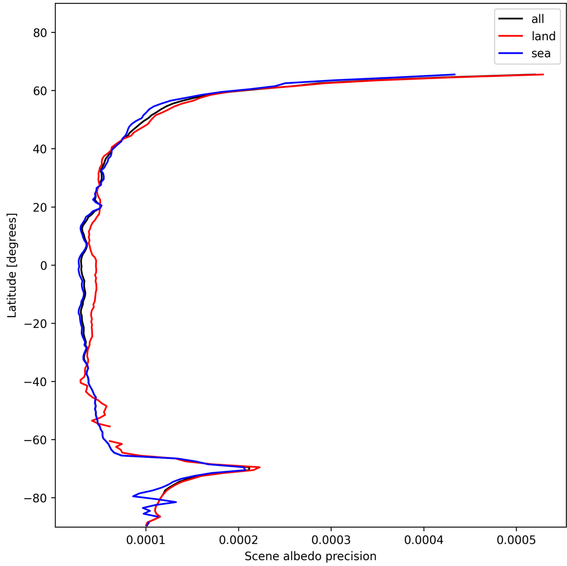
Figure 18: Zonal average of “Scene albedo precision” for 2024-12-02 to 2024-12-04.
