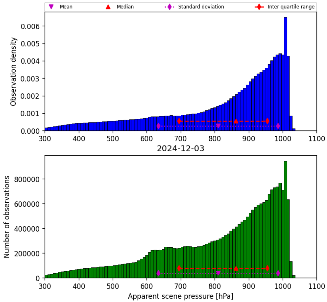
Figure 36: Histogram of “Apparent scene pressure” for 2024-12-02 to 2024-12-04
