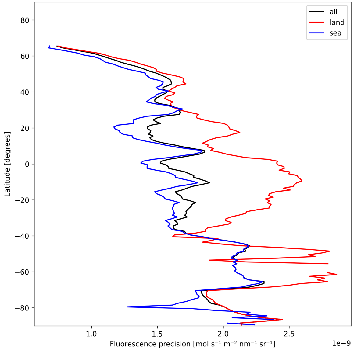
Figure 24: Zonal average of “Fluorescence precision” for 2024-12-02 to 2024-12-04.
