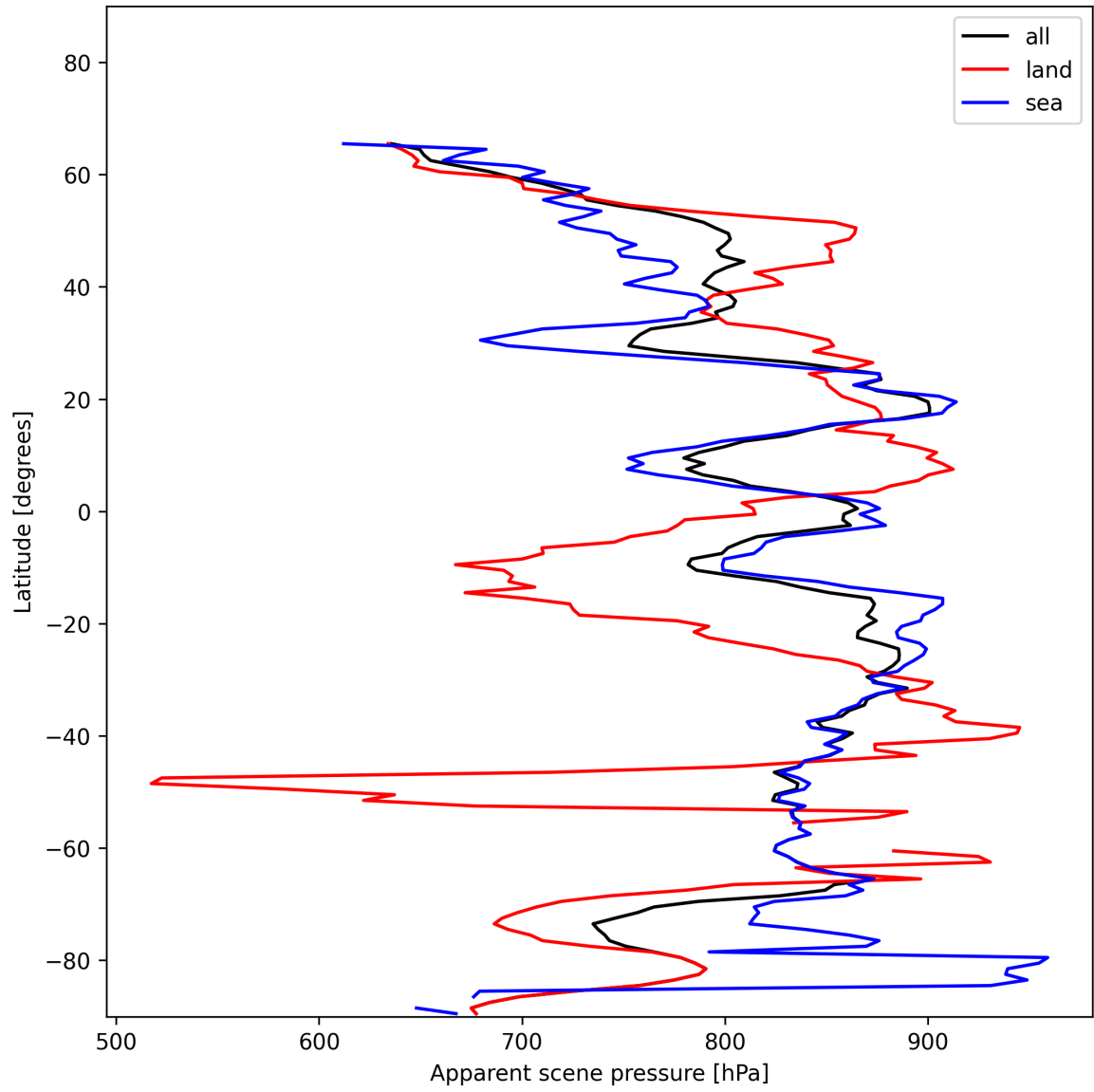
Figure 19: Zonal average of “Apparent scene pressure” for 2024-12-02 to 2024-12-04.
