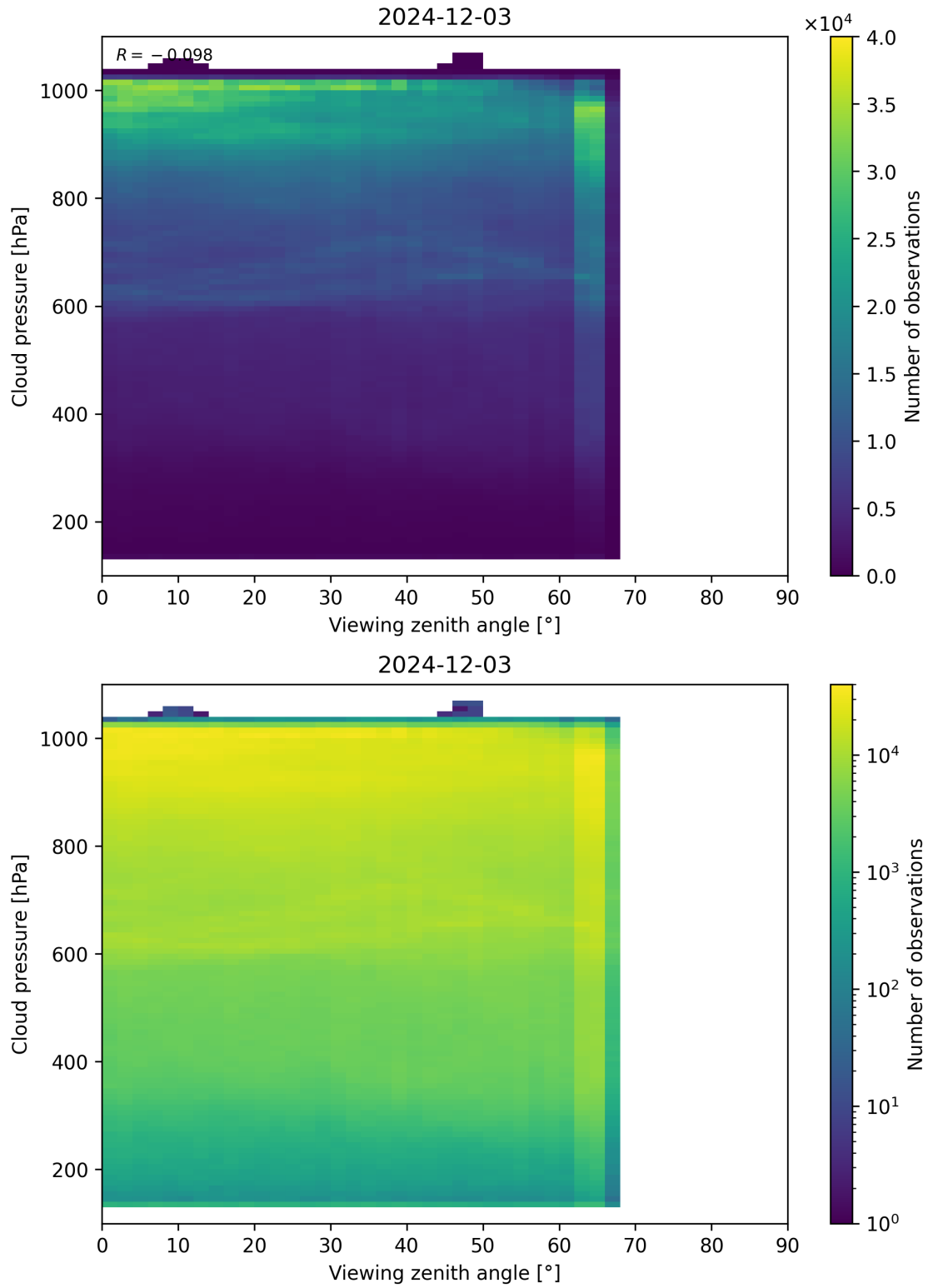
Figure 121: Scatter density plot of “Viewing zenith angle” against “Cloud pressure” for 2024-12-02 to 2024-12-04.
