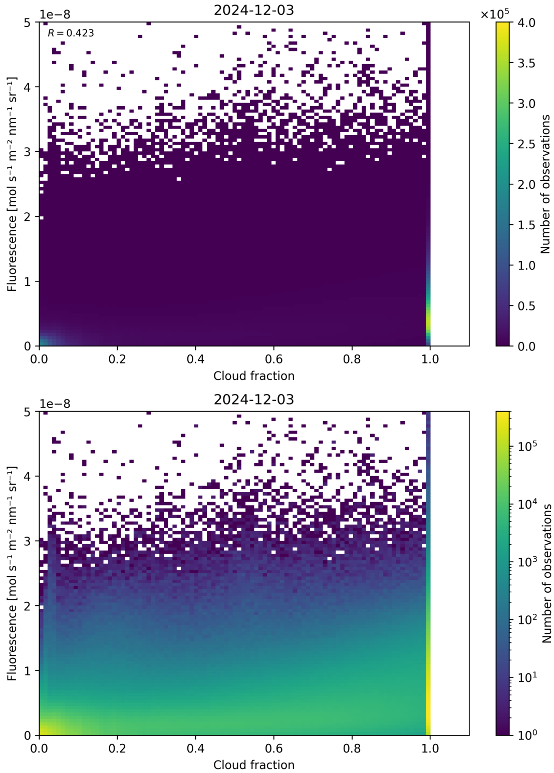
Figure 72: Scatter density plot of “Cloud fraction” against “Fluorescence” for 2024-12-02 to 2024-12-04.
