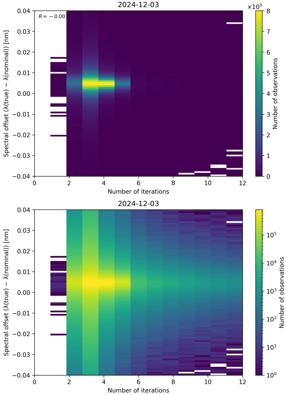
Figure 100: Scatter density plot of “Number of iterations” against “Spectral offset ( \lambda_{\text{true}} - \lambda_{\text{nominal}} )” for 2024-12-02 to 2024-12-04.
