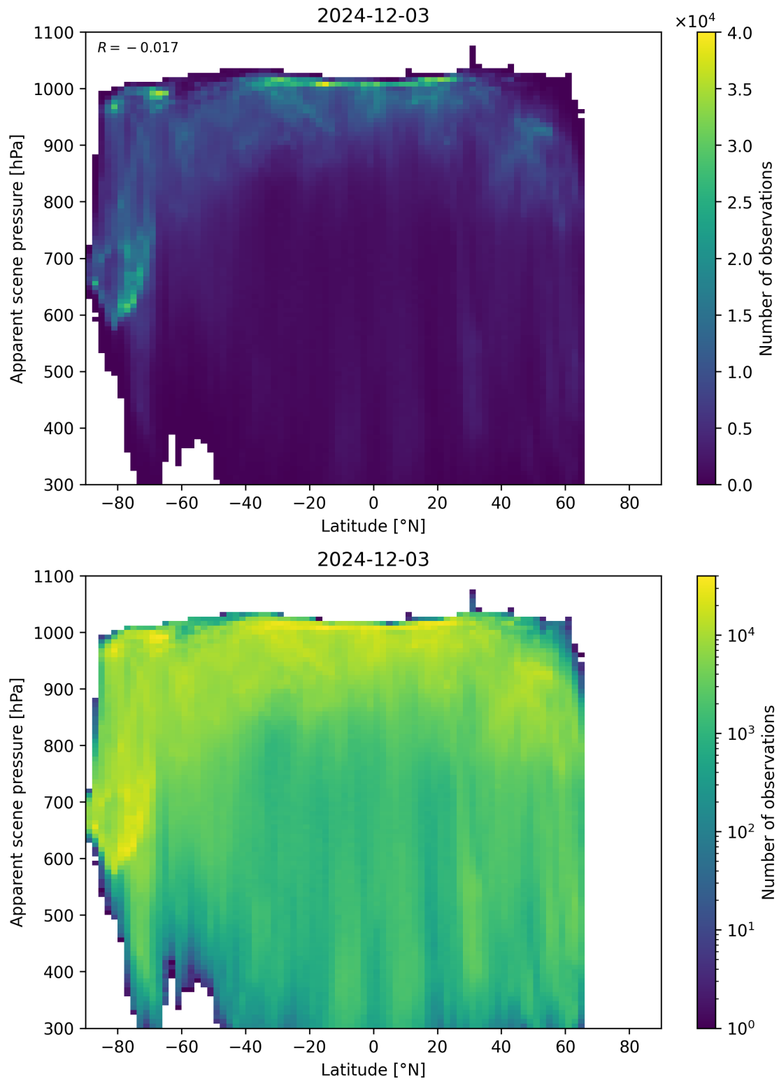
Figure 88: Scatter density plot of “Latitude” against “Apparent scene pressure” for 2024-12-02 to 2024-12-04.
