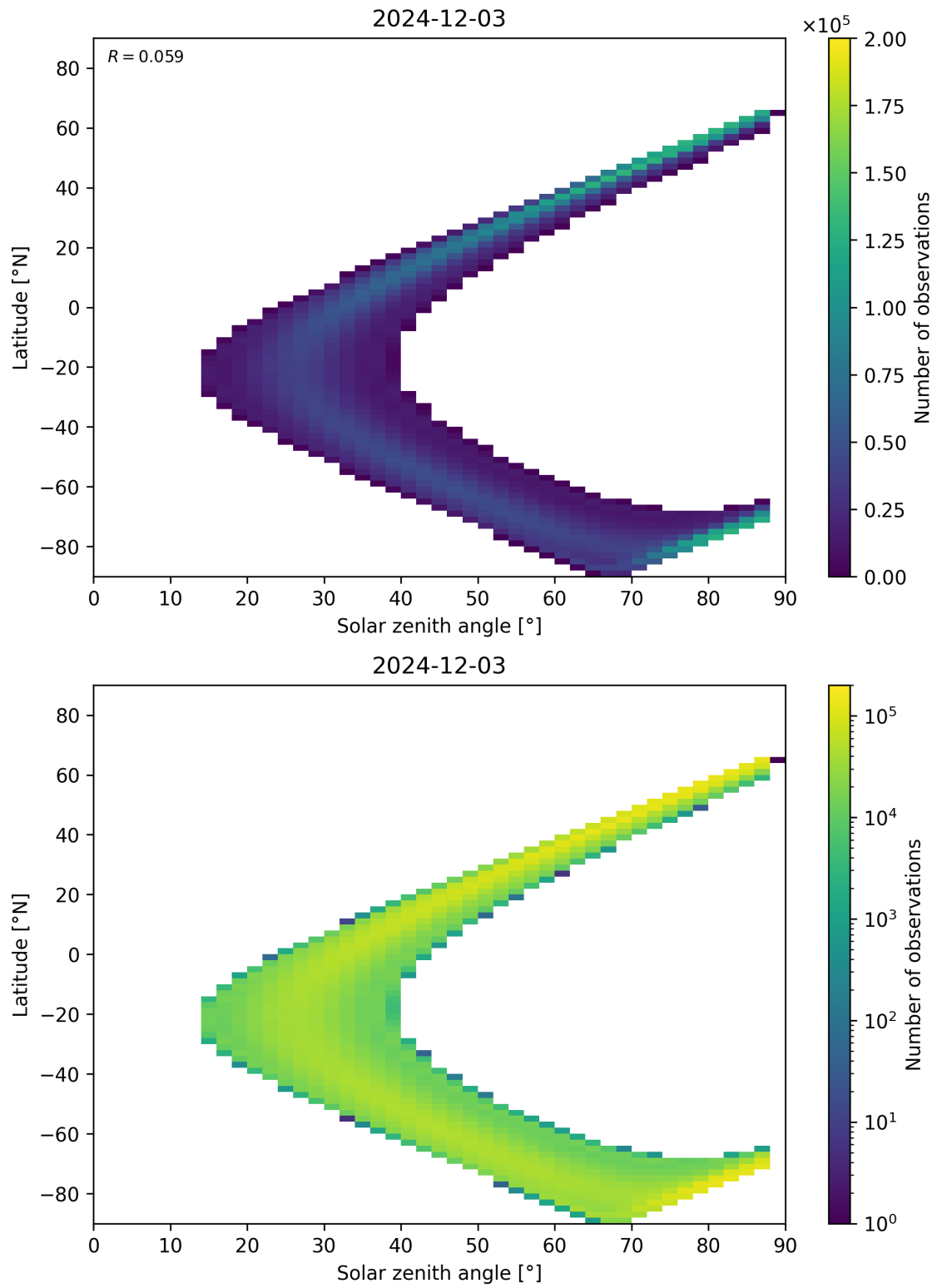
Figure 113: Scatter density plot of “Solar zenith angle” against “Latitude” for 2024-12-02 to 2024-12-04.
