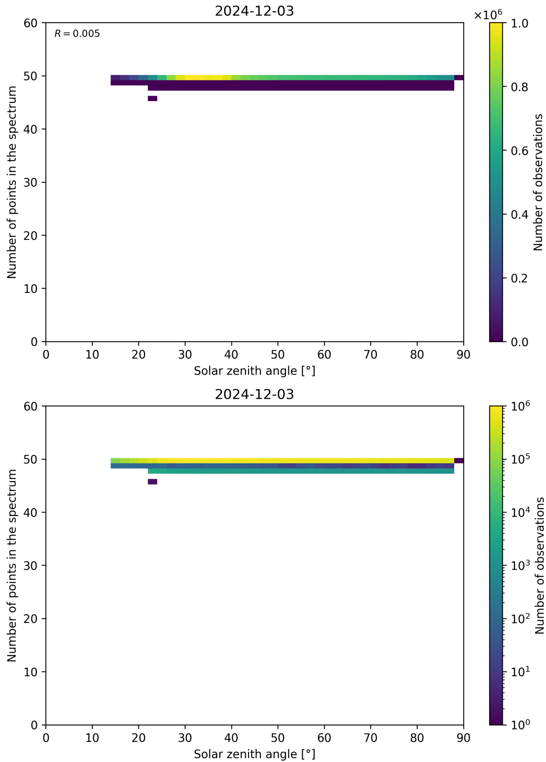
Figure 115: Scatter density plot of “Solar zenith angle” against “Number of points in the spectrum” for 2024-12-02 to 2024-12-04.
