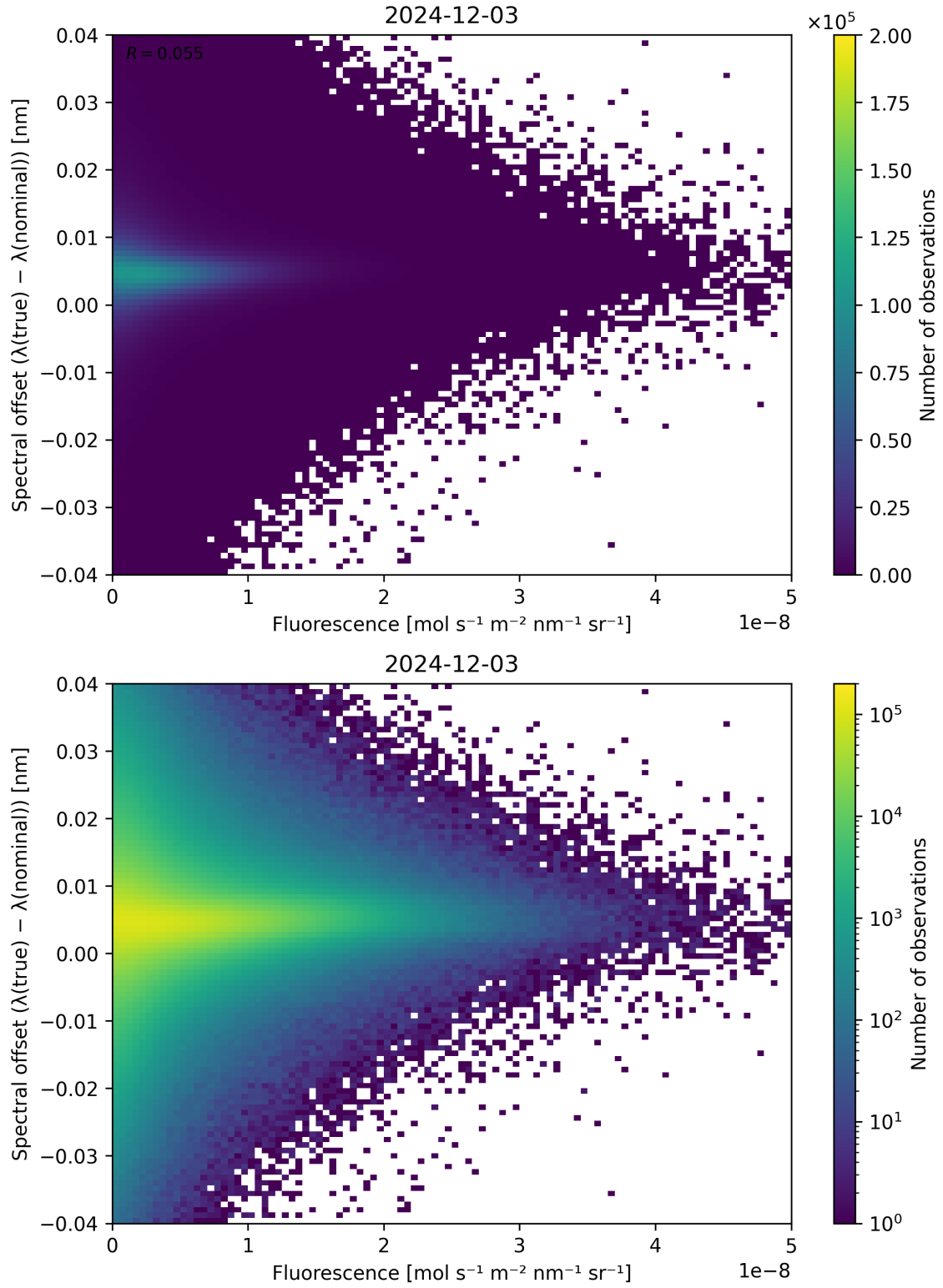
Figure 87: Scatter density plot of “Fluorescence” against “Spectral offset ( \lambda_{\text{true}} - \lambda_{\text{nominal}} )” for 2024-12-02 to 2024-12-04.
