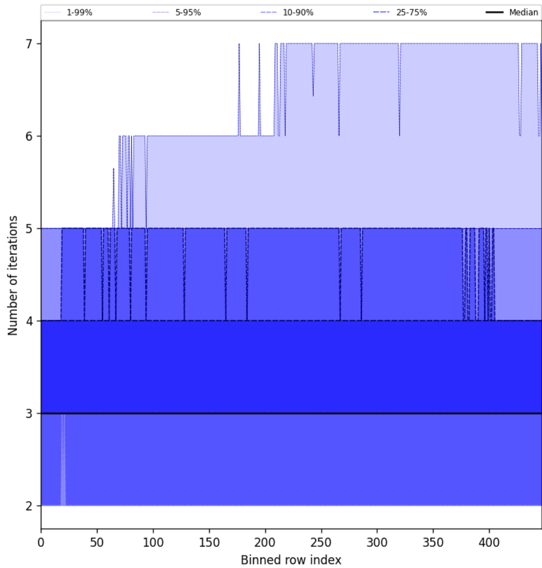
Figure 56: Along track statistics of “Number of iterations” for 2024-12-02 to 2024-12-04
