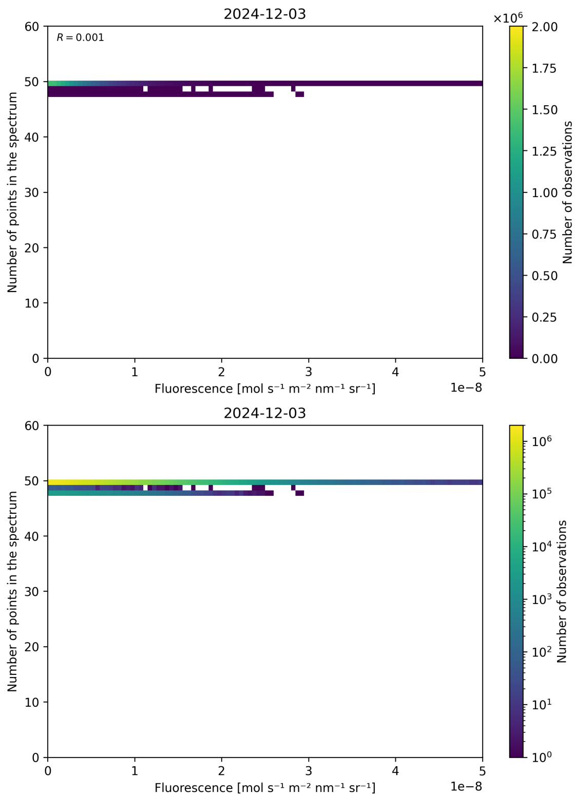
Figure 86: Scatter density plot of “Fluorescence” against “Number of points in the spectrum” for 2024-12-02 to 2024-12-04.
