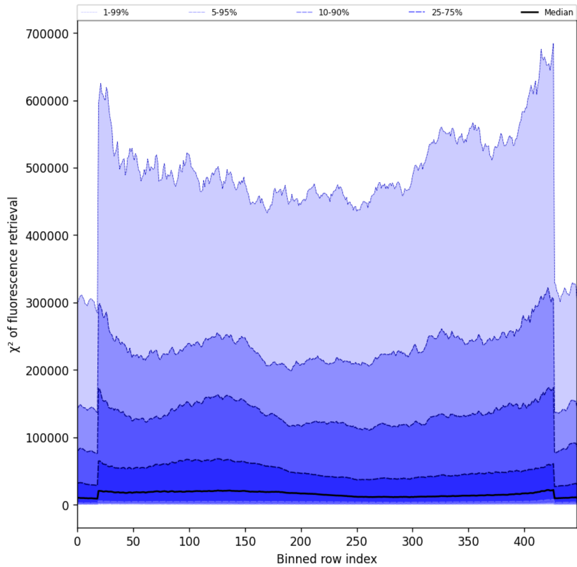
Figure 59: Along track statistics of “ \chi^2 of fluorescence retrieval” for 2024-12-02 to 2024-12-04
