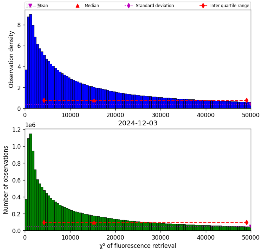
Figure 42: Histogram of “ \chi^2 of fluorescence retrieval” for 2024-12-02 to 2024-12-04
