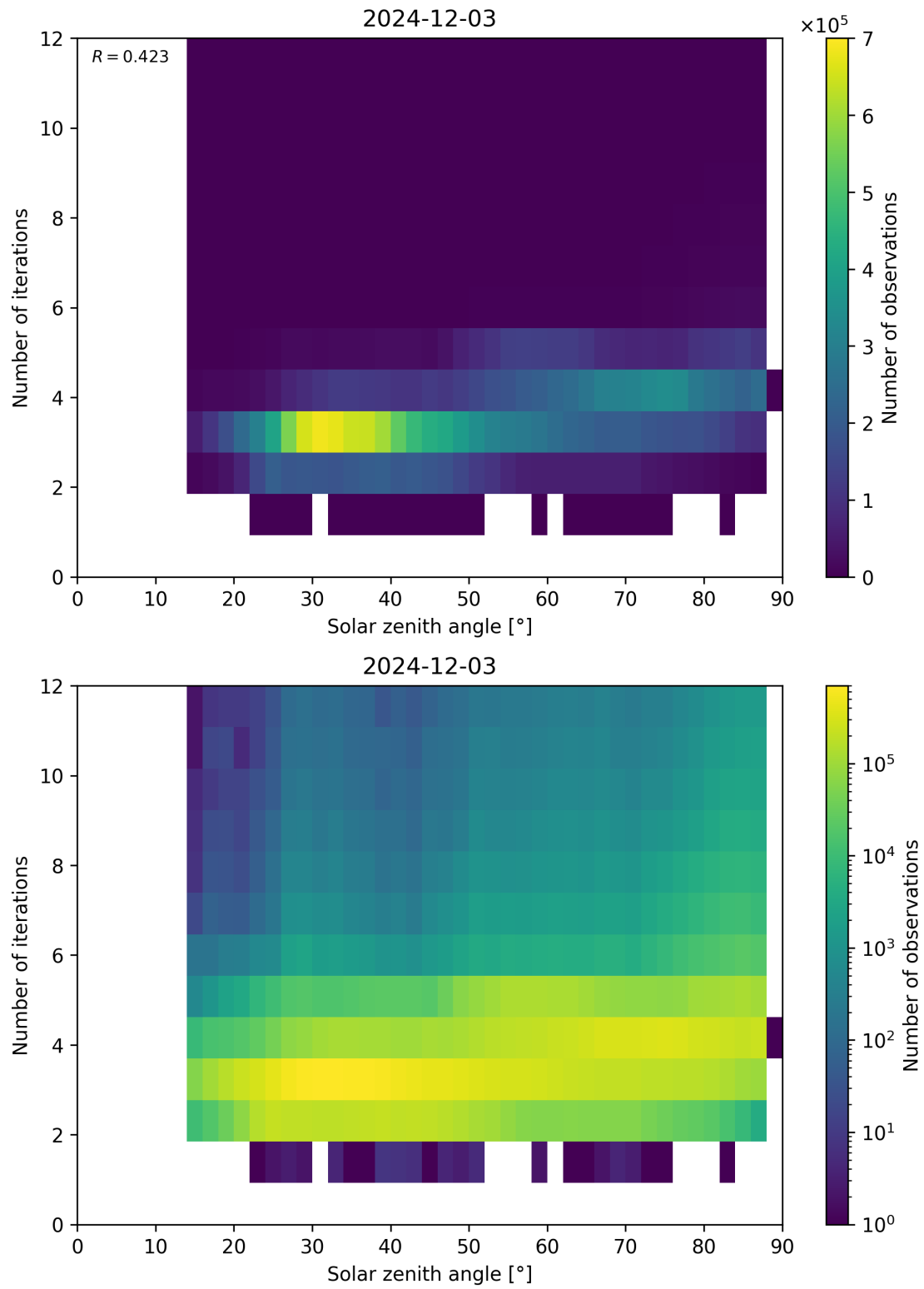
Figure 114: Scatter density plot of “Solar zenith angle” against “Number of iterations” for 2024-12-02 to 2024-12-04.
