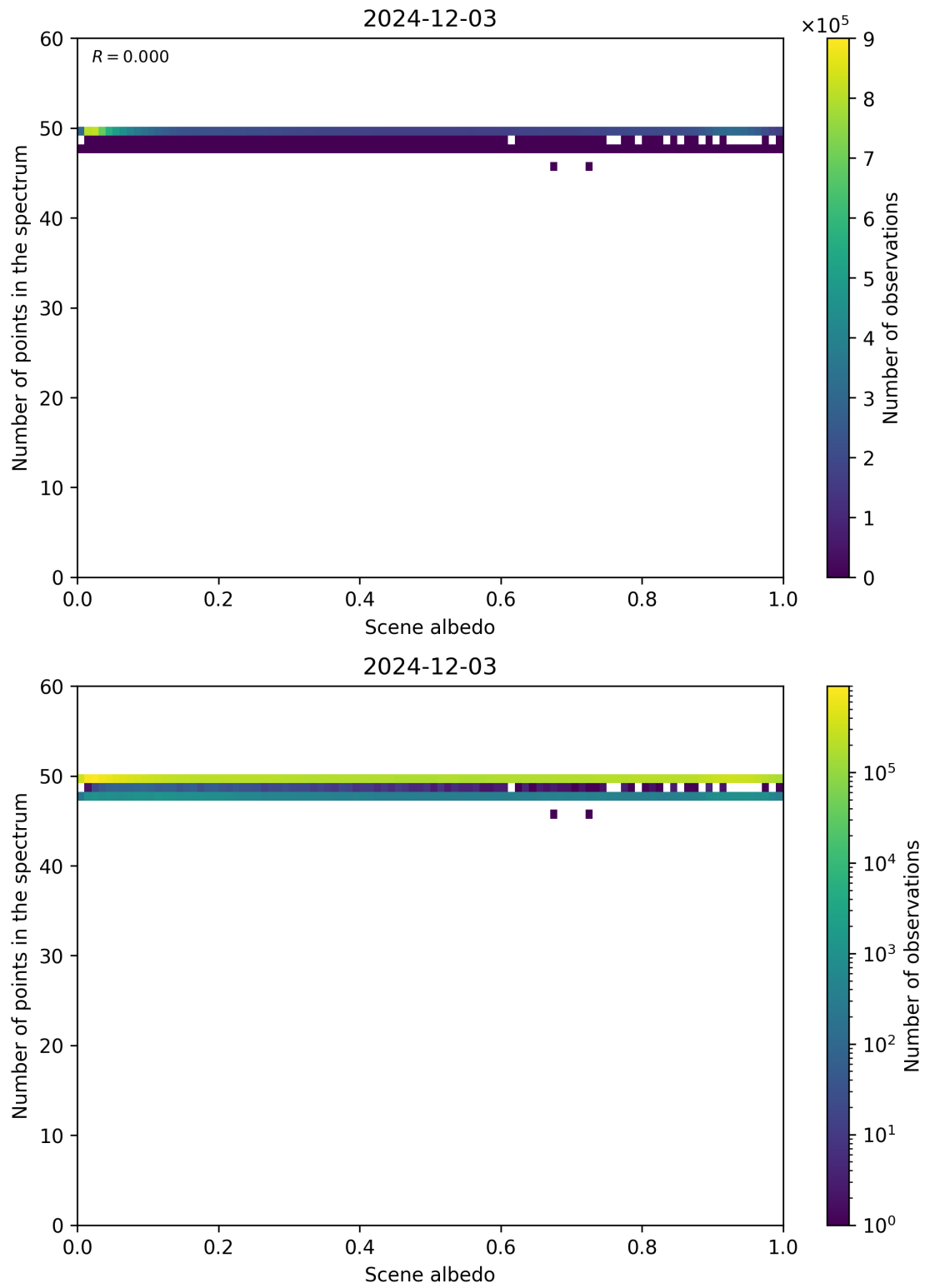
Figure 106: Scatter density plot of “Scene albedo” against “Number of points in the spectrum” for 2024-12-02 to 2024-12-04.
