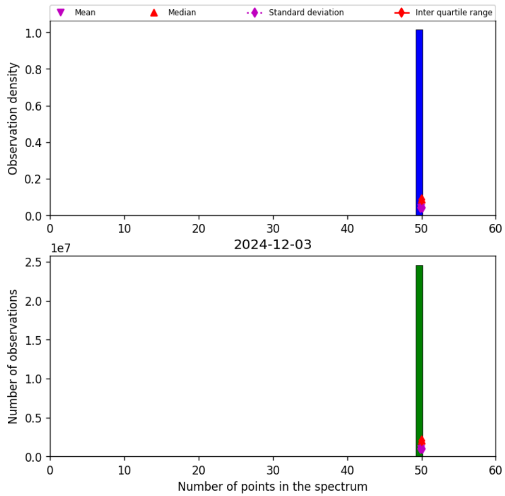
Figure 44: Histogram of "Number of points in the spectrum" for 2024-12-02 to 2024-12-04
