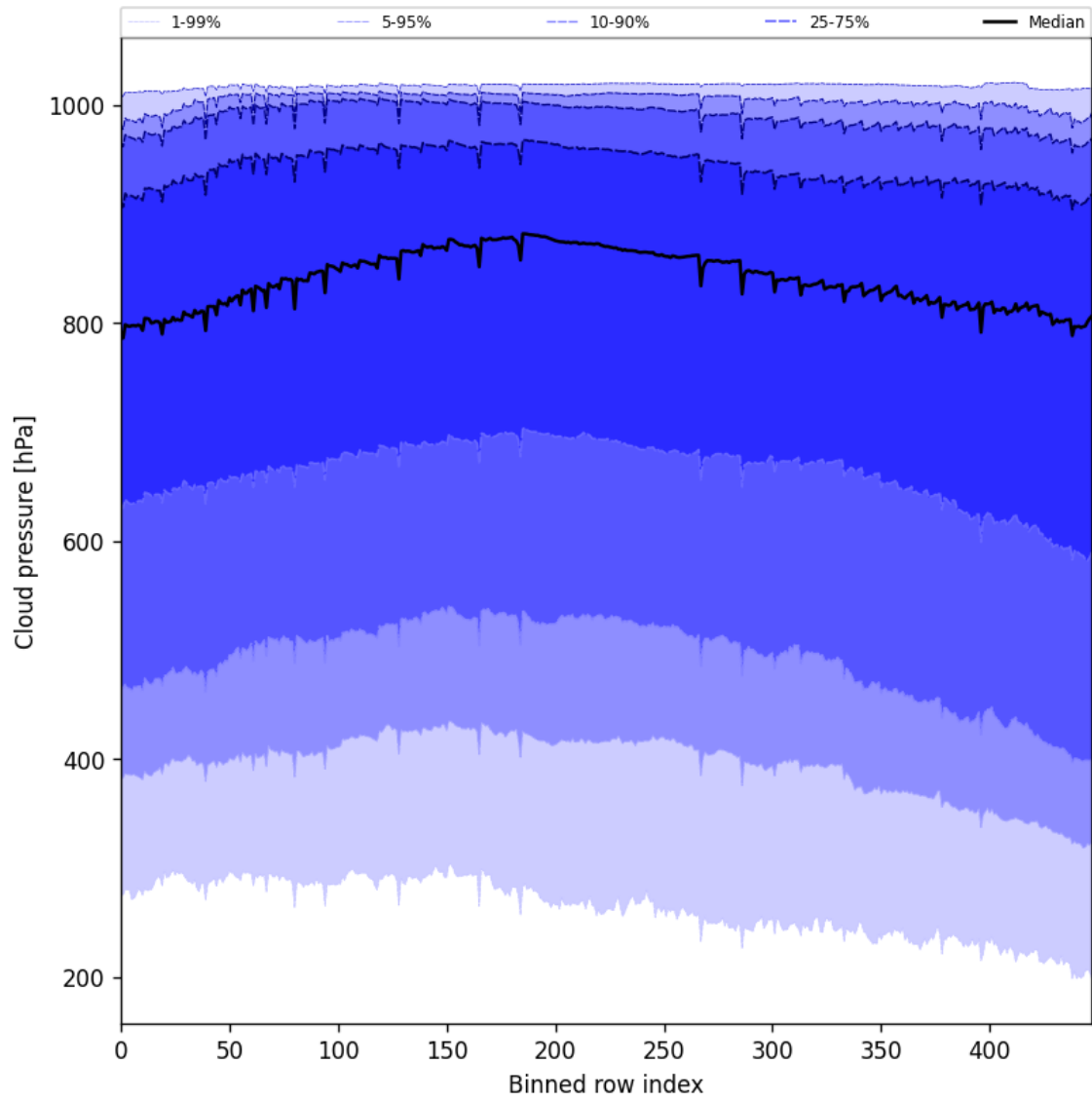
Figure 47: Along track statistics of “Cloud pressure” for 2024-12-02 to 2024-12-04
