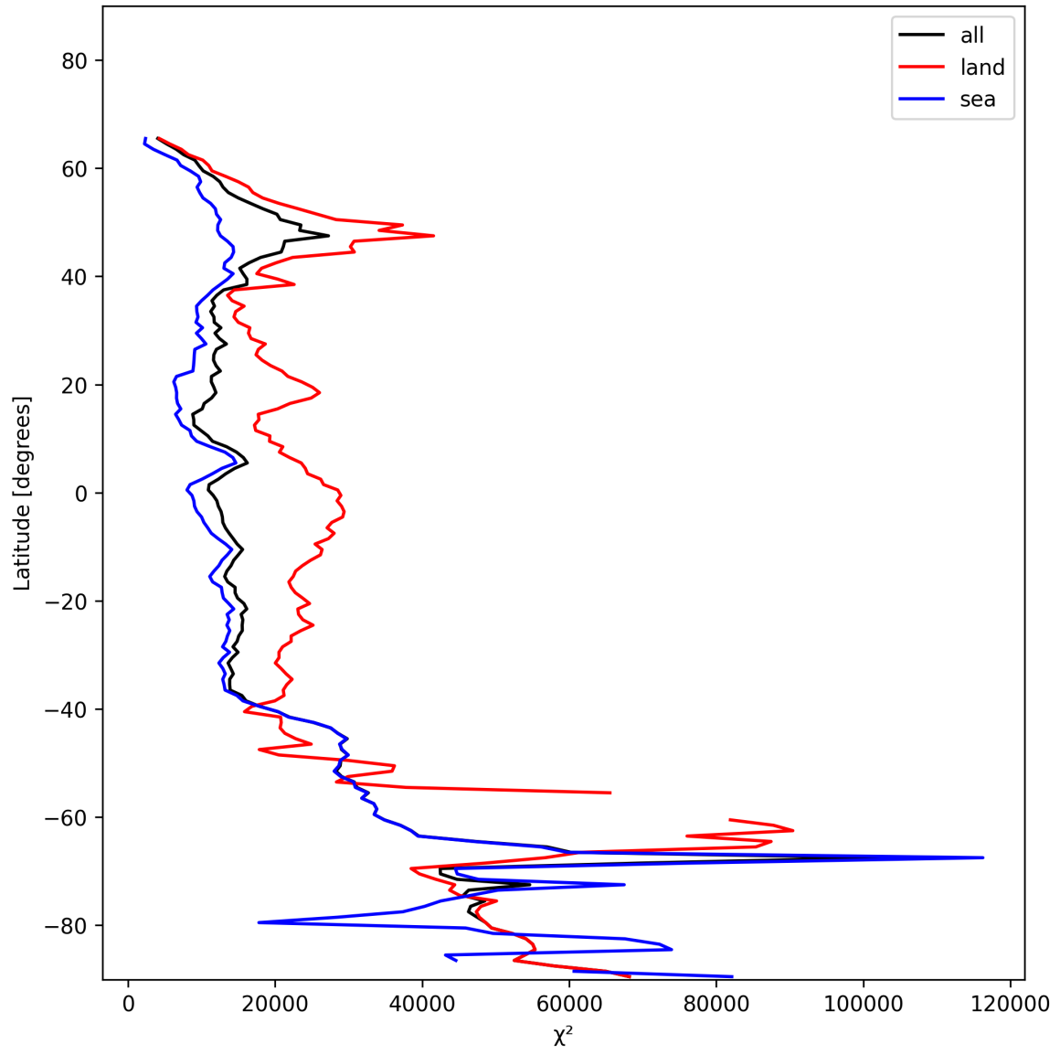
Figure 21: Zonal average of “ \chi^2 ” for 2024-12-02 to 2024-12-04.
