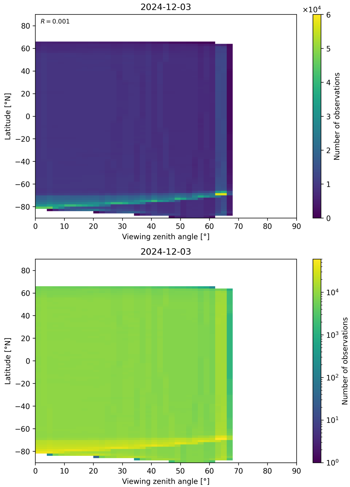
Figure 123: Scatter density plot of “Viewing zenith angle” against “Latitude” for 2024-12-02 to 2024-12-04.
