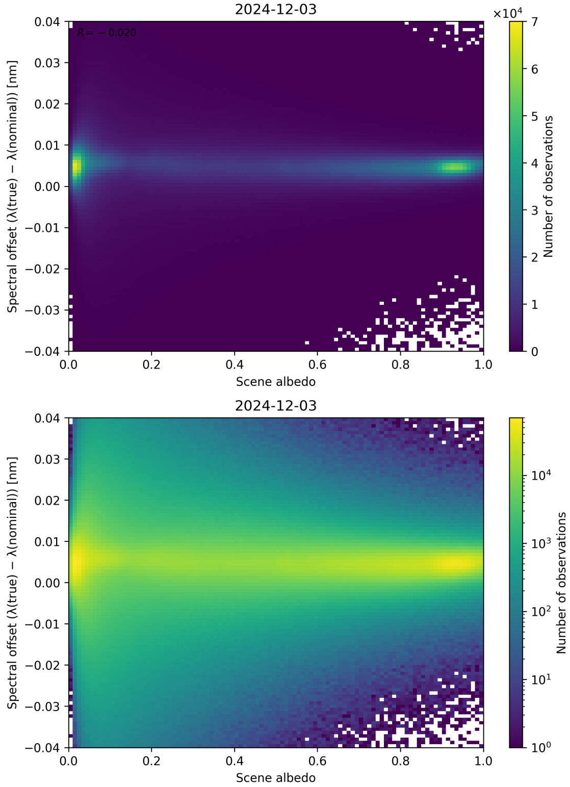
Figure 107: Scatter density plot of “Scene albedo” against “Spectral offset ( \lambda_{\text{true}} - \lambda_{\text{nominal}} )” for 2024-12-02 to 2024-12-04.
