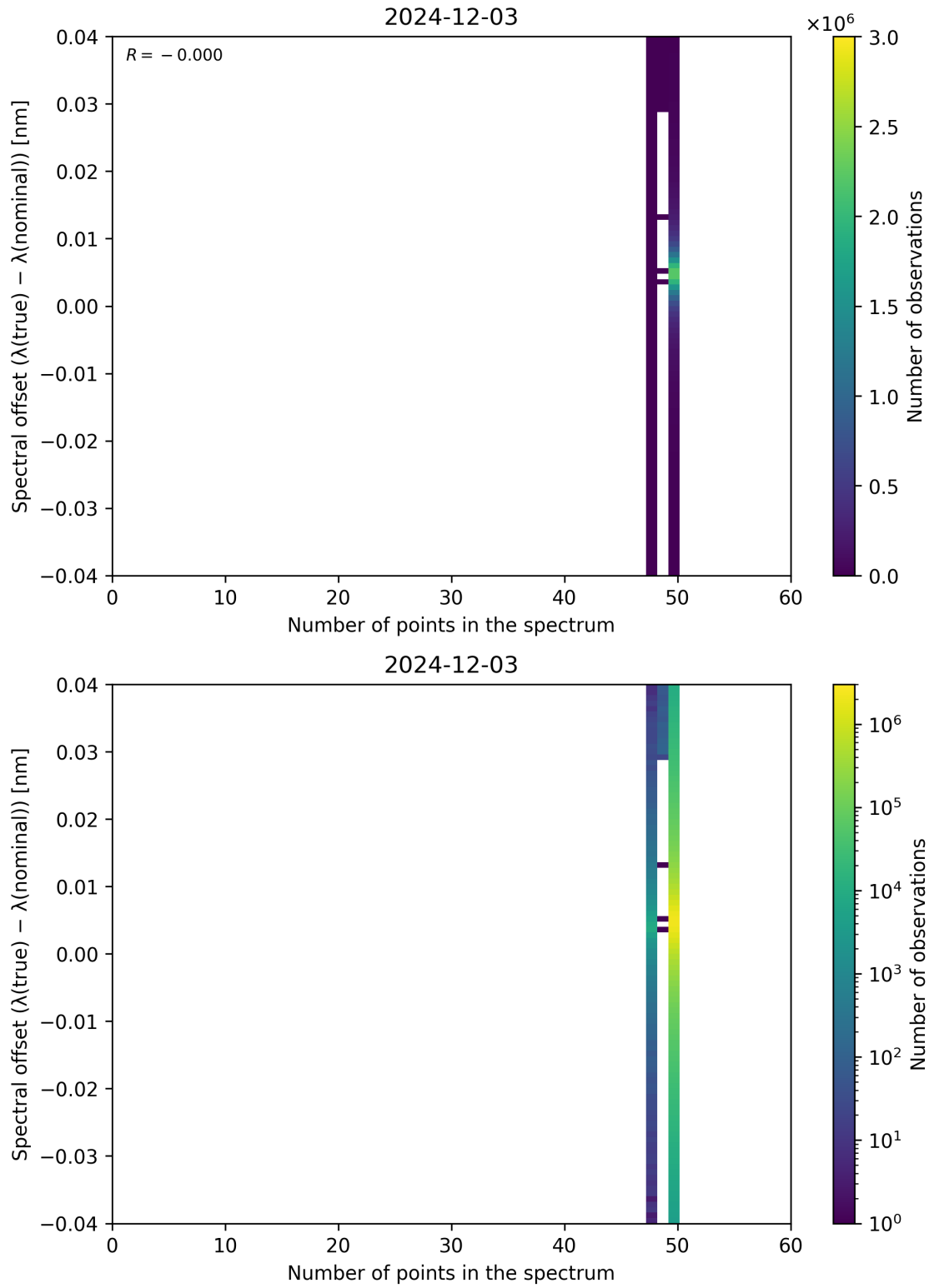
Figure 101: Scatter density plot of “Number of points in the spectrum” against “Spectral offset ( \lambda_{\text{true}} - \lambda_{\text{nominal}} )” for 2024-12-02 to 2024-12-04.
