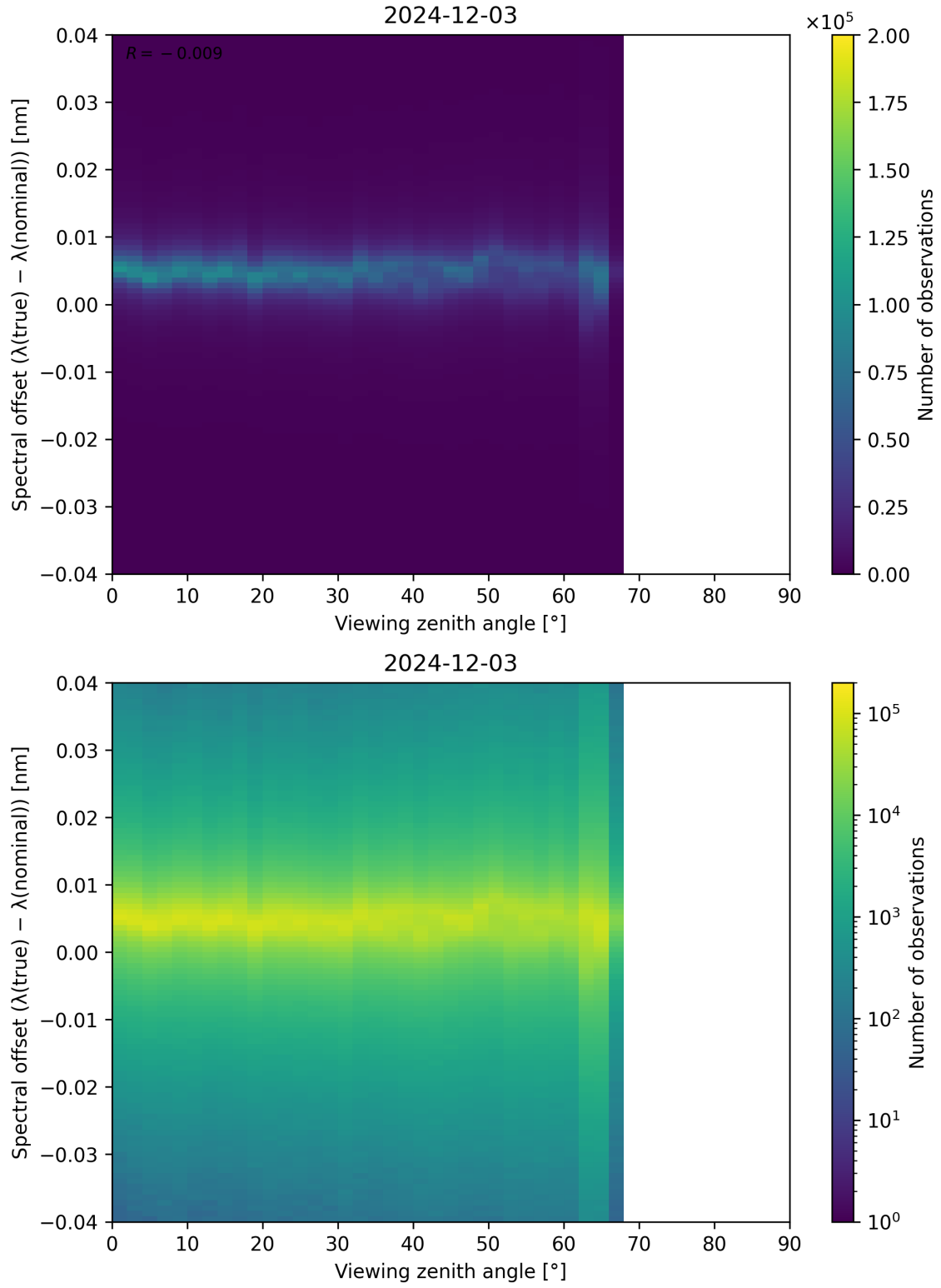
Figure 128: Scatter density plot of “Viewing zenith angle” against “Spectral offset ( \lambda_{\text{true}} - \lambda_{\text{nominal}} )” for 2024-12-02 to 2024-12-04.
