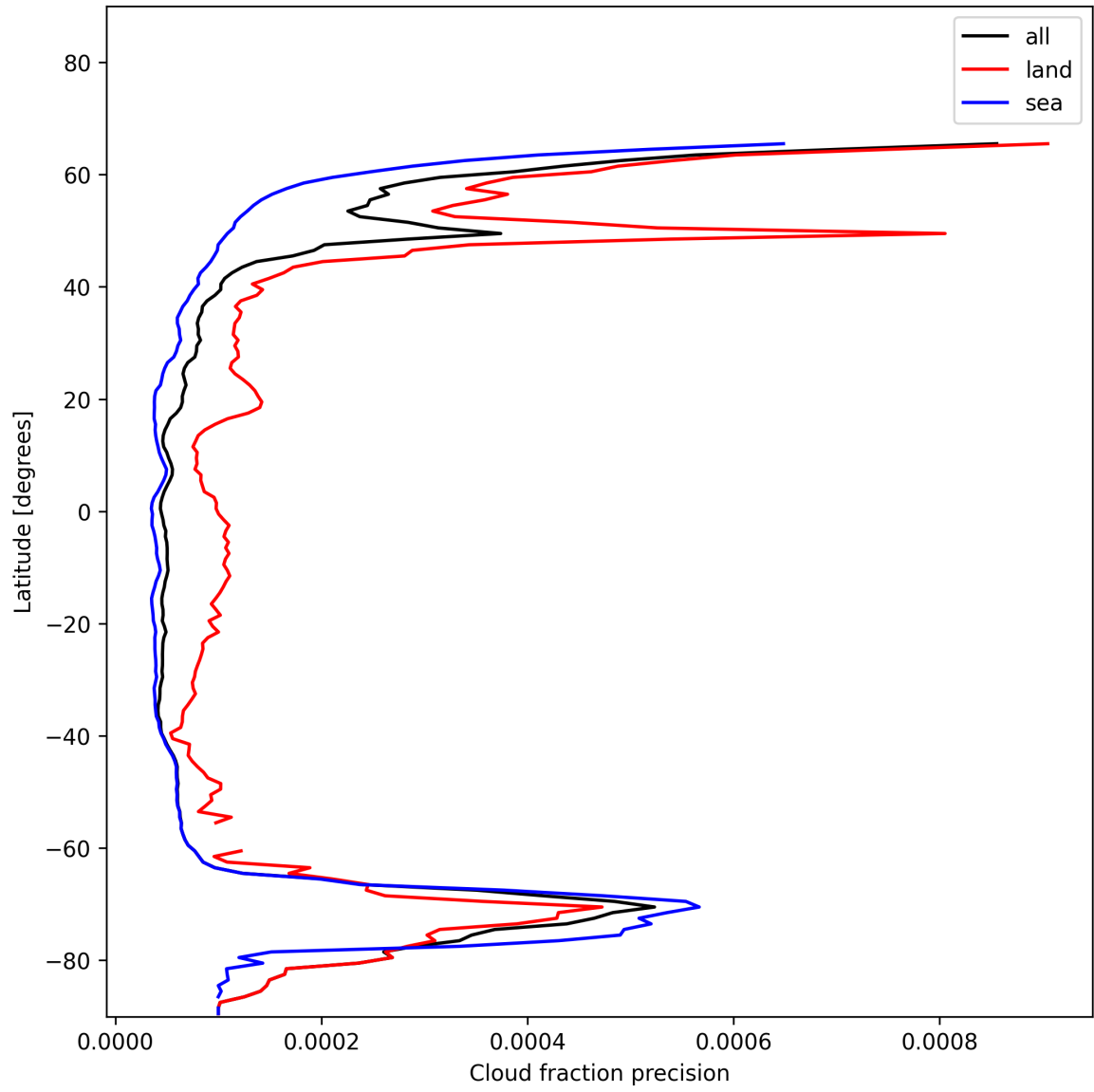
Figure 16: Zonal average of “Cloud fraction precision” for 2024-12-02 to 2024-12-04.
