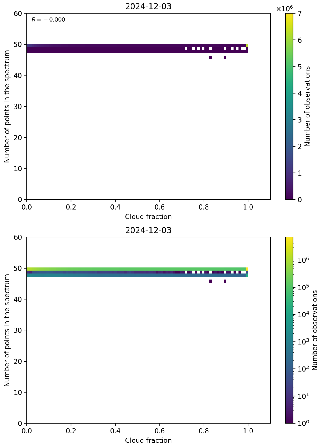
Figure 74: Scatter density plot of “Cloud fraction” against “Number of points in the spectrum” for 2024-12-02 to 2024-12-04.
