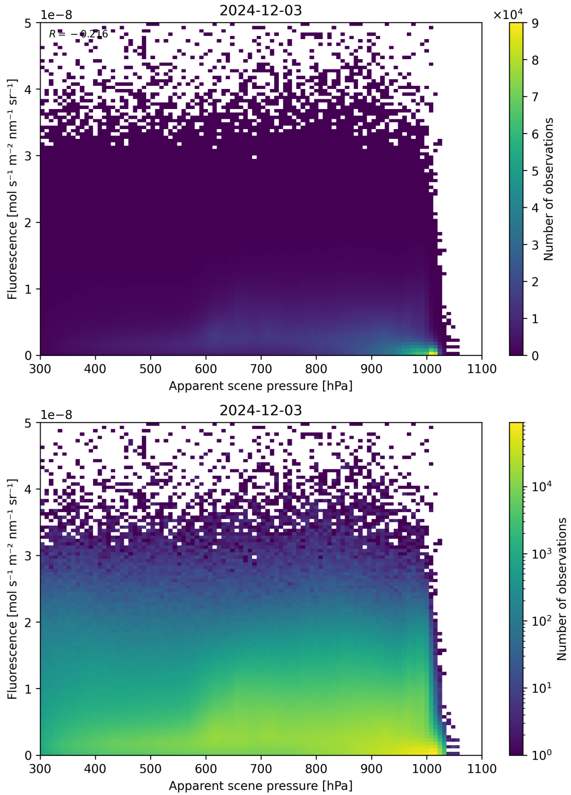
Figure 64: Scatter density plot of “Apparent scene pressure” against “Fluorescence” for 2024-12-02 to 2024-12-04.
