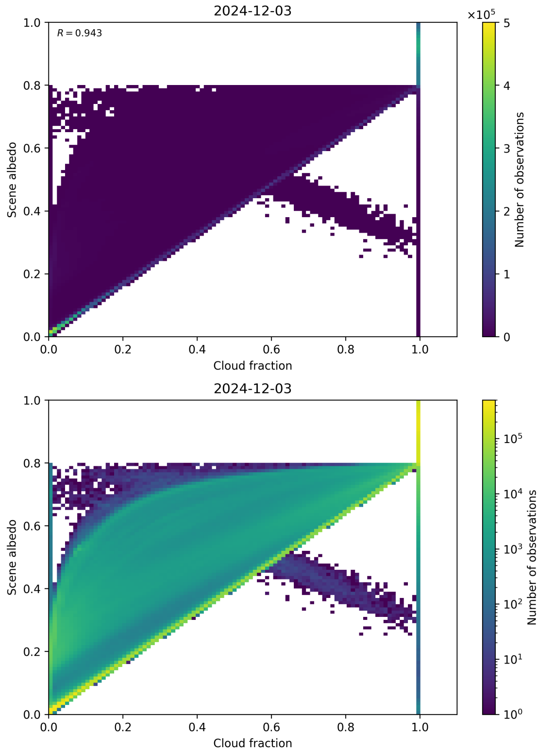
Figure 75: Scatter density plot of “Cloud fraction” against “Scene albedo” for 2024-12-02 to 2024-12-04.
