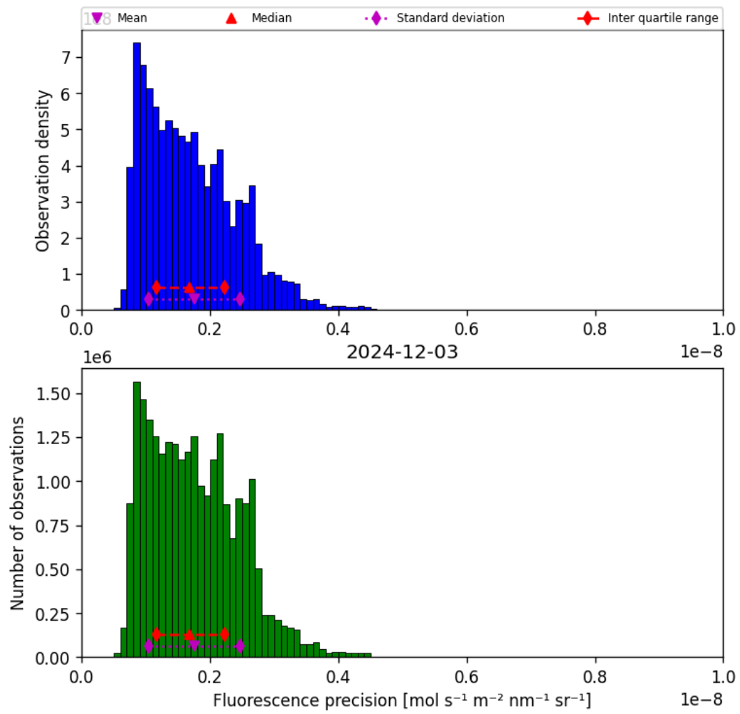
Figure 41: Histogram of “Fluorescence precision” for 2024-12-02 to 2024-12-04
