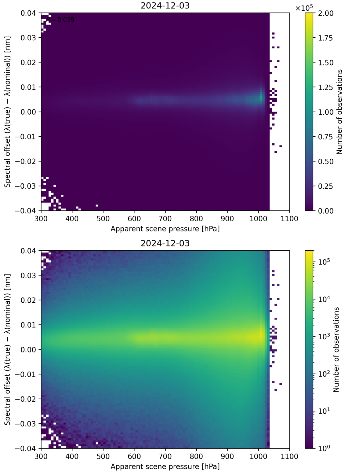
Figure 67: Scatter density plot of “Apparent scene pressure” against “Spectral offset ( \lambda_{\text{true}} - \lambda_{\text{nominal}} )” for 2024-12-02 to 2024-12-04.
