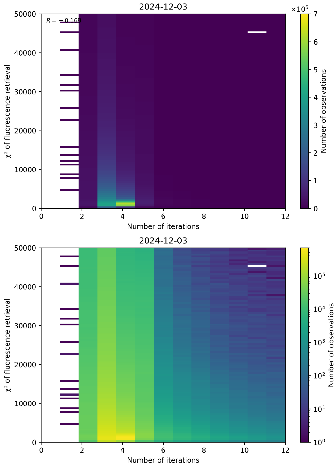
Figure 97: Scatter density plot of “Number of iterations” against “ \chi^2 of fluorescence retrieval” for 2024-12-02 to 2024-12-04.
