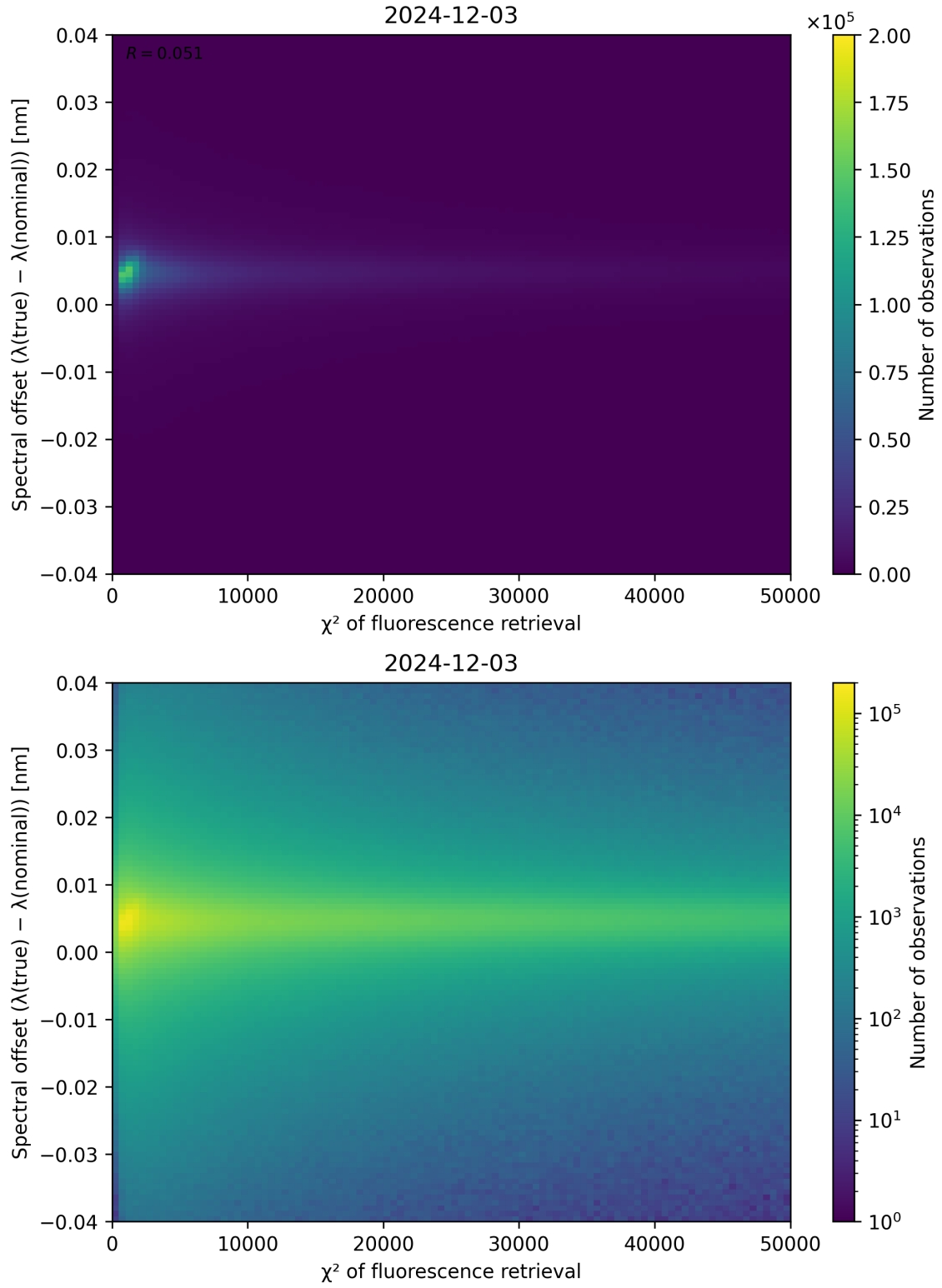
Figure 69: Scatter density plot of “ \chi^2 of fluorescence retrieval” against “Spectral offset ( \lambda_{\text{true}} - \lambda_{\text{nominal}} )” for 2024-12-02 to 2024-12-04.
