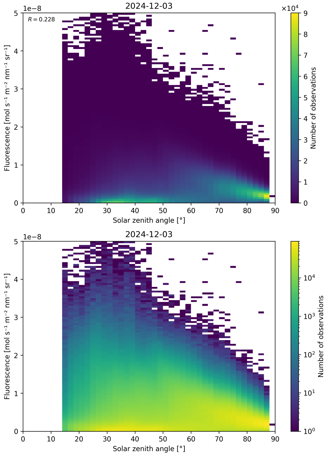
Figure 112: Scatter density plot of “Solar zenith angle” against “Fluorescence” for 2024-12-02 to 2024-12-04.
