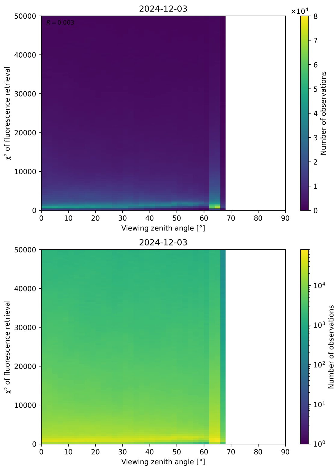
Figure 119: Scatter density plot of “Viewing zenith angle” against “ \chi^2 of fluorescence retrieval” for 2024-12-02 to 2024-12-04.
