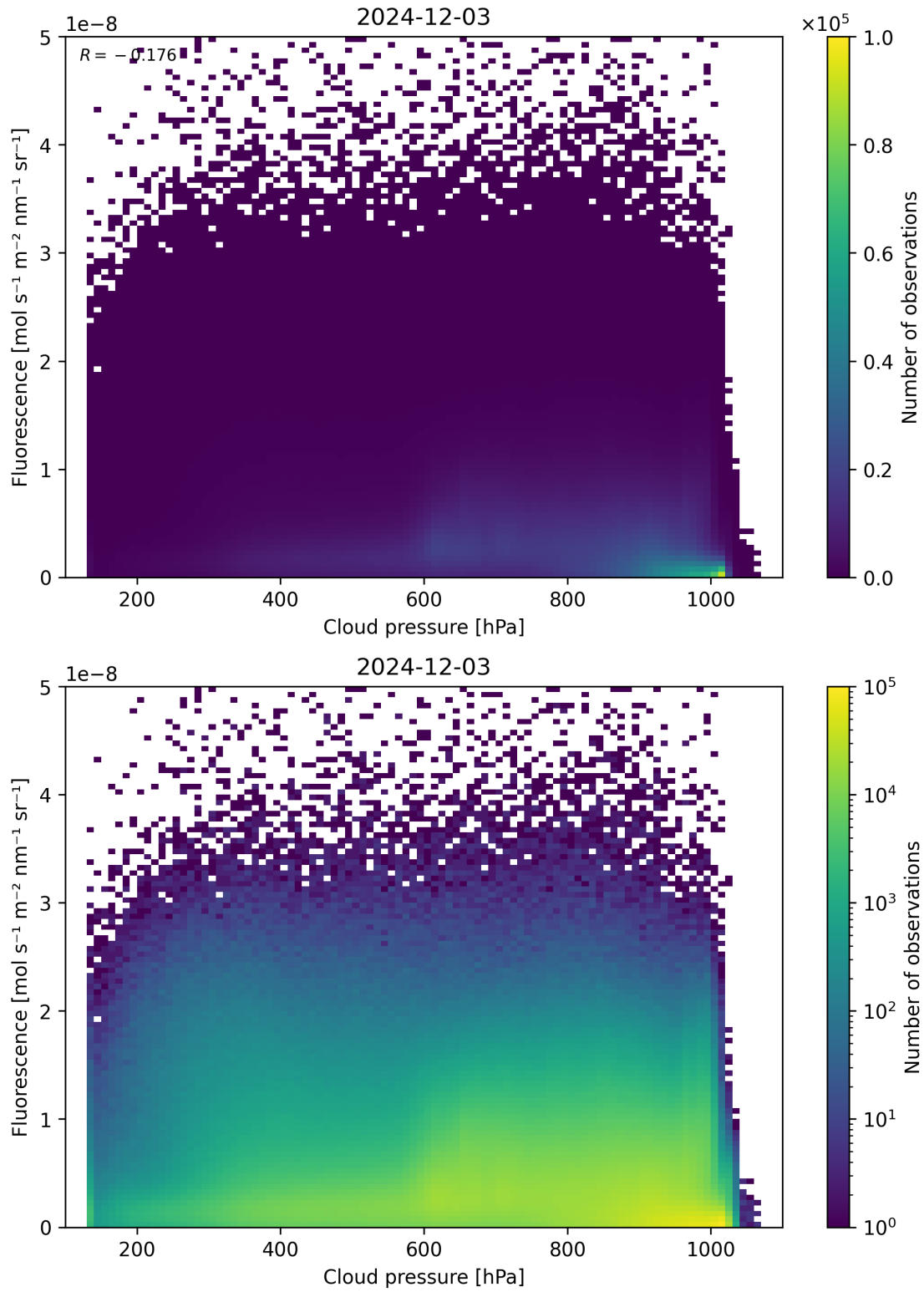
Figure 80: Scatter density plot of “Cloud pressure” against “Fluorescence” for 2024-12-02 to 2024-12-04.
