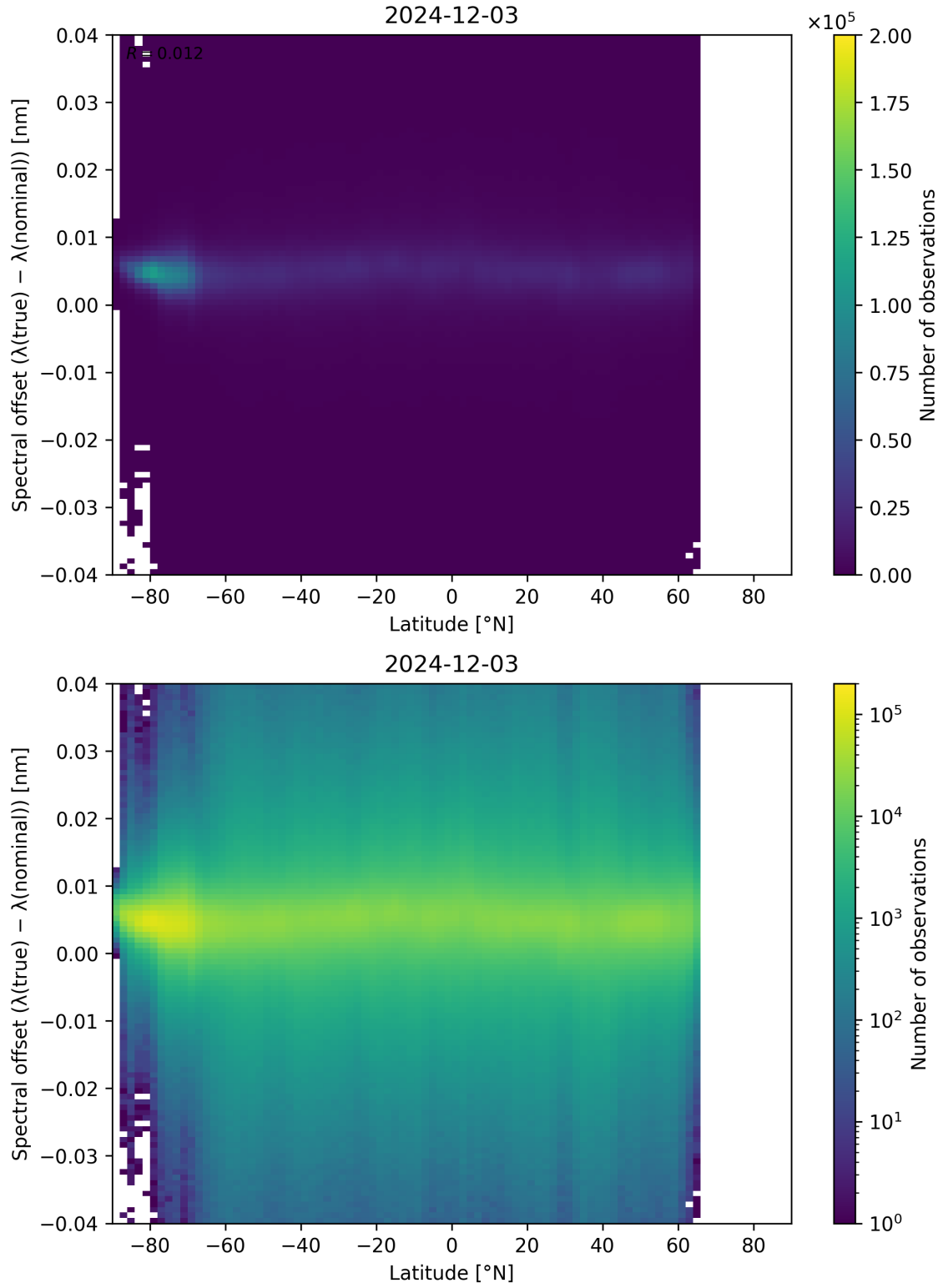
Figure 96: Scatter density plot of “Latitude” against “Spectral offset ( \lambda_{\text{true}} - \lambda_{\text{nominal}} )” for 2024-12-02 to 2024-12-04.
