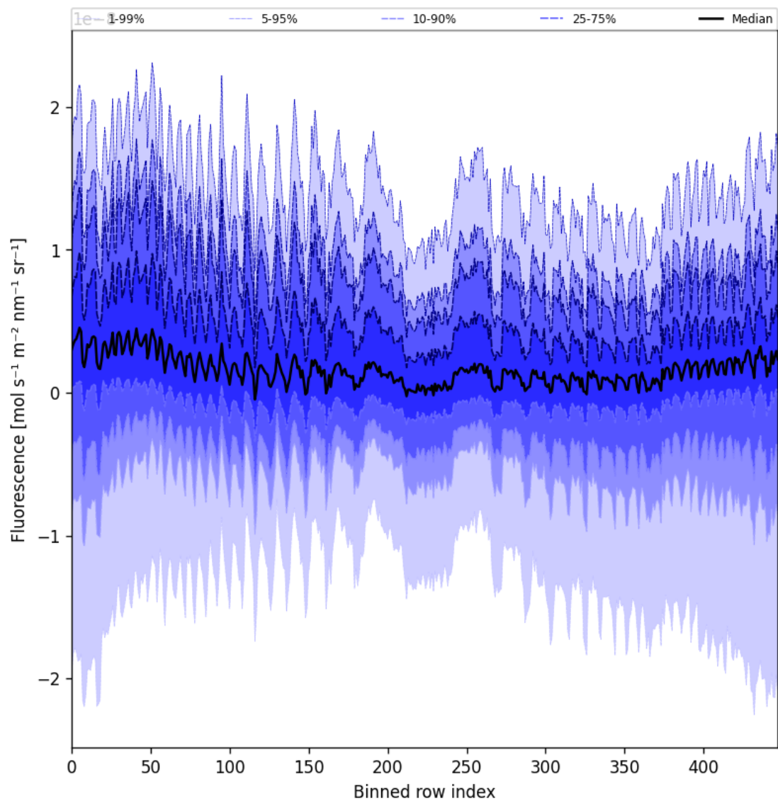
Figure 57: Along track statistics of “Fluorescence” for 2024-12-02 to 2024-12-04
