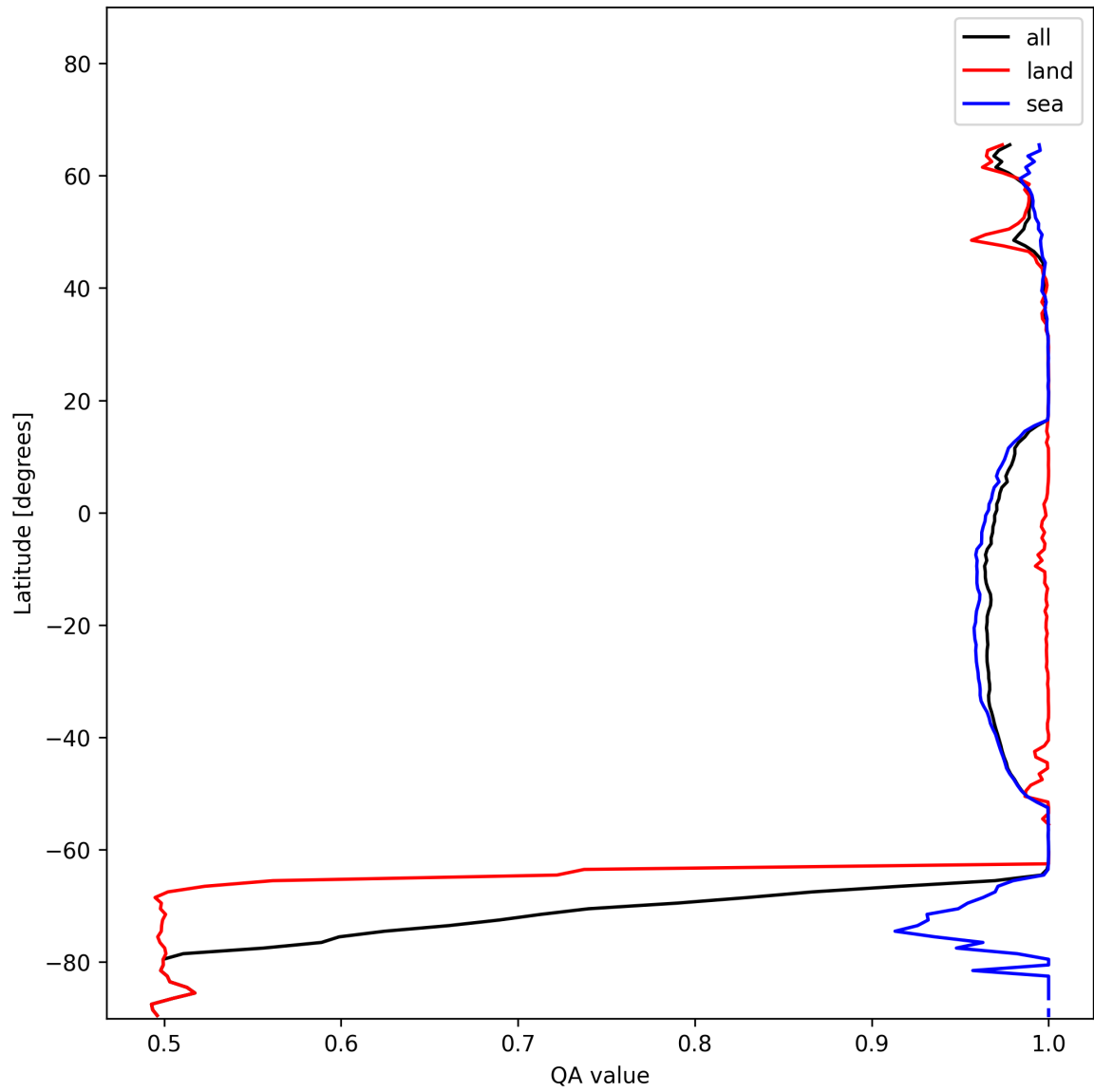
Figure 12: Zonal average of “QA value” for 2024-12-02 to 2024-12-04.
