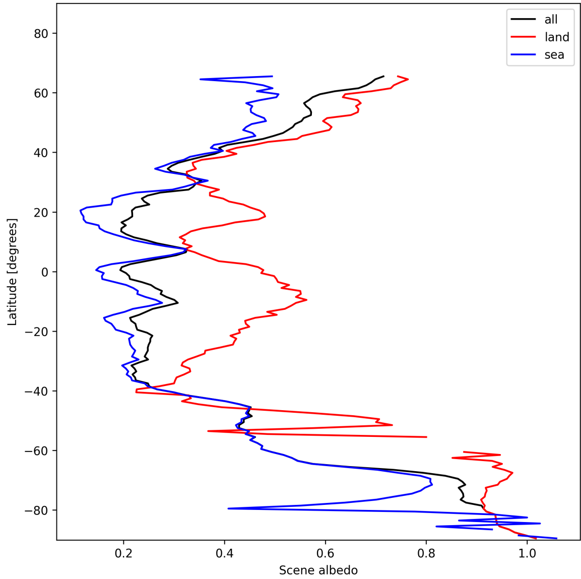
Figure 17: Zonal average of “Scene albedo” for 2024-12-02 to 2024-12-04.
