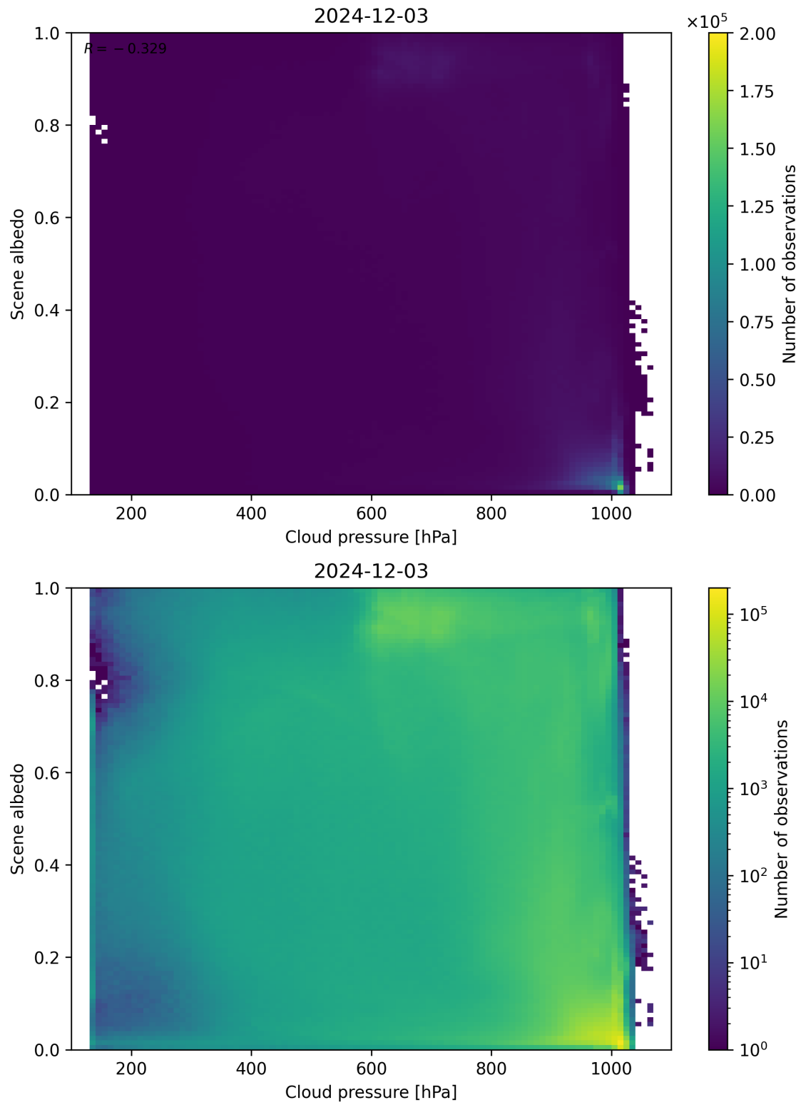
Figure 83: Scatter density plot of “Cloud pressure” against “Scene albedo” for 2024-12-02 to 2024-12-04.
