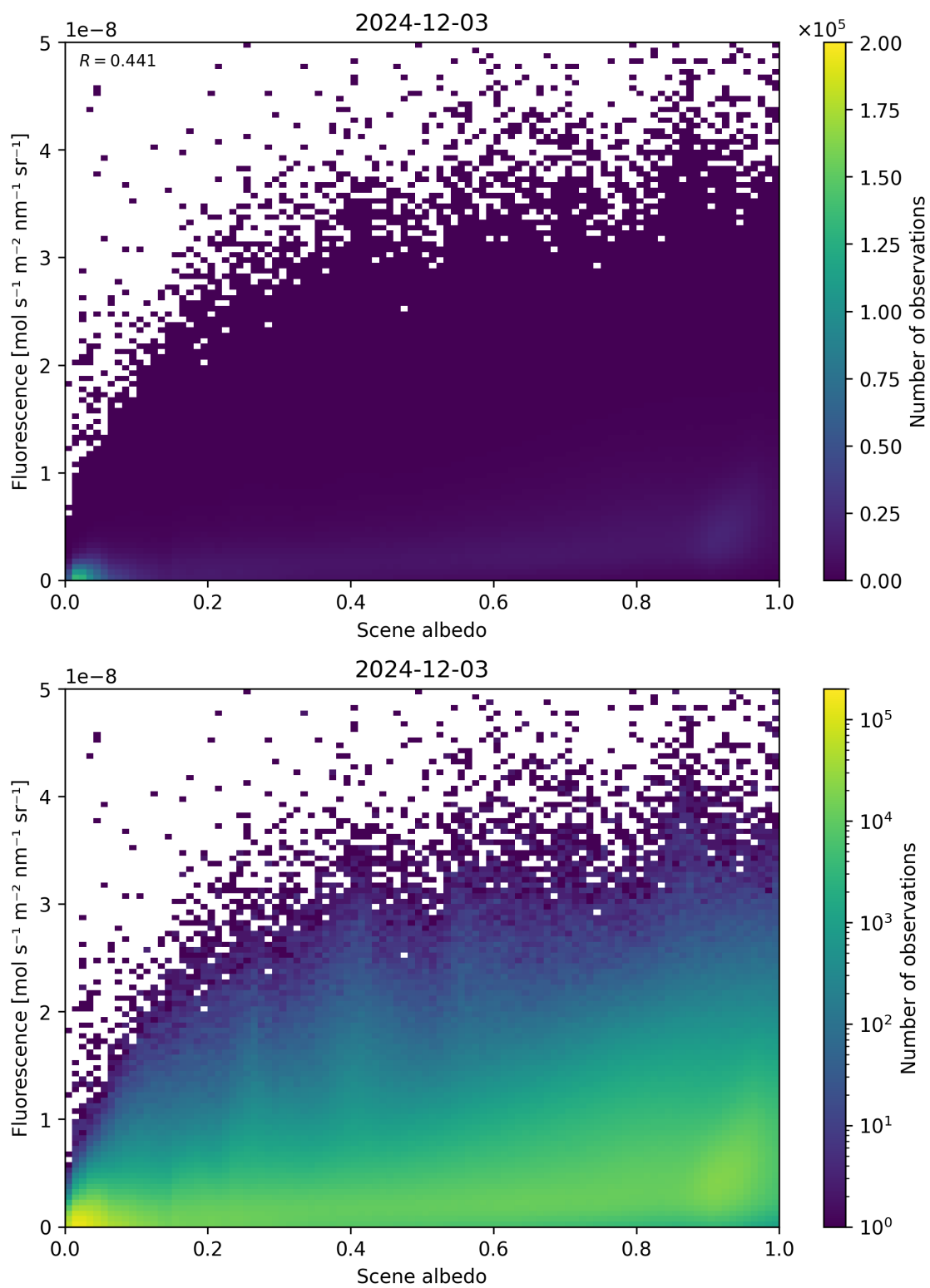
Figure 104: Scatter density plot of “Scene albedo” against “Fluorescence” for 2024-12-02 to 2024-12-04.
