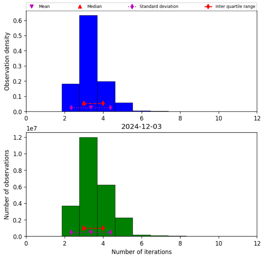
Figure 39: Histogram of “Number of iterations” for 2024-12-02 to 2024-12-04
