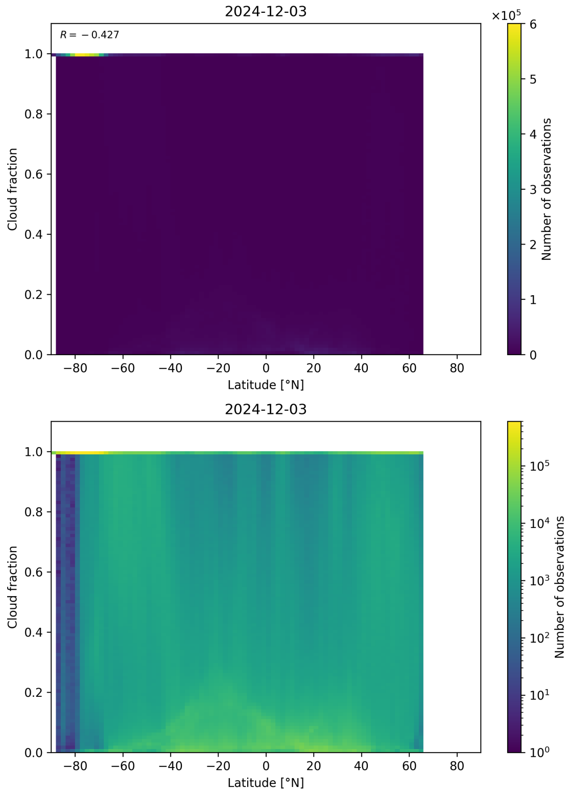
Figure 90: Scatter density plot of “Latitude” against “Cloud fraction” for 2024-12-02 to 2024-12-04.
