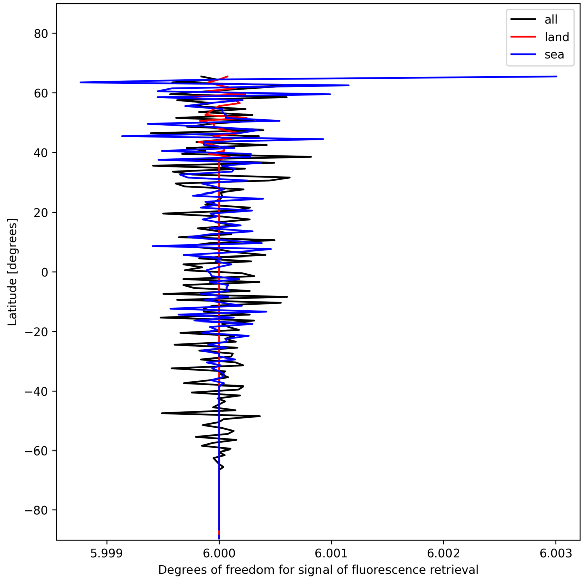
Figure 26: Zonal average of “Degrees of freedom for signal of fluorescence retrieval” for 2024-12-02 to 2024-12-04.
