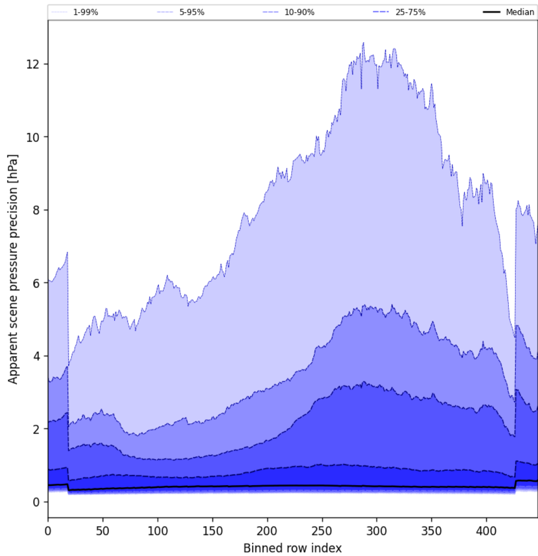
Figure 54: Along track statistics of “Apparent scene pressure precision” for 2024-12-02 to 2024-12-04
