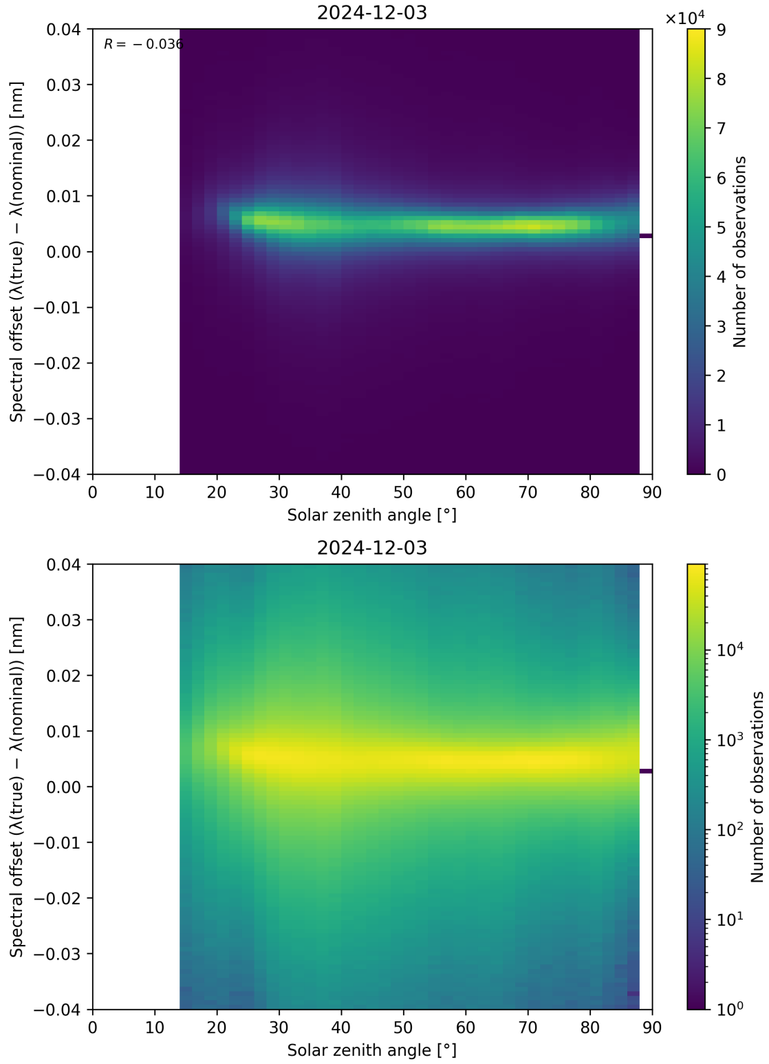
Figure 117: Scatter density plot of “Solar zenith angle” against “Spectral offset ( \lambda_{\text{true}} - \lambda_{\text{nominal}} )” for 2024-12-02 to 2024-12-04.
