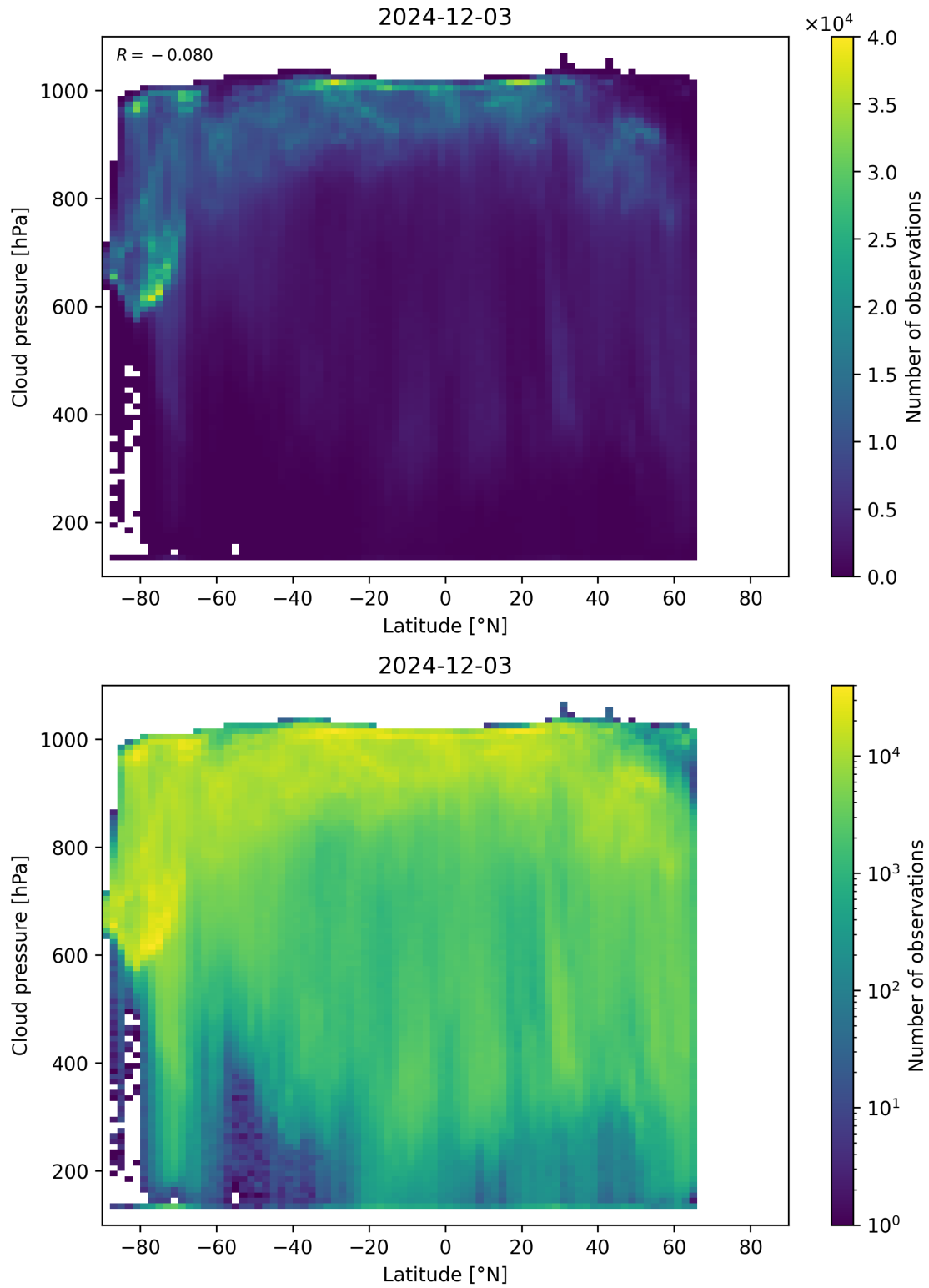
Figure 91: Scatter density plot of “Latitude” against “Cloud pressure” for 2024-12-02 to 2024-12-04.
