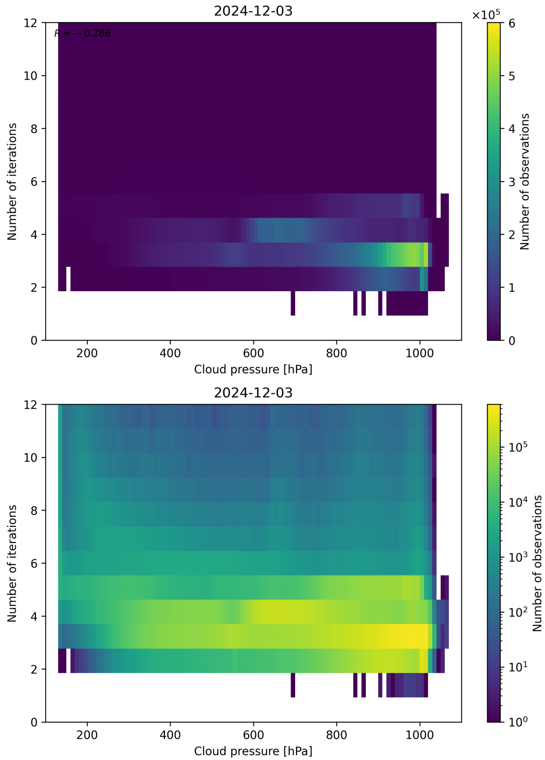
Figure 81: Scatter density plot of “Cloud pressure” against “Number of iterations” for 2024-12-02 to 2024-12-04.
