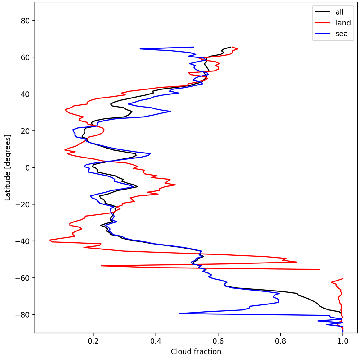
Figure 15: Zonal average of “Cloud fraction” for 2024-12-02 to 2024-12-04.
