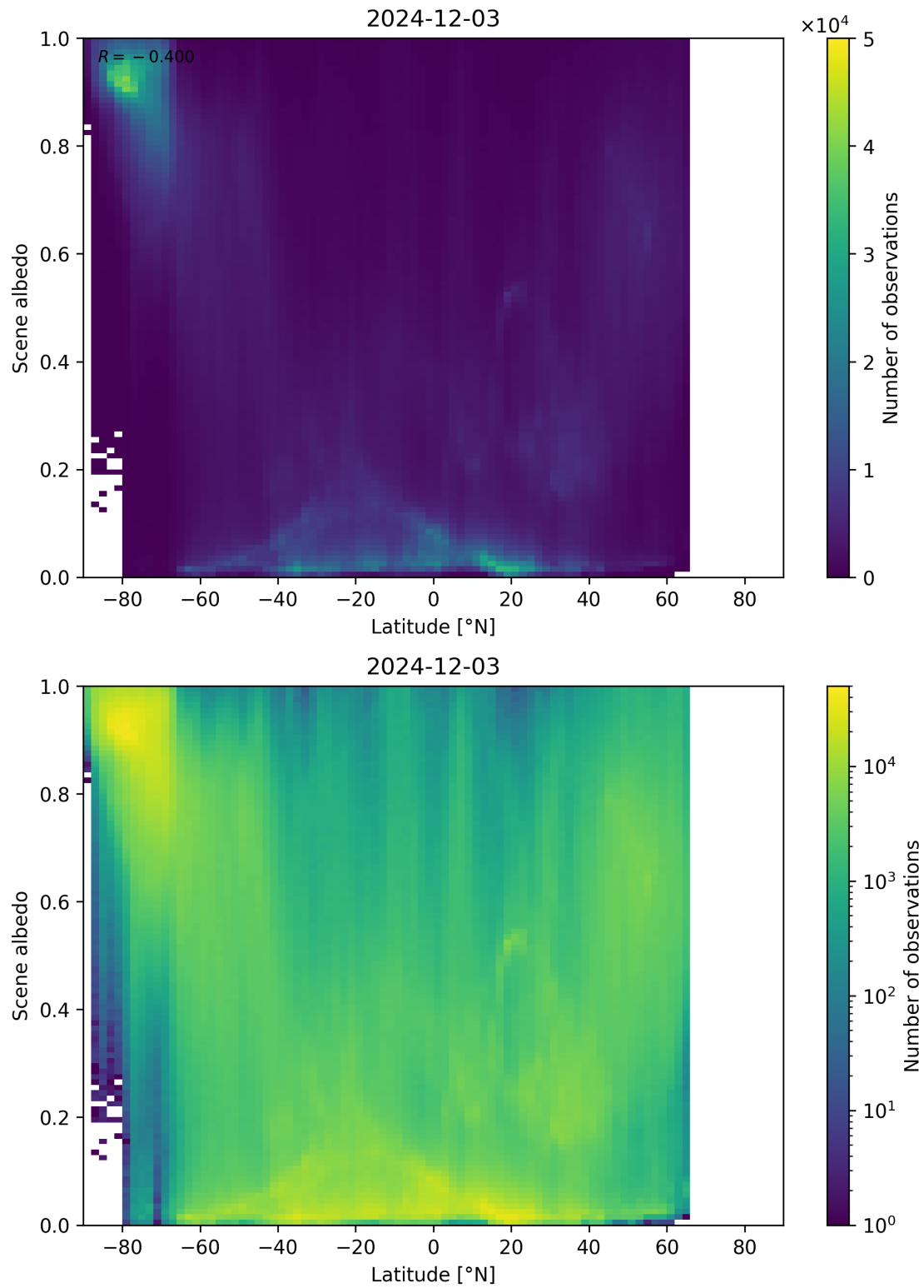
Figure 95: Scatter density plot of “Latitude” against “Scene albedo” for 2024-12-02 to 2024-12-04.
