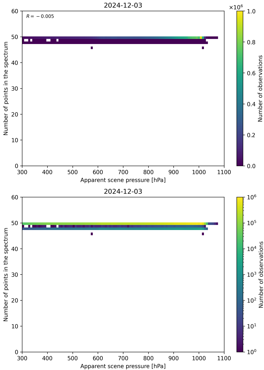
Figure 66: Scatter density plot of “Apparent scene pressure” against “Number of points in the spectrum” for 2024-12-02 to 2024-12-04.
