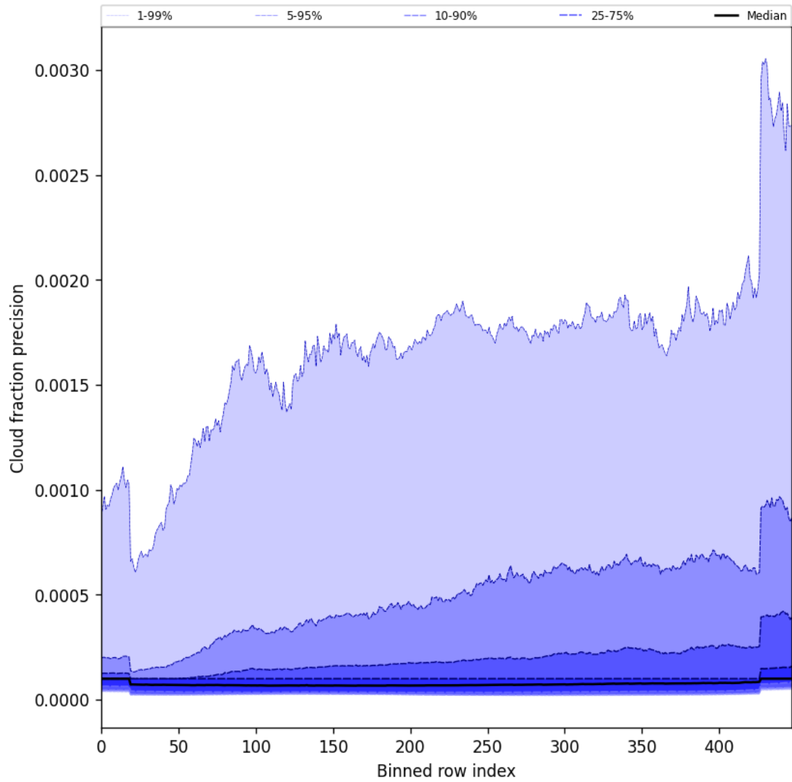
Figure 50: Along track statistics of “Cloud fraction precision” for 2024-12-02 to 2024-12-04
