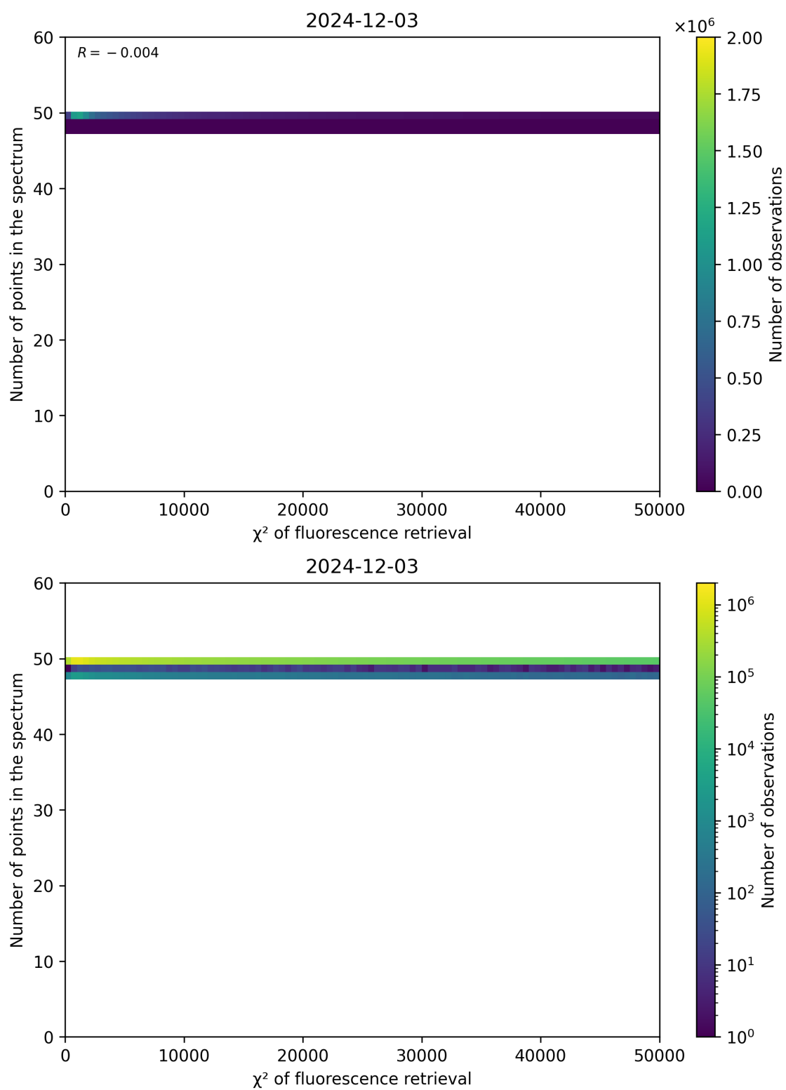
Figure 68: Scatter density plot of “ \chi^2 of fluorescence retrieval” against “Number of points in the spectrum” for 2024-12-02 to 2024-12-04.
