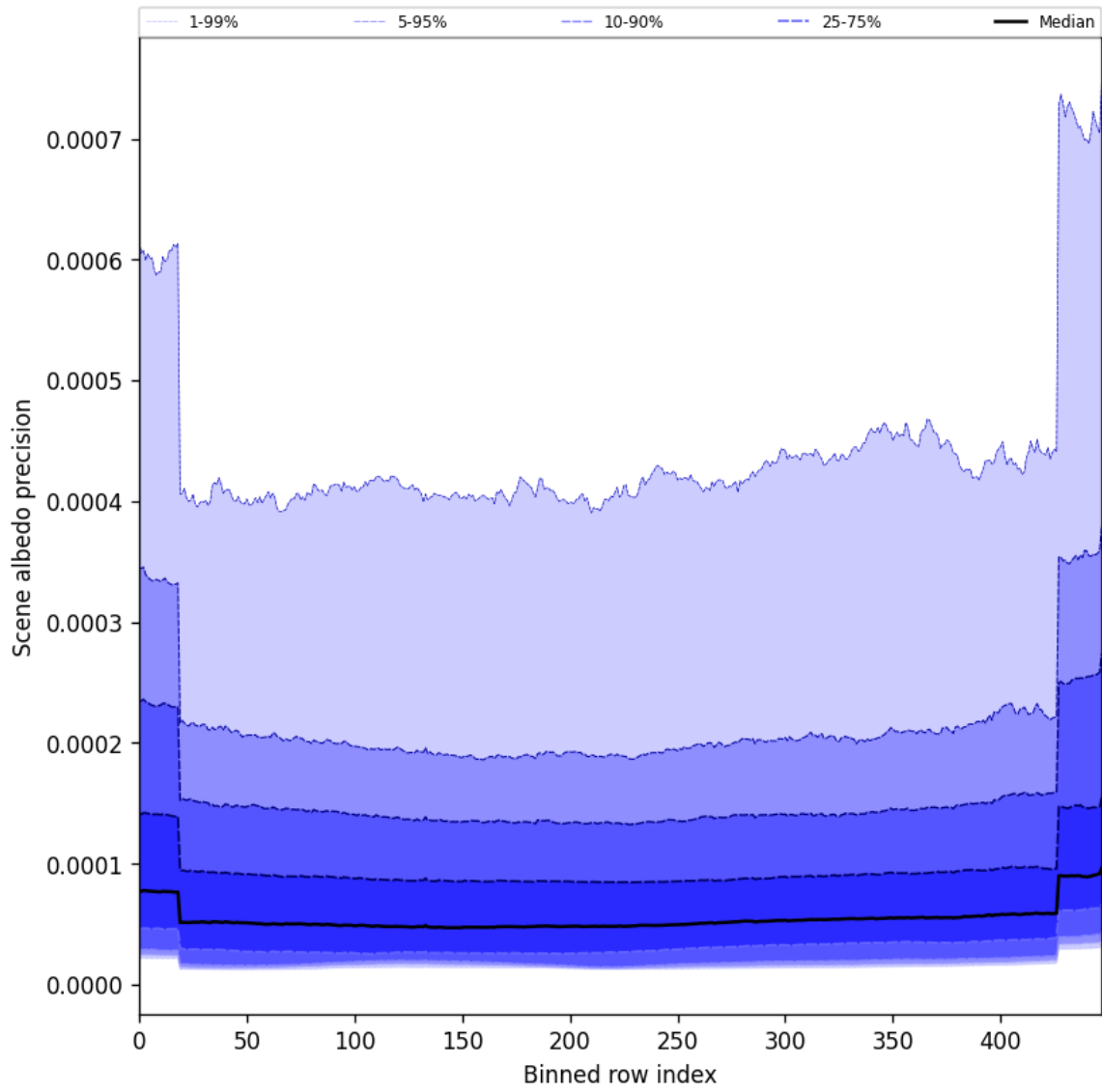
Figure 52: Along track statistics of “Scene albedo precision” for 2024-12-02 to 2024-12-04
