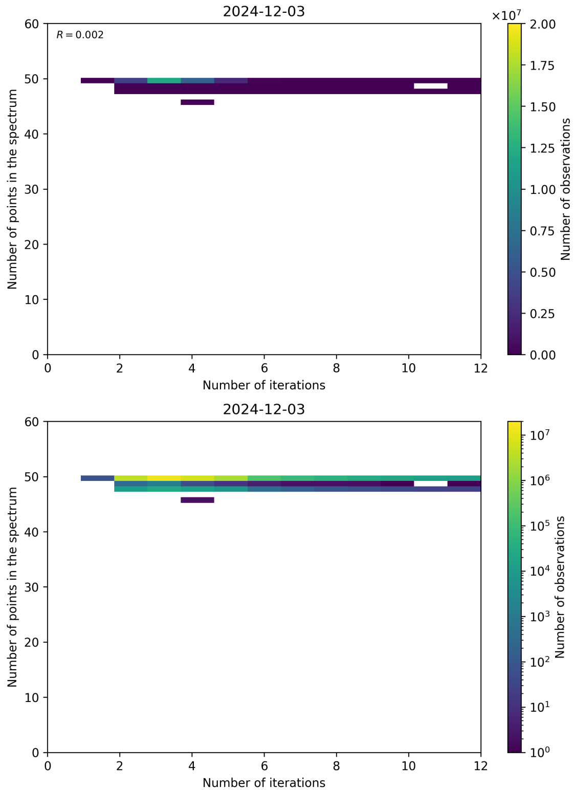
Figure 99: Scatter density plot of “Number of iterations” against “Number of points in the spectrum” for 2024-12-02 to 2024-12-04.
