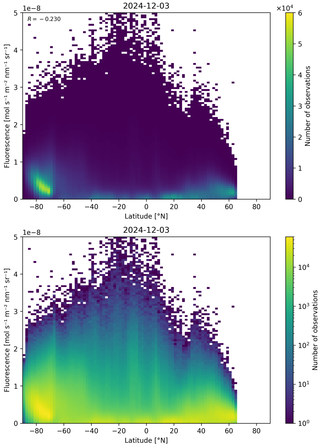
Figure 92: Scatter density plot of “Latitude” against “Fluorescence” for 2024-12-02 to 2024-12-04.
