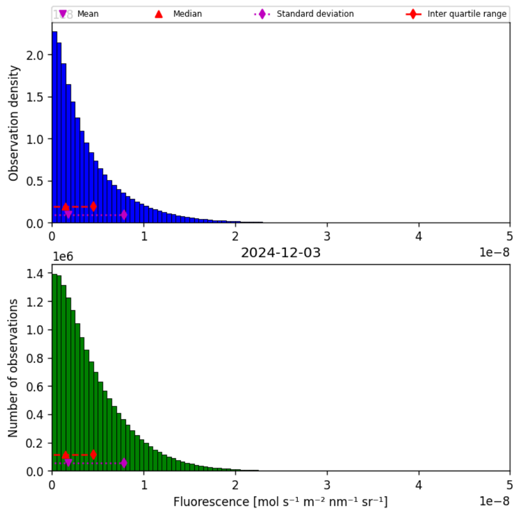
Figure 40: Histogram of “Fluorescence” for 2024-12-02 to 2024-12-04
