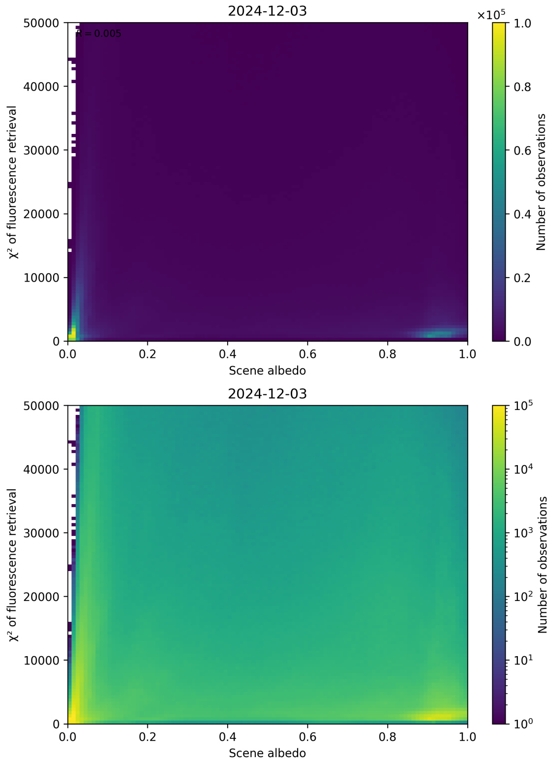
Figure 103: Scatter density plot of “Scene albedo” against “ \chi^2 of fluorescence retrieval” for 2024-12-02 to 2024-12-04.
