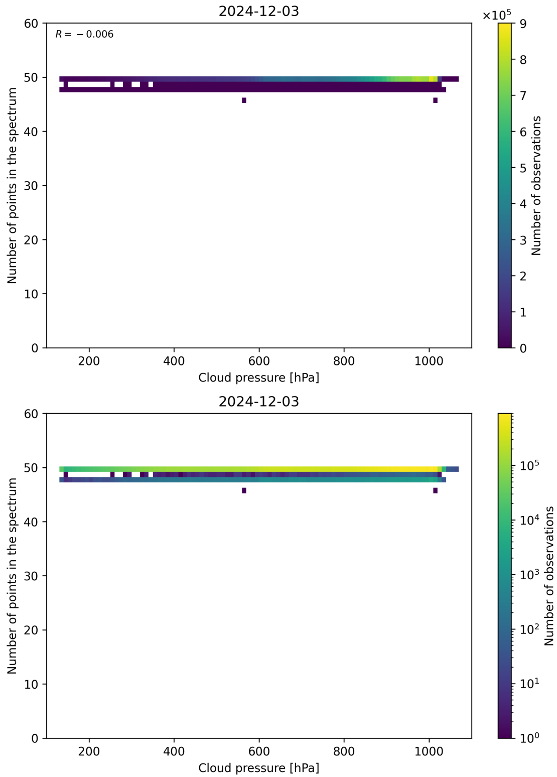
Figure 82: Scatter density plot of “Cloud pressure” against “Number of points in the spectrum” for 2024-12-02 to 2024-12-04.
