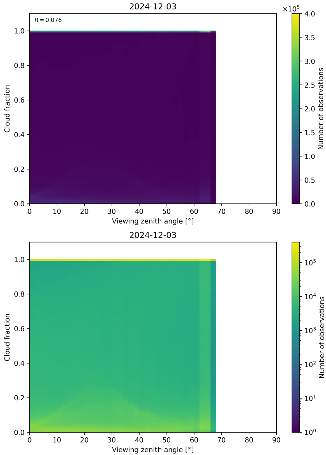
Figure 120: Scatter density plot of “Viewing zenith angle” against “Cloud fraction” for 2024-12-02 to 2024-12-04.
