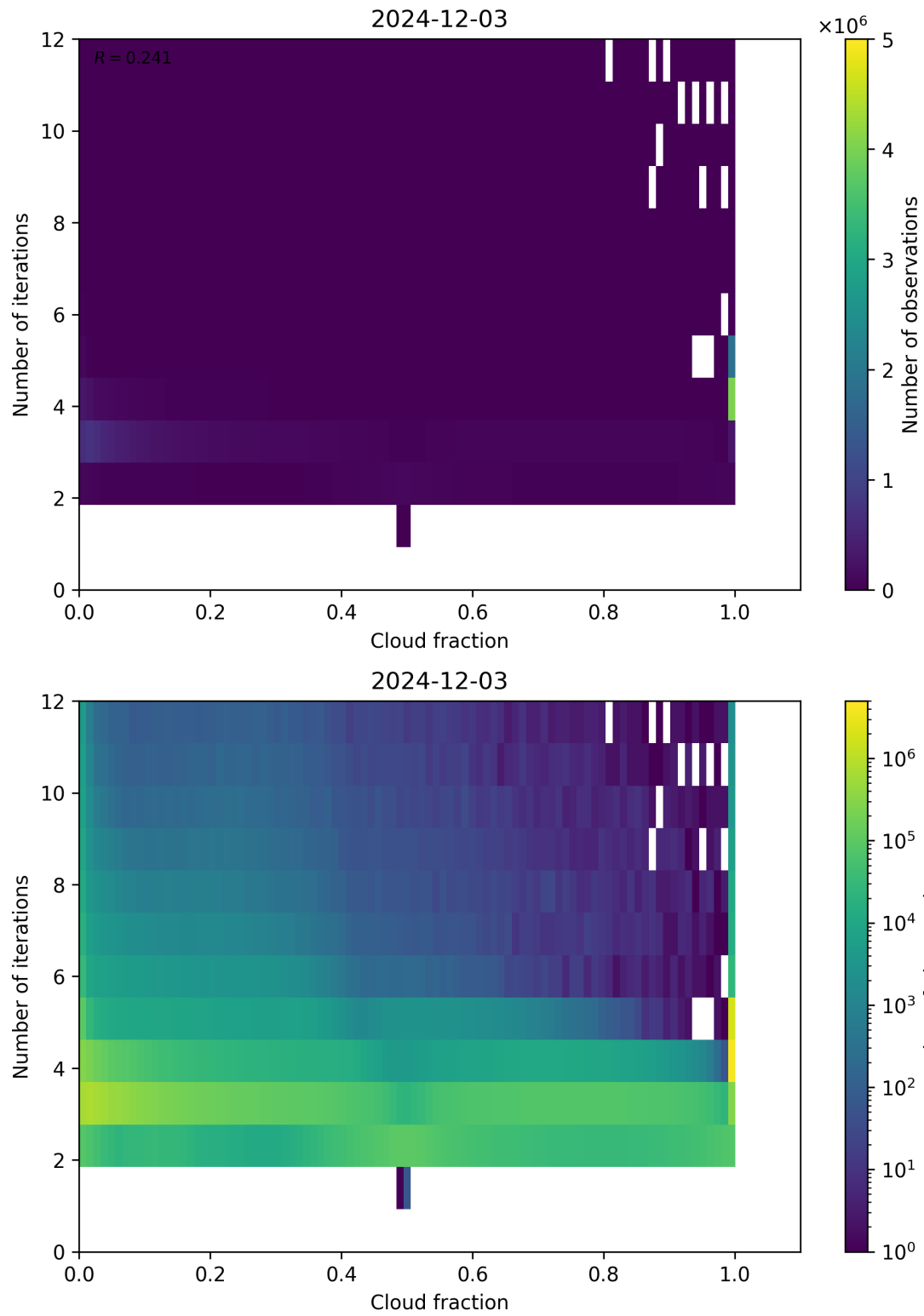
Figure 73: Scatter density plot of “Cloud fraction” against “Number of iterations” for 2024-12-02 to 2024-12-04.
