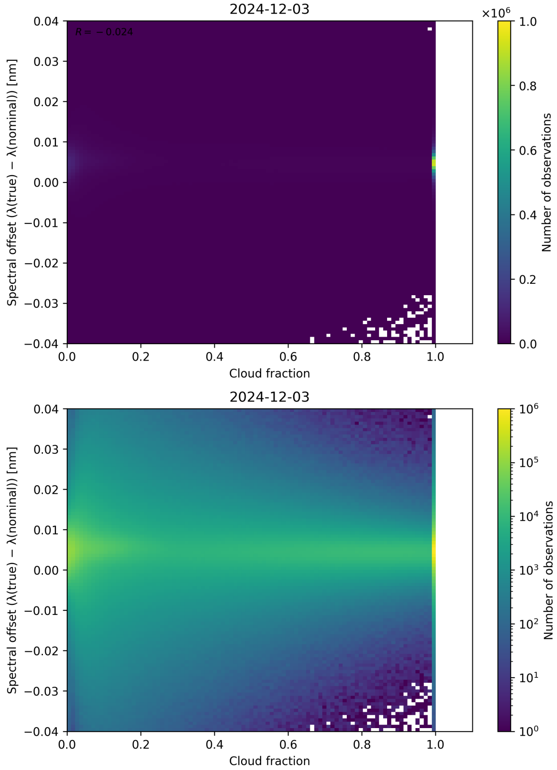
Figure 76: Scatter density plot of “Cloud fraction” against “Spectral offset ( \lambda_{\text{true}} - \lambda_{\text{nominal}} )” for 2024-12-02 to 2024-12-04.
