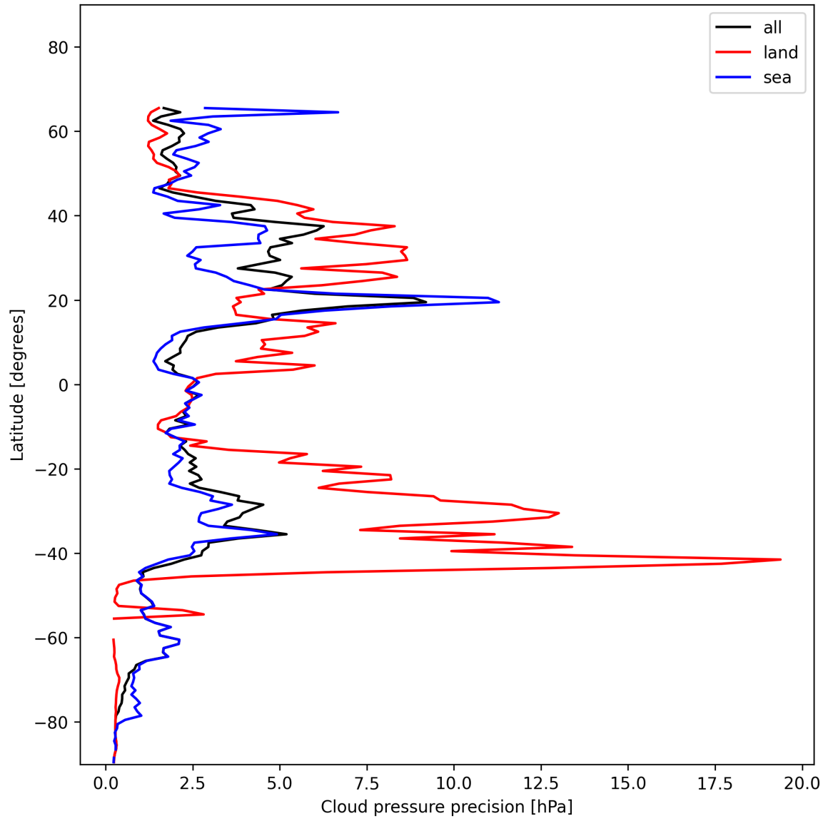
Figure 14: Zonal average of "Cloud pressure precision" for 2024-12-02 to 2024-12-04.
