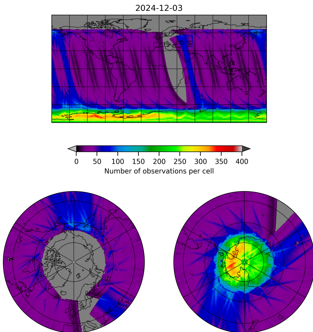
Figure 11: Map of the number of observations for 2024-12-02 to 2024-12-04
