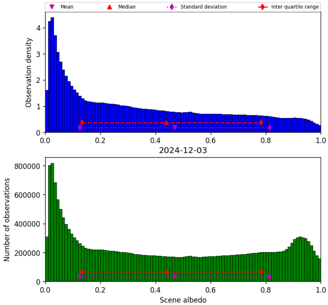
Figure 34: Histogram of “Scene albedo” for 2024-12-02 to 2024-12-04
