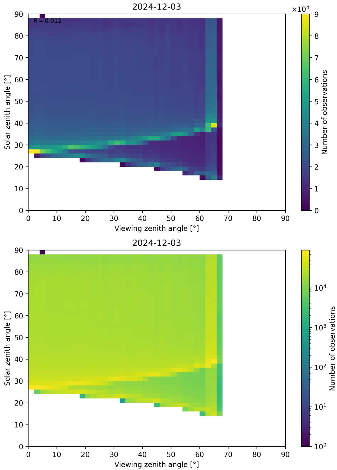
Figure 127: Scatter density plot of “Viewing zenith angle” against “Solar zenith angle” for 2024-12-02 to 2024-12-04.
