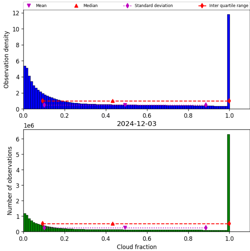
Figure 32: Histogram of “Cloud fraction” for 2024-12-02 to 2024-12-04
