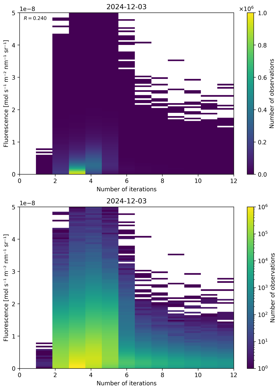
Figure 98: Scatter density plot of “Number of iterations” against “Fluorescence” for 2024-12-02 to 2024-12-04.
