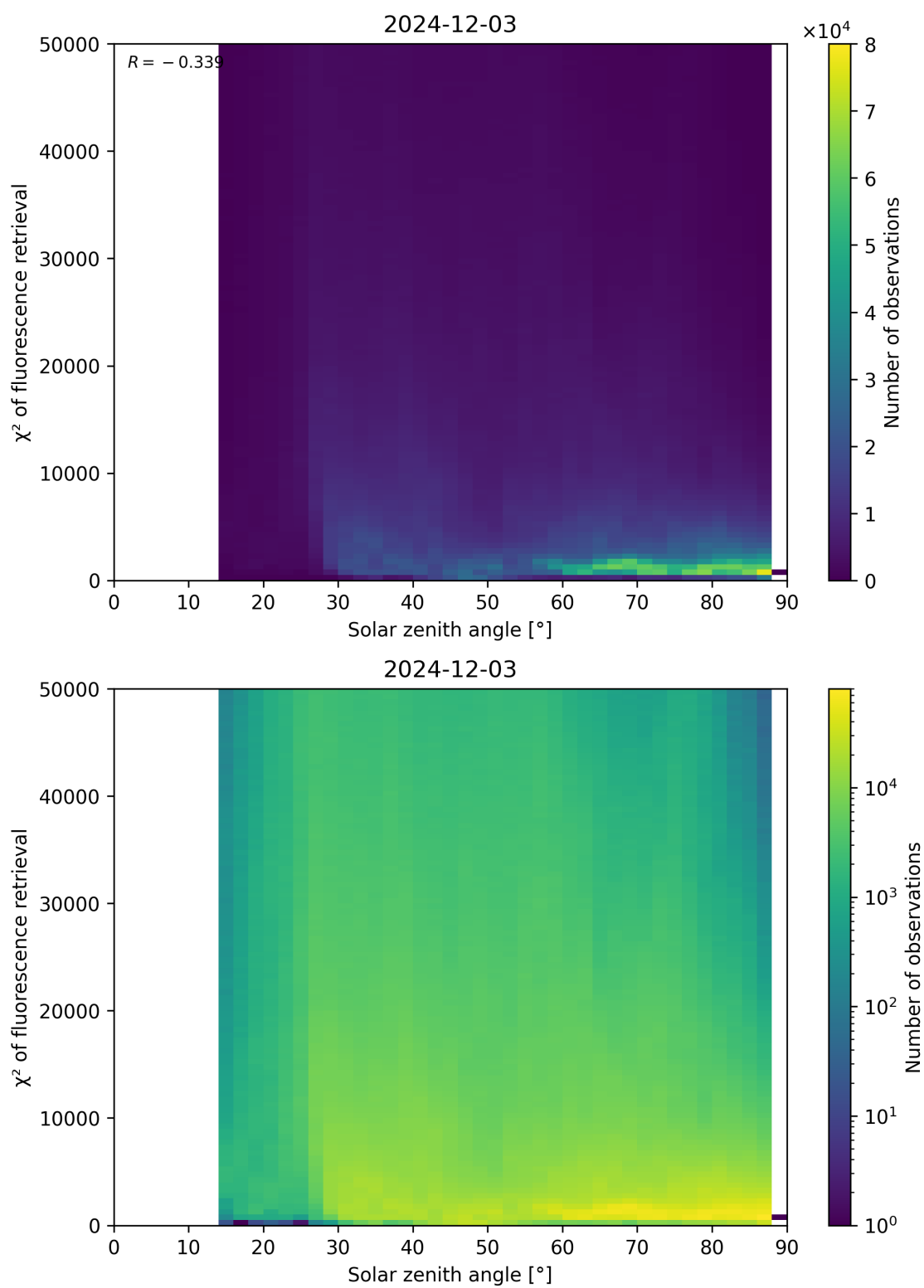
Figure 109: Scatter density plot of “Solar zenith angle” against “ \chi^2 of fluorescence retrieval” for 2024-12-02 to 2024-12-04.
