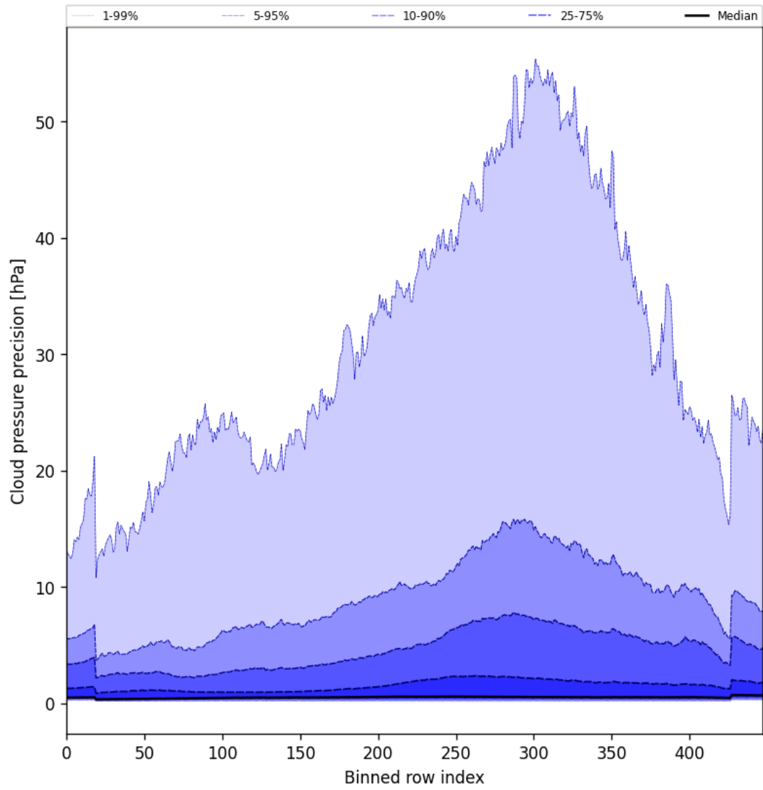
Figure 48: Along track statistics of “Cloud pressure precision” for 2024-12-02 to 2024-12-04
