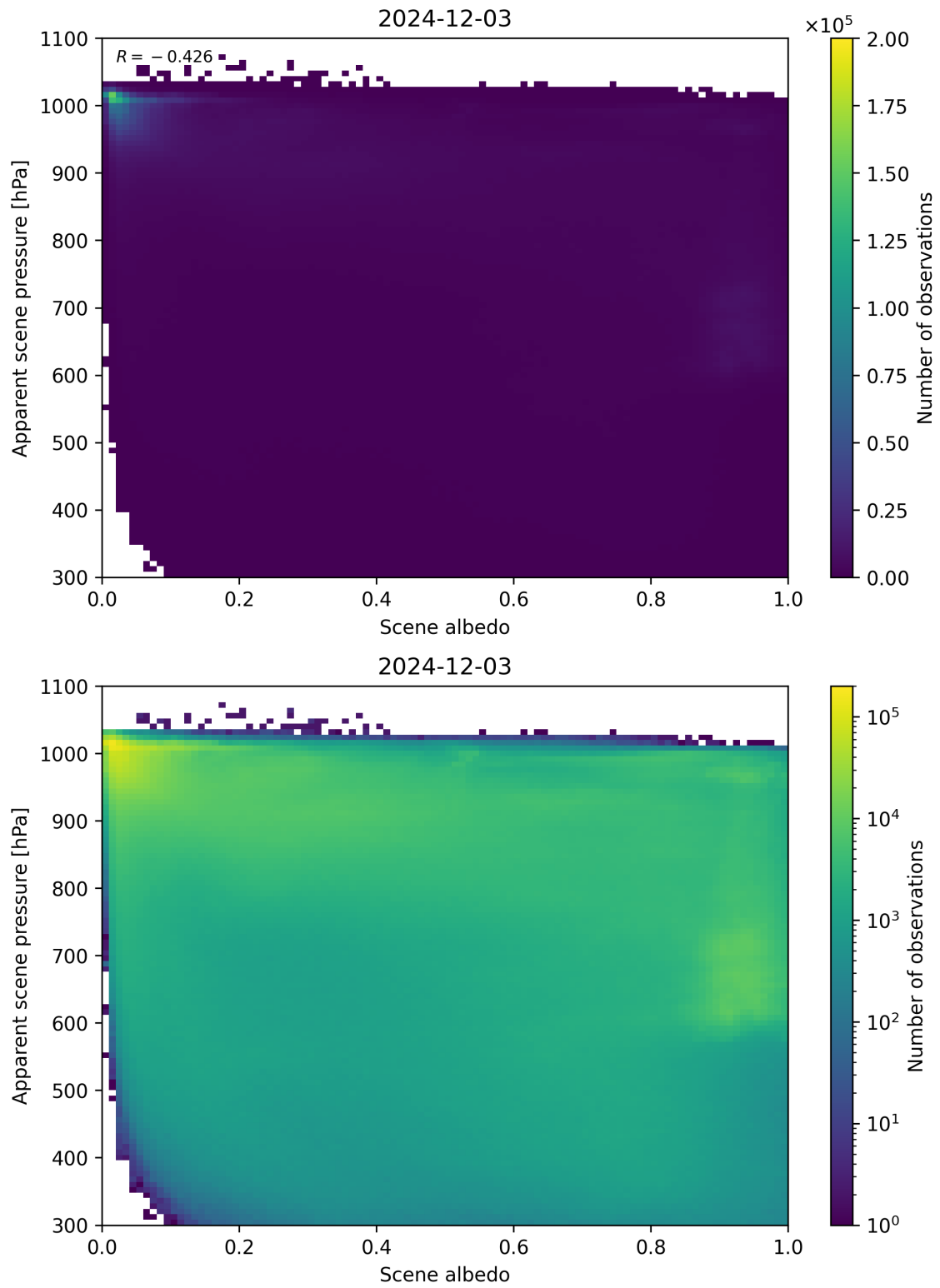
Figure 102: Scatter density plot of “Scene albedo” against “Apparent scene pressure” for 2024-12-02 to 2024-12-04.
