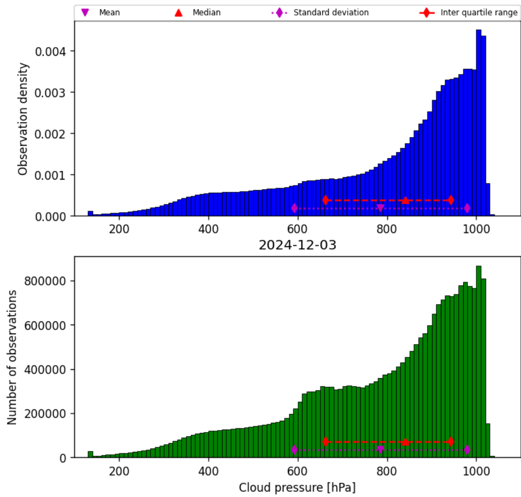
Figure 30: Histogram of “Cloud pressure” for 2024-12-02 to 2024-12-04
