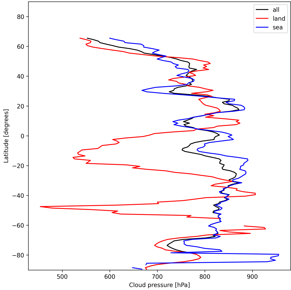
Figure 13: Zonal average of “Cloud pressure” for 2024-12-02 to 2024-12-04.
