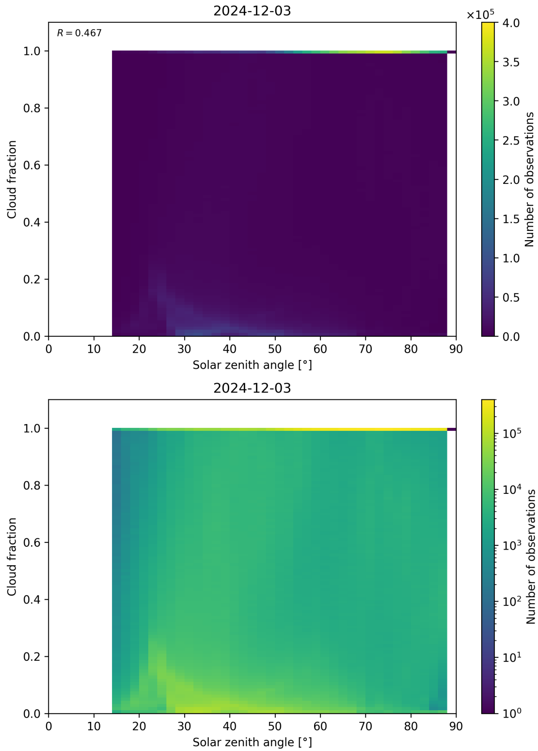
Figure 110: Scatter density plot of “Solar zenith angle” against “Cloud fraction” for 2024-12-02 to 2024-12-04.
