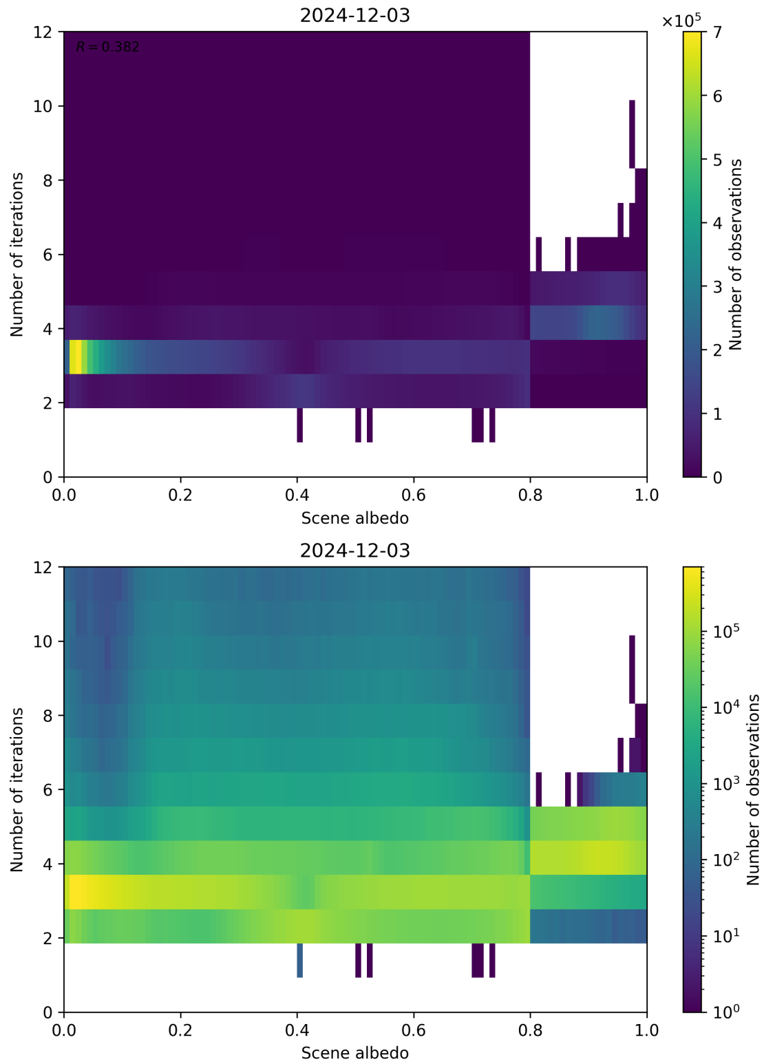
Figure 105: Scatter density plot of “Scene albedo” against “Number of iterations” for 2024-12-02 to 2024-12-04.
