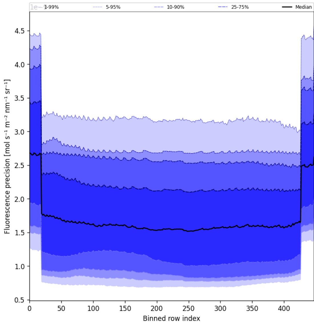
Figure 58: Along track statistics of “Fluorescence precision” for 2024-12-02 to 2024-12-04
