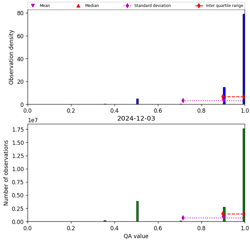
Figure 29: Histogram of “QA value” for 2024-12-02 to 2024-12-04
