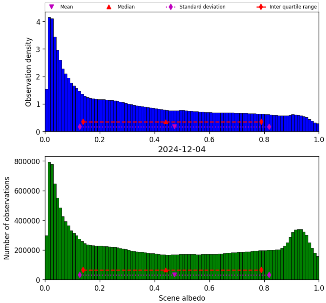
Figure 34: Histogram of “Scene albedo” for 2024-12-03 to 2024-12-05
