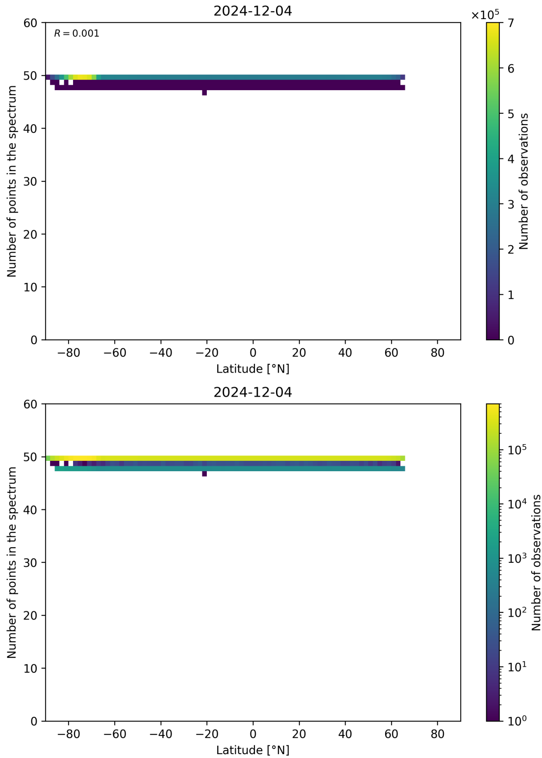
Figure 94: Scatter density plot of “Latitude” against “Number of points in the spectrum” for 2024-12-03 to 2024-12-05.
