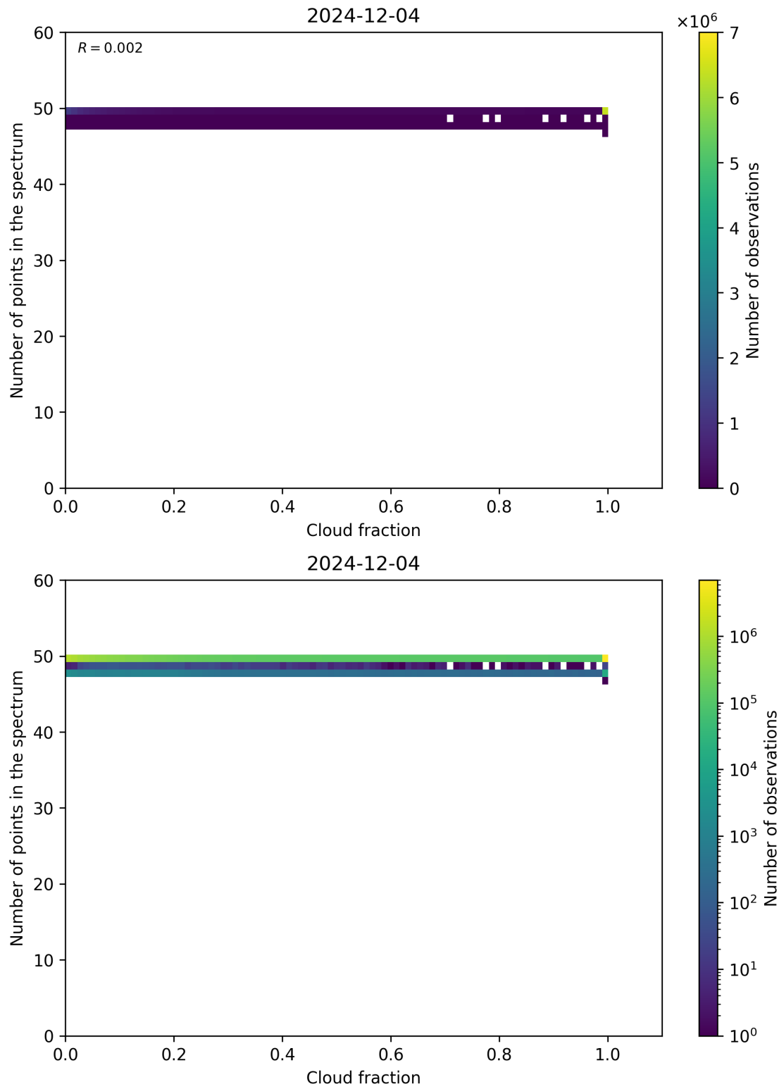
Figure 74: Scatter density plot of “Cloud fraction” against “Number of points in the spectrum” for 2024-12-03 to 2024-12-05.
