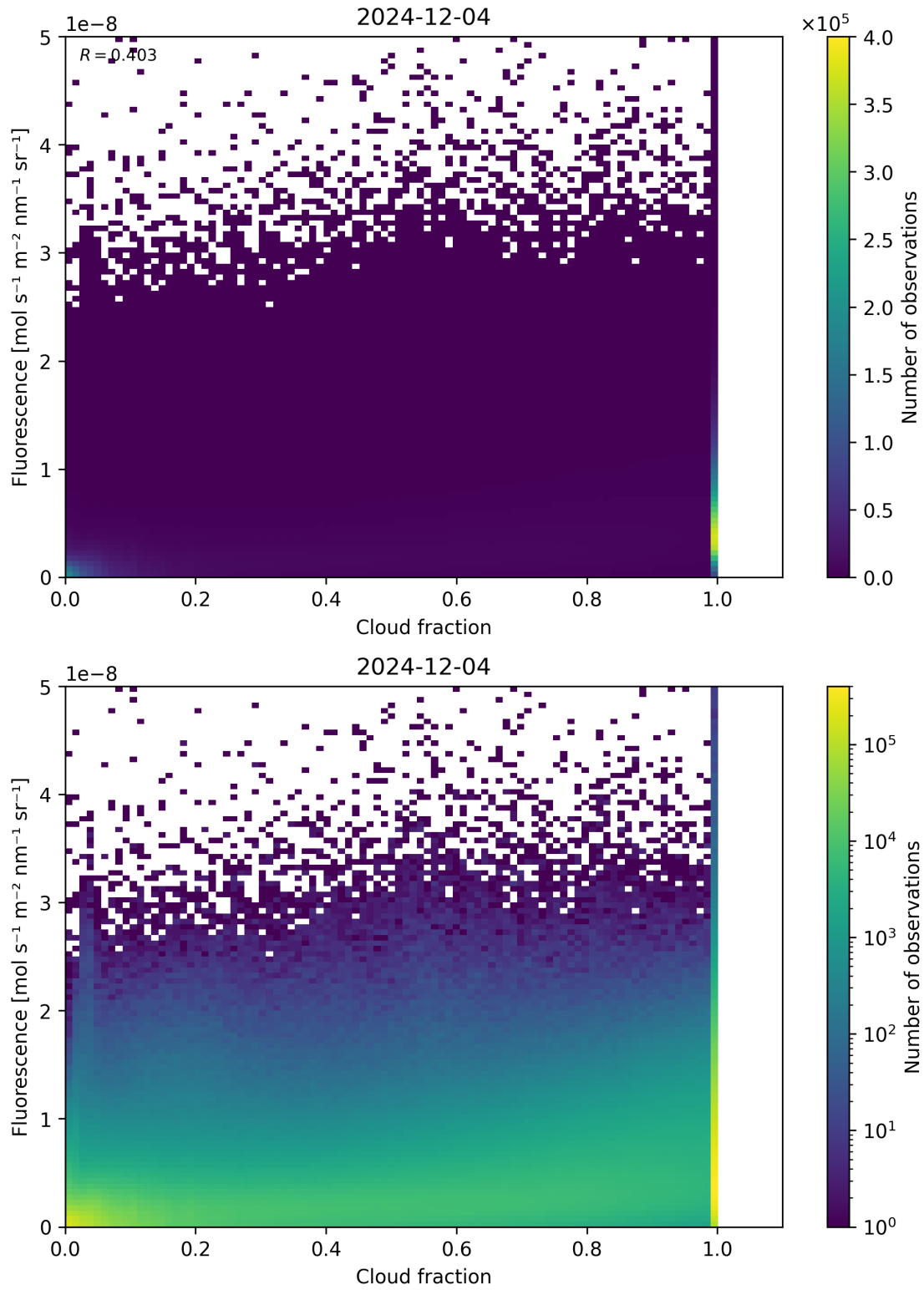
Figure 72: Scatter density plot of “Cloud fraction” against “Fluorescence” for 2024-12-03 to 2024-12-05.
