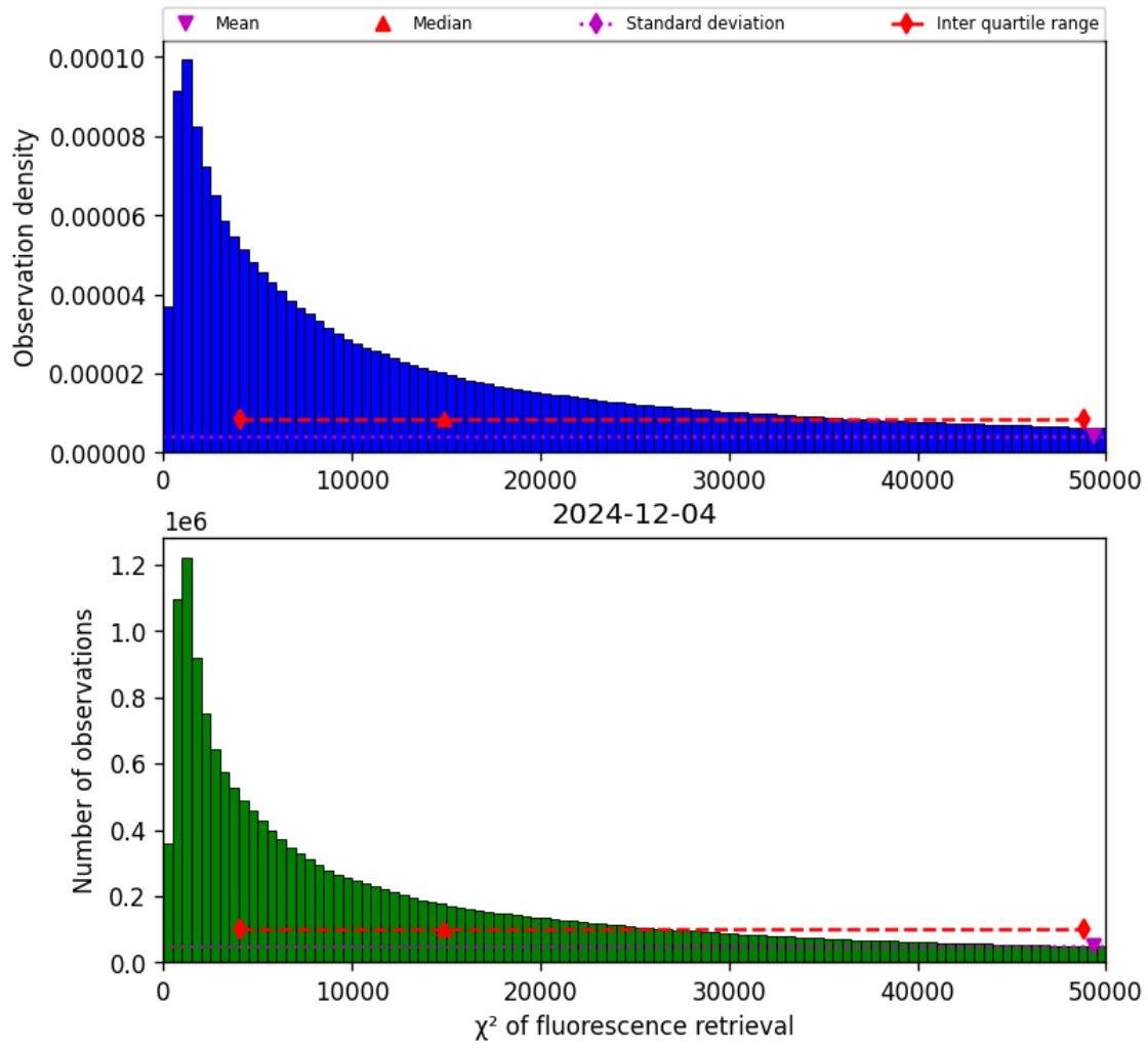
Figure 42: Histogram of “ \chi^2 of fluorescence retrieval” for 2024-12-03 to 2024-12-05
