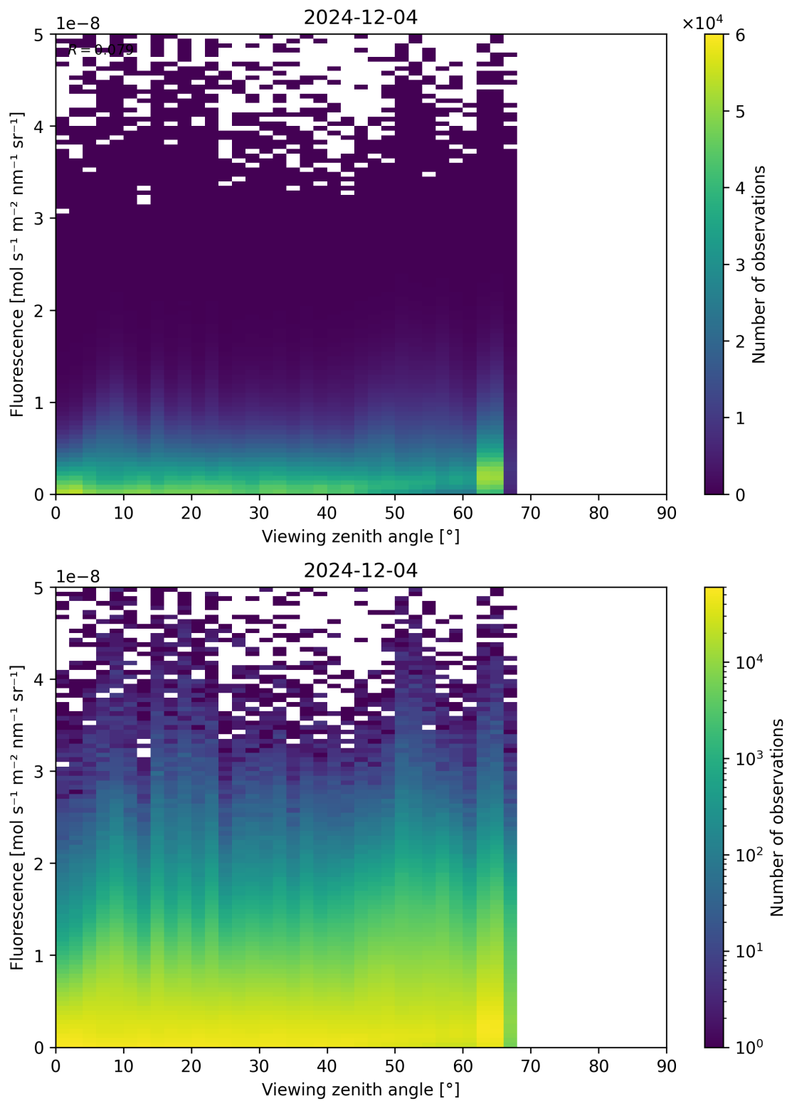
Figure 122: Scatter density plot of “Viewing zenith angle” against “Fluorescence” for 2024-12-03 to 2024-12-05.
