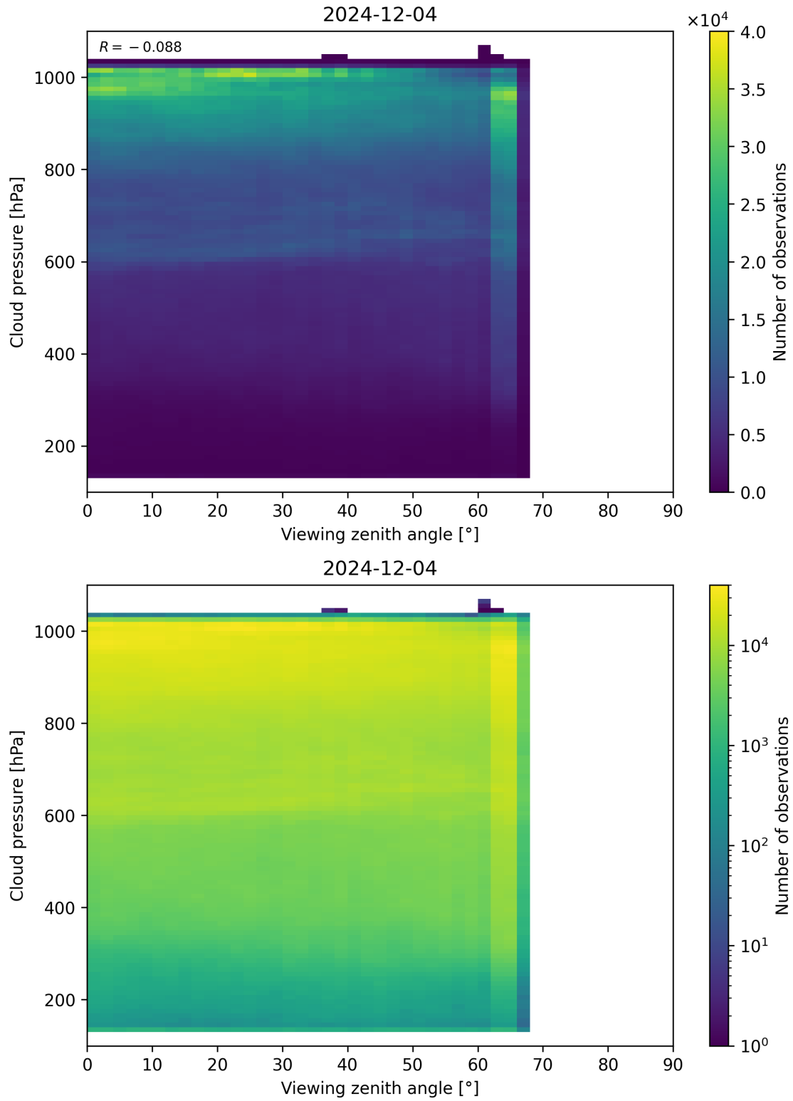
Figure 121: Scatter density plot of “Viewing zenith angle” against “Cloud pressure” for 2024-12-03 to 2024-12-05.
