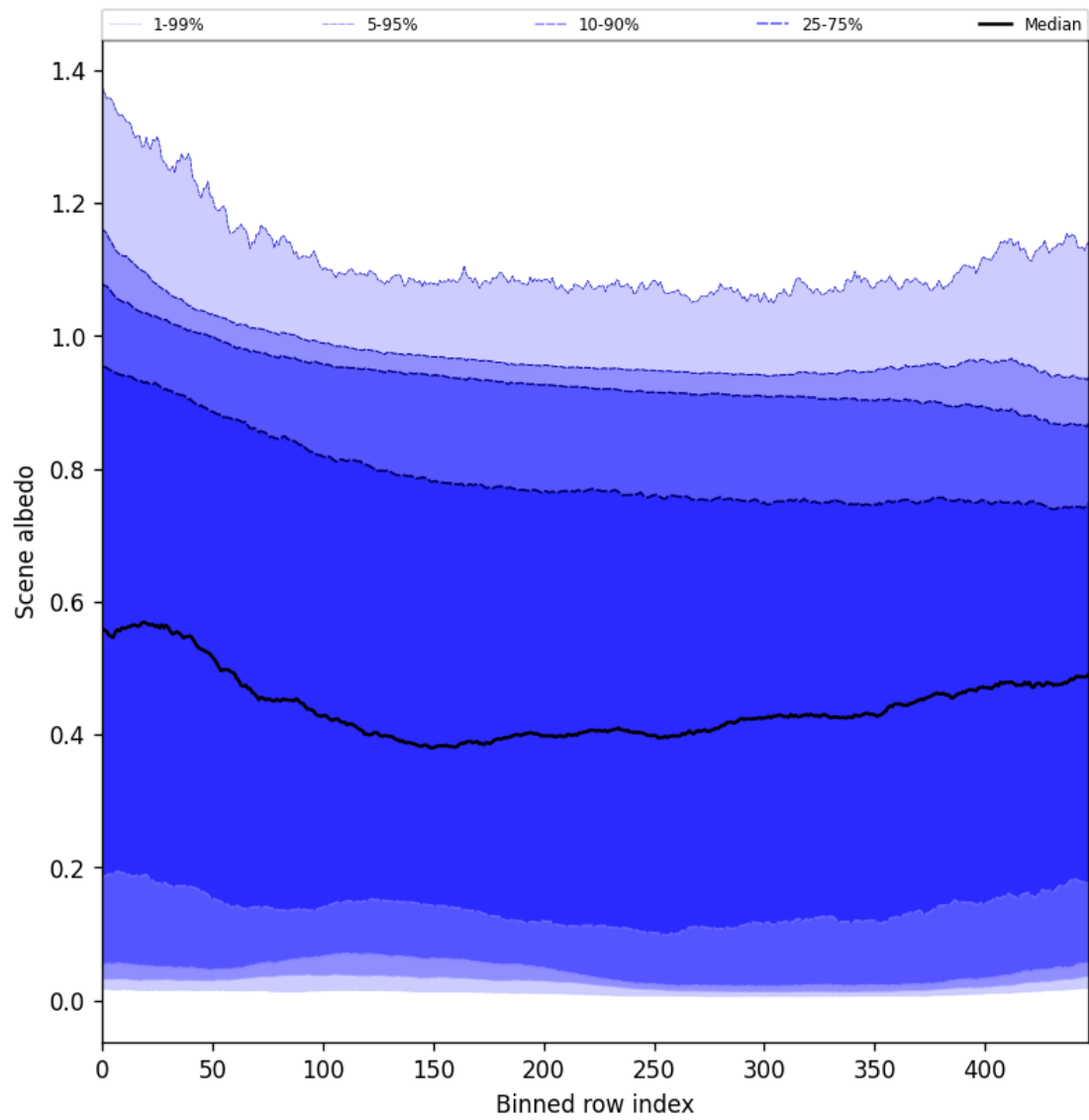
Figure 51: Along track statistics of “Scene albedo” for 2024-12-03 to 2024-12-05
