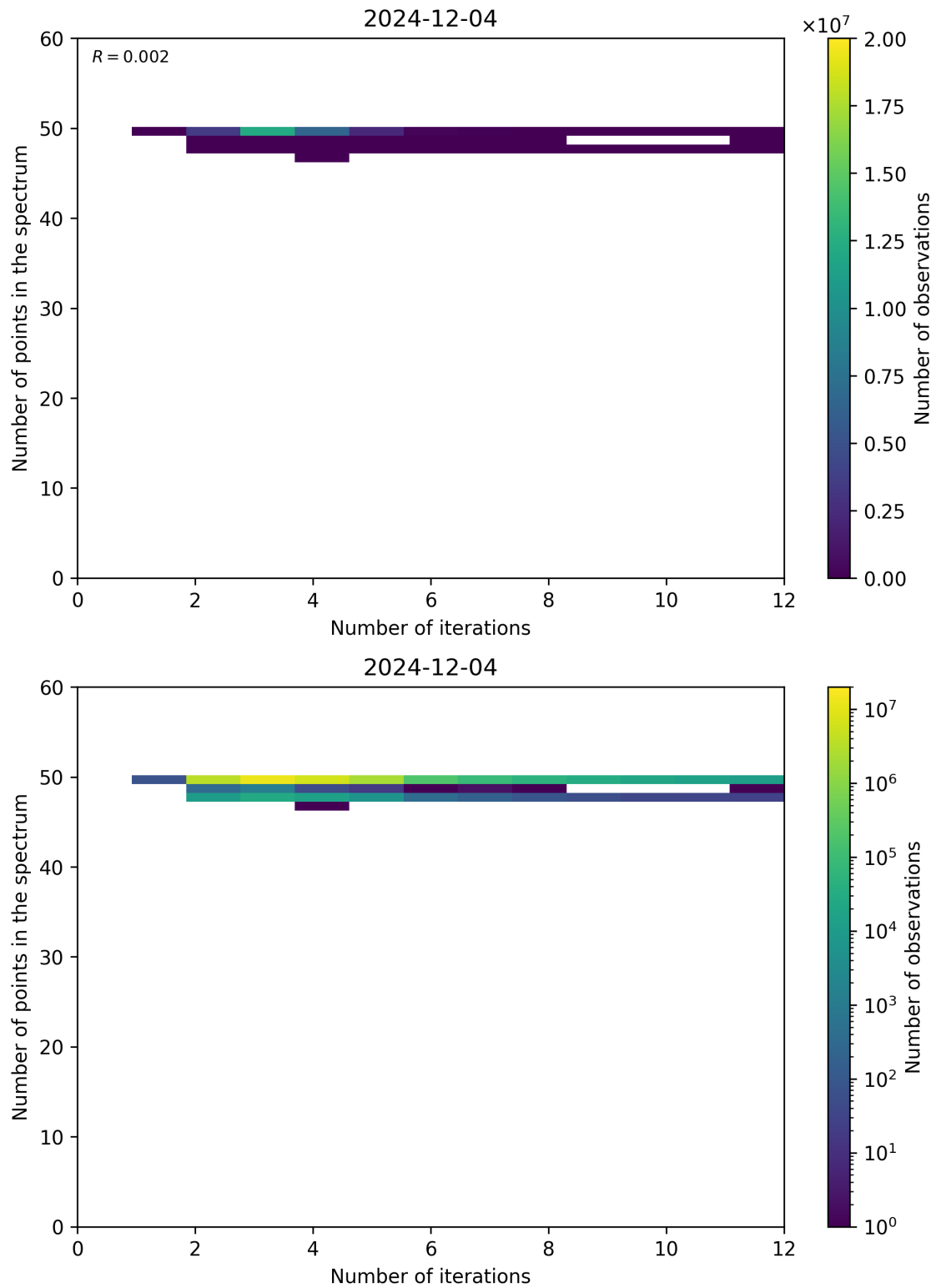
Figure 99: Scatter density plot of “Number of iterations” against “Number of points in the spectrum” for 2024-12-03 to 2024-12-05.
