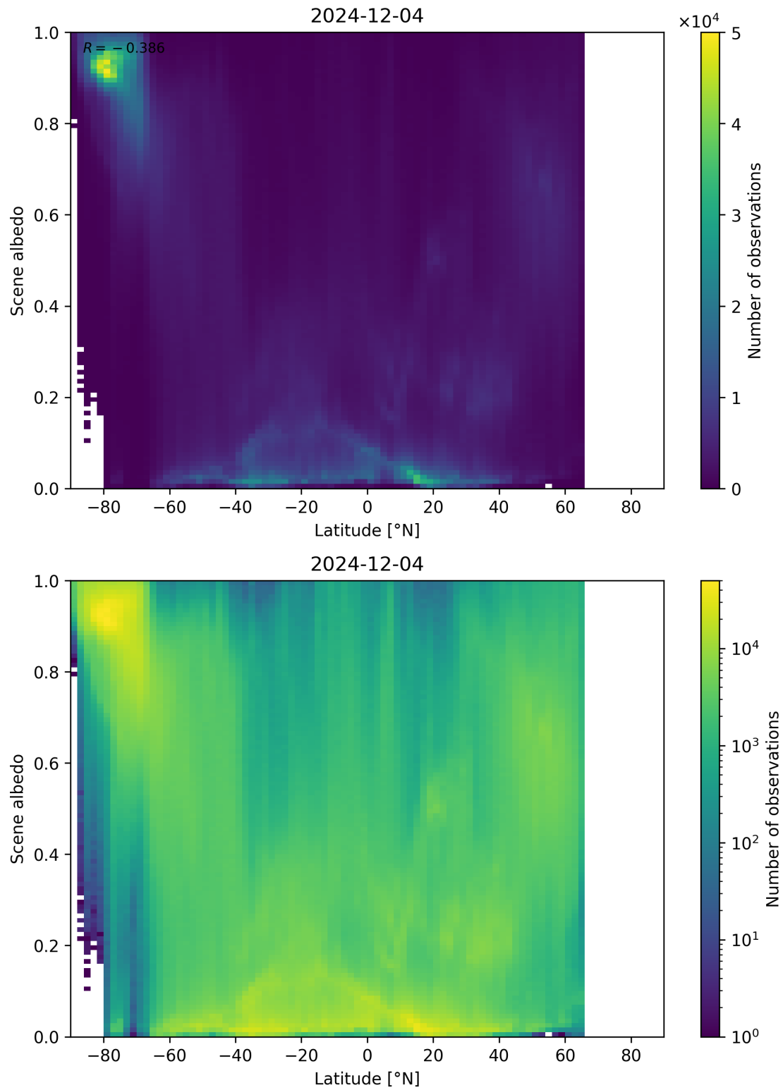
Figure 95: Scatter density plot of “Latitude” against “Scene albedo” for 2024-12-03 to 2024-12-05.
