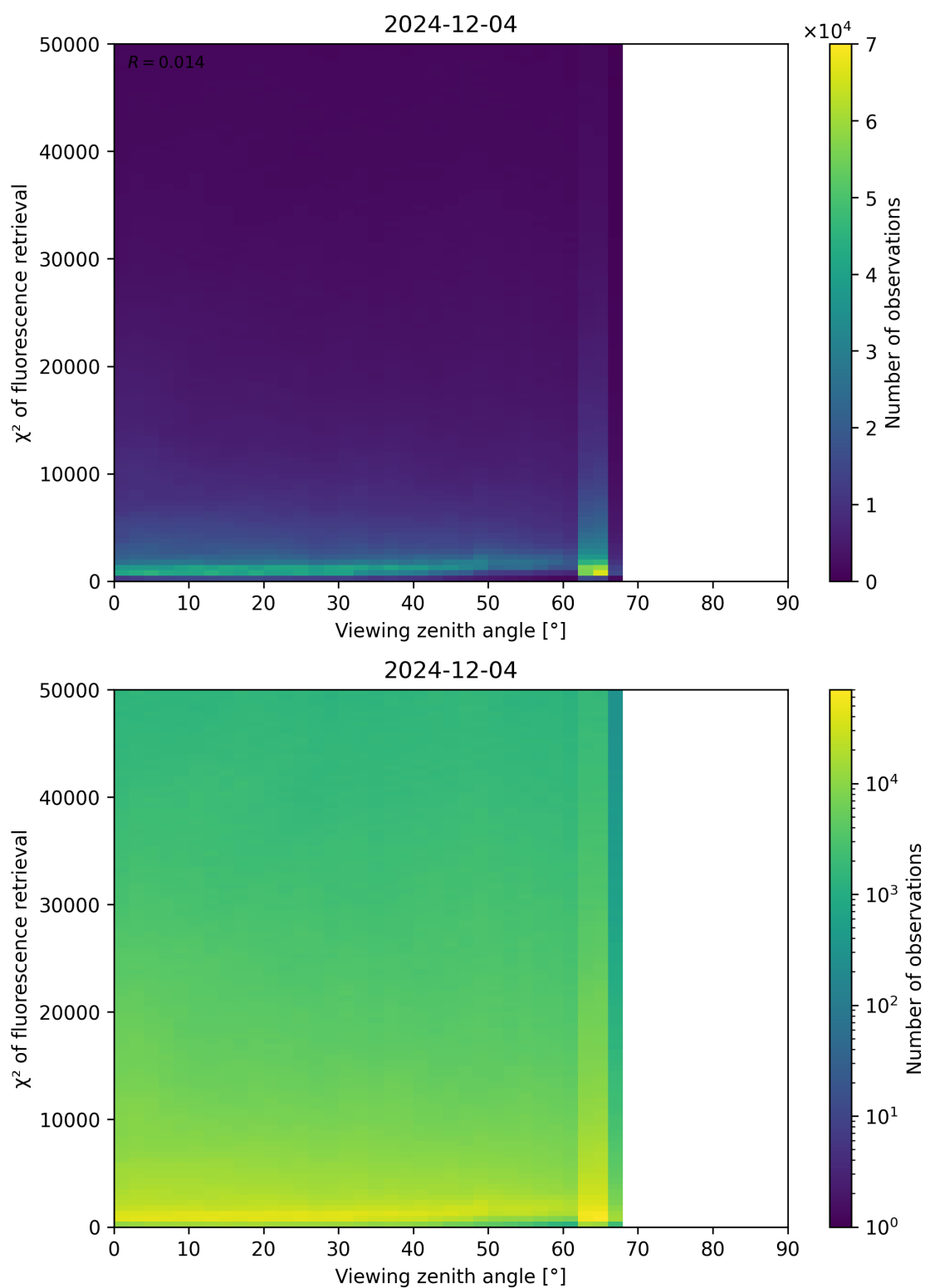
Figure 119: Scatter density plot of “Viewing zenith angle” against “ \chi^2 of fluorescence retrieval” for 2024-12-03 to 2024-12-05.
