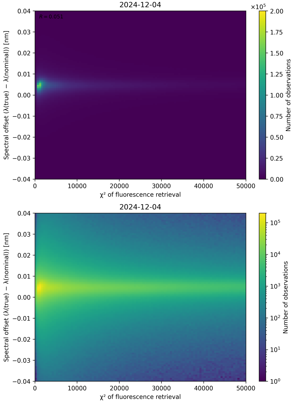
Figure 69: Scatter density plot of “ \chi^2 of fluorescence retrieval” against “Spectral offset ( \lambda_{\text{true}} - \lambda_{\text{nominal}} )” for 2024-12-03 to 2024-12-05.
