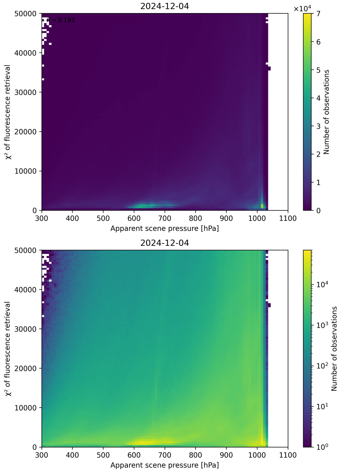
Figure 63: Scatter density plot of “Apparent scene pressure” against “ \chi^2 of fluorescence retrieval” for 2024-12-03 to 2024-12-05.
