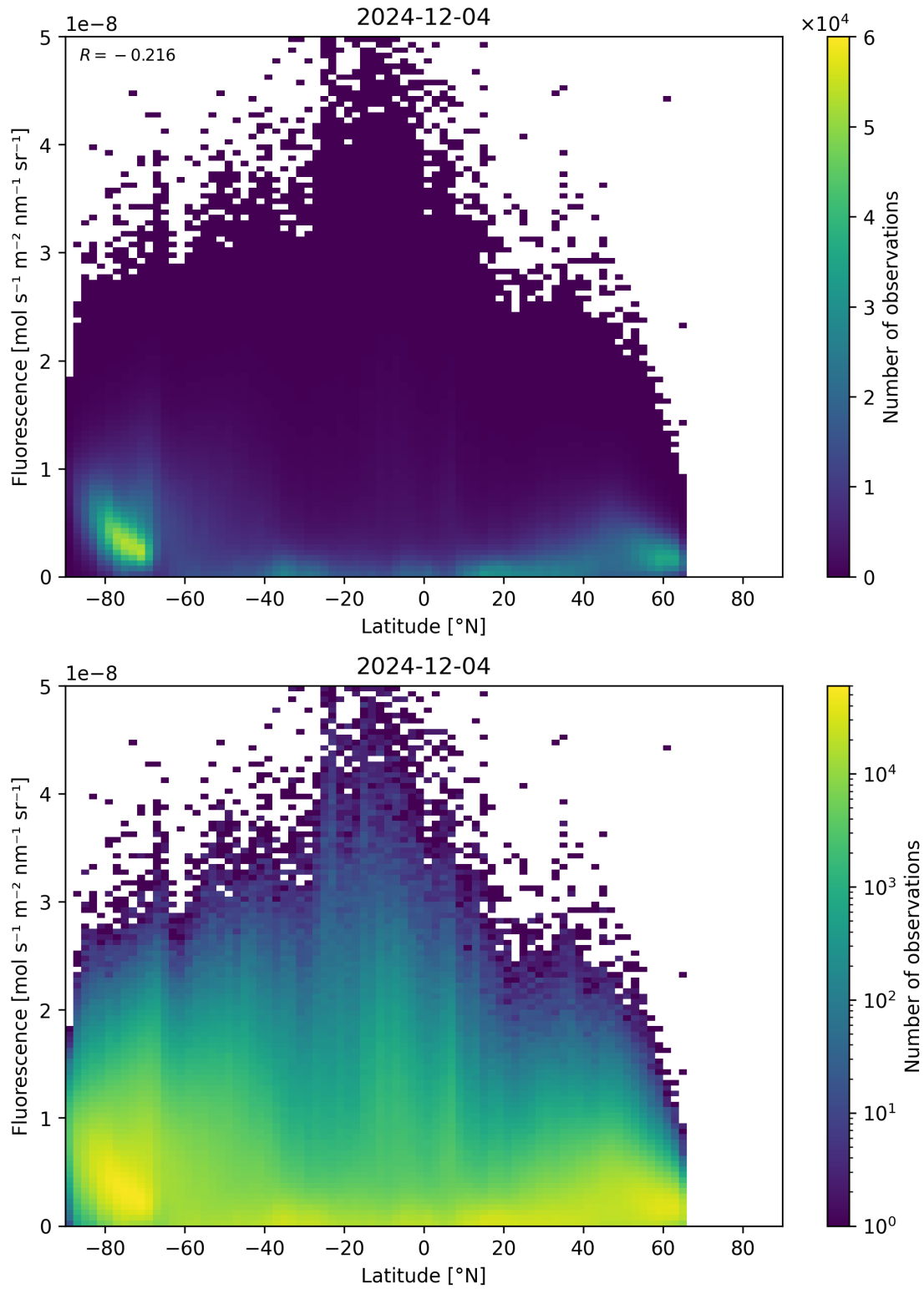
Figure 92: Scatter density plot of “Latitude” against “Fluorescence” for 2024-12-03 to 2024-12-05.
