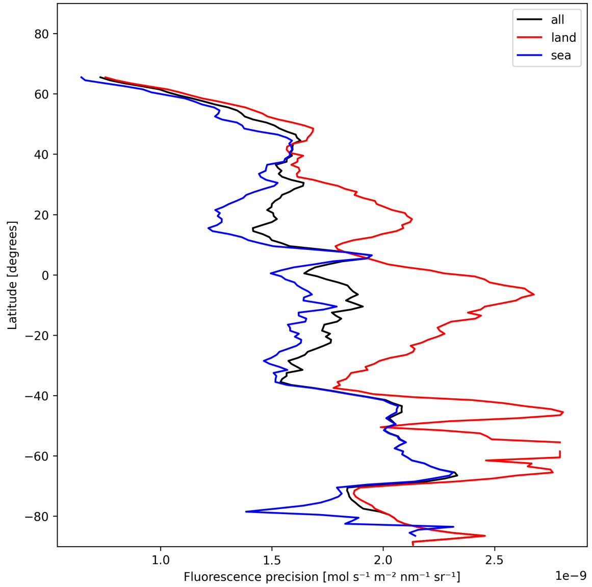
Figure 24: Zonal average of “Fluorescence precision” for 2024-12-03 to 2024-12-05.
