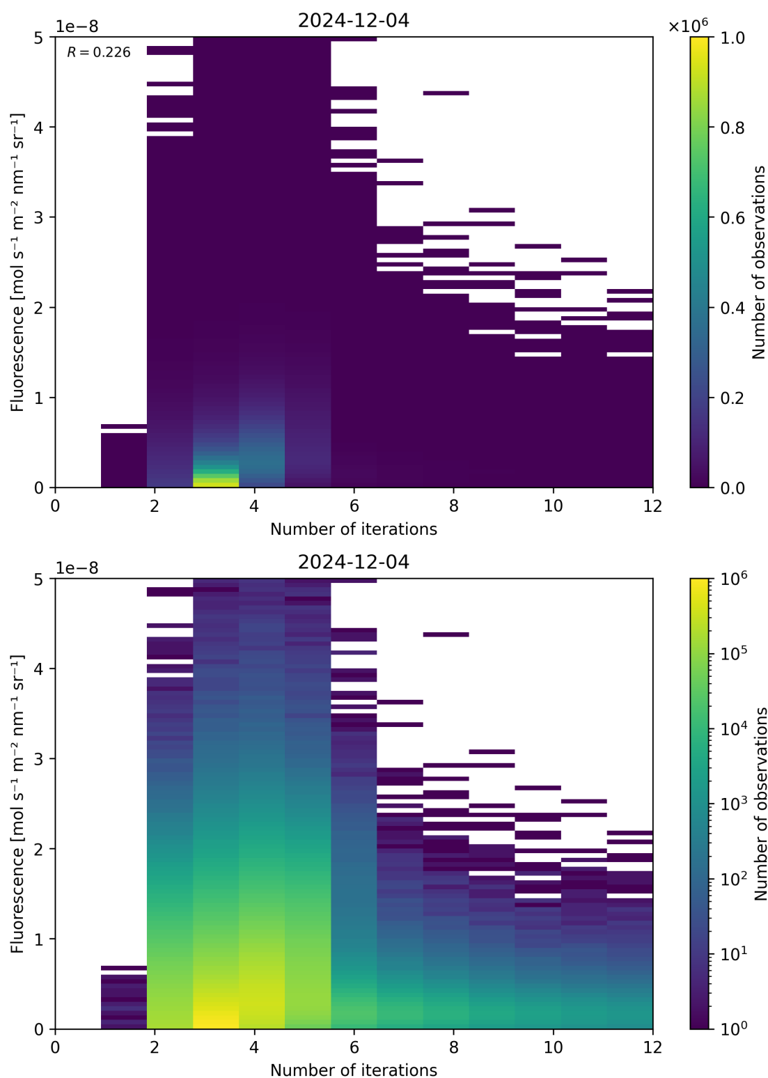
Figure 98: Scatter density plot of “Number of iterations” against “Fluorescence” for 2024-12-03 to 2024-12-05.
