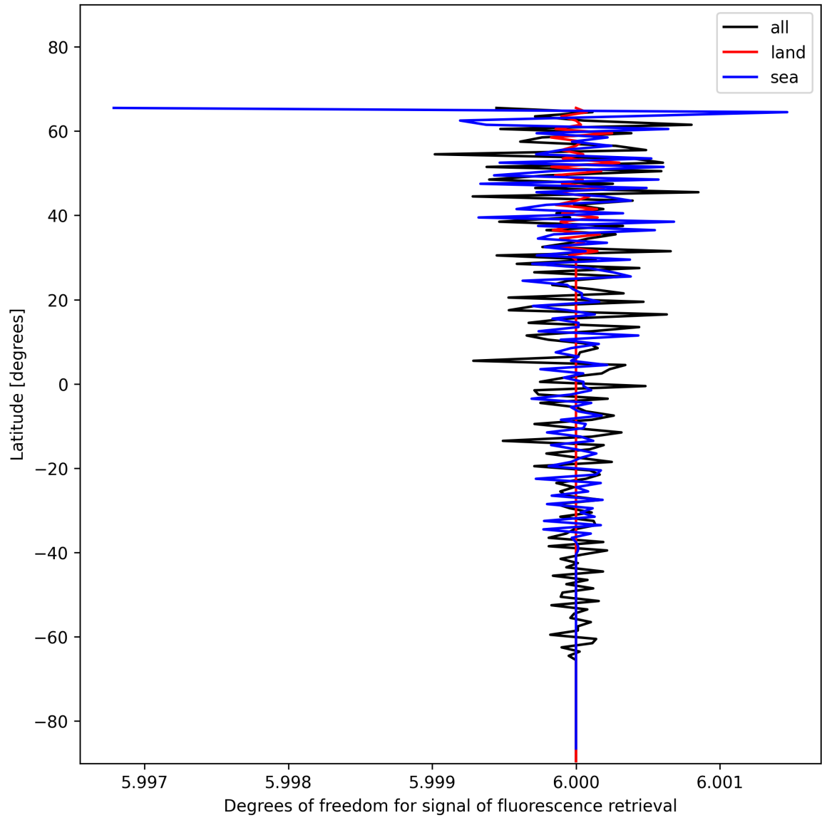
Figure 26: Zonal average of “Degrees of freedom for signal of fluorescence retrieval” for 2024-12-03 to 2024-12-05.
