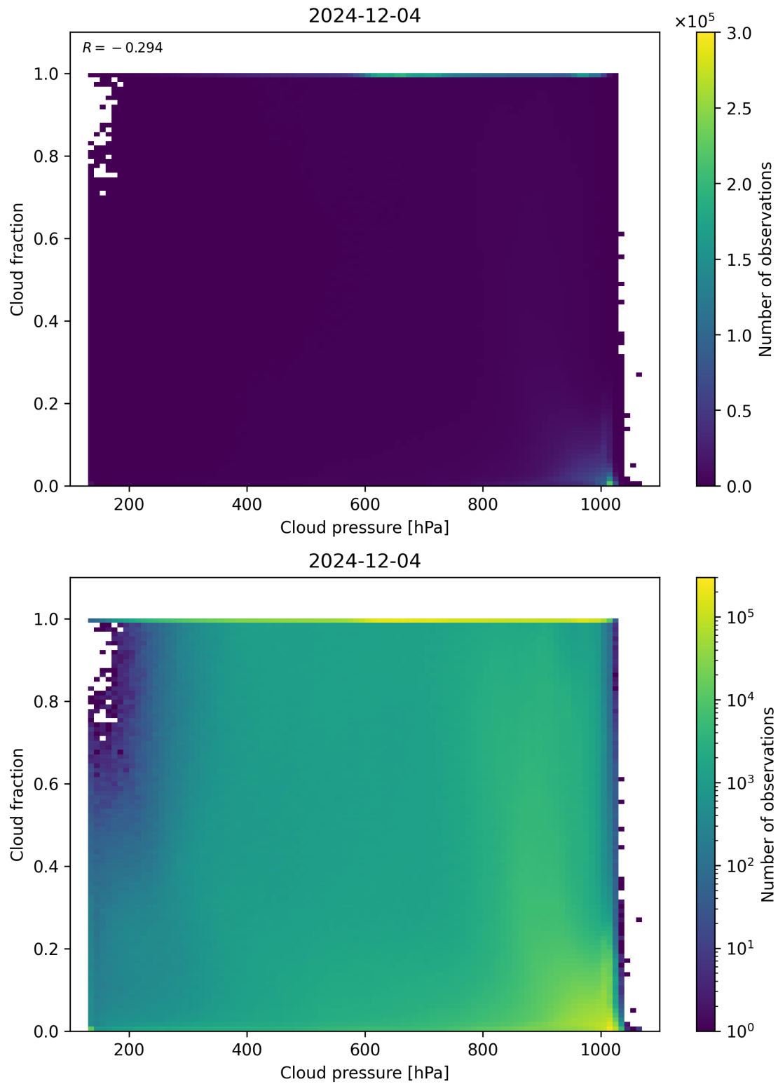
Figure 79: Scatter density plot of “Cloud pressure” against “Cloud fraction” for 2024-12-03 to 2024-12-05.
