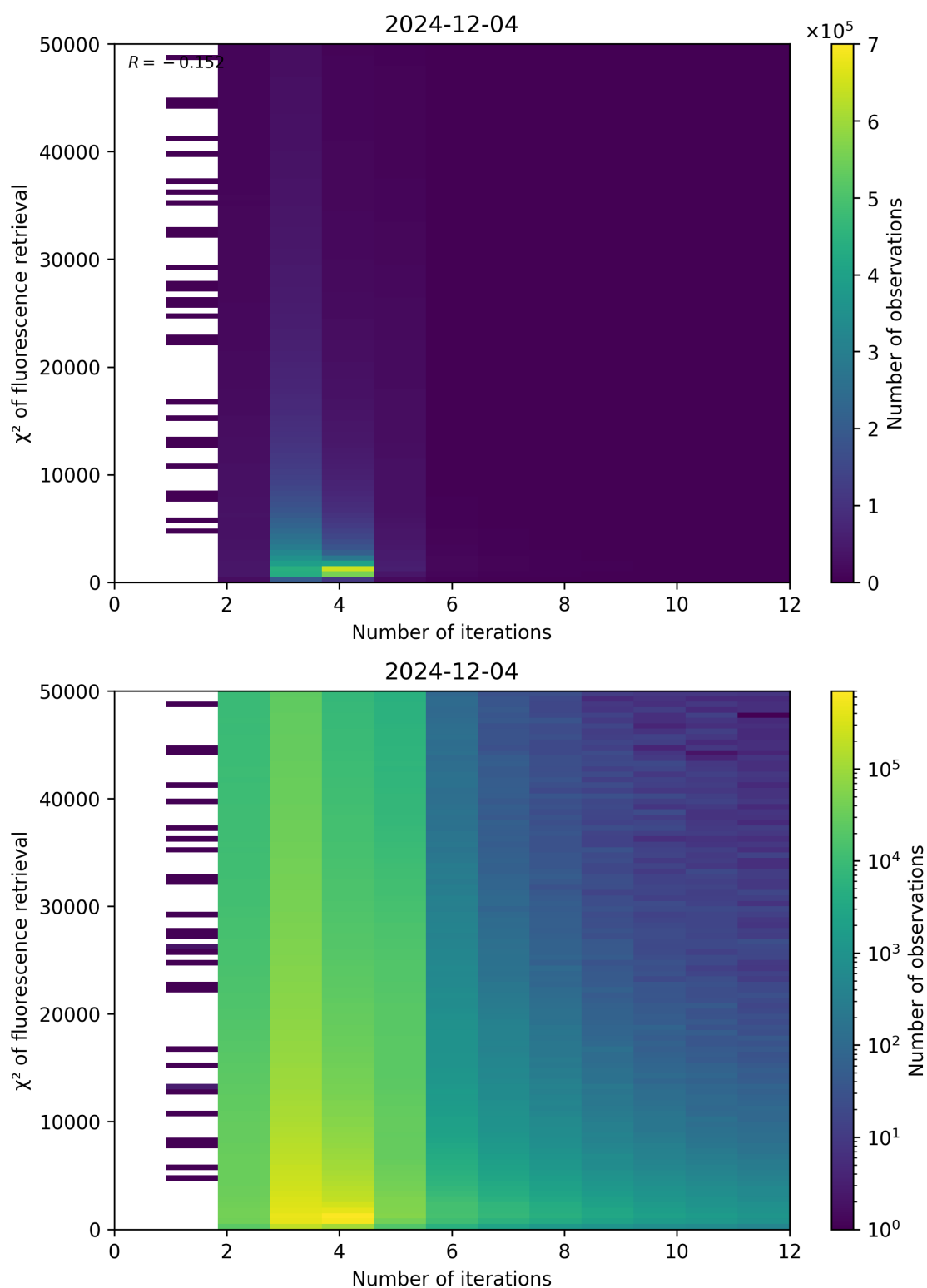
Figure 97: Scatter density plot of “Number of iterations” against “ \chi^2 of fluorescence retrieval” for 2024-12-03 to 2024-12-05.
