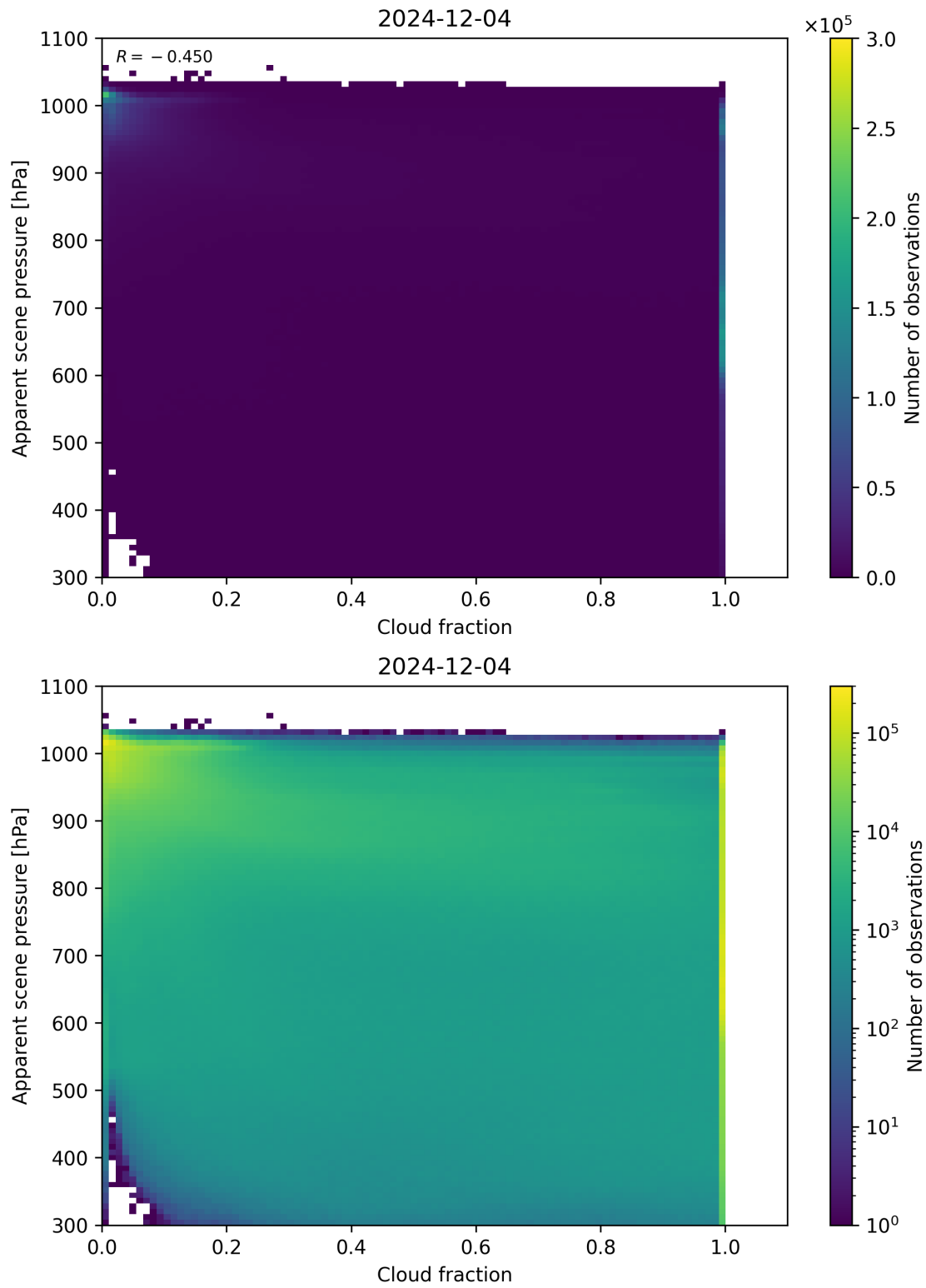
Figure 70: Scatter density plot of “Cloud fraction” against “Apparent scene pressure” for 2024-12-03 to 2024-12-05.
