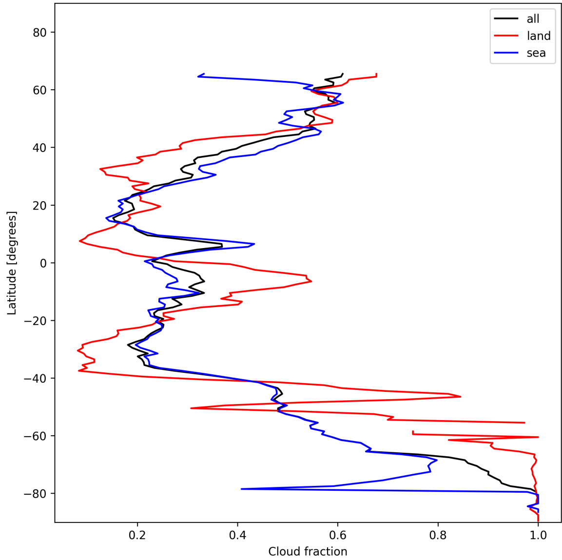
Figure 15: Zonal average of “Cloud fraction” for 2024-12-03 to 2024-12-05.
