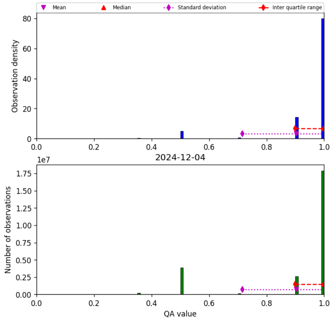
Figure 29: Histogram of “QA value” for 2024-12-03 to 2024-12-05
