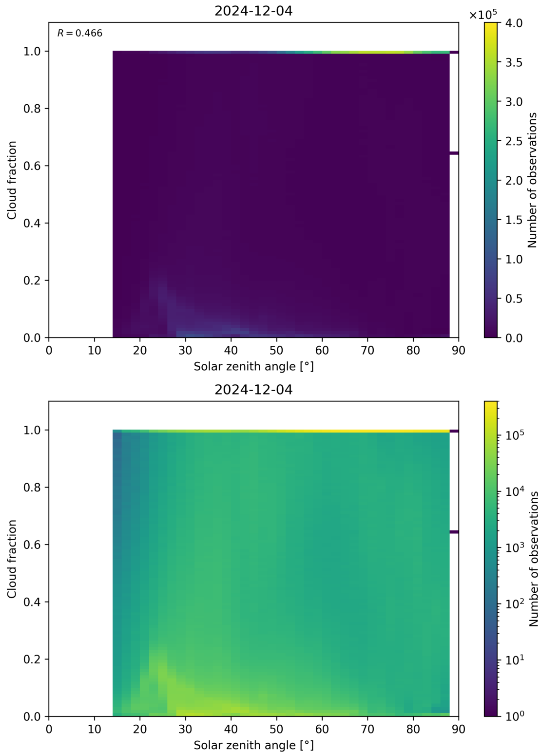
Figure 110: Scatter density plot of “Solar zenith angle” against “Cloud fraction” for 2024-12-03 to 2024-12-05.
