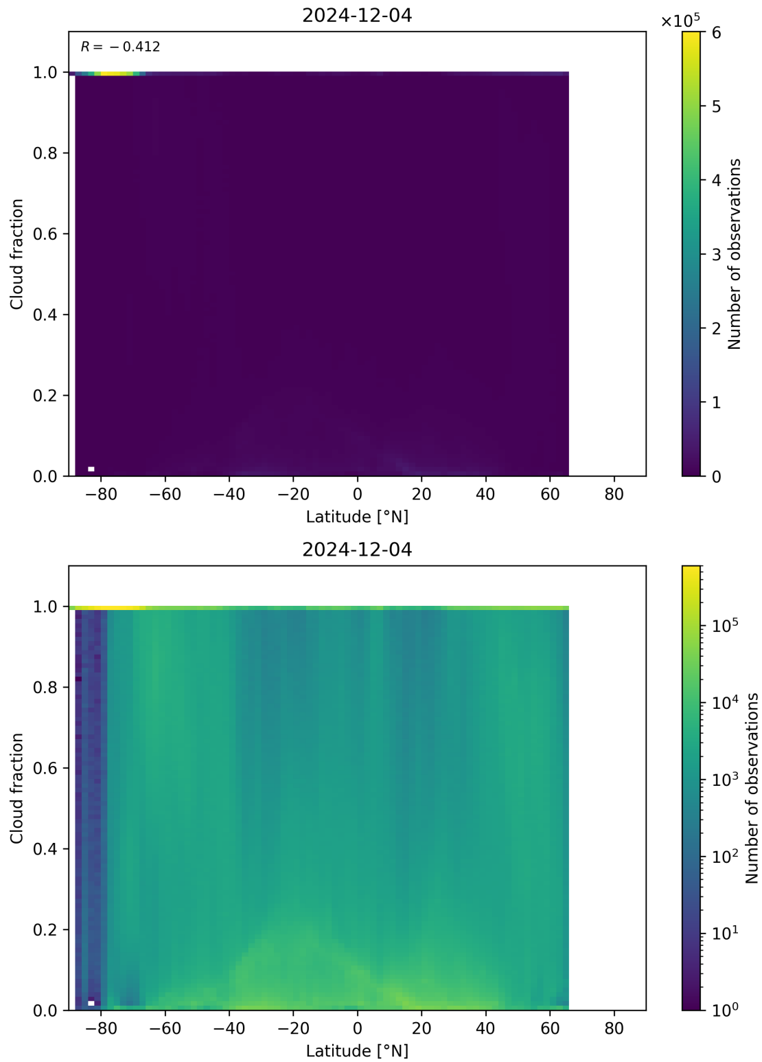
Figure 90: Scatter density plot of “Latitude” against “Cloud fraction” for 2024-12-03 to 2024-12-05.
