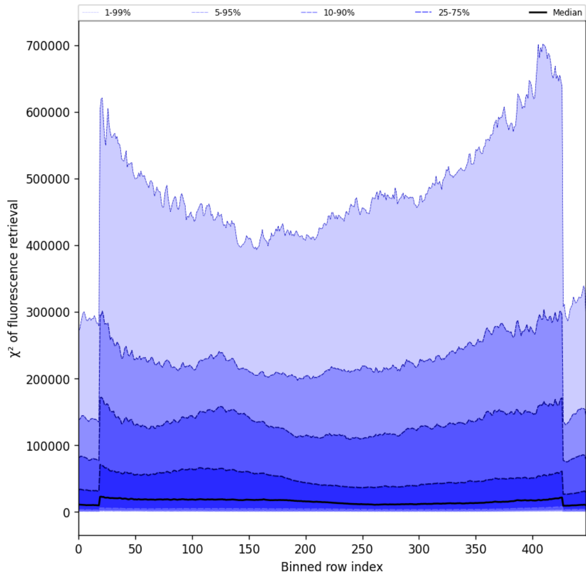
Figure 59: Along track statistics of “ \chi^2 of fluorescence retrieval” for 2024-12-03 to 2024-12-05
