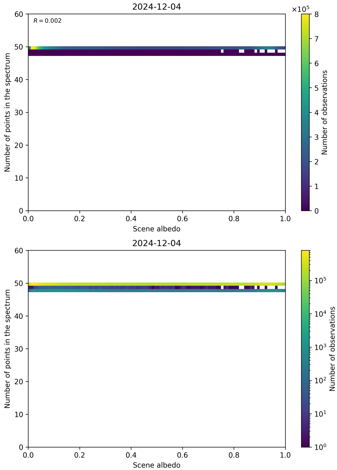
Figure 106: Scatter density plot of “Scene albedo” against “Number of points in the spectrum” for 2024-12-03 to 2024-12-05.
