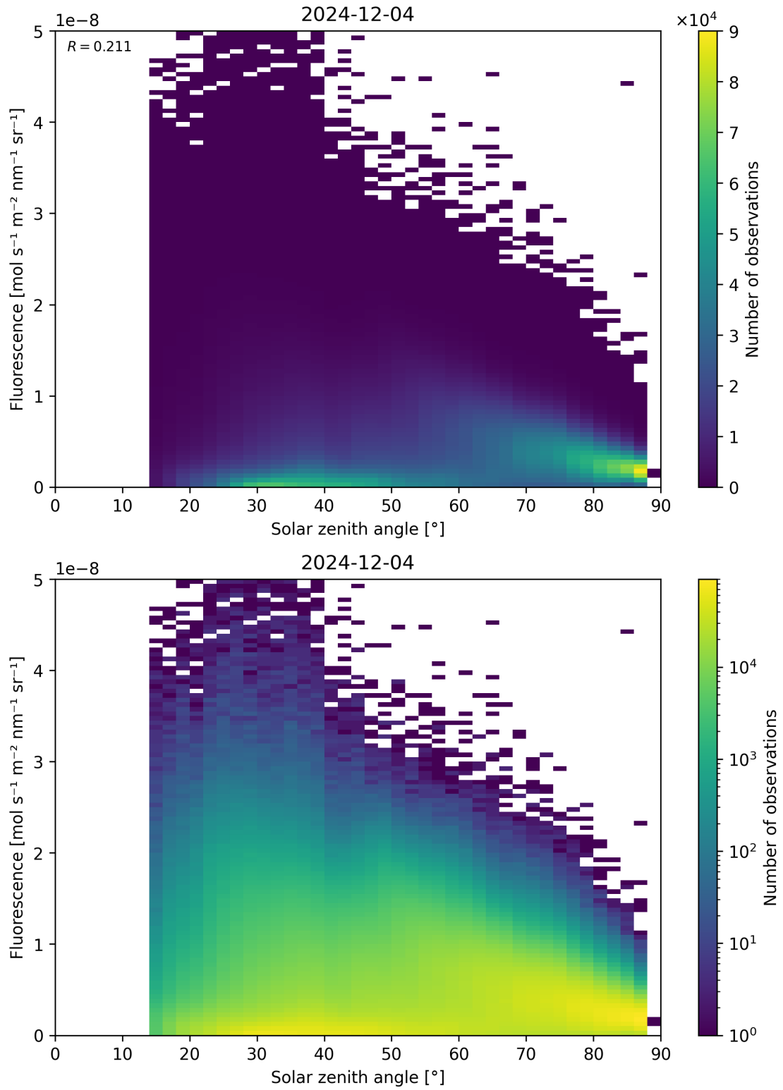
Figure 112: Scatter density plot of “Solar zenith angle” against “Fluorescence” for 2024-12-03 to 2024-12-05.
