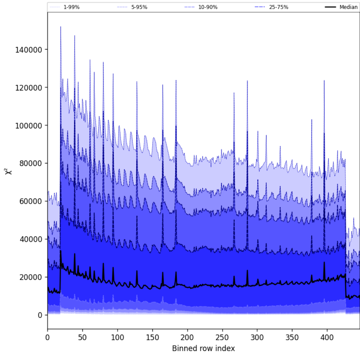
Figure 55: Along track statistics of “ \chi^2 ” for 2024-12-03 to 2024-12-05
