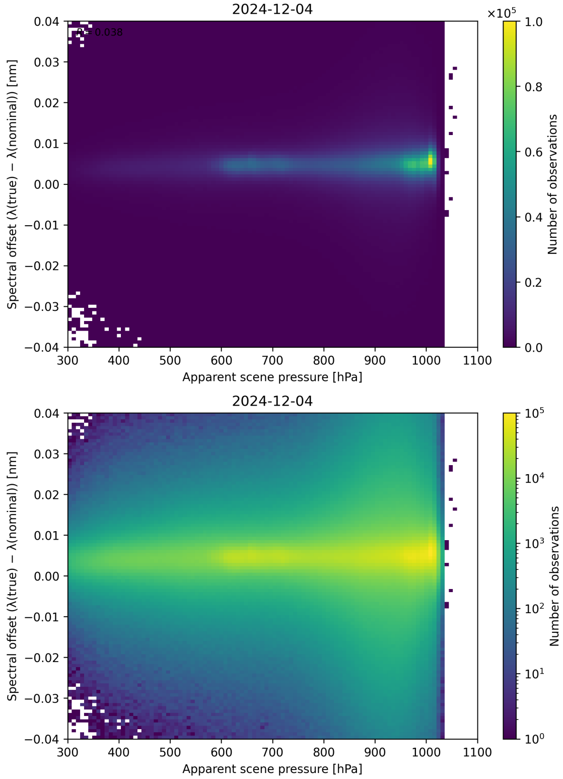
Figure 67: Scatter density plot of “Apparent scene pressure” against “Spectral offset ( \lambda_{\text{true}} - \lambda_{\text{nominal}} )” for 2024-12-03 to 2024-12-05.
