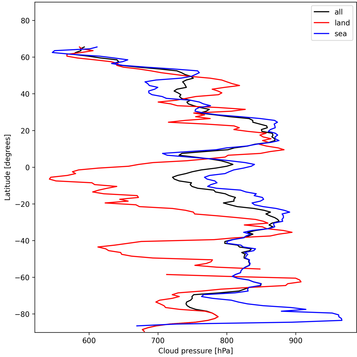
Figure 13: Zonal average of “Cloud pressure” for 2024-12-03 to 2024-12-05.
