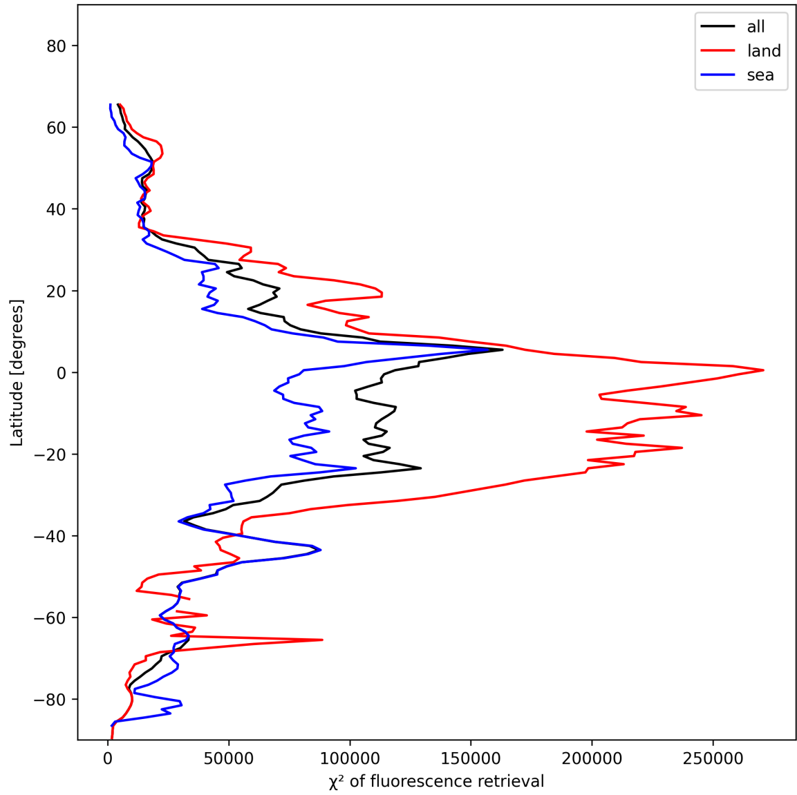
Figure 25: Zonal average of “ \chi^2 of fluorescence retrieval” for 2024-12-03 to 2024-12-05.
