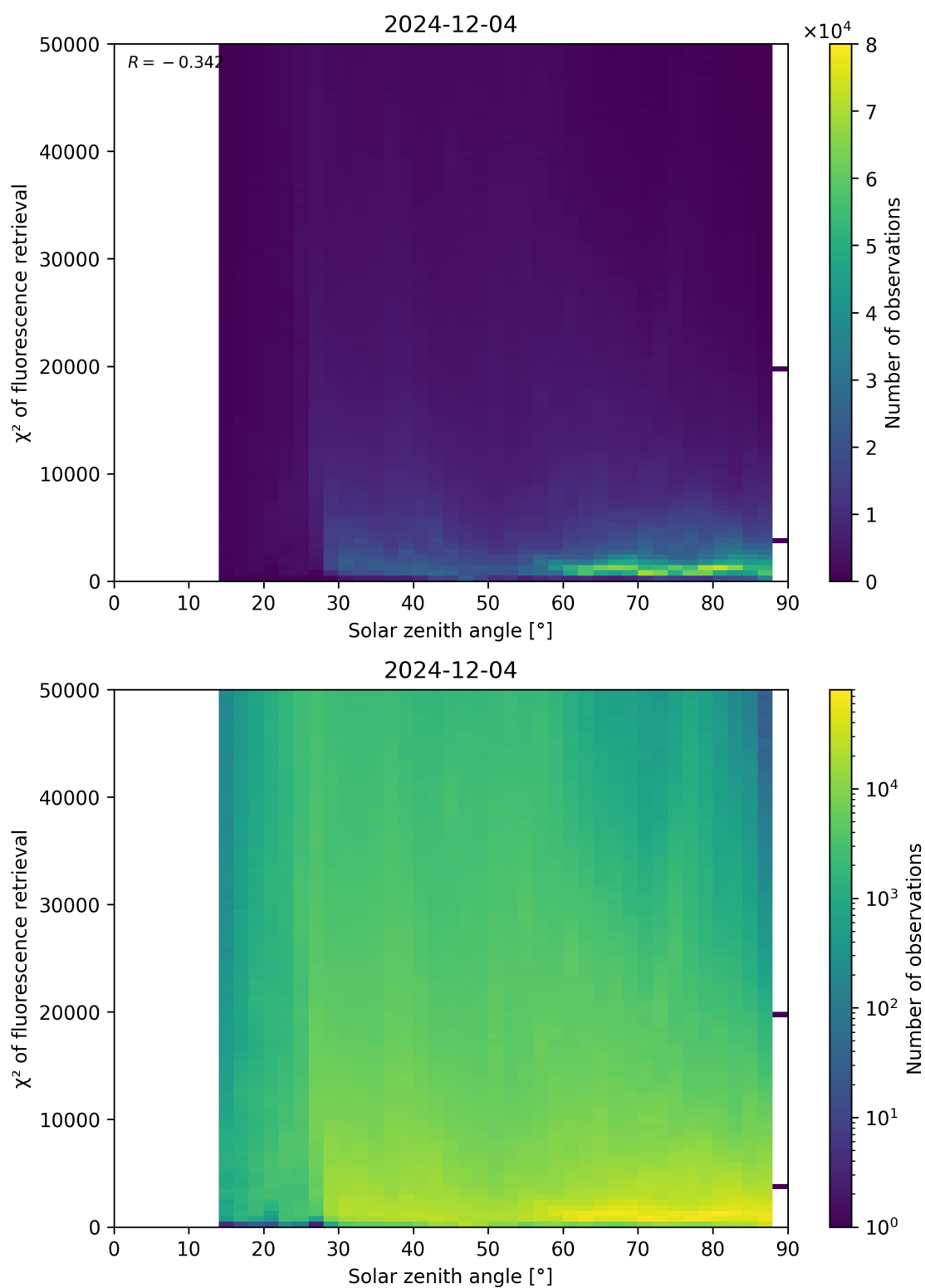
Figure 109: Scatter density plot of “Solar zenith angle” against “ \chi^2 of fluorescence retrieval” for 2024-12-03 to 2024-12-05.
