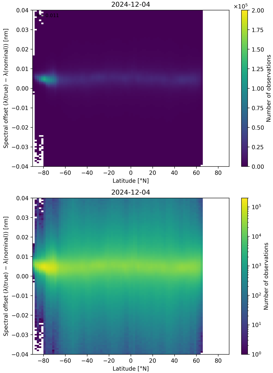
Figure 96: Scatter density plot of “Latitude” against “Spectral offset ( \lambda_{\text{true}} - \lambda_{\text{nominal}} )” for 2024-12-03 to 2024-12-05.
