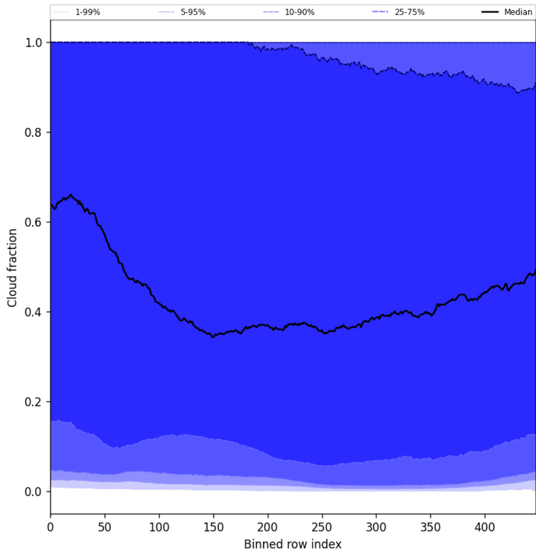
Figure 49: Along track statistics of “Cloud fraction” for 2024-12-03 to 2024-12-05
