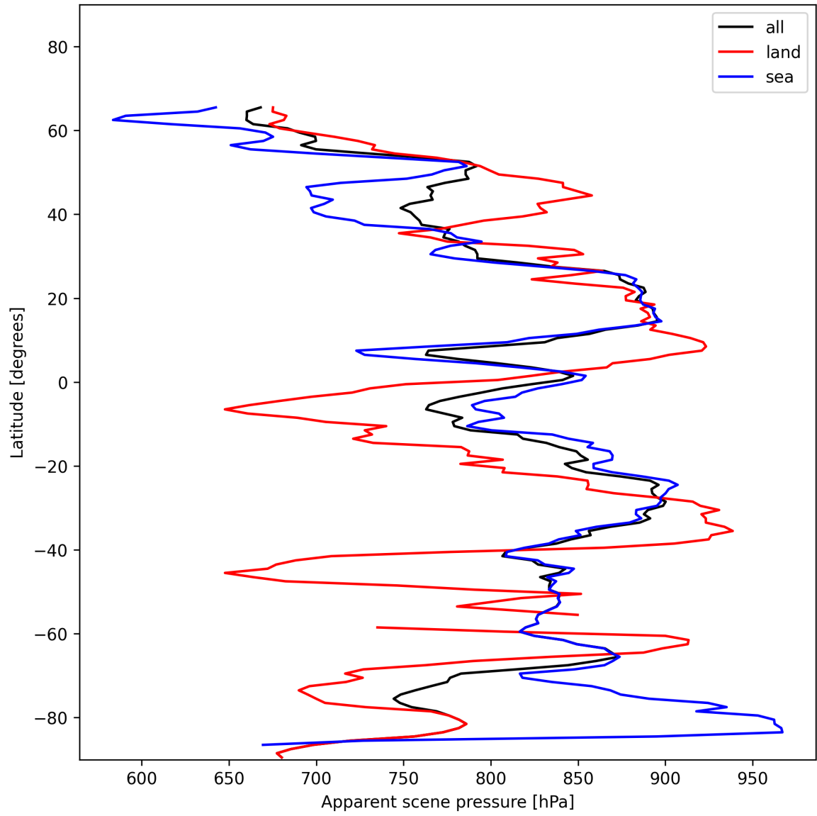
Figure 19: Zonal average of “Apparent scene pressure” for 2024-12-03 to 2024-12-05.
