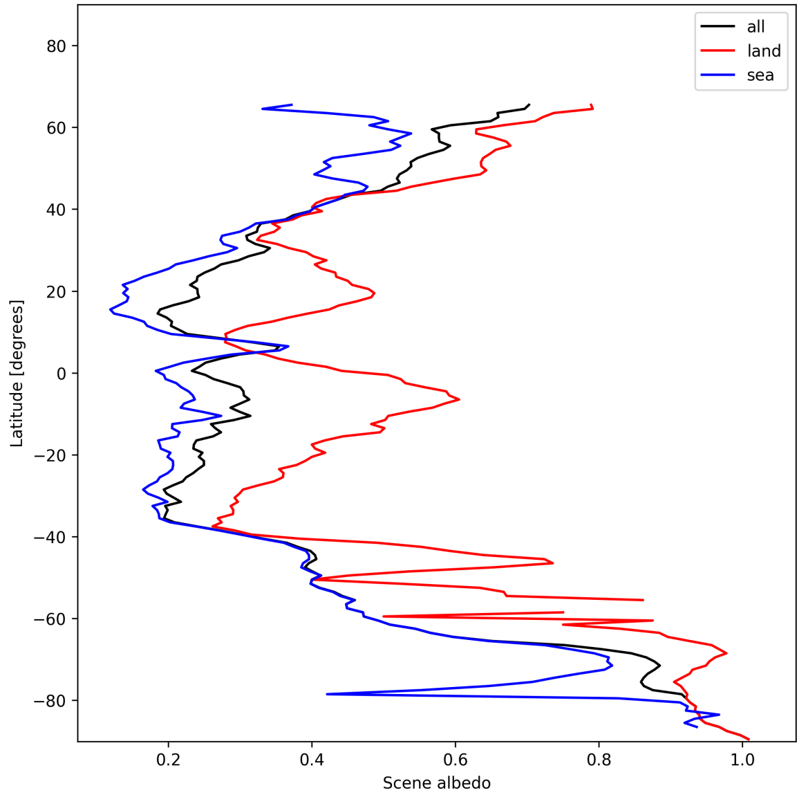
Figure 17: Zonal average of “Scene albedo” for 2024-12-03 to 2024-12-05.
