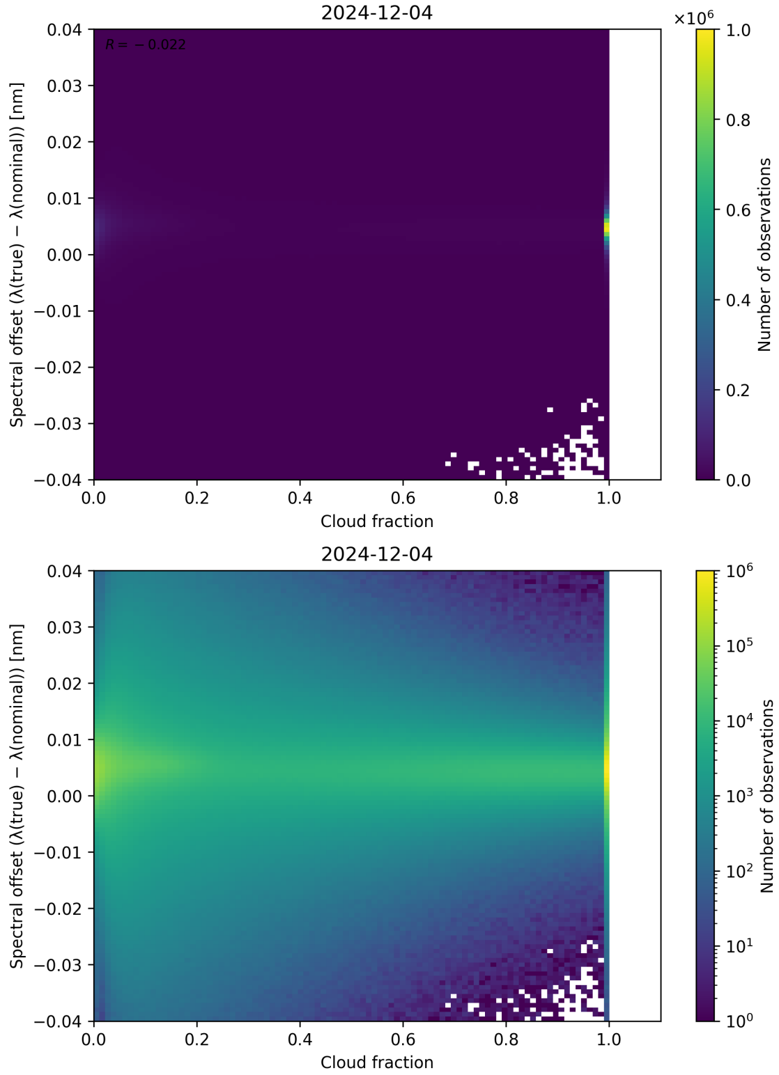
Figure 76: Scatter density plot of “Cloud fraction” against “Spectral offset ( \lambda_{\text{true}} - \lambda_{\text{nominal}} )” for 2024-12-03 to 2024-12-05.
