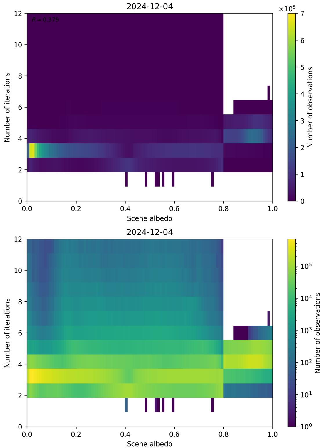
Figure 105: Scatter density plot of “Scene albedo” against “Number of iterations” for 2024-12-03 to 2024-12-05.
