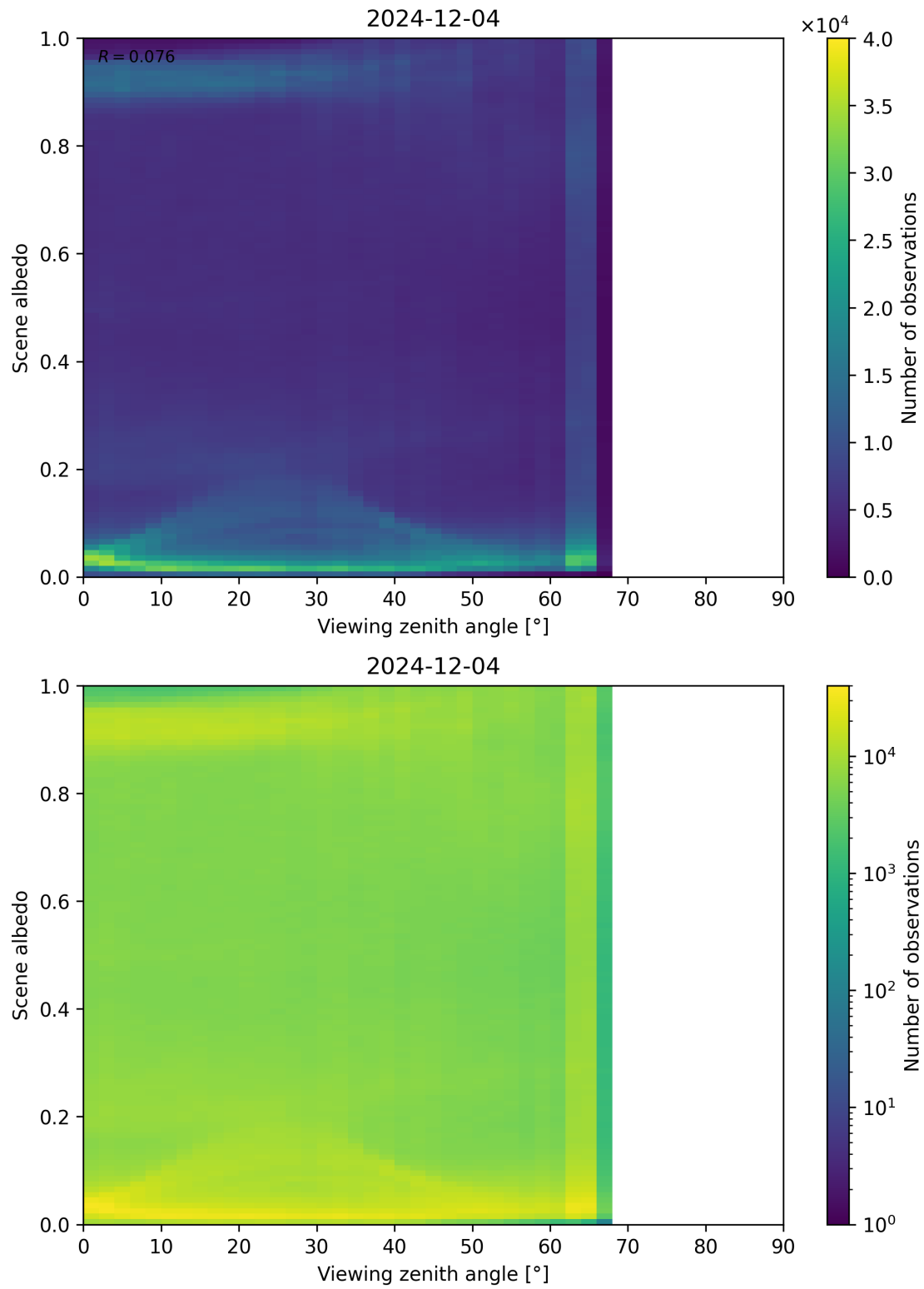
Figure 126: Scatter density plot of “Viewing zenith angle” against “Scene albedo” for 2024-12-03 to 2024-12-05.
