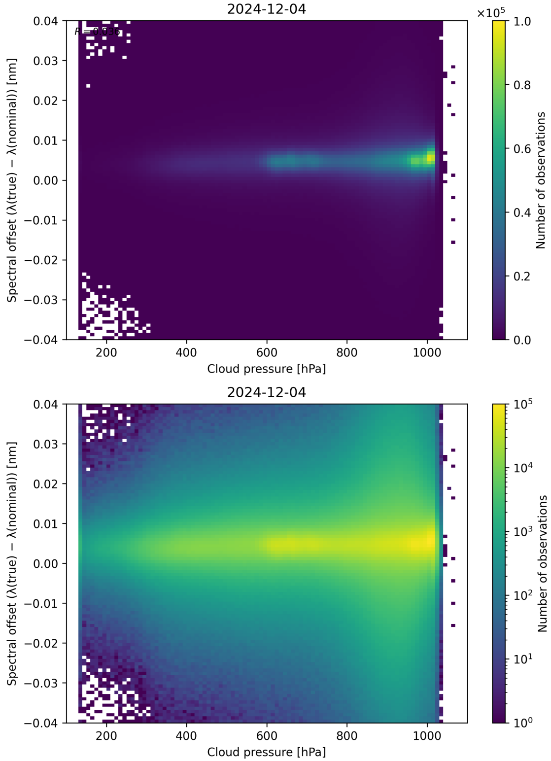
Figure 84: Scatter density plot of “Cloud pressure” against “Spectral offset ( \lambda_{\text{true}} - \lambda_{\text{nominal}} )” for 2024-12-03 to 2024-12-05.
