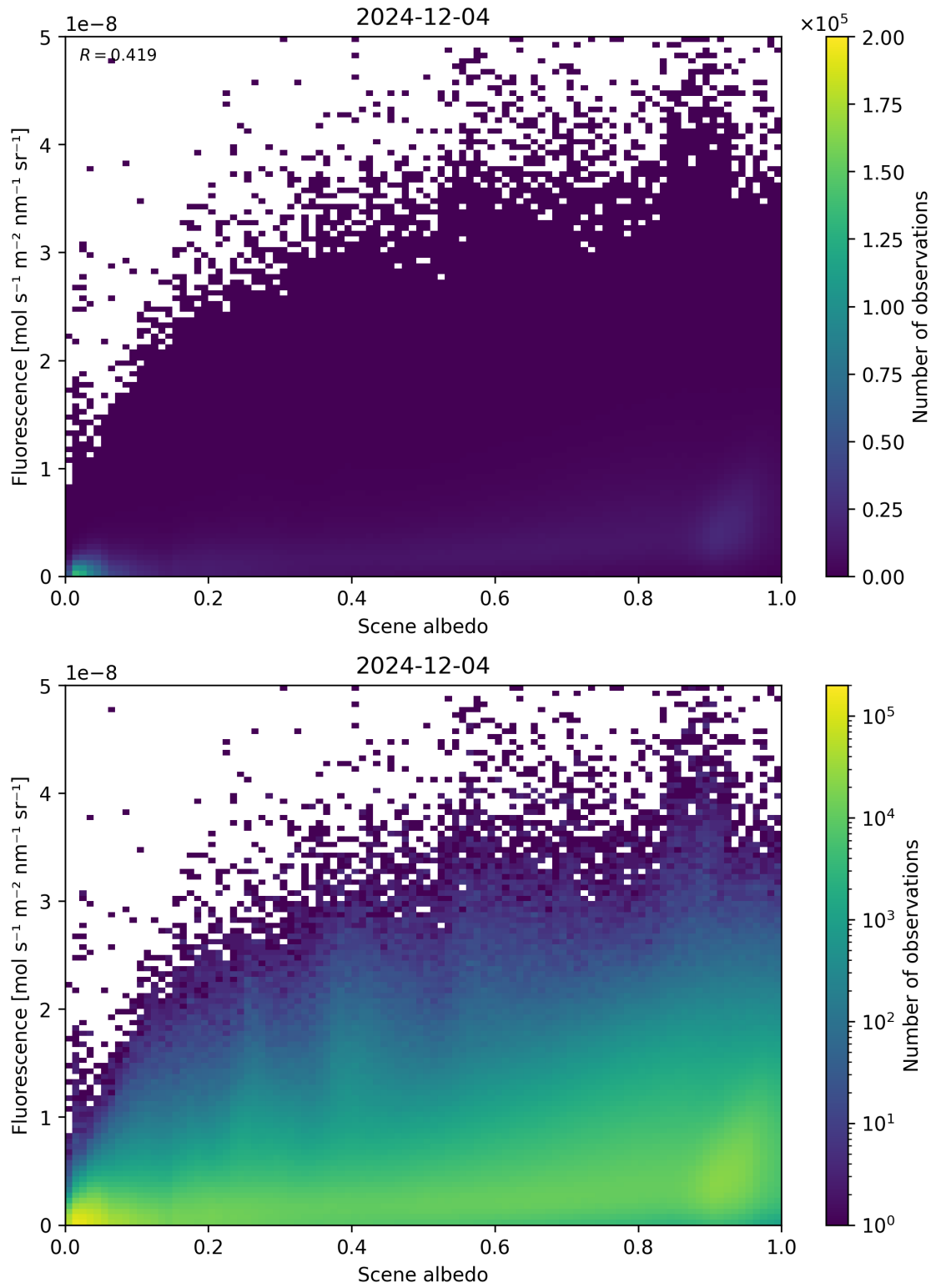
Figure 104: Scatter density plot of “Scene albedo” against “Fluorescence” for 2024-12-03 to 2024-12-05.
