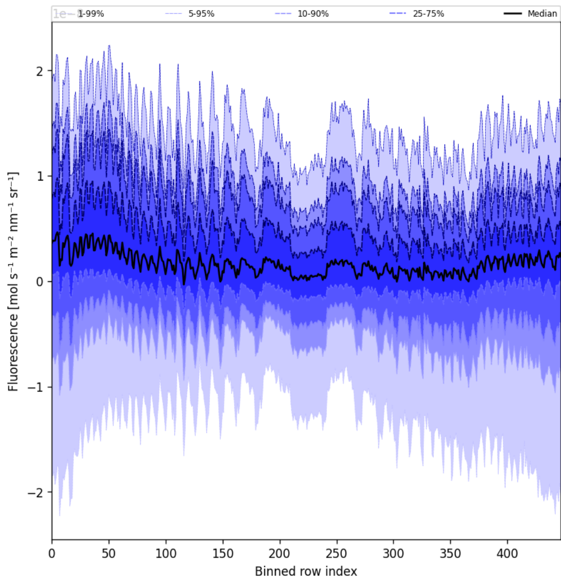
Figure 57: Along track statistics of “Fluorescence” for 2024-12-03 to 2024-12-05
