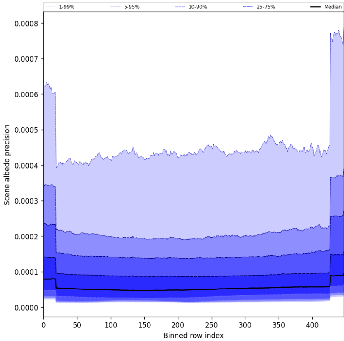
Figure 52: Along track statistics of “Scene albedo precision” for 2024-12-03 to 2024-12-05
