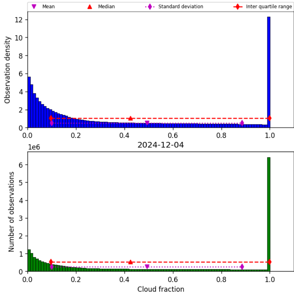
Figure 32: Histogram of “Cloud fraction” for 2024-12-03 to 2024-12-05
