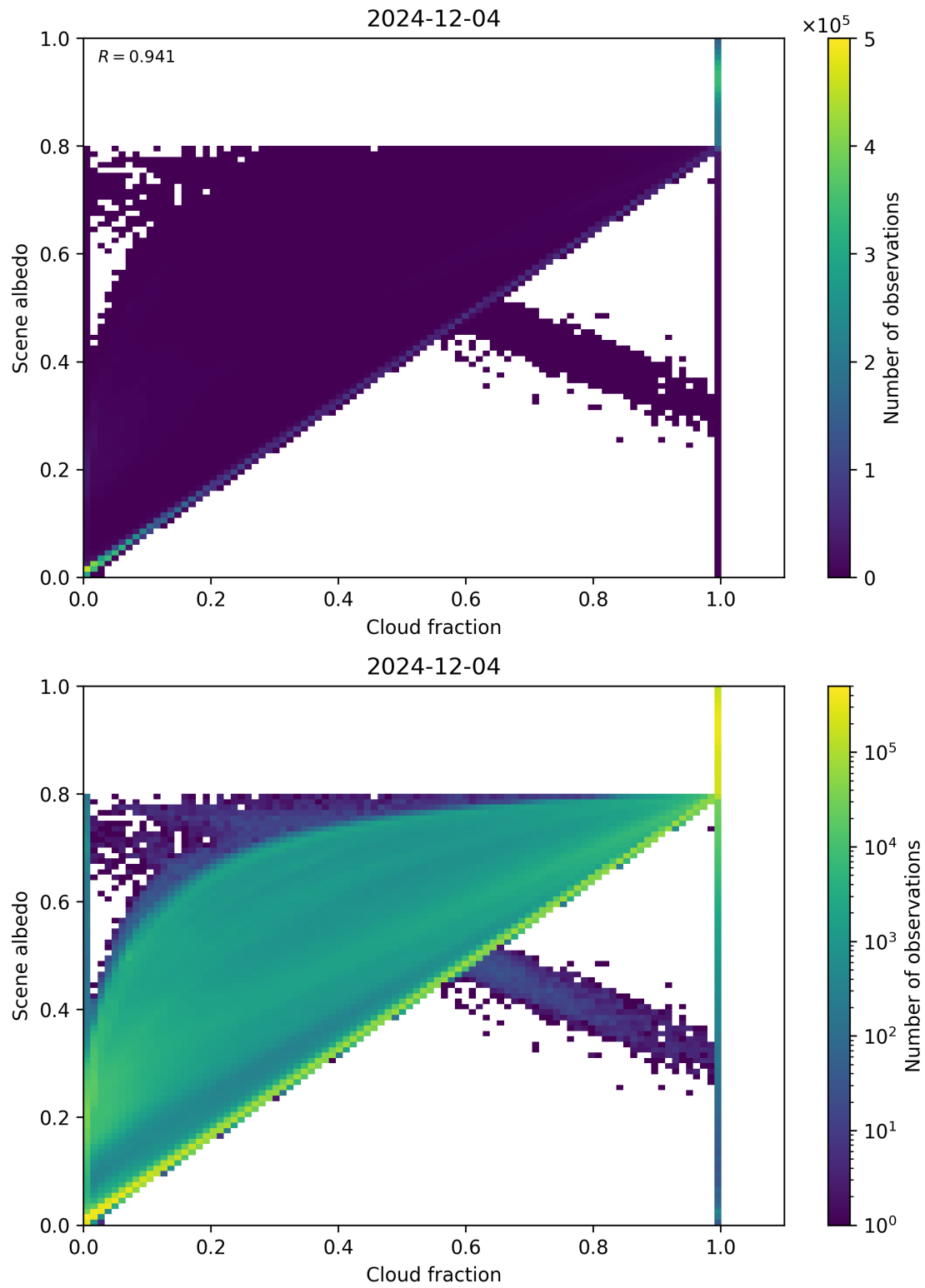
Figure 75: Scatter density plot of “Cloud fraction” against “Scene albedo” for 2024-12-03 to 2024-12-05.
