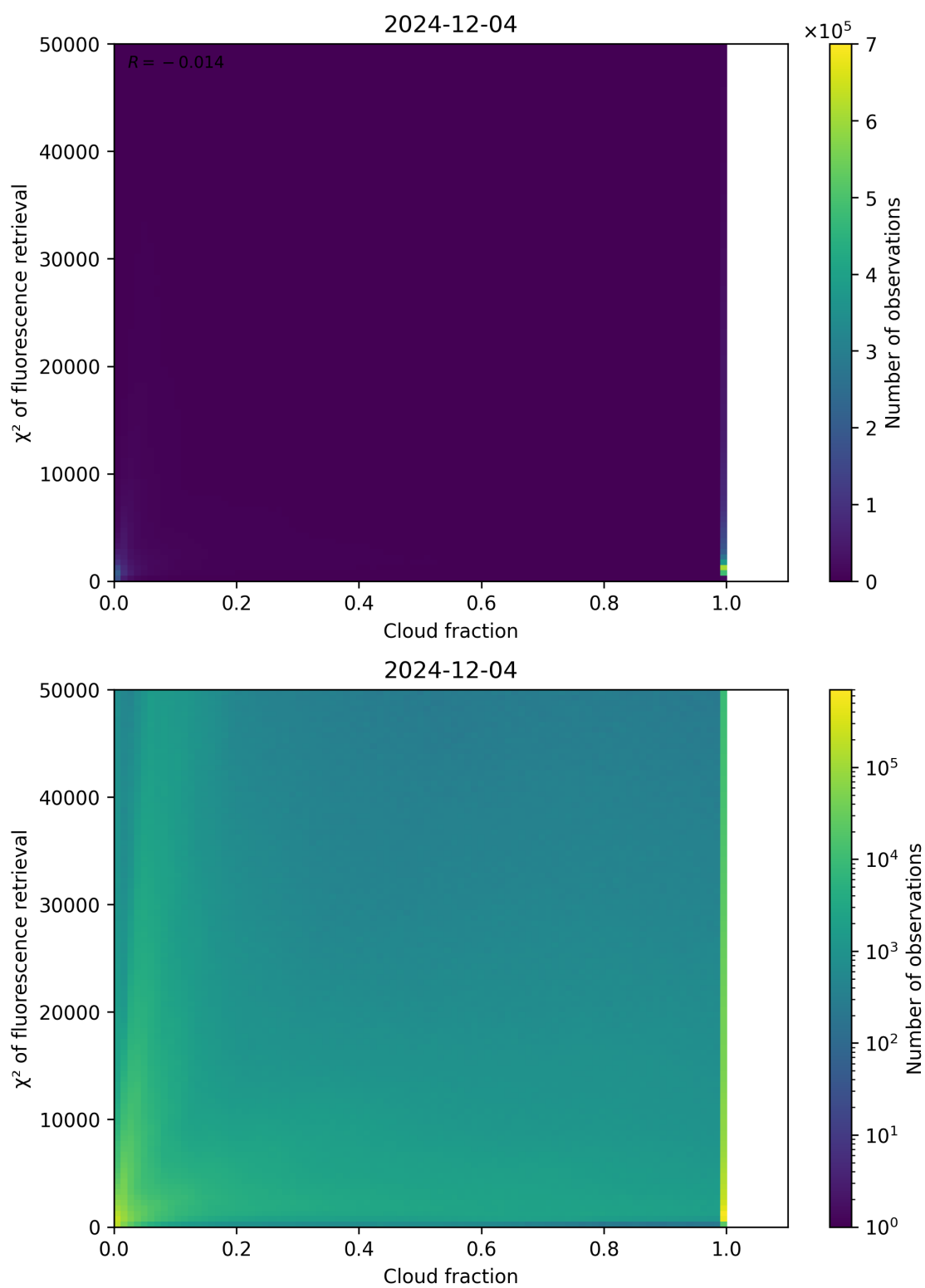
Figure 71: Scatter density plot of “Cloud fraction” against “ \chi^2 of fluorescence retrieval” for 2024-12-03 to 2024-12-05.
