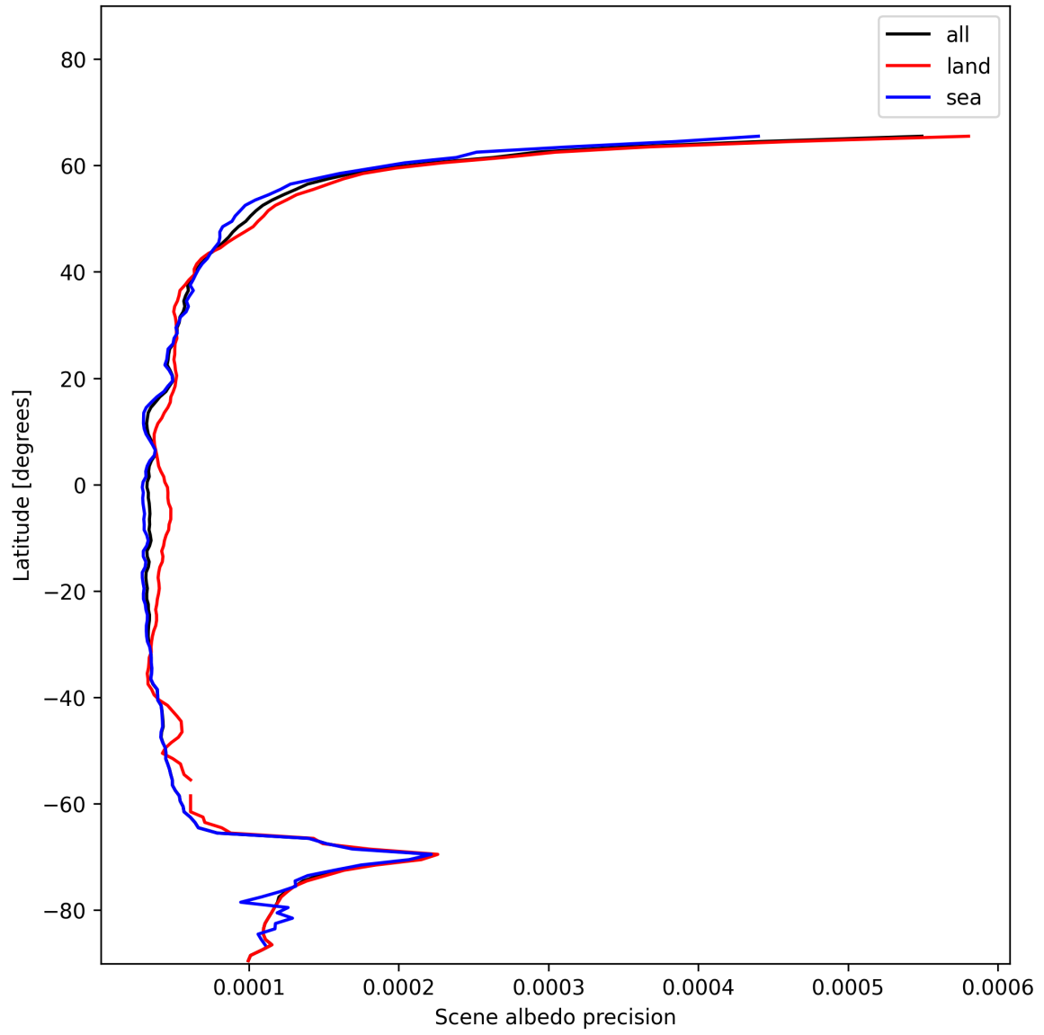
Figure 18: Zonal average of “Scene albedo precision” for 2024-12-03 to 2024-12-05.
