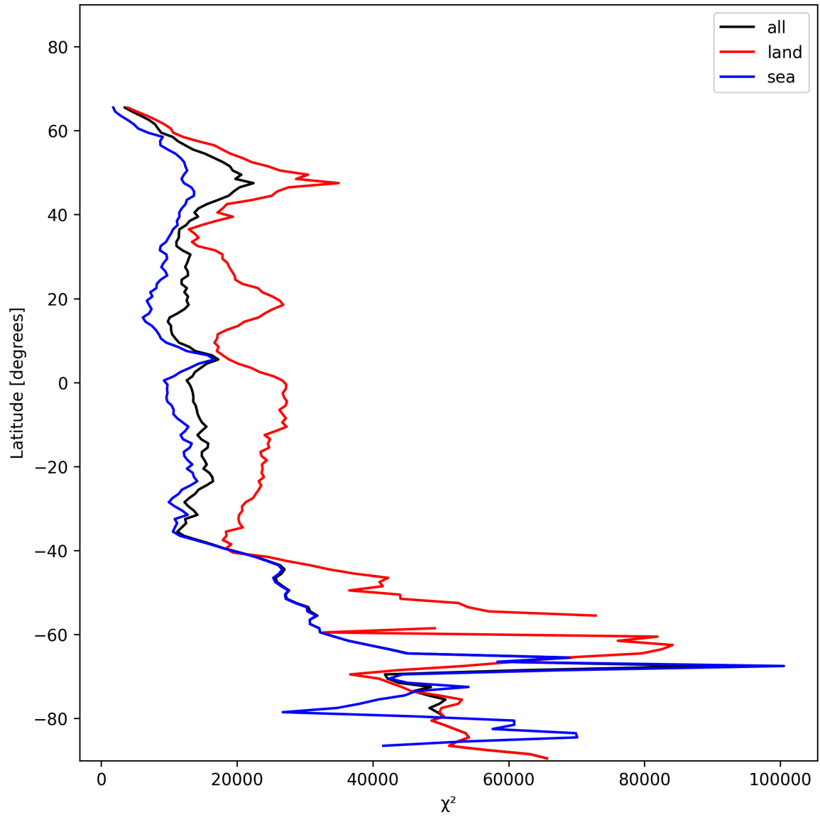
Figure 21: Zonal average of “ \chi^2 ” for 2024-12-03 to 2024-12-05.
