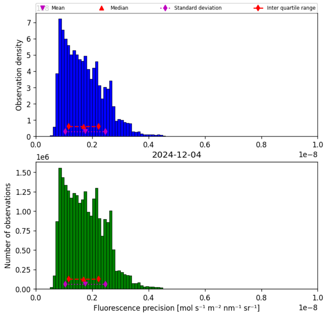
Figure 41: Histogram of “Fluorescence precision” for 2024-12-03 to 2024-12-05
