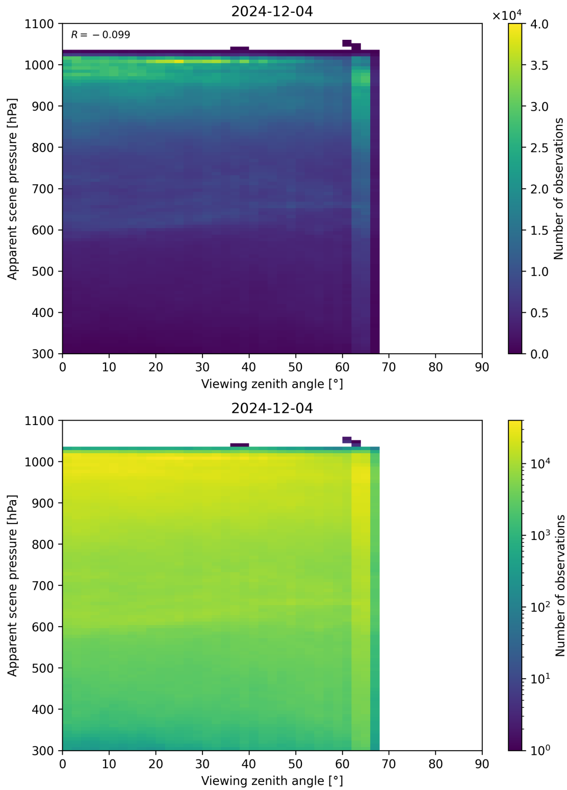
Figure 118: Scatter density plot of “Viewing zenith angle” against “Apparent scene pressure” for 2024-12-03 to 2024-12-05.
