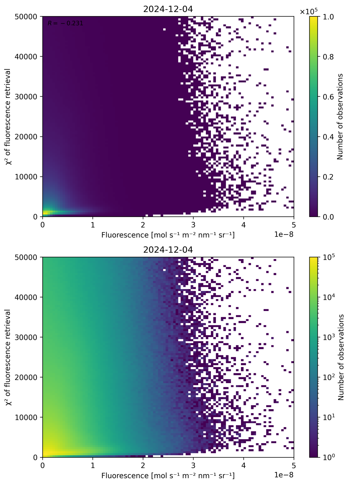
Figure 85: Scatter density plot of “Fluorescence” against “ \chi^2 of fluorescence retrieval” for 2024-12-03 to 2024-12-05.
