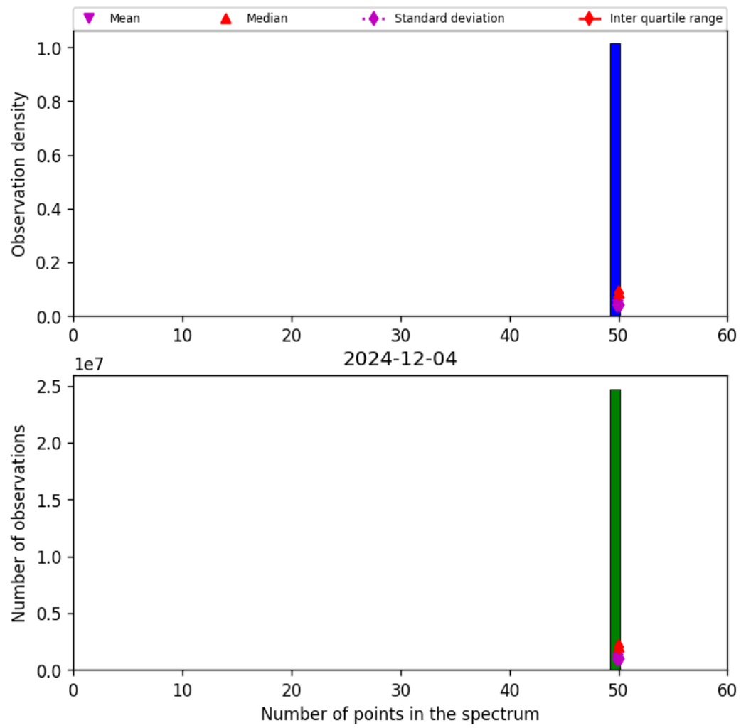
Figure 44: Histogram of “Number of points in the spectrum” for 2024-12-03 to 2024-12-05
