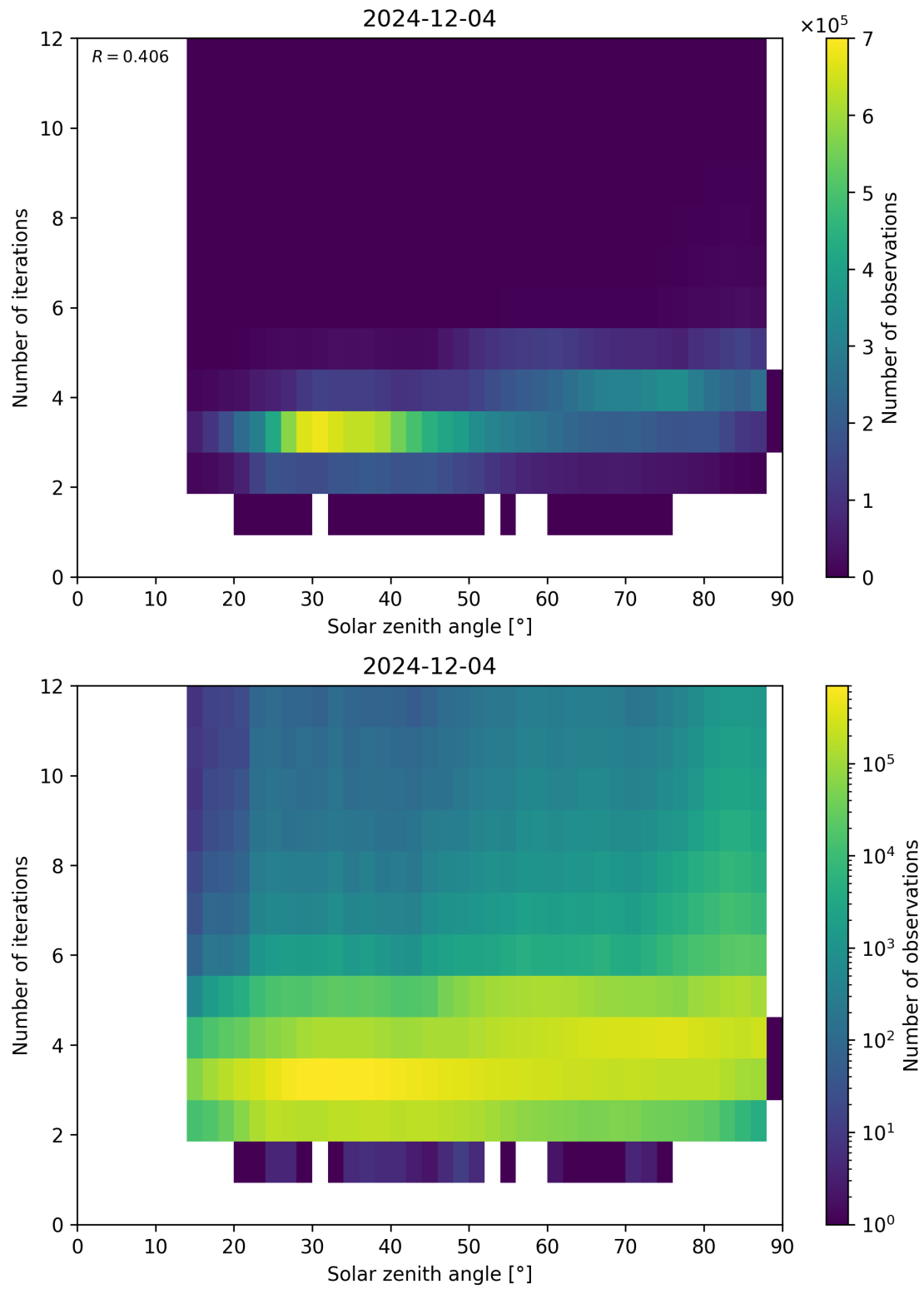
Figure 114: Scatter density plot of “Solar zenith angle” against “Number of iterations” for 2024-12-03 to 2024-12-05.
