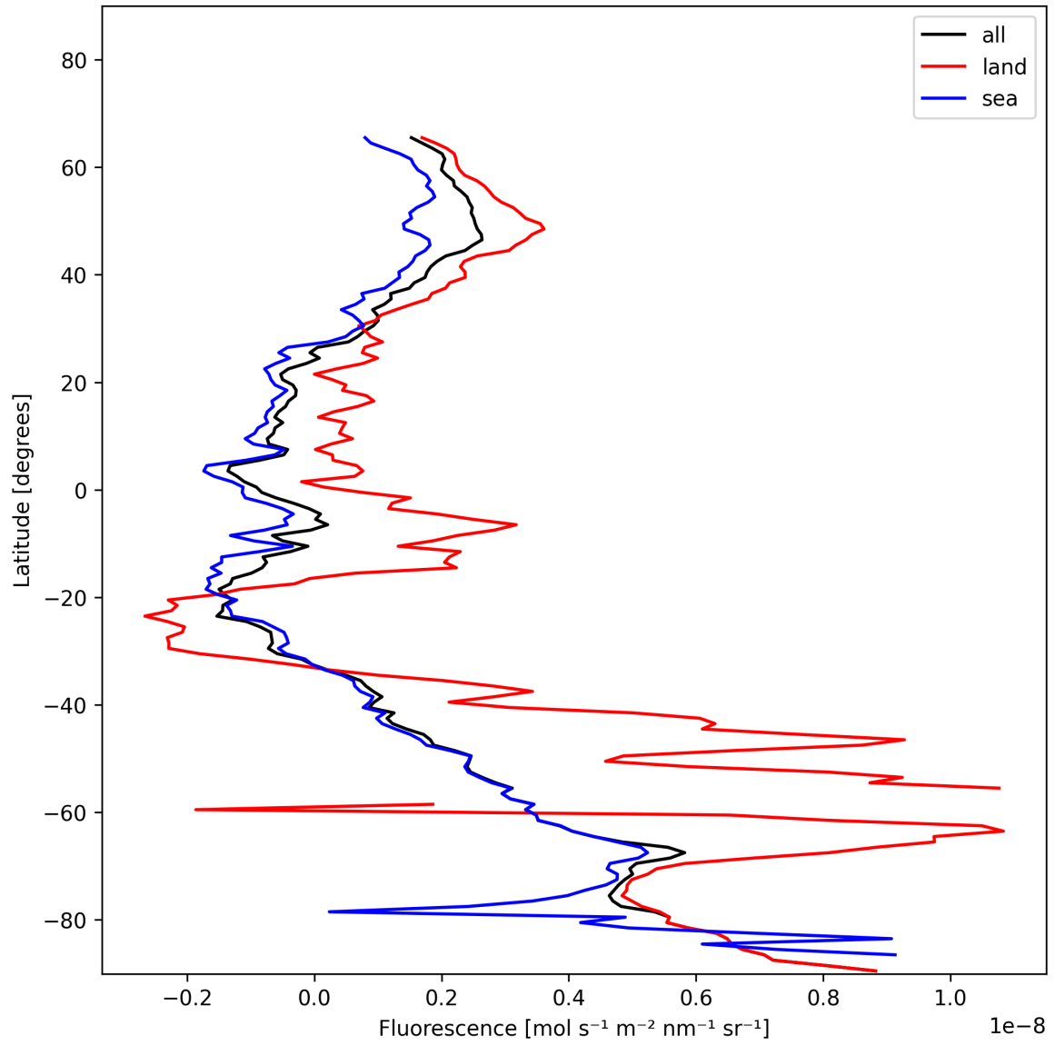
Figure 23: Zonal average of “Fluorescence” for 2024-12-03 to 2024-12-05.
