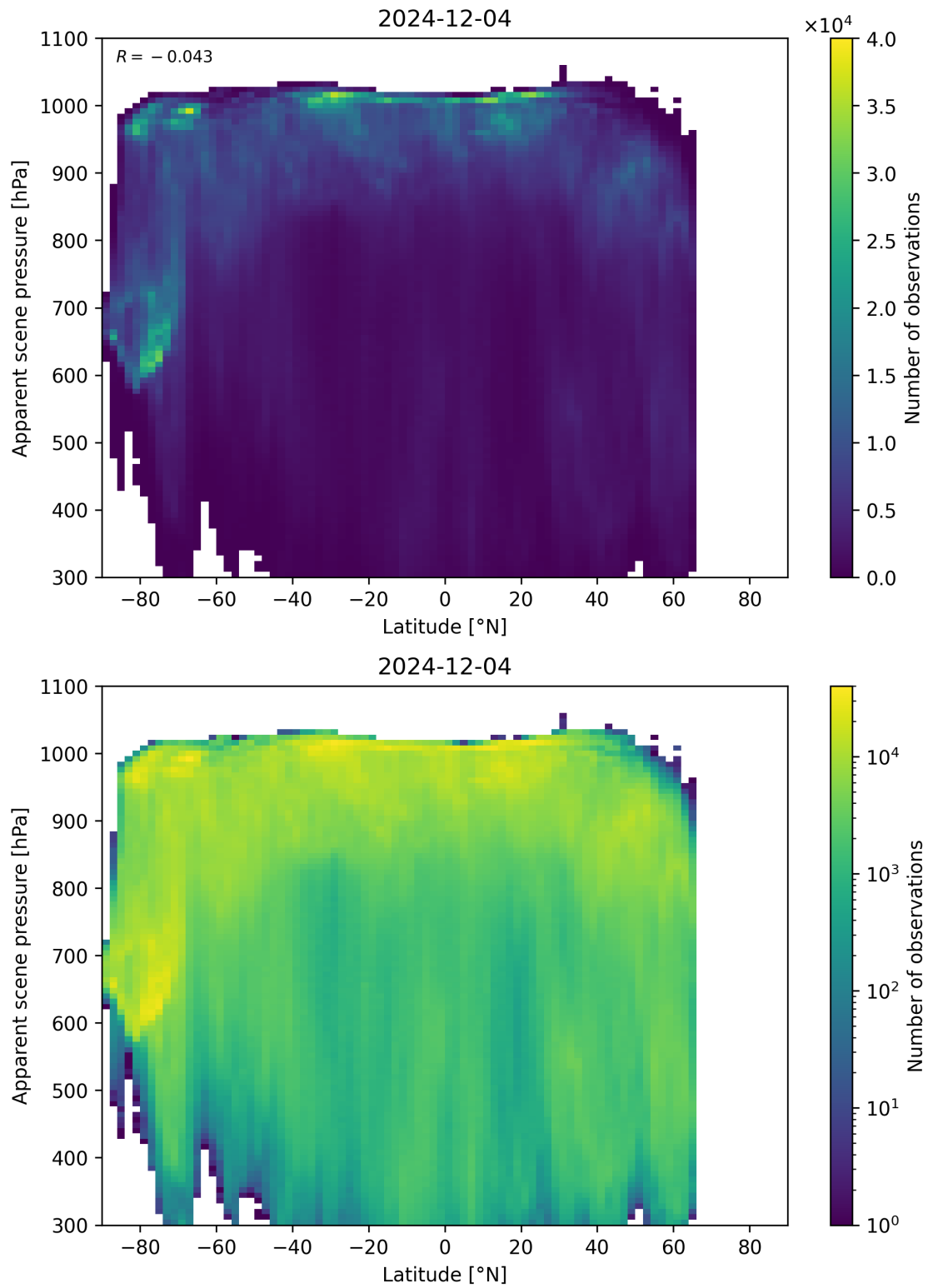
Figure 88: Scatter density plot of “Latitude” against “Apparent scene pressure” for 2024-12-03 to 2024-12-05.
