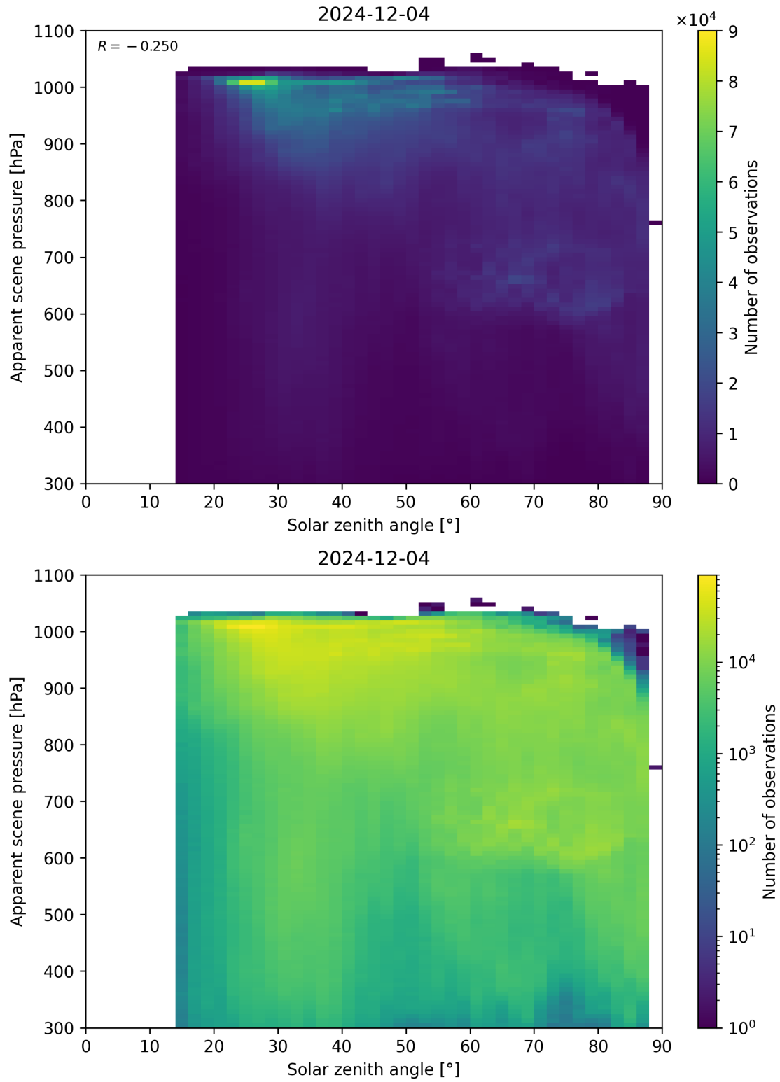
Figure 108: Scatter density plot of “Solar zenith angle” against “Apparent scene pressure” for 2024-12-03 to 2024-12-05.
