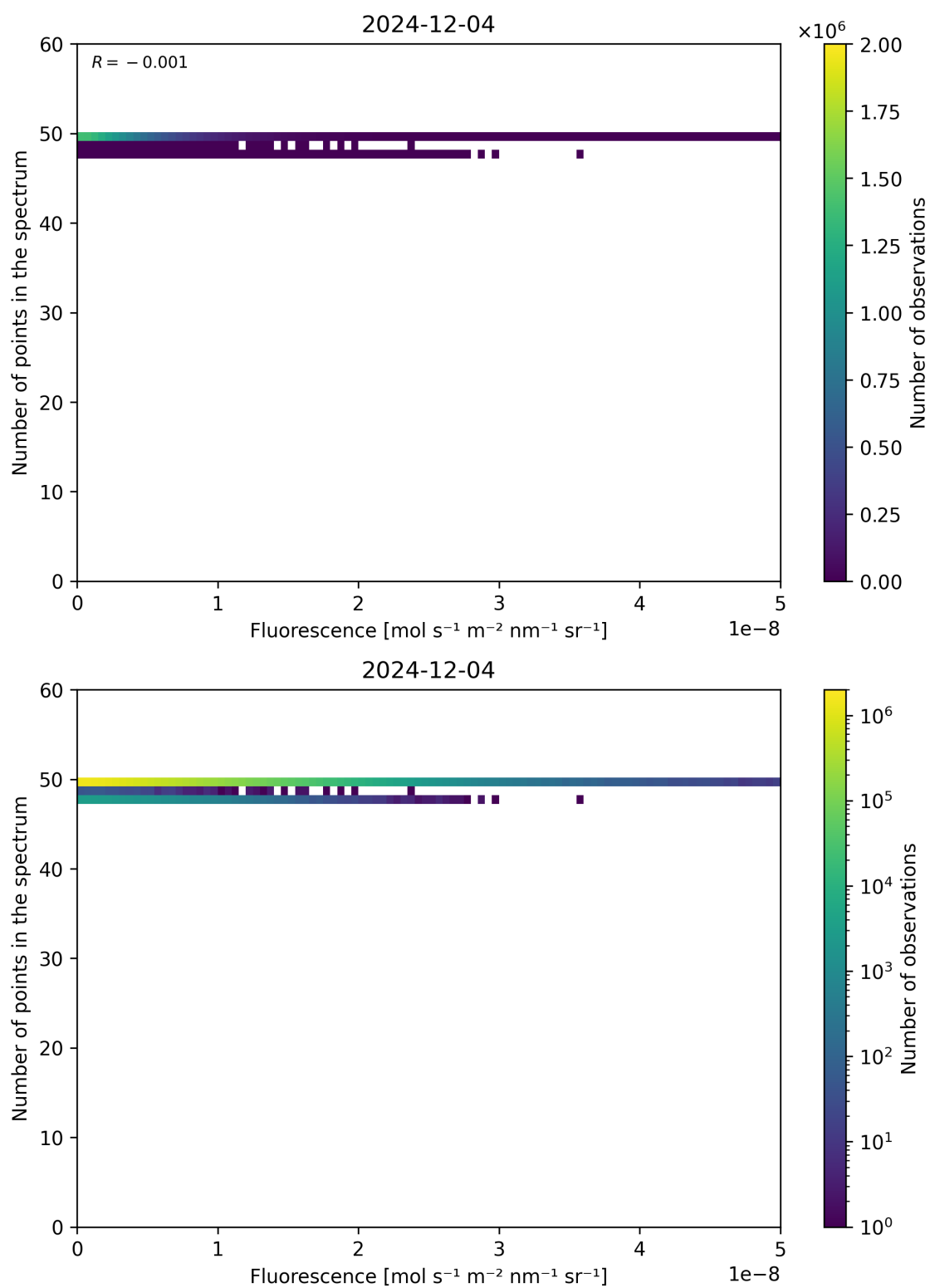
Figure 86: Scatter density plot of “Fluorescence” against “Number of points in the spectrum” for 2024-12-03 to 2024-12-05.
