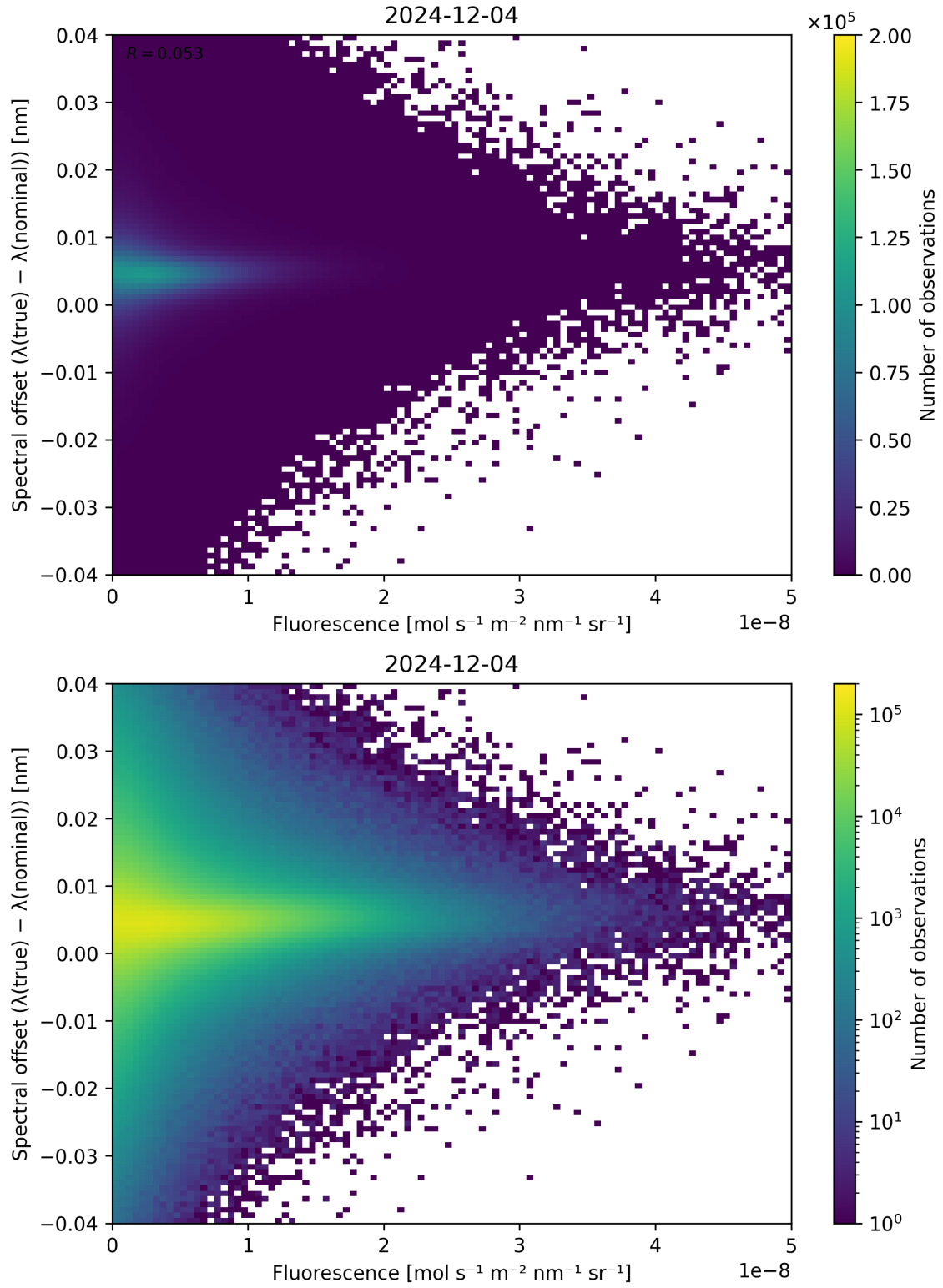
Figure 87: Scatter density plot of “Fluorescence” against “Spectral offset ( \lambda_{\text{true}} - \lambda_{\text{nominal}} )” for 2024-12-03 to 2024-12-05.
