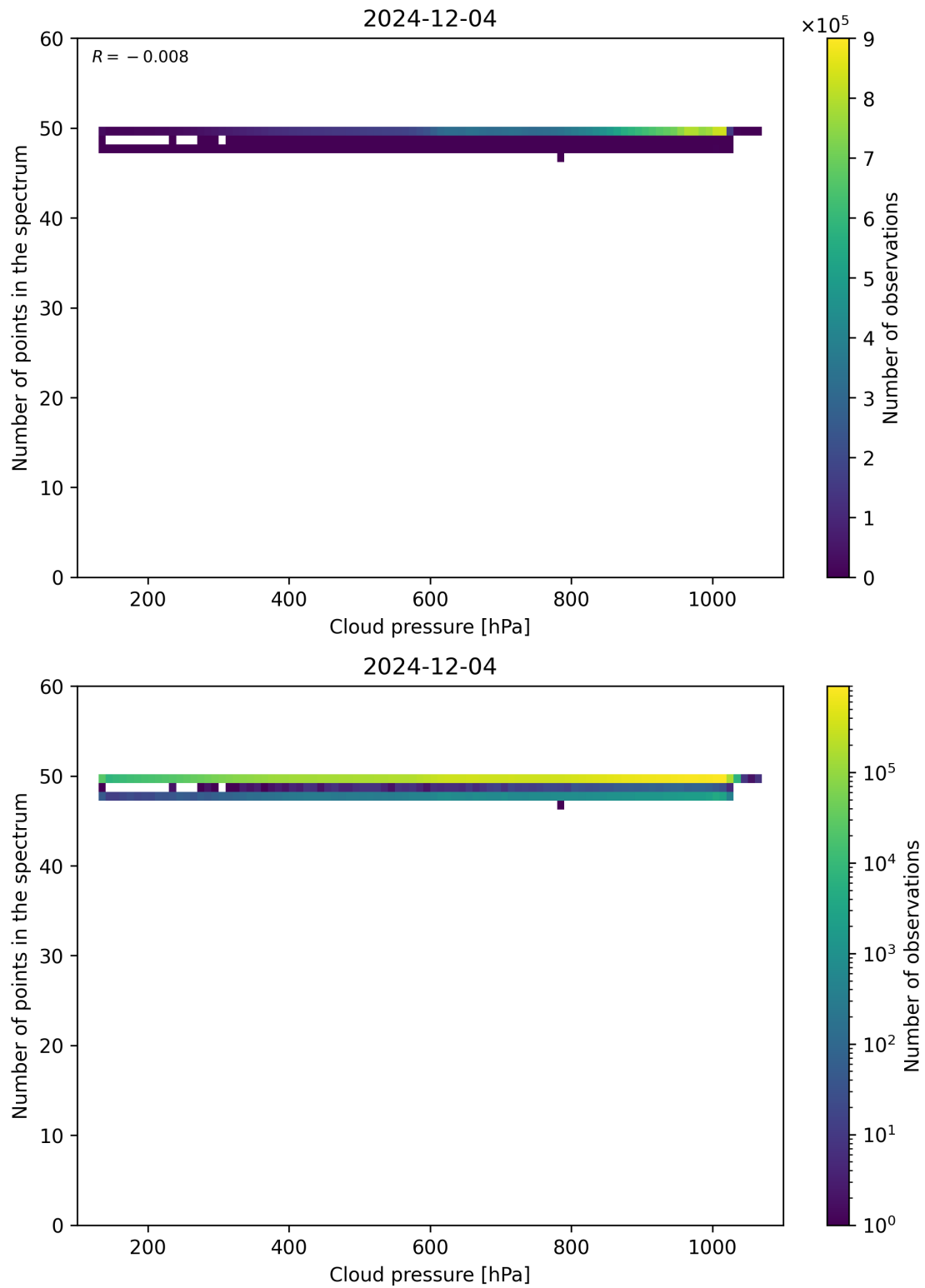
Figure 82: Scatter density plot of “Cloud pressure” against “Number of points in the spectrum” for 2024-12-03 to 2024-12-05.
