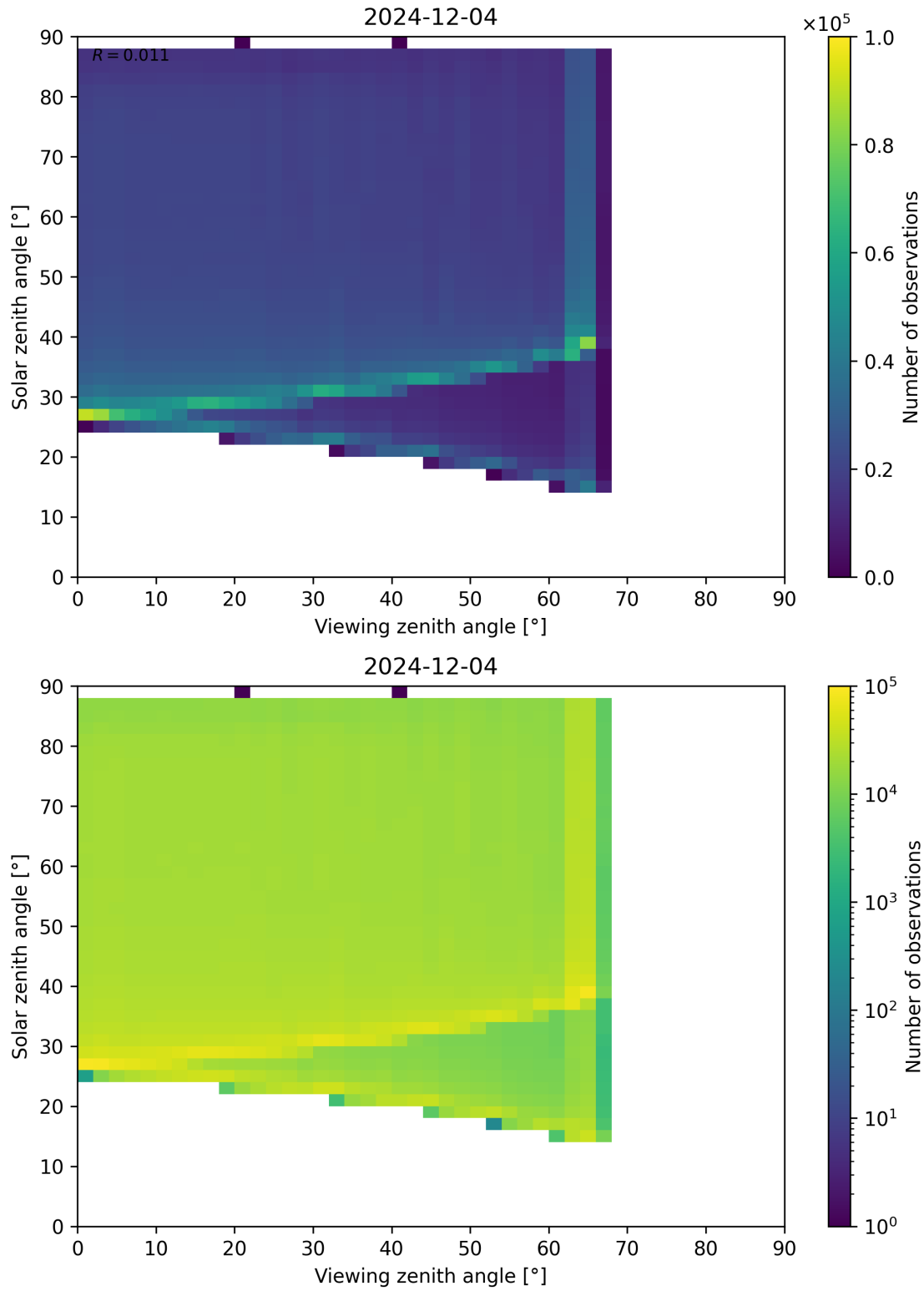
Figure 127: Scatter density plot of “Viewing zenith angle” against “Solar zenith angle” for 2024-12-03 to 2024-12-05.
