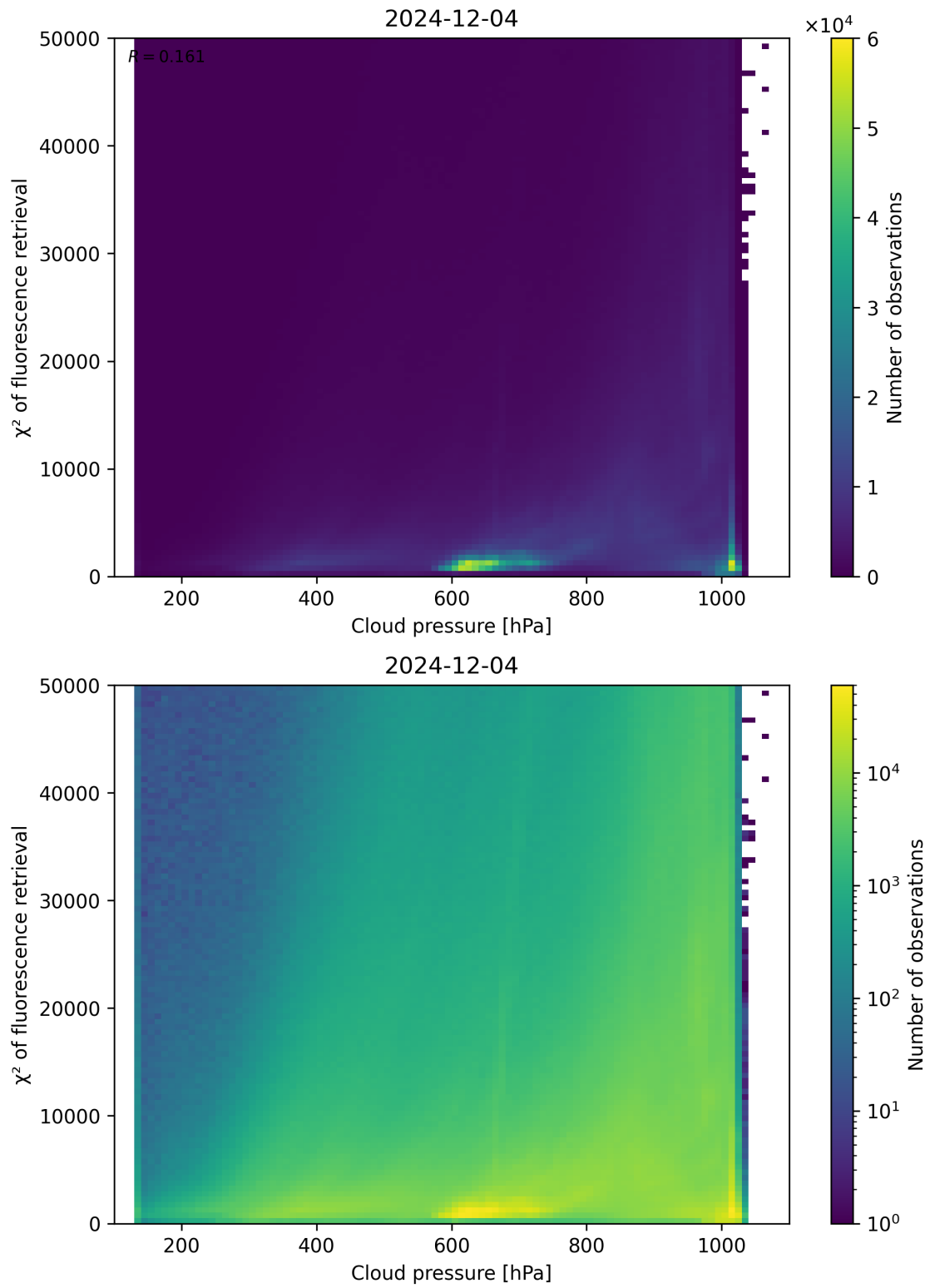
Figure 78: Scatter density plot of “Cloud pressure” against “ \chi^2 of fluorescence retrieval” for 2024-12-03 to 2024-12-05.
