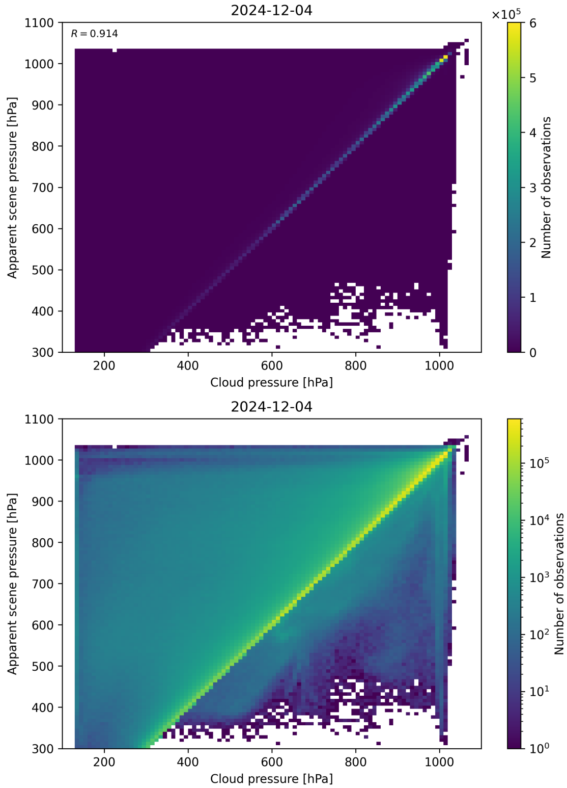
Figure 77: Scatter density plot of “Cloud pressure” against “Apparent scene pressure” for 2024-12-03 to 2024-12-05.
