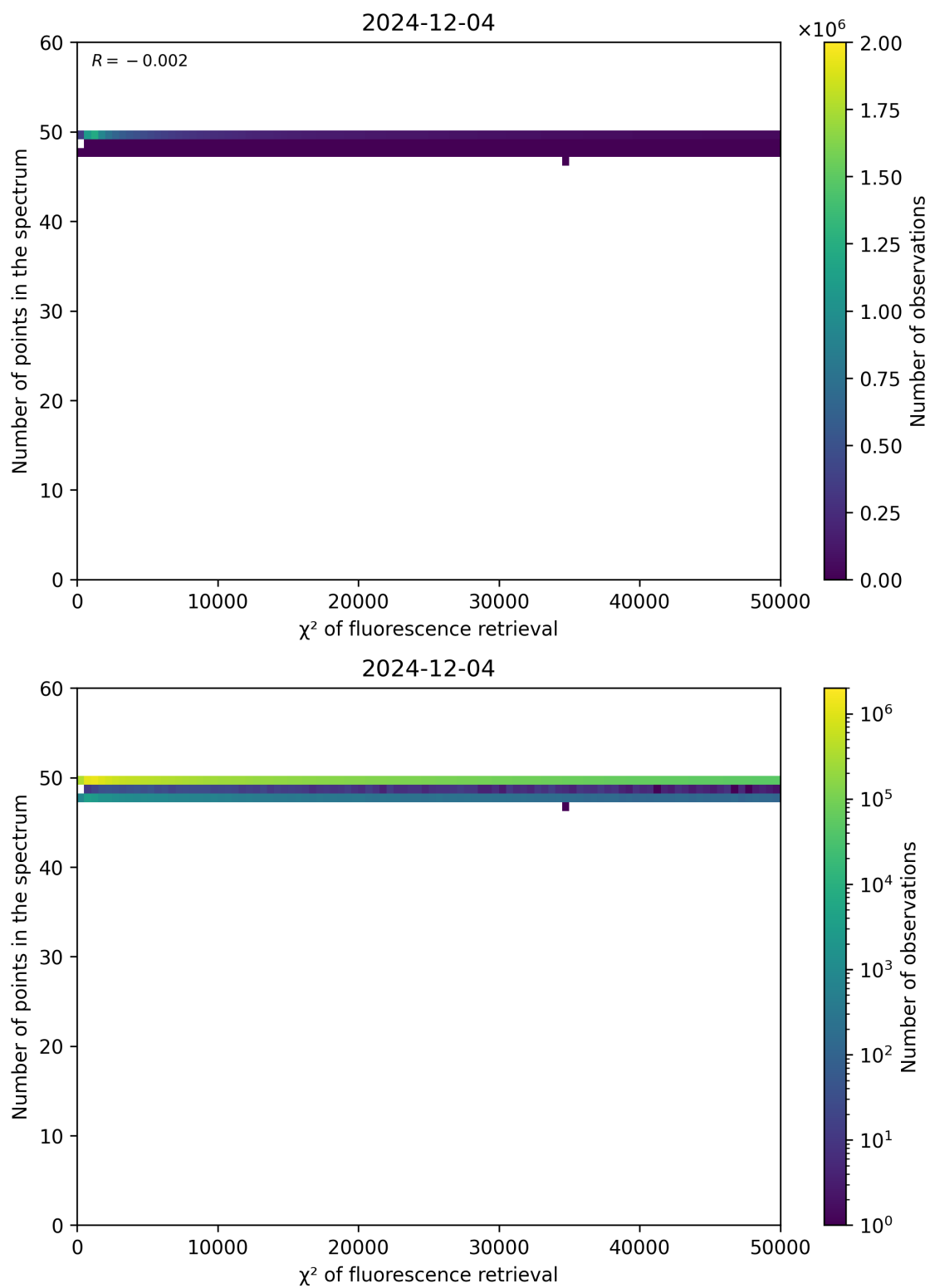
Figure 68: Scatter density plot of “ \chi^2 of fluorescence retrieval” against “Number of points in the spectrum” for 2024-12-03 to 2024-12-05.
