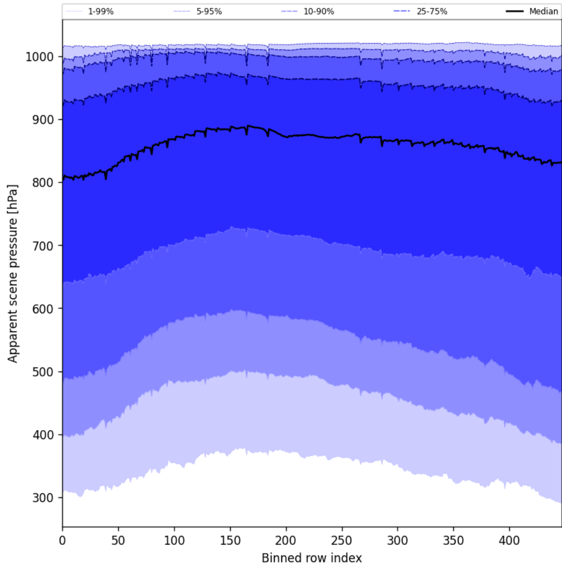
Figure 53: Along track statistics of “Apparent scene pressure” for 2024-12-03 to 2024-12-05
