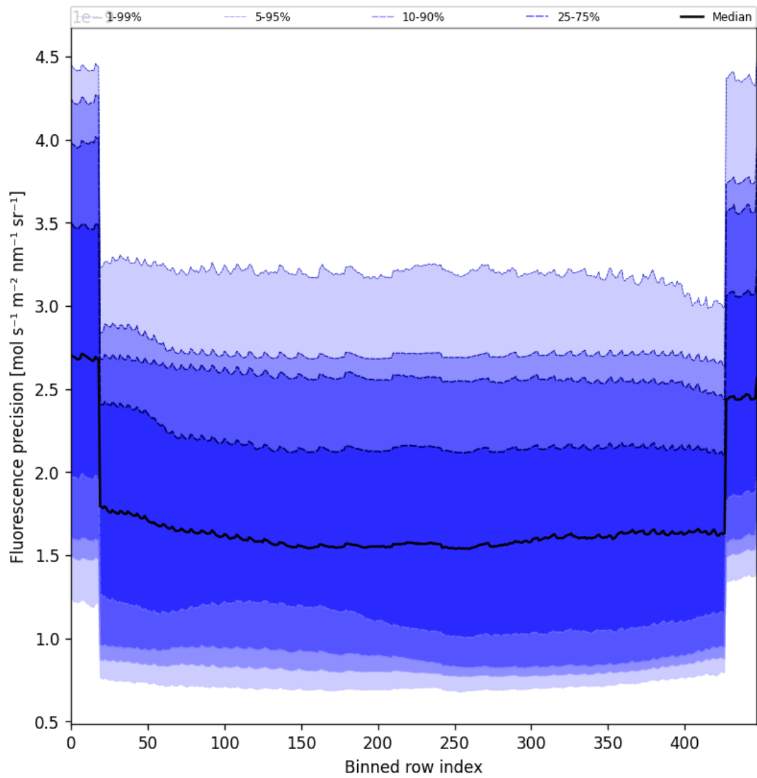
Figure 58: Along track statistics of “Fluorescence precision” for 2024-12-03 to 2024-12-05
