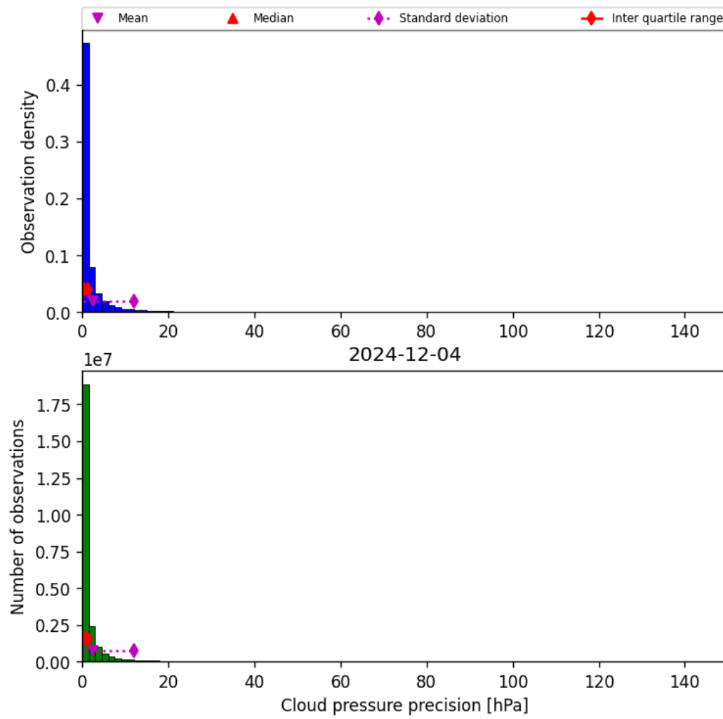
Figure 31: Histogram of “Cloud pressure precision” for 2024-12-03 to 2024-12-05
