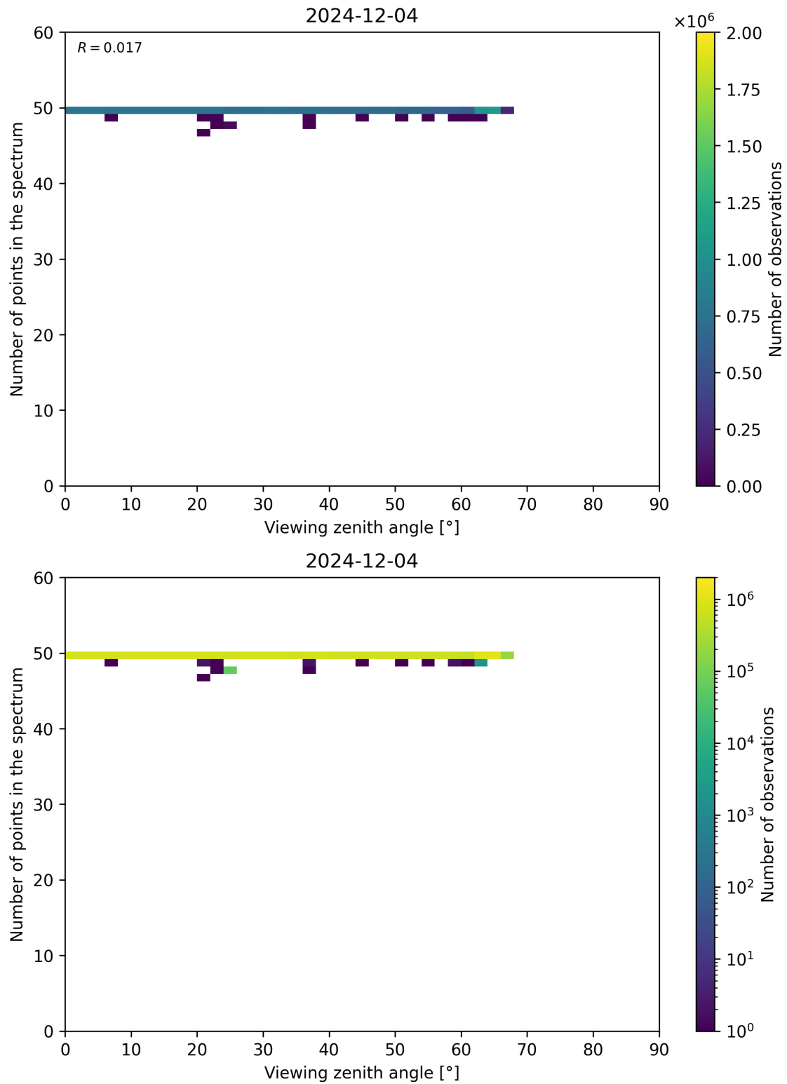
Figure 125: Scatter density plot of “Viewing zenith angle” against “Number of points in the spectrum” for 2024-12-03 to 2024-12-05.
