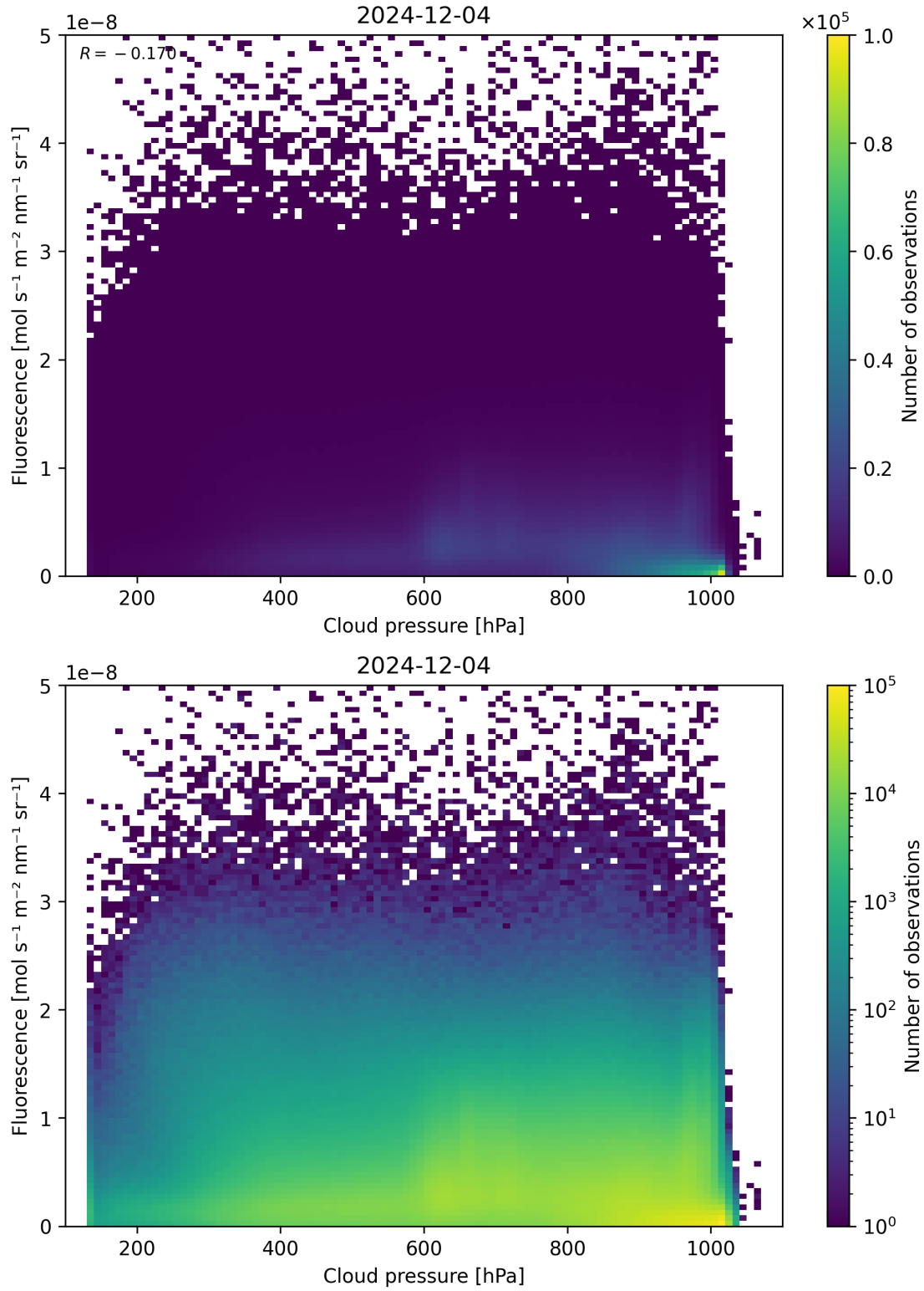
Figure 80: Scatter density plot of “Cloud pressure” against “Fluorescence” for 2024-12-03 to 2024-12-05.
