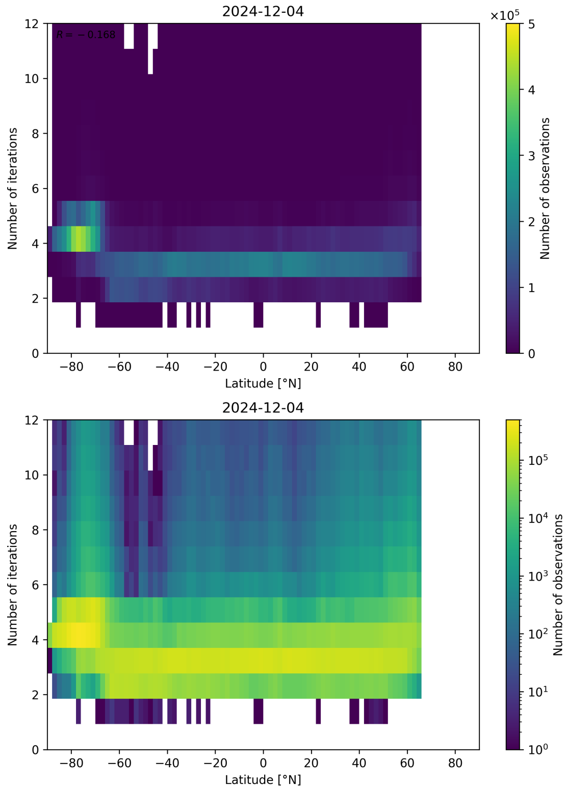
Figure 93: Scatter density plot of “Latitude” against “Number of iterations” for 2024-12-03 to 2024-12-05.
