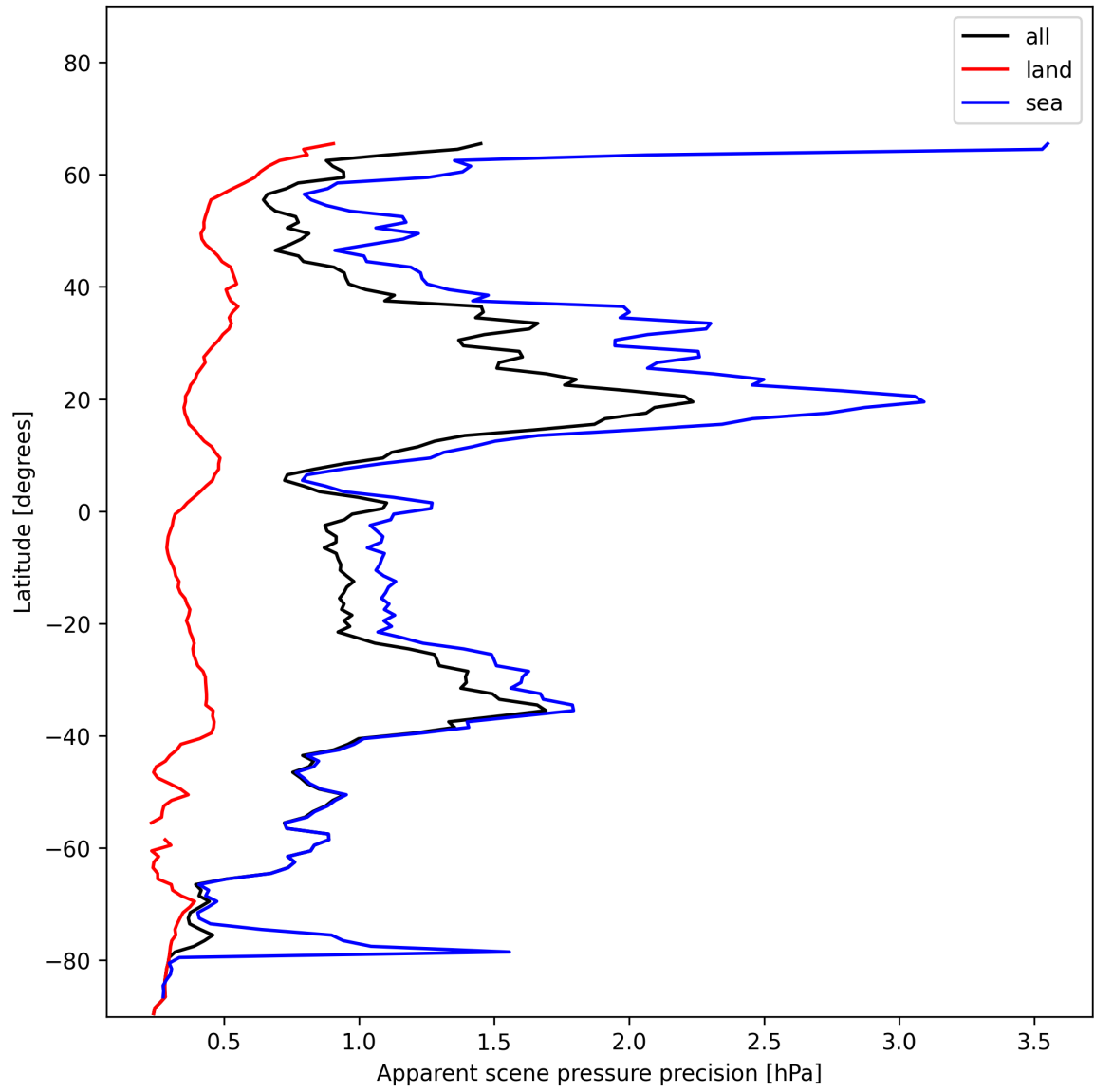
Figure 20: Zonal average of “Apparent scene pressure precision” for 2024-12-03 to 2024-12-05.
