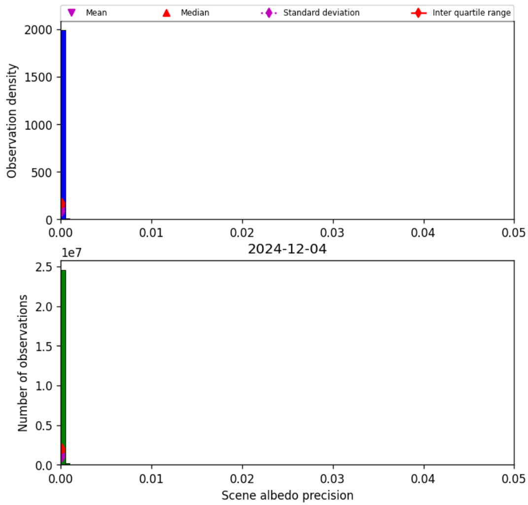
Figure 35: Histogram of “Scene albedo precision” for 2024-12-03 to 2024-12-05
