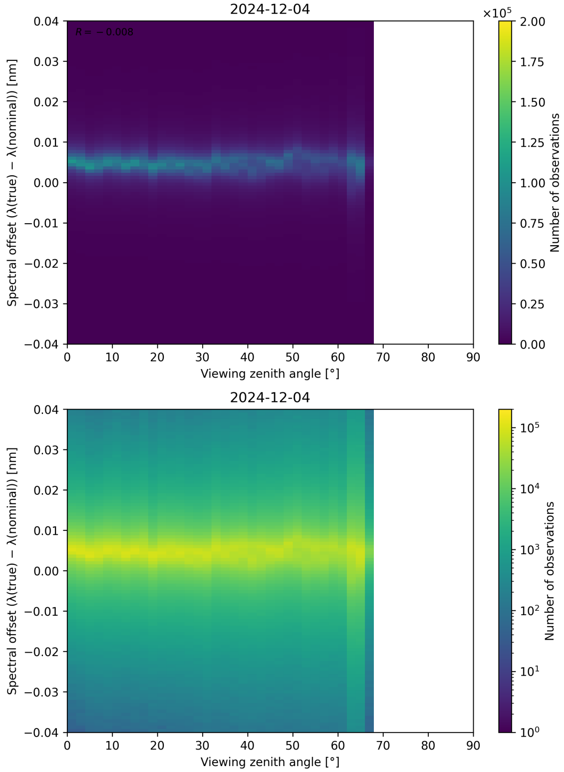
Figure 128: Scatter density plot of “Viewing zenith angle” against “Spectral offset ( \lambda_{\text{true}} - \lambda_{\text{nominal}} )” for 2024-12-03 to 2024-12-05.
