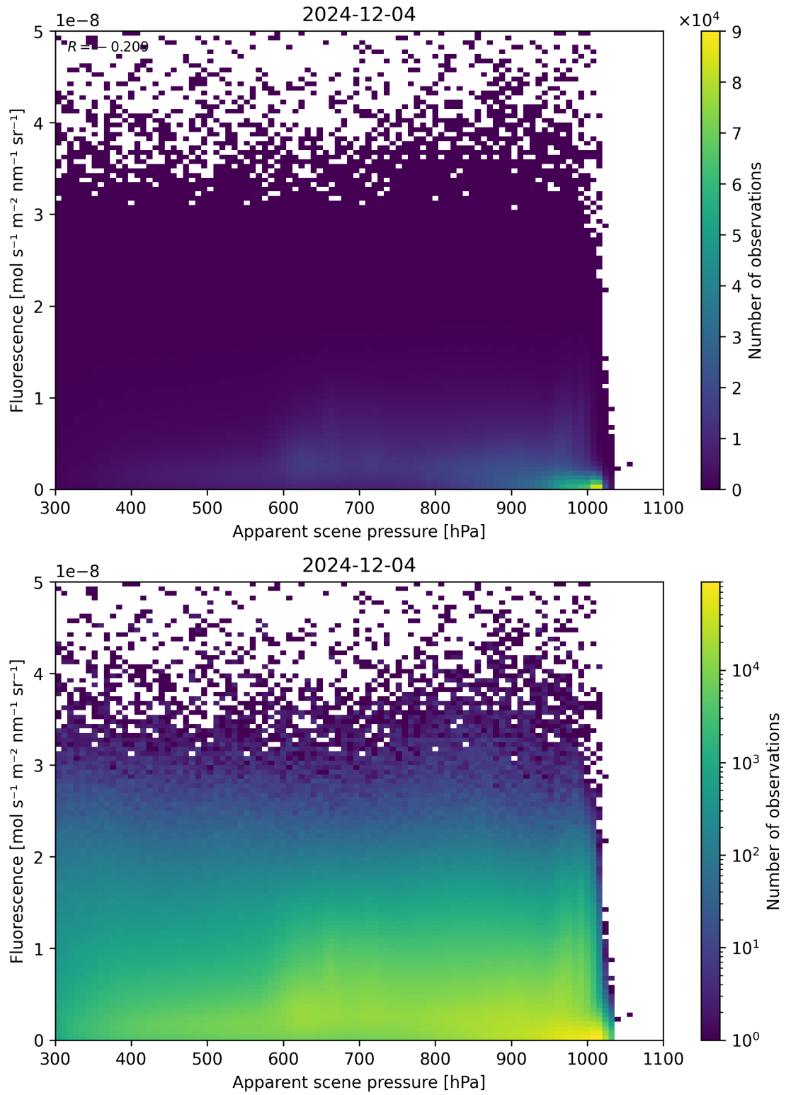
Figure 64: Scatter density plot of “Apparent scene pressure” against “Fluorescence” for 2024-12-03 to 2024-12-05.
