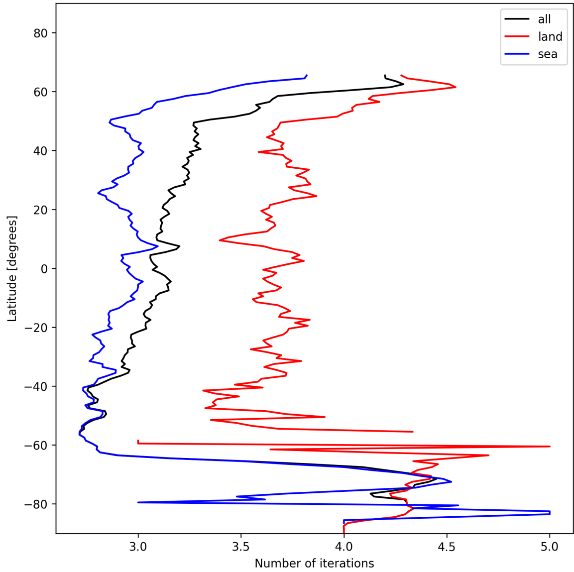
Figure 22: Zonal average of “Number of iterations” for 2024-12-03 to 2024-12-05.
