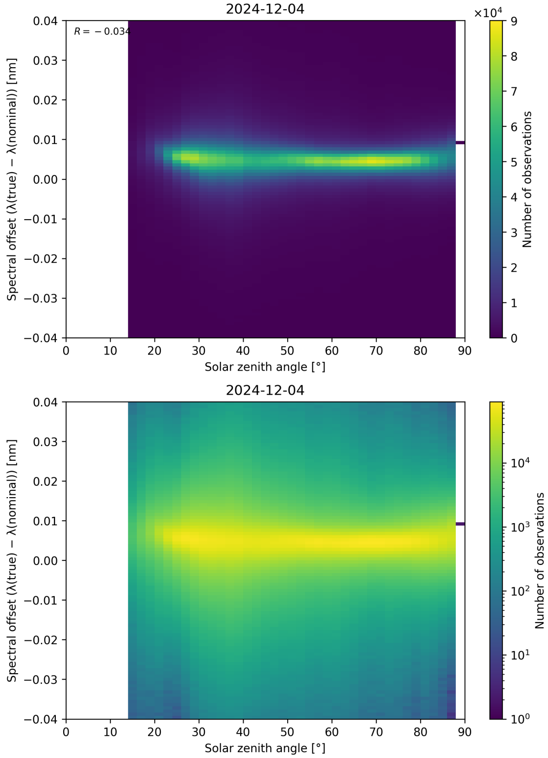
Figure 117: Scatter density plot of “Solar zenith angle” against “Spectral offset ( \lambda_{\text{true}} - \lambda_{\text{nominal}} )” for 2024-12-03 to 2024-12-05.
