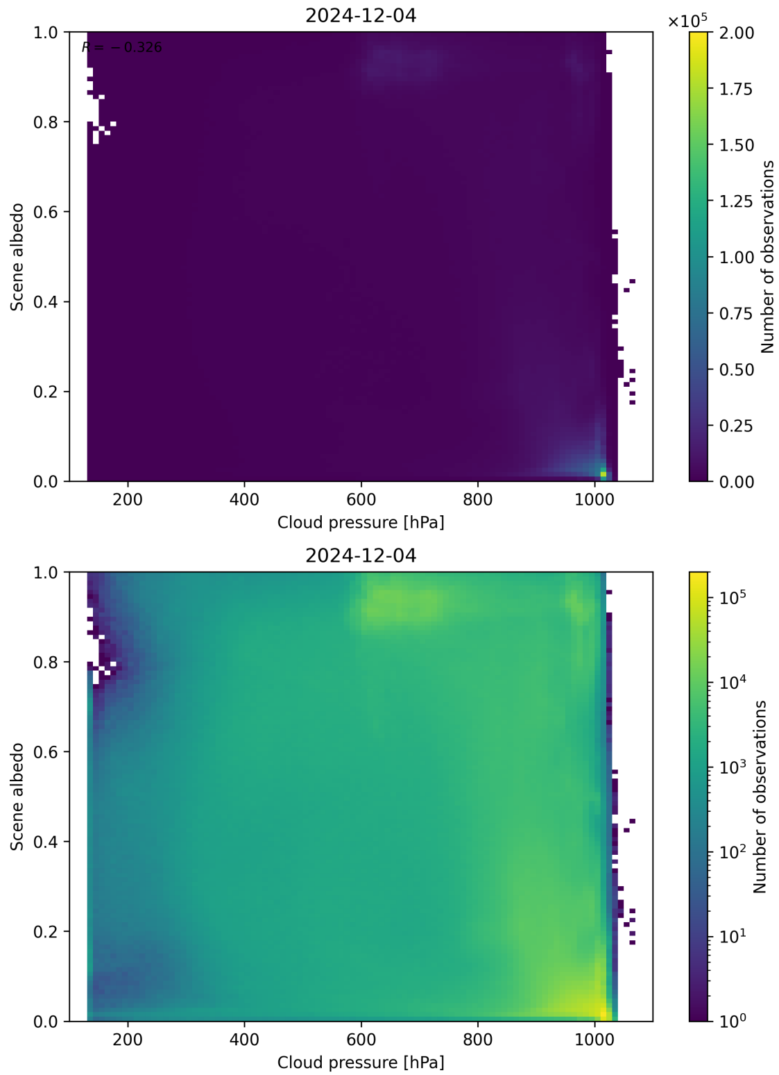
Figure 83: Scatter density plot of “Cloud pressure” against “Scene albedo” for 2024-12-03 to 2024-12-05.
