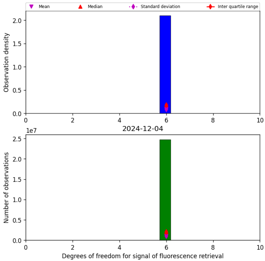
Figure 43: Histogram of “Degrees of freedom for signal of fluorescence retrieval” for 2024-12-03 to 2024-12-05
