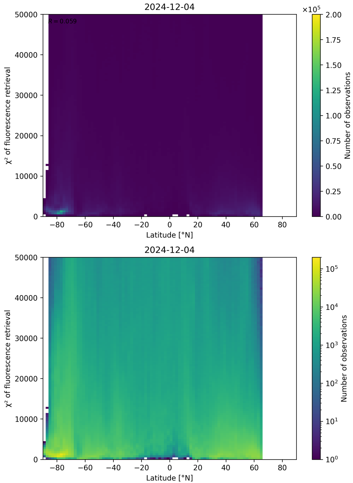
Figure 89: Scatter density plot of “Latitude” against “ \chi^2 of fluorescence retrieval” for 2024-12-03 to 2024-12-05.
