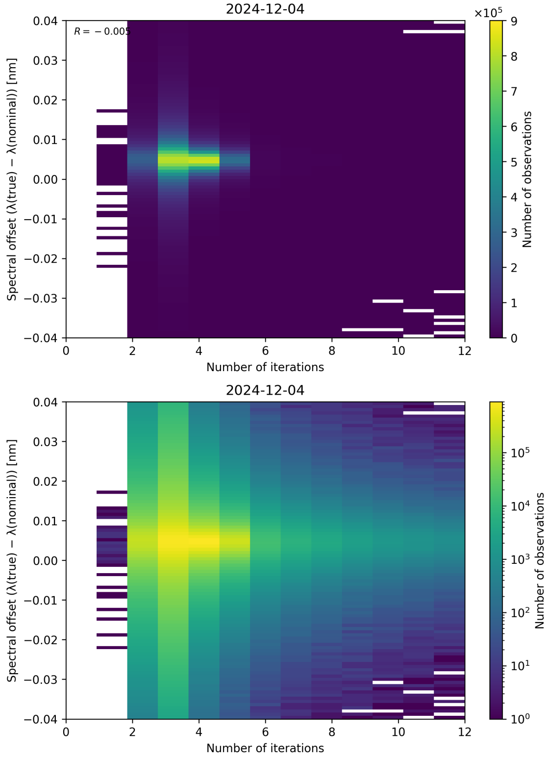
Figure 100: Scatter density plot of “Number of iterations” against “Spectral offset ( \lambda_{\text{true}} - \lambda_{\text{nominal}} )” for 2024-12-03 to 2024-12-05.
