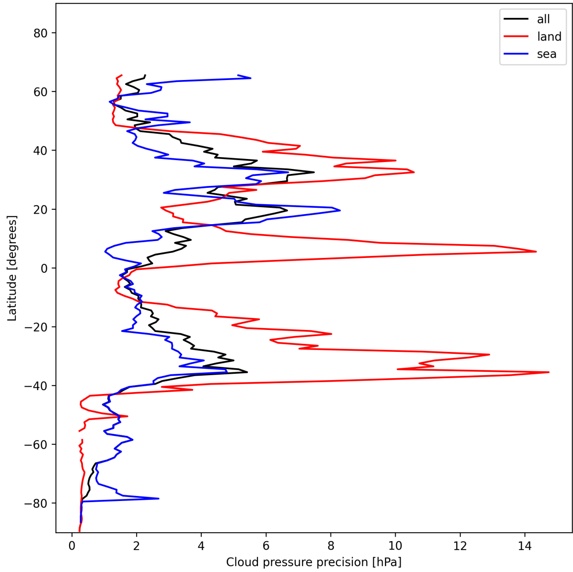
Figure 14: Zonal average of “Cloud pressure precision” for 2024-12-03 to 2024-12-05.
