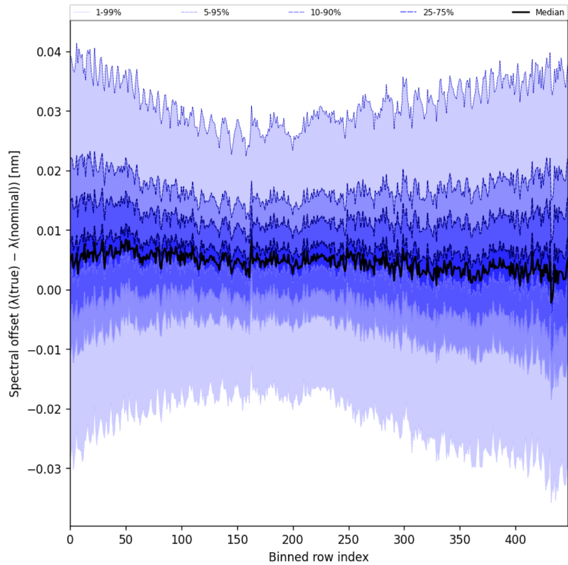
Figure 62: Along track statistics of “Spectral offset ( \lambda_{\text{true}} - \lambda_{\text{nominal}} )” for 2024-12-03 to 2024-12-05
