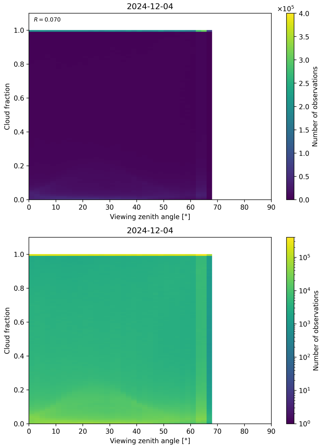
Figure 120: Scatter density plot of “Viewing zenith angle” against “Cloud fraction” for 2024-12-03 to 2024-12-05.
