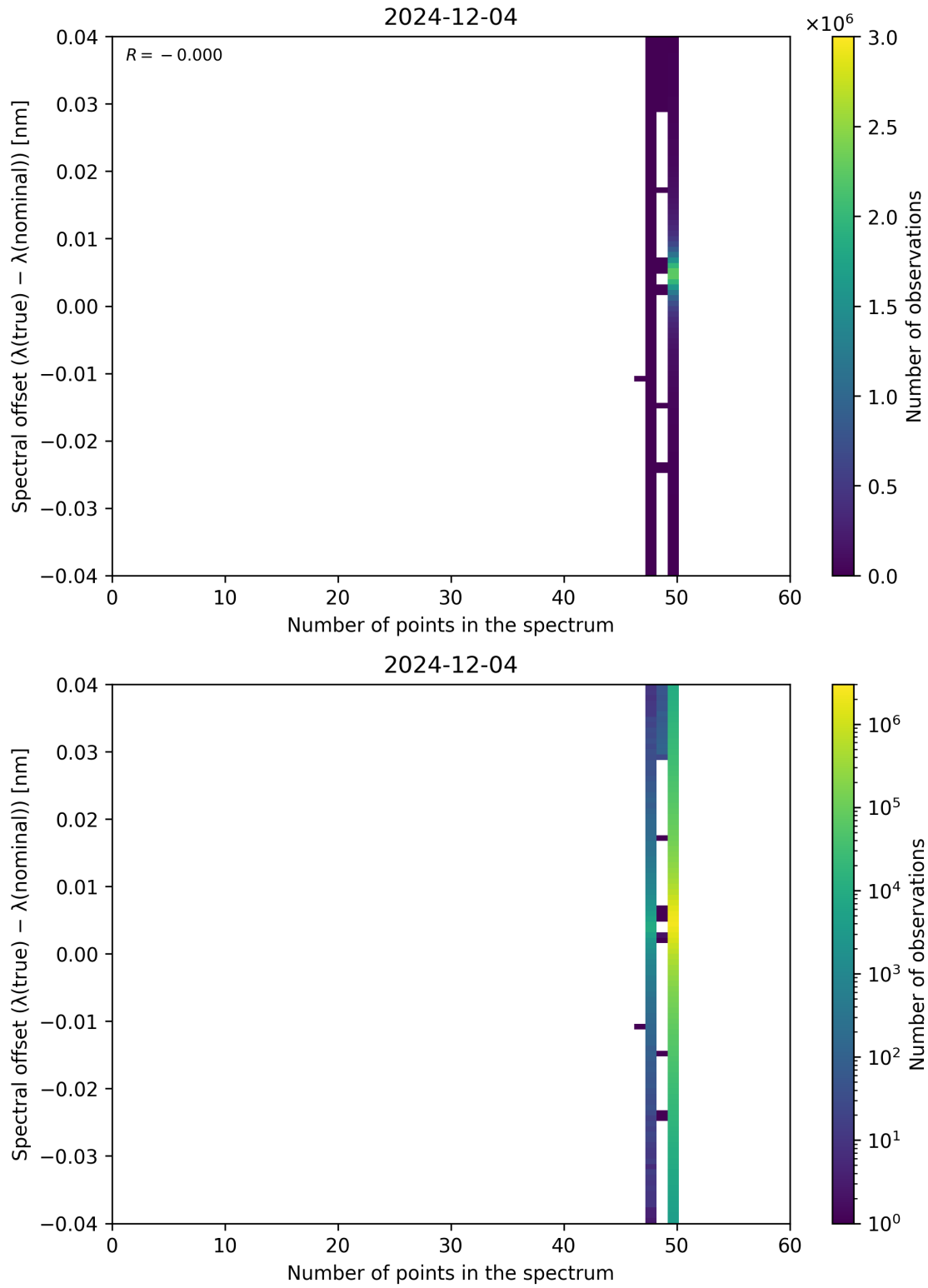
Figure 101: Scatter density plot of “Number of points in the spectrum” against “Spectral offset ( \lambda_{\text{true}} - \lambda_{\text{nominal}} )” for 2024-12-03 to 2024-12-05.
