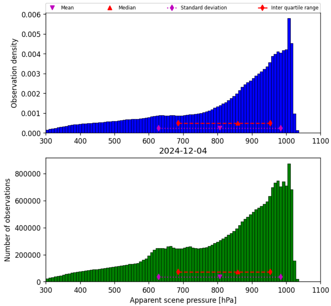
Figure 36: Histogram of “Apparent scene pressure” for 2024-12-03 to 2024-12-05
