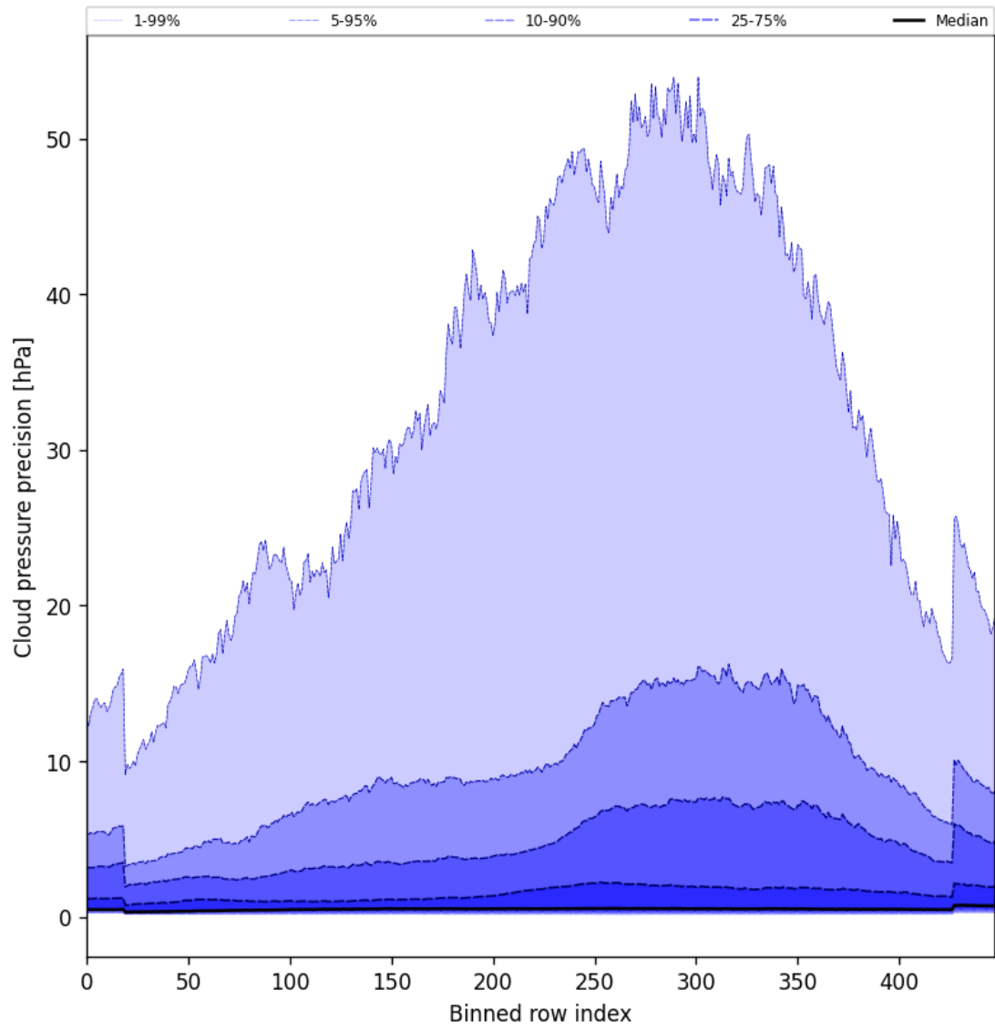
Figure 48: Along track statistics of “Cloud pressure precision” for 2024-12-03 to 2024-12-05
