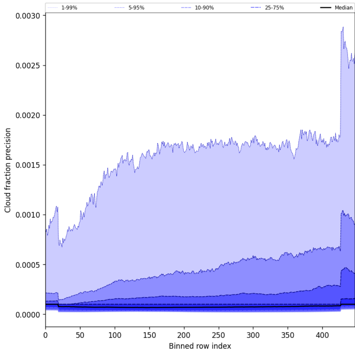
Figure 50: Along track statistics of “Cloud fraction precision” for 2024-12-03 to 2024-12-05
