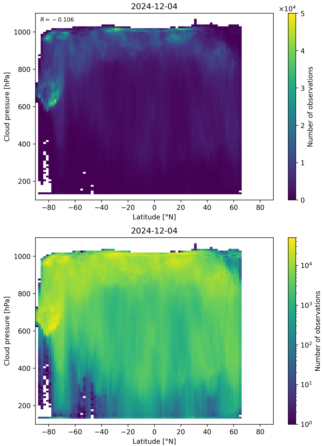
Figure 91: Scatter density plot of “Latitude” against “Cloud pressure” for 2024-12-03 to 2024-12-05.
