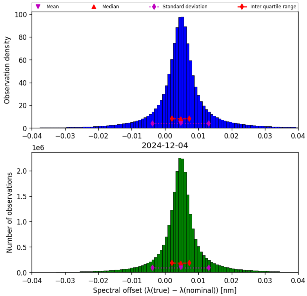
Figure 45: Histogram of “Spectral offset ( \lambda_{\text{true}} - \lambda_{\text{nominal}} )” for 2024-12-03 to 2024-12-05
