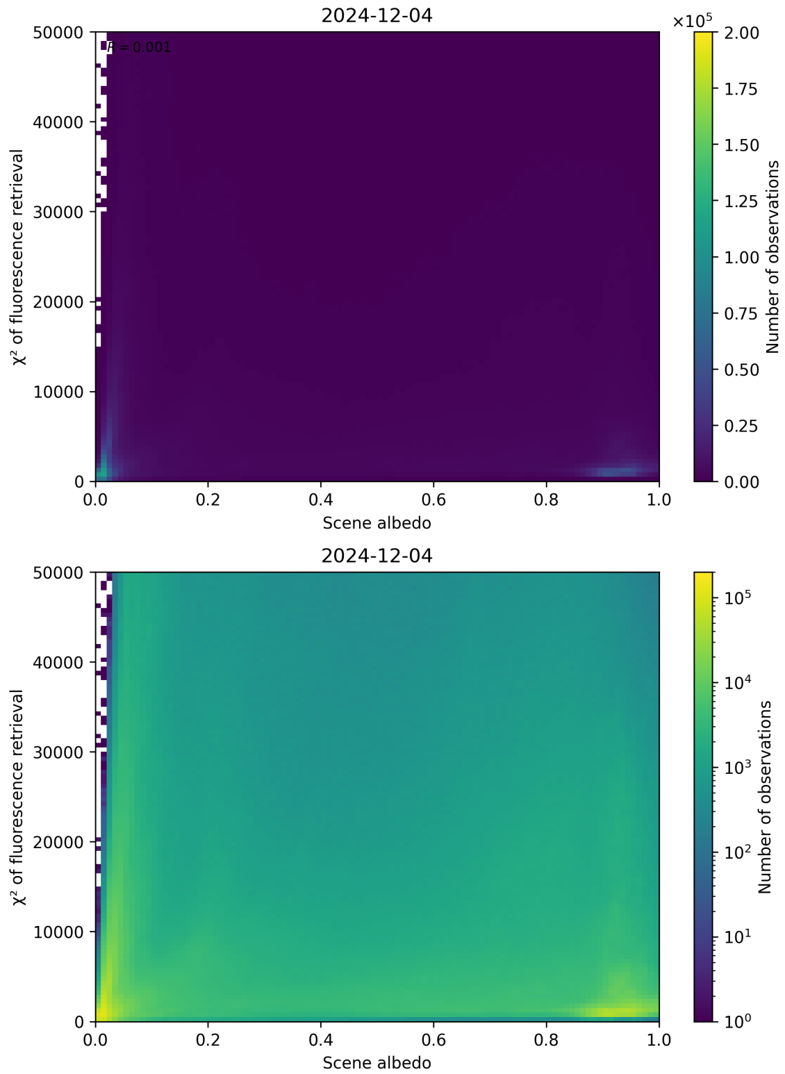
Figure 103: Scatter density plot of “Scene albedo” against “ \chi^2 of fluorescence retrieval” for 2024-12-03 to 2024-12-05.
