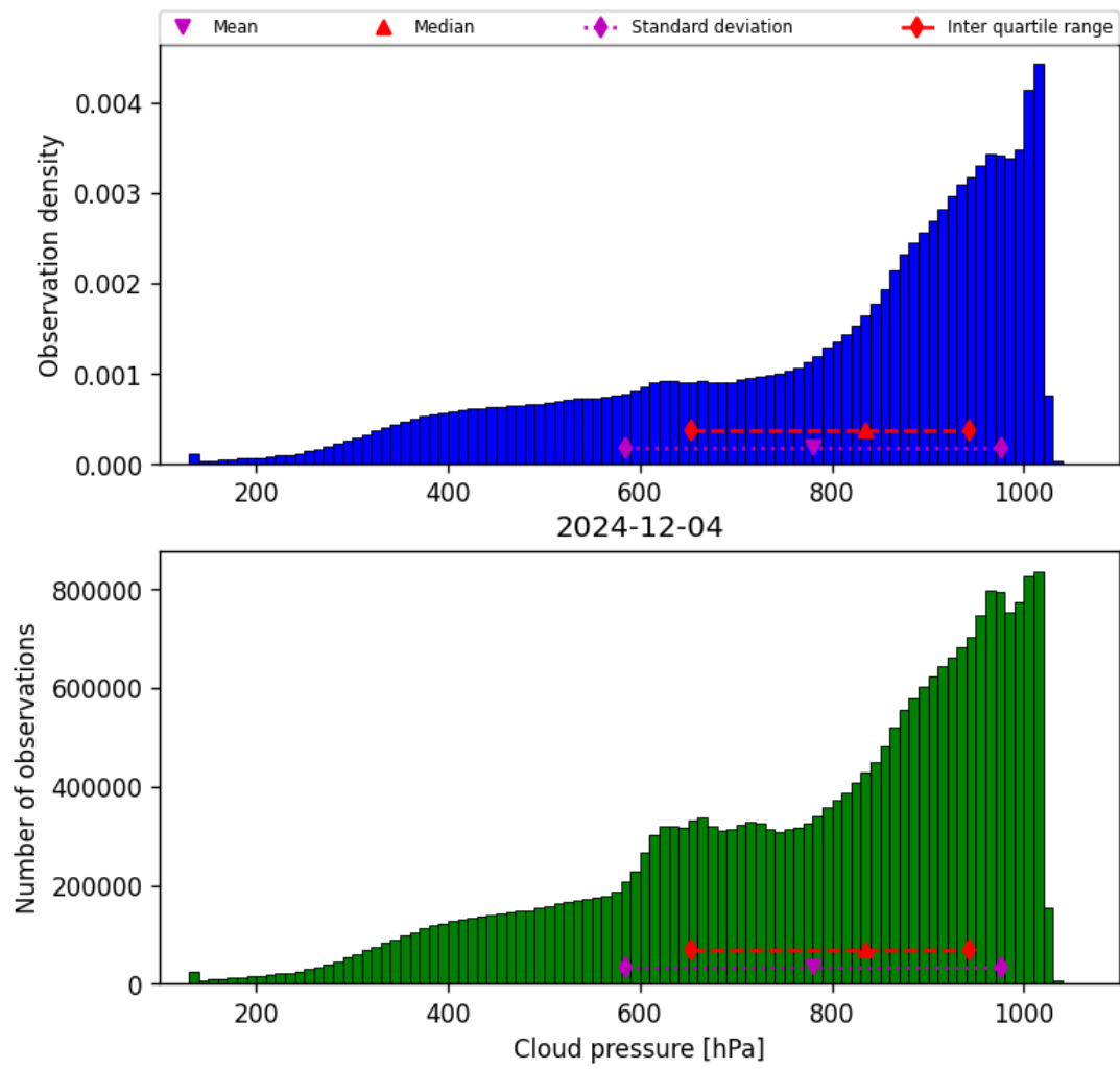
Figure 30: Histogram of “Cloud pressure” for 2024-12-03 to 2024-12-05
