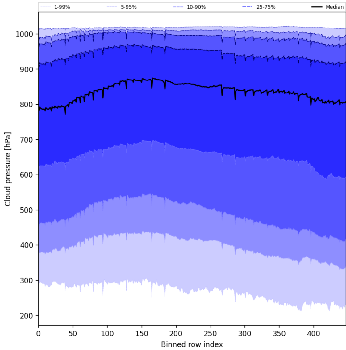
Figure 47: Along track statistics of “Cloud pressure” for 2024-12-03 to 2024-12-05
