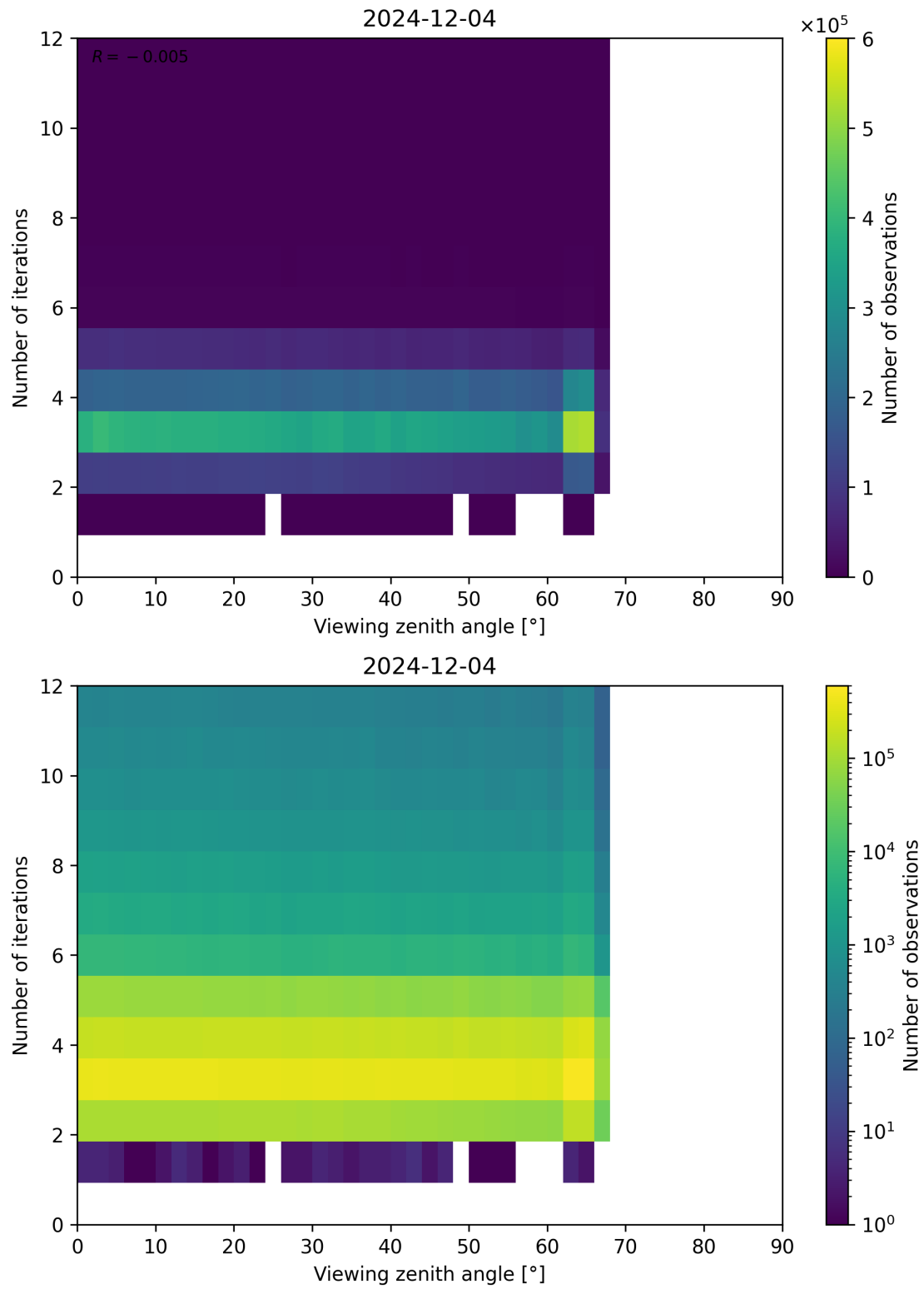
Figure 124: Scatter density plot of “Viewing zenith angle” against “Number of iterations” for 2024-12-03 to 2024-12-05.
