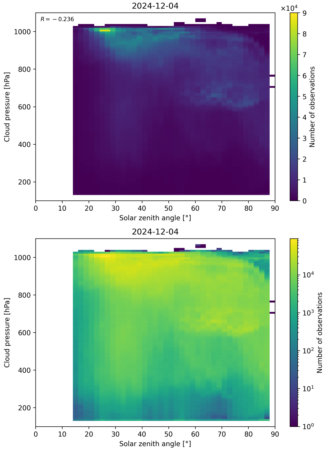
Figure 111: Scatter density plot of “Solar zenith angle” against “Cloud pressure” for 2024-12-03 to 2024-12-05.
