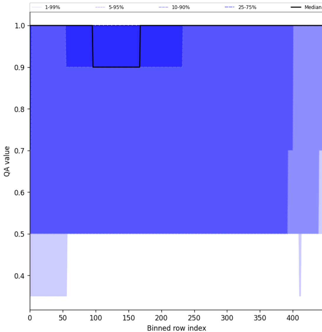
Figure 46: Along track statistics of “QA value” for 2024-12-03 to 2024-12-05
