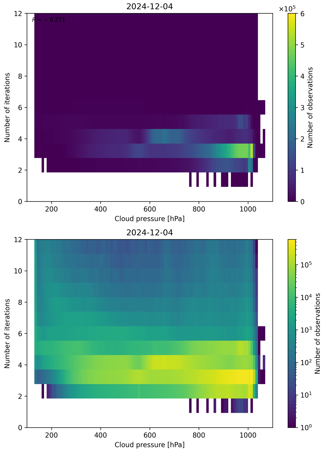
Figure 81: Scatter density plot of “Cloud pressure” against “Number of iterations” for 2024-12-03 to 2024-12-05.
