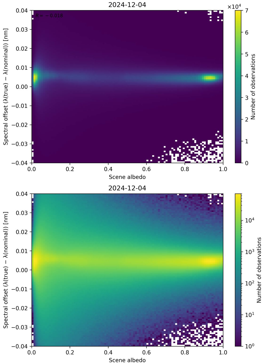
Figure 107: Scatter density plot of “Scene albedo” against “Spectral offset ( \lambda_{\text{true}} - \lambda_{\text{nominal}} )” for 2024-12-03 to 2024-12-05.
