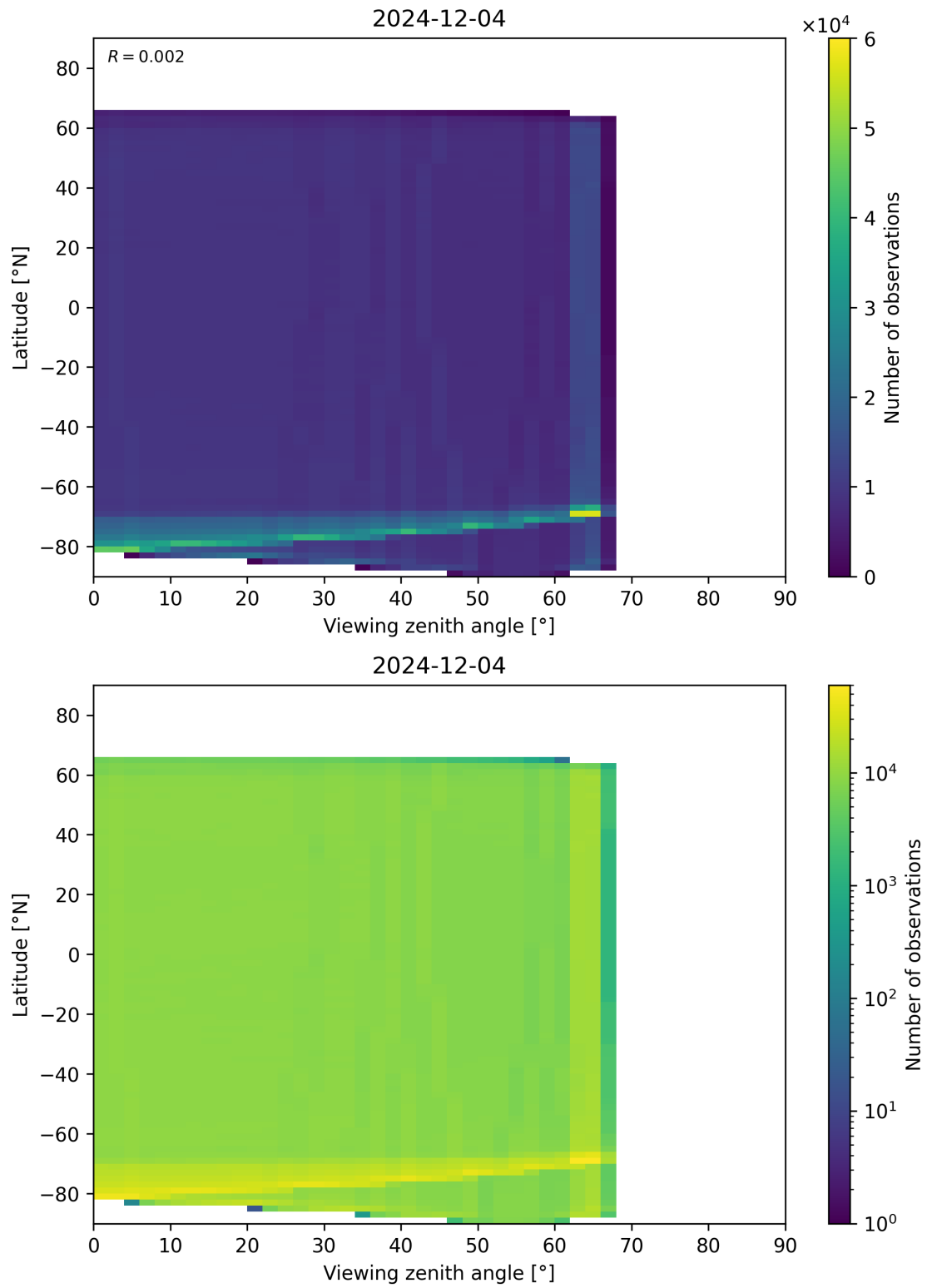
Figure 123: Scatter density plot of “Viewing zenith angle” against “Latitude” for 2024-12-03 to 2024-12-05.
