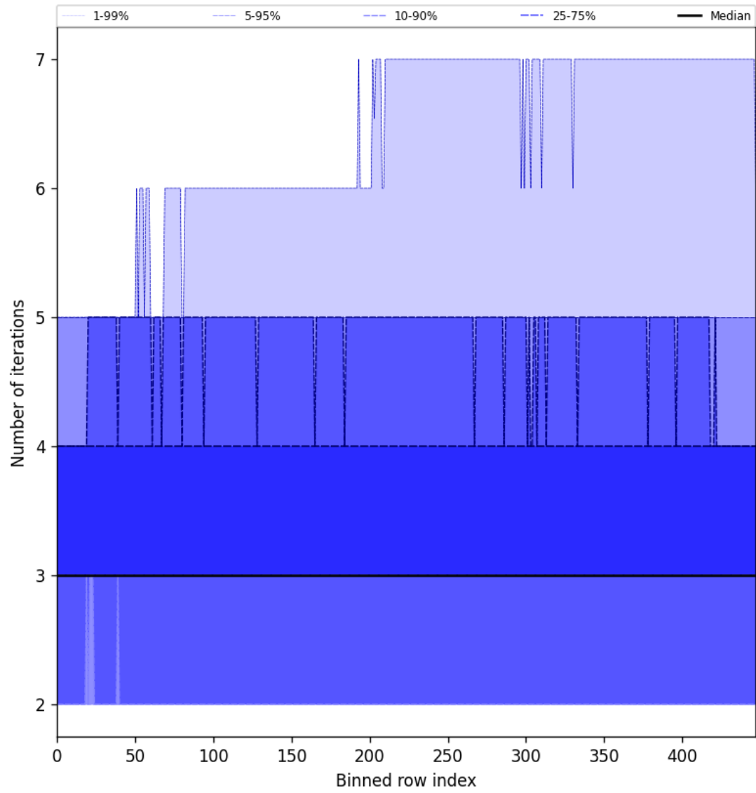
Figure 56: Along track statistics of “Number of iterations” for 2024-12-03 to 2024-12-05
