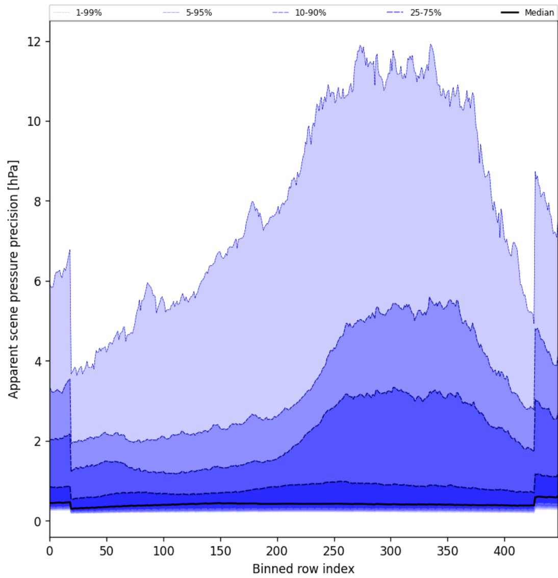
Figure 54: Along track statistics of “Apparent scene pressure precision” for 2024-12-03 to 2024-12-05
