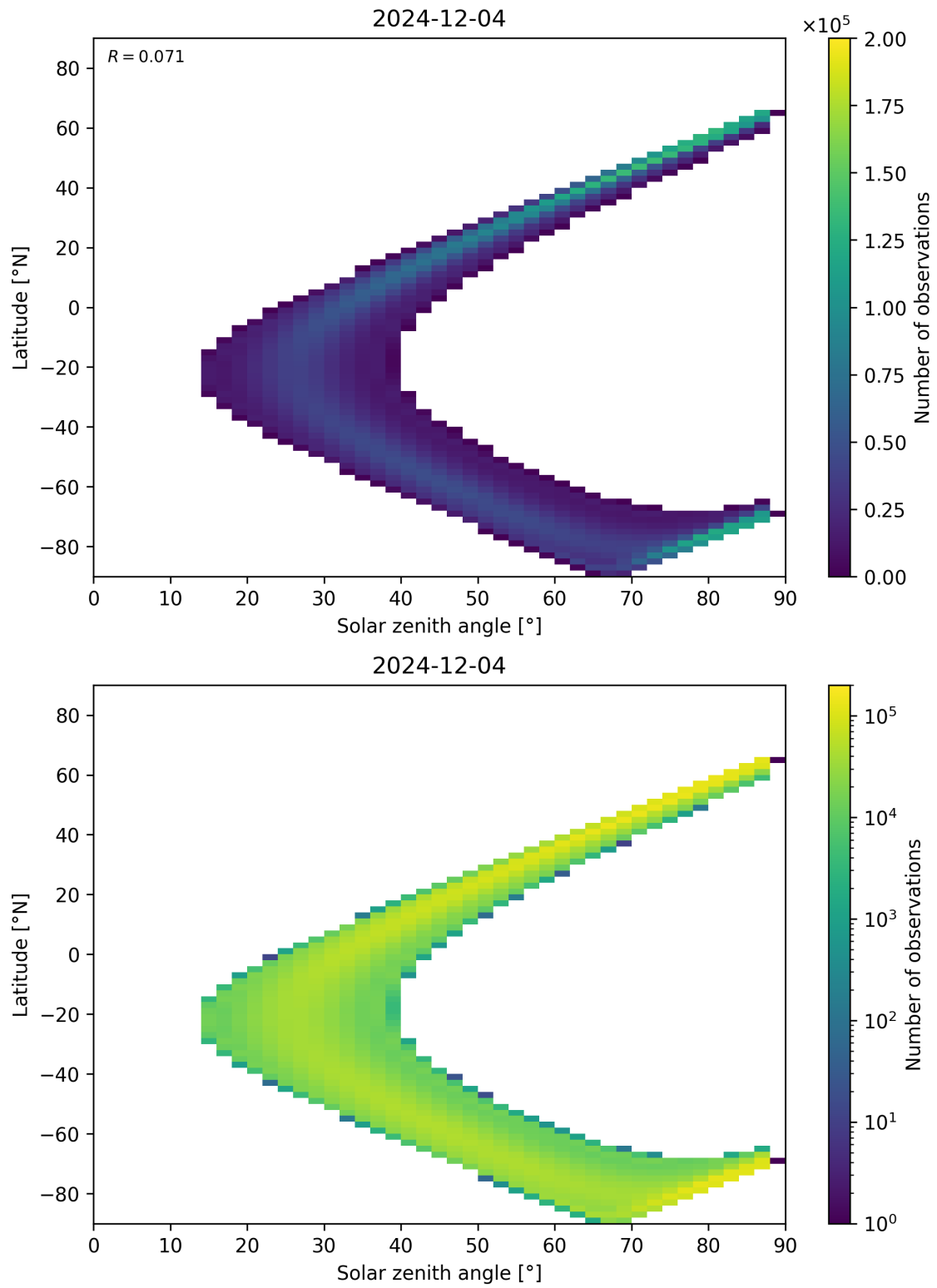
Figure 113: Scatter density plot of “Solar zenith angle” against “Latitude” for 2024-12-03 to 2024-12-05.
