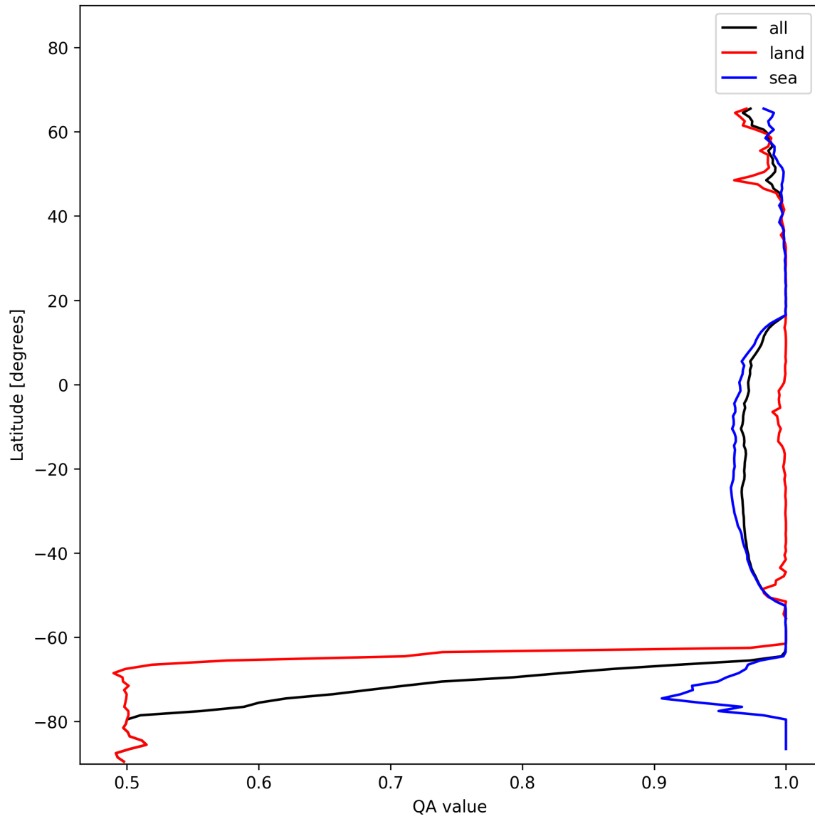
Figure 12: Zonal average of “QA value” for 2024-12-03 to 2024-12-05.
