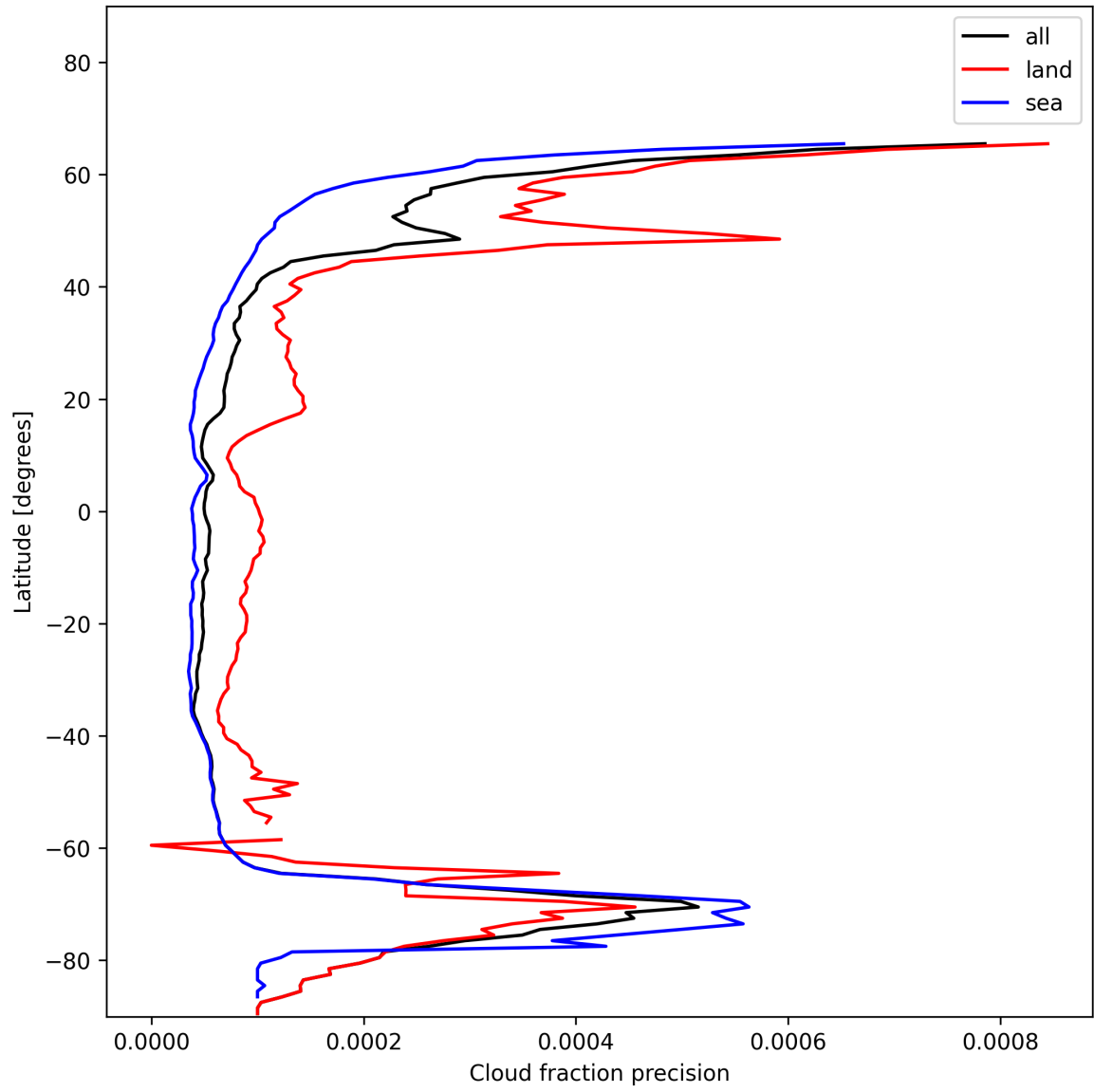
Figure 16: Zonal average of “Cloud fraction precision” for 2024-12-03 to 2024-12-05.
