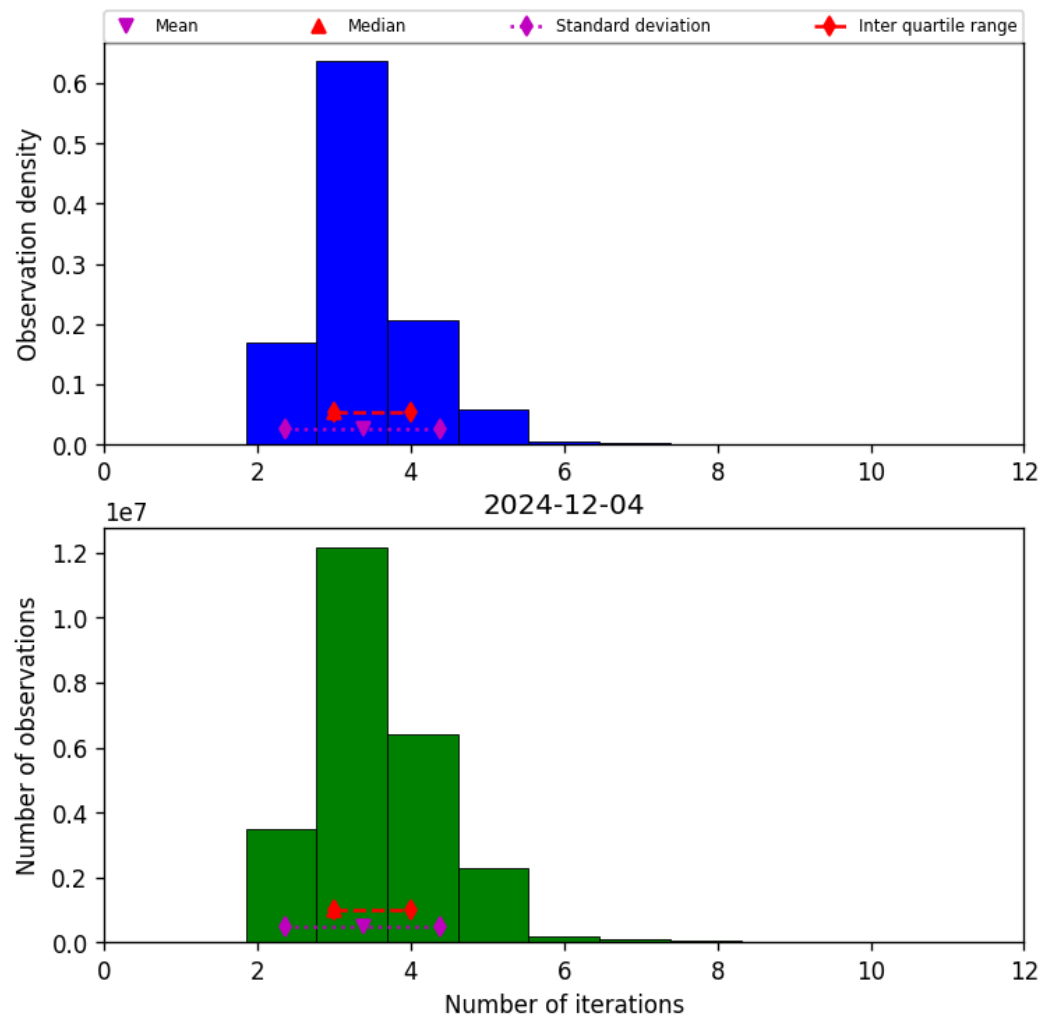
Figure 39: Histogram of “Number of iterations” for 2024-12-03 to 2024-12-05
