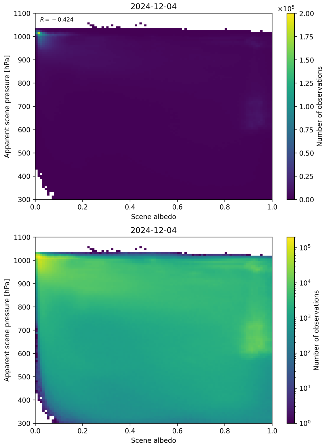
Figure 102: Scatter density plot of “Scene albedo” against “Apparent scene pressure” for 2024-12-03 to 2024-12-05.
