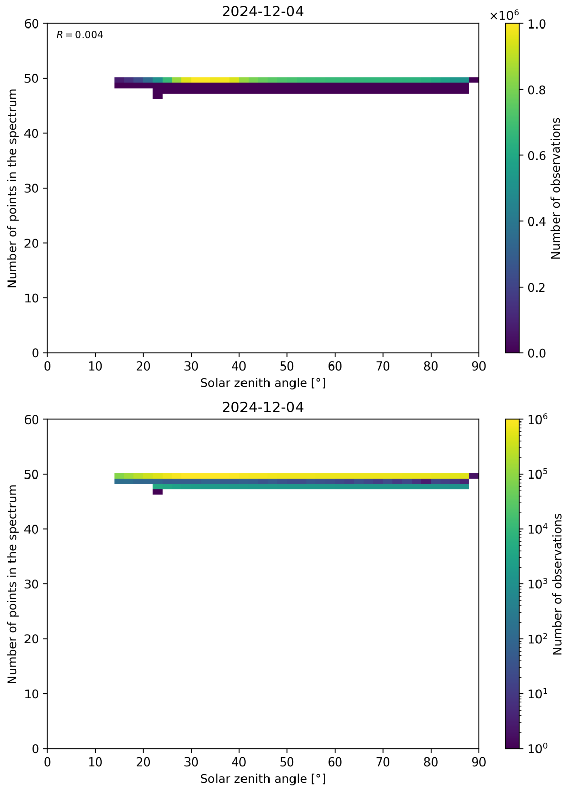
Figure 115: Scatter density plot of “Solar zenith angle” against “Number of points in the spectrum” for 2024-12-03 to 2024-12-05.
