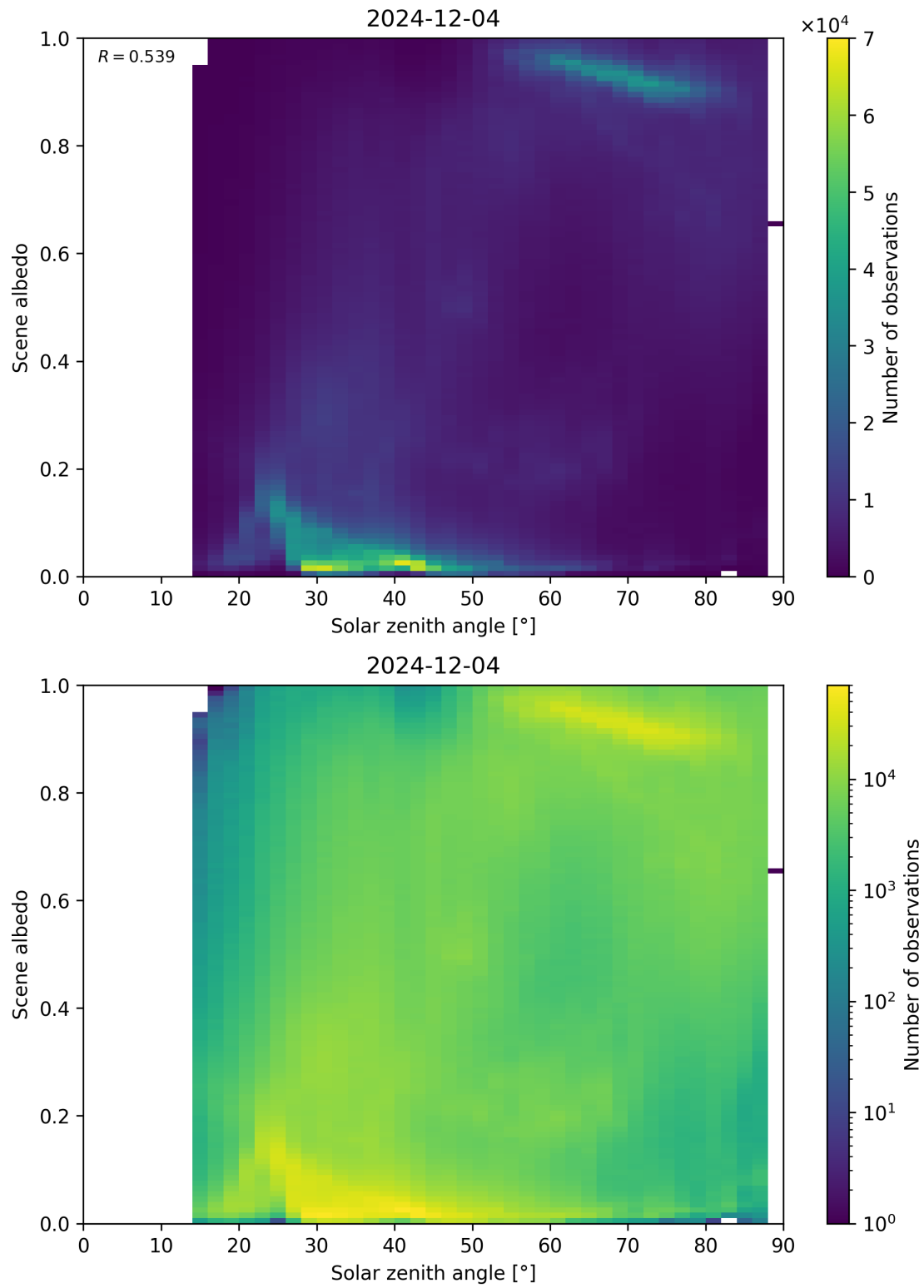
Figure 116: Scatter density plot of “Solar zenith angle” against “Scene albedo” for 2024-12-03 to 2024-12-05.
