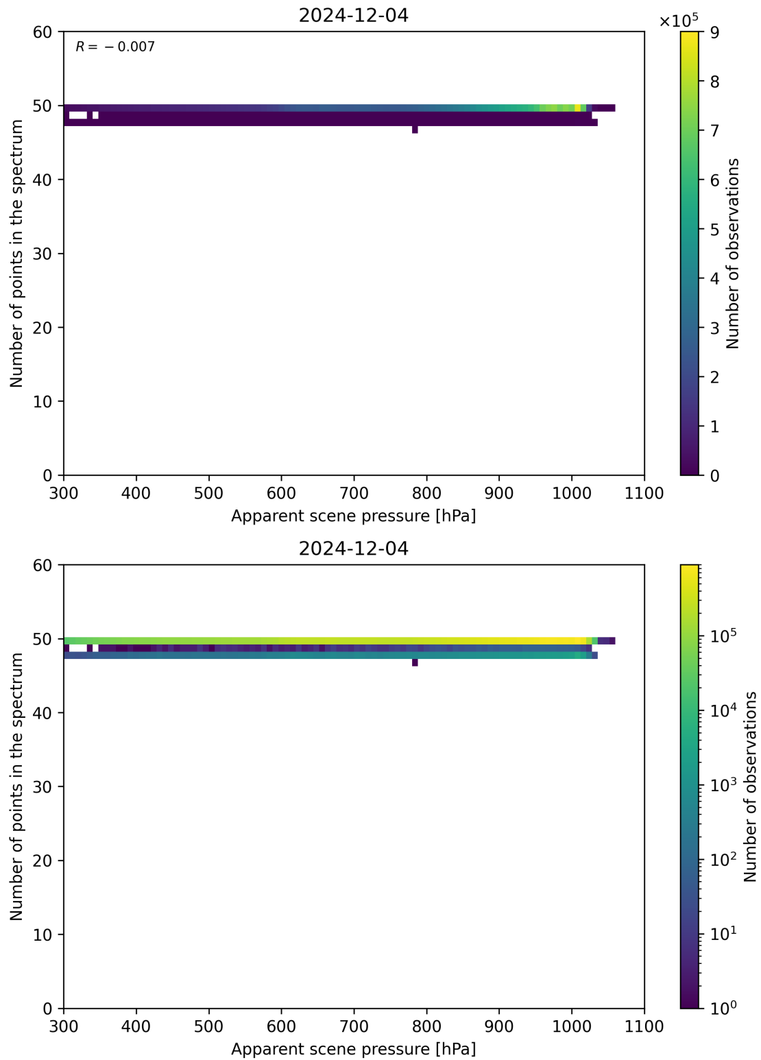
Figure 66: Scatter density plot of “Apparent scene pressure” against “Number of points in the spectrum” for 2024-12-03 to 2024-12-05.
