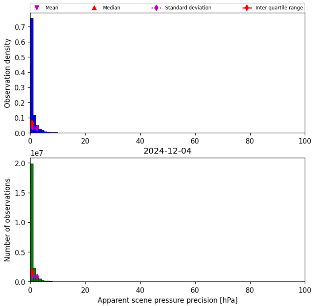
Figure 37: Histogram of “Apparent scene pressure precision” for 2024-12-03 to 2024-12-05
