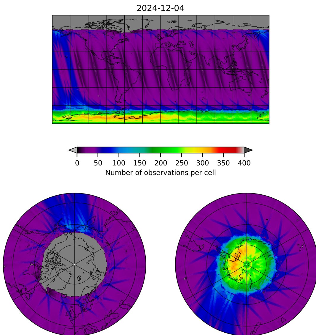
Figure 11: Map of the number of observations for 2024-12-03 to 2024-12-05
