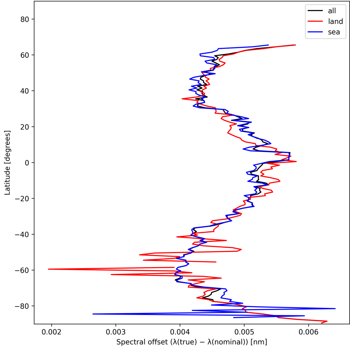
Figure 28: Zonal average of “Spectral offset ( \lambda_{\text{true}} - \lambda_{\text{nominal}} )” for 2024-12-03 to 2024-12-05.
