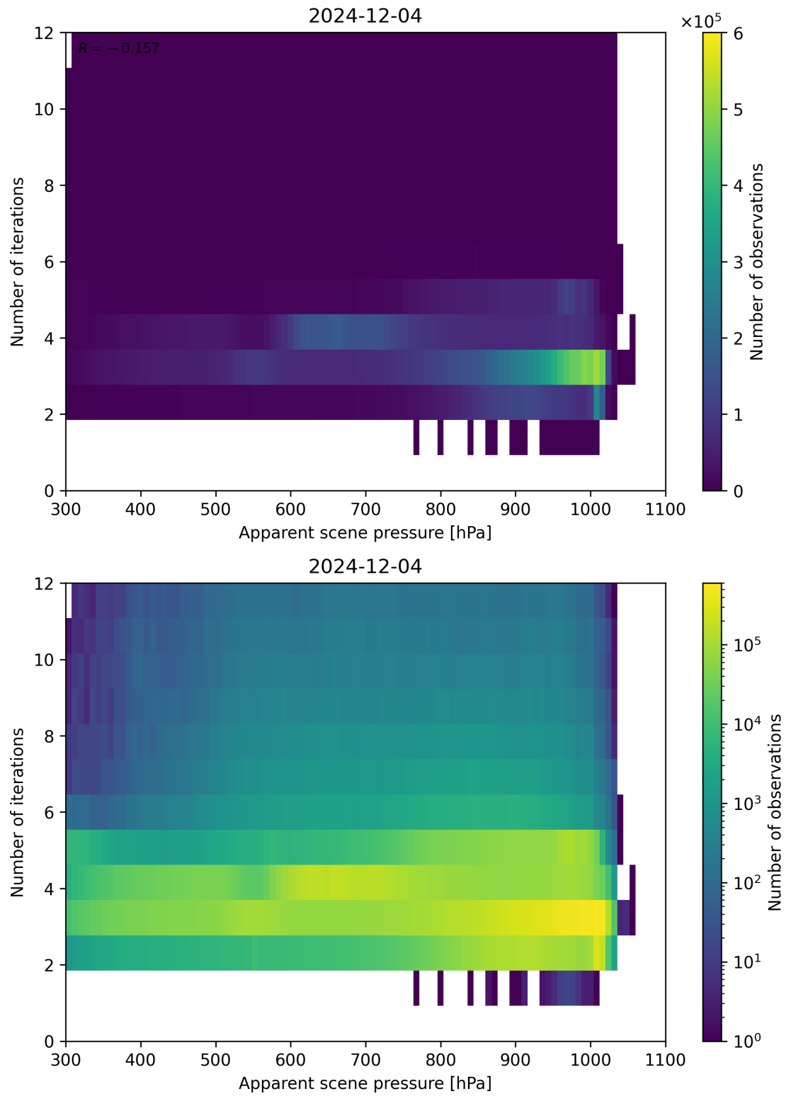
Figure 65: Scatter density plot of “Apparent scene pressure” against “Number of iterations” for 2024-12-03 to 2024-12-05.
