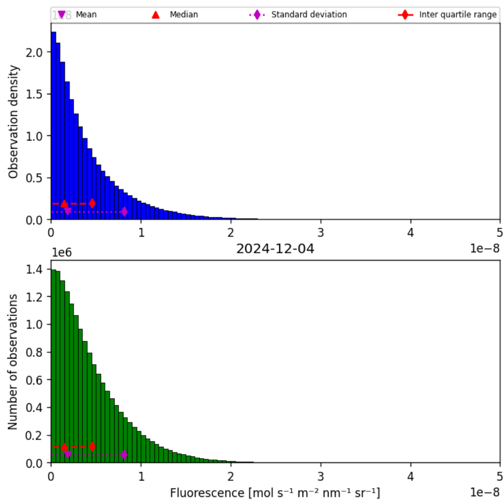
Figure 40: Histogram of “Fluorescence” for 2024-12-03 to 2024-12-05
