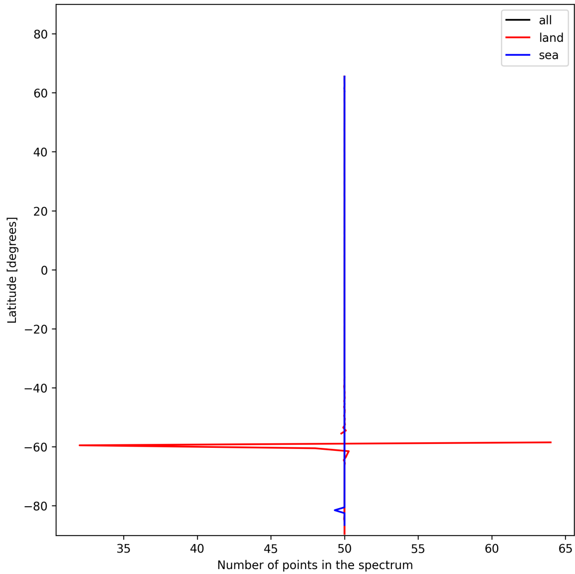
Figure 27: Zonal average of “Number of points in the spectrum” for 2024-12-03 to 2024-12-05.
