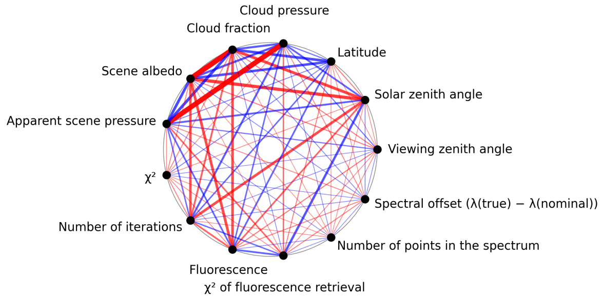
Figure 1: Map of correlation graph for 2024-12-03 to 2024-12-05.
