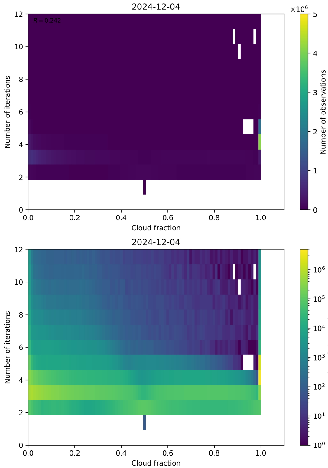
Figure 73: Scatter density plot of “Cloud fraction” against “Number of iterations” for 2024-12-03 to 2024-12-05.
