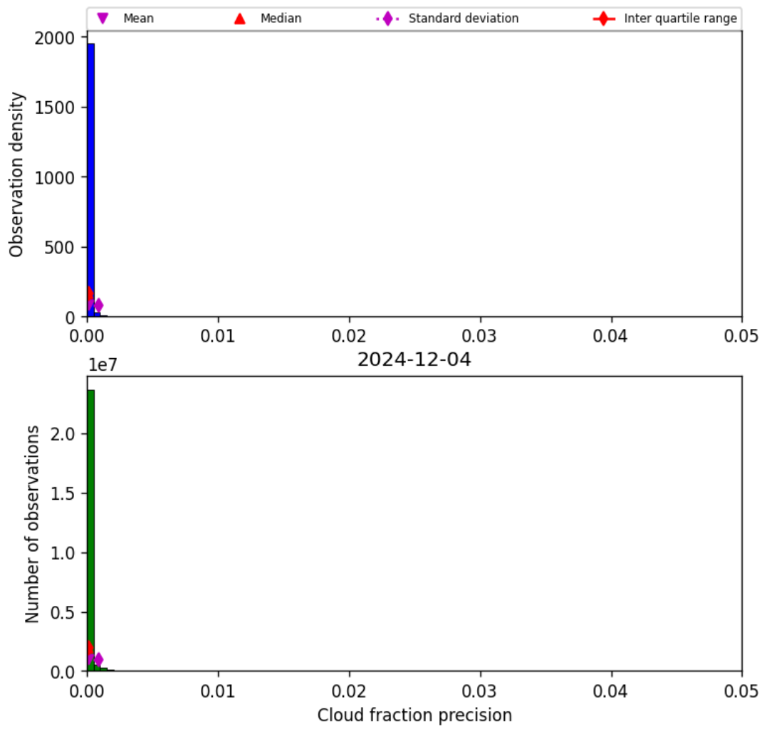
Figure 33: Histogram of “Cloud fraction precision” for 2024-12-03 to 2024-12-05
