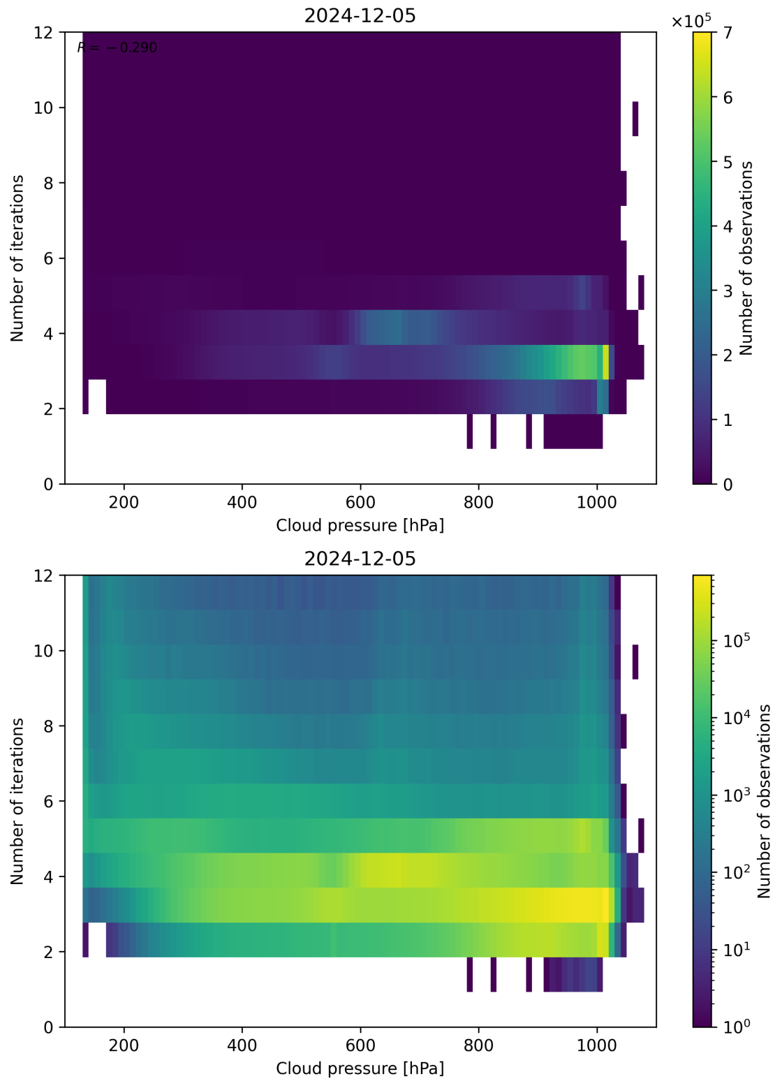
Figure 81: Scatter density plot of “Cloud pressure” against “Number of iterations” for 2024-12-04 to 2024-12-06.
