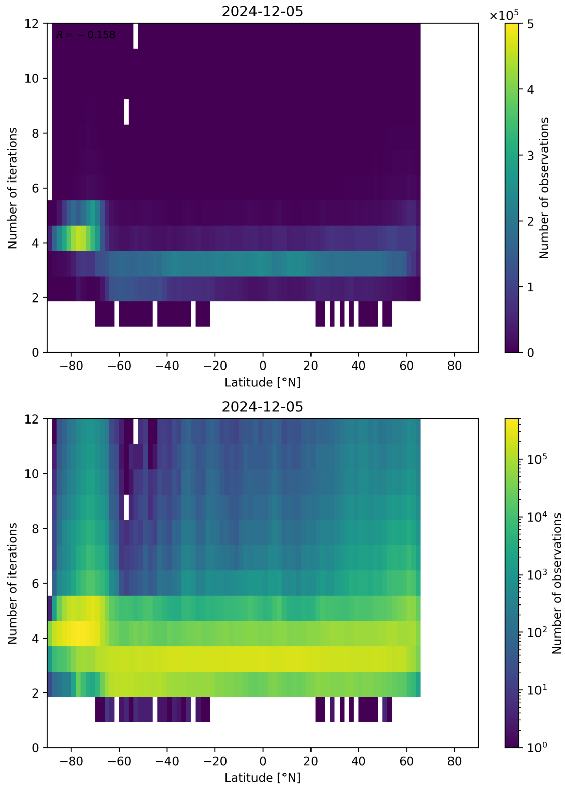
Figure 93: Scatter density plot of “Latitude” against “Number of iterations” for 2024-12-04 to 2024-12-06.
