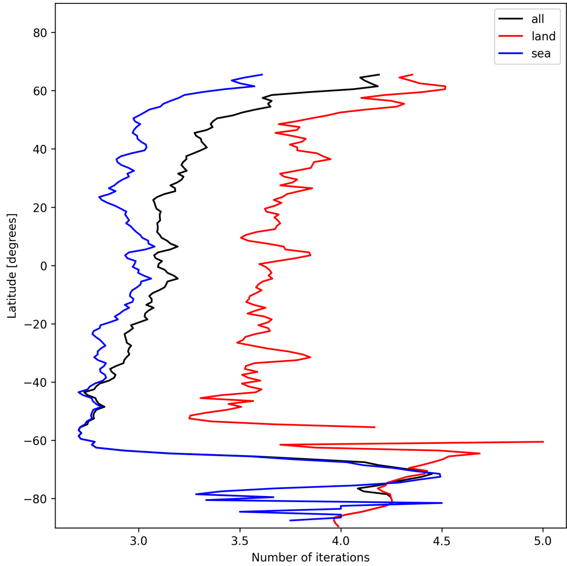
Figure 22: Zonal average of “Number of iterations” for 2024-12-04 to 2024-12-06.
