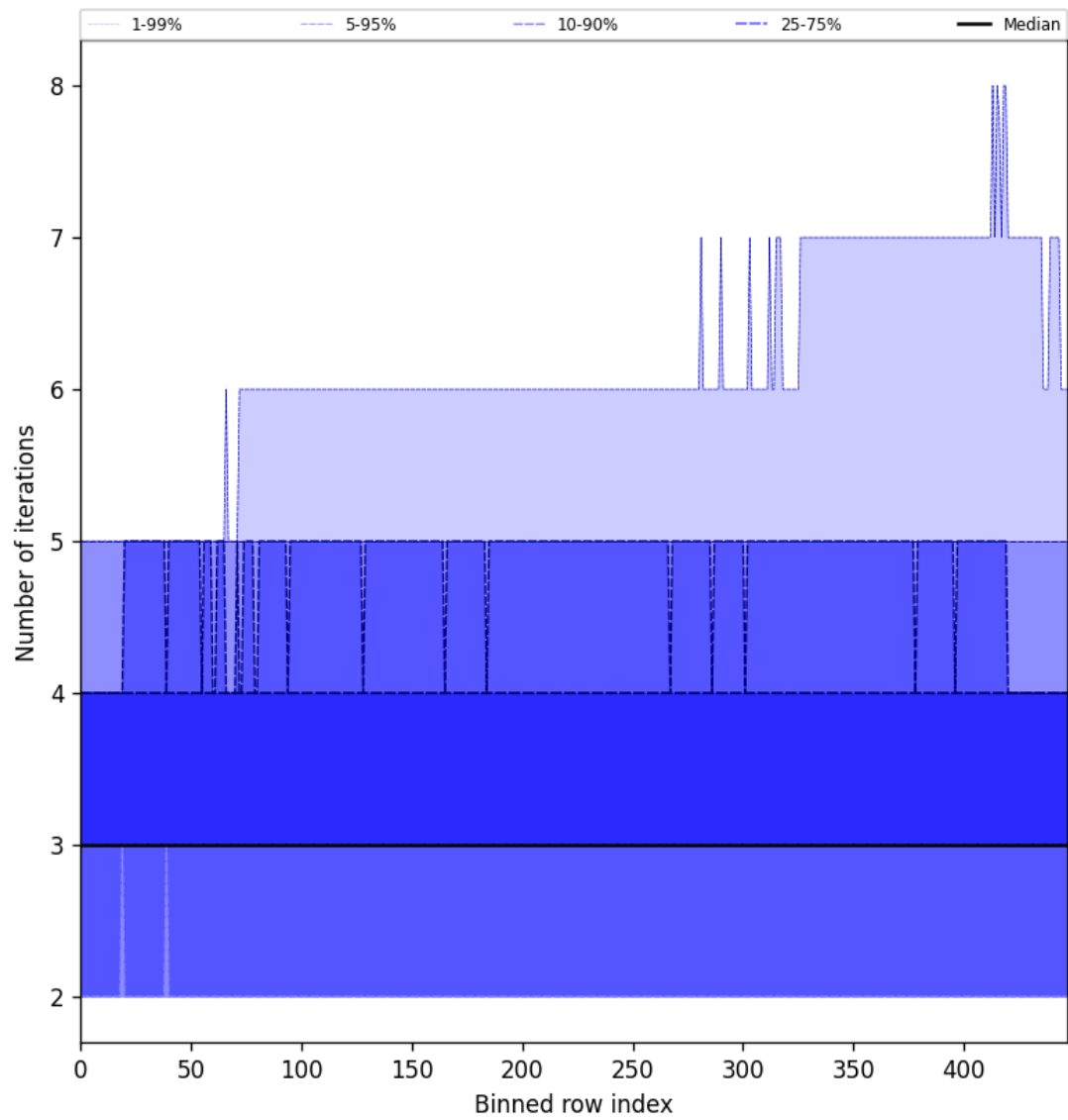
Figure 56: Along track statistics of “Number of iterations” for 2024-12-04 to 2024-12-06
