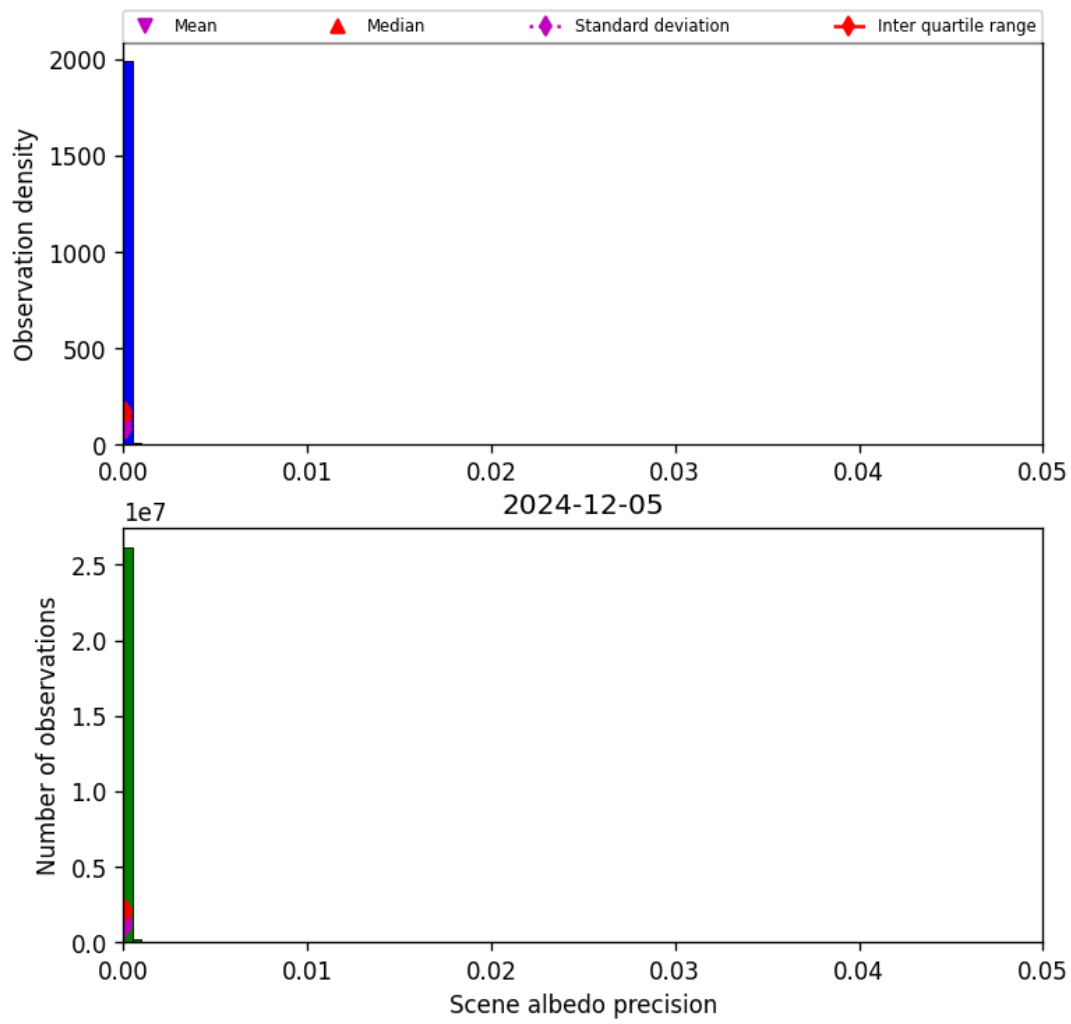
Figure 35: Histogram of “Scene albedo precision” for 2024-12-04 to 2024-12-06
