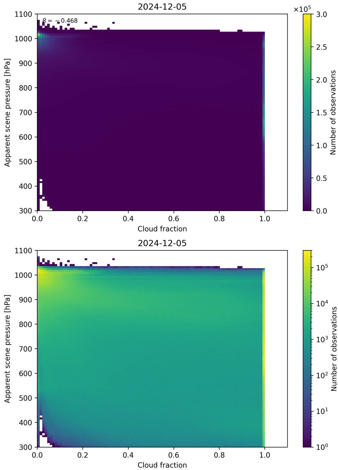
Figure 70: Scatter density plot of “Cloud fraction” against “Apparent scene pressure” for 2024-12-04 to 2024-12-06.
