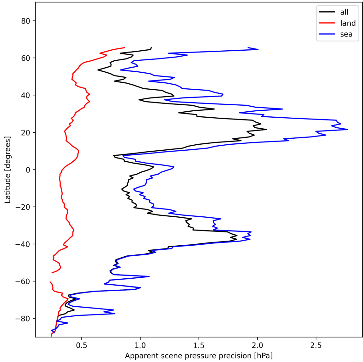
Figure 20: Zonal average of “Apparent scene pressure precision” for 2024-12-04 to 2024-12-06.
