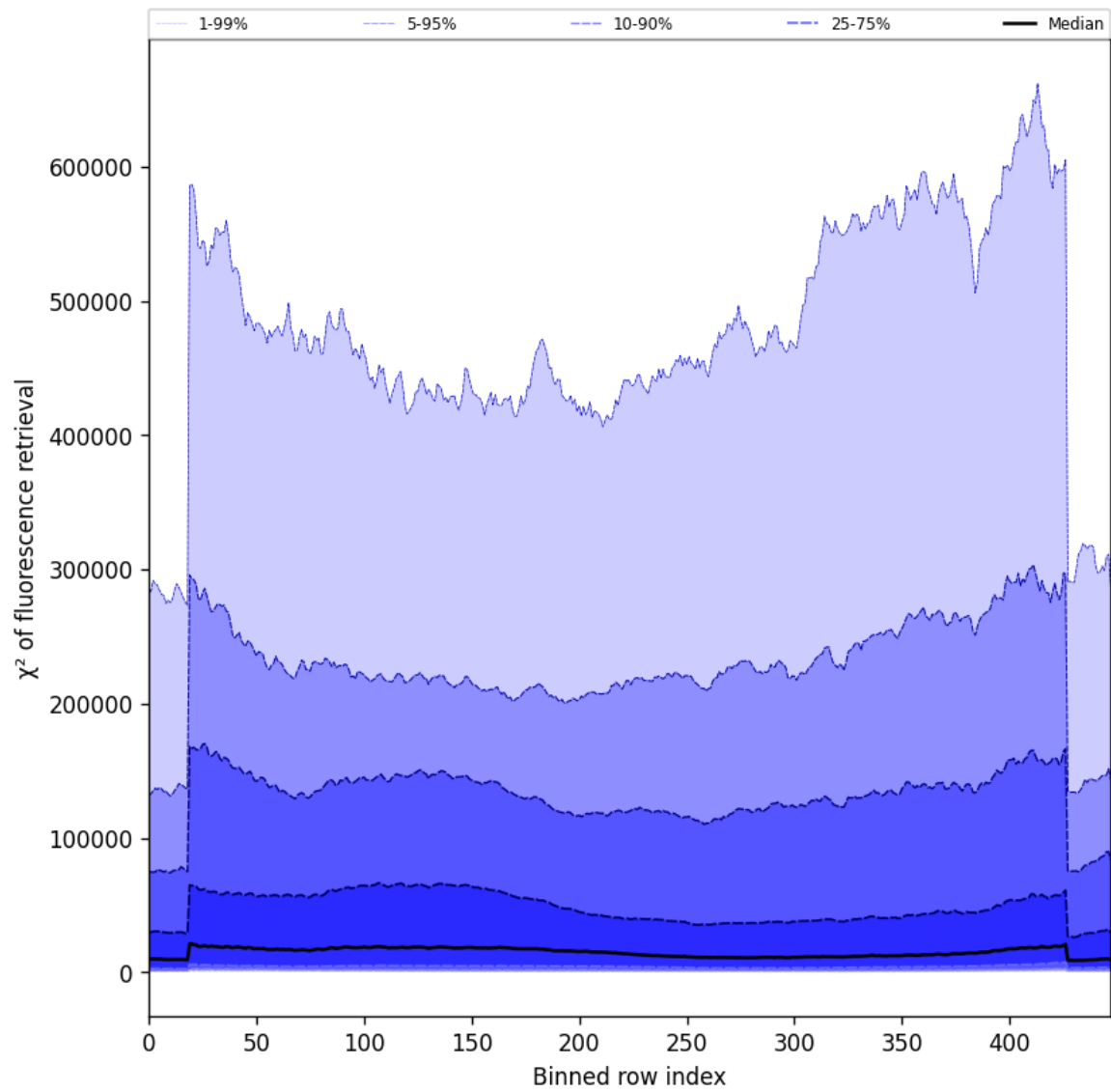
Figure 59: Along track statistics of “ \chi^2 of fluorescence retrieval” for 2024-12-04 to 2024-12-06
