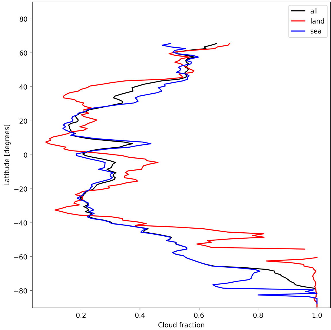
Figure 15: Zonal average of “Cloud fraction” for 2024-12-04 to 2024-12-06.
