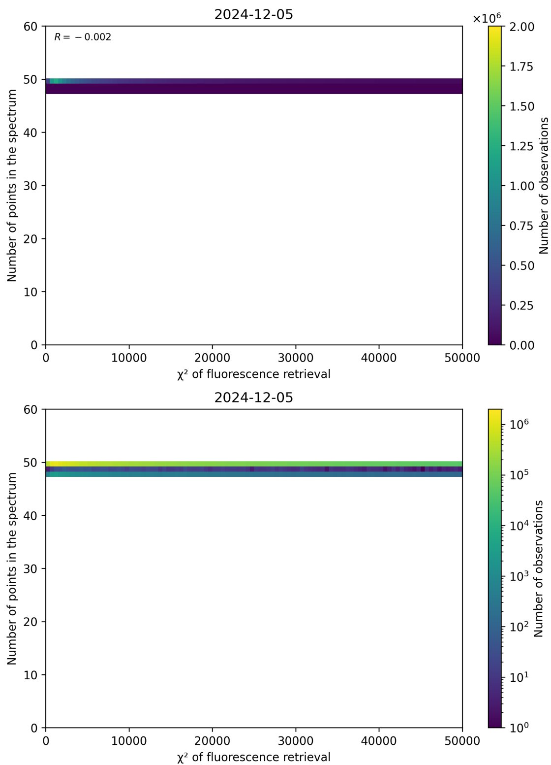
Figure 68: Scatter density plot of " \chi^2 of fluorescence retrieval" against "Number of points in the spectrum" for 2024-12-04 to 2024-12-06.
