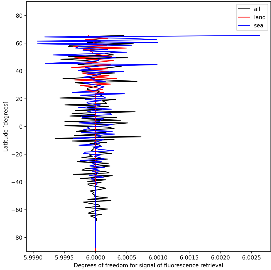
Figure 26: Zonal average of “Degrees of freedom for signal of fluorescence retrieval” for 2024-12-04 to 2024-12-06.
