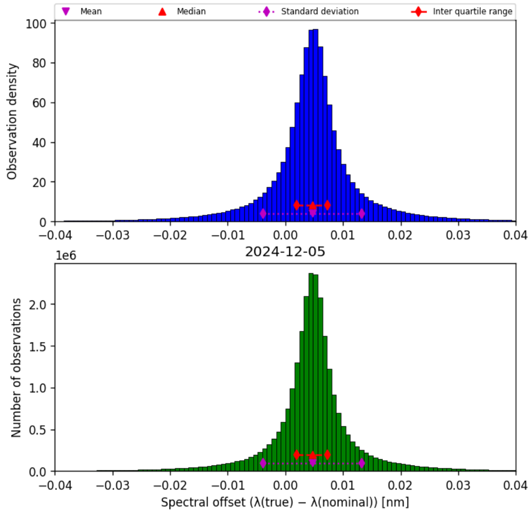
Figure 45: Histogram of “Spectral offset ( \lambda_{\text{true}} - \lambda_{\text{nominal}} )” for 2024-12-04 to 2024-12-06
