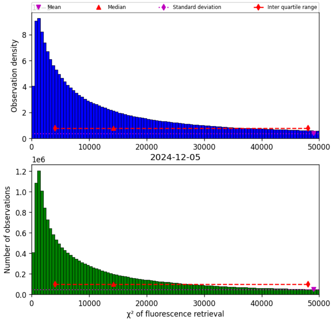
Figure 42: Histogram of “ \chi^2 of fluorescence retrieval” for 2024-12-04 to 2024-12-06
