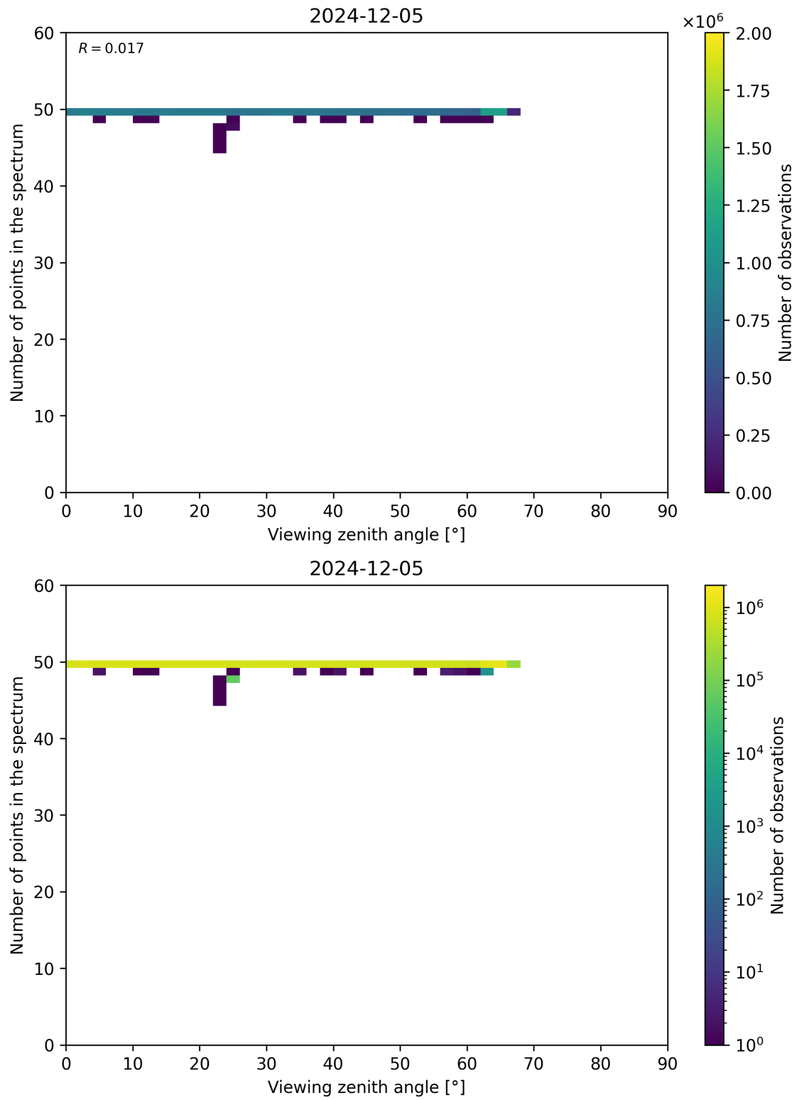
Figure 125: Scatter density plot of “Viewing zenith angle” against “Number of points in the spectrum” for 2024-12-04 to 2024-12-06.
