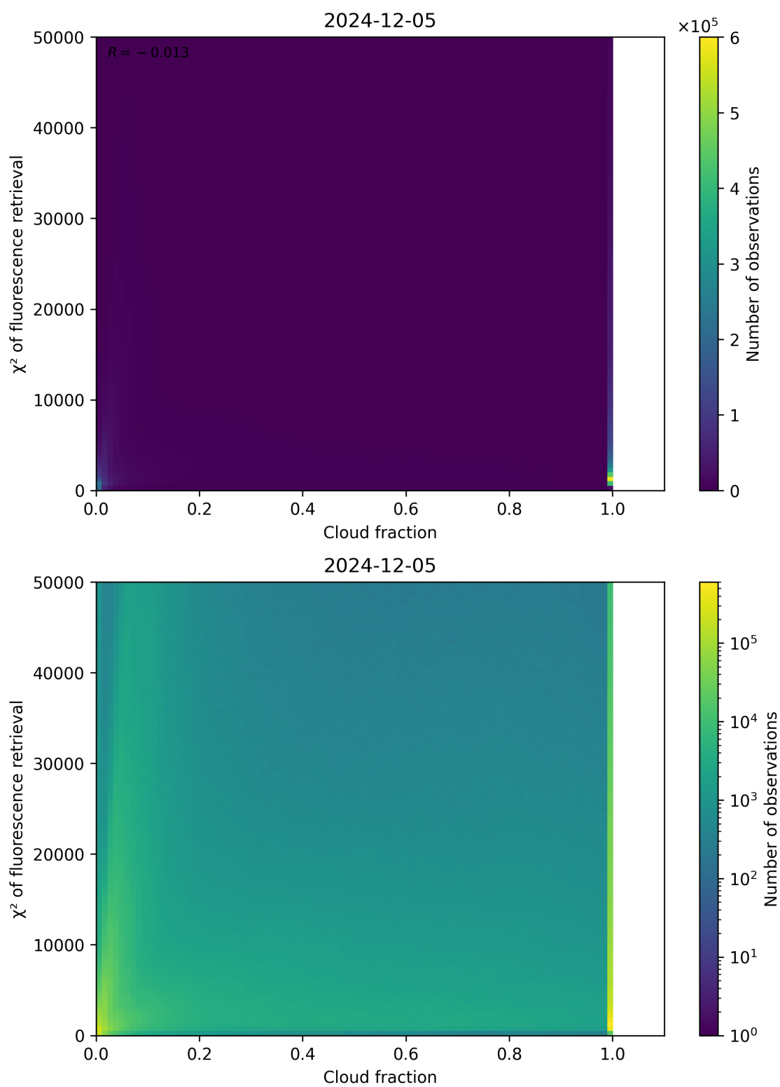
Figure 71: Scatter density plot of “Cloud fraction” against “ \chi^2 of fluorescence retrieval” for 2024-12-04 to 2024-12-06.
