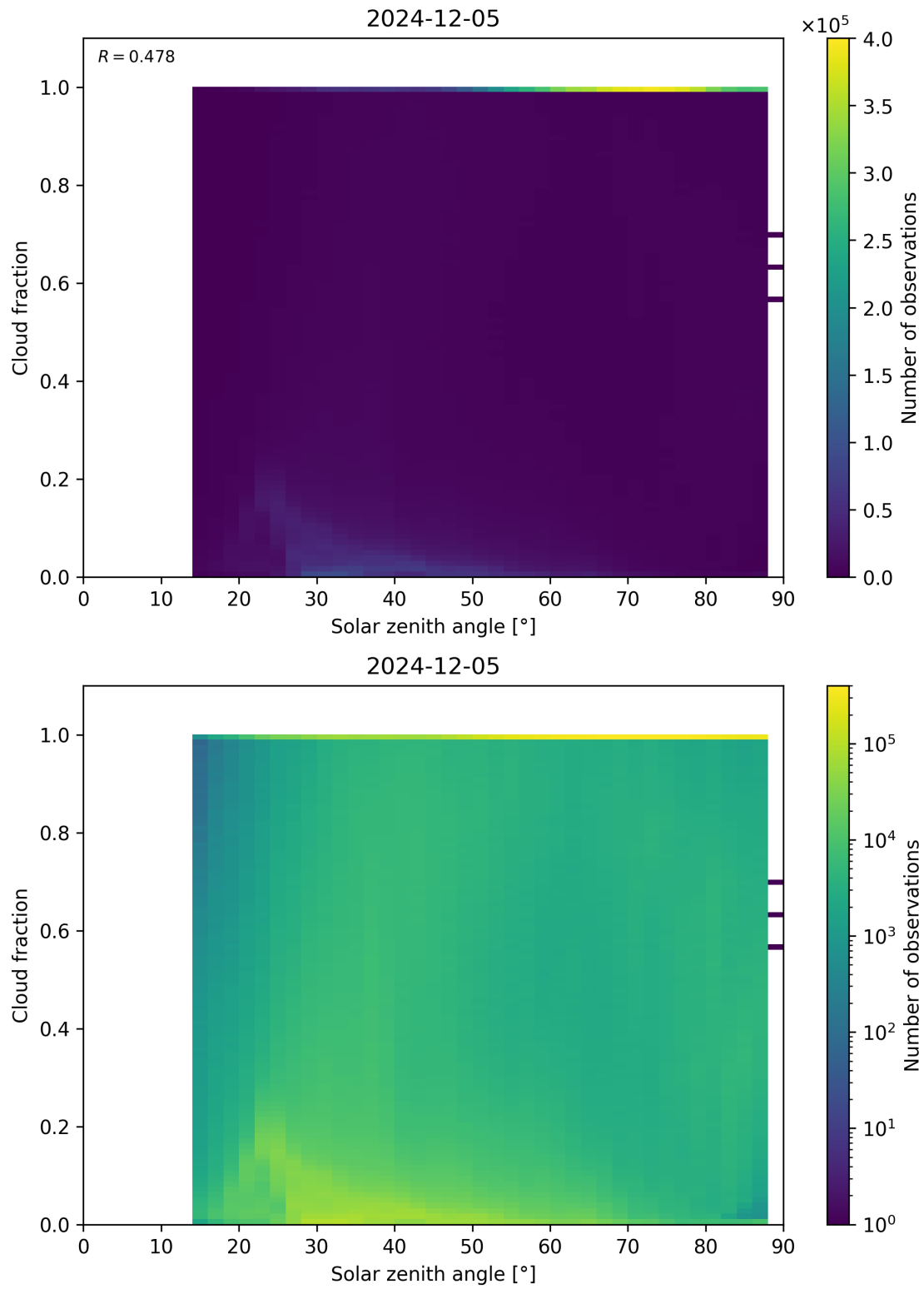
Figure 110: Scatter density plot of “Solar zenith angle” against “Cloud fraction” for 2024-12-04 to 2024-12-06.
