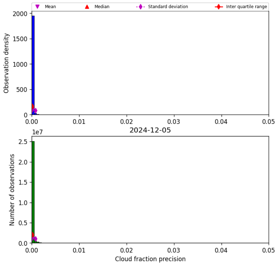
Figure 33: Histogram of “Cloud fraction precision” for 2024-12-04 to 2024-12-06
