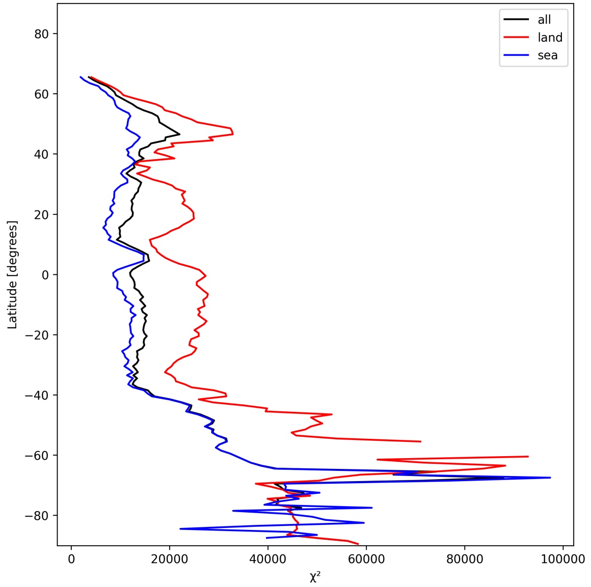
Figure 21: Zonal average of “ \chi^2 ” for 2024-12-04 to 2024-12-06.
