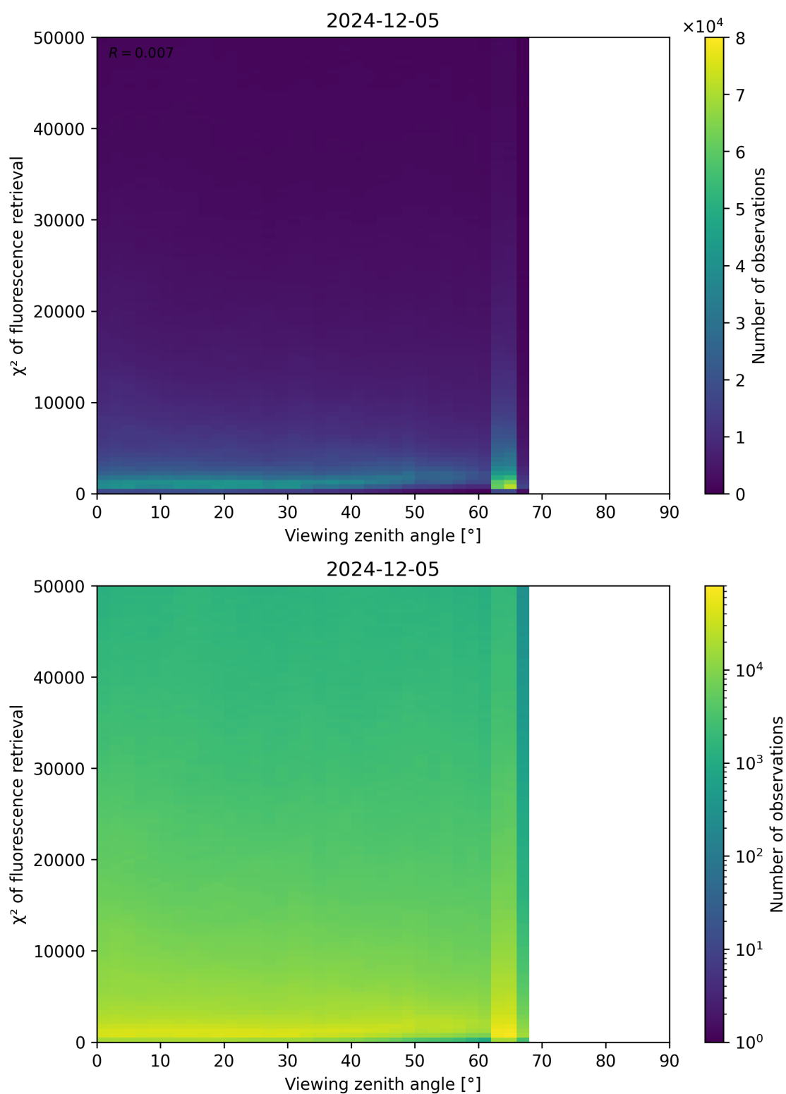
Figure 119: Scatter density plot of “Viewing zenith angle” against “ \chi^2 of fluorescence retrieval” for 2024-12-04 to 2024-12-06.
