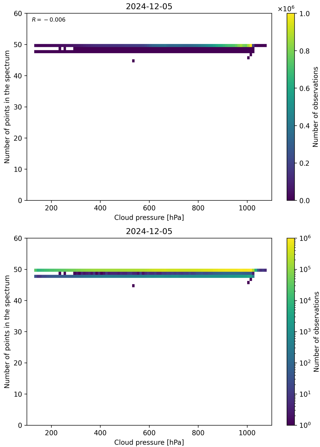
Figure 82: Scatter density plot of “Cloud pressure” against “Number of points in the spectrum” for 2024-12-04 to 2024-12-06.
