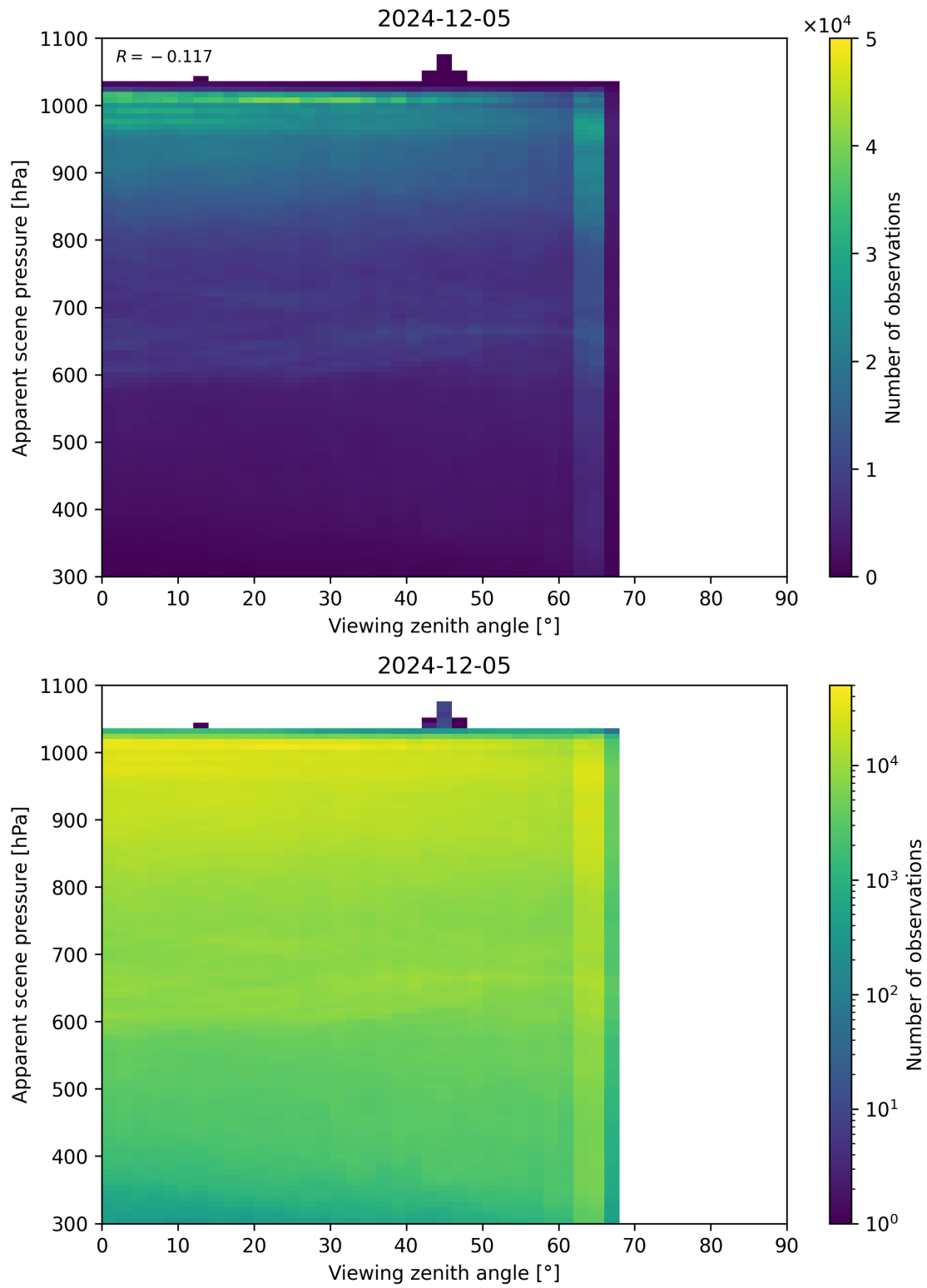
Figure 118: Scatter density plot of “Viewing zenith angle” against “Apparent scene pressure” for 2024-12-04 to 2024-12-06.
