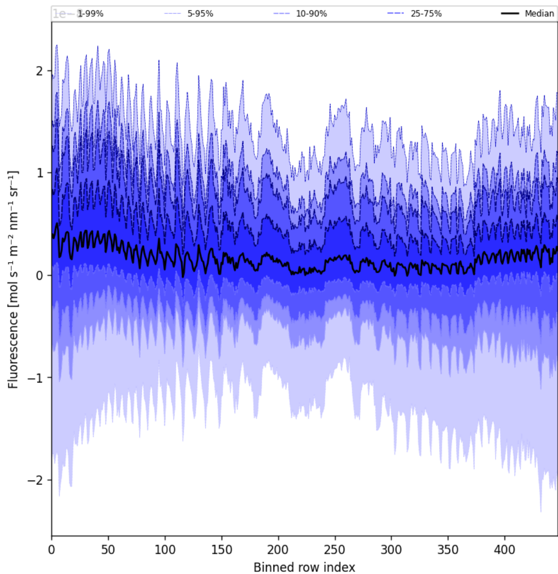
Figure 57: Along track statistics of “Fluorescence” for 2024-12-04 to 2024-12-06
