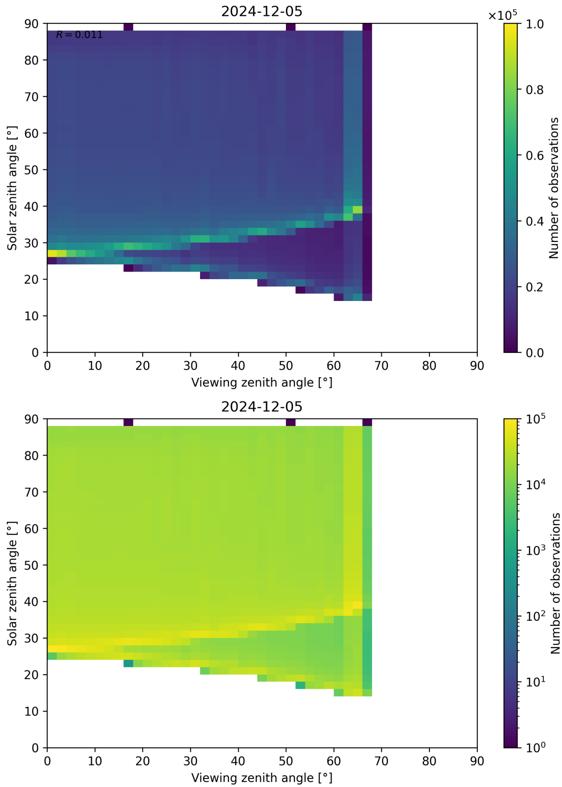
Figure 127: Scatter density plot of “Viewing zenith angle” against “Solar zenith angle” for 2024-12-04 to 2024-12-06.
