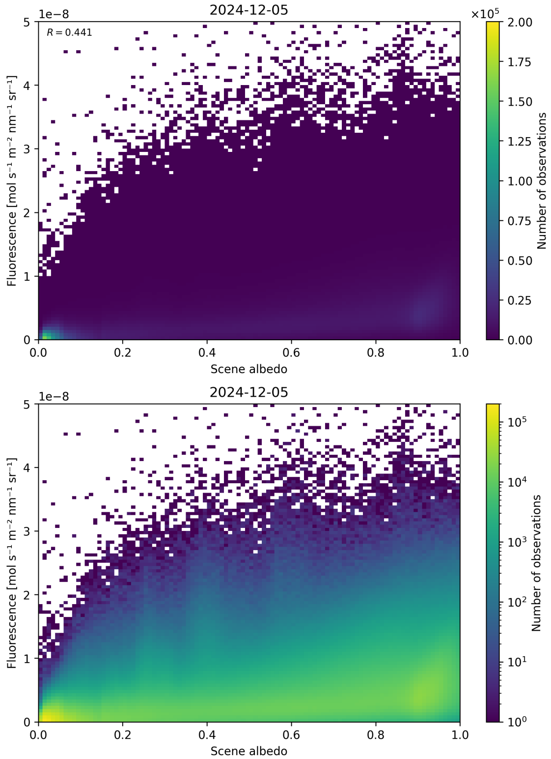
Figure 104: Scatter density plot of “Scene albedo” against “Fluorescence” for 2024-12-04 to 2024-12-06.
