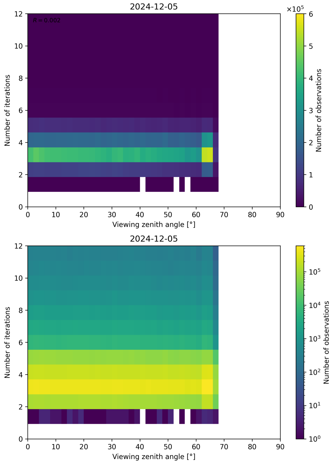
Figure 124: Scatter density plot of “Viewing zenith angle” against “Number of iterations” for 2024-12-04 to 2024-12-06.
