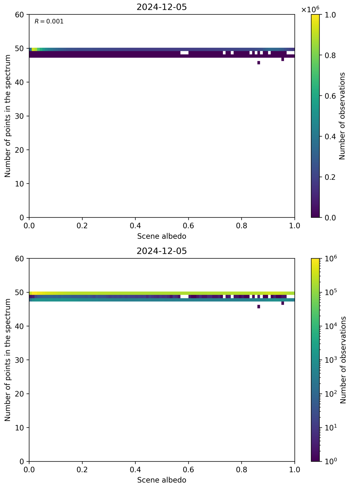
Figure 106: Scatter density plot of “Scene albedo” against “Number of points in the spectrum” for 2024-12-04 to 2024-12-06.
