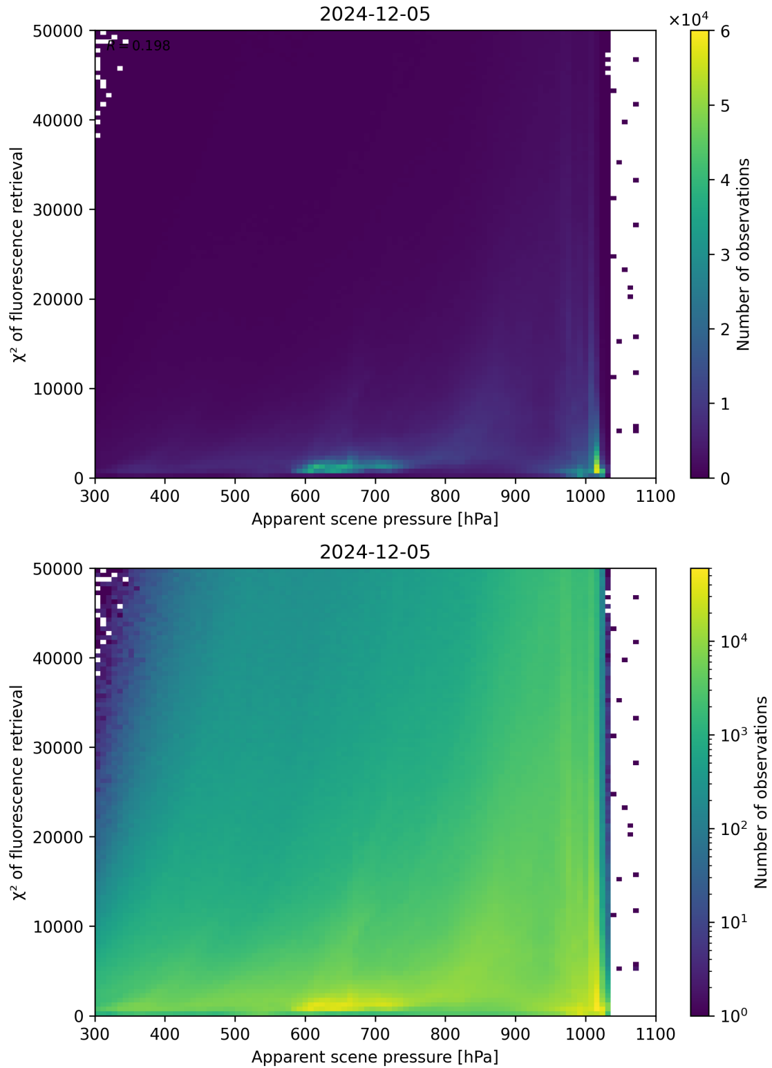
Figure 63: Scatter density plot of “Apparent scene pressure” against “ \chi^2 of fluorescence retrieval” for 2024-12-04 to 2024-12-06.
