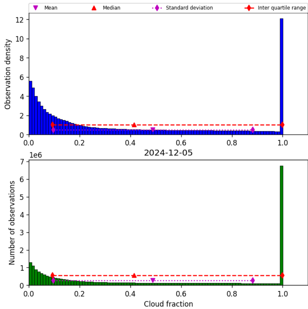
Figure 32: Histogram of “Cloud fraction” for 2024-12-04 to 2024-12-06
