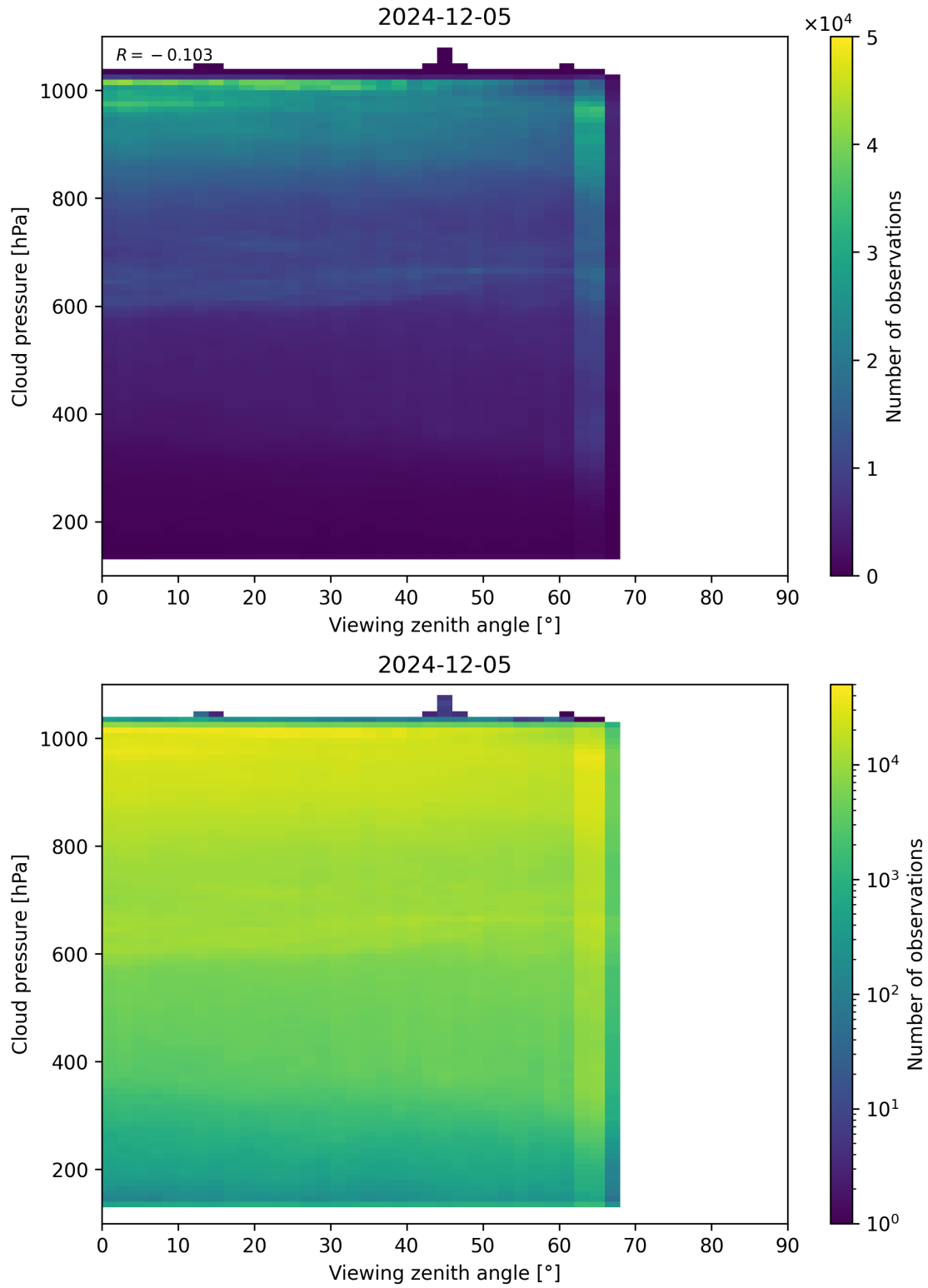
Figure 121: Scatter density plot of “Viewing zenith angle” against “Cloud pressure” for 2024-12-04 to 2024-12-06.
