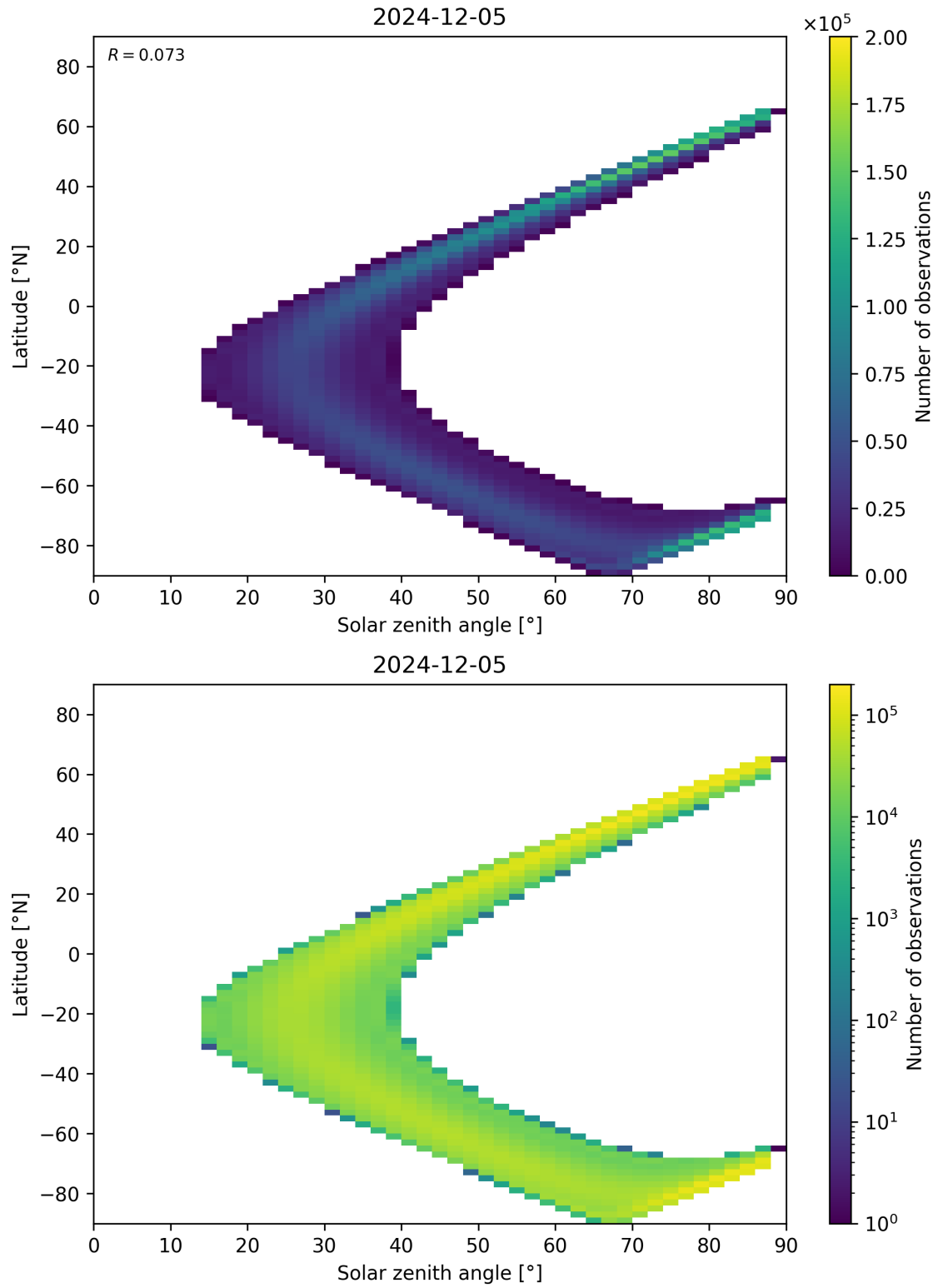
Figure 113: Scatter density plot of “Solar zenith angle” against “Latitude” for 2024-12-04 to 2024-12-06.
