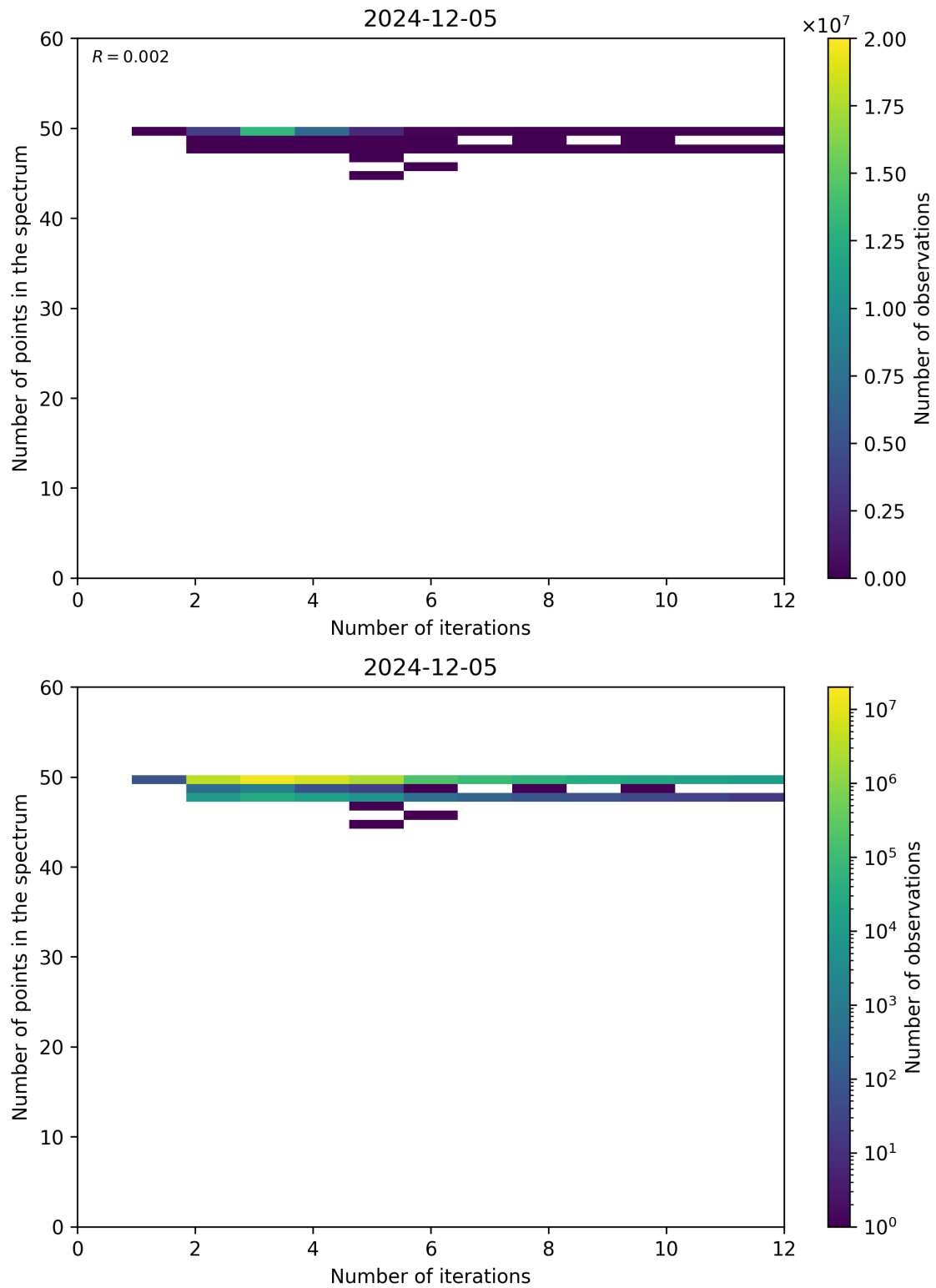
Figure 99: Scatter density plot of “Number of iterations” against “Number of points in the spectrum” for 2024-12-04 to 2024-12-06.
