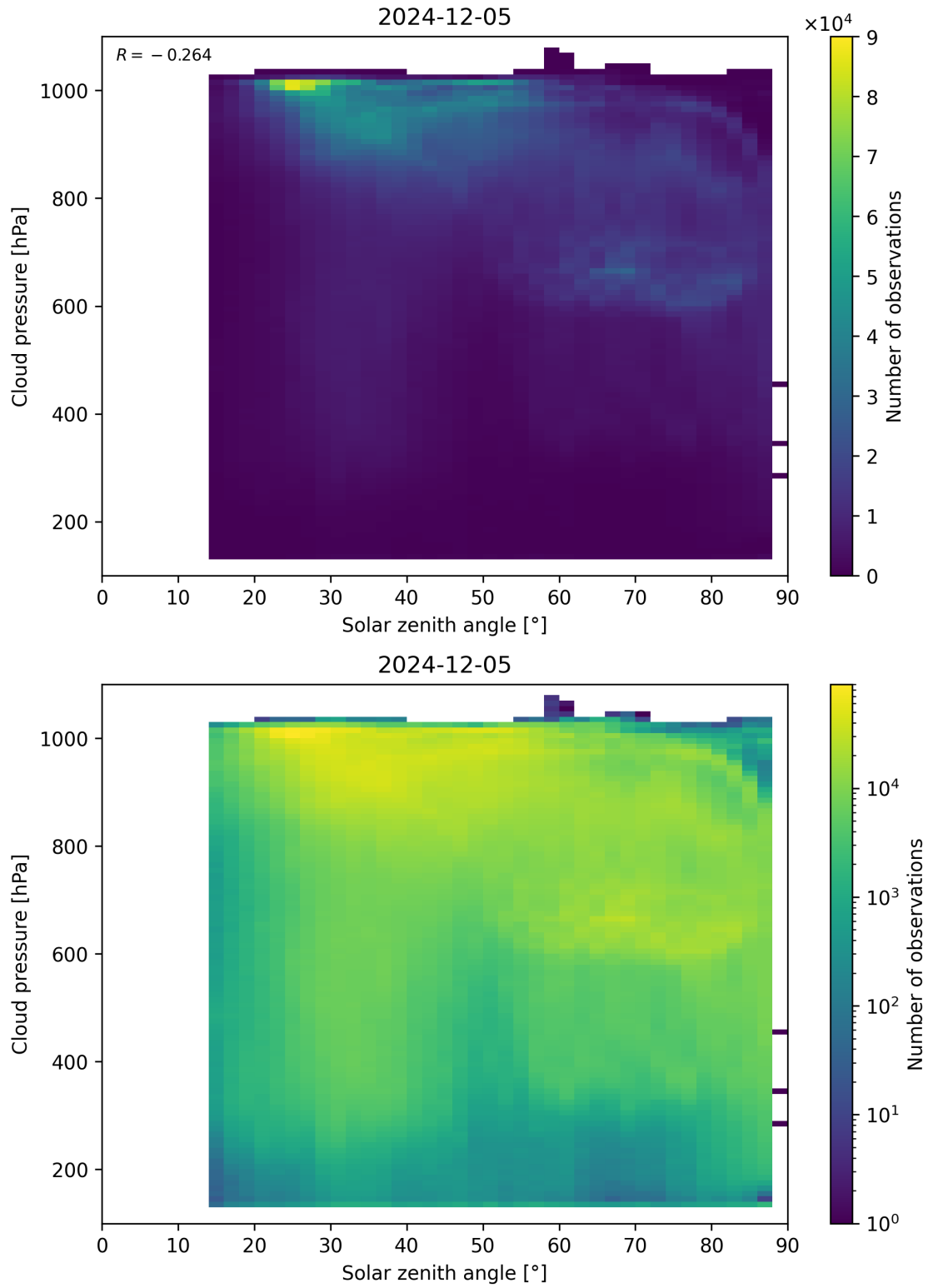
Figure 111: Scatter density plot of “Solar zenith angle” against “Cloud pressure” for 2024-12-04 to 2024-12-06.
