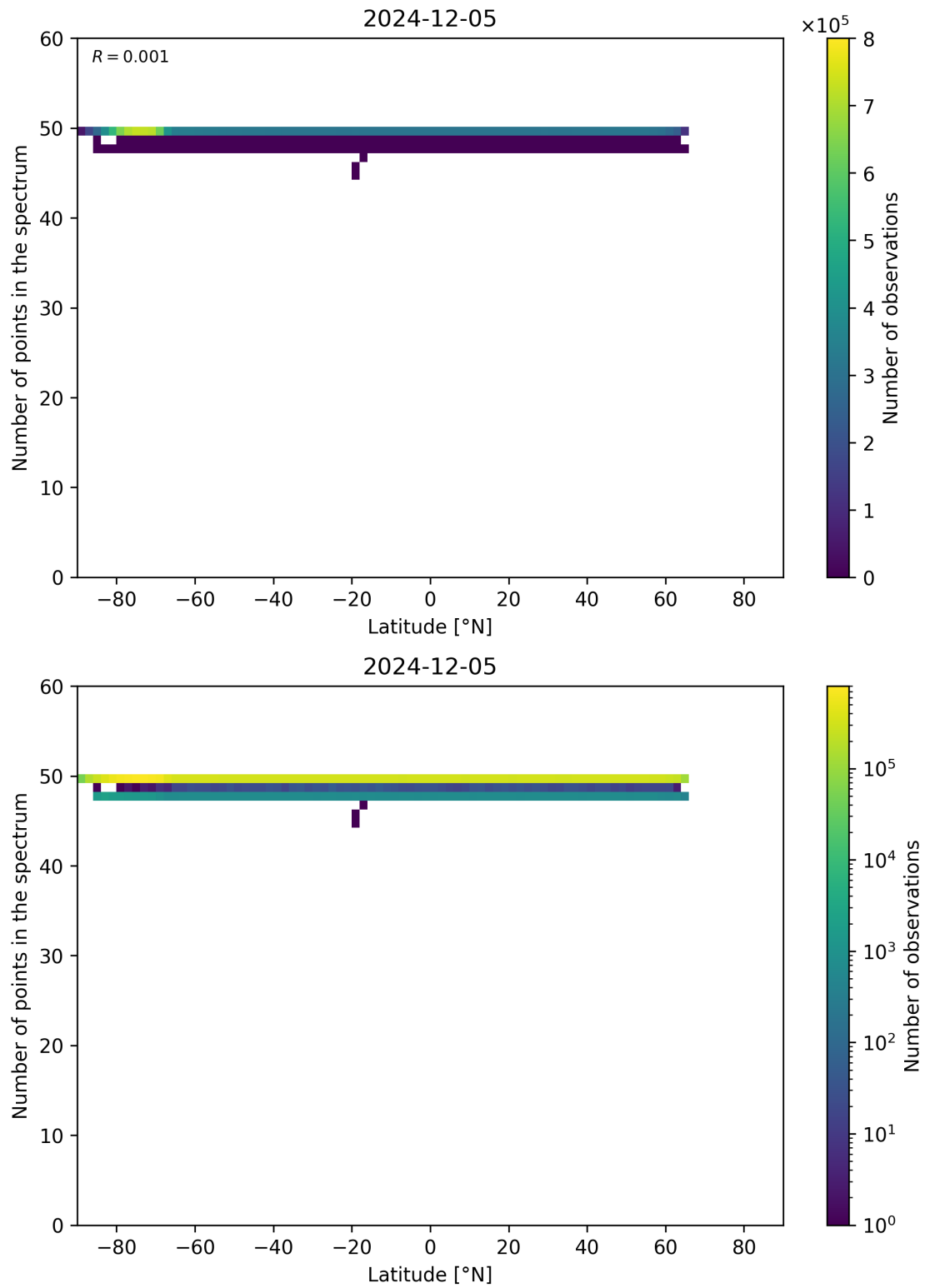
Figure 94: Scatter density plot of “Latitude” against “Number of points in the spectrum” for 2024-12-04 to 2024-12-06.
