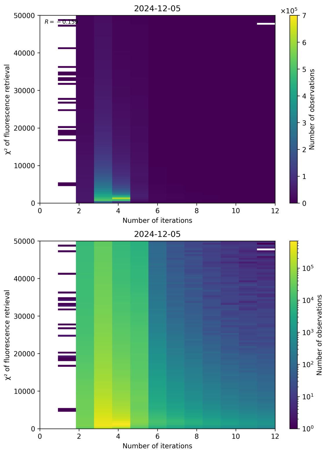
Figure 97: Scatter density plot of “Number of iterations” against “ \chi^2 of fluorescence retrieval” for 2024-12-04 to 2024-12-06.
