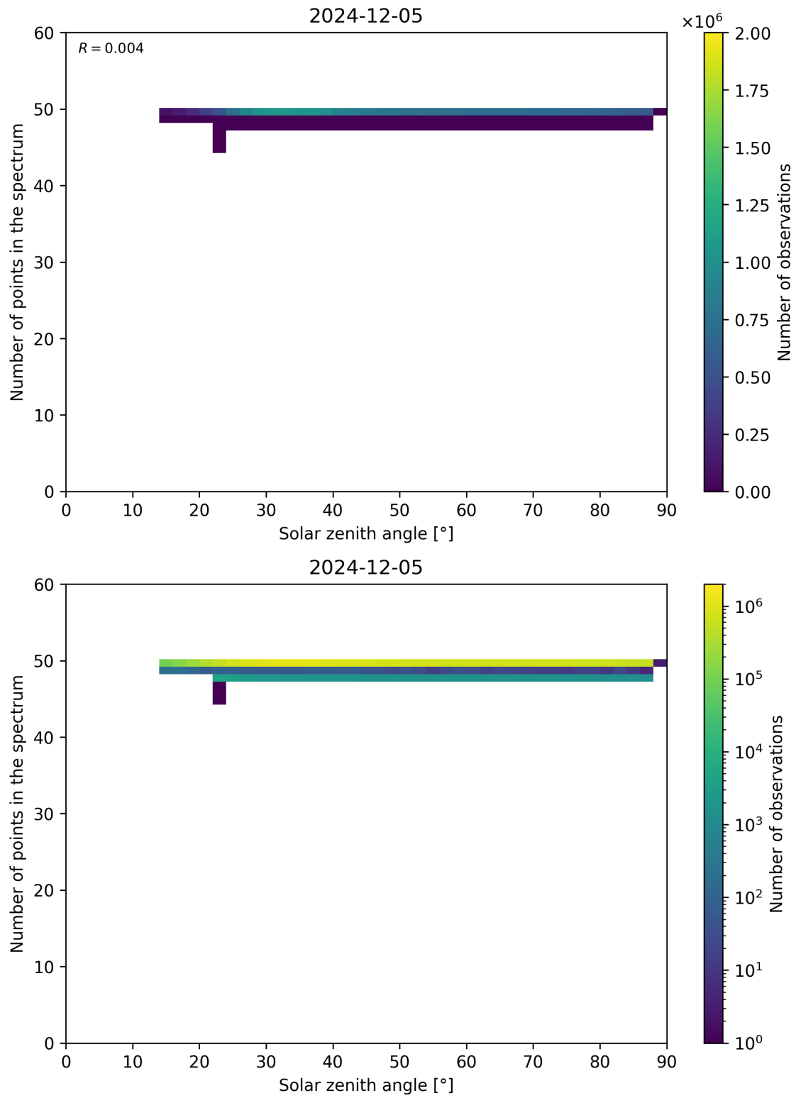
Figure 115: Scatter density plot of “Solar zenith angle” against “Number of points in the spectrum” for 2024-12-04 to 2024-12-06.
