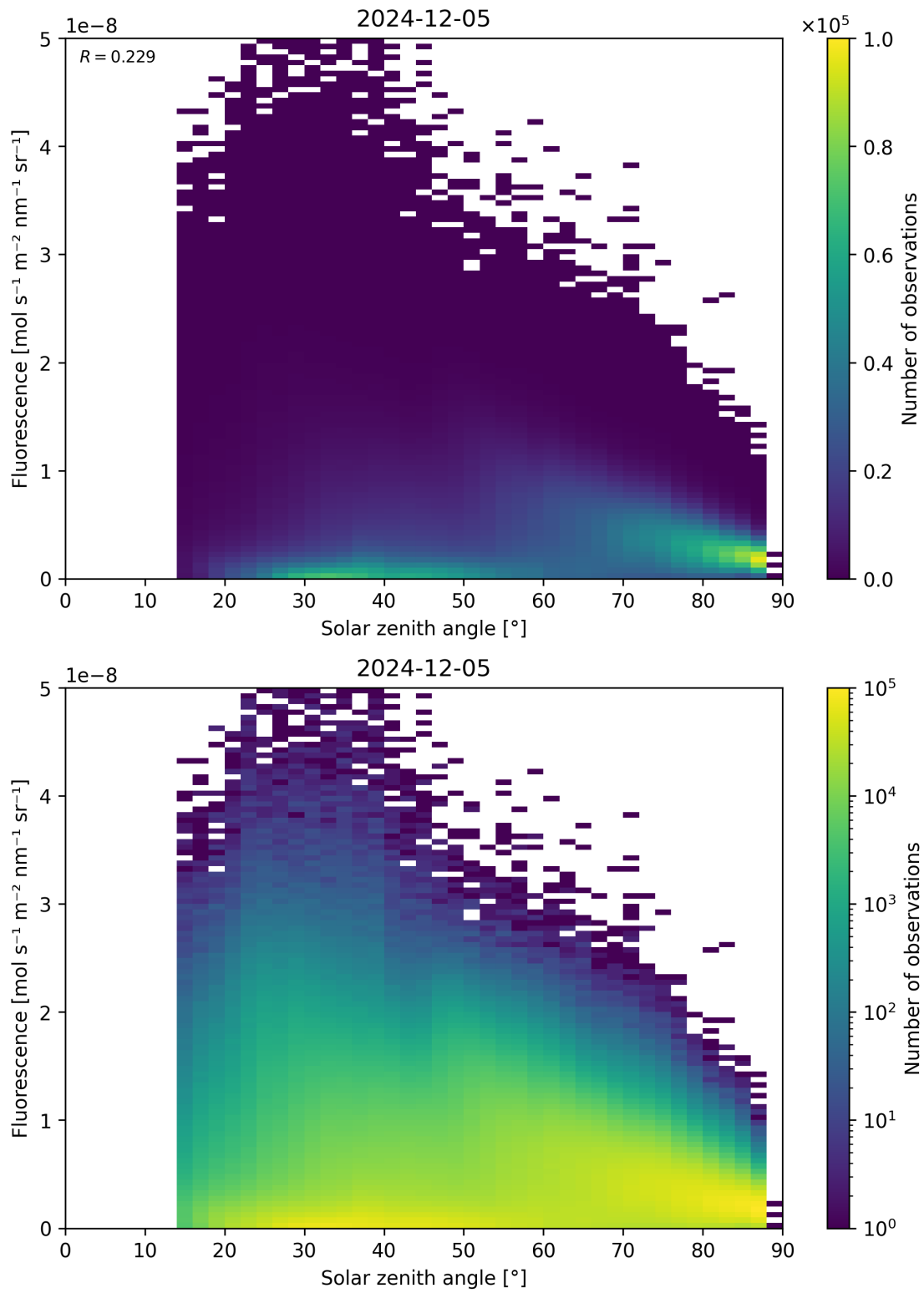
Figure 112: Scatter density plot of “Solar zenith angle” against “Fluorescence” for 2024-12-04 to 2024-12-06.
