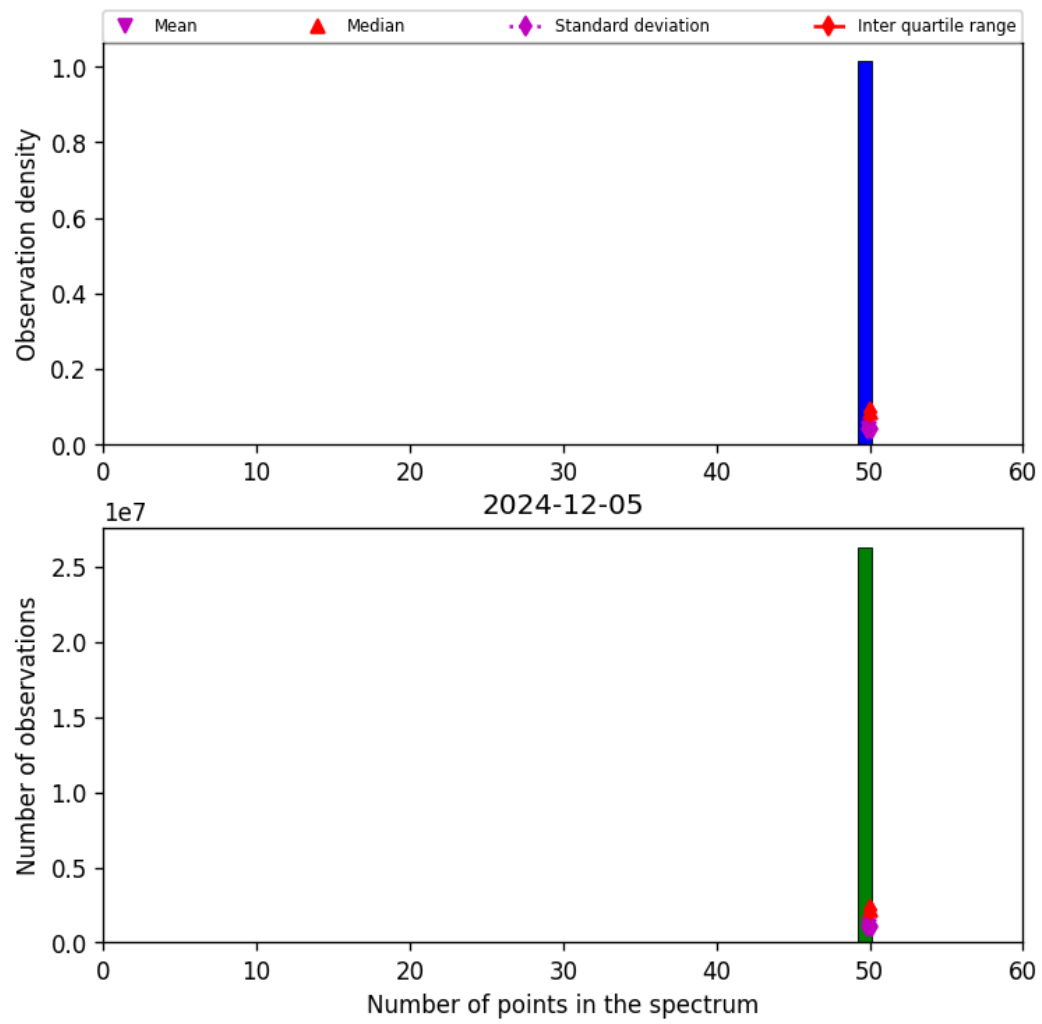
Figure 44: Histogram of “Number of points in the spectrum” for 2024-12-04 to 2024-12-06
