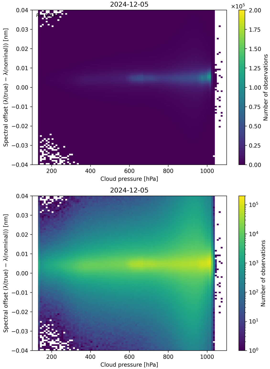
Figure 84: Scatter density plot of “Cloud pressure” against “Spectral offset ( \lambda_{\text{true}} - \lambda_{\text{nominal}} )” for 2024-12-04 to 2024-12-06.
