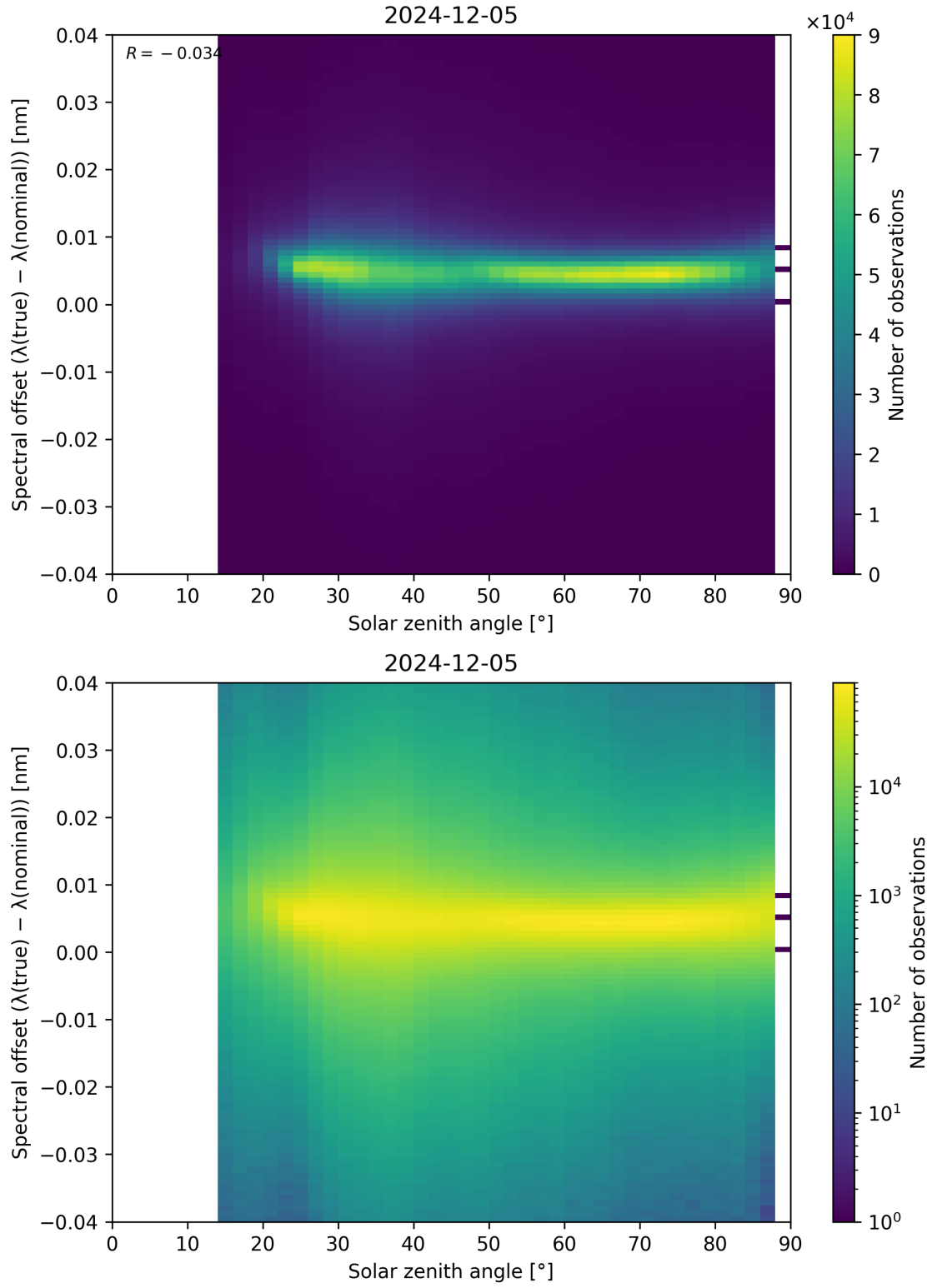
Figure 117: Scatter density plot of “Solar zenith angle” against “Spectral offset ( \lambda_{\text{true}} - \lambda_{\text{nominal}} )” for 2024-12-04 to 2024-12-06.
