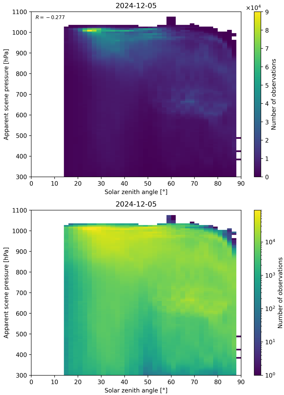
Figure 108: Scatter density plot of “Solar zenith angle” against “Apparent scene pressure” for 2024-12-04 to 2024-12-06.
