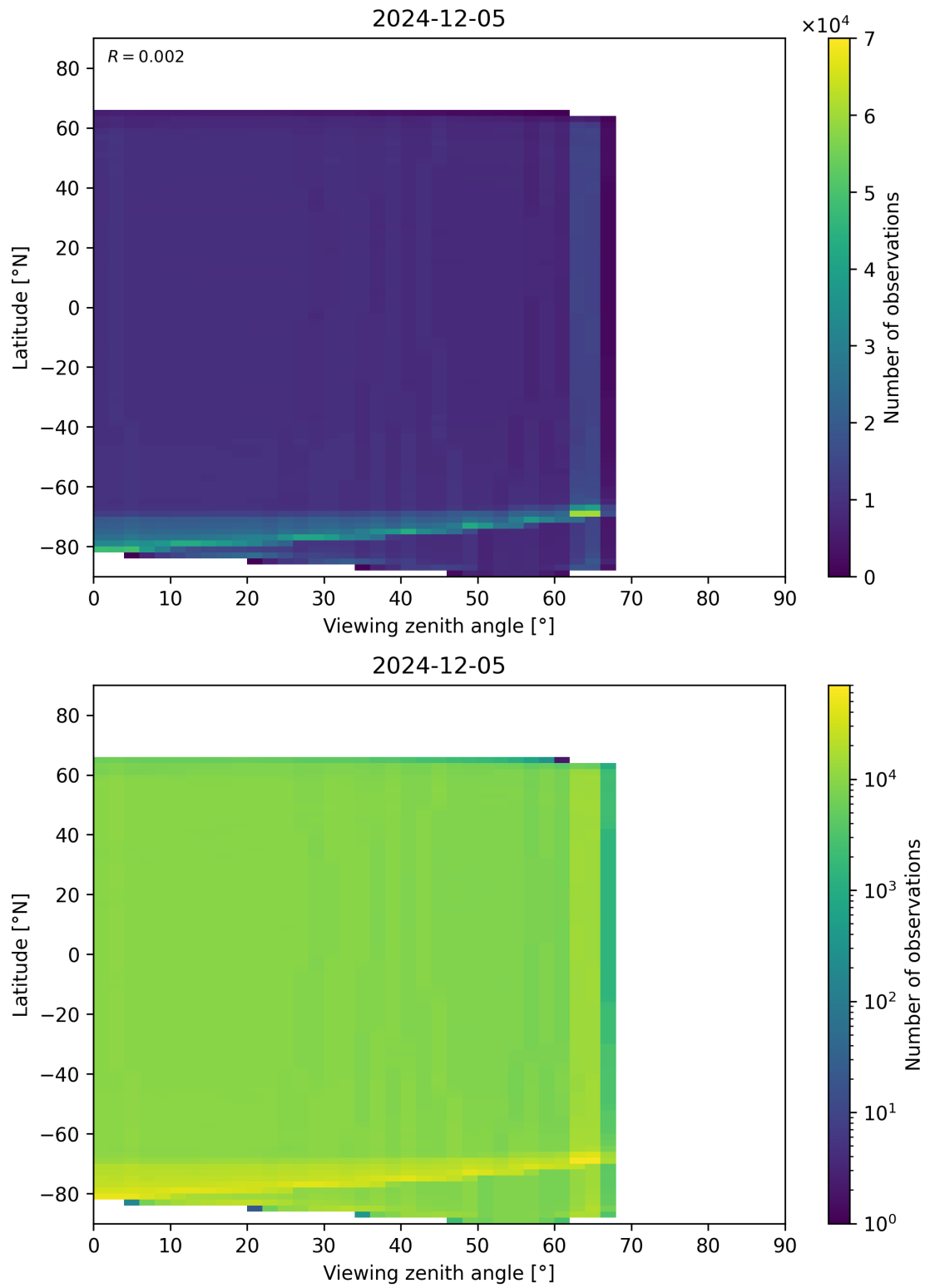
Figure 123: Scatter density plot of “Viewing zenith angle” against “Latitude” for 2024-12-04 to 2024-12-06.
