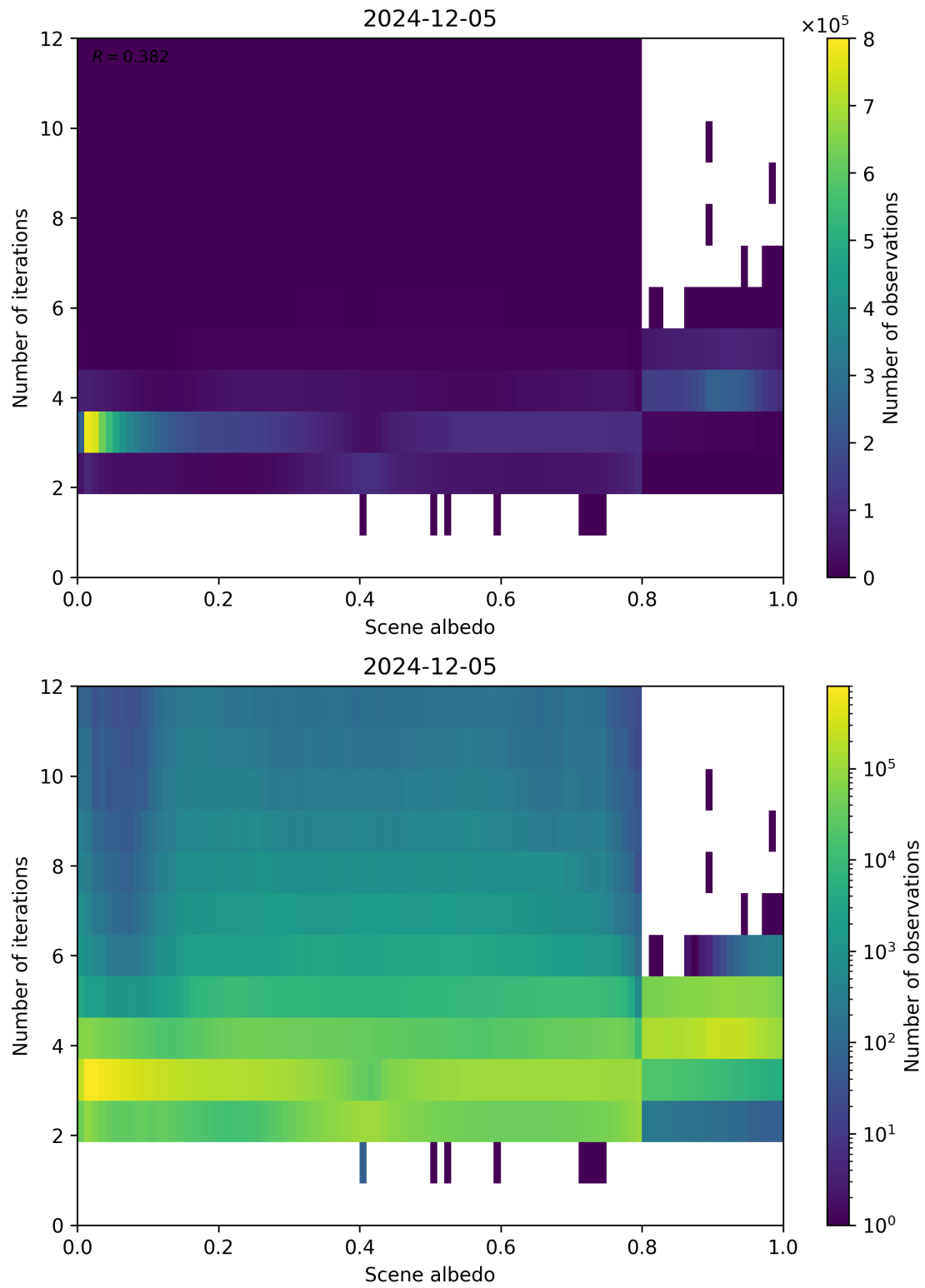
Figure 105: Scatter density plot of “Scene albedo” against “Number of iterations” for 2024-12-04 to 2024-12-06.
