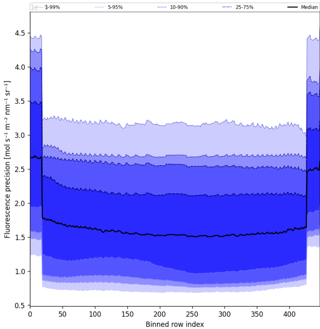
Figure 58: Along track statistics of “Fluorescence precision” for 2024-12-04 to 2024-12-06
