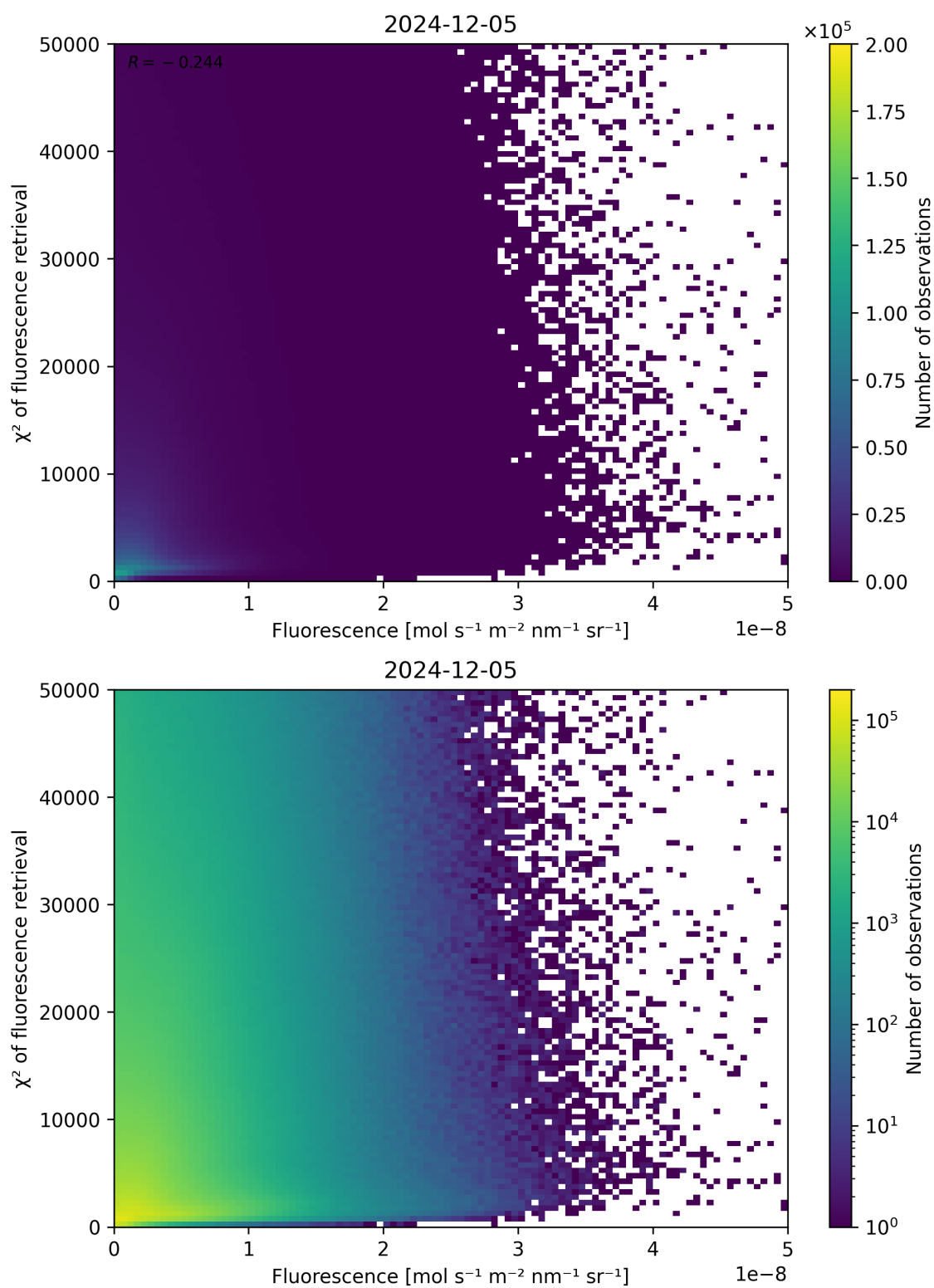
Figure 85: Scatter density plot of “Fluorescence” against “ \chi^2 of fluorescence retrieval” for 2024-12-04 to 2024-12-06.
