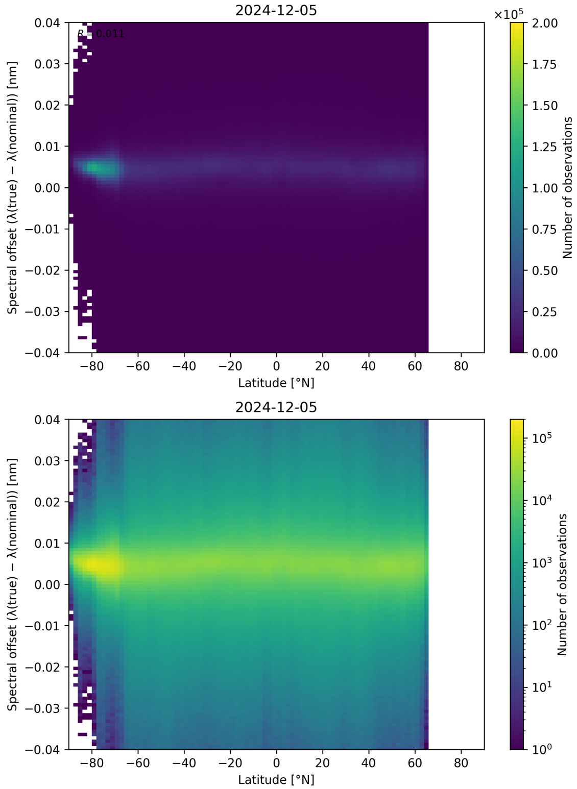
Figure 96: Scatter density plot of “Latitude” against “Spectral offset ( \lambda_{\text{true}} - \lambda_{\text{nominal}} )” for 2024-12-04 to 2024-12-06.
