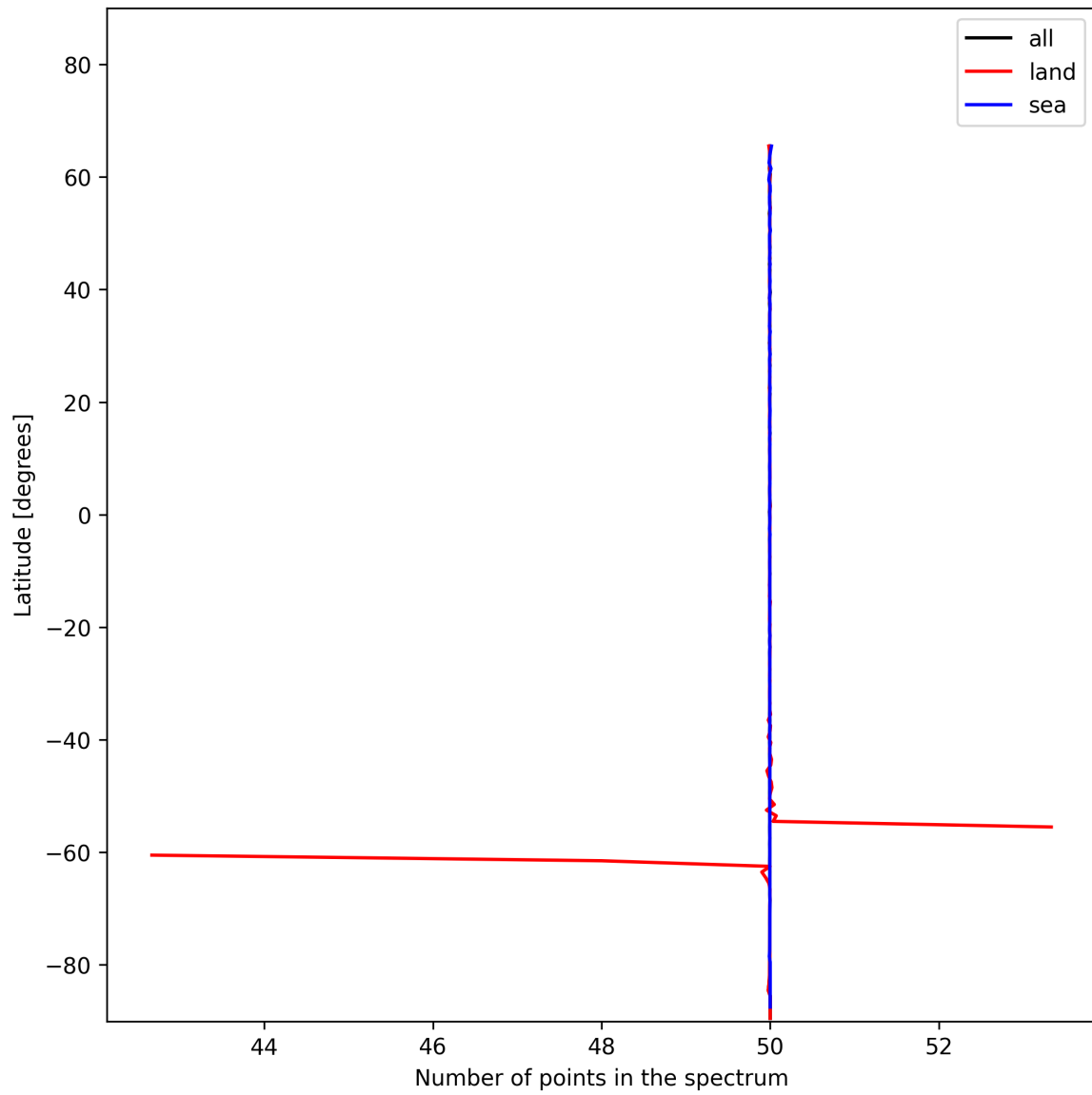
Figure 27: Zonal average of “Number of points in the spectrum” for 2024-12-04 to 2024-12-06.
