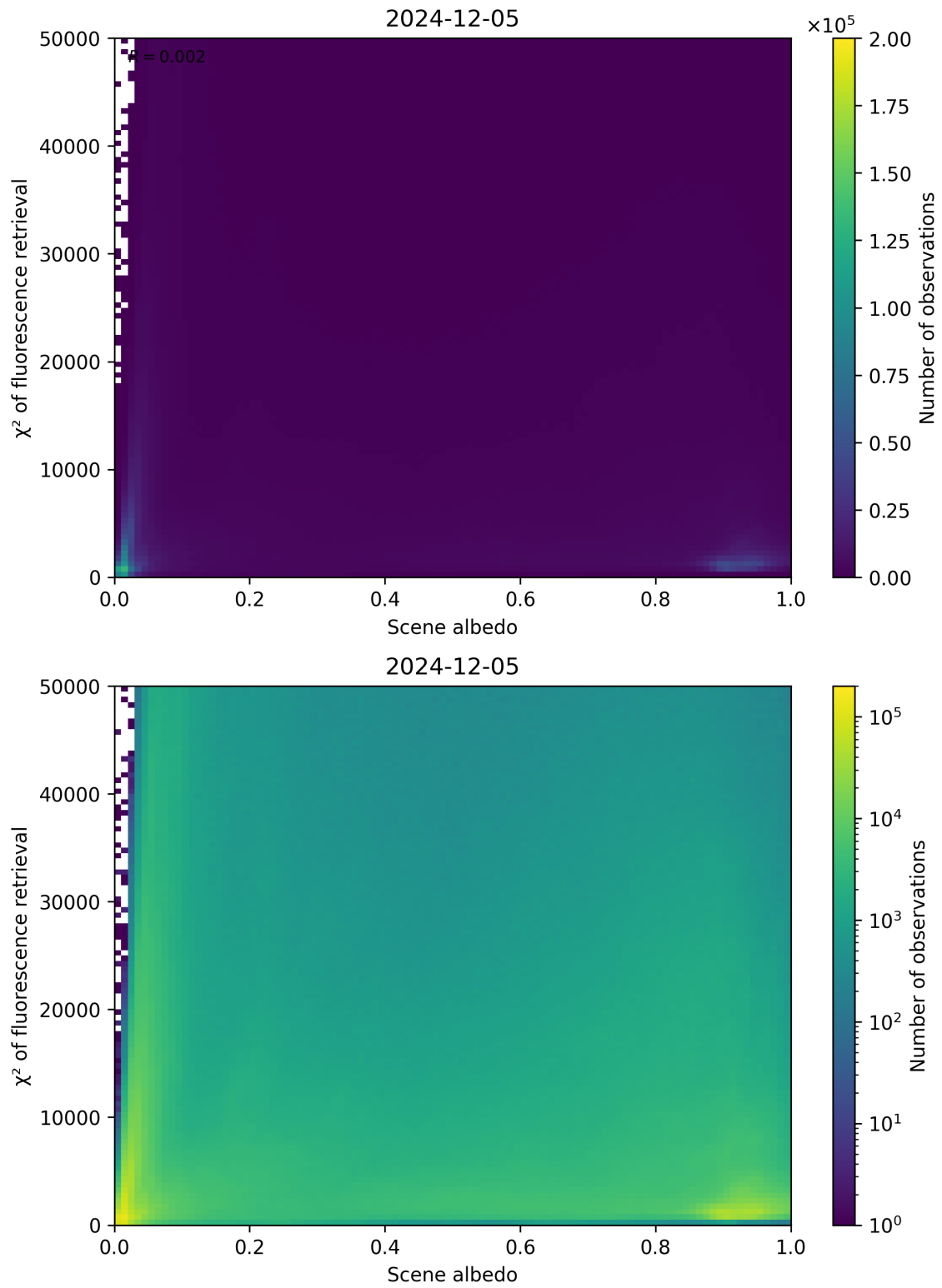
Figure 103: Scatter density plot of “Scene albedo” against “ \chi^2 of fluorescence retrieval” for 2024-12-04 to 2024-12-06.
