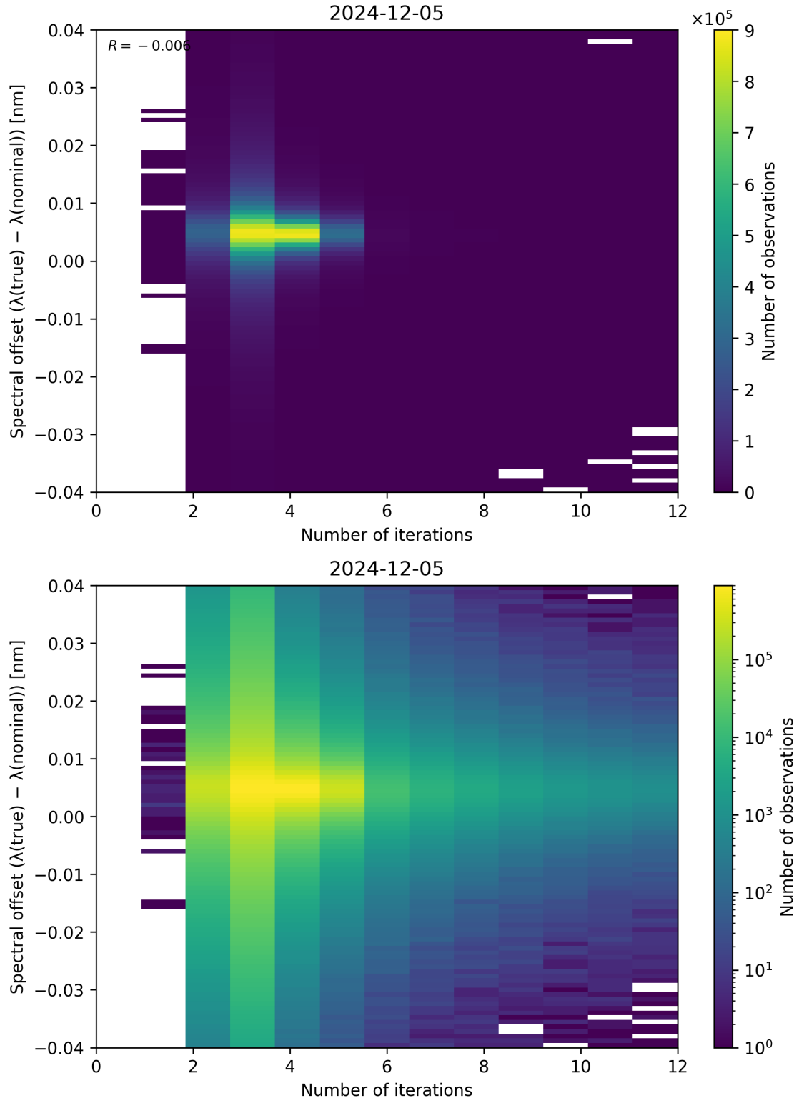
Figure 100: Scatter density plot of “Number of iterations” against “Spectral offset ( \lambda_{\text{true}} - \lambda_{\text{nominal}} )” for 2024-12-04 to 2024-12-06.
