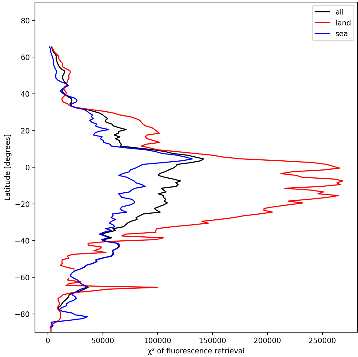
Figure 25: Zonal average of “ \chi^2 of fluorescence retrieval” for 2024-12-04 to 2024-12-06.
