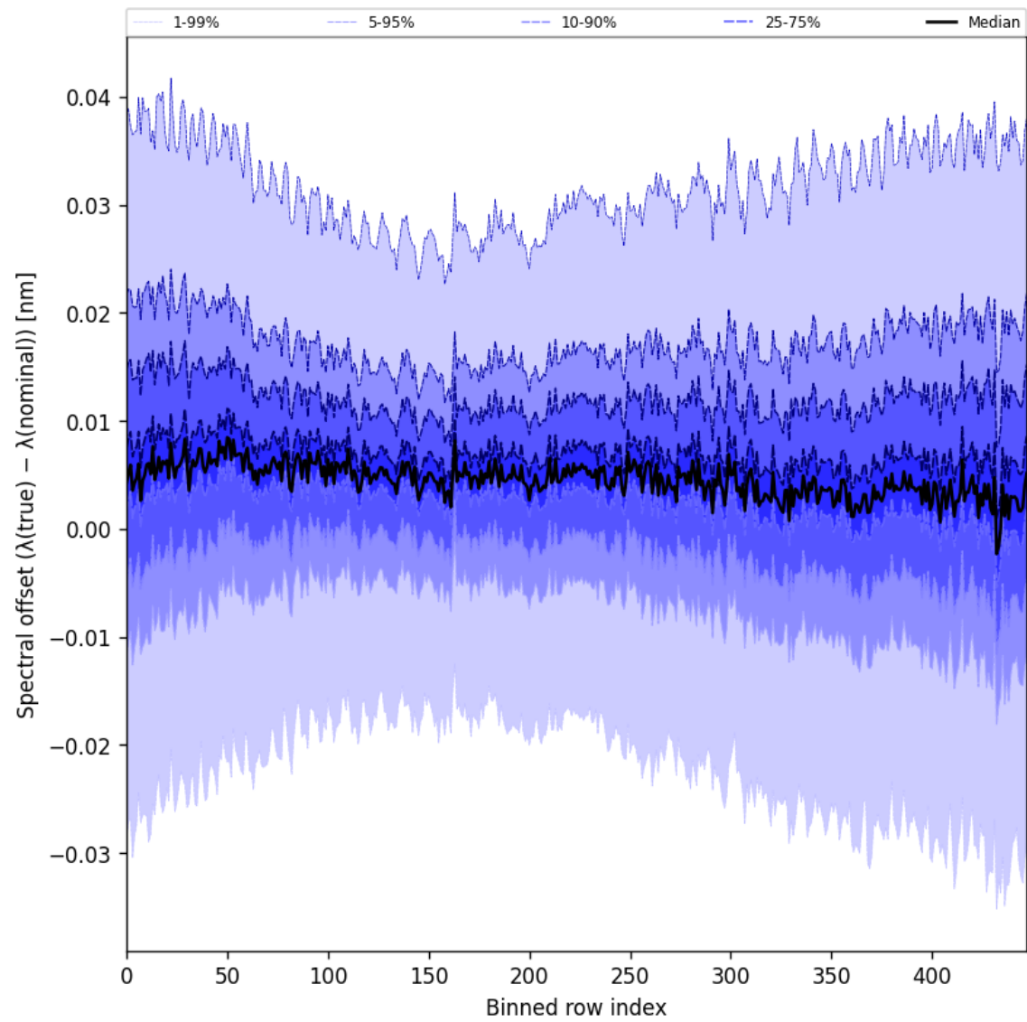
Figure 62: Along track statistics of “Spectral offset ( \lambda_{\text{true}} - \lambda_{\text{nominal}} )” for 2024-12-04 to 2024-12-06
