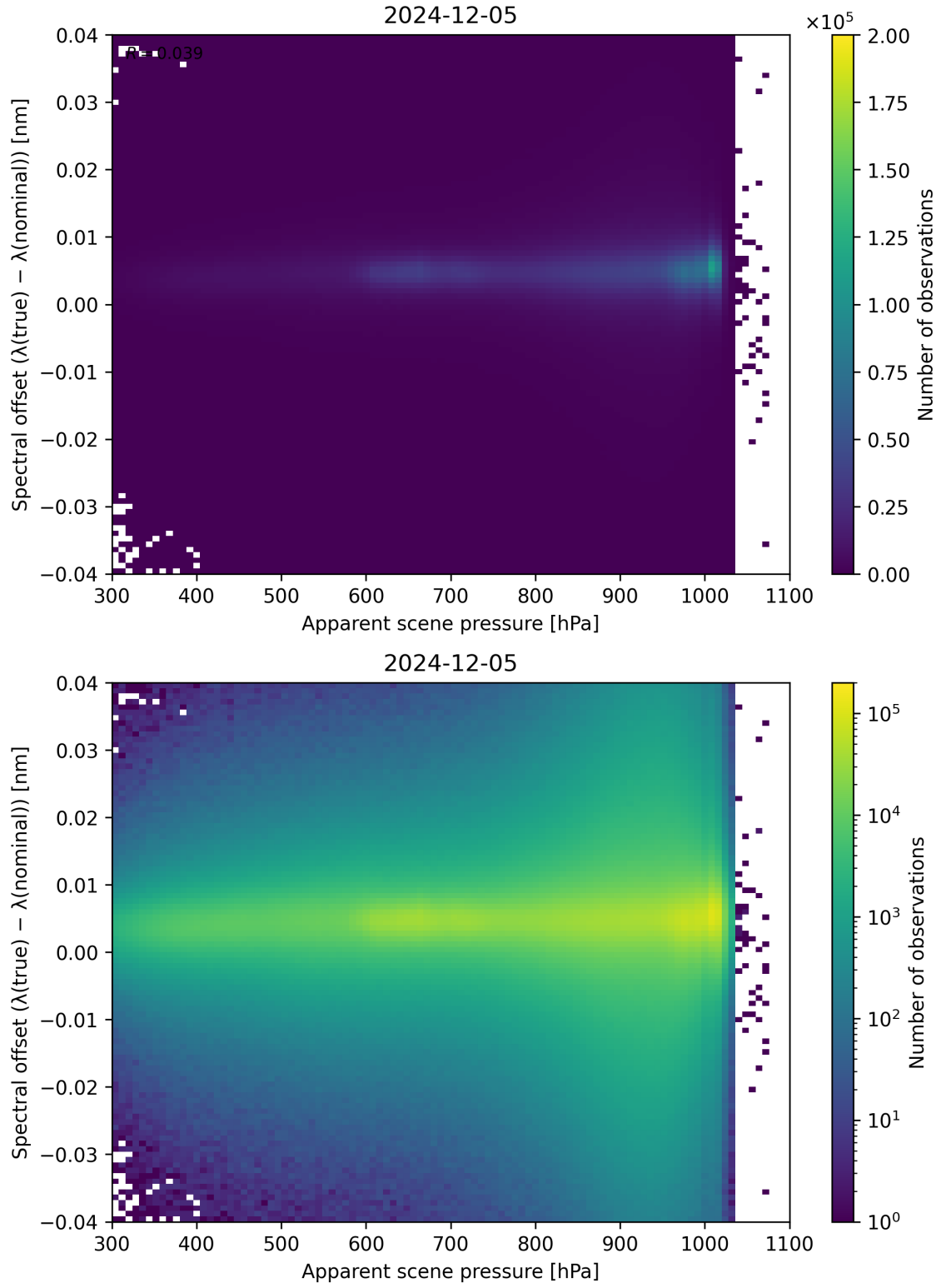
Figure 67: Scatter density plot of “Apparent scene pressure” against “Spectral offset ( \lambda_{\text{true}} - \lambda_{\text{nominal}} )” for 2024-12-04 to 2024-12-06.
