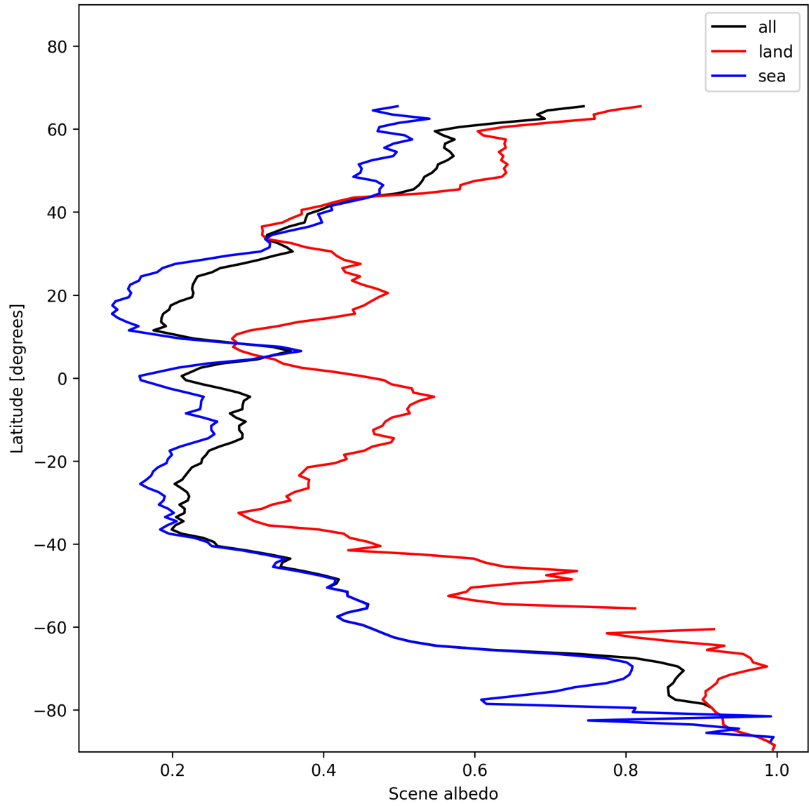
Figure 17: Zonal average of “Scene albedo” for 2024-12-04 to 2024-12-06.
