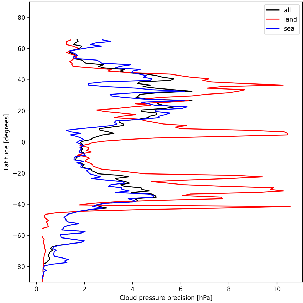
Figure 14: Zonal average of "Cloud pressure precision" for 2024-12-04 to 2024-12-06.
