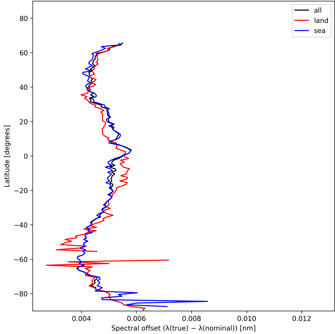
Figure 28: Zonal average of “Spectral offset ( \lambda_{\text{true}} - \lambda_{\text{nominal}} )” for 2024-12-04 to 2024-12-06.
