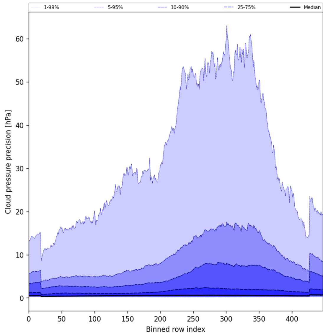
Figure 48: Along track statistics of “Cloud pressure precision” for 2024-12-04 to 2024-12-06
