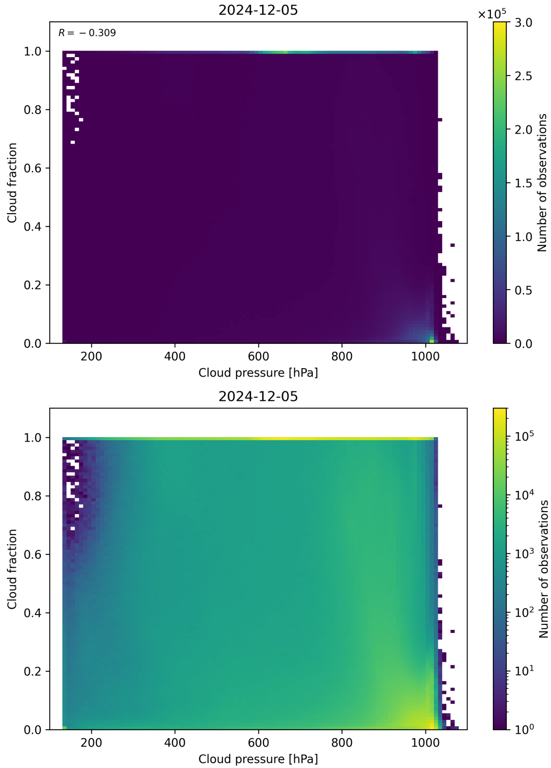
Figure 79: Scatter density plot of “Cloud pressure” against “Cloud fraction” for 2024-12-04 to 2024-12-06.
