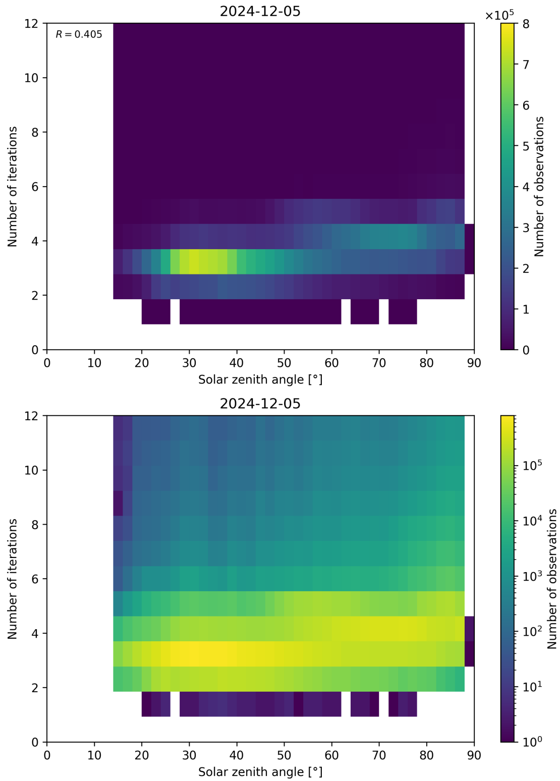
Figure 114: Scatter density plot of “Solar zenith angle” against “Number of iterations” for 2024-12-04 to 2024-12-06.
