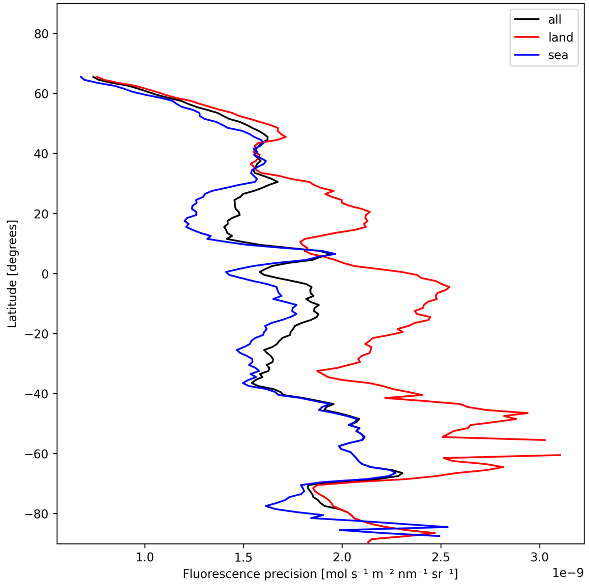
Figure 24: Zonal average of “Fluorescence precision” for 2024-12-04 to 2024-12-06.
