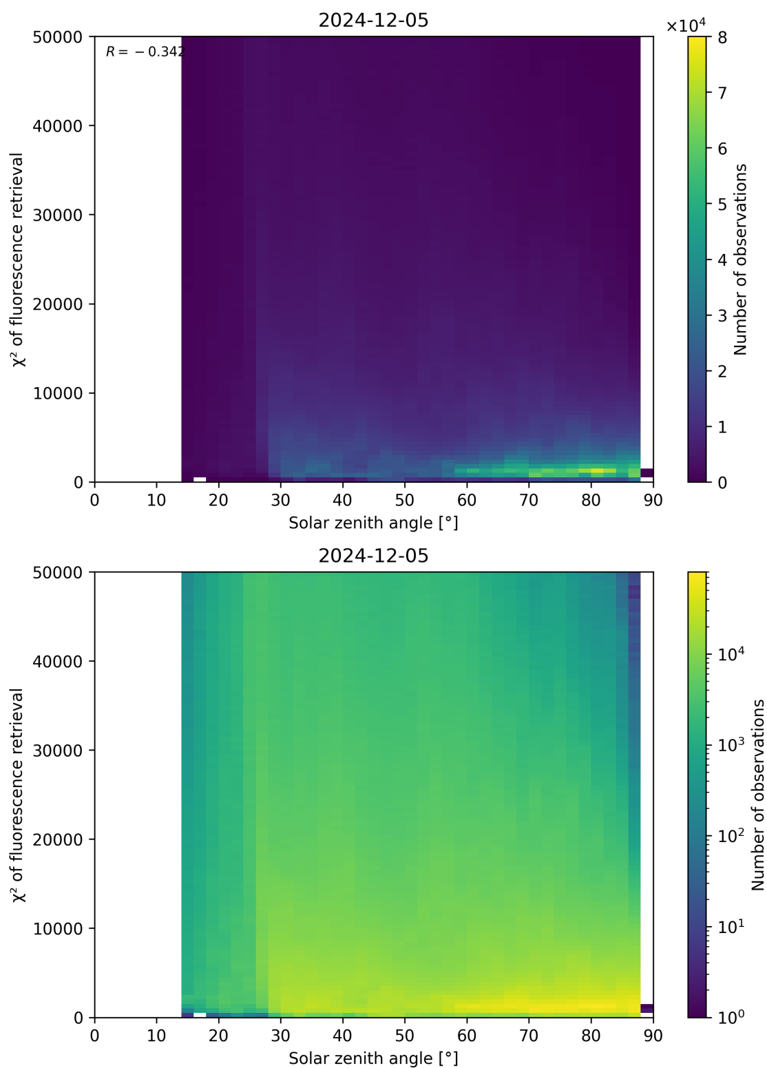
Figure 109: Scatter density plot of “Solar zenith angle” against “ \chi^2 of fluorescence retrieval” for 2024-12-04 to 2024-12-06.
