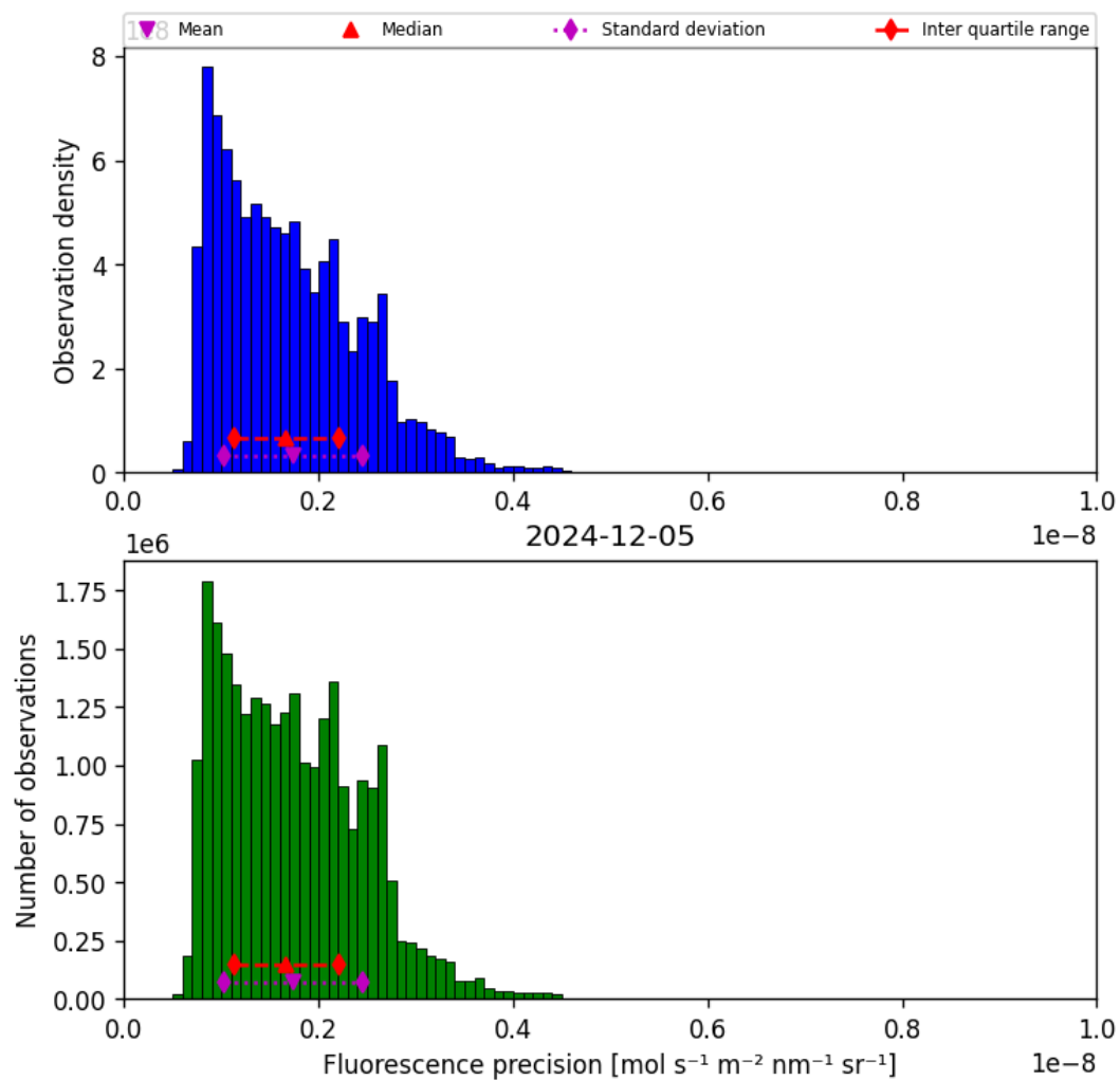
Figure 41: Histogram of “Fluorescence precision” for 2024-12-04 to 2024-12-06
