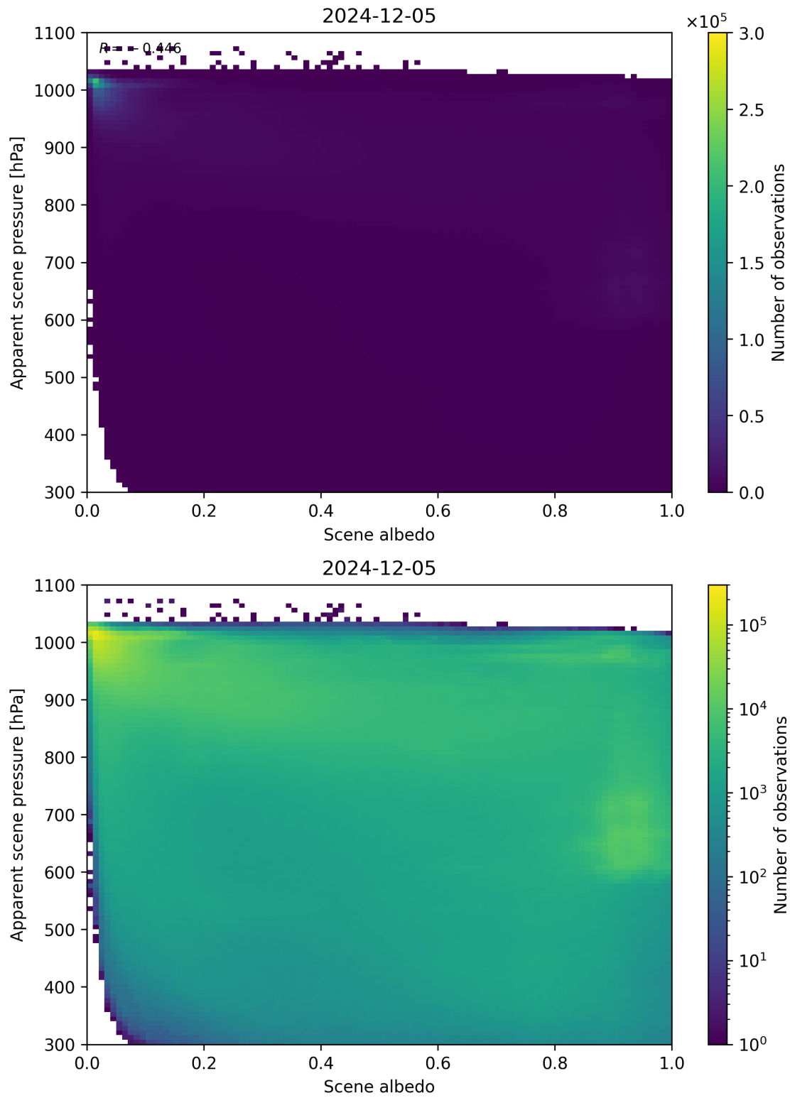
Figure 102: Scatter density plot of “Scene albedo” against “Apparent scene pressure” for 2024-12-04 to 2024-12-06.
