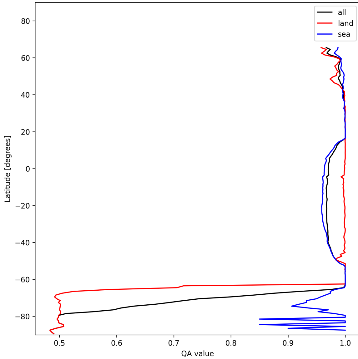
Figure 12: Zonal average of “QA value” for 2024-12-04 to 2024-12-06.
