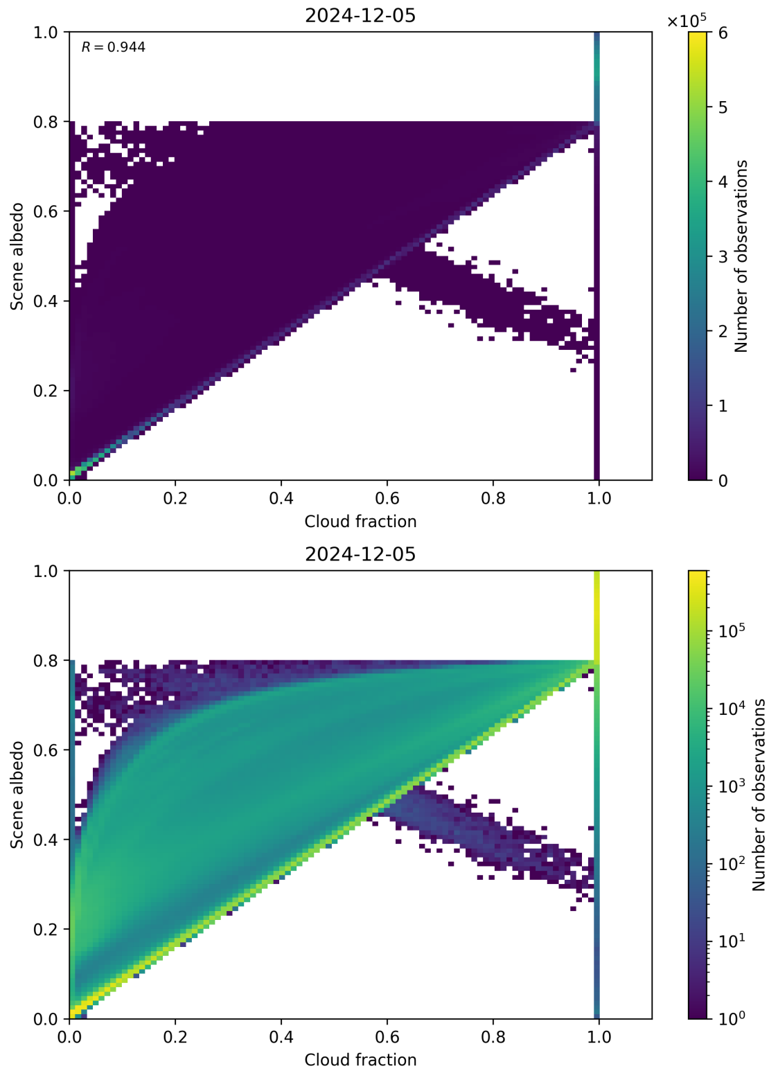
Figure 75: Scatter density plot of “Cloud fraction” against “Scene albedo” for 2024-12-04 to 2024-12-06.
