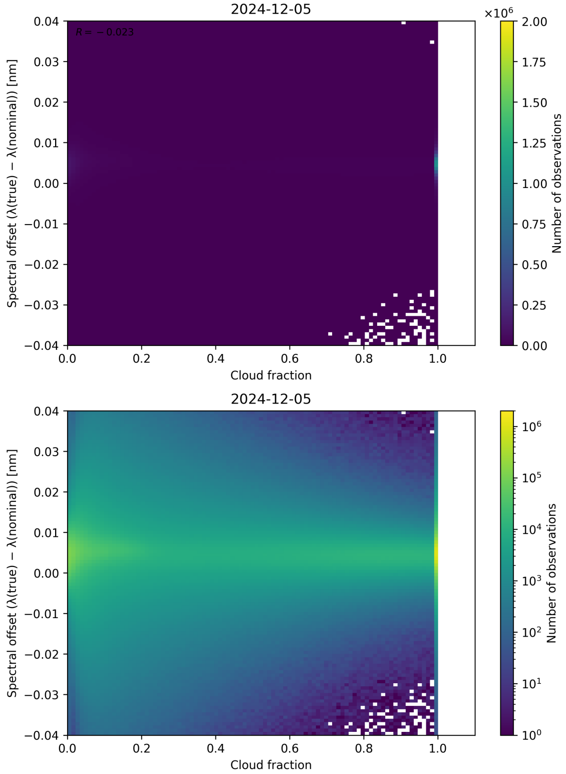
Figure 76: Scatter density plot of “Cloud fraction” against “Spectral offset ( \lambda_{\text{true}} - \lambda_{\text{nominal}} )” for 2024-12-04 to 2024-12-06.
