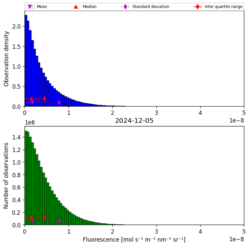
Figure 40: Histogram of “Fluorescence” for 2024-12-04 to 2024-12-06
