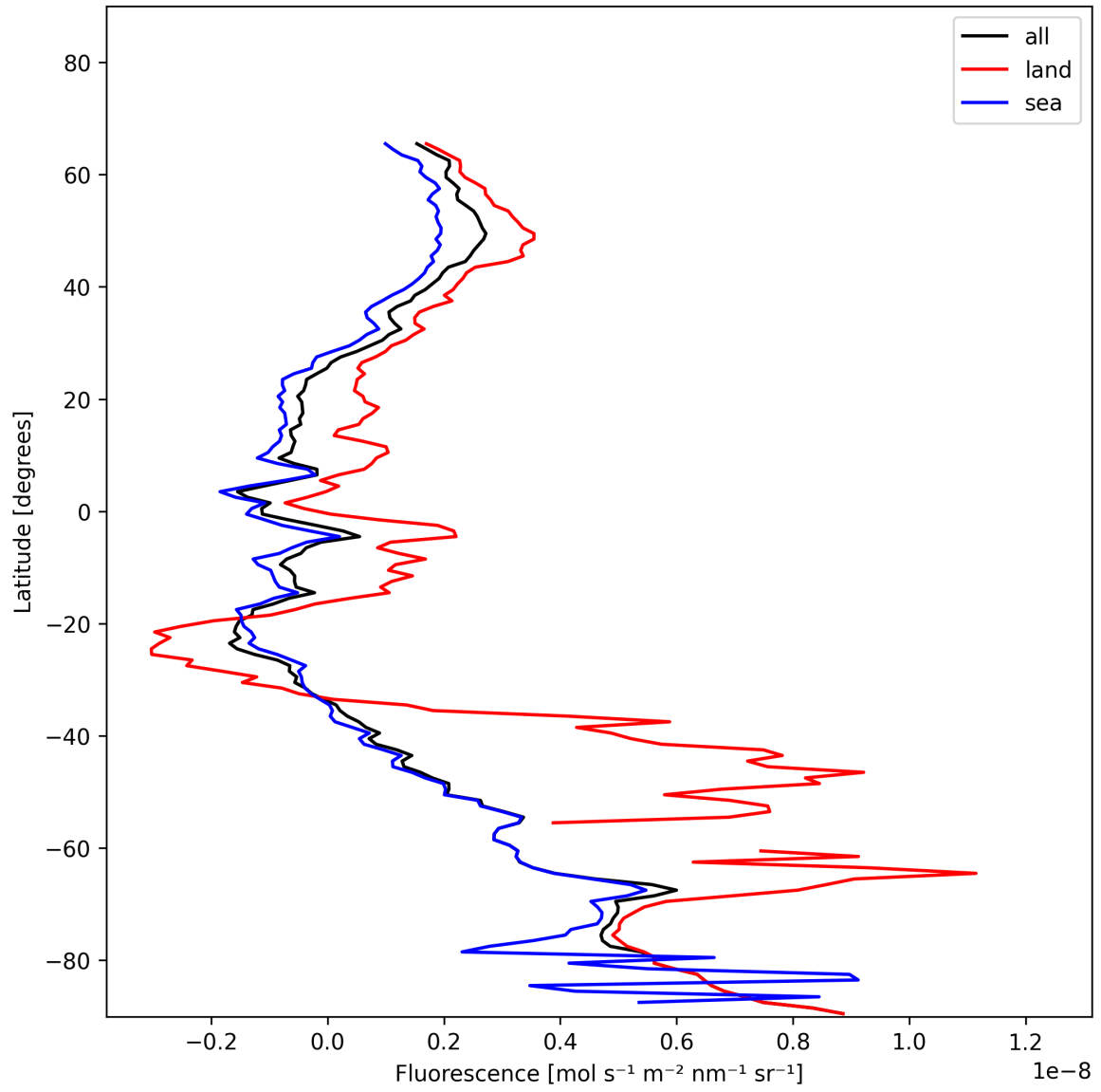
Figure 23: Zonal average of “Fluorescence” for 2024-12-04 to 2024-12-06.
