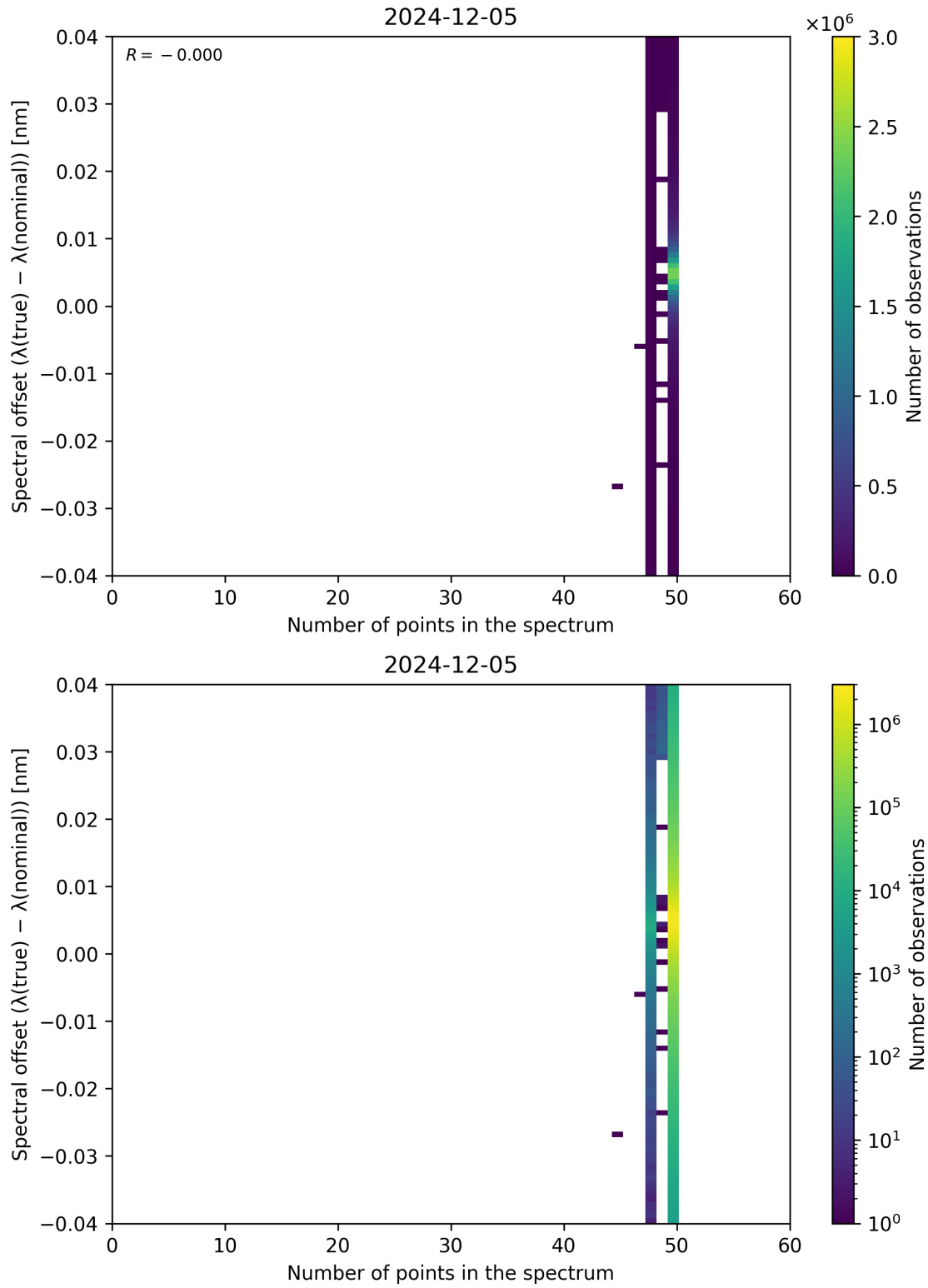
Figure 101: Scatter density plot of “Number of points in the spectrum” against “Spectral offset ( \lambda_{\text{true}} - \lambda_{\text{nominal}} )” for 2024-12-04 to 2024-12-06.
