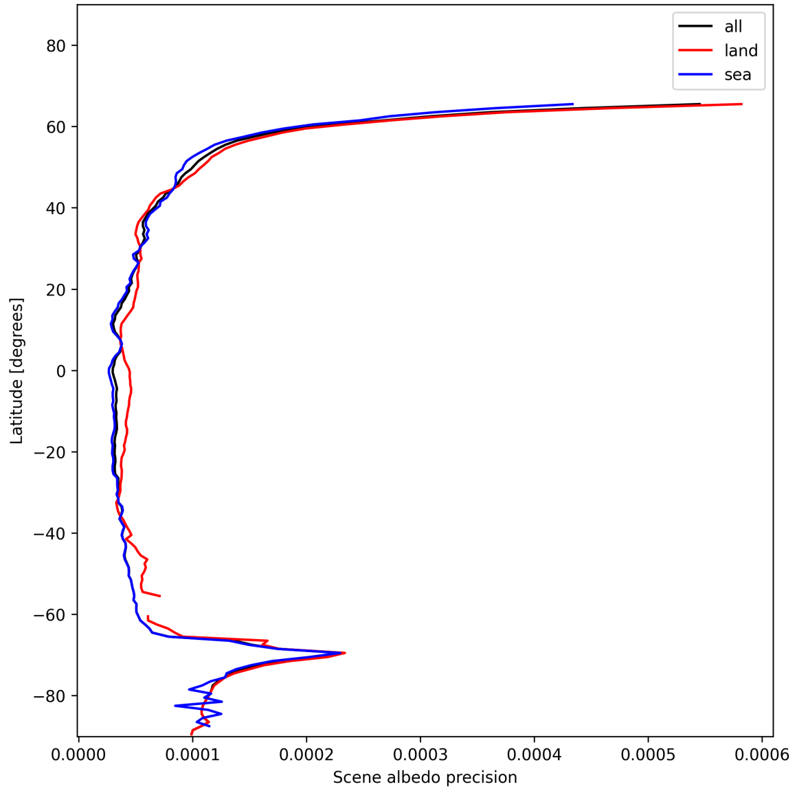
Figure 18: Zonal average of “Scene albedo precision” for 2024-12-04 to 2024-12-06.
