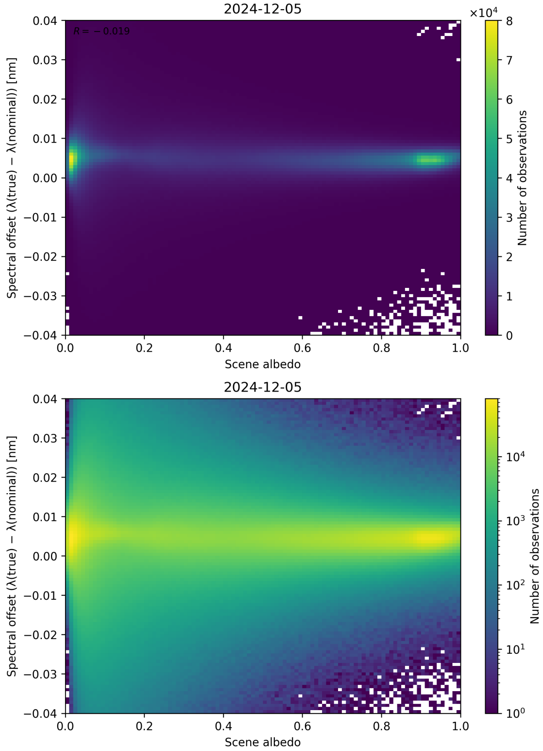
Figure 107: Scatter density plot of “Scene albedo” against “Spectral offset ( \lambda_{\text{true}} - \lambda_{\text{nominal}} )” for 2024-12-04 to 2024-12-06.
