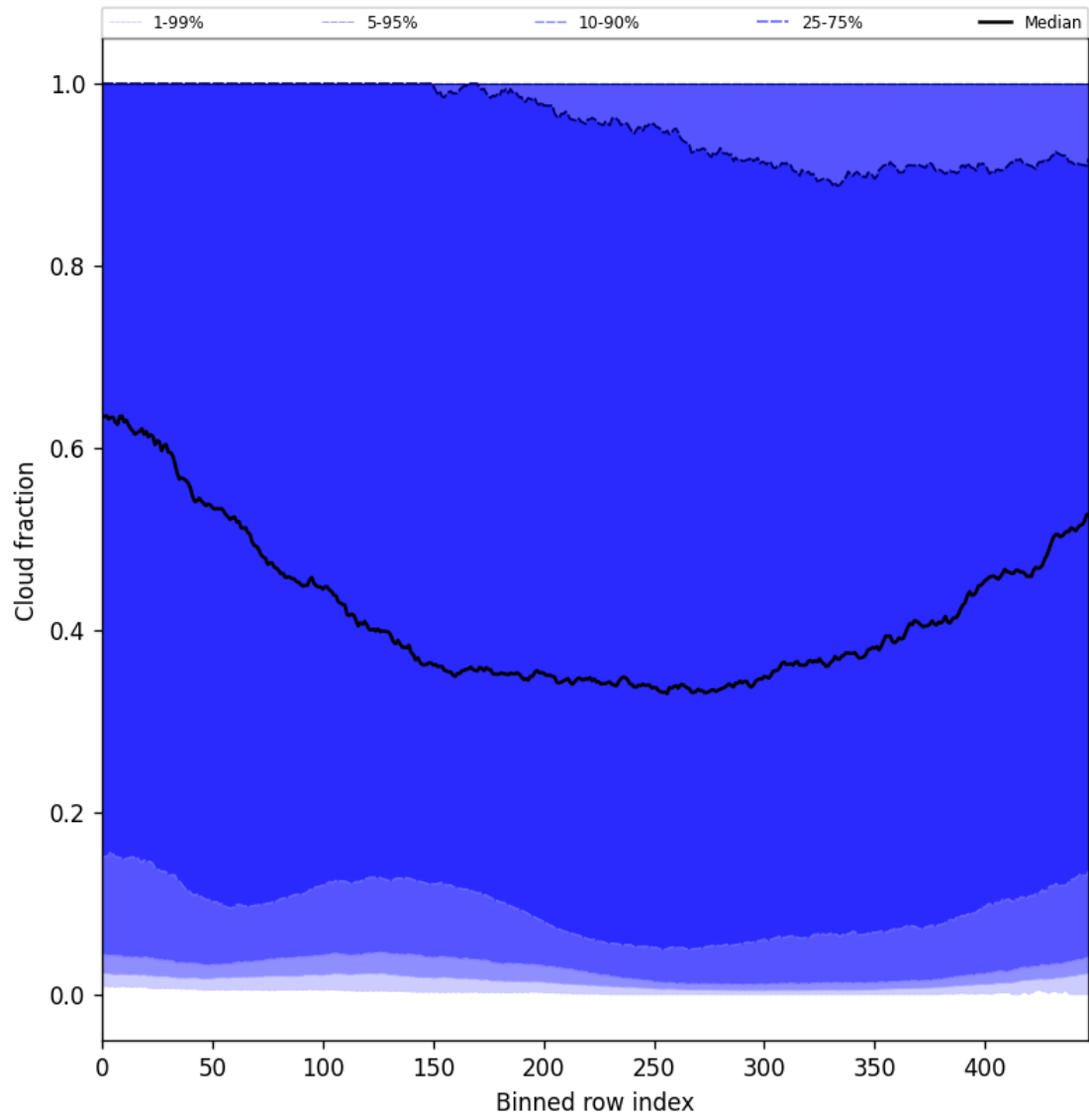
Figure 49: Along track statistics of “Cloud fraction” for 2024-12-04 to 2024-12-06
