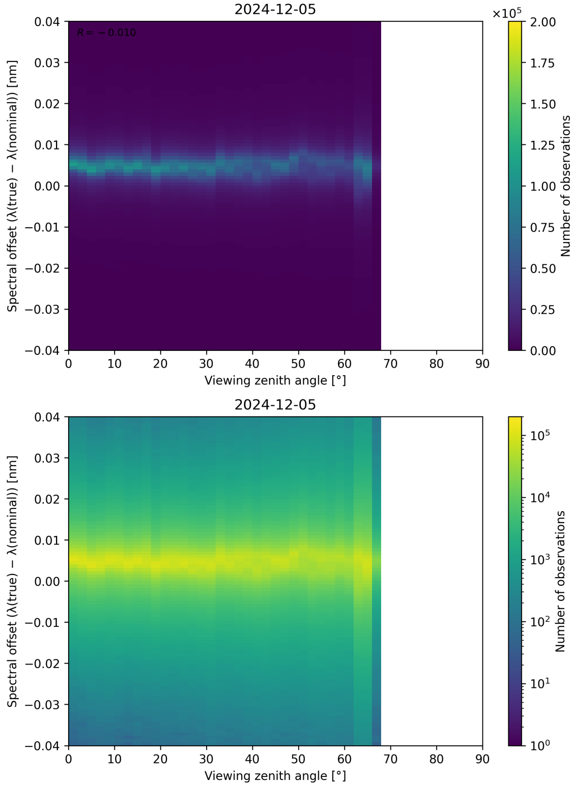
Figure 128: Scatter density plot of “Viewing zenith angle” against “Spectral offset ( \lambda_{\text{true}} - \lambda_{\text{nominal}} )” for 2024-12-04 to 2024-12-06.
