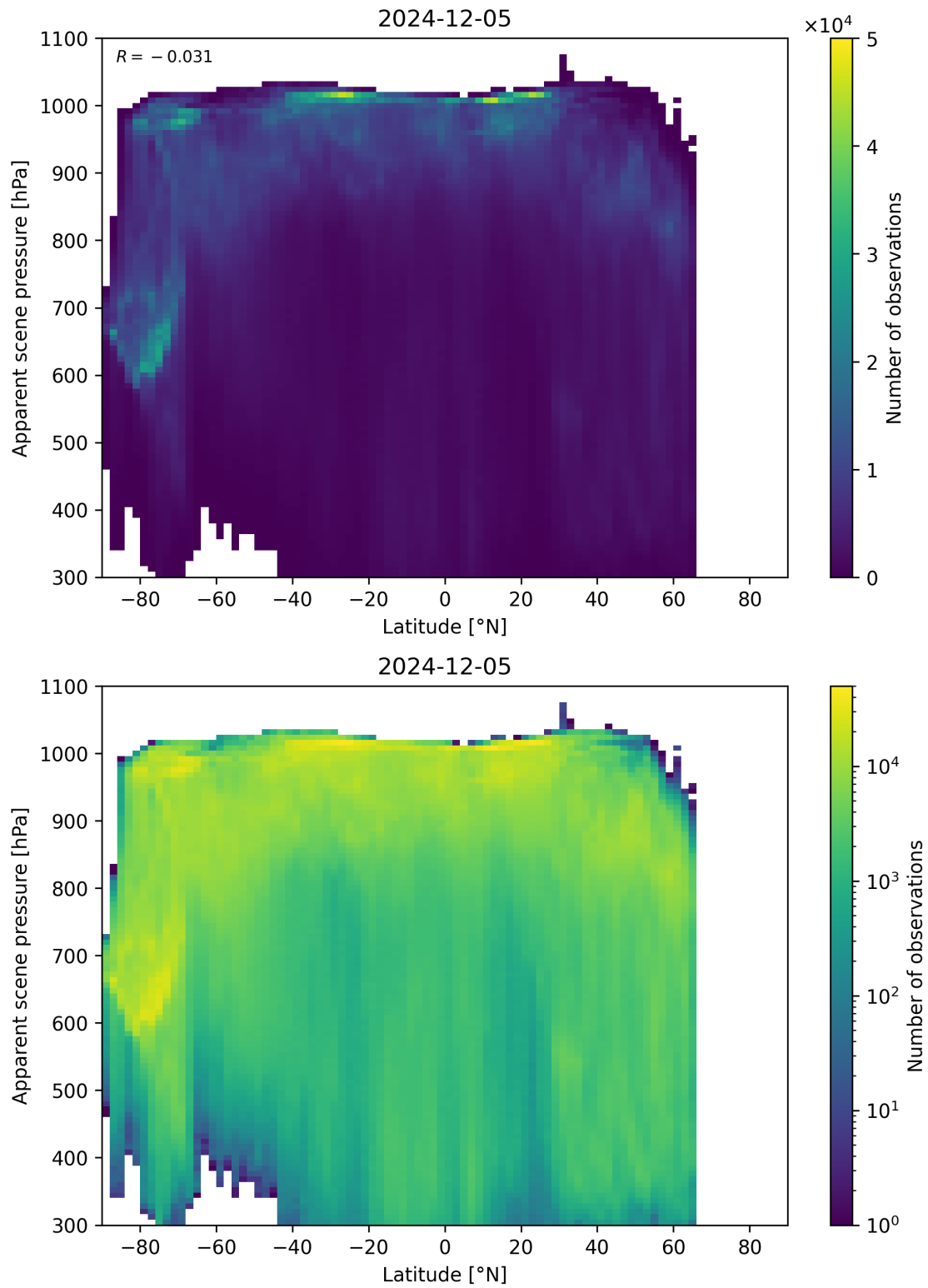
Figure 88: Scatter density plot of “Latitude” against “Apparent scene pressure” for 2024-12-04 to 2024-12-06.
