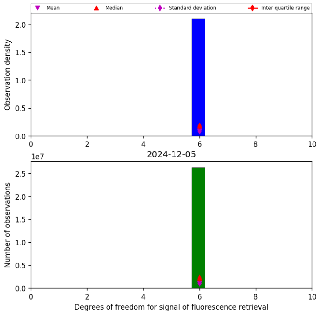
Figure 43: Histogram of "Degrees of freedom for signal of fluorescence retrieval" for 2024-12-04 to 2024-12-06
