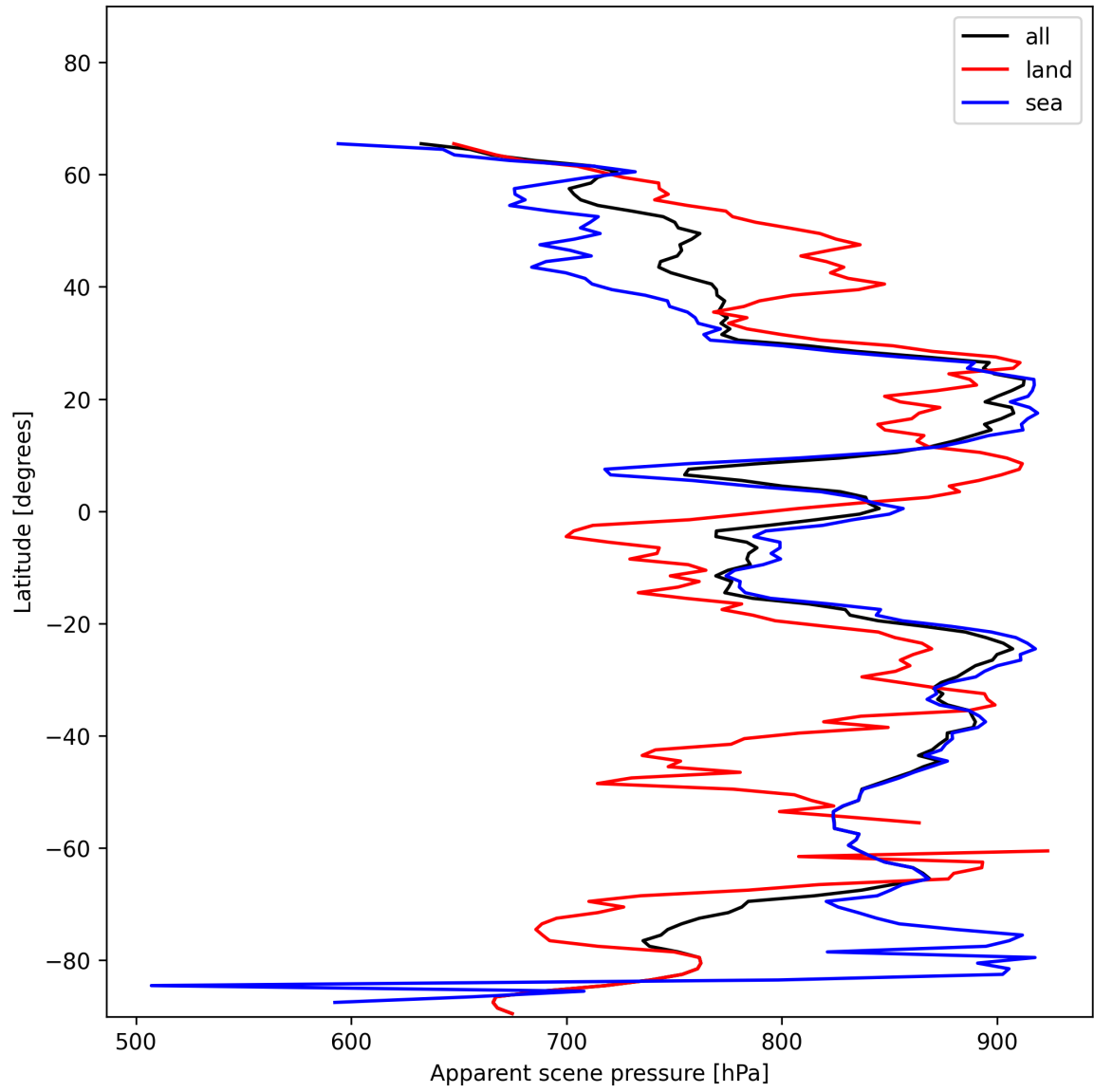
Figure 19: Zonal average of “Apparent scene pressure” for 2024-12-04 to 2024-12-06.
