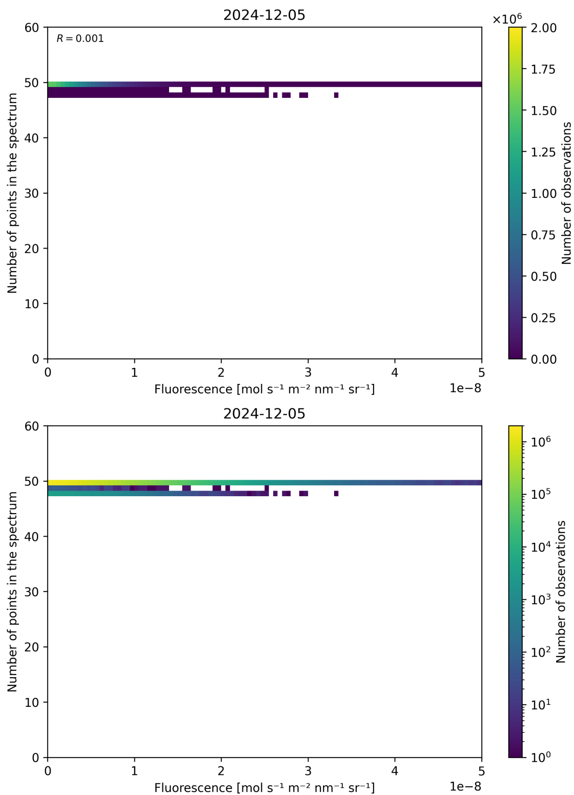
Figure 86: Scatter density plot of “Fluorescence” against “Number of points in the spectrum” for 2024-12-04 to 2024-12-06.
