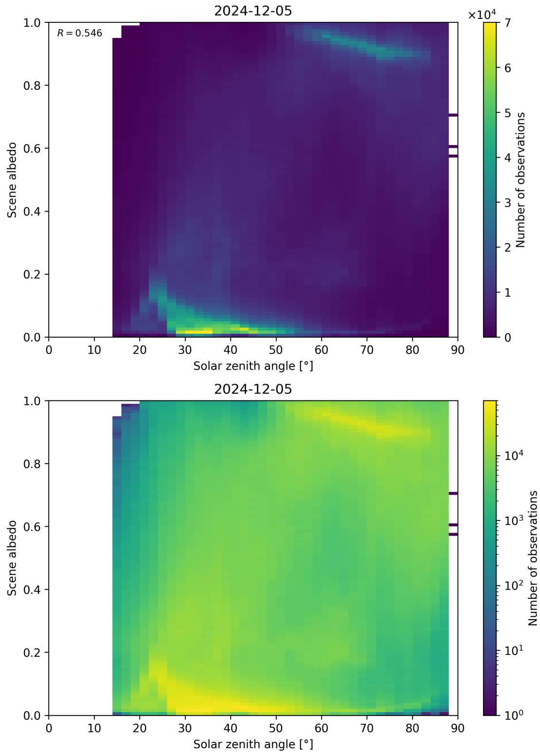
Figure 116: Scatter density plot of “Solar zenith angle” against “Scene albedo” for 2024-12-04 to 2024-12-06.
