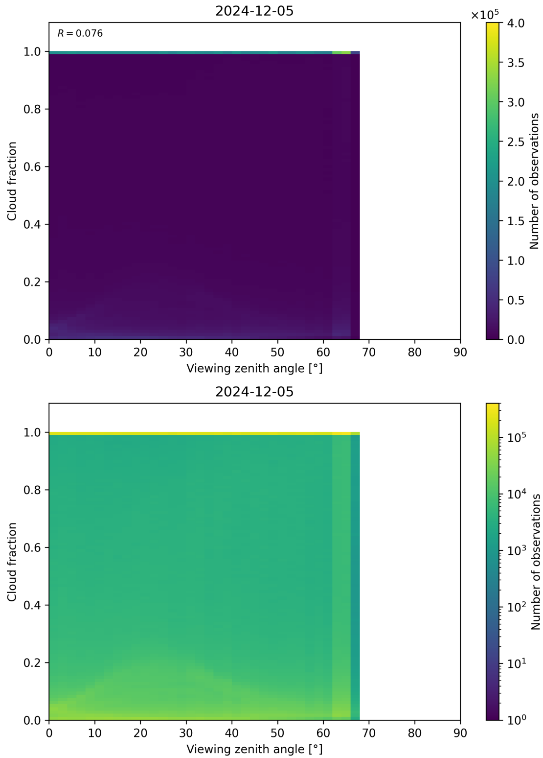
Figure 120: Scatter density plot of “Viewing zenith angle” against “Cloud fraction” for 2024-12-04 to 2024-12-06.
