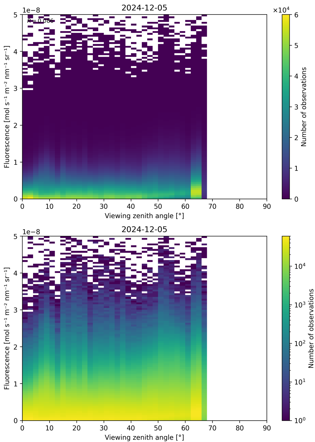
Figure 122: Scatter density plot of “Viewing zenith angle” against “Fluorescence” for 2024-12-04 to 2024-12-06.
