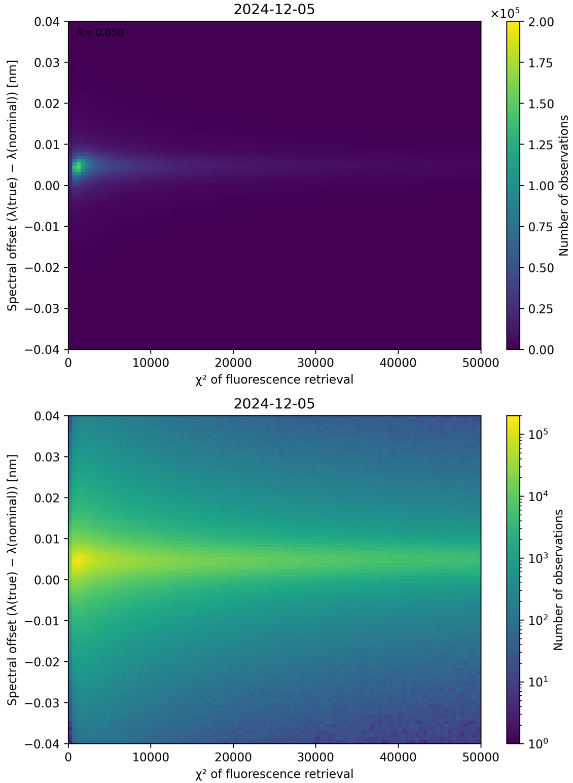
Figure 69: Scatter density plot of “ \chi^2 of fluorescence retrieval” against “Spectral offset ( \lambda_{\text{true}} - \lambda_{\text{nominal}} )” for 2024-12-04 to 2024-12-06.
