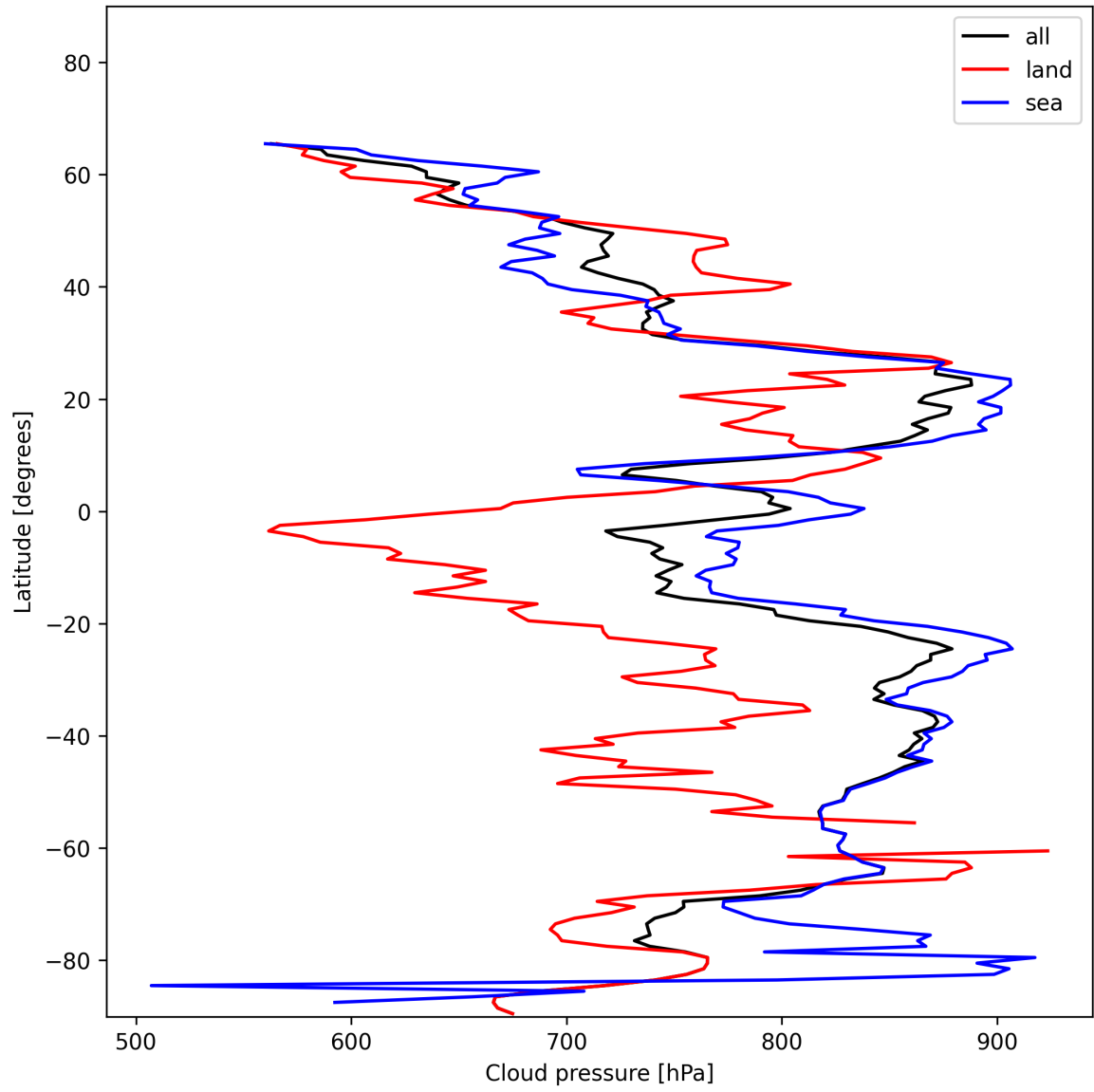
Figure 13: Zonal average of “Cloud pressure” for 2024-12-04 to 2024-12-06.
