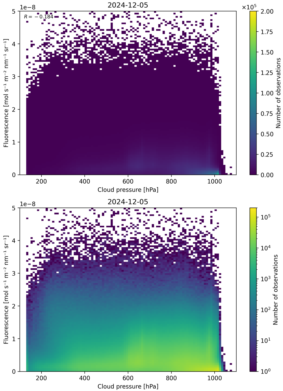
Figure 80: Scatter density plot of “Cloud pressure” against “Fluorescence” for 2024-12-04 to 2024-12-06.
