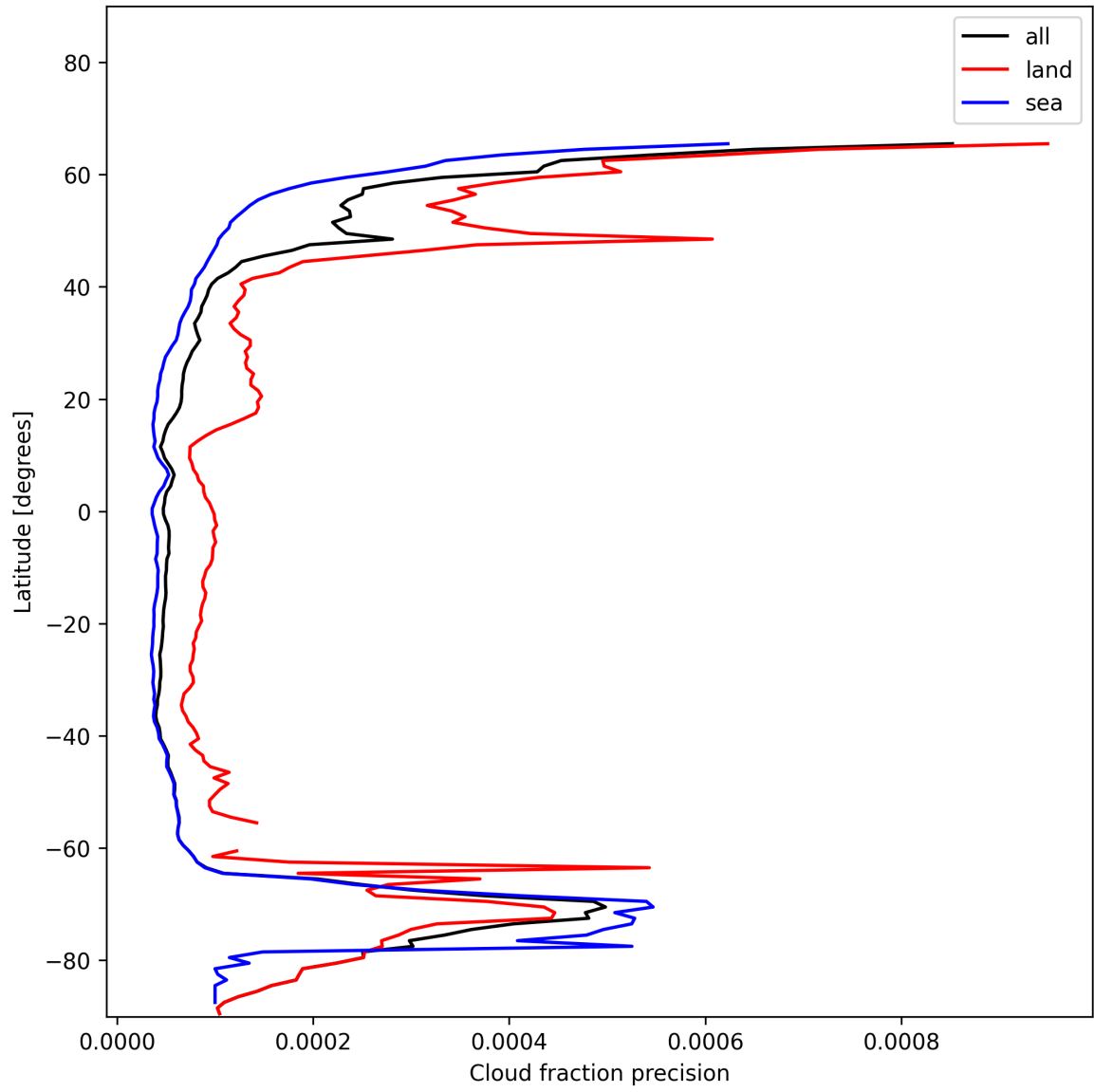
Figure 16: Zonal average of “Cloud fraction precision” for 2024-12-04 to 2024-12-06.
