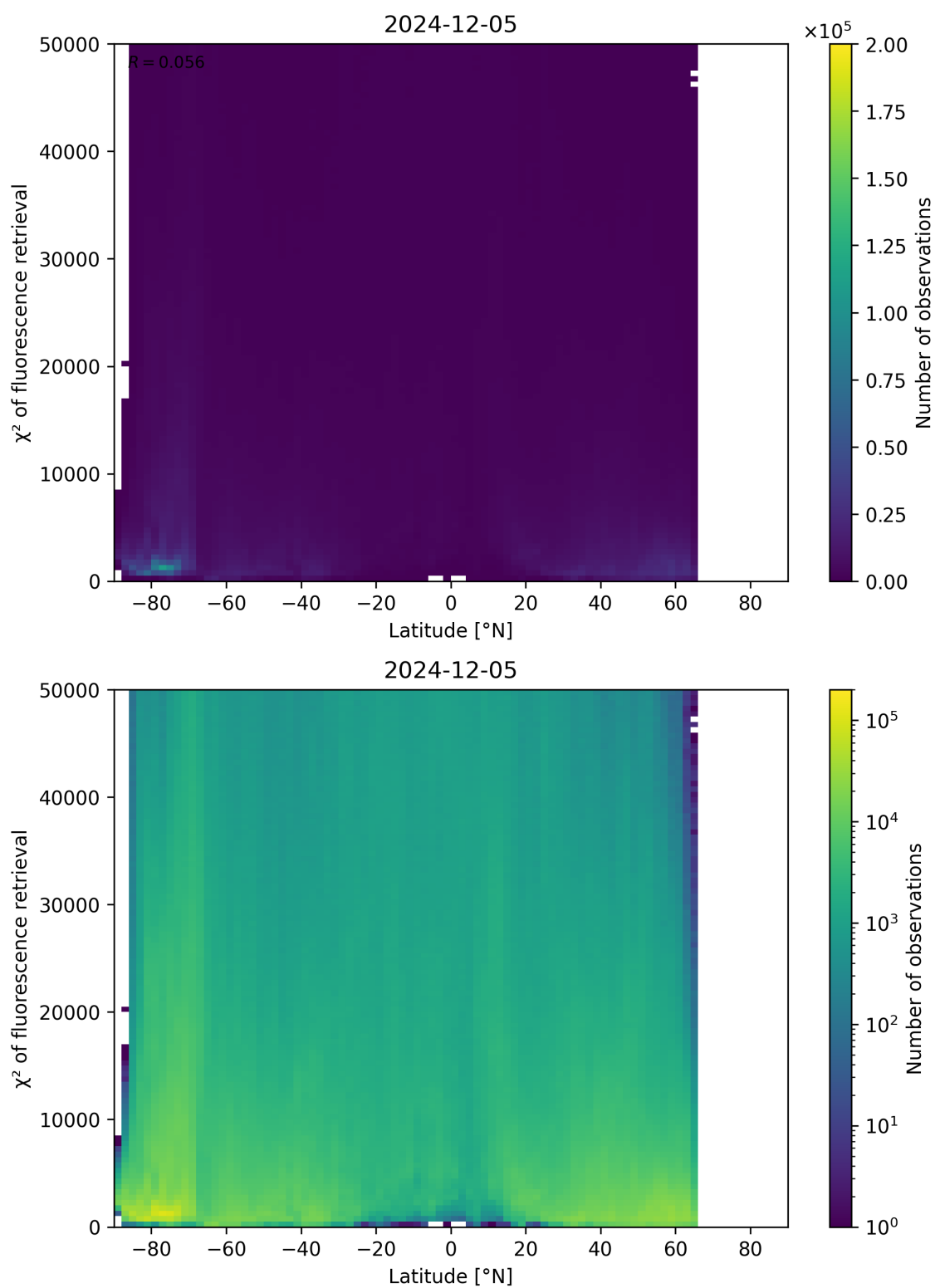
Figure 89: Scatter density plot of “Latitude” against “ \chi^2 of fluorescence retrieval” for 2024-12-04 to 2024-12-06.
