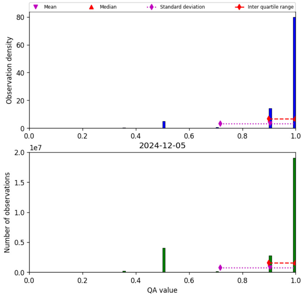
Figure 29: Histogram of “QA value” for 2024-12-04 to 2024-12-06
