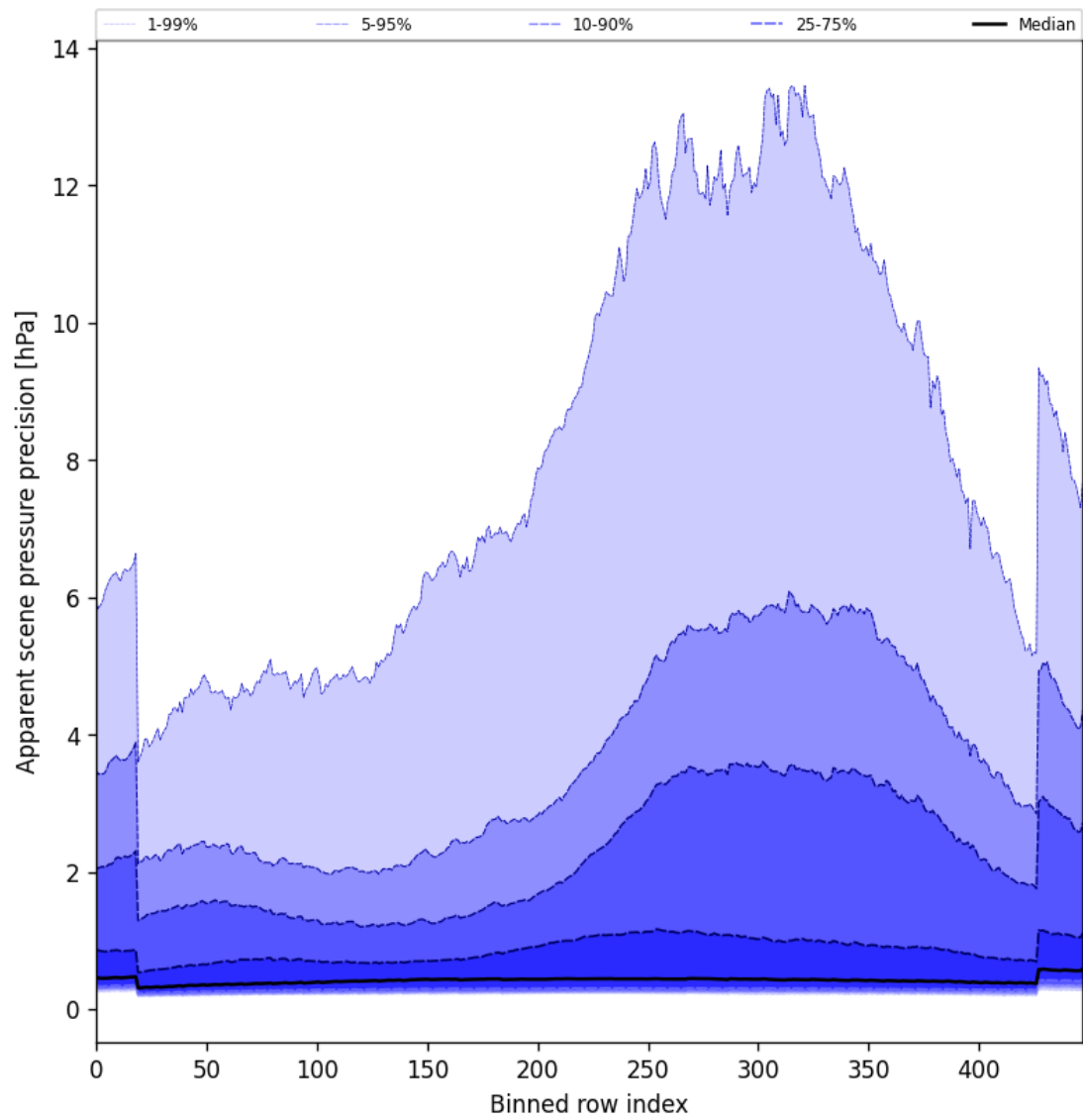
Figure 54: Along track statistics of “Apparent scene pressure precision” for 2024-12-04 to 2024-12-06
