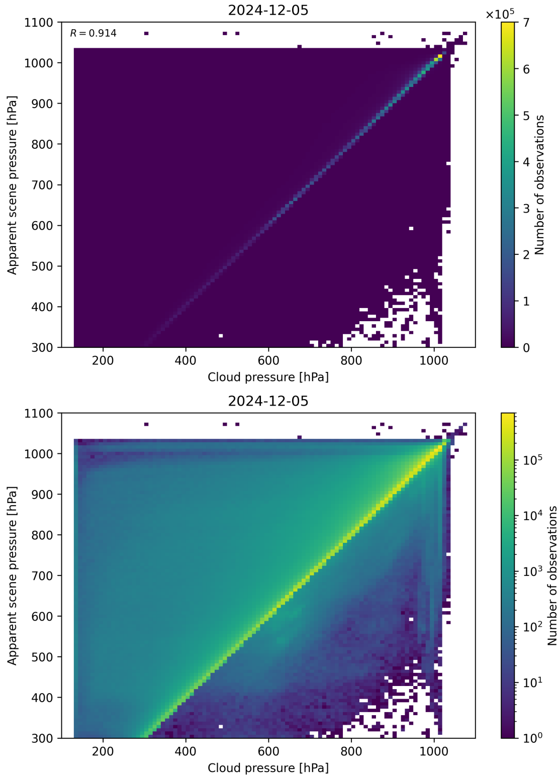
Figure 77: Scatter density plot of “Cloud pressure” against “Apparent scene pressure” for 2024-12-04 to 2024-12-06.
