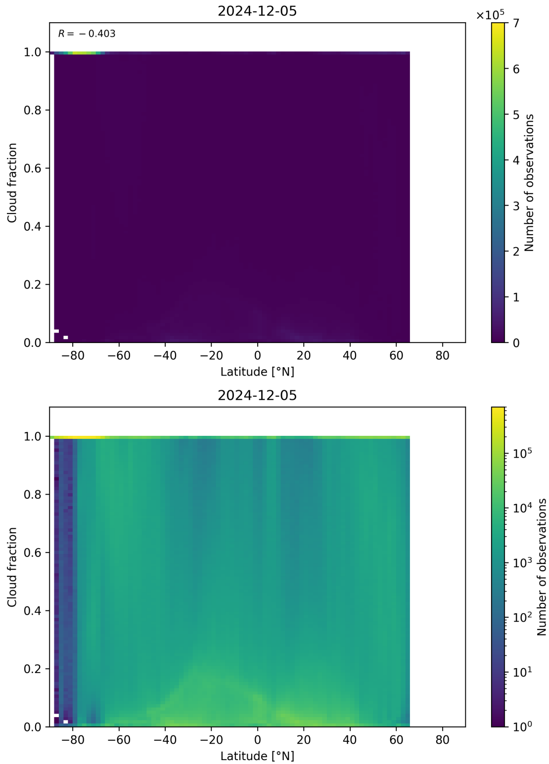
Figure 90: Scatter density plot of “Latitude” against “Cloud fraction” for 2024-12-04 to 2024-12-06.
