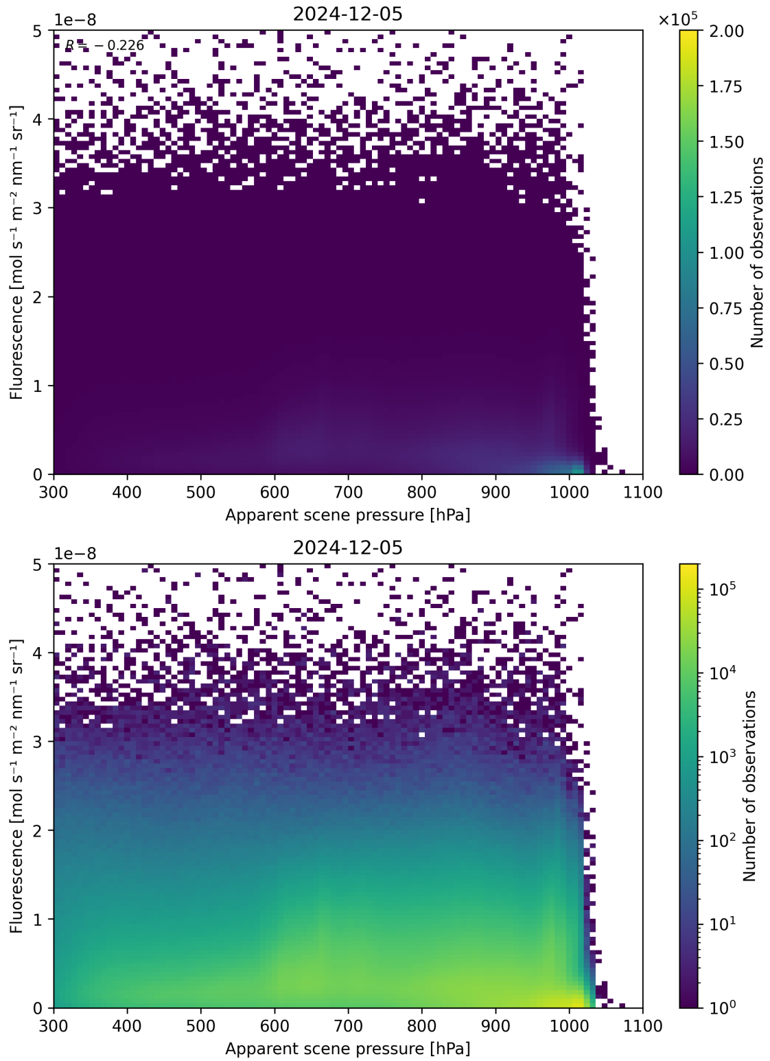
Figure 64: Scatter density plot of “Apparent scene pressure” against “Fluorescence” for 2024-12-04 to 2024-12-06.
