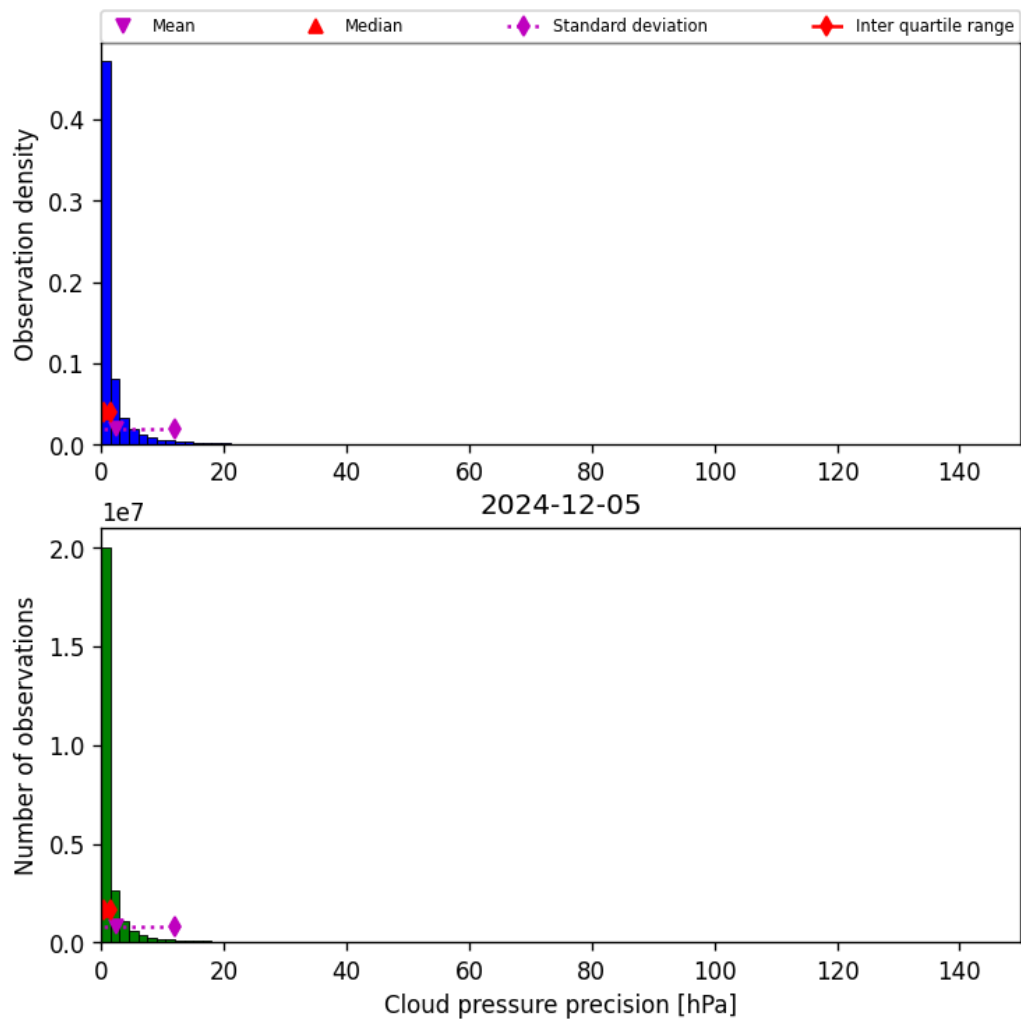
Figure 31: Histogram of “Cloud pressure precision” for 2024-12-04 to 2024-12-06
