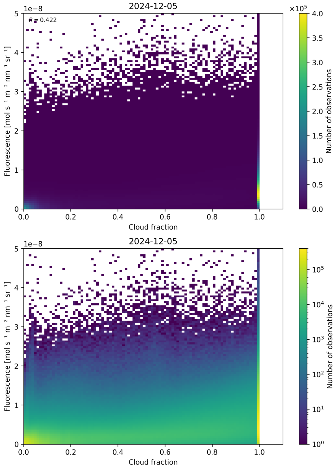
Figure 72: Scatter density plot of “Cloud fraction” against “Fluorescence” for 2024-12-04 to 2024-12-06.
