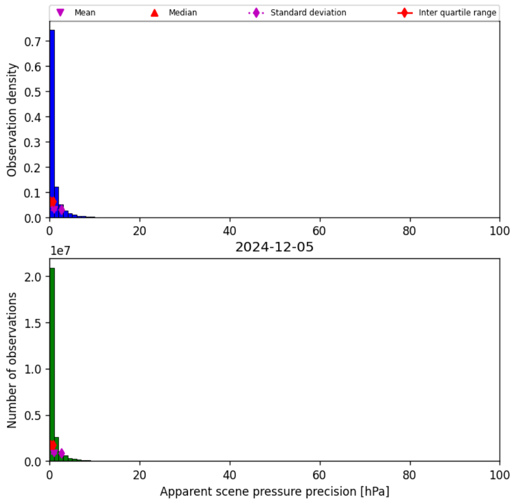
Figure 37: Histogram of “Apparent scene pressure precision” for 2024-12-04 to 2024-12-06
