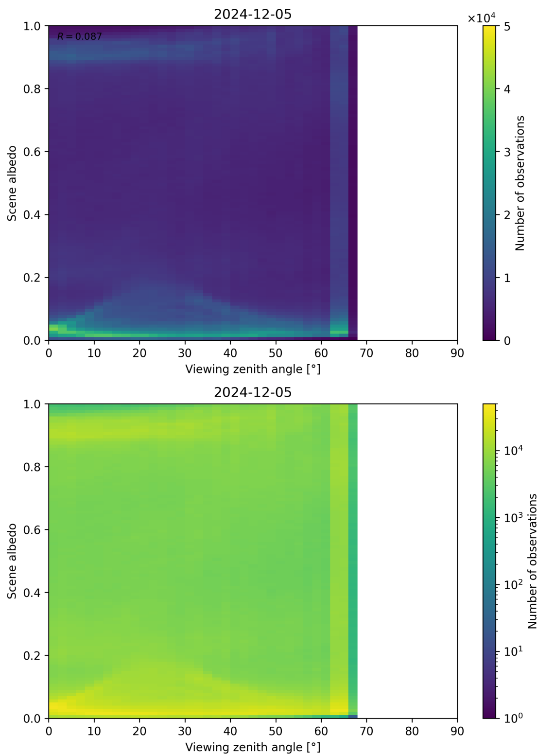
Figure 126: Scatter density plot of “Viewing zenith angle” against “Scene albedo” for 2024-12-04 to 2024-12-06.
