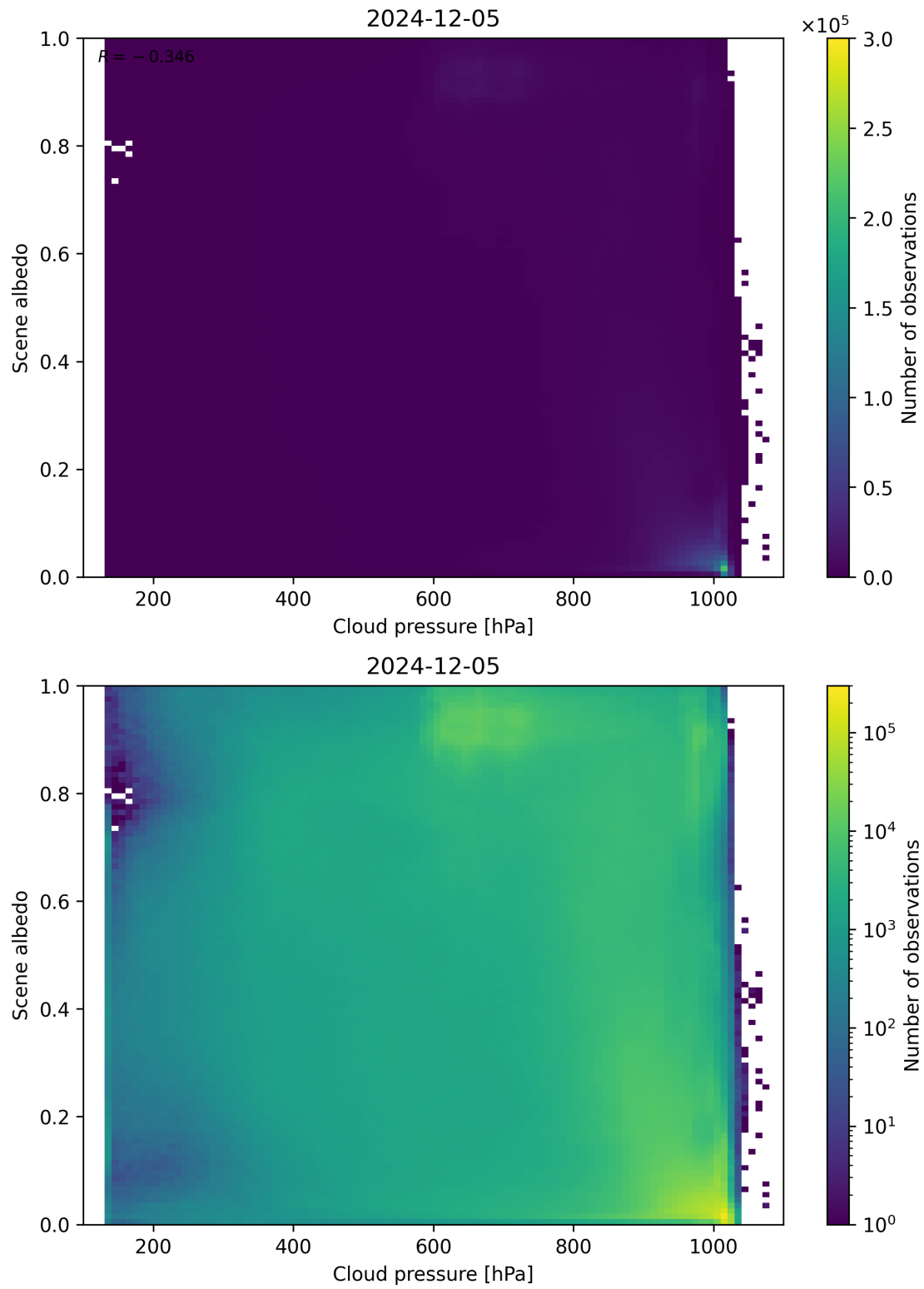
Figure 83: Scatter density plot of “Cloud pressure” against “Scene albedo” for 2024-12-04 to 2024-12-06.
