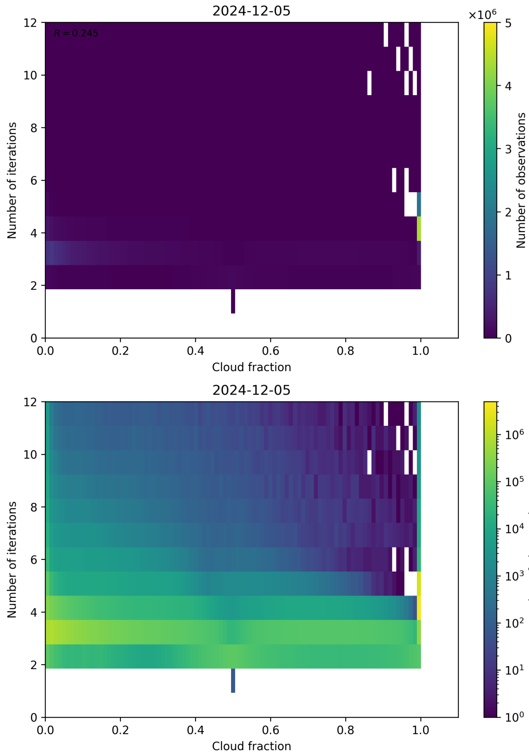
Figure 73: Scatter density plot of “Cloud fraction” against “Number of iterations” for 2024-12-04 to 2024-12-06.
