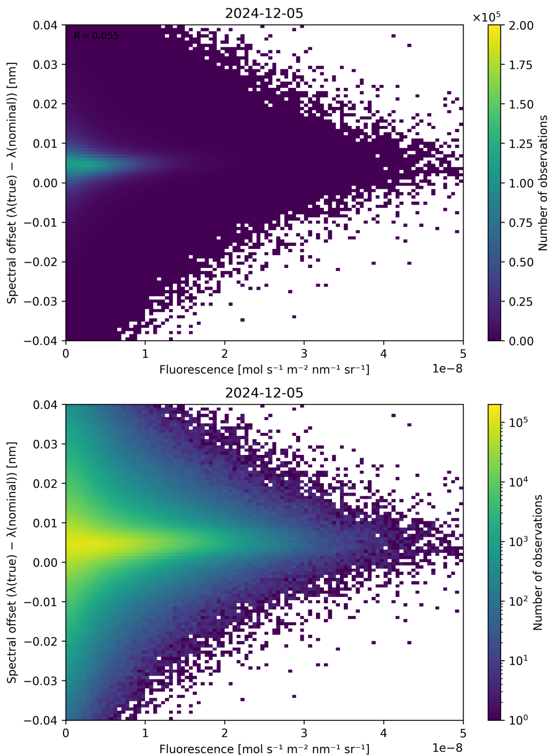
Figure 87: Scatter density plot of “Fluorescence” against “Spectral offset ( \lambda_{\text{true}} - \lambda_{\text{nominal}} )” for 2024-12-04 to 2024-12-06.
