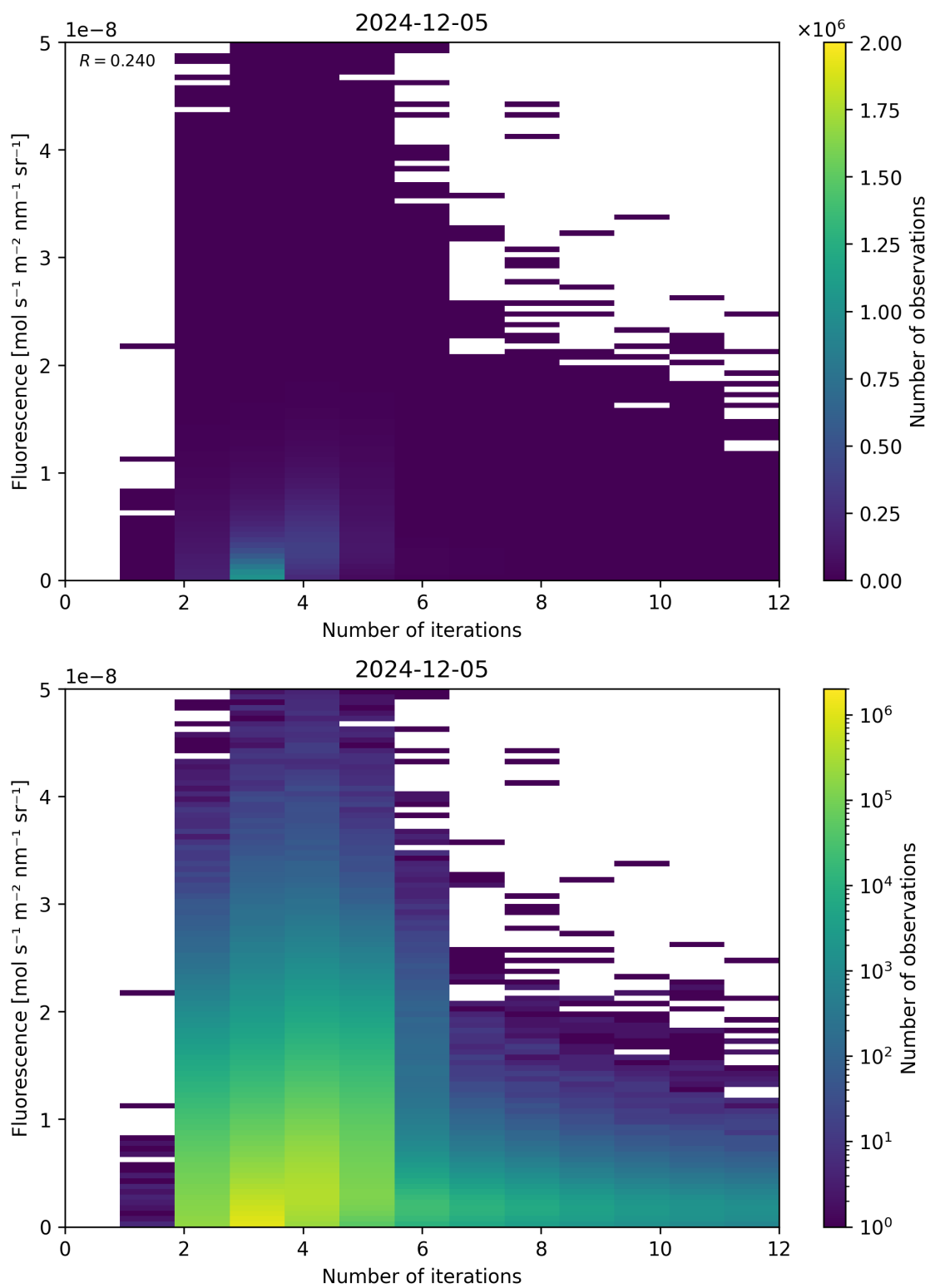
Figure 98: Scatter density plot of “Number of iterations” against “Fluorescence” for 2024-12-04 to 2024-12-06.
