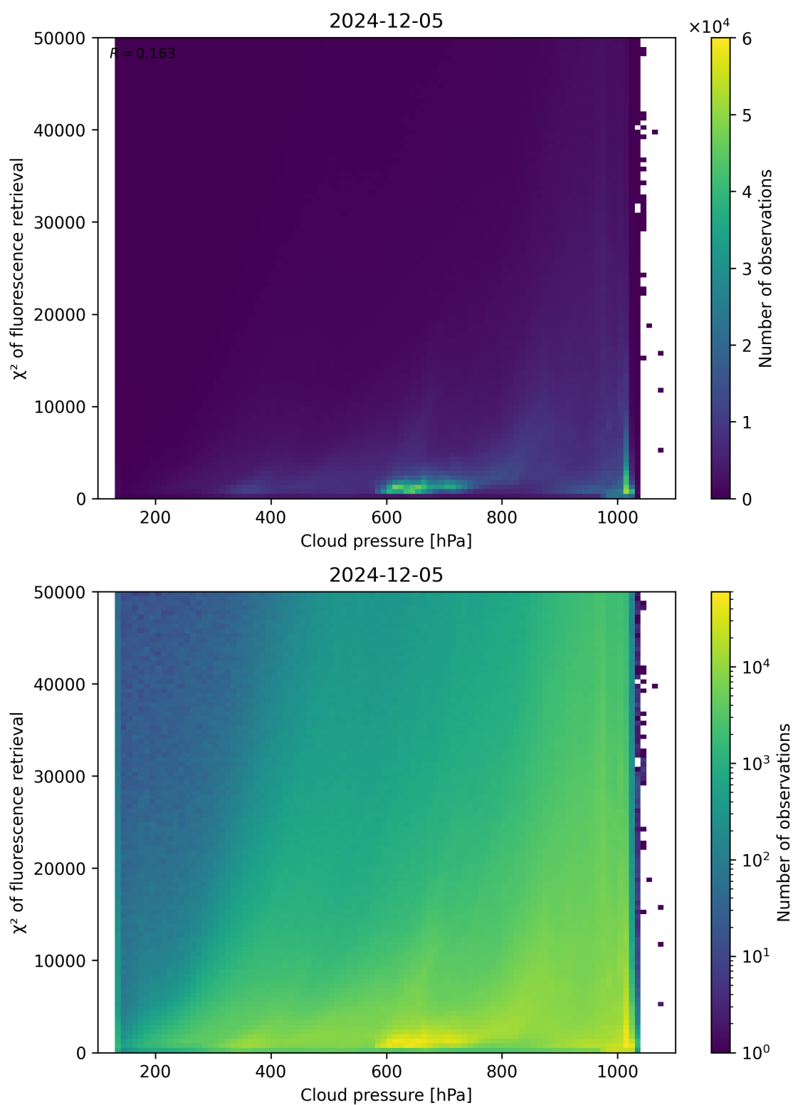
Figure 78: Scatter density plot of “Cloud pressure” against “ \chi^2 of fluorescence retrieval” for 2024-12-04 to 2024-12-06.
