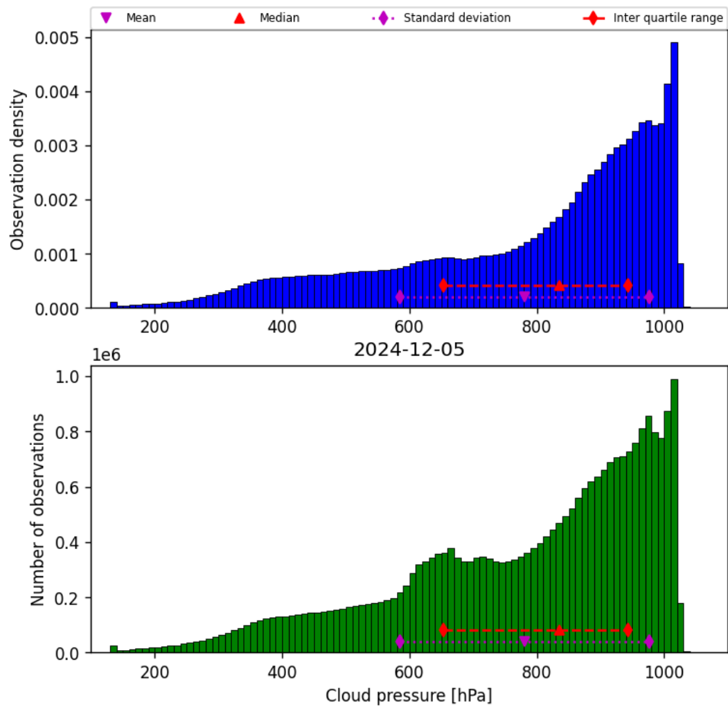
Figure 30: Histogram of “Cloud pressure” for 2024-12-04 to 2024-12-06
