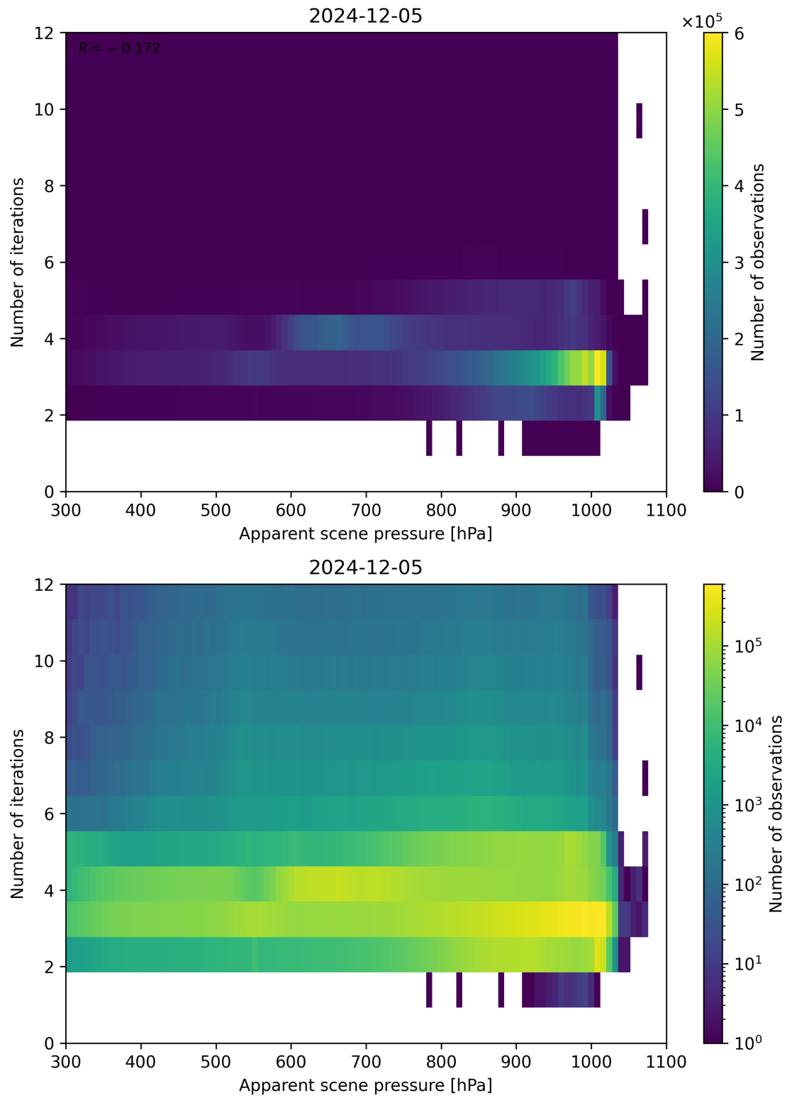
Figure 65: Scatter density plot of “Apparent scene pressure” against “Number of iterations” for 2024-12-04 to 2024-12-06.
