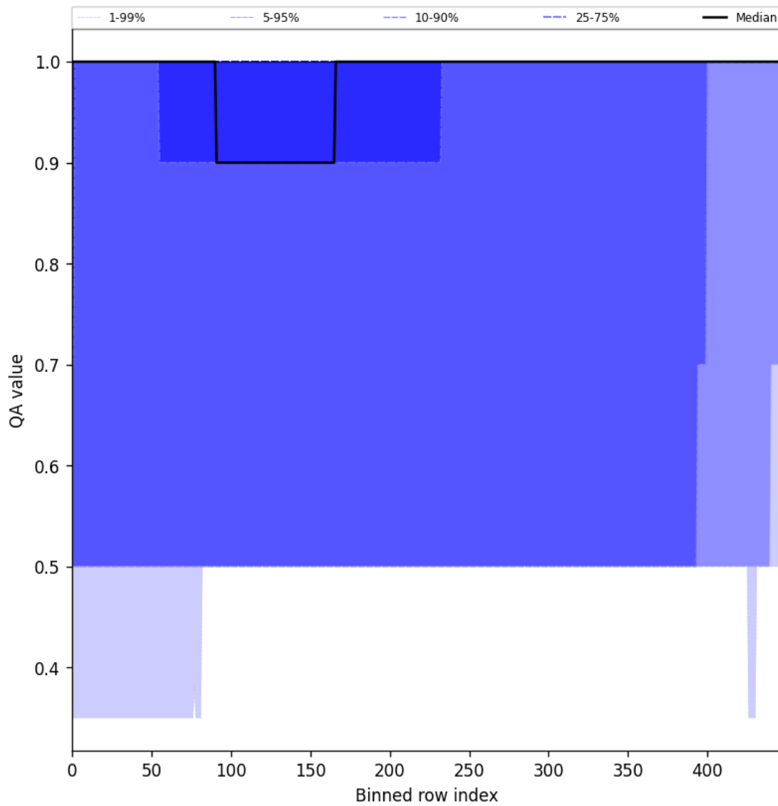
Figure 46: Along track statistics of “QA value” for 2024-12-04 to 2024-12-06
