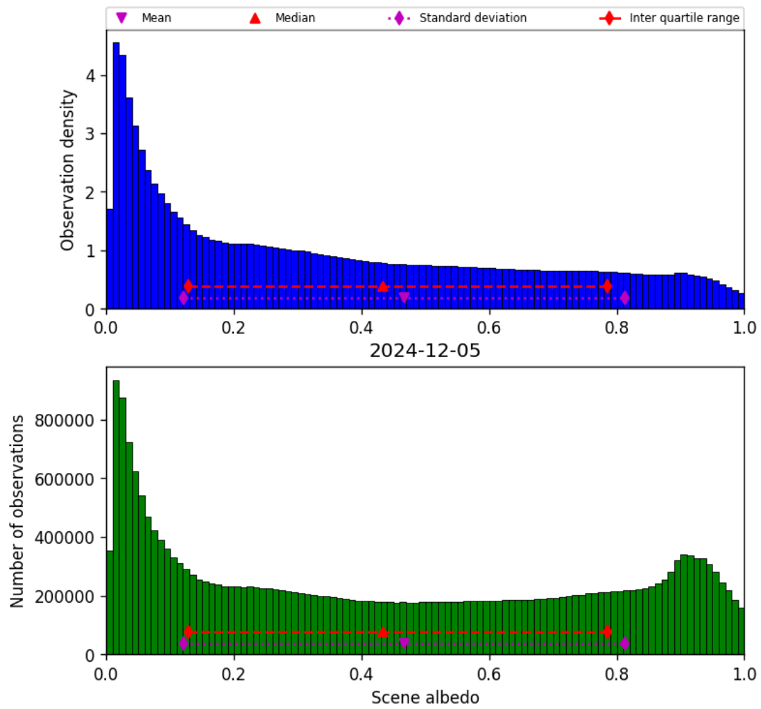
Figure 34: Histogram of “Scene albedo” for 2024-12-04 to 2024-12-06
