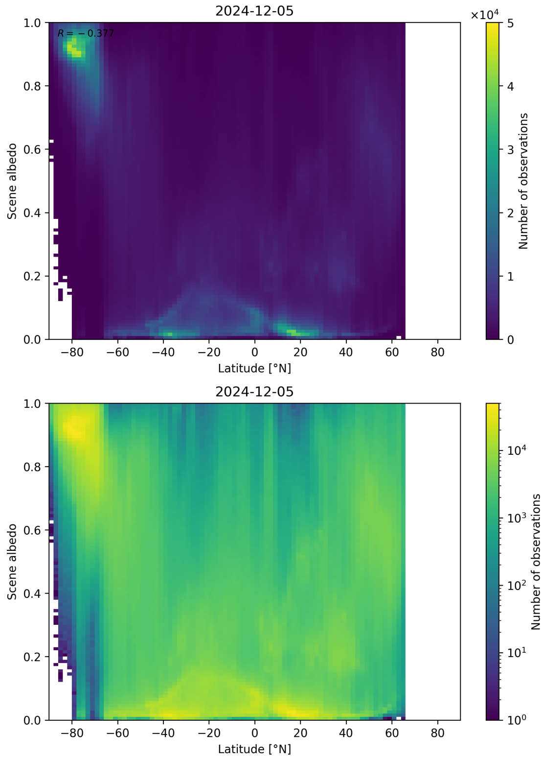
Figure 95: Scatter density plot of “Latitude” against “Scene albedo” for 2024-12-04 to 2024-12-06.
