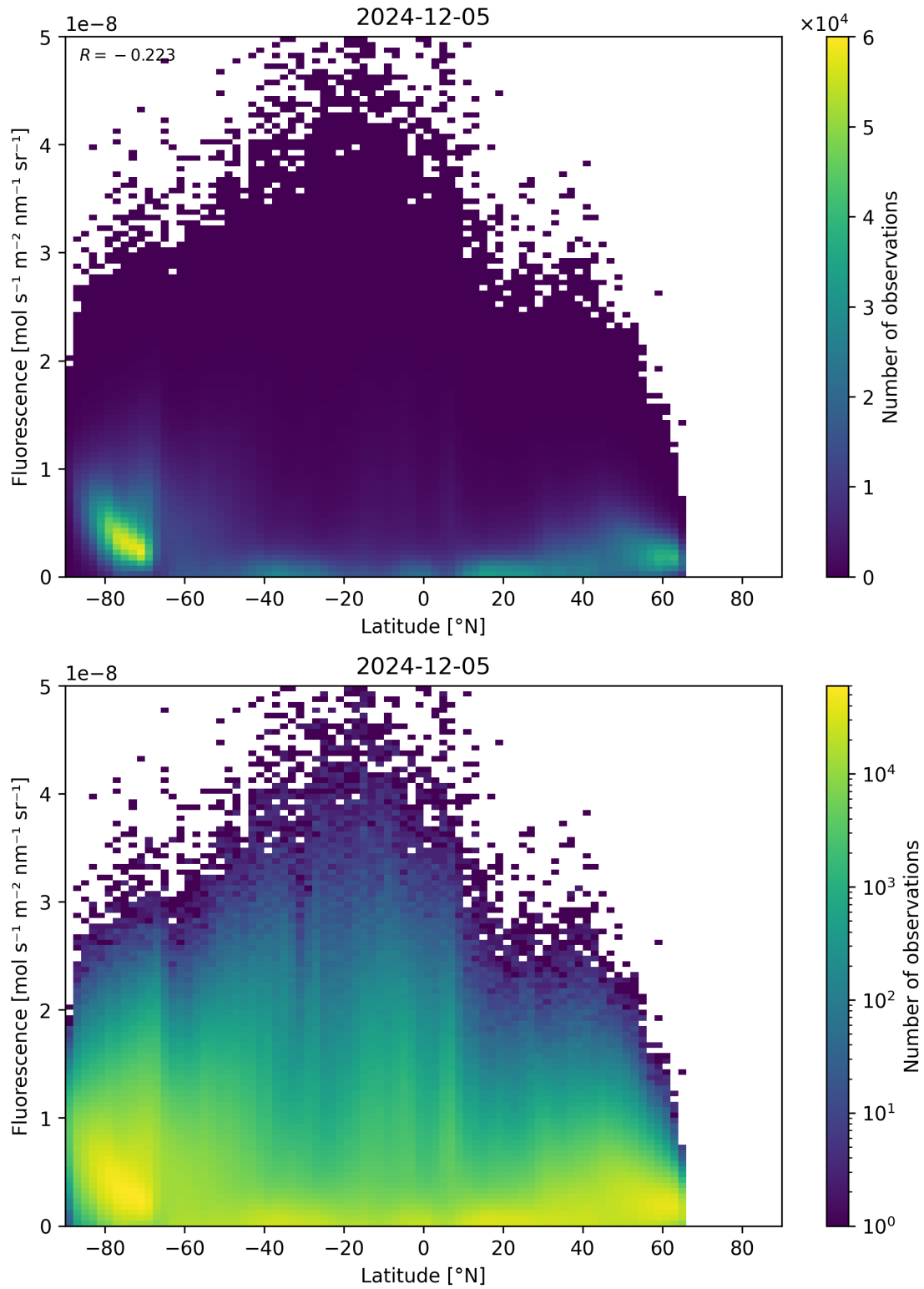
Figure 92: Scatter density plot of “Latitude” against “Fluorescence” for 2024-12-04 to 2024-12-06.
