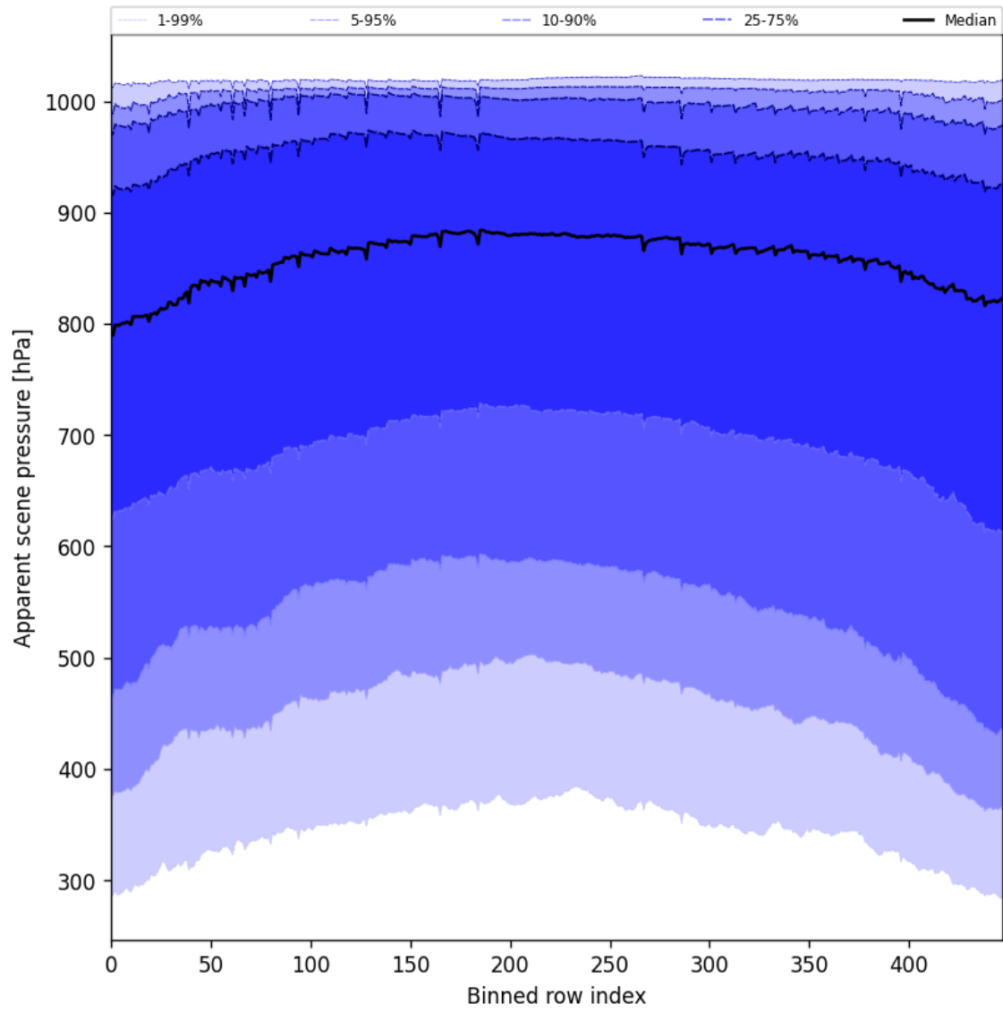
Figure 53: Along track statistics of “Apparent scene pressure” for 2024-12-04 to 2024-12-06
