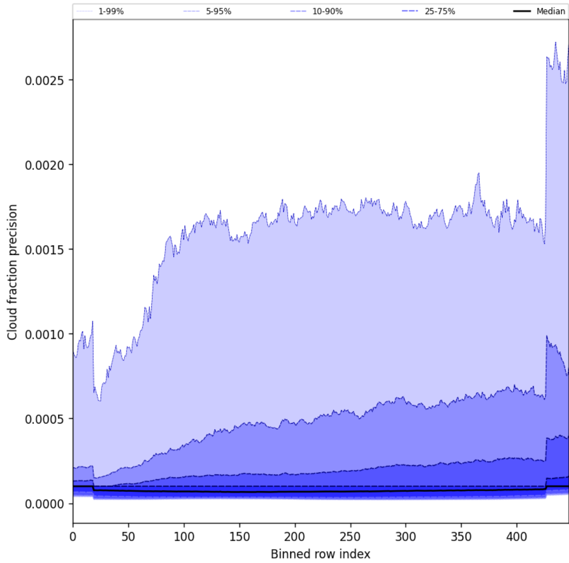
Figure 50: Along track statistics of “Cloud fraction precision” for 2024-12-04 to 2024-12-06
