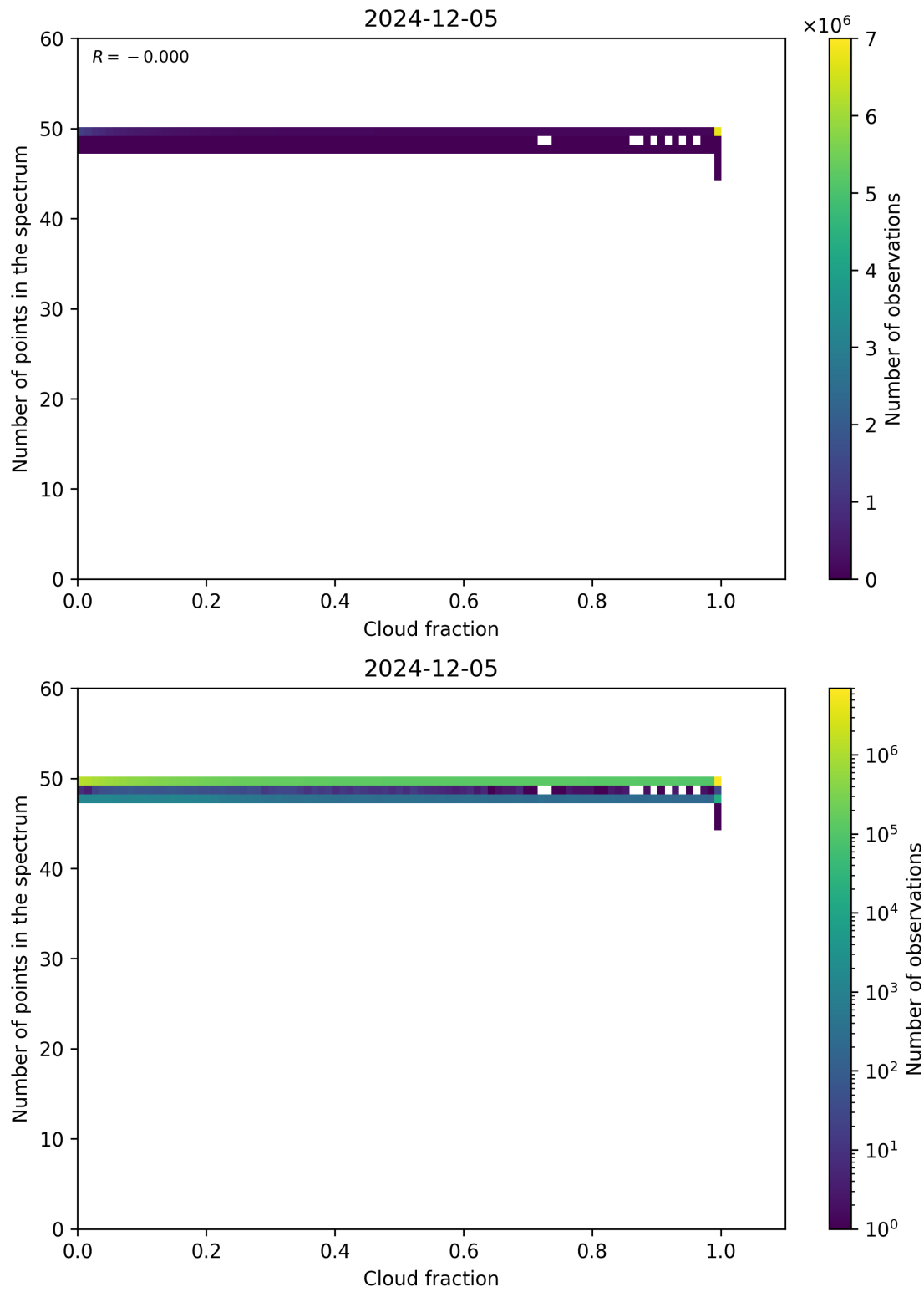
Figure 74: Scatter density plot of “Cloud fraction” against “Number of points in the spectrum” for 2024-12-04 to 2024-12-06.
