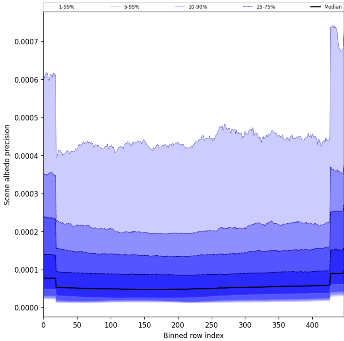
Figure 52: Along track statistics of “Scene albedo precision” for 2024-12-04 to 2024-12-06
