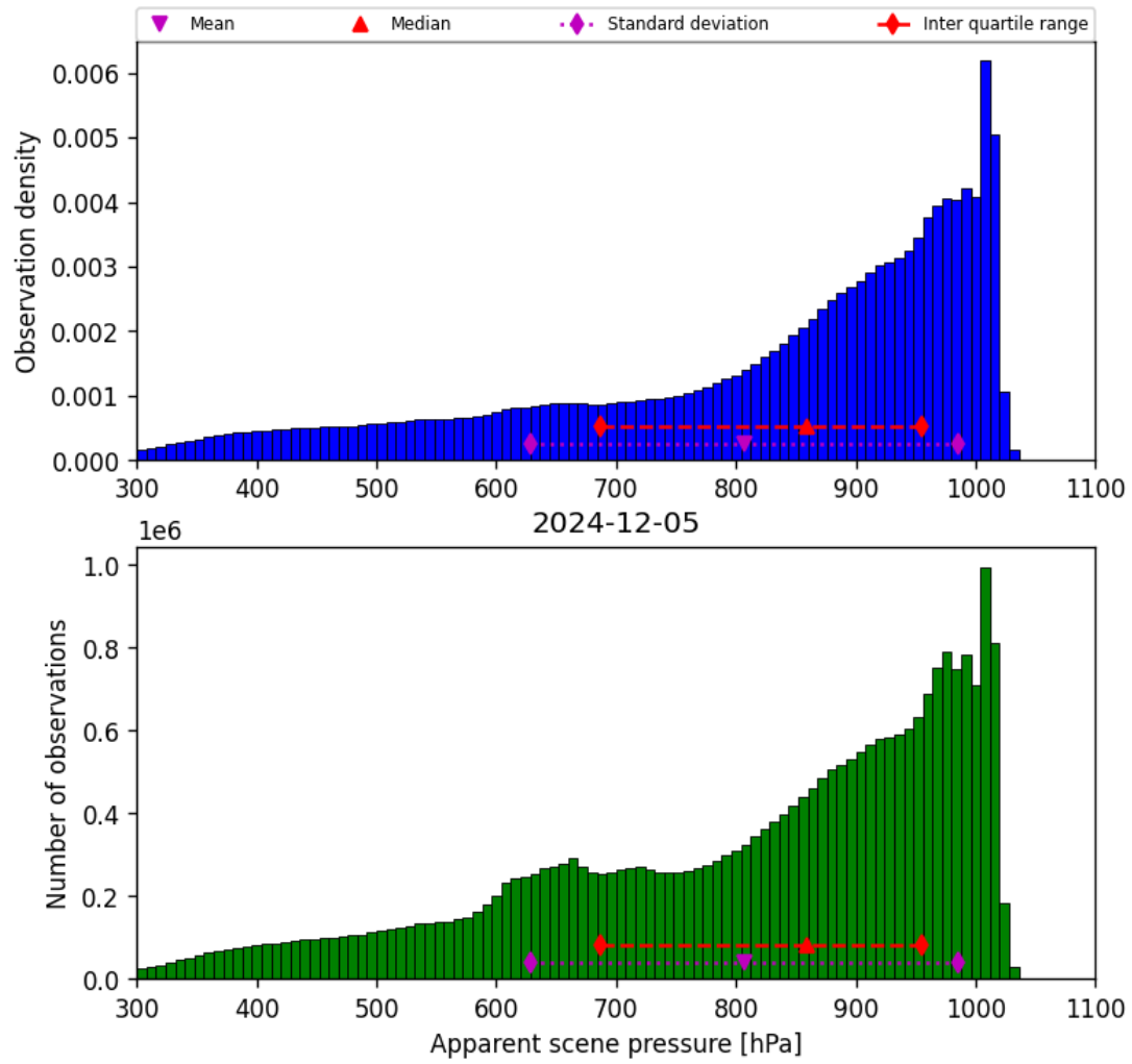
Figure 36: Histogram of “Apparent scene pressure” for 2024-12-04 to 2024-12-06
