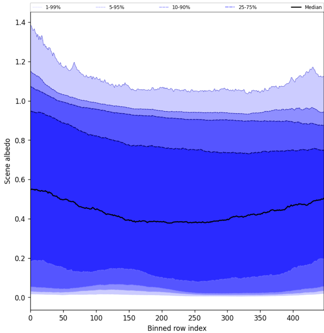
Figure 51: Along track statistics of “Scene albedo” for 2024-12-04 to 2024-12-06
