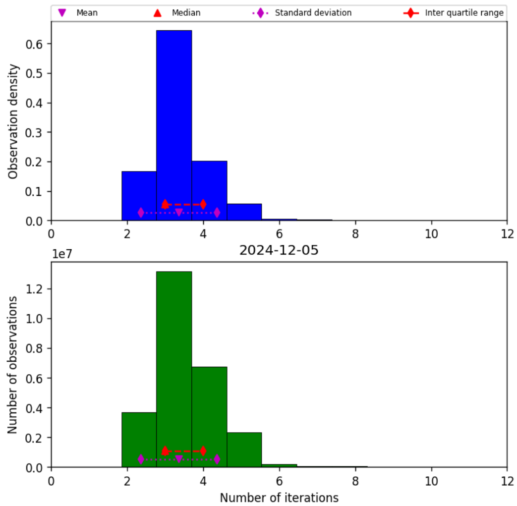
Figure 39: Histogram of “Number of iterations” for 2024-12-04 to 2024-12-06
