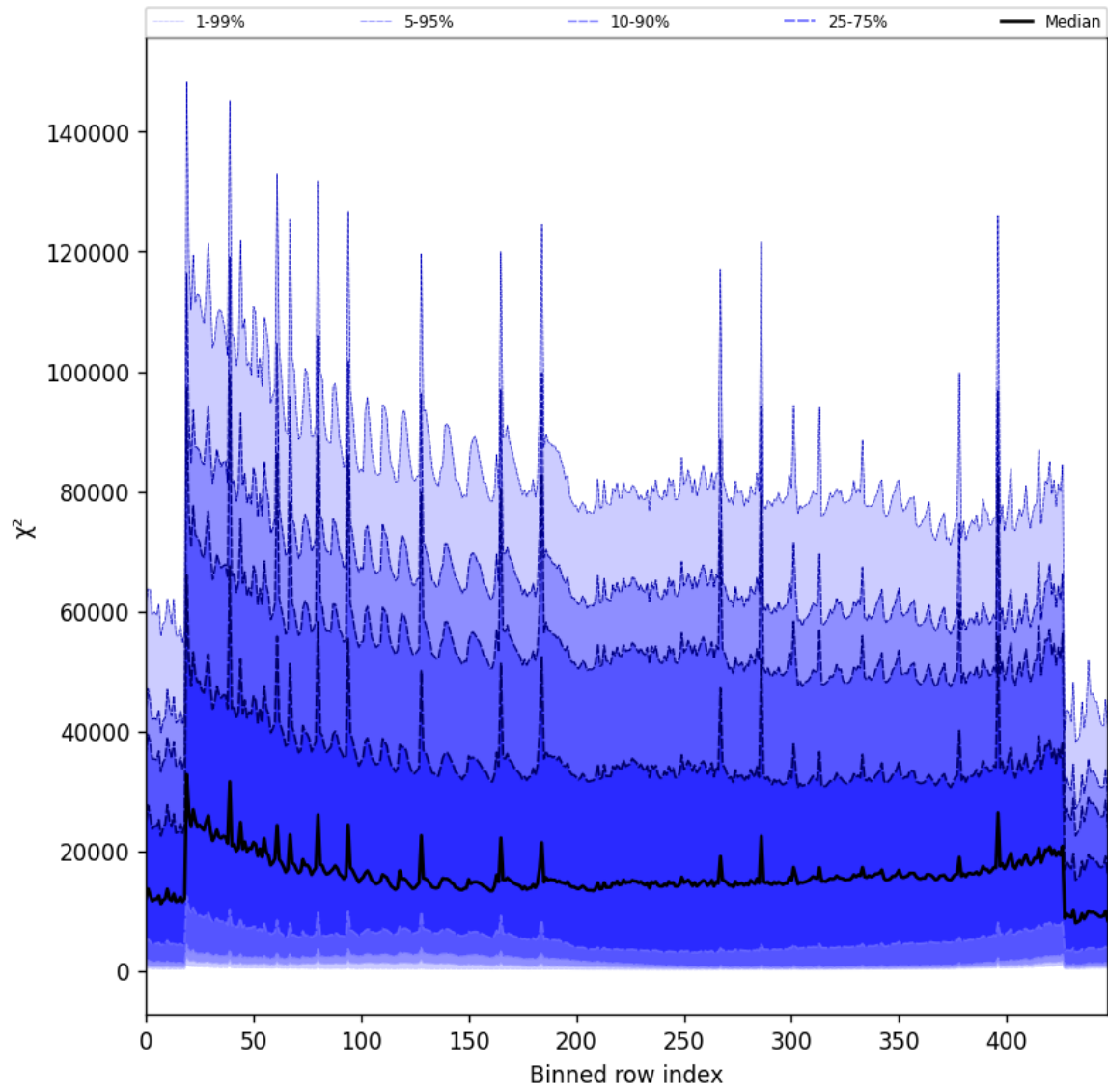
Figure 55: Along track statistics of “ \chi^2 ” for 2024-12-04 to 2024-12-06
