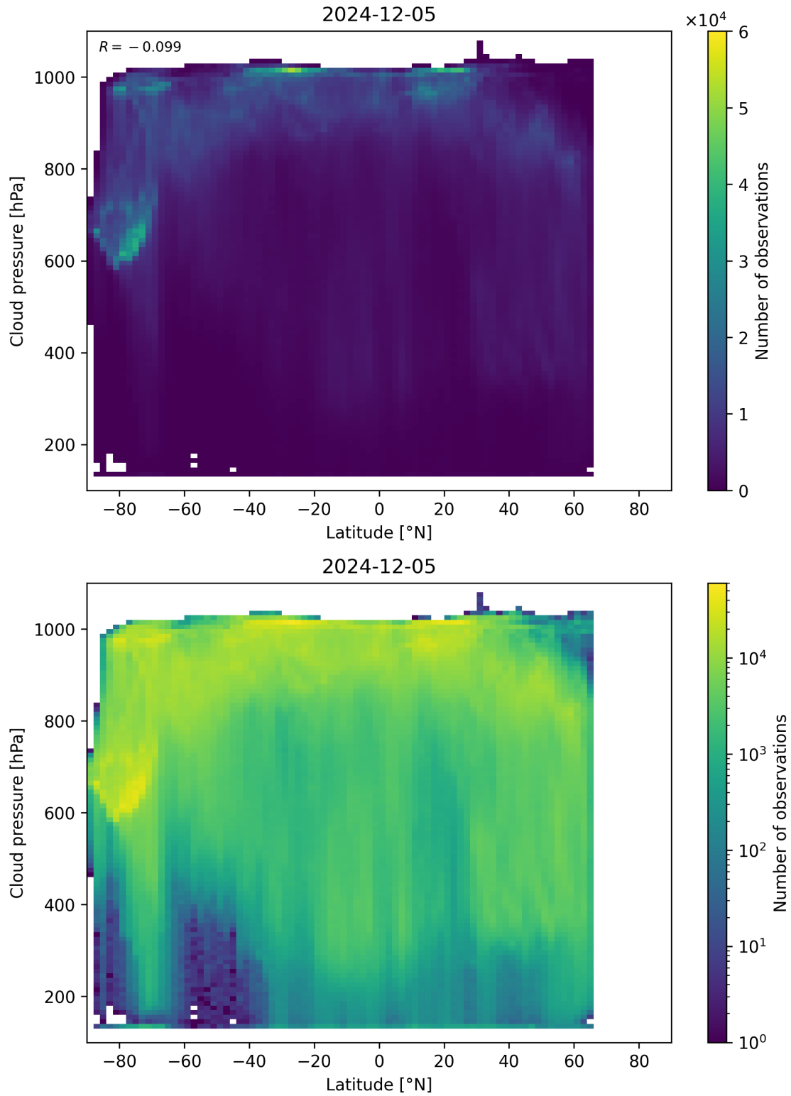
Figure 91: Scatter density plot of “Latitude” against “Cloud pressure” for 2024-12-04 to 2024-12-06.
