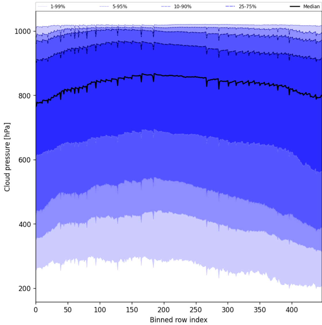
Figure 47: Along track statistics of “Cloud pressure” for 2024-12-04 to 2024-12-06
