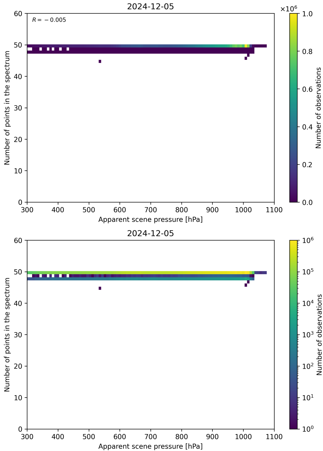
Figure 66: Scatter density plot of “Apparent scene pressure” against “Number of points in the spectrum” for 2024-12-04 to 2024-12-06.
