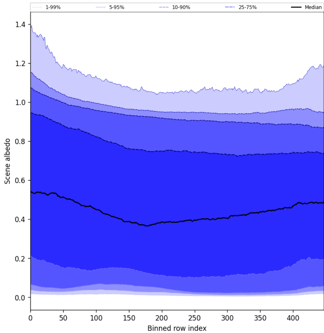
Figure 51: Along track statistics of “Scene albedo” for 2024-12-06 to 2024-12-07
