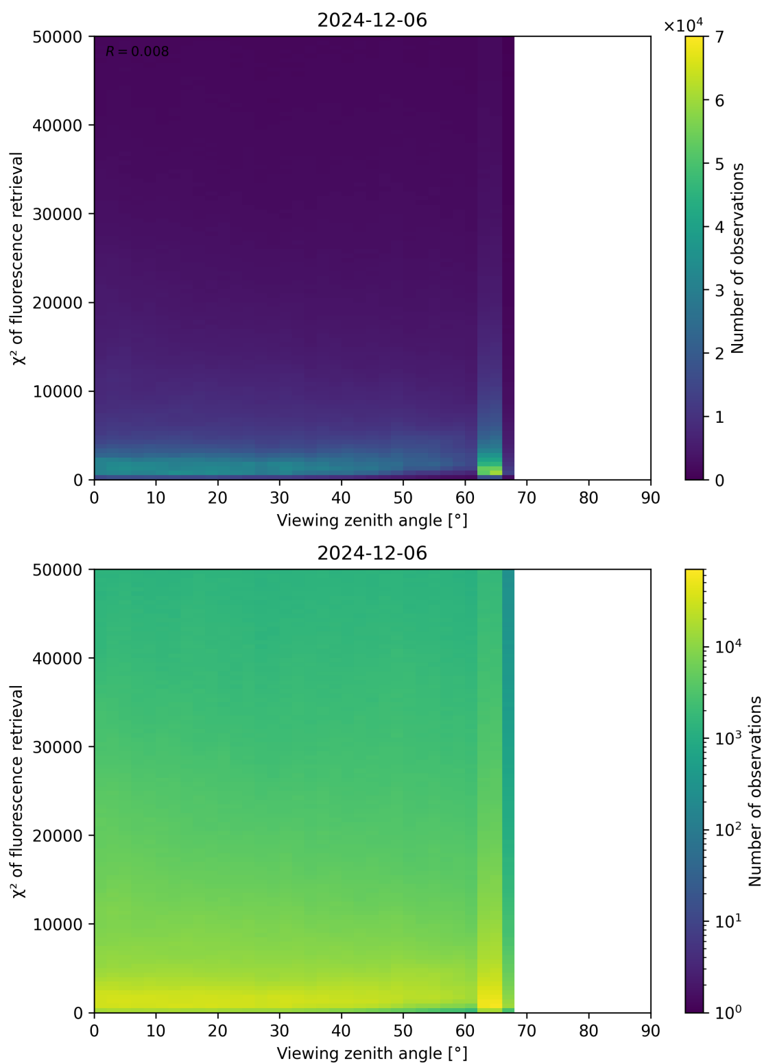
Figure 119: Scatter density plot of “Viewing zenith angle” against “ \chi^2 of fluorescence retrieval” for 2024-12-06 to 2024-12-07.
