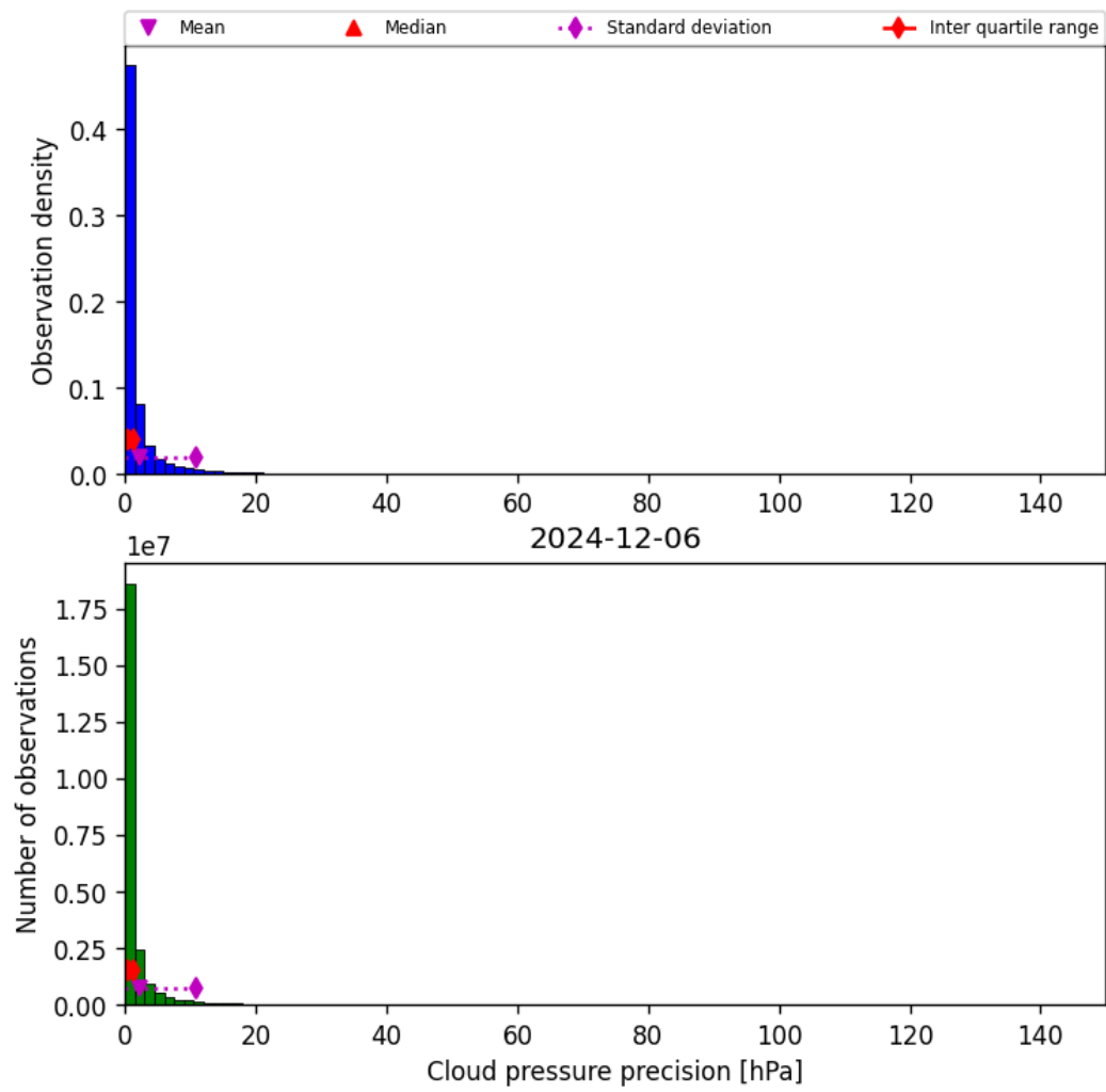
Figure 31: Histogram of “Cloud pressure precision” for 2024-12-06 to 2024-12-07
