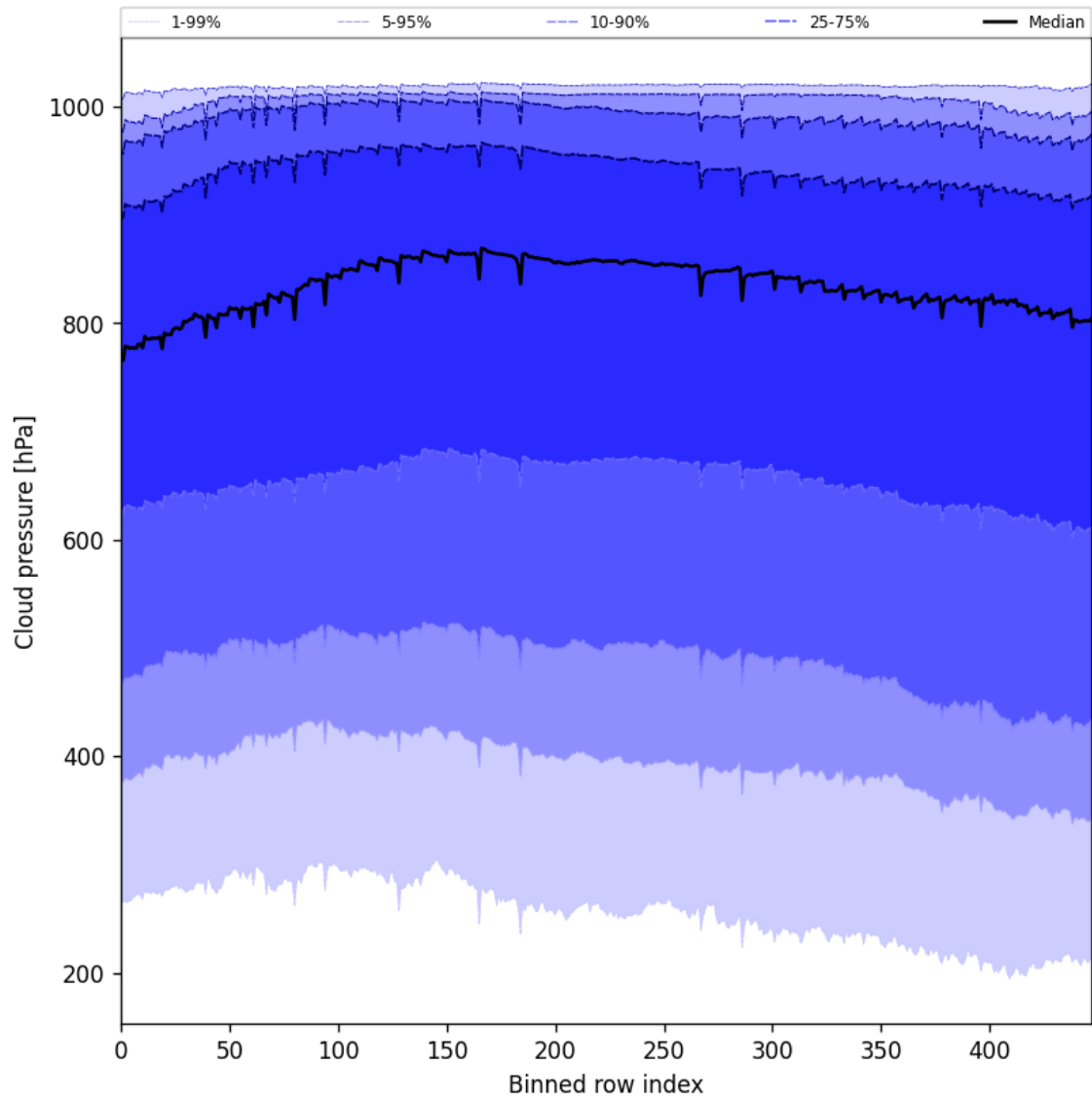
Figure 47: Along track statistics of “Cloud pressure” for 2024-12-06 to 2024-12-07
