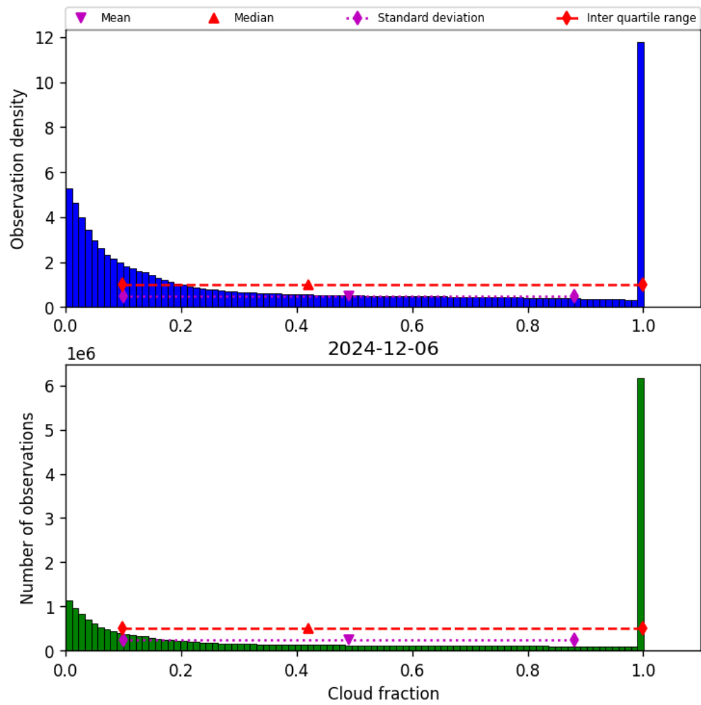
Figure 32: Histogram of “Cloud fraction” for 2024-12-06 to 2024-12-07
