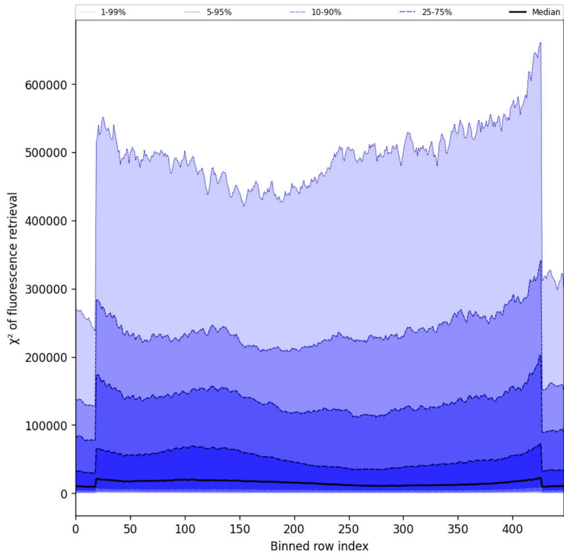
Figure 59: Along track statistics of “ \chi^2 of fluorescence retrieval” for 2024-12-06 to 2024-12-07
