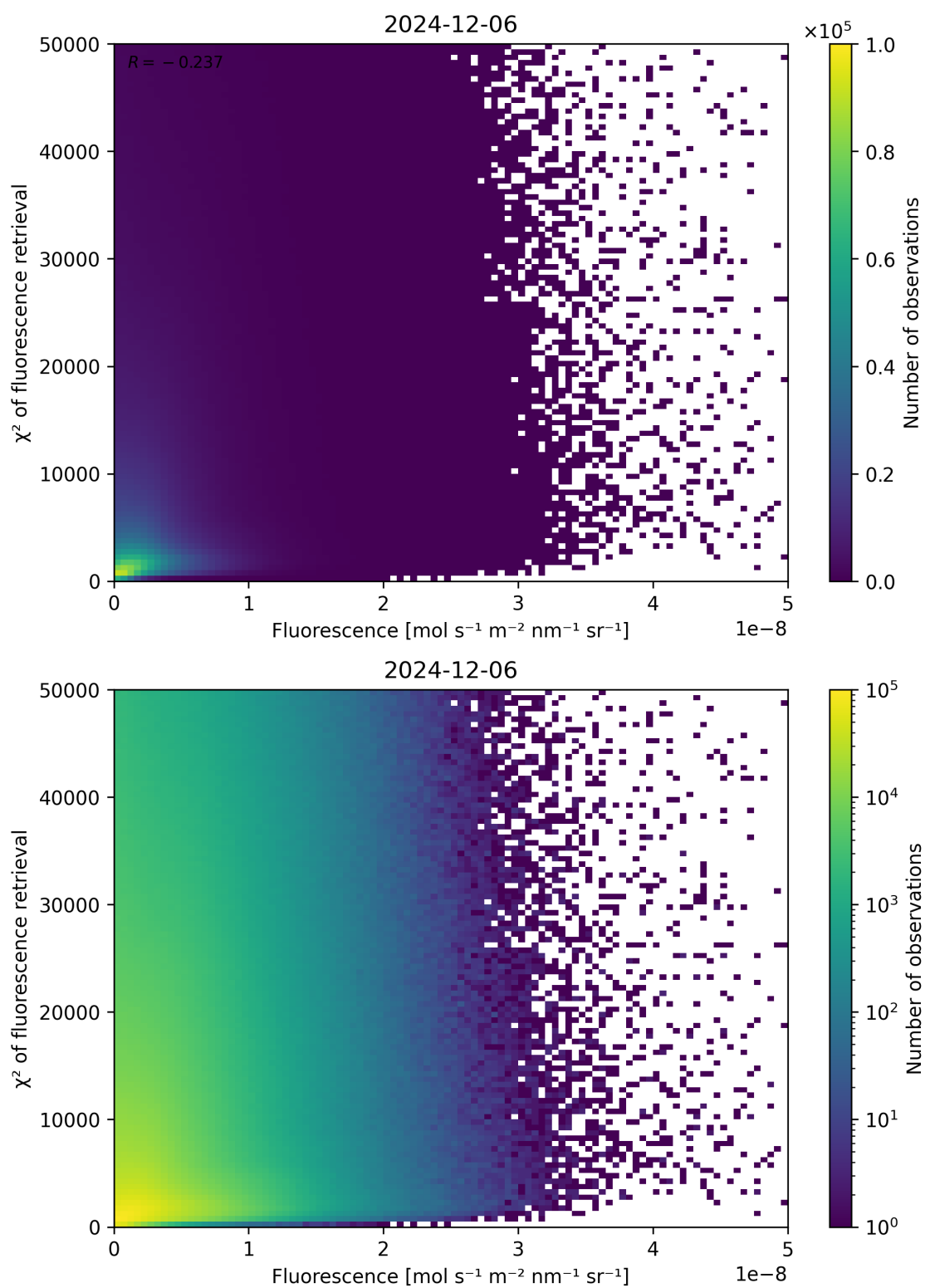
Figure 85: Scatter density plot of “Fluorescence” against “ \chi^2 of fluorescence retrieval” for 2024-12-06 to 2024-12-07.
