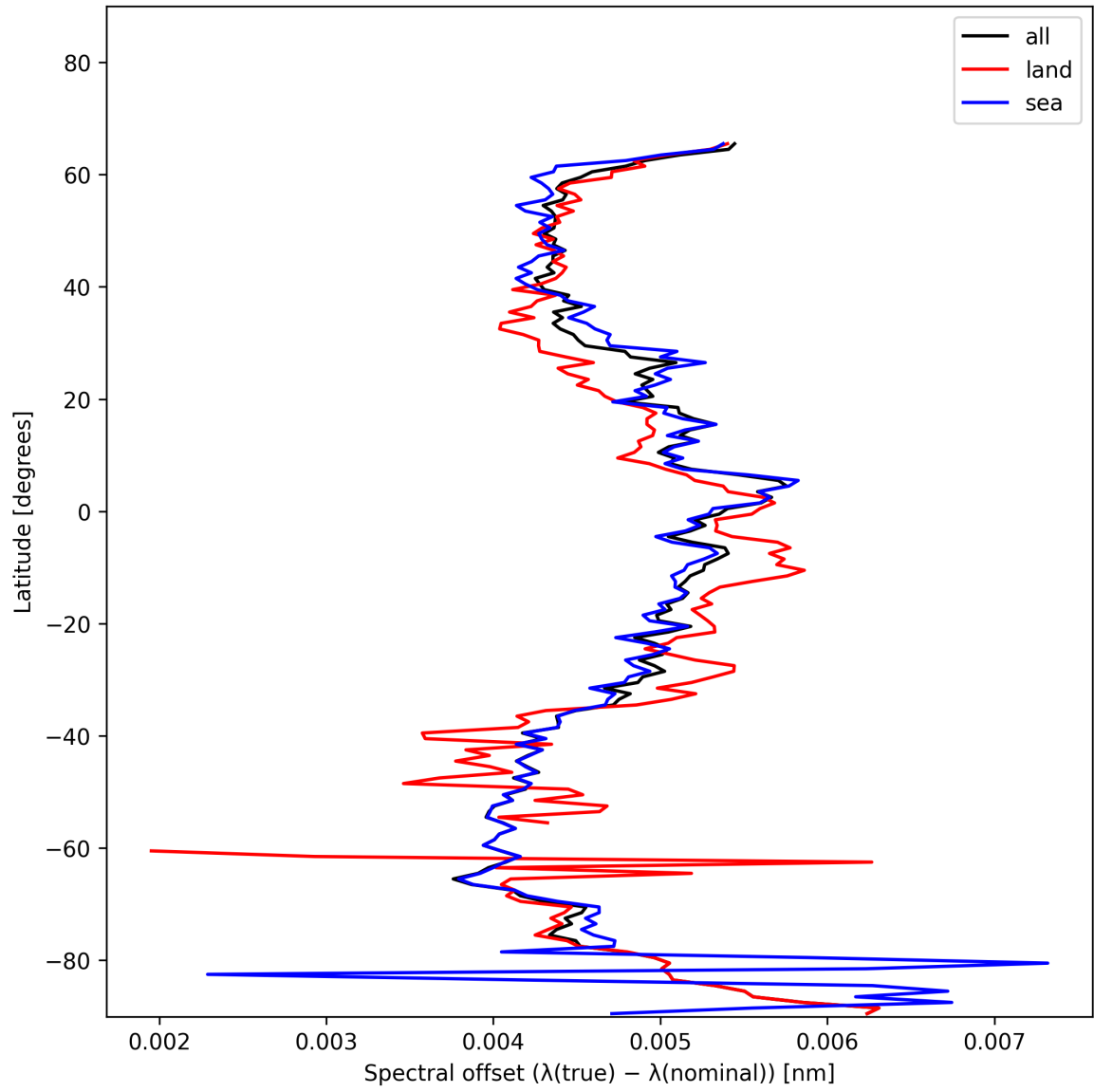
Figure 28: Zonal average of “Spectral offset ( \lambda_{\text{true}} - \lambda_{\text{nominal}} )” for 2024-12-06 to 2024-12-07.
