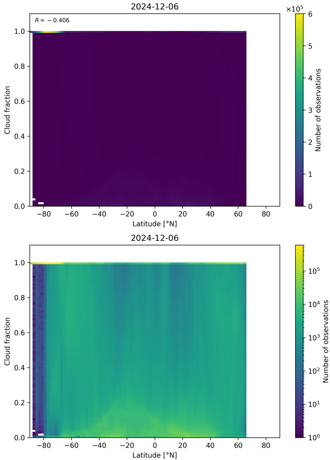
Figure 90: Scatter density plot of “Latitude” against “Cloud fraction” for 2024-12-06 to 2024-12-07.
