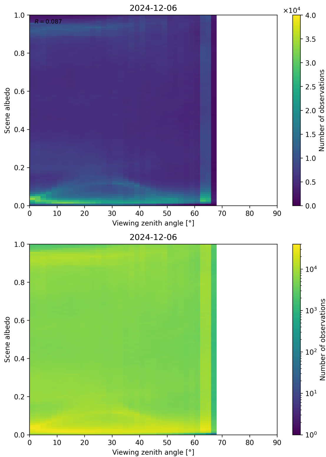
Figure 126: Scatter density plot of “Viewing zenith angle” against “Scene albedo” for 2024-12-06 to 2024-12-07.
