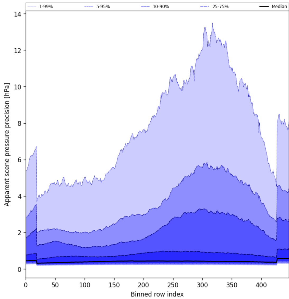
Figure 54: Along track statistics of “Apparent scene pressure precision” for 2024-12-06 to 2024-12-07
