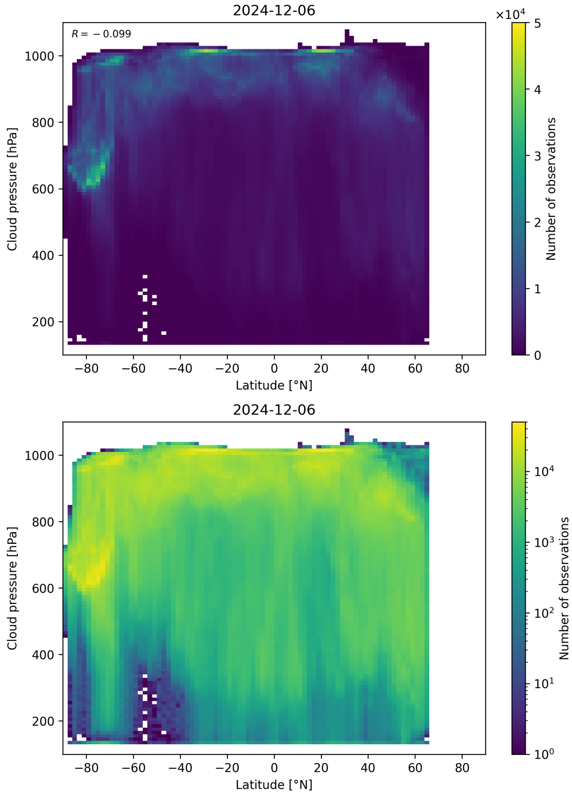
Figure 91: Scatter density plot of “Latitude” against “Cloud pressure” for 2024-12-06 to 2024-12-07.
