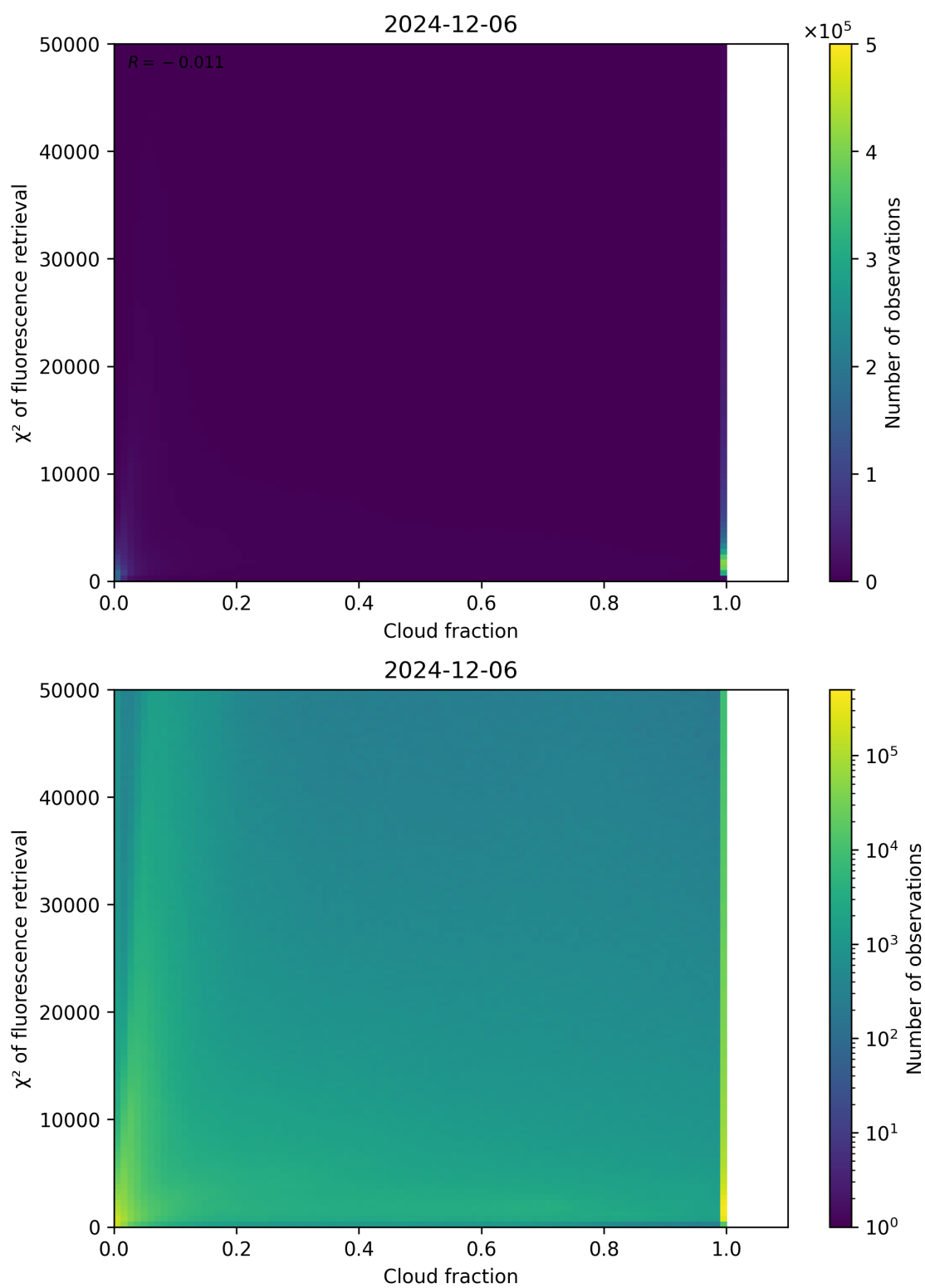
Figure 71: Scatter density plot of “Cloud fraction” against “ \chi^2 of fluorescence retrieval” for 2024-12-06 to 2024-12-07.
