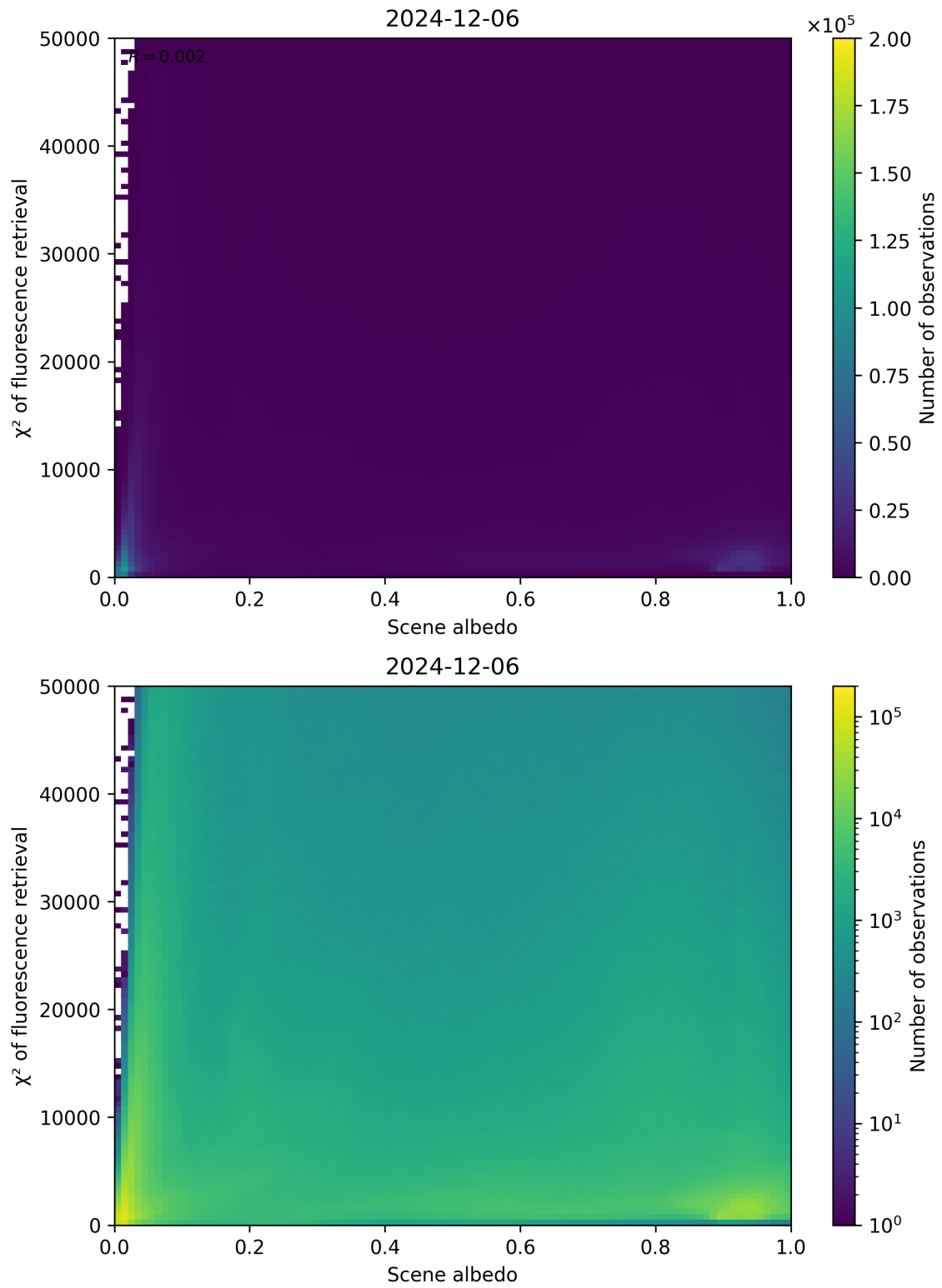
Figure 103: Scatter density plot of “Scene albedo” against “ \chi^2 of fluorescence retrieval” for 2024-12-06 to 2024-12-07.
