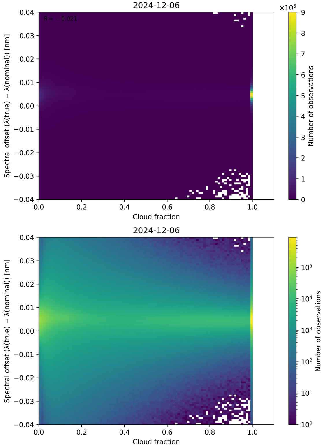
Figure 76: Scatter density plot of “Cloud fraction” against “Spectral offset ( \lambda_{\text{true}} - \lambda_{\text{nominal}} )” for 2024-12-06 to 2024-12-07.
