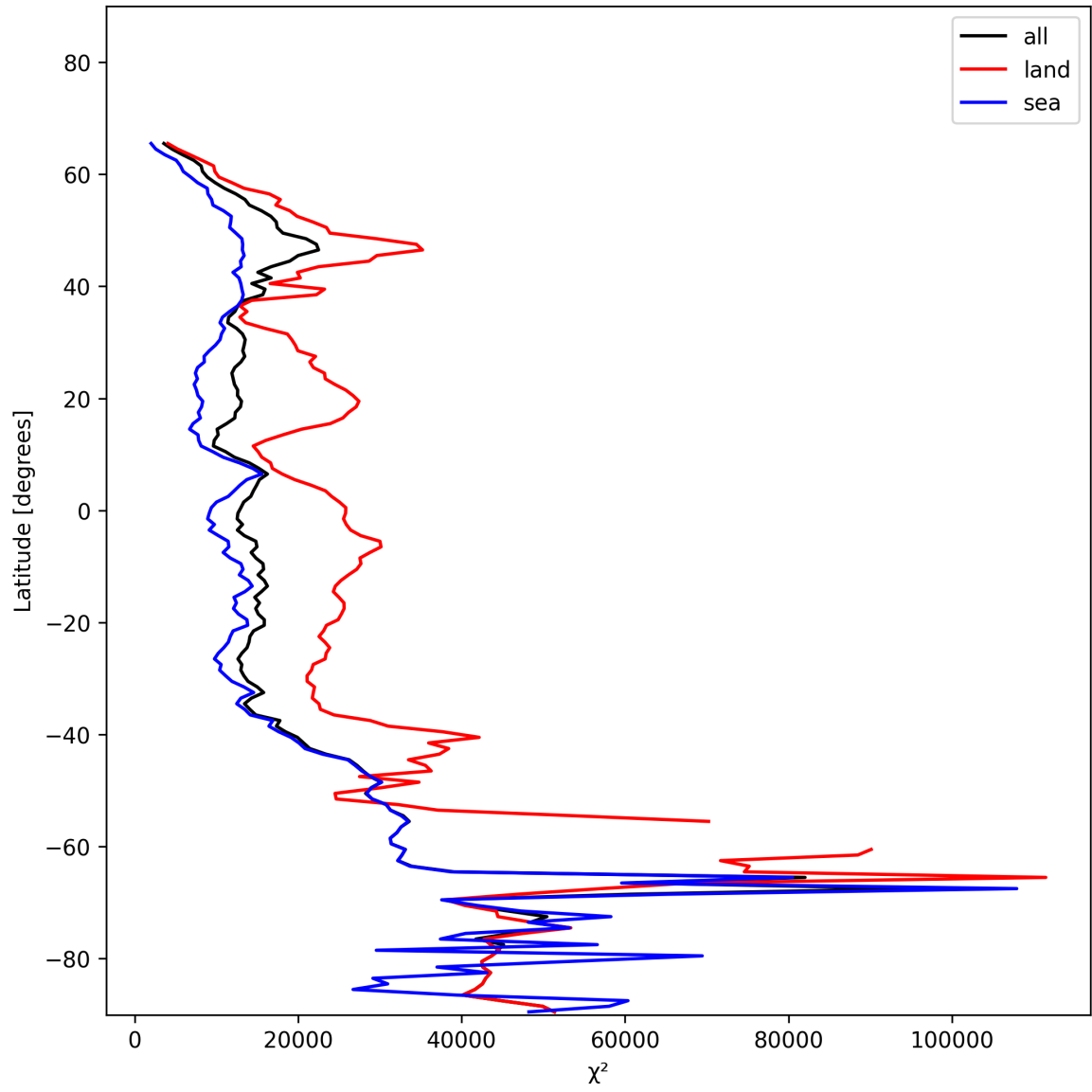
Figure 21: Zonal average of “ \chi^2 ” for 2024-12-06 to 2024-12-07.
