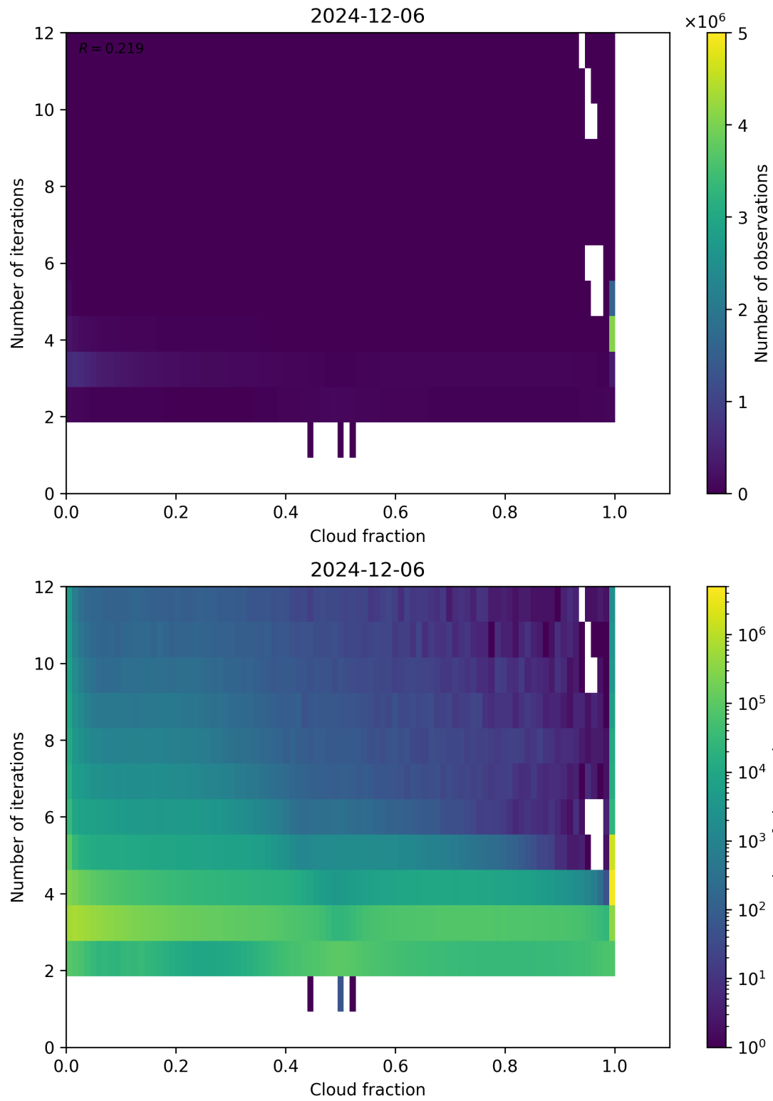
Figure 73: Scatter density plot of “Cloud fraction” against “Number of iterations” for 2024-12-06 to 2024-12-07.
