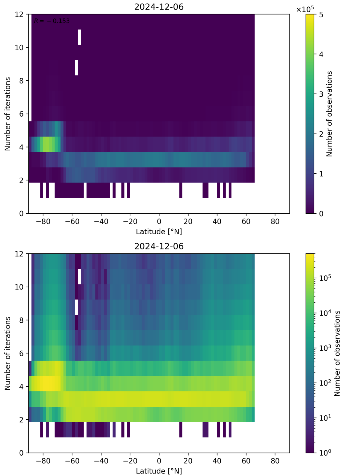
Figure 93: Scatter density plot of “Latitude” against “Number of iterations” for 2024-12-06 to 2024-12-07.
