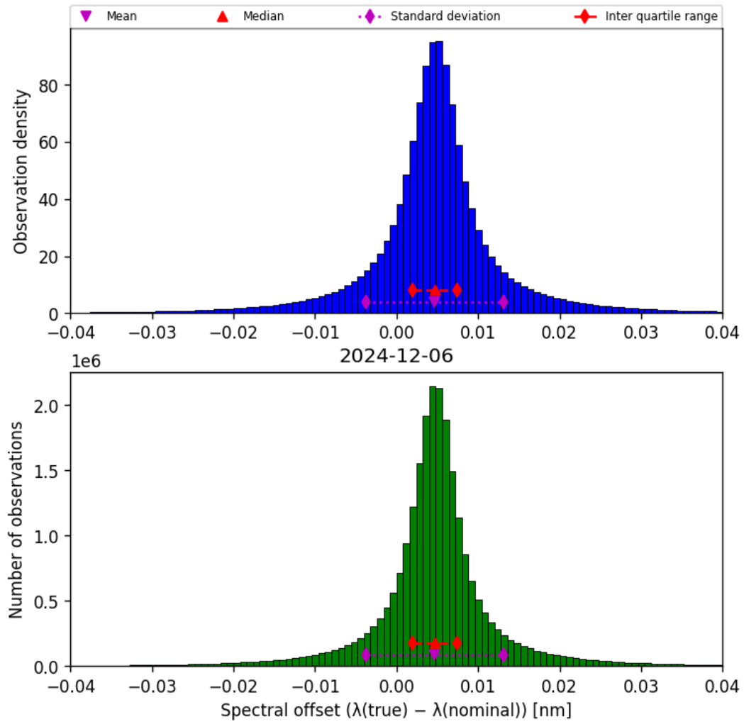
Figure 45: Histogram of “Spectral offset ( \lambda_{\text{true}} - \lambda_{\text{nominal}} )” for 2024-12-06 to 2024-12-07
