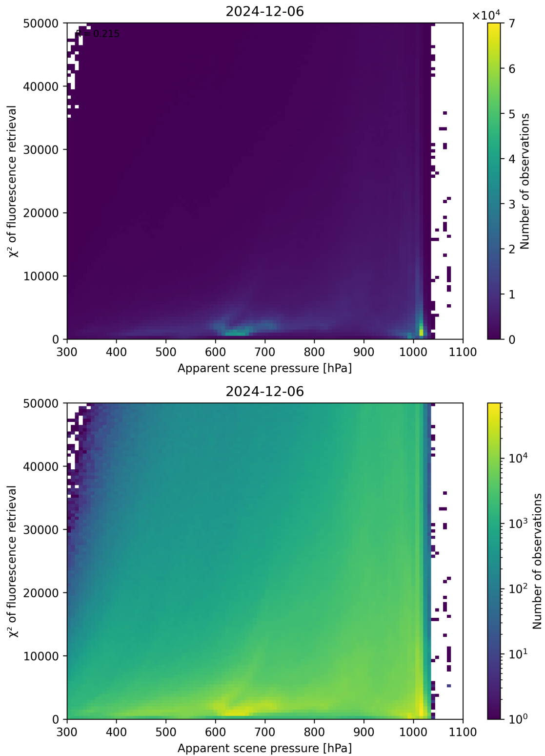
Figure 63: Scatter density plot of “Apparent scene pressure” against “ \chi^2 of fluorescence retrieval” for 2024-12-06 to 2024-12-07.
