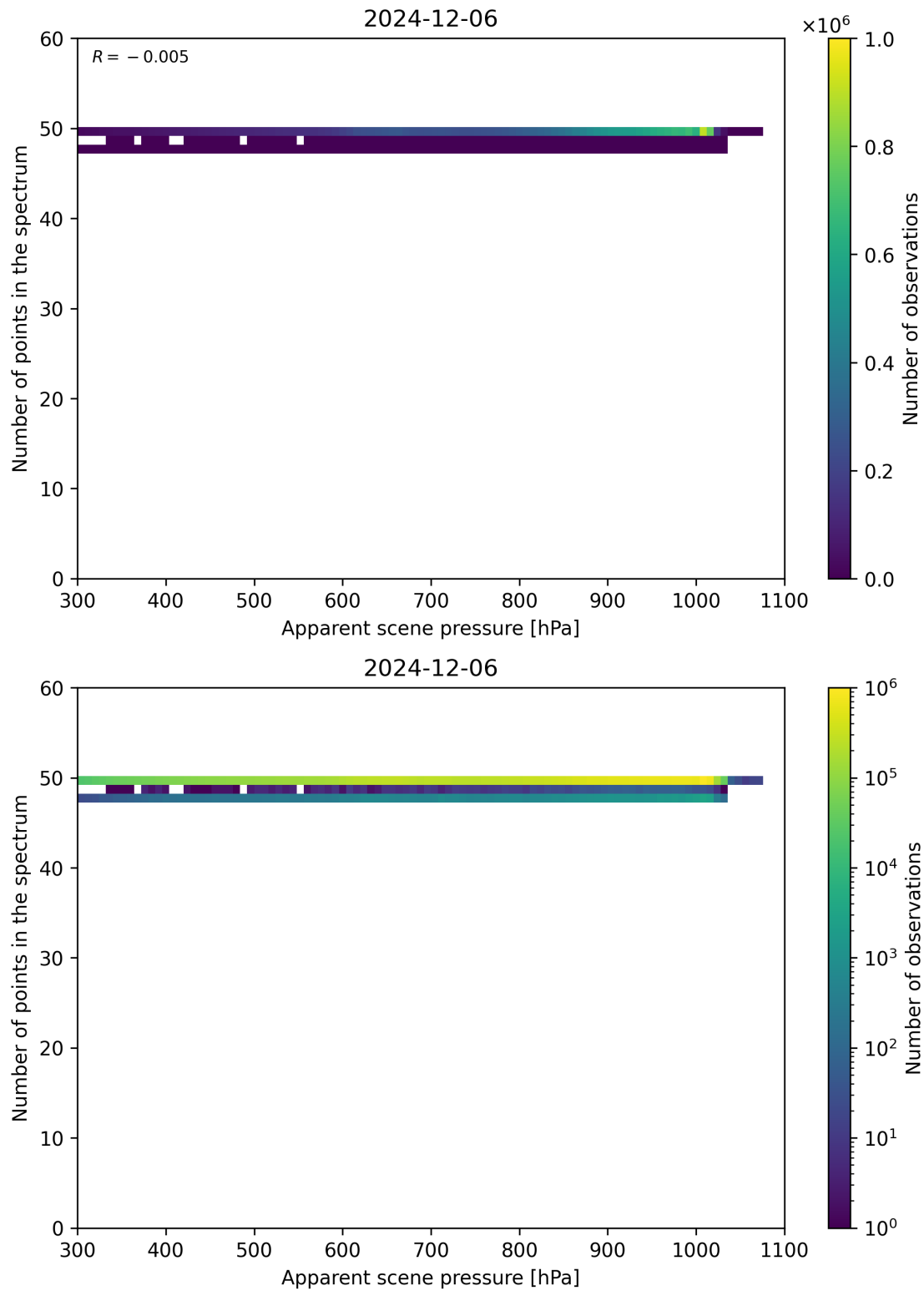
Figure 66: Scatter density plot of “Apparent scene pressure” against “Number of points in the spectrum” for 2024-12-06 to 2024-12-07.
