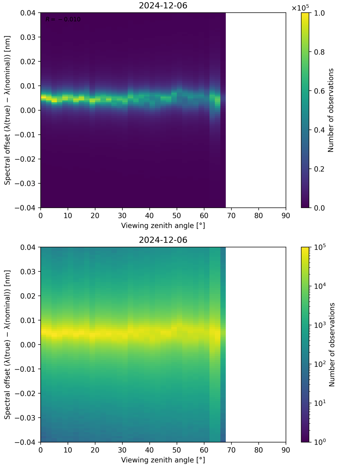
Figure 128: Scatter density plot of “Viewing zenith angle” against “Spectral offset ( \lambda_{\text{true}} - \lambda_{\text{nominal}} )” for 2024-12-06 to 2024-12-07.
