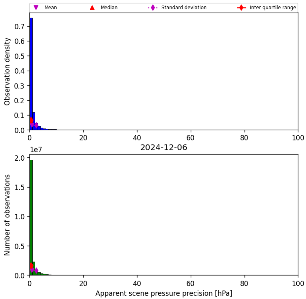
Figure 37: Histogram of “Apparent scene pressure precision” for 2024-12-06 to 2024-12-07
