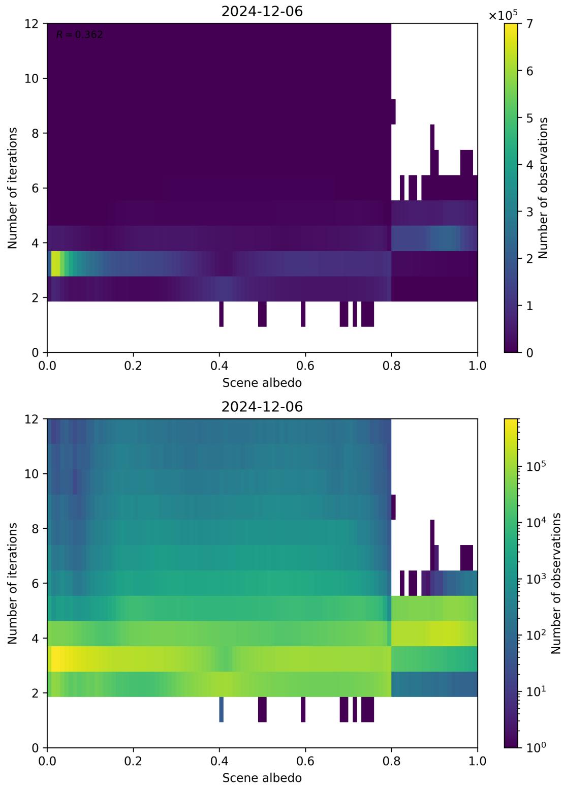
Figure 105: Scatter density plot of “Scene albedo” against “Number of iterations” for 2024-12-06 to 2024-12-07.
