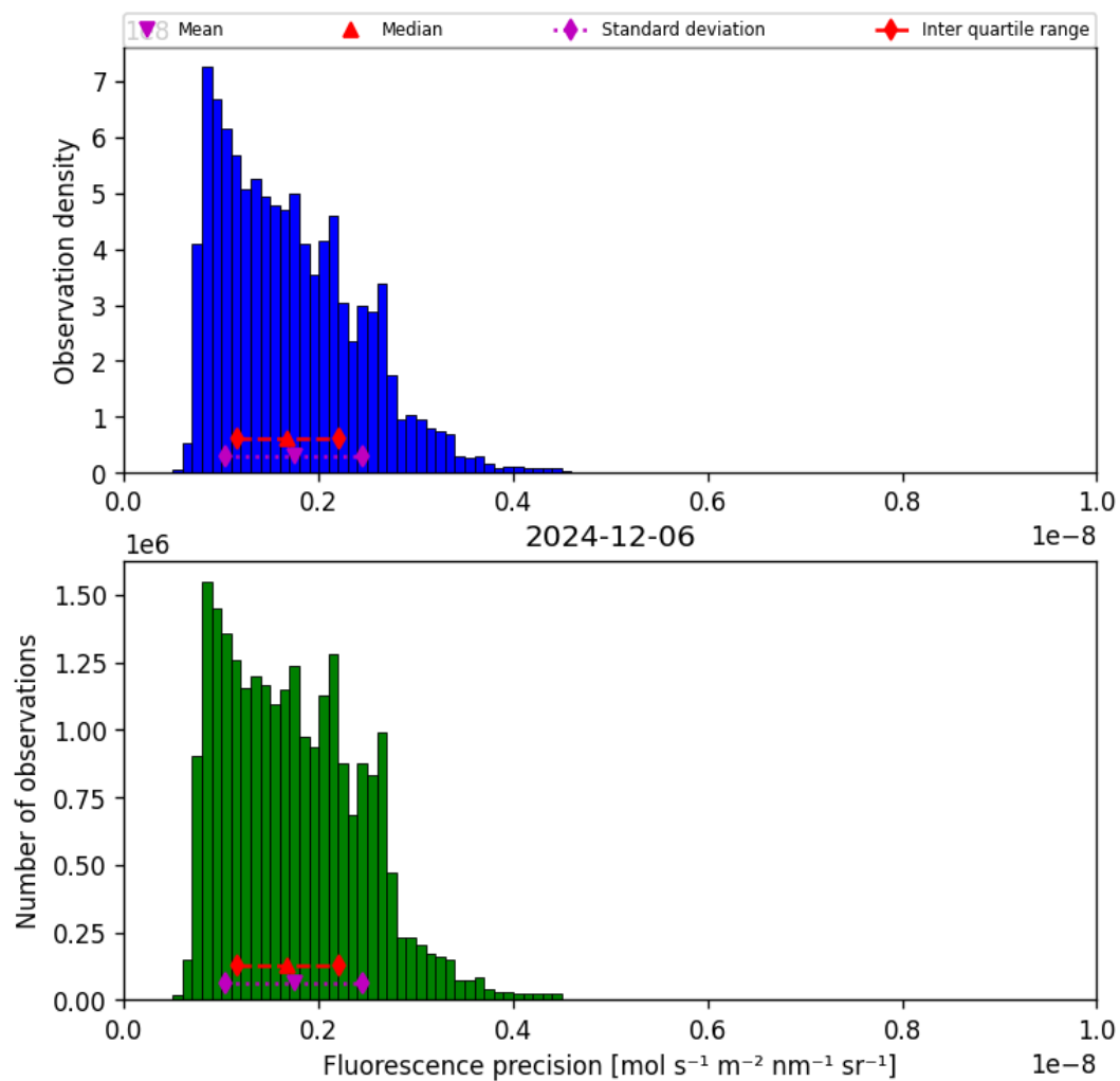
Figure 41: Histogram of “Fluorescence precision” for 2024-12-06 to 2024-12-07
