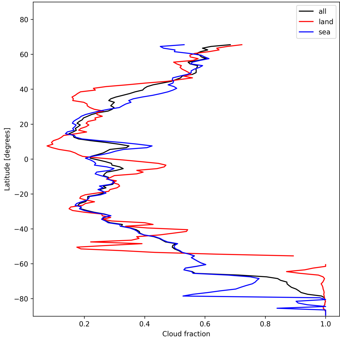
Figure 15: Zonal average of “Cloud fraction” for 2024-12-06 to 2024-12-07.
