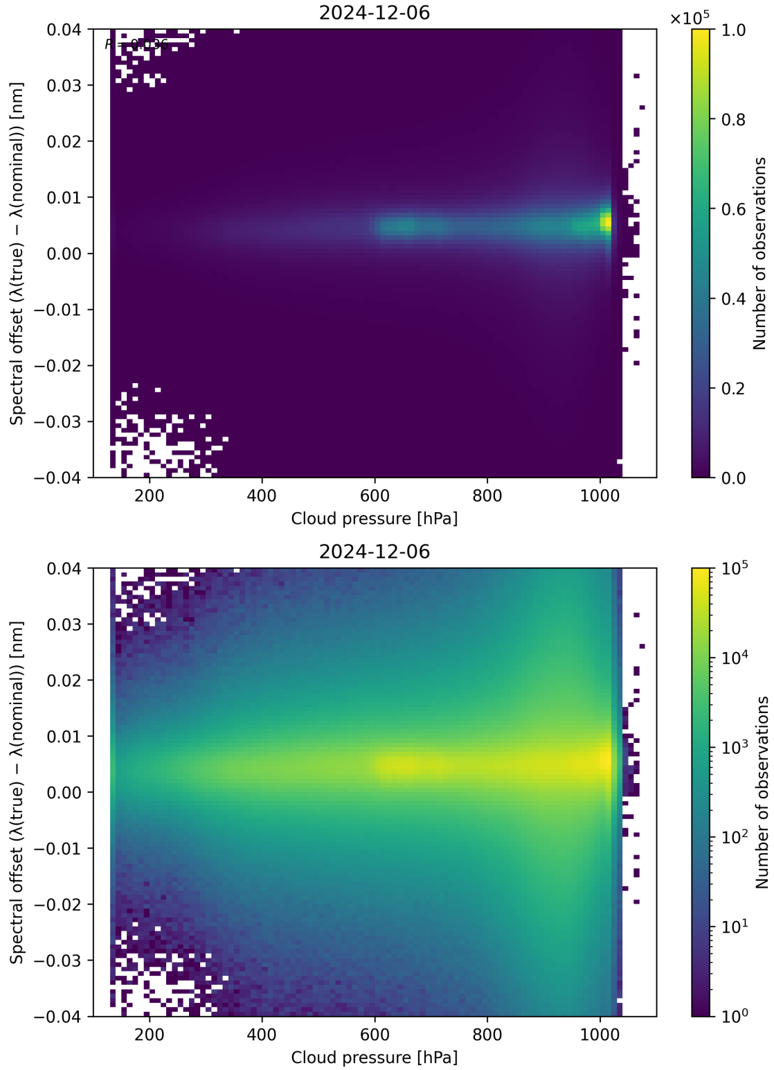
Figure 84: Scatter density plot of “Cloud pressure” against “Spectral offset ( \lambda_{\text{true}} - \lambda_{\text{nominal}} )” for 2024-12-06 to 2024-12-07.
