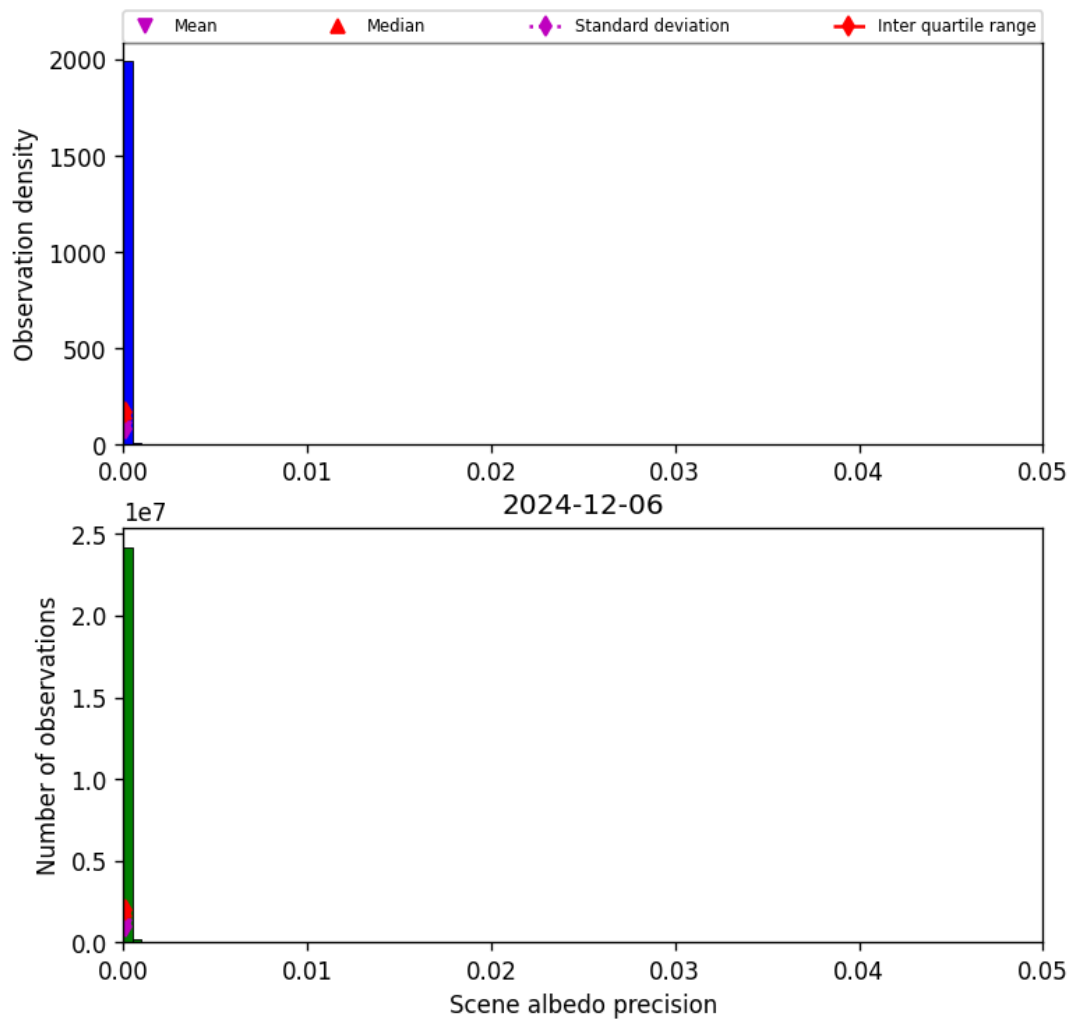
Figure 35: Histogram of “Scene albedo precision” for 2024-12-06 to 2024-12-07
