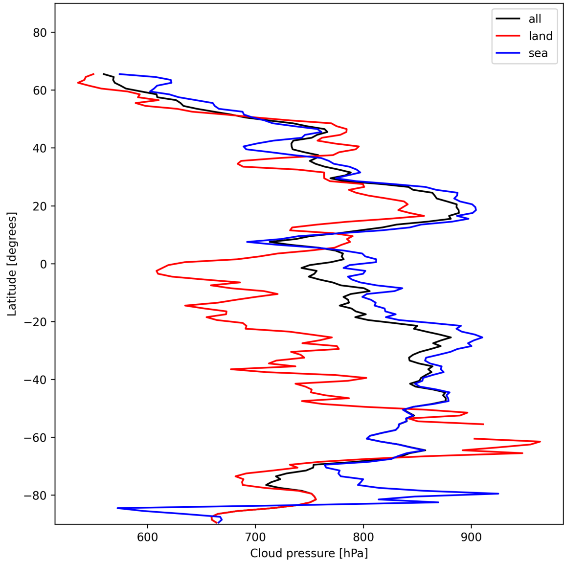
Figure 13: Zonal average of “Cloud pressure” for 2024-12-06 to 2024-12-07.
