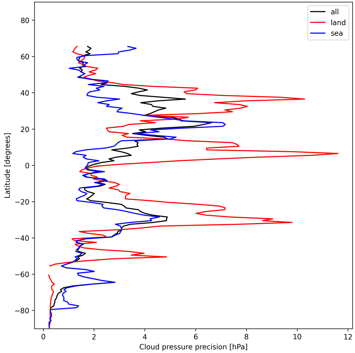
Figure 14: Zonal average of “Cloud pressure precision” for 2024-12-06 to 2024-12-07.
