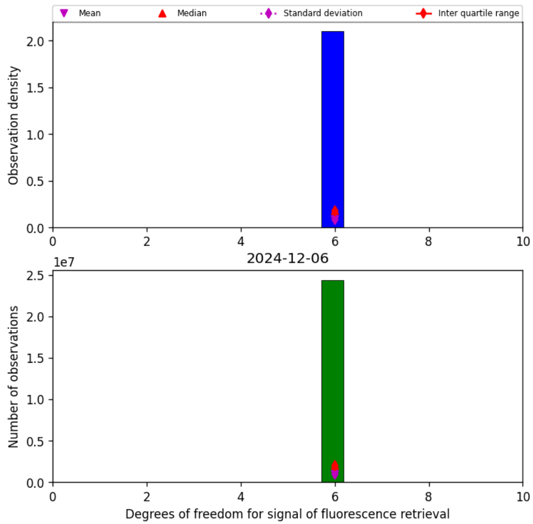
Figure 43: Histogram of “Degrees of freedom for signal of fluorescence retrieval” for 2024-12-06 to 2024-12-07
