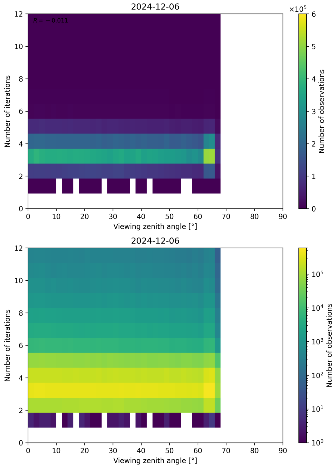
Figure 124: Scatter density plot of “Viewing zenith angle” against “Number of iterations” for 2024-12-06 to 2024-12-07.
