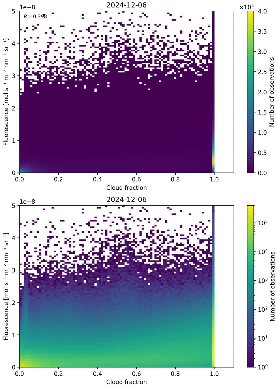
Figure 72: Scatter density plot of “Cloud fraction” against “Fluorescence” for 2024-12-06 to 2024-12-07.
