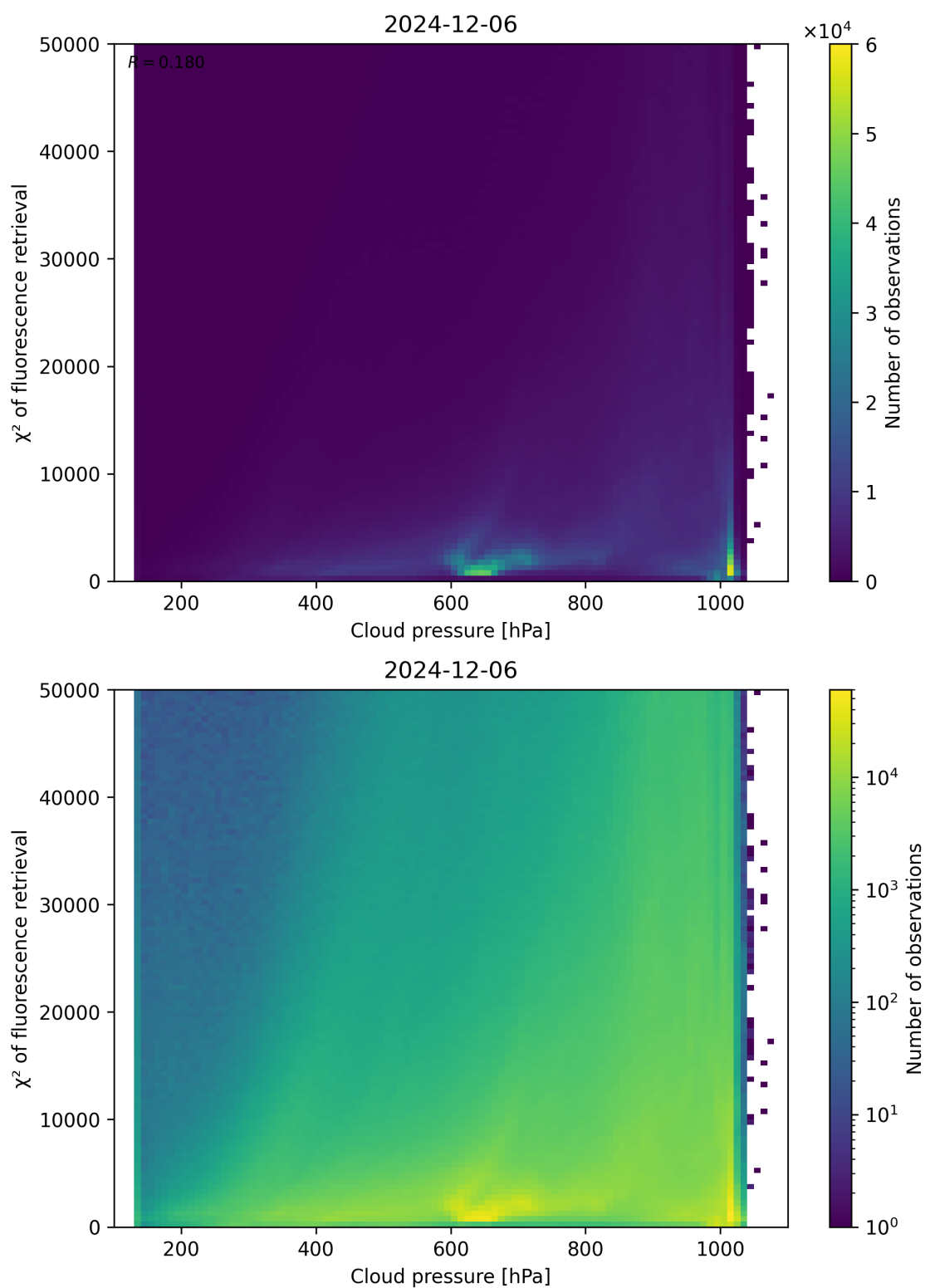
Figure 78: Scatter density plot of “Cloud pressure” against “ \chi^2 of fluorescence retrieval” for 2024-12-06 to 2024-12-07.
