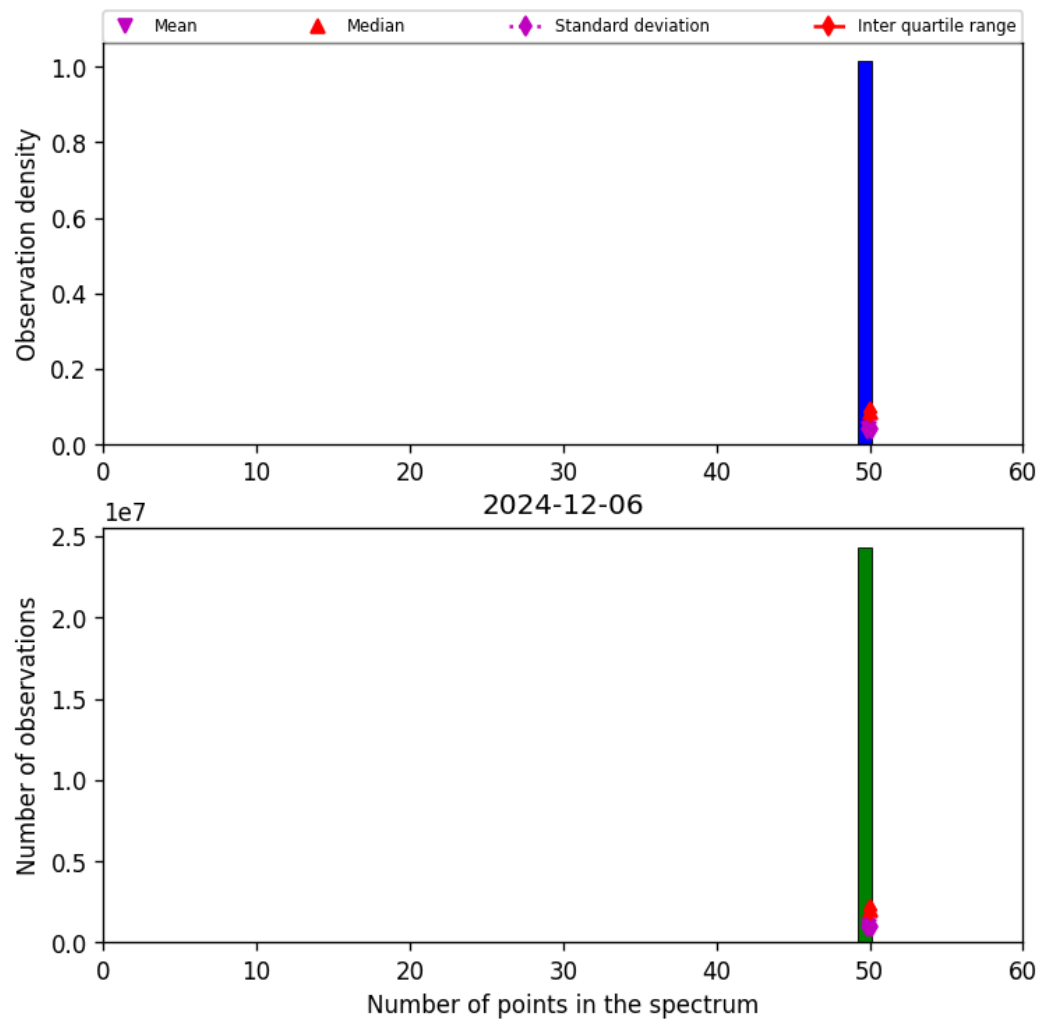
Figure 44: Histogram of “Number of points in the spectrum” for 2024-12-06 to 2024-12-07
