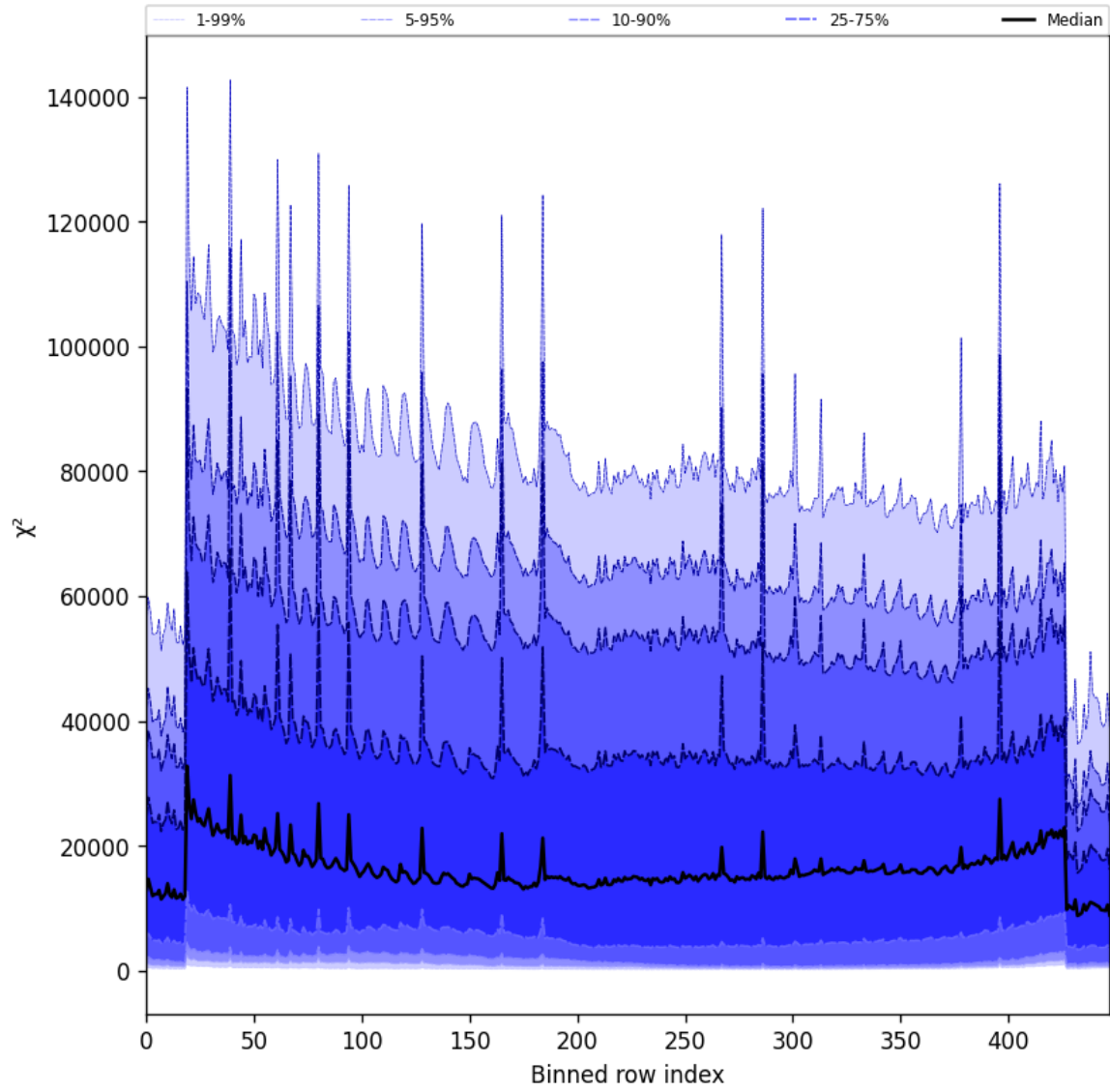
Figure 55: Along track statistics of “ \chi^2 ” for 2024-12-06 to 2024-12-07
