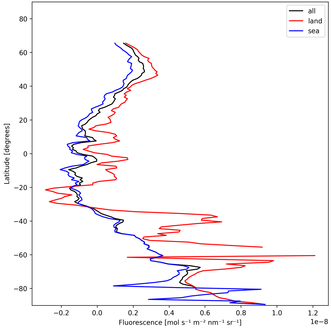
Figure 23: Zonal average of “Fluorescence” for 2024-12-06 to 2024-12-07.
