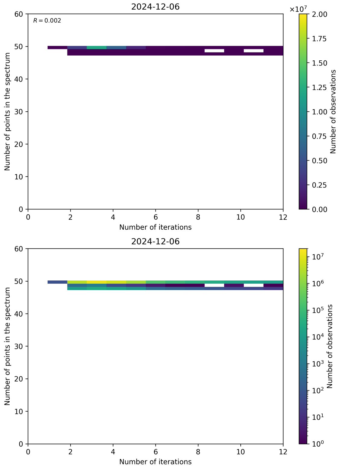
Figure 99: Scatter density plot of “Number of iterations” against “Number of points in the spectrum” for 2024-12-06 to 2024-12-07.
