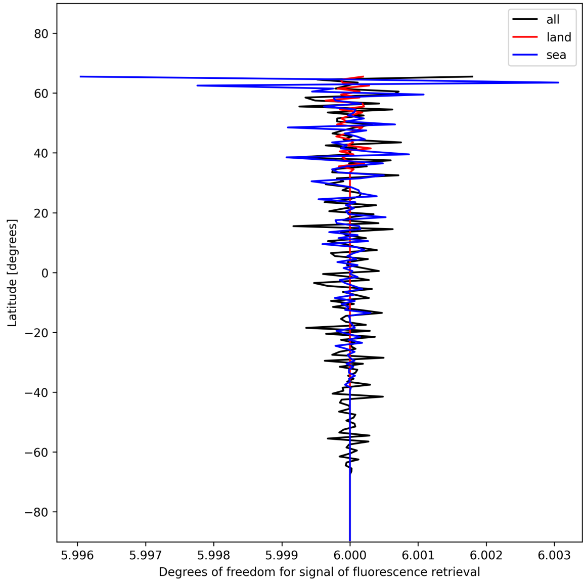
Figure 26: Zonal average of “Degrees of freedom for signal of fluorescence retrieval” for 2024-12-06 to 2024-12-07.
