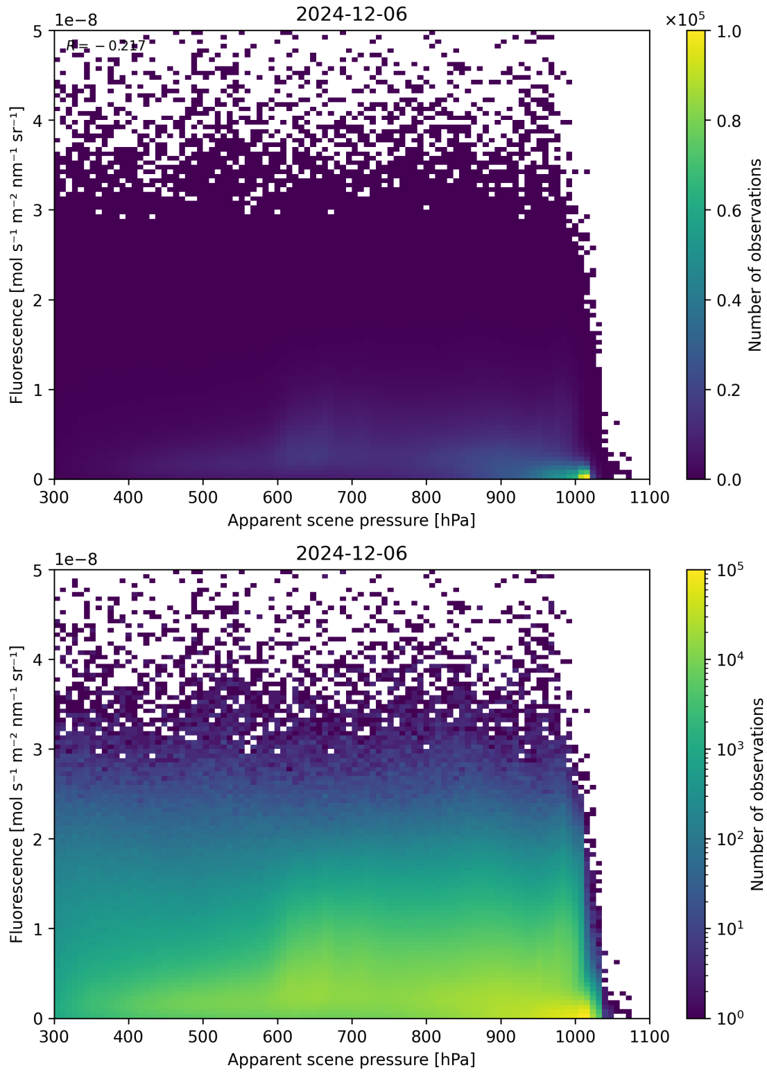
Figure 64: Scatter density plot of “Apparent scene pressure” against “Fluorescence” for 2024-12-06 to 2024-12-07.
