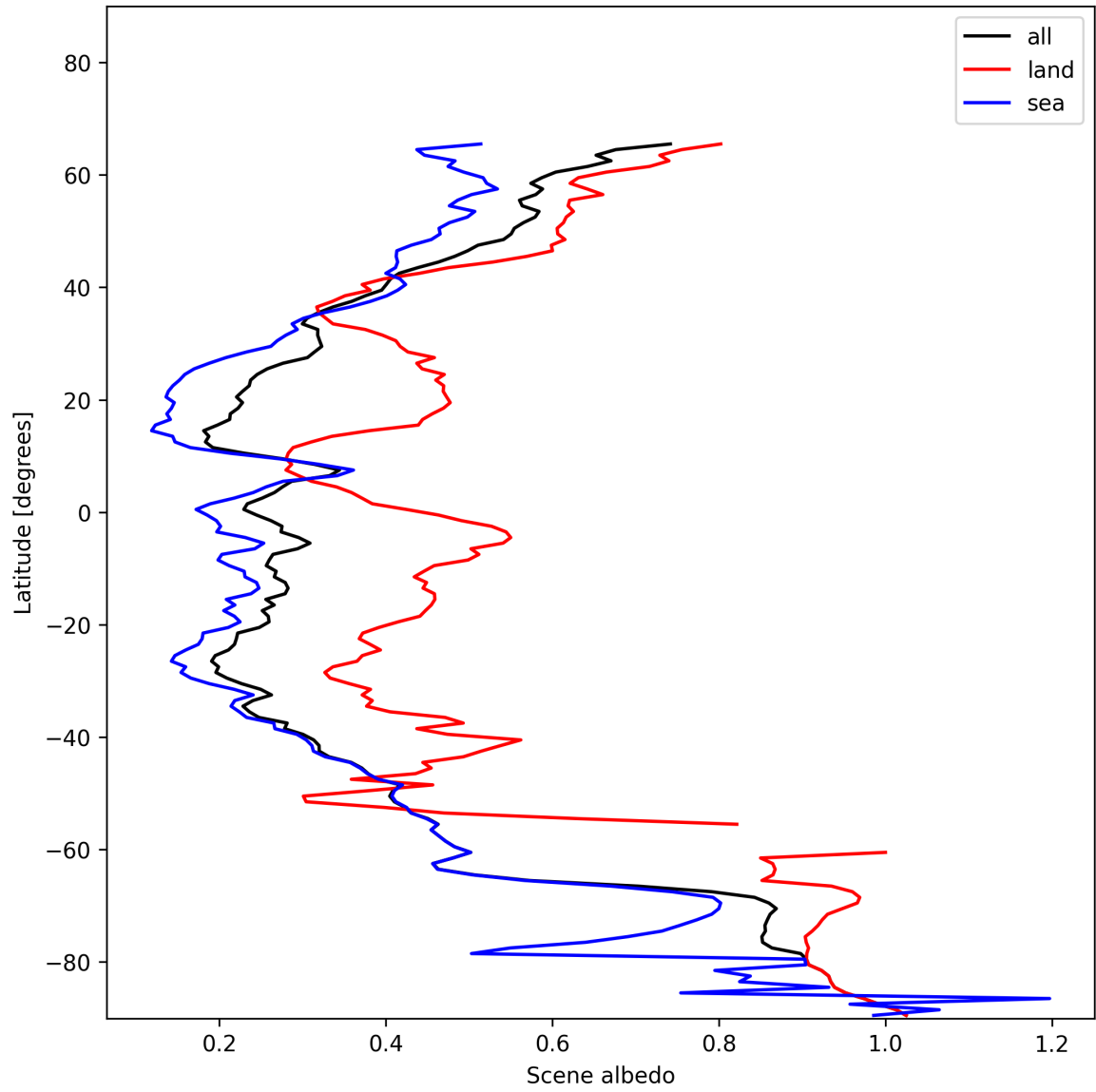
Figure 17: Zonal average of “Scene albedo” for 2024-12-06 to 2024-12-07.
