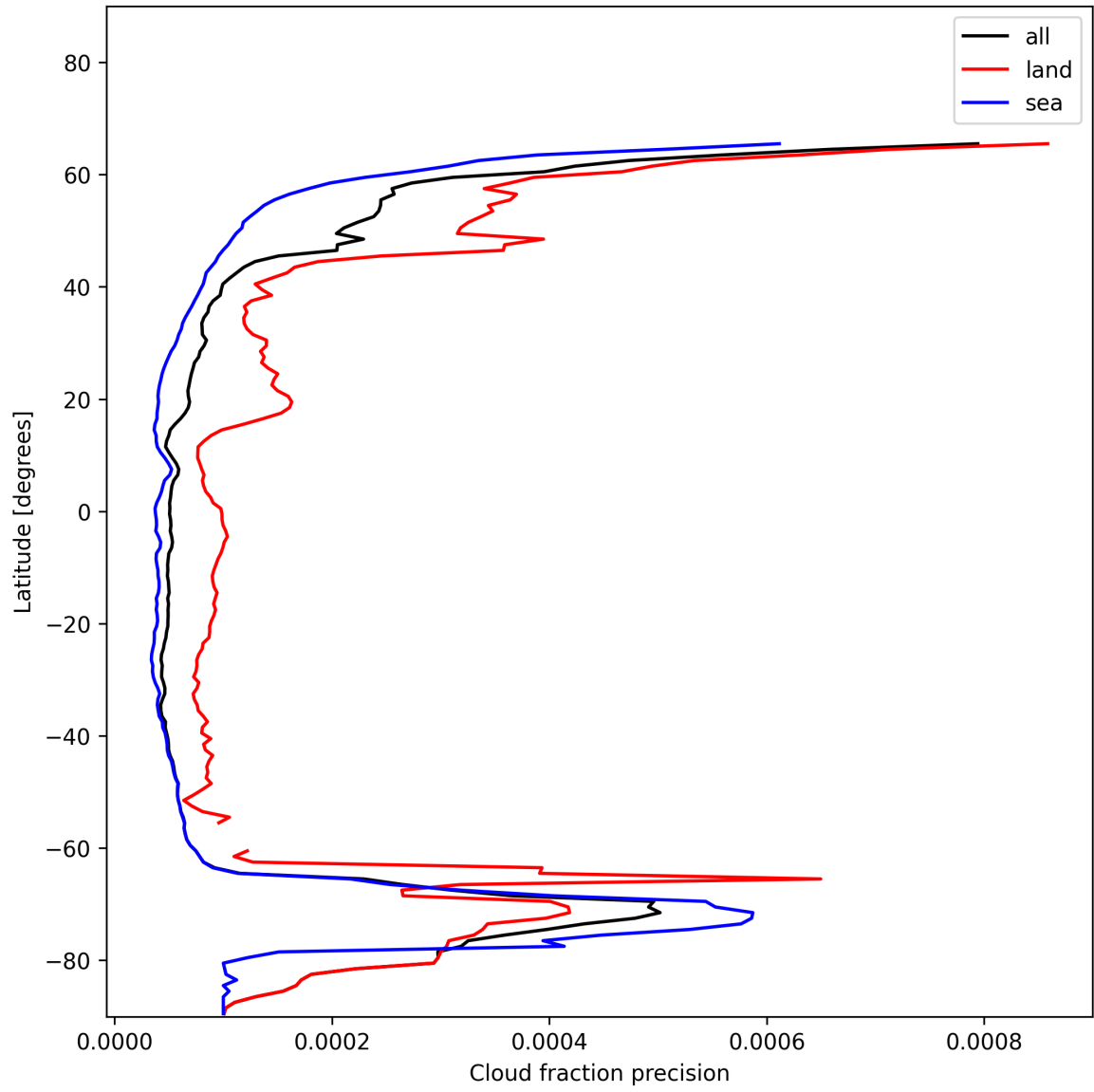
Figure 16: Zonal average of “Cloud fraction precision” for 2024-12-06 to 2024-12-07.
