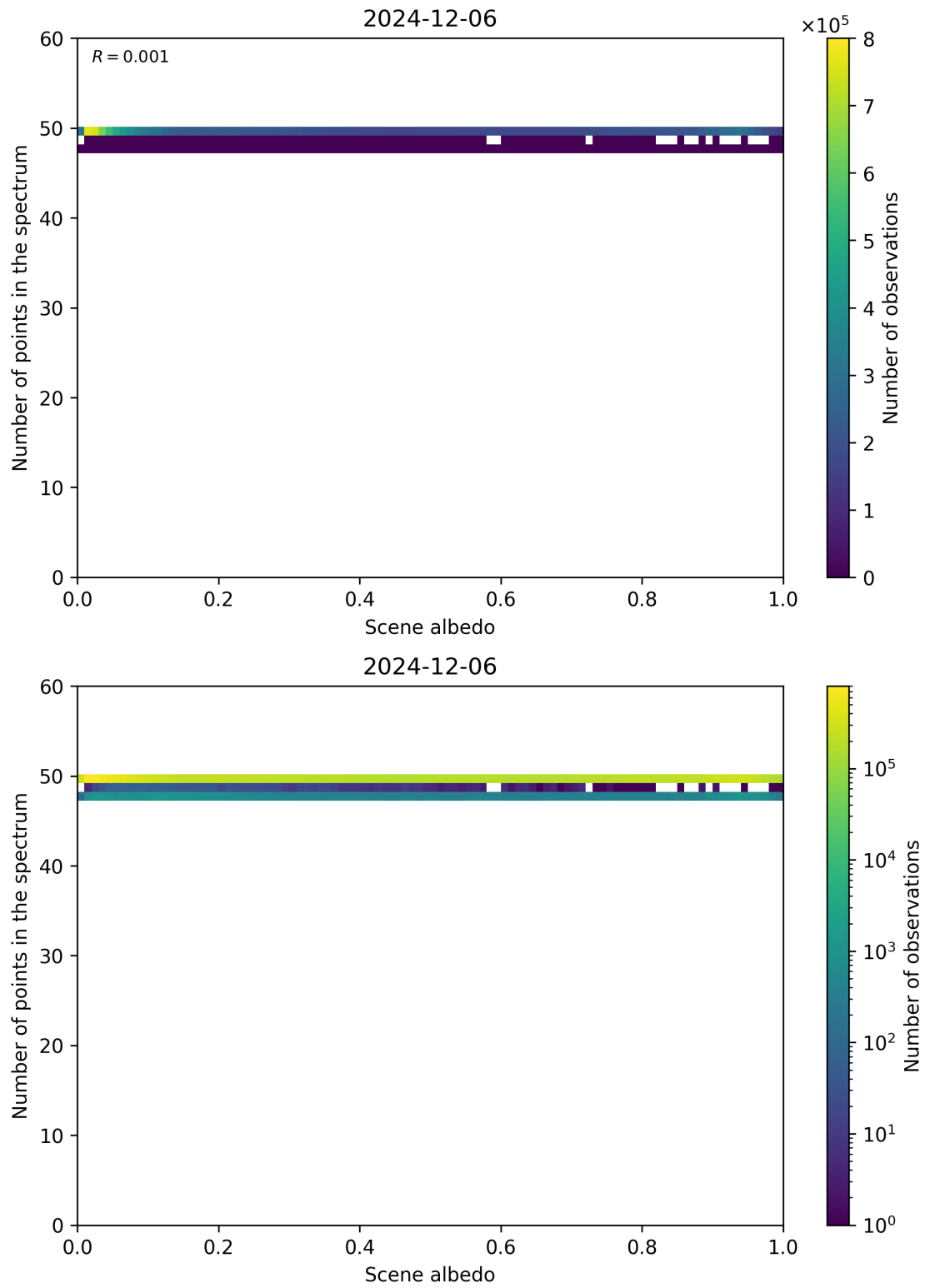
Figure 106: Scatter density plot of “Scene albedo” against “Number of points in the spectrum” for 2024-12-06 to 2024-12-07.
