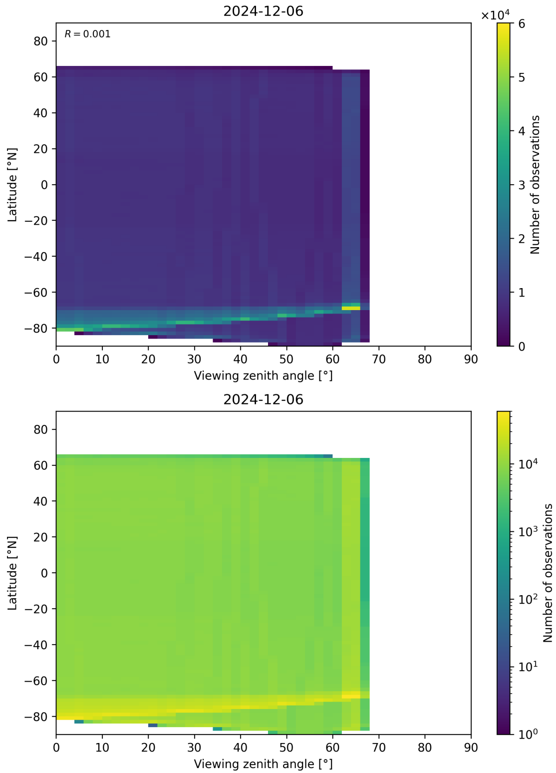
Figure 123: Scatter density plot of “Viewing zenith angle” against “Latitude” for 2024-12-06 to 2024-12-07.
