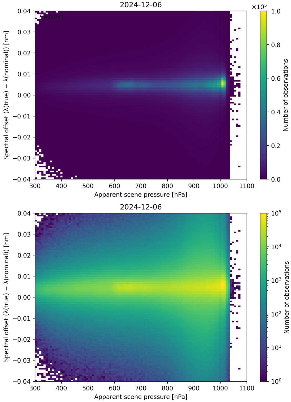
Figure 67: Scatter density plot of “Apparent scene pressure” against “Spectral offset ( \lambda_{\text{true}} - \lambda_{\text{nominal}} )” for 2024-12-06 to 2024-12-07.
