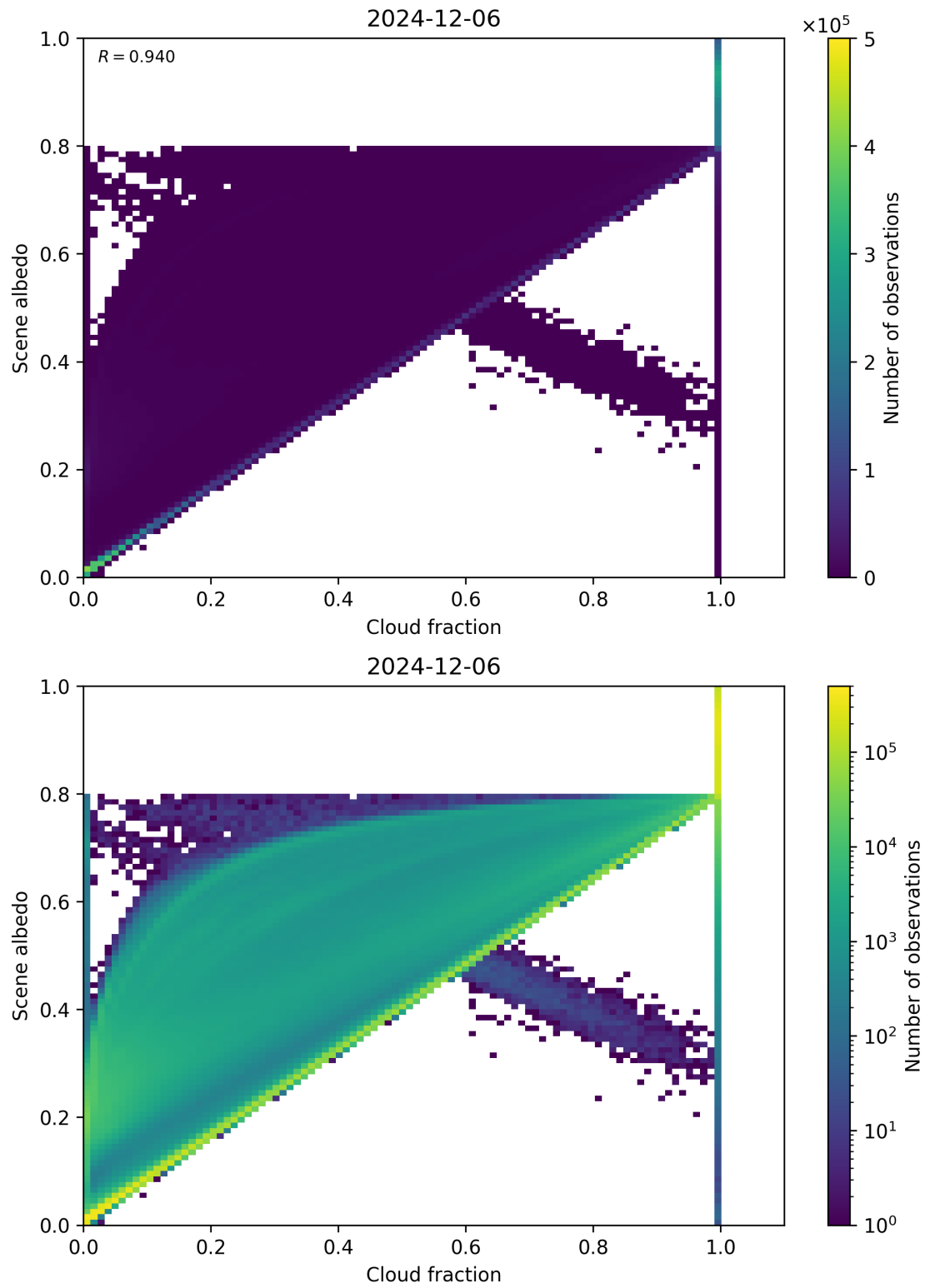
Figure 75: Scatter density plot of “Cloud fraction” against “Scene albedo” for 2024-12-06 to 2024-12-07.
