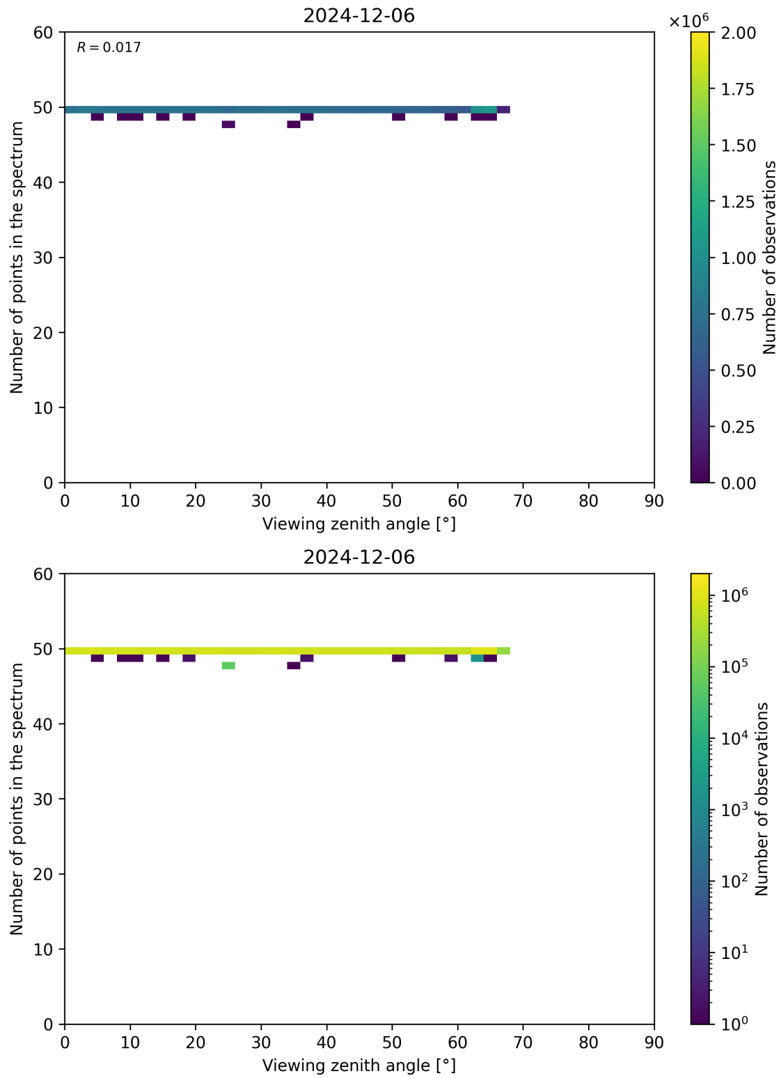
Figure 125: Scatter density plot of “Viewing zenith angle” against “Number of points in the spectrum” for 2024-12-06 to 2024-12-07.
