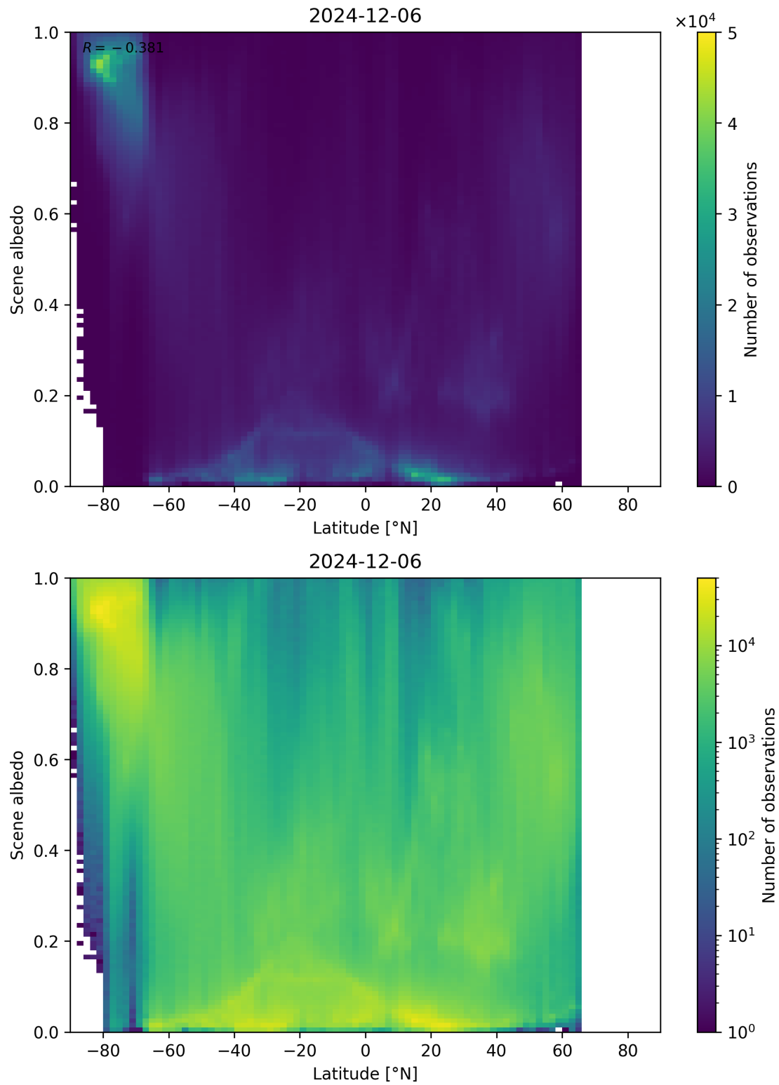
Figure 95: Scatter density plot of “Latitude” against “Scene albedo” for 2024-12-06 to 2024-12-07.
