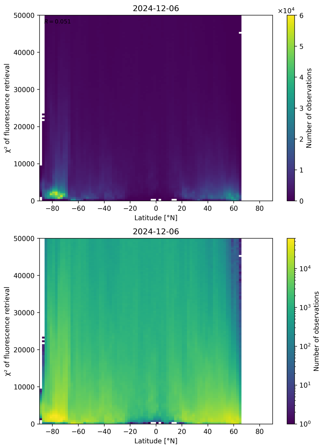
Figure 89: Scatter density plot of “Latitude” against “ \chi^2 of fluorescence retrieval” for 2024-12-06 to 2024-12-07.
