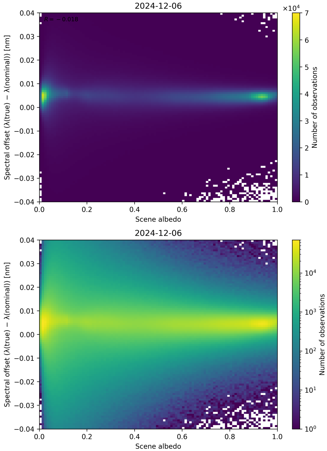
Figure 107: Scatter density plot of “Scene albedo” against “Spectral offset ( \lambda_{\text{true}} - \lambda_{\text{nominal}} )” for 2024-12-06 to 2024-12-07.
