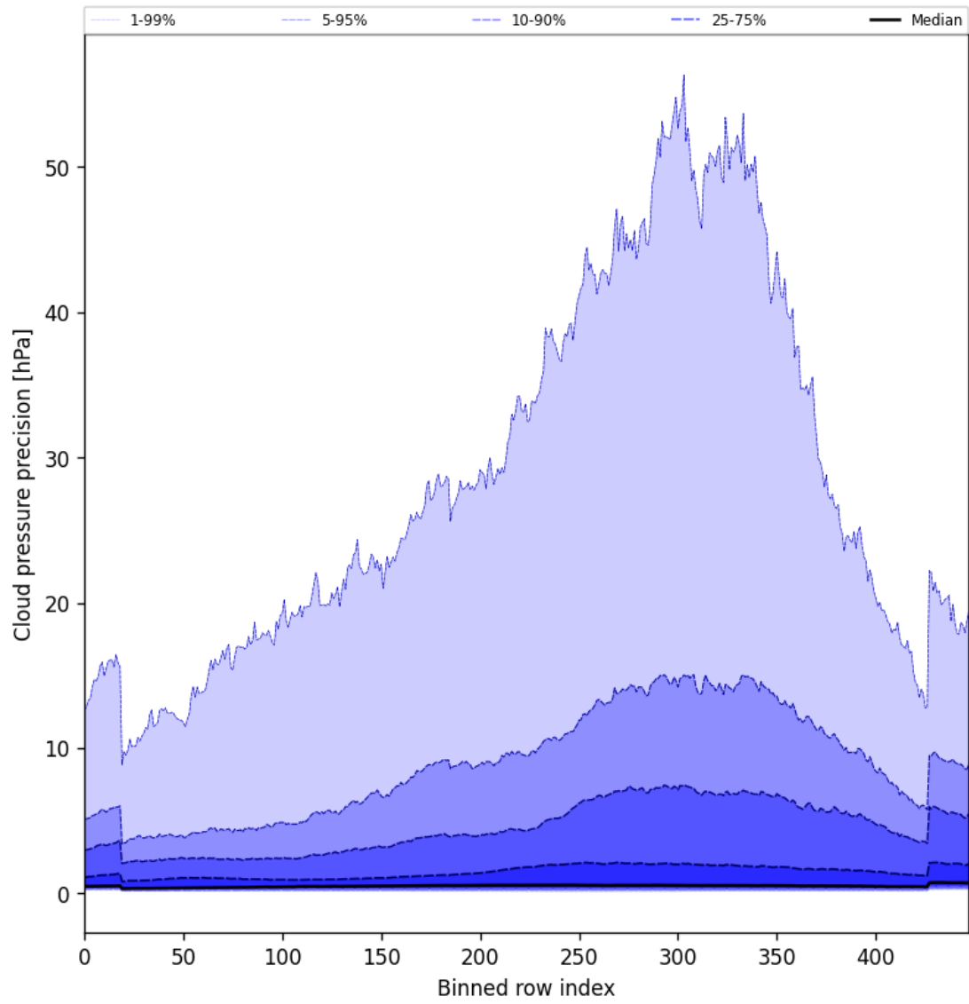
Figure 48: Along track statistics of “Cloud pressure precision” for 2024-12-06 to 2024-12-07
