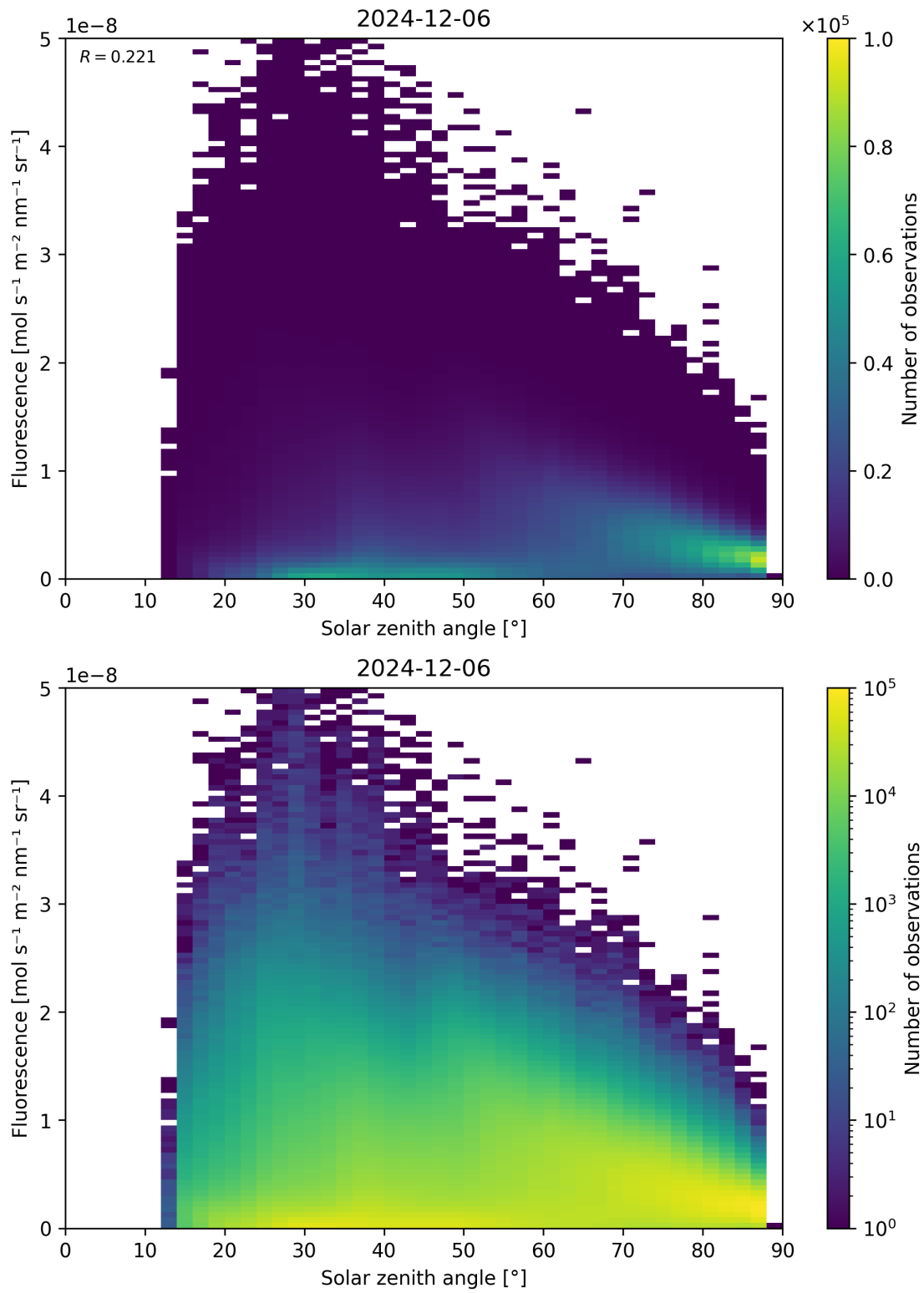
Figure 112: Scatter density plot of “Solar zenith angle” against “Fluorescence” for 2024-12-06 to 2024-12-07.
