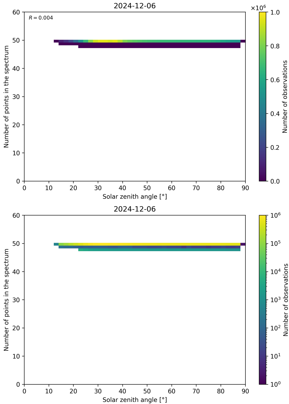
Figure 115: Scatter density plot of “Solar zenith angle” against “Number of points in the spectrum” for 2024-12-06 to 2024-12-07.
