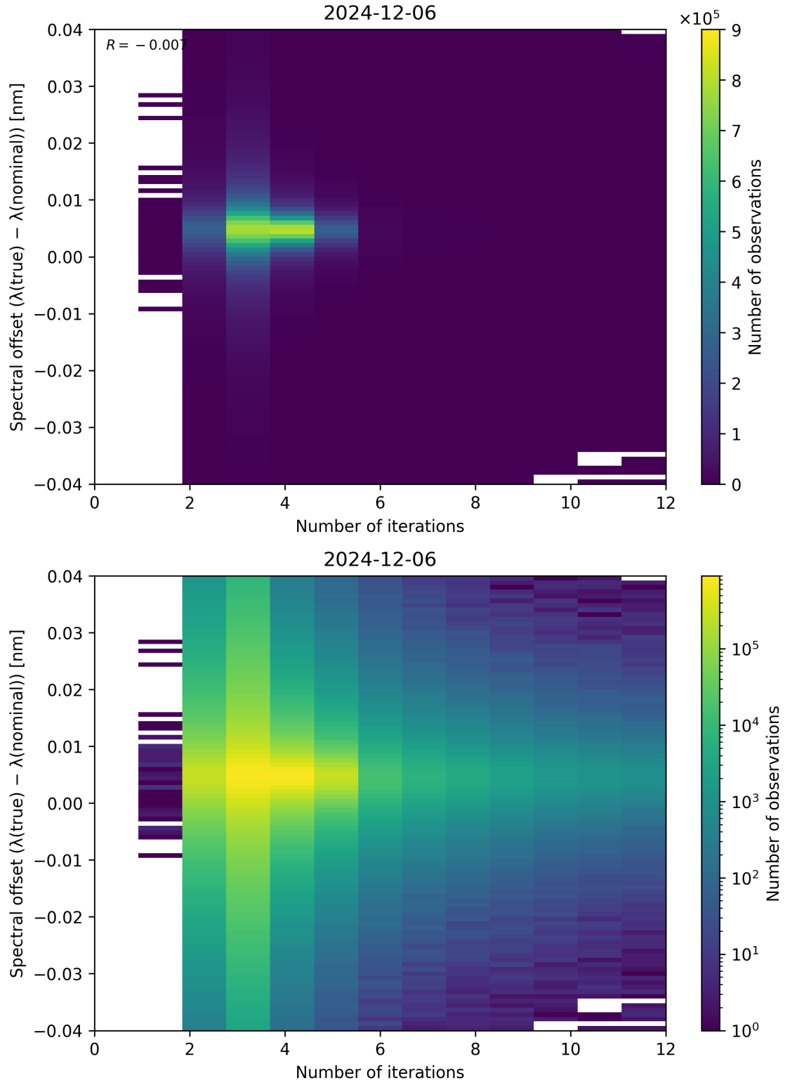
Figure 100: Scatter density plot of “Number of iterations” against “Spectral offset ( \lambda_{\text{true}} - \lambda_{\text{nominal}} )” for 2024-12-06 to 2024-12-07.
