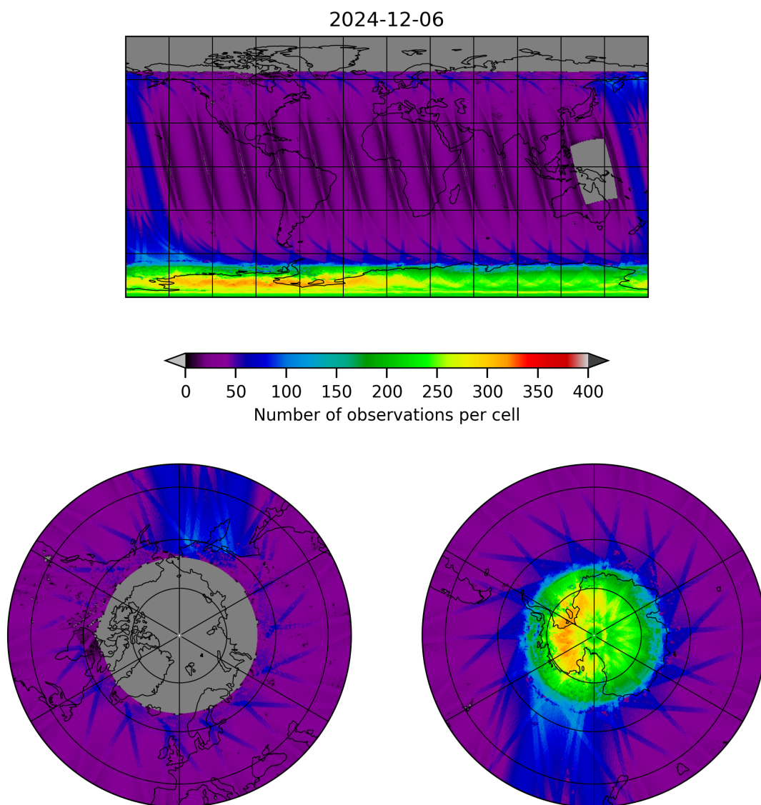
Figure 11: Map of the number of observations for 2024-12-06 to 2024-12-07
