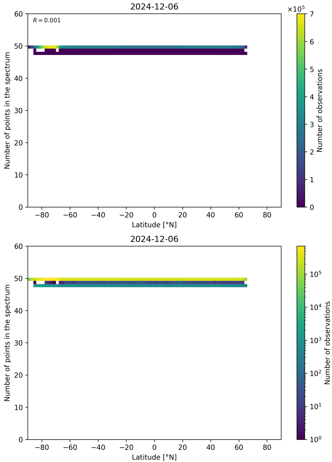
Figure 94: Scatter density plot of “Latitude” against “Number of points in the spectrum” for 2024-12-06 to 2024-12-07.
