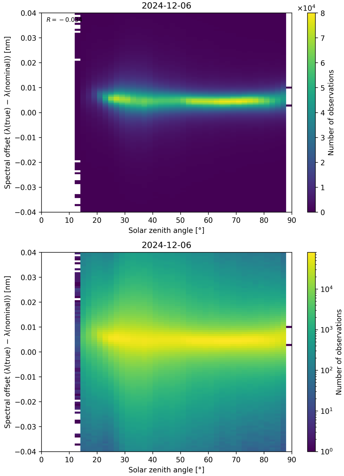
Figure 117: Scatter density plot of “Solar zenith angle” against “Spectral offset ( \lambda_{\text{true}} - \lambda_{\text{nominal}} )” for 2024-12-06 to 2024-12-07.
