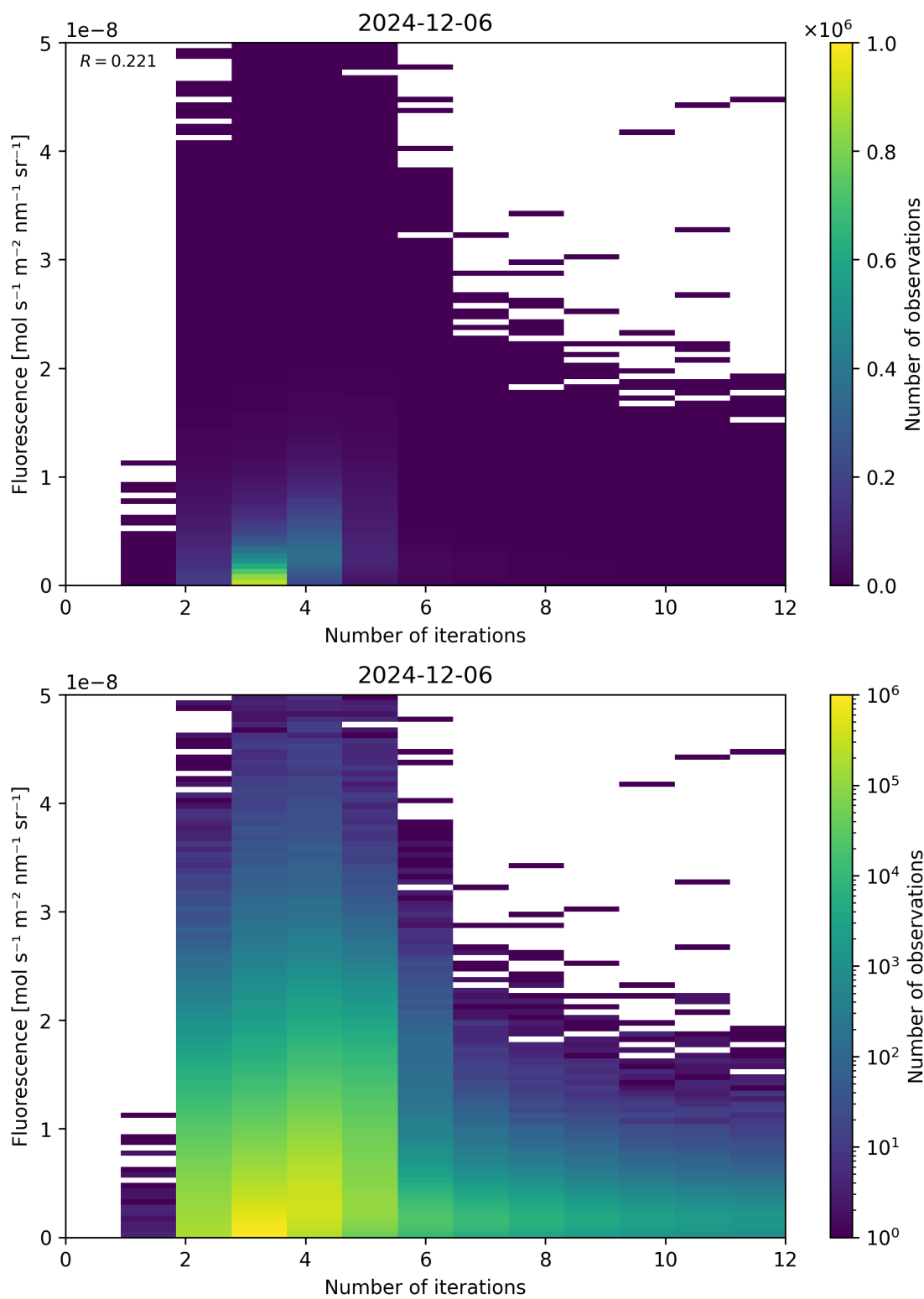
Figure 98: Scatter density plot of "Number of iterations" against "Fluorescence" for 2024-12-06 to 2024-12-07.
