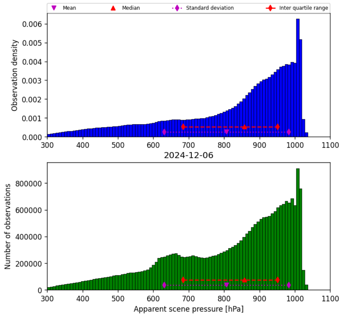
Figure 36: Histogram of “Apparent scene pressure” for 2024-12-06 to 2024-12-07
