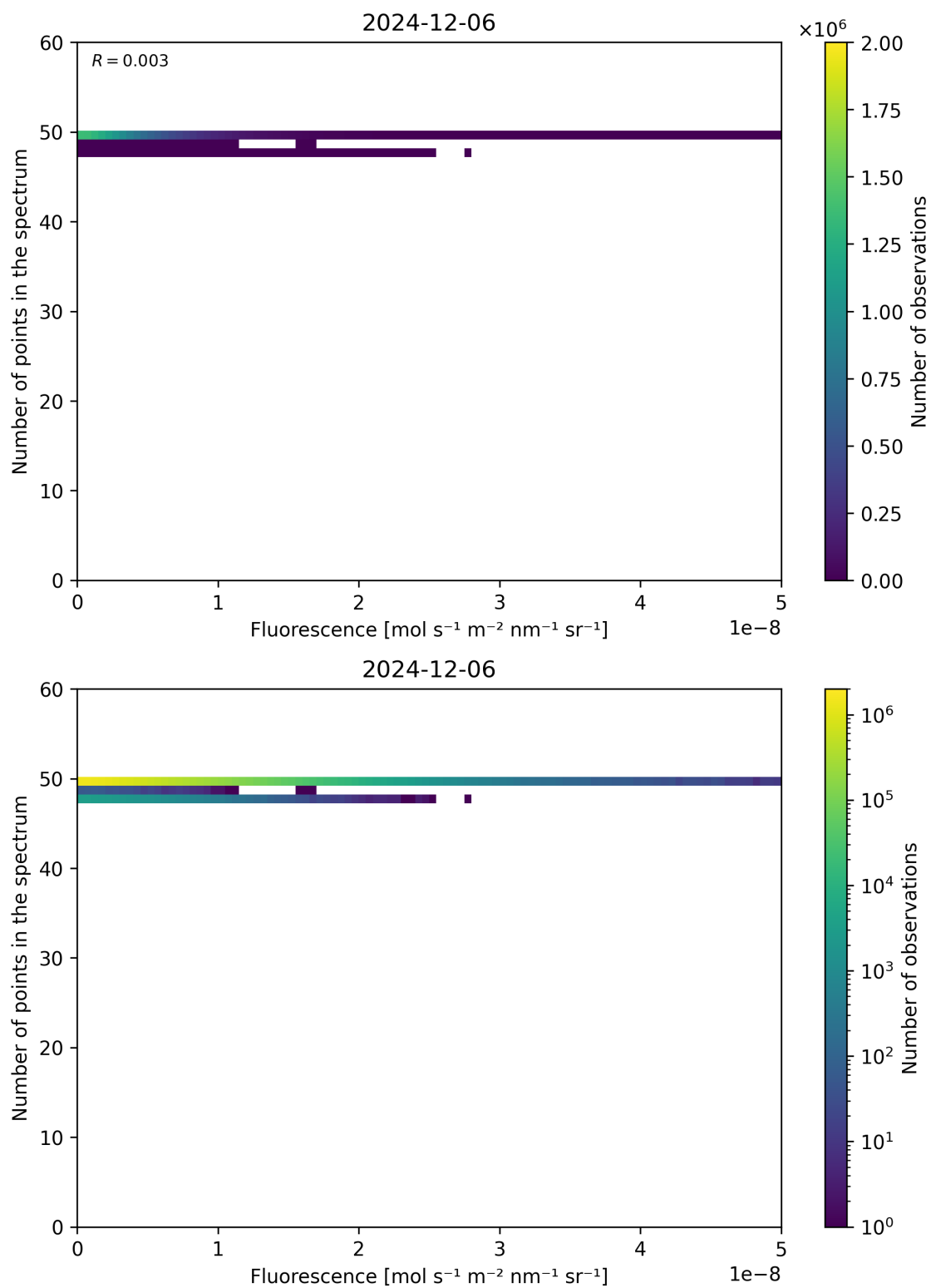
Figure 86: Scatter density plot of “Fluorescence” against “Number of points in the spectrum” for 2024-12-06 to 2024-12-07.
