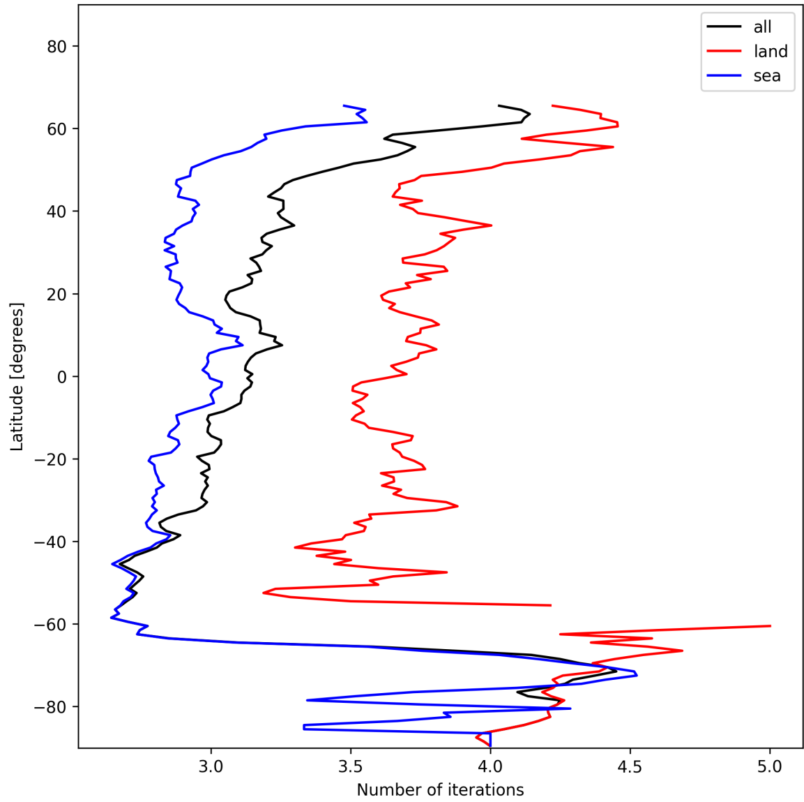
Figure 22: Zonal average of “Number of iterations” for 2024-12-06 to 2024-12-07.
