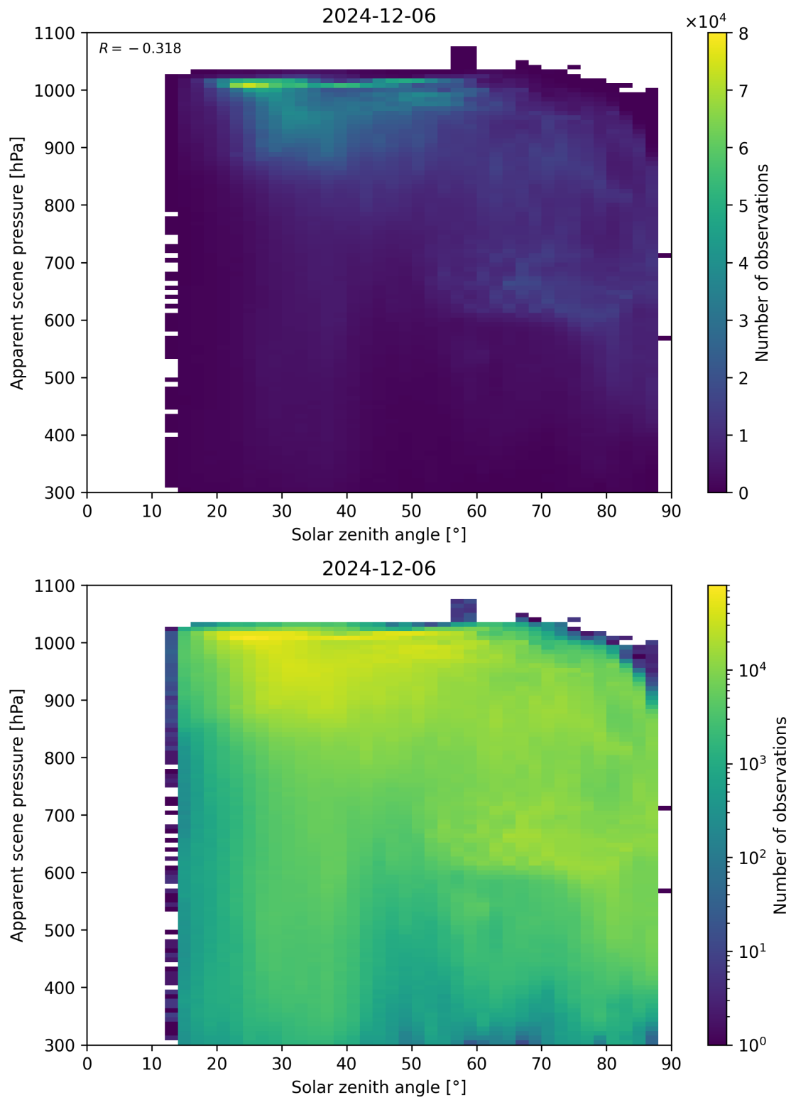
Figure 108: Scatter density plot of “Solar zenith angle” against “Apparent scene pressure” for 2024-12-06 to 2024-12-07.
