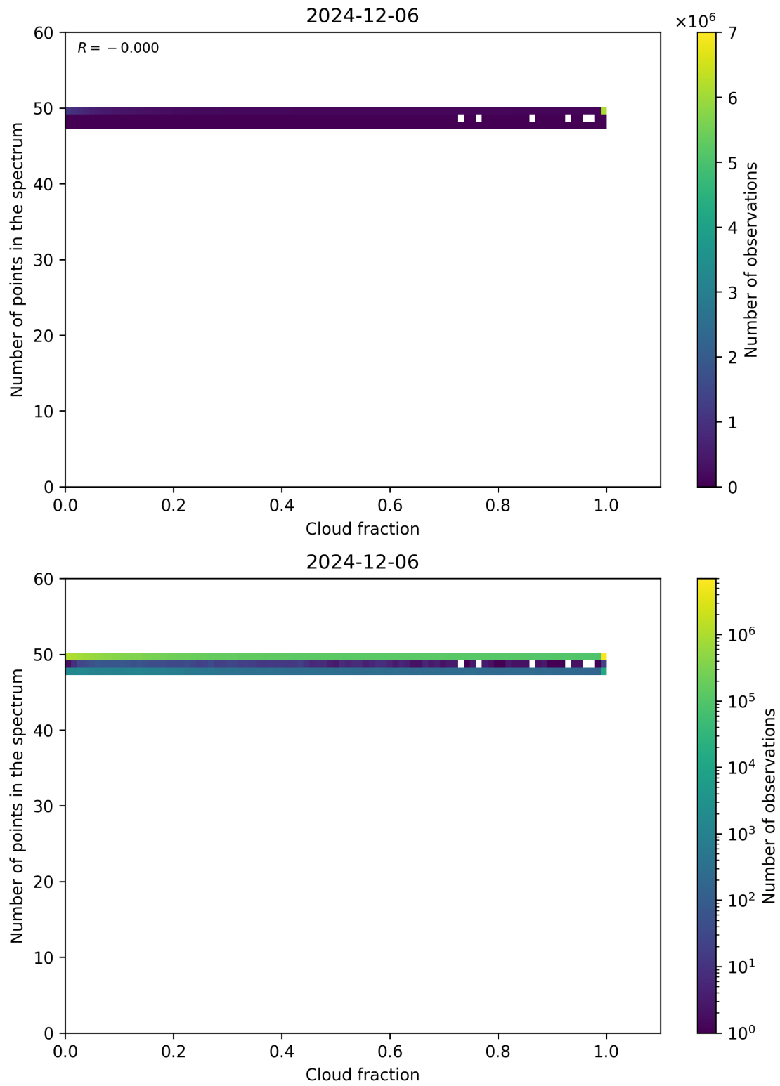
Figure 74: Scatter density plot of “Cloud fraction” against “Number of points in the spectrum” for 2024-12-06 to 2024-12-07.
