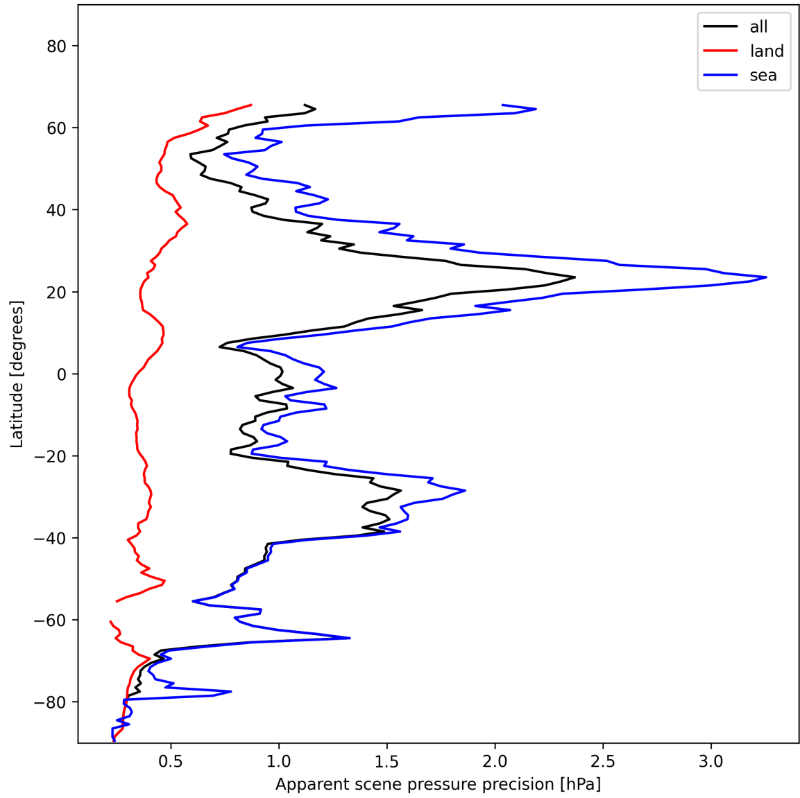
Figure 20: Zonal average of “Apparent scene pressure precision” for 2024-12-06 to 2024-12-07.
