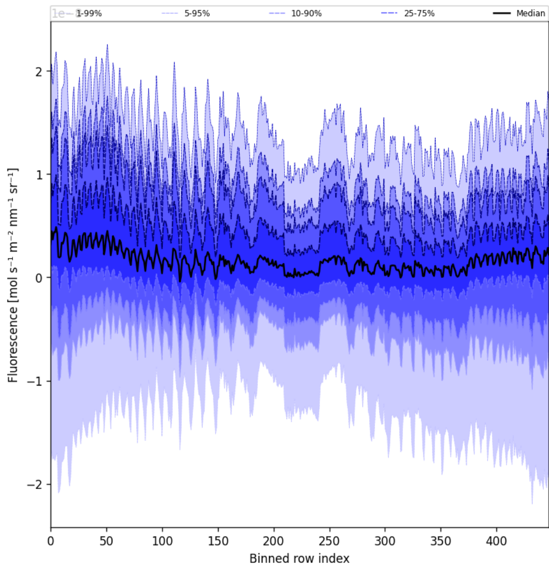
Figure 57: Along track statistics of “Fluorescence” for 2024-12-06 to 2024-12-07
