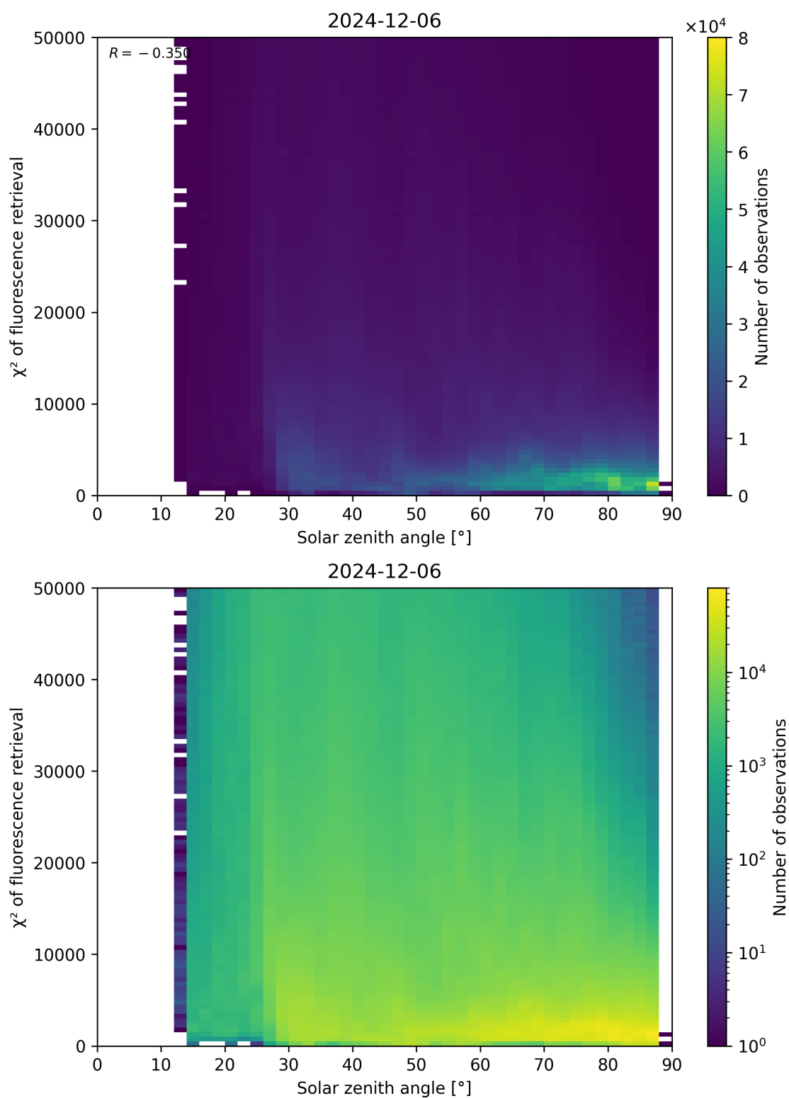
Figure 109: Scatter density plot of “Solar zenith angle” against “ \chi^2 of fluorescence retrieval” for 2024-12-06 to 2024-12-07.
