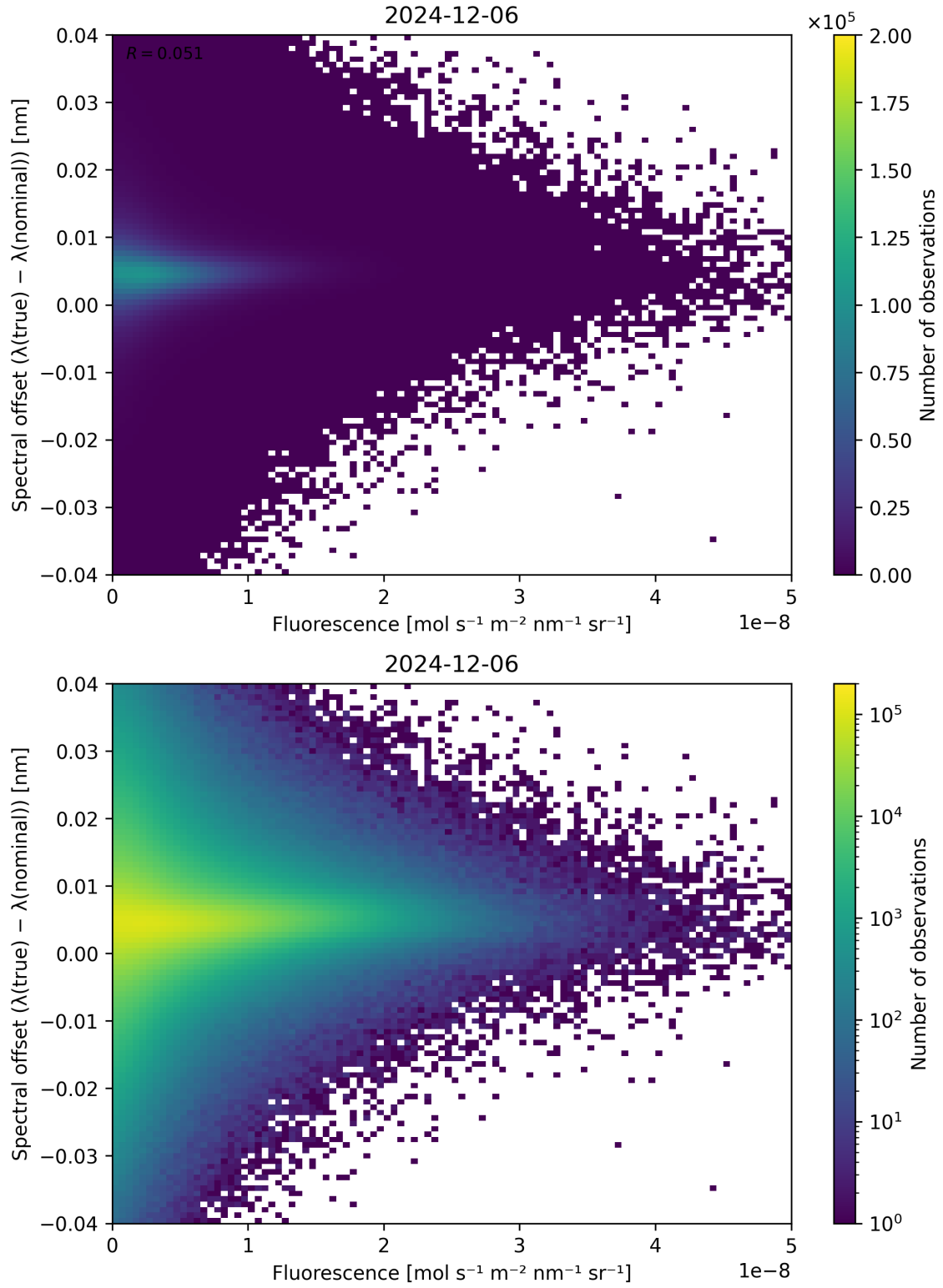
Figure 87: Scatter density plot of “Fluorescence” against “Spectral offset ( \lambda_{\text{true}} - \lambda_{\text{nominal}} )” for 2024-12-06 to 2024-12-07.
