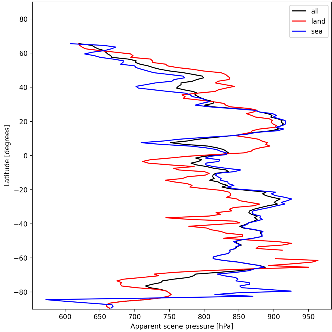
Figure 19: Zonal average of “Apparent scene pressure” for 2024-12-06 to 2024-12-07.
