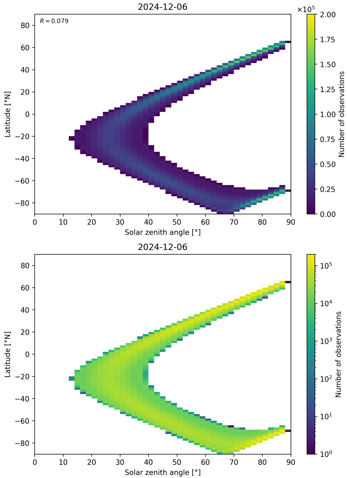
Figure 113: Scatter density plot of “Solar zenith angle” against “Latitude” for 2024-12-06 to 2024-12-07.
