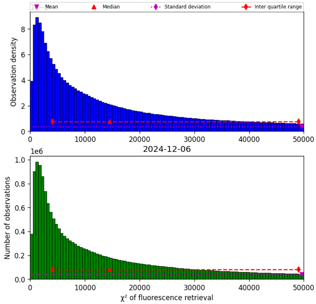
Figure 42: Histogram of “ \chi^2 of fluorescence retrieval” for 2024-12-06 to 2024-12-07
