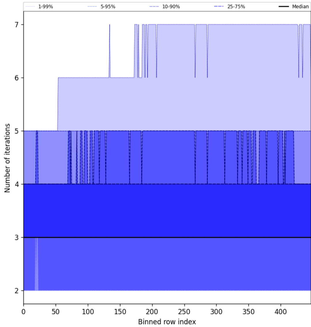
Figure 56: Along track statistics of “Number of iterations” for 2024-12-06 to 2024-12-07
