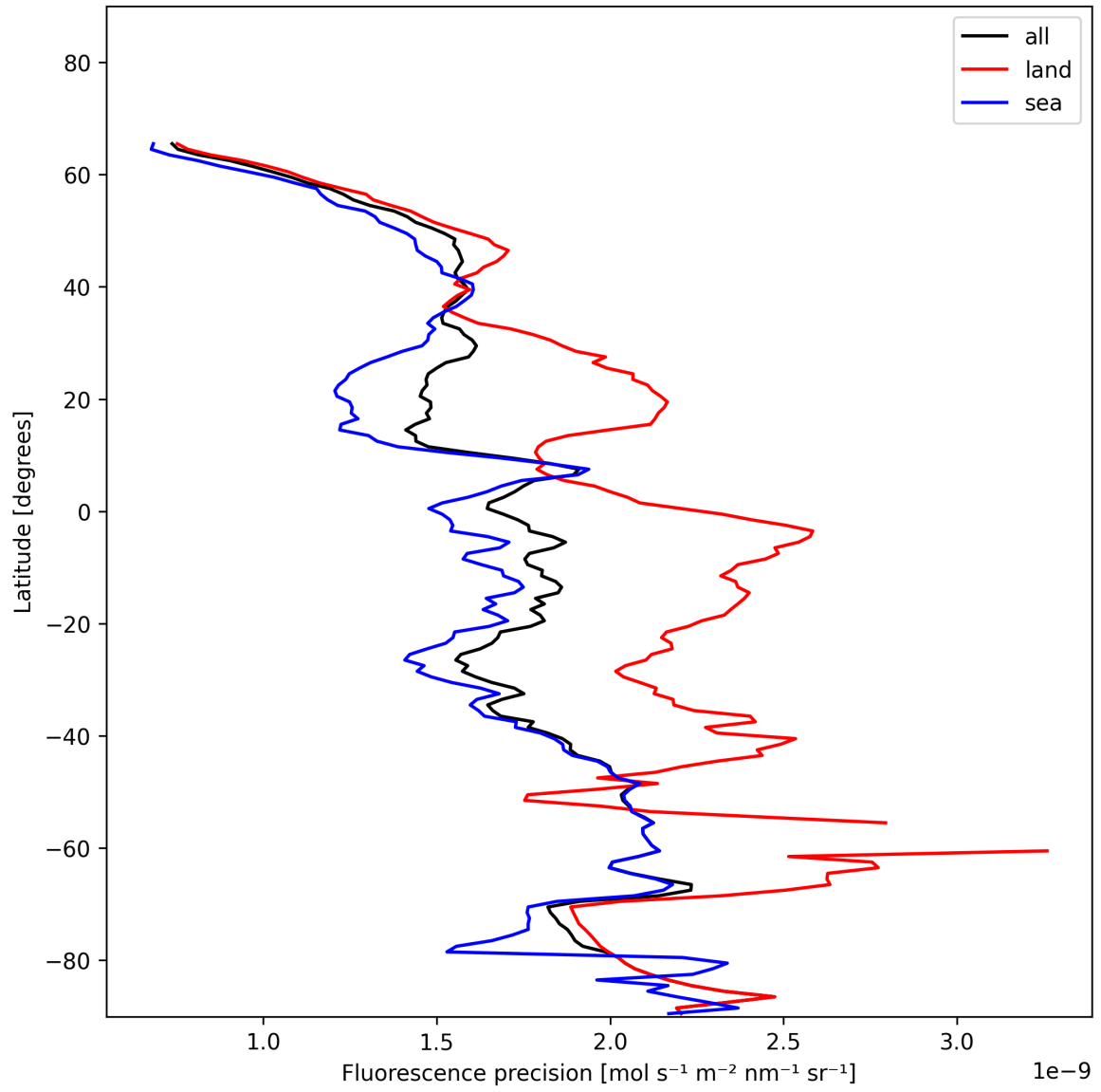
Figure 24: Zonal average of “Fluorescence precision” for 2024-12-06 to 2024-12-07.
