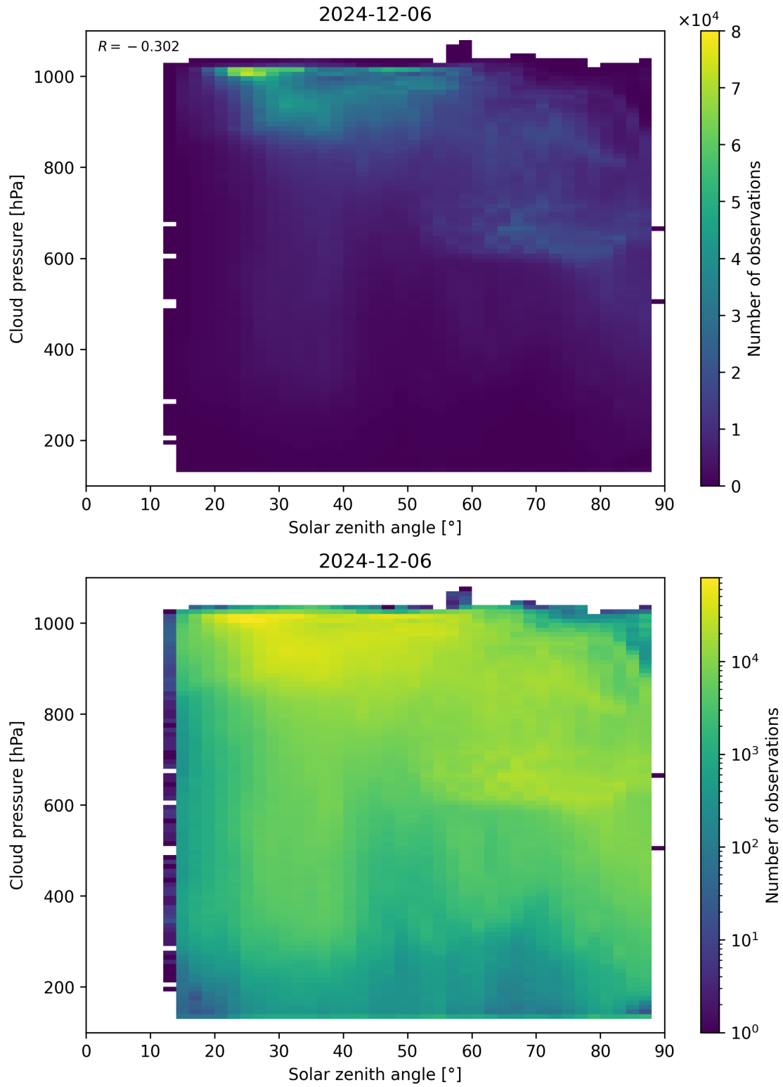
Figure 111: Scatter density plot of “Solar zenith angle” against “Cloud pressure” for 2024-12-06 to 2024-12-07.
