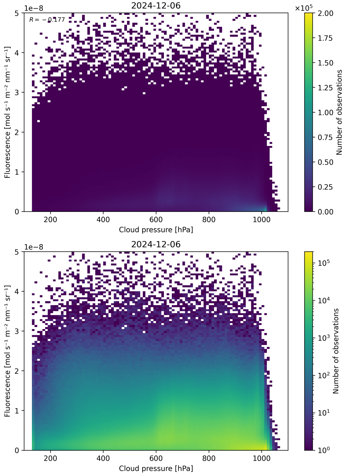
Figure 80: Scatter density plot of “Cloud pressure” against “Fluorescence” for 2024-12-06 to 2024-12-07.
