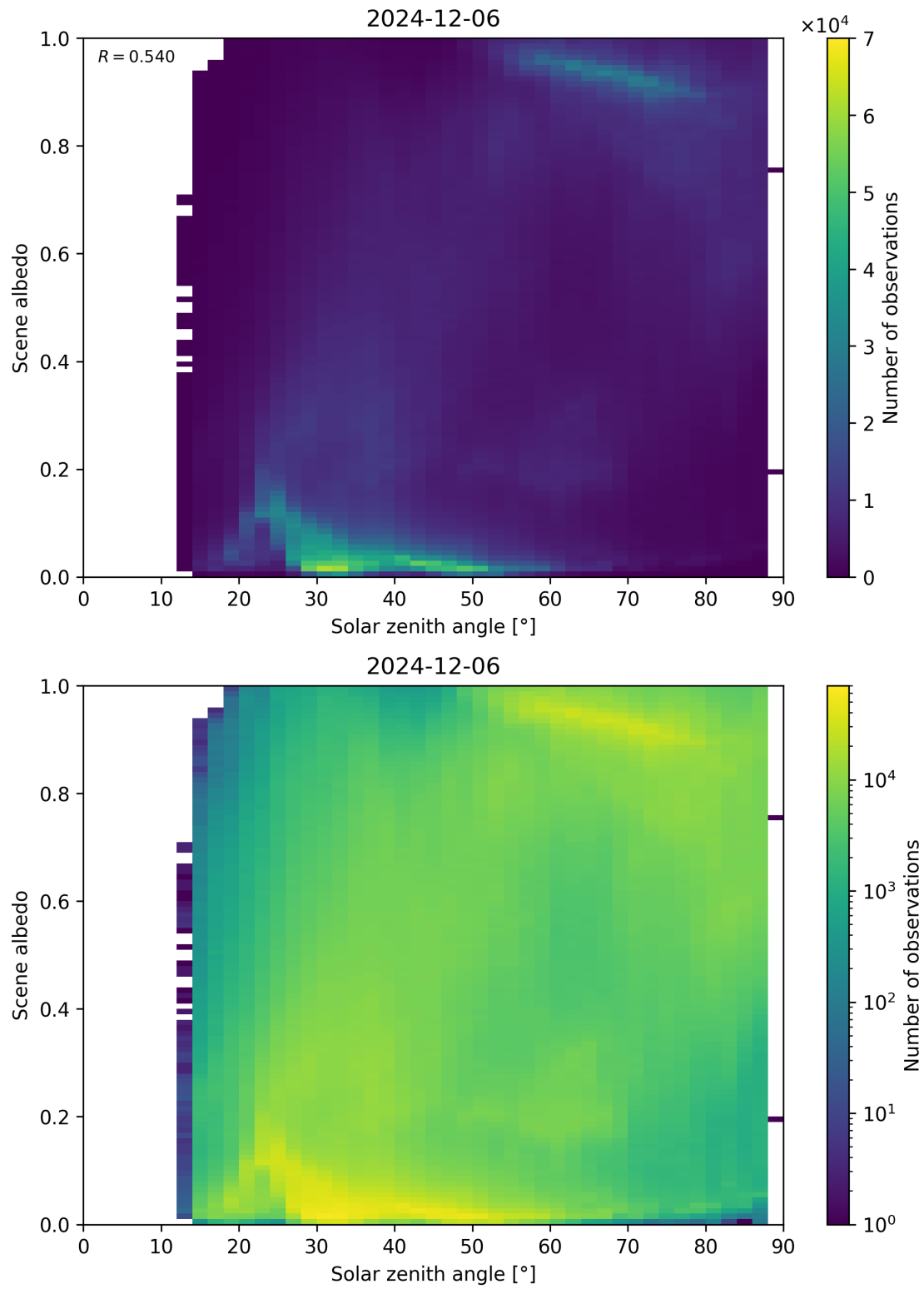
Figure 116: Scatter density plot of “Solar zenith angle” against “Scene albedo” for 2024-12-06 to 2024-12-07.
