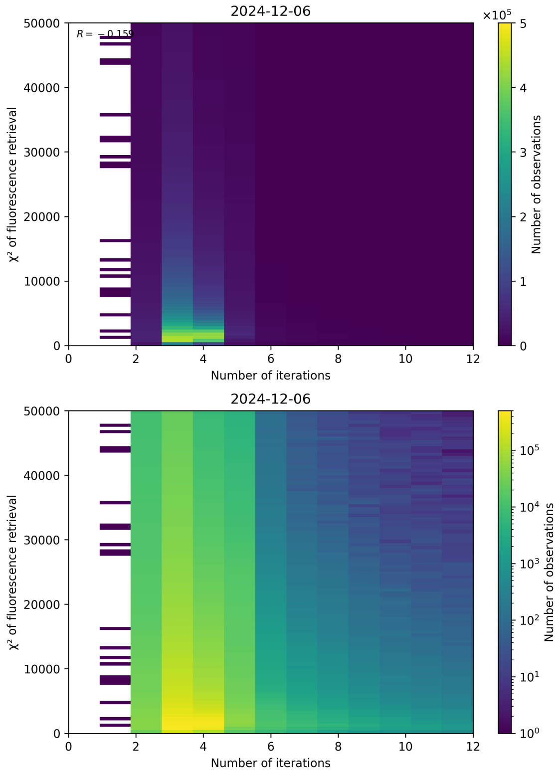
Figure 97: Scatter density plot of “Number of iterations” against “ \chi^2 of fluorescence retrieval” for 2024-12-06 to 2024-12-07.
