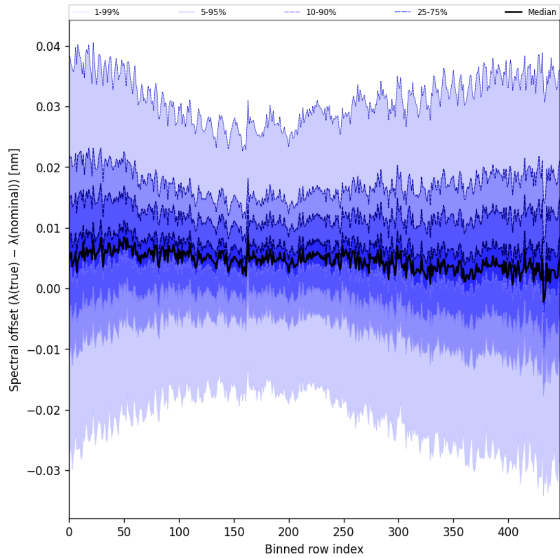
Figure 62: Along track statistics of “Spectral offset ( \lambda_{\text{true}} - \lambda_{\text{nominal}} )” for 2024-12-06 to 2024-12-07
