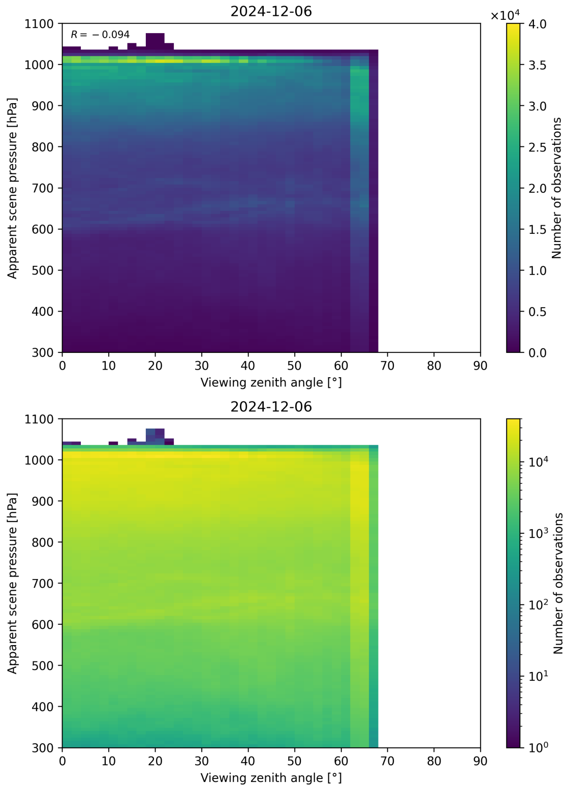
Figure 118: Scatter density plot of “Viewing zenith angle” against “Apparent scene pressure” for 2024-12-06 to 2024-12-07.
