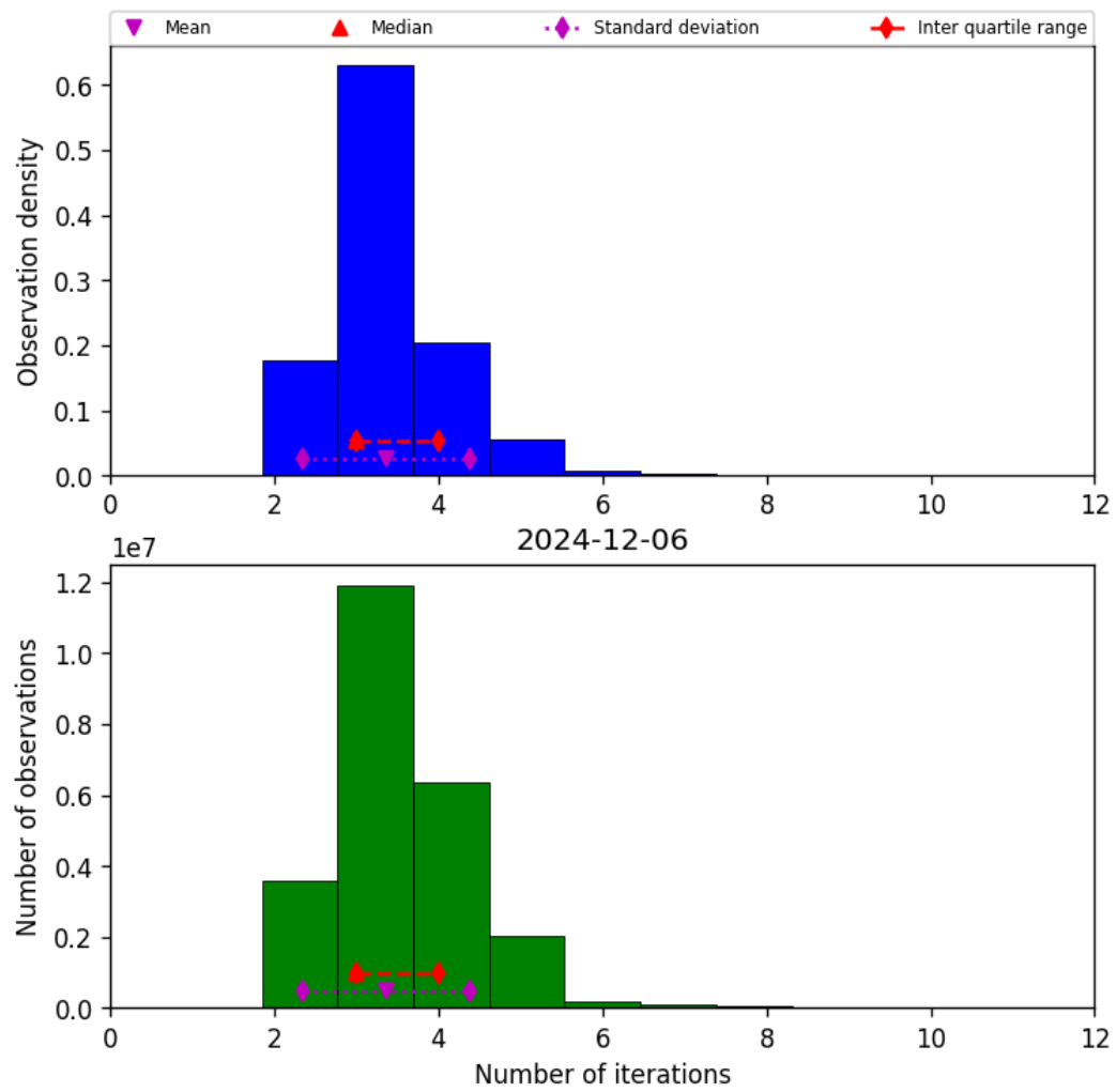
Figure 39: Histogram of “Number of iterations” for 2024-12-06 to 2024-12-07
