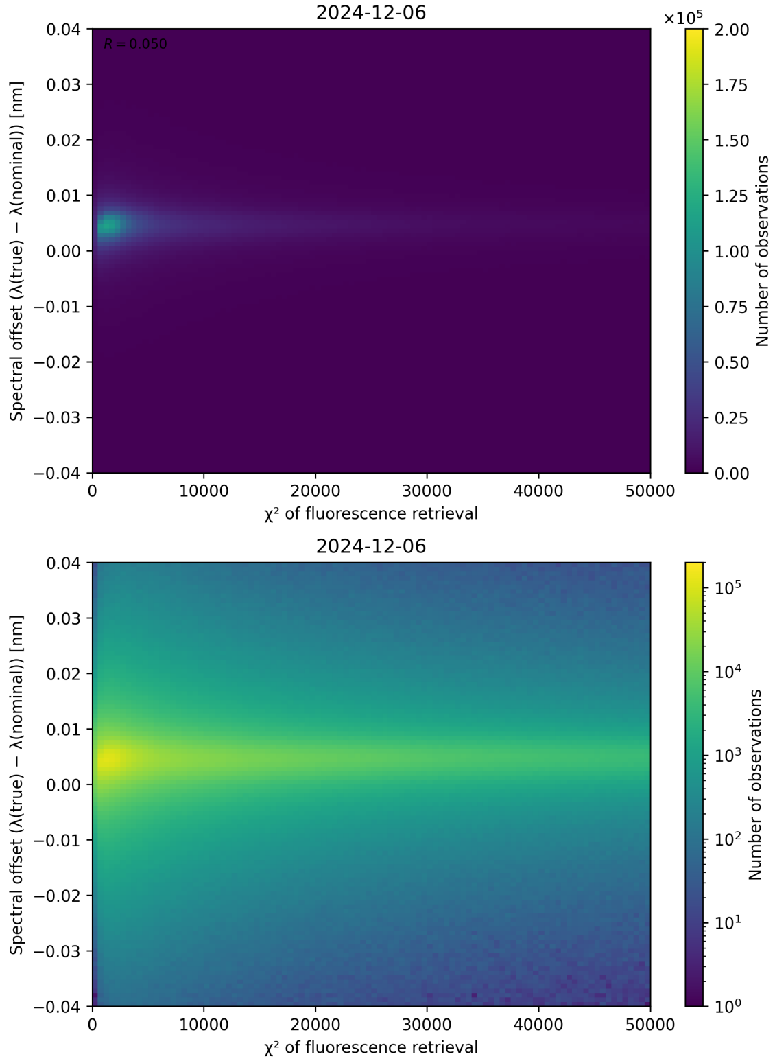
Figure 69: Scatter density plot of “ \chi^2 of fluorescence retrieval” against “Spectral offset ( \lambda_{\text{true}} - \lambda_{\text{nominal}} )” for 2024-12-06 to 2024-12-07.
