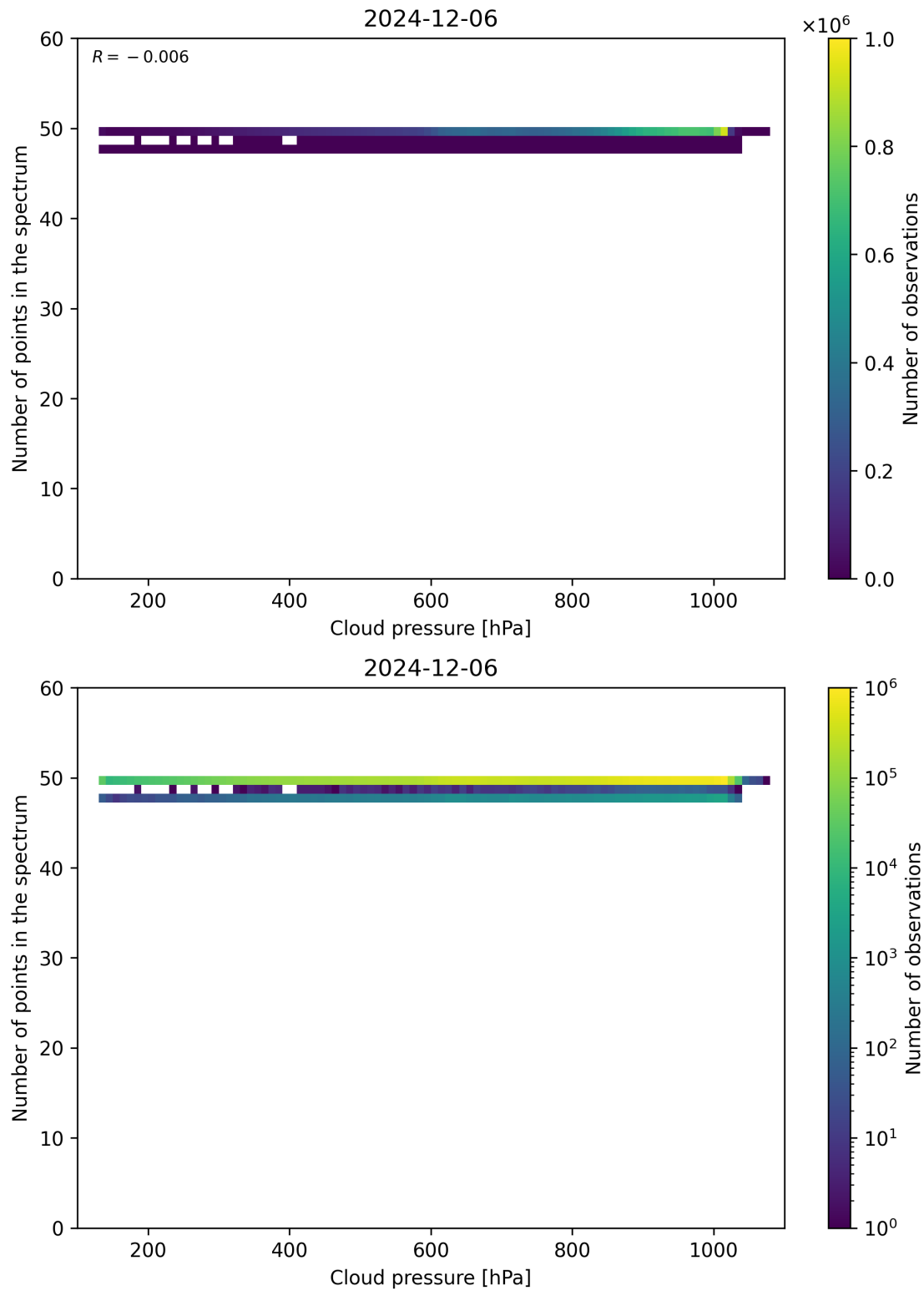
Figure 82: Scatter density plot of “Cloud pressure” against “Number of points in the spectrum” for 2024-12-06 to 2024-12-07.
