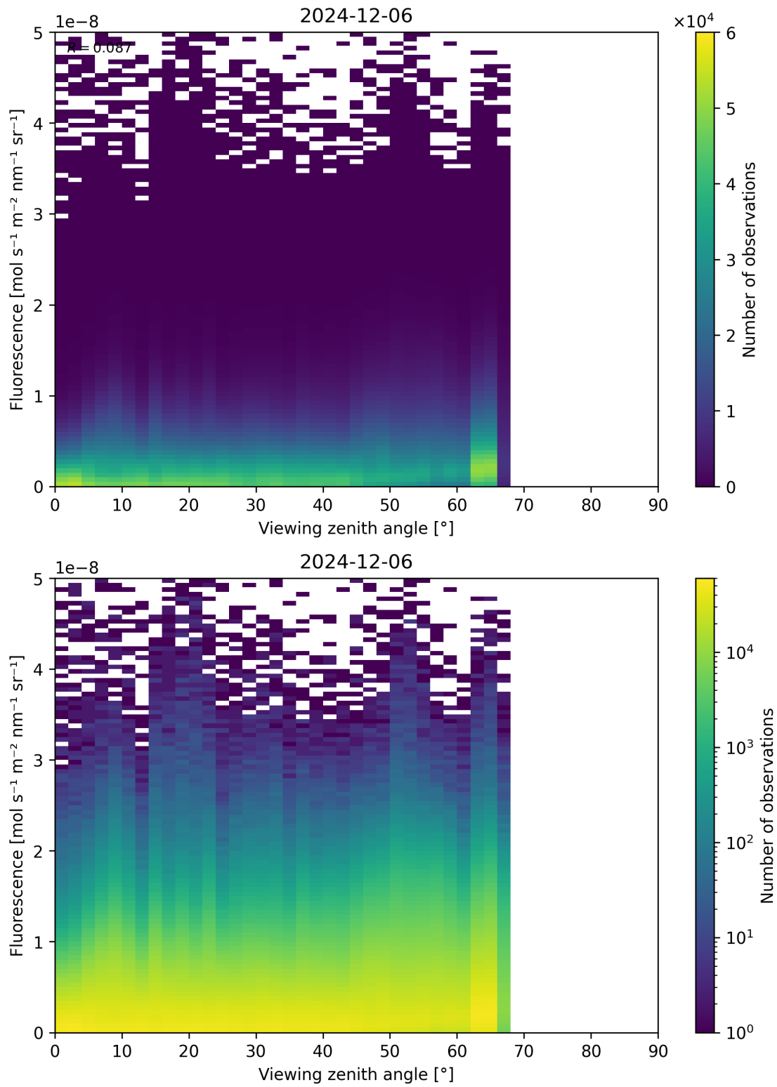
Figure 122: Scatter density plot of “Viewing zenith angle” against “Fluorescence” for 2024-12-06 to 2024-12-07.
