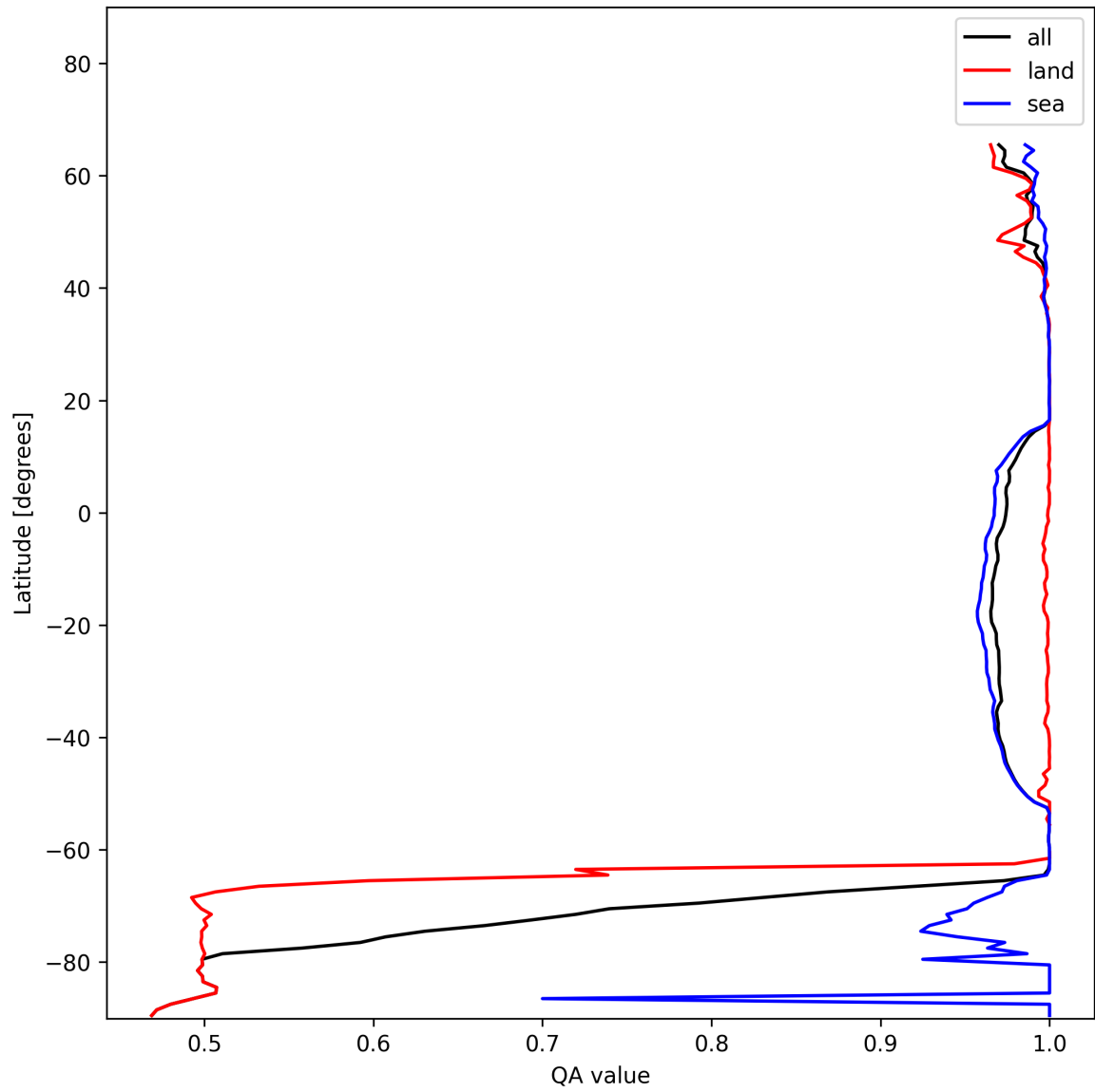
Figure 12: Zonal average of “QA value” for 2024-12-06 to 2024-12-07.
