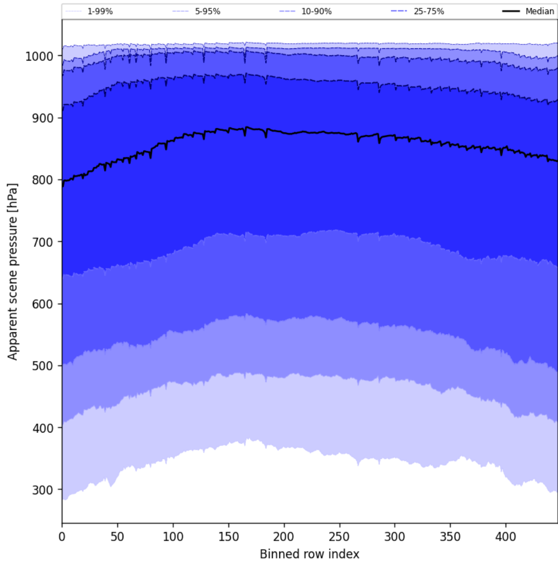
Figure 53: Along track statistics of “Apparent scene pressure” for 2024-12-06 to 2024-12-07
