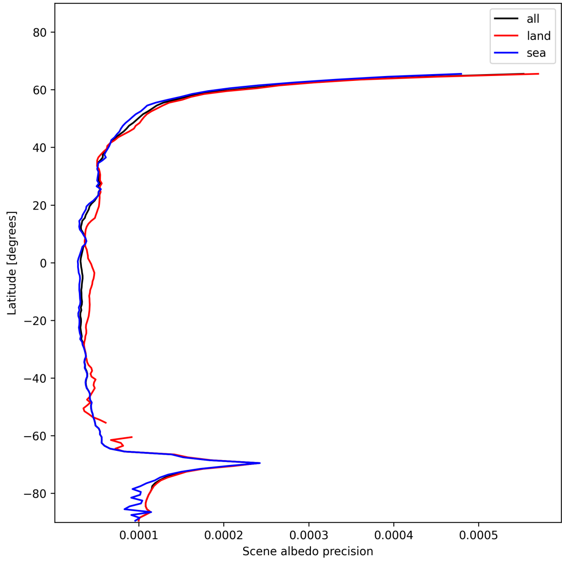
Figure 18: Zonal average of “Scene albedo precision” for 2024-12-06 to 2024-12-07.
