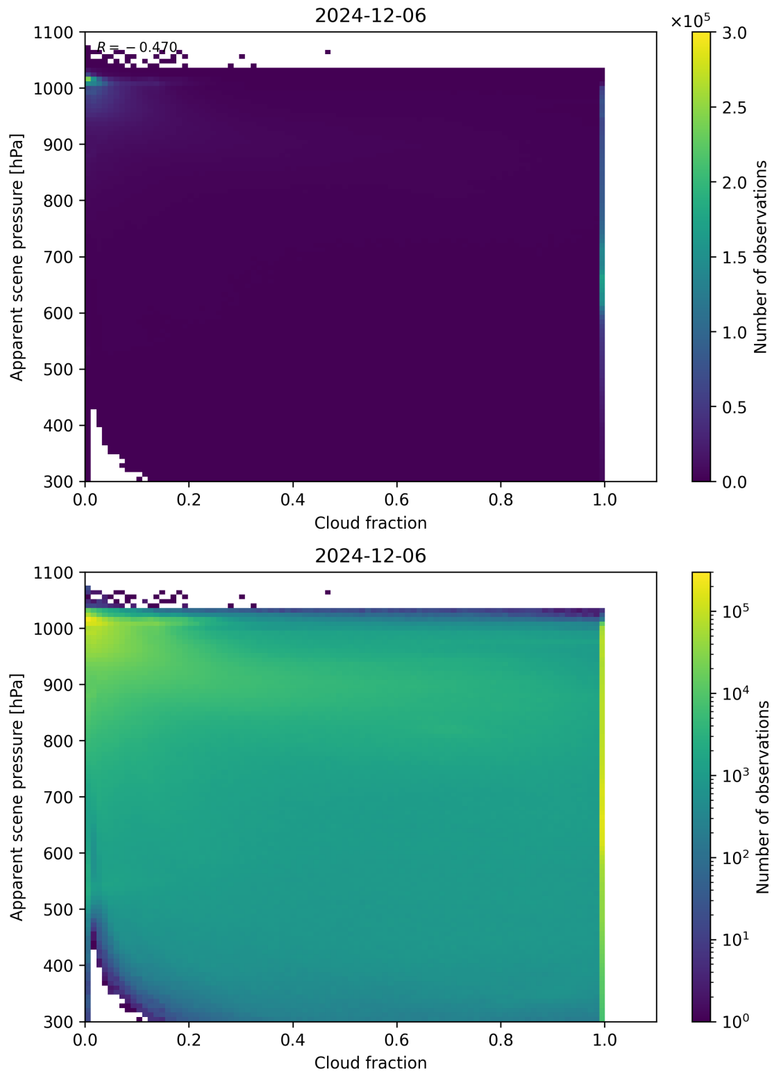
Figure 70: Scatter density plot of “Cloud fraction” against “Apparent scene pressure” for 2024-12-06 to 2024-12-07.
