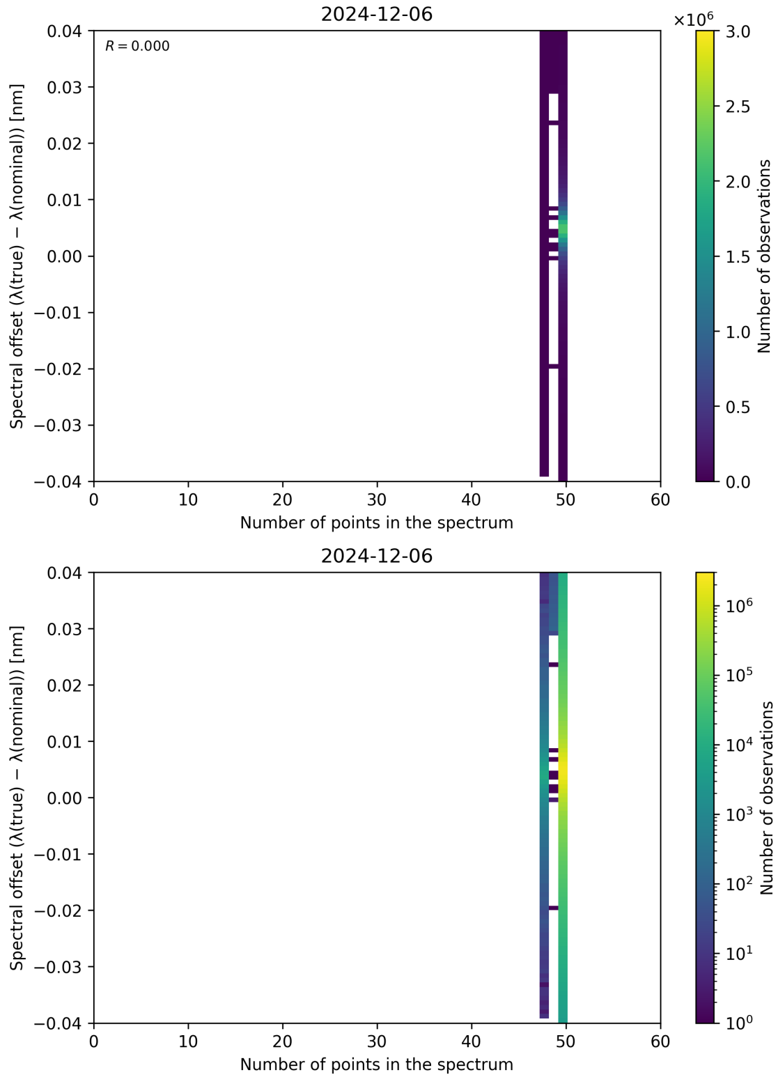
Figure 101: Scatter density plot of “Number of points in the spectrum” against “Spectral offset ( \lambda_{\text{true}} - \lambda_{\text{nominal}} )” for 2024-12-06 to 2024-12-07.
