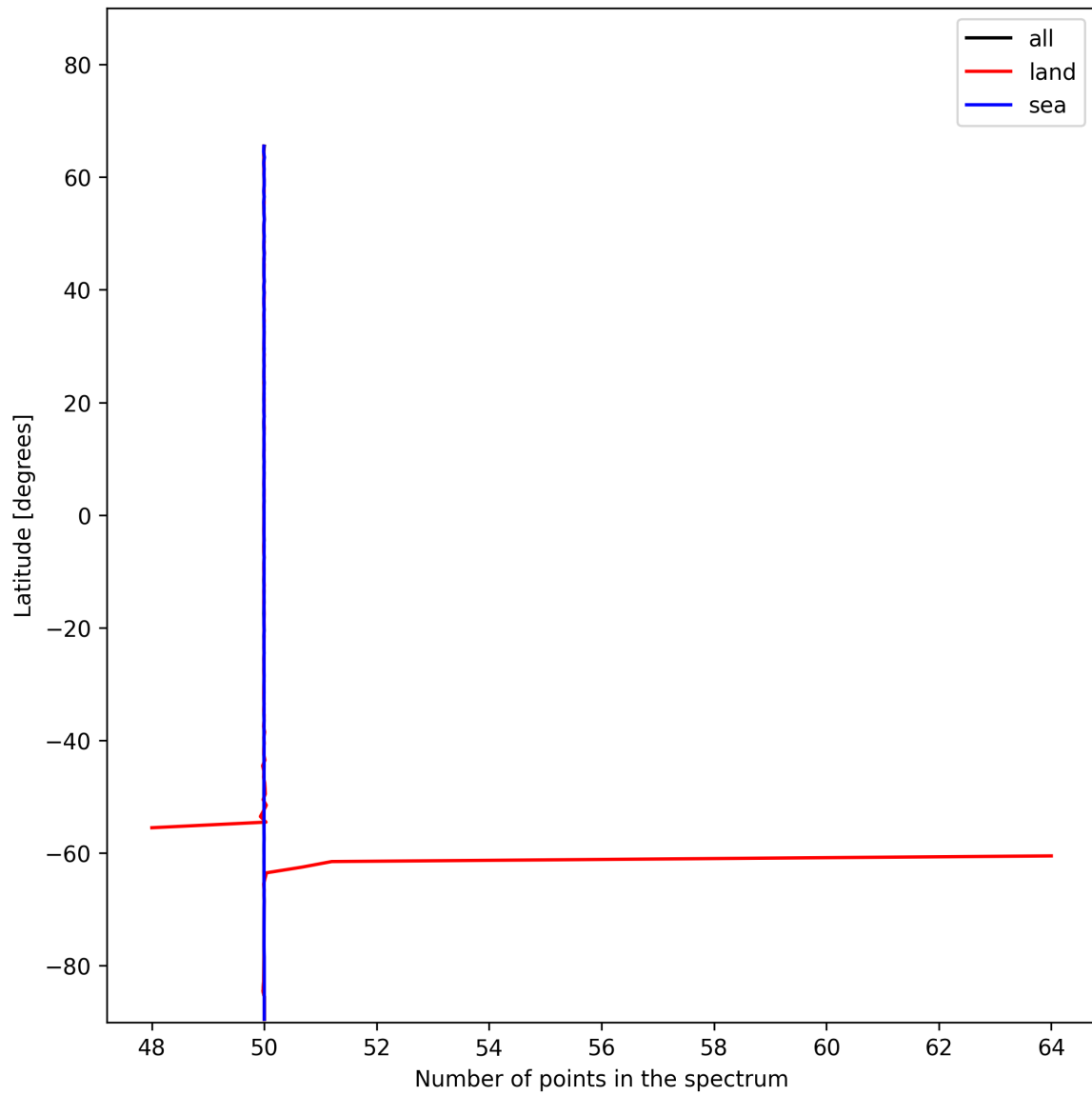
Figure 27: Zonal average of “Number of points in the spectrum” for 2024-12-06 to 2024-12-07.
