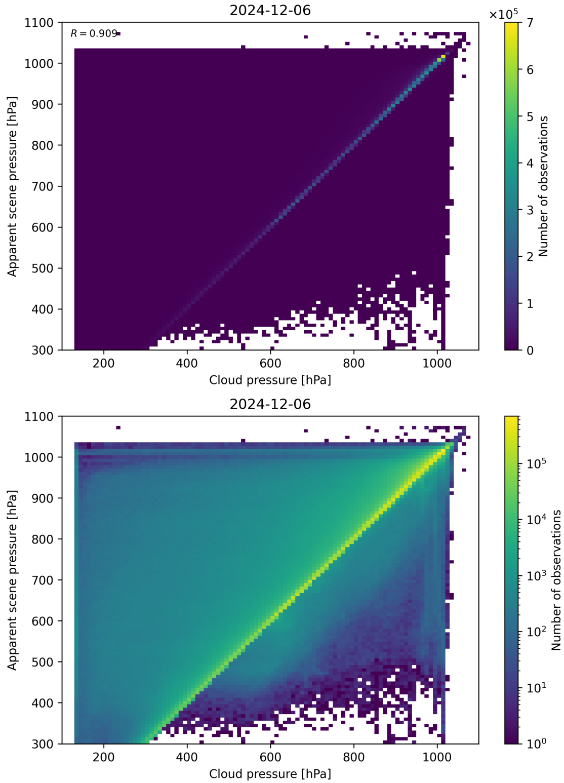
Figure 77: Scatter density plot of “Cloud pressure” against “Apparent scene pressure” for 2024-12-06 to 2024-12-07.
