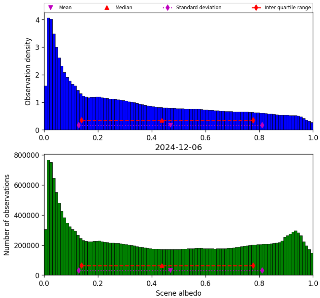
Figure 34: Histogram of “Scene albedo” for 2024-12-06 to 2024-12-07
