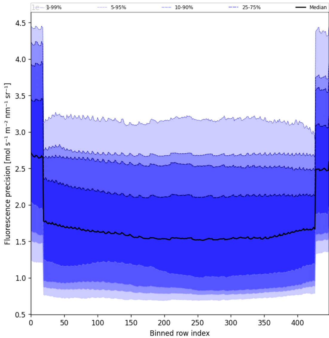
Figure 58: Along track statistics of “Fluorescence precision” for 2024-12-06 to 2024-12-07
