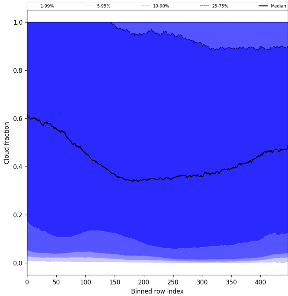
Figure 49: Along track statistics of “Cloud fraction” for 2024-12-06 to 2024-12-07
