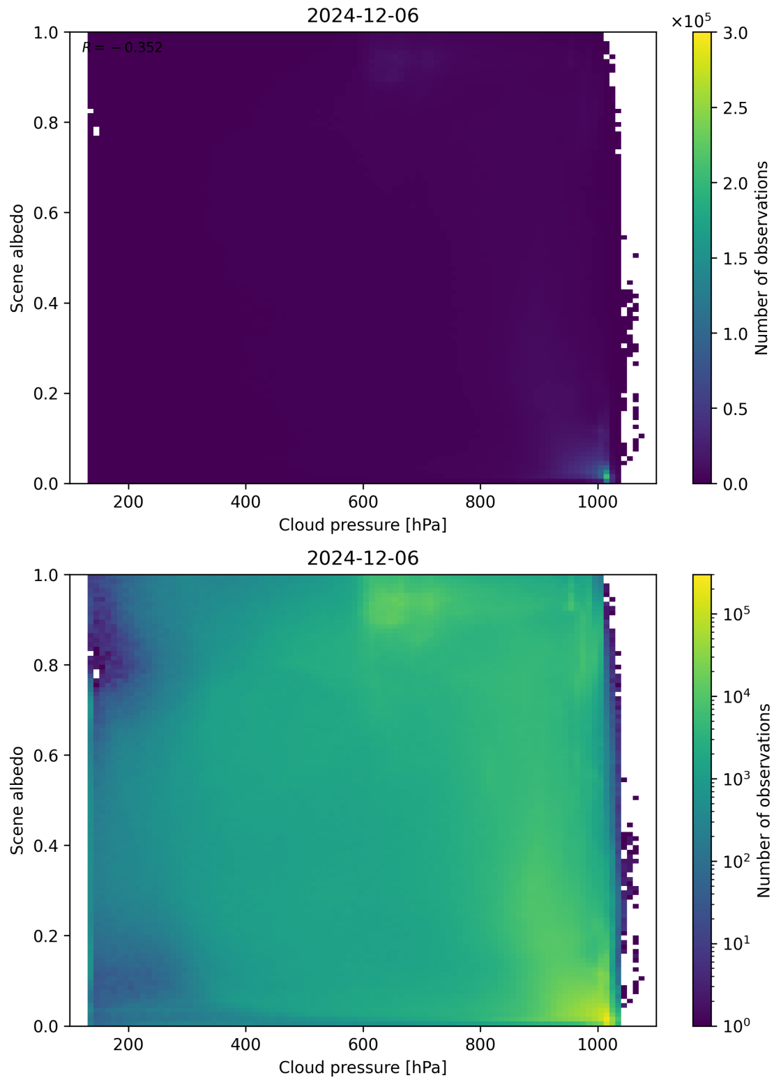
Figure 83: Scatter density plot of “Cloud pressure” against “Scene albedo” for 2024-12-06 to 2024-12-07.
