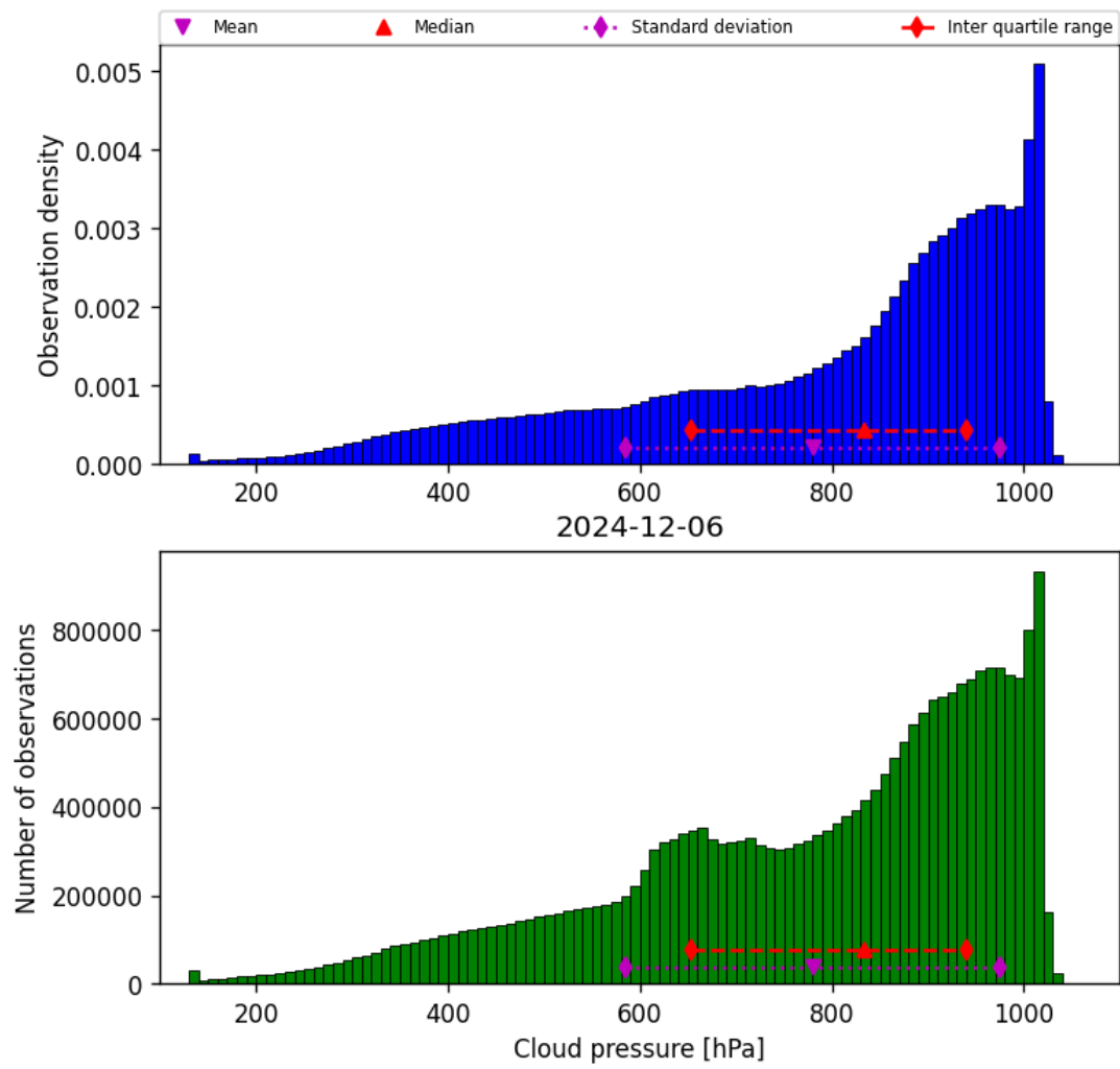
Figure 30: Histogram of “Cloud pressure” for 2024-12-06 to 2024-12-07
