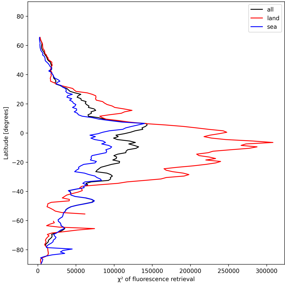
Figure 25: Zonal average of “ \chi^2 of fluorescence retrieval” for 2024-12-06 to 2024-12-07.
