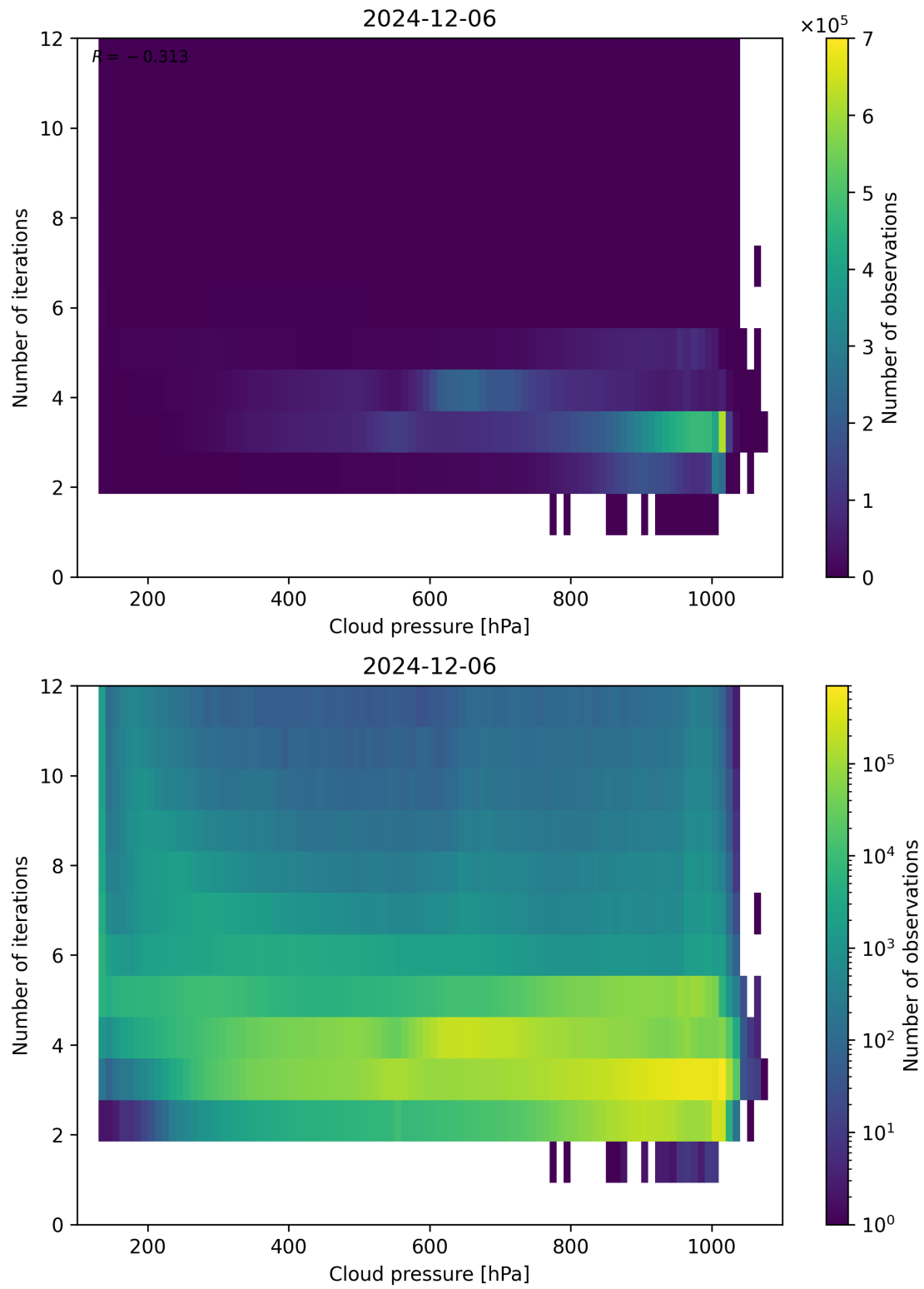
Figure 81: Scatter density plot of “Cloud pressure” against “Number of iterations” for 2024-12-06 to 2024-12-07.
