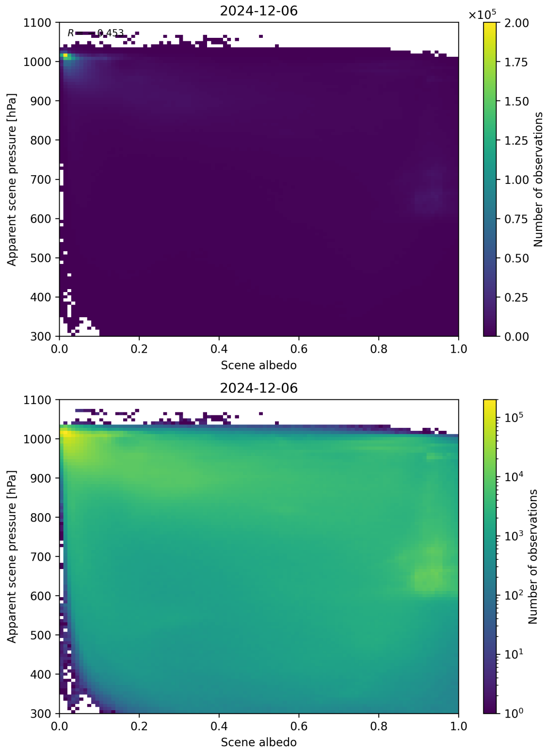
Figure 102: Scatter density plot of “Scene albedo” against “Apparent scene pressure” for 2024-12-06 to 2024-12-07.
