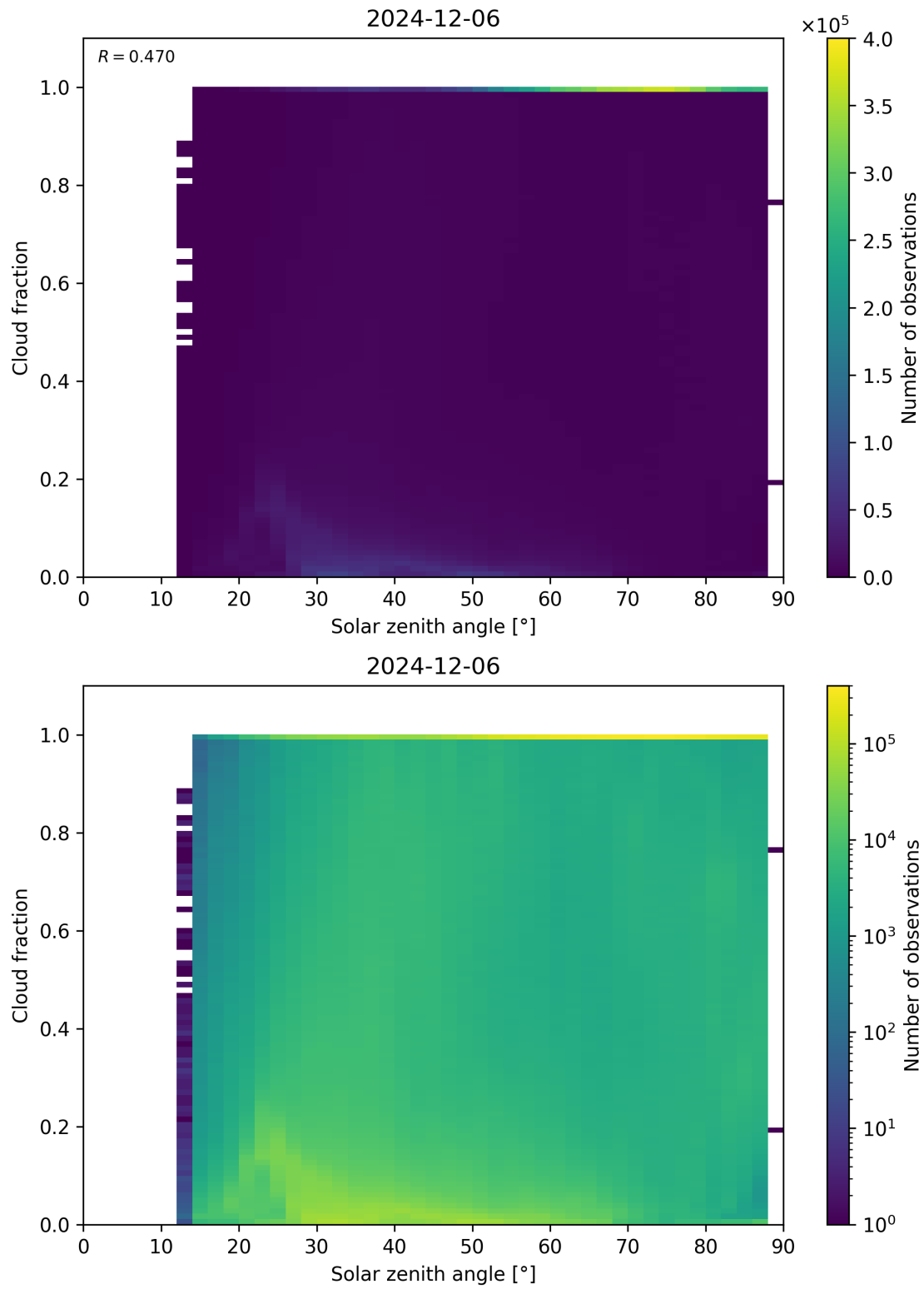
Figure 110: Scatter density plot of “Solar zenith angle” against “Cloud fraction” for 2024-12-06 to 2024-12-07.
