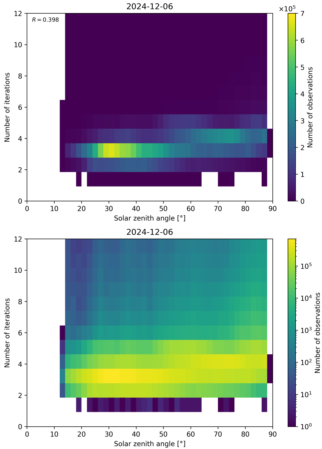
Figure 114: Scatter density plot of “Solar zenith angle” against “Number of iterations” for 2024-12-06 to 2024-12-07.
