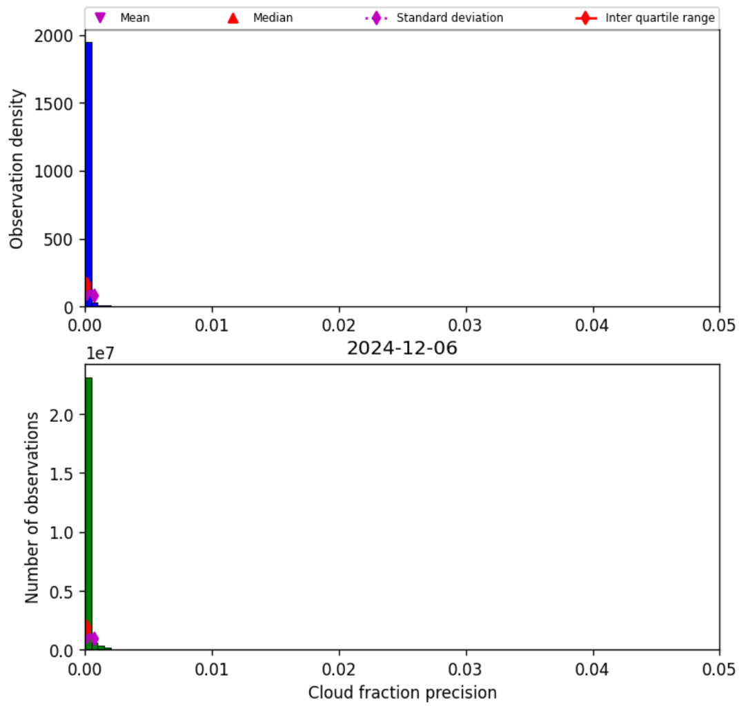
Figure 33: Histogram of “Cloud fraction precision” for 2024-12-06 to 2024-12-07
