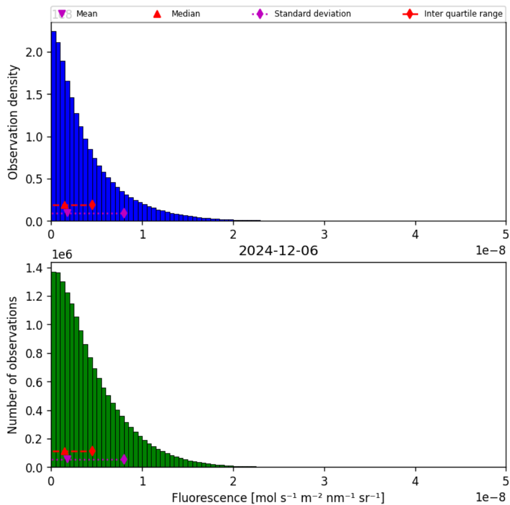
Figure 40: Histogram of “Fluorescence” for 2024-12-06 to 2024-12-07
