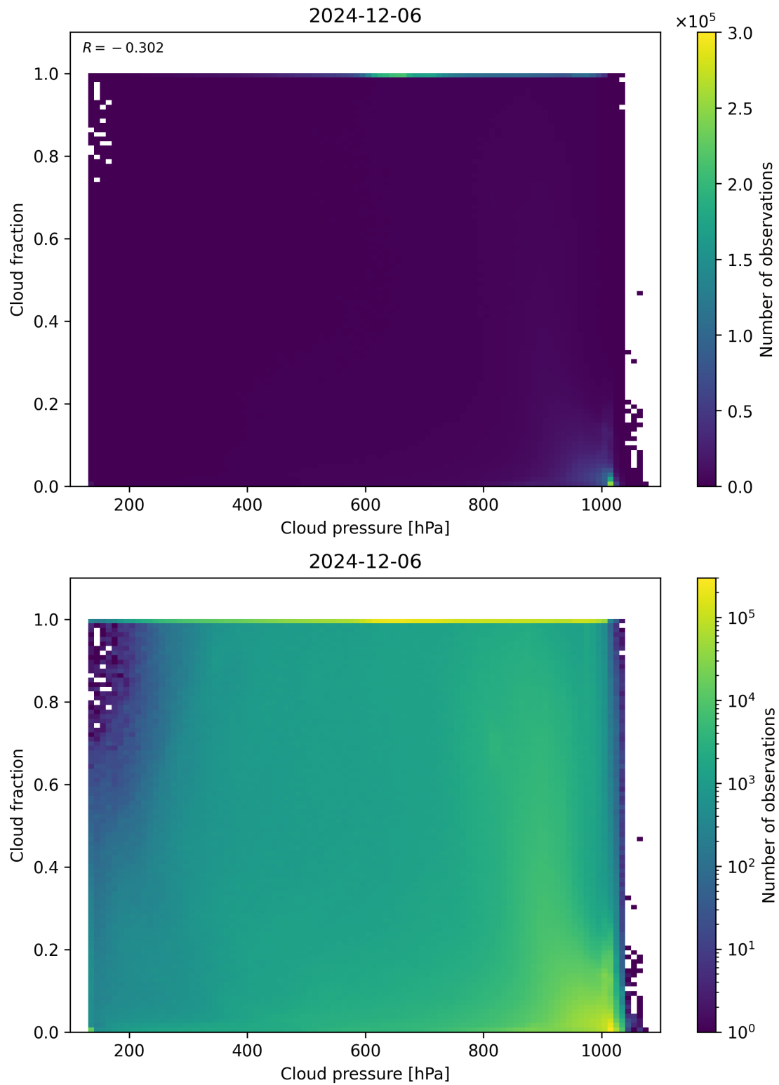
Figure 79: Scatter density plot of “Cloud pressure” against “Cloud fraction” for 2024-12-06 to 2024-12-07.
