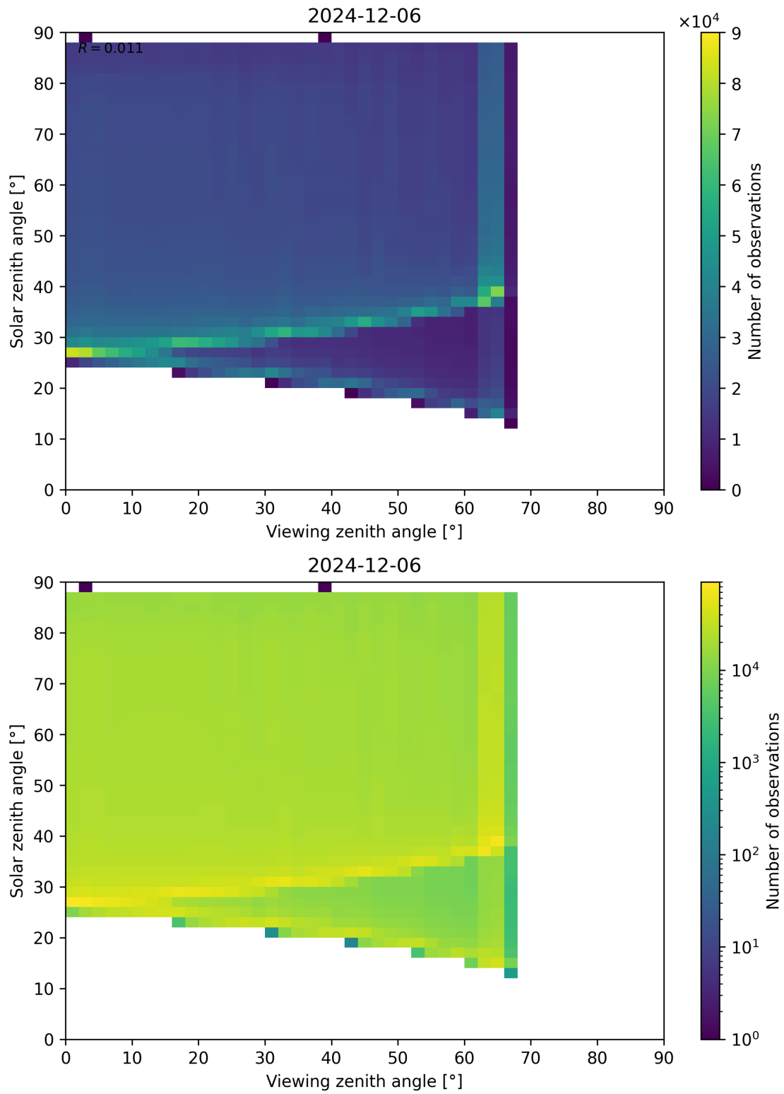
Figure 127: Scatter density plot of “Viewing zenith angle” against “Solar zenith angle” for 2024-12-06 to 2024-12-07.
