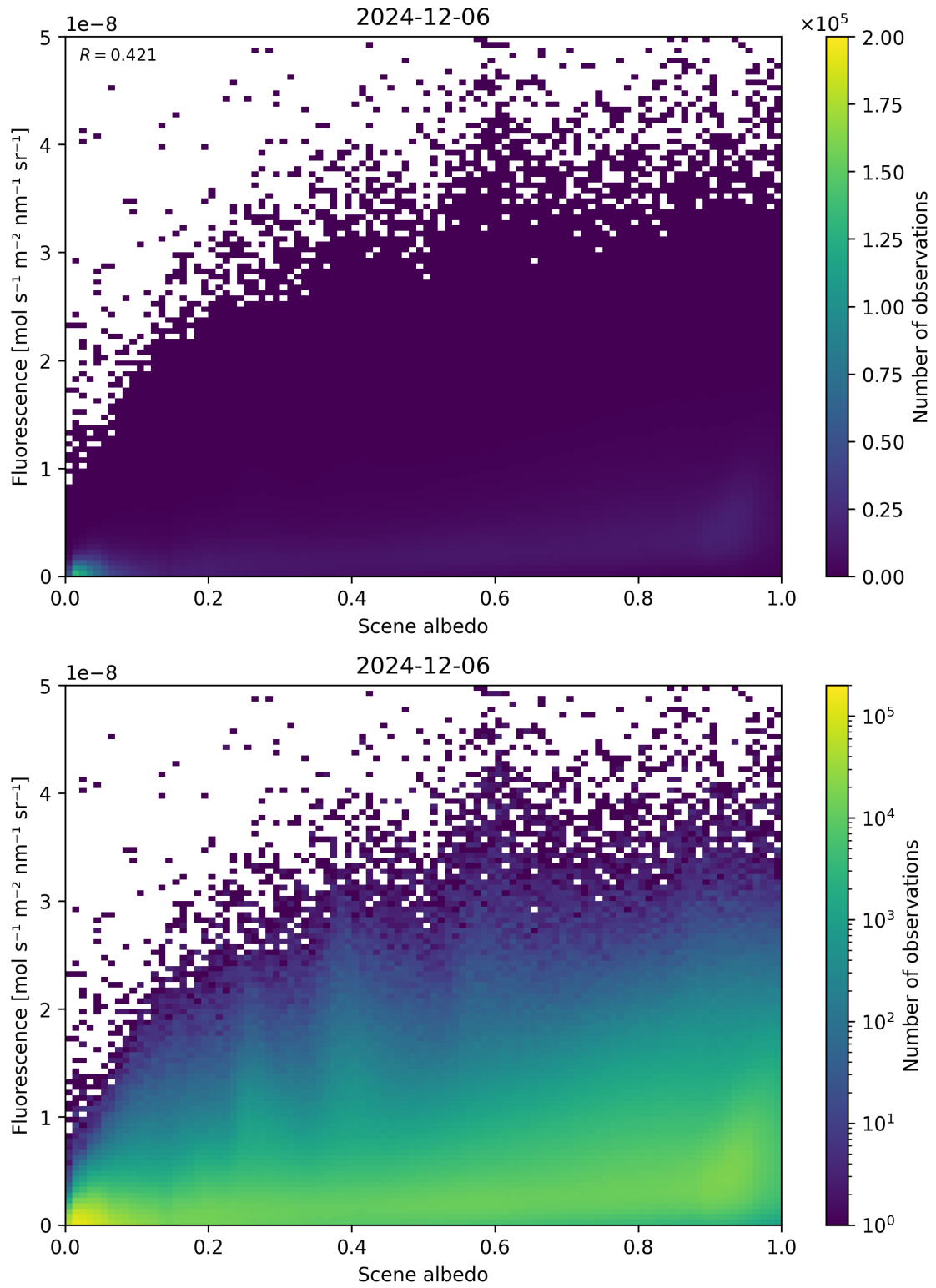
Figure 104: Scatter density plot of “Scene albedo” against “Fluorescence” for 2024-12-06 to 2024-12-07.
