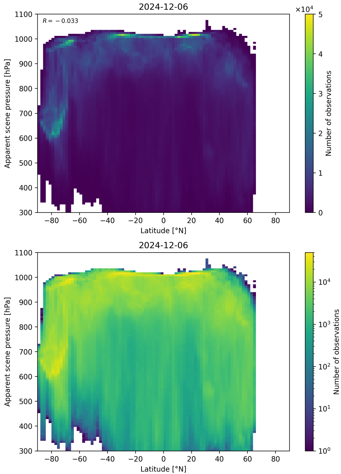
Figure 88: Scatter density plot of “Latitude” against “Apparent scene pressure” for 2024-12-06 to 2024-12-07.
