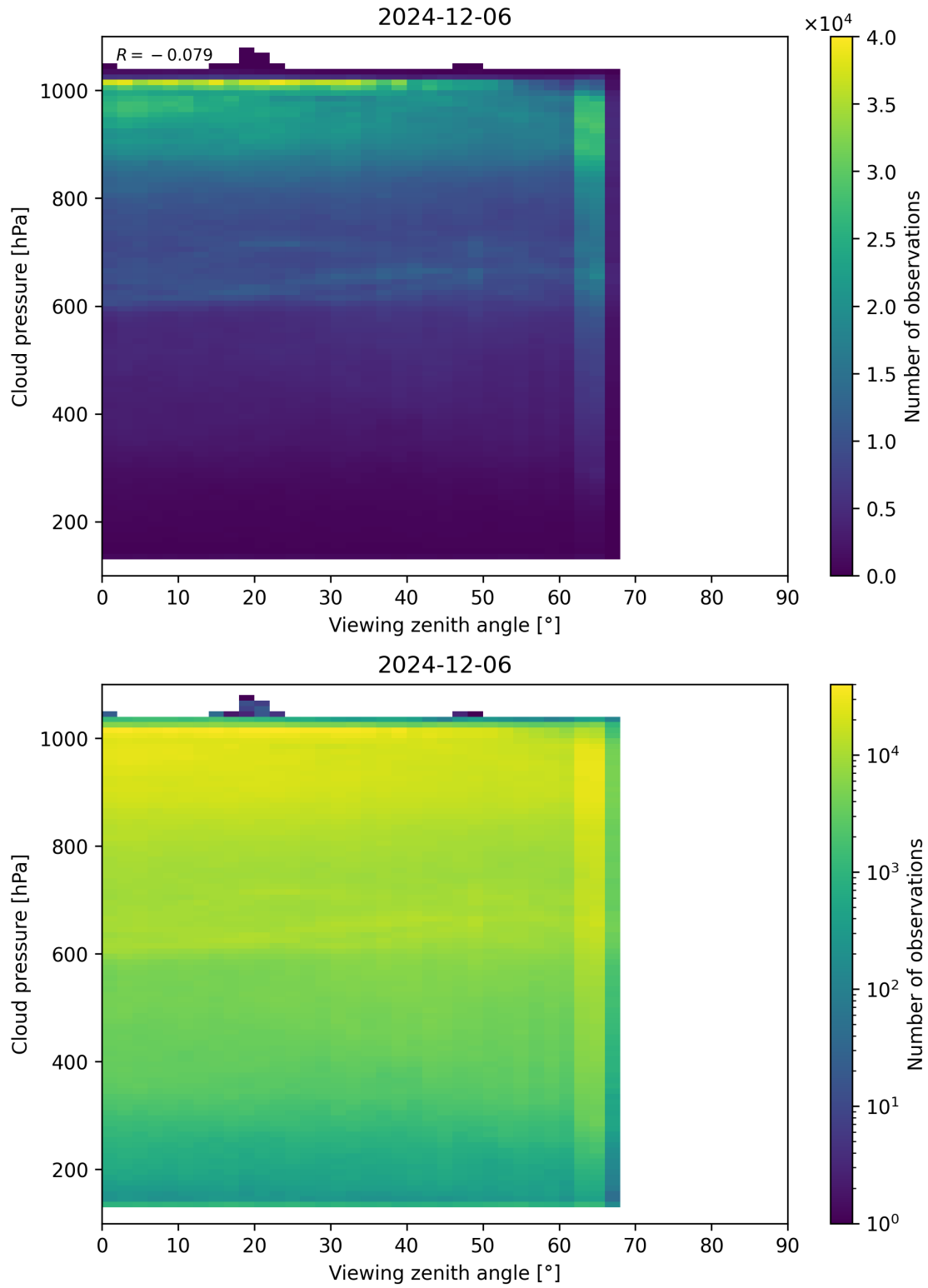
Figure 121: Scatter density plot of “Viewing zenith angle” against “Cloud pressure” for 2024-12-06 to 2024-12-07.
