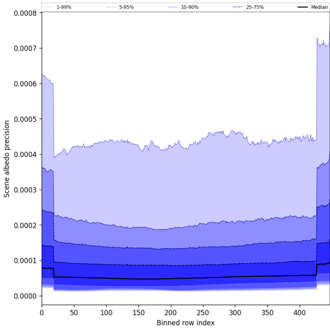
Figure 52: Along track statistics of “Scene albedo precision” for 2024-12-06 to 2024-12-07
