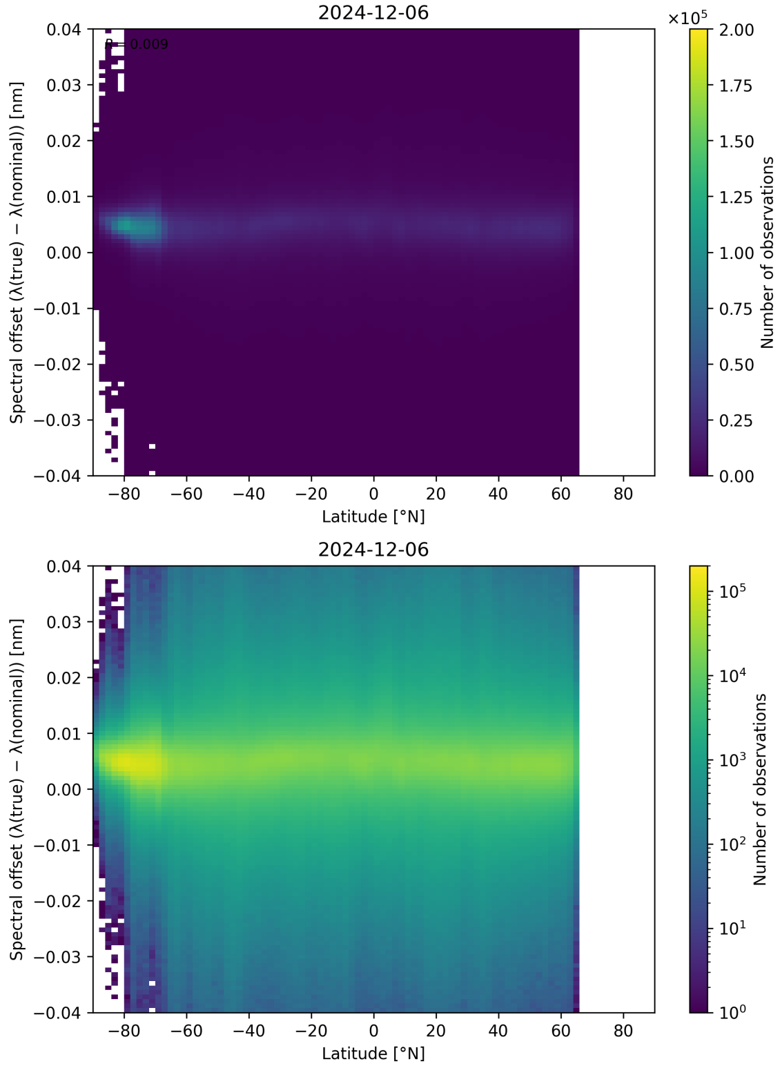
Figure 96: Scatter density plot of “Latitude” against “Spectral offset ( \lambda_{\text{true}} - \lambda_{\text{nominal}} )” for 2024-12-06 to 2024-12-07.
