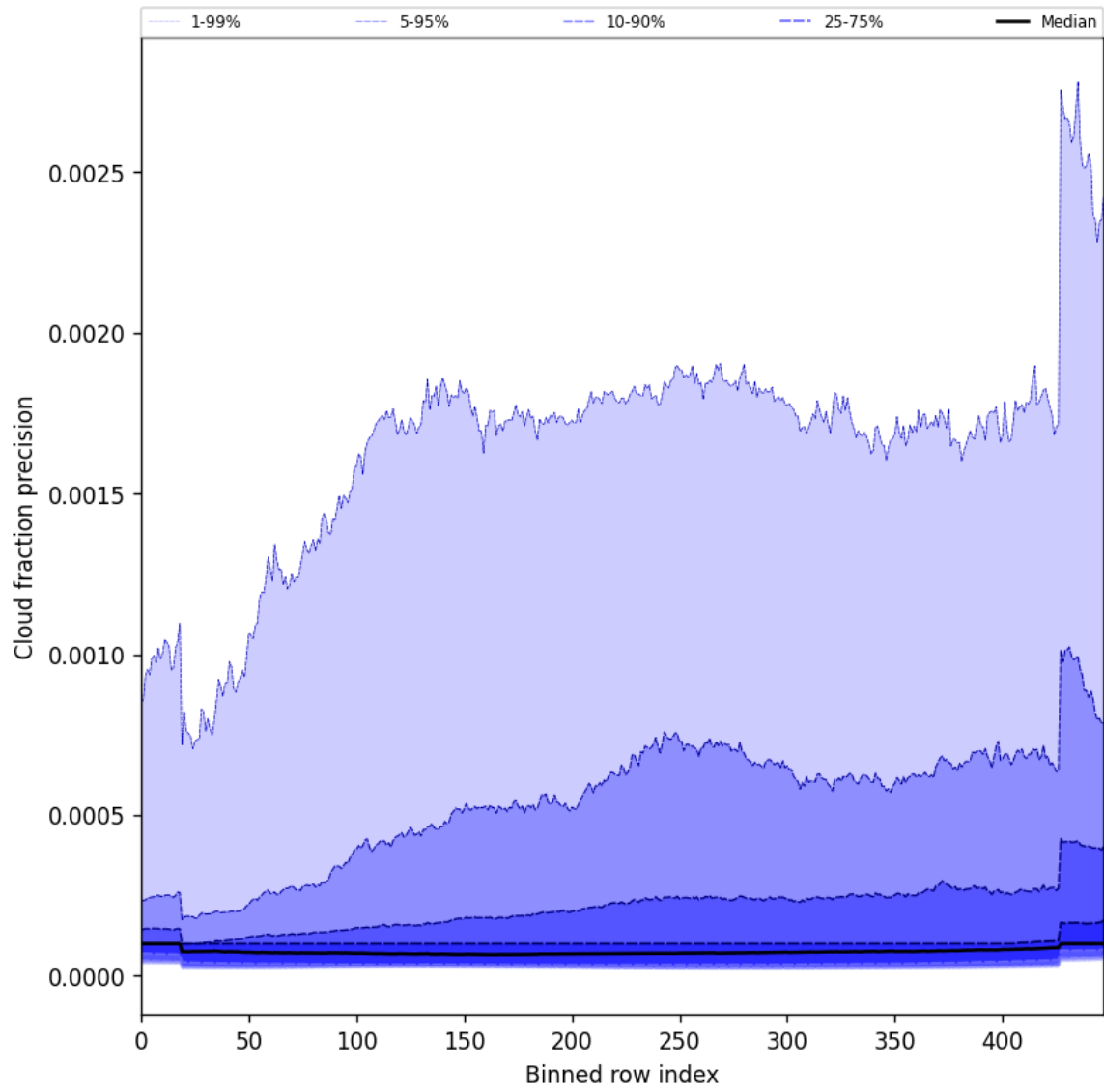
Figure 50: Along track statistics of “Cloud fraction precision” for 2024-12-06 to 2024-12-07
