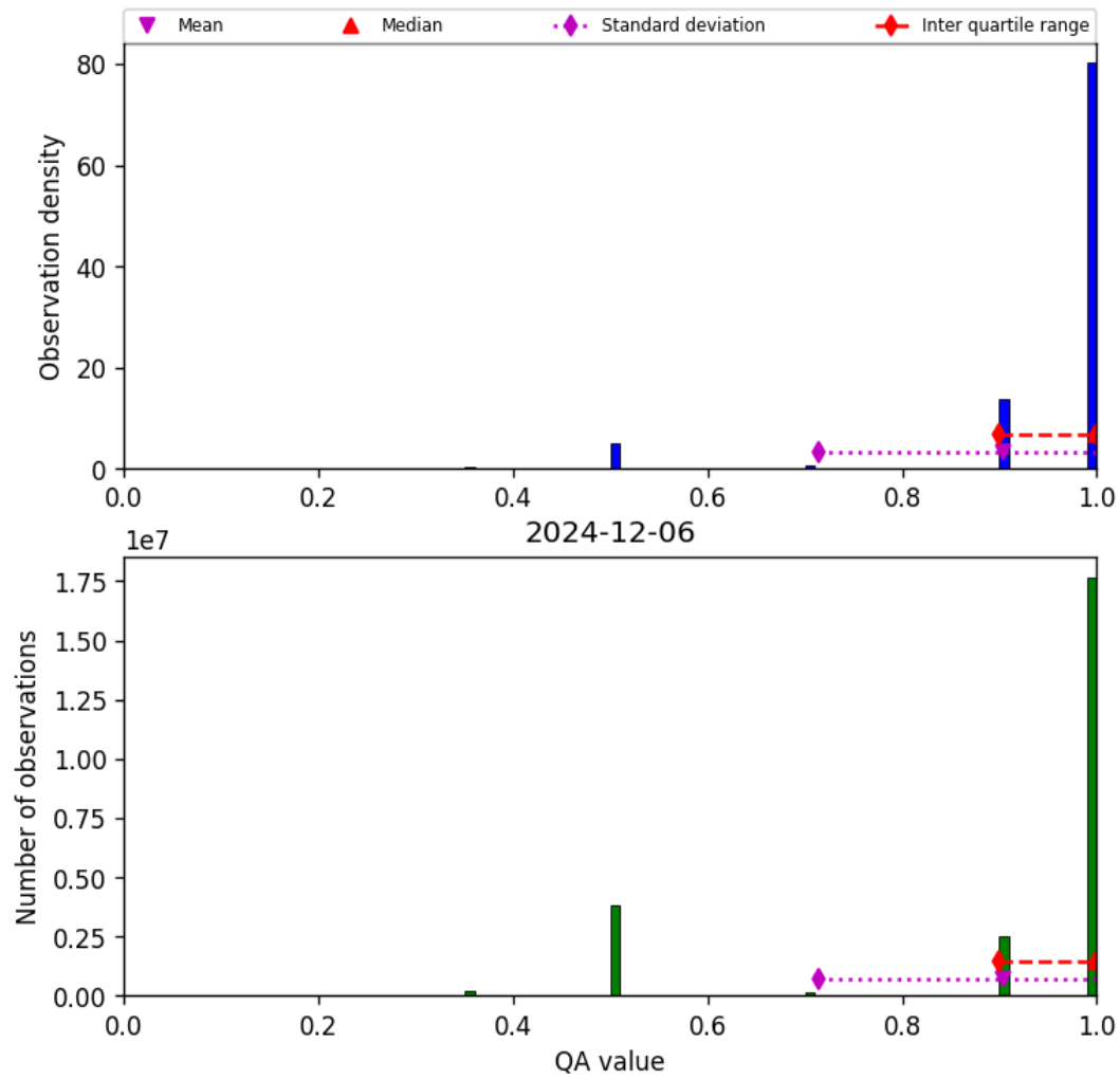
Figure 29: Histogram of “QA value” for 2024-12-06 to 2024-12-07
