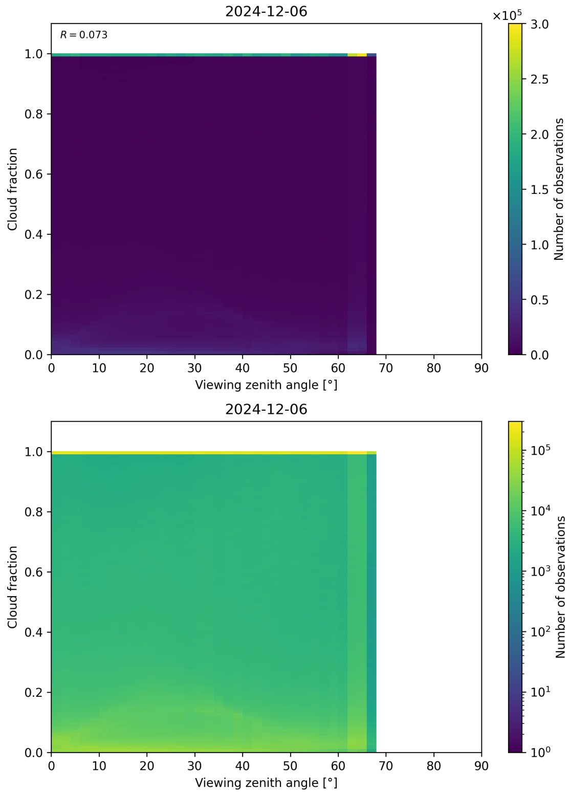
Figure 120: Scatter density plot of “Viewing zenith angle” against “Cloud fraction” for 2024-12-06 to 2024-12-07.
