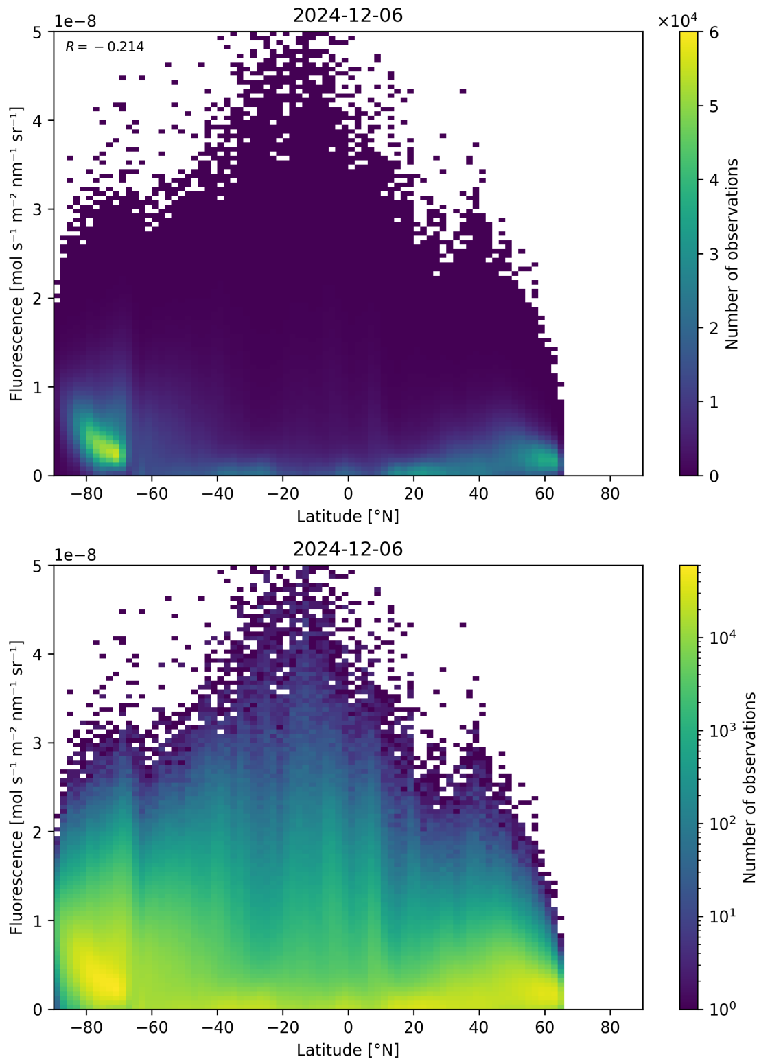
Figure 92: Scatter density plot of “Latitude” against “Fluorescence” for 2024-12-06 to 2024-12-07.
