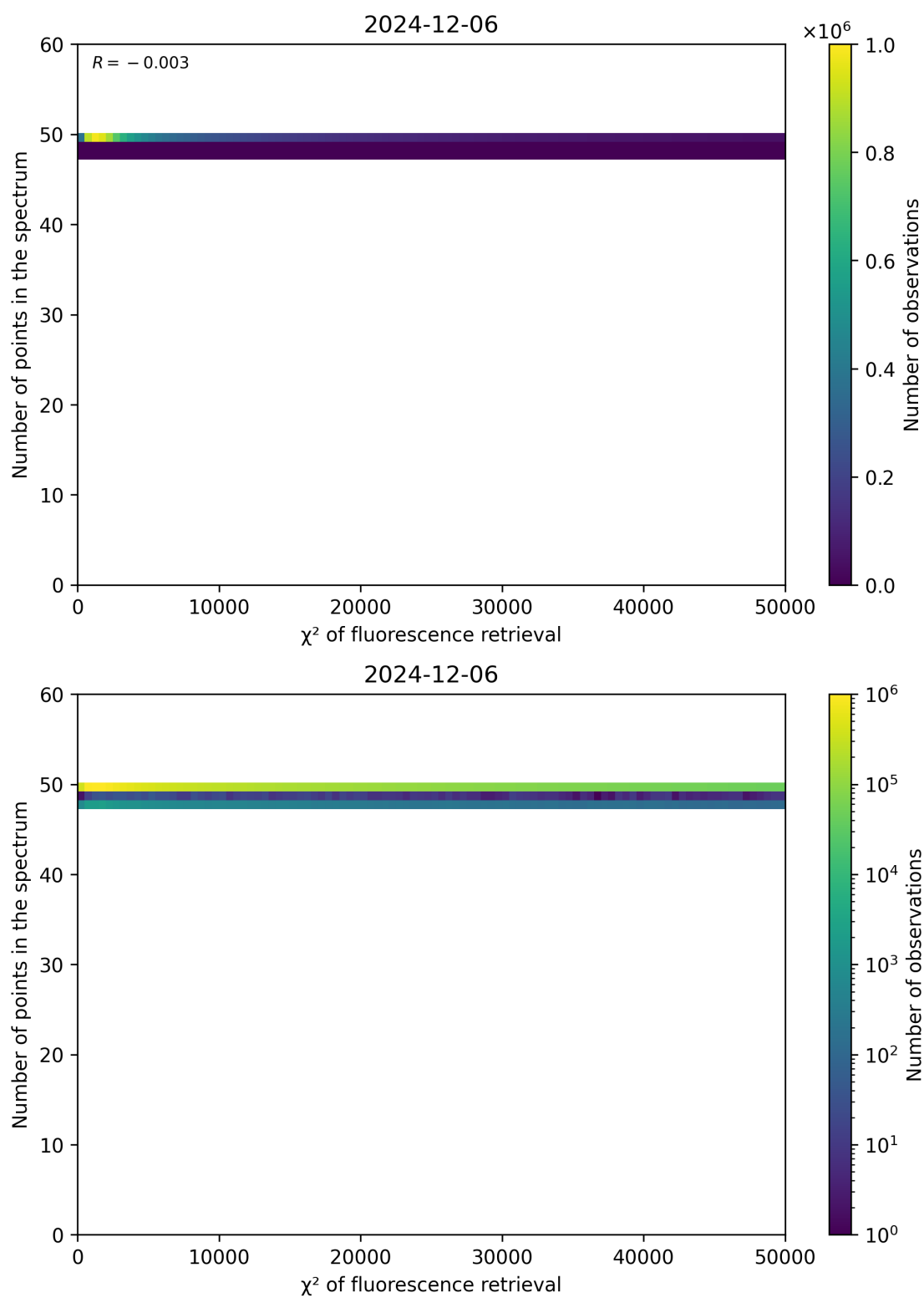
Figure 68: Scatter density plot of " \chi^2 of fluorescence retrieval" against "Number of points in the spectrum" for 2024-12-06 to 2024-12-07.
