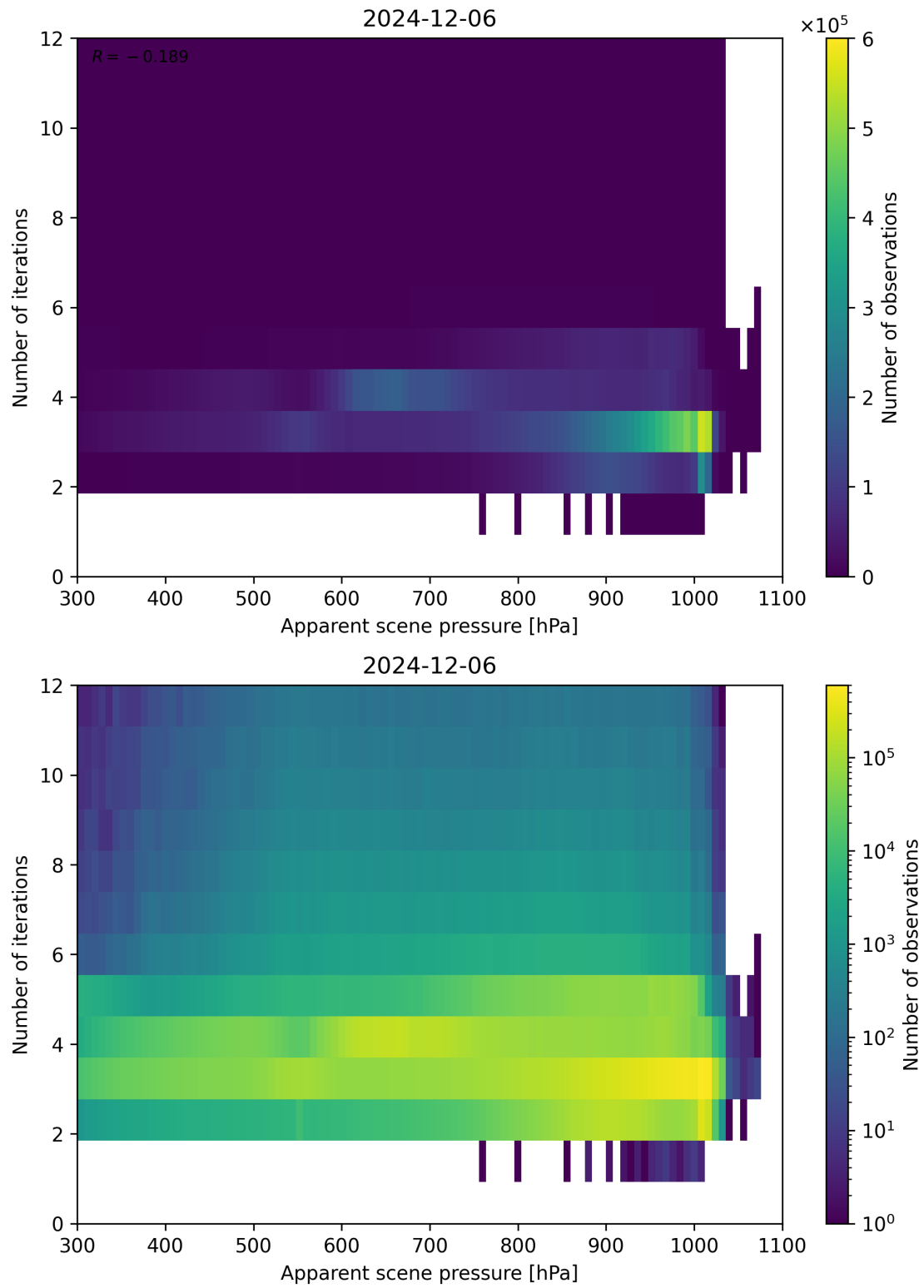
Figure 65: Scatter density plot of “Apparent scene pressure” against “Number of iterations” for 2024-12-06 to 2024-12-07.
