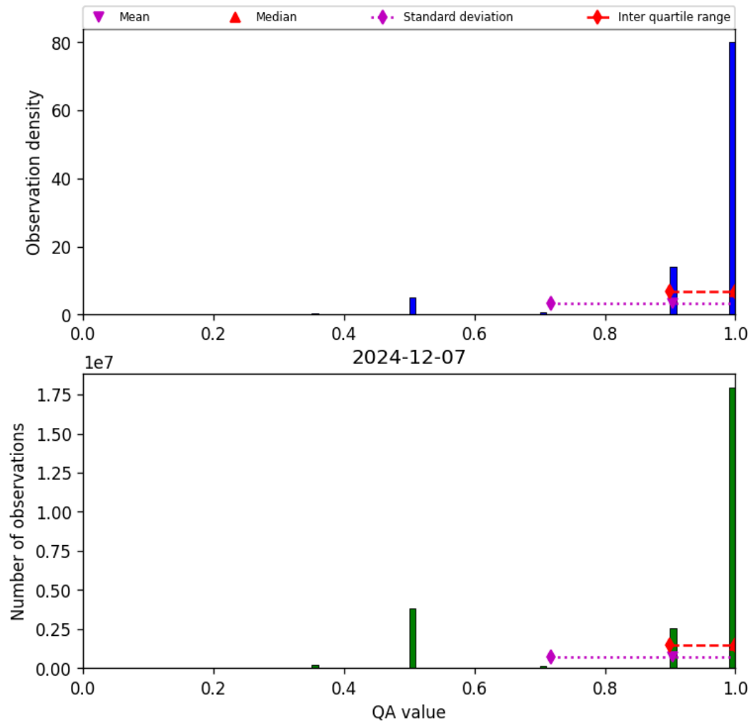
Figure 29: Histogram of “QA value” for 2024-12-06 to 2024-12-08
