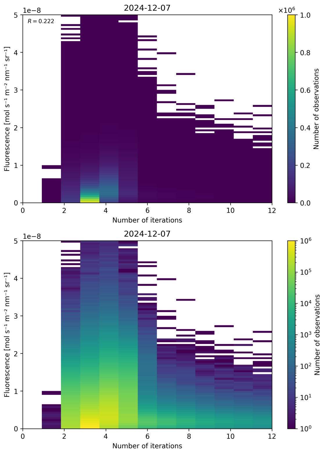
Figure 98: Scatter density plot of “Number of iterations” against “Fluorescence” for 2024-12-06 to 2024-12-08.
