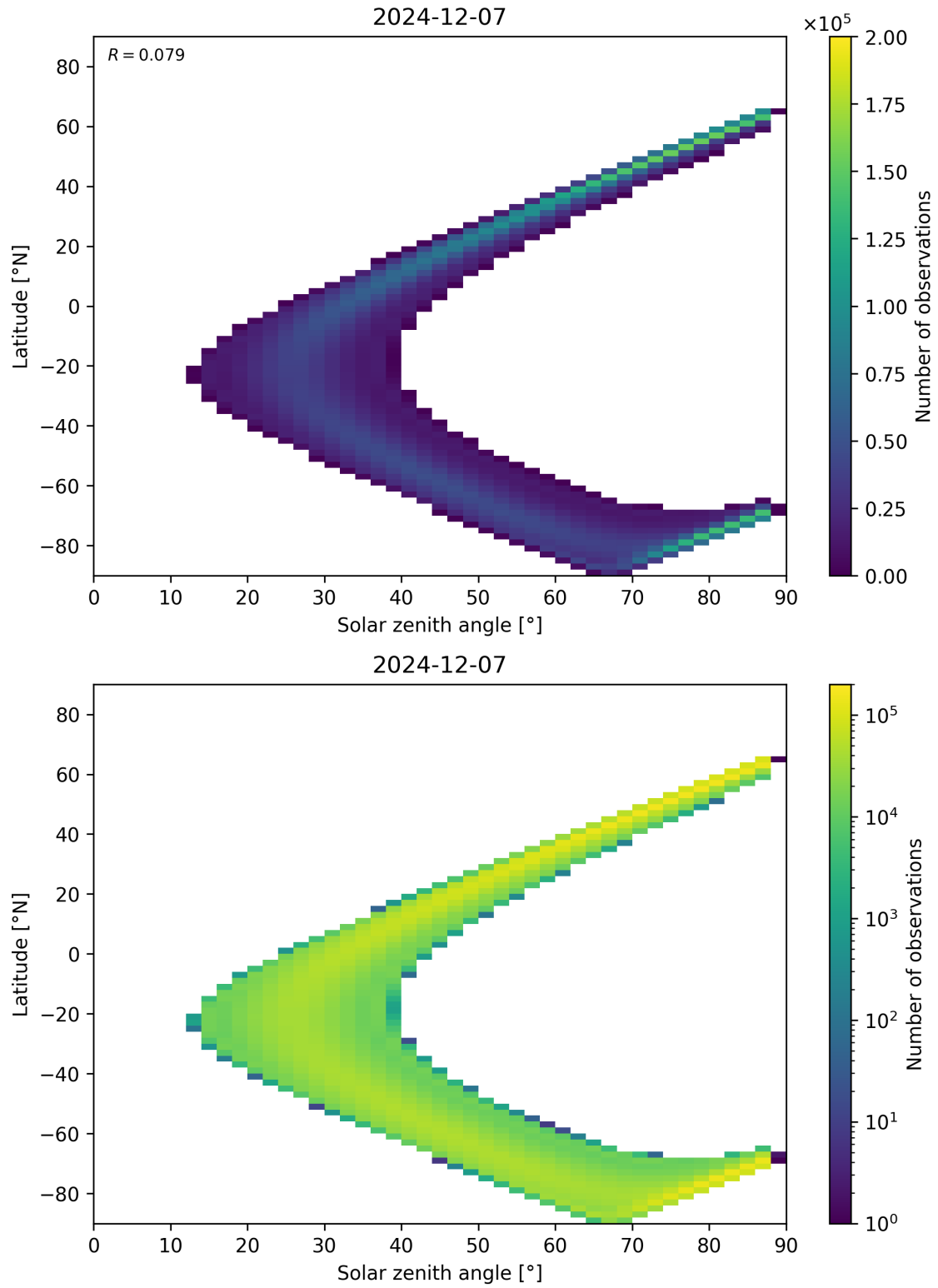
Figure 113: Scatter density plot of “Solar zenith angle” against “Latitude” for 2024-12-06 to 2024-12-08.
