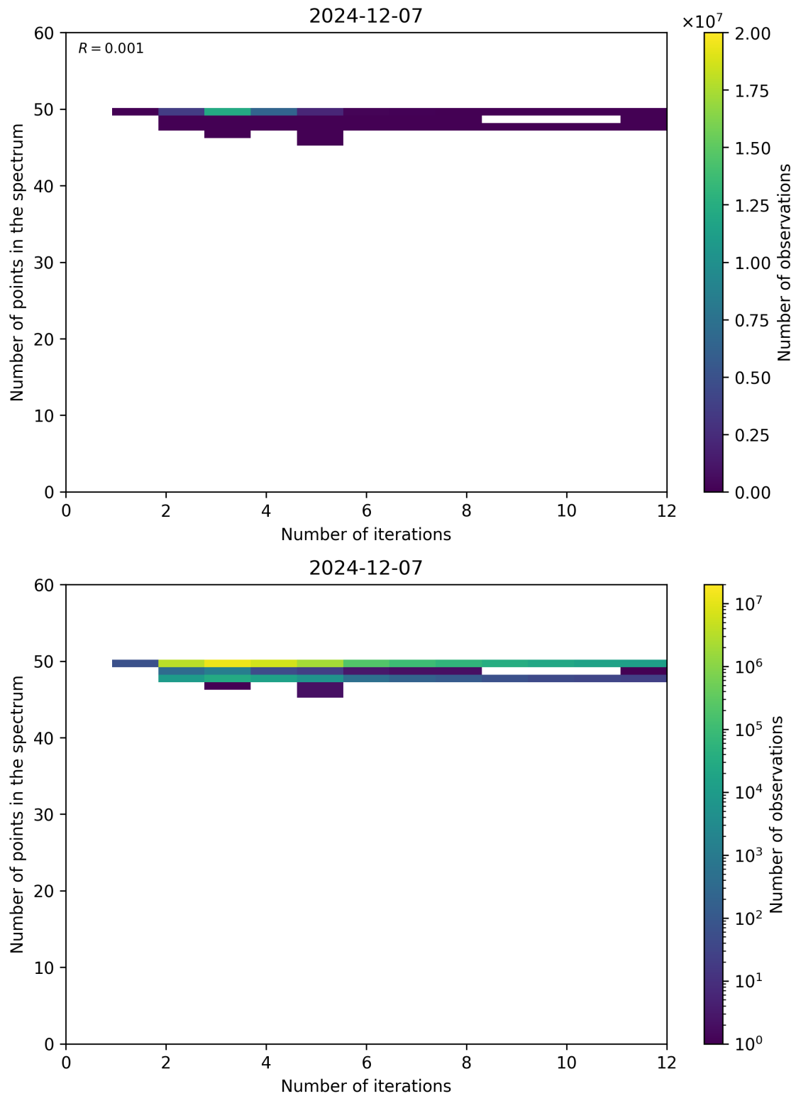
Figure 99: Scatter density plot of “Number of iterations” against “Number of points in the spectrum” for 2024-12-06 to 2024-12-08.
