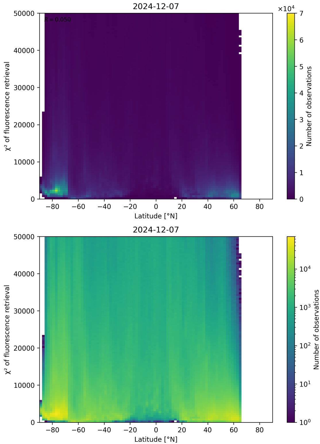
Figure 89: Scatter density plot of “Latitude” against “ \chi^2 of fluorescence retrieval” for 2024-12-06 to 2024-12-08.
