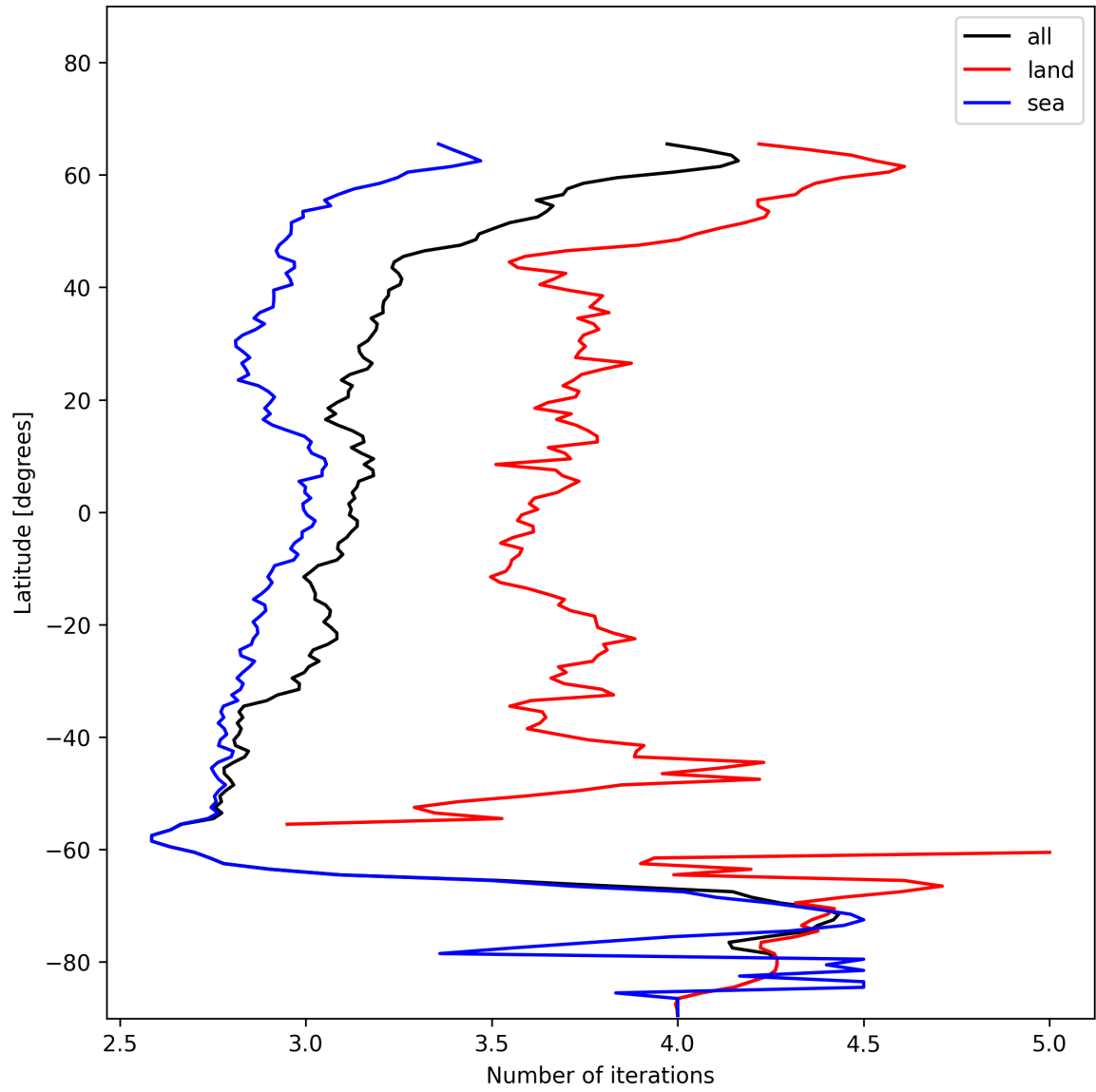
Figure 22: Zonal average of “Number of iterations” for 2024-12-06 to 2024-12-08.
