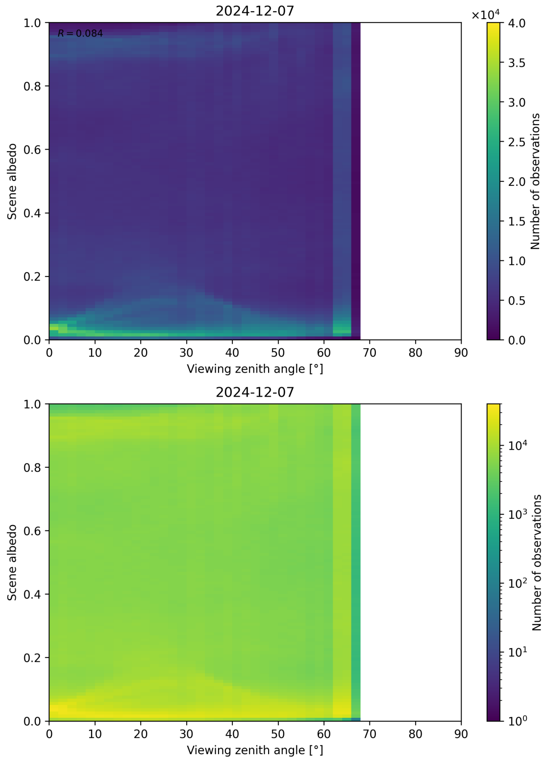
Figure 126: Scatter density plot of “Viewing zenith angle” against “Scene albedo” for 2024-12-06 to 2024-12-08.
