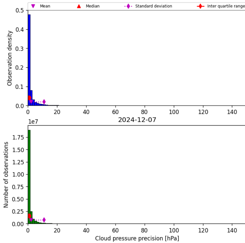
Figure 31: Histogram of “Cloud pressure precision” for 2024-12-06 to 2024-12-08
