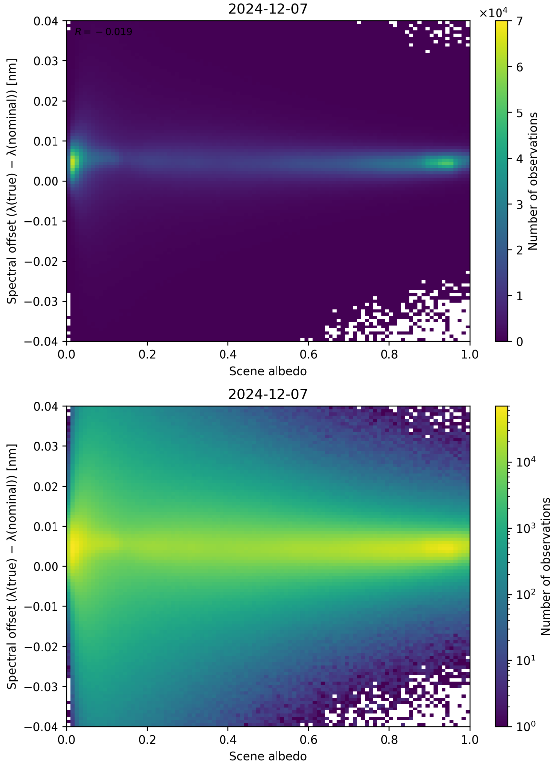
Figure 107: Scatter density plot of “Scene albedo” against “Spectral offset ( \lambda_{\text{true}} - \lambda_{\text{nominal}} )” for 2024-12-06 to 2024-12-08.
