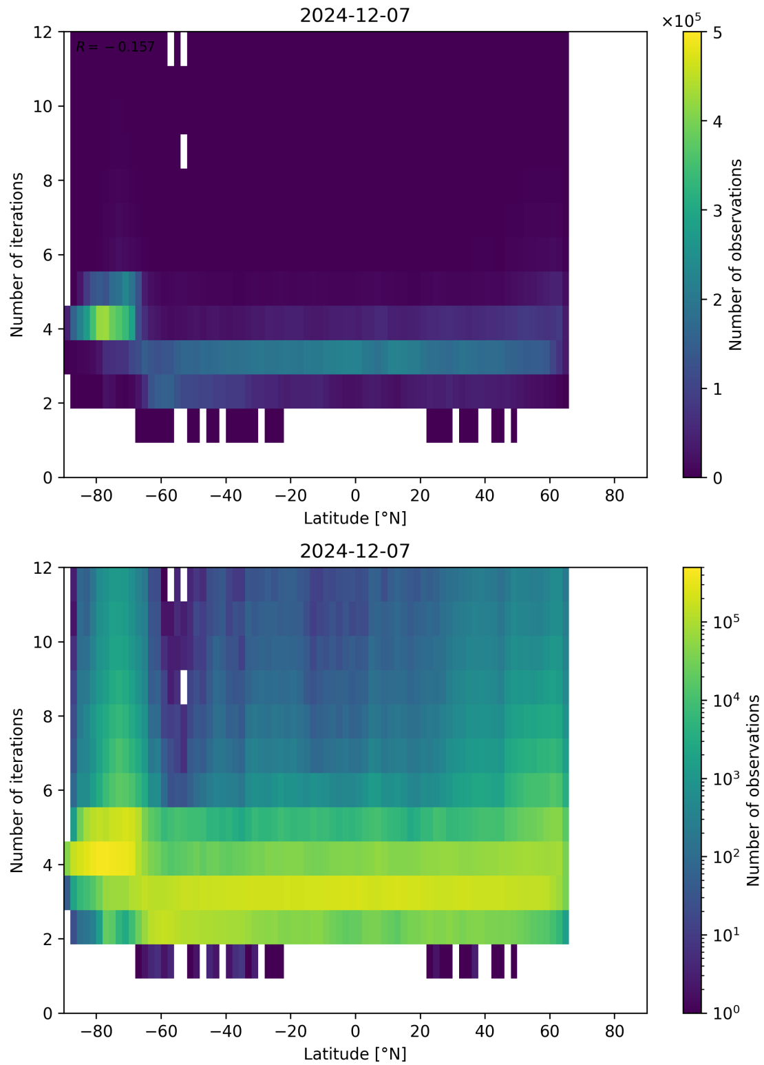
Figure 93: Scatter density plot of “Latitude” against “Number of iterations” for 2024-12-06 to 2024-12-08.
