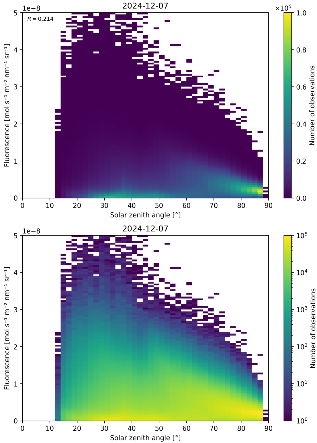
Figure 112: Scatter density plot of “Solar zenith angle” against “Fluorescence” for 2024-12-06 to 2024-12-08.
