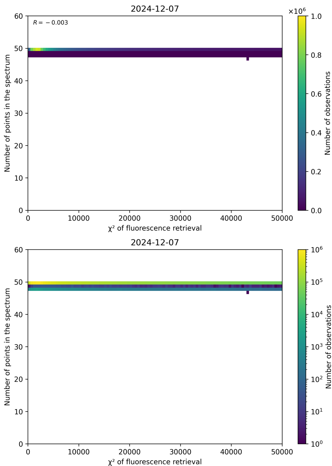
Figure 68: Scatter density plot of " \chi^2 of fluorescence retrieval" against "Number of points in the spectrum" for 2024-12-06 to 2024-12-08.
