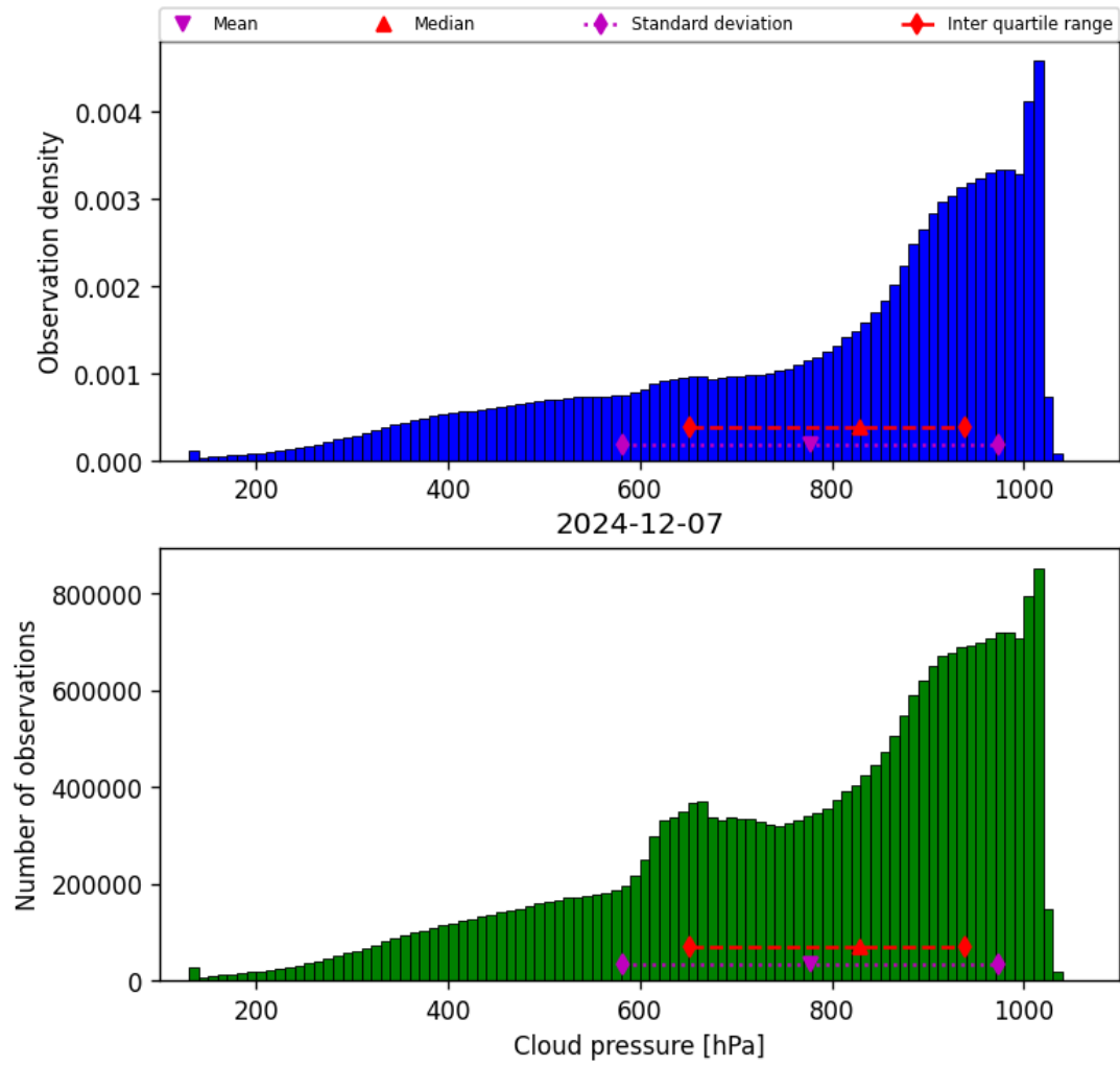
Figure 30: Histogram of “Cloud pressure” for 2024-12-06 to 2024-12-08
