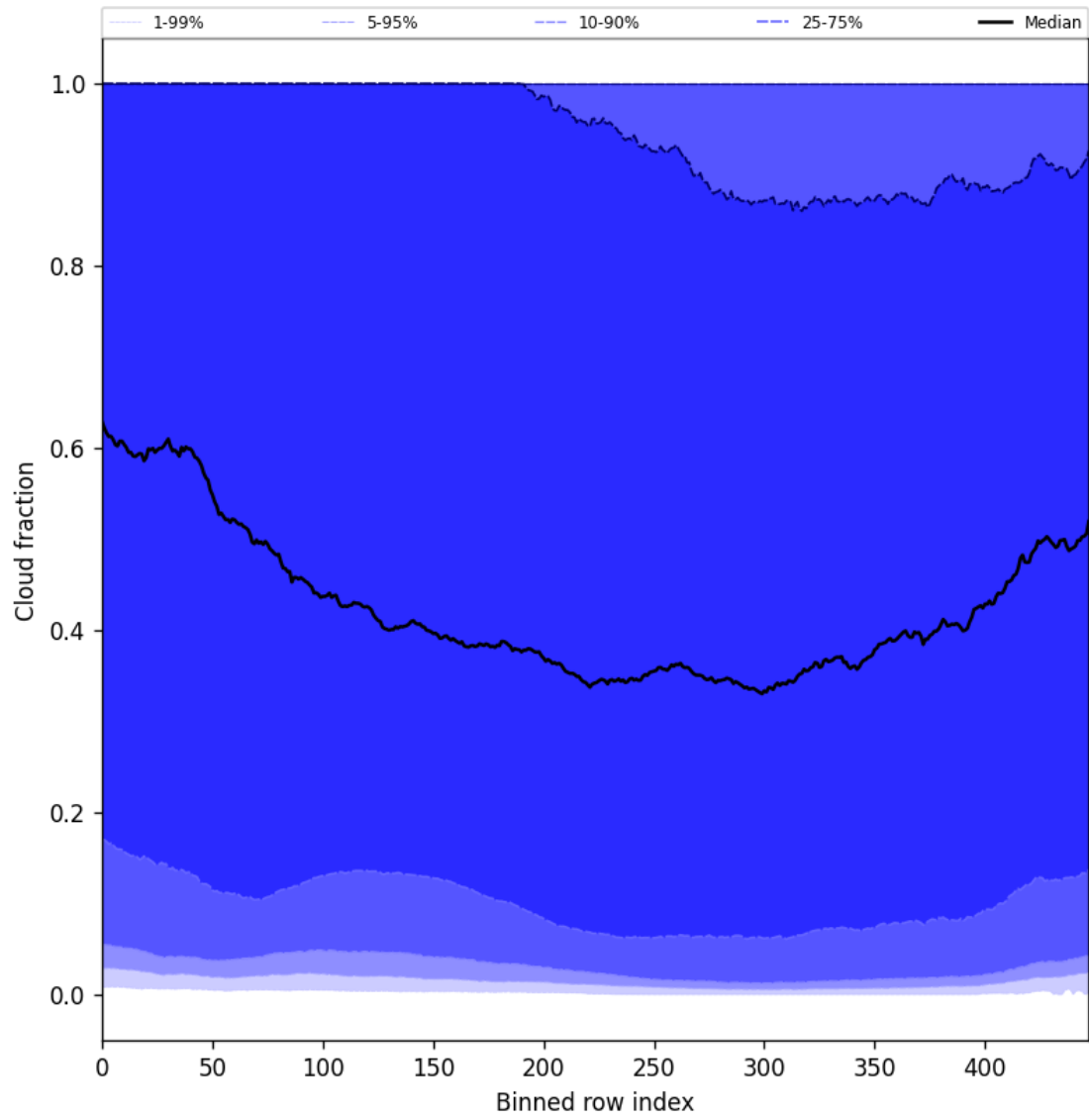
Figure 49: Along track statistics of “Cloud fraction” for 2024-12-06 to 2024-12-08
