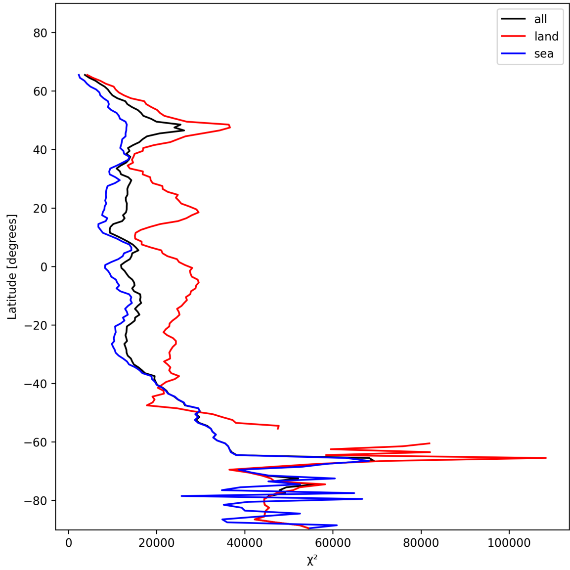
Figure 21: Zonal average of “ \chi^2 ” for 2024-12-06 to 2024-12-08.
