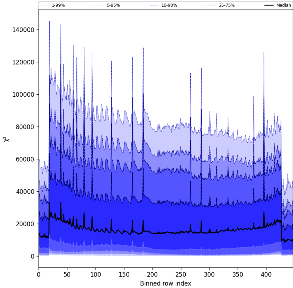
Figure 55: Along track statistics of “ \chi^2 ” for 2024-12-06 to 2024-12-08
