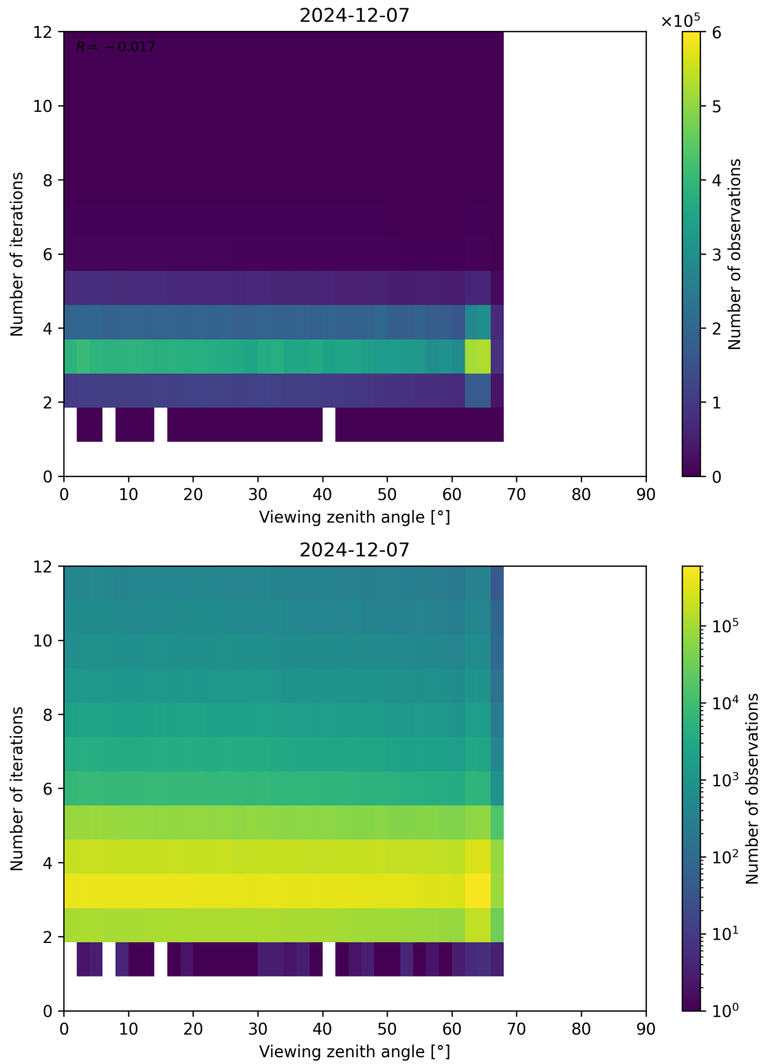
Figure 124: Scatter density plot of “Viewing zenith angle” against “Number of iterations” for 2024-12-06 to 2024-12-08.
