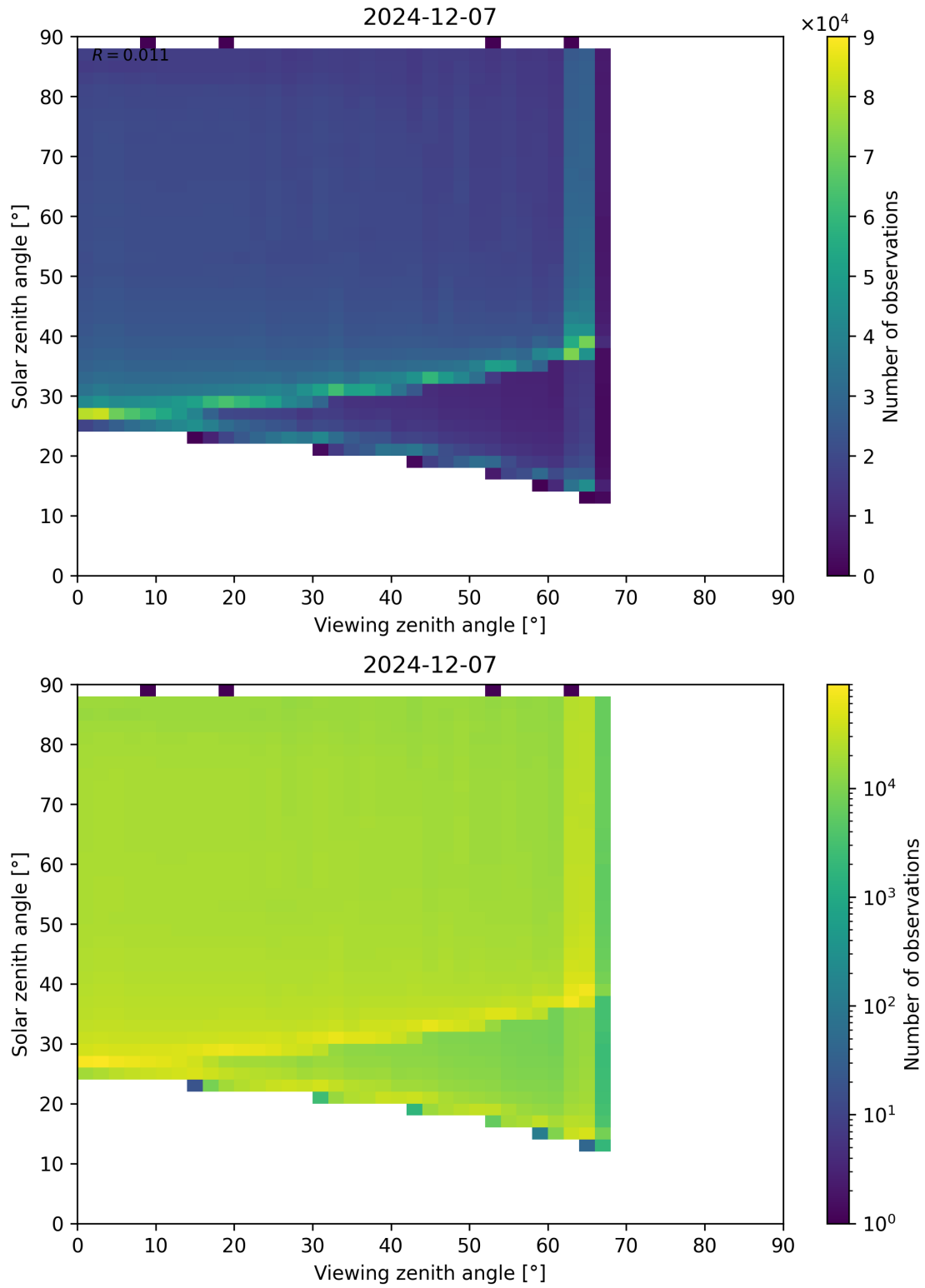
Figure 127: Scatter density plot of “Viewing zenith angle” against “Solar zenith angle” for 2024-12-06 to 2024-12-08.
