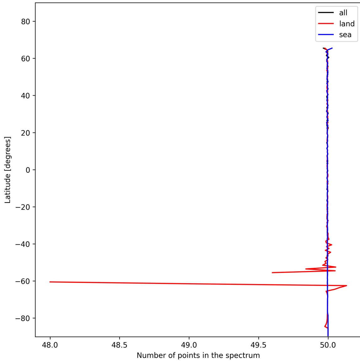
Figure 27: Zonal average of “Number of points in the spectrum” for 2024-12-06 to 2024-12-08.
