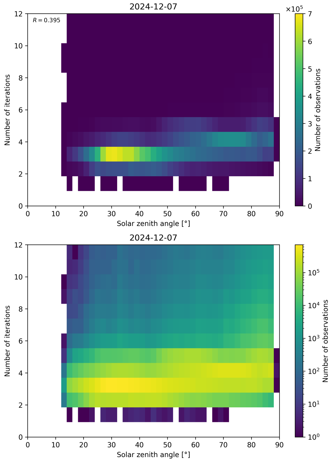
Figure 114: Scatter density plot of “Solar zenith angle” against “Number of iterations” for 2024-12-06 to 2024-12-08.
