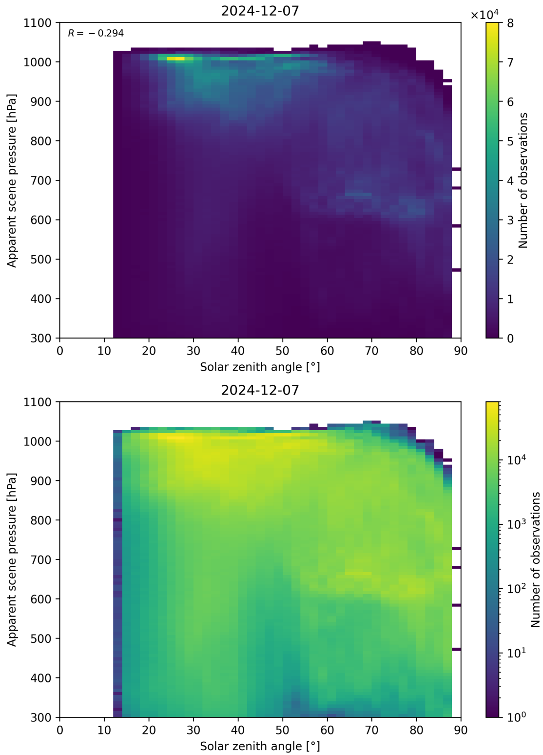
Figure 108: Scatter density plot of “Solar zenith angle” against “Apparent scene pressure” for 2024-12-06 to 2024-12-08.
