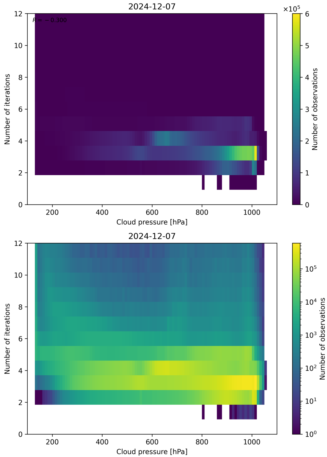
Figure 81: Scatter density plot of “Cloud pressure” against “Number of iterations” for 2024-12-06 to 2024-12-08.
