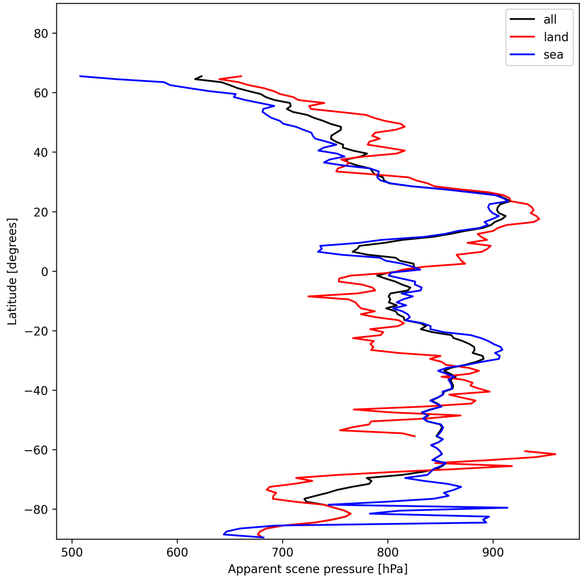
Figure 19: Zonal average of “Apparent scene pressure” for 2024-12-06 to 2024-12-08.
