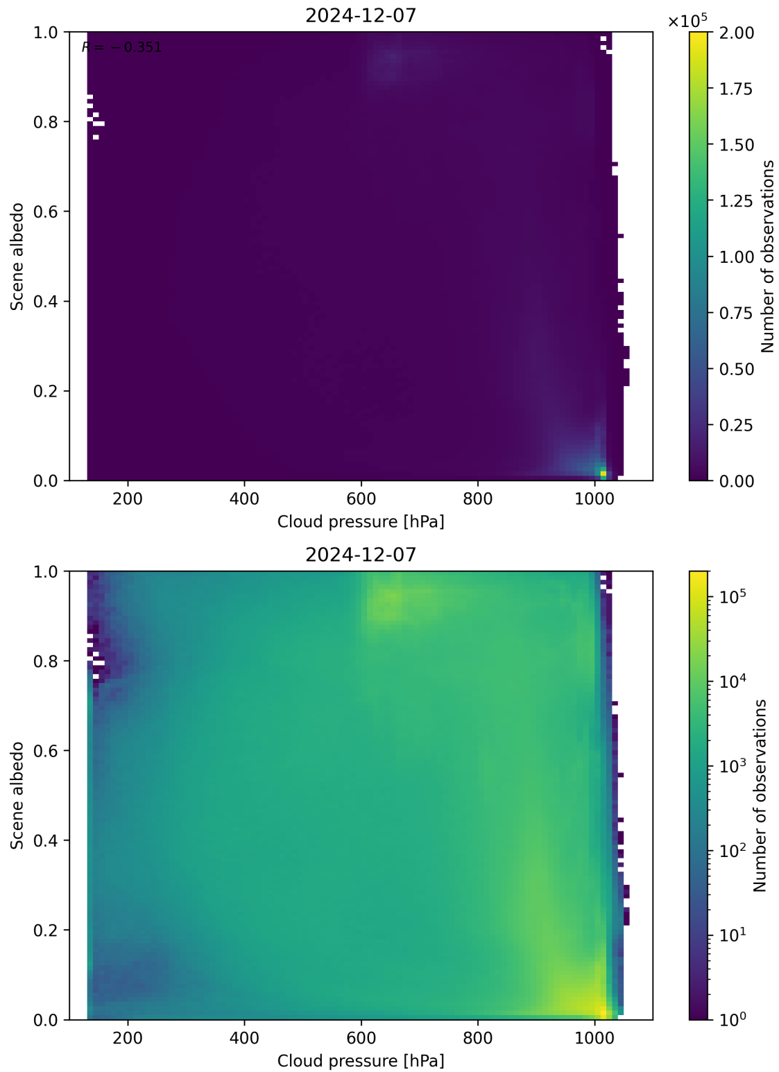
Figure 83: Scatter density plot of “Cloud pressure” against “Scene albedo” for 2024-12-06 to 2024-12-08.
