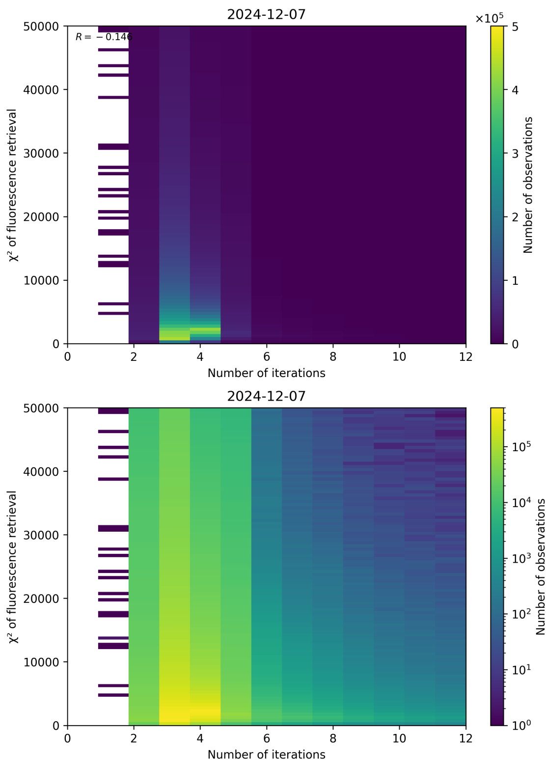
Figure 97: Scatter density plot of “Number of iterations” against “ \chi^2 of fluorescence retrieval” for 2024-12-06 to 2024-12-08.
