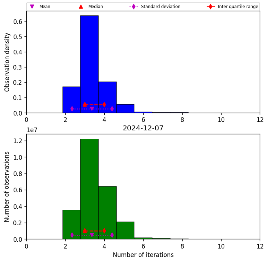
Figure 39: Histogram of “Number of iterations” for 2024-12-06 to 2024-12-08
