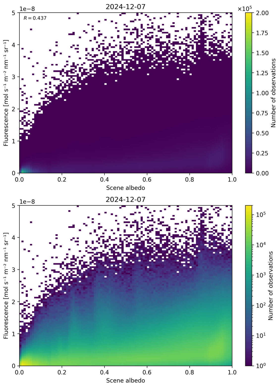
Figure 104: Scatter density plot of “Scene albedo” against “Fluorescence” for 2024-12-06 to 2024-12-08.
