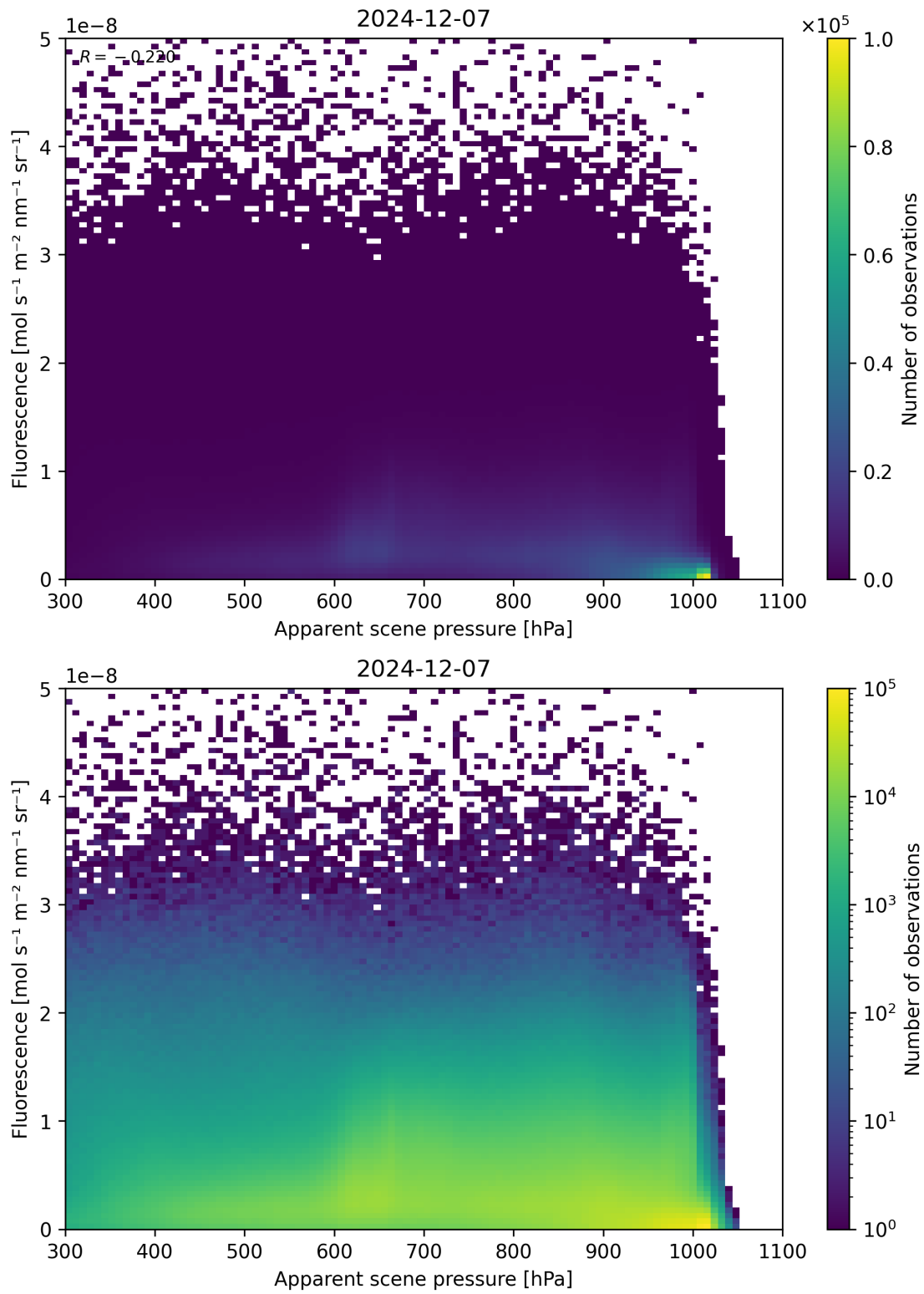
Figure 64: Scatter density plot of “Apparent scene pressure” against “Fluorescence” for 2024-12-06 to 2024-12-08.
