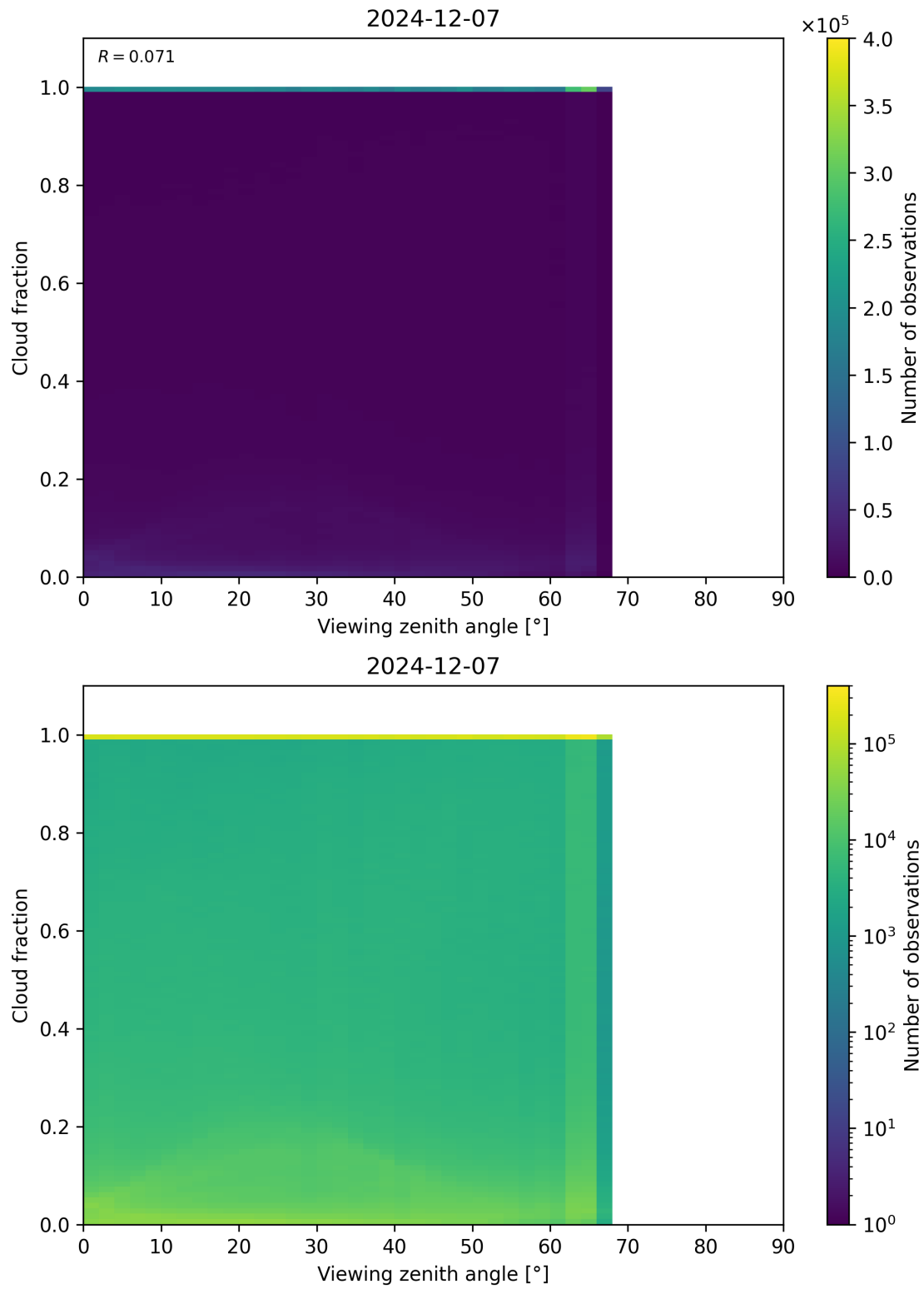
Figure 120: Scatter density plot of “Viewing zenith angle” against “Cloud fraction” for 2024-12-06 to 2024-12-08.
