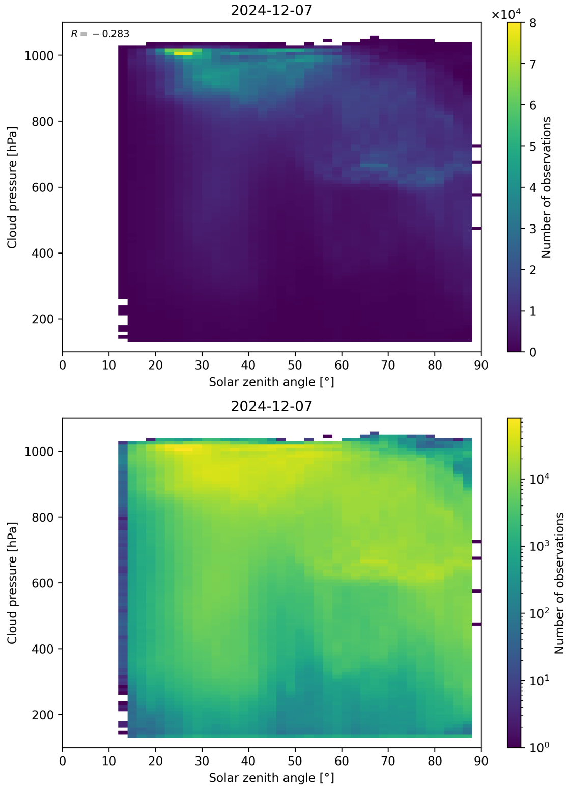
Figure 111: Scatter density plot of “Solar zenith angle” against “Cloud pressure” for 2024-12-06 to 2024-12-08.
