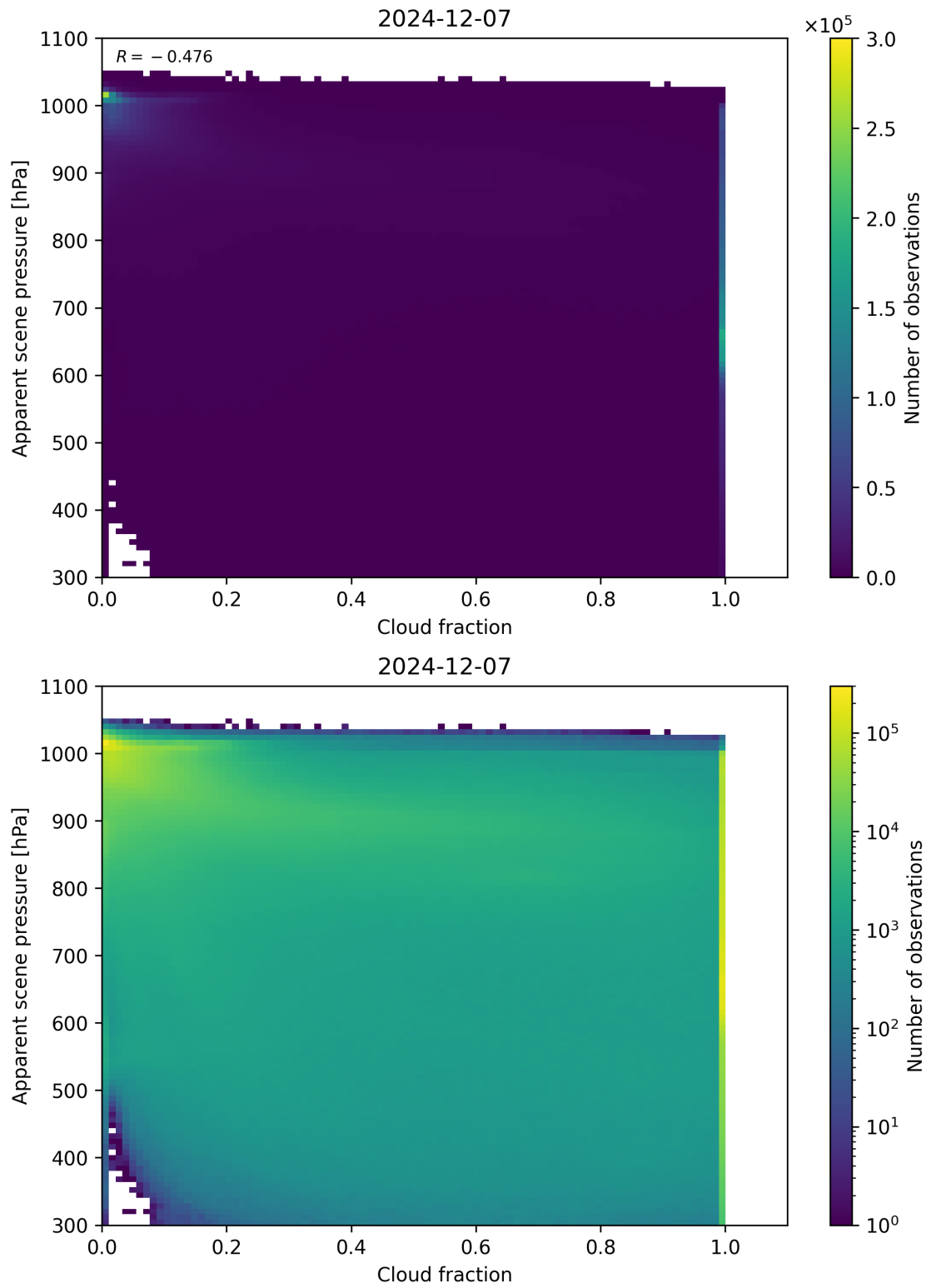
Figure 70: Scatter density plot of “Cloud fraction” against “Apparent scene pressure” for 2024-12-06 to 2024-12-08.
