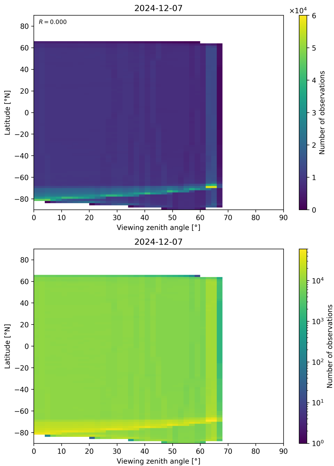
Figure 123: Scatter density plot of “Viewing zenith angle” against “Latitude” for 2024-12-06 to 2024-12-08.
