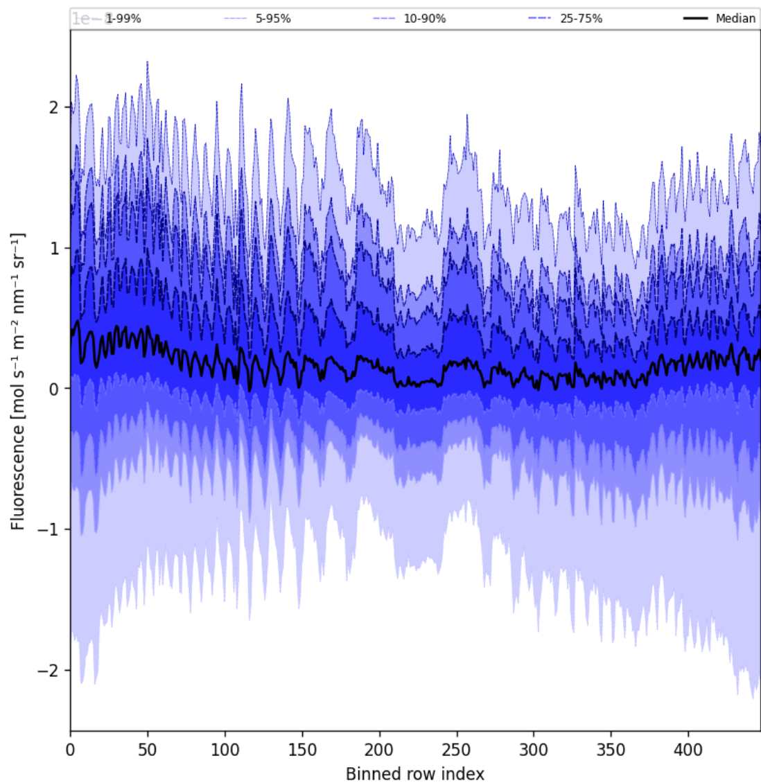
Figure 57: Along track statistics of “Fluorescence” for 2024-12-06 to 2024-12-08
