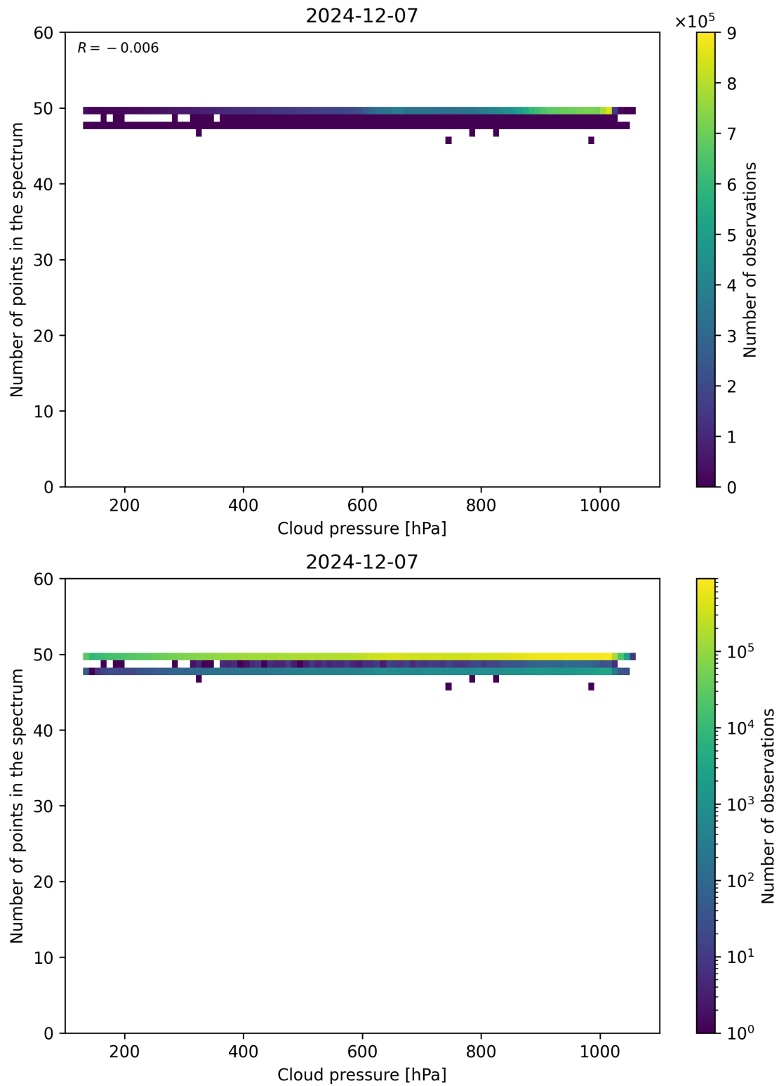
Figure 82: Scatter density plot of “Cloud pressure” against “Number of points in the spectrum” for 2024-12-06 to 2024-12-08.
