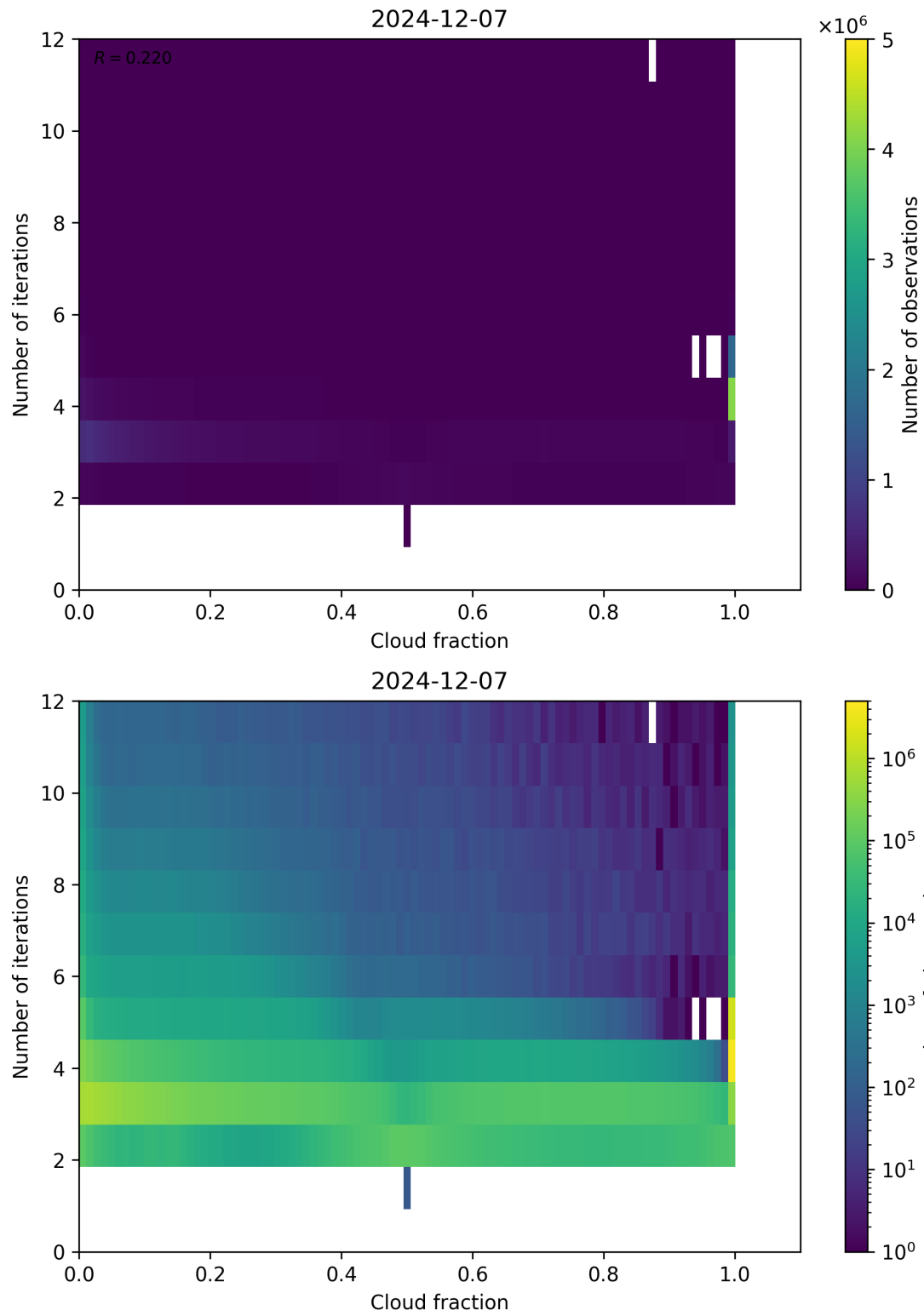
Figure 73: Scatter density plot of “Cloud fraction” against “Number of iterations” for 2024-12-06 to 2024-12-08.
