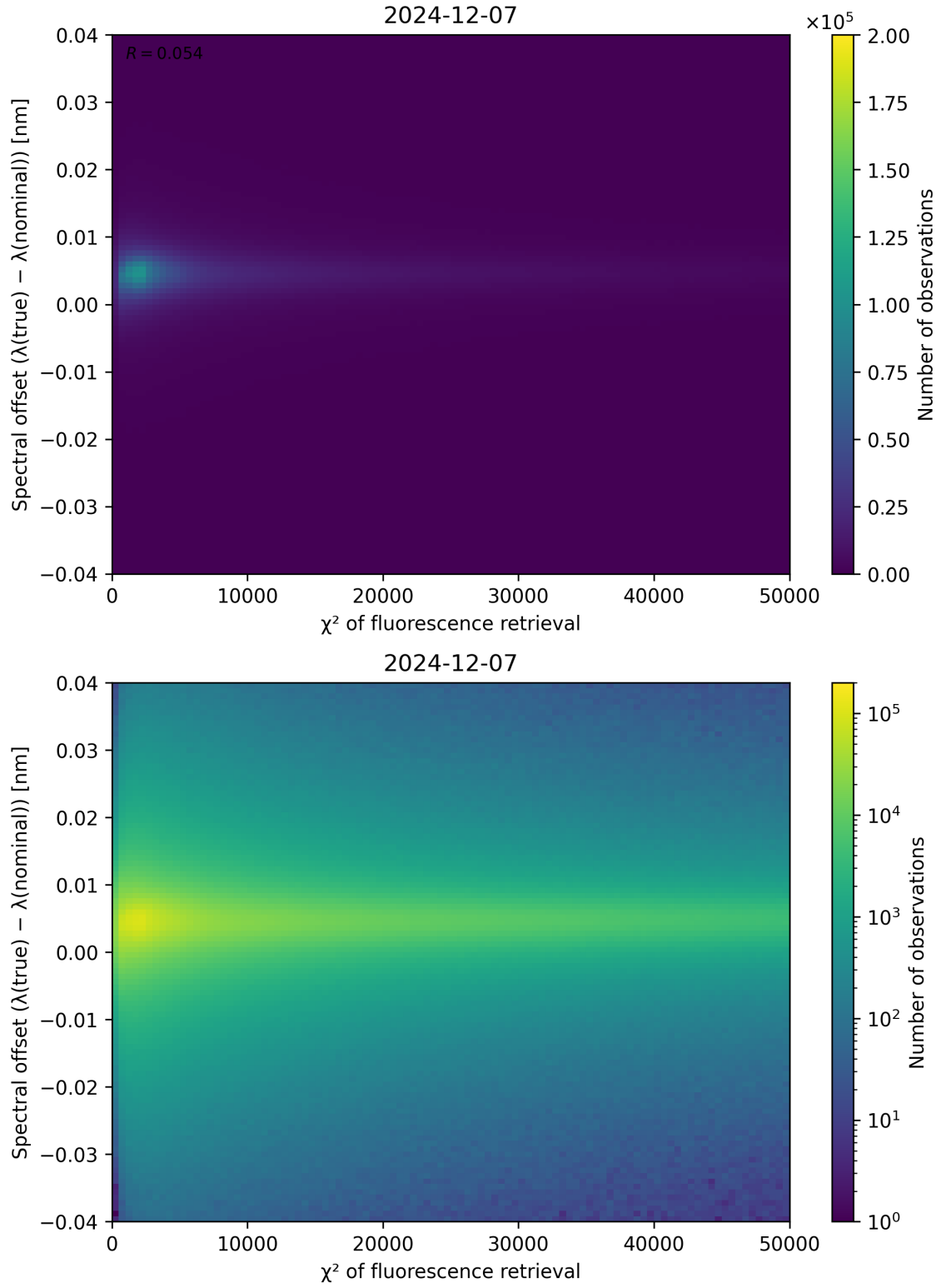
Figure 69: Scatter density plot of “ \chi^2 of fluorescence retrieval” against “Spectral offset ( \lambda_{\text{true}} - \lambda_{\text{nominal}} )” for 2024-12-06 to 2024-12-08.
