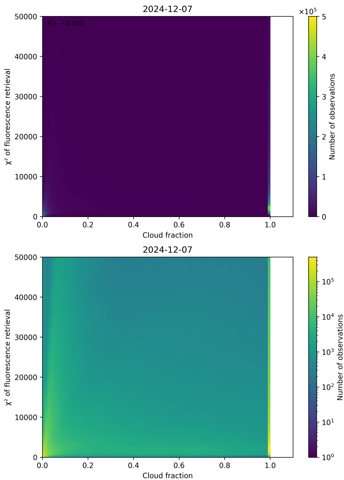
Figure 71: Scatter density plot of “Cloud fraction” against “ \chi^2 of fluorescence retrieval” for 2024-12-06 to 2024-12-08.
