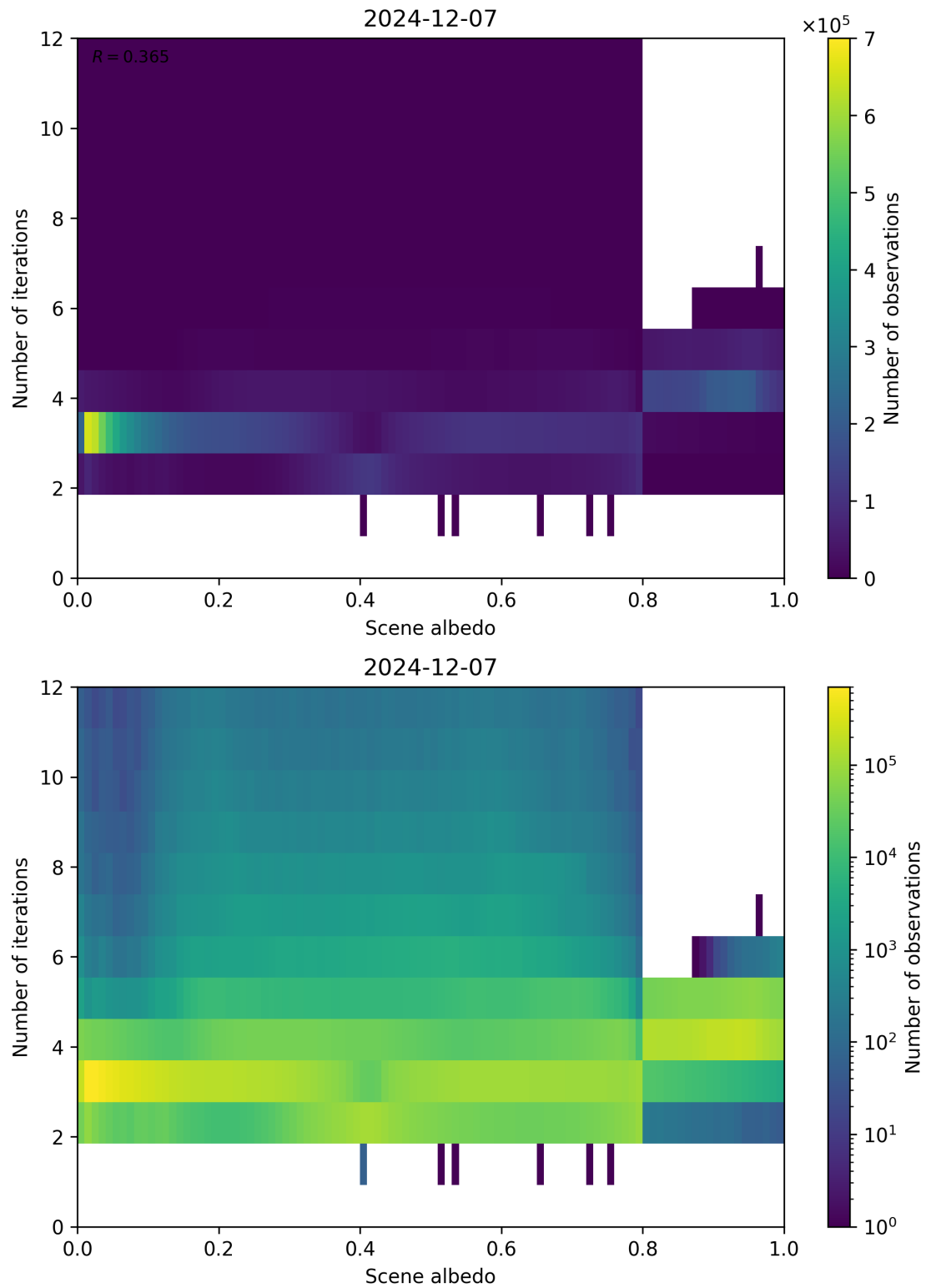
Figure 105: Scatter density plot of “Scene albedo” against “Number of iterations” for 2024-12-06 to 2024-12-08.
