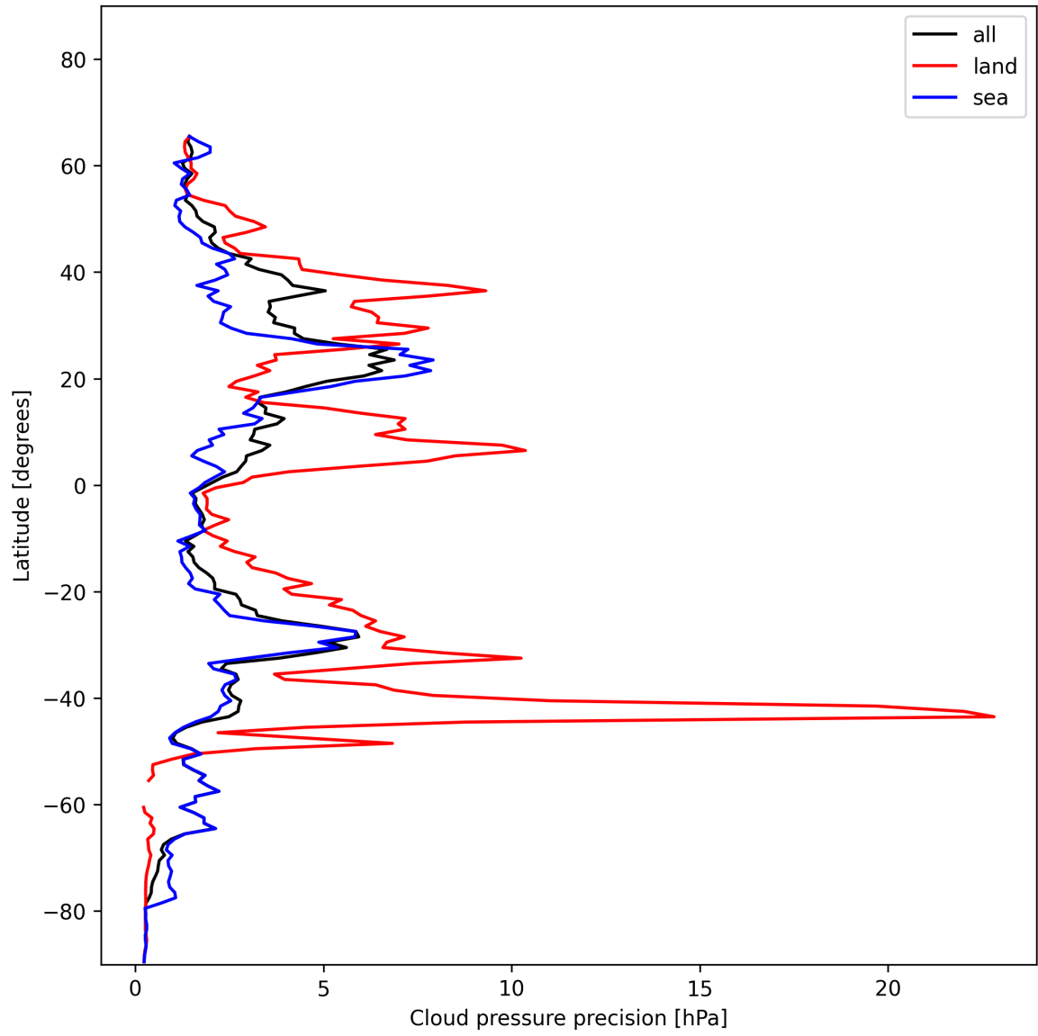
Figure 14: Zonal average of “Cloud pressure precision” for 2024-12-06 to 2024-12-08.
