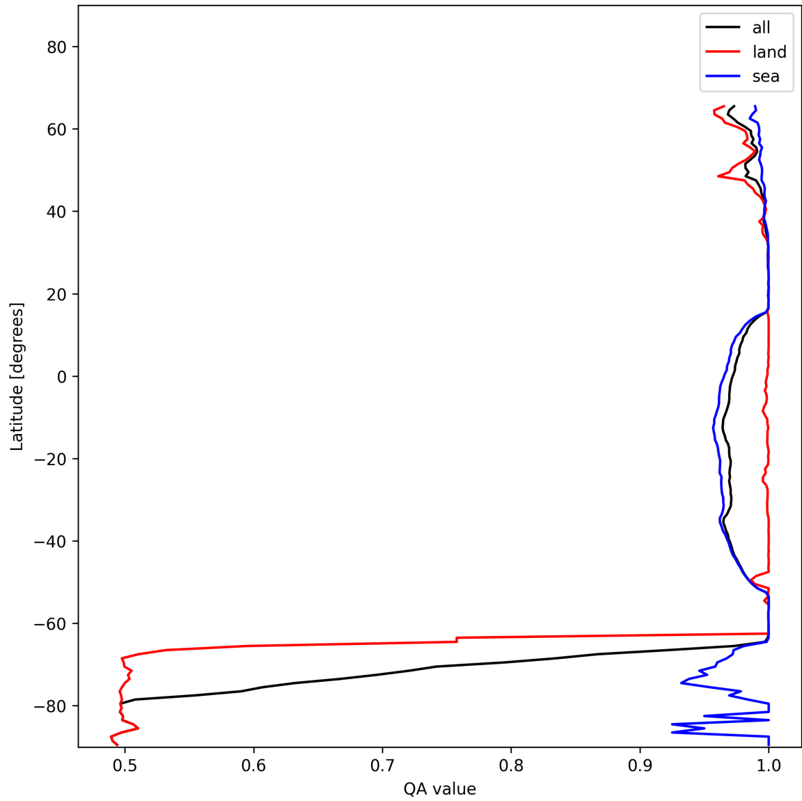
Figure 12: Zonal average of “QA value” for 2024-12-06 to 2024-12-08.
