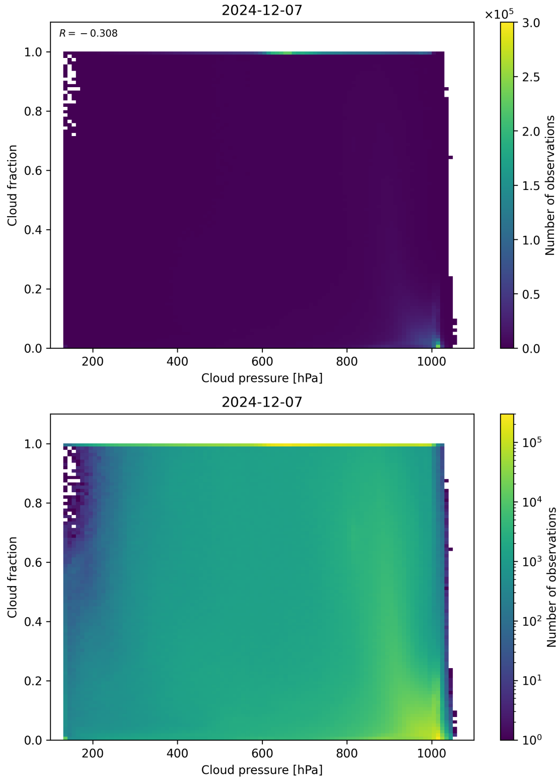
Figure 79: Scatter density plot of “Cloud pressure” against “Cloud fraction” for 2024-12-06 to 2024-12-08.
