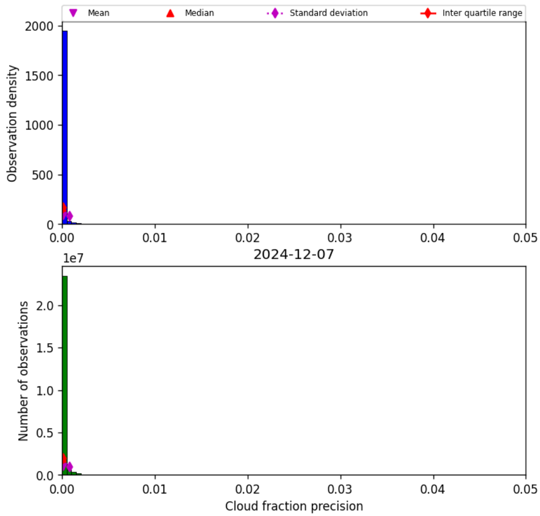
Figure 33: Histogram of “Cloud fraction precision” for 2024-12-06 to 2024-12-08
