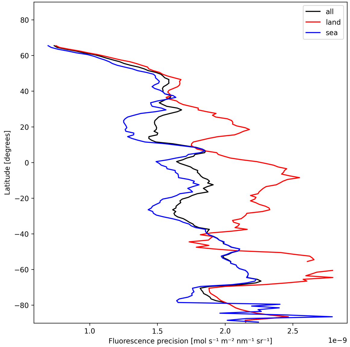
Figure 24: Zonal average of “Fluorescence precision” for 2024-12-06 to 2024-12-08.
