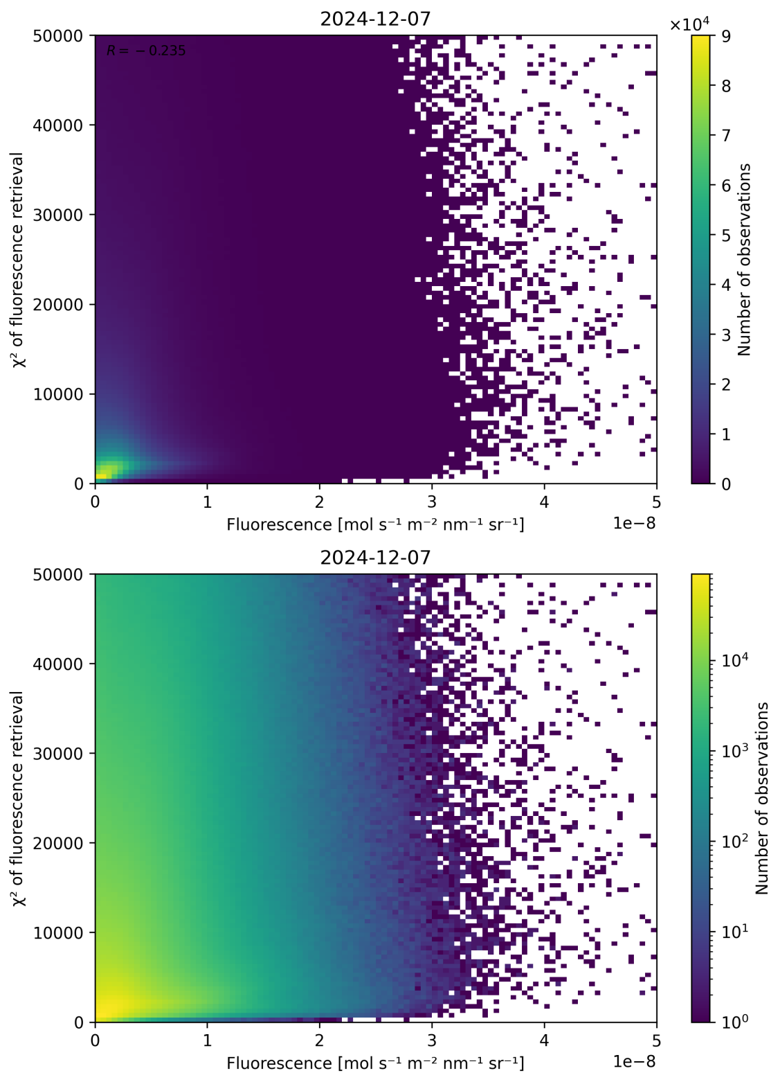
Figure 85: Scatter density plot of “Fluorescence” against “ \chi^2 of fluorescence retrieval” for 2024-12-06 to 2024-12-08.
