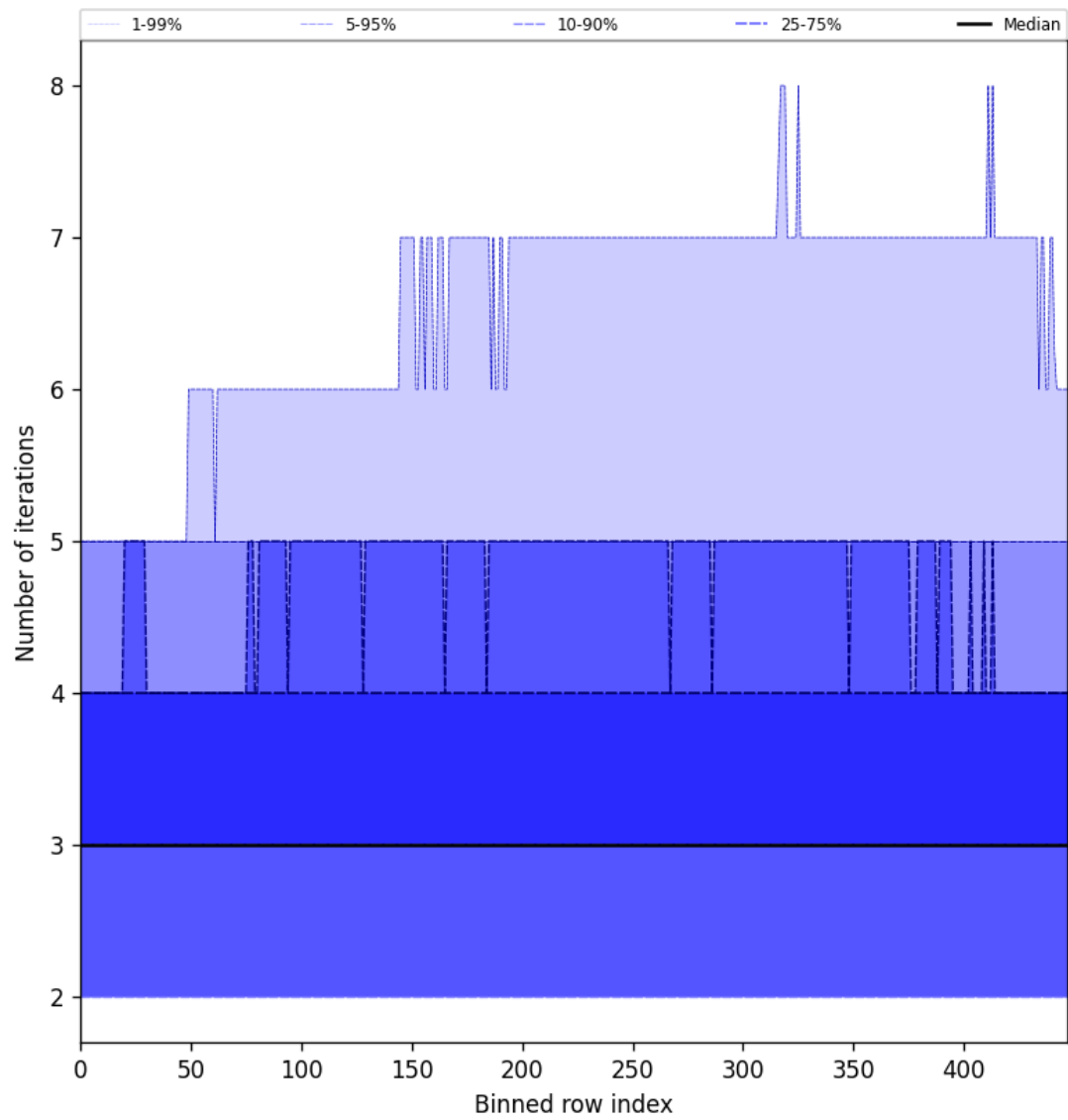
Figure 56: Along track statistics of “Number of iterations” for 2024-12-06 to 2024-12-08
