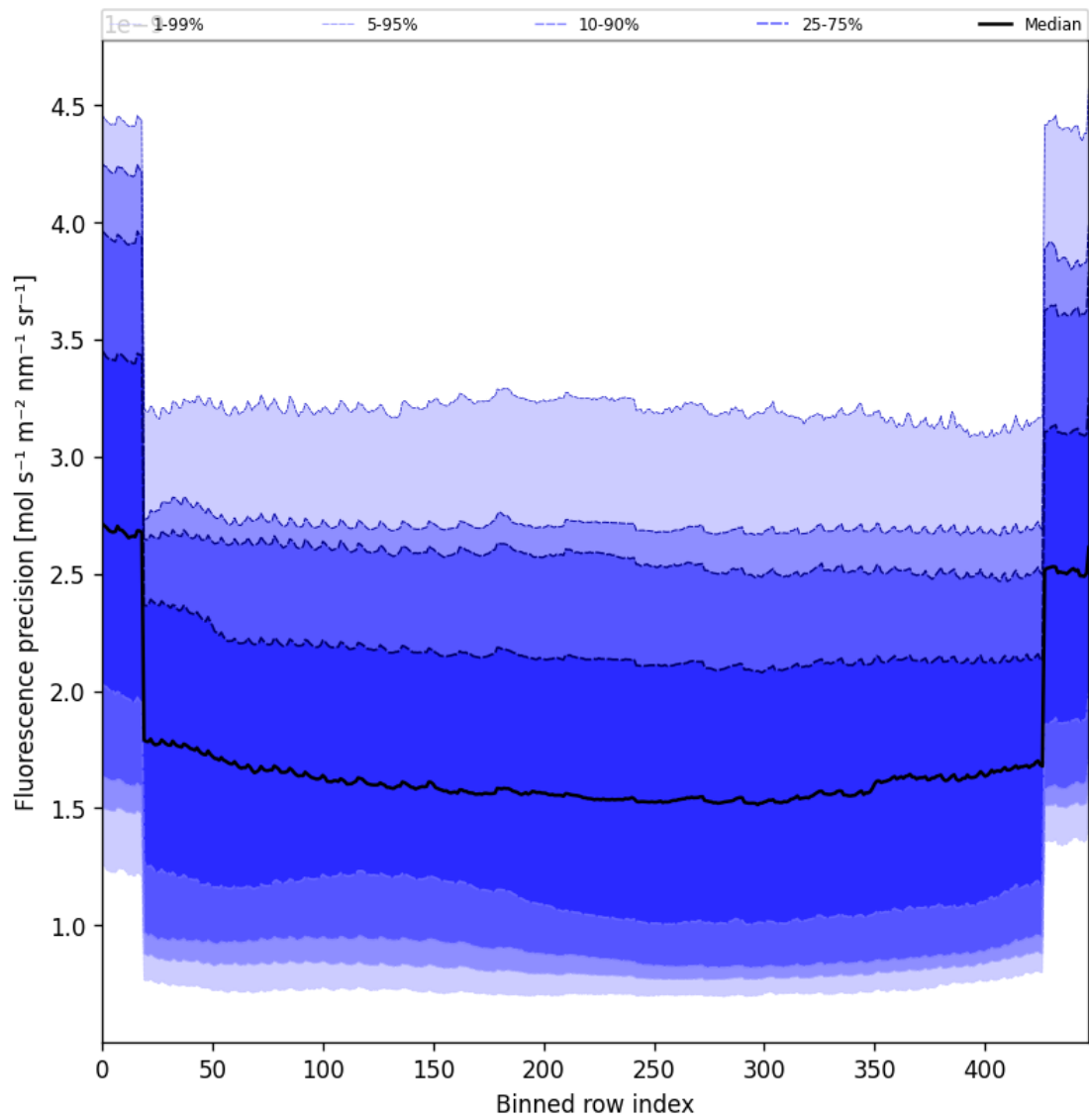
Figure 58: Along track statistics of “Fluorescence precision” for 2024-12-06 to 2024-12-08
