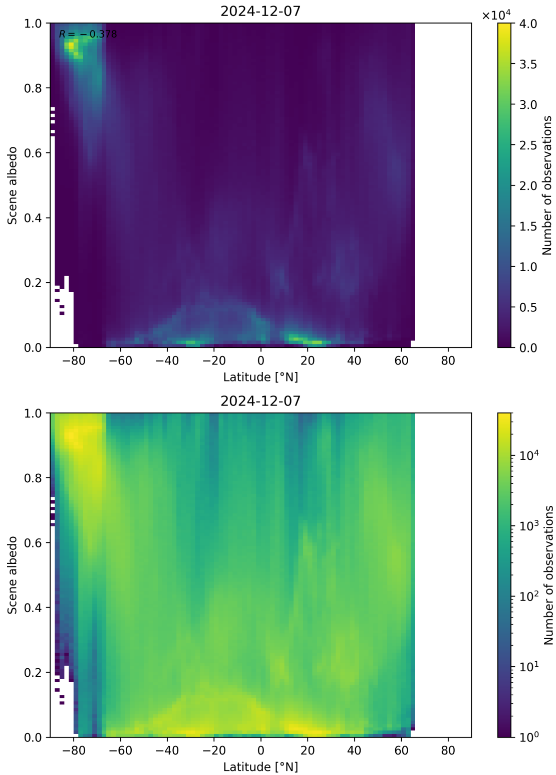
Figure 95: Scatter density plot of “Latitude” against “Scene albedo” for 2024-12-06 to 2024-12-08.
