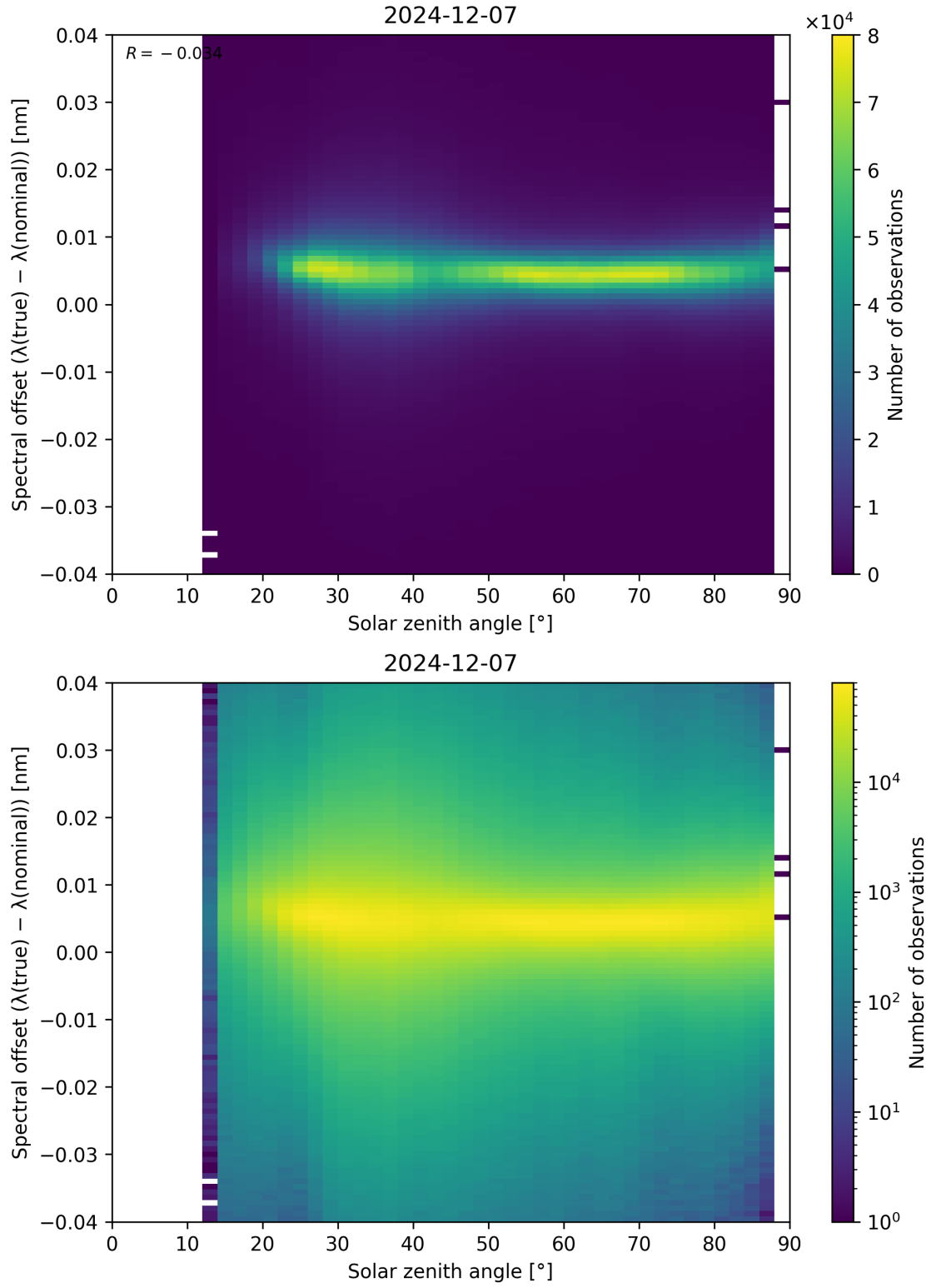
Figure 117: Scatter density plot of “Solar zenith angle” against “Spectral offset ( \lambda_{\text{true}} - \lambda_{\text{nominal}} )” for 2024-12-06 to 2024-12-08.
