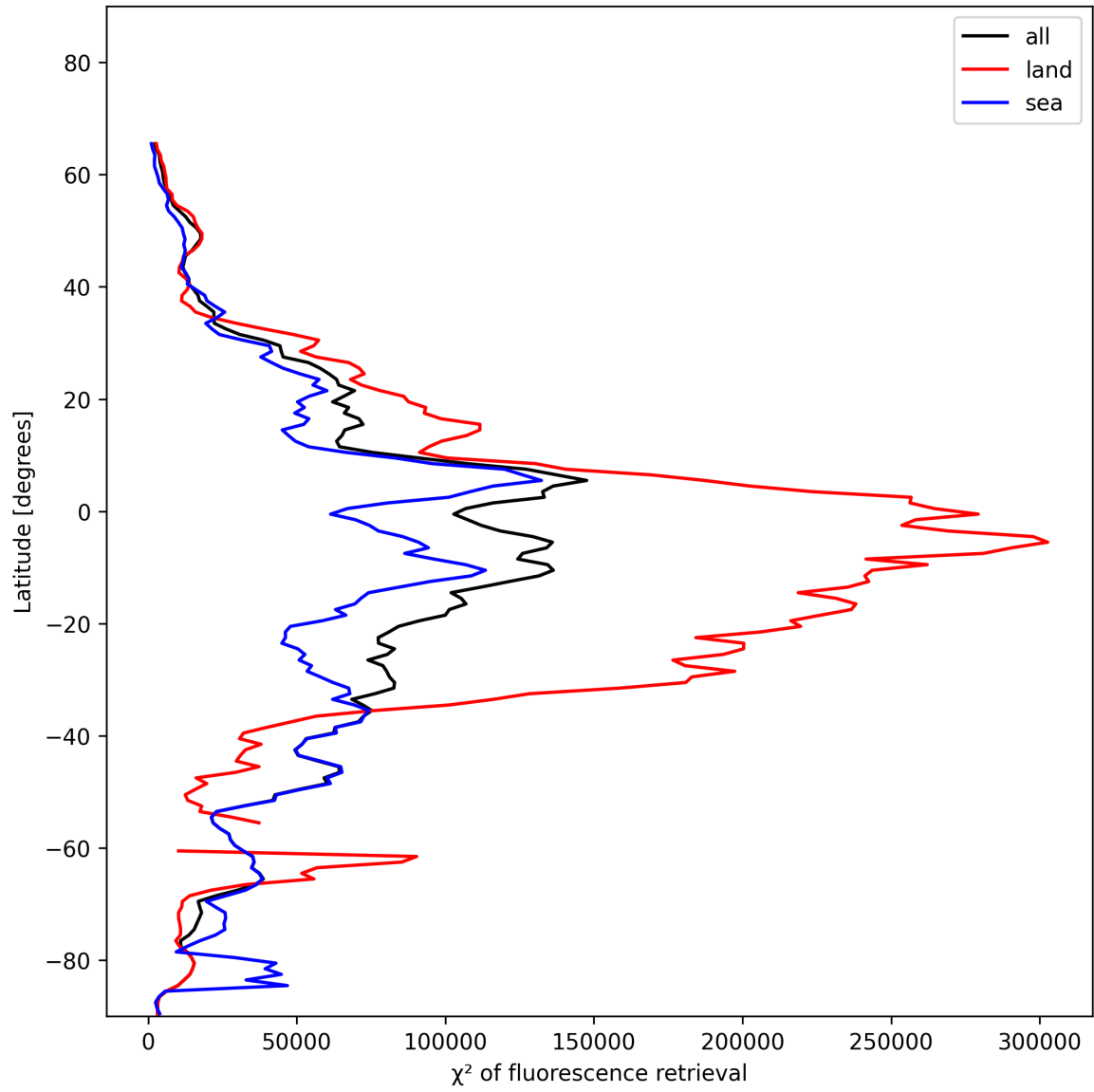
Figure 25: Zonal average of “ \chi^2 of fluorescence retrieval” for 2024-12-06 to 2024-12-08.
