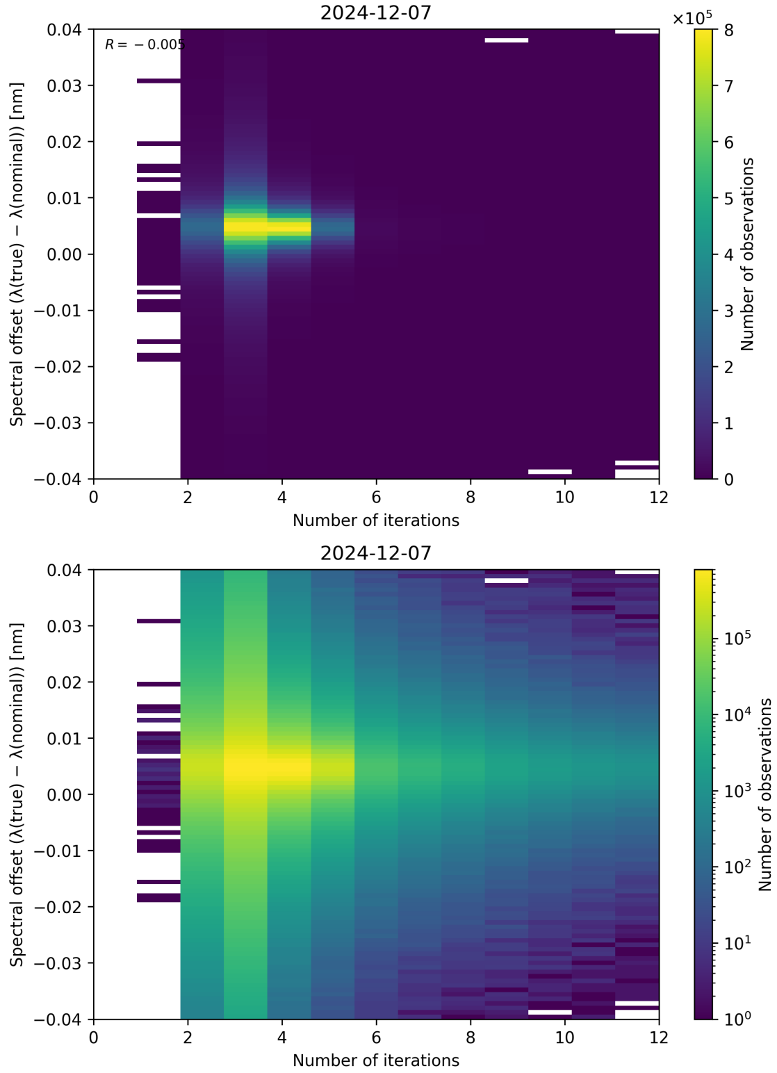
Figure 100: Scatter density plot of “Number of iterations” against “Spectral offset ( \lambda_{\text{true}} - \lambda_{\text{nominal}} )” for 2024-12-06 to 2024-12-08.
