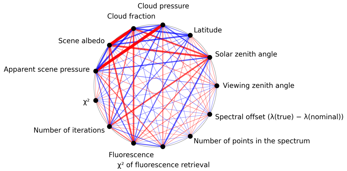
Figure 1: Map of correlation graph for 2024-12-06 to 2024-12-08.
