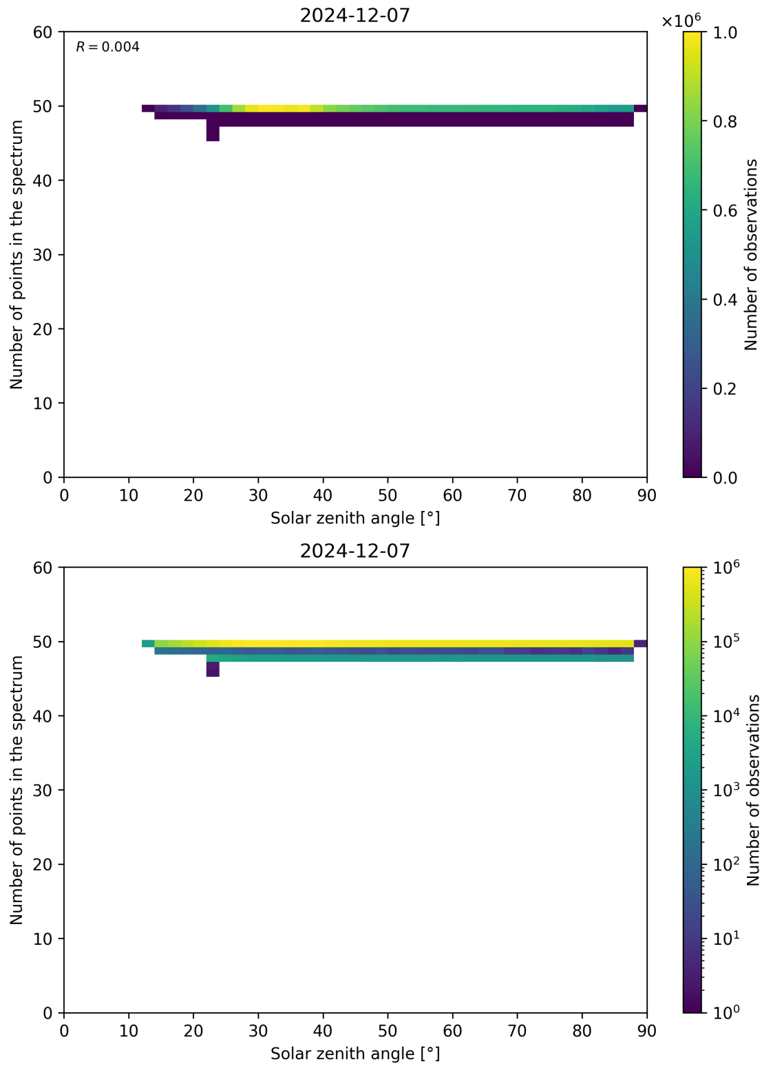
Figure 115: Scatter density plot of “Solar zenith angle” against “Number of points in the spectrum” for 2024-12-06 to 2024-12-08.
