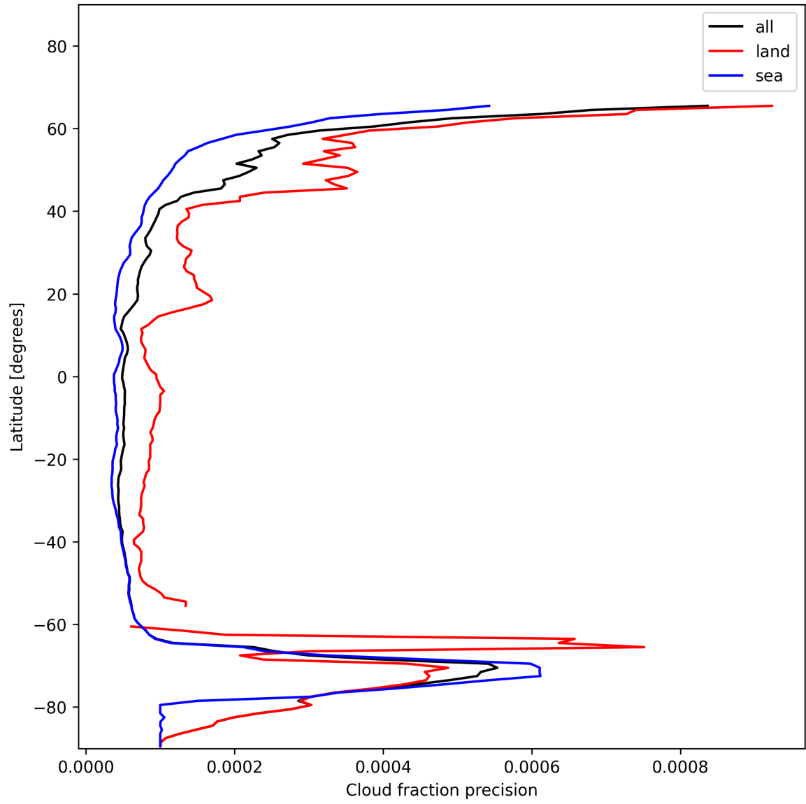
Figure 16: Zonal average of “Cloud fraction precision” for 2024-12-06 to 2024-12-08.
