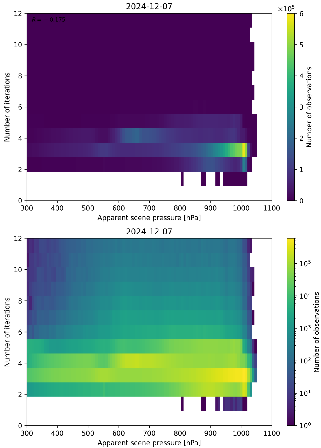
Figure 65: Scatter density plot of “Apparent scene pressure” against “Number of iterations” for 2024-12-06 to 2024-12-08.
