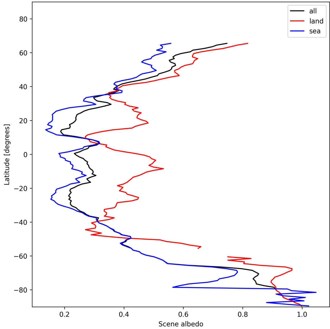
Figure 17: Zonal average of “Scene albedo” for 2024-12-06 to 2024-12-08.
