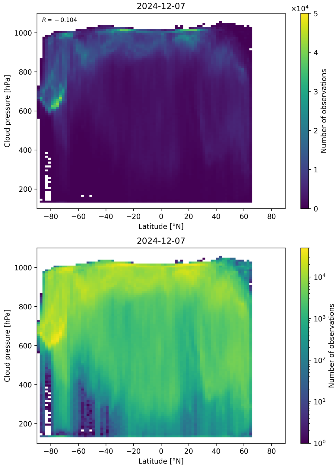
Figure 91: Scatter density plot of “Latitude” against “Cloud pressure” for 2024-12-06 to 2024-12-08.
