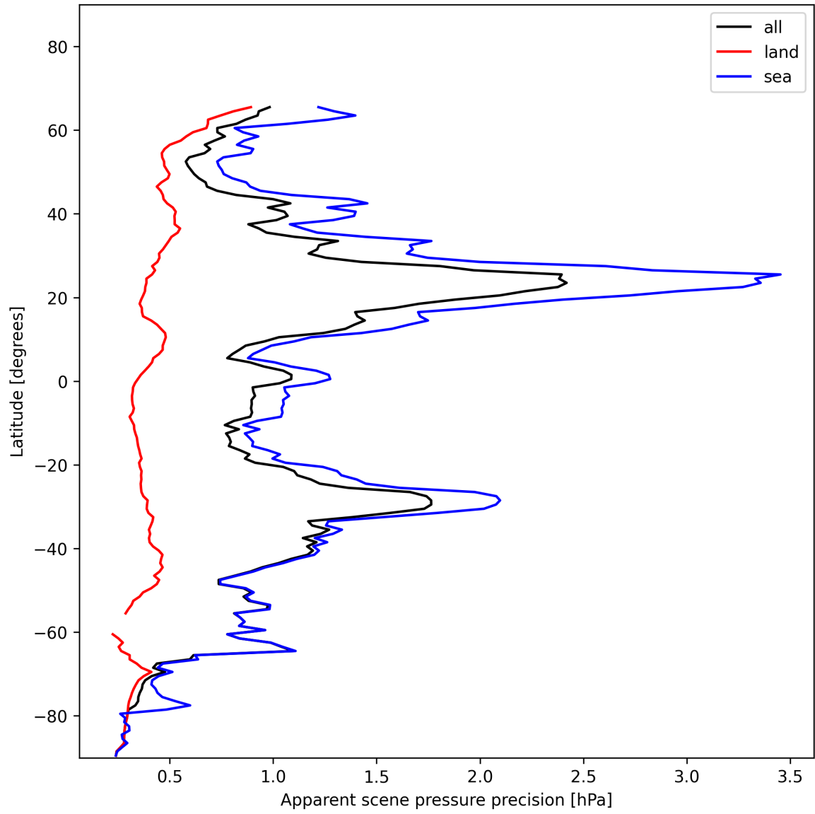
Figure 20: Zonal average of “Apparent scene pressure precision” for 2024-12-06 to 2024-12-08.
