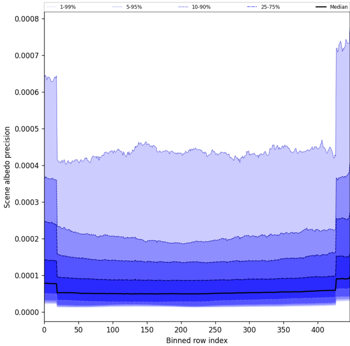
Figure 52: Along track statistics of “Scene albedo precision” for 2024-12-06 to 2024-12-08
