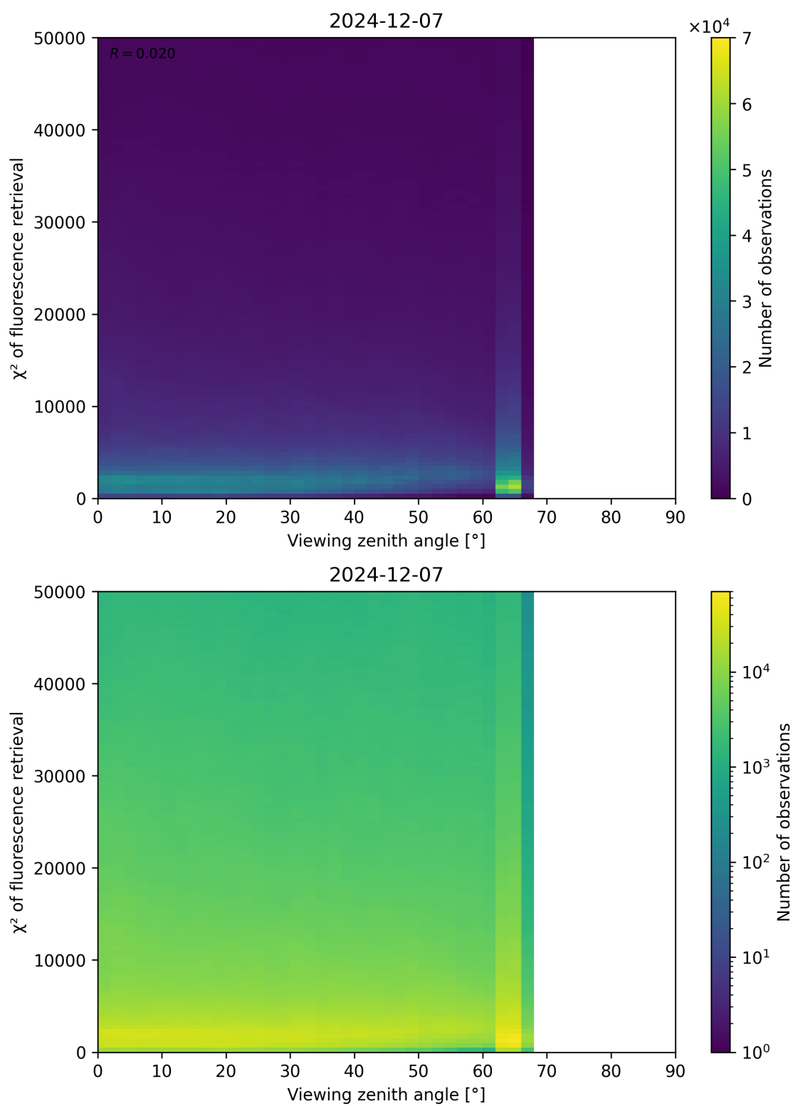
Figure 119: Scatter density plot of “Viewing zenith angle” against “ \chi^2 of fluorescence retrieval” for 2024-12-06 to 2024-12-08.
