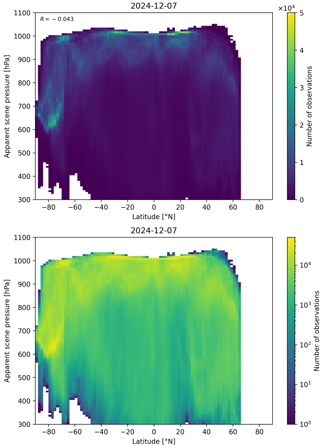
Figure 88: Scatter density plot of “Latitude” against “Apparent scene pressure” for 2024-12-06 to 2024-12-08.
