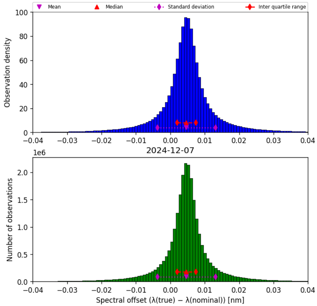
Figure 45: Histogram of “Spectral offset ( \lambda_{\text{true}} - \lambda_{\text{nominal}} )” for 2024-12-06 to 2024-12-08
