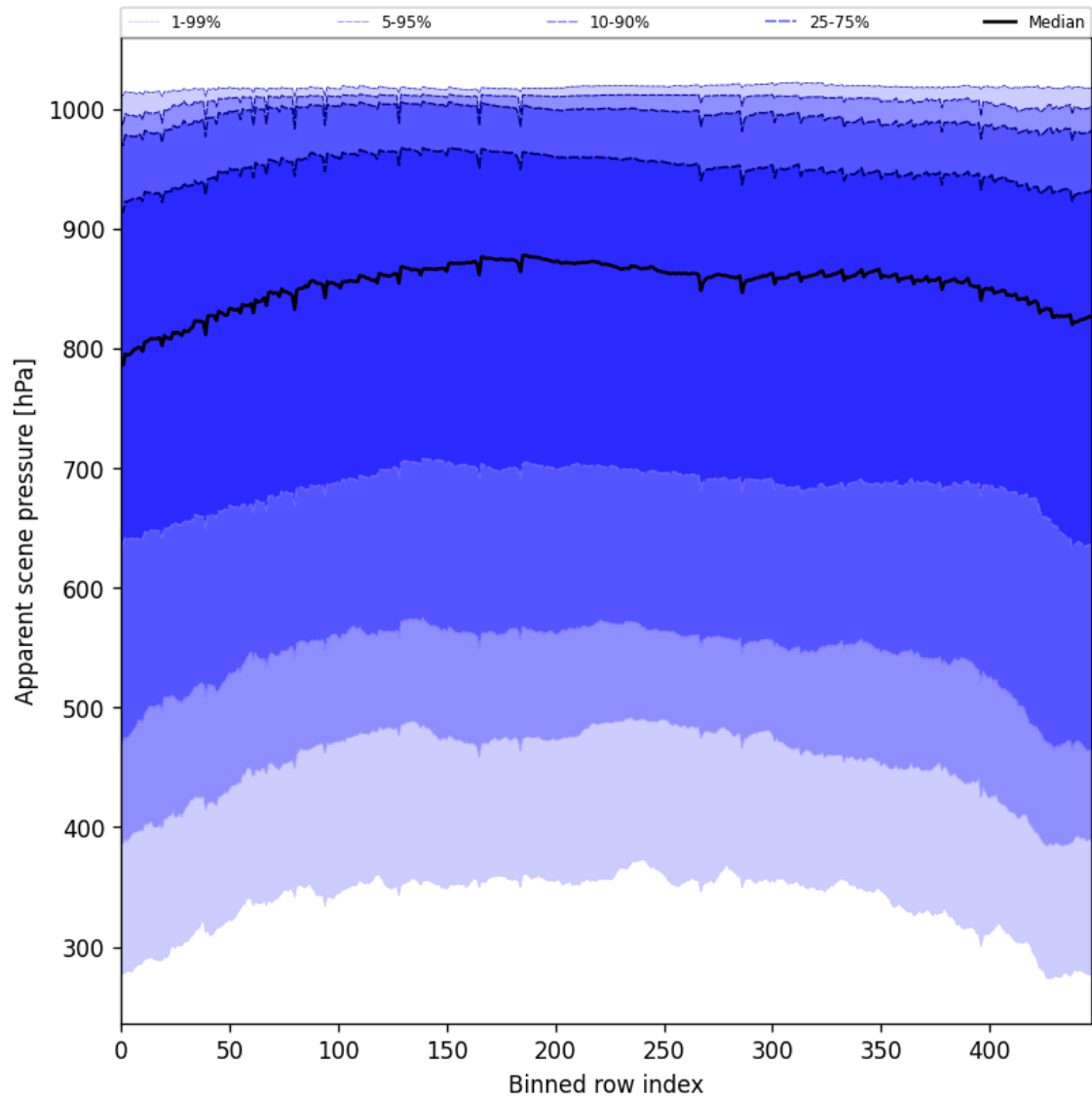
Figure 53: Along track statistics of “Apparent scene pressure” for 2024-12-06 to 2024-12-08
