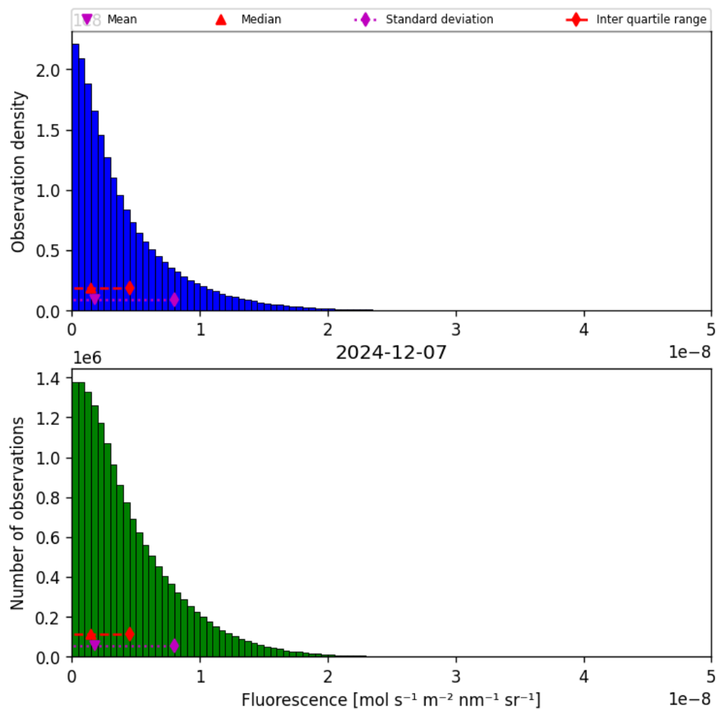
Figure 40: Histogram of “Fluorescence” for 2024-12-06 to 2024-12-08
