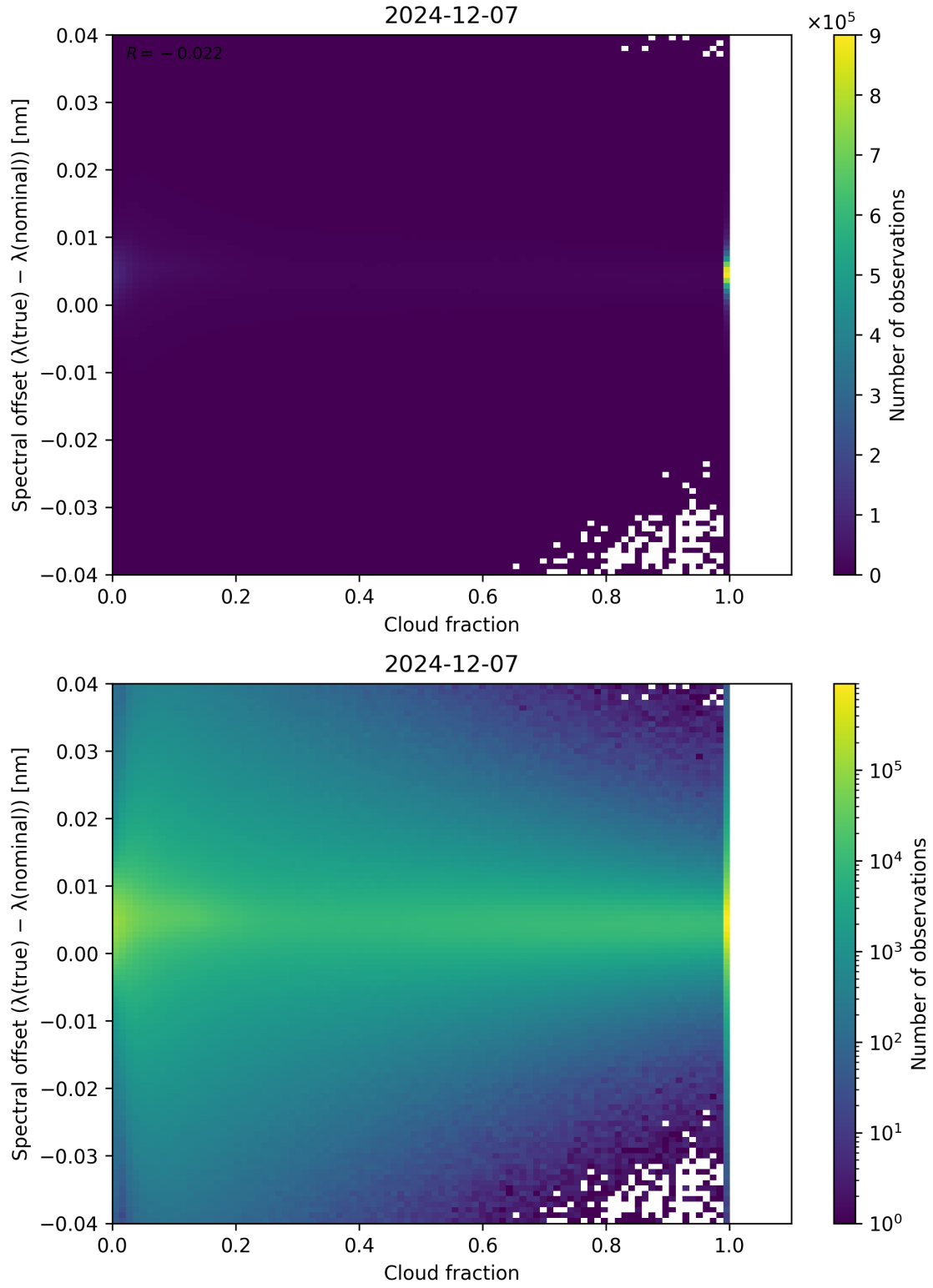
Figure 76: Scatter density plot of “Cloud fraction” against “Spectral offset ( \lambda_{\text{true}} - \lambda_{\text{nominal}} )” for 2024-12-06 to 2024-12-08.
