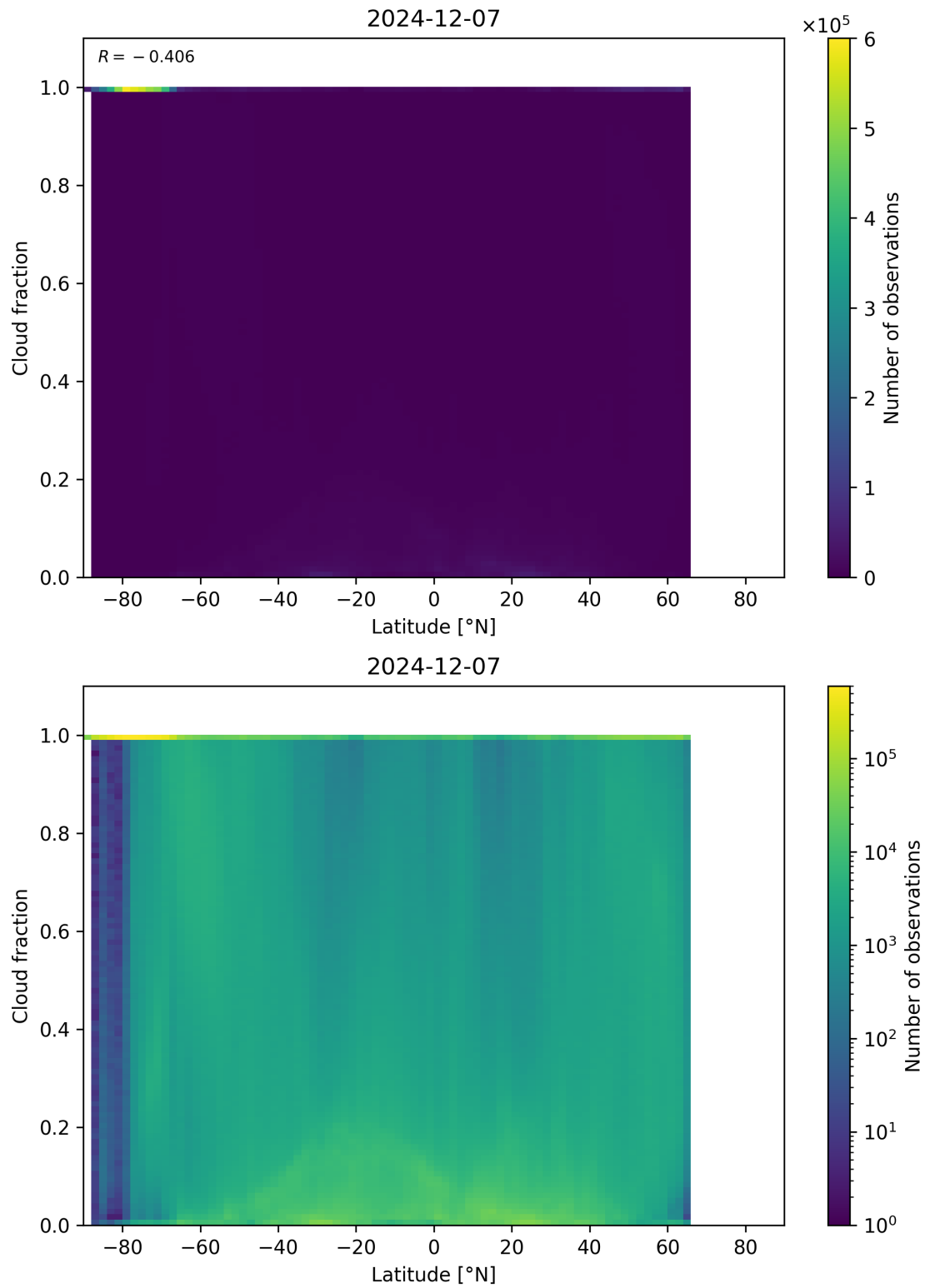
Figure 90: Scatter density plot of “Latitude” against “Cloud fraction” for 2024-12-06 to 2024-12-08.
