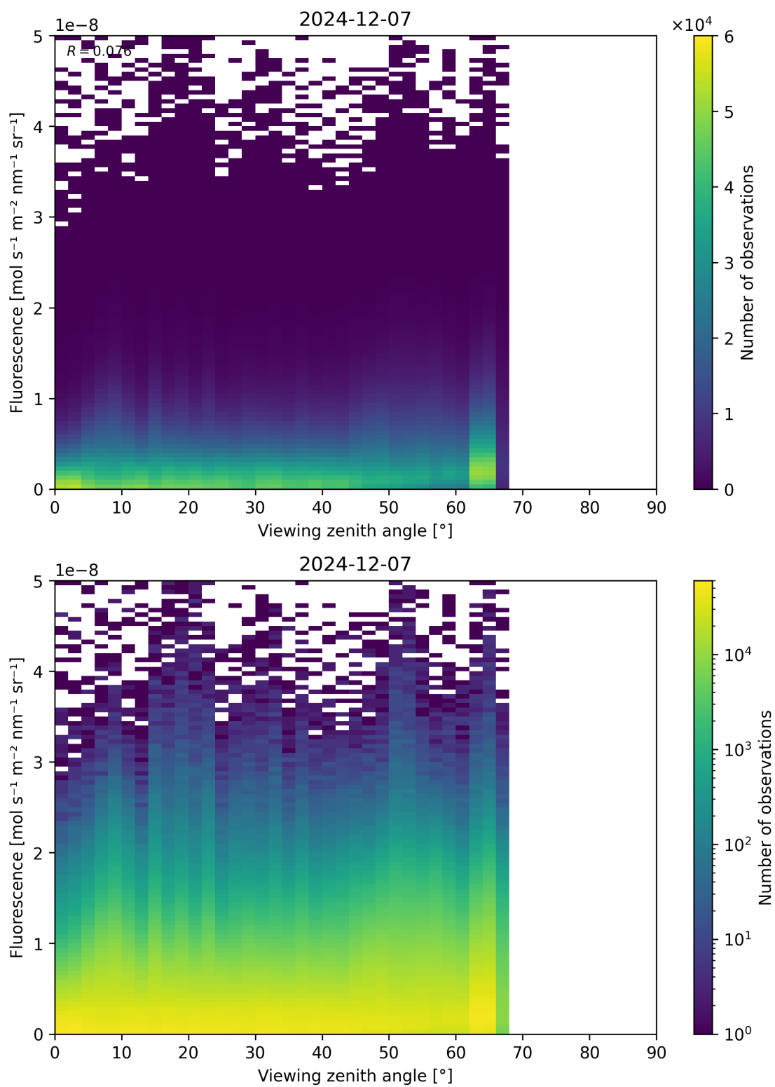
Figure 122: Scatter density plot of “Viewing zenith angle” against “Fluorescence” for 2024-12-06 to 2024-12-08.
