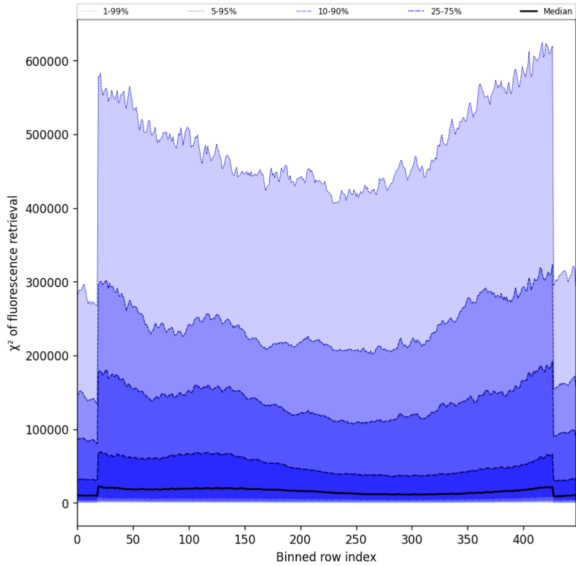
Figure 59: Along track statistics of “ \chi^2 of fluorescence retrieval” for 2024-12-06 to 2024-12-08
