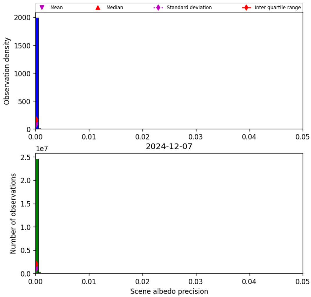
Figure 35: Histogram of “Scene albedo precision” for 2024-12-06 to 2024-12-08
