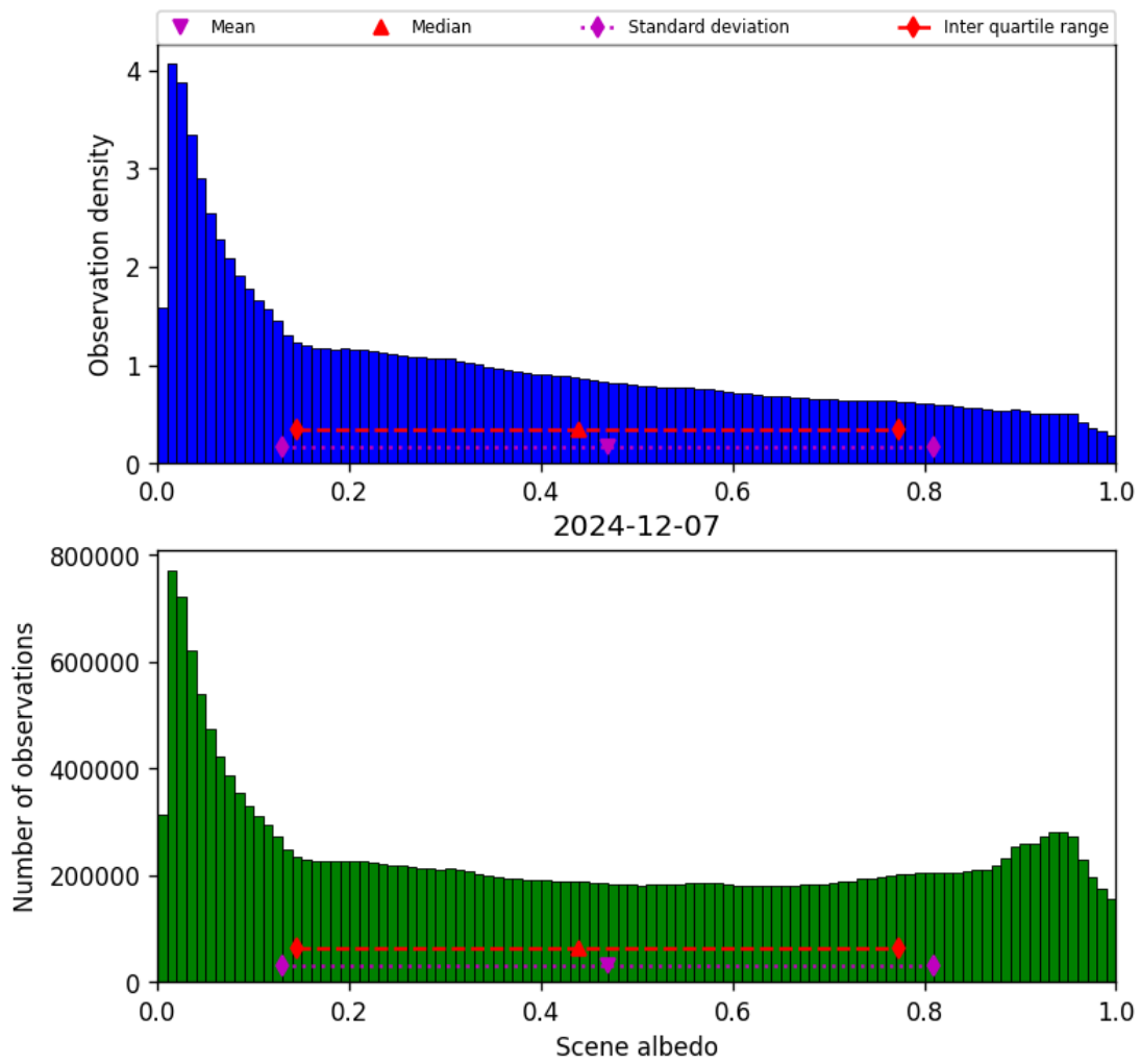
Figure 34: Histogram of “Scene albedo” for 2024-12-06 to 2024-12-08
