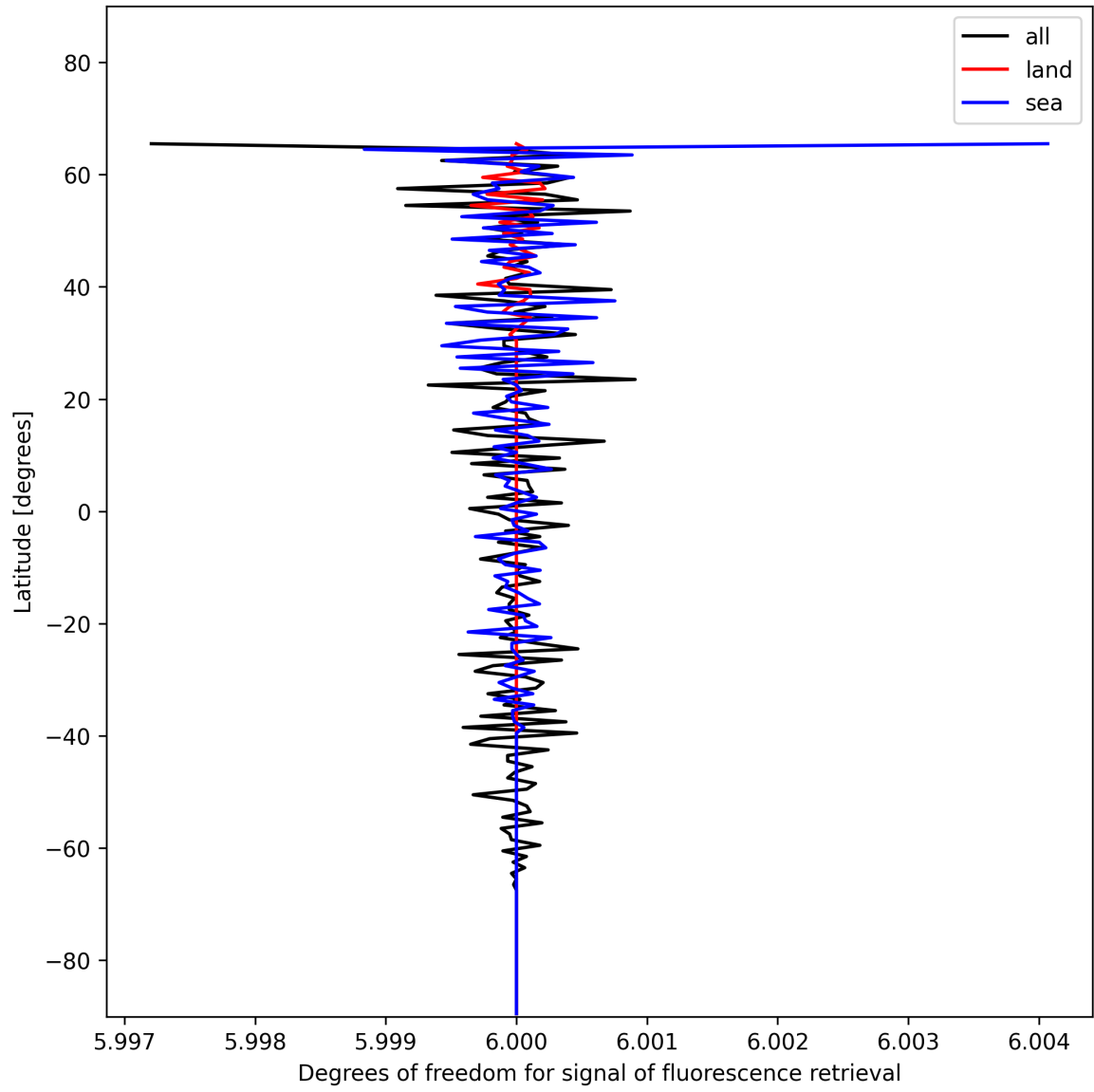
Figure 26: Zonal average of “Degrees of freedom for signal of fluorescence retrieval” for 2024-12-06 to 2024-12-08.
