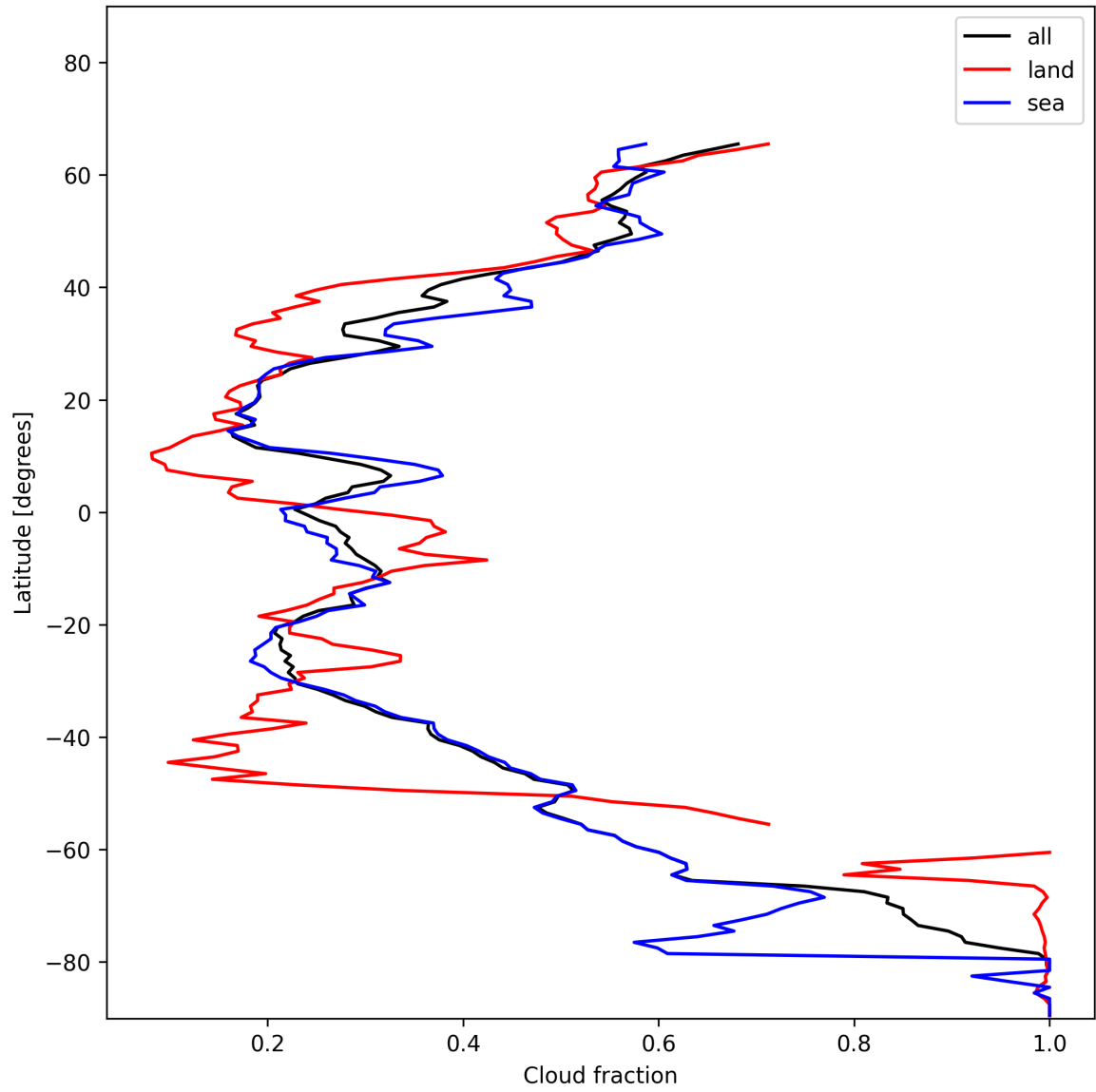
Figure 15: Zonal average of “Cloud fraction” for 2024-12-06 to 2024-12-08.
