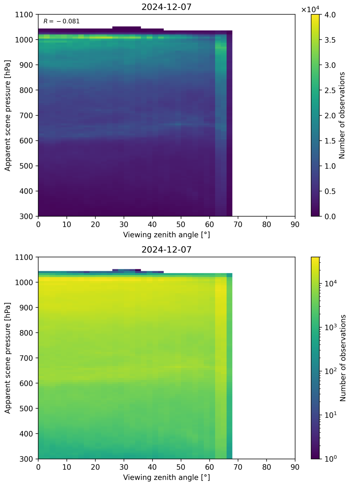
Figure 118: Scatter density plot of “Viewing zenith angle” against “Apparent scene pressure” for 2024-12-06 to 2024-12-08.
