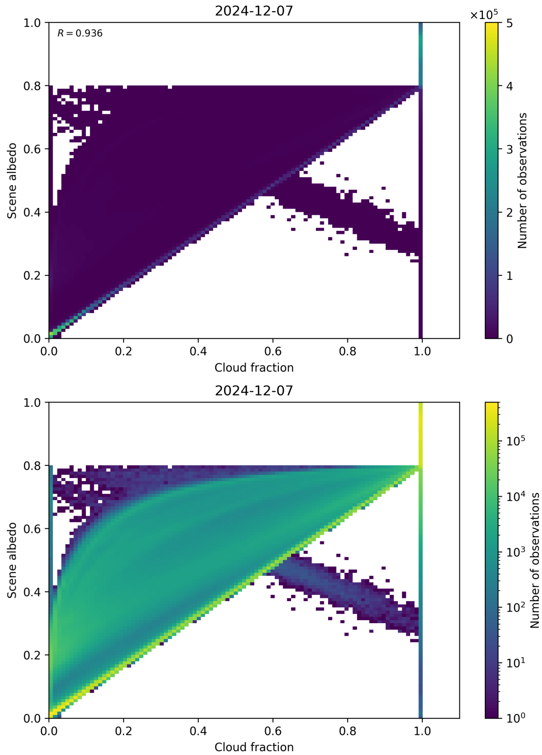
Figure 75: Scatter density plot of “Cloud fraction” against “Scene albedo” for 2024-12-06 to 2024-12-08.
