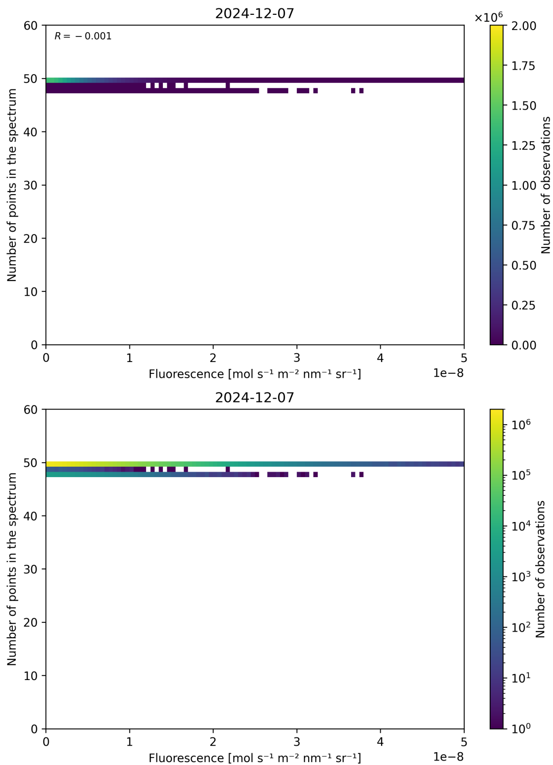
Figure 86: Scatter density plot of “Fluorescence” against “Number of points in the spectrum” for 2024-12-06 to 2024-12-08.
