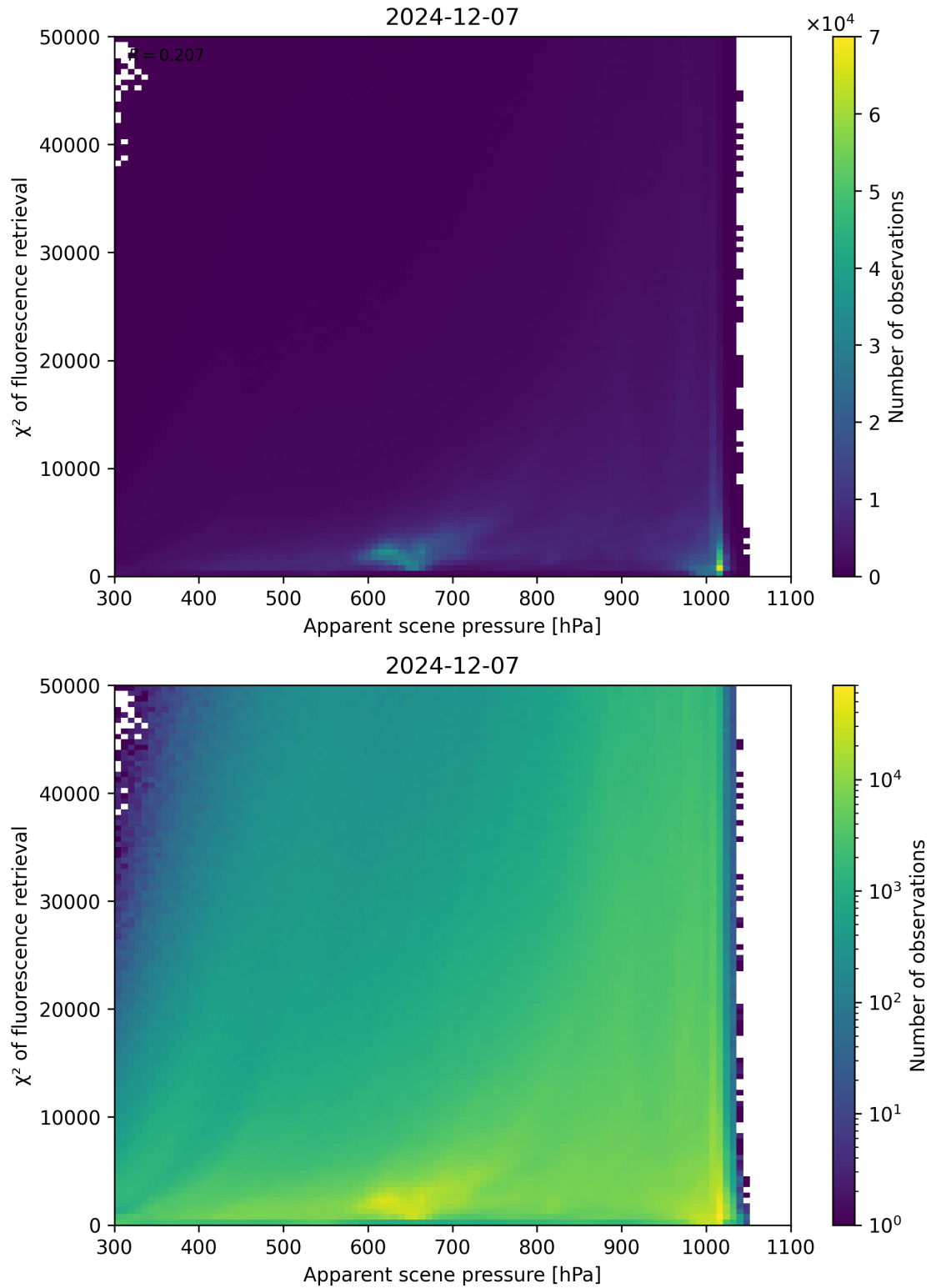
Figure 63: Scatter density plot of “Apparent scene pressure” against “ \chi^2 of fluorescence retrieval” for 2024-12-06 to 2024-12-08.
