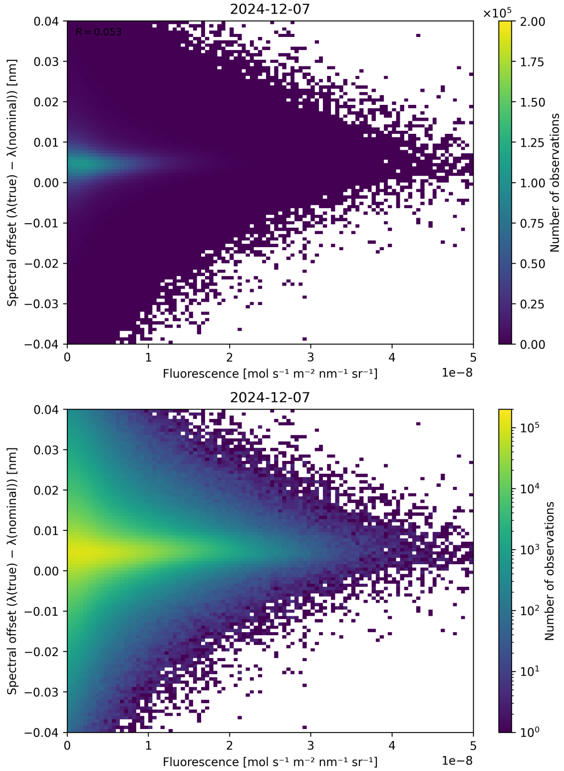
Figure 87: Scatter density plot of “Fluorescence” against “Spectral offset ( \lambda_{\text{true}} - \lambda_{\text{nominal}} )” for 2024-12-06 to 2024-12-08.
