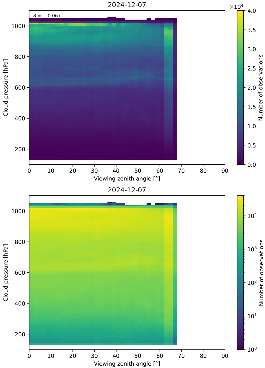
Figure 121: Scatter density plot of “Viewing zenith angle” against “Cloud pressure” for 2024-12-06 to 2024-12-08.
