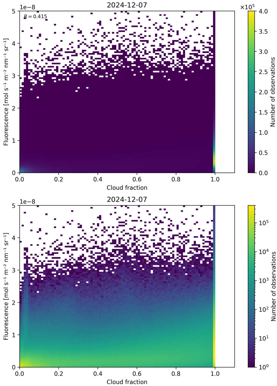
Figure 72: Scatter density plot of “Cloud fraction” against “Fluorescence” for 2024-12-06 to 2024-12-08.
