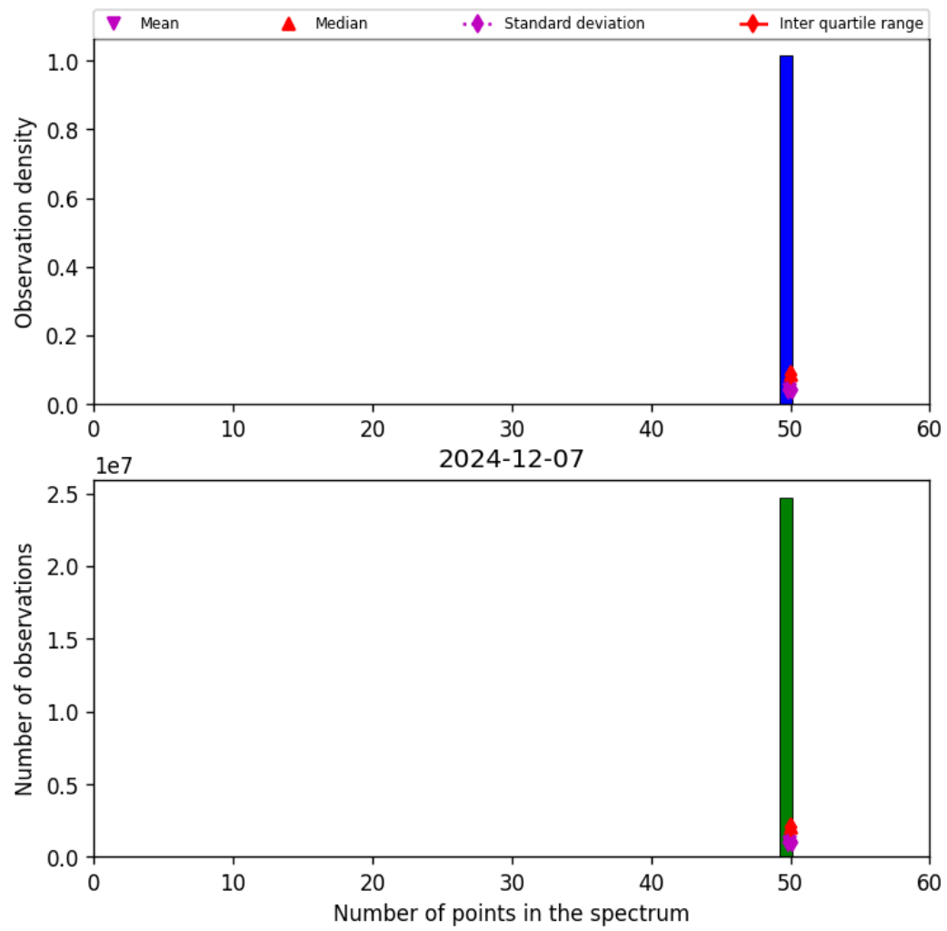
Figure 44: Histogram of “Number of points in the spectrum” for 2024-12-06 to 2024-12-08
