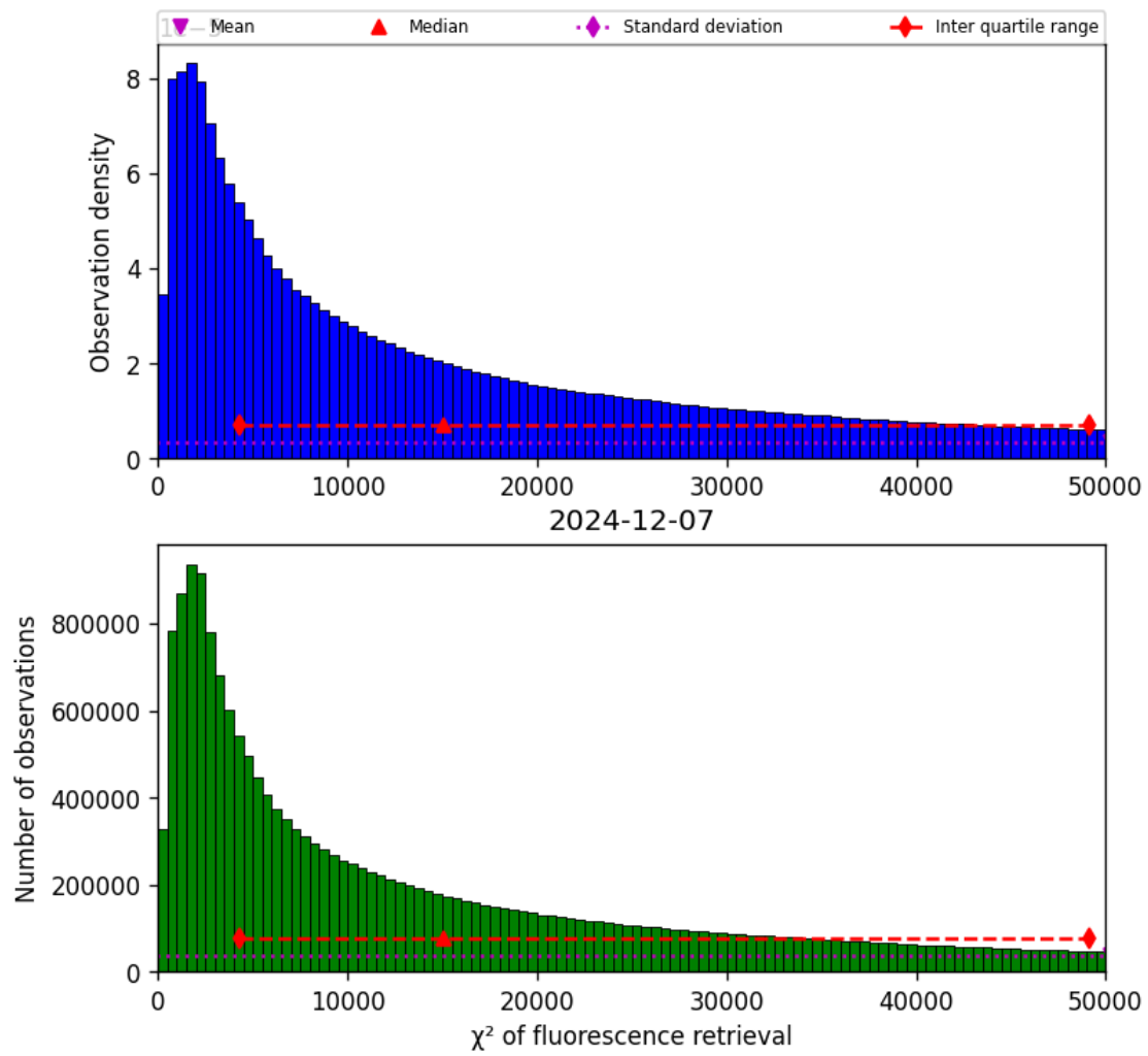
Figure 42: Histogram of “ \chi^2 of fluorescence retrieval” for 2024-12-06 to 2024-12-08
