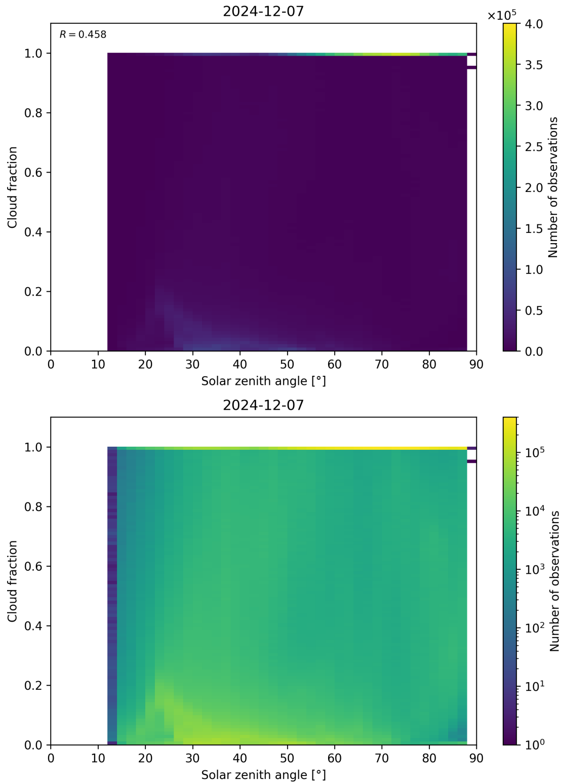
Figure 110: Scatter density plot of “Solar zenith angle” against “Cloud fraction” for 2024-12-06 to 2024-12-08.
