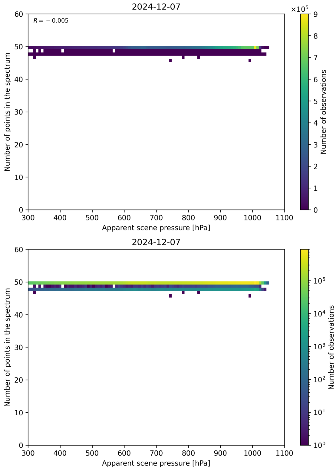
Figure 66: Scatter density plot of “Apparent scene pressure” against “Number of points in the spectrum” for 2024-12-06 to 2024-12-08.
