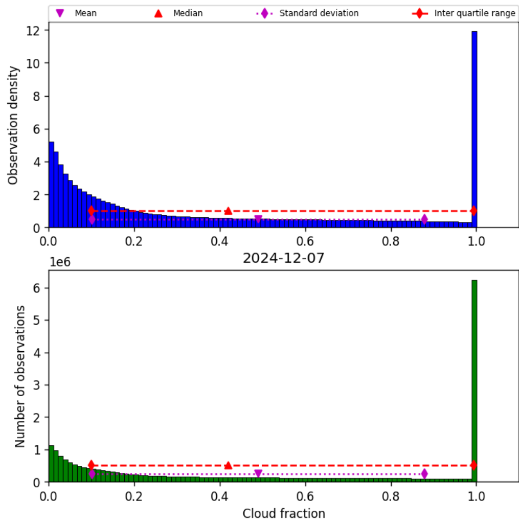
Figure 32: Histogram of “Cloud fraction” for 2024-12-06 to 2024-12-08
