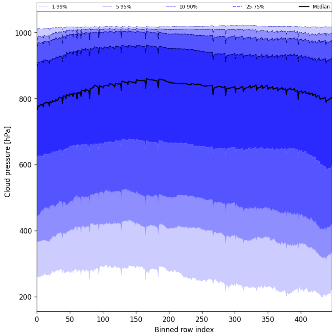
Figure 47: Along track statistics of “Cloud pressure” for 2024-12-06 to 2024-12-08
