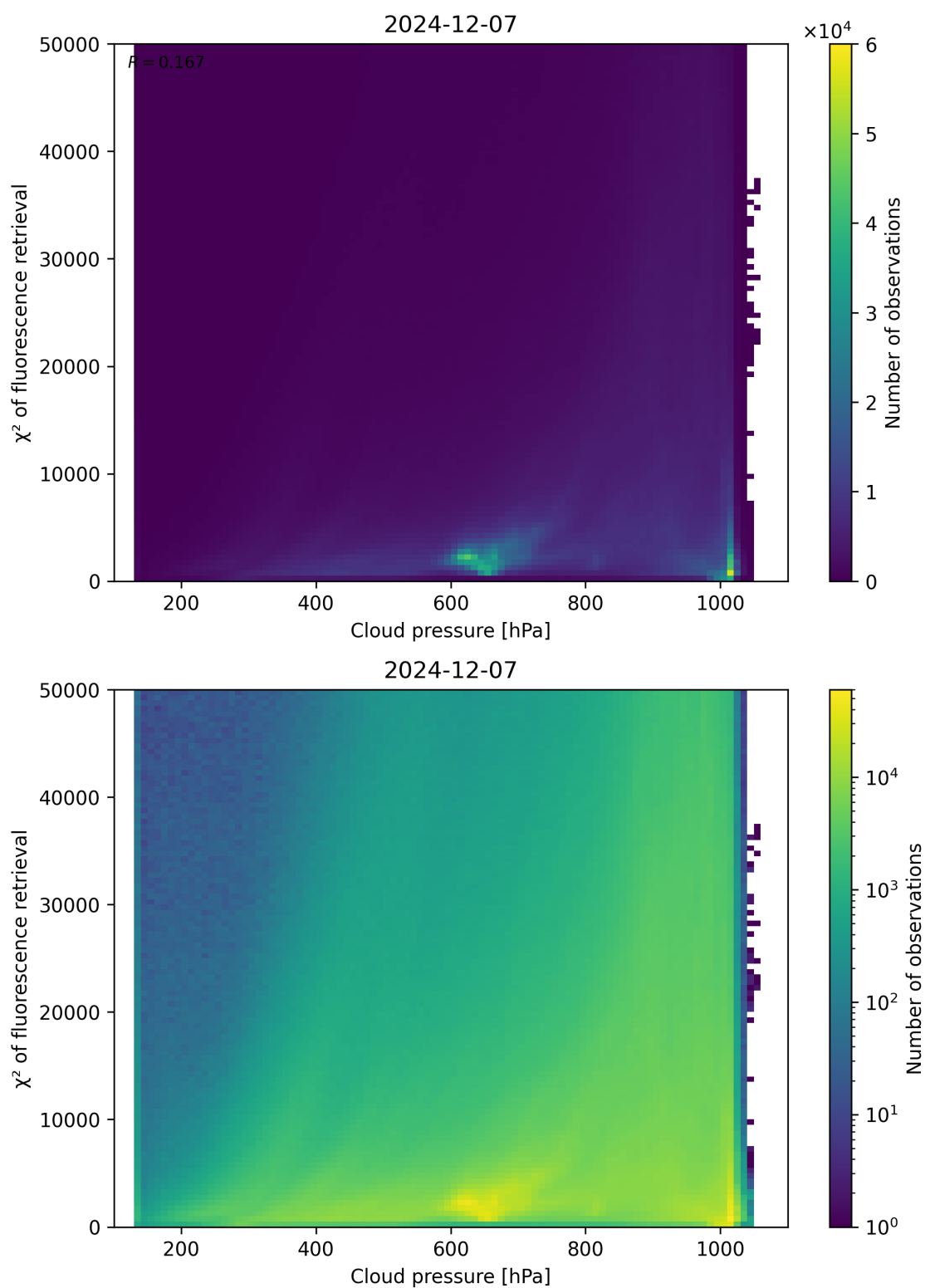
Figure 78: Scatter density plot of “Cloud pressure” against “ \chi^2 of fluorescence retrieval” for 2024-12-06 to 2024-12-08.
