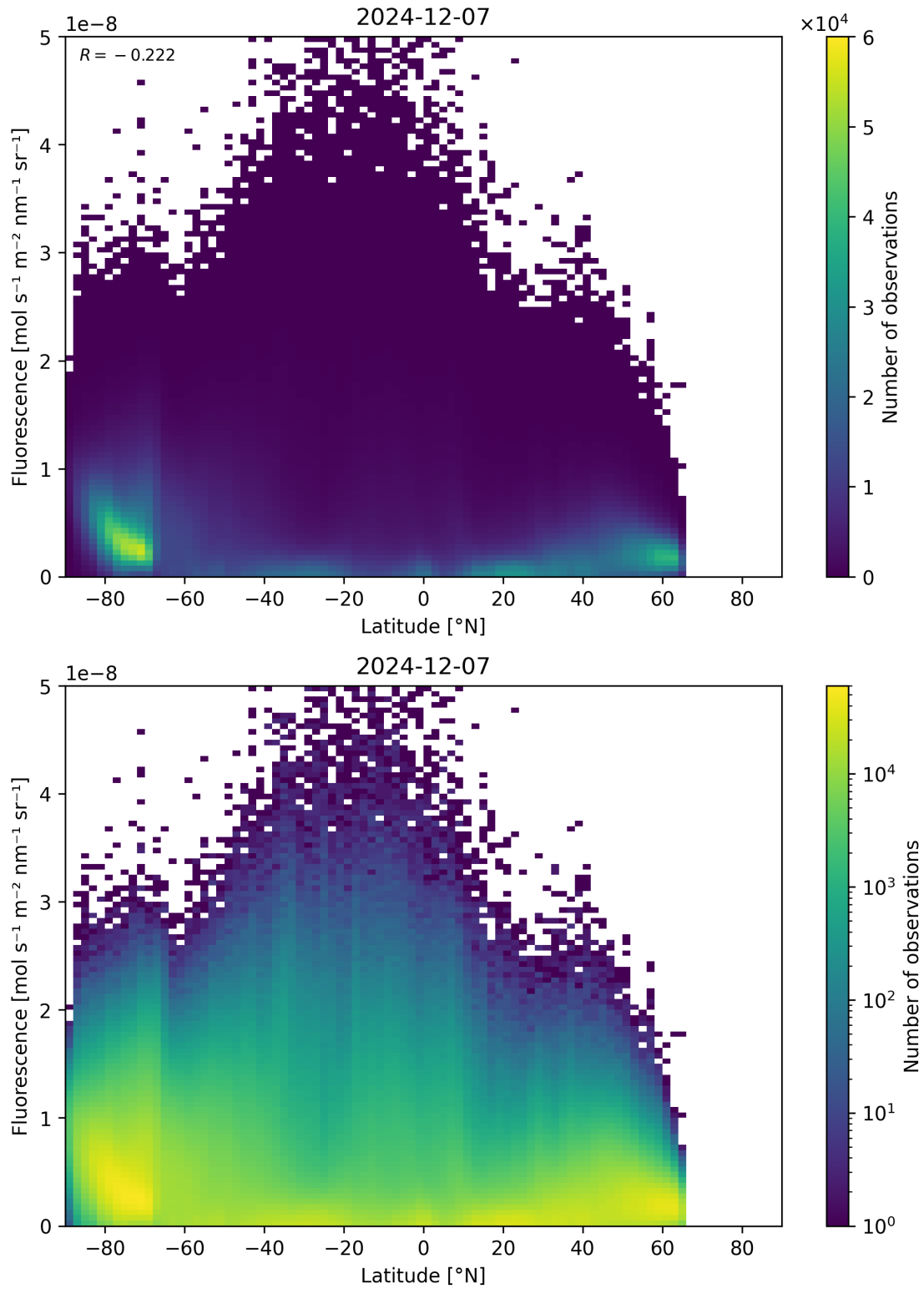
Figure 92: Scatter density plot of “Latitude” against “Fluorescence” for 2024-12-06 to 2024-12-08.
