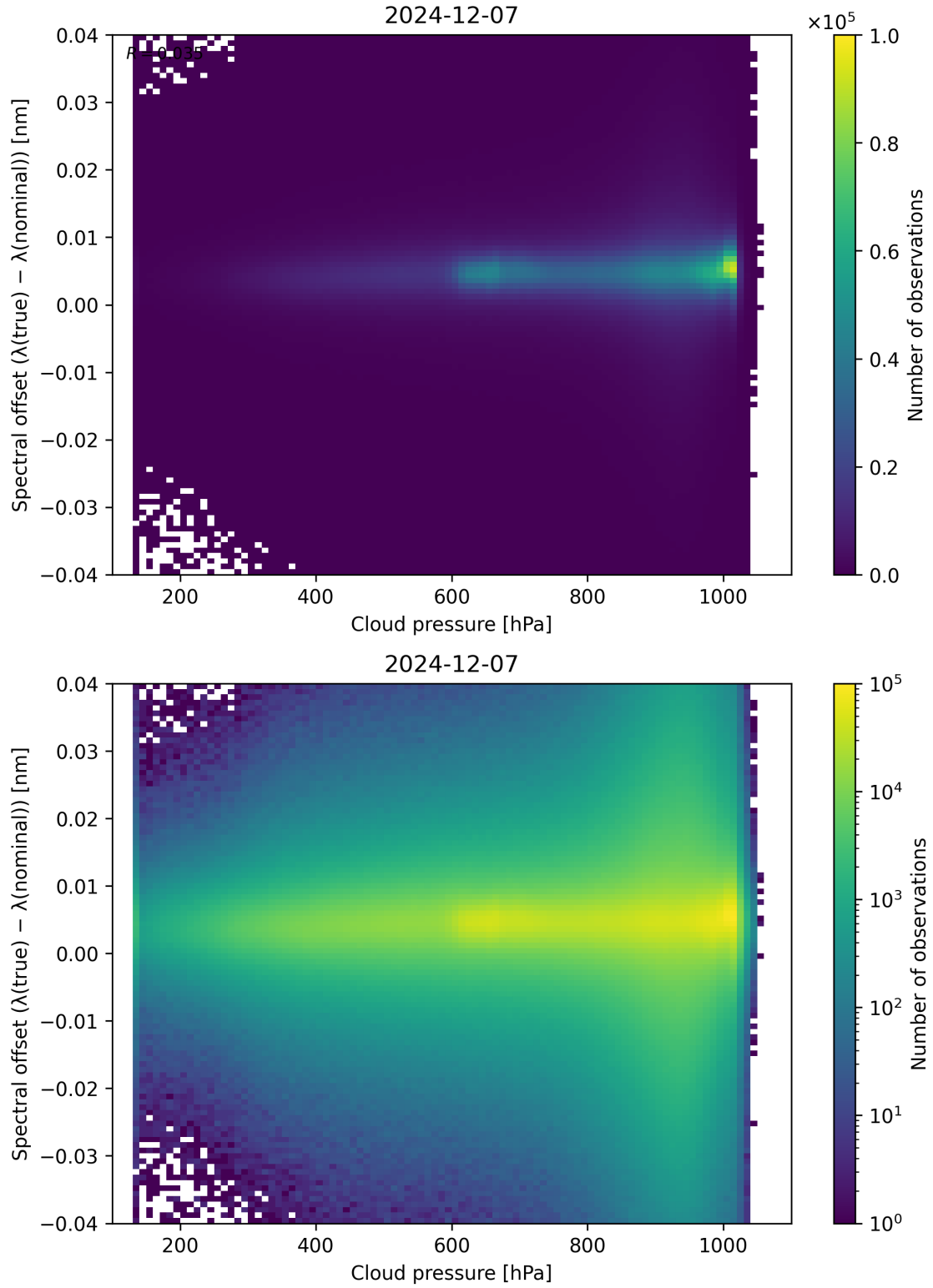
Figure 84: Scatter density plot of “Cloud pressure” against “Spectral offset ( \lambda_{\text{true}} - \lambda_{\text{nominal}} )” for 2024-12-06 to 2024-12-08.
