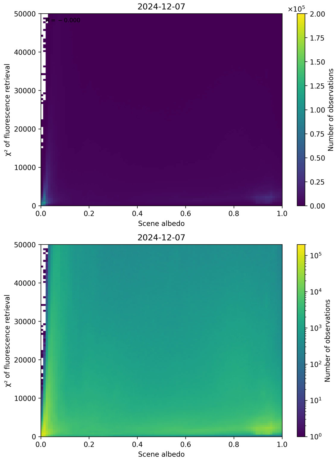
Figure 103: Scatter density plot of “Scene albedo” against “ \chi^2 of fluorescence retrieval” for 2024-12-06 to 2024-12-08.
