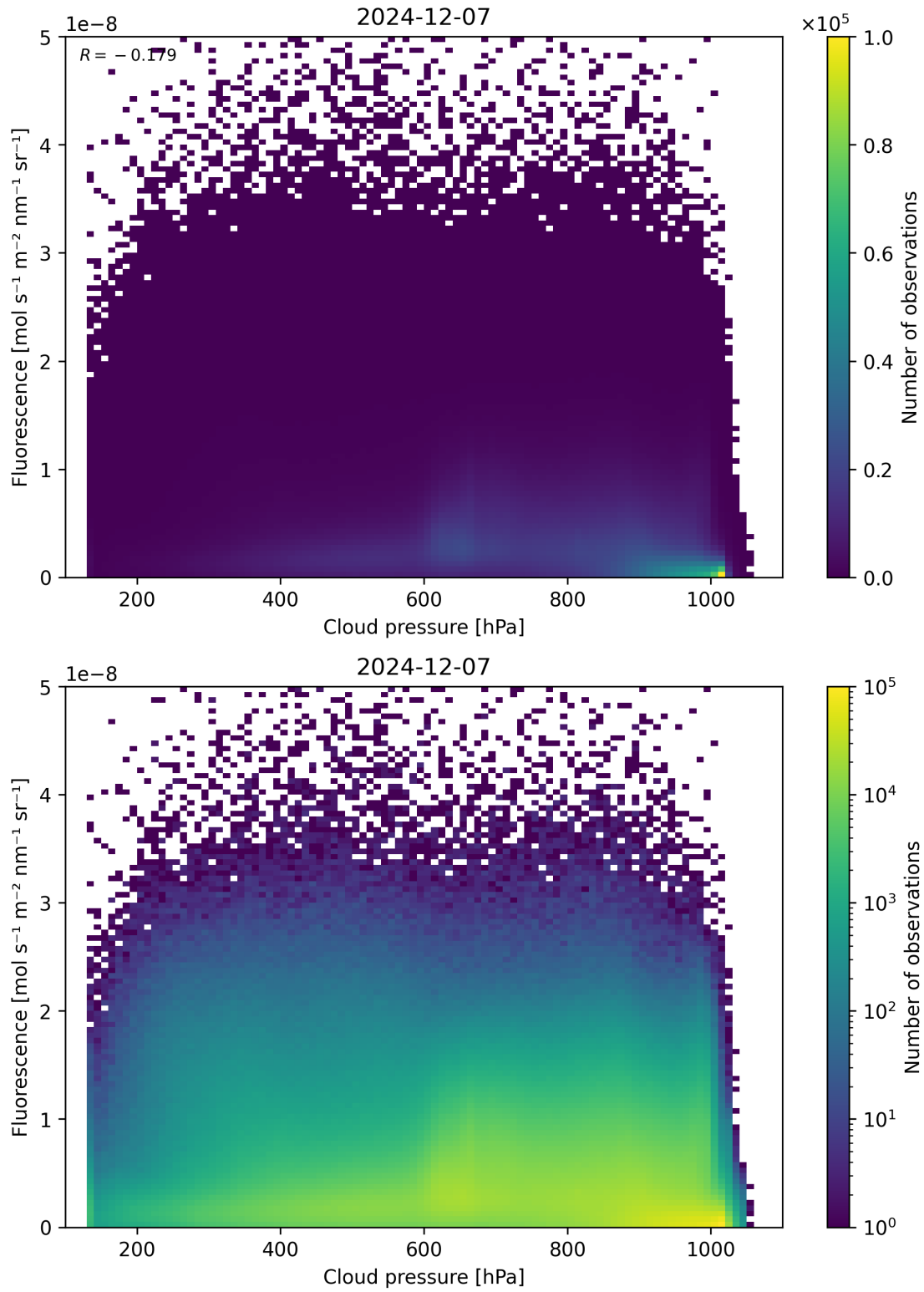
Figure 80: Scatter density plot of “Cloud pressure” against “Fluorescence” for 2024-12-06 to 2024-12-08.
