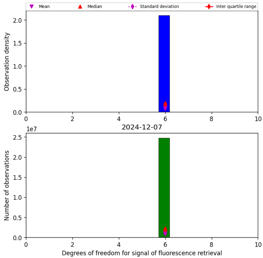
Figure 43: Histogram of "Degrees of freedom for signal of fluorescence retrieval" for 2024-12-06 to 2024-12-08
