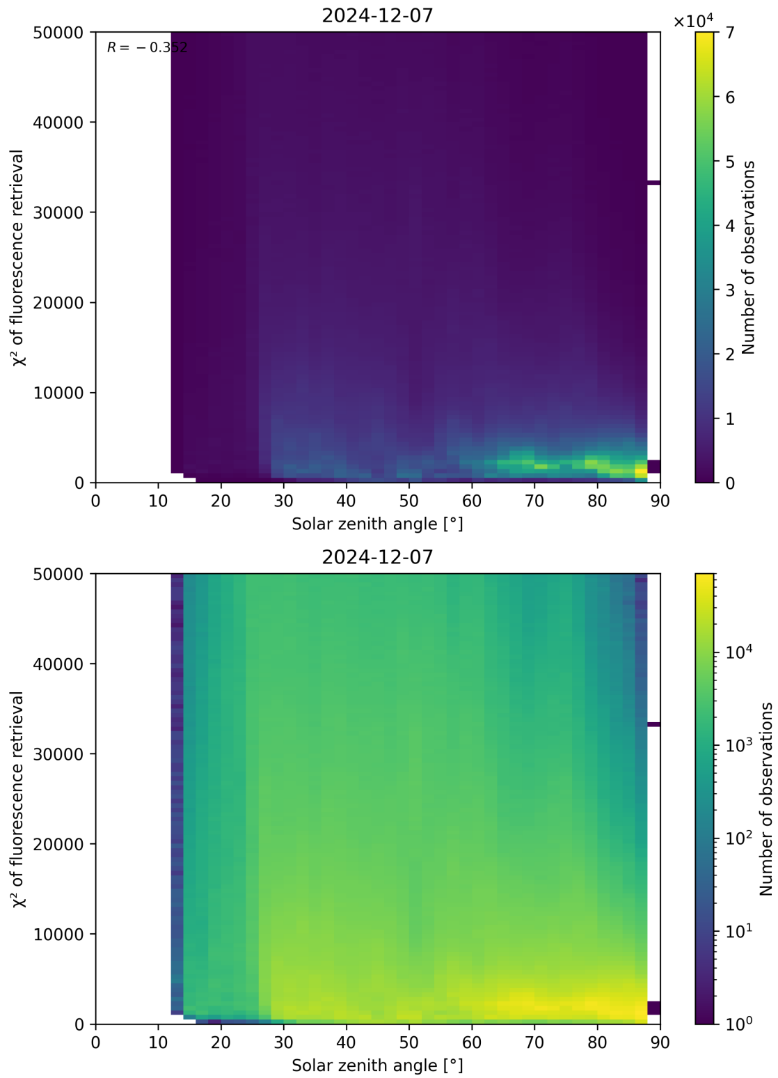
Figure 109: Scatter density plot of “Solar zenith angle” against “ \chi^2 of fluorescence retrieval” for 2024-12-06 to 2024-12-08.
