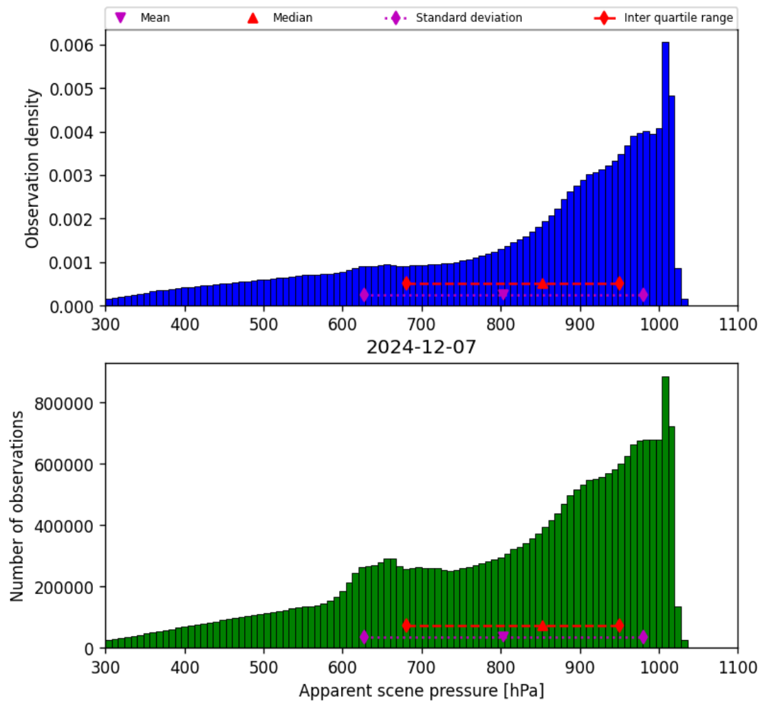
Figure 36: Histogram of “Apparent scene pressure” for 2024-12-06 to 2024-12-08
