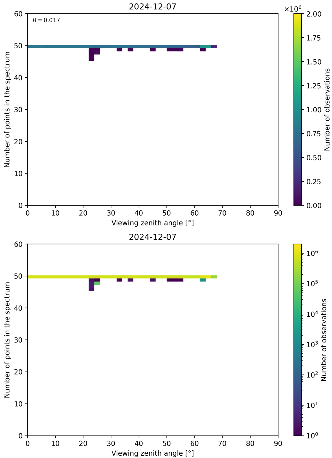
Figure 125: Scatter density plot of “Viewing zenith angle” against “Number of points in the spectrum” for 2024-12-06 to 2024-12-08.
