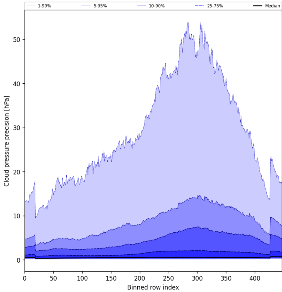
Figure 48: Along track statistics of “Cloud pressure precision” for 2024-12-06 to 2024-12-08
