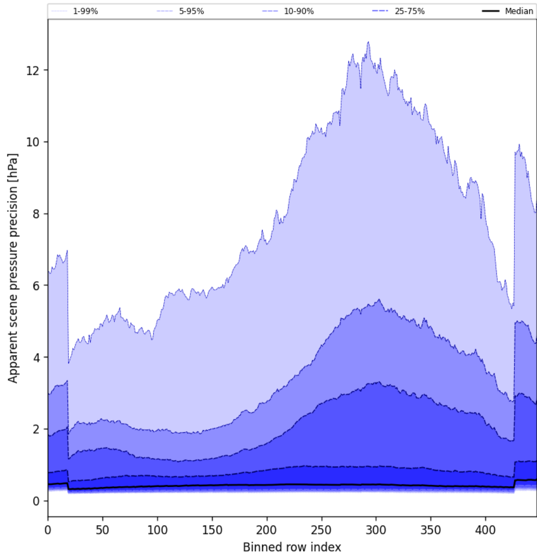
Figure 54: Along track statistics of “Apparent scene pressure precision” for 2024-12-06 to 2024-12-08
