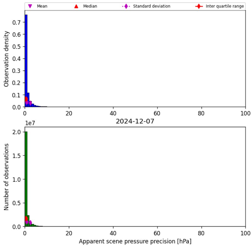
Figure 37: Histogram of “Apparent scene pressure precision” for 2024-12-06 to 2024-12-08
