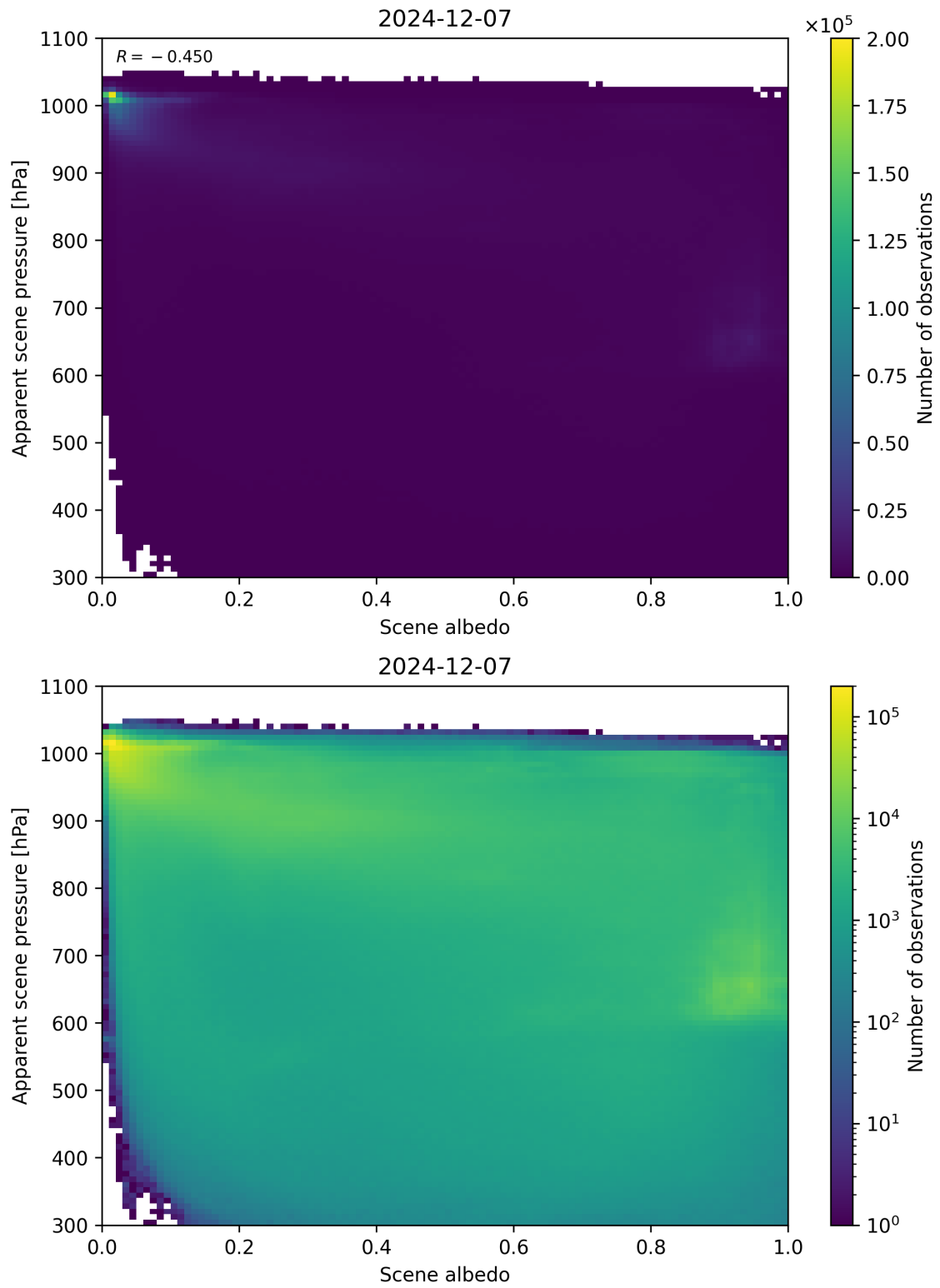
Figure 102: Scatter density plot of “Scene albedo” against “Apparent scene pressure” for 2024-12-06 to 2024-12-08.
