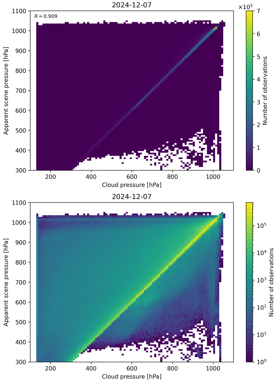
Figure 77: Scatter density plot of “Cloud pressure” against “Apparent scene pressure” for 2024-12-06 to 2024-12-08.
