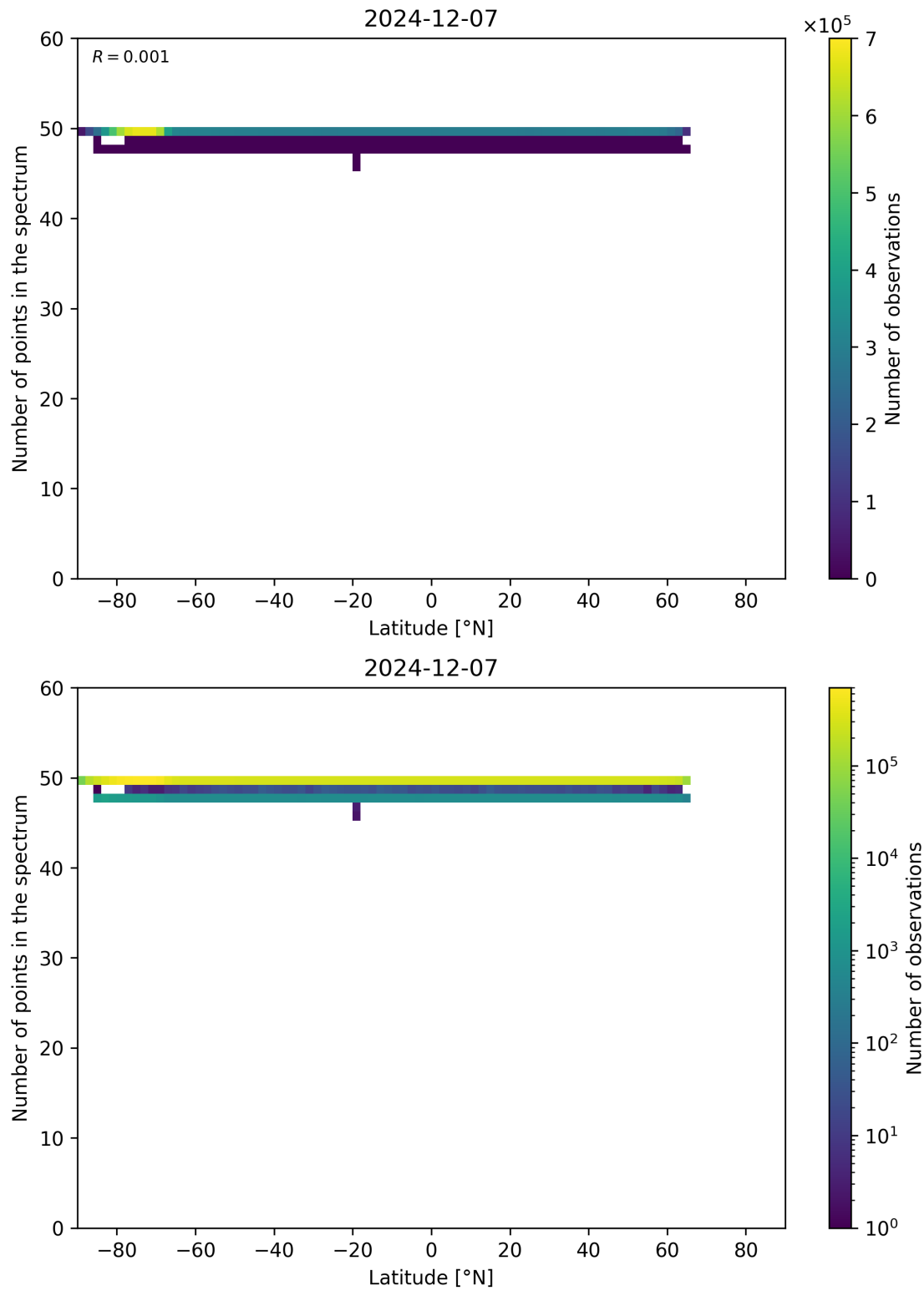
Figure 94: Scatter density plot of “Latitude” against “Number of points in the spectrum” for 2024-12-06 to 2024-12-08.
