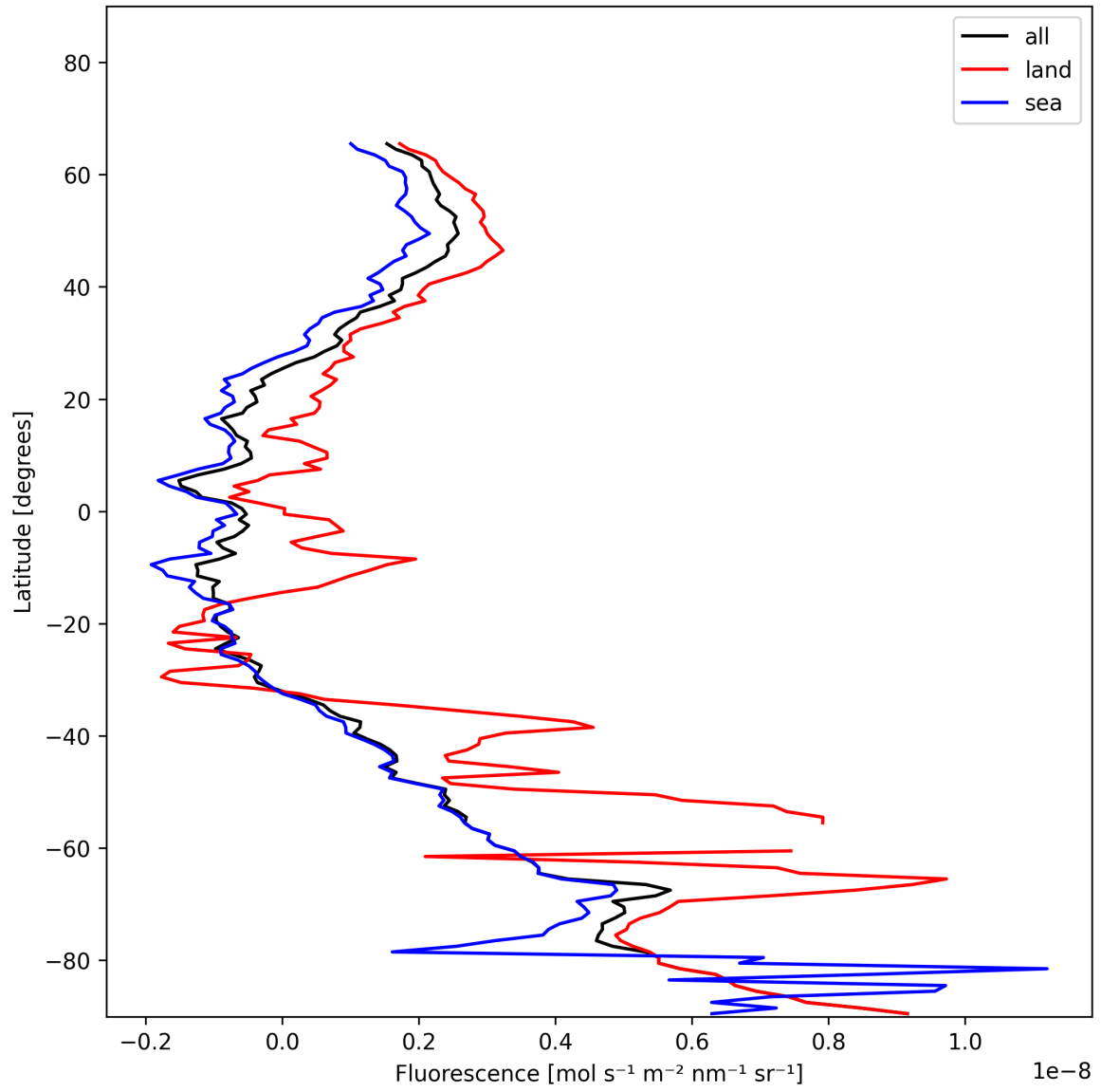
Figure 23: Zonal average of “Fluorescence” for 2024-12-06 to 2024-12-08.
