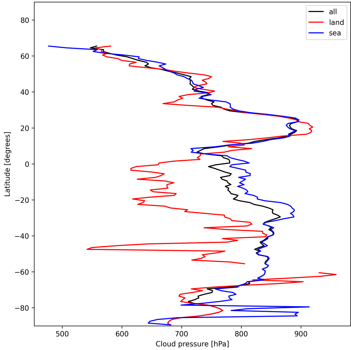
Figure 13: Zonal average of “Cloud pressure” for 2024-12-06 to 2024-12-08.
