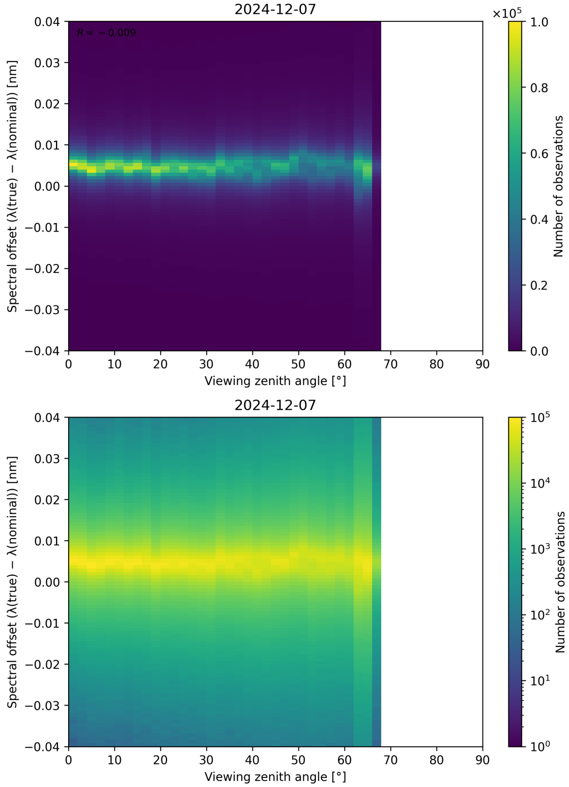
Figure 128: Scatter density plot of “Viewing zenith angle” against “Spectral offset ( \lambda_{\text{true}} - \lambda_{\text{nominal}} )” for 2024-12-06 to 2024-12-08.
