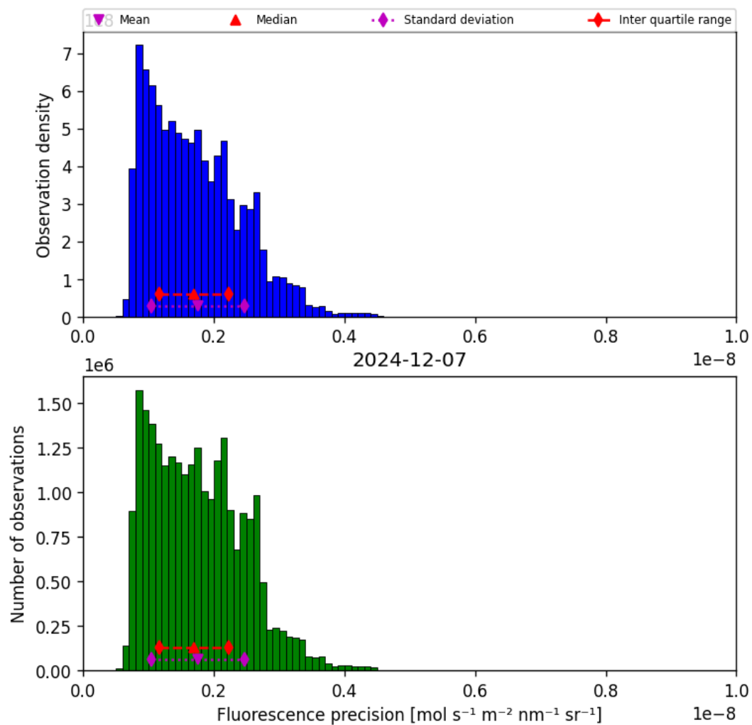
Figure 41: Histogram of “Fluorescence precision” for 2024-12-06 to 2024-12-08
