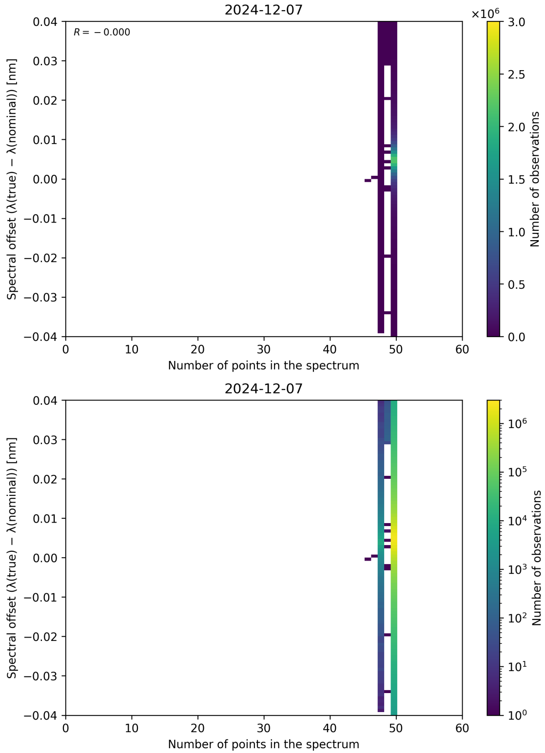
Figure 101: Scatter density plot of “Number of points in the spectrum” against “Spectral offset ( \lambda_{\text{true}} - \lambda_{\text{nominal}} )” for 2024-12-06 to 2024-12-08.
