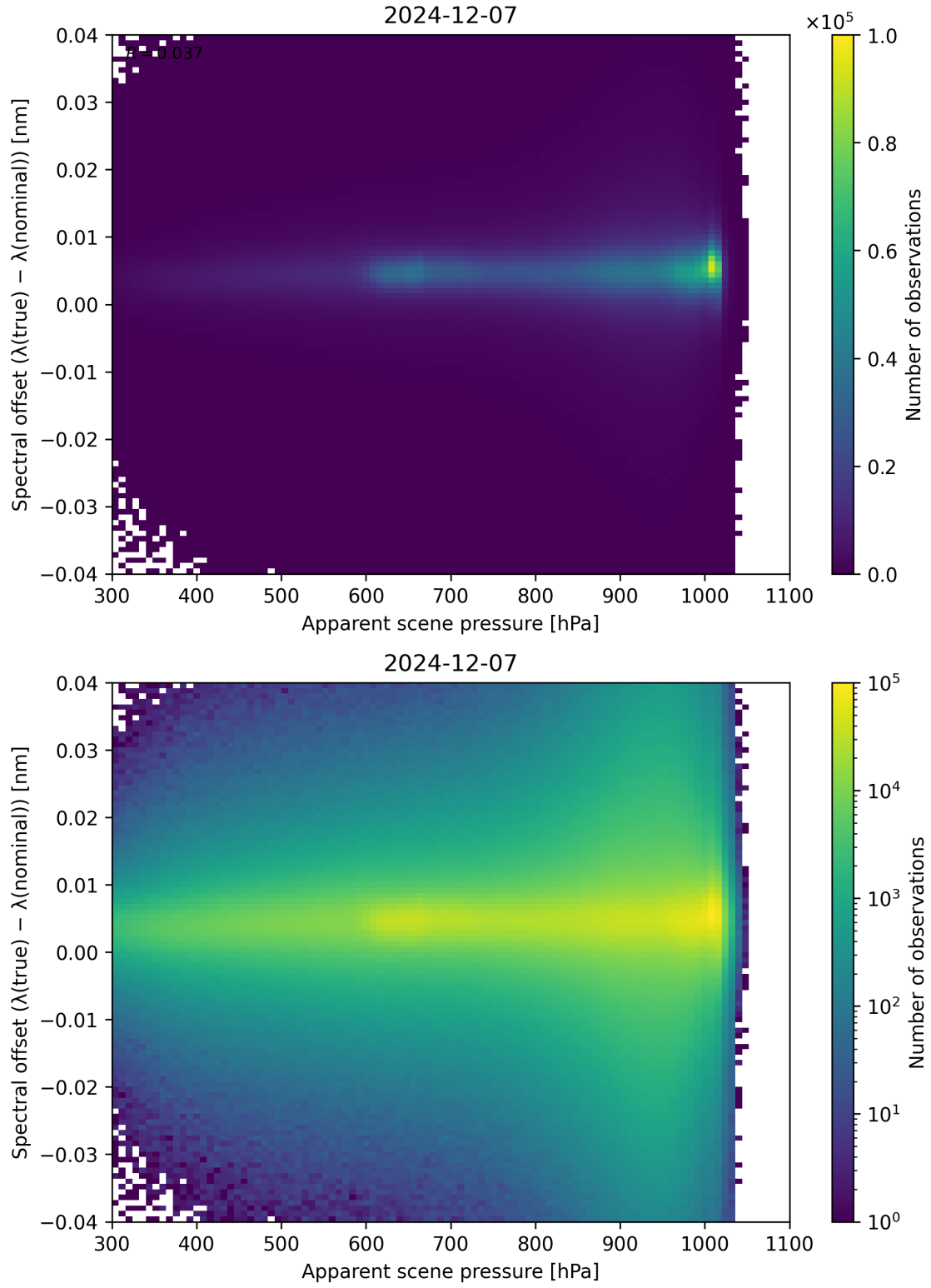
Figure 67: Scatter density plot of “Apparent scene pressure” against “Spectral offset ( \lambda_{\text{true}} - \lambda_{\text{nominal}} )” for 2024-12-06 to 2024-12-08.
