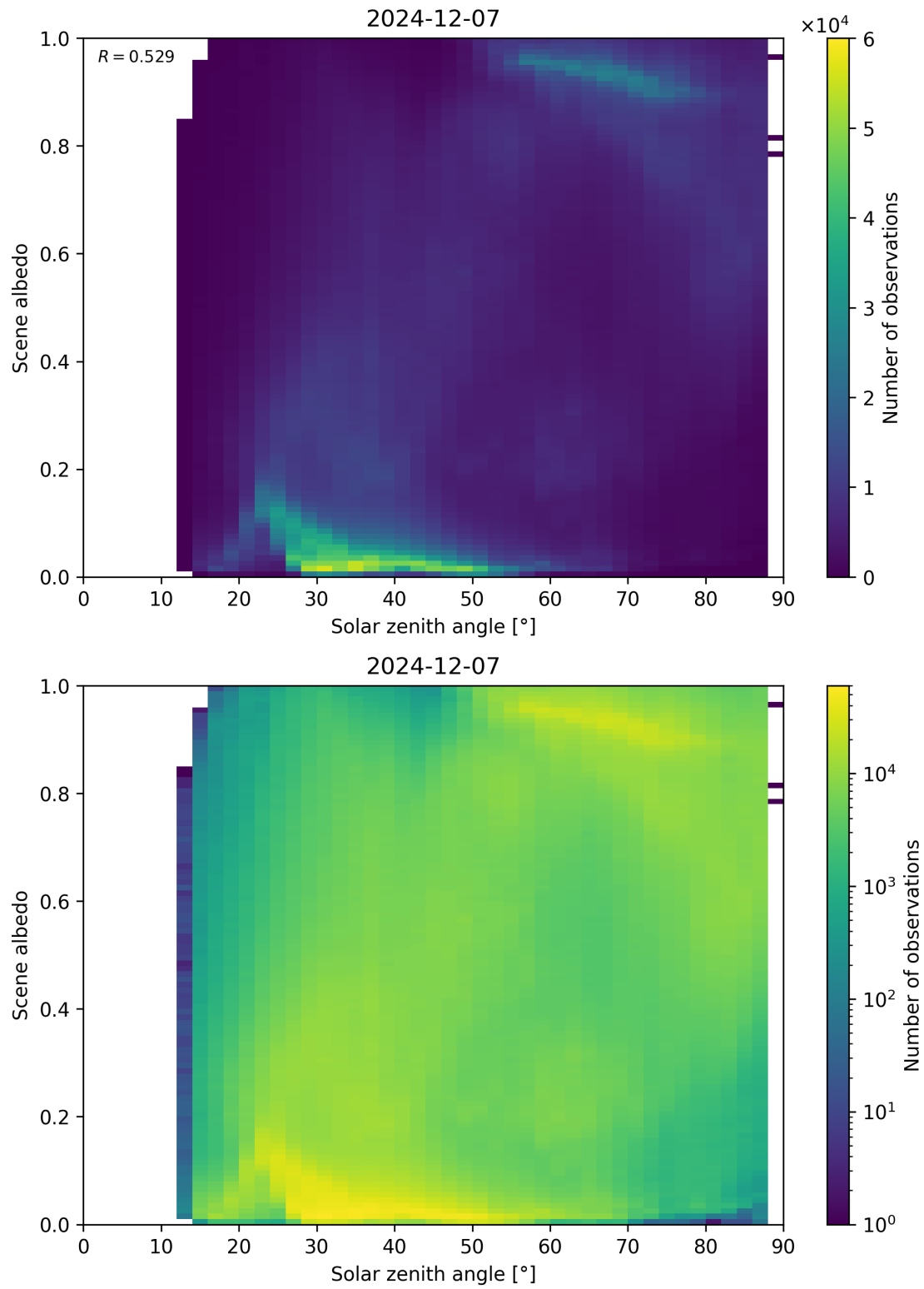
Figure 116: Scatter density plot of “Solar zenith angle” against “Scene albedo” for 2024-12-06 to 2024-12-08.
