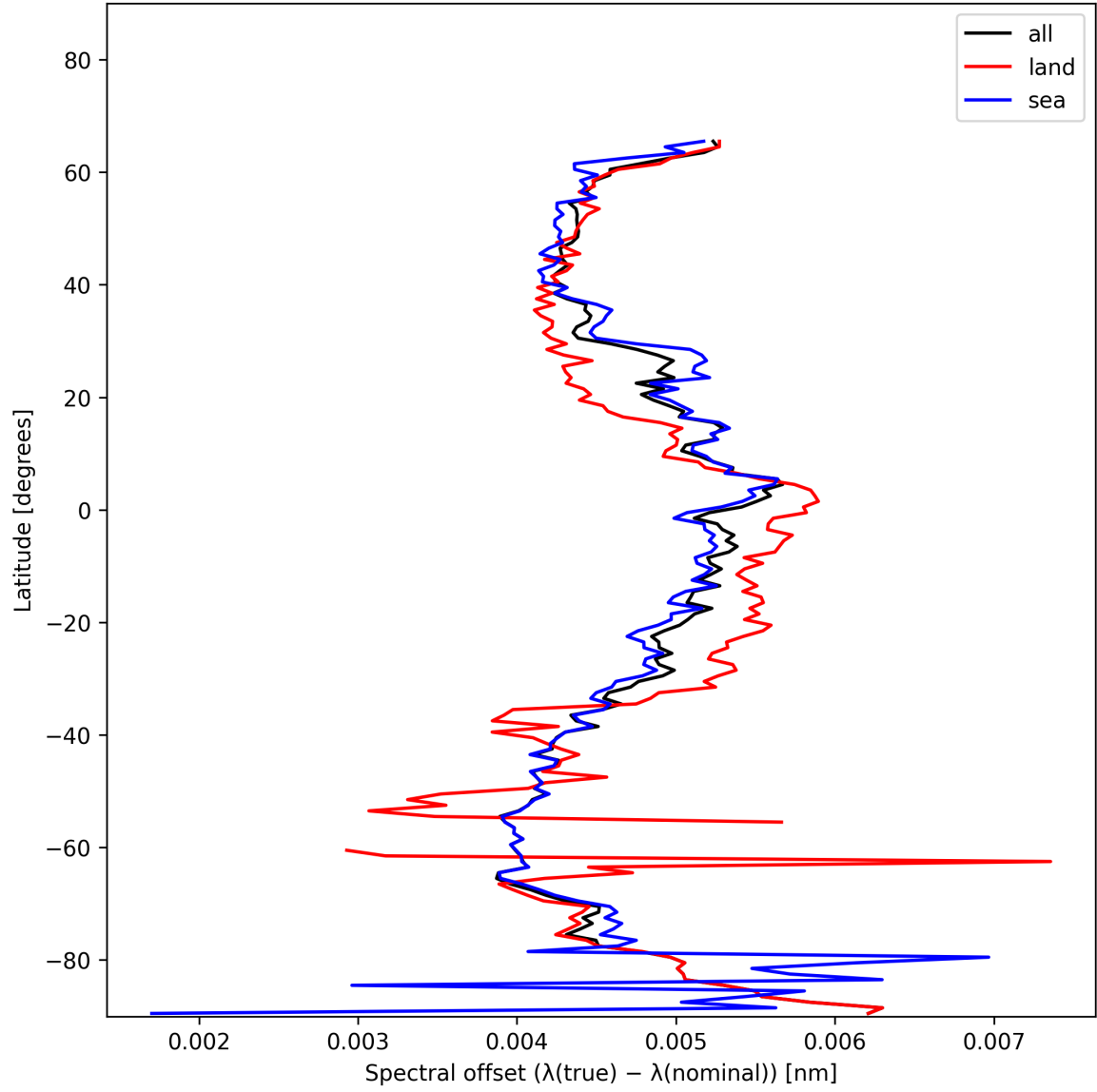
Figure 28: Zonal average of “Spectral offset ( \lambda_{\text{true}} - \lambda_{\text{nominal}} )” for 2024-12-06 to 2024-12-08.
