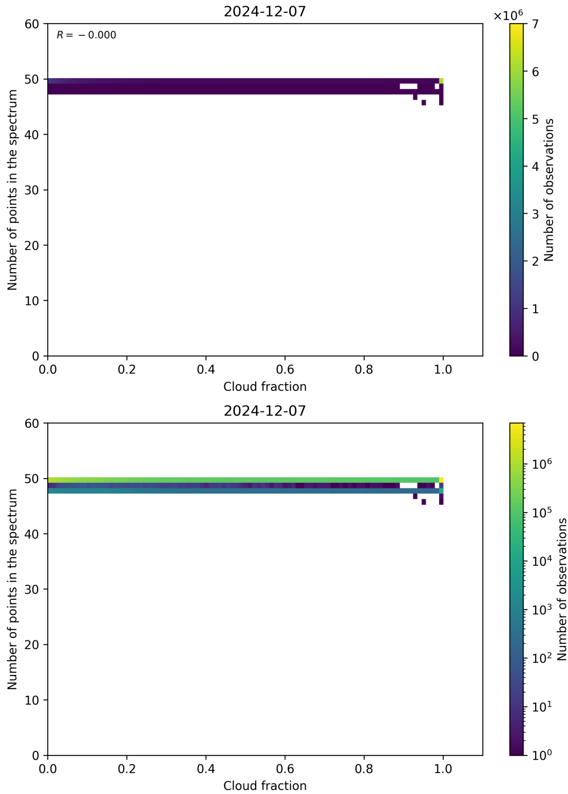
Figure 74: Scatter density plot of “Cloud fraction” against “Number of points in the spectrum” for 2024-12-06 to 2024-12-08.
