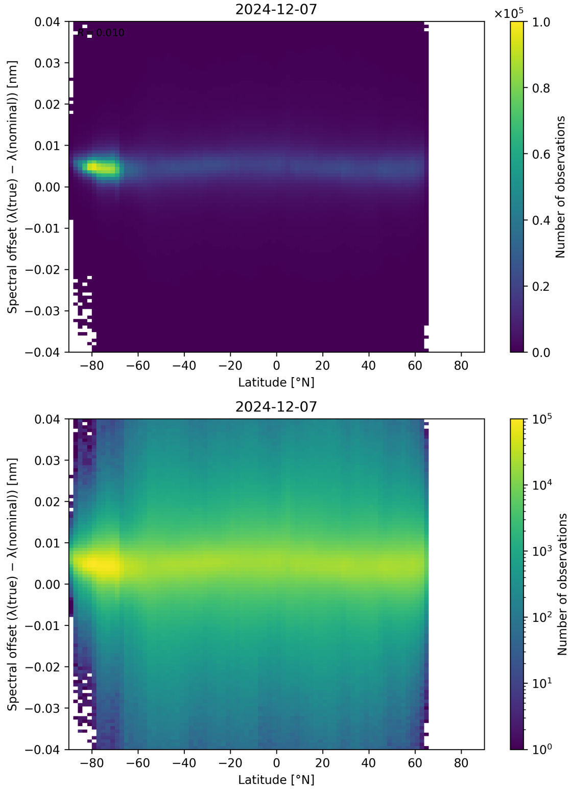
Figure 96: Scatter density plot of “Latitude” against “Spectral offset ( \lambda_{\text{true}} - \lambda_{\text{nominal}} )” for 2024-12-06 to 2024-12-08.
