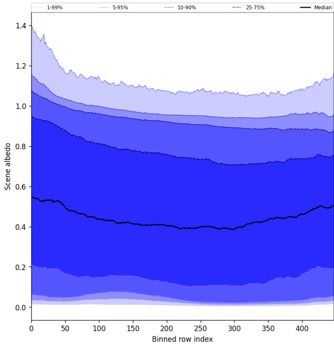
Figure 51: Along track statistics of “Scene albedo” for 2024-12-06 to 2024-12-08
