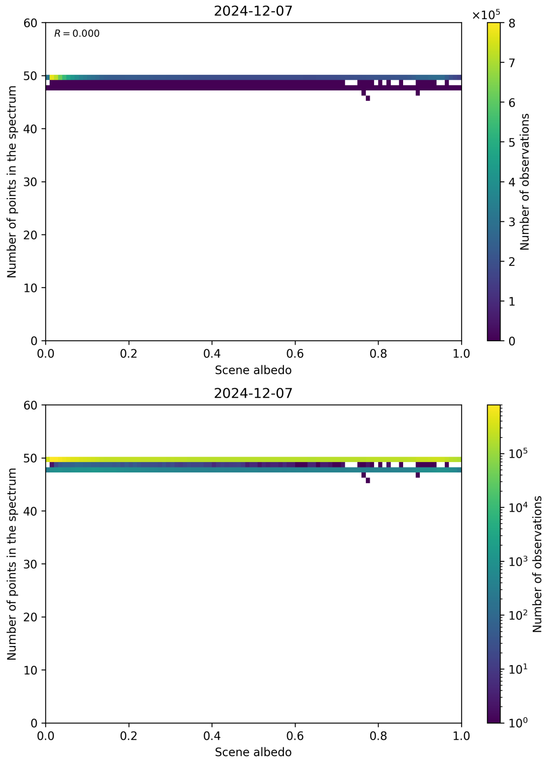
Figure 106: Scatter density plot of “Scene albedo” against “Number of points in the spectrum” for 2024-12-06 to 2024-12-08.
