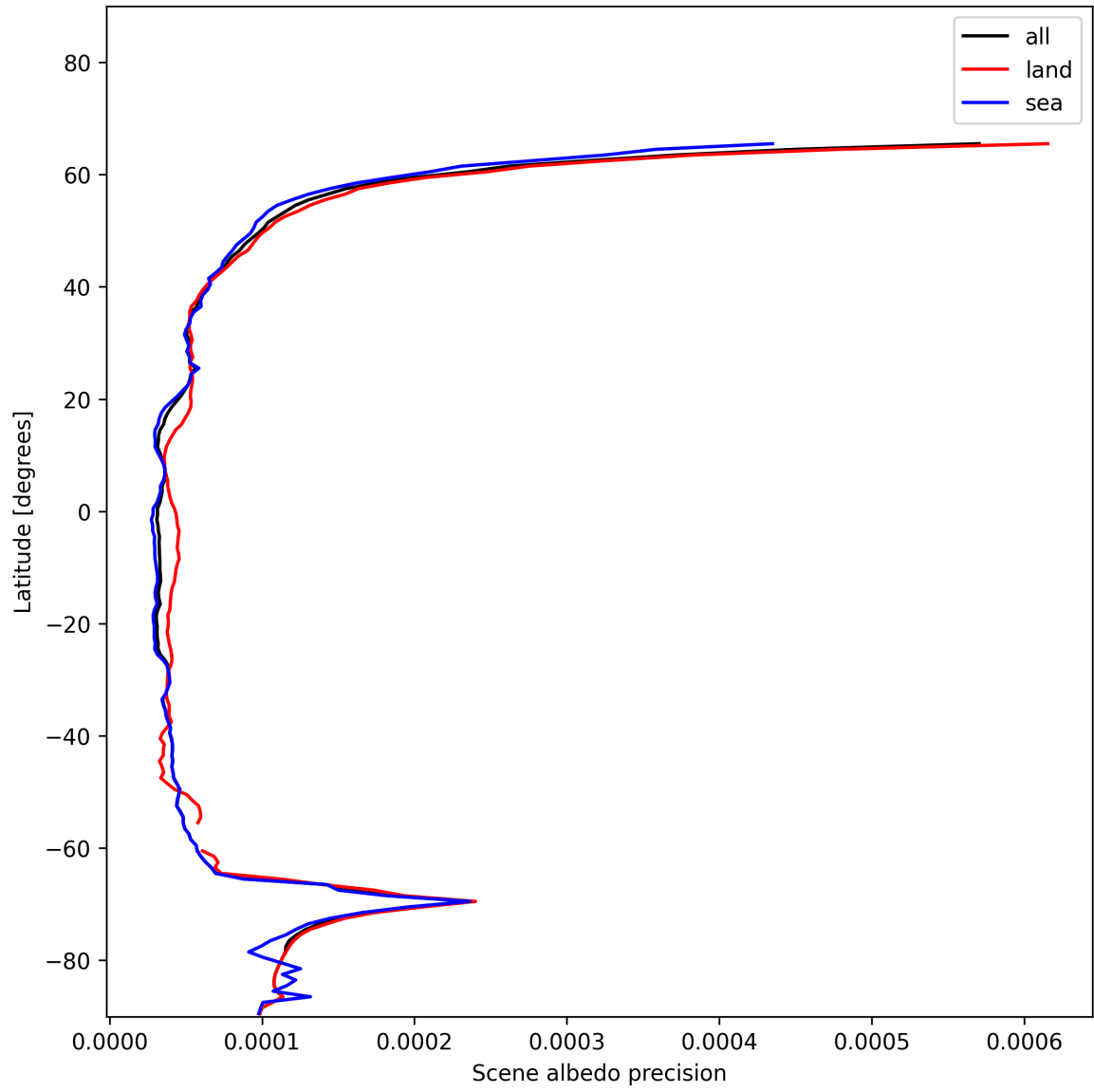
Figure 18: Zonal average of “Scene albedo precision” for 2024-12-06 to 2024-12-08.
