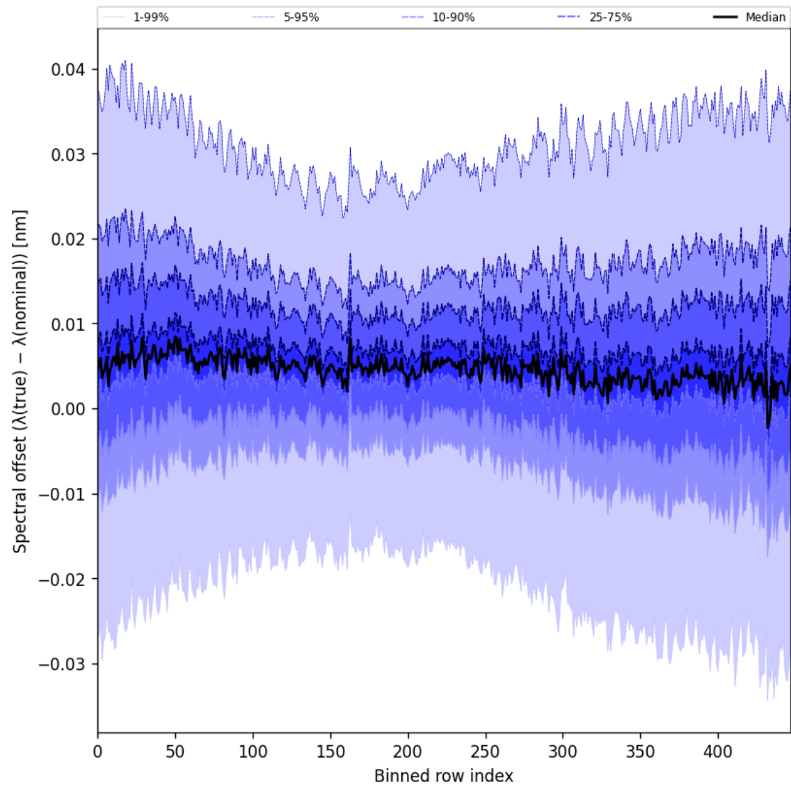
Figure 62: Along track statistics of “Spectral offset ( \lambda_{\text{true}} - \lambda_{\text{nominal}} )” for 2024-12-06 to 2024-12-08
