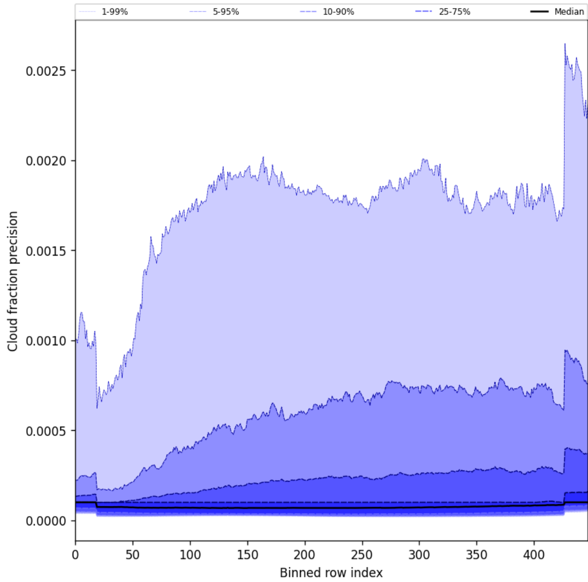
Figure 50: Along track statistics of “Cloud fraction precision” for 2024-12-06 to 2024-12-08
