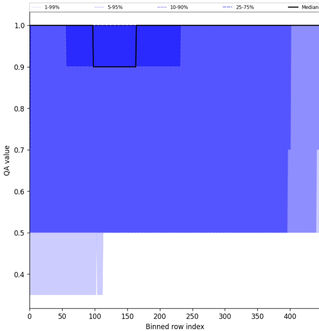
Figure 46: Along track statistics of “QA value” for 2024-12-06 to 2024-12-08
