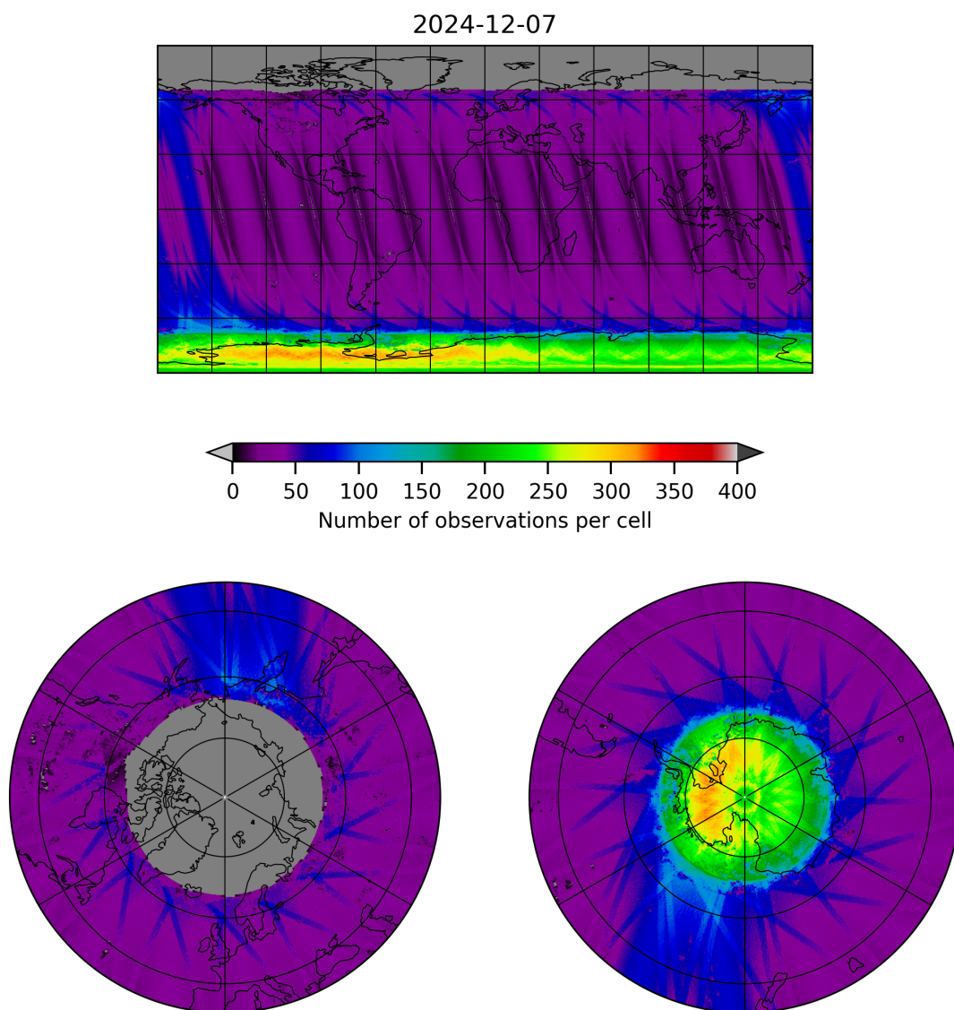
Figure 11: Map of the number of observations for 2024-12-06 to 2024-12-08
