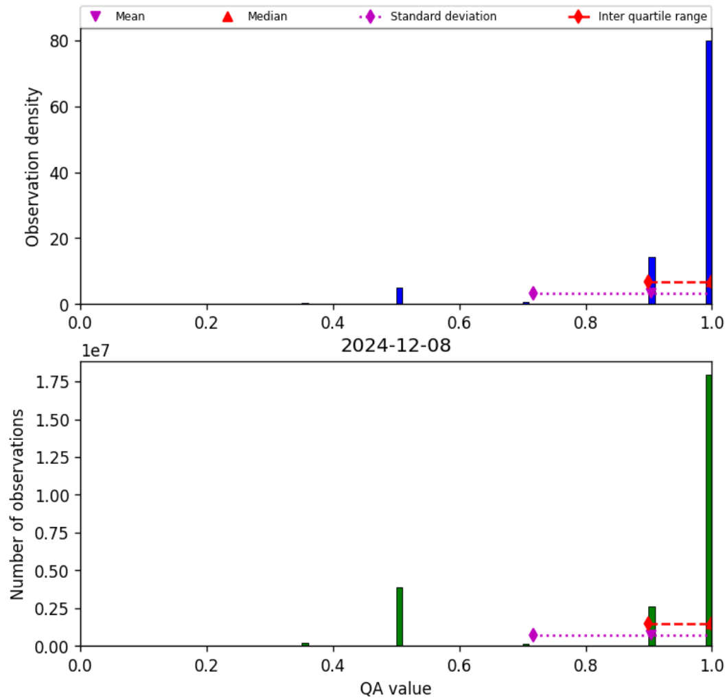
Figure 29: Histogram of “QA value” for 2024-12-07 to 2024-12-09
