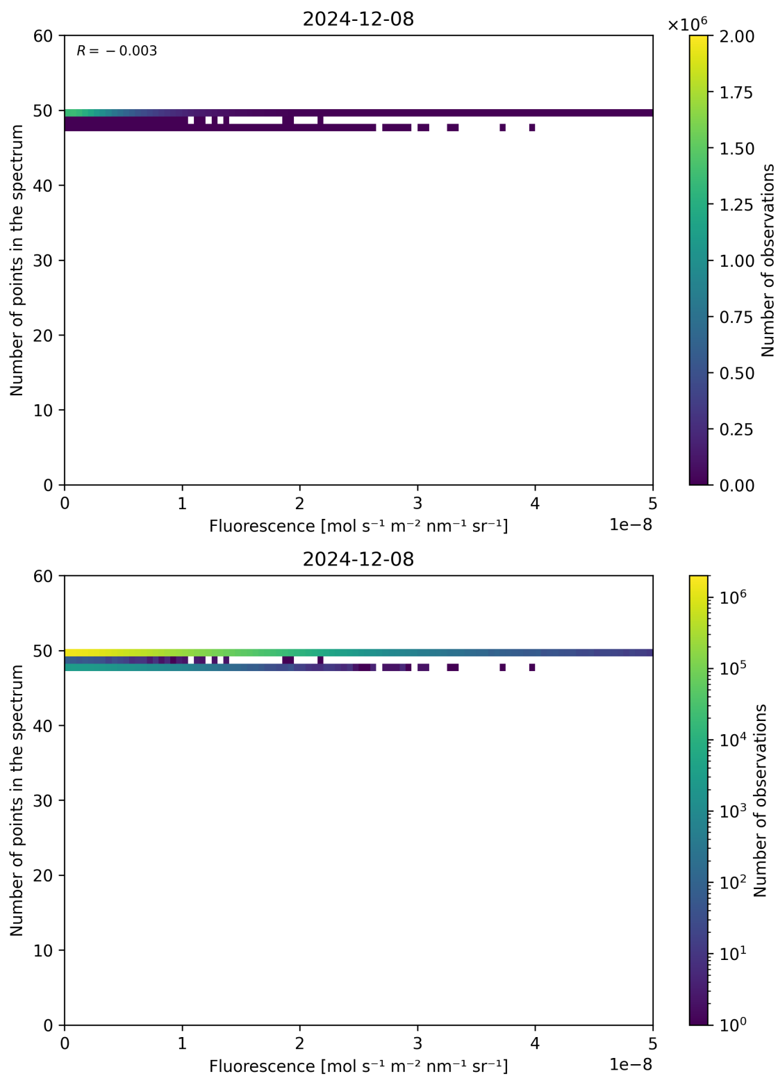
Figure 86: Scatter density plot of “Fluorescence” against “Number of points in the spectrum” for 2024-12-07 to 2024-12-09.
