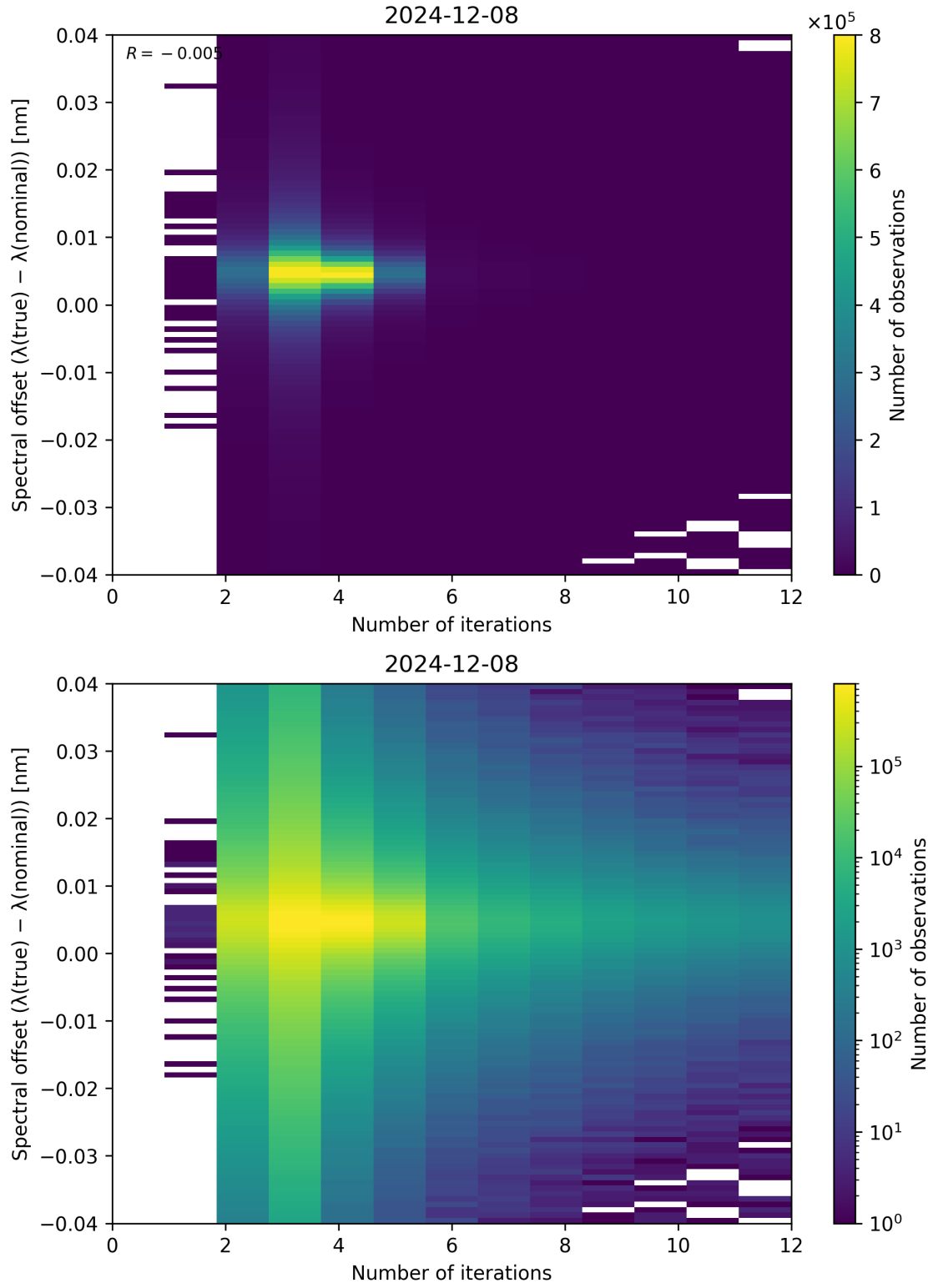
Figure 100: Scatter density plot of “Number of iterations” against “Spectral offset ( \lambda_{\text{true}} - \lambda_{\text{nominal}} )” for 2024-12-07 to 2024-12-09.
