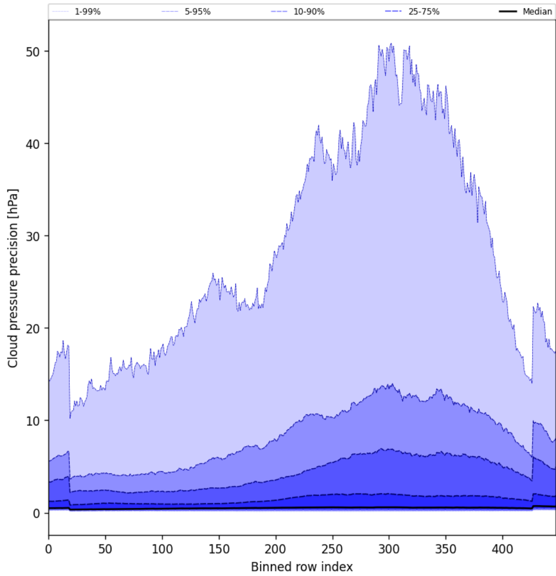
Figure 48: Along track statistics of “Cloud pressure precision” for 2024-12-07 to 2024-12-09
