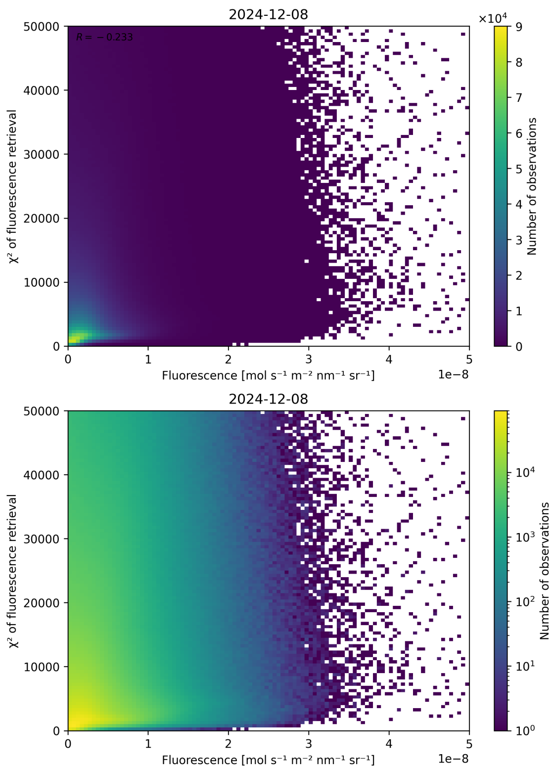
Figure 85: Scatter density plot of “Fluorescence” against “ \chi^2 of fluorescence retrieval” for 2024-12-07 to 2024-12-09.
