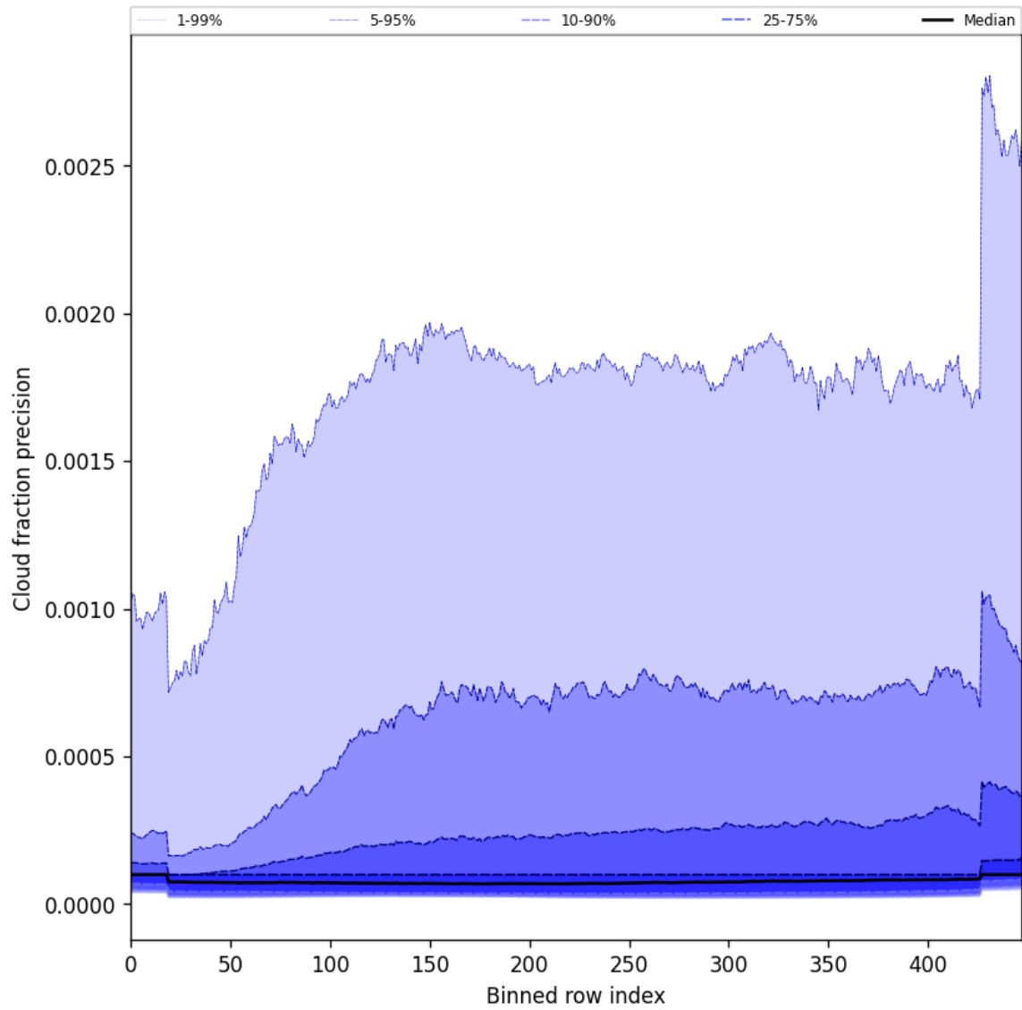
Figure 50: Along track statistics of “Cloud fraction precision” for 2024-12-07 to 2024-12-09
