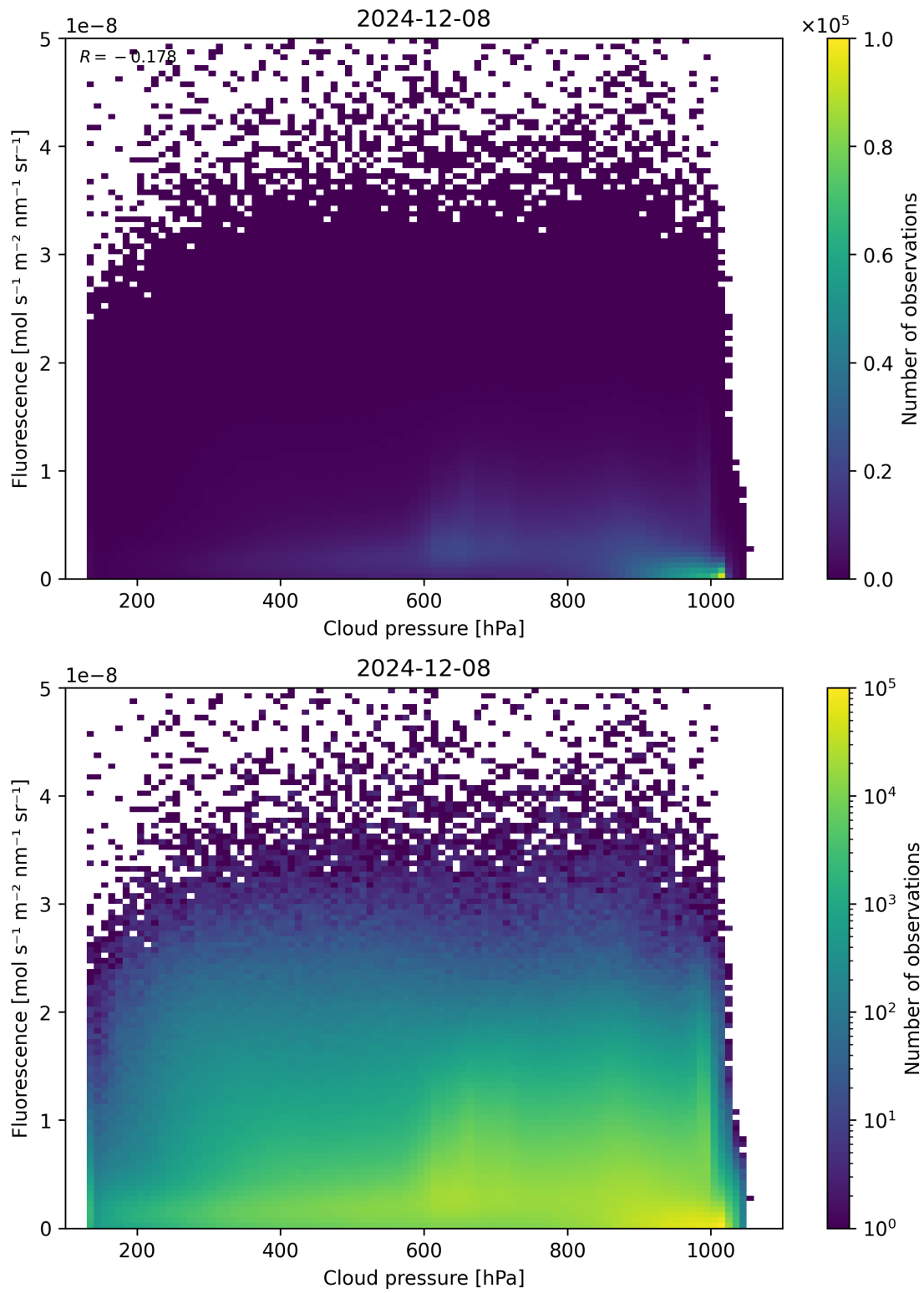
Figure 80: Scatter density plot of “Cloud pressure” against “Fluorescence” for 2024-12-07 to 2024-12-09.
