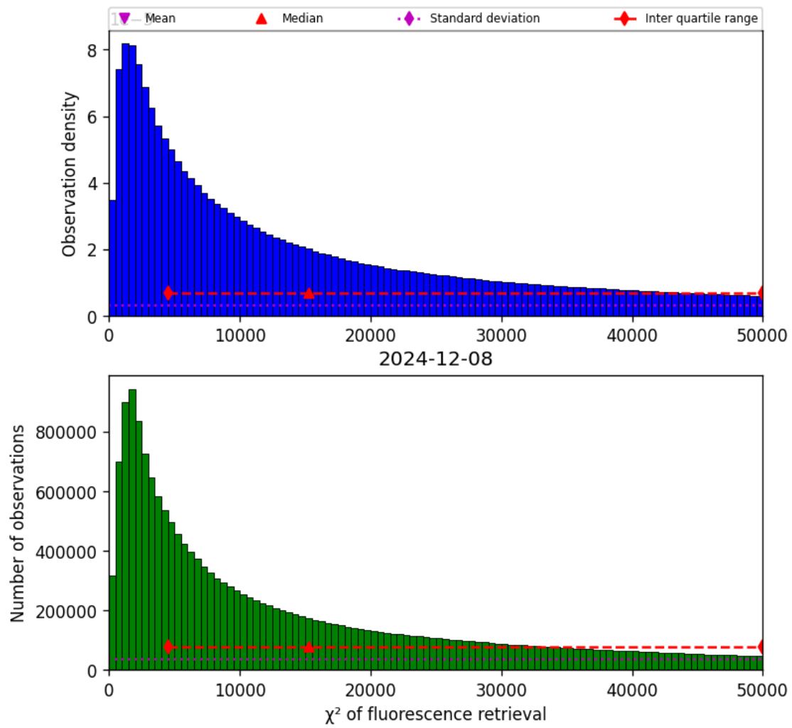
Figure 42: Histogram of “ \chi^2 of fluorescence retrieval” for 2024-12-07 to 2024-12-09
