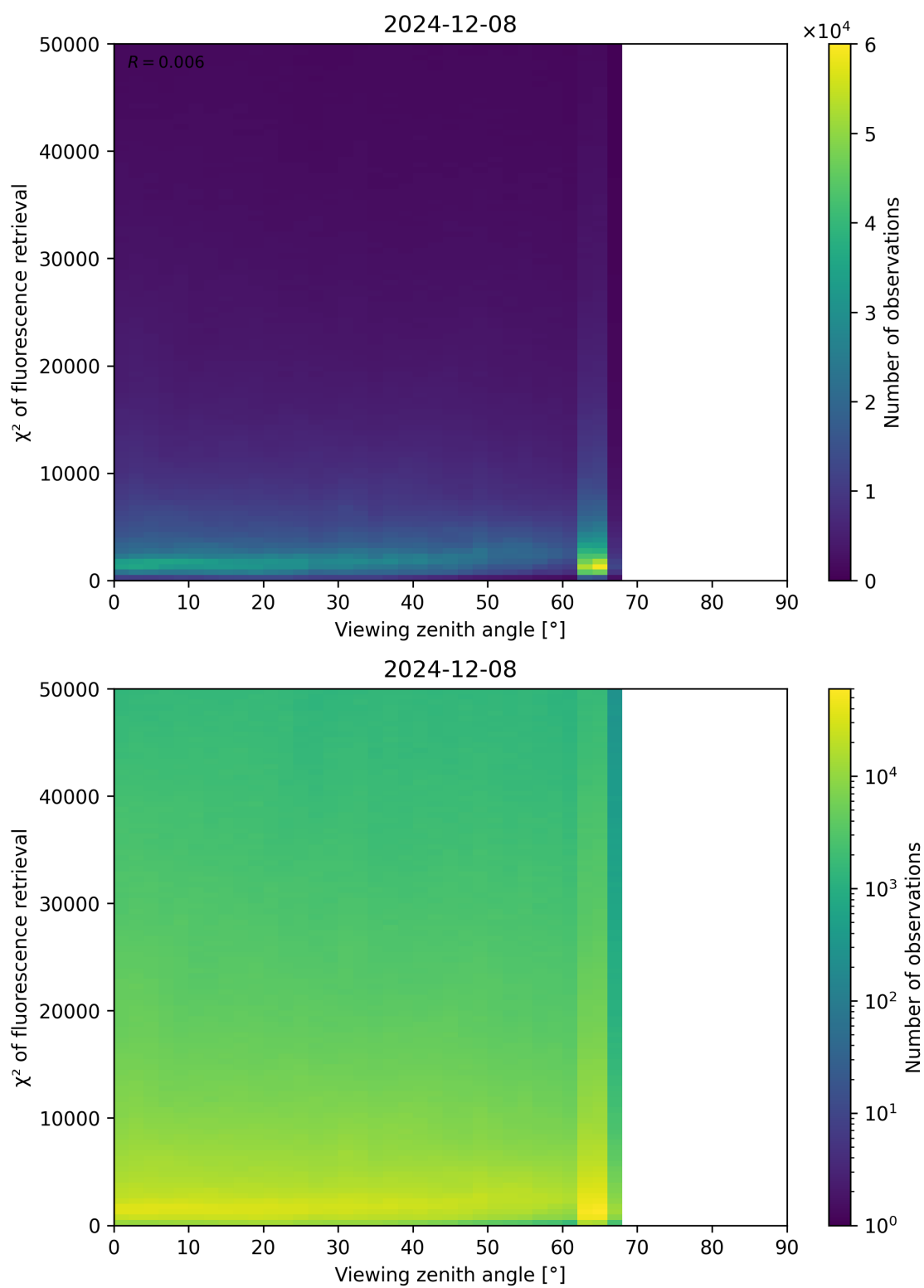
Figure 119: Scatter density plot of “Viewing zenith angle” against “ \chi^2 of fluorescence retrieval” for 2024-12-07 to 2024-12-09.
