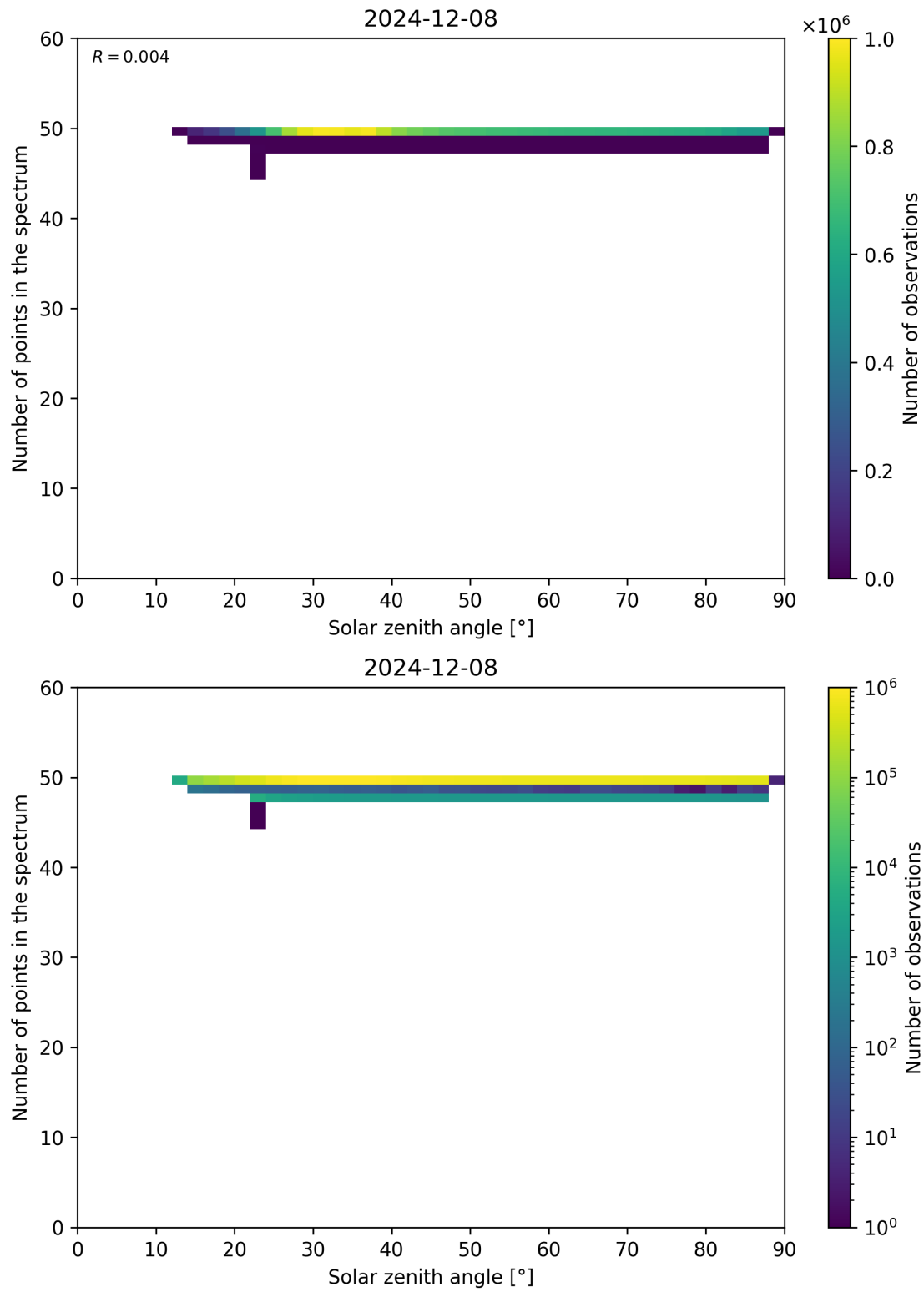
Figure 115: Scatter density plot of “Solar zenith angle” against “Number of points in the spectrum” for 2024-12-07 to 2024-12-09.
