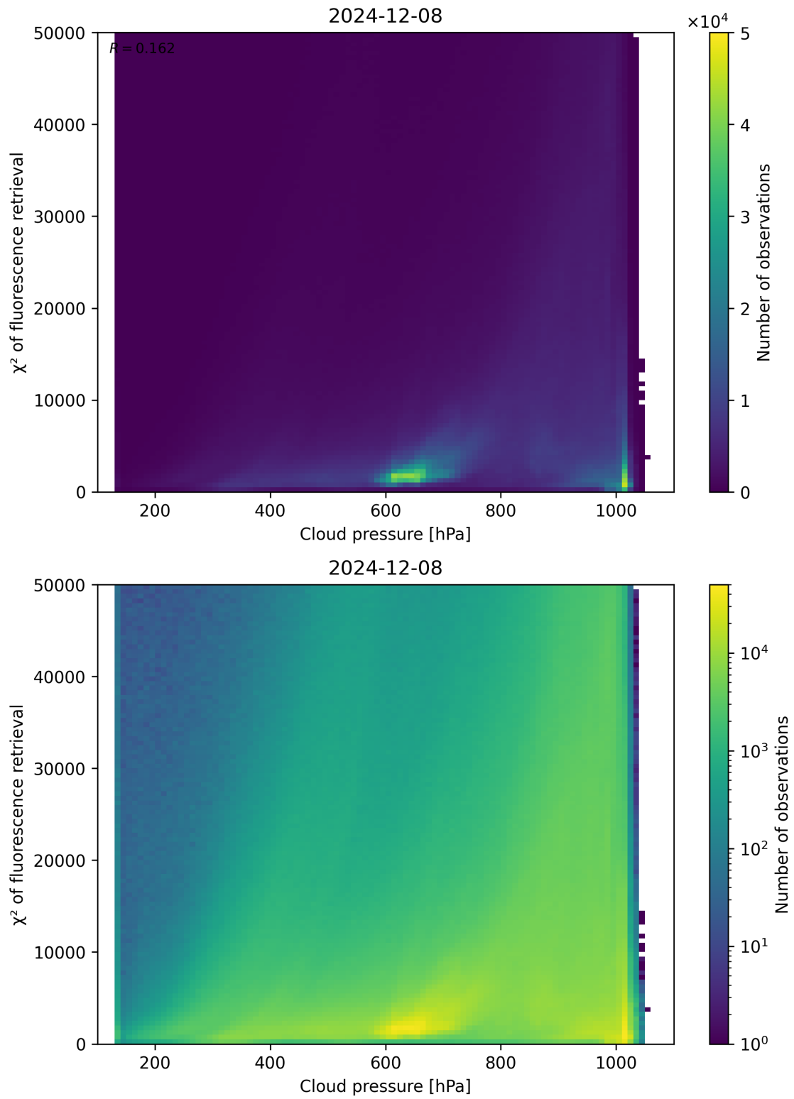
Figure 78: Scatter density plot of “Cloud pressure” against “ \chi^2 of fluorescence retrieval” for 2024-12-07 to 2024-12-09.
