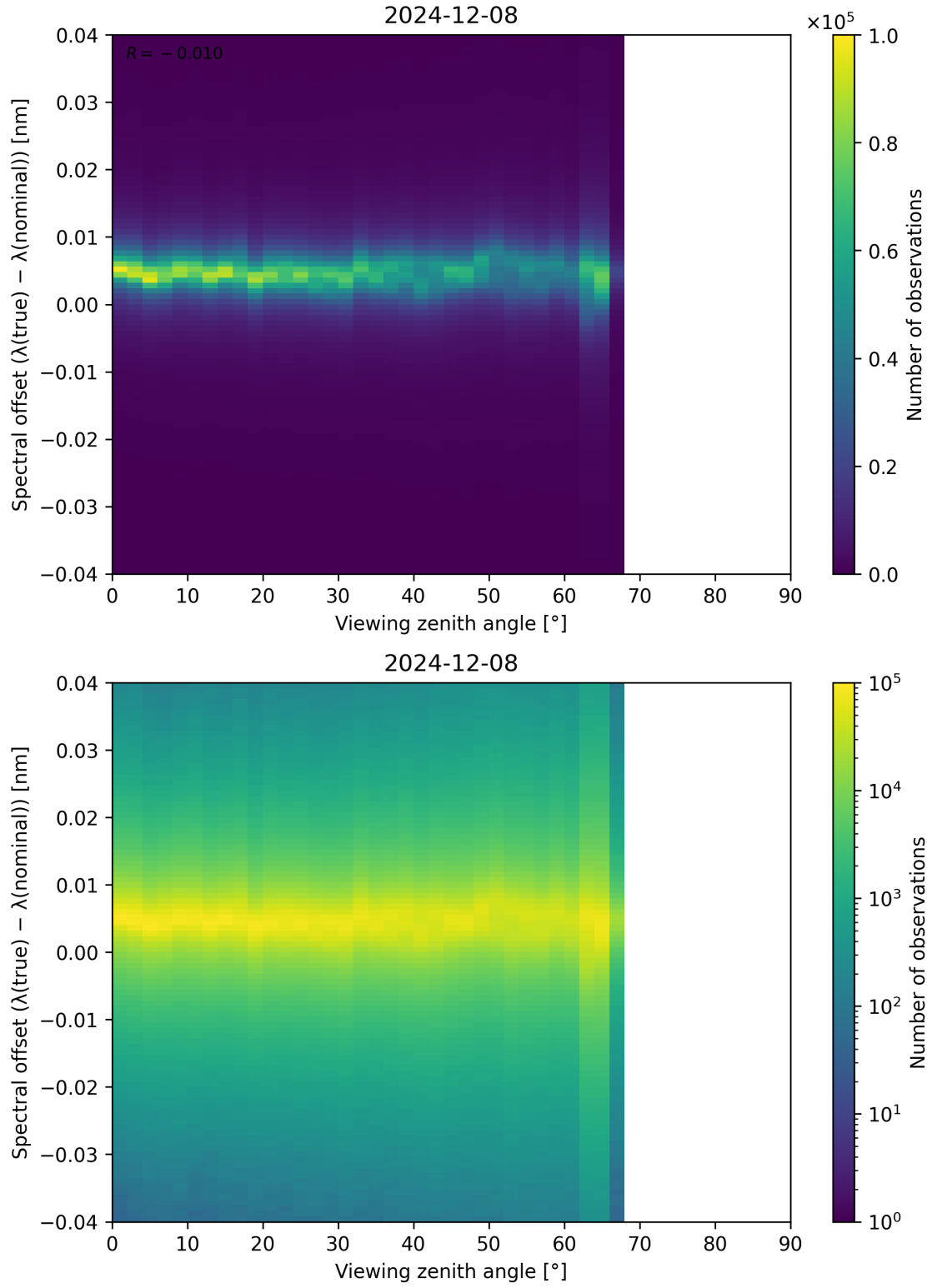
Figure 128: Scatter density plot of “Viewing zenith angle” against “Spectral offset ( \lambda_{\text{true}} - \lambda_{\text{nominal}} )” for 2024-12-07 to 2024-12-09.
