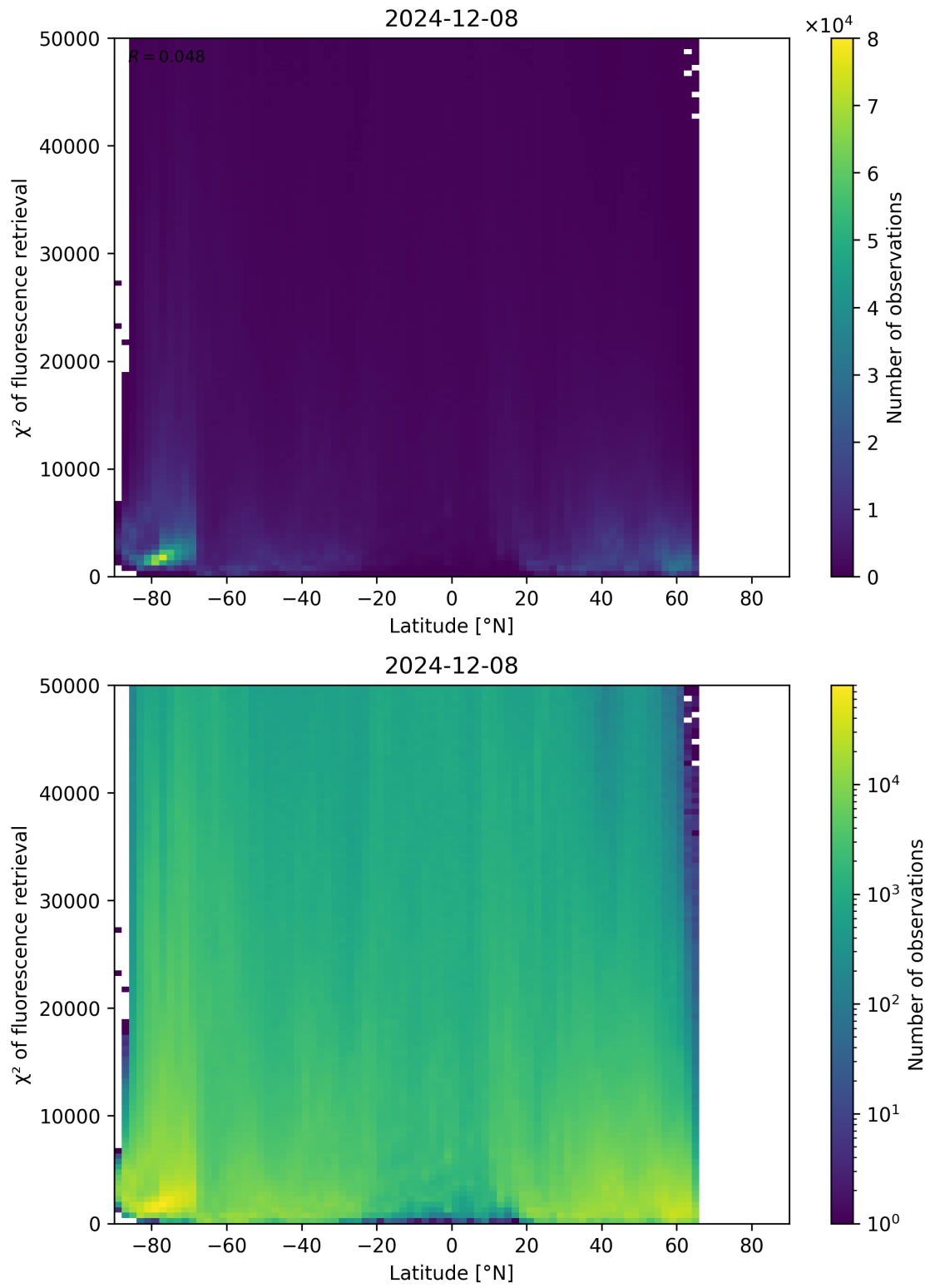
Figure 89: Scatter density plot of “Latitude” against “ \chi^2 of fluorescence retrieval” for 2024-12-07 to 2024-12-09.
