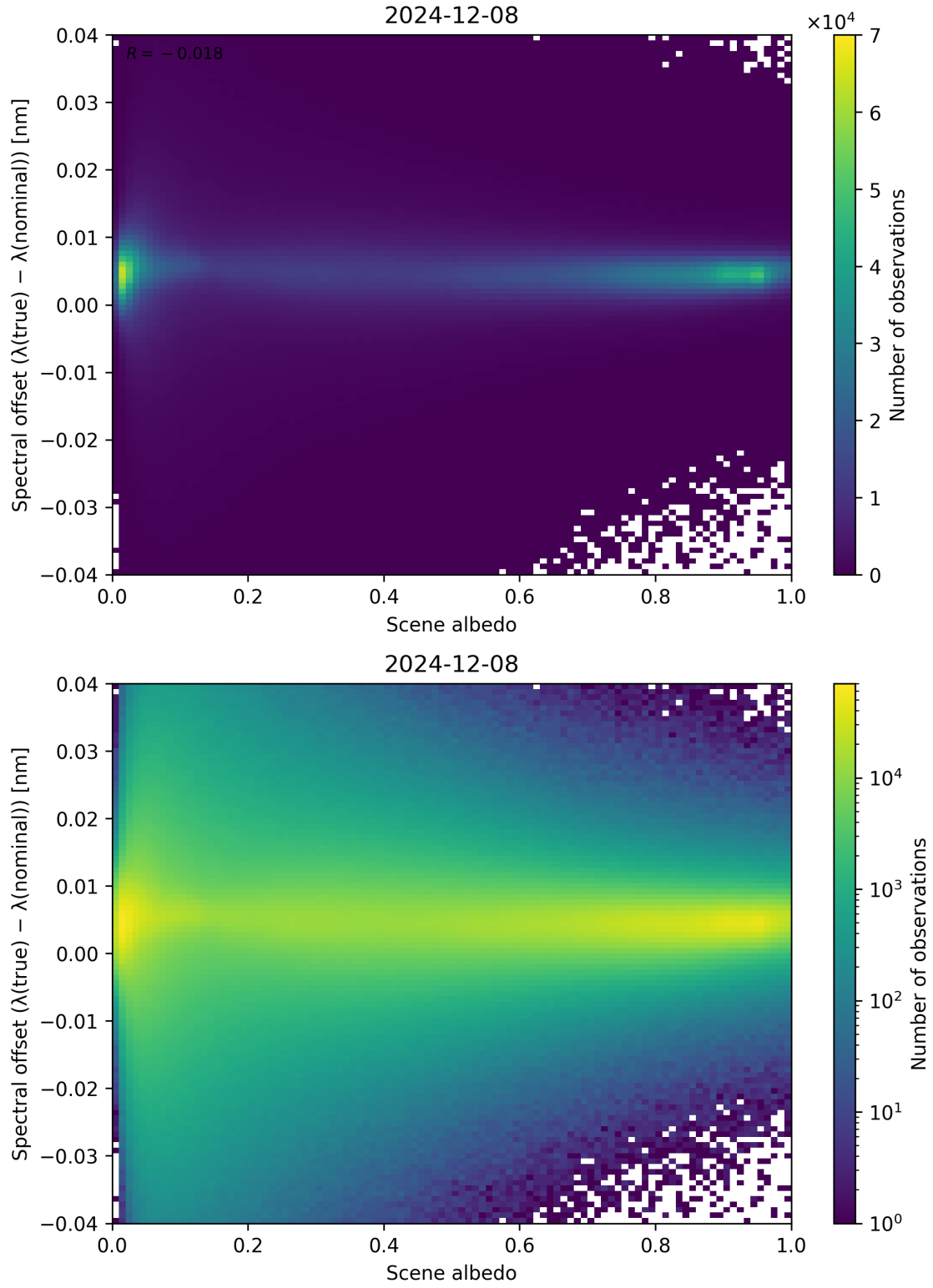
Figure 107: Scatter density plot of “Scene albedo” against “Spectral offset ( \lambda_{\text{true}} - \lambda_{\text{nominal}} )” for 2024-12-07 to 2024-12-09.
