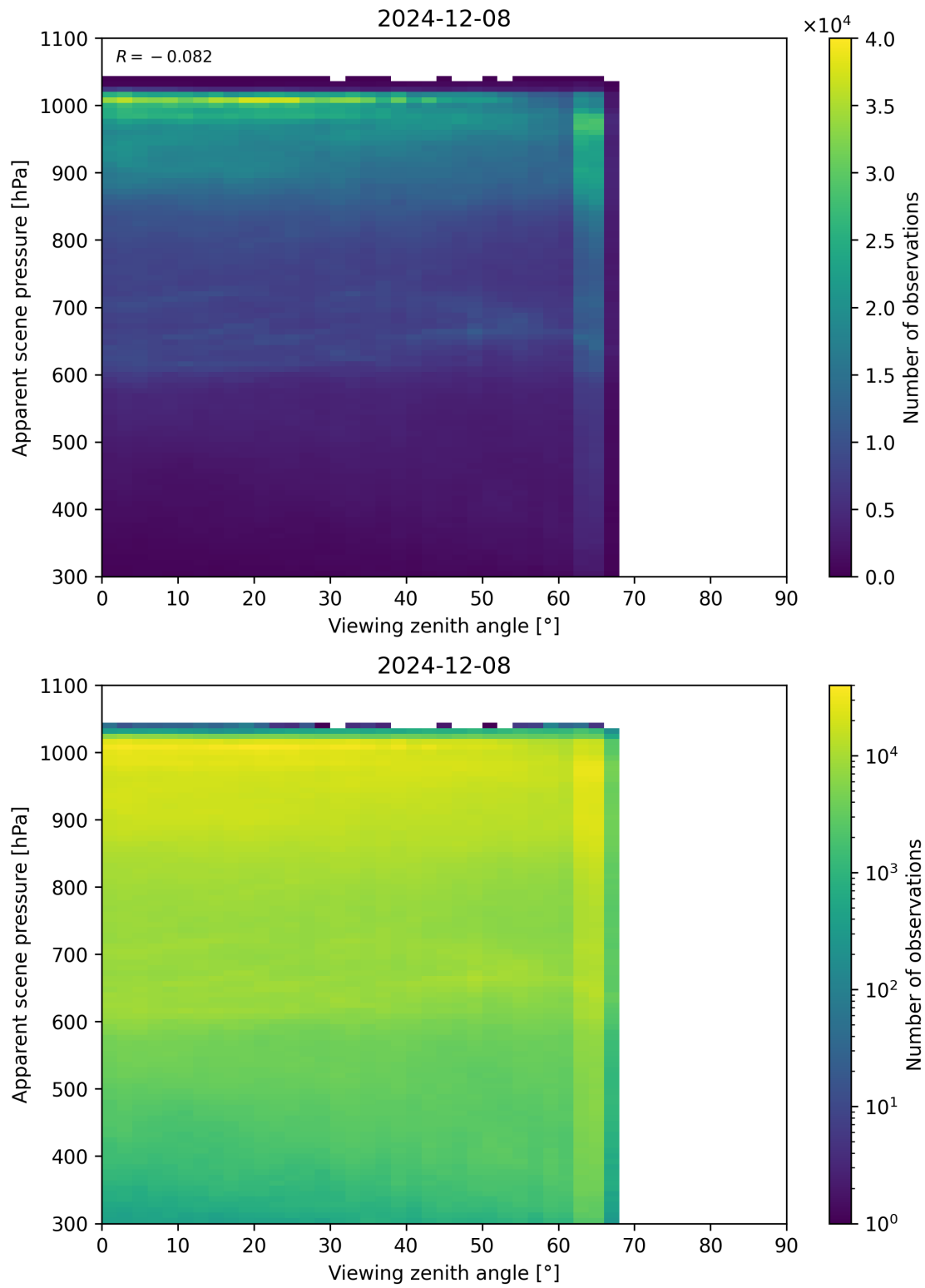
Figure 118: Scatter density plot of “Viewing zenith angle” against “Apparent scene pressure” for 2024-12-07 to 2024-12-09.
