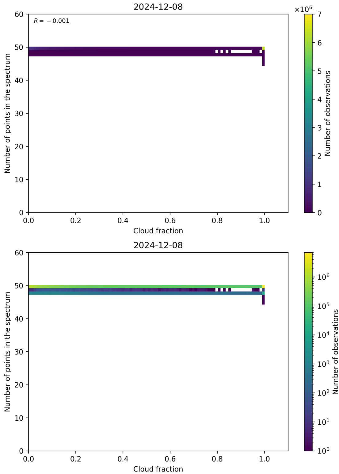
Figure 74: Scatter density plot of “Cloud fraction” against “Number of points in the spectrum” for 2024-12-07 to 2024-12-09.
