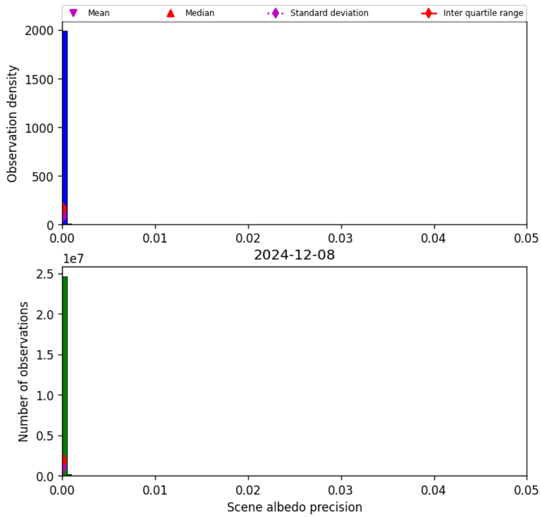
Figure 35: Histogram of “Scene albedo precision” for 2024-12-07 to 2024-12-09
