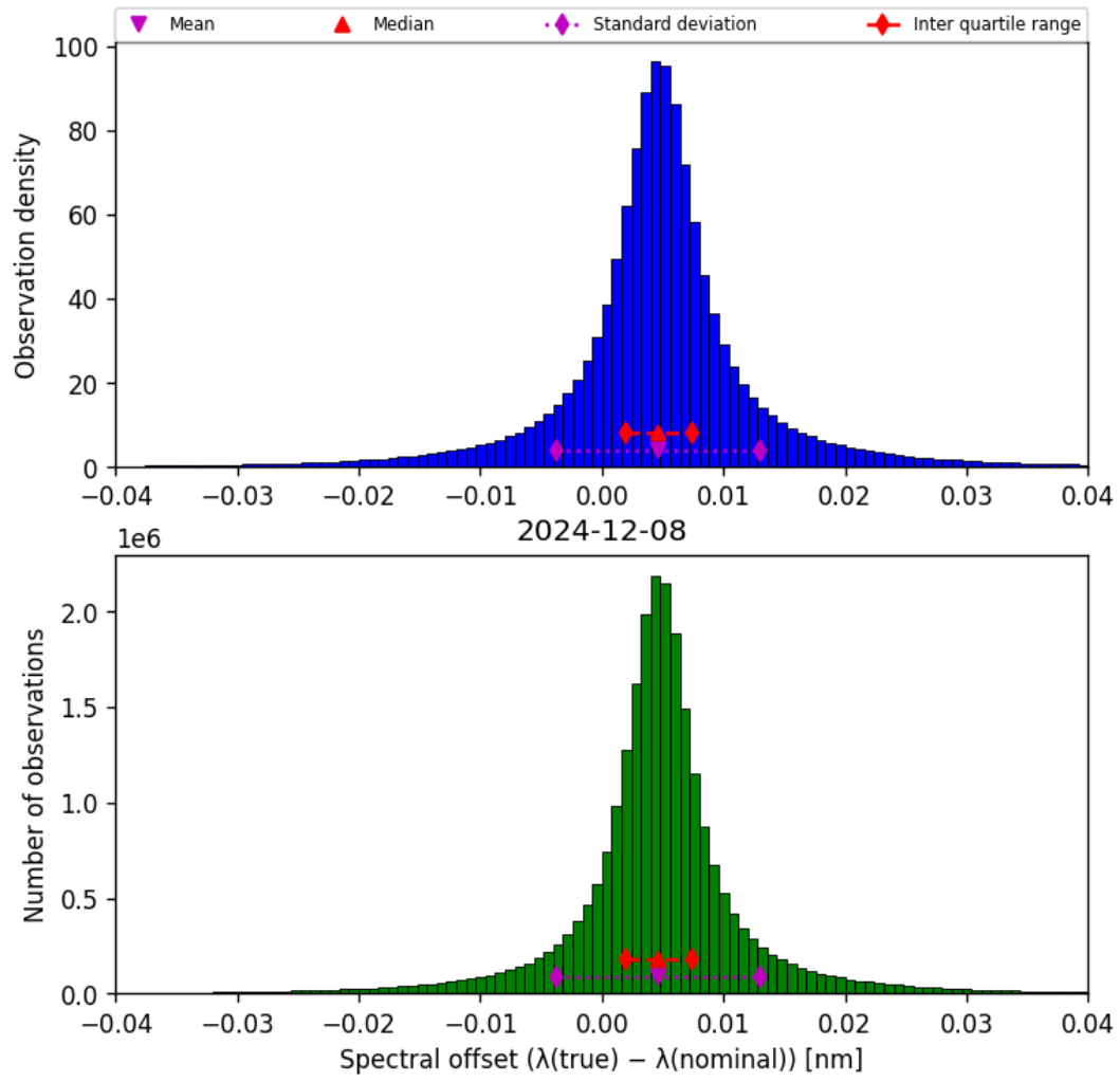
Figure 45: Histogram of “Spectral offset ( \lambda_{\text{true}} - \lambda_{\text{nominal}} )” for 2024-12-07 to 2024-12-09
