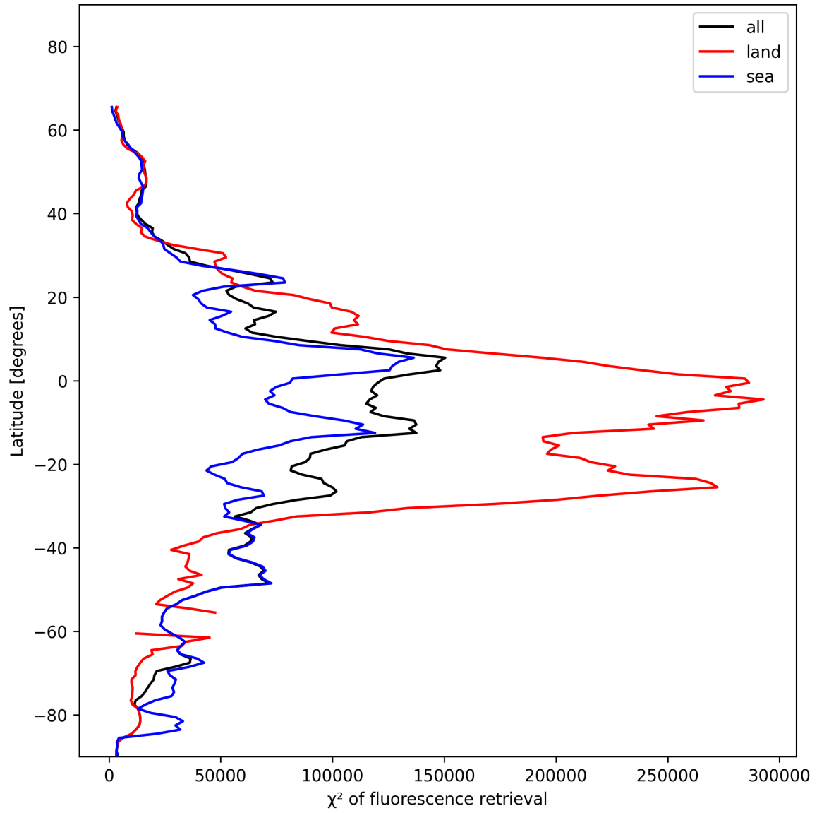
Figure 25: Zonal average of “ \chi^2 of fluorescence retrieval” for 2024-12-07 to 2024-12-09.
