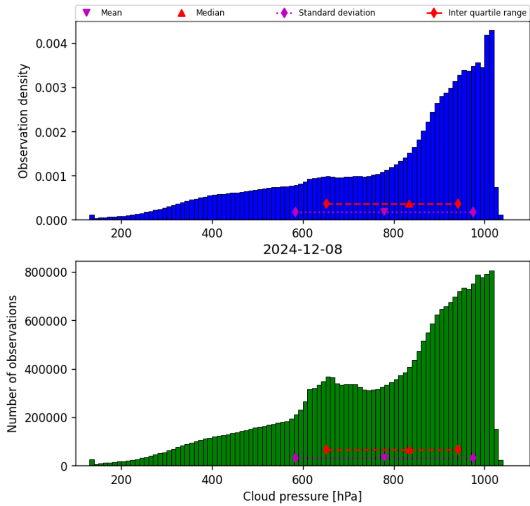
Figure 30: Histogram of “Cloud pressure” for 2024-12-07 to 2024-12-09
