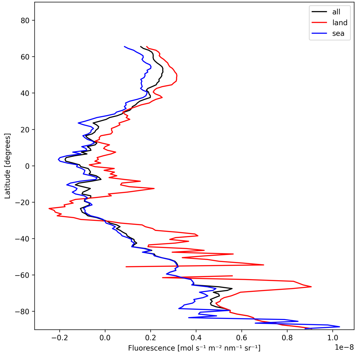
Figure 23: Zonal average of “Fluorescence” for 2024-12-07 to 2024-12-09.
