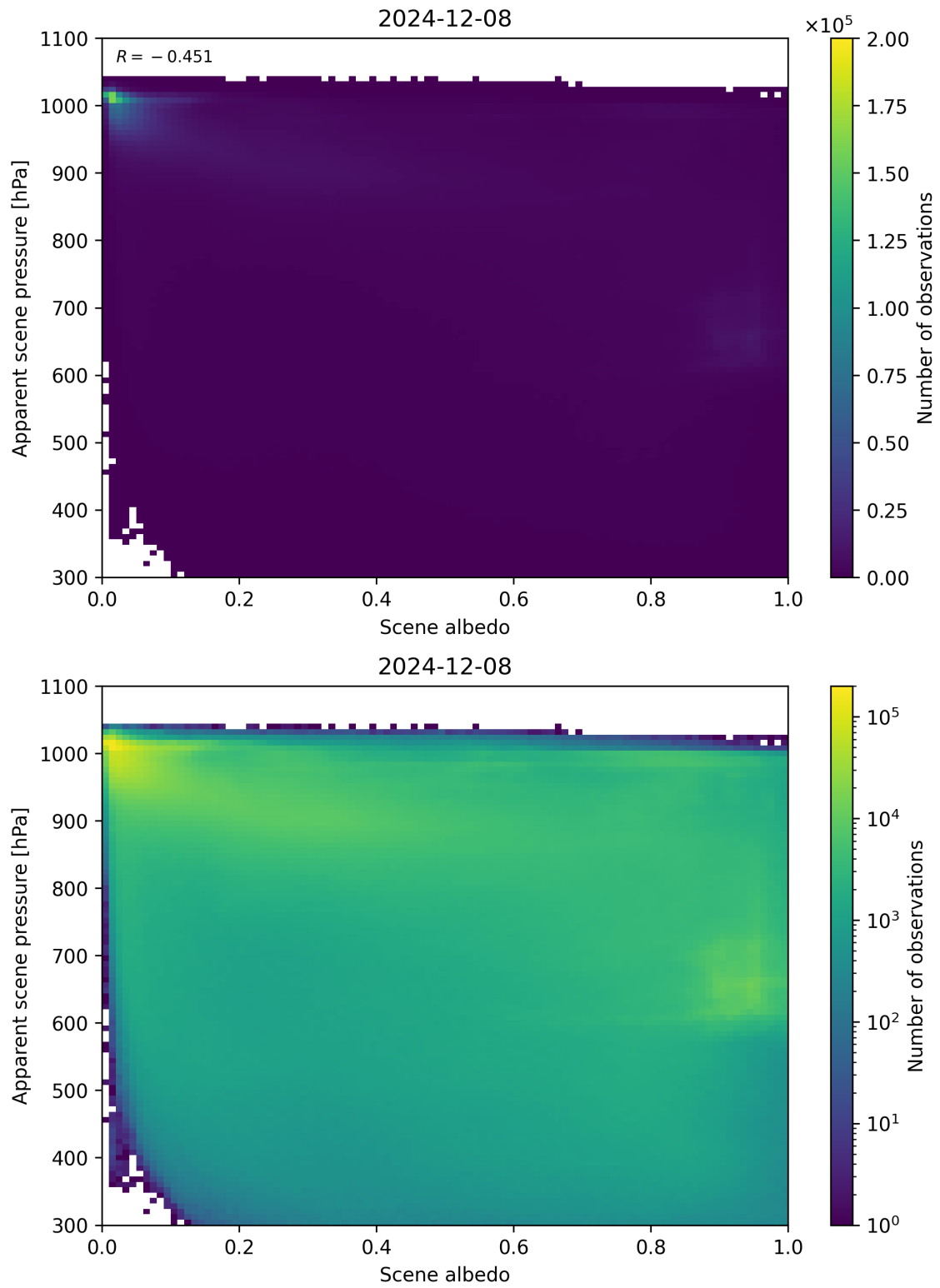
Figure 102: Scatter density plot of “Scene albedo” against “Apparent scene pressure” for 2024-12-07 to 2024-12-09.
