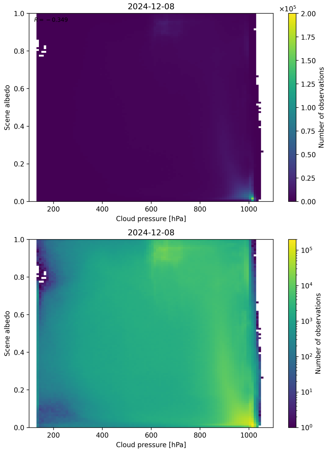
Figure 83: Scatter density plot of “Cloud pressure” against “Scene albedo” for 2024-12-07 to 2024-12-09.
