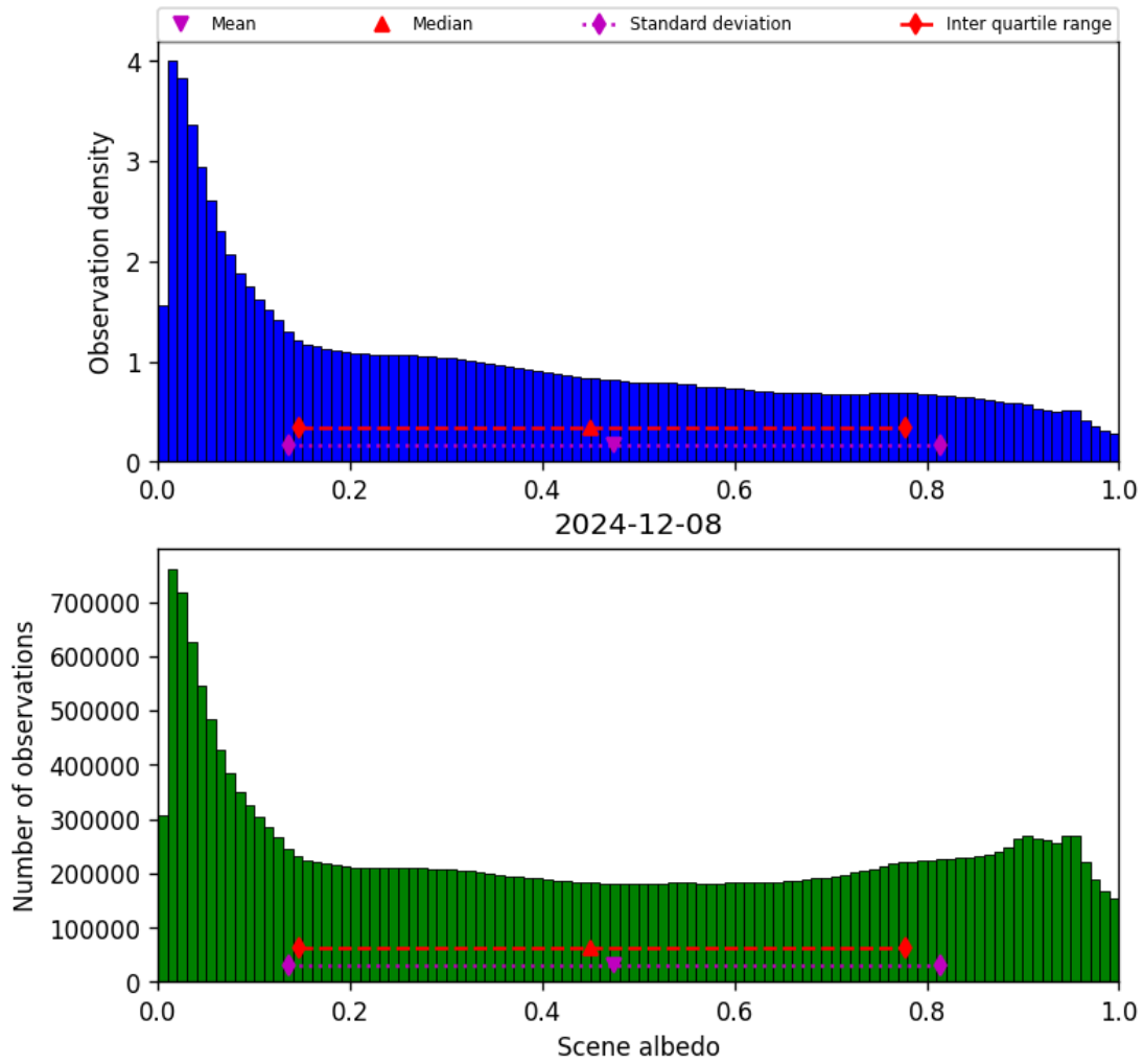
Figure 34: Histogram of “Scene albedo” for 2024-12-07 to 2024-12-09
