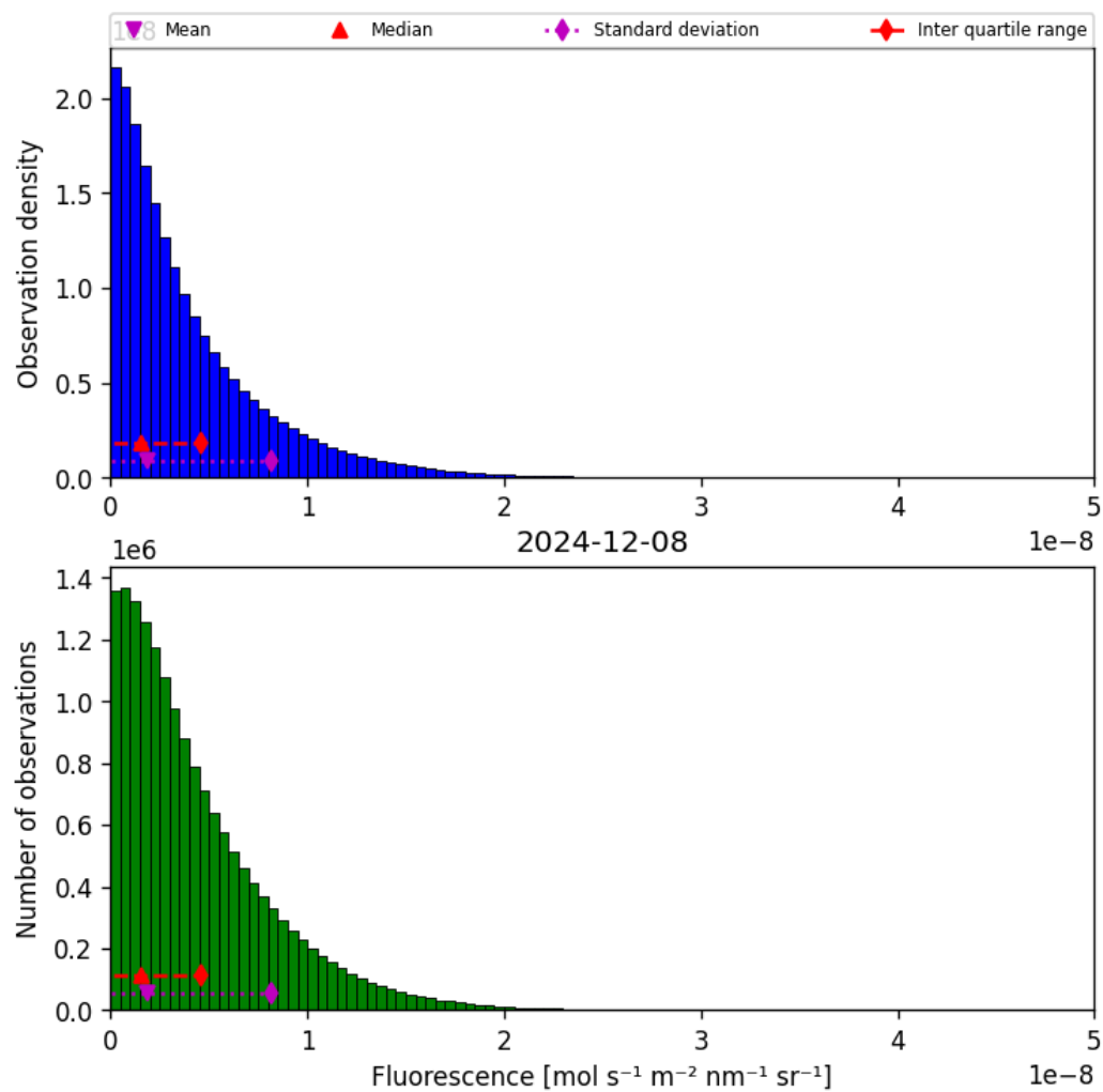
Figure 40: Histogram of “Fluorescence” for 2024-12-07 to 2024-12-09
