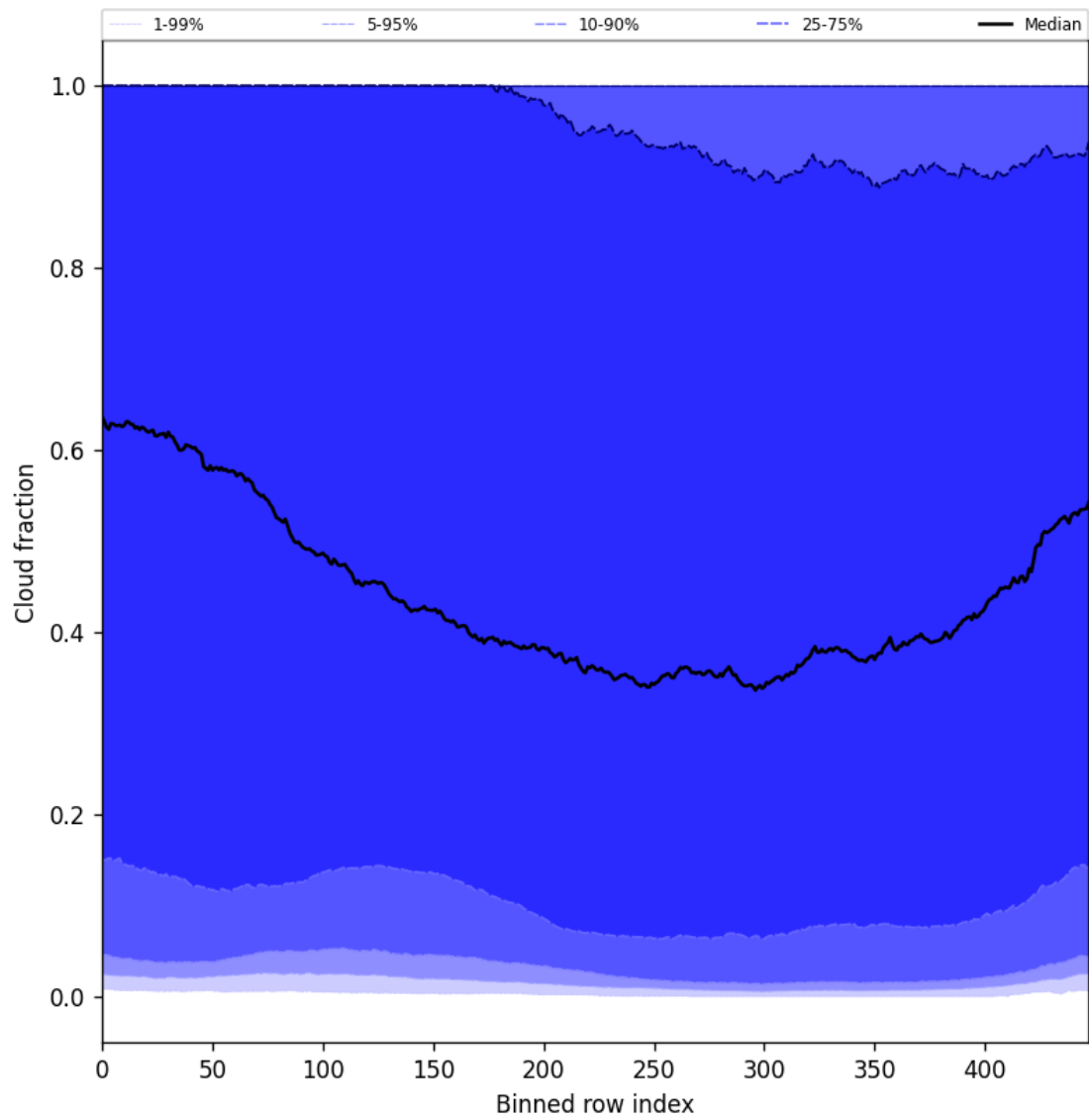
Figure 49: Along track statistics of “Cloud fraction” for 2024-12-07 to 2024-12-09
