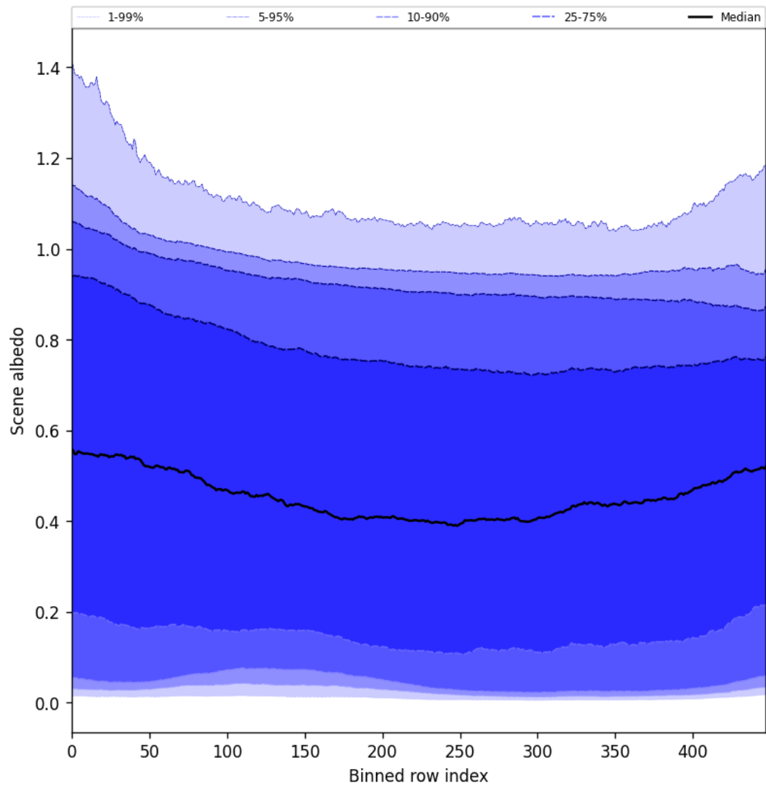
Figure 51: Along track statistics of “Scene albedo” for 2024-12-07 to 2024-12-09
