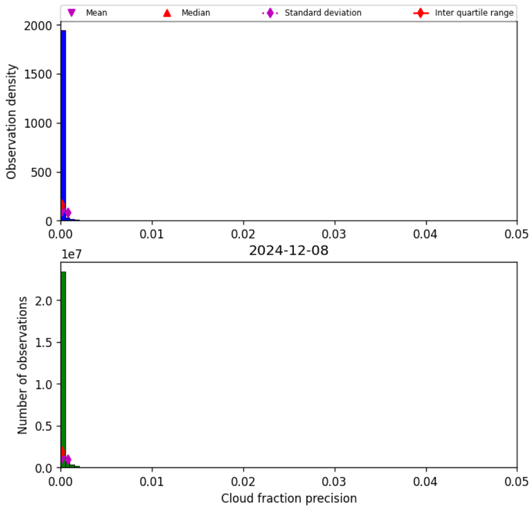
Figure 33: Histogram of “Cloud fraction precision” for 2024-12-07 to 2024-12-09
