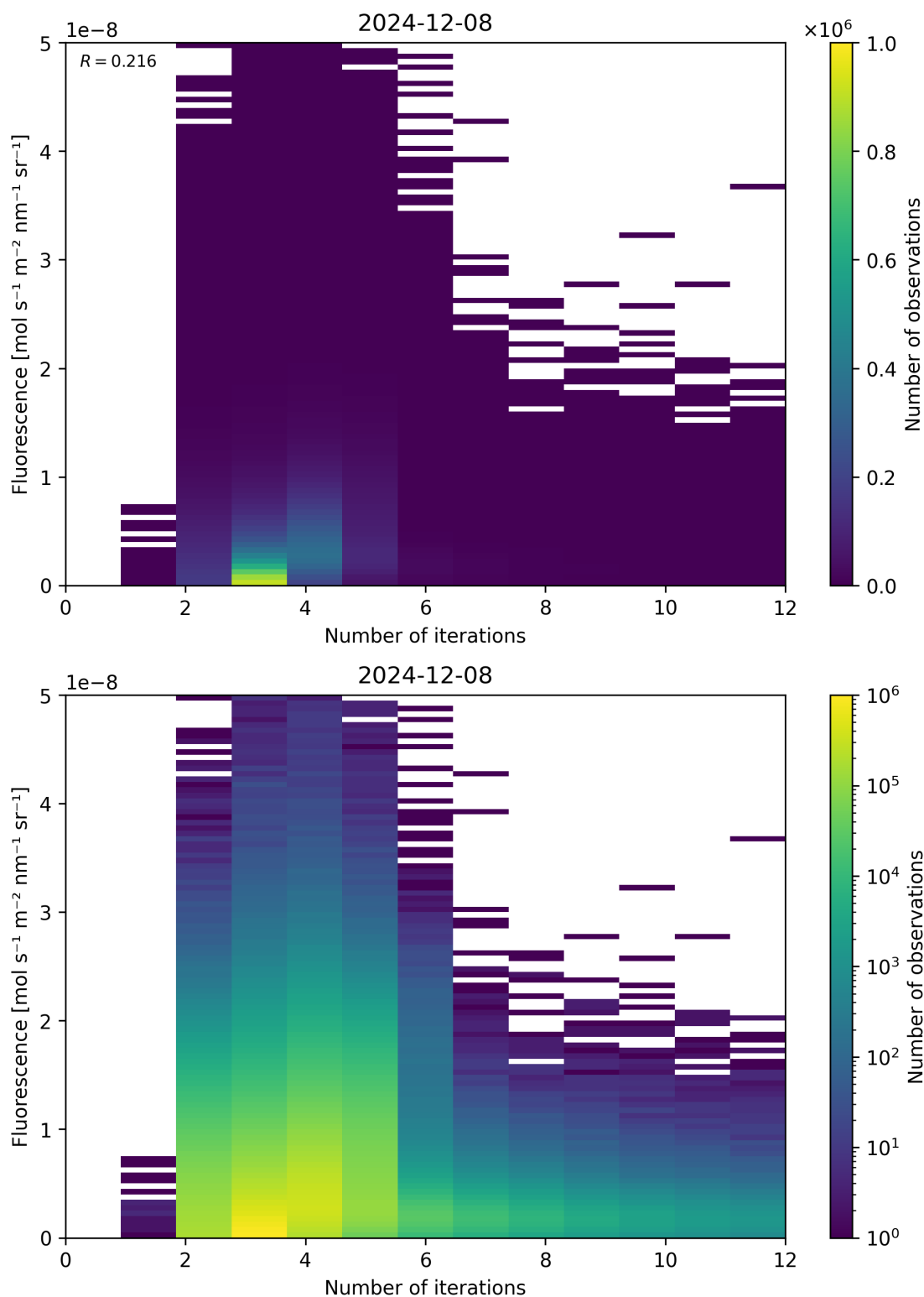
Figure 98: Scatter density plot of “Number of iterations” against “Fluorescence” for 2024-12-07 to 2024-12-09.
