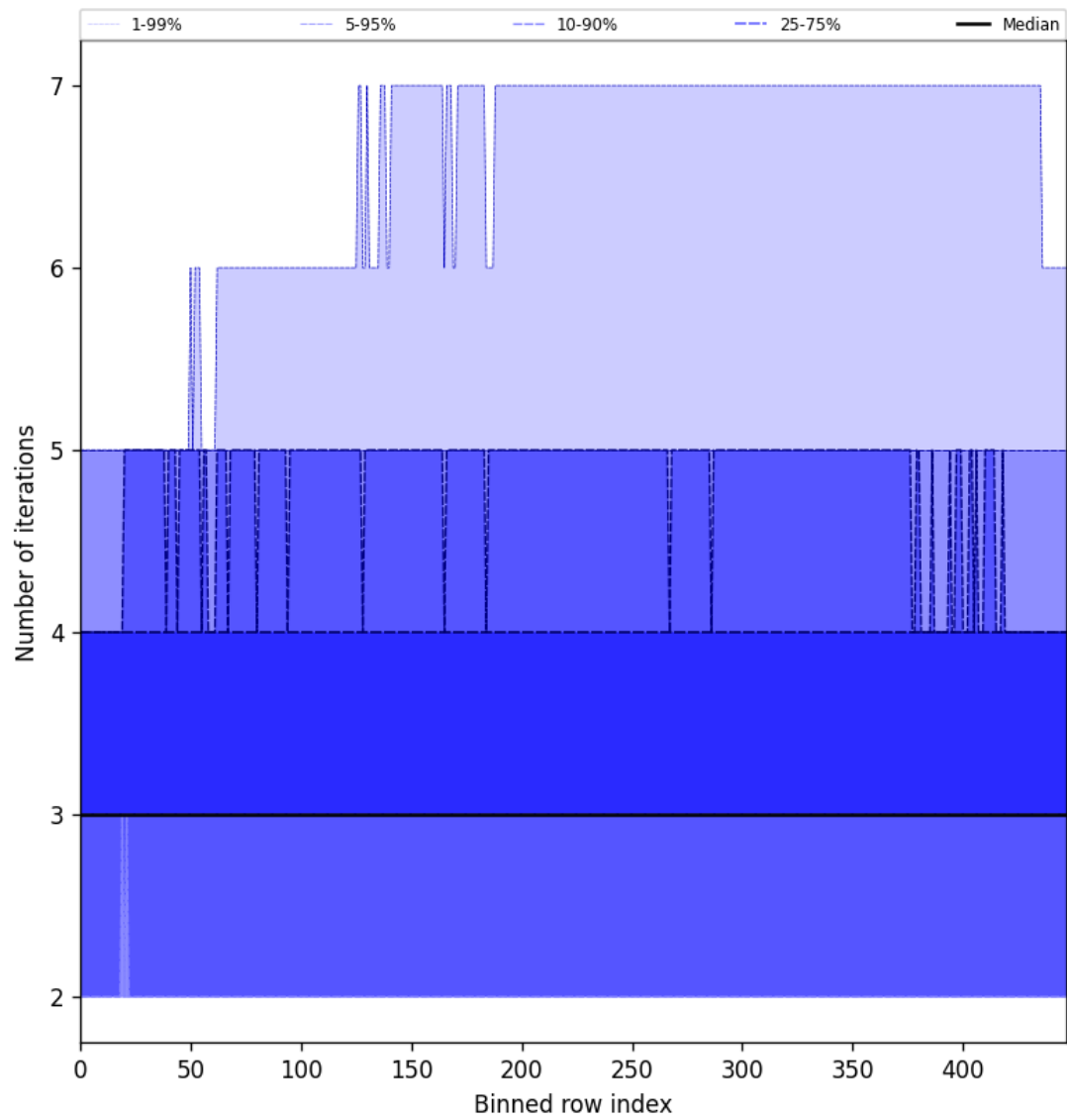
Figure 56: Along track statistics of “Number of iterations” for 2024-12-07 to 2024-12-09
