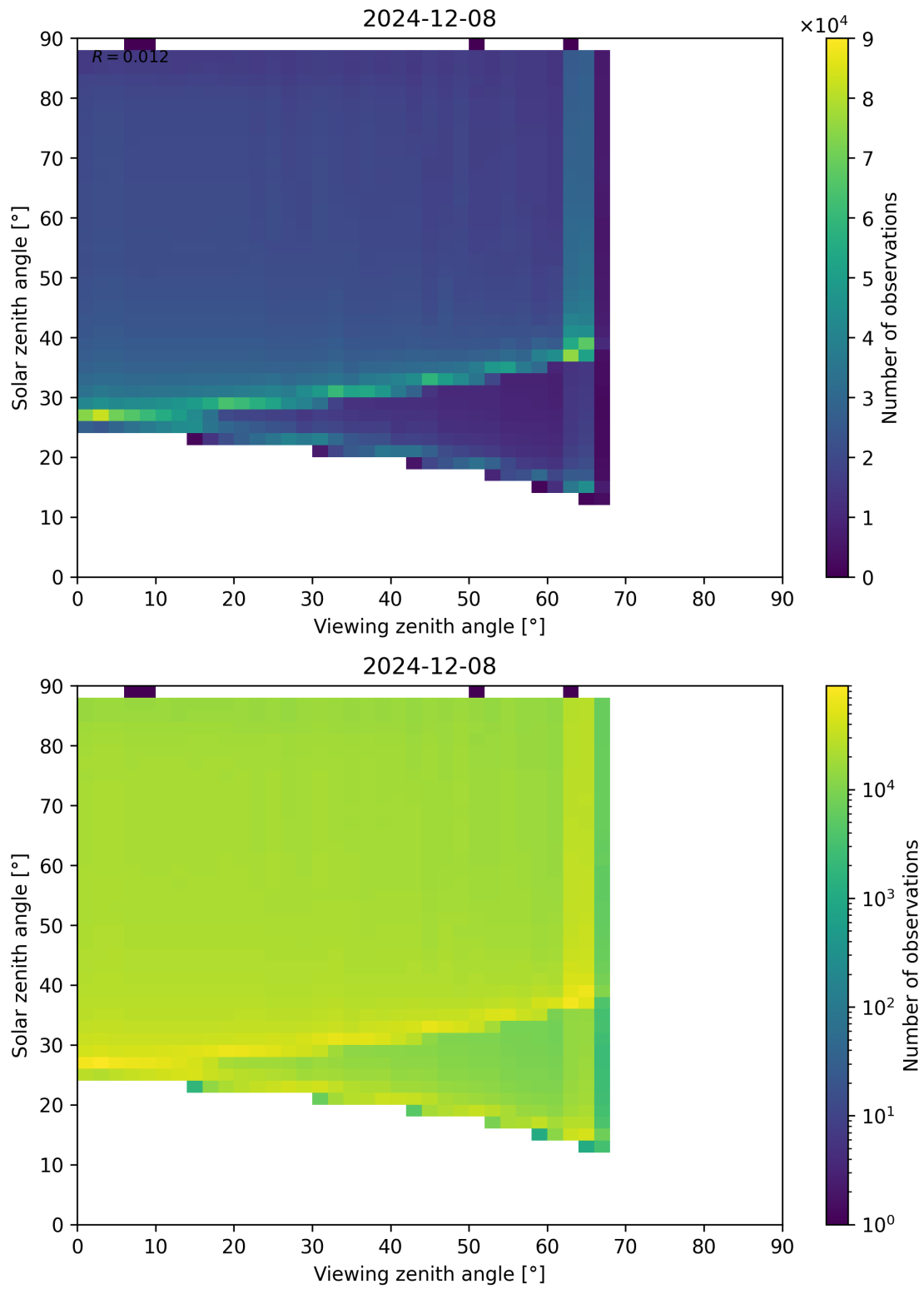
Figure 127: Scatter density plot of “Viewing zenith angle” against “Solar zenith angle” for 2024-12-07 to 2024-12-09.
