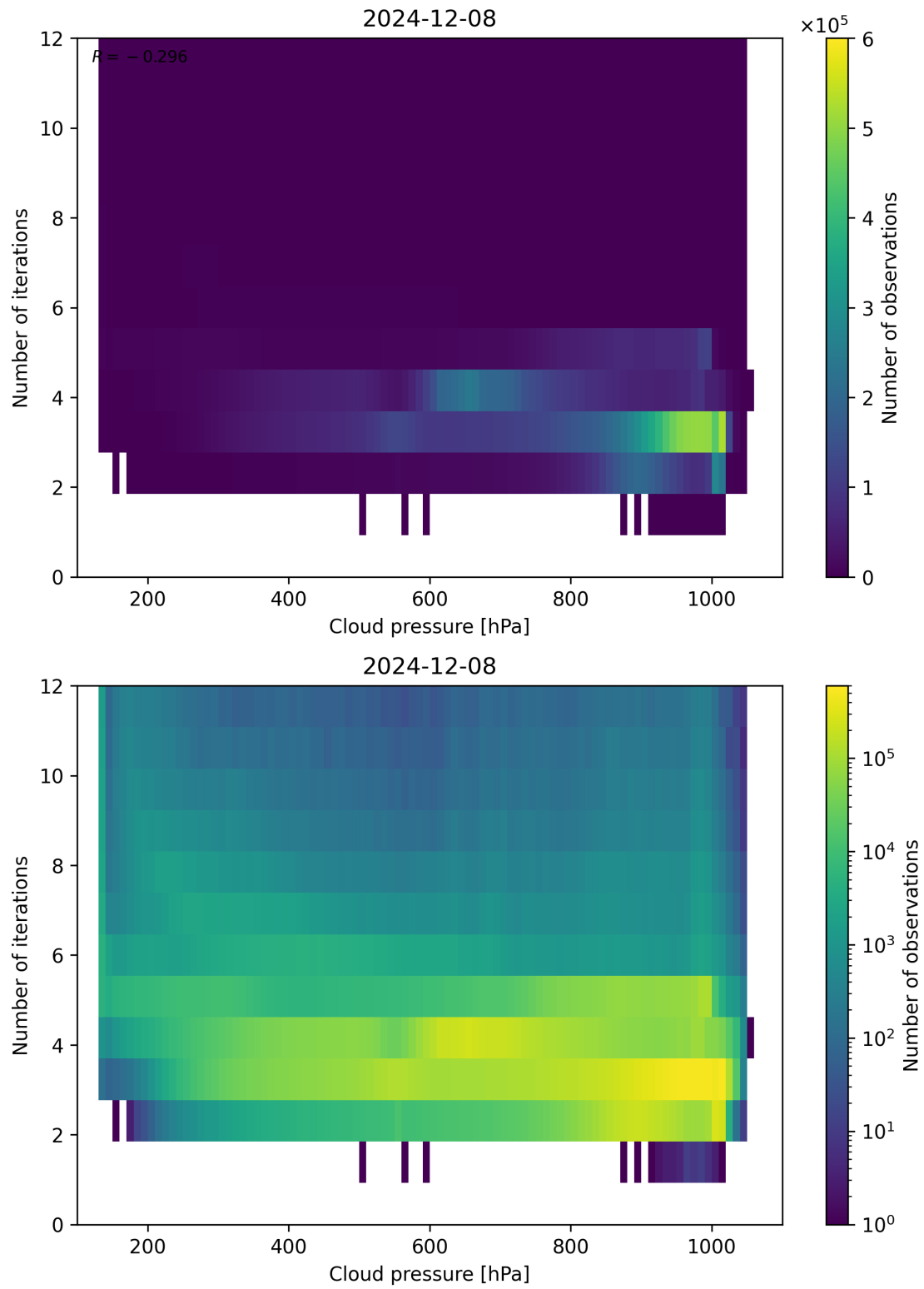
Figure 81: Scatter density plot of “Cloud pressure” against “Number of iterations” for 2024-12-07 to 2024-12-09.
