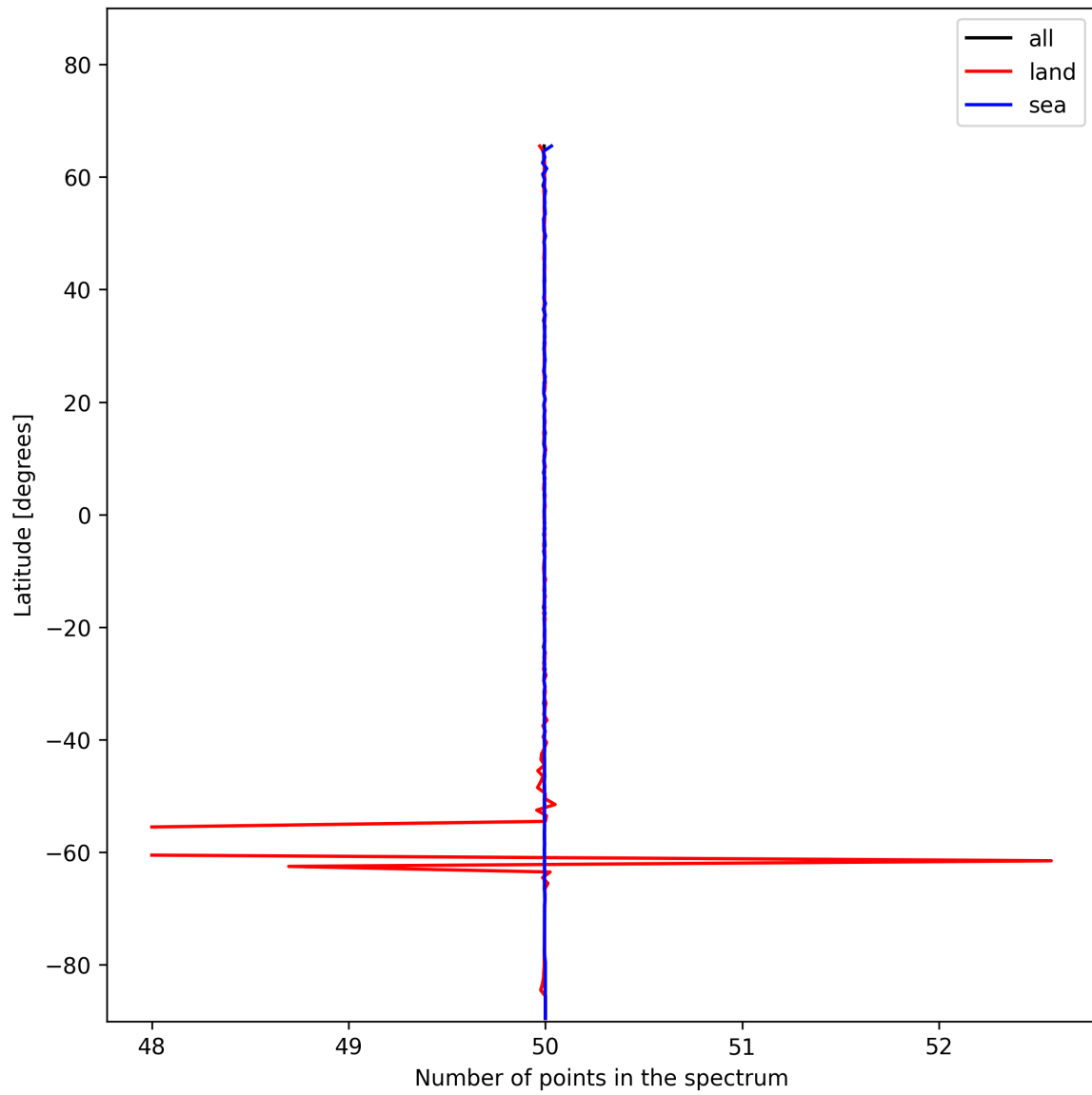
Figure 27: Zonal average of “Number of points in the spectrum” for 2024-12-07 to 2024-12-09.
