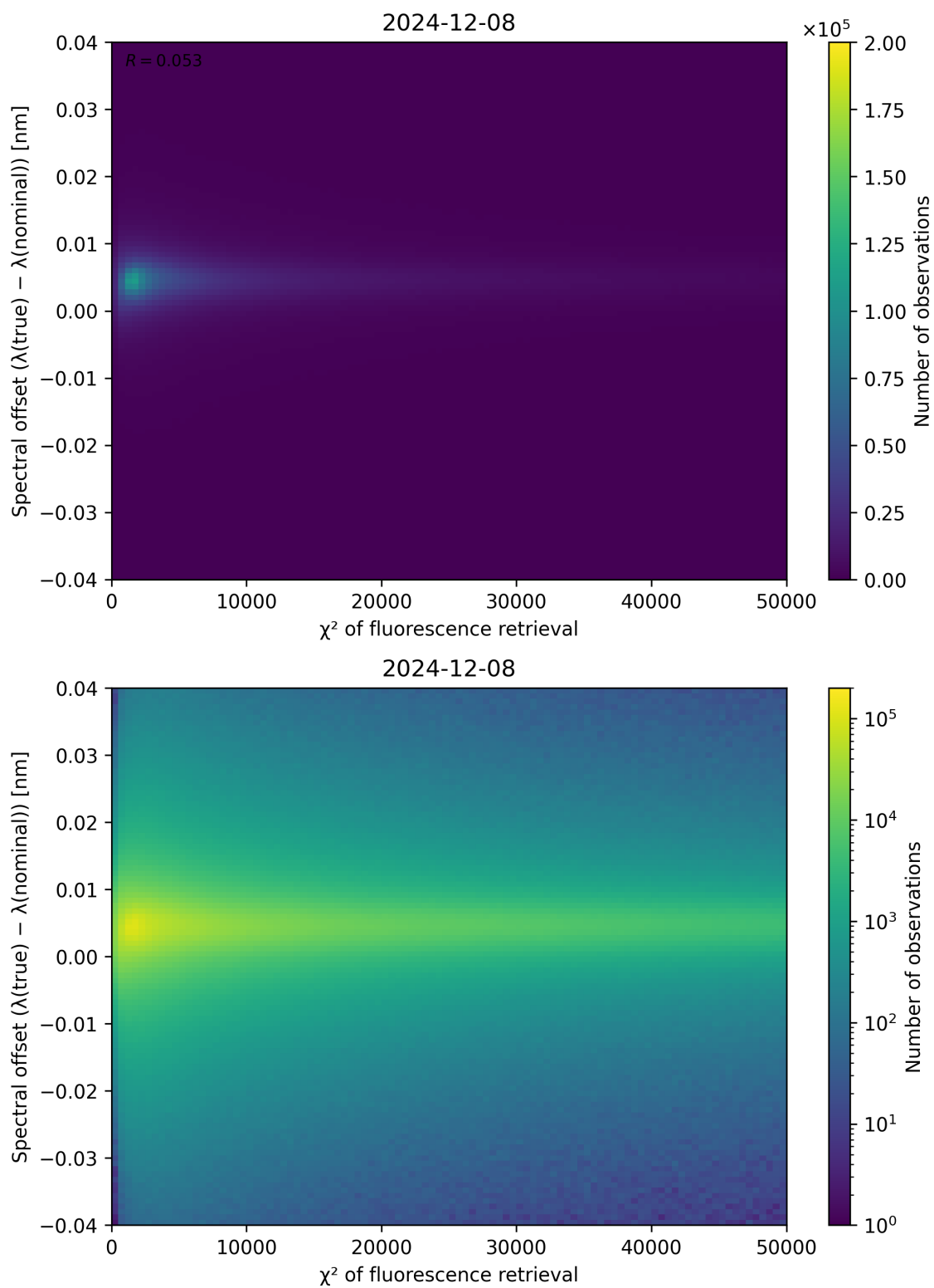
Figure 69: Scatter density plot of “ \chi^2 of fluorescence retrieval” against “Spectral offset ( \lambda_{\text{true}} - \lambda_{\text{nominal}} )” for 2024-12-07 to 2024-12-09.
