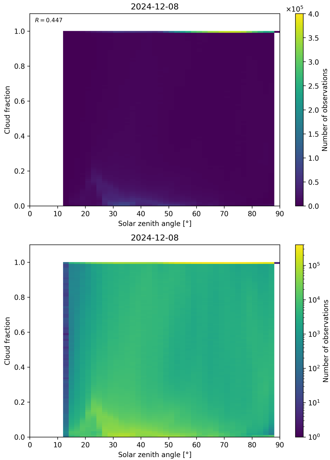
Figure 110: Scatter density plot of “Solar zenith angle” against “Cloud fraction” for 2024-12-07 to 2024-12-09.
