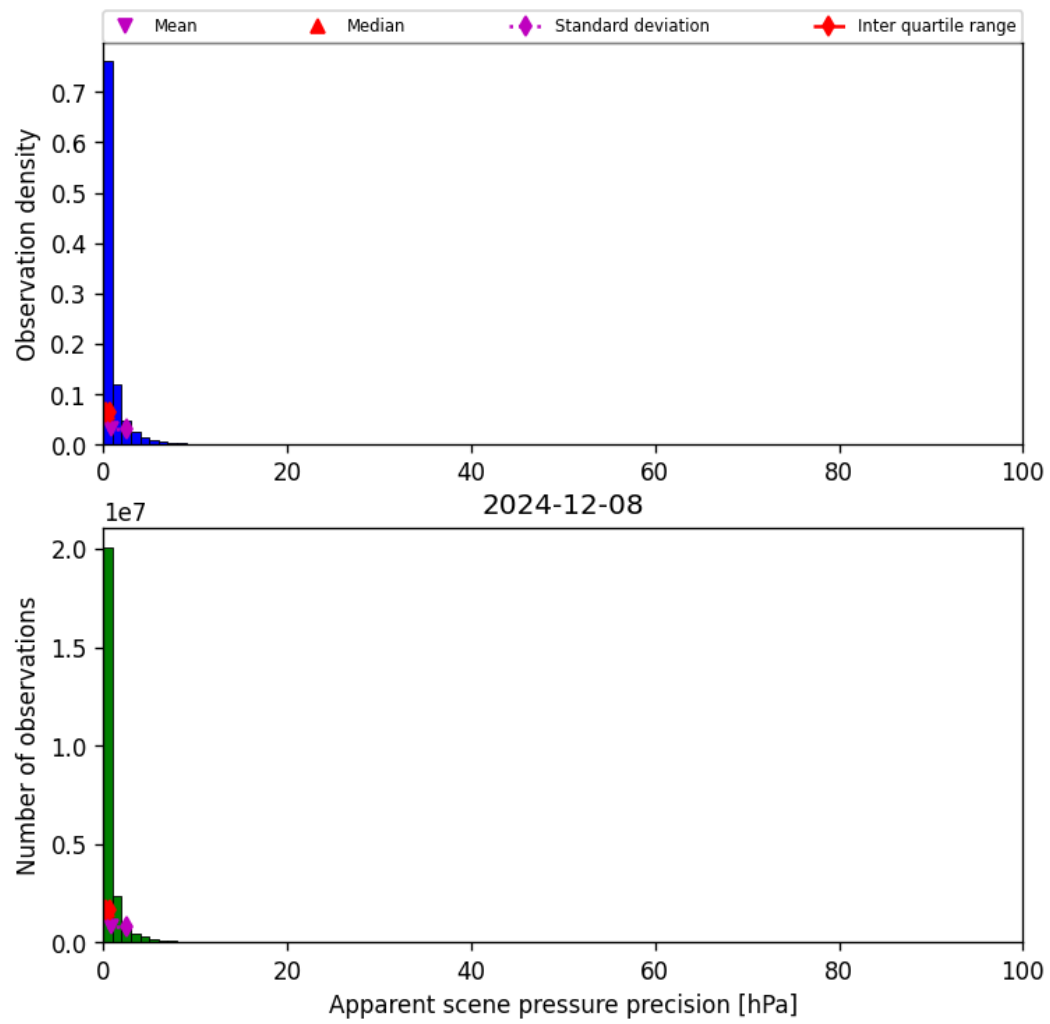
Figure 37: Histogram of “Apparent scene pressure precision” for 2024-12-07 to 2024-12-09
