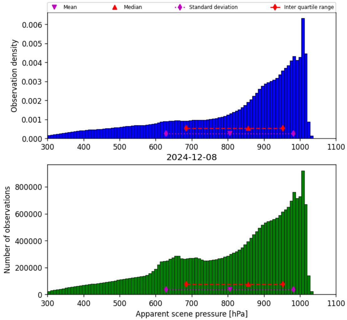
Figure 36: Histogram of “Apparent scene pressure” for 2024-12-07 to 2024-12-09
