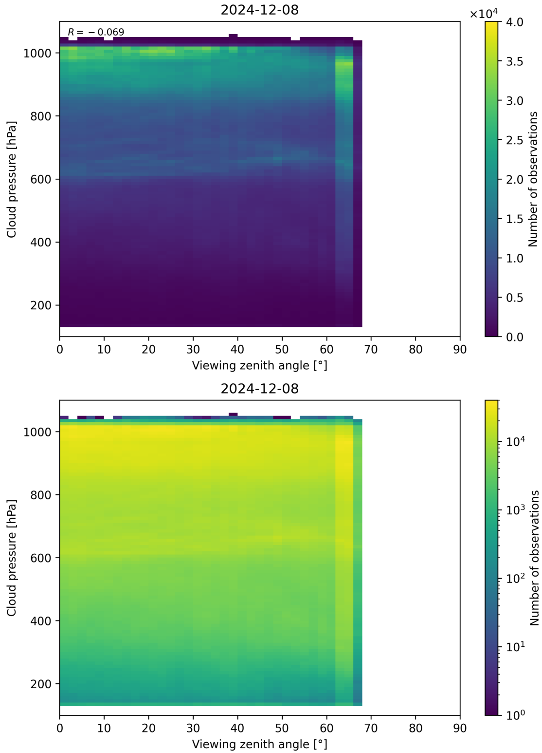
Figure 121: Scatter density plot of “Viewing zenith angle” against “Cloud pressure” for 2024-12-07 to 2024-12-09.
