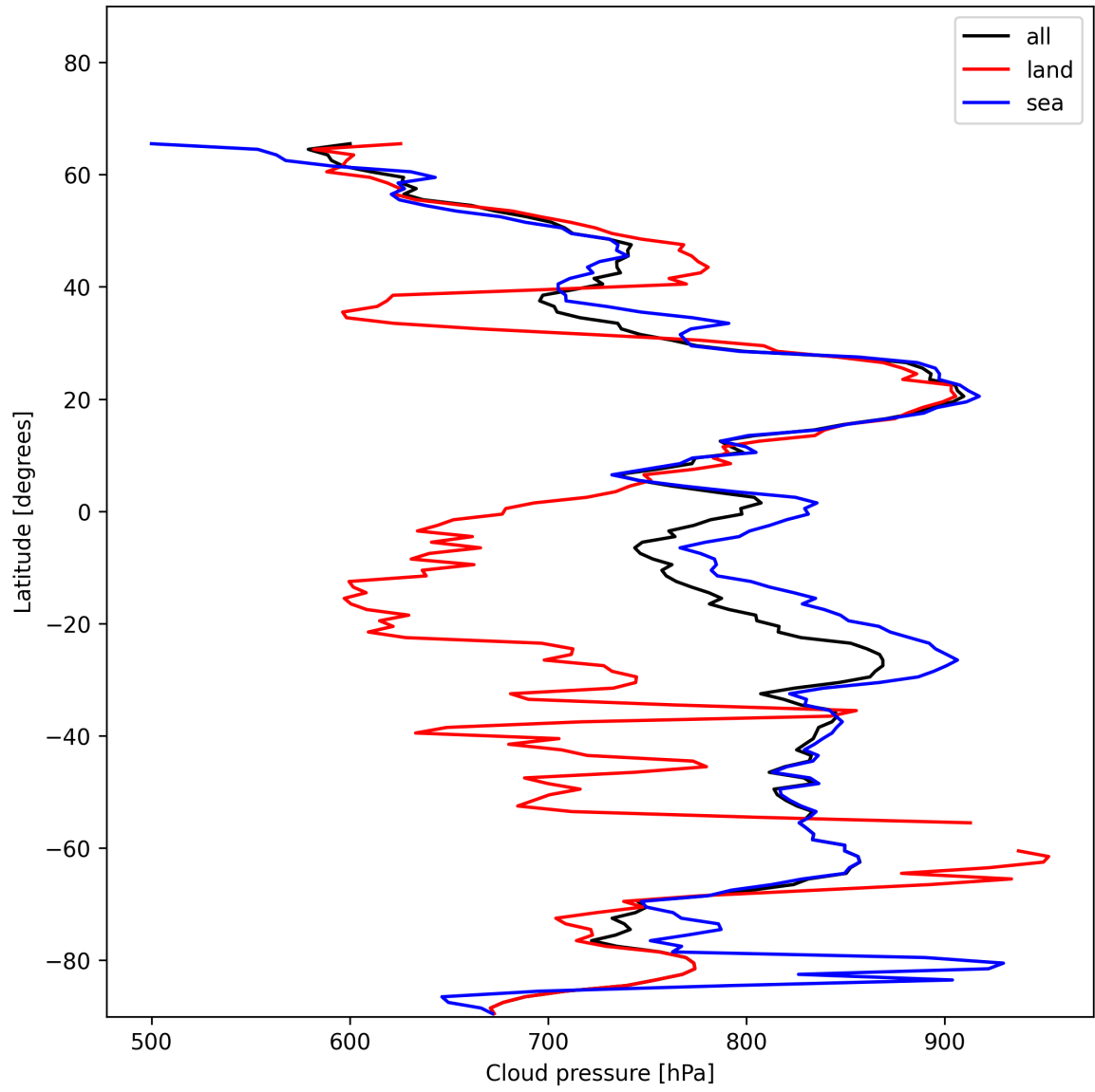
Figure 13: Zonal average of “Cloud pressure” for 2024-12-07 to 2024-12-09.
