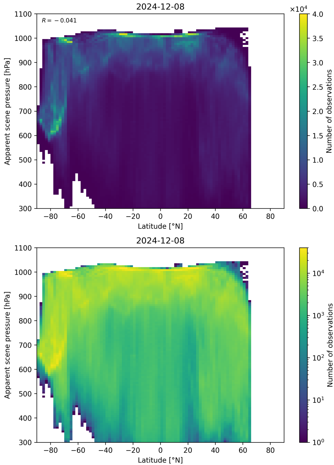
Figure 88: Scatter density plot of “Latitude” against “Apparent scene pressure” for 2024-12-07 to 2024-12-09.
