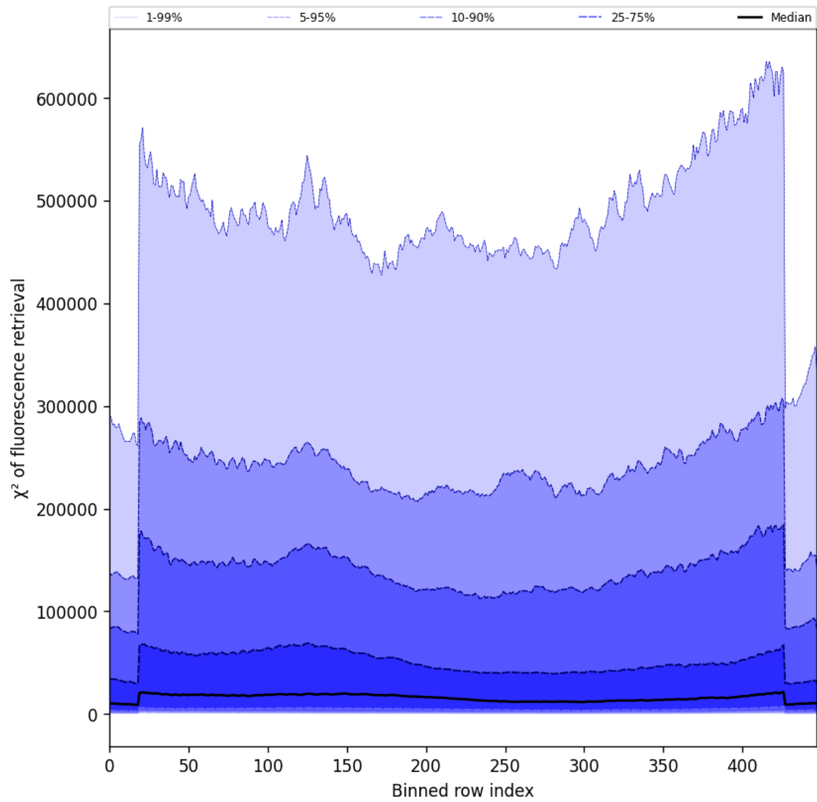
Figure 59: Along track statistics of “ \chi^2 of fluorescence retrieval” for 2024-12-07 to 2024-12-09
