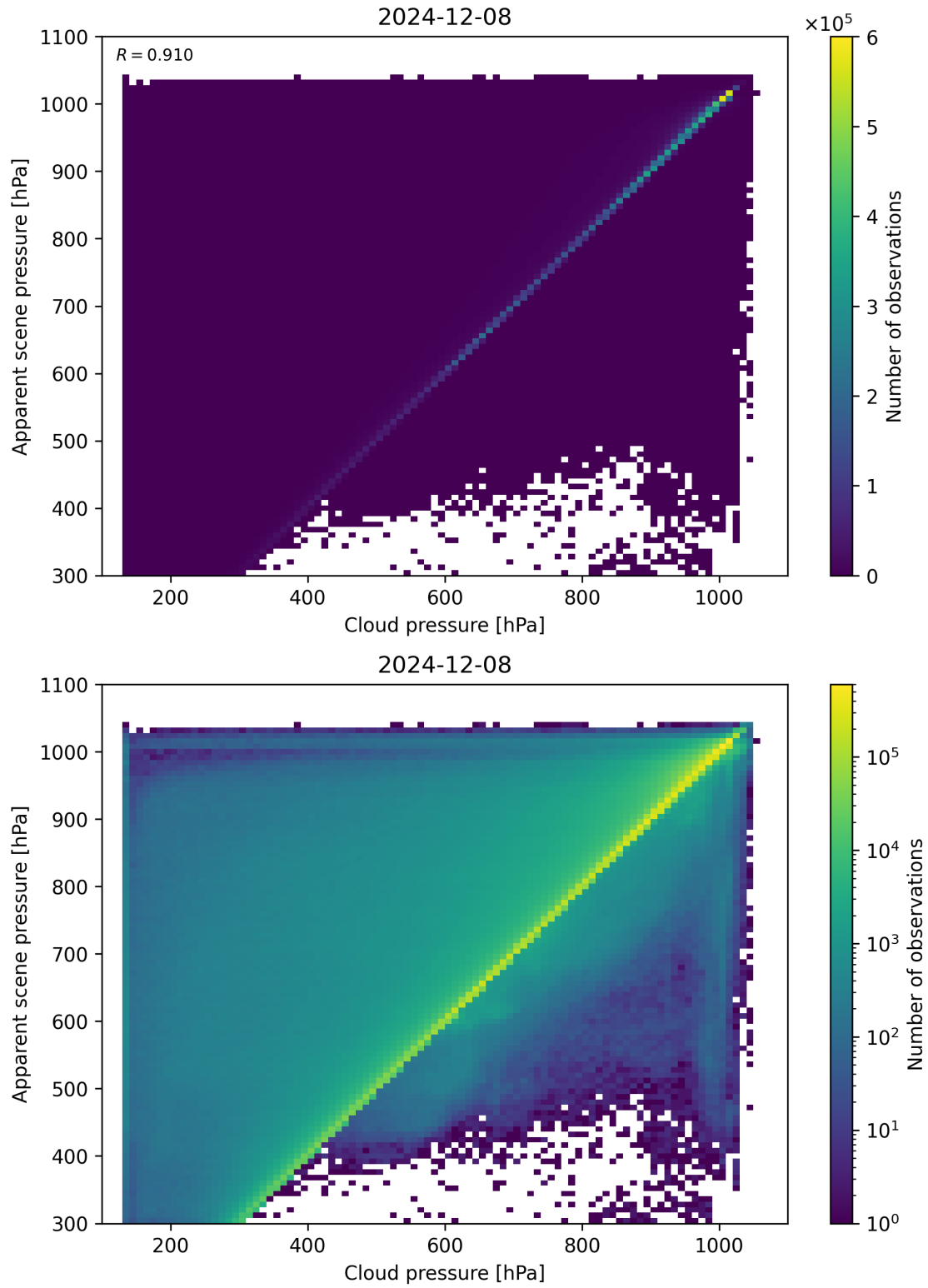
Figure 77: Scatter density plot of “Cloud pressure” against “Apparent scene pressure” for 2024-12-07 to 2024-12-09.
