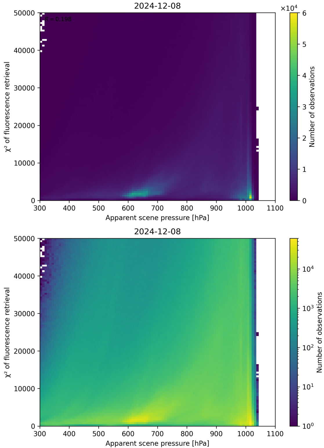
Figure 63: Scatter density plot of “Apparent scene pressure” against “ \chi^2 of fluorescence retrieval” for 2024-12-07 to 2024-12-09.
