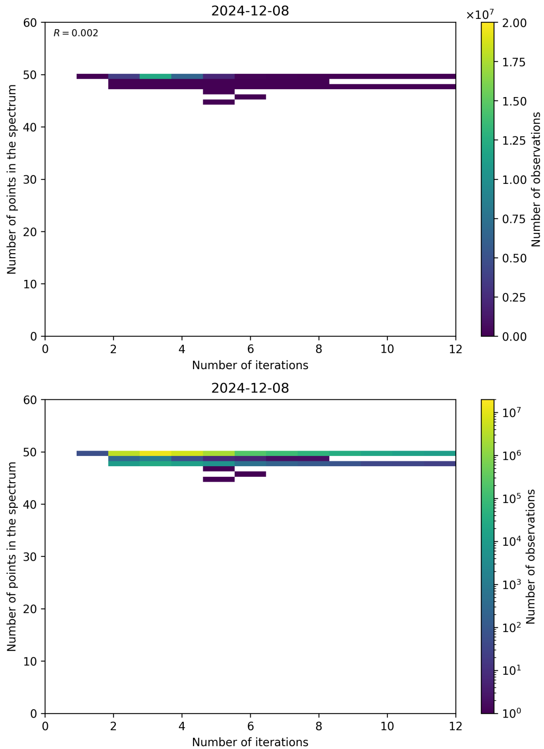
Figure 99: Scatter density plot of “Number of iterations” against “Number of points in the spectrum” for 2024-12-07 to 2024-12-09.
