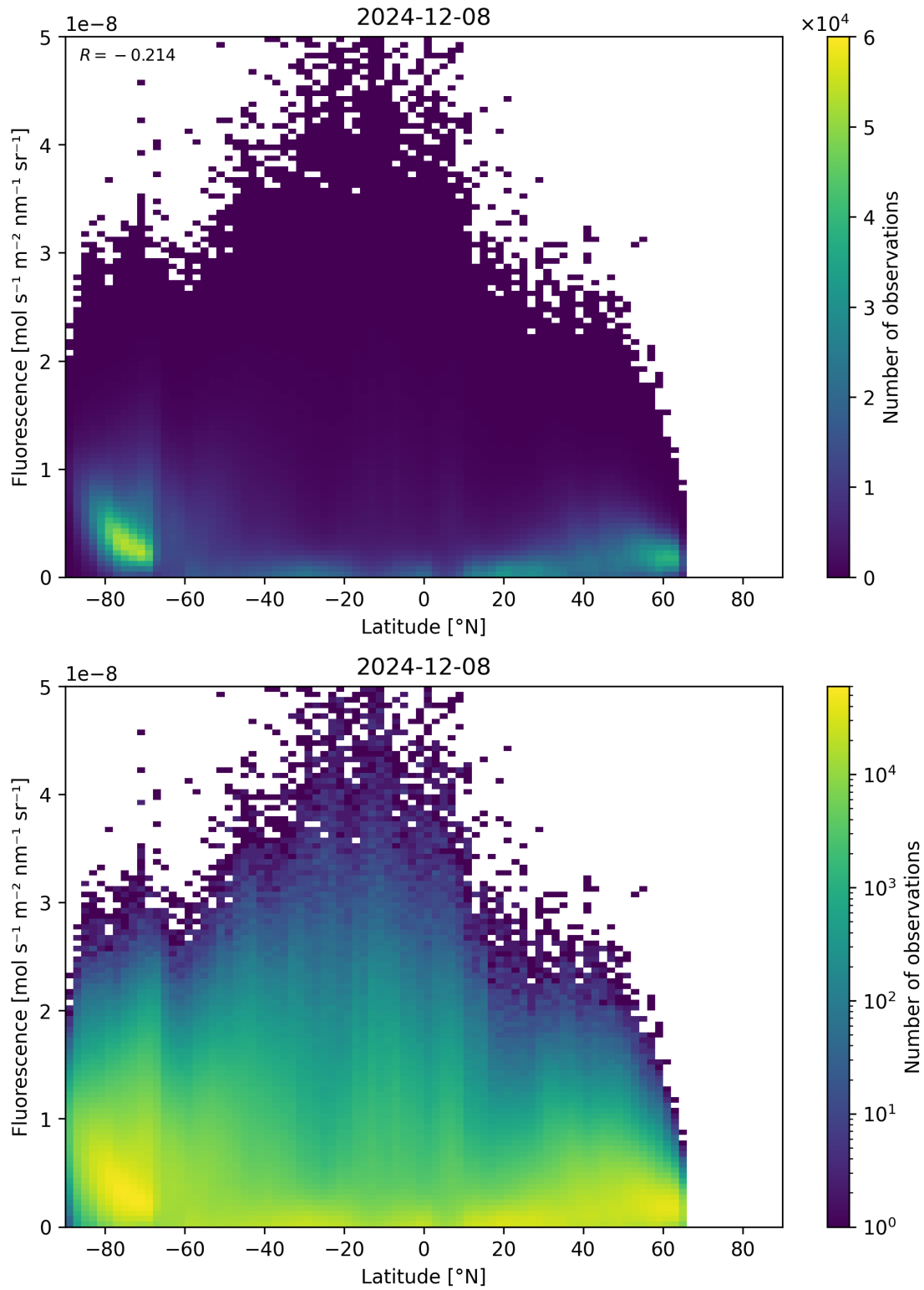
Figure 92: Scatter density plot of “Latitude” against “Fluorescence” for 2024-12-07 to 2024-12-09.
