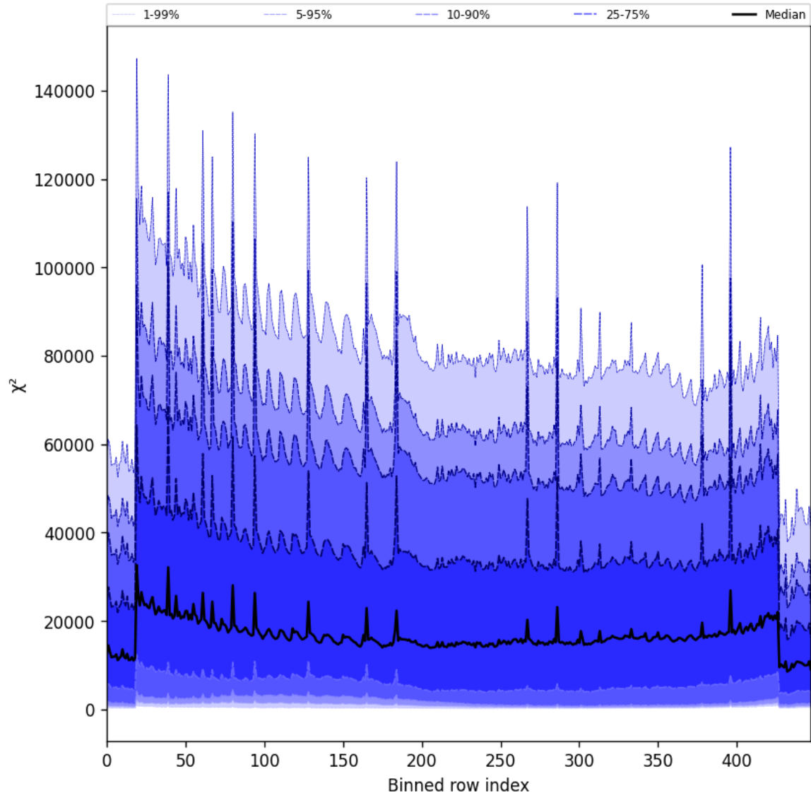
Figure 55: Along track statistics of “ \chi^2 ” for 2024-12-07 to 2024-12-09
