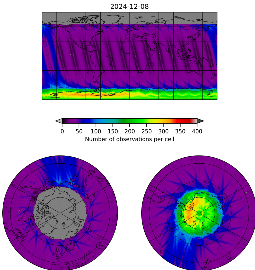
Figure 11: Map of the number of observations for 2024-12-07 to 2024-12-09
