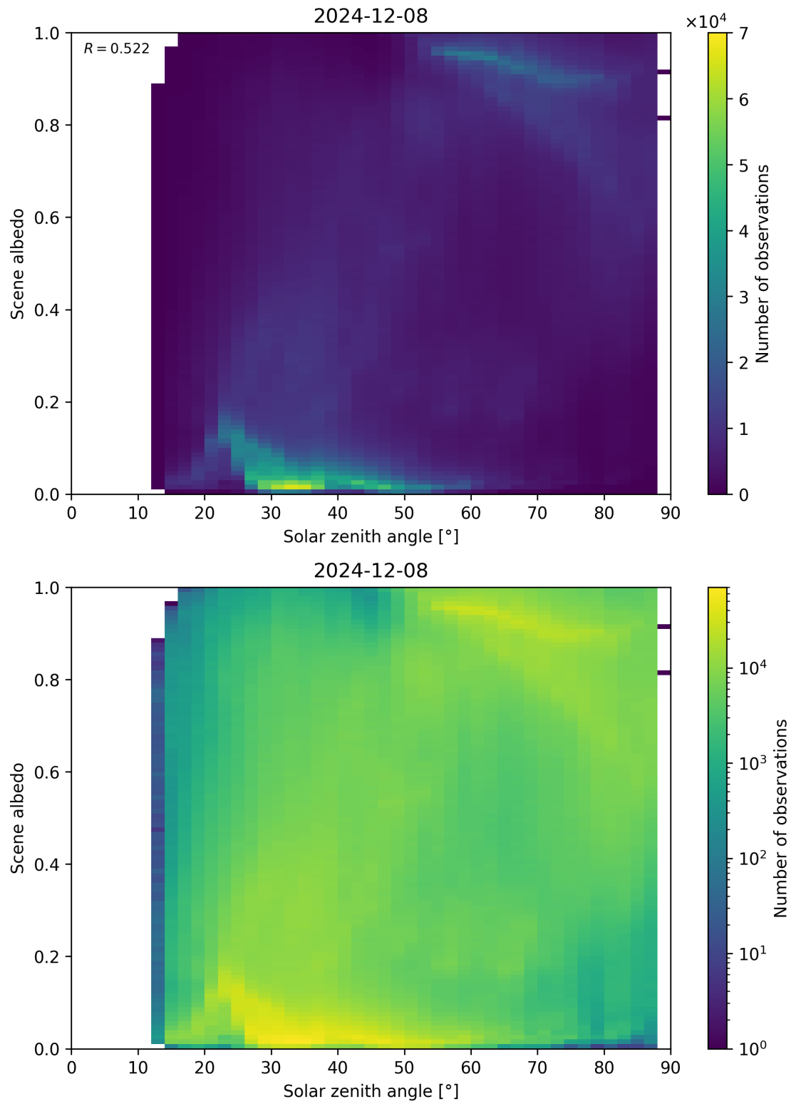
Figure 116: Scatter density plot of “Solar zenith angle” against “Scene albedo” for 2024-12-07 to 2024-12-09.
