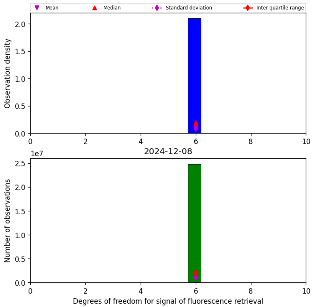
Figure 43: Histogram of “Degrees of freedom for signal of fluorescence retrieval” for 2024-12-07 to 2024-12-09
