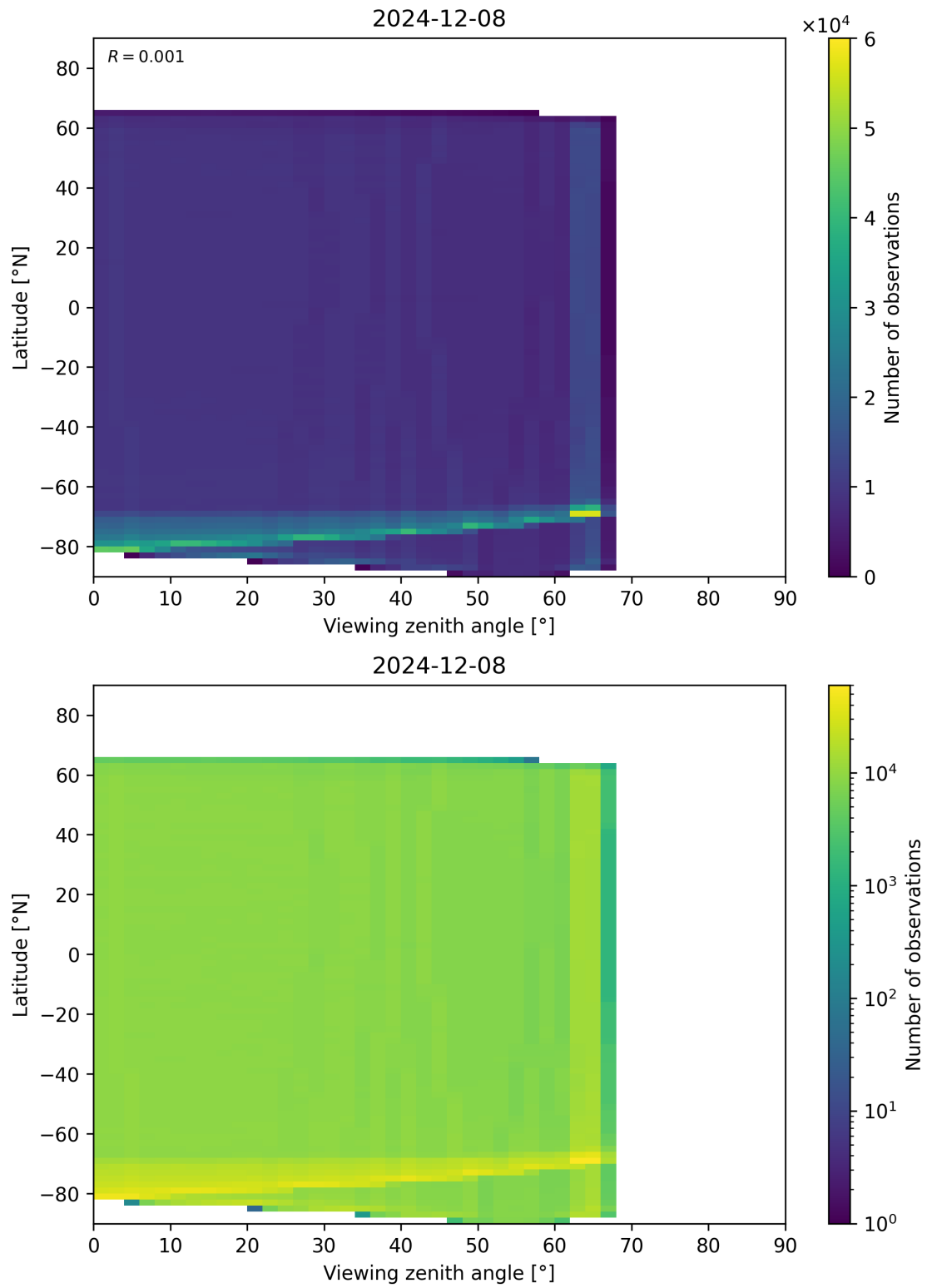
Figure 123: Scatter density plot of “Viewing zenith angle” against “Latitude” for 2024-12-07 to 2024-12-09.
