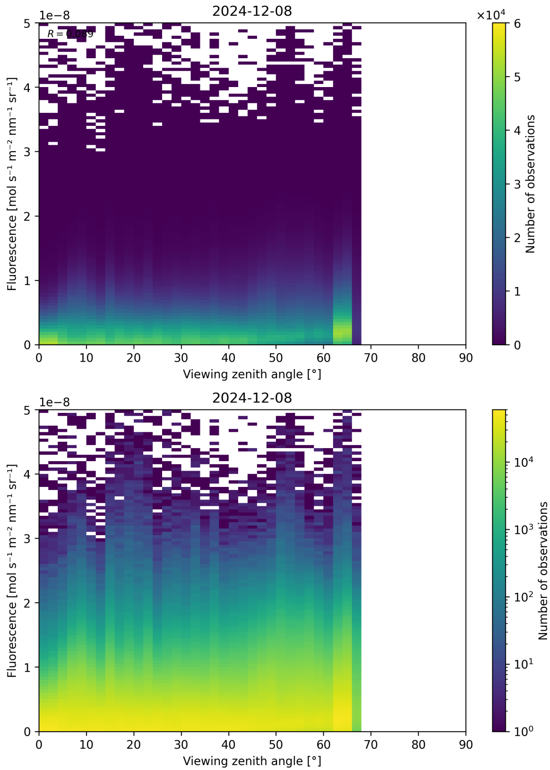
Figure 122: Scatter density plot of “Viewing zenith angle” against “Fluorescence” for 2024-12-07 to 2024-12-09.
