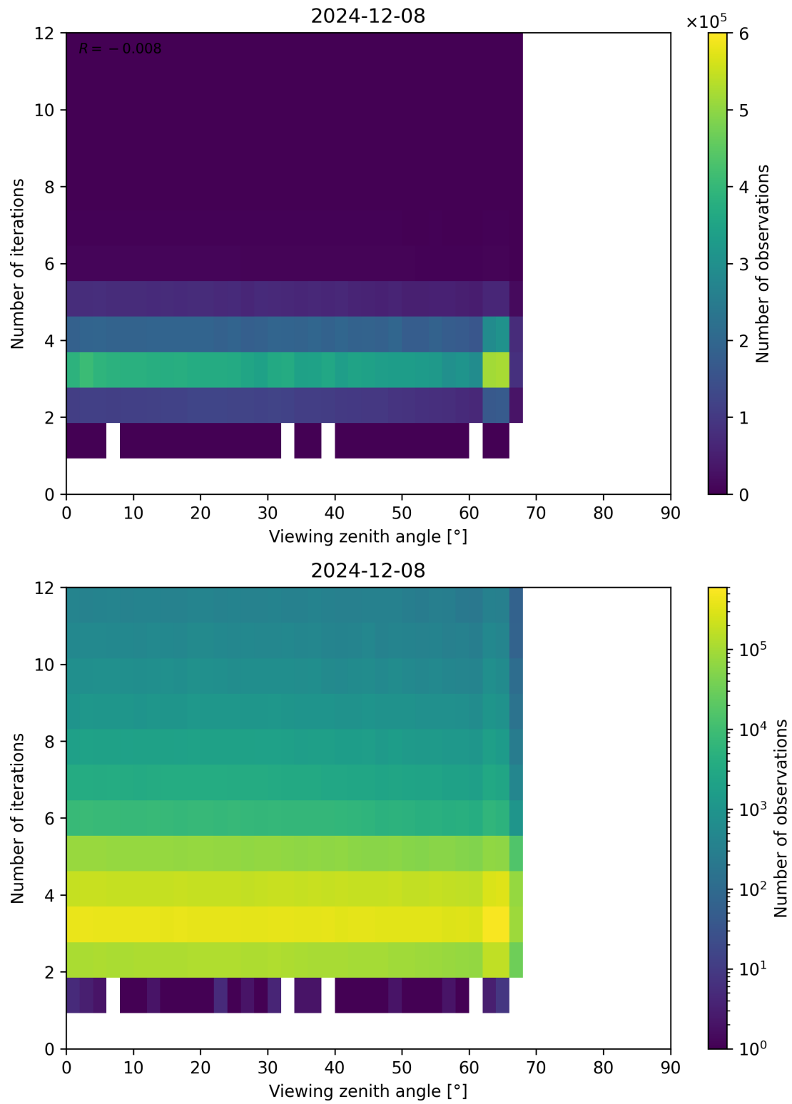
Figure 124: Scatter density plot of “Viewing zenith angle” against “Number of iterations” for 2024-12-07 to 2024-12-09.
