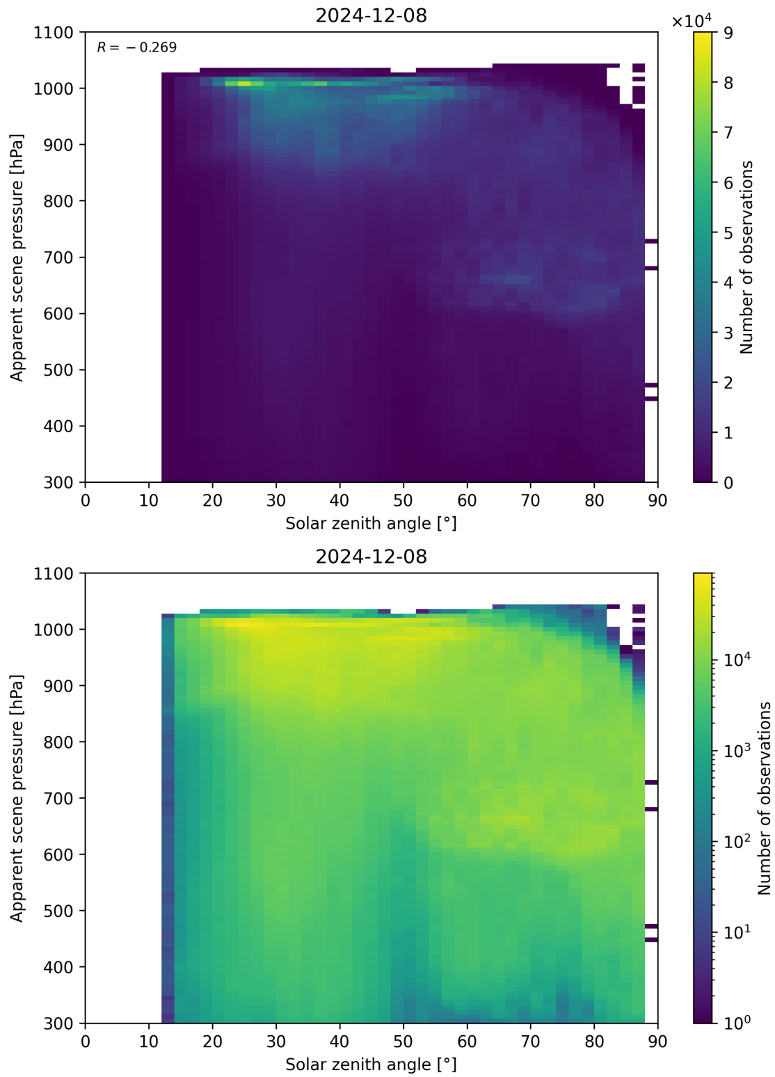
Figure 108: Scatter density plot of “Solar zenith angle” against “Apparent scene pressure” for 2024-12-07 to 2024-12-09.
