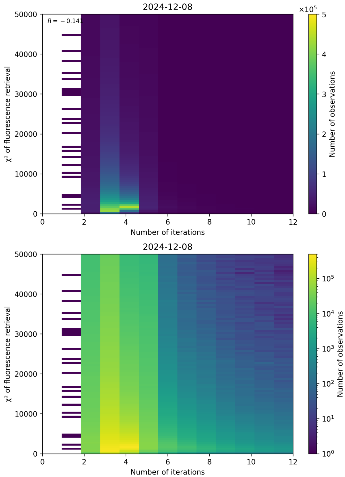
Figure 97: Scatter density plot of “Number of iterations” against “ \chi^2 of fluorescence retrieval” for 2024-12-07 to 2024-12-09.
