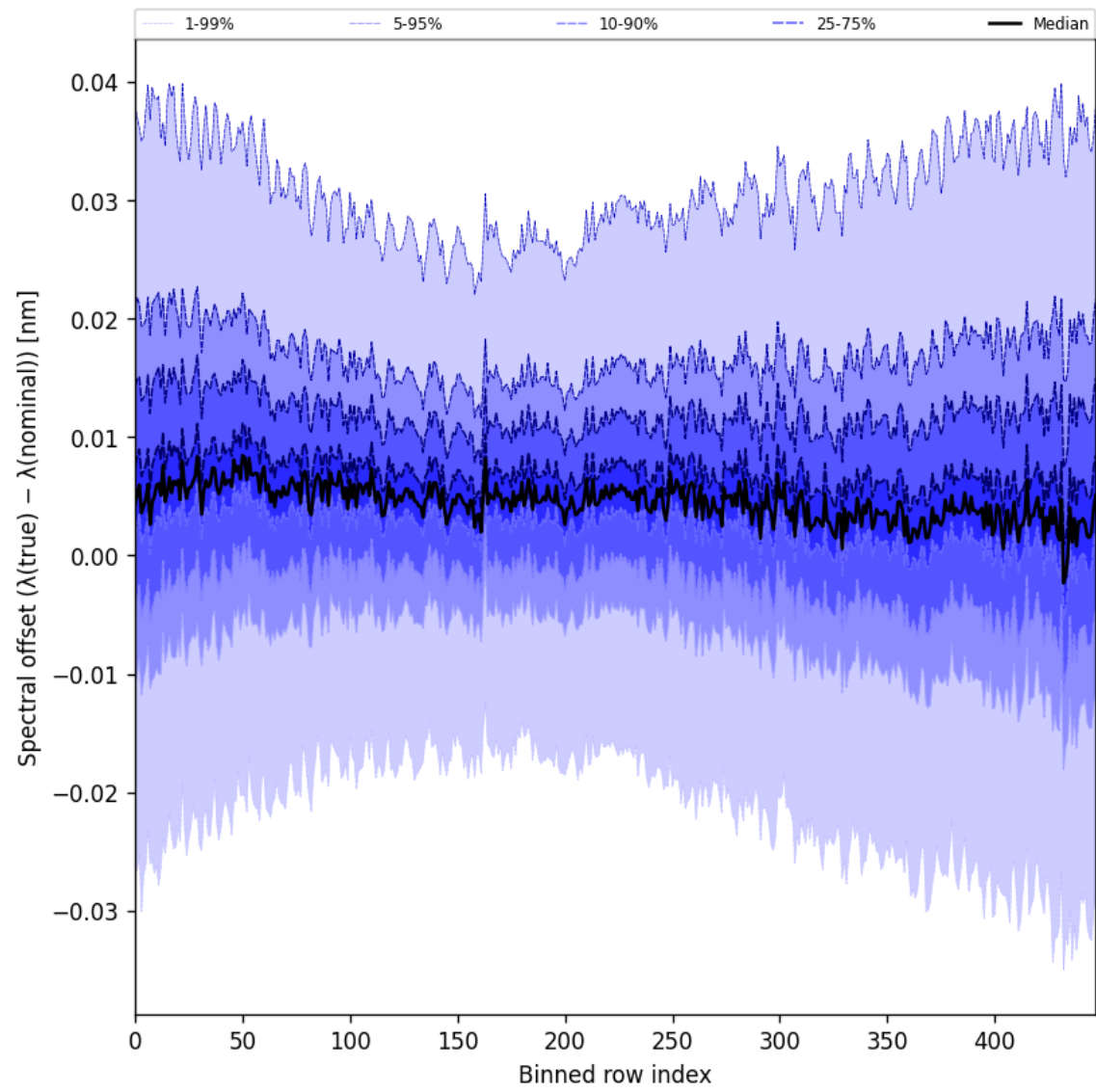
Figure 62: Along track statistics of “Spectral offset ( \lambda_{\text{true}} - \lambda_{\text{nominal}} )” for 2024-12-07 to 2024-12-09
