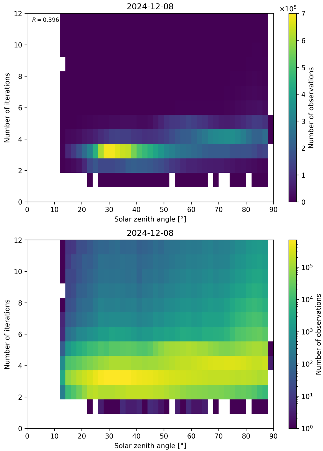
Figure 114: Scatter density plot of “Solar zenith angle” against “Number of iterations” for 2024-12-07 to 2024-12-09.
