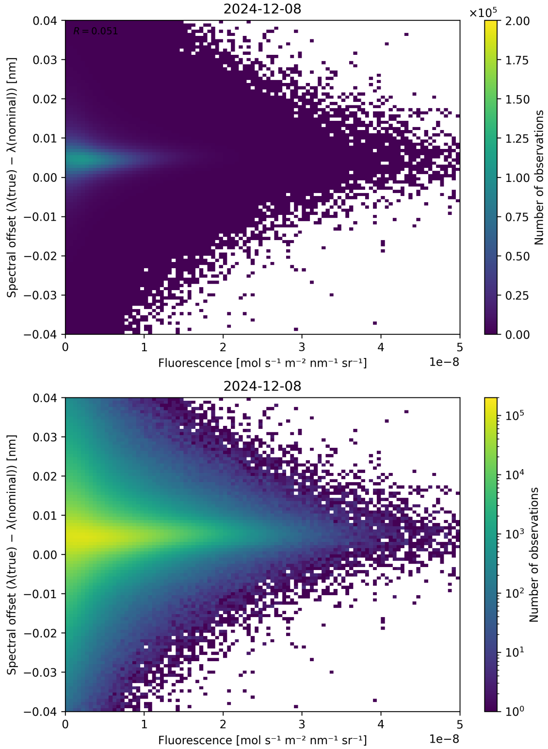
Figure 87: Scatter density plot of “Fluorescence” against “Spectral offset ( \lambda_{\text{true}} - \lambda_{\text{nominal}} )” for 2024-12-07 to 2024-12-09.
