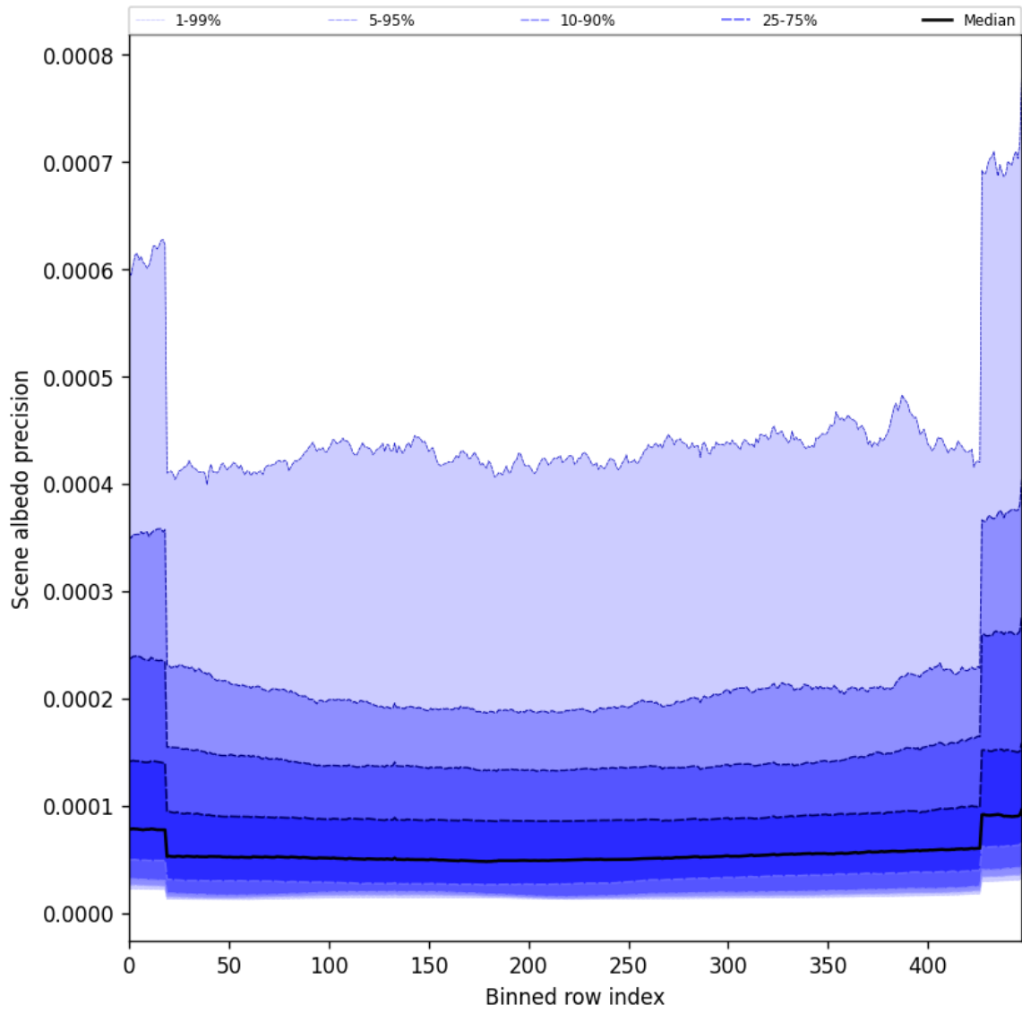
Figure 52: Along track statistics of “Scene albedo precision” for 2024-12-07 to 2024-12-09
