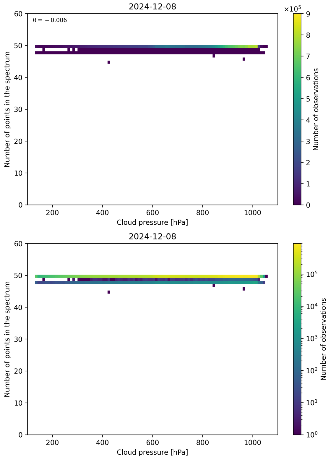
Figure 82: Scatter density plot of “Cloud pressure” against “Number of points in the spectrum” for 2024-12-07 to 2024-12-09.
