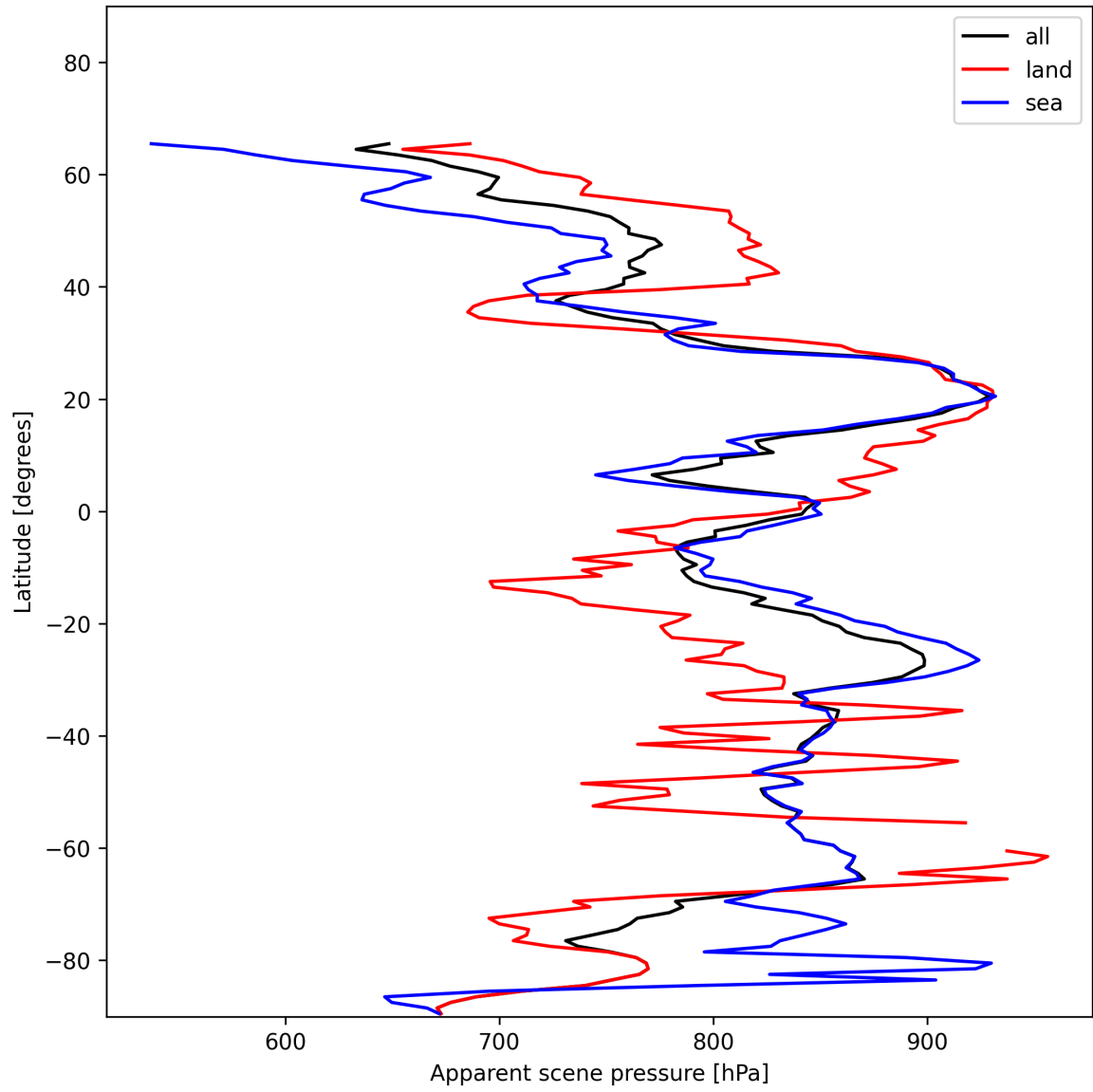
Figure 19: Zonal average of “Apparent scene pressure” for 2024-12-07 to 2024-12-09.
