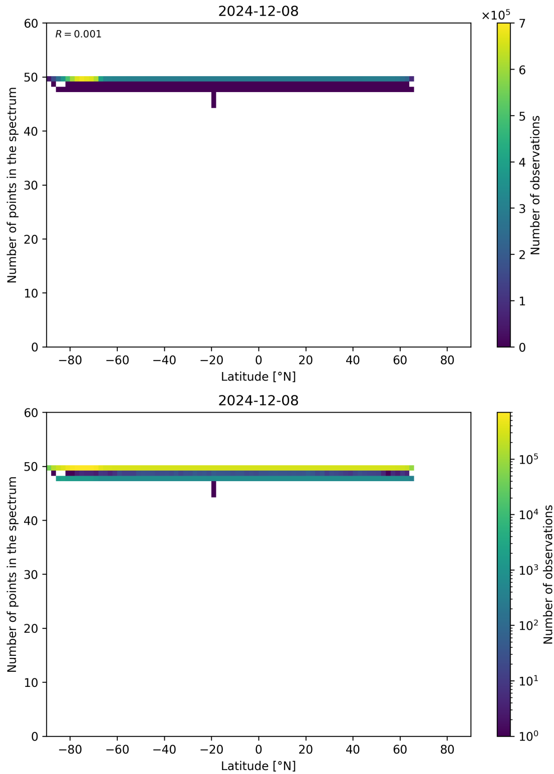
Figure 94: Scatter density plot of “Latitude” against “Number of points in the spectrum” for 2024-12-07 to 2024-12-09.
