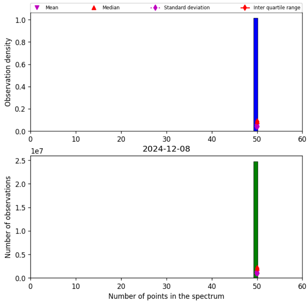
Figure 44: Histogram of “Number of points in the spectrum” for 2024-12-07 to 2024-12-09
