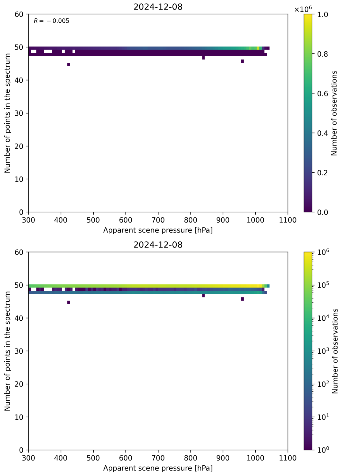
Figure 66: Scatter density plot of “Apparent scene pressure” against “Number of points in the spectrum” for 2024-12-07 to 2024-12-09.
