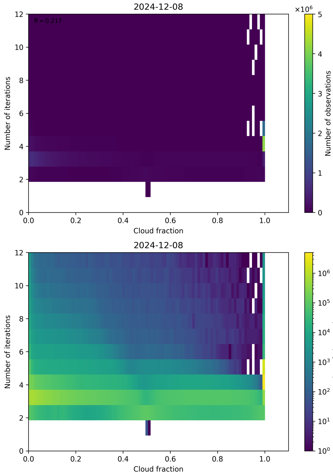
Figure 73: Scatter density plot of “Cloud fraction” against “Number of iterations” for 2024-12-07 to 2024-12-09.
