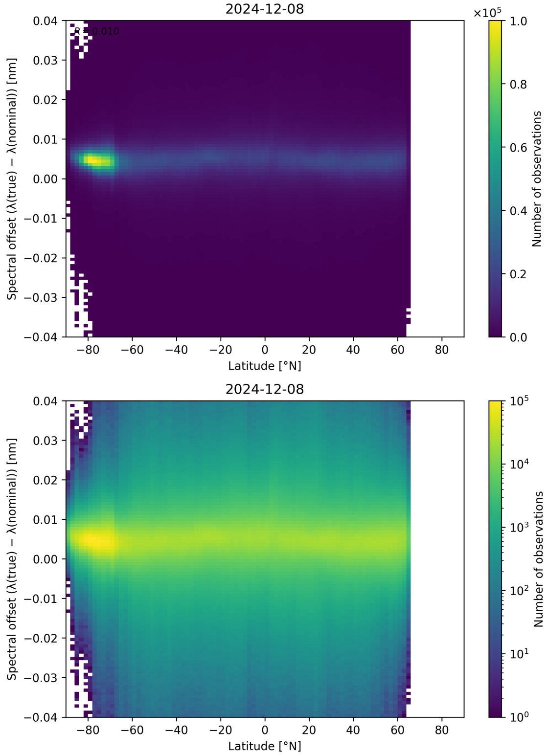
Figure 96: Scatter density plot of “Latitude” against “Spectral offset ( \lambda_{\text{true}} - \lambda_{\text{nominal}} )” for 2024-12-07 to 2024-12-09.
