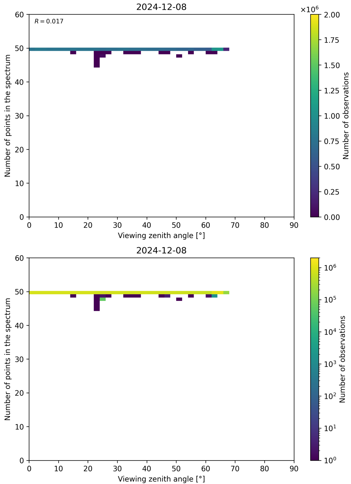
Figure 125: Scatter density plot of “Viewing zenith angle” against “Number of points in the spectrum” for 2024-12-07 to 2024-12-09.
