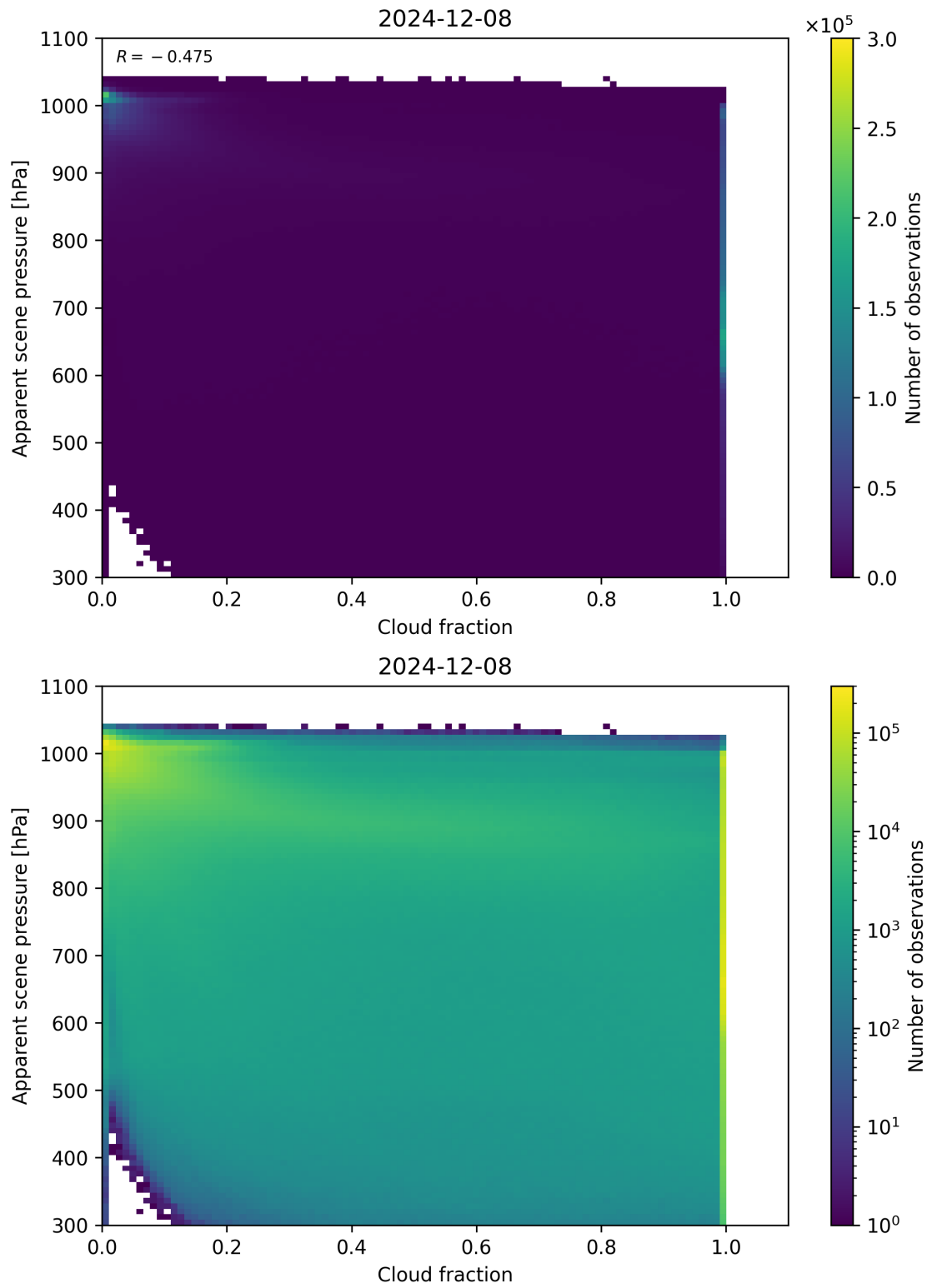
Figure 70: Scatter density plot of “Cloud fraction” against “Apparent scene pressure” for 2024-12-07 to 2024-12-09.
