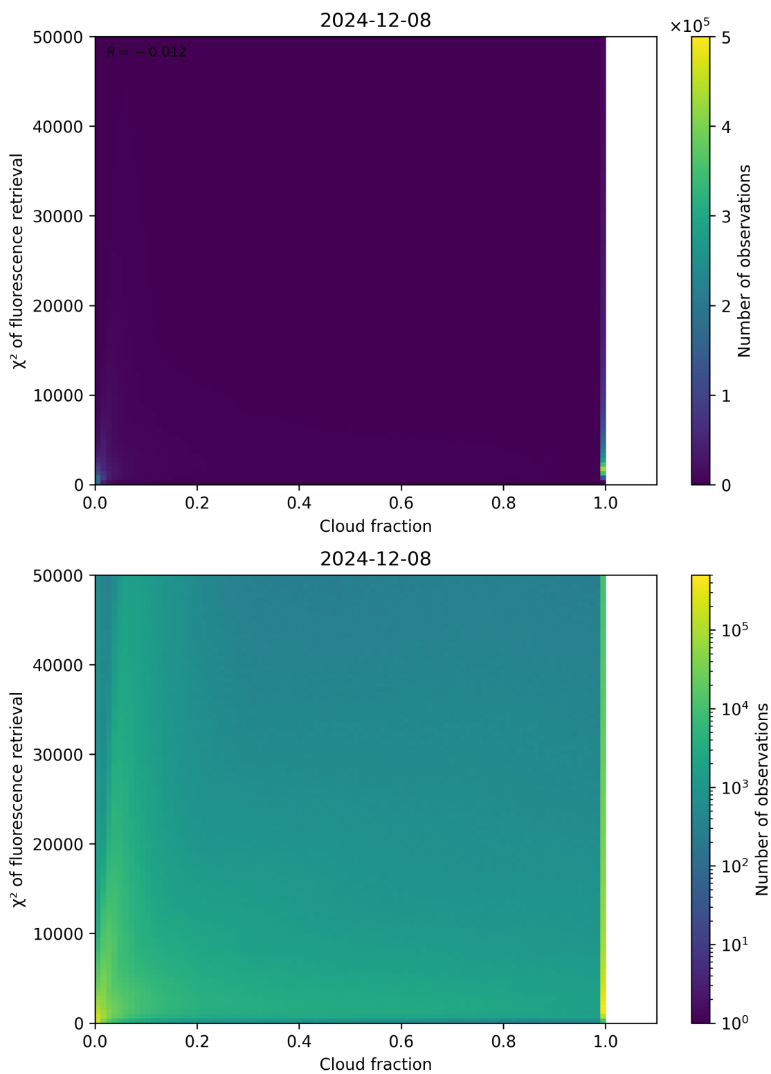
Figure 71: Scatter density plot of “Cloud fraction” against “ \chi^2 of fluorescence retrieval” for 2024-12-07 to 2024-12-09.
