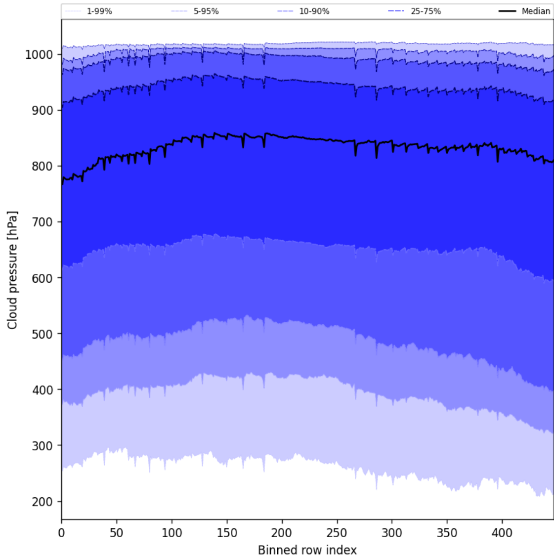
Figure 47: Along track statistics of “Cloud pressure” for 2024-12-07 to 2024-12-09
