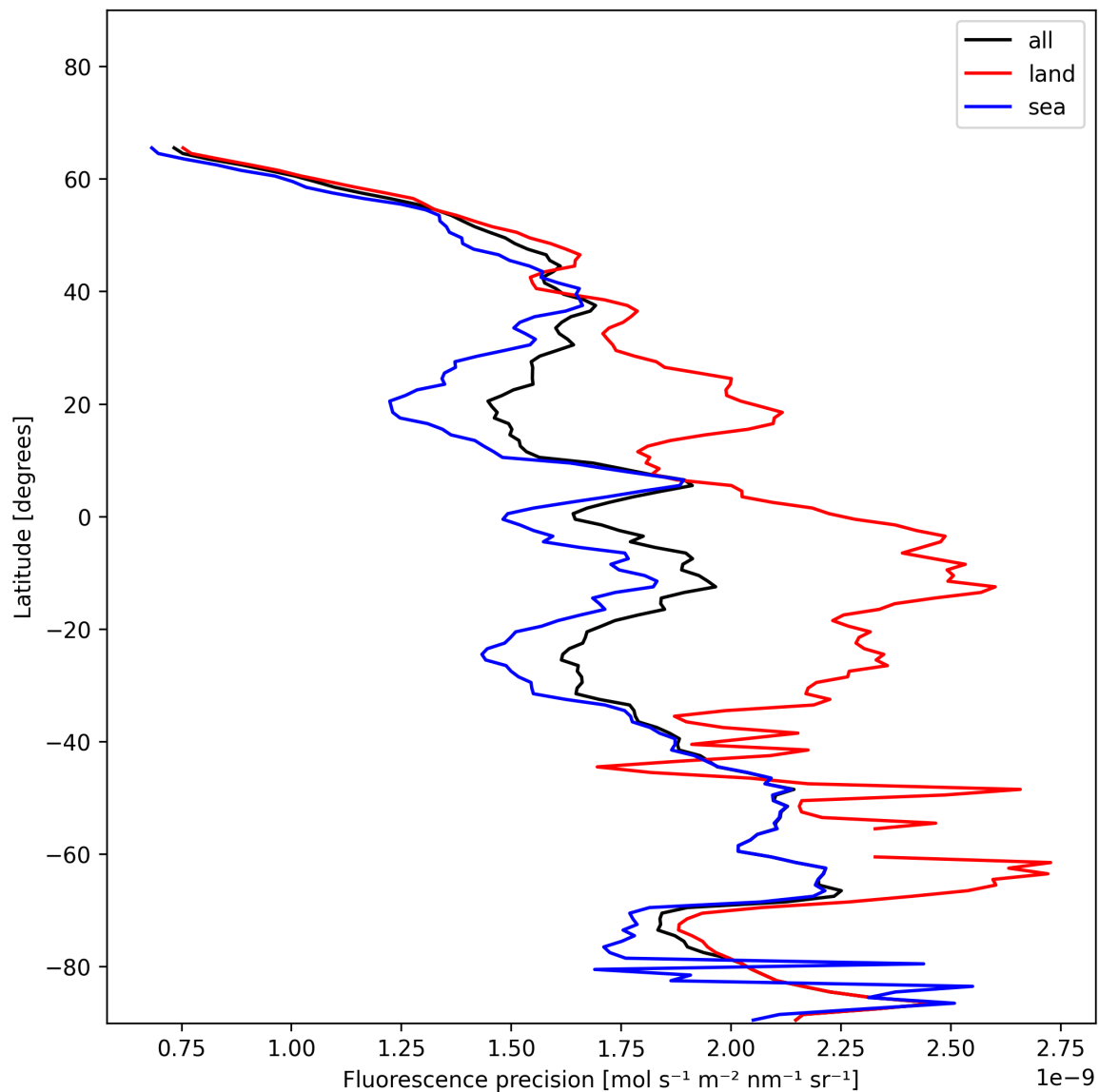
Figure 24: Zonal average of “Fluorescence precision” for 2024-12-07 to 2024-12-09.
