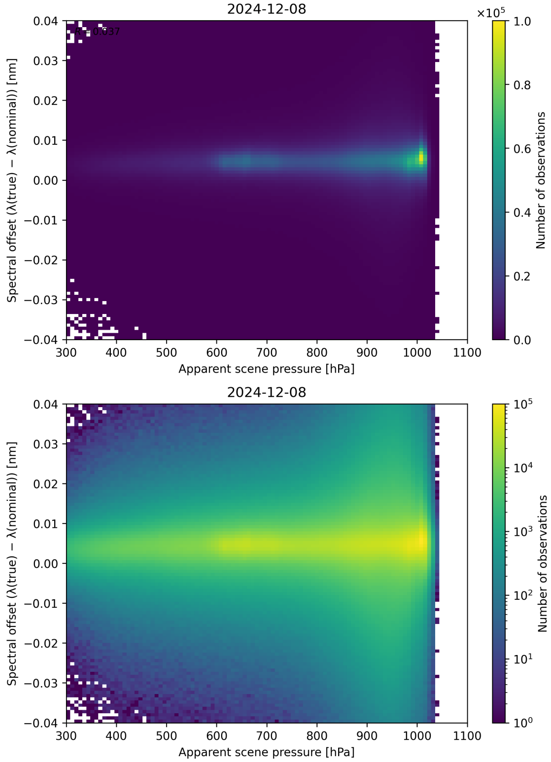
Figure 67: Scatter density plot of “Apparent scene pressure” against “Spectral offset ( \lambda_{\text{true}} - \lambda_{\text{nominal}} )” for 2024-12-07 to 2024-12-09.
