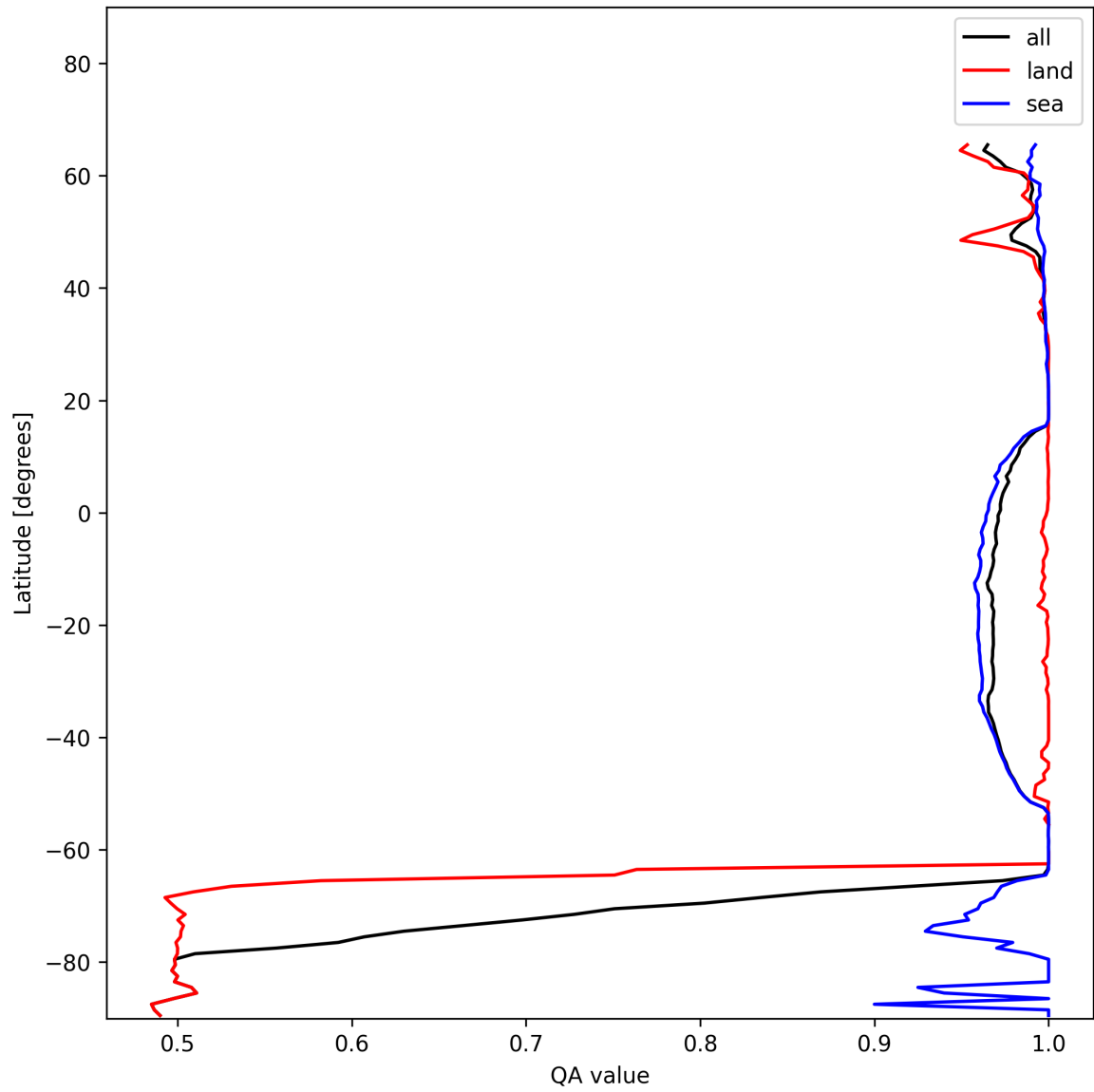
Figure 12: Zonal average of “QA value” for 2024-12-07 to 2024-12-09.
