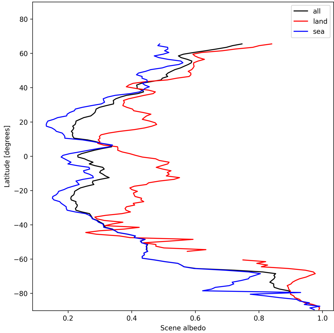
Figure 17: Zonal average of “Scene albedo” for 2024-12-07 to 2024-12-09.
