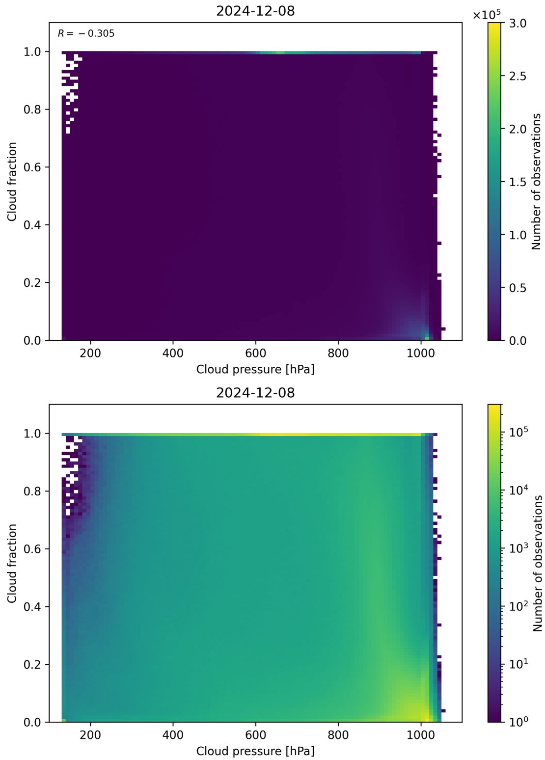
Figure 79: Scatter density plot of “Cloud pressure” against “Cloud fraction” for 2024-12-07 to 2024-12-09.
