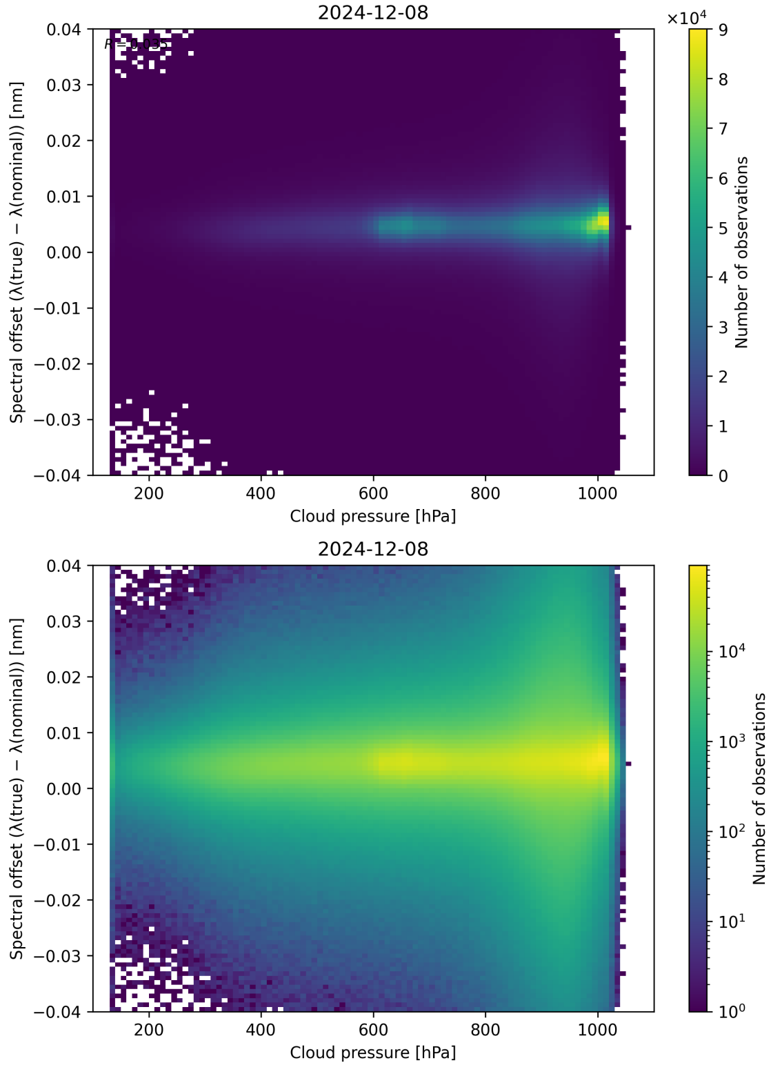
Figure 84: Scatter density plot of “Cloud pressure” against “Spectral offset ( \lambda_{\text{true}} - \lambda_{\text{nominal}} )” for 2024-12-07 to 2024-12-09.
