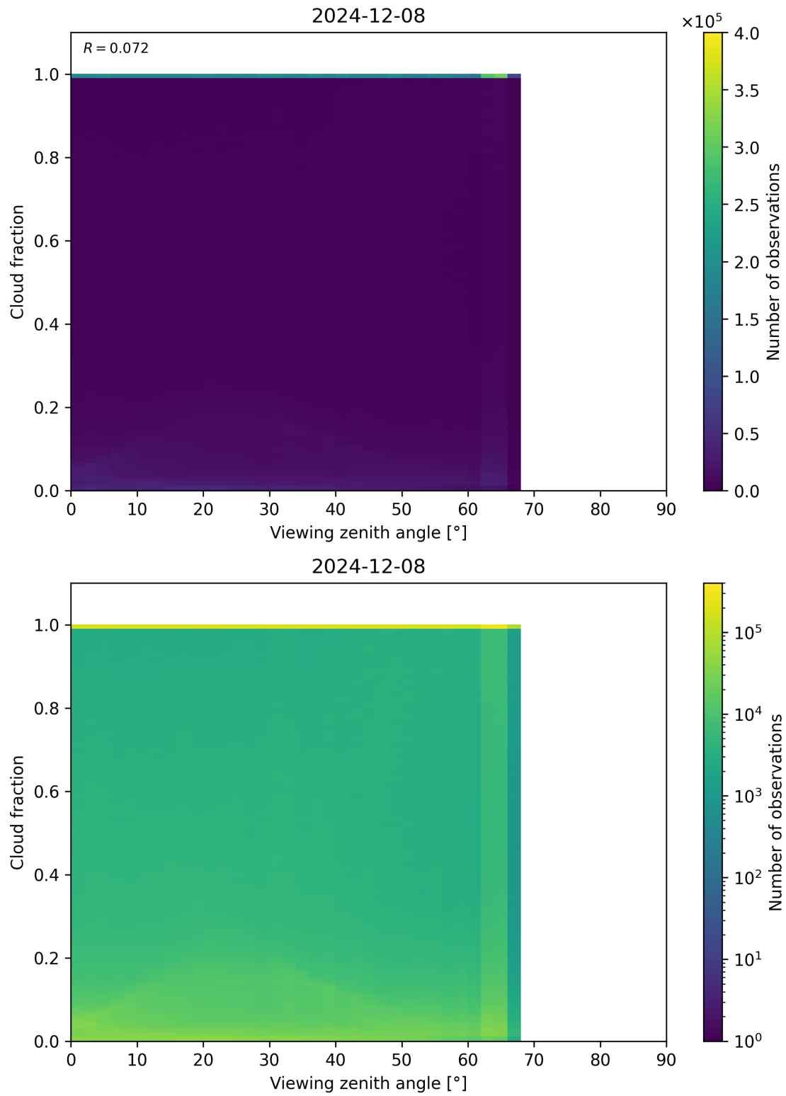
Figure 120: Scatter density plot of “Viewing zenith angle” against “Cloud fraction” for 2024-12-07 to 2024-12-09.
