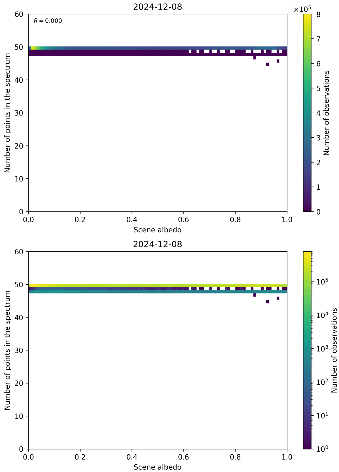
Figure 106: Scatter density plot of “Scene albedo” against “Number of points in the spectrum” for 2024-12-07 to 2024-12-09.
