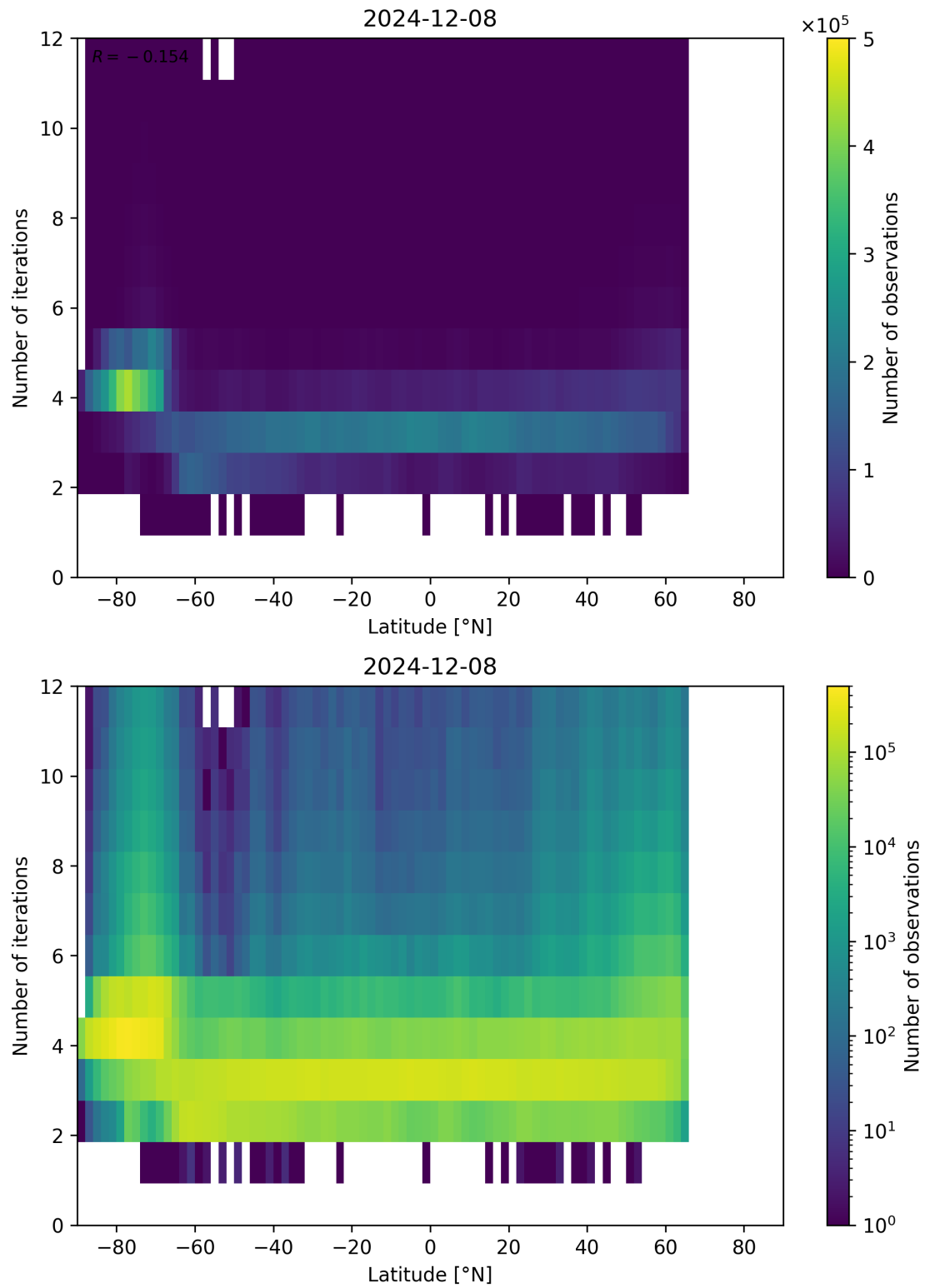
Figure 93: Scatter density plot of “Latitude” against “Number of iterations” for 2024-12-07 to 2024-12-09.
