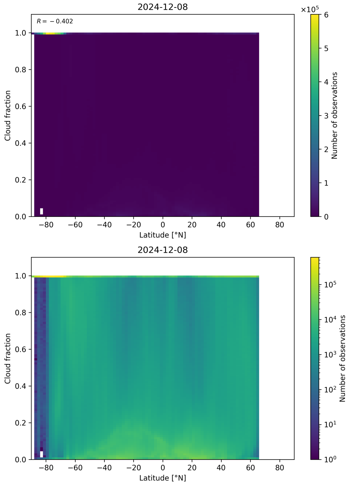
Figure 90: Scatter density plot of “Latitude” against “Cloud fraction” for 2024-12-07 to 2024-12-09.
