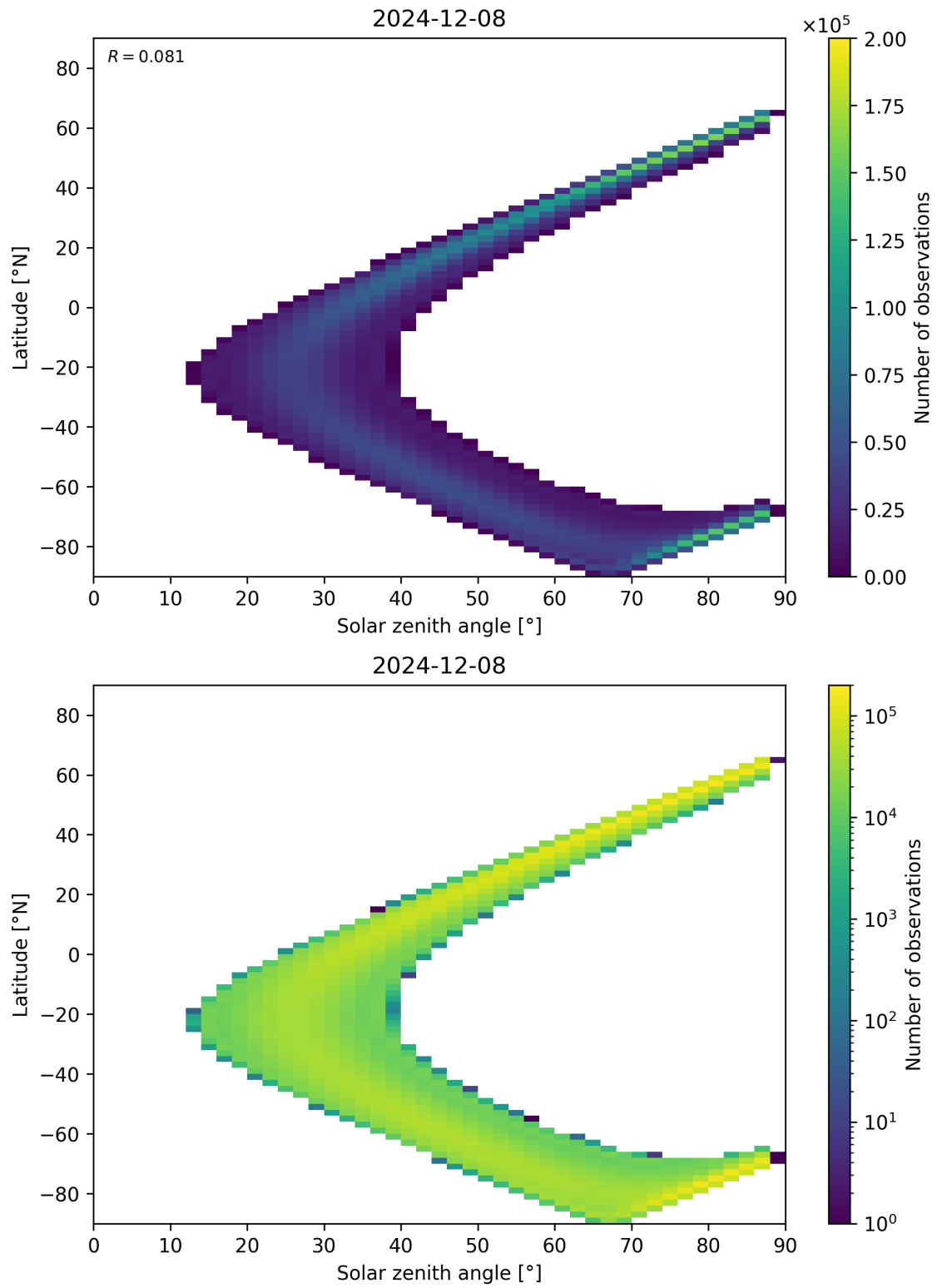
Figure 113: Scatter density plot of “Solar zenith angle” against “Latitude” for 2024-12-07 to 2024-12-09.
