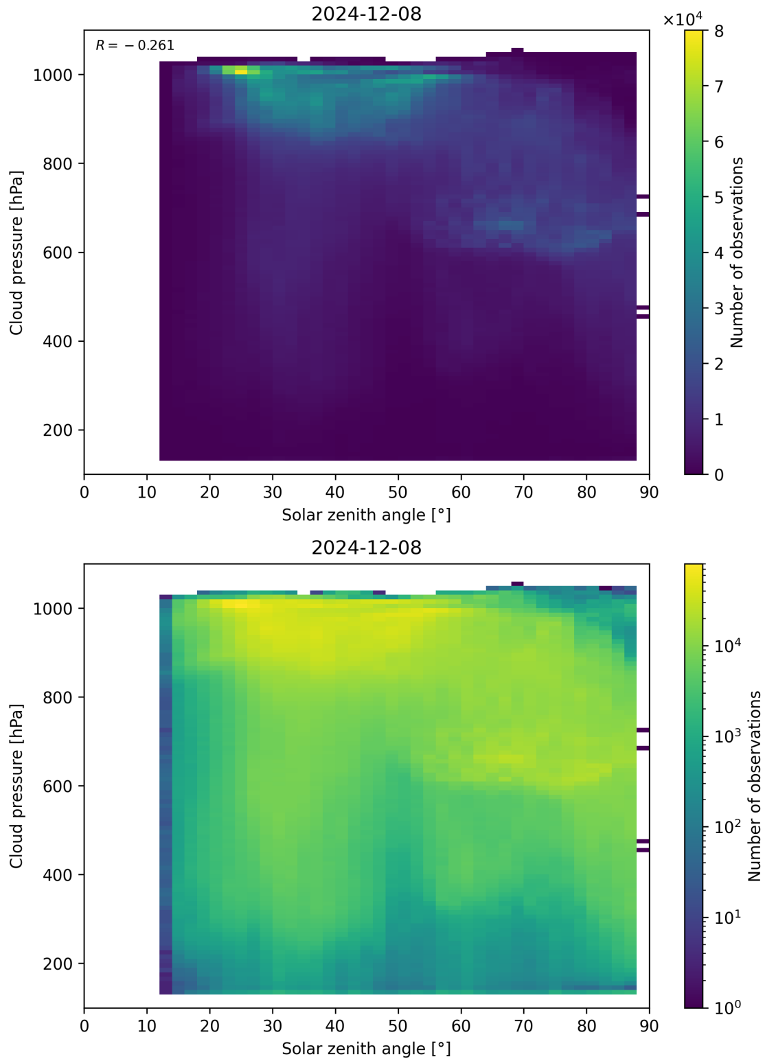
Figure 111: Scatter density plot of “Solar zenith angle” against “Cloud pressure” for 2024-12-07 to 2024-12-09.
