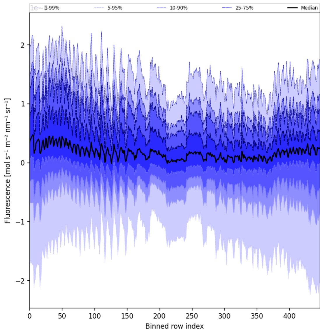
Figure 57: Along track statistics of “Fluorescence” for 2024-12-07 to 2024-12-09
