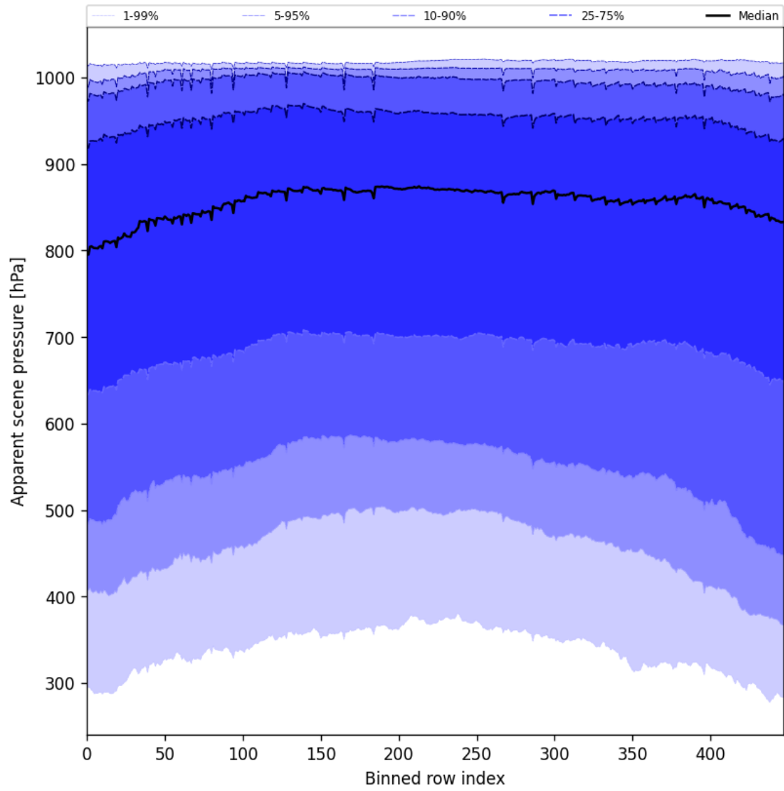
Figure 53: Along track statistics of “Apparent scene pressure” for 2024-12-07 to 2024-12-09
