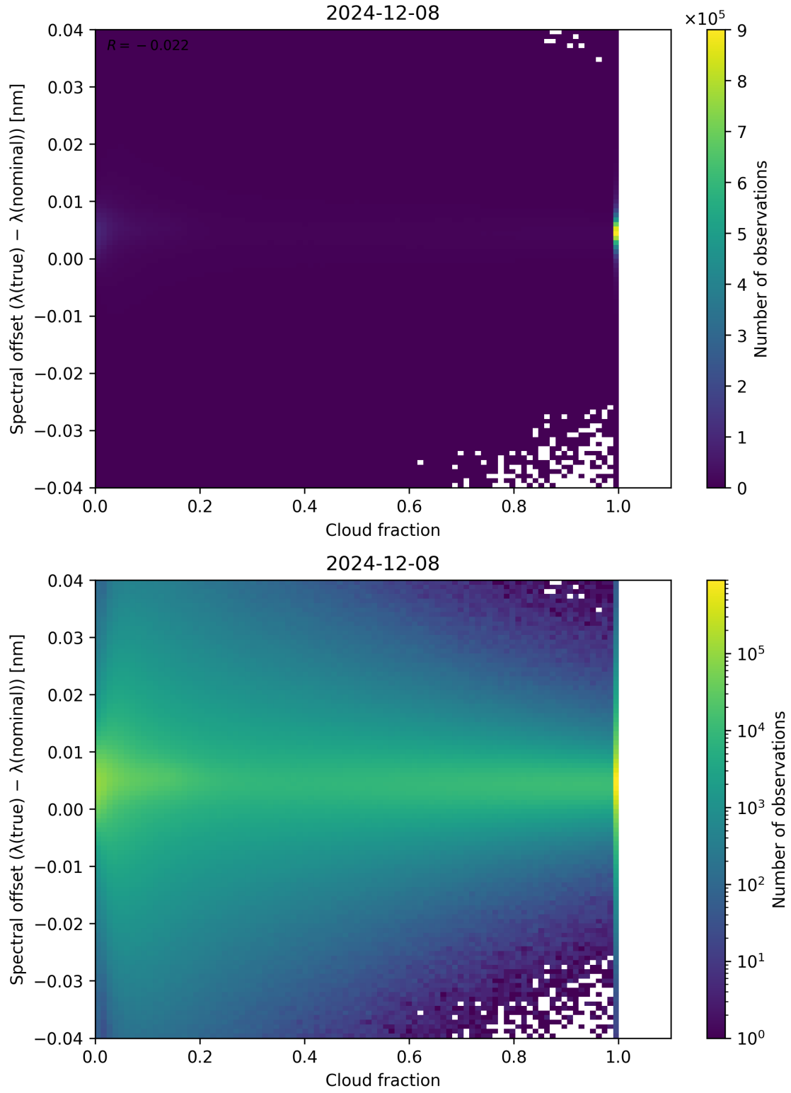
Figure 76: Scatter density plot of “Cloud fraction” against “Spectral offset ( \lambda_{\text{true}} - \lambda_{\text{nominal}} )” for 2024-12-07 to 2024-12-09.
