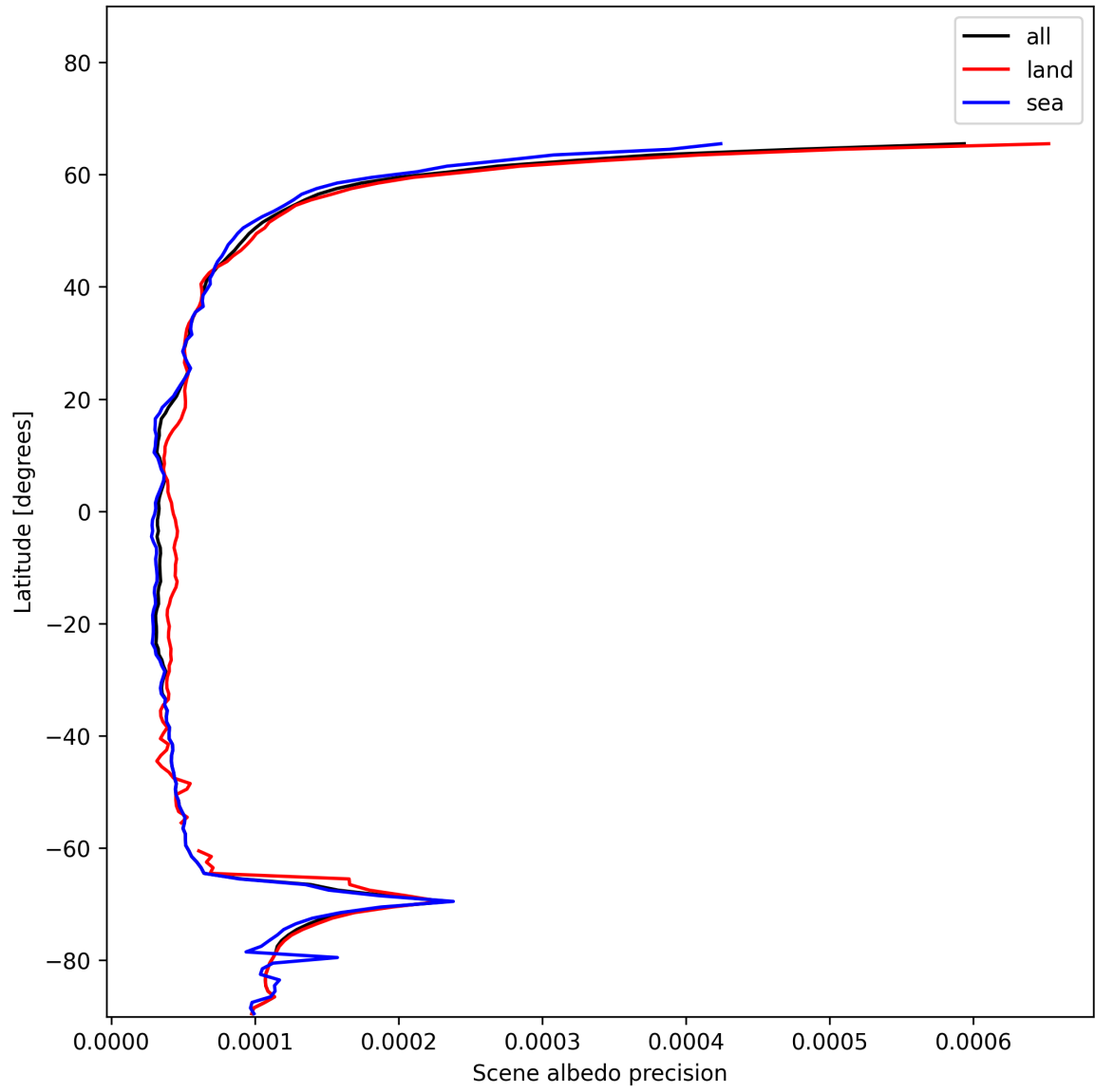
Figure 18: Zonal average of “Scene albedo precision” for 2024-12-07 to 2024-12-09.
