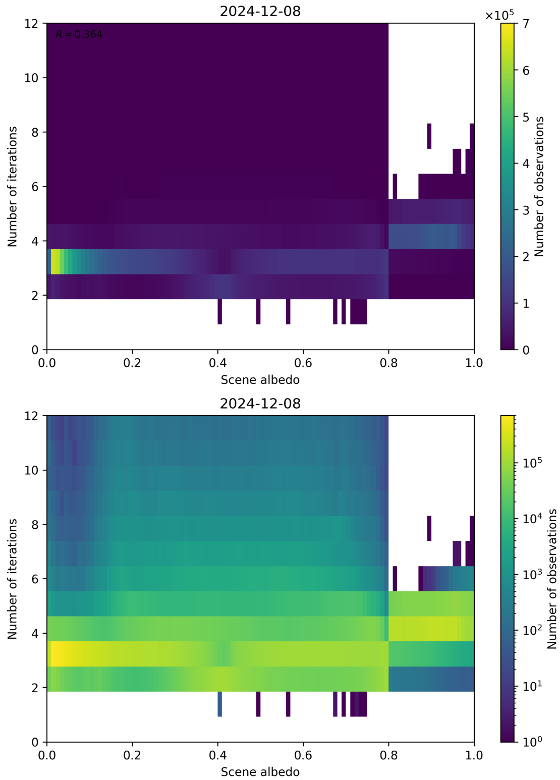
Figure 105: Scatter density plot of “Scene albedo” against “Number of iterations” for 2024-12-07 to 2024-12-09.
