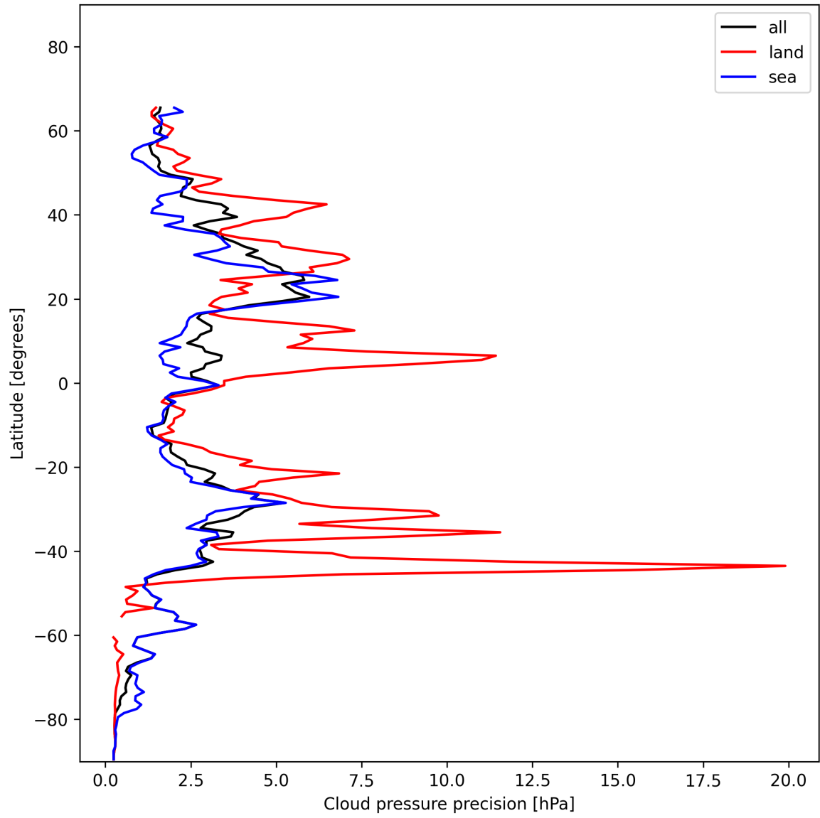
Figure 14: Zonal average of "Cloud pressure precision" for 2024-12-07 to 2024-12-09.
