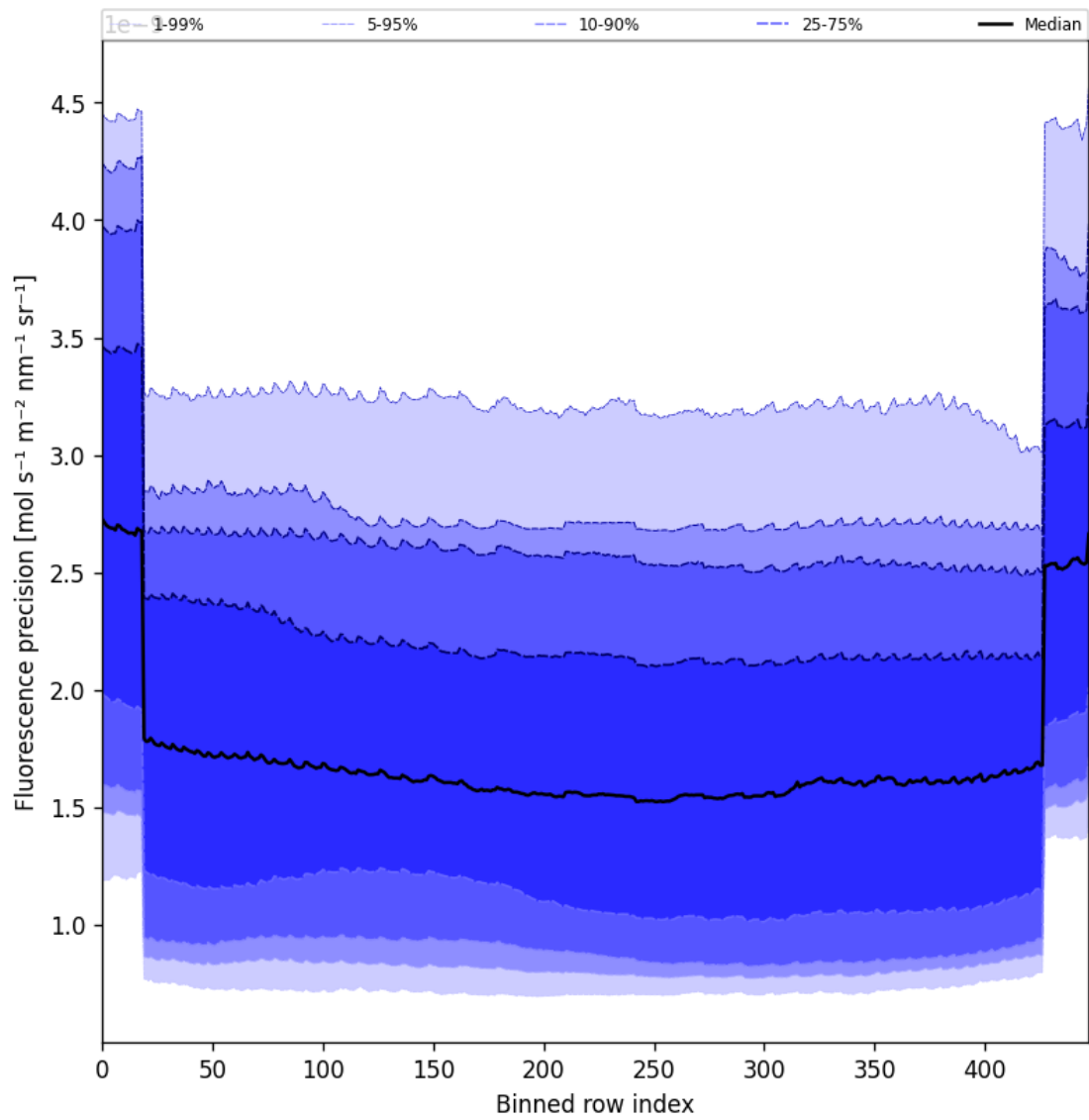
Figure 58: Along track statistics of “Fluorescence precision” for 2024-12-07 to 2024-12-09
