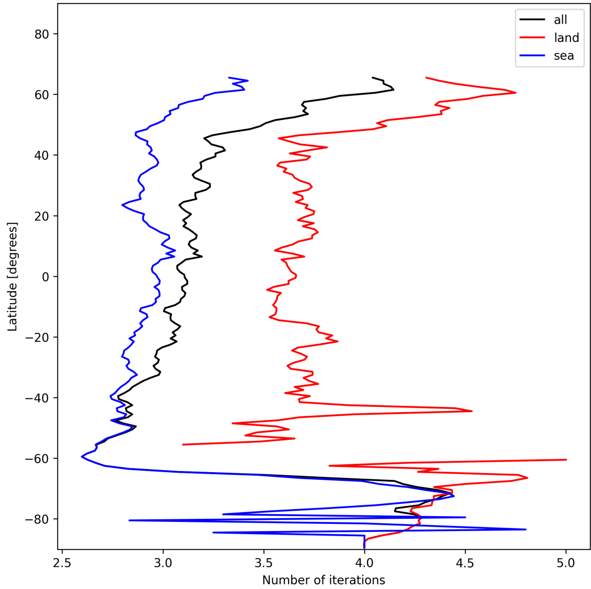
Figure 22: Zonal average of “Number of iterations” for 2024-12-07 to 2024-12-09.
