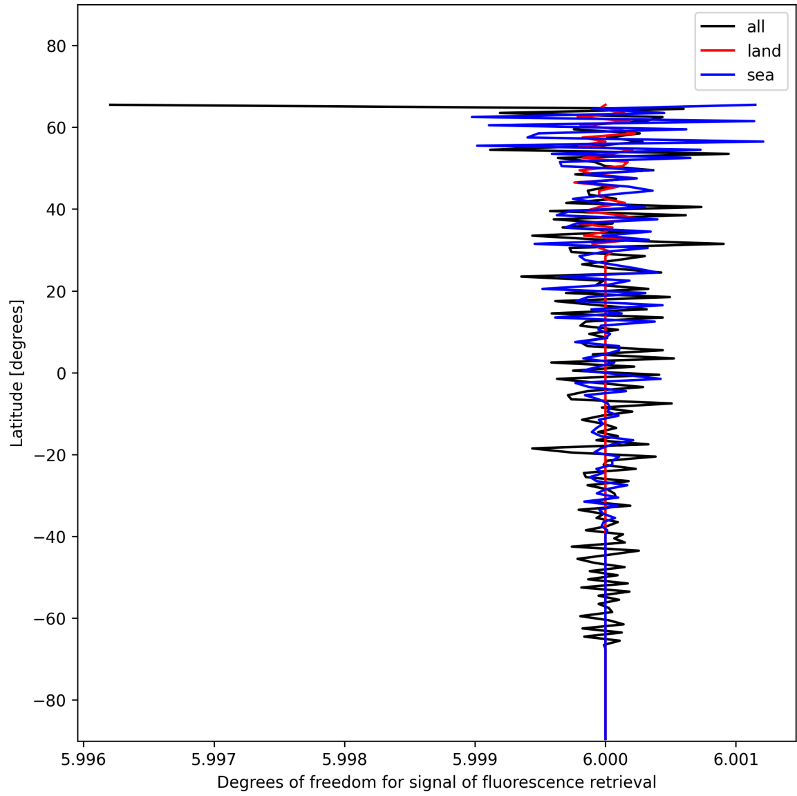
Figure 26: Zonal average of “Degrees of freedom for signal of fluorescence retrieval” for 2024-12-07 to 2024-12-09.
