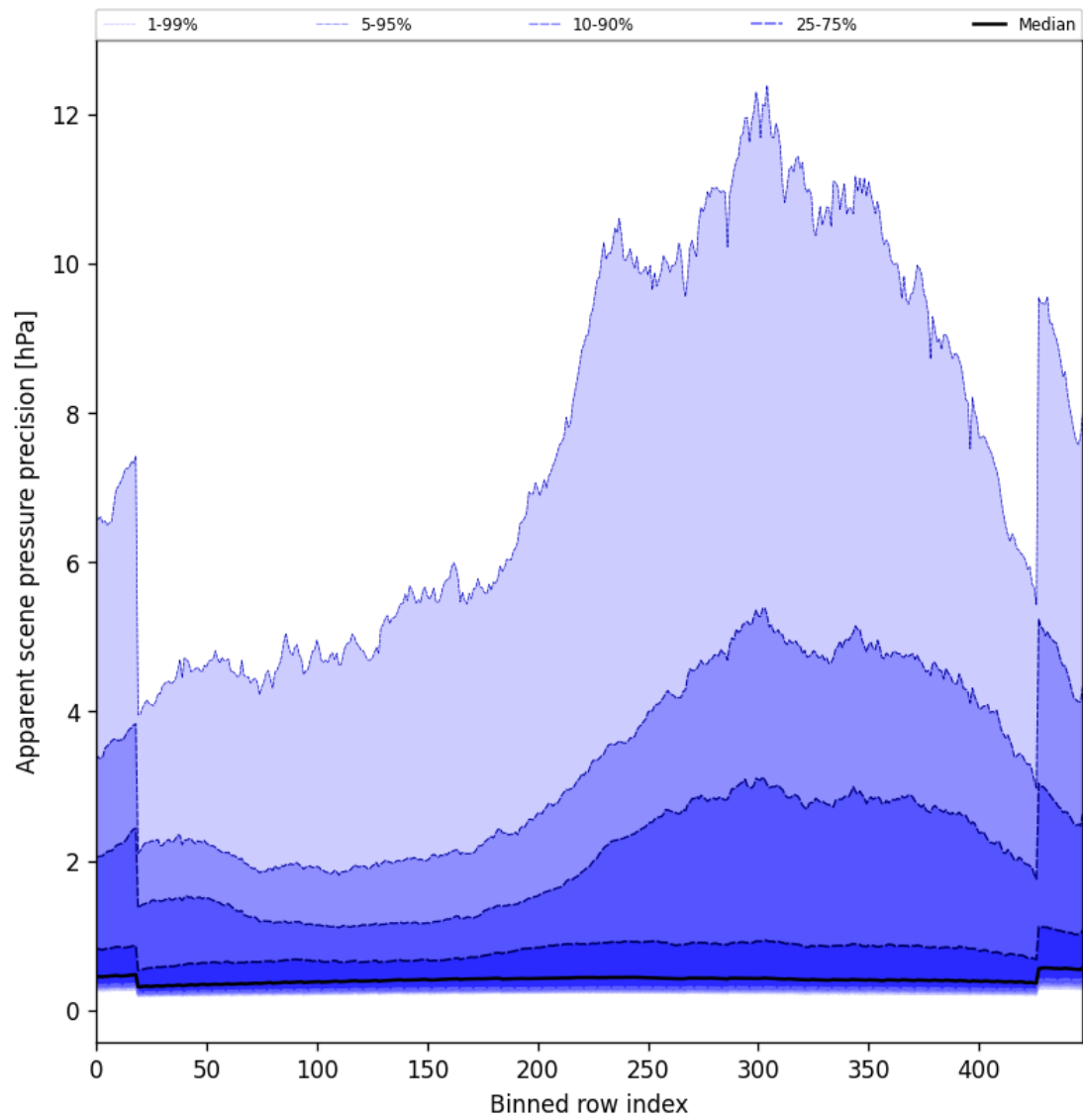
Figure 54: Along track statistics of “Apparent scene pressure precision” for 2024-12-07 to 2024-12-09
