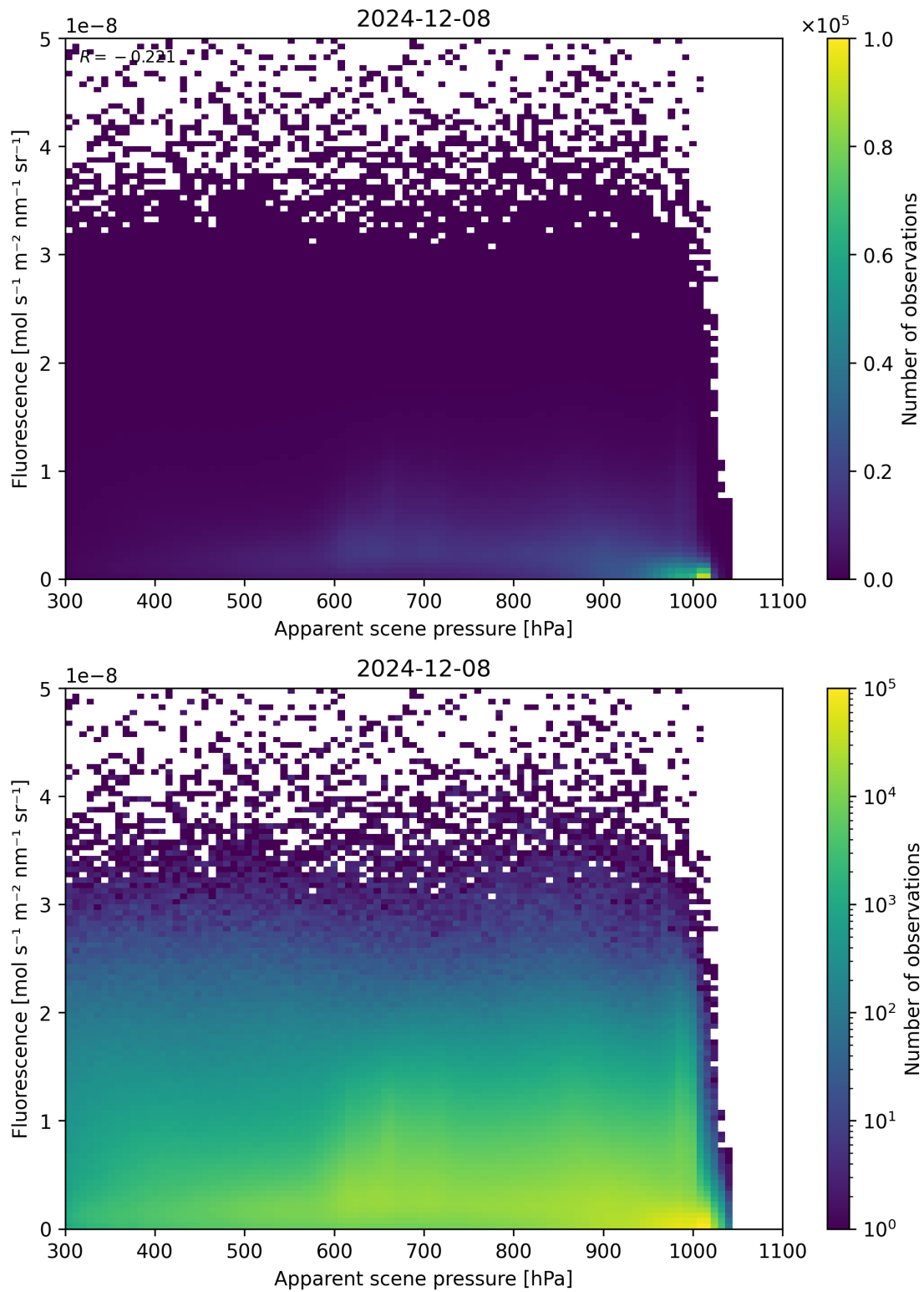
Figure 64: Scatter density plot of “Apparent scene pressure” against “Fluorescence” for 2024-12-07 to 2024-12-09.
