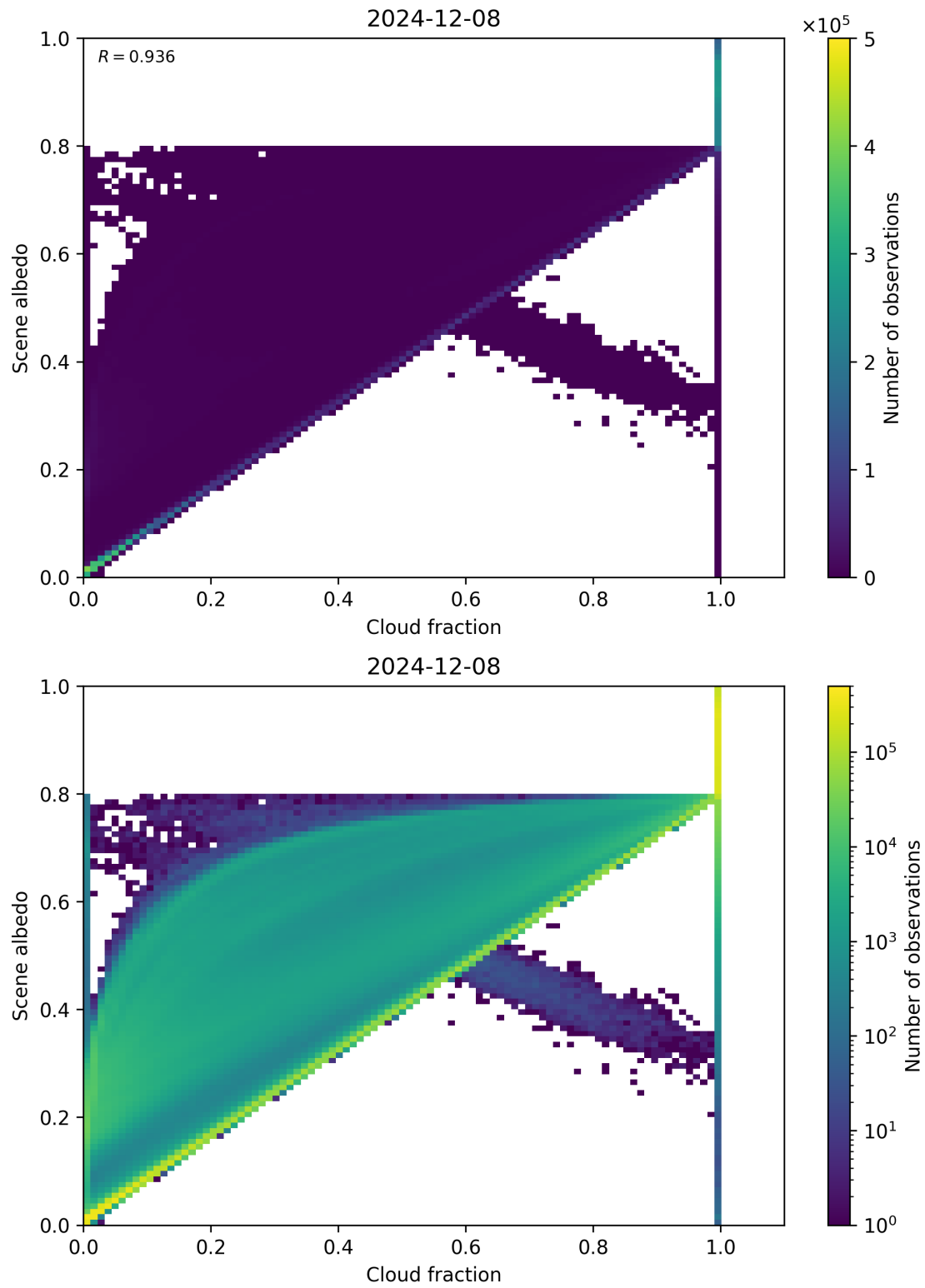
Figure 75: Scatter density plot of “Cloud fraction” against “Scene albedo” for 2024-12-07 to 2024-12-09.
