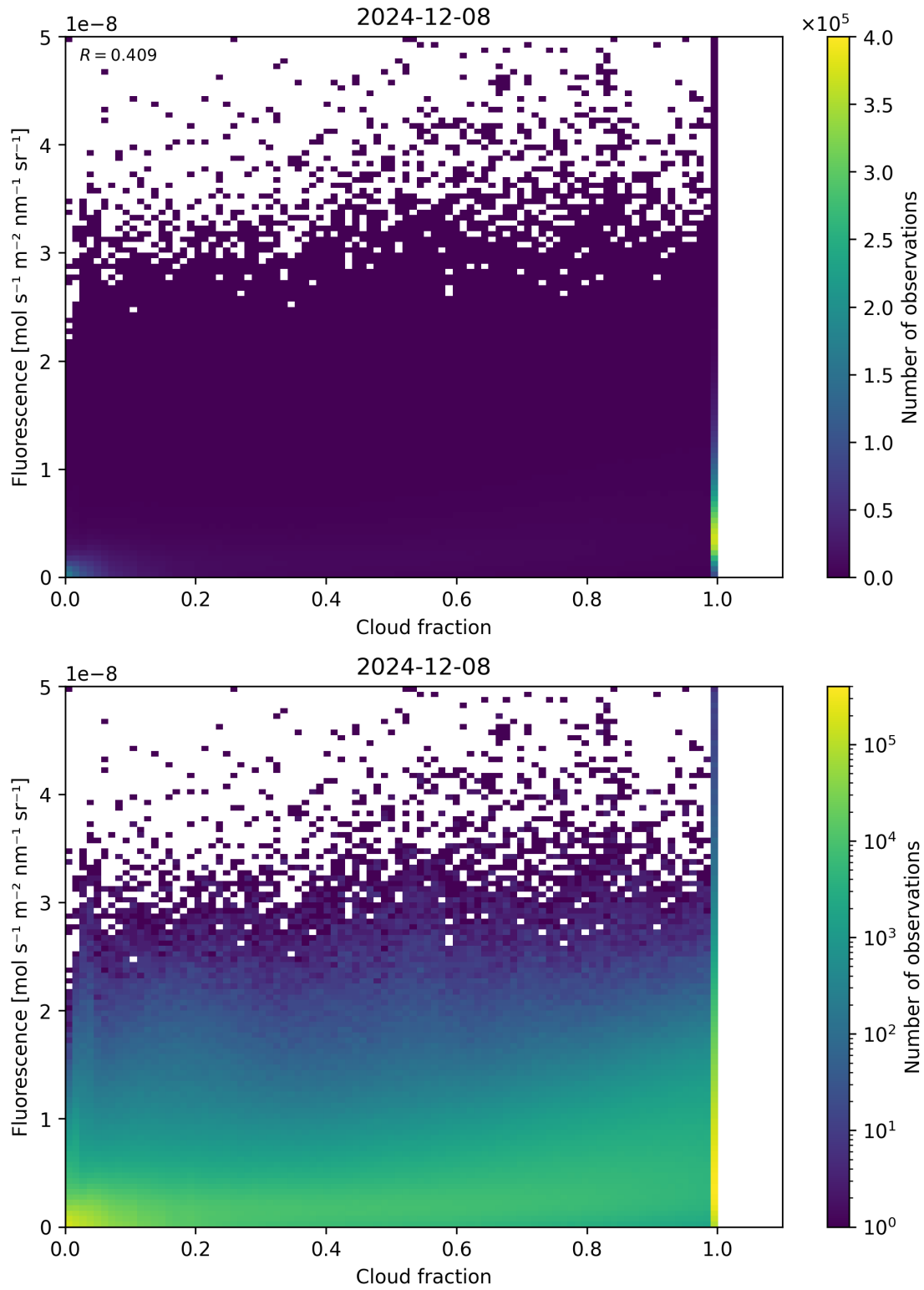
Figure 72: Scatter density plot of “Cloud fraction” against “Fluorescence” for 2024-12-07 to 2024-12-09.
