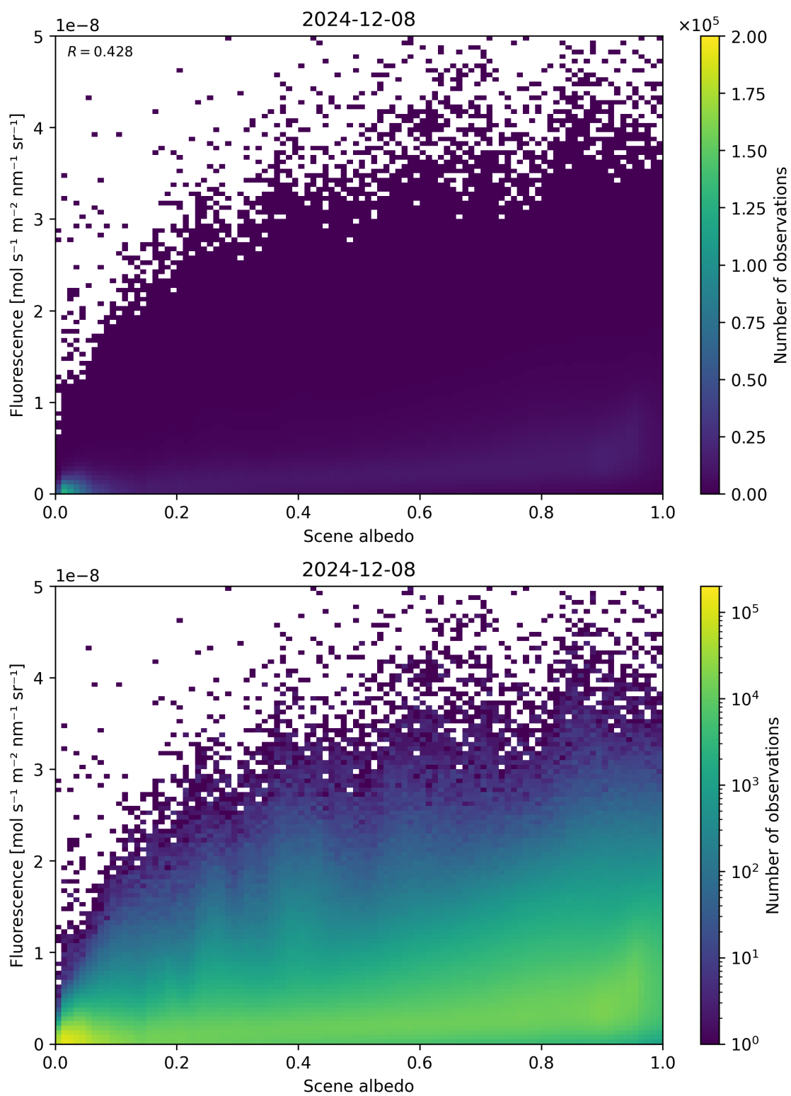
Figure 104: Scatter density plot of “Scene albedo” against “Fluorescence” for 2024-12-07 to 2024-12-09.
