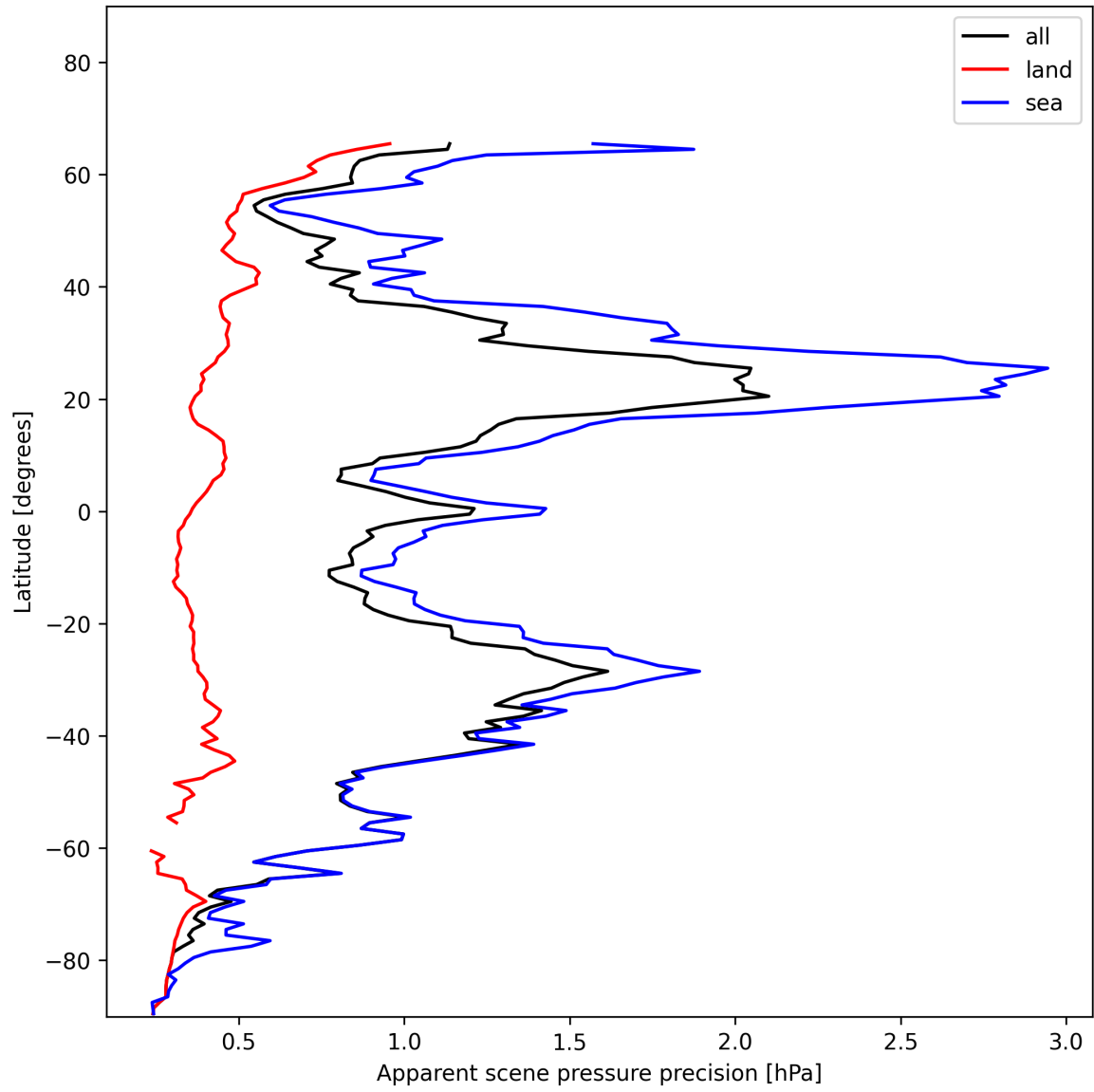
Figure 20: Zonal average of “Apparent scene pressure precision” for 2024-12-07 to 2024-12-09.
