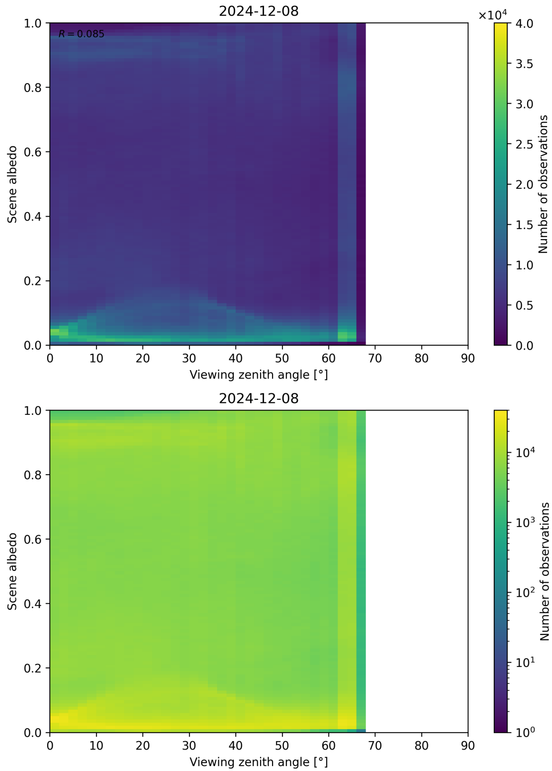
Figure 126: Scatter density plot of “Viewing zenith angle” against “Scene albedo” for 2024-12-07 to 2024-12-09.
