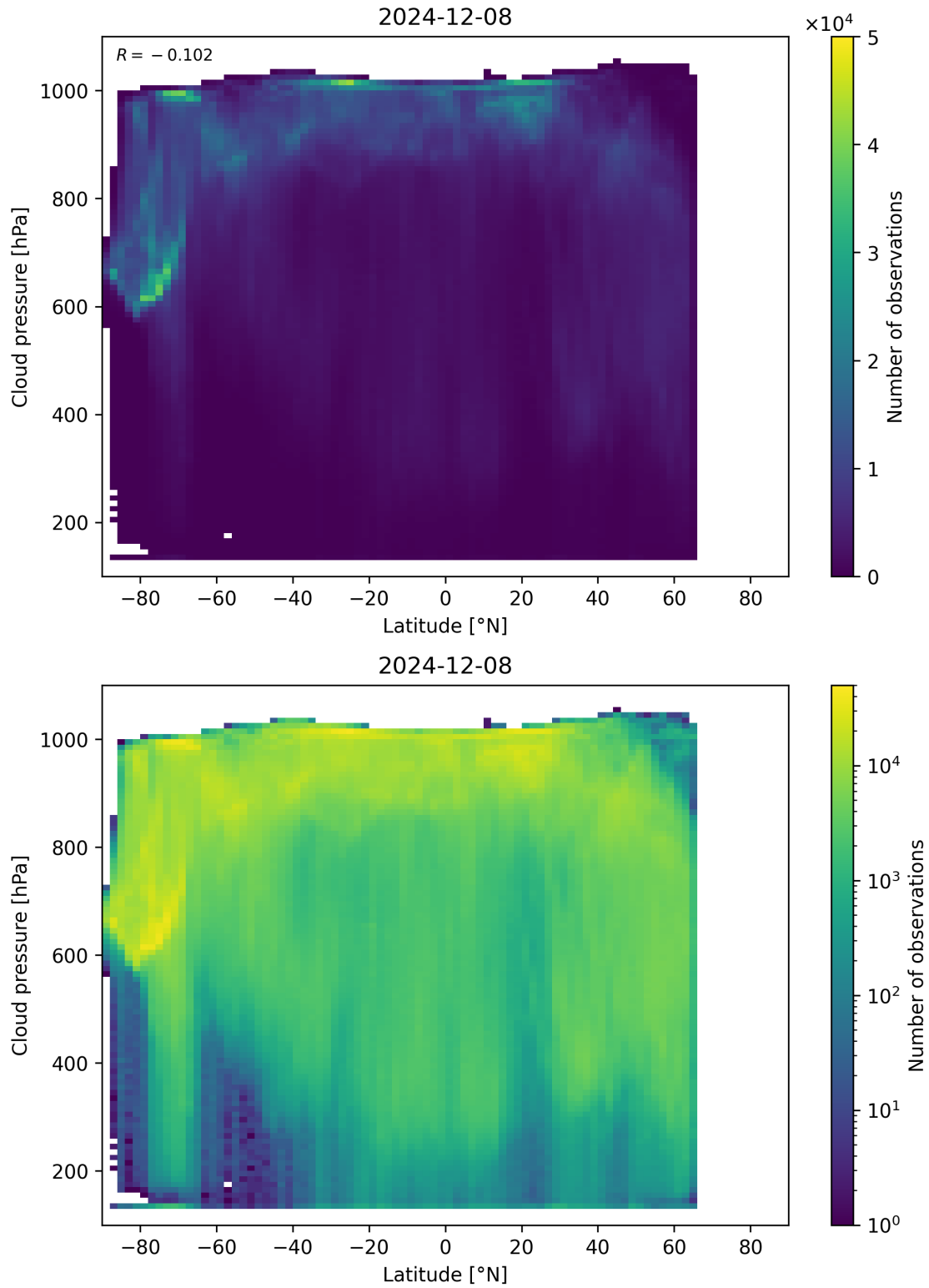
Figure 91: Scatter density plot of “Latitude” against “Cloud pressure” for 2024-12-07 to 2024-12-09.
