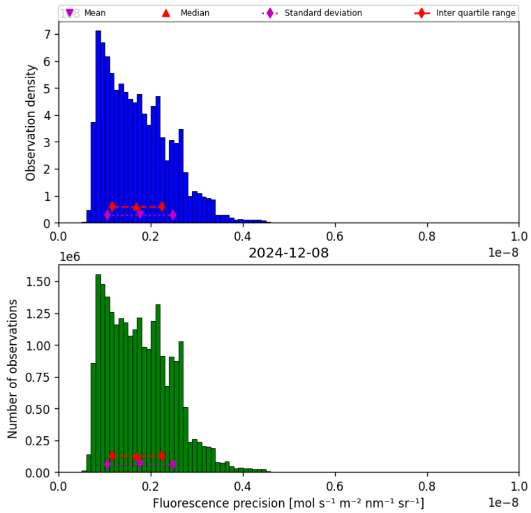
Figure 41: Histogram of “Fluorescence precision” for 2024-12-07 to 2024-12-09
