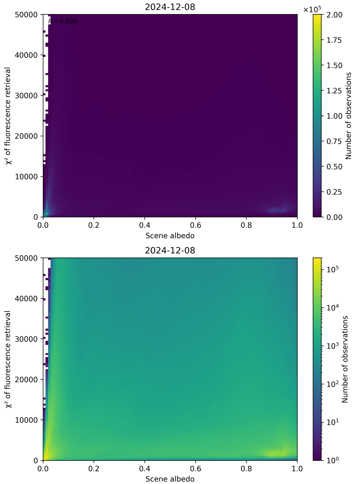
Figure 103: Scatter density plot of “Scene albedo” against “ \chi^2 of fluorescence retrieval” for 2024-12-07 to 2024-12-09.
