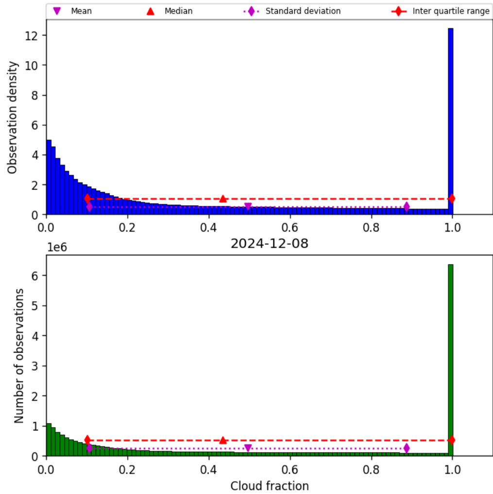
Figure 32: Histogram of “Cloud fraction” for 2024-12-07 to 2024-12-09
