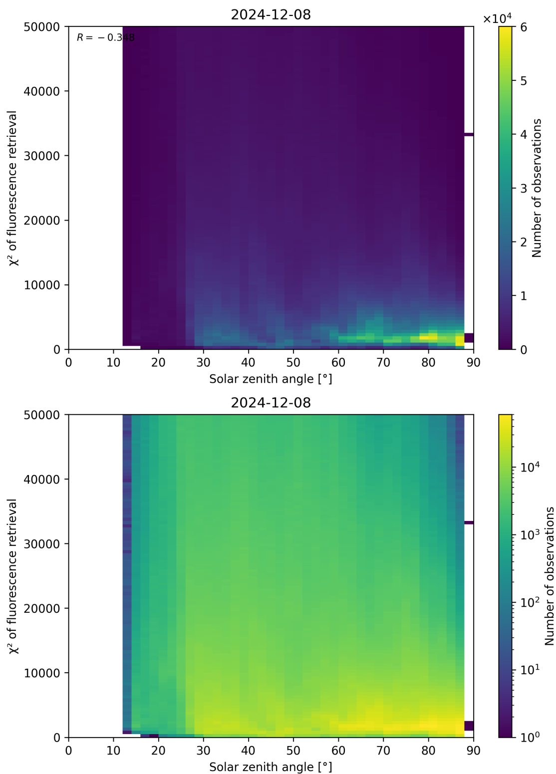
Figure 109: Scatter density plot of “Solar zenith angle” against “ \chi^2 of fluorescence retrieval” for 2024-12-07 to 2024-12-09.
