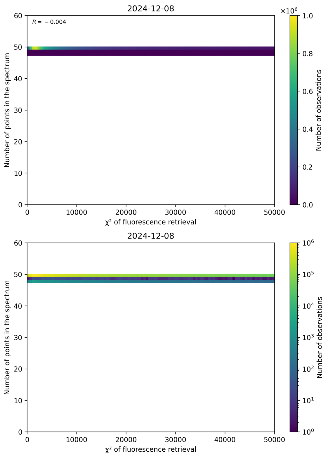
Figure 68: Scatter density plot of " \chi^2 of fluorescence retrieval" against "Number of points in the spectrum" for 2024-12-07 to 2024-12-09.
