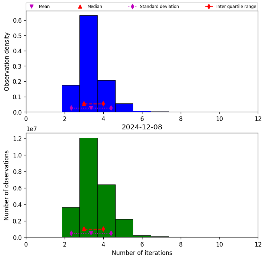
Figure 39: Histogram of “Number of iterations” for 2024-12-07 to 2024-12-09
