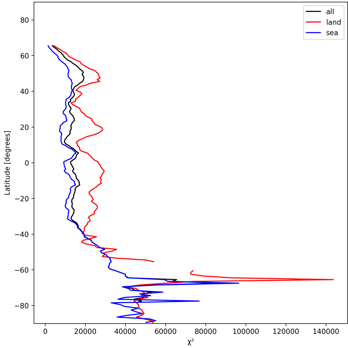
Figure 21: Zonal average of “ \chi^2 ” for 2024-12-07 to 2024-12-09.
