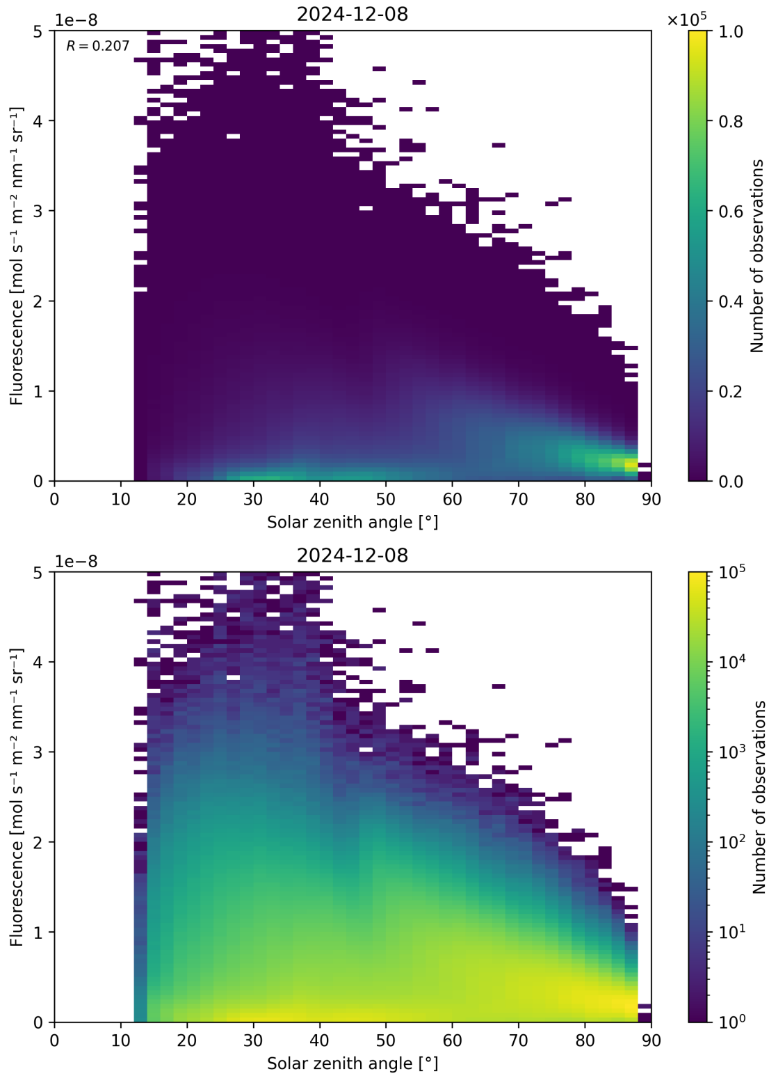
Figure 112: Scatter density plot of “Solar zenith angle” against “Fluorescence” for 2024-12-07 to 2024-12-09.
