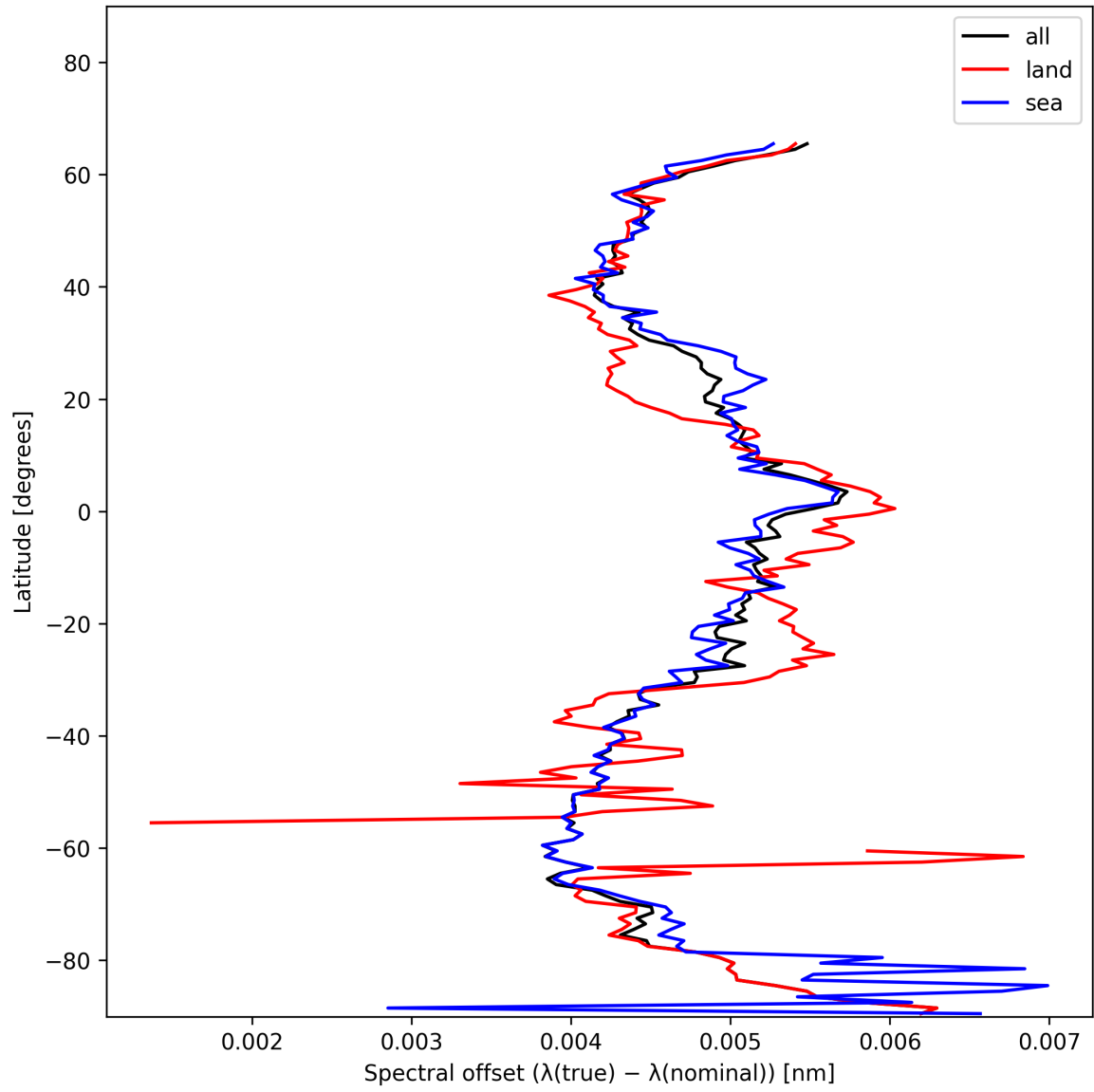
Figure 28: Zonal average of “Spectral offset ( \lambda_{\text{true}} - \lambda_{\text{nominal}} )” for 2024-12-07 to 2024-12-09.
