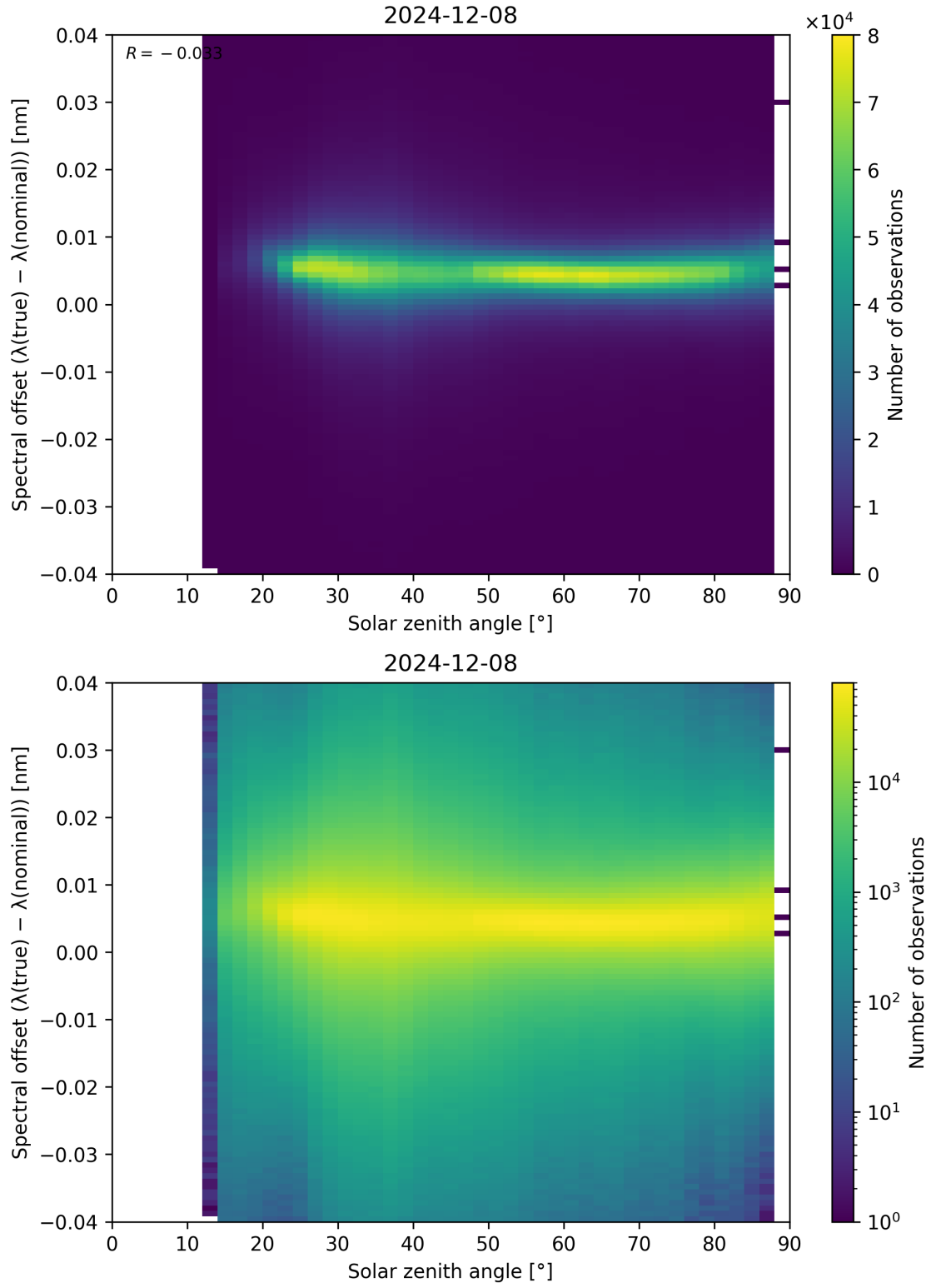
Figure 117: Scatter density plot of “Solar zenith angle” against “Spectral offset ( \lambda_{\text{true}} - \lambda_{\text{nominal}} )” for 2024-12-07 to 2024-12-09.
