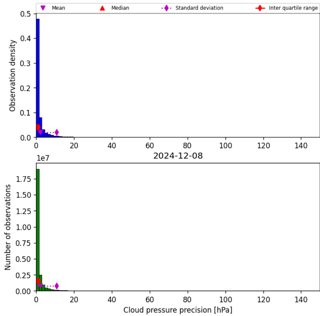
Figure 31: Histogram of “Cloud pressure precision” for 2024-12-07 to 2024-12-09
