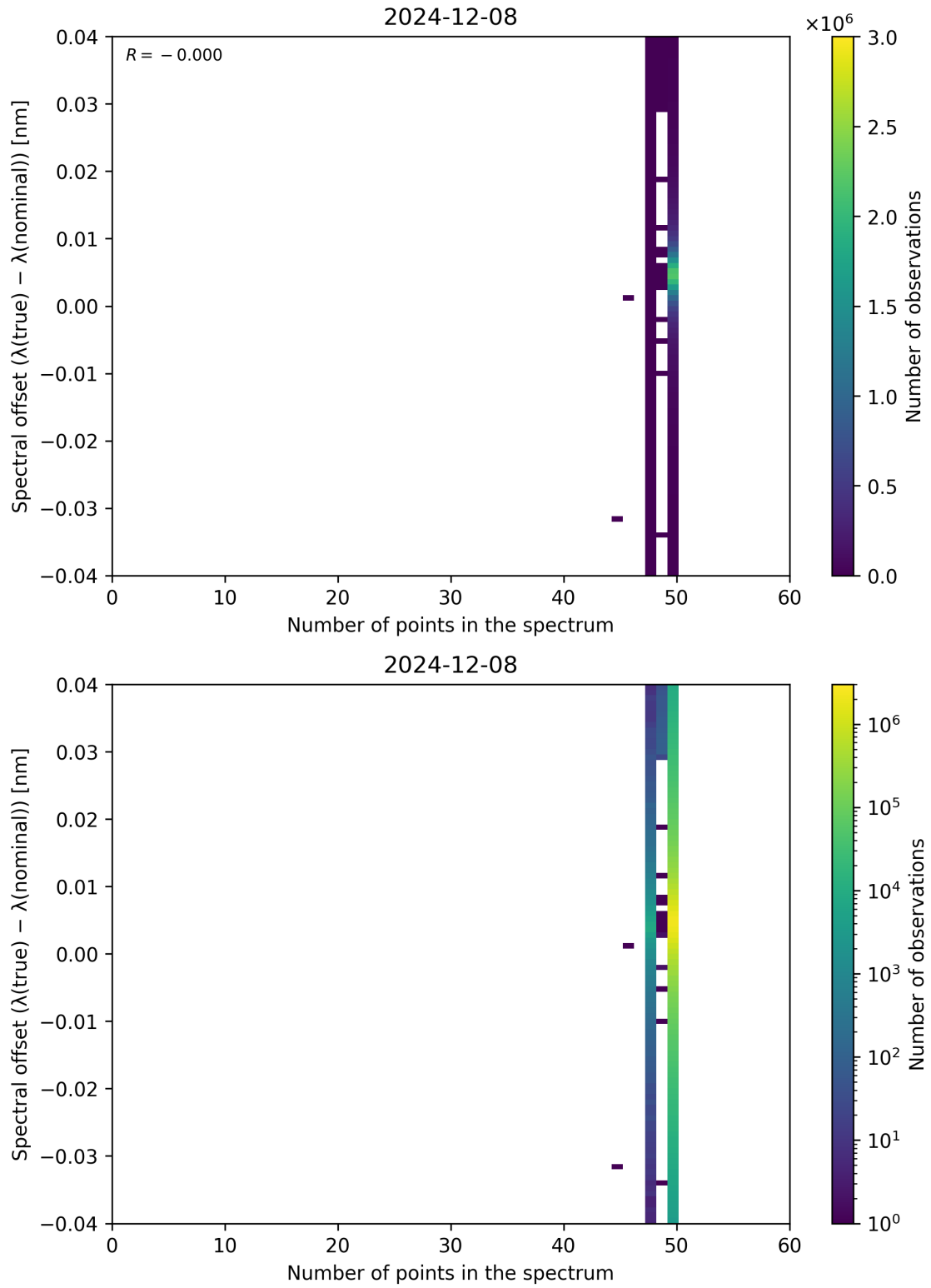
Figure 101: Scatter density plot of “Number of points in the spectrum” against “Spectral offset ( \lambda_{\text{true}} - \lambda_{\text{nominal}} )” for 2024-12-07 to 2024-12-09.
