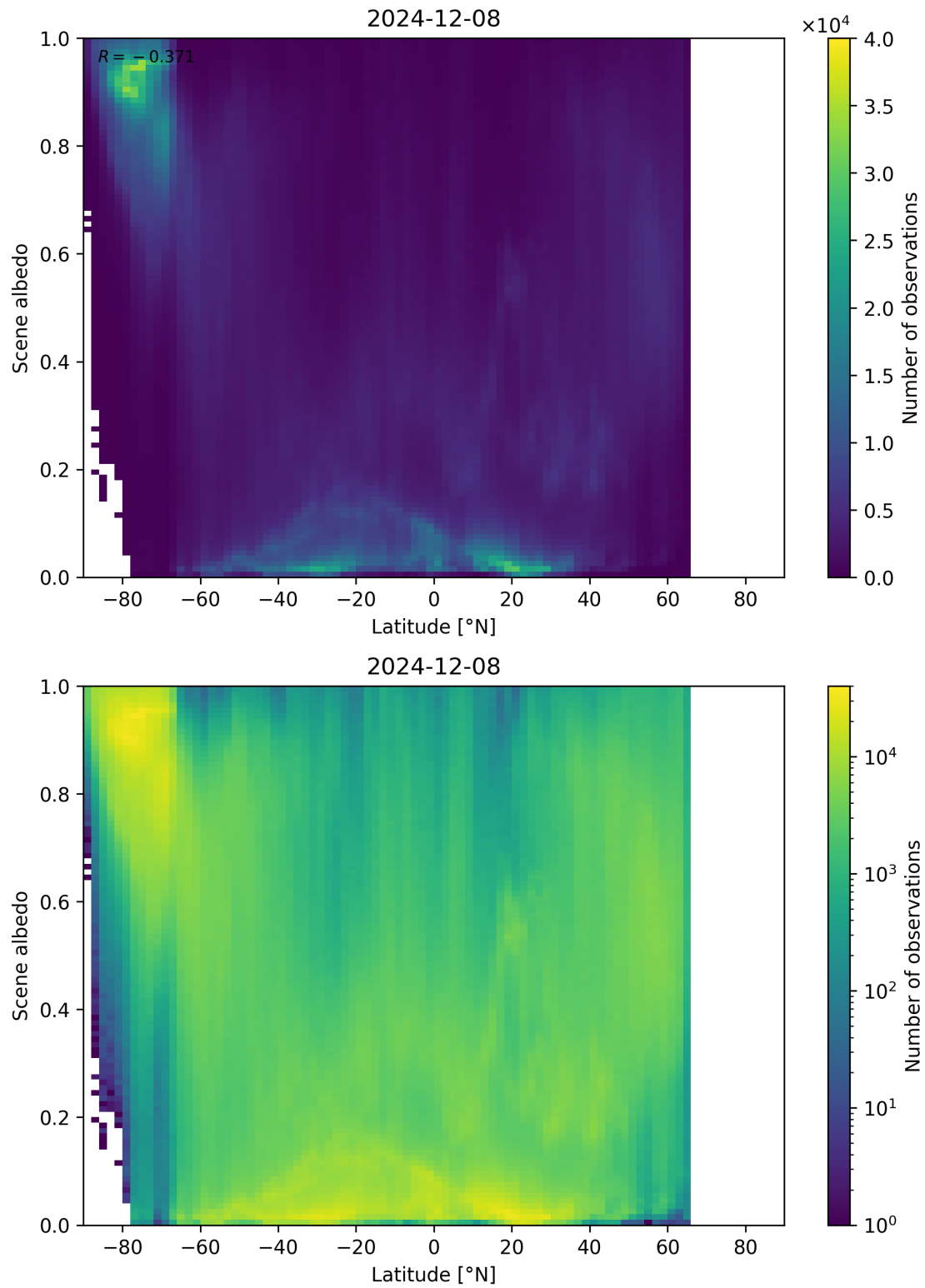
Figure 95: Scatter density plot of “Latitude” against “Scene albedo” for 2024-12-07 to 2024-12-09.
