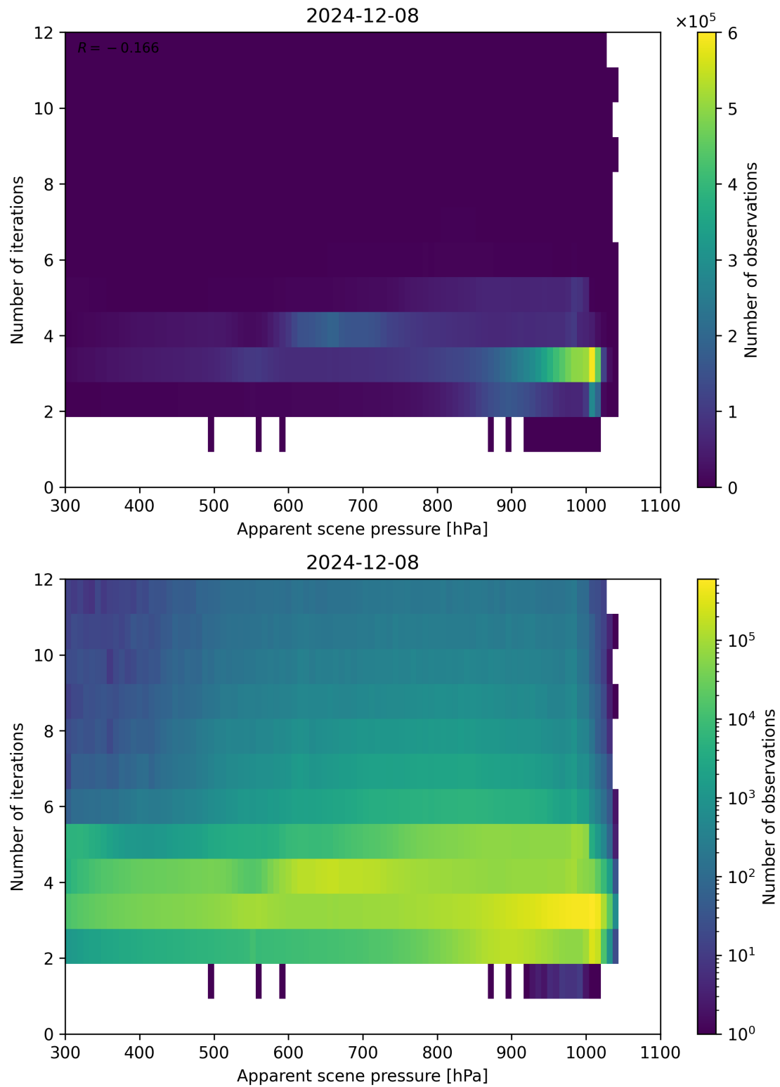
Figure 65: Scatter density plot of “Apparent scene pressure” against “Number of iterations” for 2024-12-07 to 2024-12-09.
