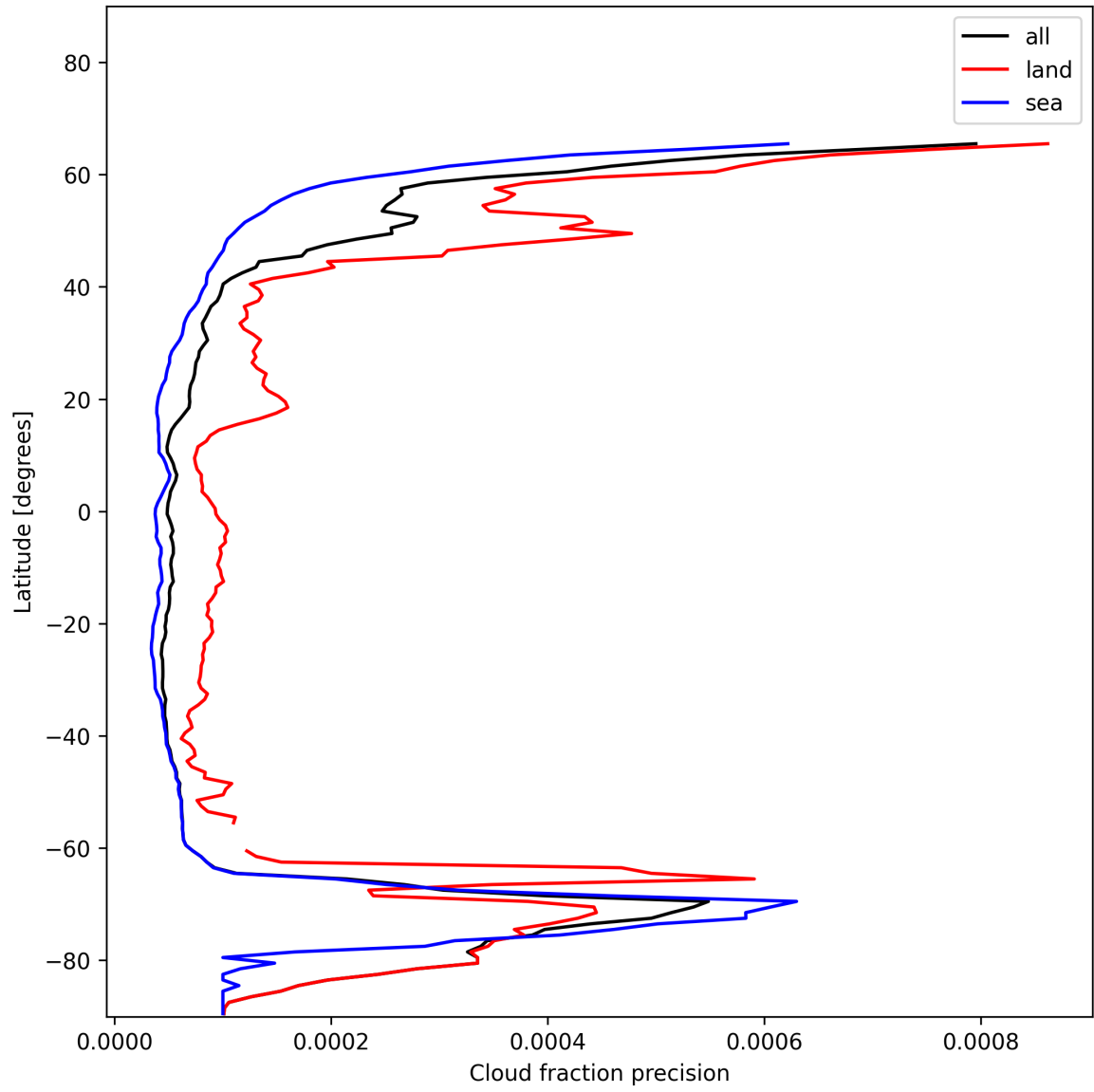
Figure 16: Zonal average of “Cloud fraction precision” for 2024-12-07 to 2024-12-09.
