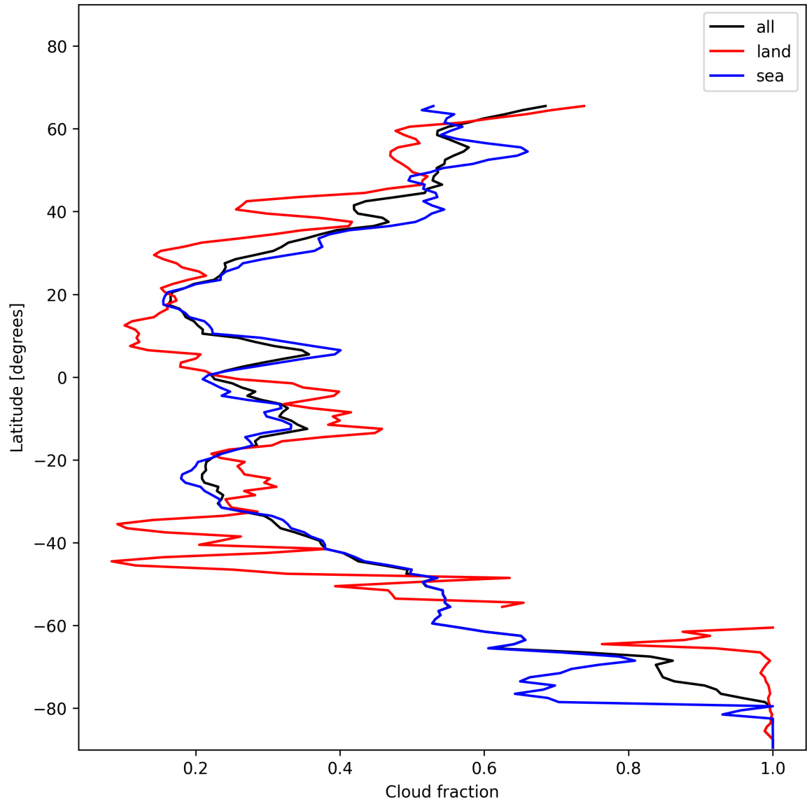
Figure 15: Zonal average of “Cloud fraction” for 2024-12-07 to 2024-12-09.
