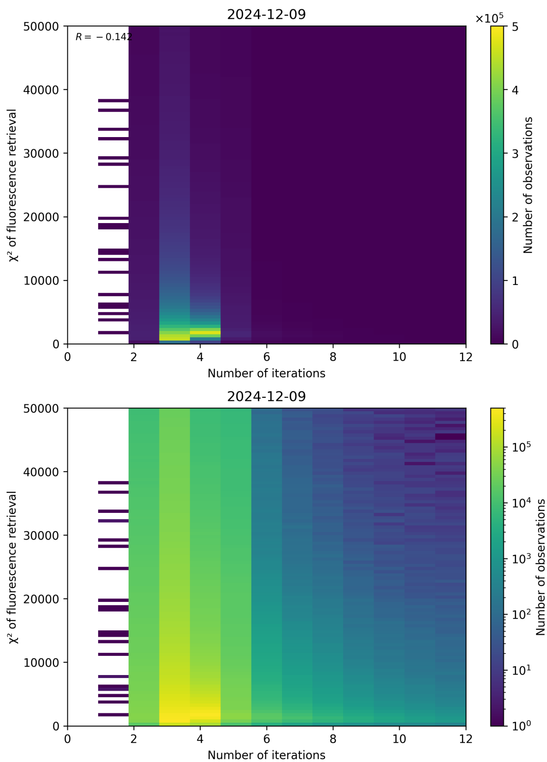
Figure 97: Scatter density plot of “Number of iterations” against “ \chi^2 of fluorescence retrieval” for 2024-12-08 to 2024-12-10.
