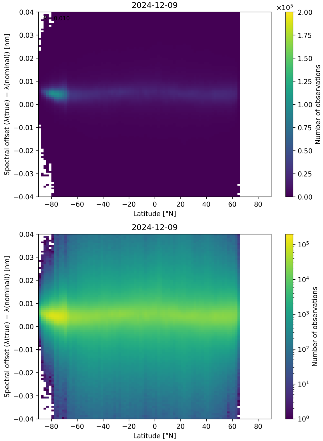
Figure 96: Scatter density plot of “Latitude” against “Spectral offset ( \lambda_{\text{true}} - \lambda_{\text{nominal}} )” for 2024-12-08 to 2024-12-10.
