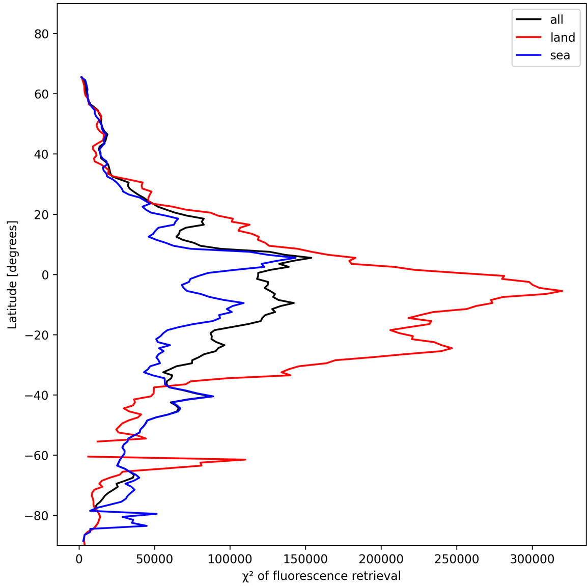
Figure 25: Zonal average of “ \chi^2 of fluorescence retrieval” for 2024-12-08 to 2024-12-10.
