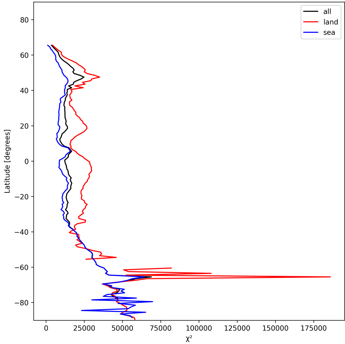
Figure 21: Zonal average of “ \chi^2 ” for 2024-12-08 to 2024-12-10.
