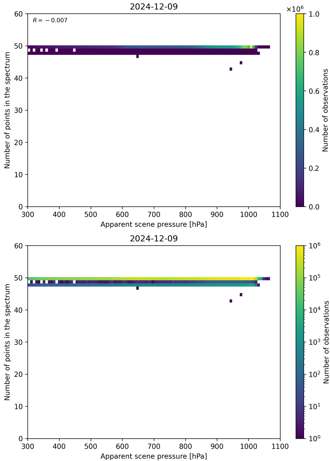
Figure 66: Scatter density plot of “Apparent scene pressure” against “Number of points in the spectrum” for 2024-12-08 to 2024-12-10.
