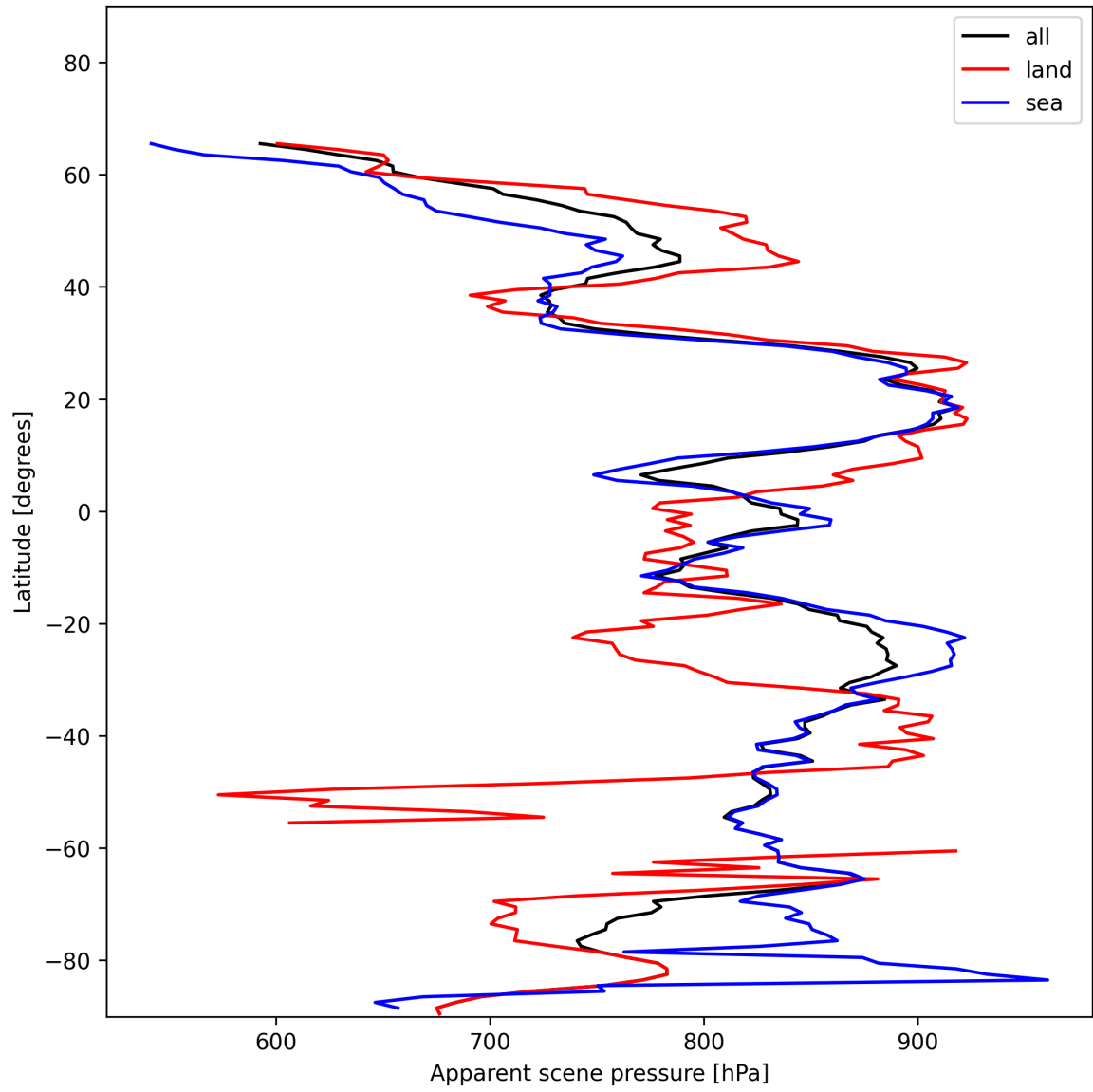
Figure 19: Zonal average of “Apparent scene pressure” for 2024-12-08 to 2024-12-10.
