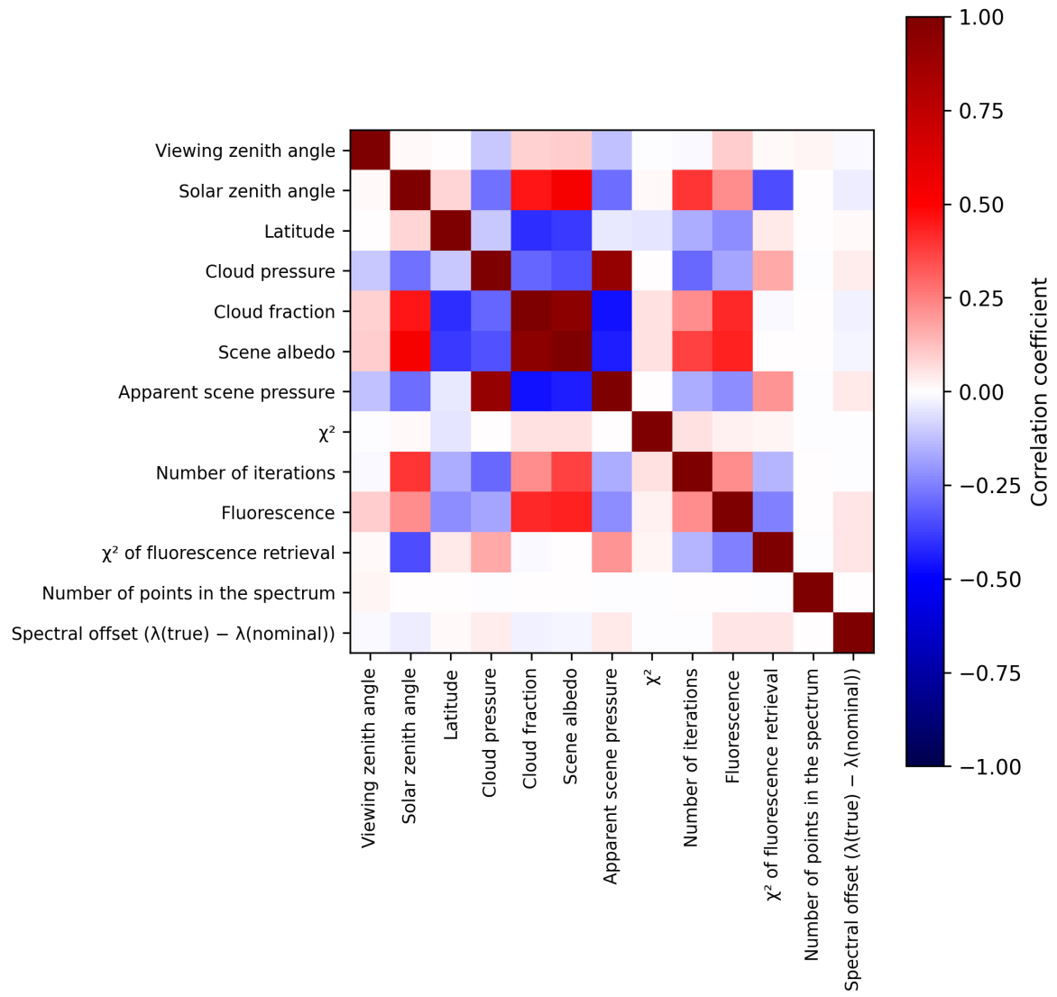
Figure 2: Map of correlation matrix for 2024-12-08 to 2024-12-10.
