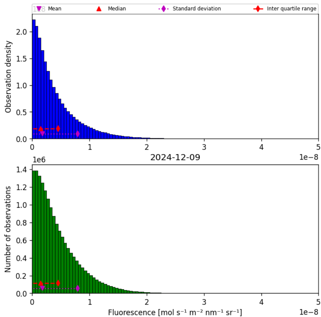
Figure 40: Histogram of “Fluorescence” for 2024-12-08 to 2024-12-10
