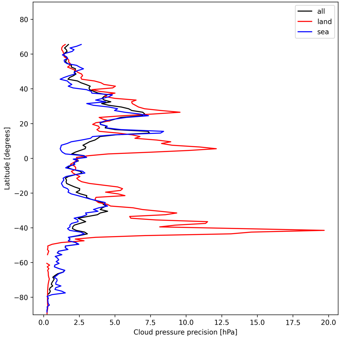
Figure 14: Zonal average of “Cloud pressure precision” for 2024-12-08 to 2024-12-10.
