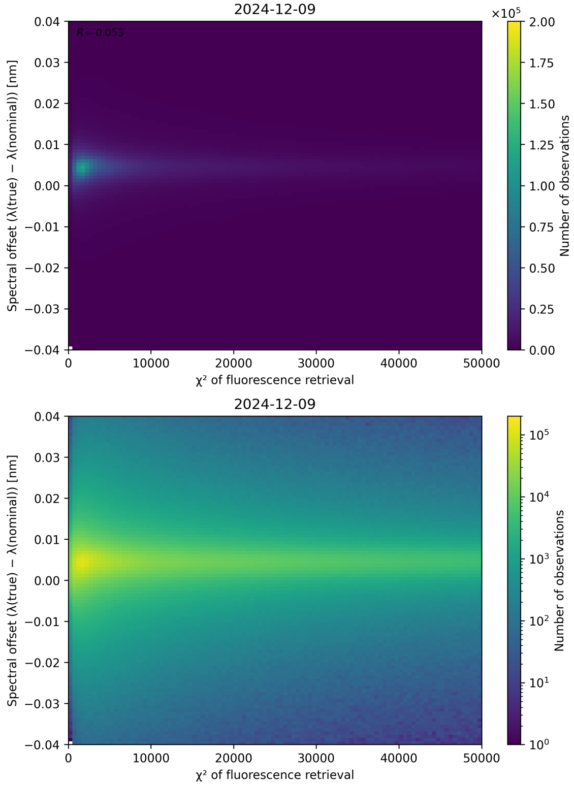
Figure 69: Scatter density plot of “ \chi^2 of fluorescence retrieval” against “Spectral offset ( \lambda_{\text{true}} - \lambda_{\text{nominal}} )” for 2024-12-08 to 2024-12-10.
