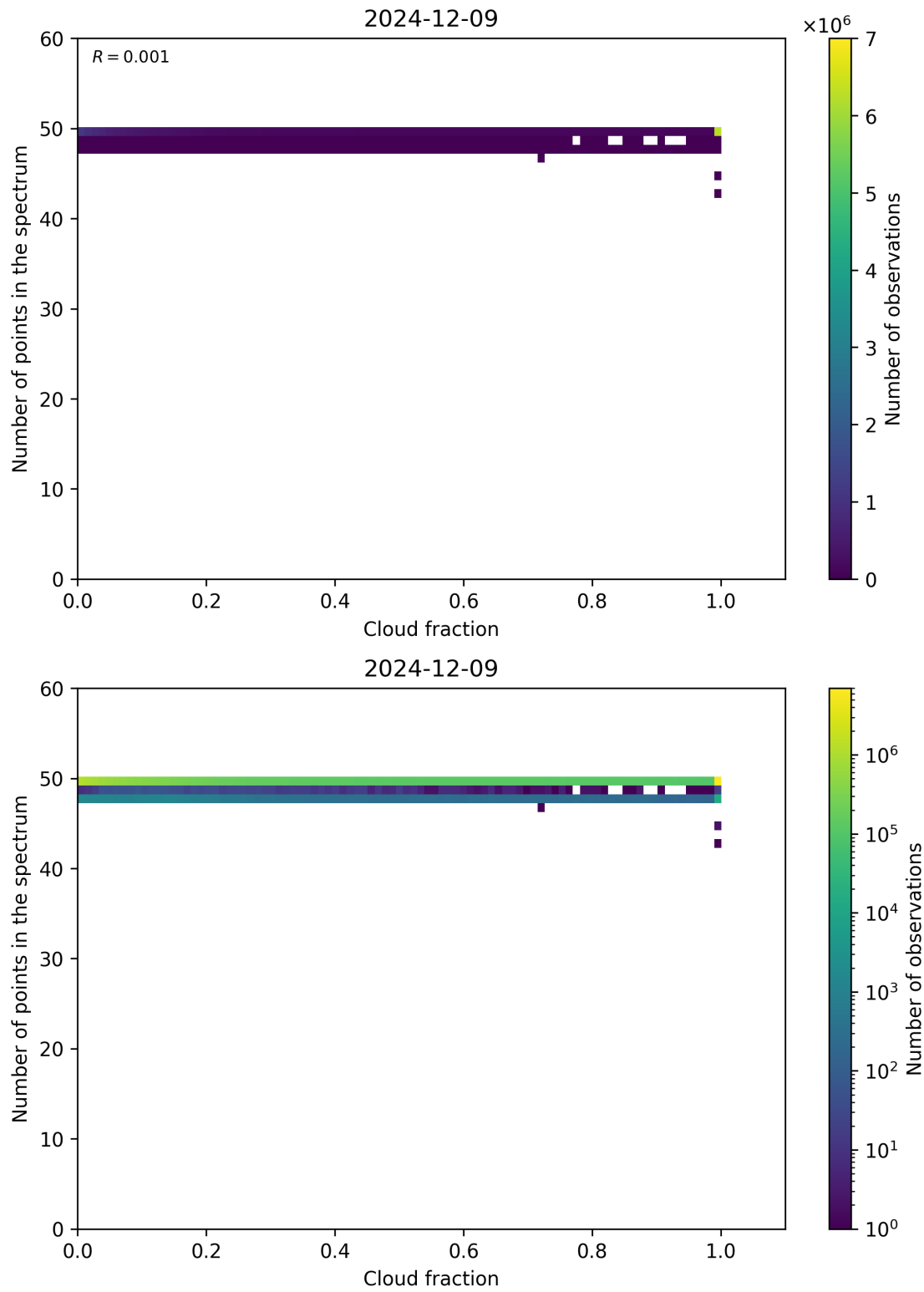
Figure 74: Scatter density plot of “Cloud fraction” against “Number of points in the spectrum” for 2024-12-08 to 2024-12-10.
