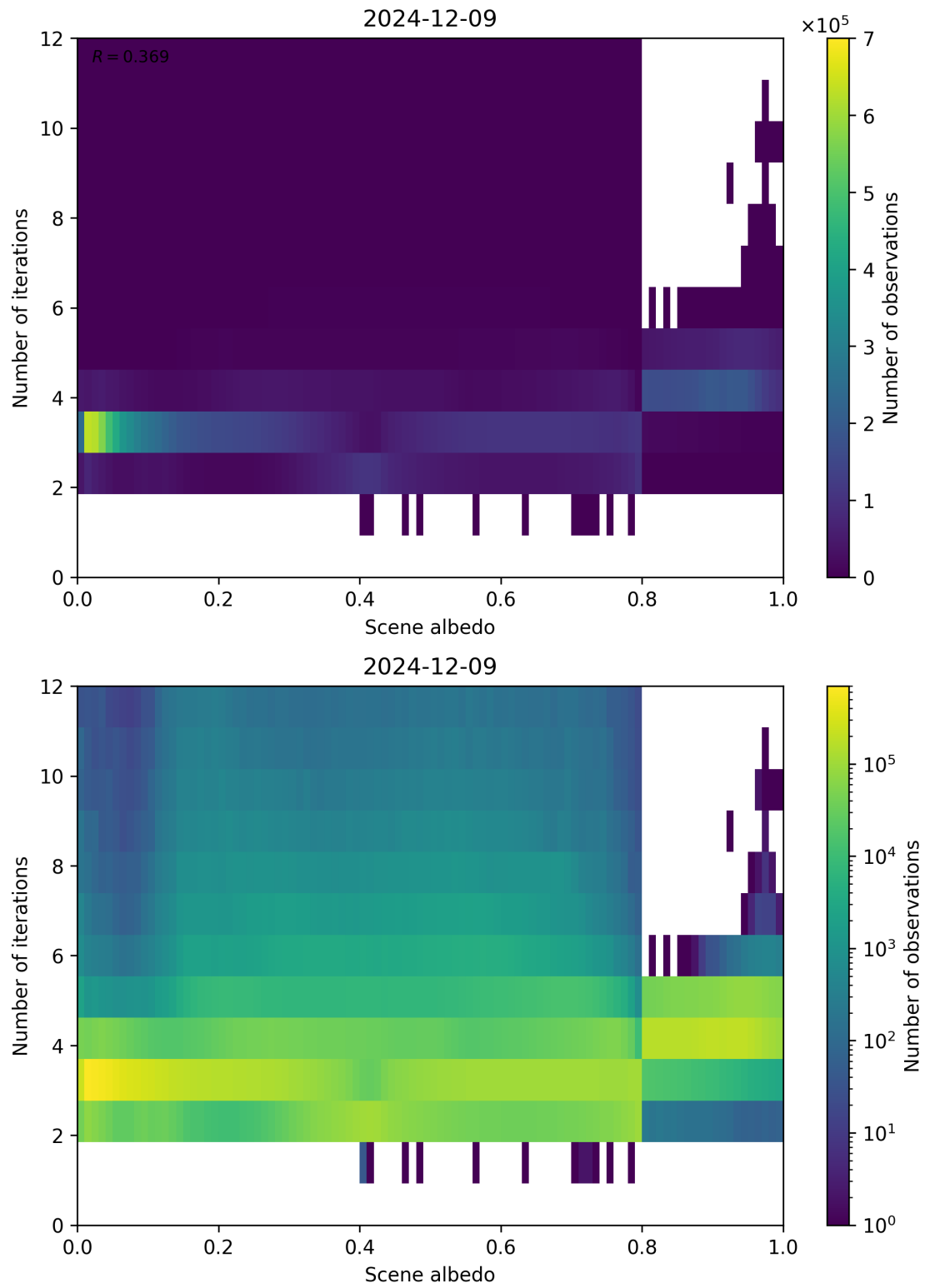
Figure 105: Scatter density plot of “Scene albedo” against “Number of iterations” for 2024-12-08 to 2024-12-10.
