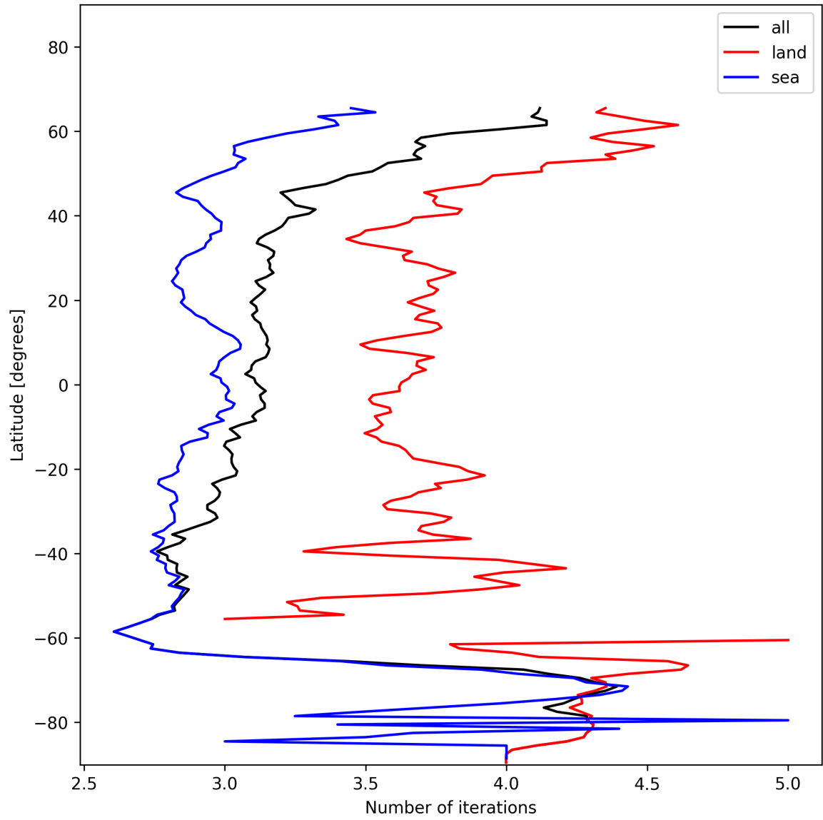
Figure 22: Zonal average of “Number of iterations” for 2024-12-08 to 2024-12-10.
