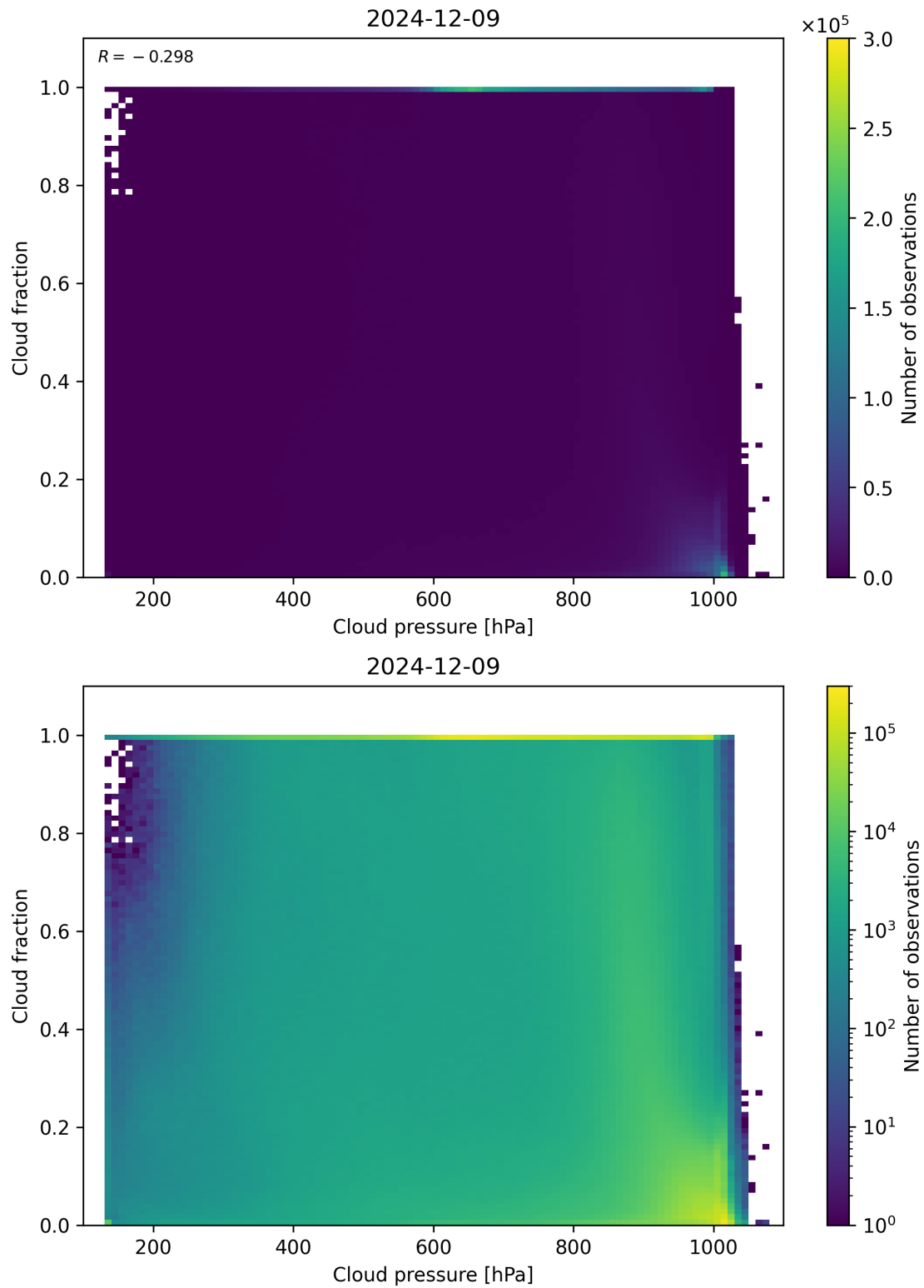
Figure 79: Scatter density plot of “Cloud pressure” against “Cloud fraction” for 2024-12-08 to 2024-12-10.
