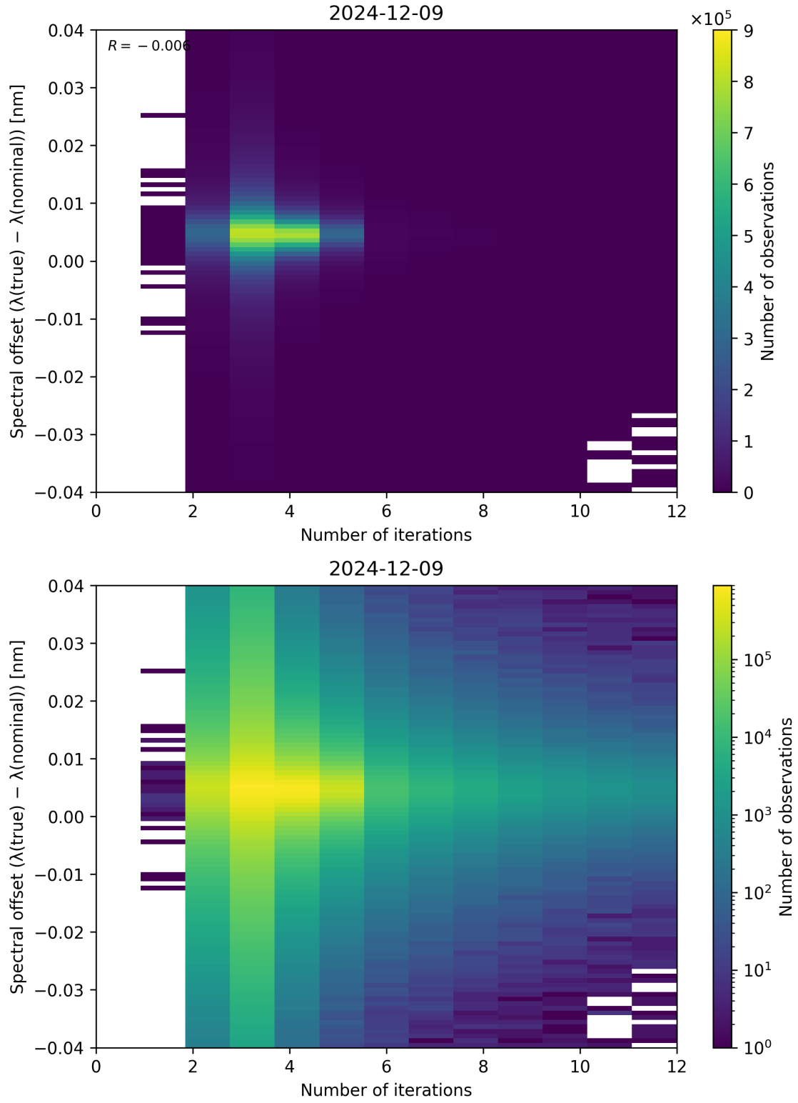
Figure 100: Scatter density plot of “Number of iterations” against “Spectral offset ( \lambda_{\text{true}} - \lambda_{\text{nominal}} )” for 2024-12-08 to 2024-12-10.
