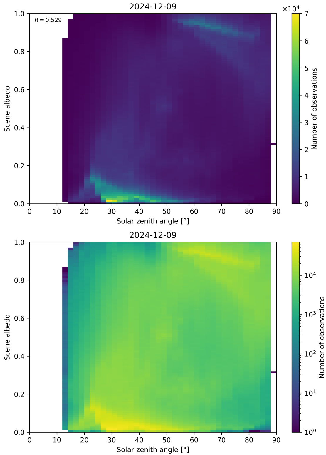
Figure 116: Scatter density plot of “Solar zenith angle” against “Scene albedo” for 2024-12-08 to 2024-12-10.
