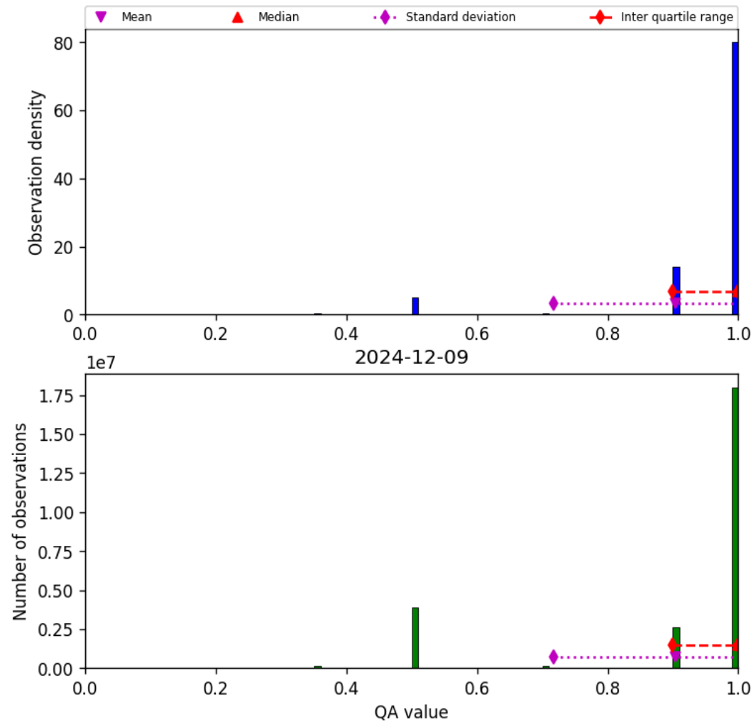
Figure 29: Histogram of “QA value” for 2024-12-08 to 2024-12-10
