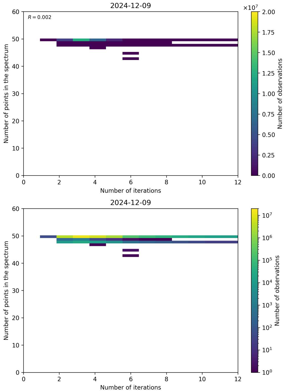
Figure 99: Scatter density plot of “Number of iterations” against “Number of points in the spectrum” for 2024-12-08 to 2024-12-10.
