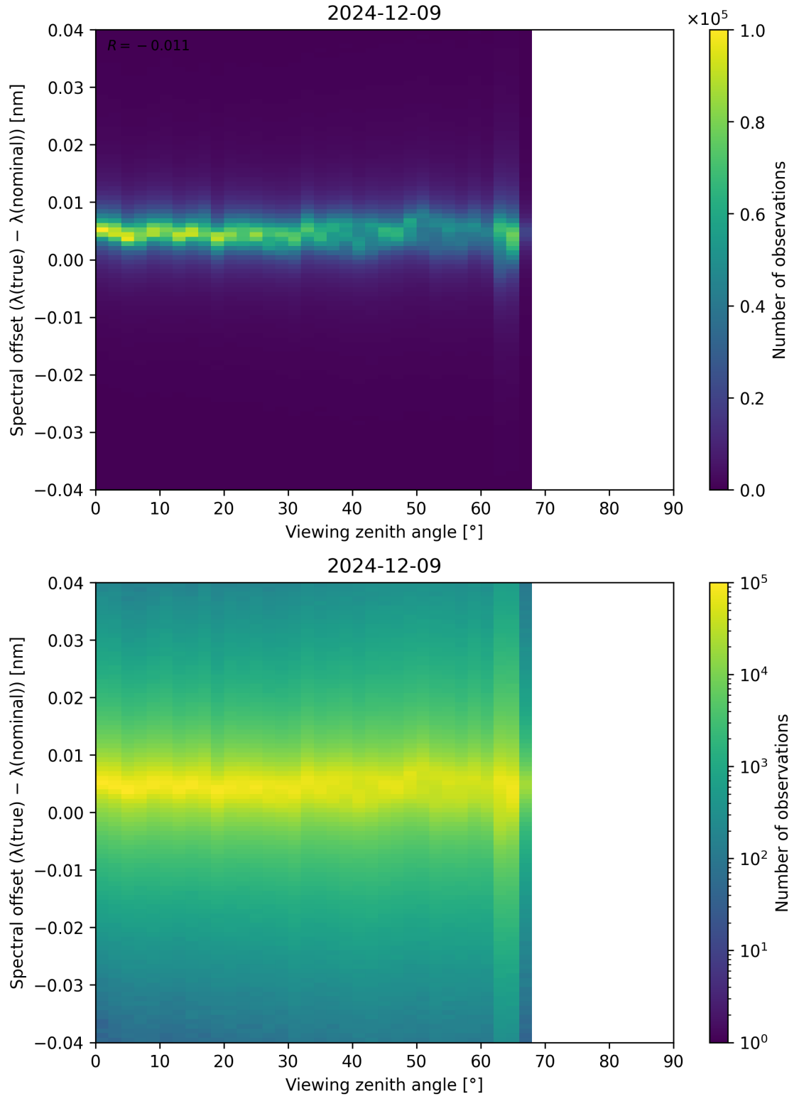
Figure 128: Scatter density plot of “Viewing zenith angle” against “Spectral offset ( \lambda_{\text{true}} - \lambda_{\text{nominal}} )” for 2024-12-08 to 2024-12-10.
