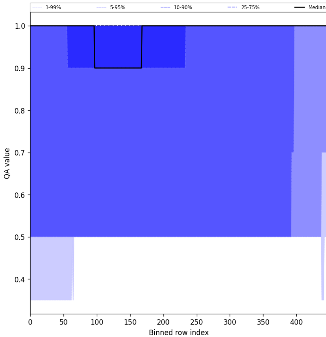
Figure 46: Along track statistics of “QA value” for 2024-12-08 to 2024-12-10
