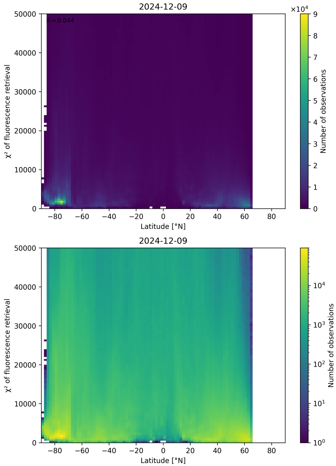
Figure 89: Scatter density plot of “Latitude” against “ \chi^2 of fluorescence retrieval” for 2024-12-08 to 2024-12-10.
