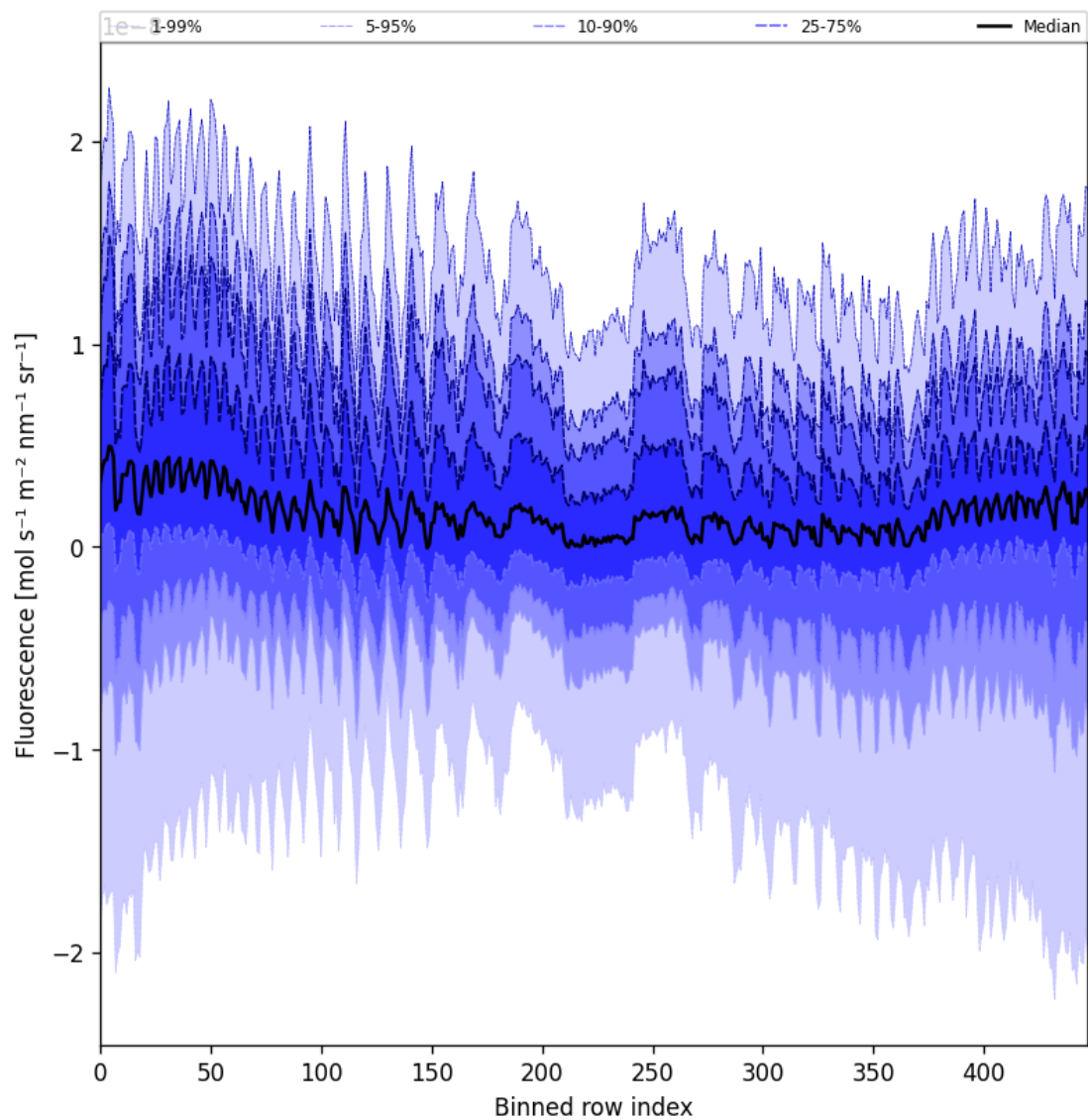
Figure 57: Along track statistics of “Fluorescence” for 2024-12-08 to 2024-12-10
