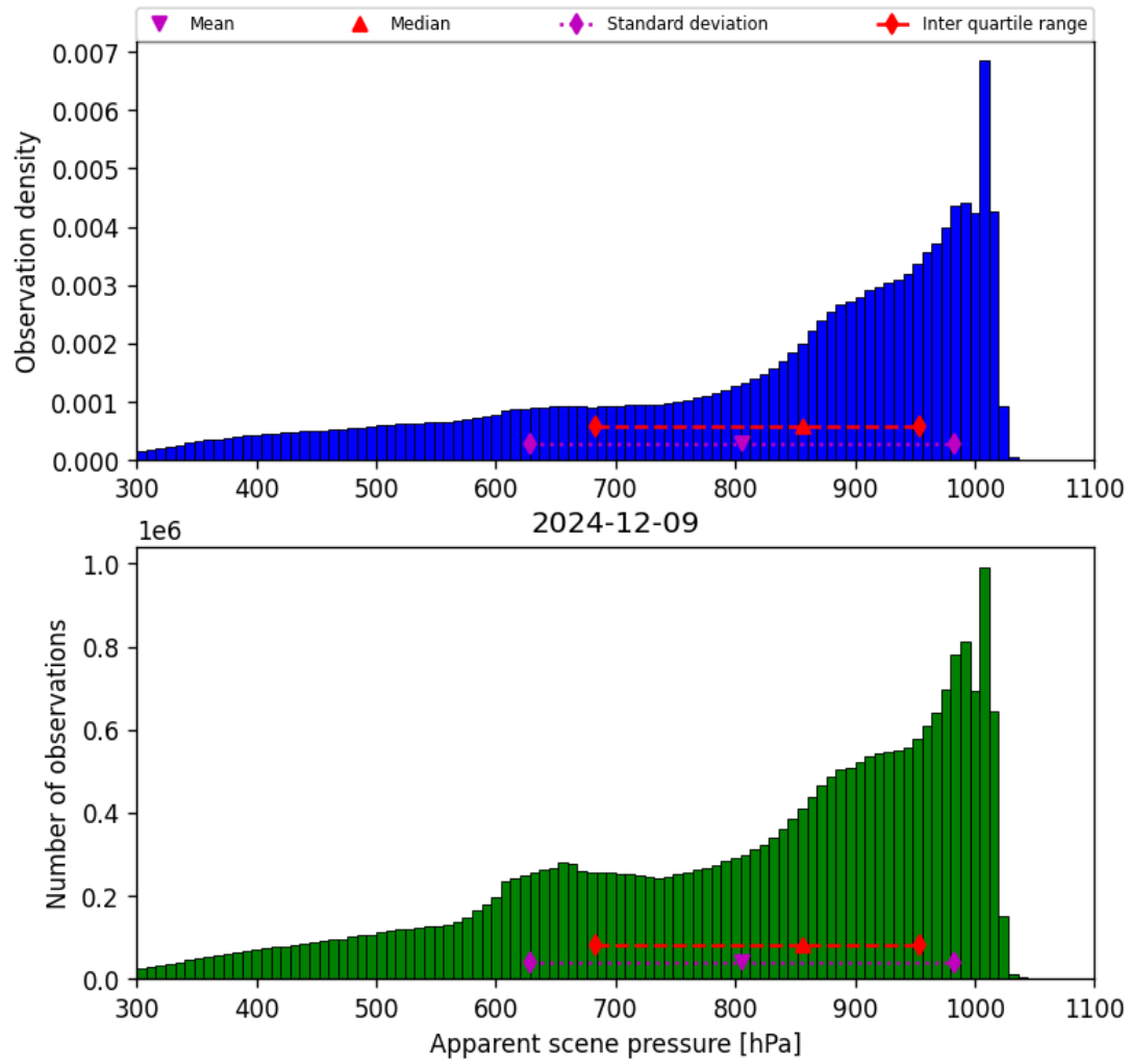
Figure 36: Histogram of “Apparent scene pressure” for 2024-12-08 to 2024-12-10
