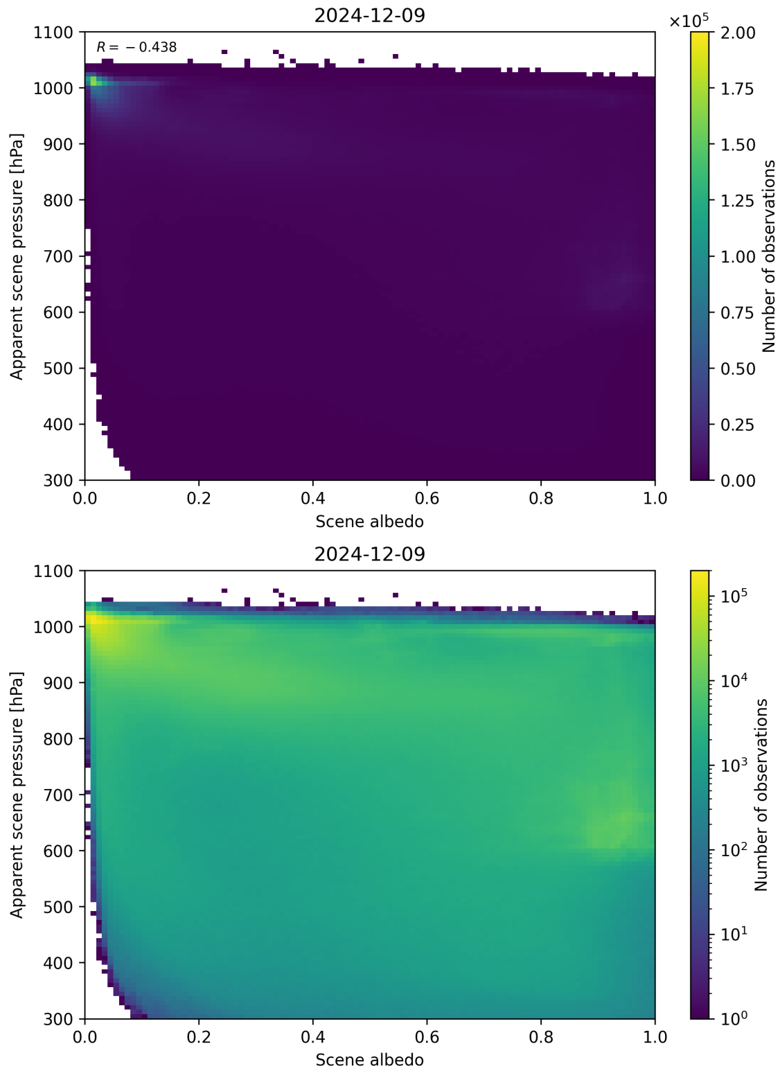
Figure 102: Scatter density plot of “Scene albedo” against “Apparent scene pressure” for 2024-12-08 to 2024-12-10.
