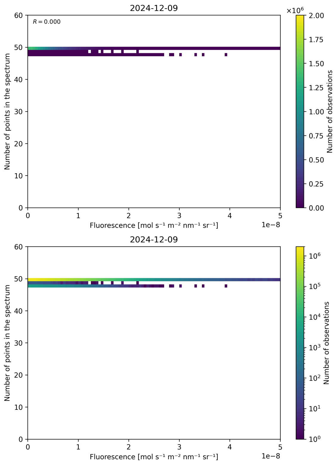
Figure 86: Scatter density plot of “Fluorescence” against “Number of points in the spectrum” for 2024-12-08 to 2024-12-10.
