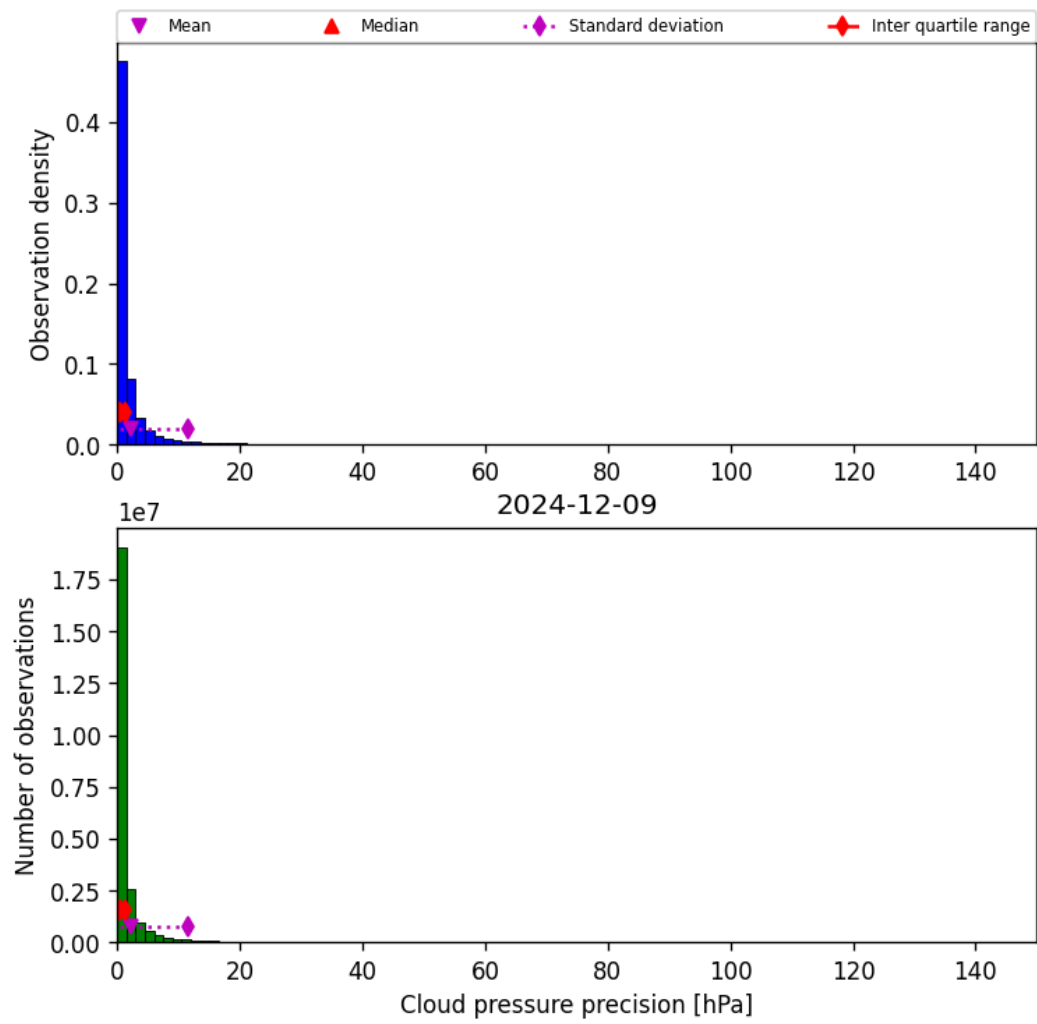
Figure 31: Histogram of “Cloud pressure precision” for 2024-12-08 to 2024-12-10
