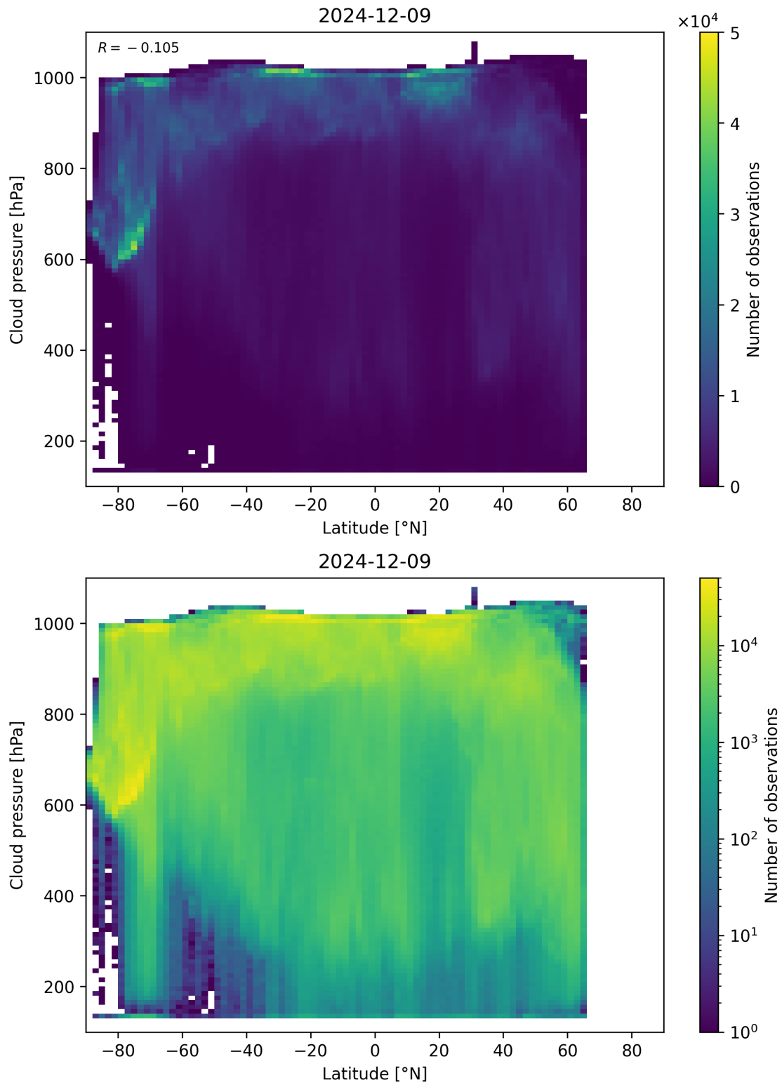
Figure 91: Scatter density plot of “Latitude” against “Cloud pressure” for 2024-12-08 to 2024-12-10.
