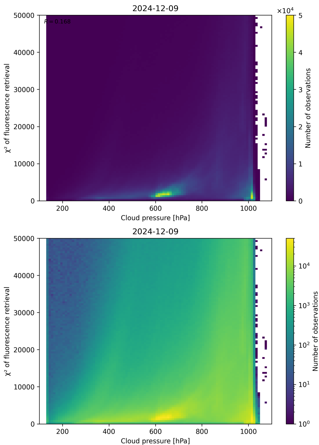
Figure 78: Scatter density plot of “Cloud pressure” against “ \chi^2 of fluorescence retrieval” for 2024-12-08 to 2024-12-10.
