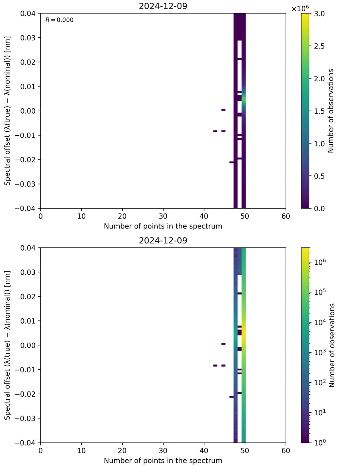
Figure 101: Scatter density plot of “Number of points in the spectrum” against “Spectral offset ( \lambda_{\text{true}} - \lambda_{\text{nominal}} )” for 2024-12-08 to 2024-12-10.
