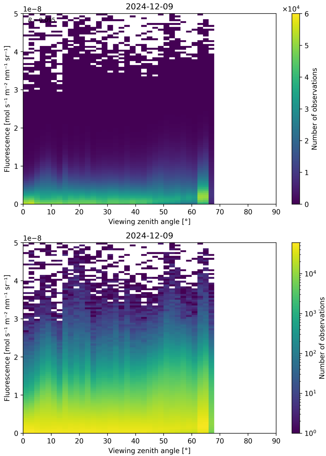
Figure 122: Scatter density plot of “Viewing zenith angle” against “Fluorescence” for 2024-12-08 to 2024-12-10.
