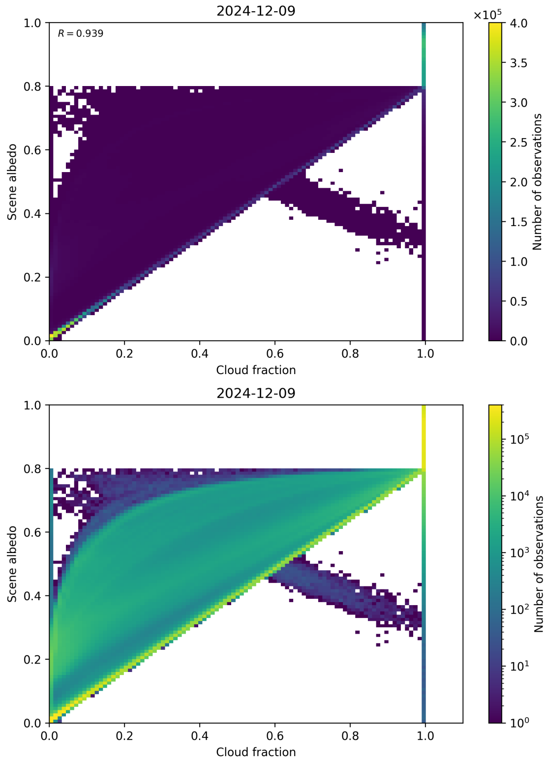
Figure 75: Scatter density plot of “Cloud fraction” against “Scene albedo” for 2024-12-08 to 2024-12-10.
