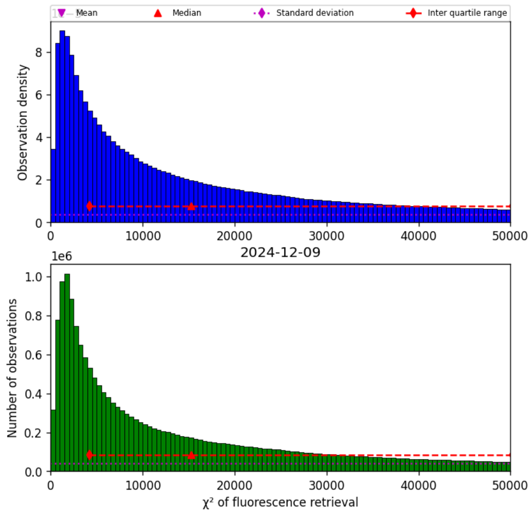
Figure 42: Histogram of “ \chi^2 of fluorescence retrieval” for 2024-12-08 to 2024-12-10
