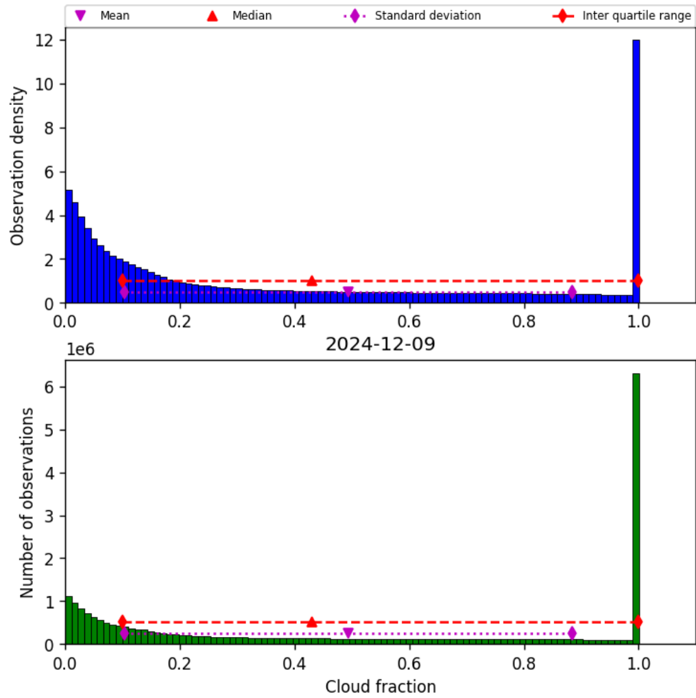
Figure 32: Histogram of “Cloud fraction” for 2024-12-08 to 2024-12-10
