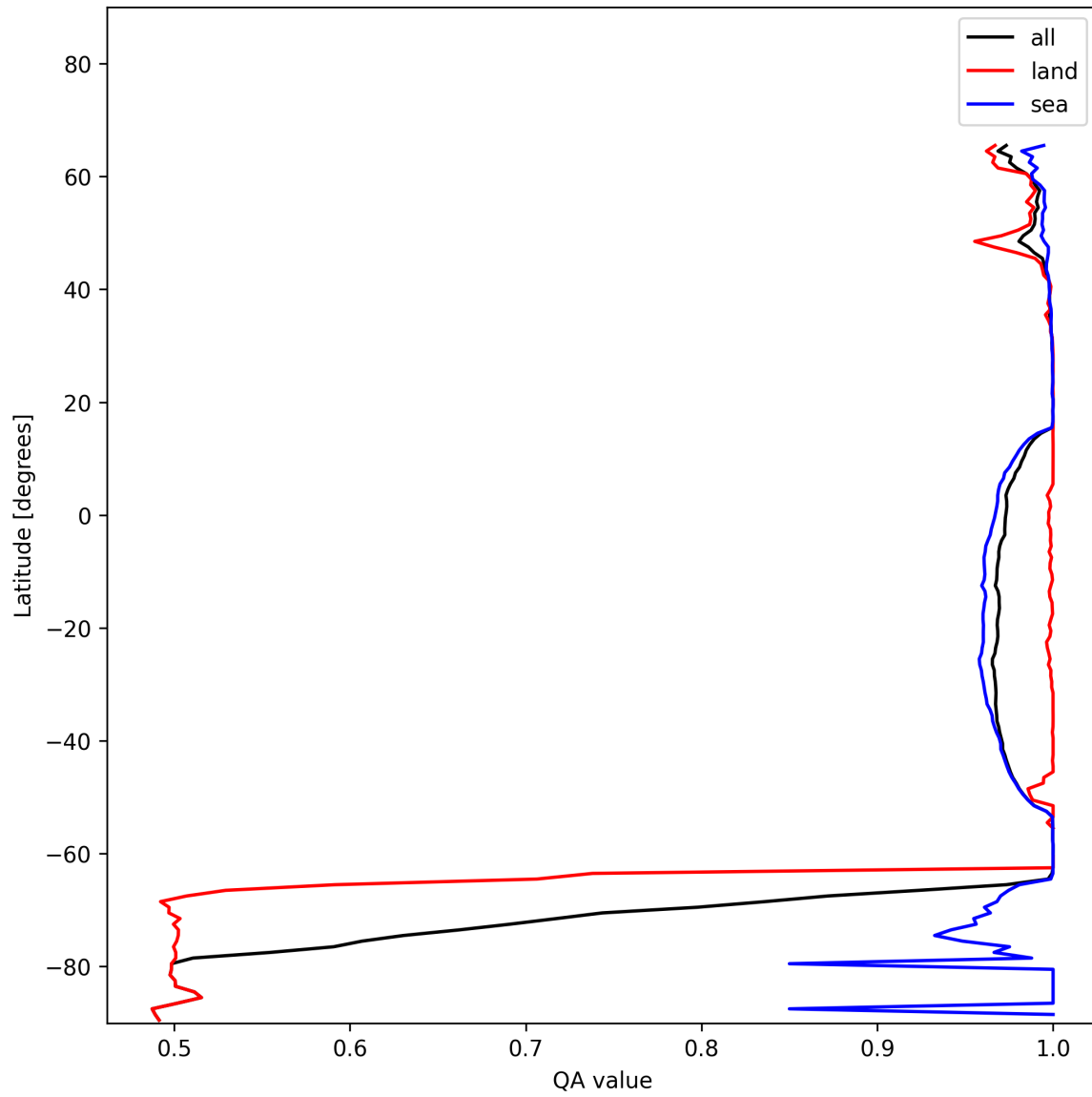
Figure 12: Zonal average of “QA value” for 2024-12-08 to 2024-12-10.
