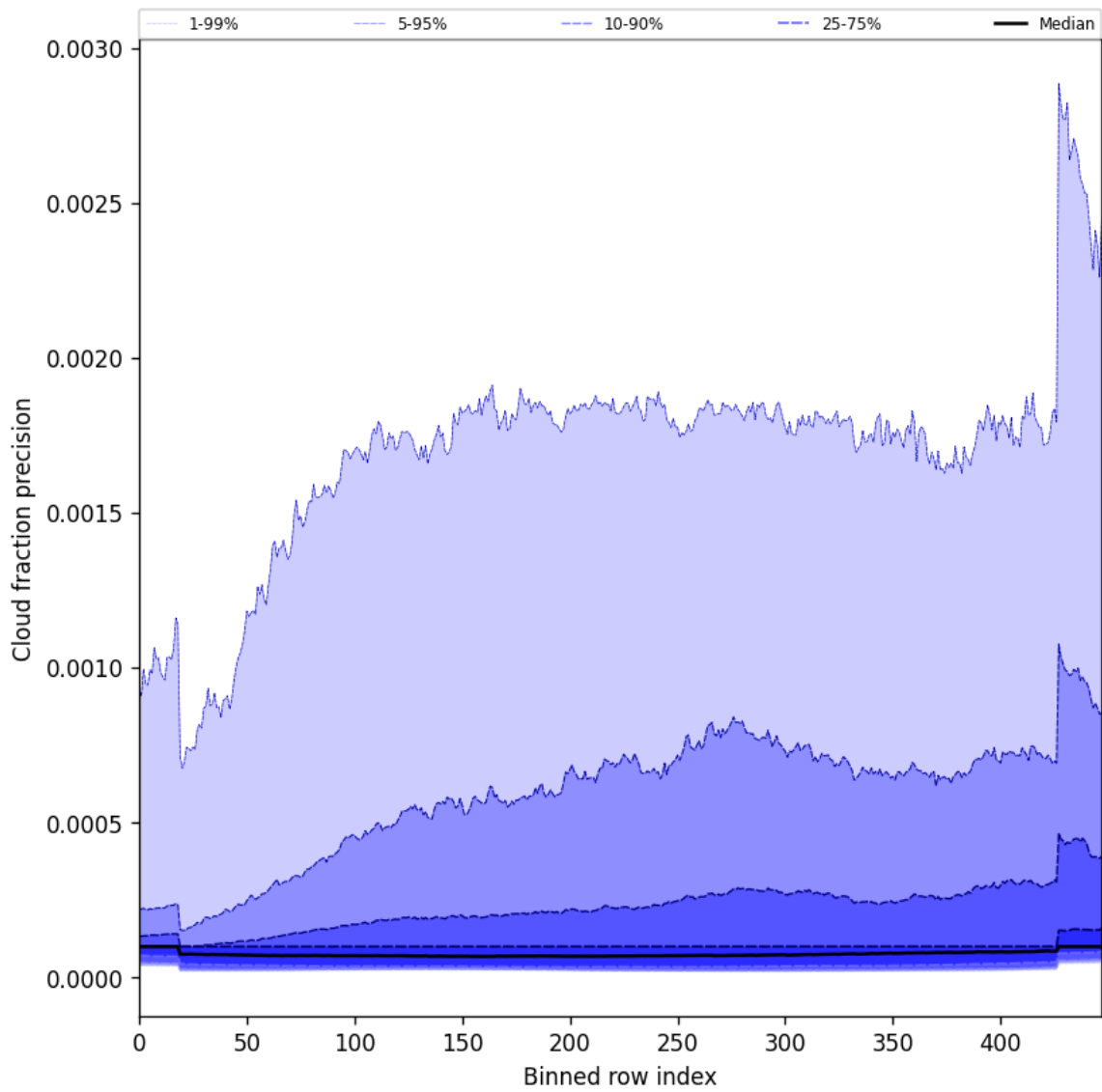
Figure 50: Along track statistics of “Cloud fraction precision” for 2024-12-08 to 2024-12-10
