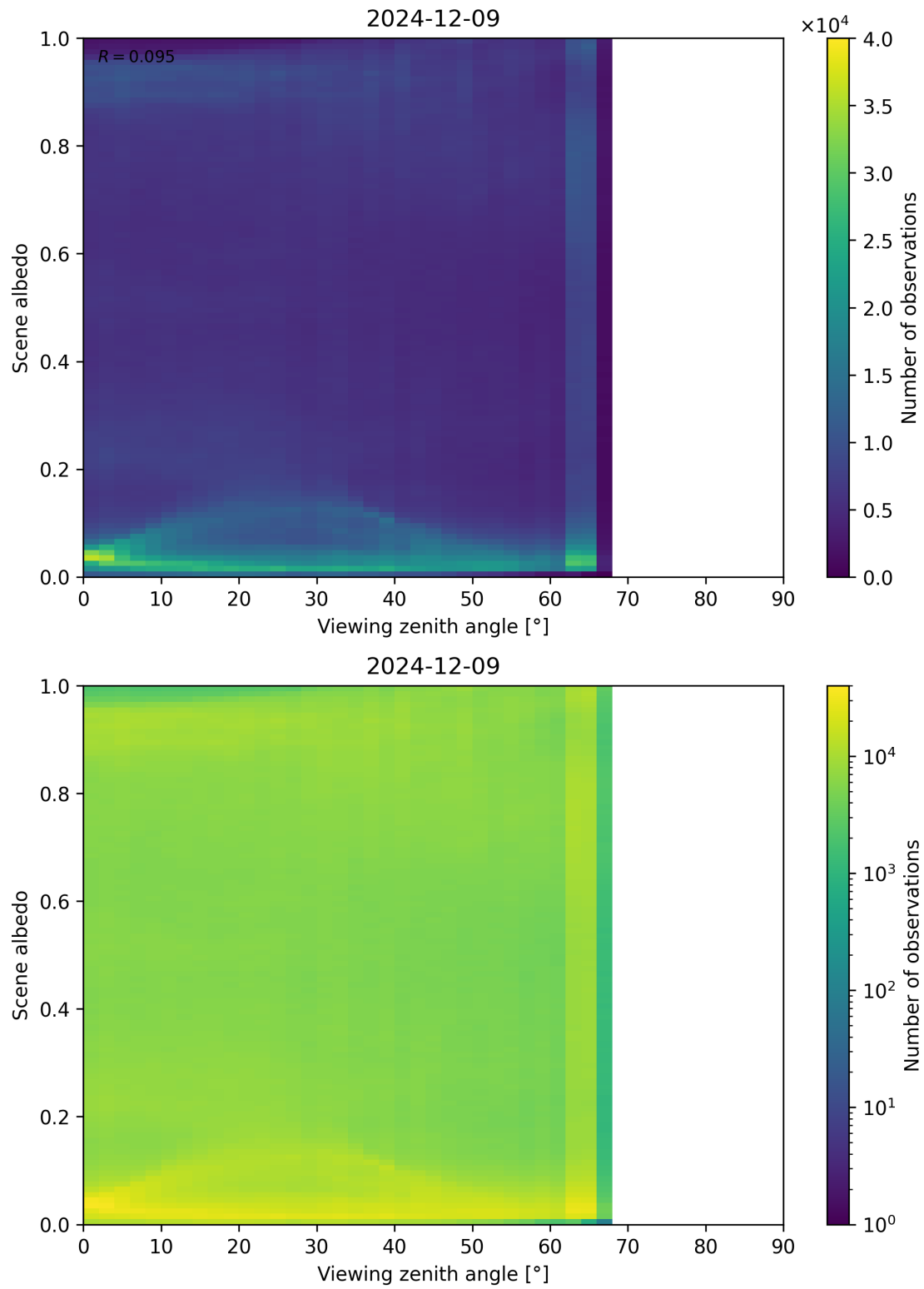
Figure 126: Scatter density plot of “Viewing zenith angle” against “Scene albedo” for 2024-12-08 to 2024-12-10.
