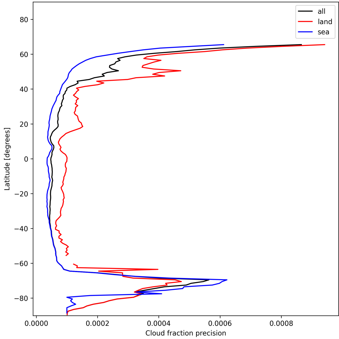
Figure 16: Zonal average of “Cloud fraction precision” for 2024-12-08 to 2024-12-10.
