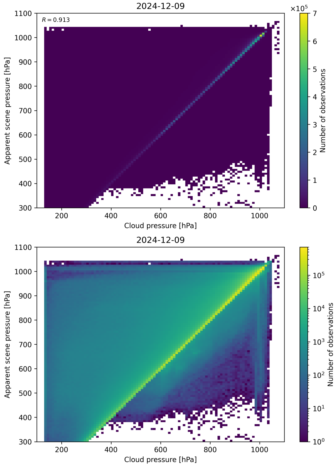
Figure 77: Scatter density plot of “Cloud pressure” against “Apparent scene pressure” for 2024-12-08 to 2024-12-10.
