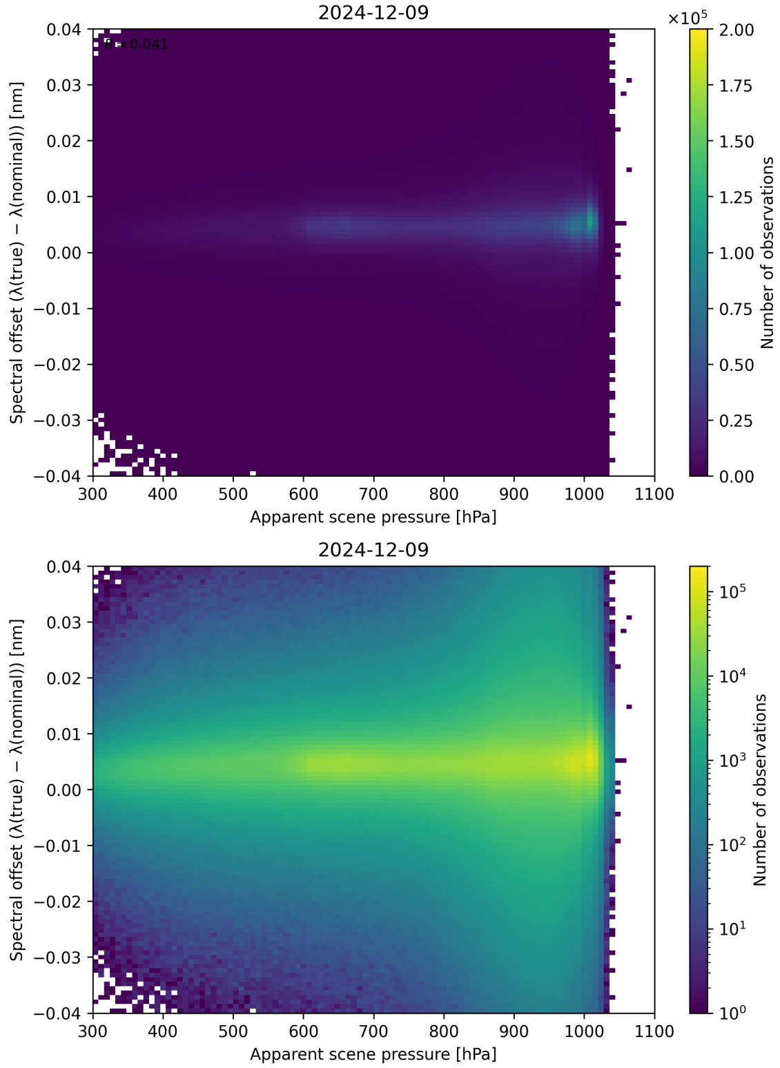
Figure 67: Scatter density plot of “Apparent scene pressure” against “Spectral offset ( \lambda_{\text{true}} - \lambda_{\text{nominal}} )” for 2024-12-08 to 2024-12-10.
