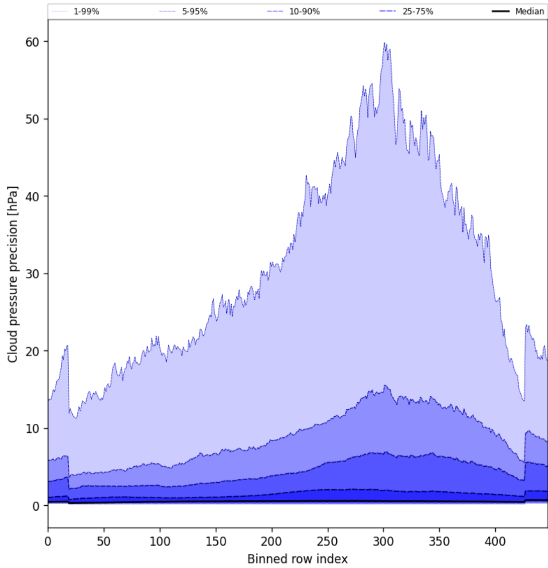
Figure 48: Along track statistics of “Cloud pressure precision” for 2024-12-08 to 2024-12-10
