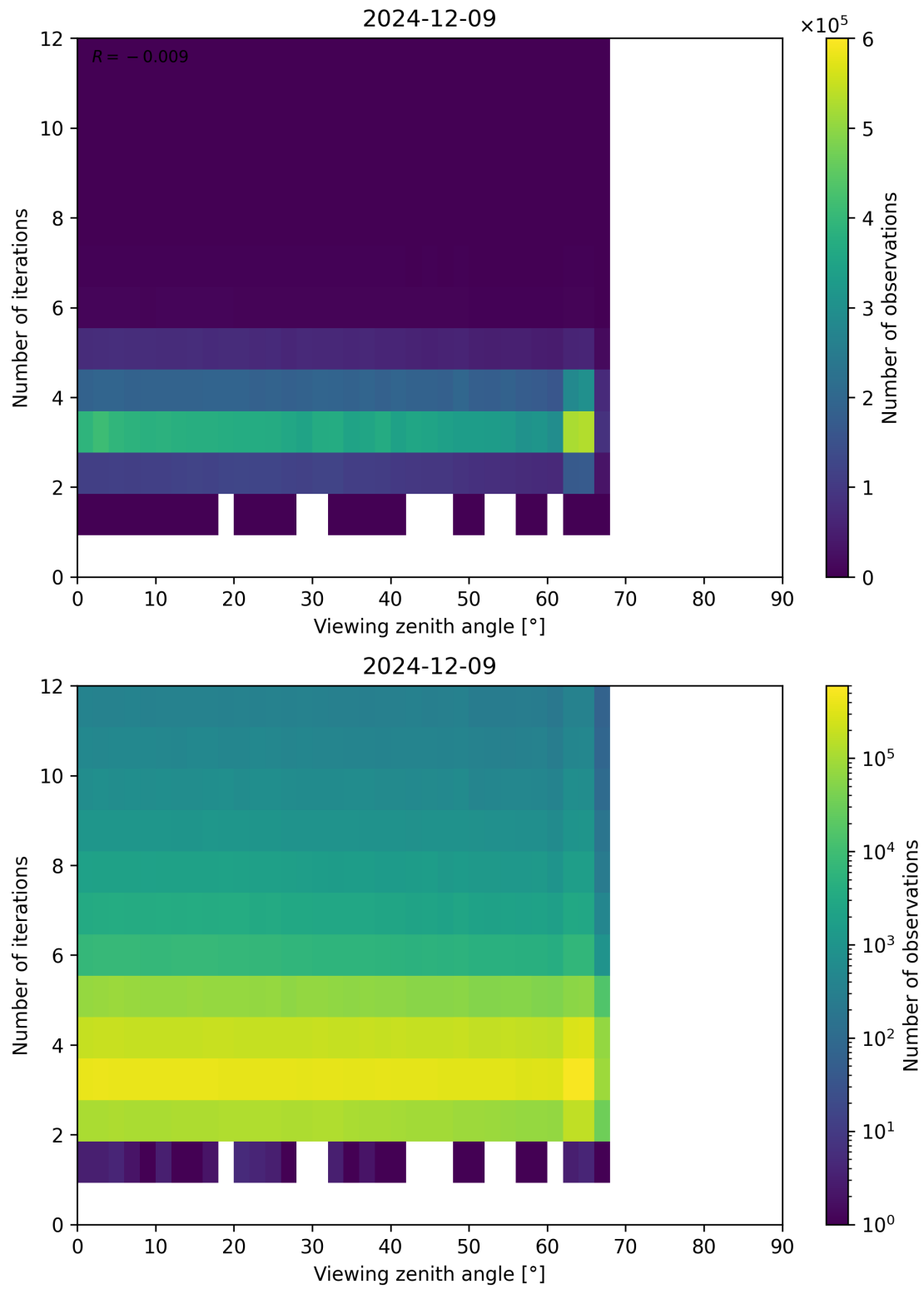
Figure 124: Scatter density plot of “Viewing zenith angle” against “Number of iterations” for 2024-12-08 to 2024-12-10.
