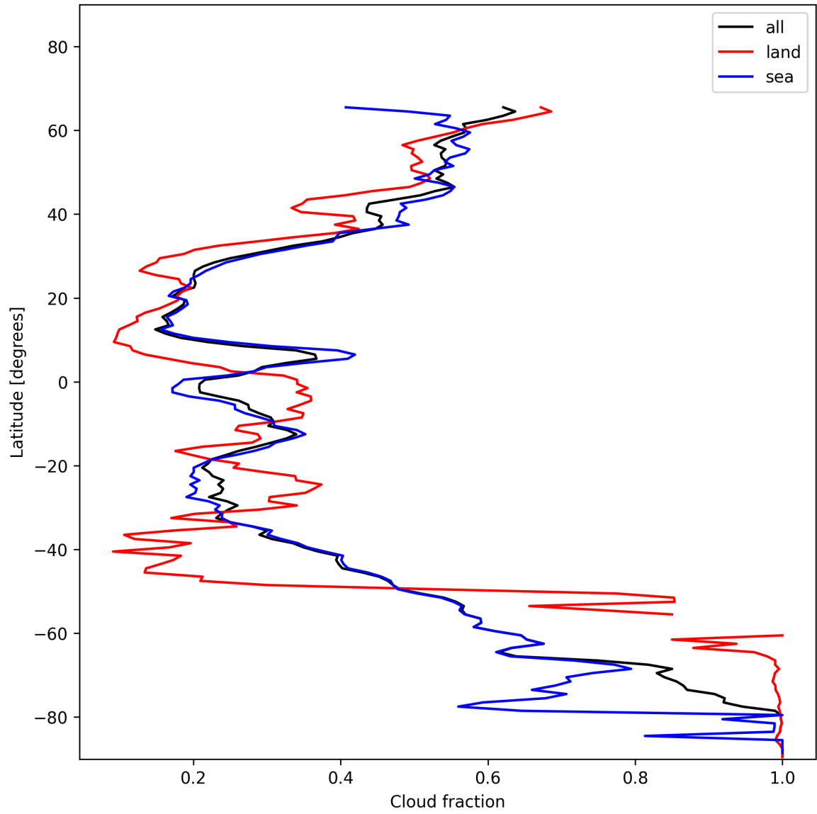
Figure 15: Zonal average of “Cloud fraction” for 2024-12-08 to 2024-12-10.
