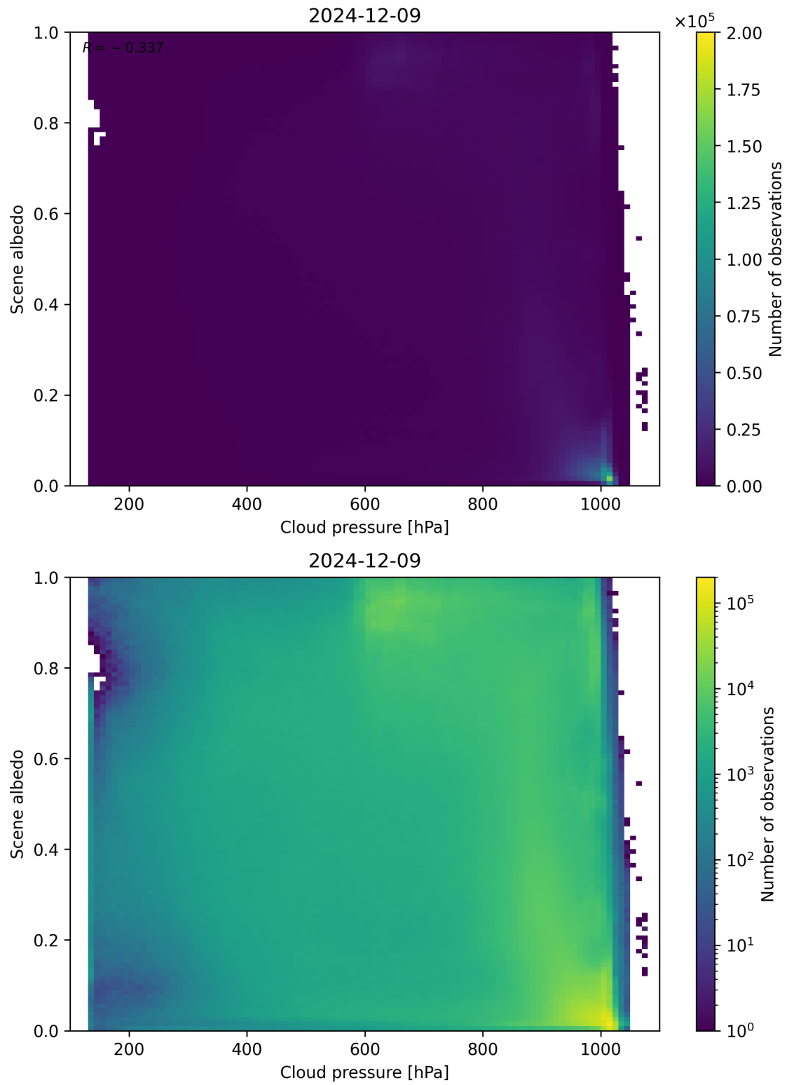
Figure 83: Scatter density plot of “Cloud pressure” against “Scene albedo” for 2024-12-08 to 2024-12-10.
