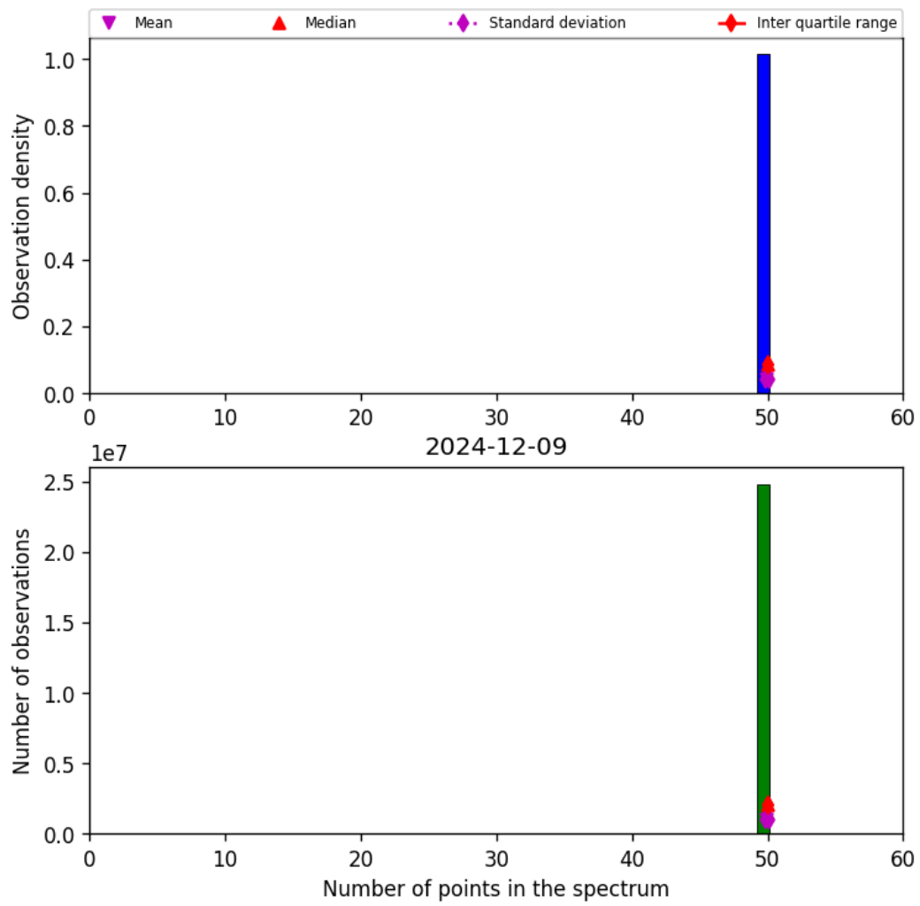
Figure 44: Histogram of “Number of points in the spectrum” for 2024-12-08 to 2024-12-10
