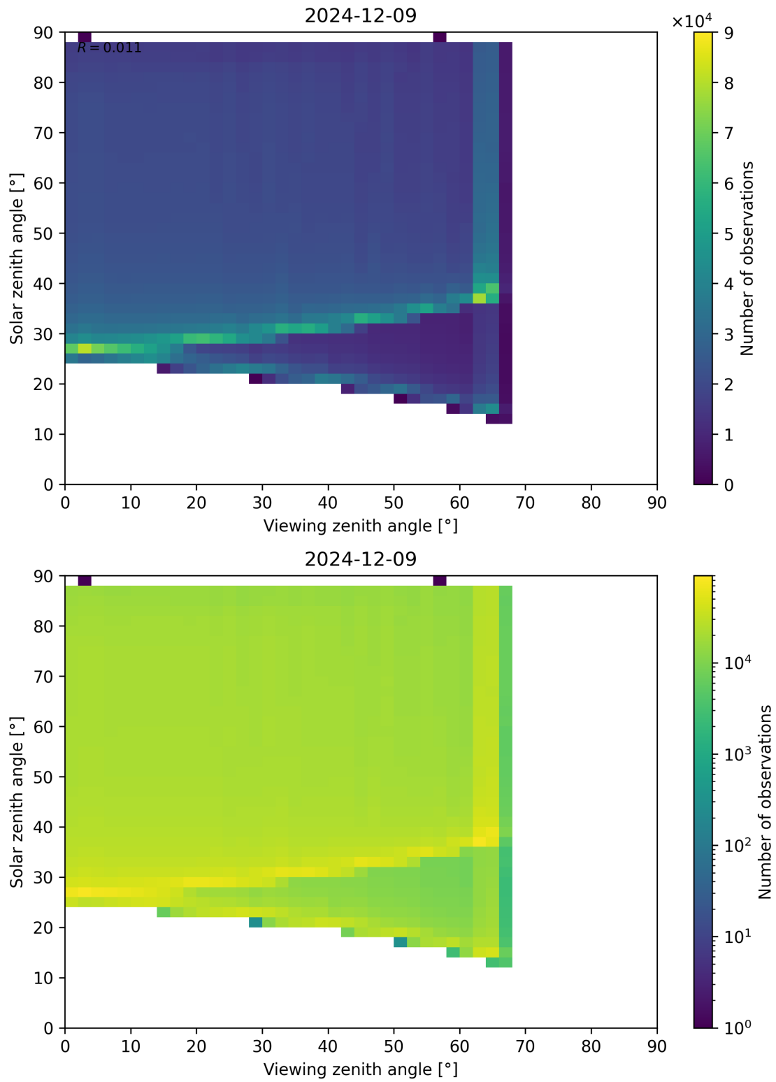
Figure 127: Scatter density plot of “Viewing zenith angle” against “Solar zenith angle” for 2024-12-08 to 2024-12-10.
