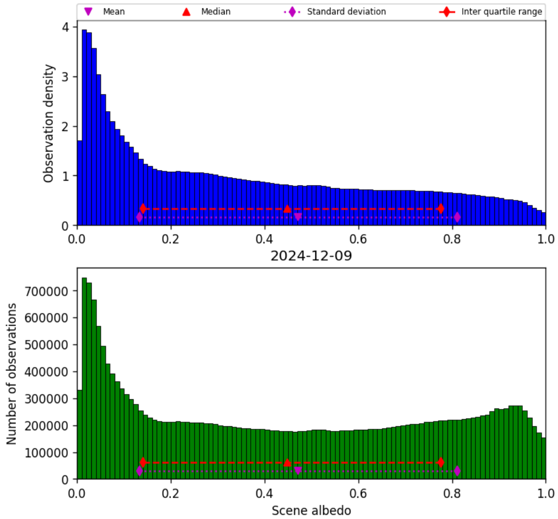
Figure 34: Histogram of “Scene albedo” for 2024-12-08 to 2024-12-10
