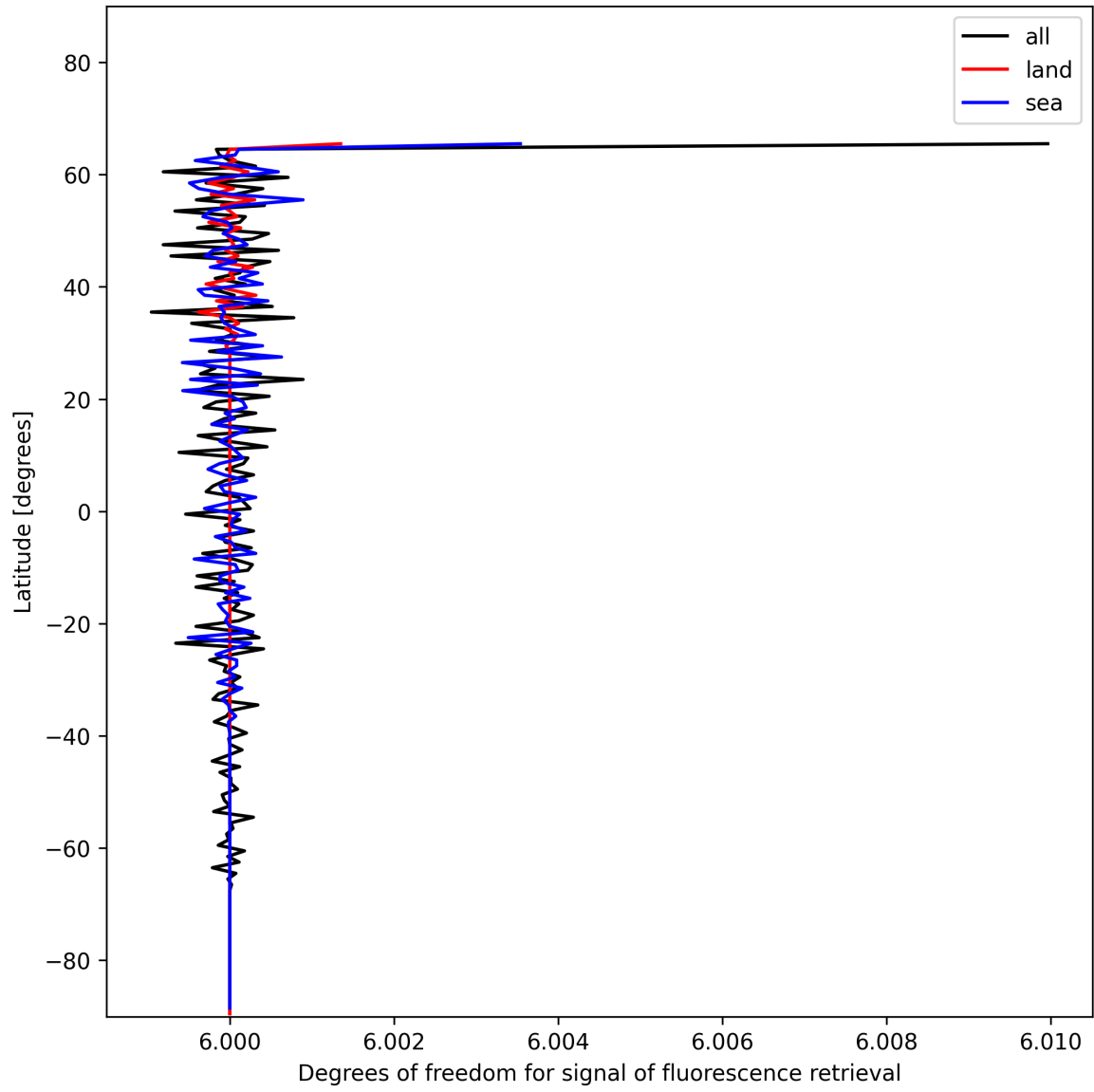
Figure 26: Zonal average of “Degrees of freedom for signal of fluorescence retrieval” for 2024-12-08 to 2024-12-10.
