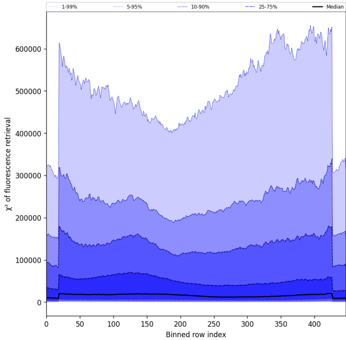
Figure 59: Along track statistics of “ \chi^2 of fluorescence retrieval” for 2024-12-08 to 2024-12-10
