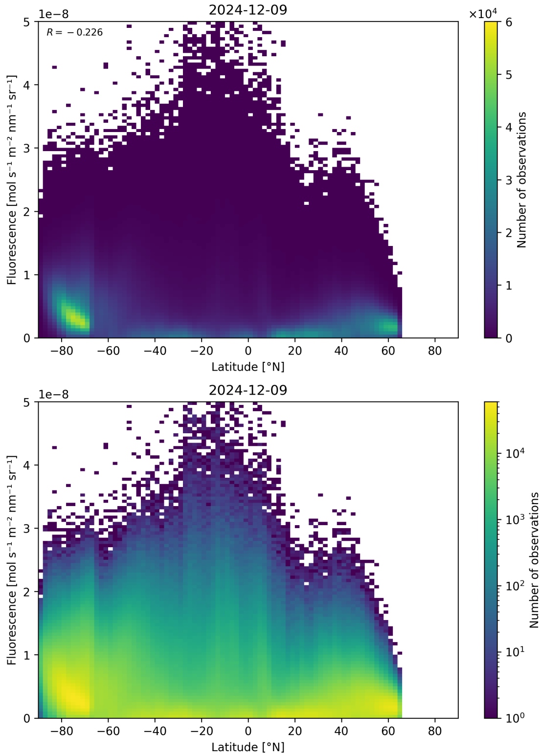
Figure 92: Scatter density plot of “Latitude” against “Fluorescence” for 2024-12-08 to 2024-12-10.
