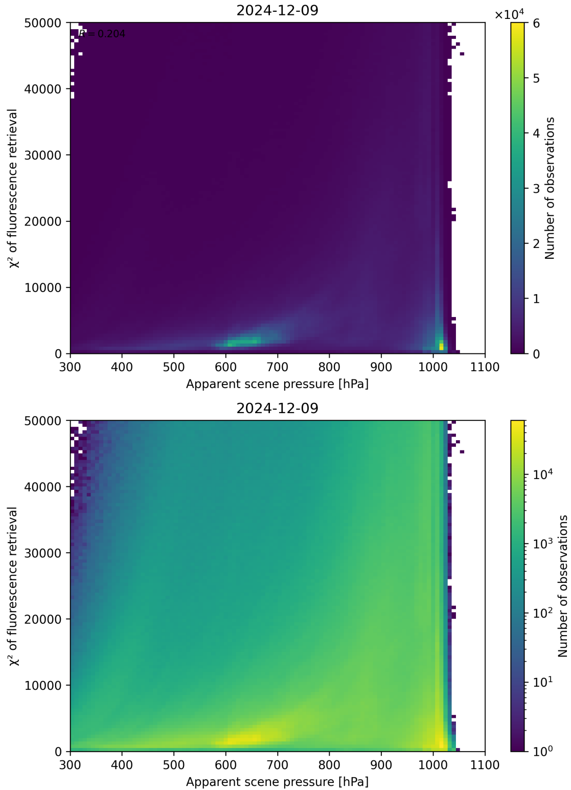
Figure 63: Scatter density plot of “Apparent scene pressure” against “ \chi^2 of fluorescence retrieval” for 2024-12-08 to 2024-12-10.
