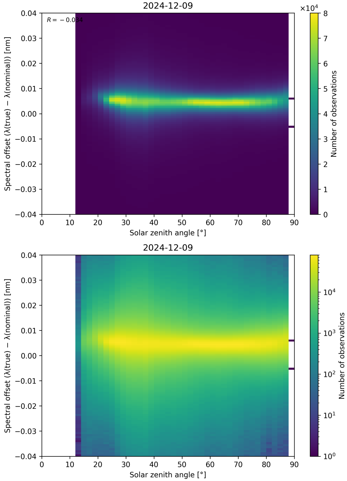
Figure 117: Scatter density plot of “Solar zenith angle” against “Spectral offset ( \lambda_{\text{true}} - \lambda_{\text{nominal}} )” for 2024-12-08 to 2024-12-10.
