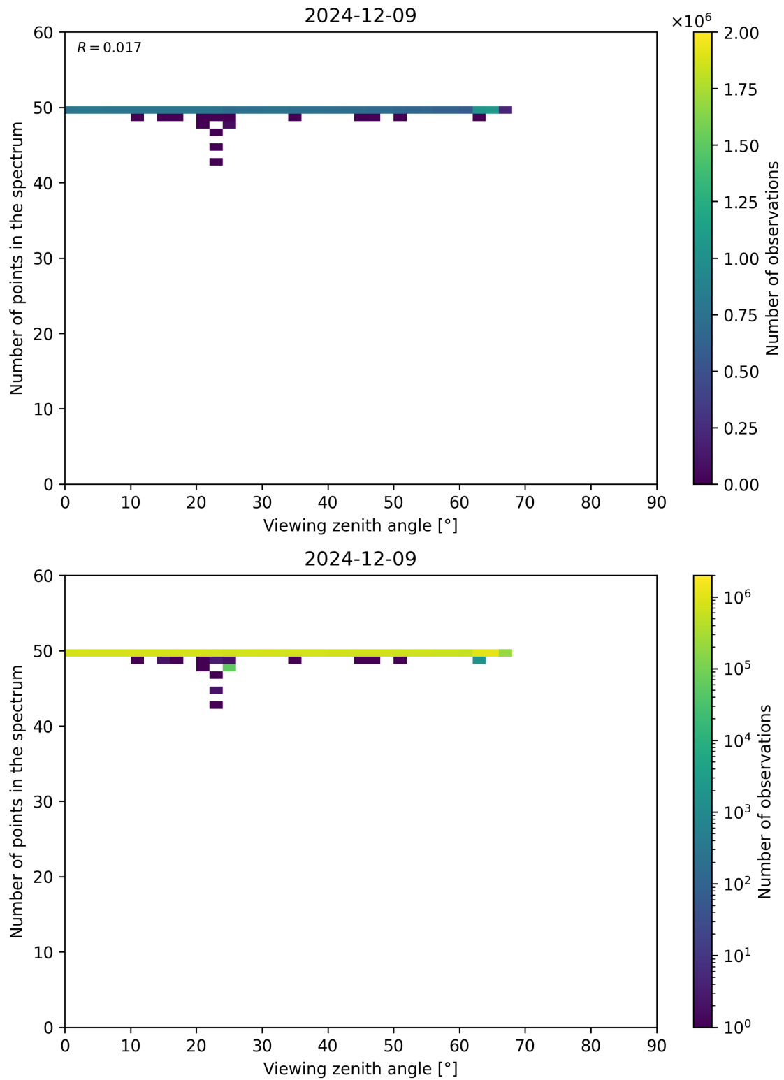
Figure 125: Scatter density plot of “Viewing zenith angle” against “Number of points in the spectrum” for 2024-12-08 to 2024-12-10.
