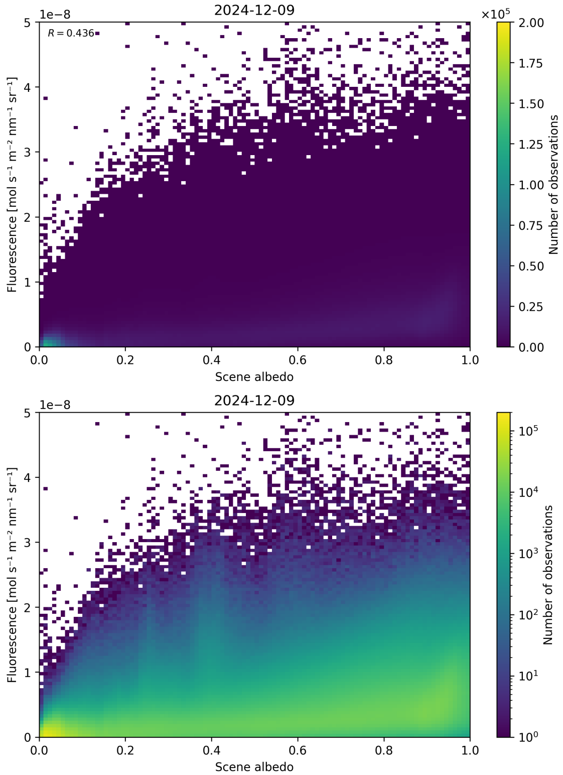
Figure 104: Scatter density plot of “Scene albedo” against “Fluorescence” for 2024-12-08 to 2024-12-10.
