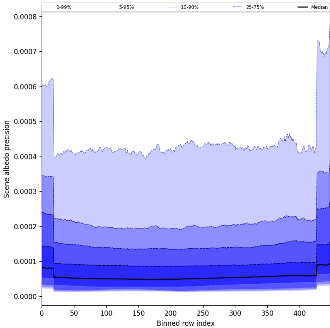
Figure 52: Along track statistics of “Scene albedo precision” for 2024-12-08 to 2024-12-10
