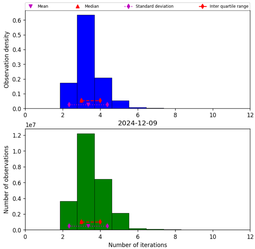
Figure 39: Histogram of “Number of iterations” for 2024-12-08 to 2024-12-10
