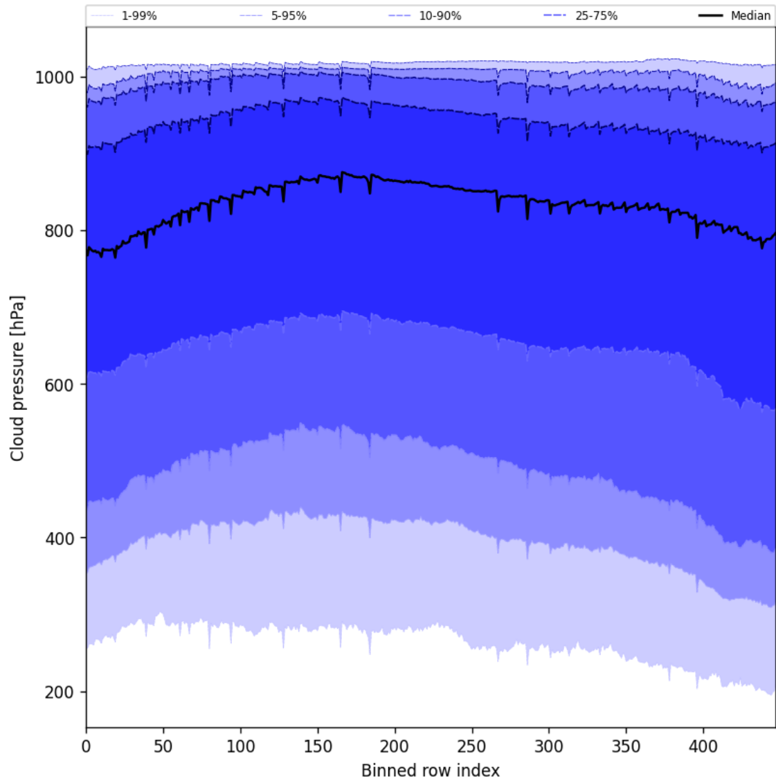
Figure 47: Along track statistics of “Cloud pressure” for 2024-12-08 to 2024-12-10
