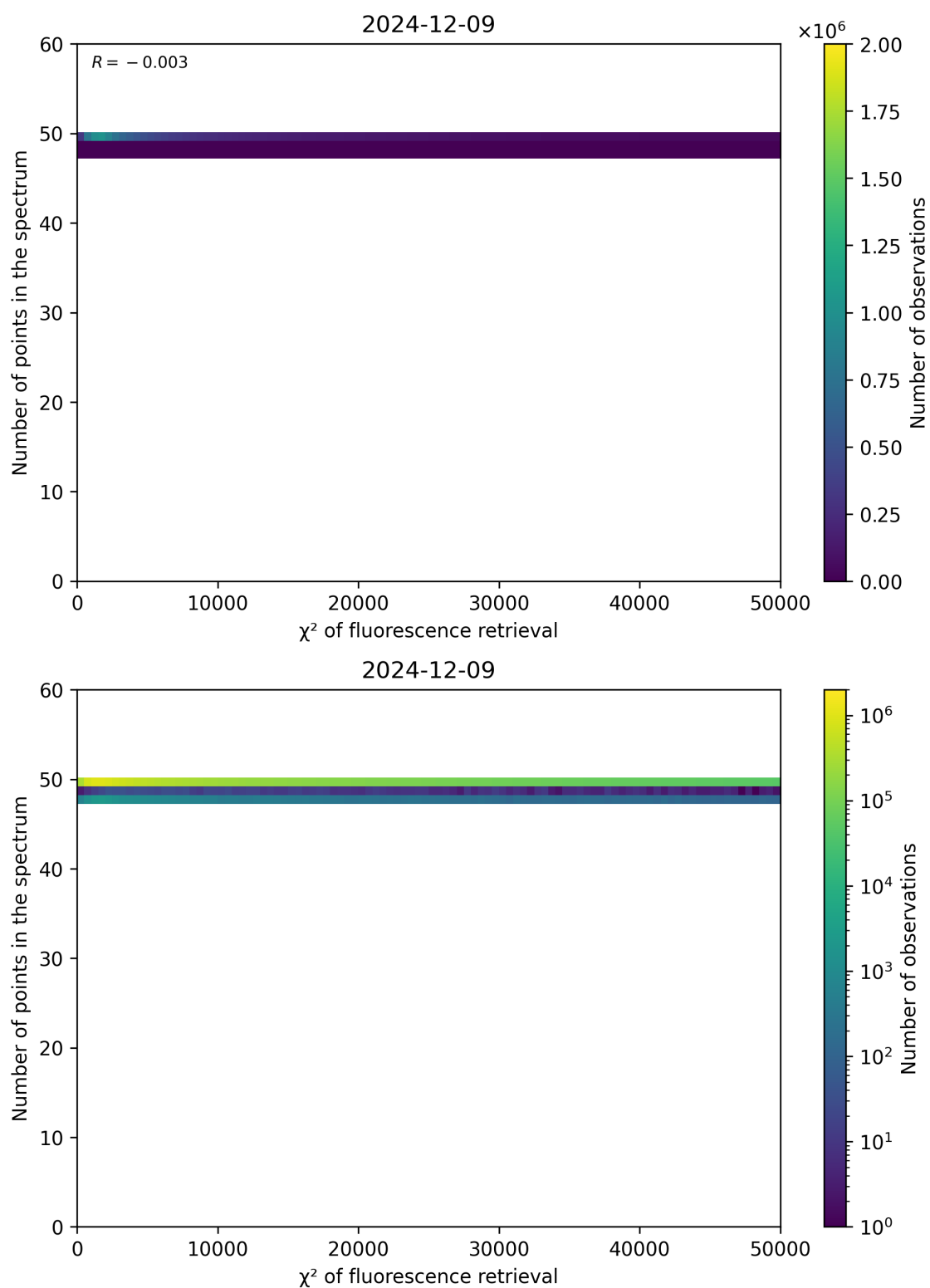
Figure 68: Scatter density plot of “ \chi^2 of fluorescence retrieval” against “Number of points in the spectrum” for 2024-12-08 to 2024-12-10.
