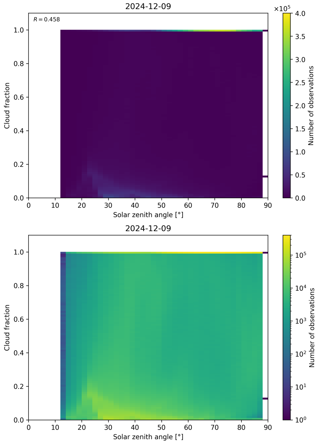
Figure 110: Scatter density plot of “Solar zenith angle” against “Cloud fraction” for 2024-12-08 to 2024-12-10.
