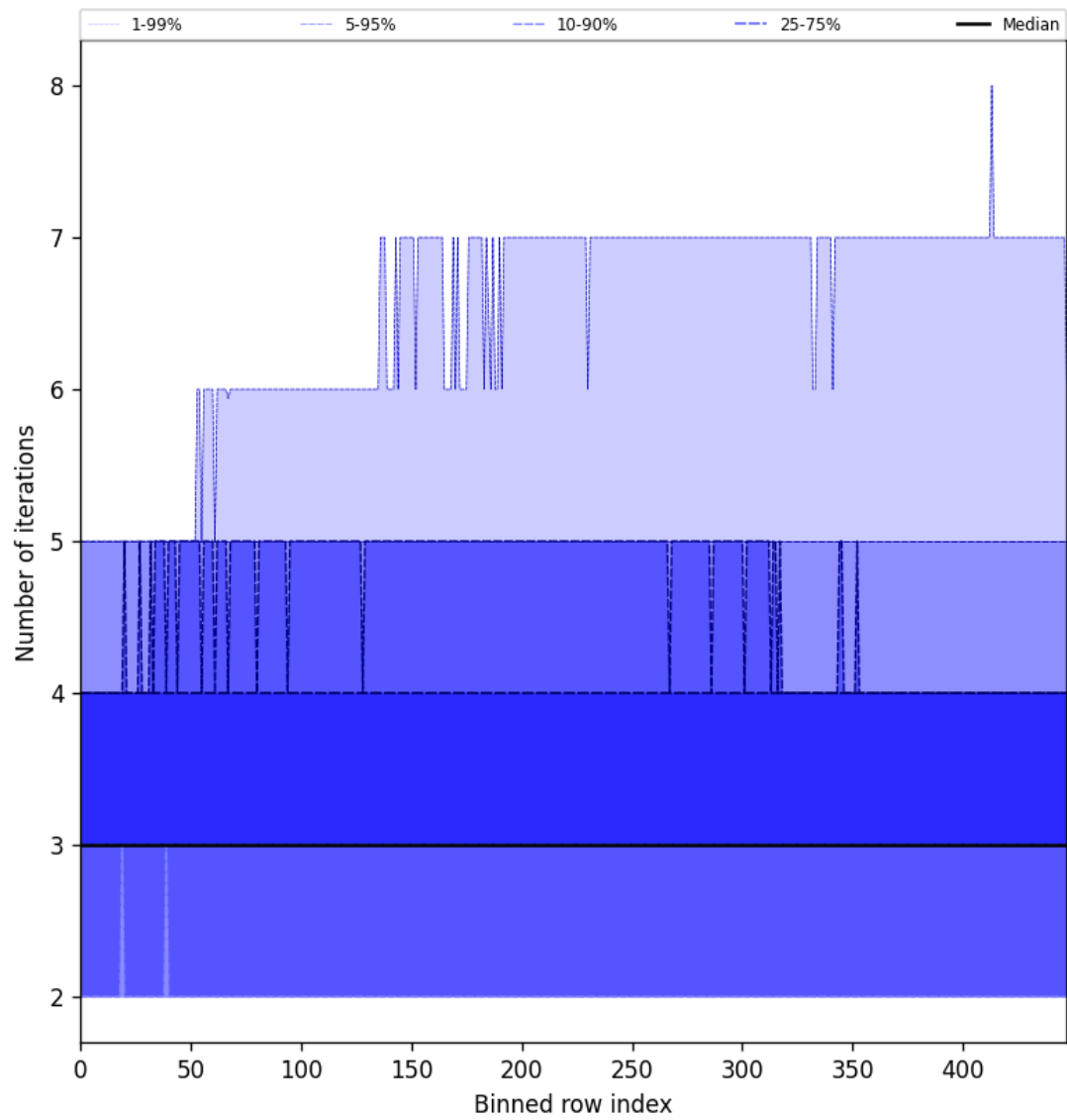
Figure 56: Along track statistics of “Number of iterations” for 2024-12-08 to 2024-12-10
