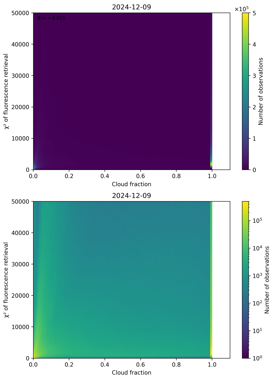
Figure 71: Scatter density plot of “Cloud fraction” against “ \chi^2 of fluorescence retrieval” for 2024-12-08 to 2024-12-10.
