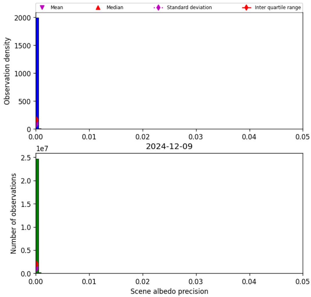
Figure 35: Histogram of “Scene albedo precision” for 2024-12-08 to 2024-12-10
