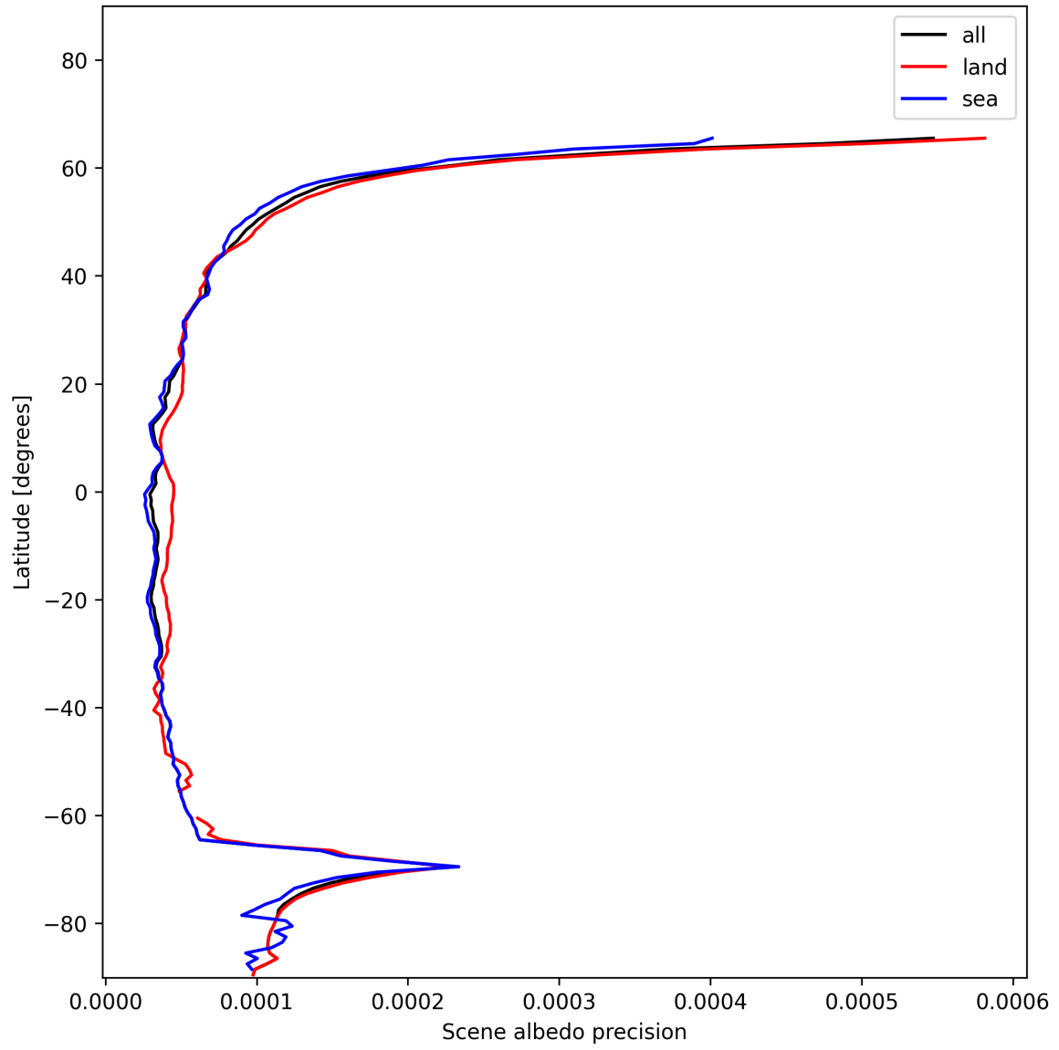
Figure 18: Zonal average of “Scene albedo precision” for 2024-12-08 to 2024-12-10.
