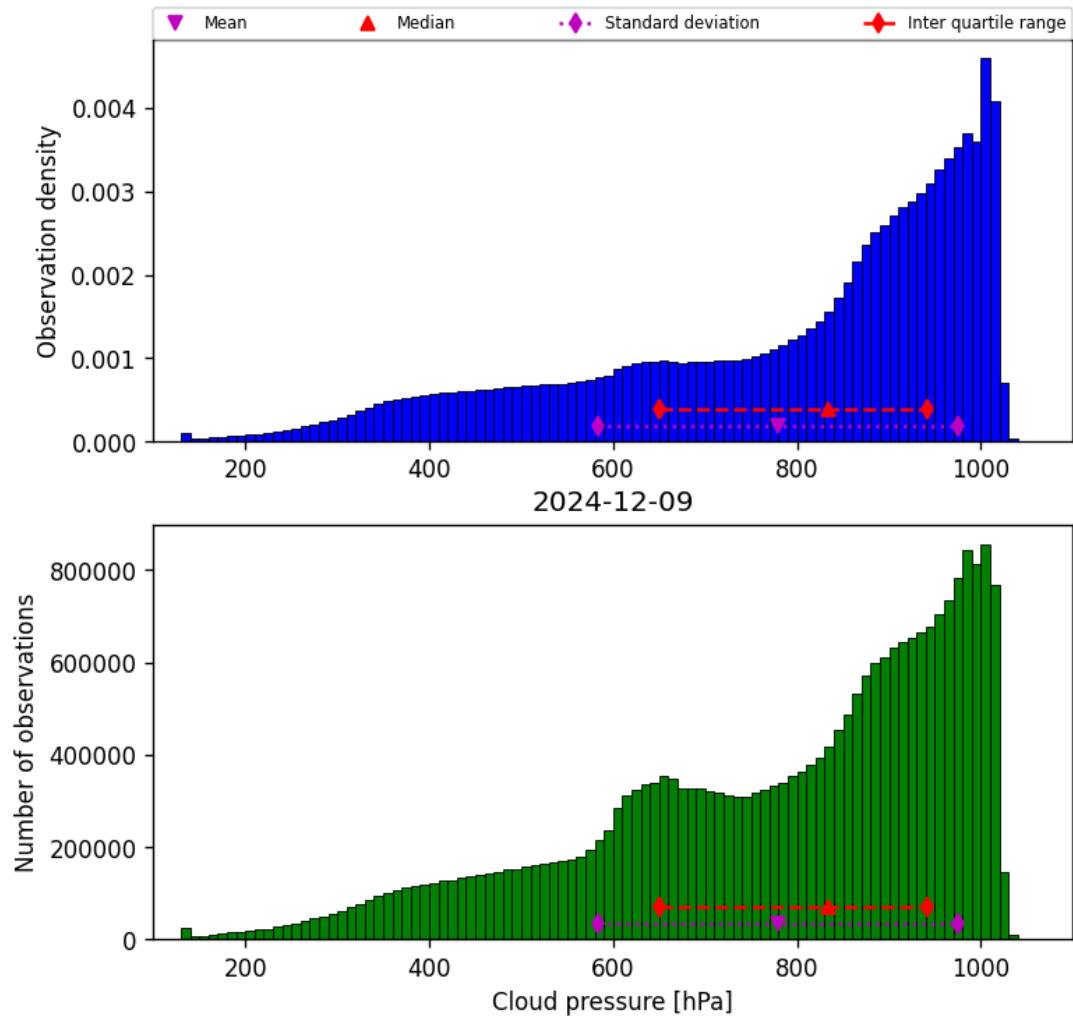
Figure 30: Histogram of “Cloud pressure” for 2024-12-08 to 2024-12-10
