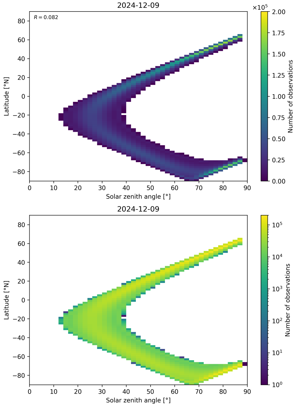
Figure 113: Scatter density plot of “Solar zenith angle” against “Latitude” for 2024-12-08 to 2024-12-10.
