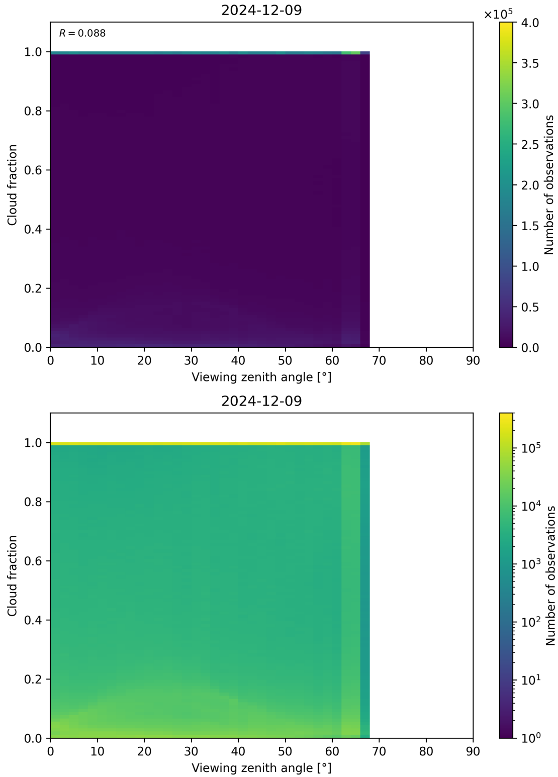
Figure 120: Scatter density plot of “Viewing zenith angle” against “Cloud fraction” for 2024-12-08 to 2024-12-10.
