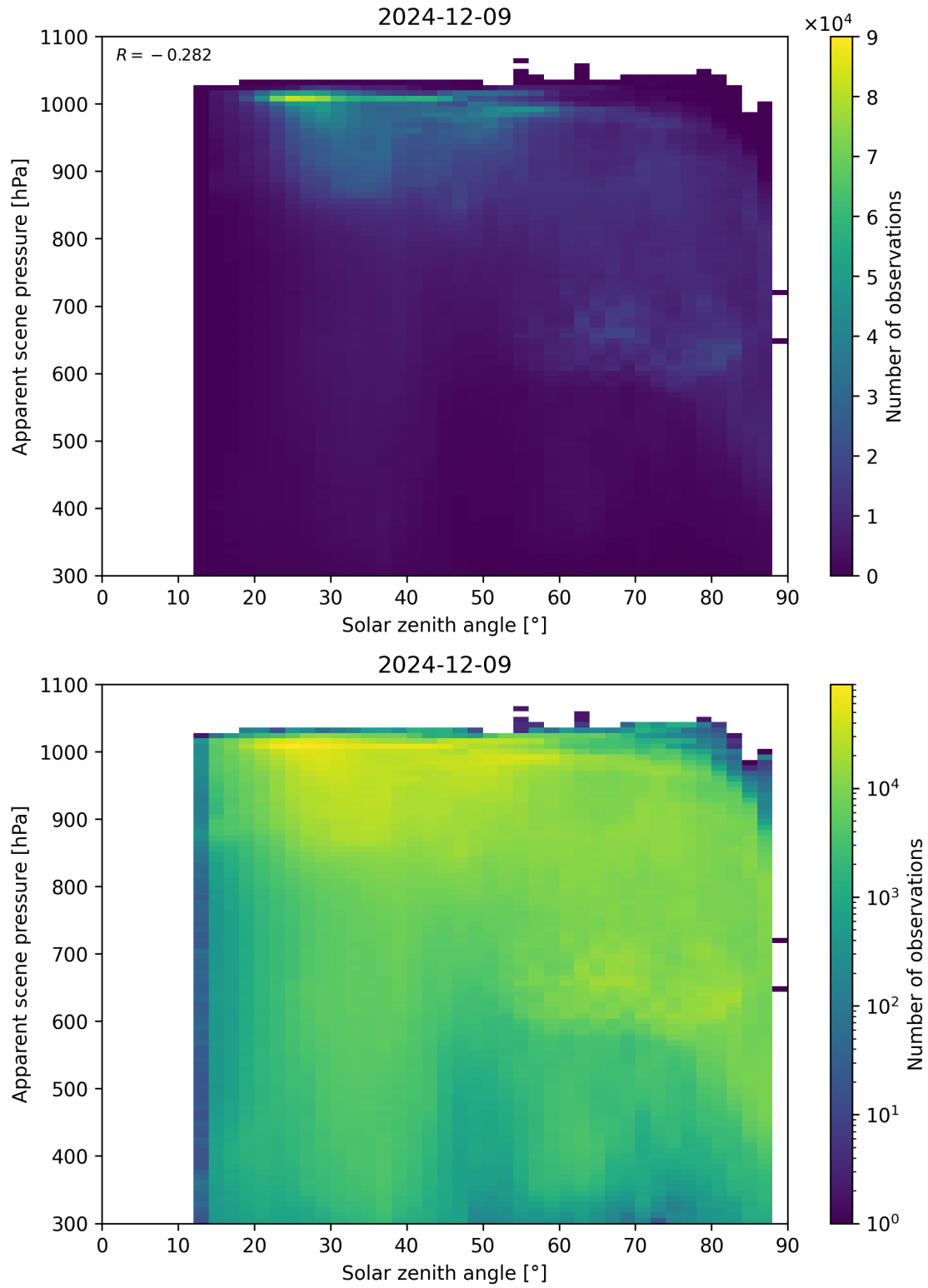
Figure 108: Scatter density plot of “Solar zenith angle” against “Apparent scene pressure” for 2024-12-08 to 2024-12-10.
