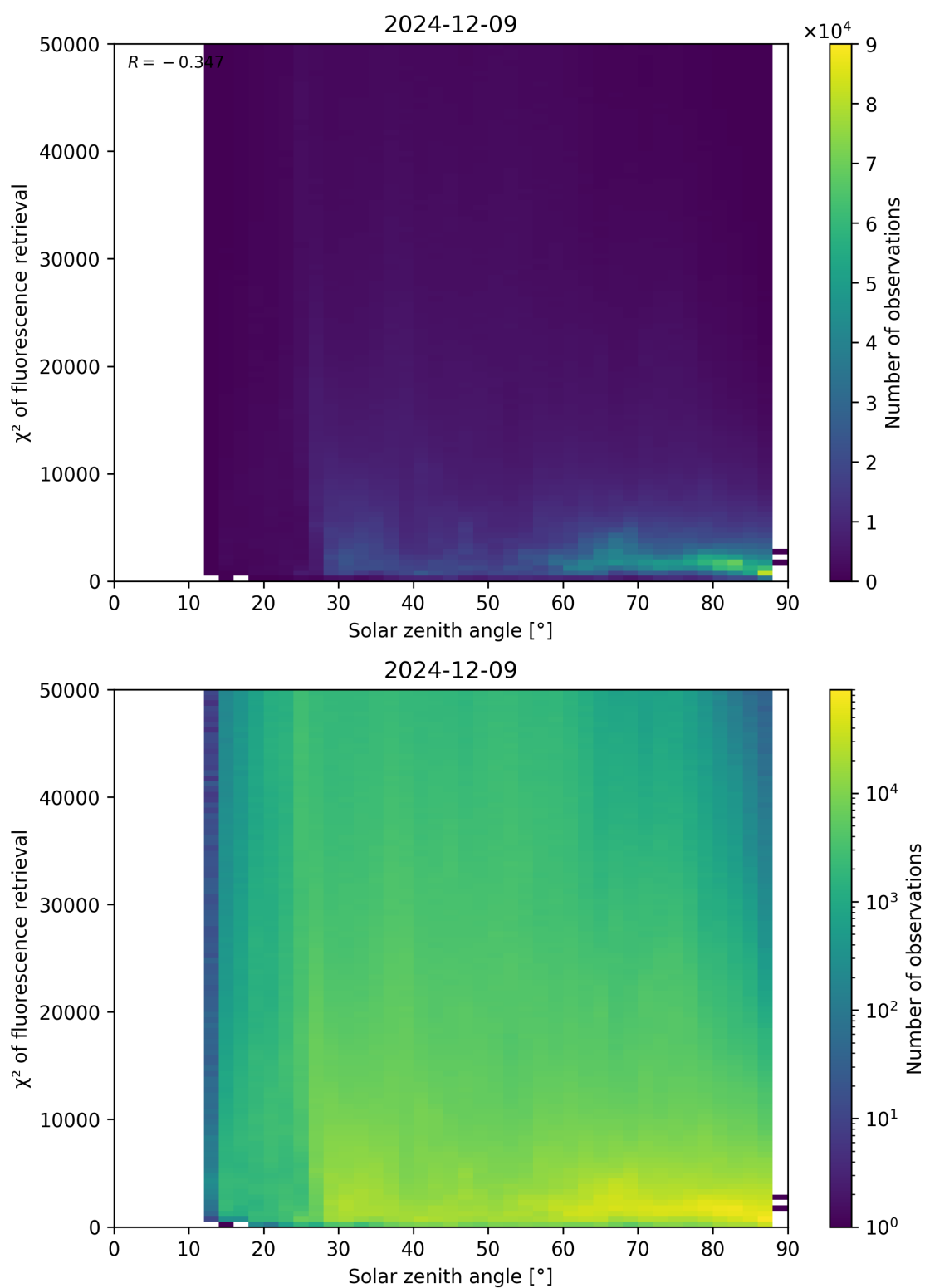
Figure 109: Scatter density plot of “Solar zenith angle” against “ \chi^2 of fluorescence retrieval” for 2024-12-08 to 2024-12-10.
