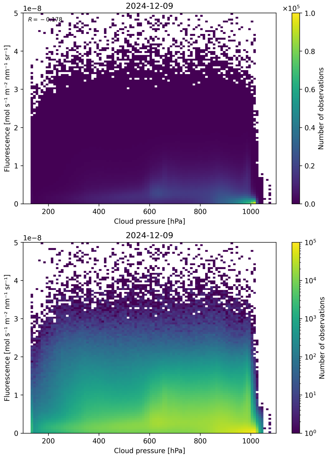
Figure 80: Scatter density plot of “Cloud pressure” against “Fluorescence” for 2024-12-08 to 2024-12-10.
