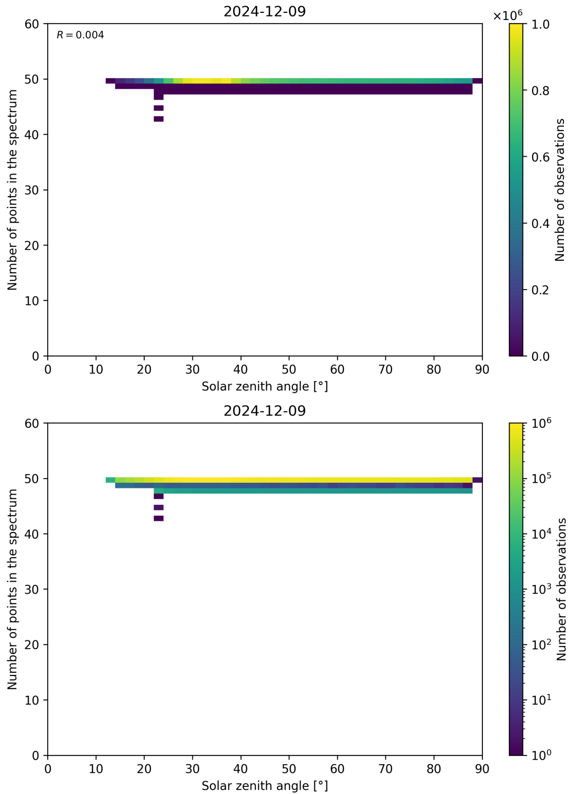
Figure 115: Scatter density plot of “Solar zenith angle” against “Number of points in the spectrum” for 2024-12-08 to 2024-12-10.
