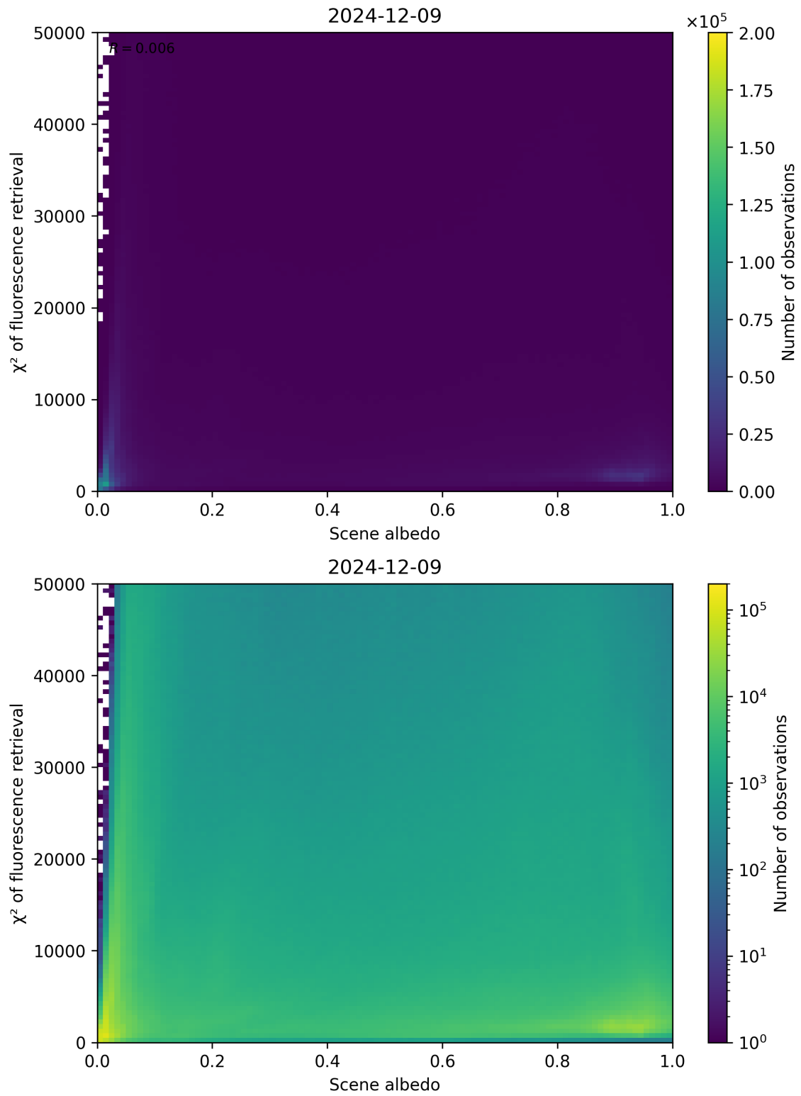
Figure 103: Scatter density plot of “Scene albedo” against “ \chi^2 of fluorescence retrieval” for 2024-12-08 to 2024-12-10.
