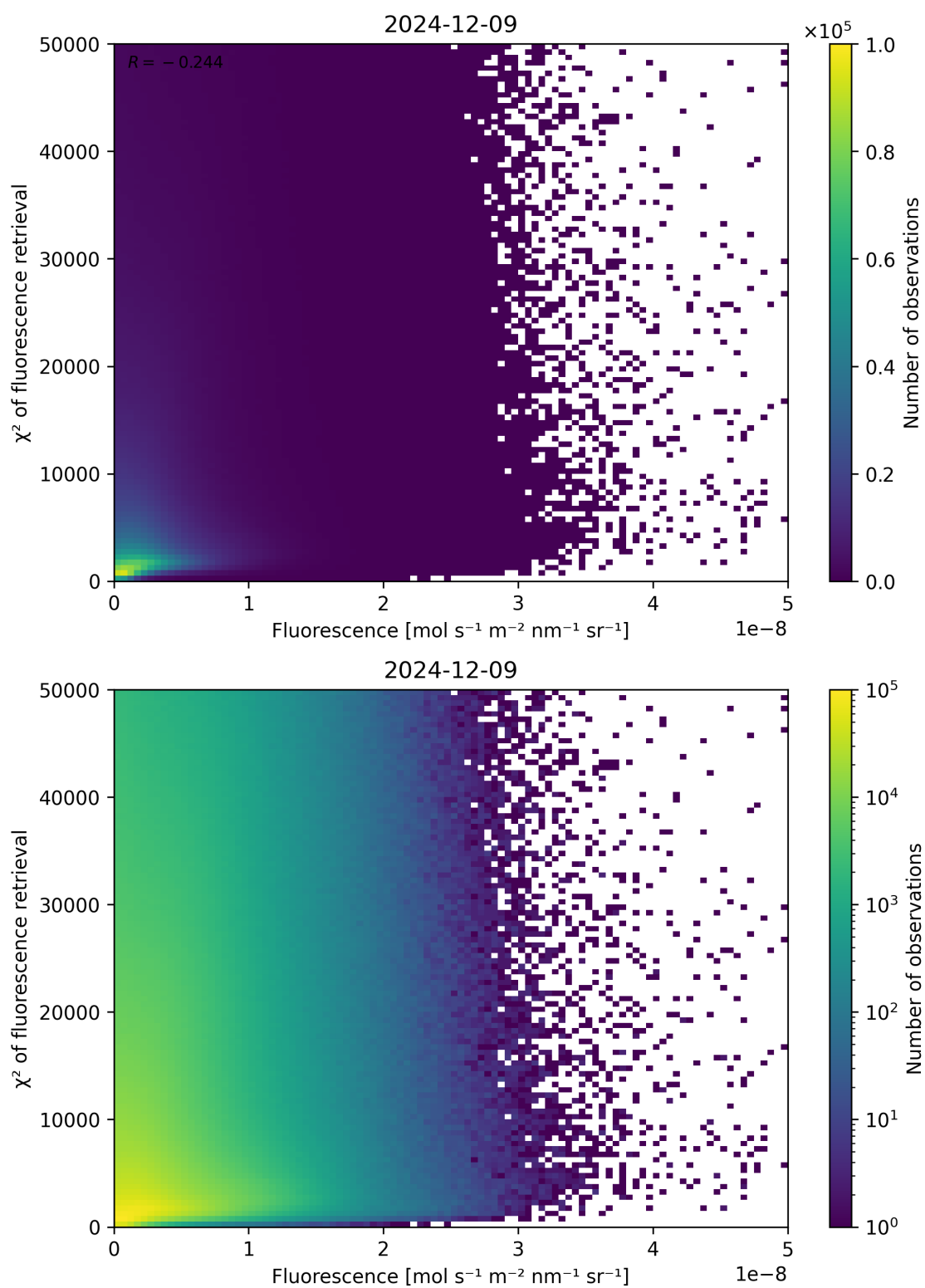
Figure 85: Scatter density plot of “Fluorescence” against “ \chi^2 of fluorescence retrieval” for 2024-12-08 to 2024-12-10.
