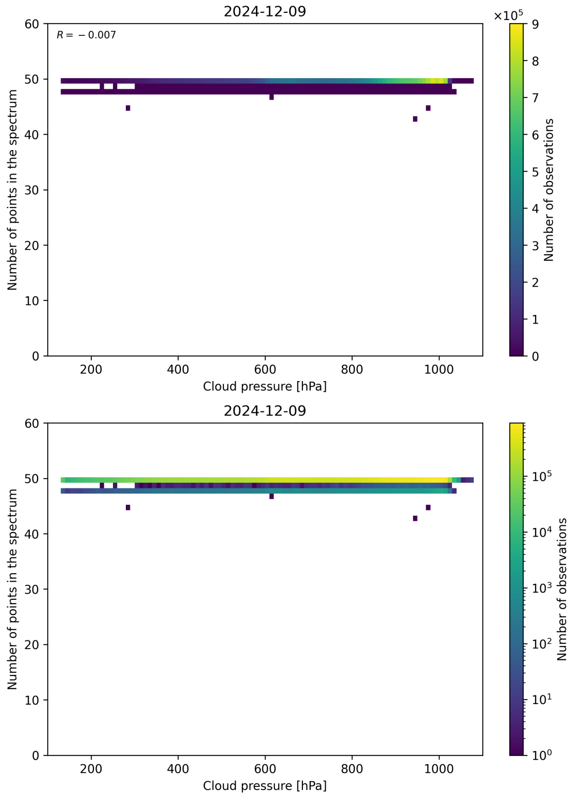
Figure 82: Scatter density plot of “Cloud pressure” against “Number of points in the spectrum” for 2024-12-08 to 2024-12-10.
