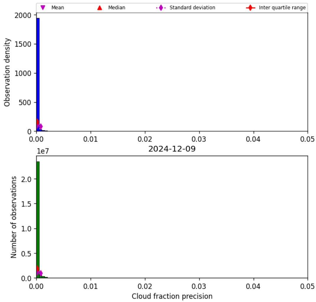
Figure 33: Histogram of “Cloud fraction precision” for 2024-12-08 to 2024-12-10
