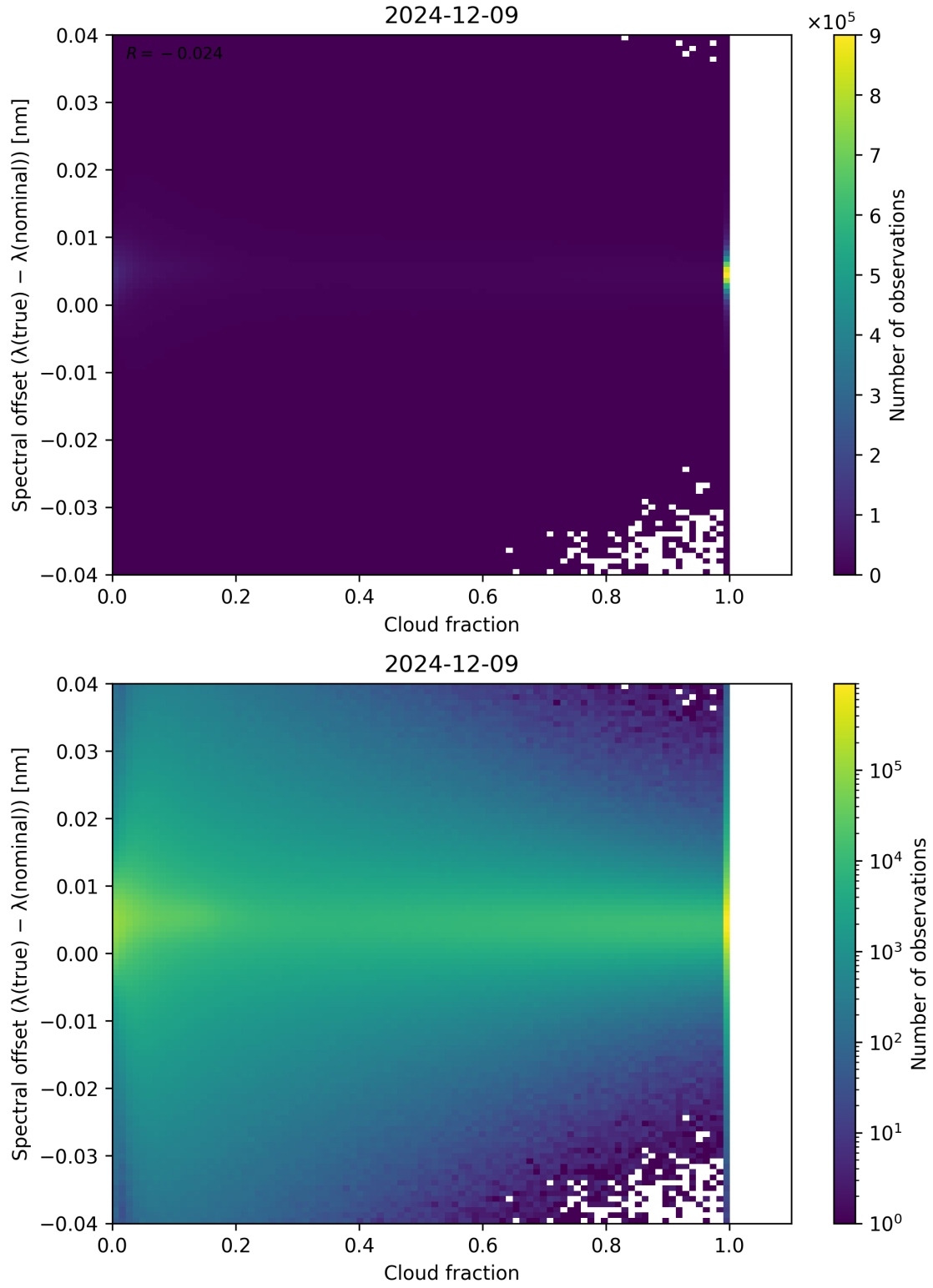
Figure 76: Scatter density plot of “Cloud fraction” against “Spectral offset ( \lambda_{\text{true}} - \lambda_{\text{nominal}} )” for 2024-12-08 to 2024-12-10.
