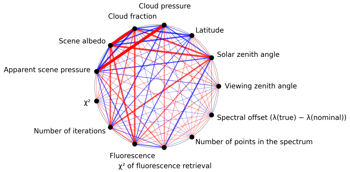
Figure 1: Map of correlation graph for 2024-12-08 to 2024-12-10.
