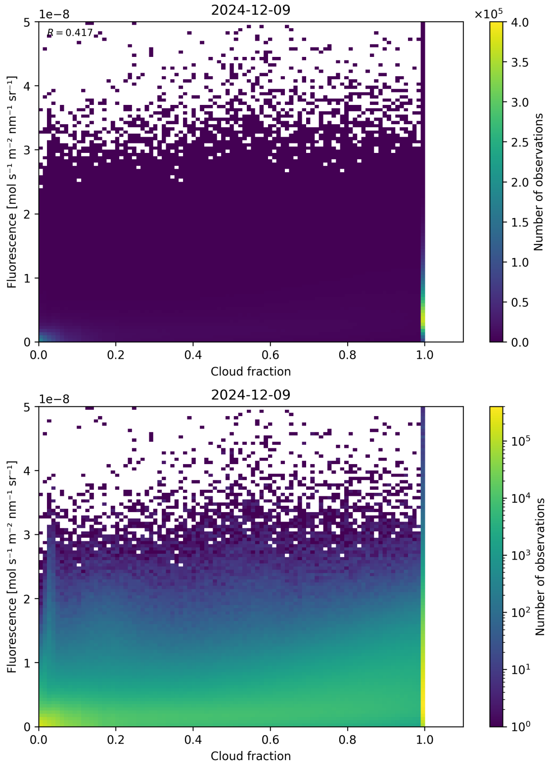
Figure 72: Scatter density plot of “Cloud fraction” against “Fluorescence” for 2024-12-08 to 2024-12-10.
