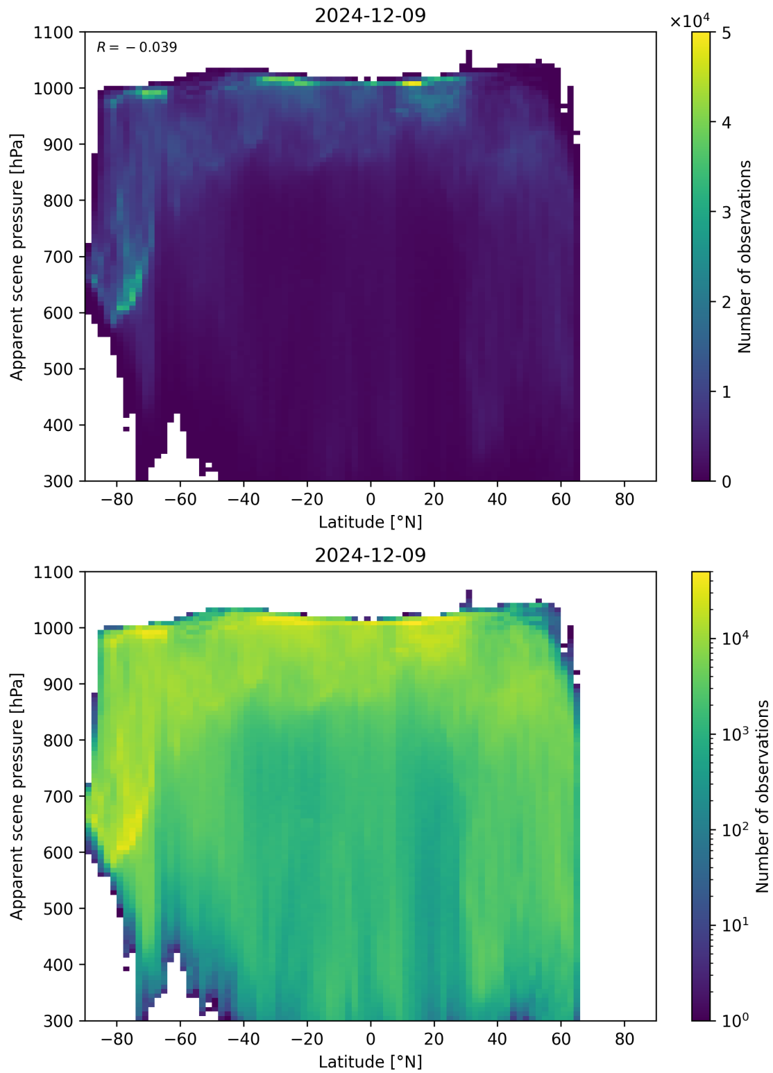
Figure 88: Scatter density plot of “Latitude” against “Apparent scene pressure” for 2024-12-08 to 2024-12-10.
