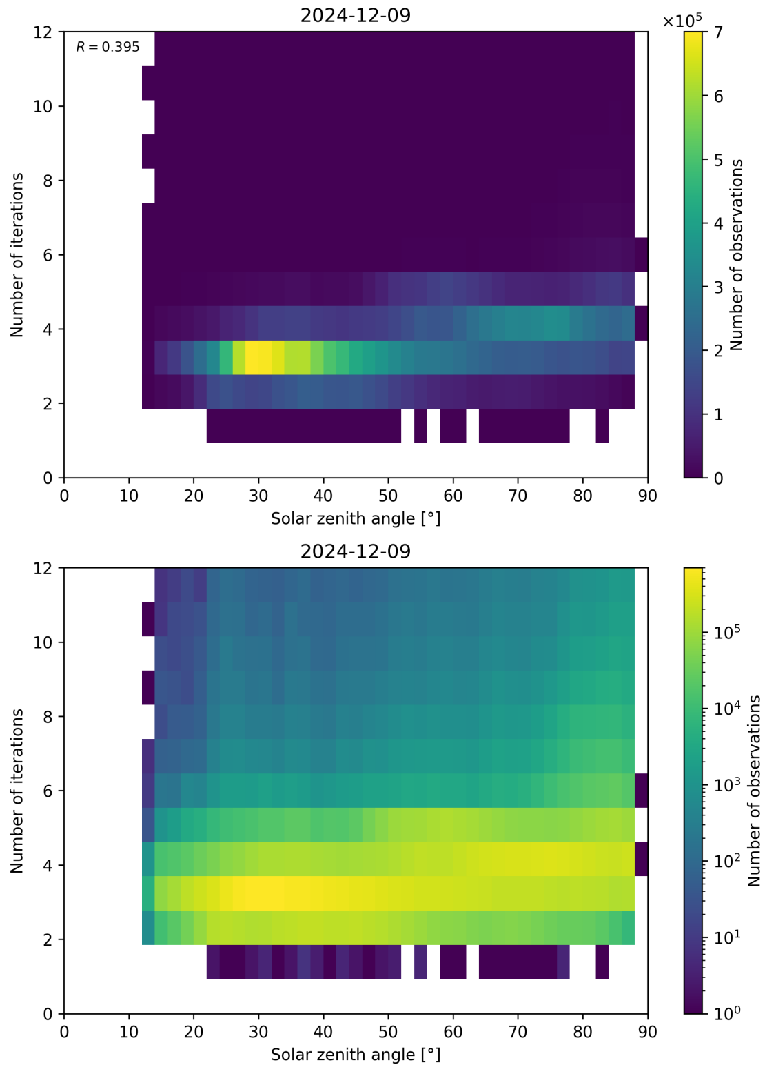
Figure 114: Scatter density plot of “Solar zenith angle” against “Number of iterations” for 2024-12-08 to 2024-12-10.
