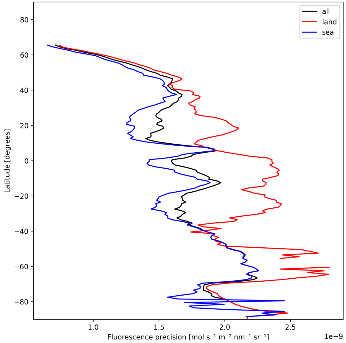
Figure 24: Zonal average of “Fluorescence precision” for 2024-12-08 to 2024-12-10.
