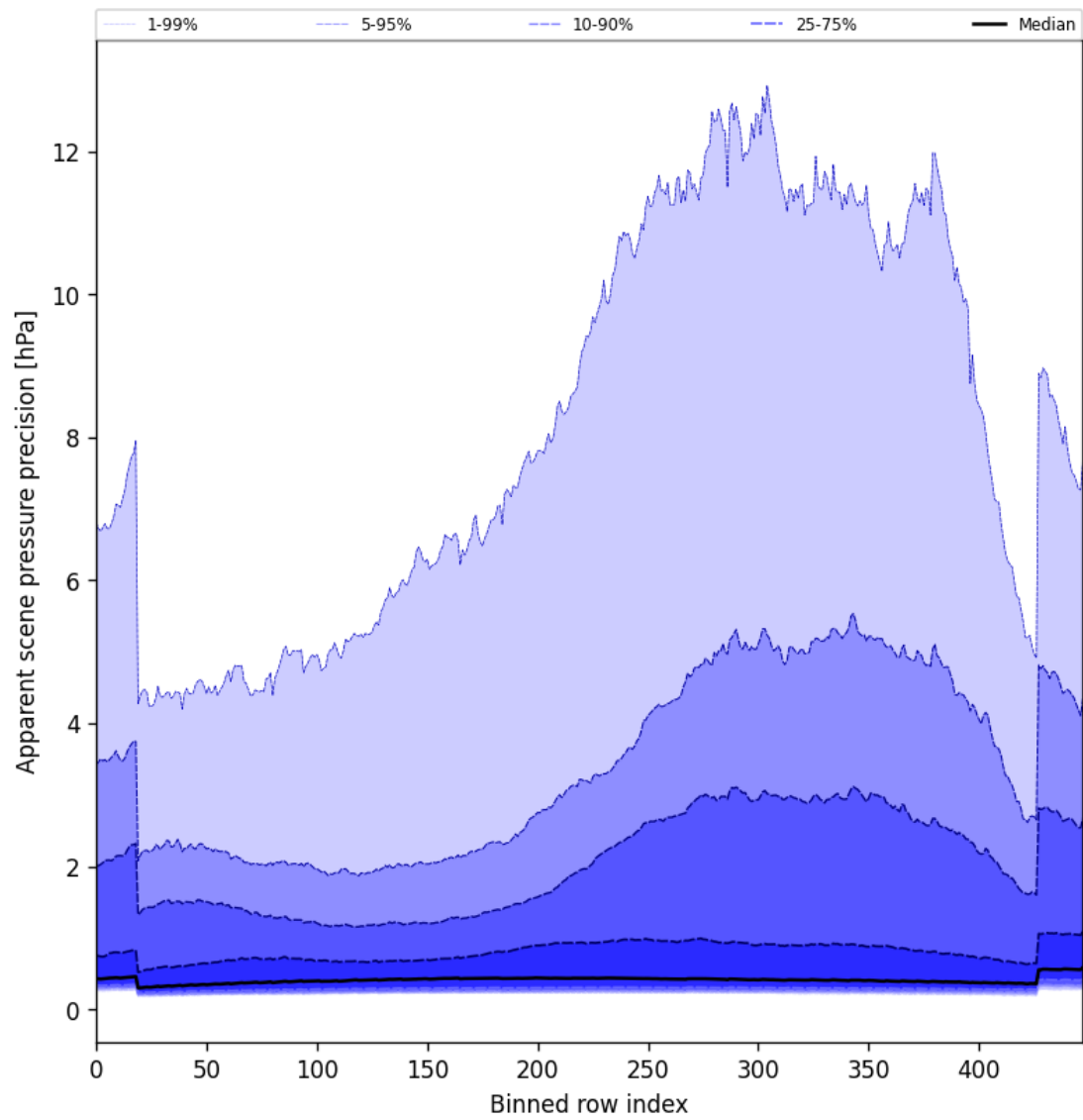
Figure 54: Along track statistics of “Apparent scene pressure precision” for 2024-12-08 to 2024-12-10
