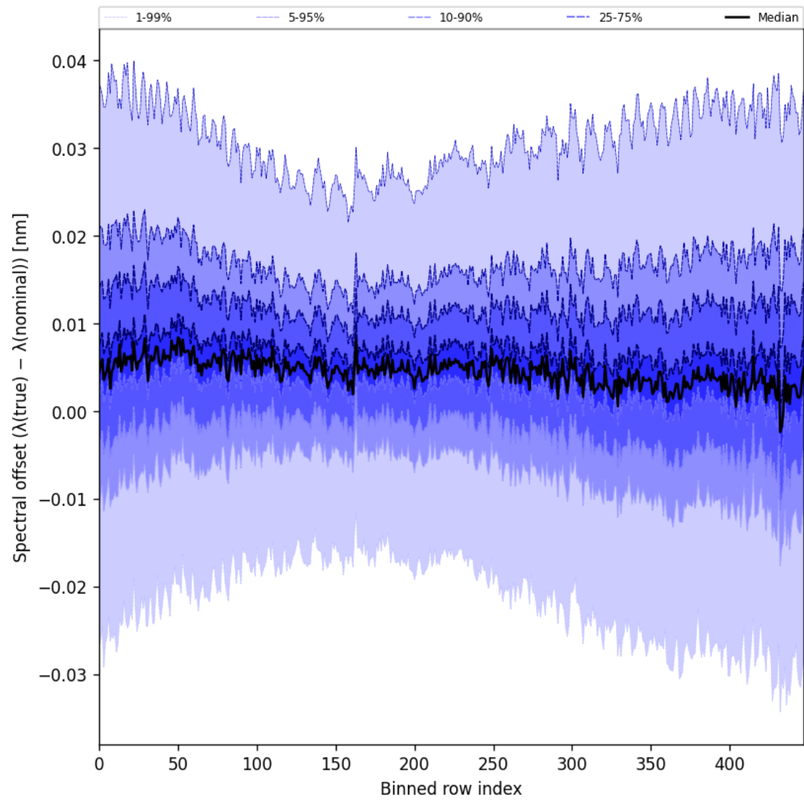
Figure 62: Along track statistics of “Spectral offset ( \lambda_{\text{true}} - \lambda_{\text{nominal}} )” for 2024-12-08 to 2024-12-10
