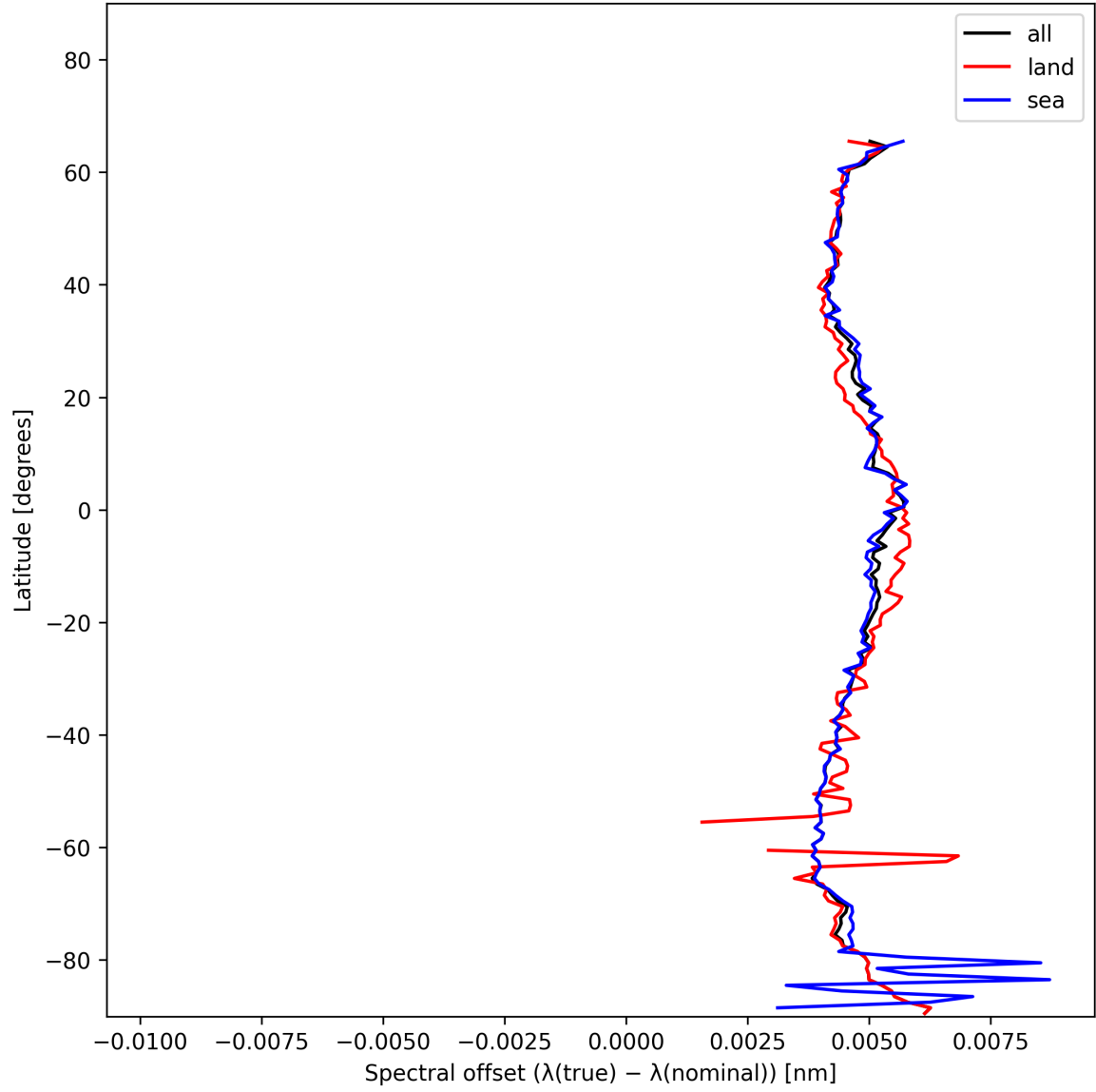
Figure 28: Zonal average of “Spectral offset ( \lambda_{\text{true}} - \lambda_{\text{nominal}} )” for 2024-12-08 to 2024-12-10.
