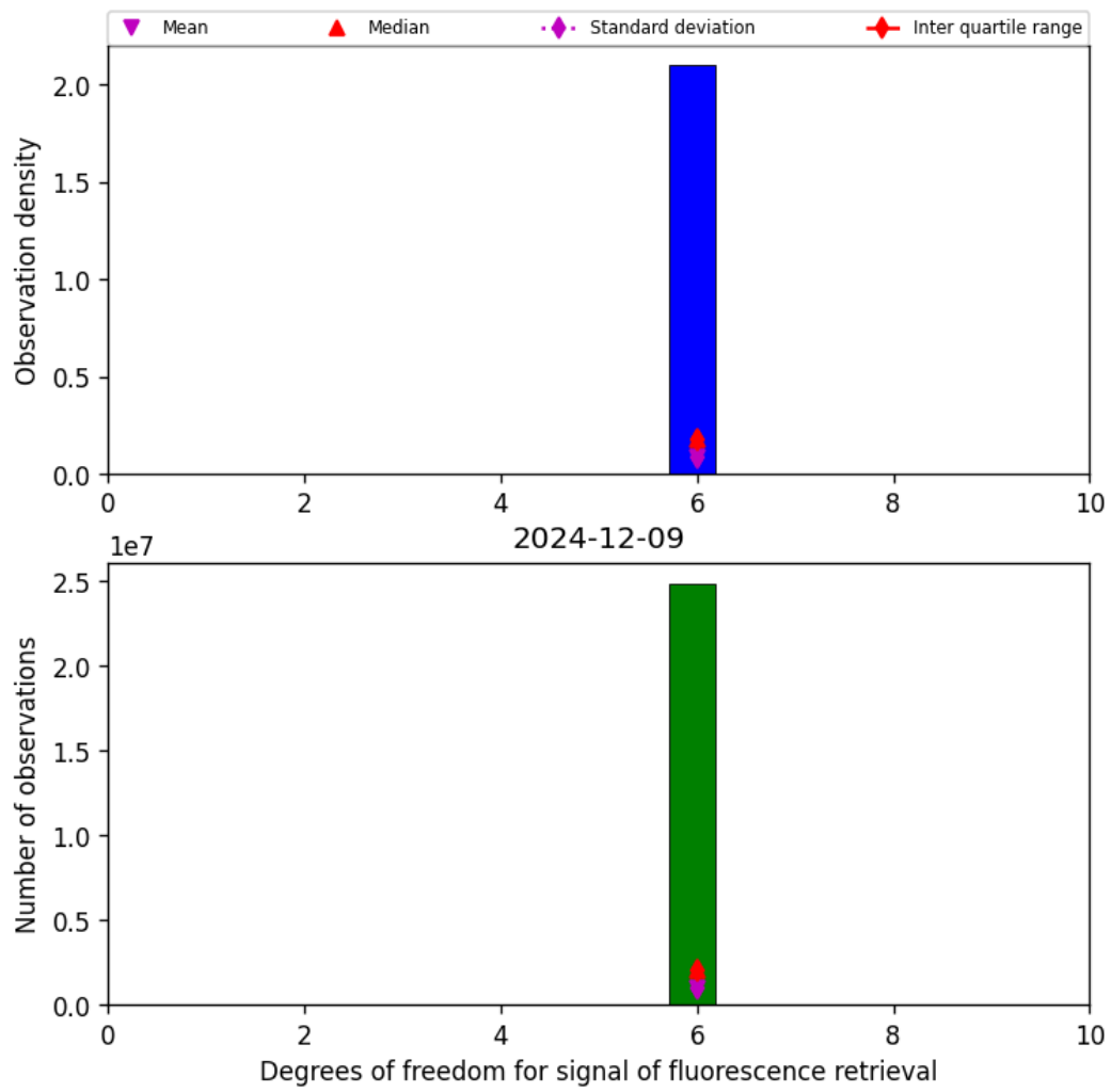
Figure 43: Histogram of “Degrees of freedom for signal of fluorescence retrieval” for 2024-12-08 to 2024-12-10
