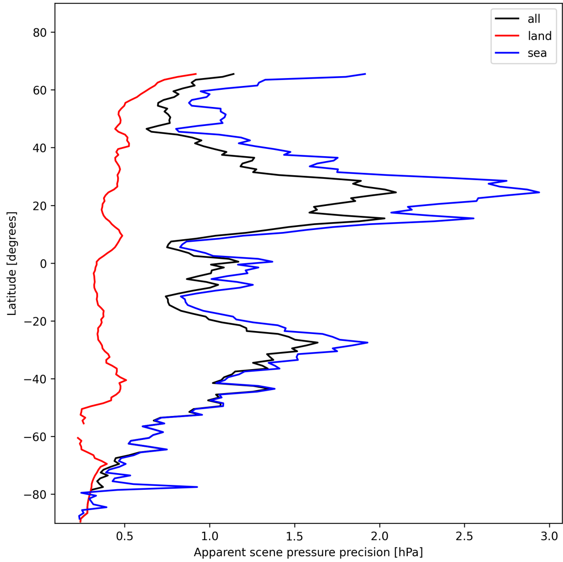
Figure 20: Zonal average of “Apparent scene pressure precision” for 2024-12-08 to 2024-12-10.
