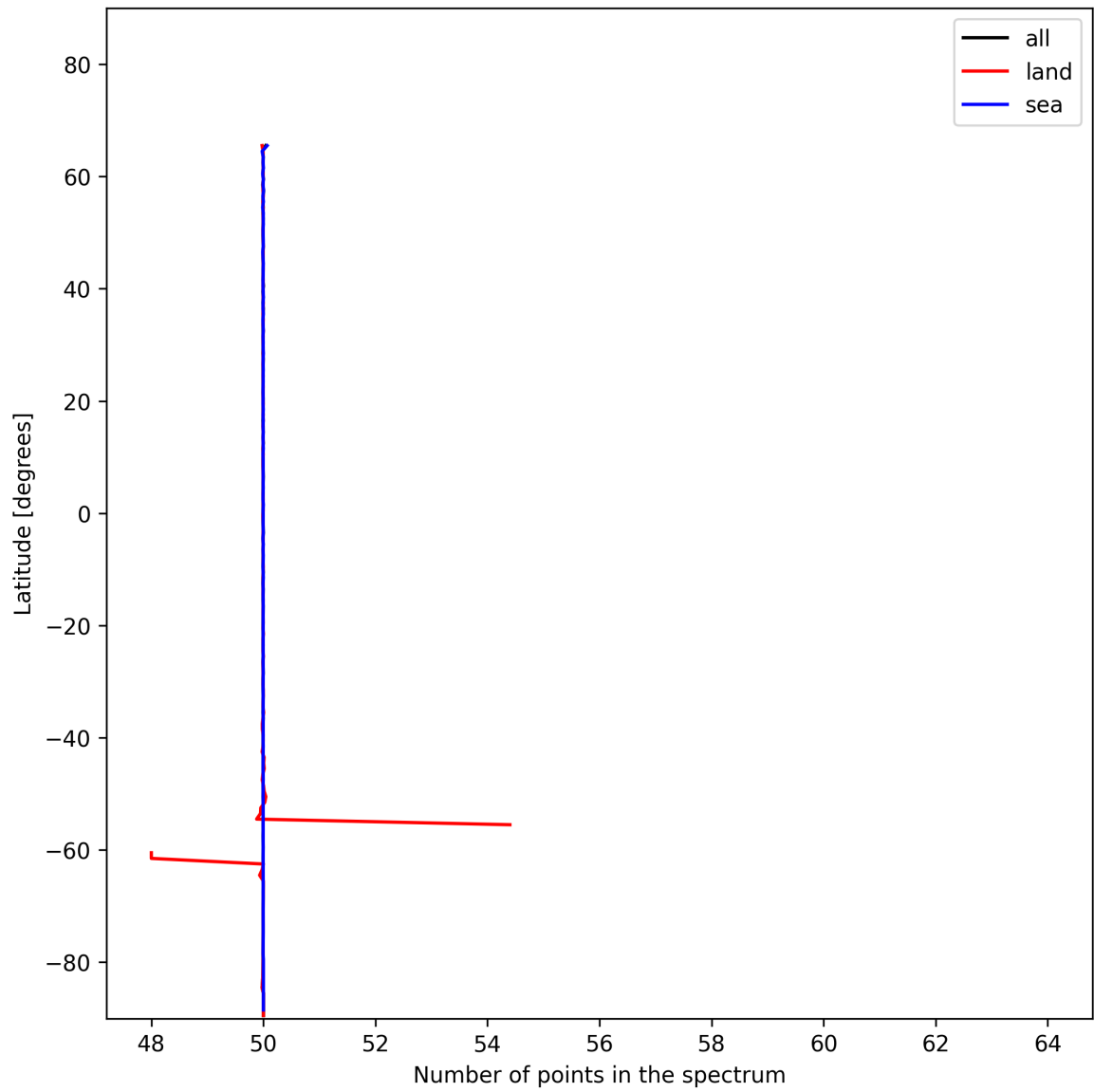
Figure 27: Zonal average of “Number of points in the spectrum” for 2024-12-08 to 2024-12-10.
