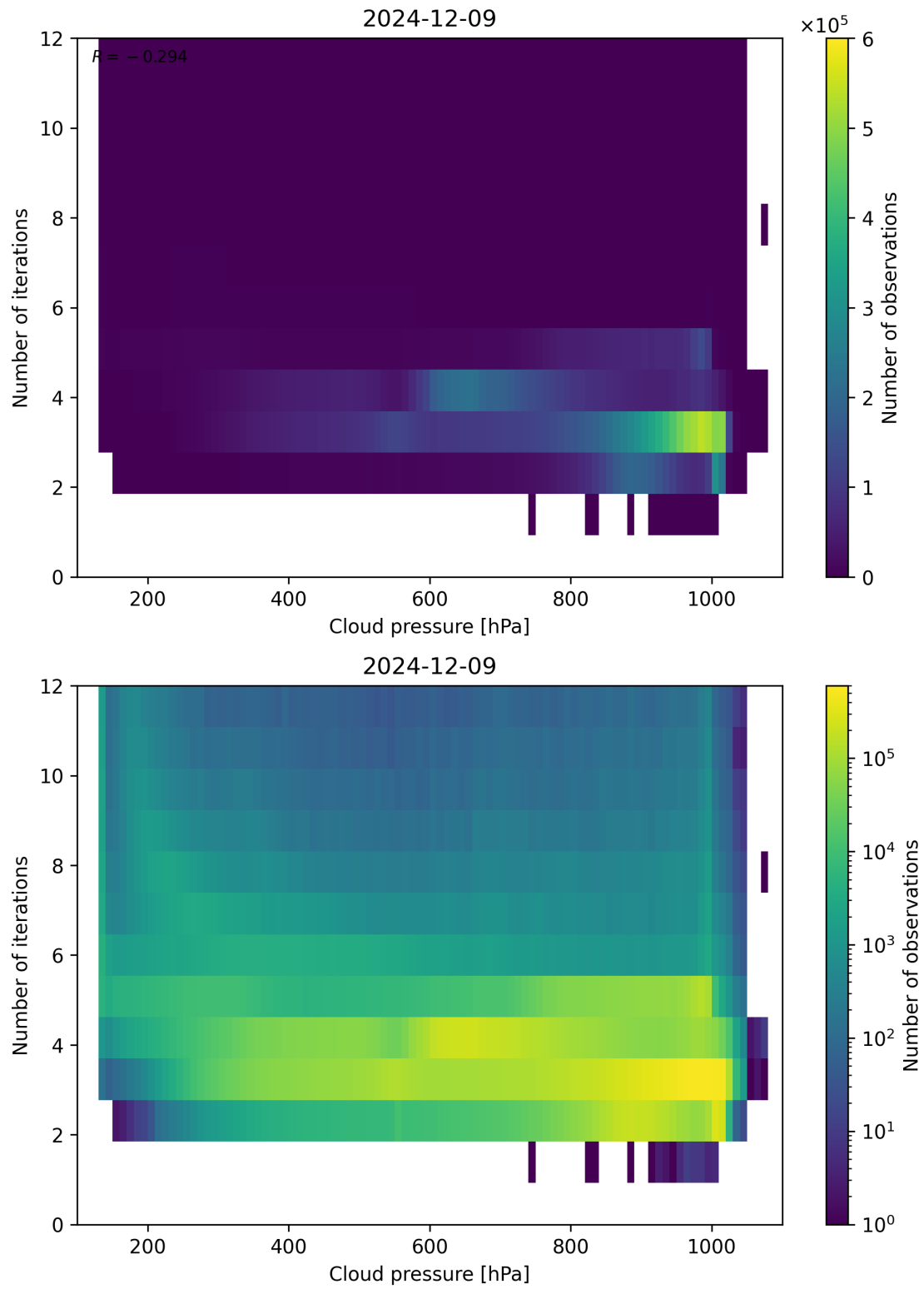
Figure 81: Scatter density plot of “Cloud pressure” against “Number of iterations” for 2024-12-08 to 2024-12-10.
