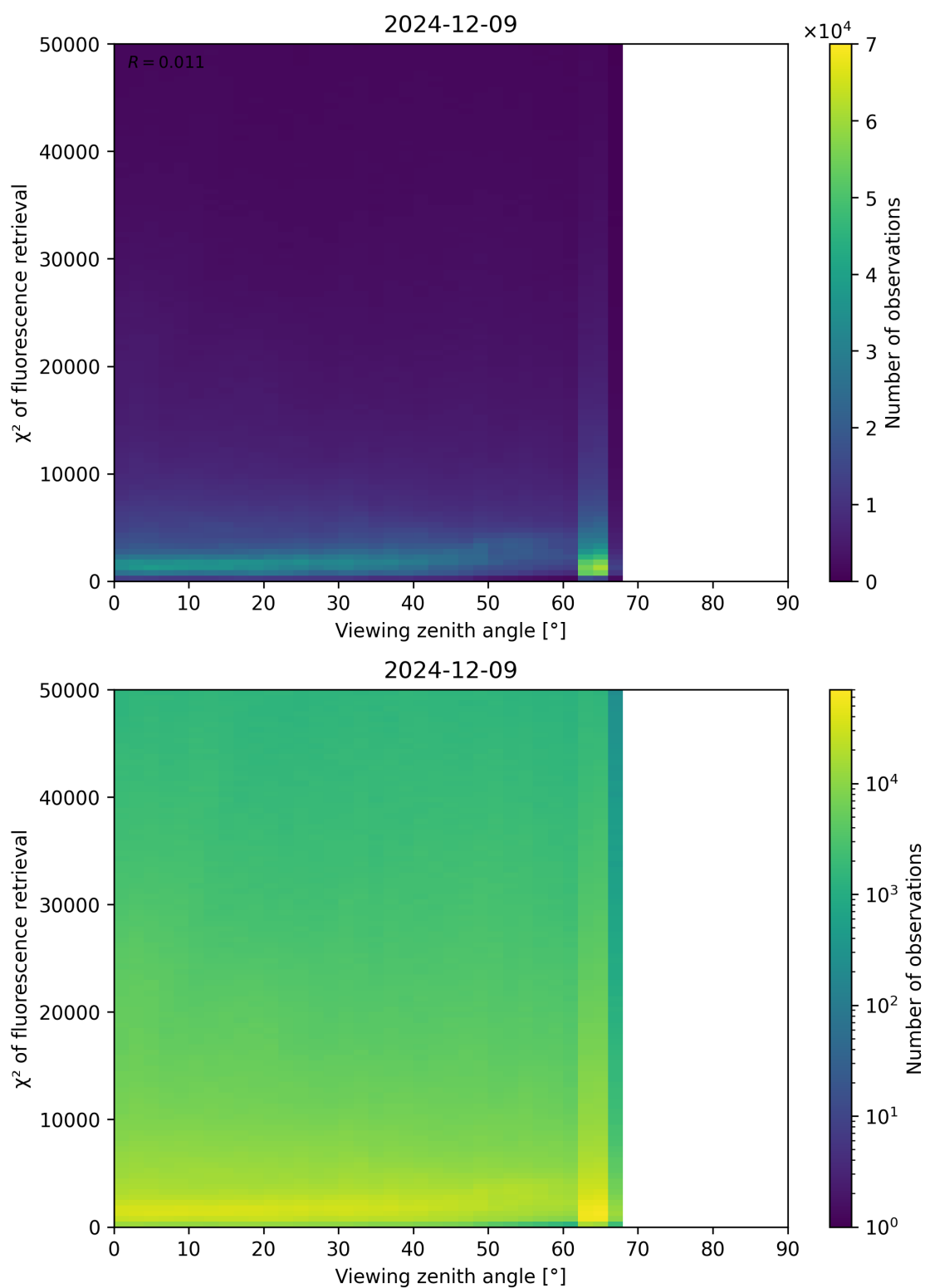
Figure 119: Scatter density plot of “Viewing zenith angle” against “ \chi^2 of fluorescence retrieval” for 2024-12-08 to 2024-12-10.
