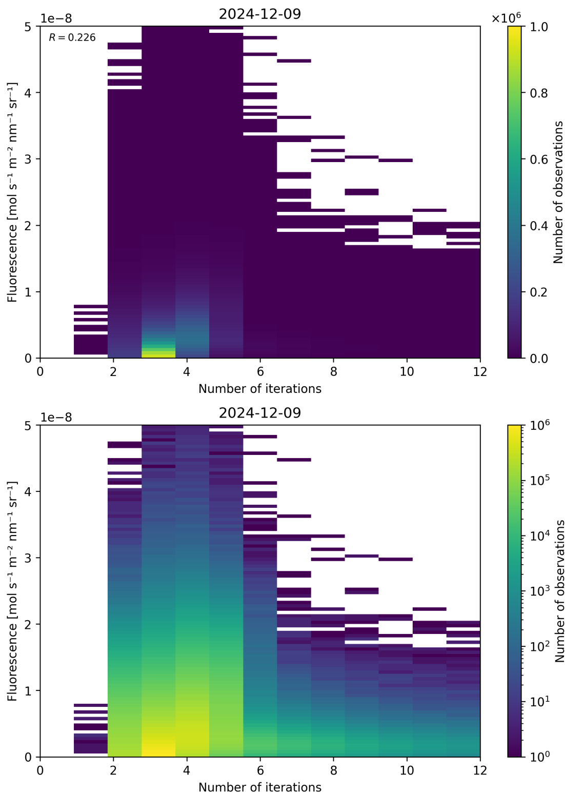
Figure 98: Scatter density plot of “Number of iterations” against “Fluorescence” for 2024-12-08 to 2024-12-10.
