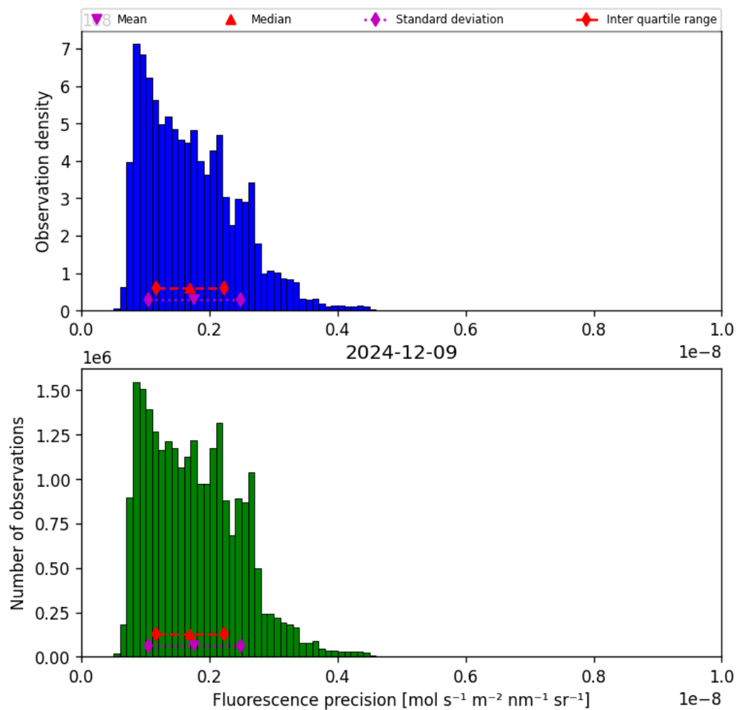
Figure 41: Histogram of “Fluorescence precision” for 2024-12-08 to 2024-12-10
