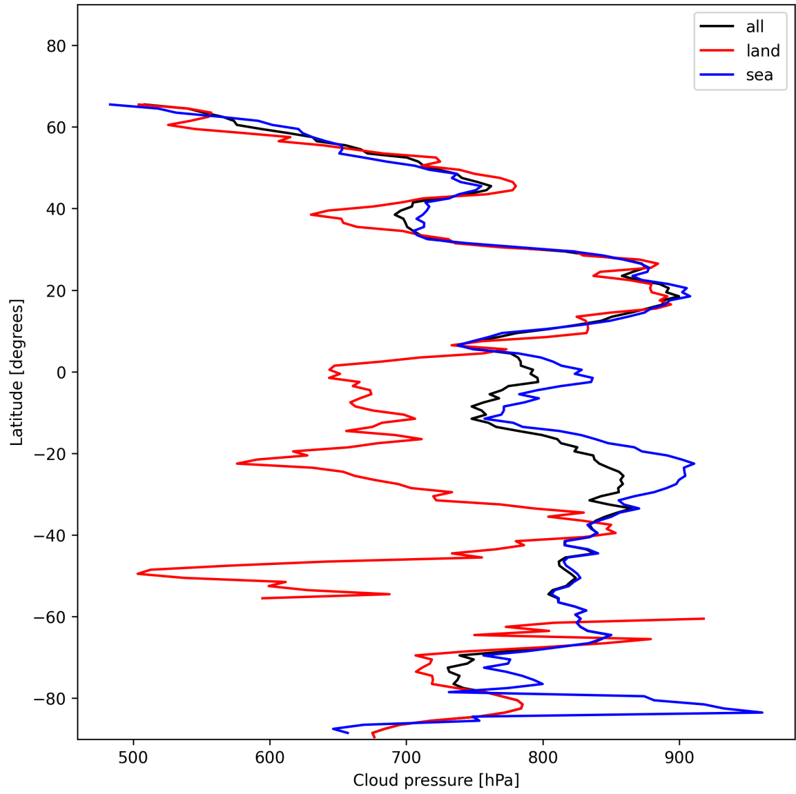
Figure 13: Zonal average of “Cloud pressure” for 2024-12-08 to 2024-12-10.
