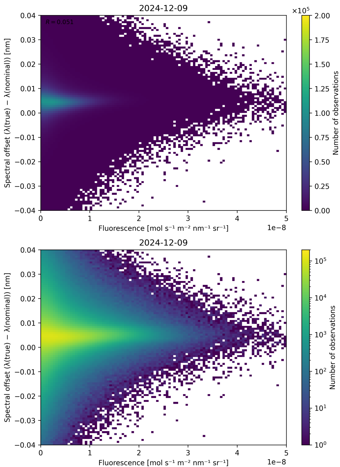
Figure 87: Scatter density plot of “Fluorescence” against “Spectral offset ( \lambda_{\text{true}} - \lambda_{\text{nominal}} )” for 2024-12-08 to 2024-12-10.
