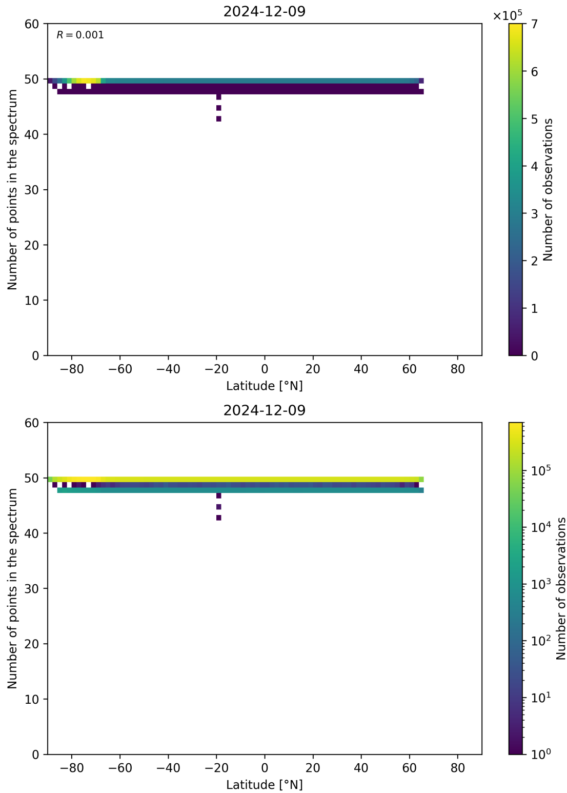
Figure 94: Scatter density plot of “Latitude” against “Number of points in the spectrum” for 2024-12-08 to 2024-12-10.
