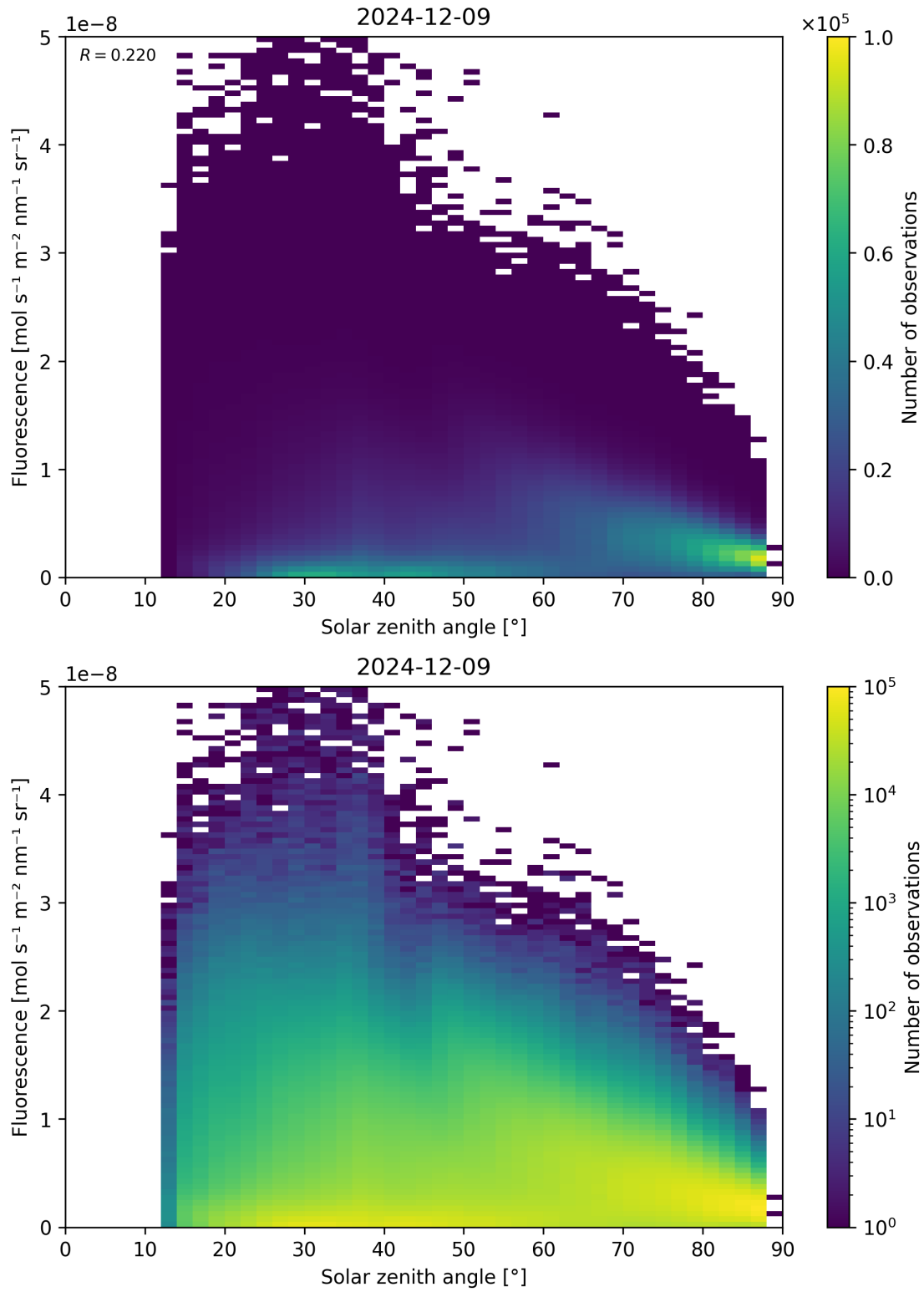
Figure 112: Scatter density plot of “Solar zenith angle” against “Fluorescence” for 2024-12-08 to 2024-12-10.
