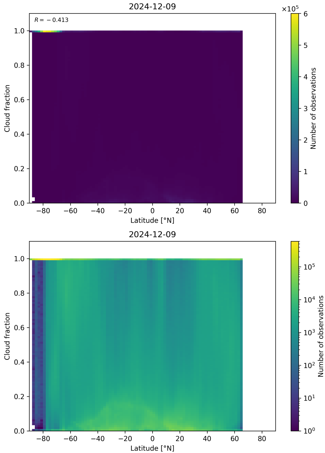
Figure 90: Scatter density plot of “Latitude” against “Cloud fraction” for 2024-12-08 to 2024-12-10.
