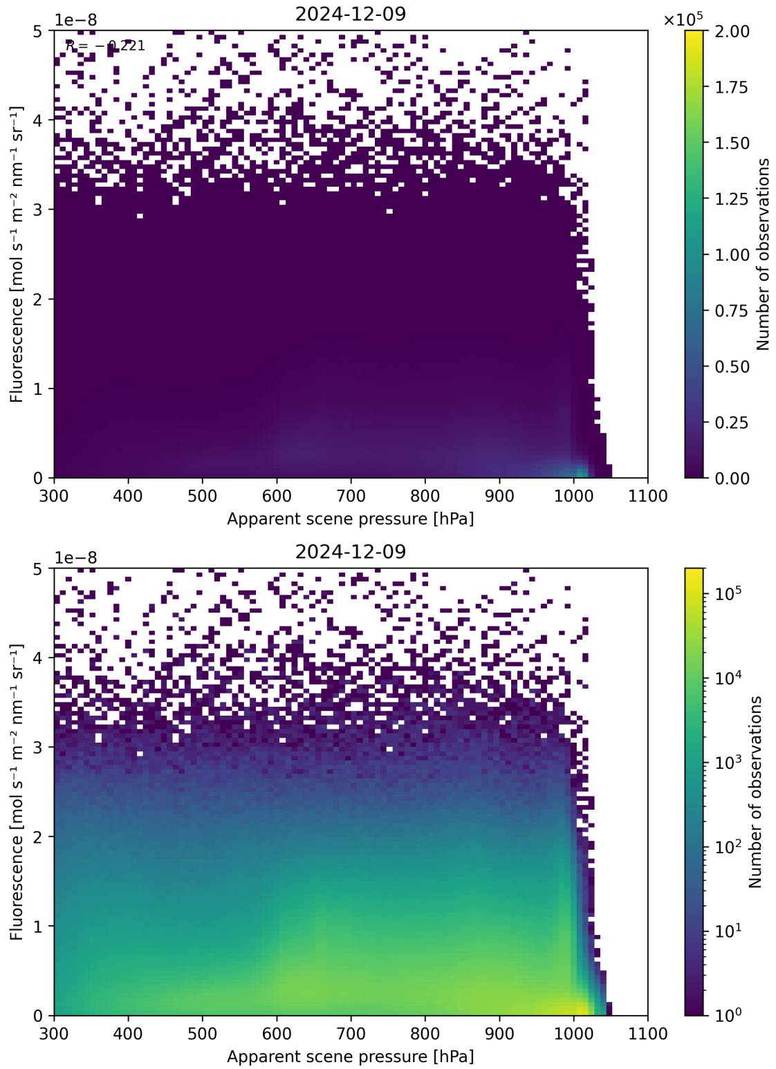
Figure 64: Scatter density plot of “Apparent scene pressure” against “Fluorescence” for 2024-12-08 to 2024-12-10.
