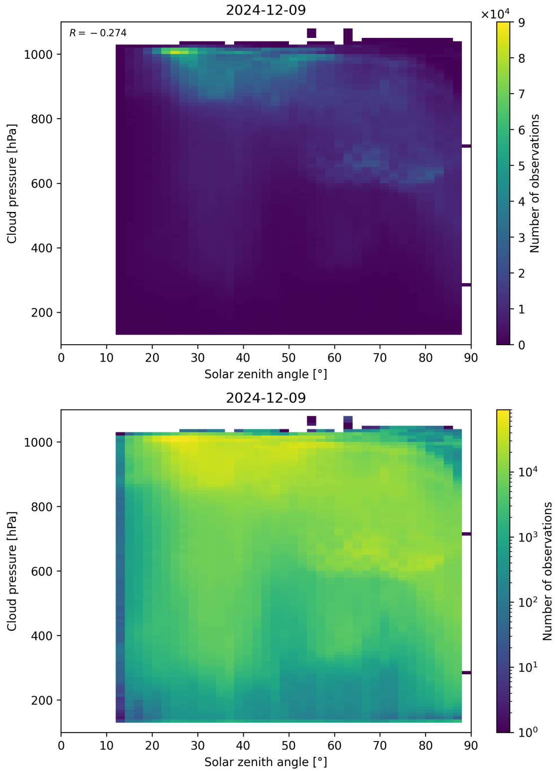
Figure 111: Scatter density plot of “Solar zenith angle” against “Cloud pressure” for 2024-12-08 to 2024-12-10.
