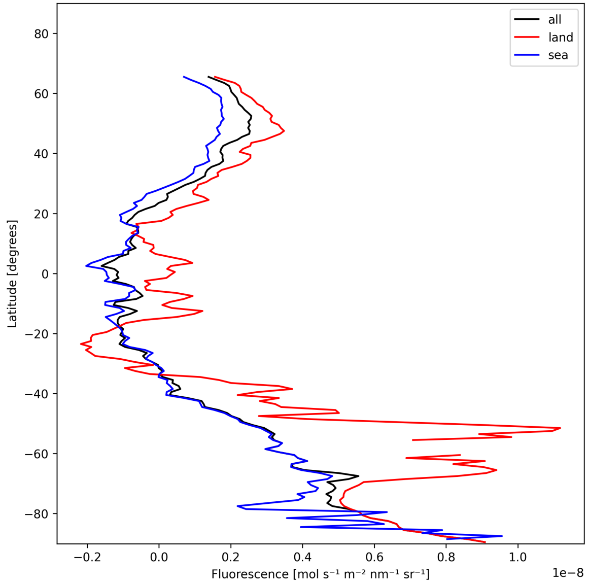
Figure 23: Zonal average of “Fluorescence” for 2024-12-08 to 2024-12-10.
