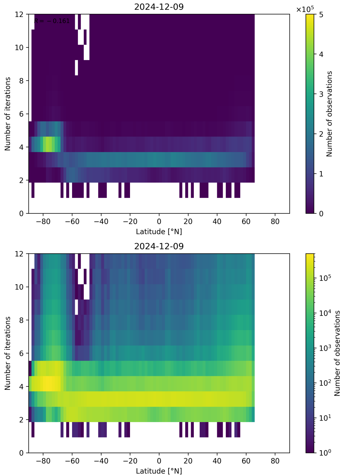
Figure 93: Scatter density plot of “Latitude” against “Number of iterations” for 2024-12-08 to 2024-12-10.
