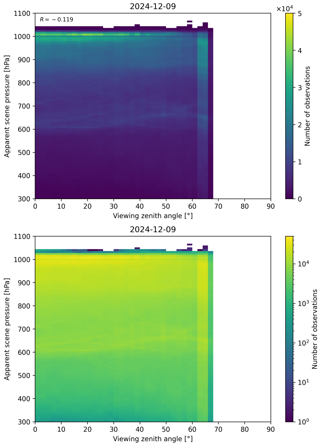
Figure 118: Scatter density plot of “Viewing zenith angle” against “Apparent scene pressure” for 2024-12-08 to 2024-12-10.
