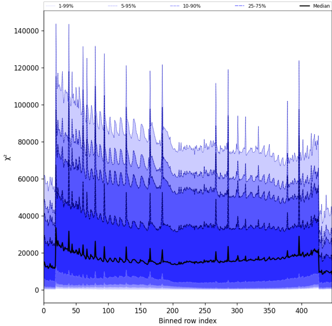
Figure 55: Along track statistics of “ \chi^2 ” for 2024-12-08 to 2024-12-10
