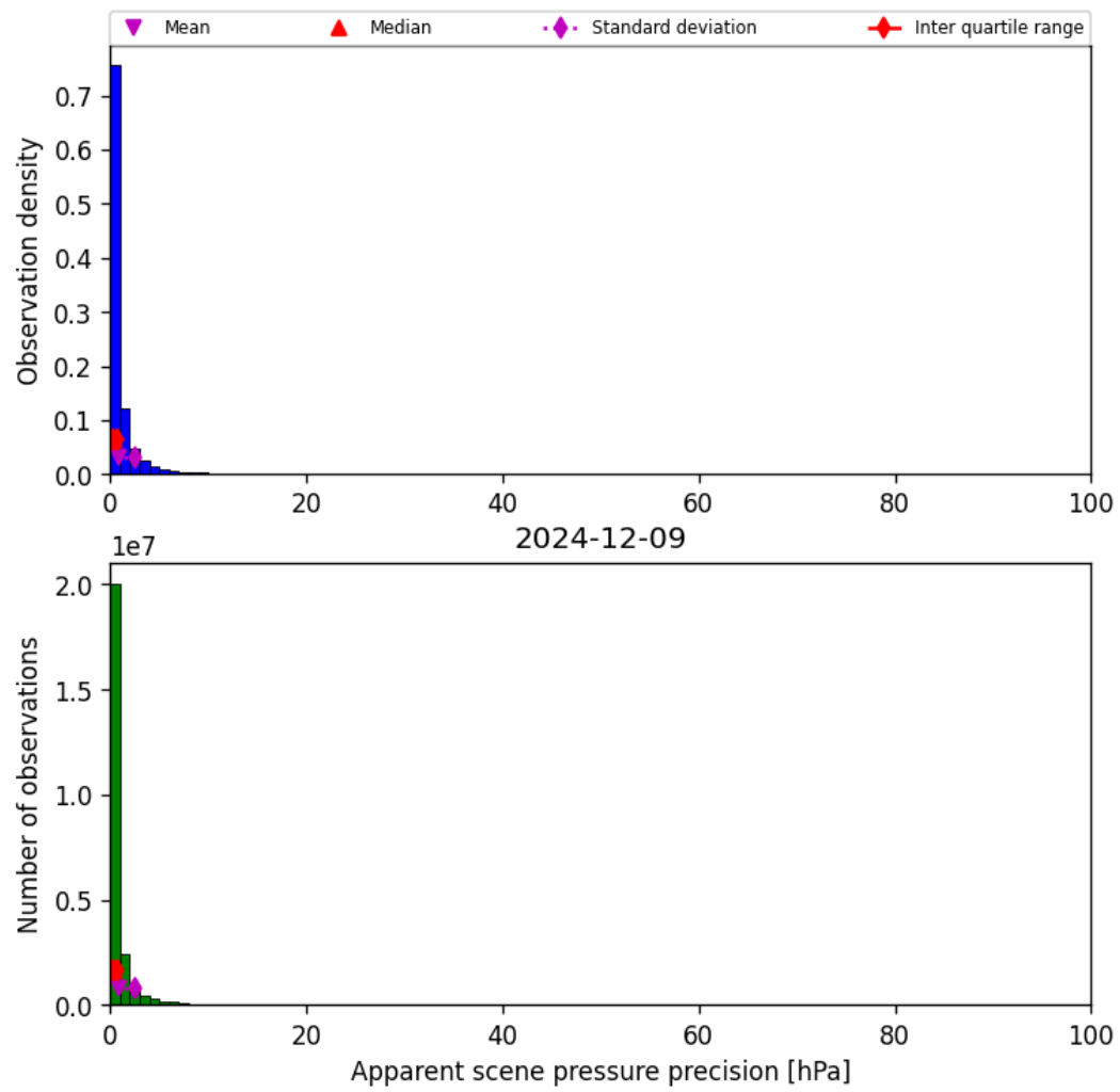
Figure 37: Histogram of “Apparent scene pressure precision” for 2024-12-08 to 2024-12-10
