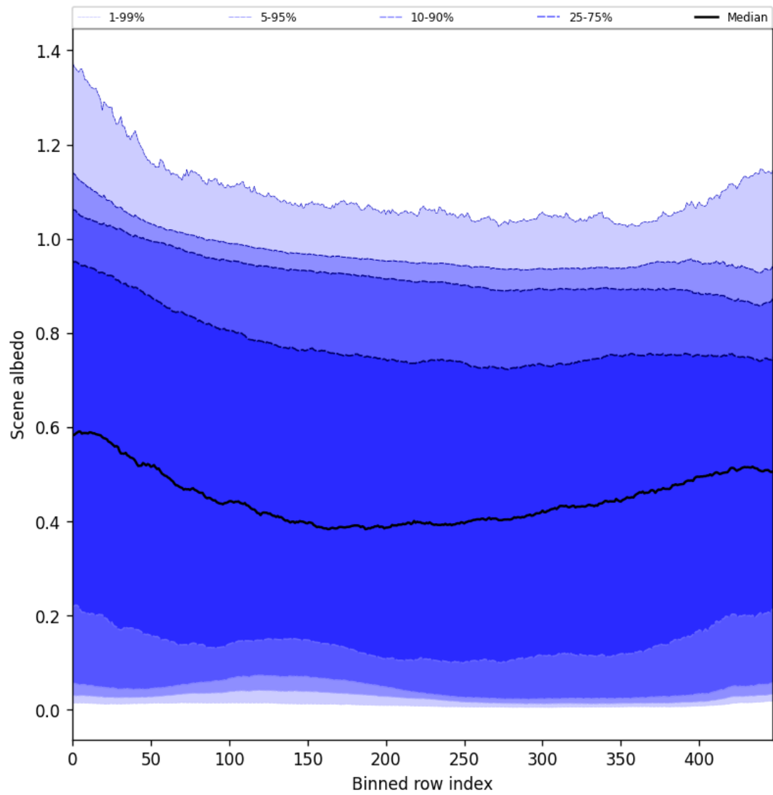
Figure 51: Along track statistics of “Scene albedo” for 2024-12-08 to 2024-12-10
