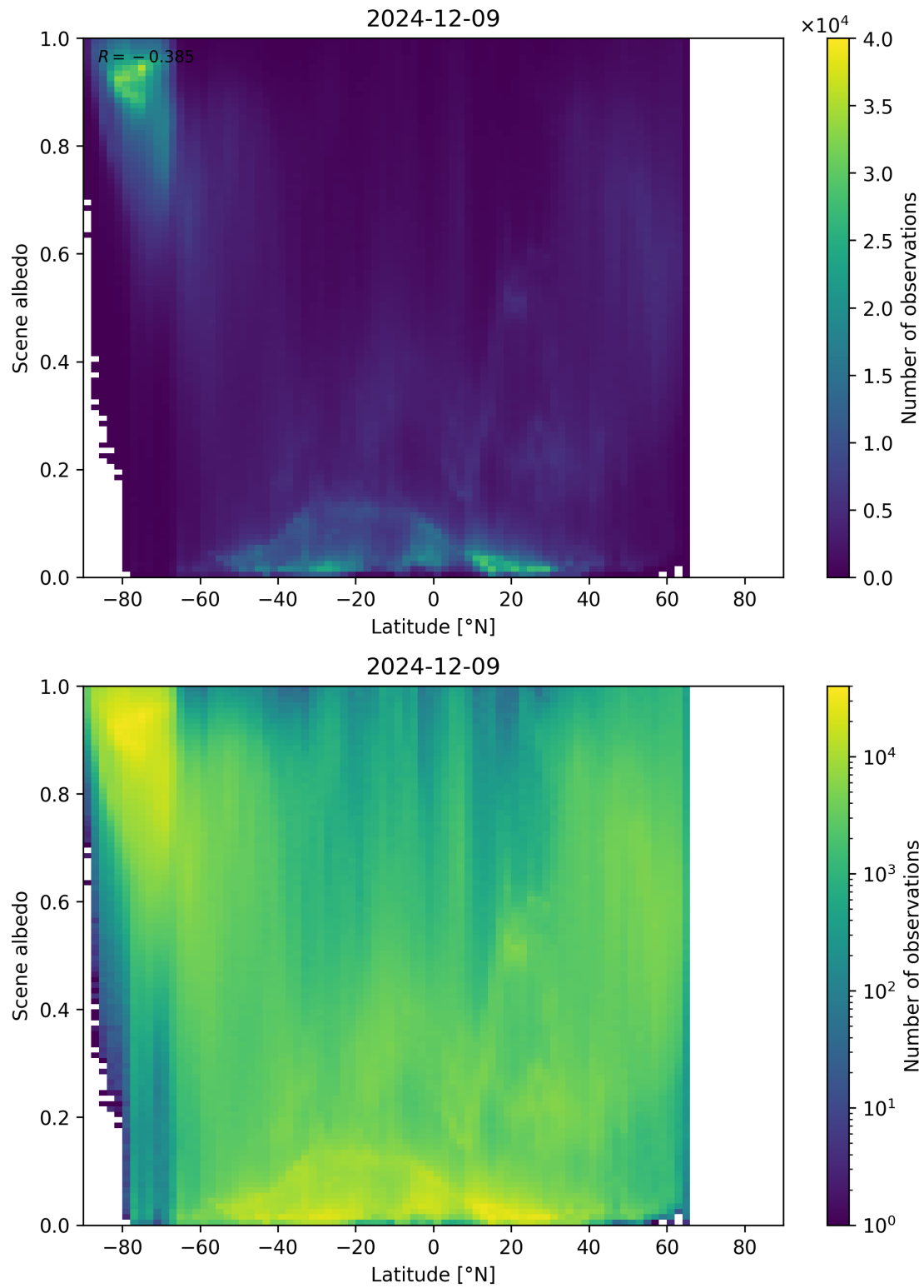
Figure 95: Scatter density plot of “Latitude” against “Scene albedo” for 2024-12-08 to 2024-12-10.
