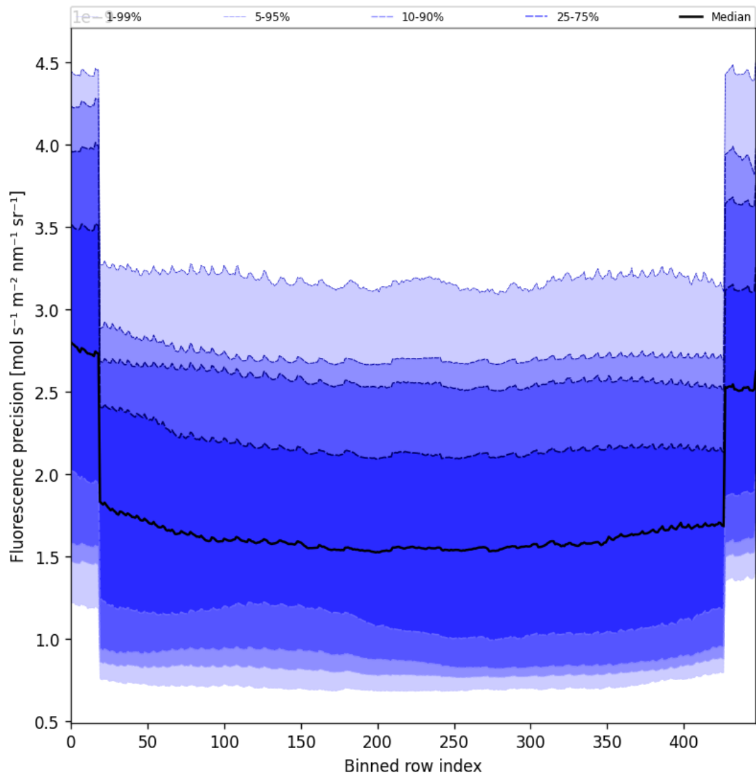
Figure 58: Along track statistics of “Fluorescence precision” for 2024-12-08 to 2024-12-10
