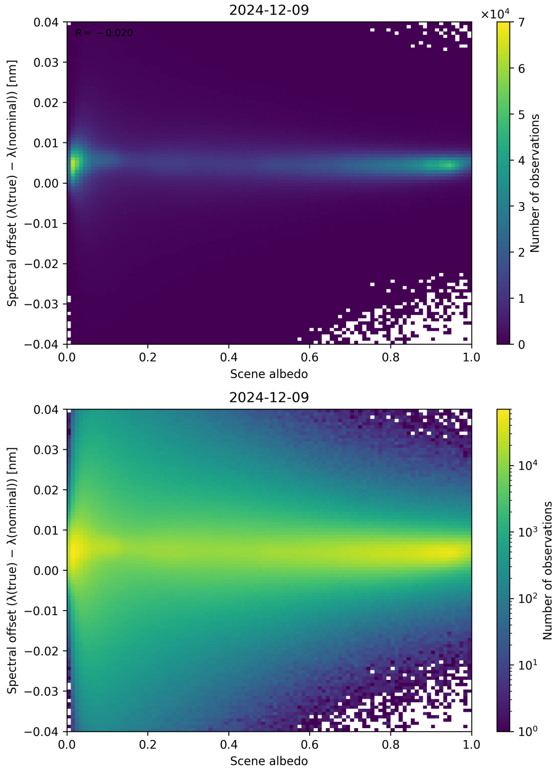
Figure 107: Scatter density plot of “Scene albedo” against “Spectral offset ( \lambda_{\text{true}} - \lambda_{\text{nominal}} )” for 2024-12-08 to 2024-12-10.
