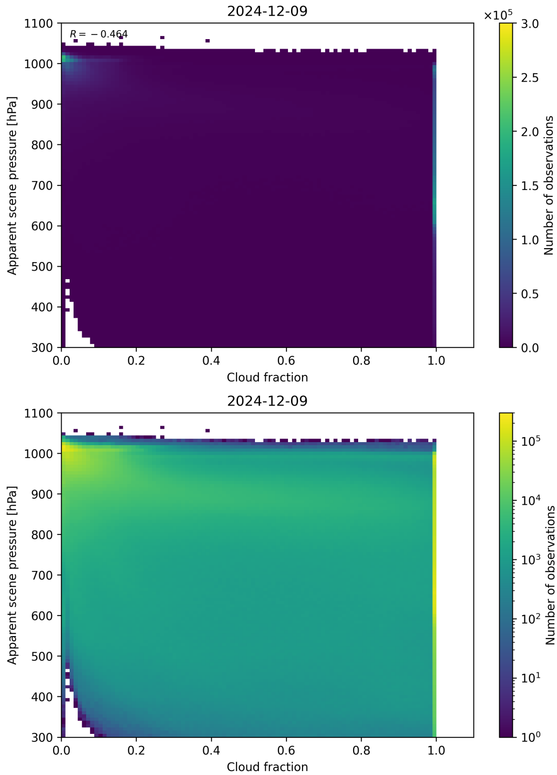
Figure 70: Scatter density plot of “Cloud fraction” against “Apparent scene pressure” for 2024-12-08 to 2024-12-10.
