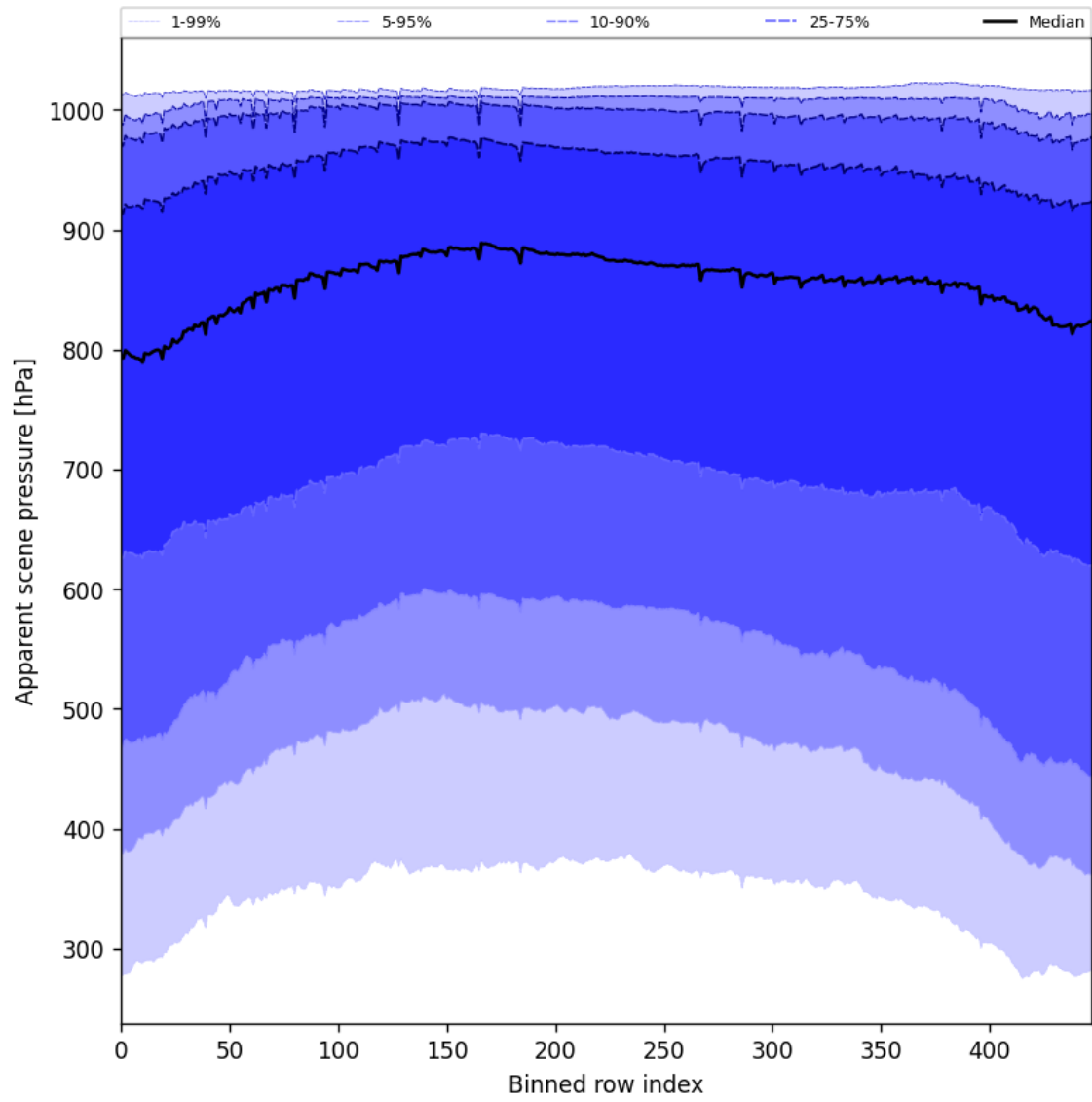
Figure 53: Along track statistics of "Apparent scene pressure" for 2024-12-08 to 2024-12-10
