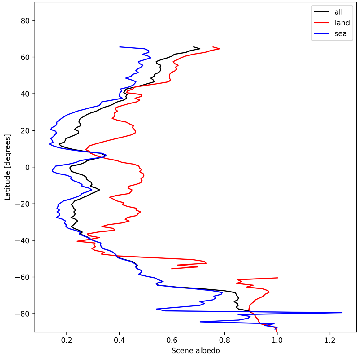
Figure 17: Zonal average of “Scene albedo” for 2024-12-08 to 2024-12-10.
