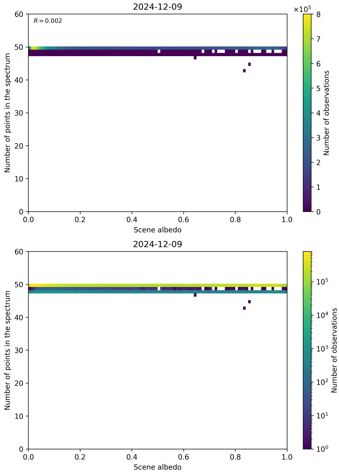
Figure 106: Scatter density plot of “Scene albedo” against “Number of points in the spectrum” for 2024-12-08 to 2024-12-10.
