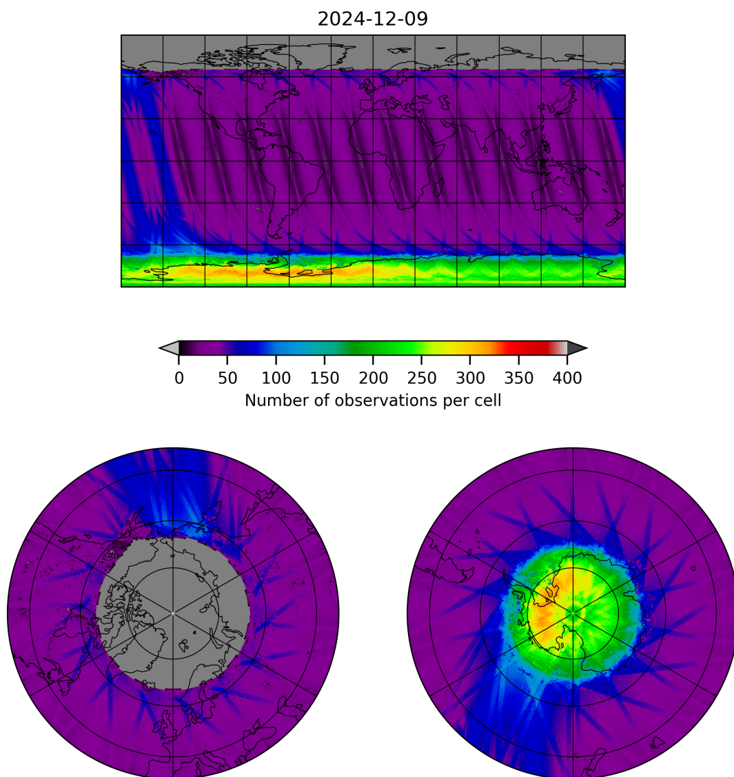
Figure 11: Map of the number of observations for 2024-12-08 to 2024-12-10
