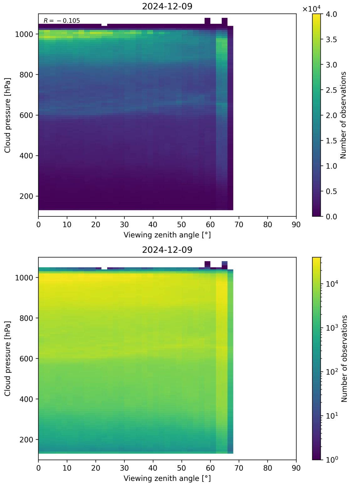
Figure 121: Scatter density plot of “Viewing zenith angle” against “Cloud pressure” for 2024-12-08 to 2024-12-10.
