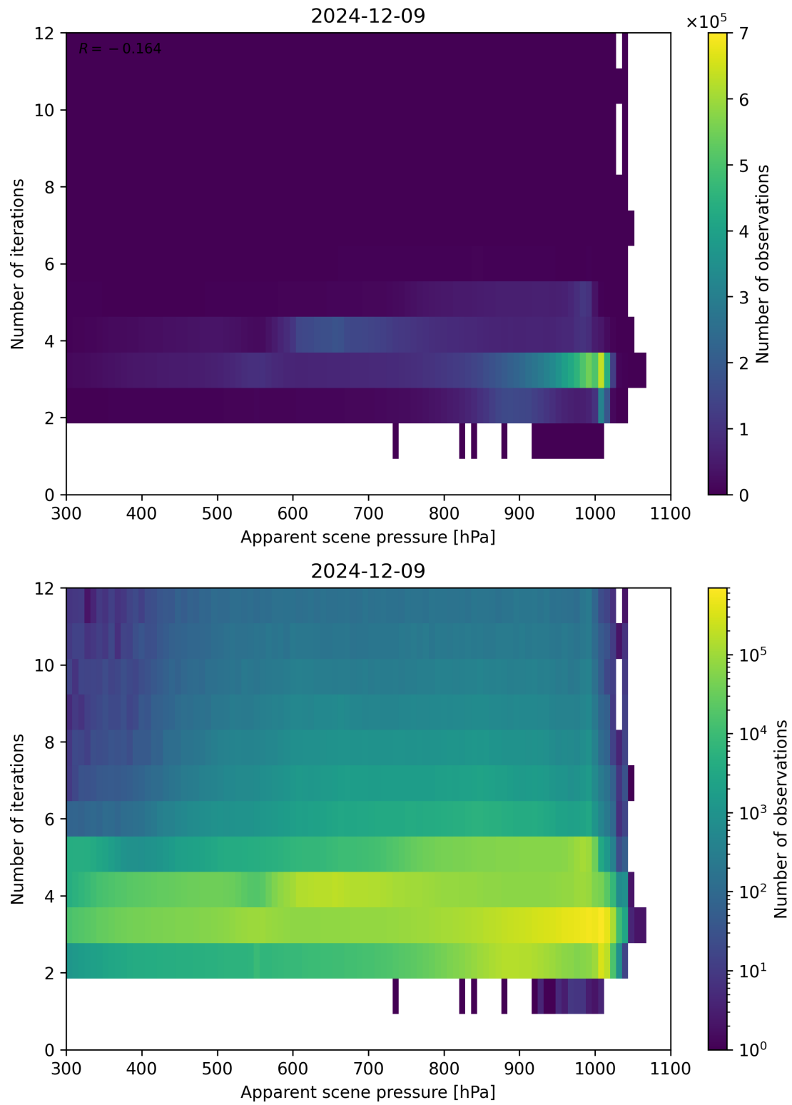
Figure 65: Scatter density plot of “Apparent scene pressure” against “Number of iterations” for 2024-12-08 to 2024-12-10.
