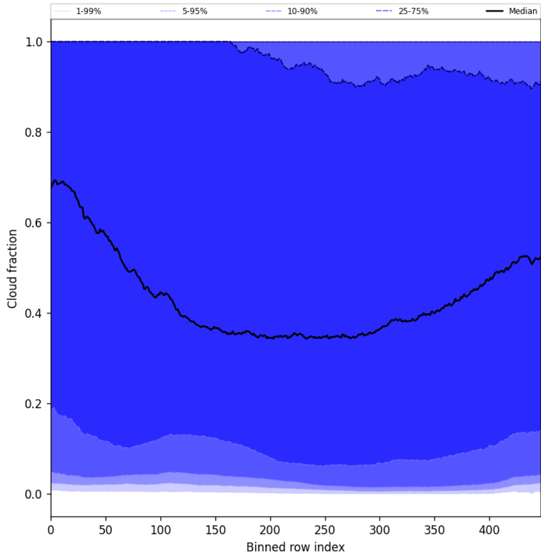
Figure 49: Along track statistics of “Cloud fraction” for 2024-12-08 to 2024-12-10
