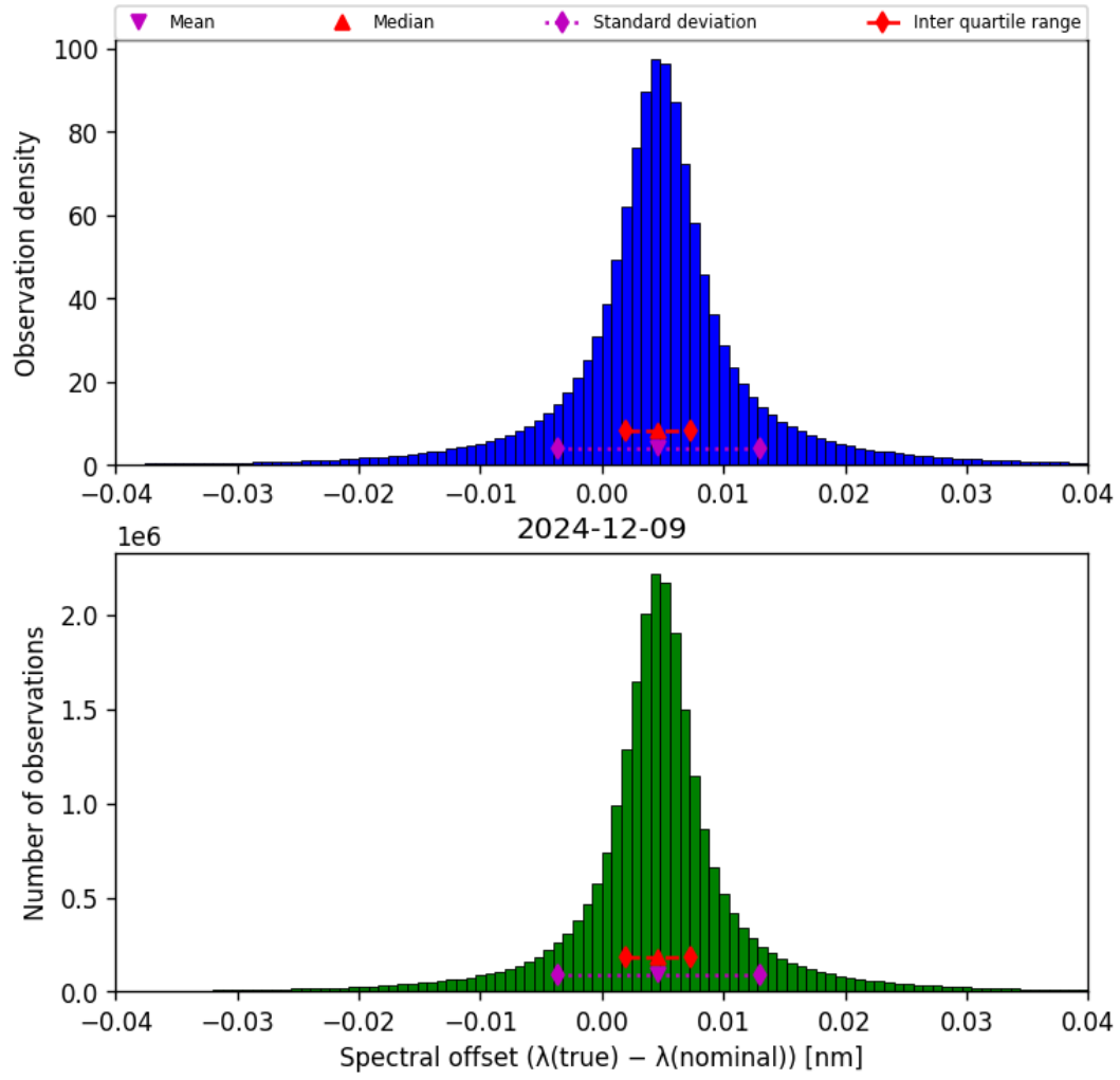
Figure 45: Histogram of “Spectral offset ( \lambda_{\text{true}} - \lambda_{\text{nominal}} )” for 2024-12-08 to 2024-12-10
