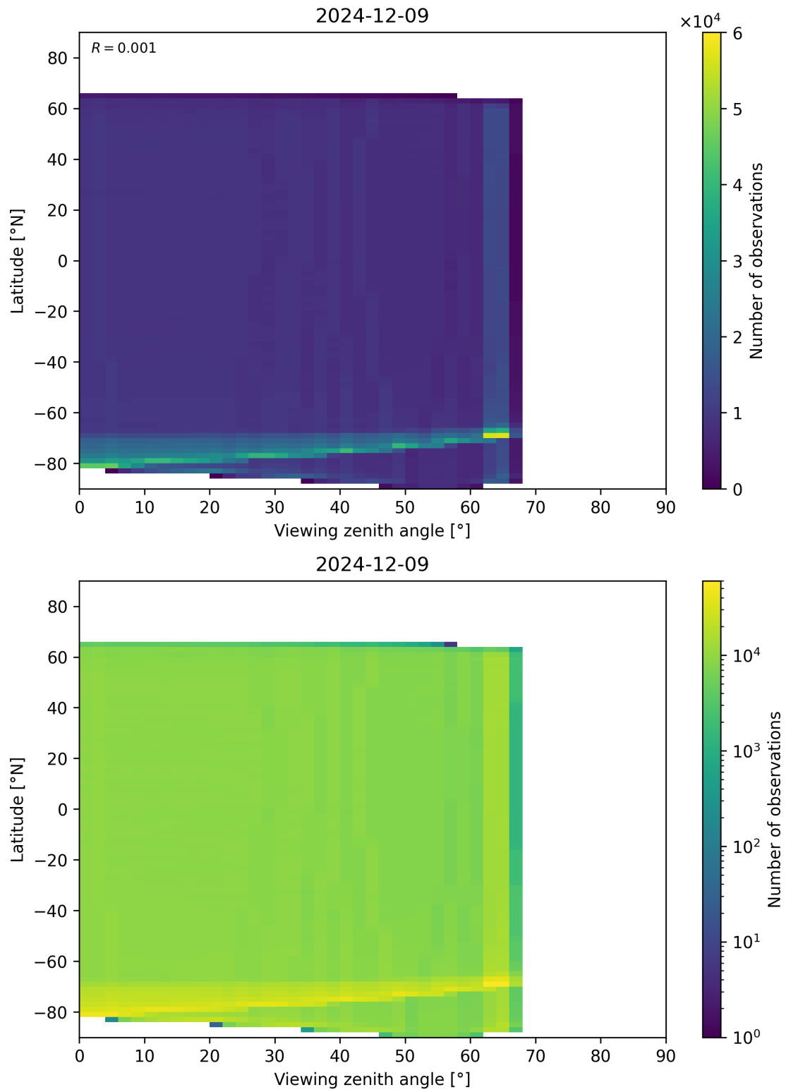
Figure 123: Scatter density plot of “Viewing zenith angle” against “Latitude” for 2024-12-08 to 2024-12-10.
