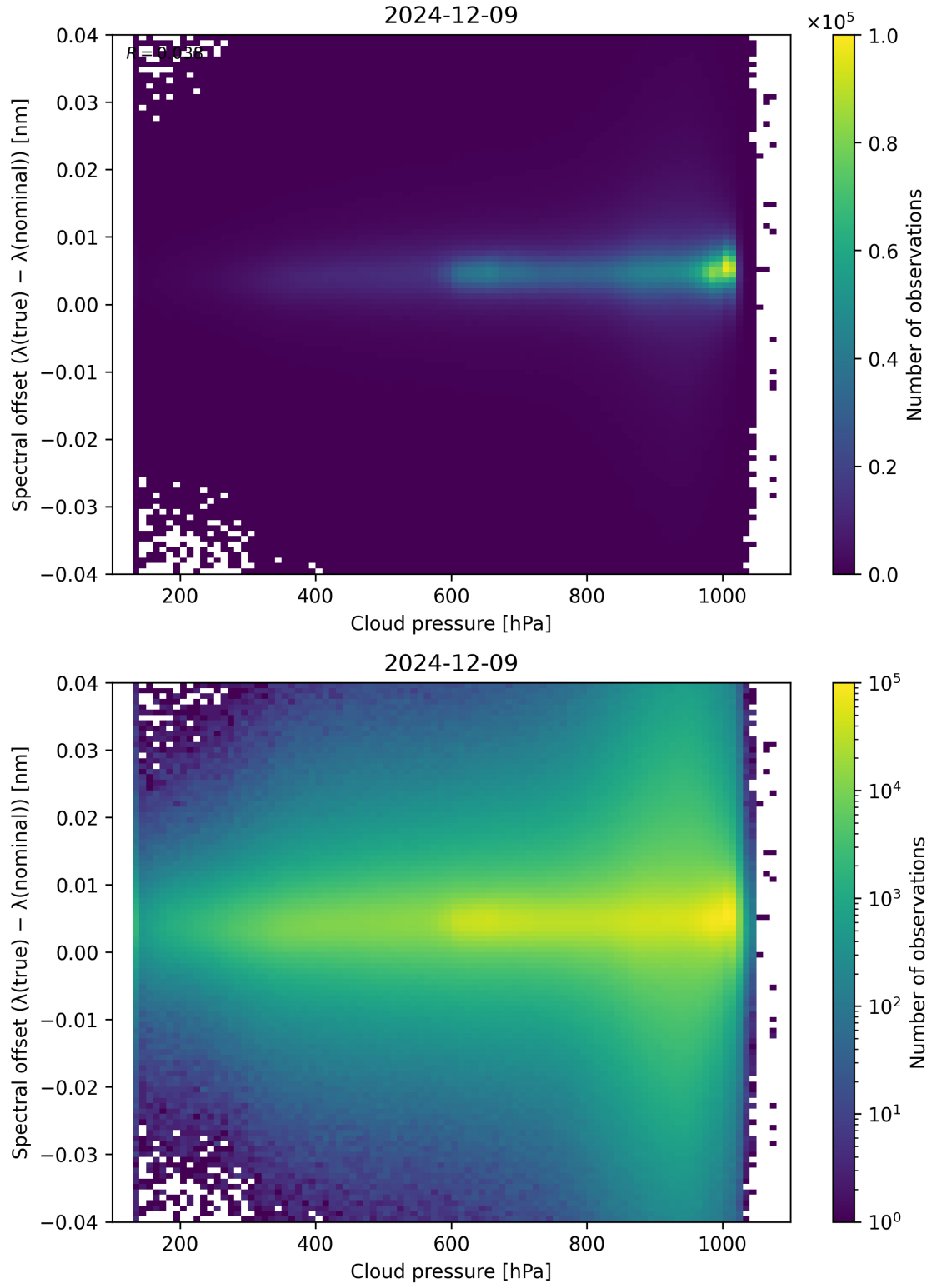
Figure 84: Scatter density plot of “Cloud pressure” against “Spectral offset ( \lambda_{\text{true}} - \lambda_{\text{nominal}} )” for 2024-12-08 to 2024-12-10.
