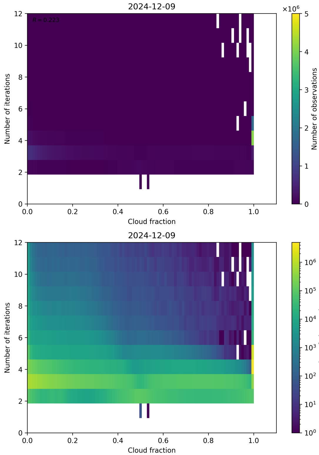
Figure 73: Scatter density plot of “Cloud fraction” against “Number of iterations” for 2024-12-08 to 2024-12-10.
