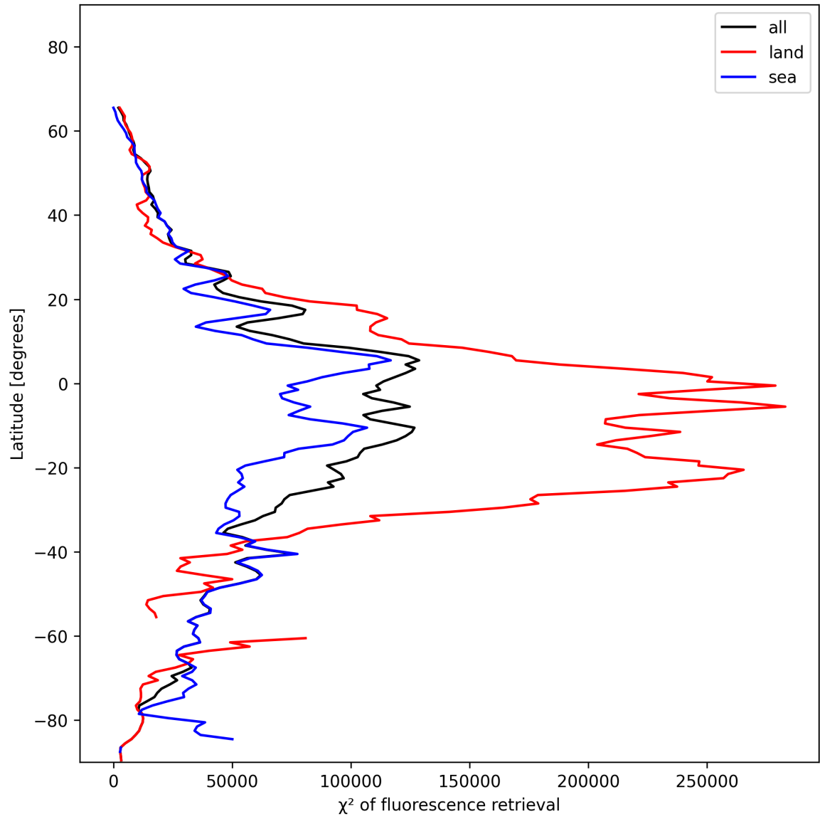
Figure 25: Zonal average of “ \chi^2 of fluorescence retrieval” for 2024-12-09 to 2024-12-11.
