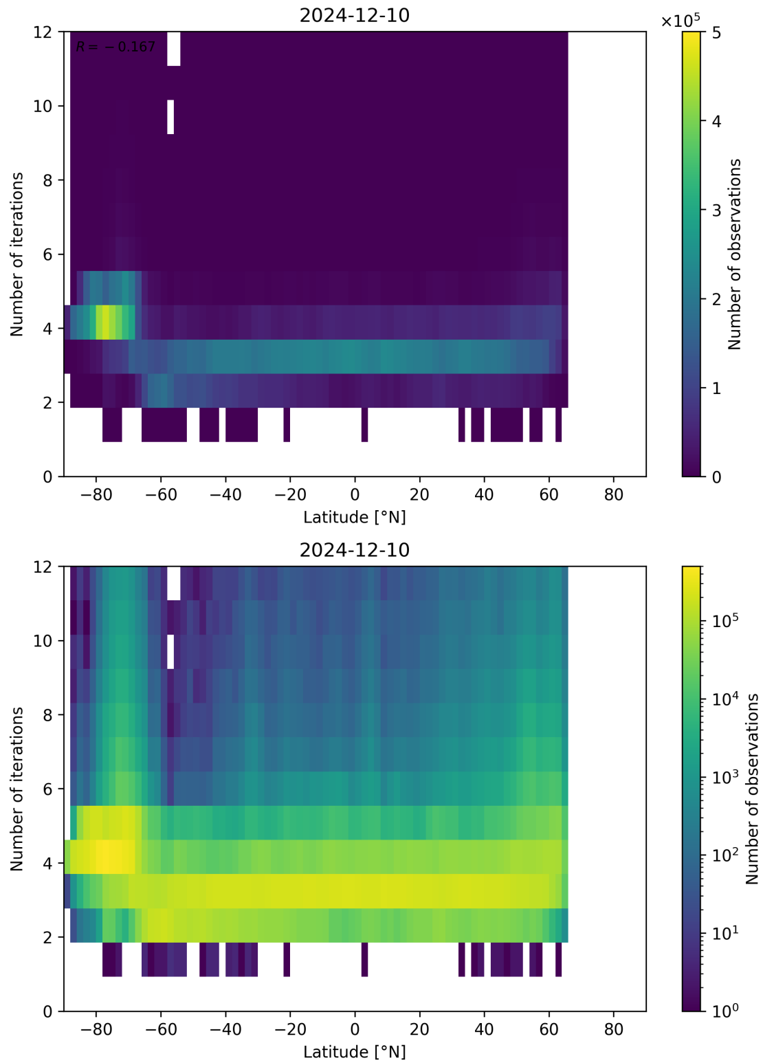
Figure 93: Scatter density plot of “Latitude” against “Number of iterations” for 2024-12-09 to 2024-12-11.
