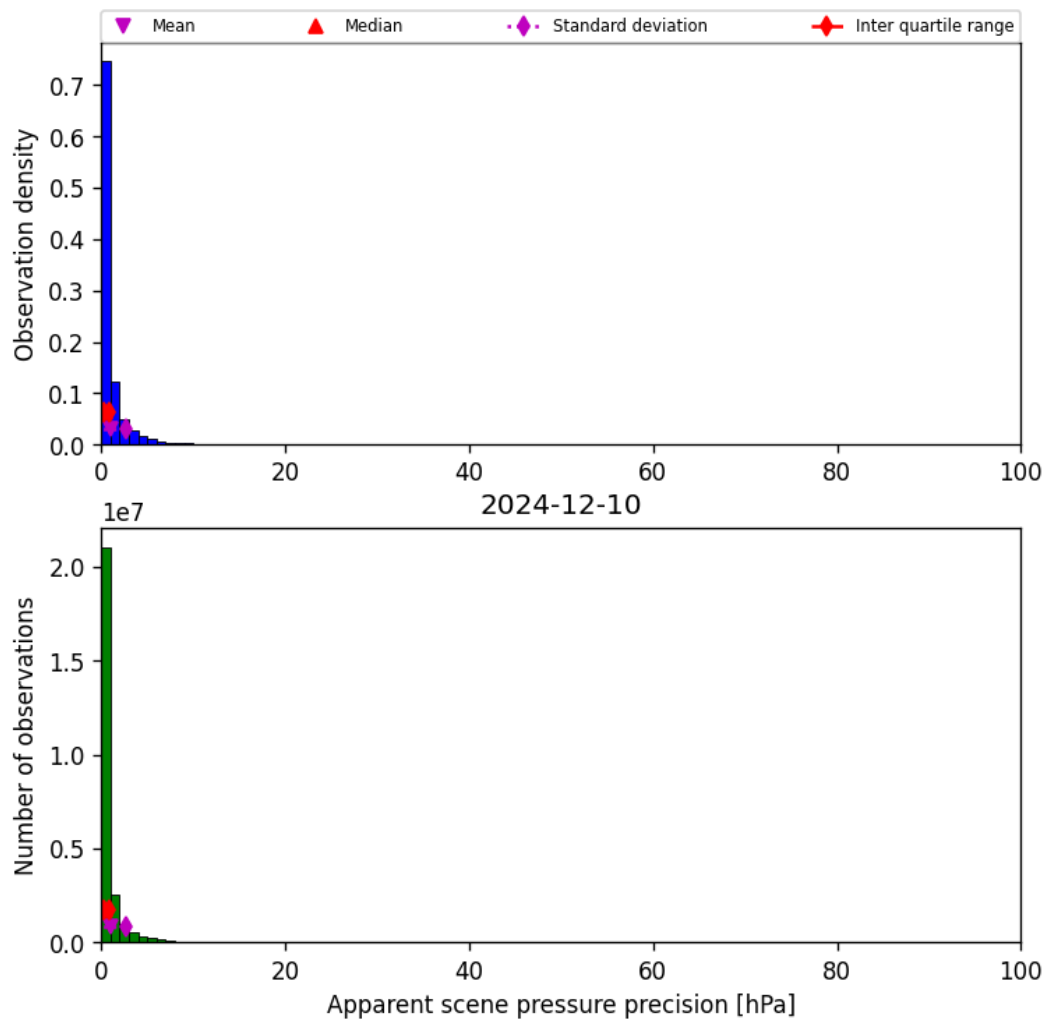
Figure 37: Histogram of “Apparent scene pressure precision” for 2024-12-09 to 2024-12-11
