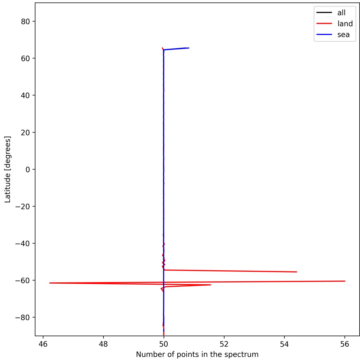
Figure 27: Zonal average of “Number of points in the spectrum” for 2024-12-09 to 2024-12-11.
