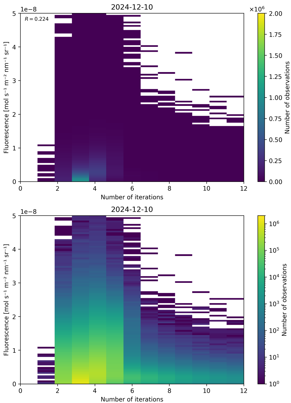
Figure 98: Scatter density plot of “Number of iterations” against “Fluorescence” for 2024-12-09 to 2024-12-11.
