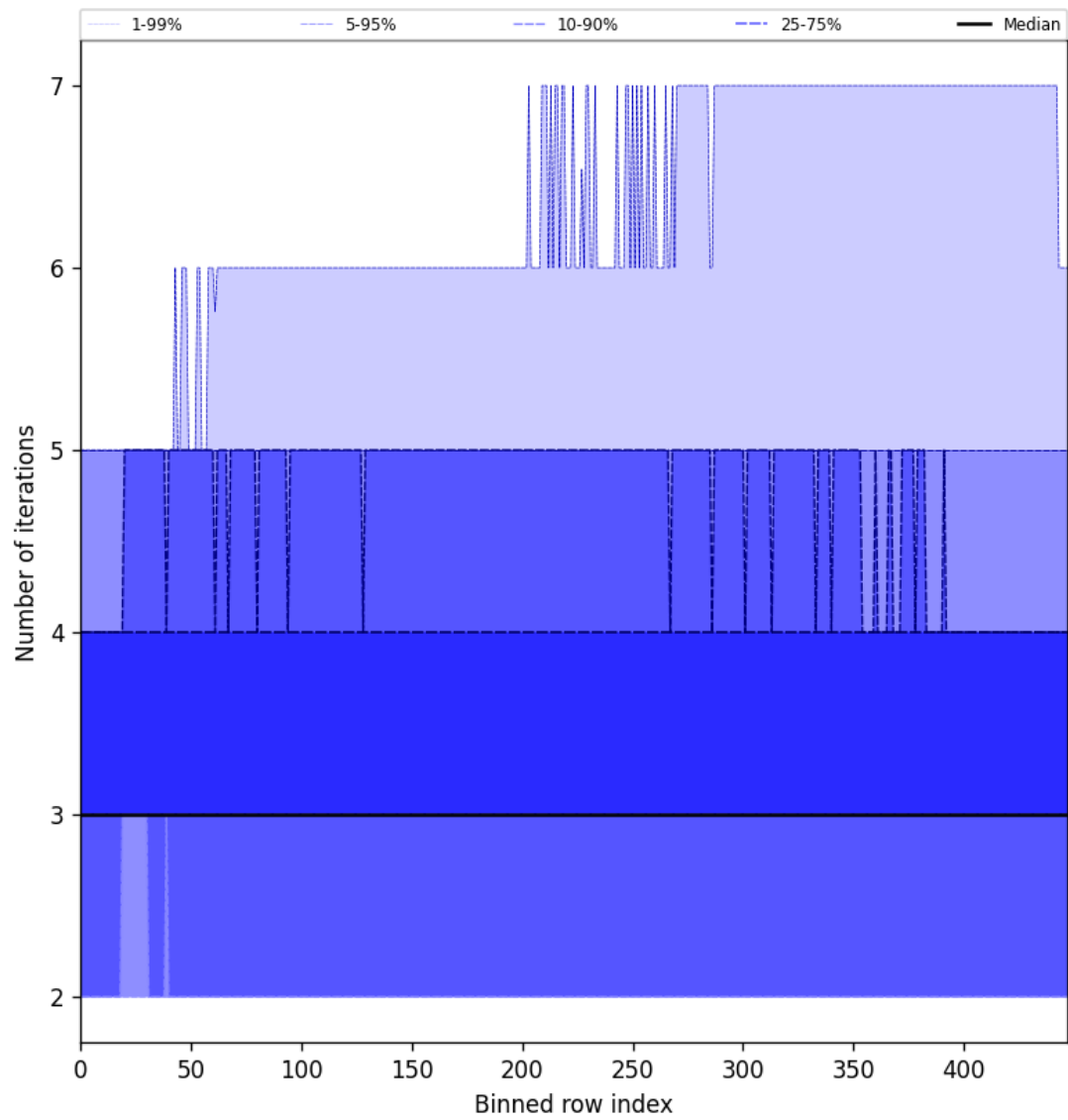
Figure 56: Along track statistics of “Number of iterations” for 2024-12-09 to 2024-12-11
