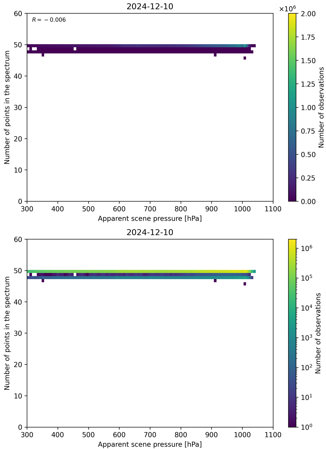
Figure 66: Scatter density plot of “Apparent scene pressure” against “Number of points in the spectrum” for 2024-12-09 to 2024-12-11.
