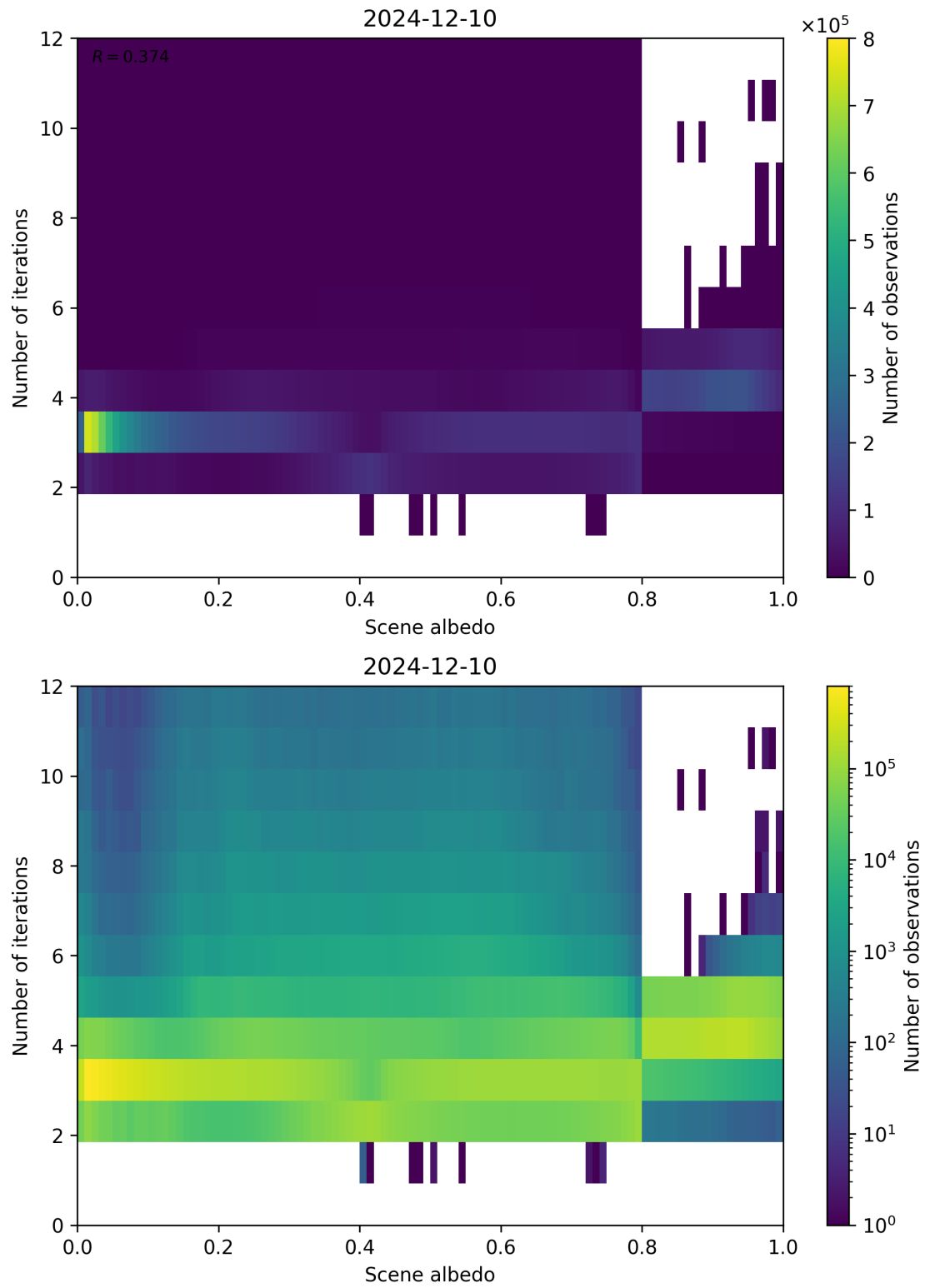
Figure 105: Scatter density plot of “Scene albedo” against “Number of iterations” for 2024-12-09 to 2024-12-11.
