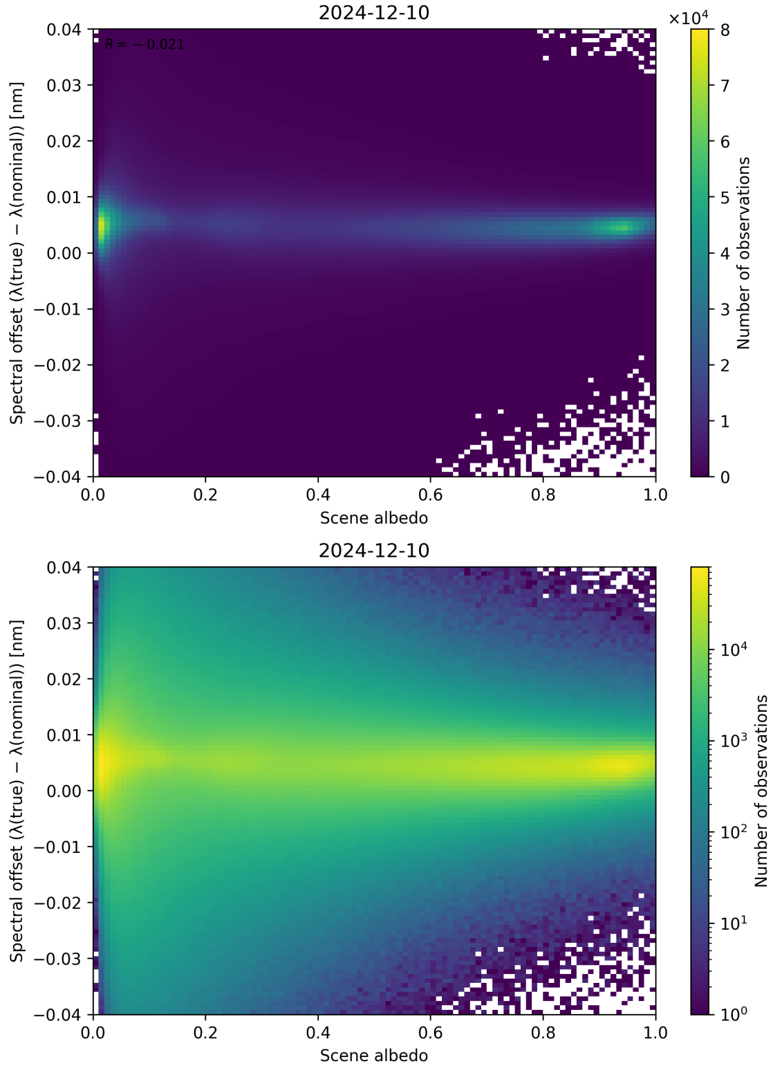
Figure 107: Scatter density plot of “Scene albedo” against “Spectral offset ( \lambda_{\text{true}} - \lambda_{\text{nominal}} )” for 2024-12-09 to 2024-12-11.
