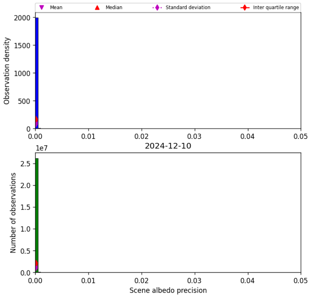
Figure 35: Histogram of “Scene albedo precision” for 2024-12-09 to 2024-12-11
