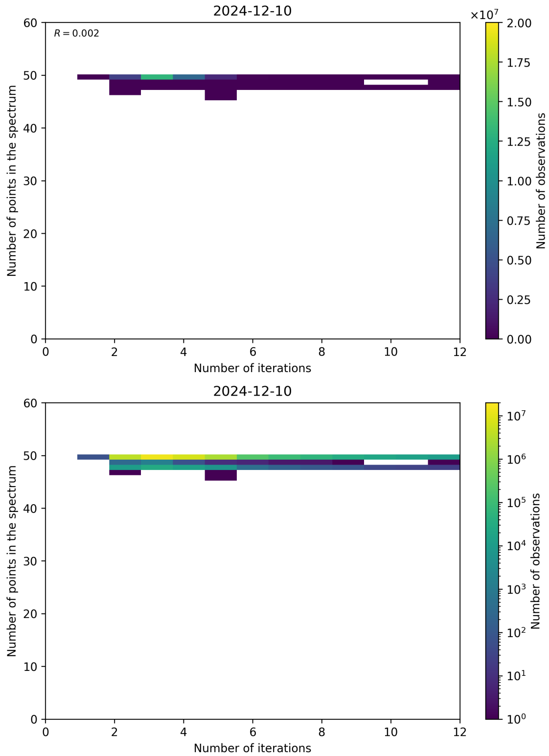
Figure 99: Scatter density plot of “Number of iterations” against “Number of points in the spectrum” for 2024-12-09 to 2024-12-11.
