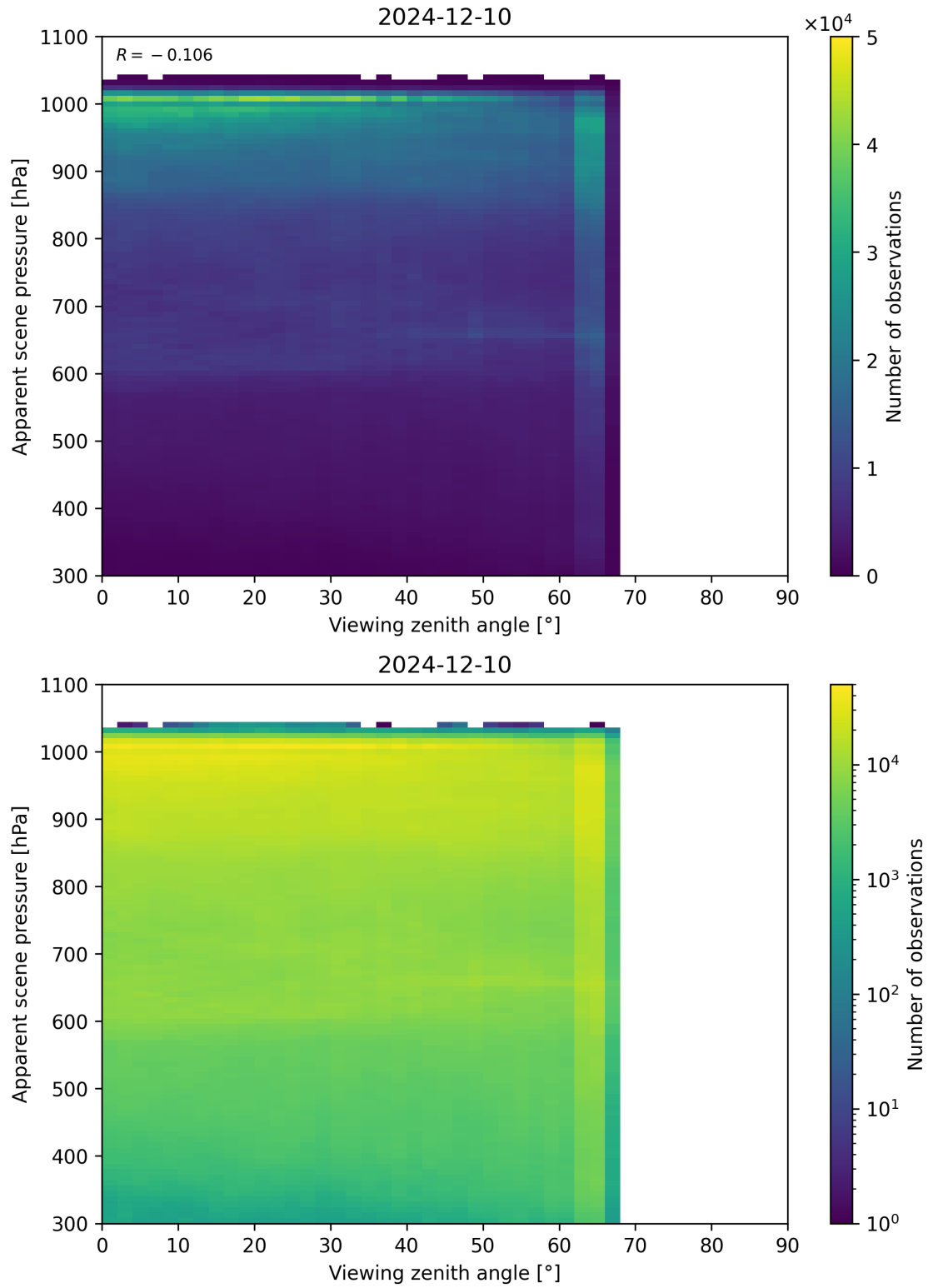
Figure 118: Scatter density plot of “Viewing zenith angle” against “Apparent scene pressure” for 2024-12-09 to 2024-12-11.
