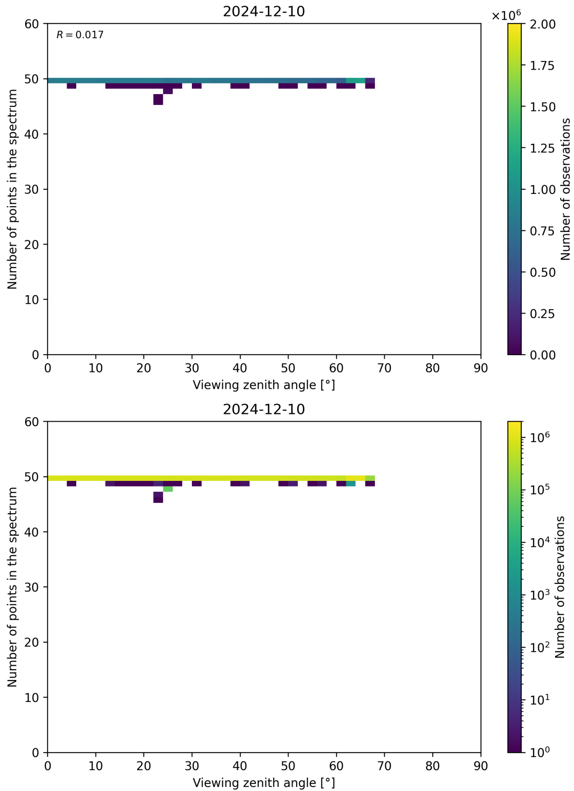
Figure 125: Scatter density plot of “Viewing zenith angle” against “Number of points in the spectrum” for 2024-12-09 to 2024-12-11.
