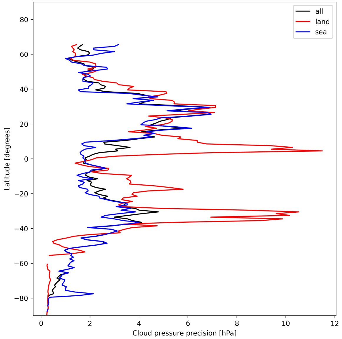
Figure 14: Zonal average of “Cloud pressure precision” for 2024-12-09 to 2024-12-11.
