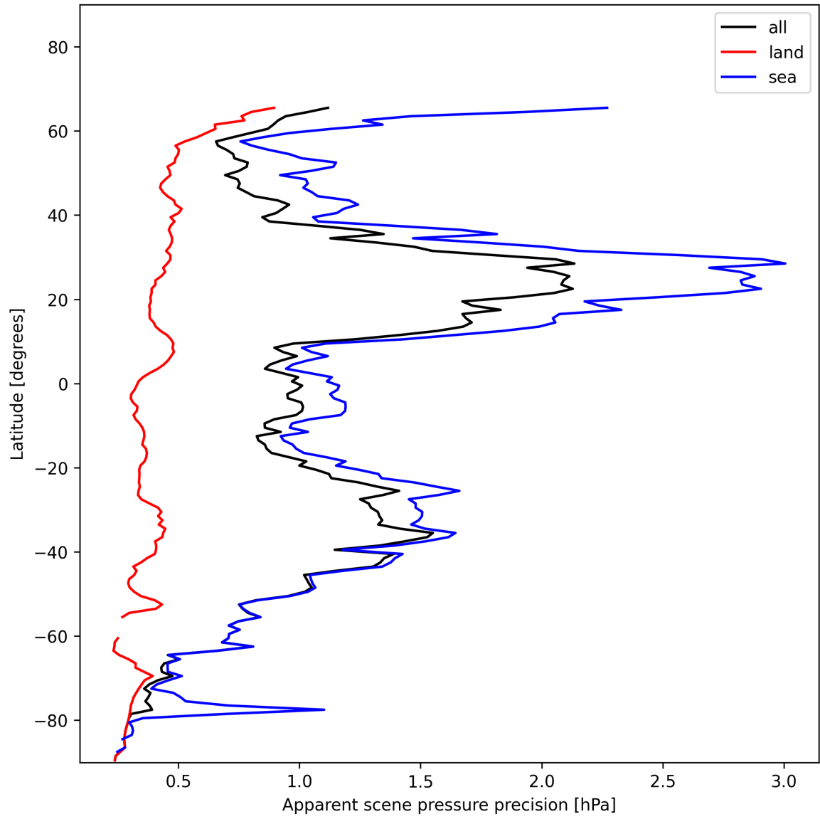
Figure 20: Zonal average of “Apparent scene pressure precision” for 2024-12-09 to 2024-12-11.
