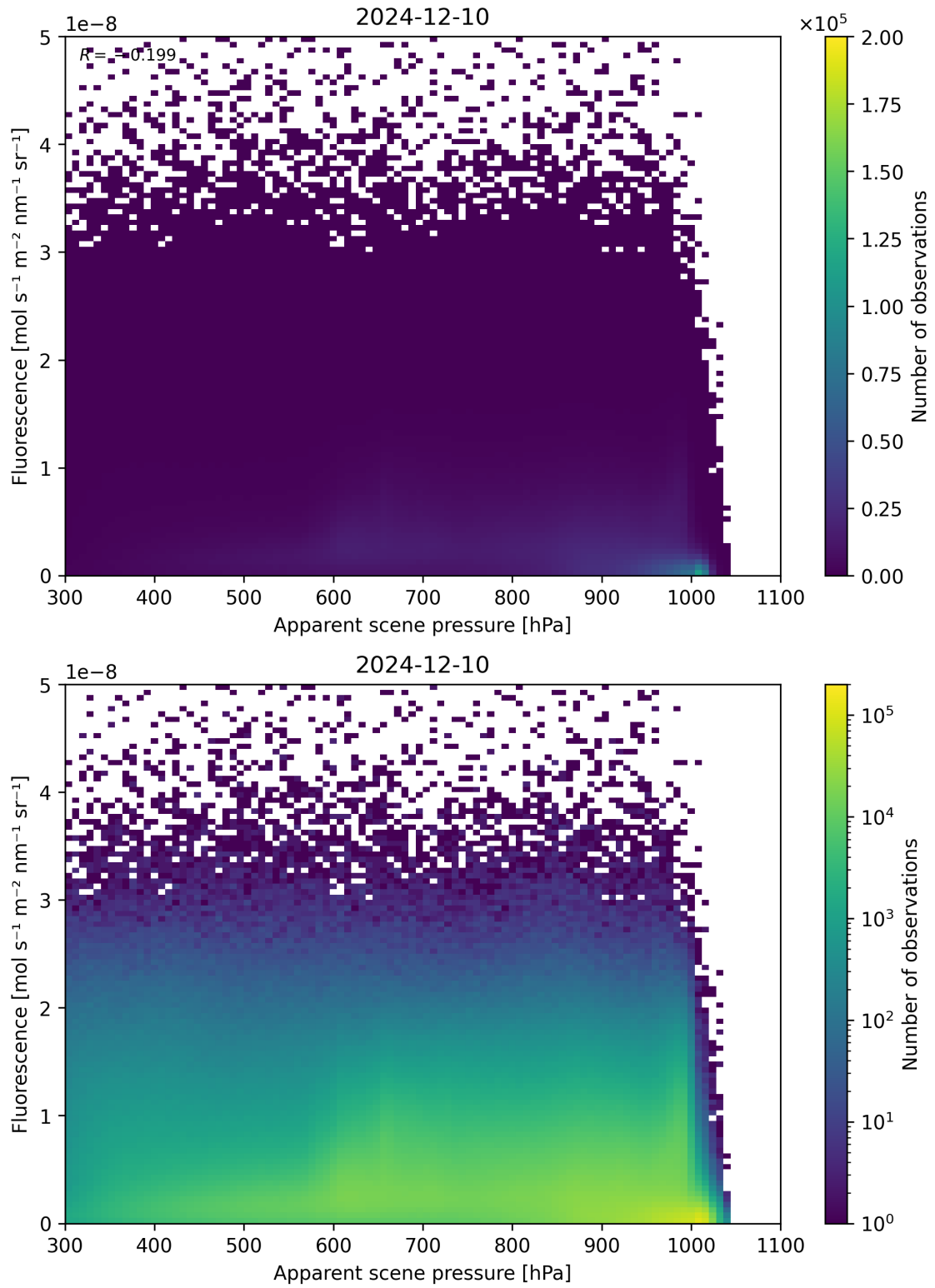
Figure 64: Scatter density plot of “Apparent scene pressure” against “Fluorescence” for 2024-12-09 to 2024-12-11.
