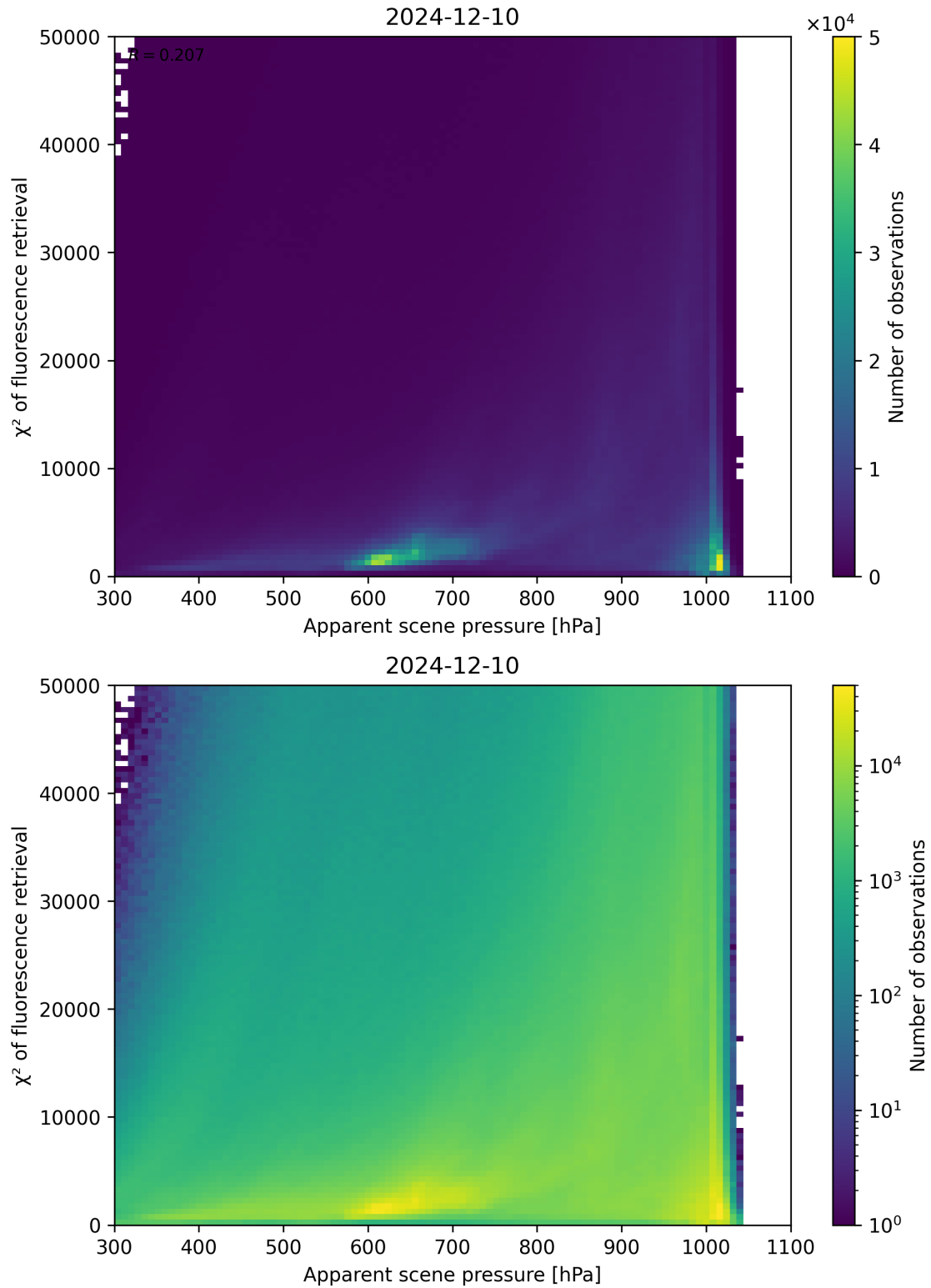
Figure 63: Scatter density plot of “Apparent scene pressure” against “ \chi^2 of fluorescence retrieval” for 2024-12-09 to 2024-12-11.
