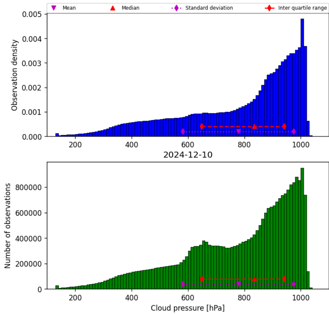
Figure 30: Histogram of “Cloud pressure” for 2024-12-09 to 2024-12-11
