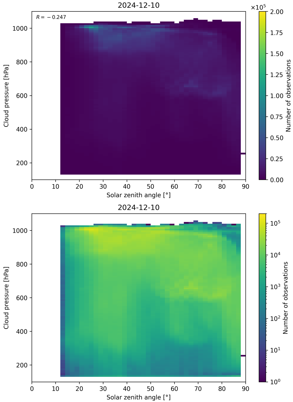
Figure 111: Scatter density plot of “Solar zenith angle” against “Cloud pressure” for 2024-12-09 to 2024-12-11.
