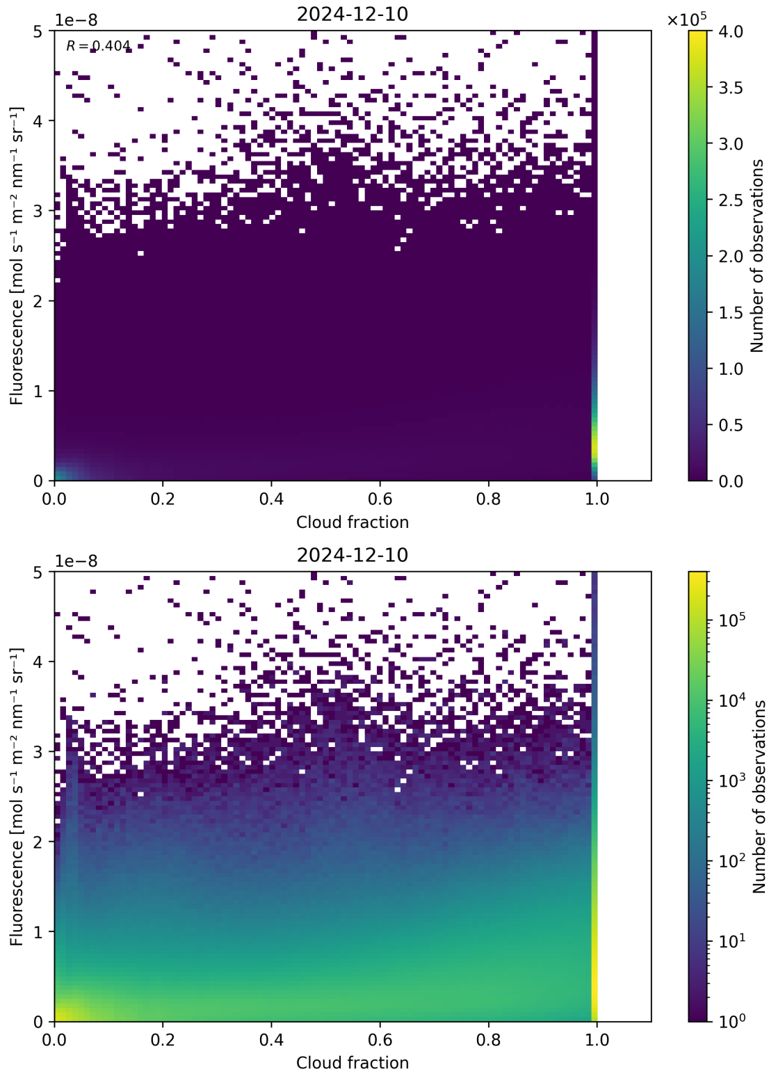
Figure 72: Scatter density plot of “Cloud fraction” against “Fluorescence” for 2024-12-09 to 2024-12-11.
