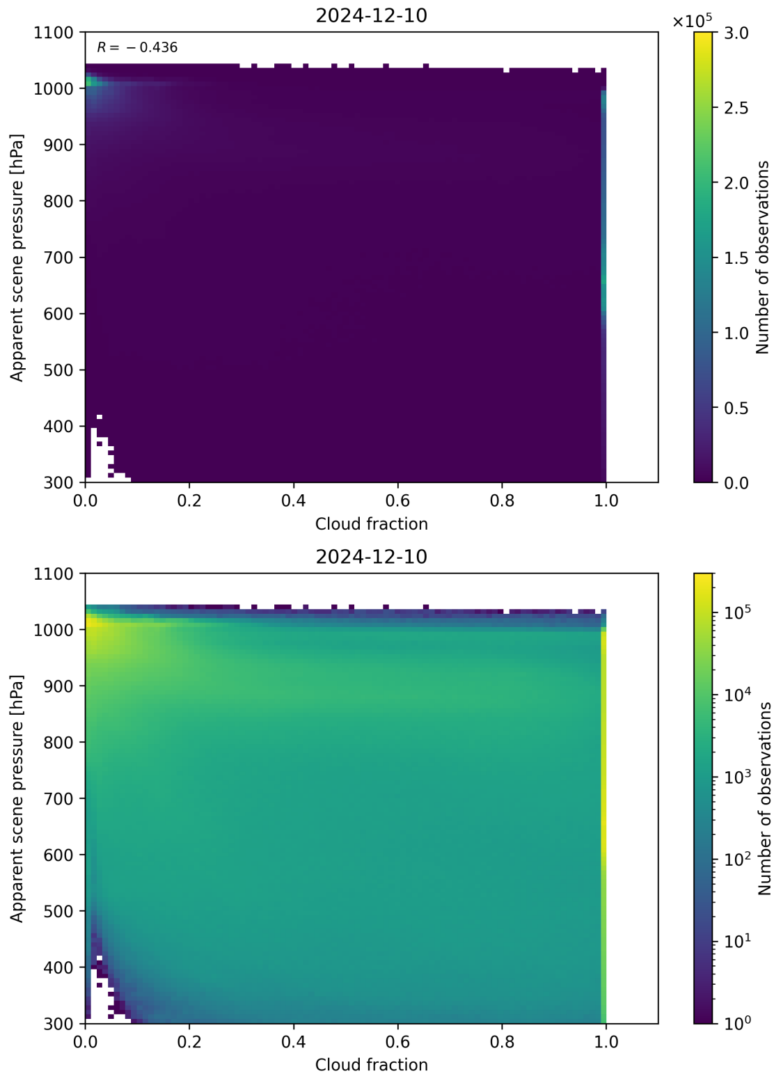
Figure 70: Scatter density plot of “Cloud fraction” against “Apparent scene pressure” for 2024-12-09 to 2024-12-11.
