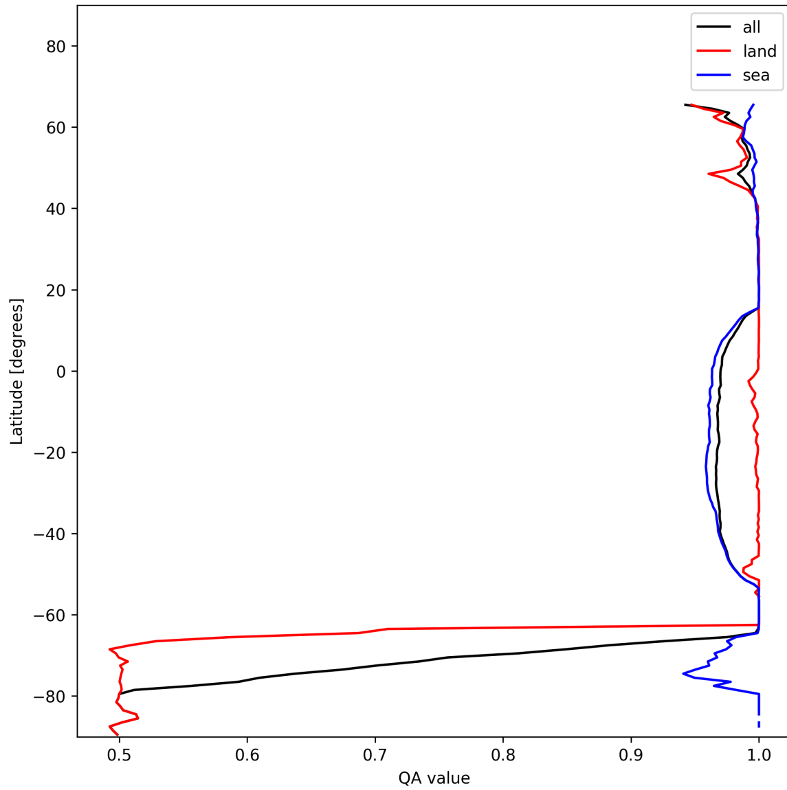
Figure 12: Zonal average of “QA value” for 2024-12-09 to 2024-12-11.
