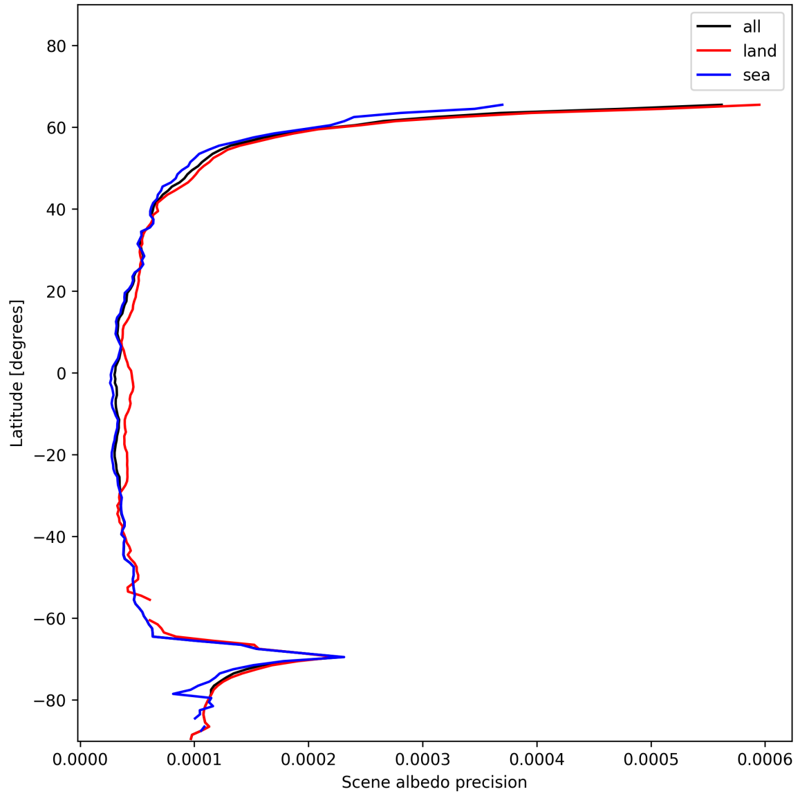
Figure 18: Zonal average of “Scene albedo precision” for 2024-12-09 to 2024-12-11.
