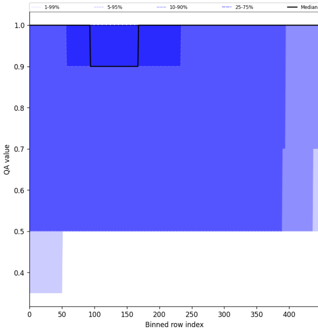
Figure 46: Along track statistics of “QA value” for 2024-12-09 to 2024-12-11
