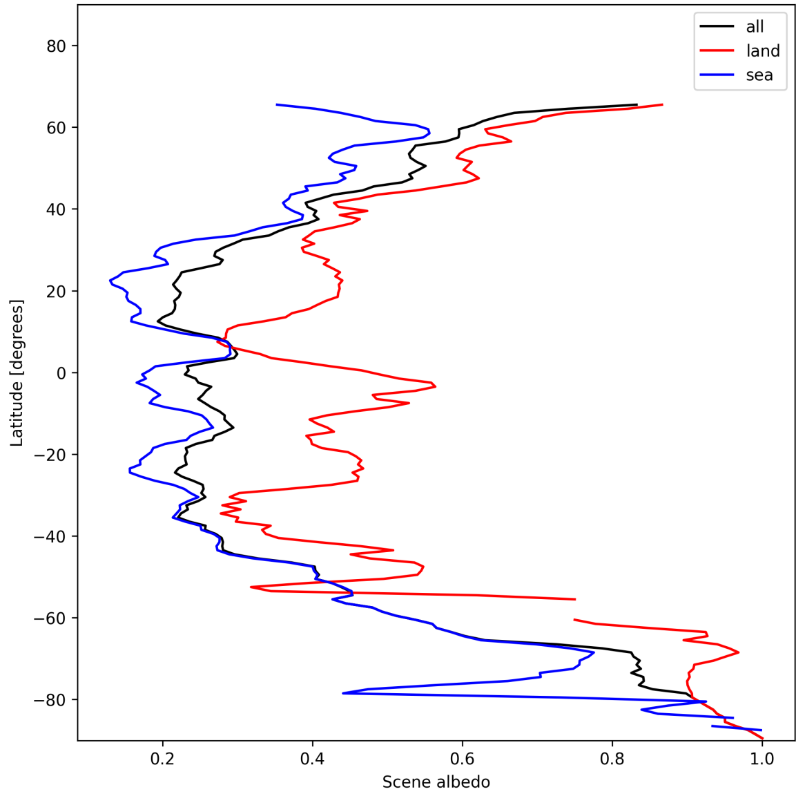
Figure 17: Zonal average of "Scene albedo" for 2024-12-09 to 2024-12-11.
