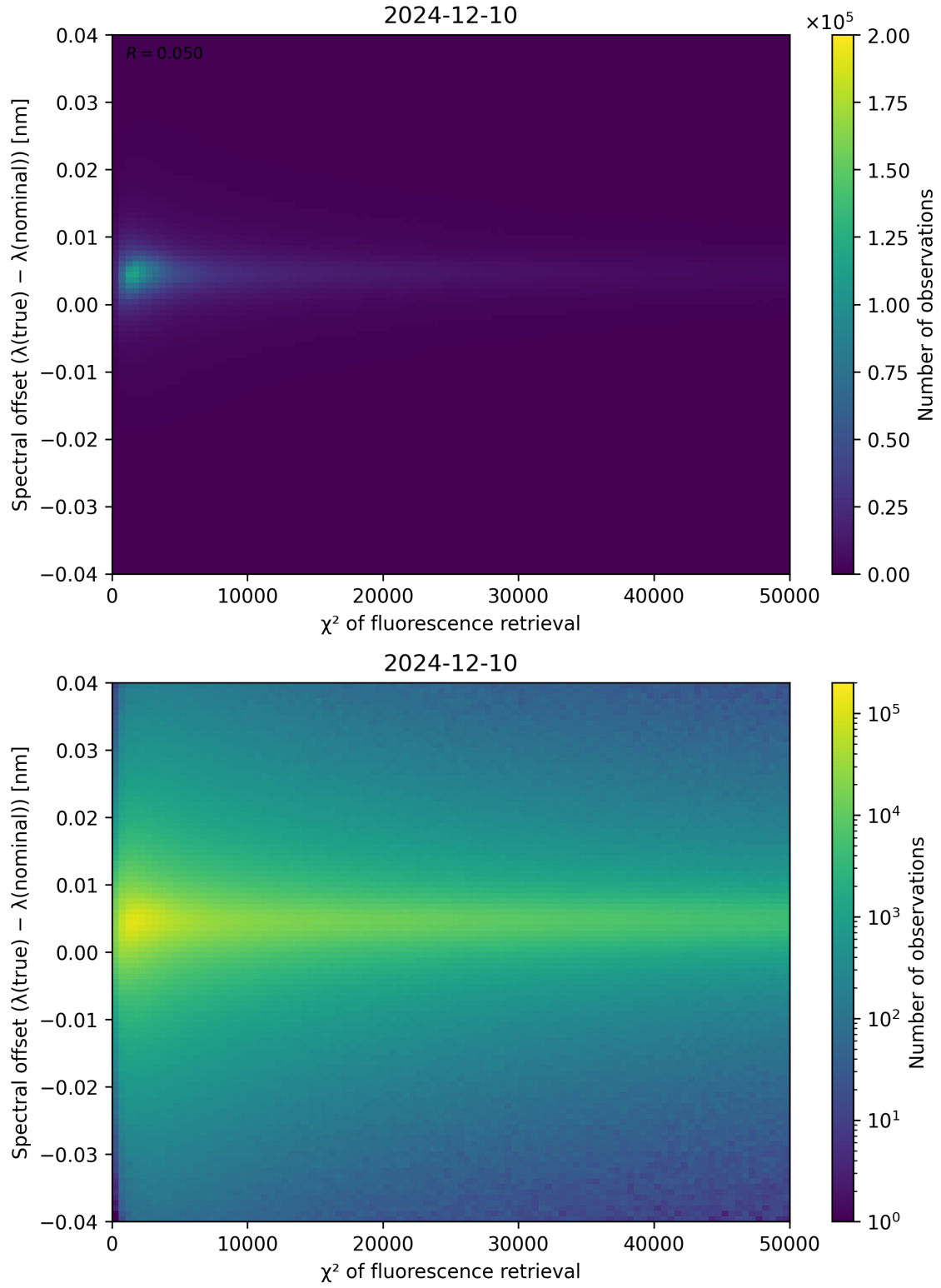
Figure 69: Scatter density plot of “ \chi^2 of fluorescence retrieval” against “Spectral offset ( \lambda_{\text{true}} - \lambda_{\text{nominal}} )” for 2024-12-09 to 2024-12-11.
