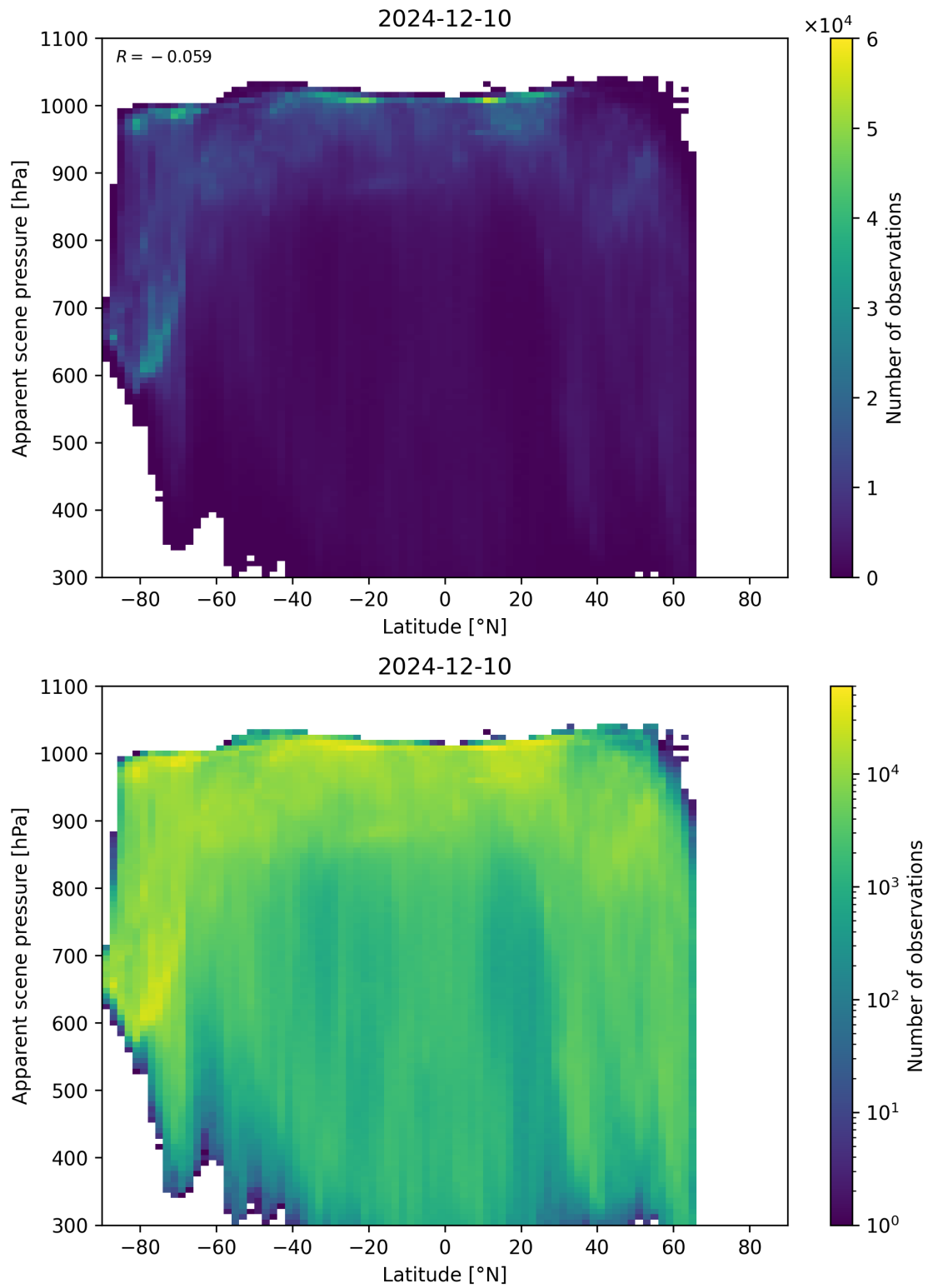
Figure 88: Scatter density plot of “Latitude” against “Apparent scene pressure” for 2024-12-09 to 2024-12-11.
