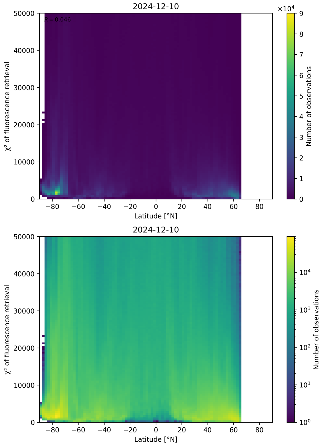
Figure 89: Scatter density plot of “Latitude” against “ \chi^2 of fluorescence retrieval” for 2024-12-09 to 2024-12-11.
