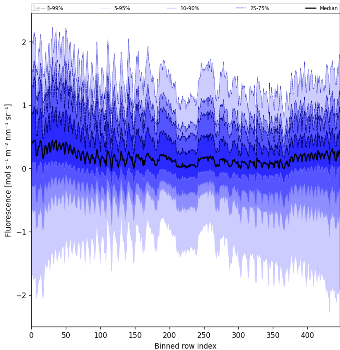
Figure 57: Along track statistics of “Fluorescence” for 2024-12-09 to 2024-12-11
