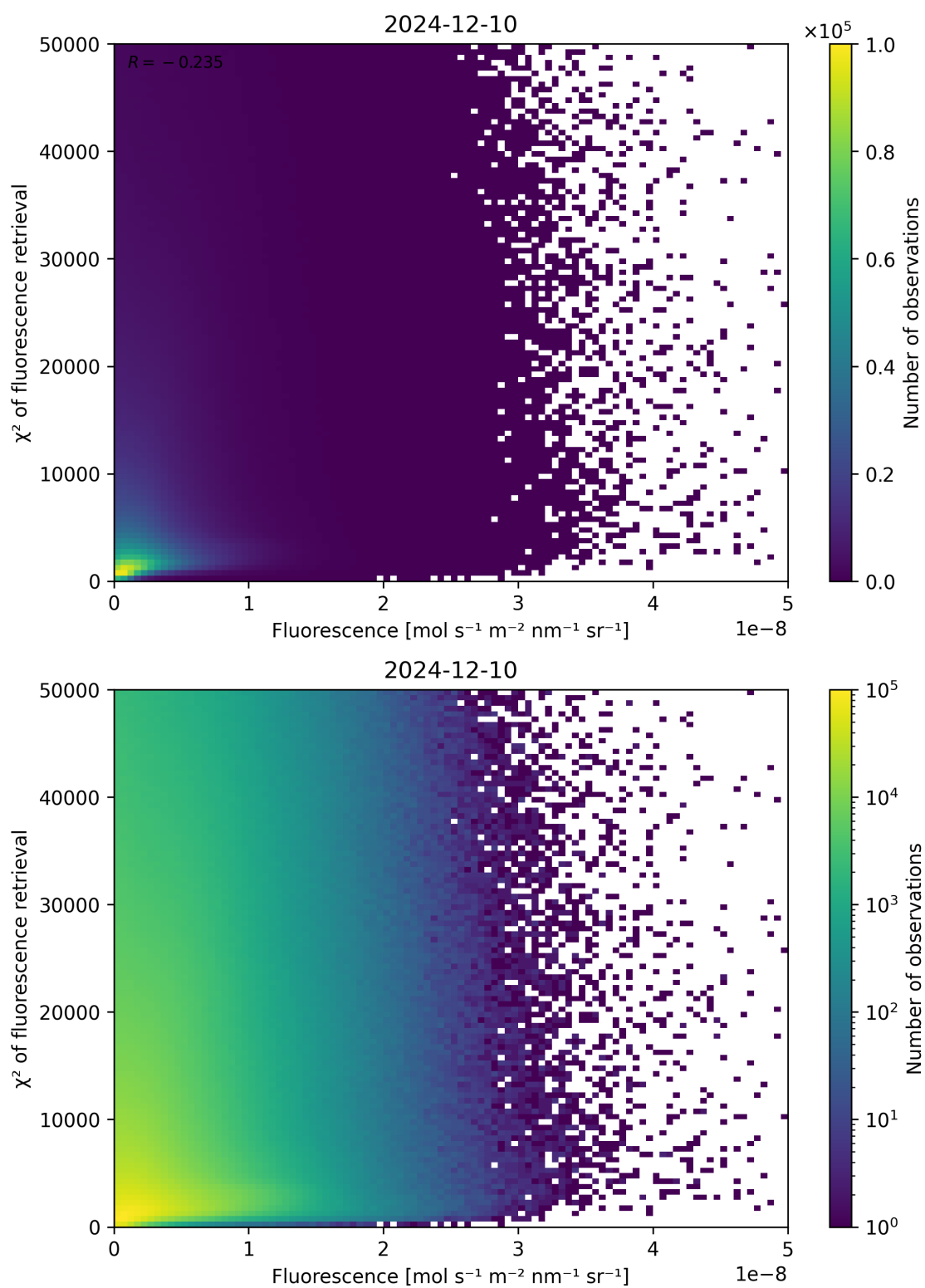
Figure 85: Scatter density plot of “Fluorescence” against “ \chi^2 of fluorescence retrieval” for 2024-12-09 to 2024-12-11.
