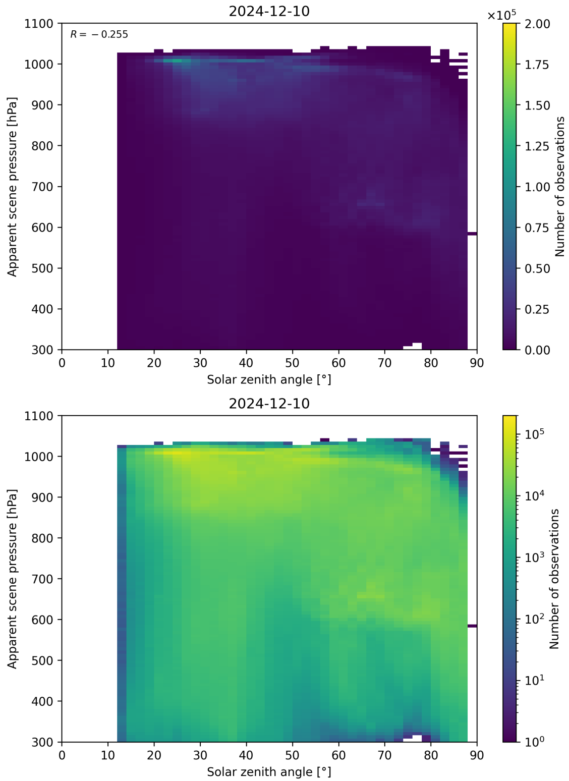
Figure 108: Scatter density plot of “Solar zenith angle” against “Apparent scene pressure” for 2024-12-09 to 2024-12-11.
