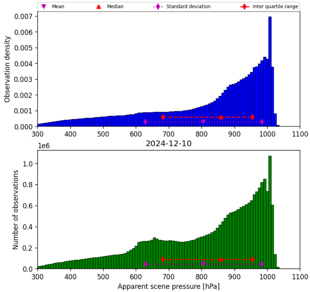
Figure 36: Histogram of “Apparent scene pressure” for 2024-12-09 to 2024-12-11
