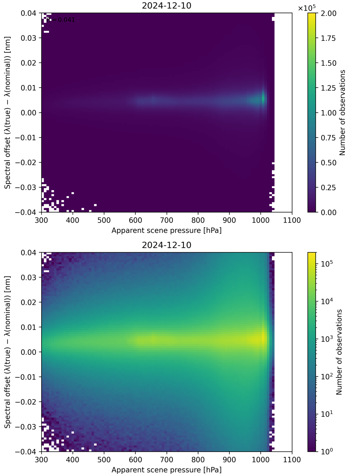
Figure 67: Scatter density plot of “Apparent scene pressure” against “Spectral offset ( \lambda_{\text{true}} - \lambda_{\text{nominal}} )” for 2024-12-09 to 2024-12-11.
