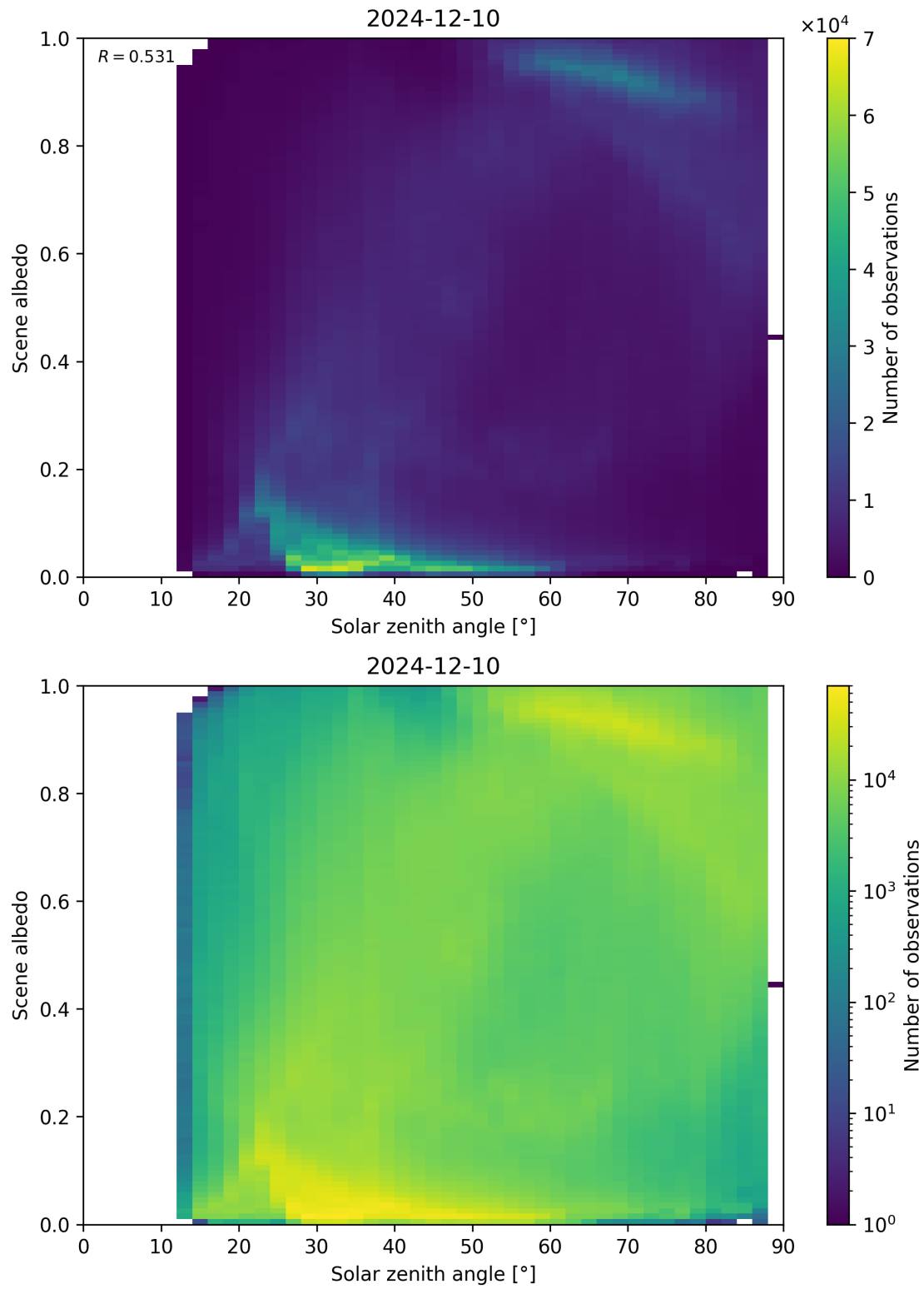
Figure 116: Scatter density plot of “Solar zenith angle” against “Scene albedo” for 2024-12-09 to 2024-12-11.
