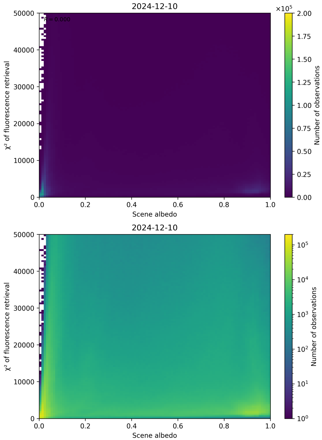
Figure 103: Scatter density plot of “Scene albedo” against “ \chi^2 of fluorescence retrieval” for 2024-12-09 to 2024-12-11.
