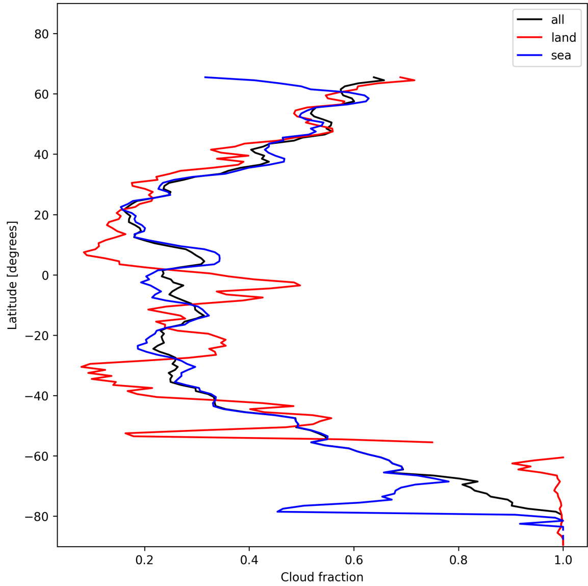
Figure 15: Zonal average of “Cloud fraction” for 2024-12-09 to 2024-12-11.
