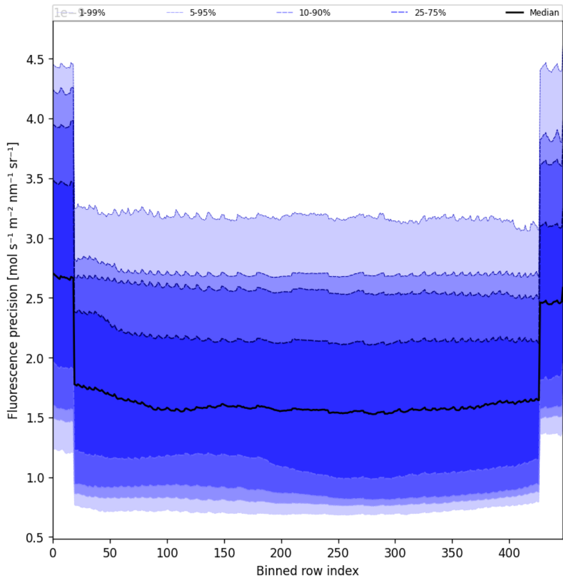
Figure 58: Along track statistics of “Fluorescence precision” for 2024-12-09 to 2024-12-11
