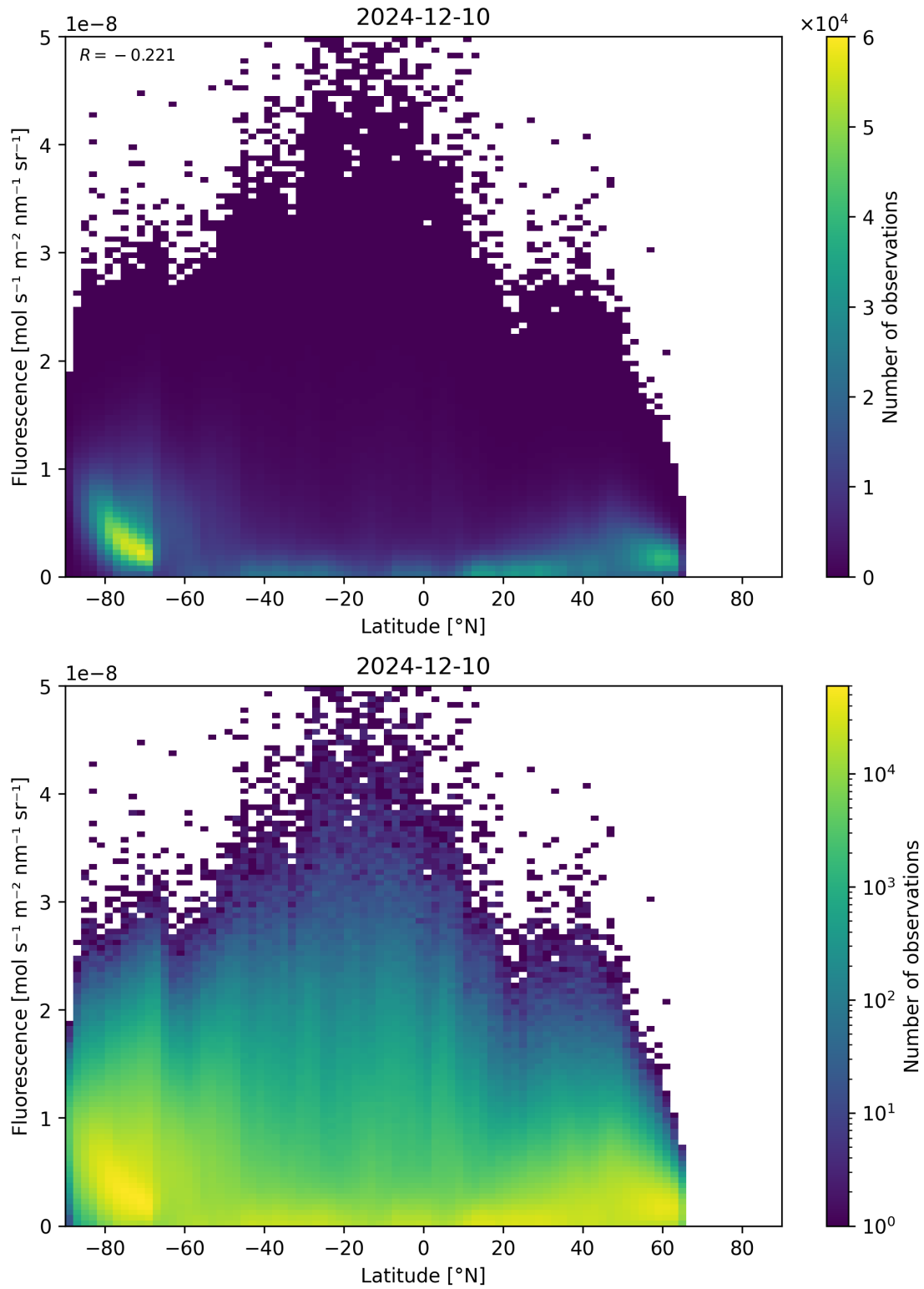
Figure 92: Scatter density plot of “Latitude” against “Fluorescence” for 2024-12-09 to 2024-12-11.
