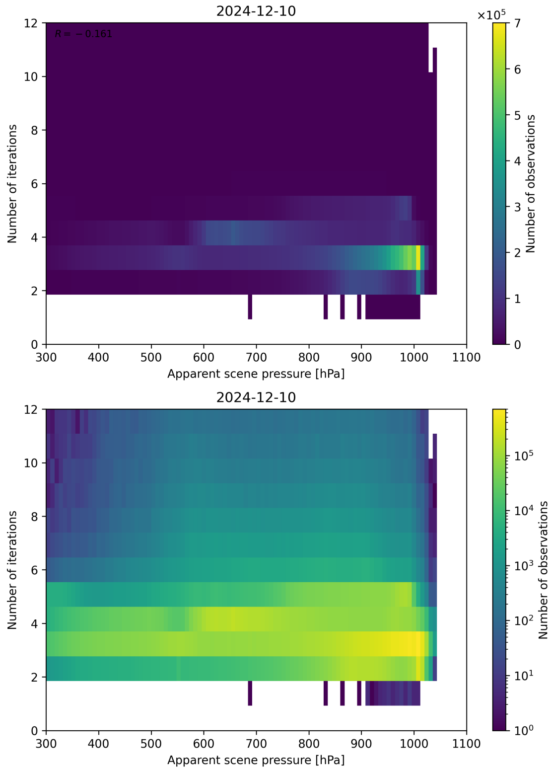
Figure 65: Scatter density plot of “Apparent scene pressure” against “Number of iterations” for 2024-12-09 to 2024-12-11.
