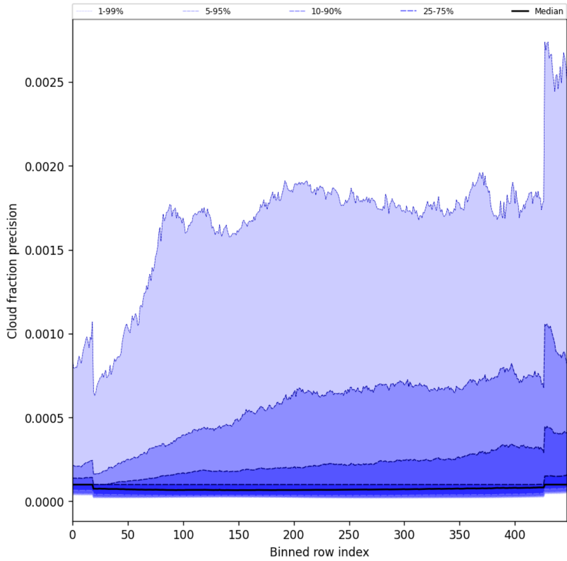
Figure 50: Along track statistics of “Cloud fraction precision” for 2024-12-09 to 2024-12-11
