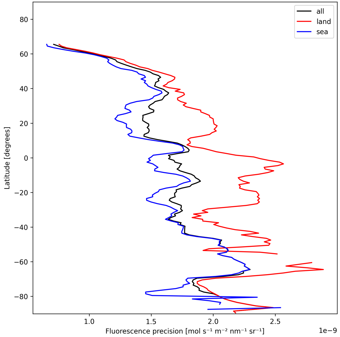
Figure 24: Zonal average of “Fluorescence precision” for 2024-12-09 to 2024-12-11.
