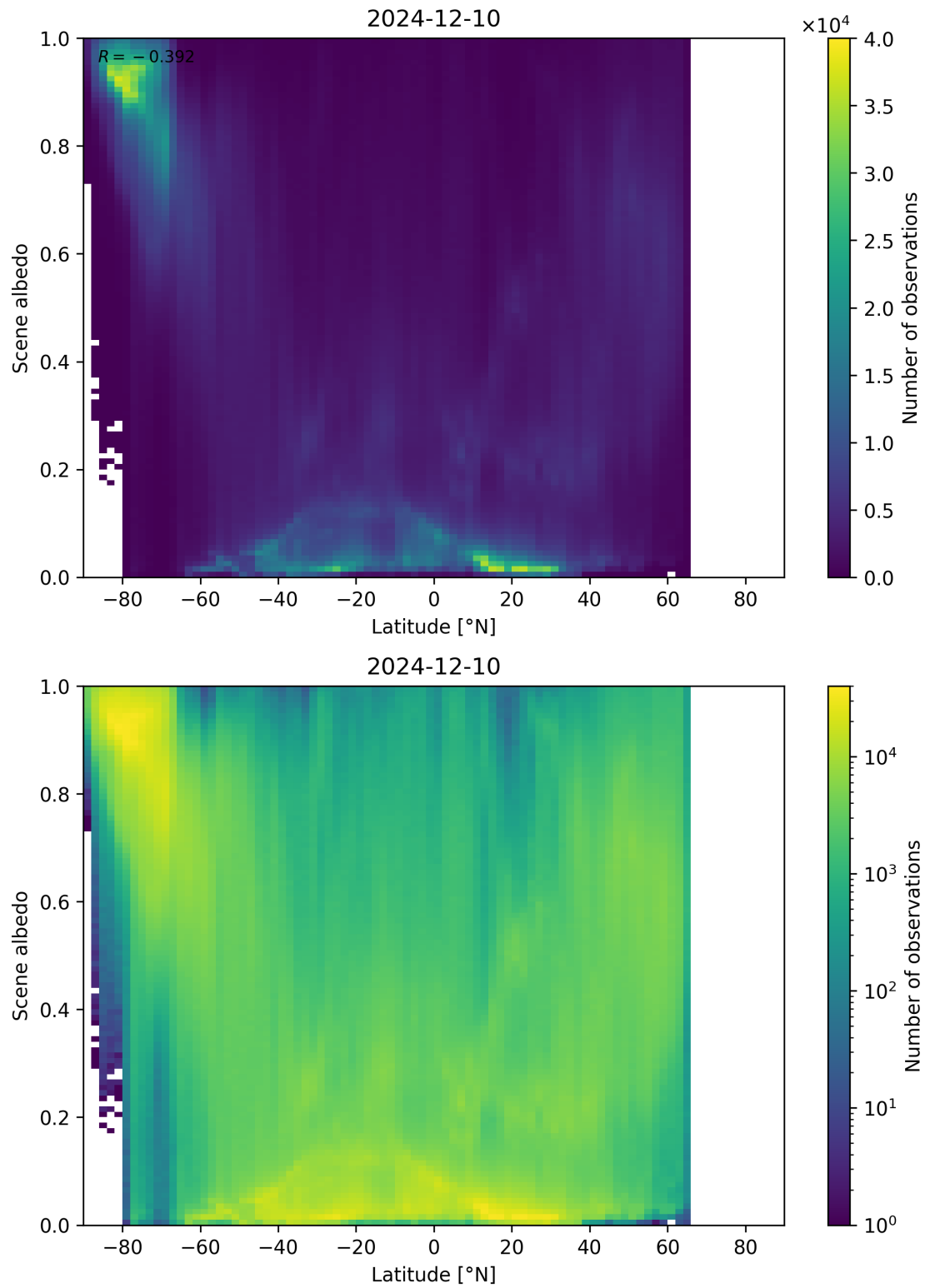
Figure 95: Scatter density plot of “Latitude” against “Scene albedo” for 2024-12-09 to 2024-12-11.
