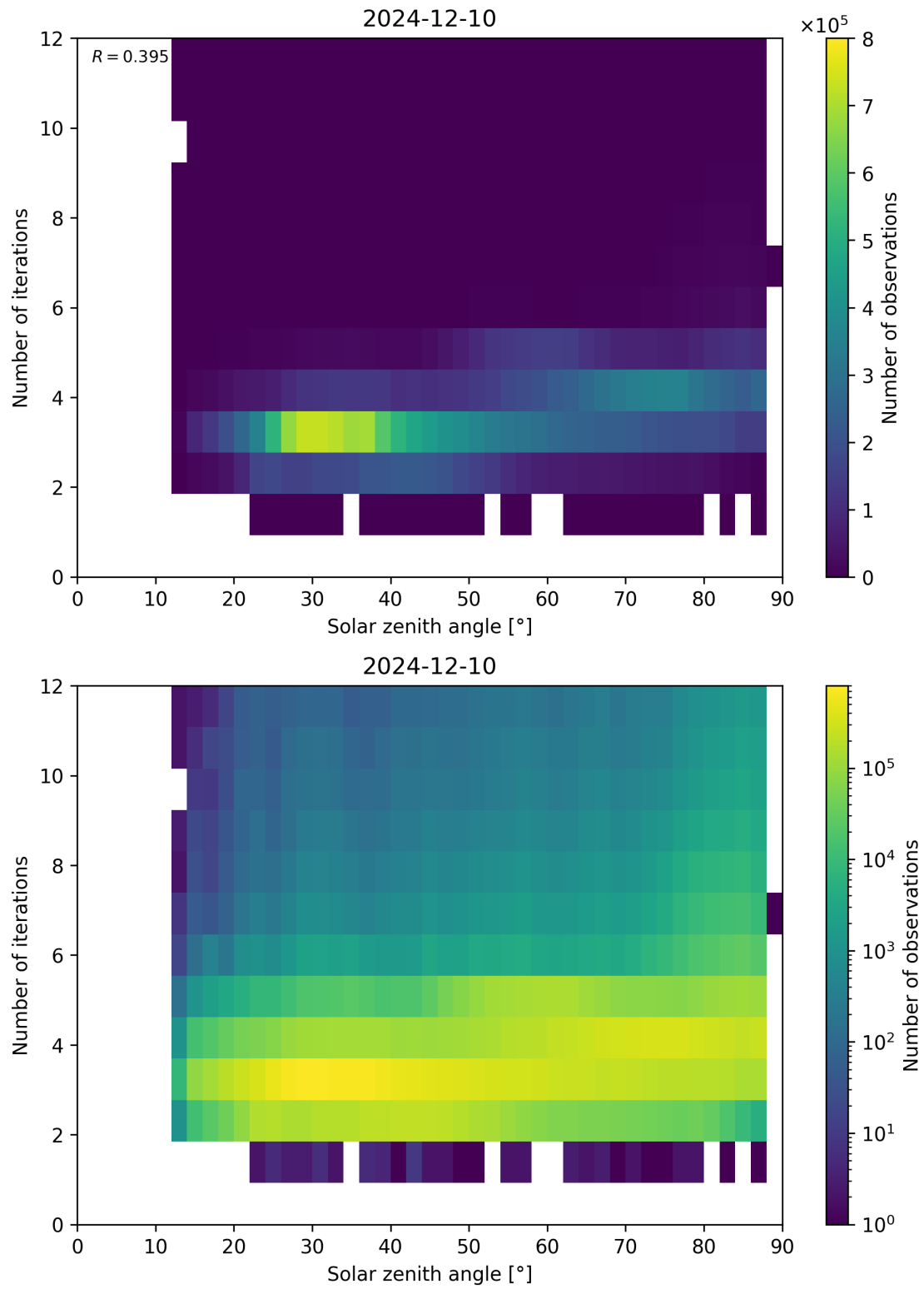
Figure 114: Scatter density plot of “Solar zenith angle” against “Number of iterations” for 2024-12-09 to 2024-12-11.
