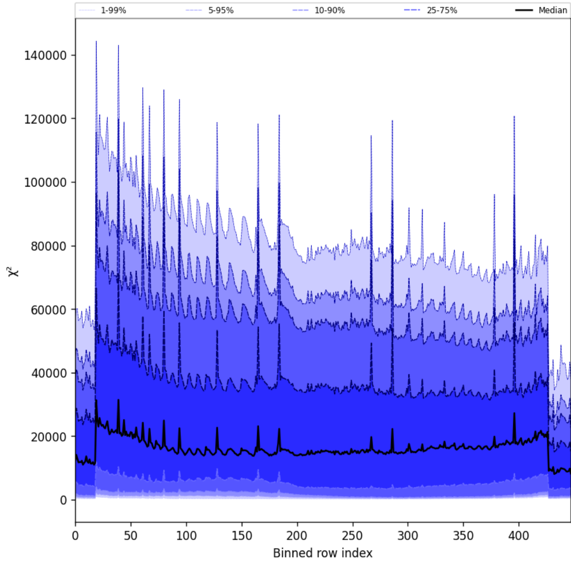
Figure 55: Along track statistics of “ \chi^2 ” for 2024-12-09 to 2024-12-11
