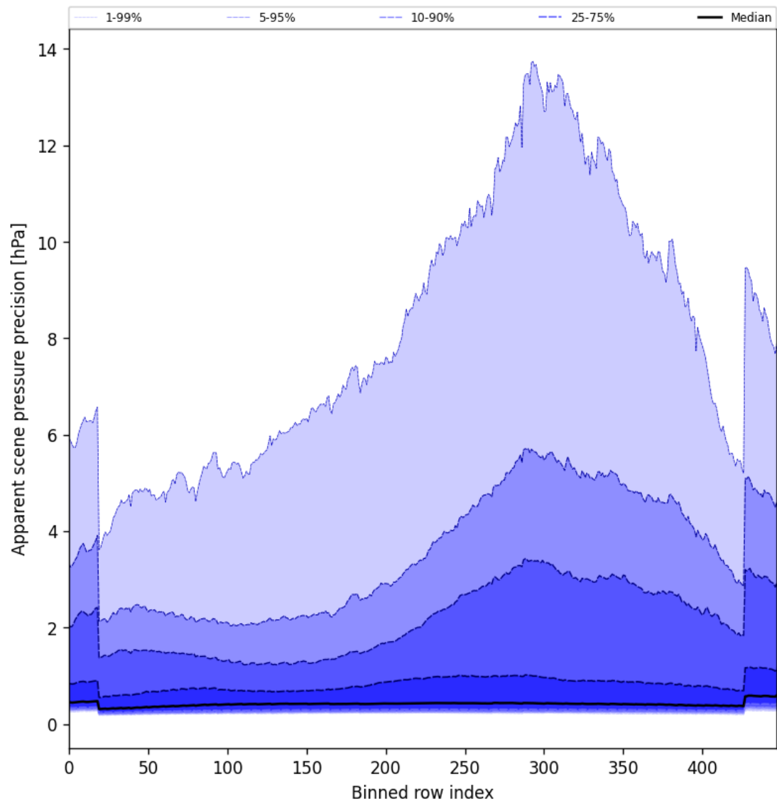
Figure 54: Along track statistics of “Apparent scene pressure precision” for 2024-12-09 to 2024-12-11
