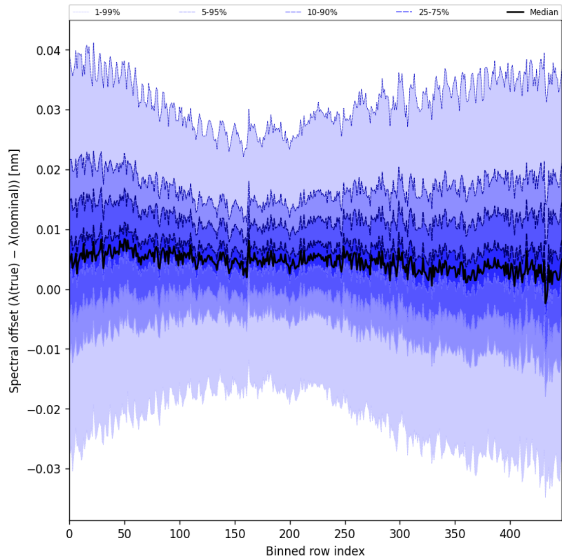
Figure 62: Along track statistics of “Spectral offset (\lambda_{\text{true}} - \lambda_{\text{nominal}}) ” for 2024-12-09 to 2024-12-11
