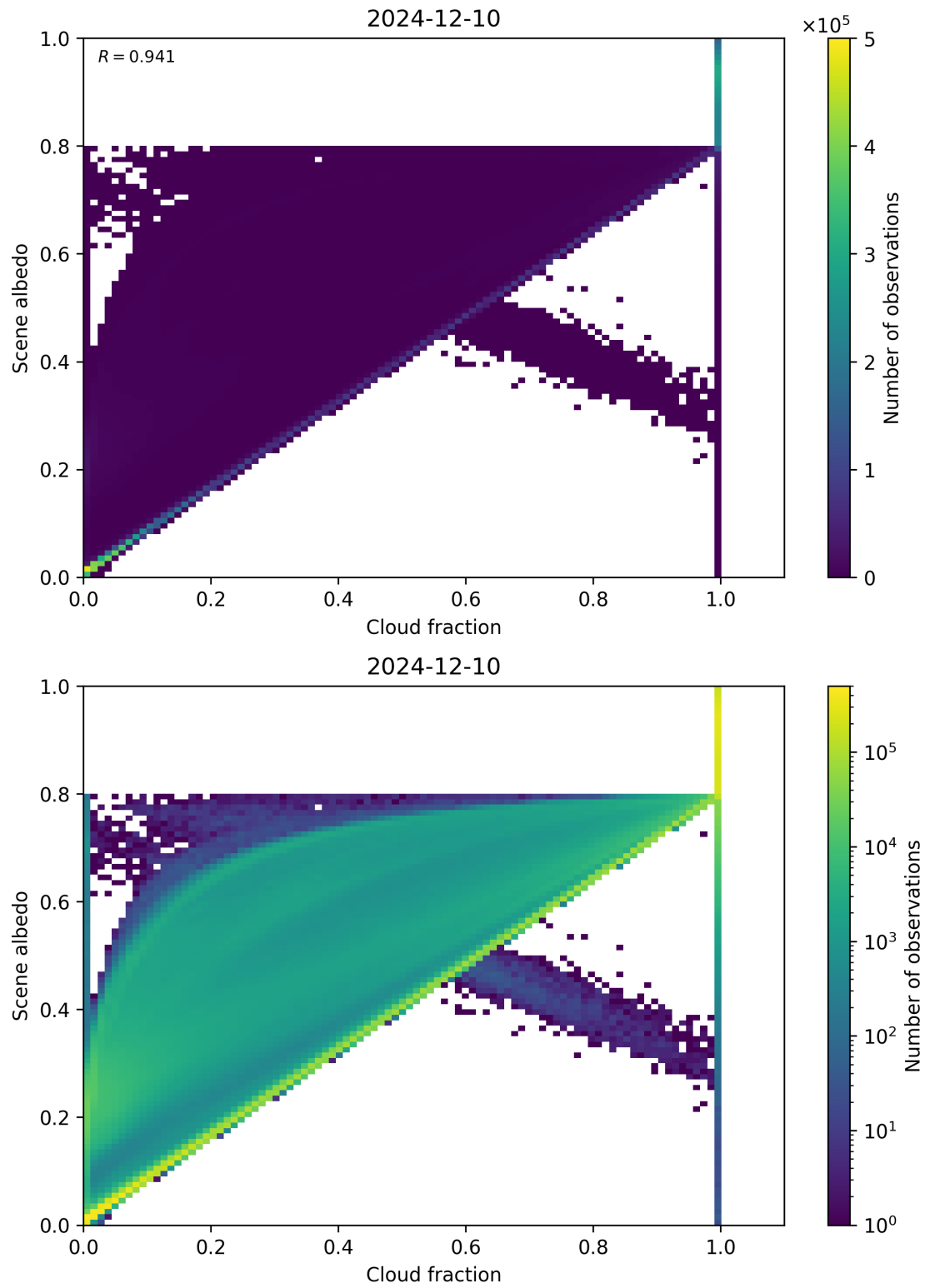
Figure 75: Scatter density plot of “Cloud fraction” against “Scene albedo” for 2024-12-09 to 2024-12-11.
