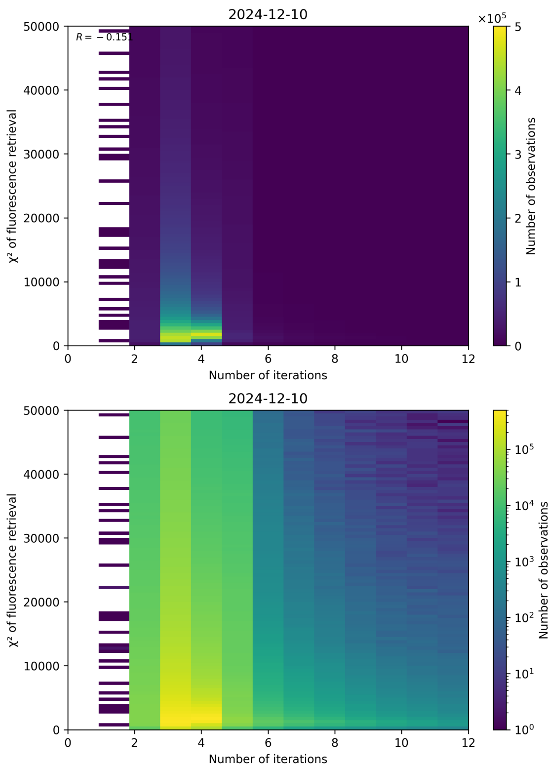
Figure 97: Scatter density plot of “Number of iterations” against “ \chi^2 of fluorescence retrieval” for 2024-12-09 to 2024-12-11.
