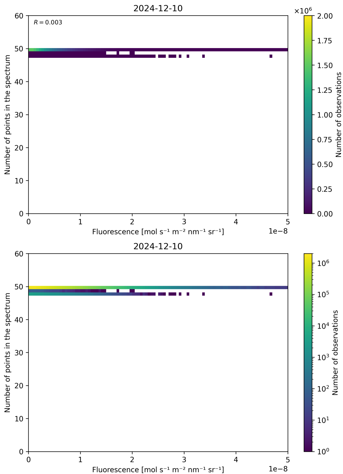
Figure 86: Scatter density plot of “Fluorescence” against “Number of points in the spectrum” for 2024-12-09 to 2024-12-11.
