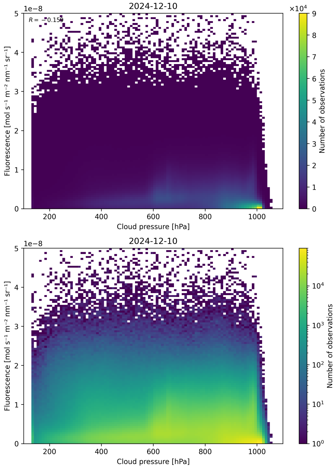
Figure 80: Scatter density plot of “Cloud pressure” against “Fluorescence” for 2024-12-09 to 2024-12-11.
