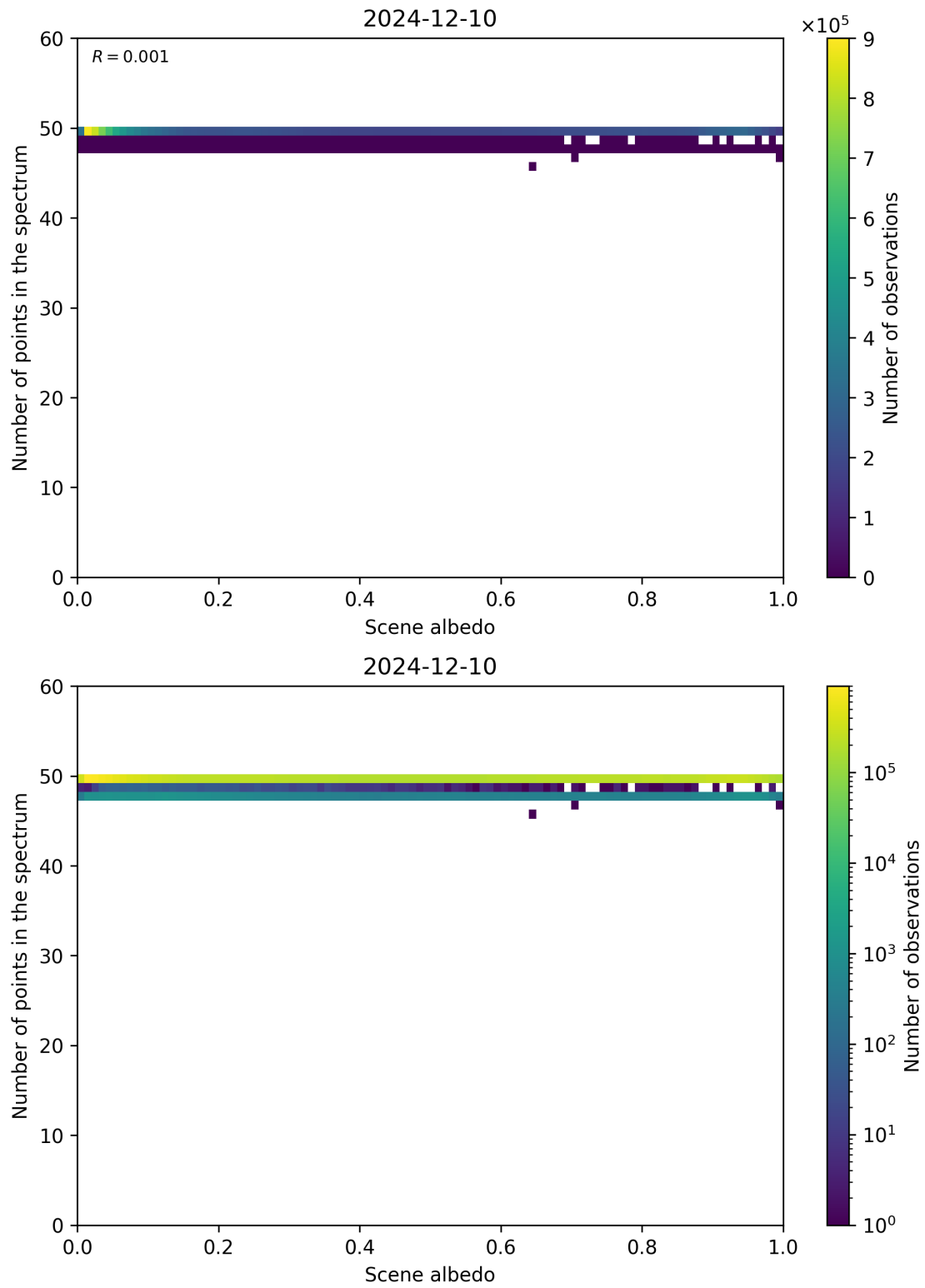
Figure 106: Scatter density plot of “Scene albedo” against “Number of points in the spectrum” for 2024-12-09 to 2024-12-11.
