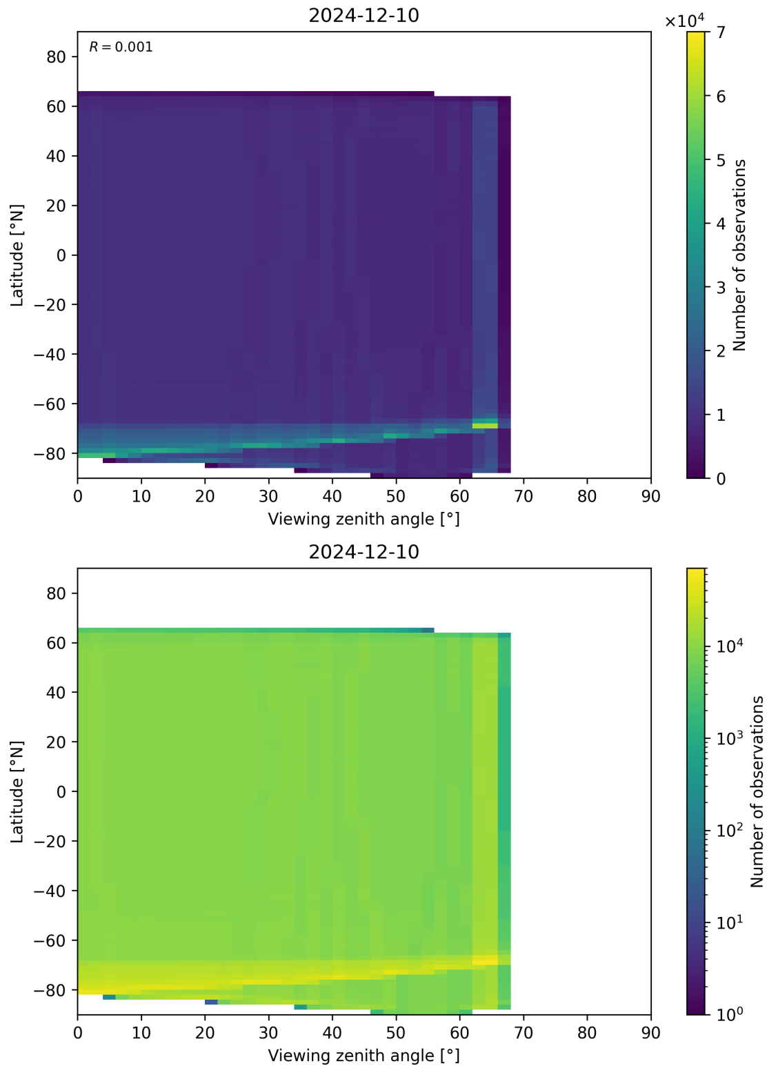
Figure 123: Scatter density plot of “Viewing zenith angle” against “Latitude” for 2024-12-09 to 2024-12-11.
