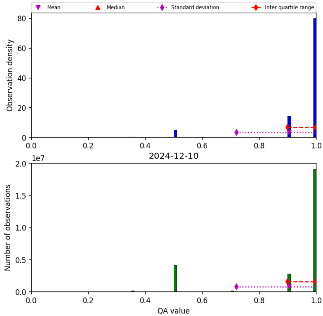
Figure 29: Histogram of “QA value” for 2024-12-09 to 2024-12-11
