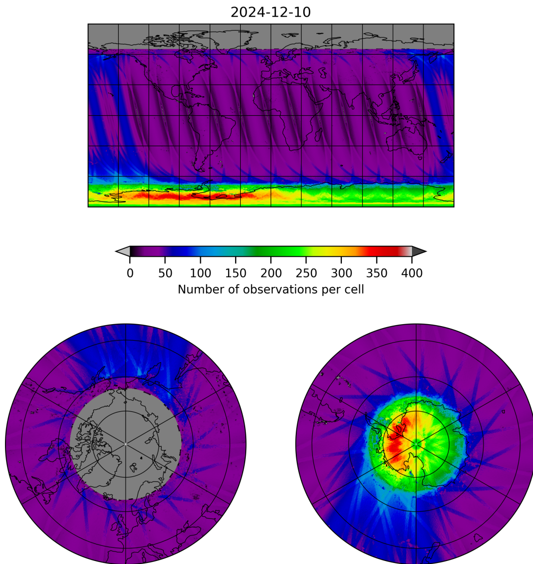
Figure 11: Map of the number of observations for 2024-12-09 to 2024-12-11
