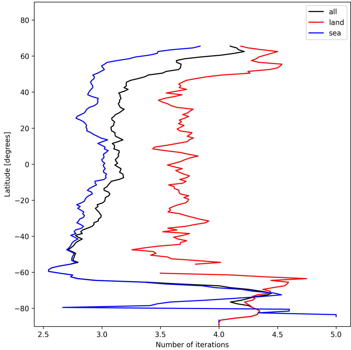
Figure 22: Zonal average of “Number of iterations” for 2024-12-09 to 2024-12-11.
