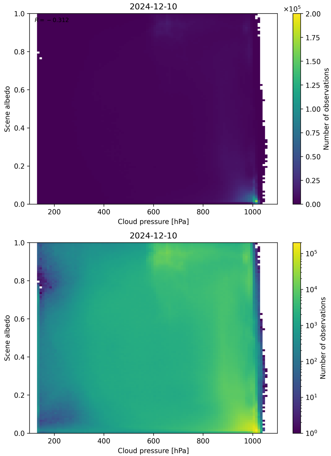
Figure 83: Scatter density plot of “Cloud pressure” against “Scene albedo” for 2024-12-09 to 2024-12-11.
