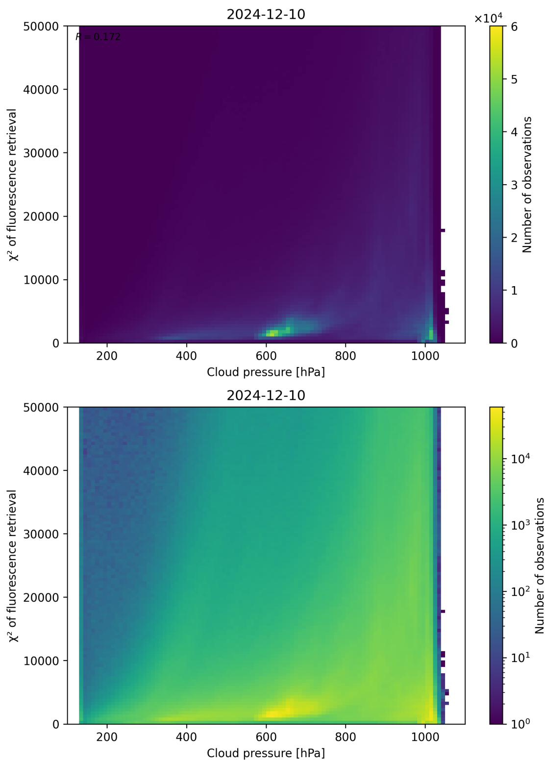
Figure 78: Scatter density plot of “Cloud pressure” against “ \chi^2 of fluorescence retrieval” for 2024-12-09 to 2024-12-11.
