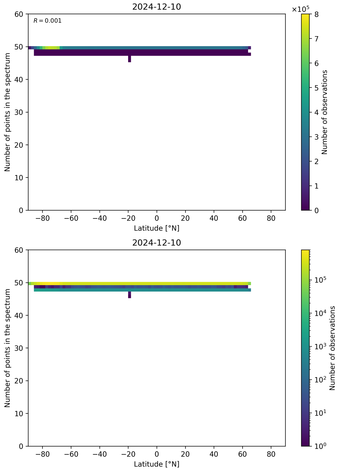
Figure 94: Scatter density plot of “Latitude” against “Number of points in the spectrum” for 2024-12-09 to 2024-12-11.
