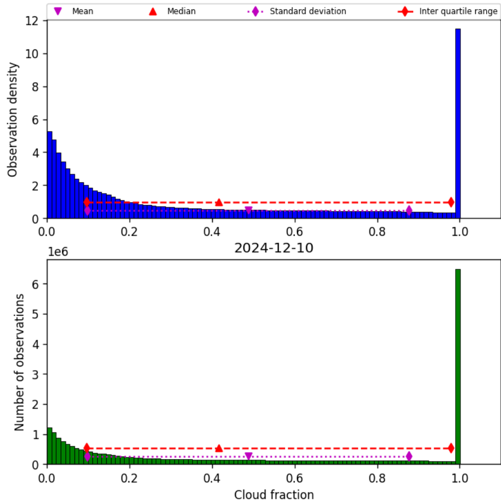
Figure 32: Histogram of “Cloud fraction” for 2024-12-09 to 2024-12-11
