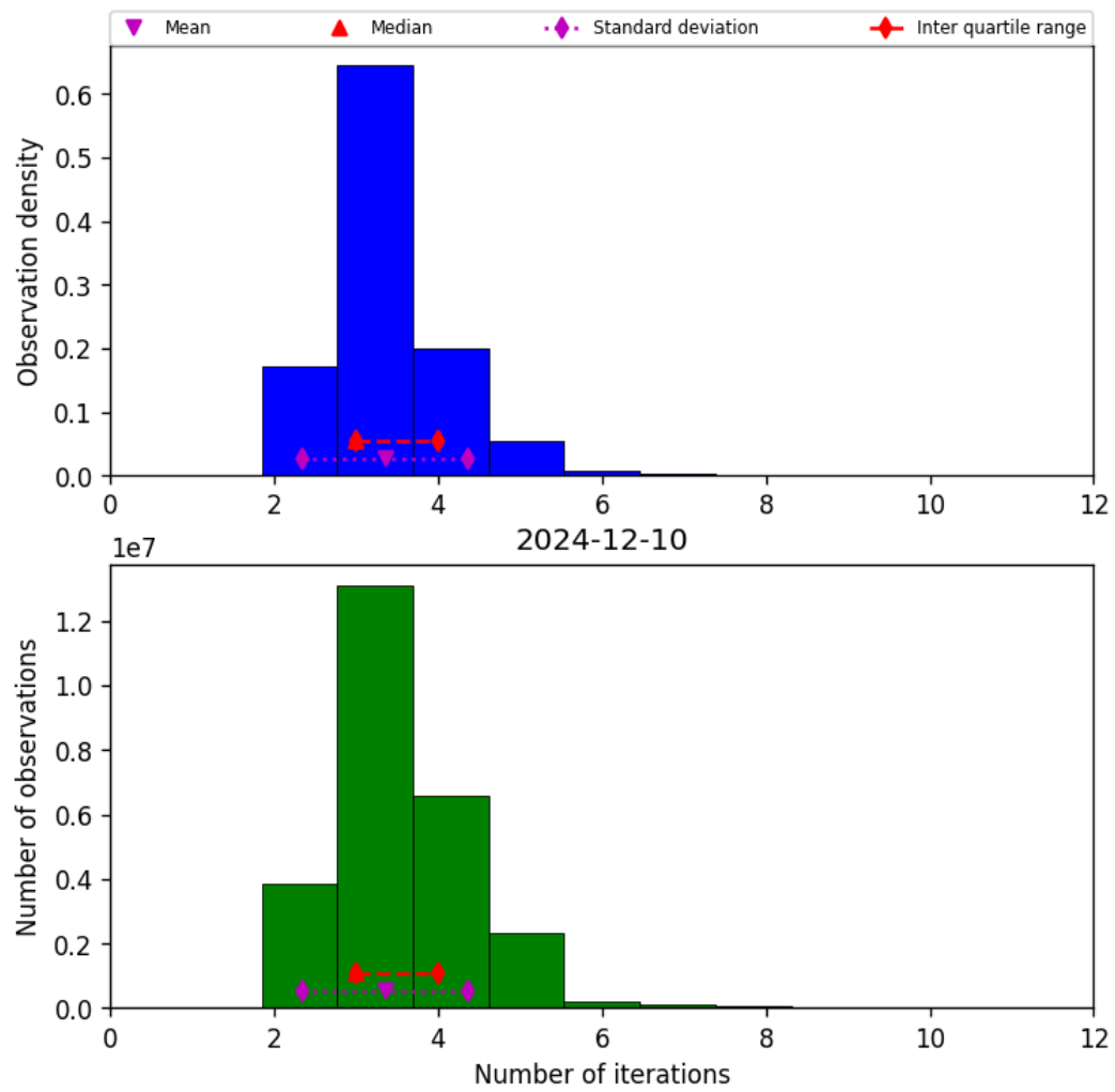
Figure 39: Histogram of “Number of iterations” for 2024-12-09 to 2024-12-11
