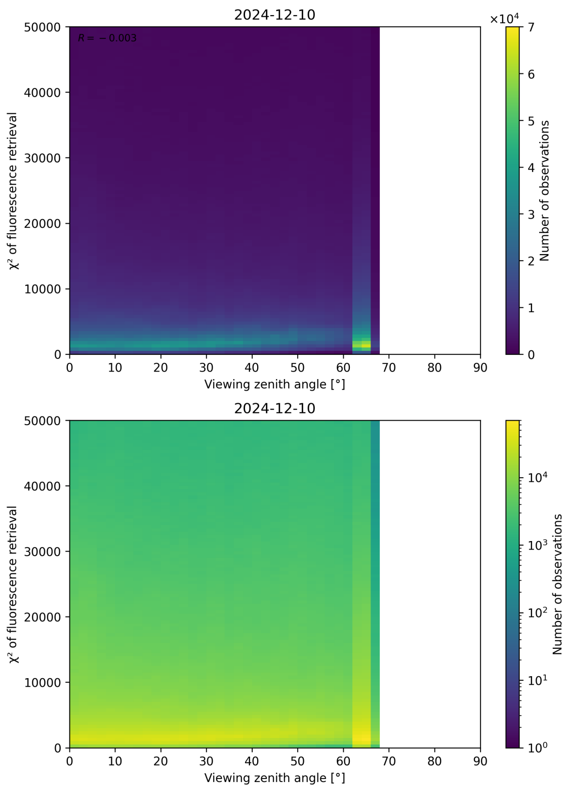
Figure 119: Scatter density plot of “Viewing zenith angle” against “ \chi^2 of fluorescence retrieval” for 2024-12-09 to 2024-12-11.
