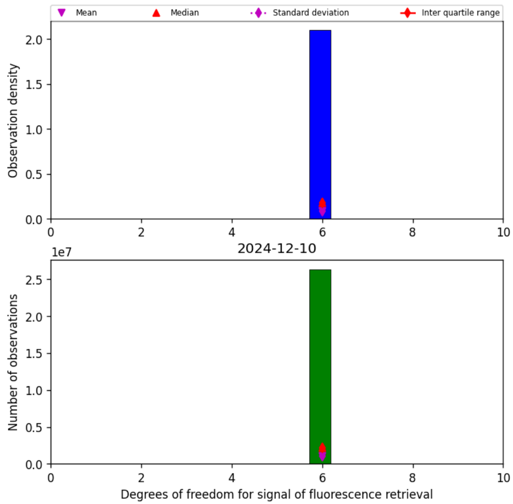
Figure 43: Histogram of "Degrees of freedom for signal of fluorescence retrieval" for 2024-12-09 to 2024-12-11
