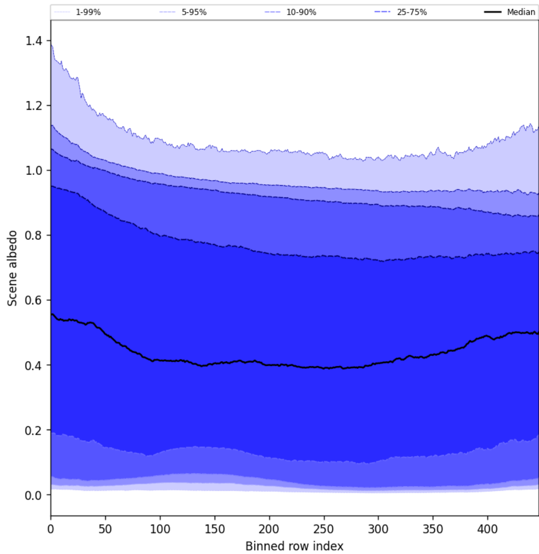
Figure 51: Along track statistics of “Scene albedo” for 2024-12-09 to 2024-12-11
