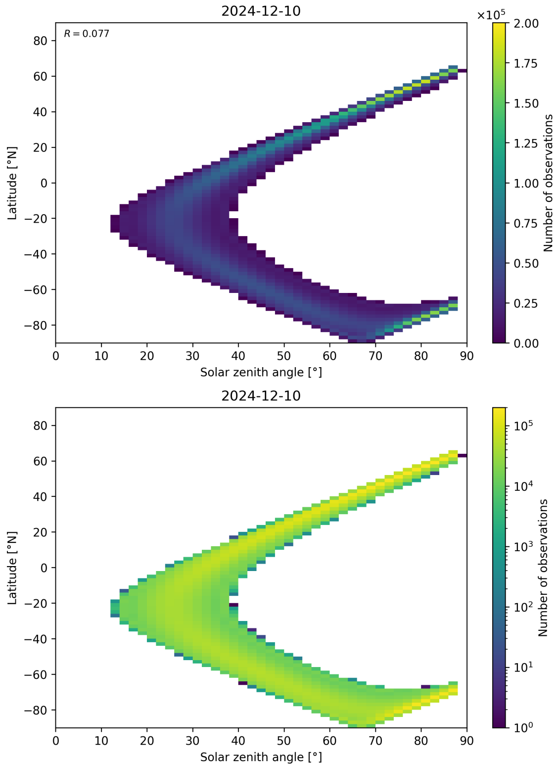
Figure 113: Scatter density plot of “Solar zenith angle” against “Latitude” for 2024-12-09 to 2024-12-11.
