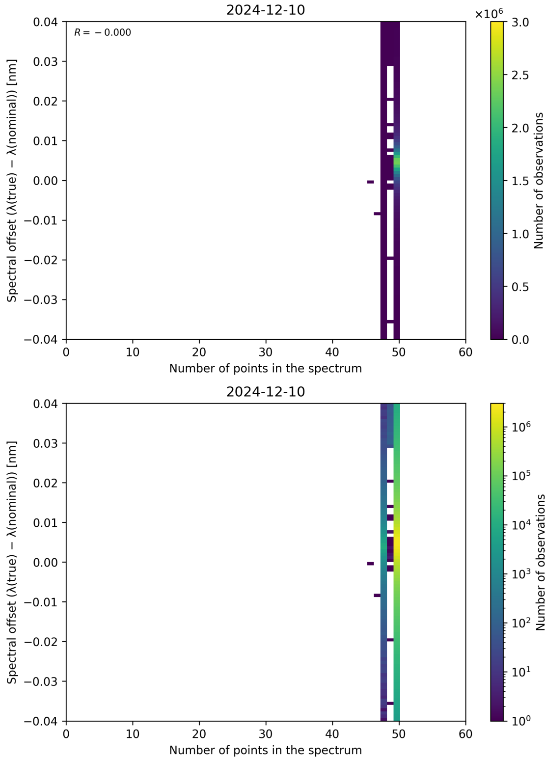
Figure 101: Scatter density plot of “Number of points in the spectrum” against “Spectral offset ( \lambda_{\text{true}} - \lambda_{\text{nominal}} )” for 2024-12-09 to 2024-12-11.
