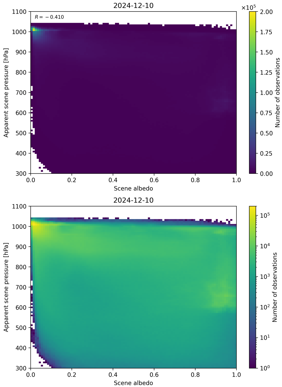
Figure 102: Scatter density plot of “Scene albedo” against “Apparent scene pressure” for 2024-12-09 to 2024-12-11.
