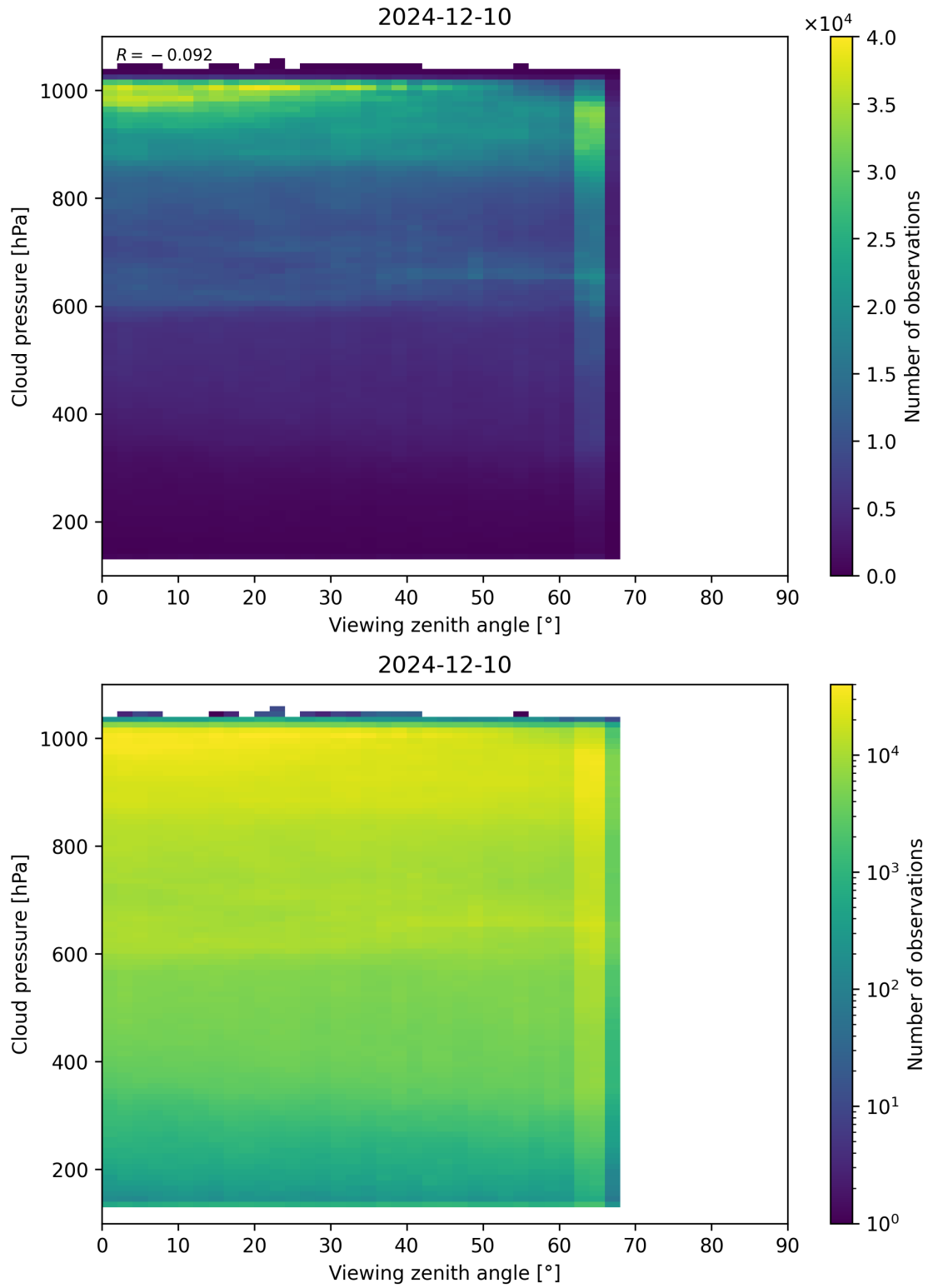
Figure 121: Scatter density plot of “Viewing zenith angle” against “Cloud pressure” for 2024-12-09 to 2024-12-11.
