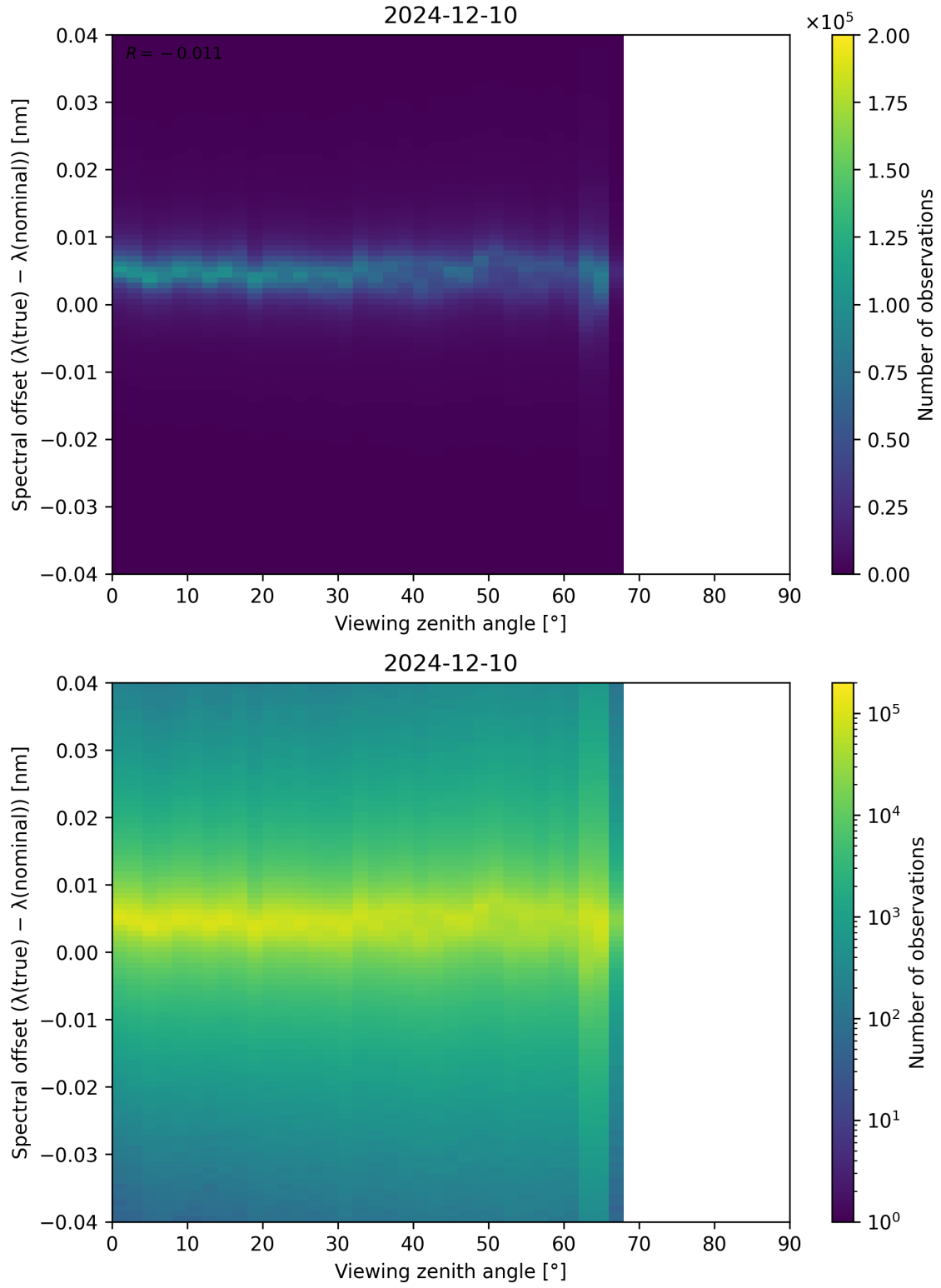
Figure 128: Scatter density plot of “Viewing zenith angle” against “Spectral offset ( \lambda_{\text{true}} - \lambda_{\text{nominal}} )” for 2024-12-09 to 2024-12-11.
