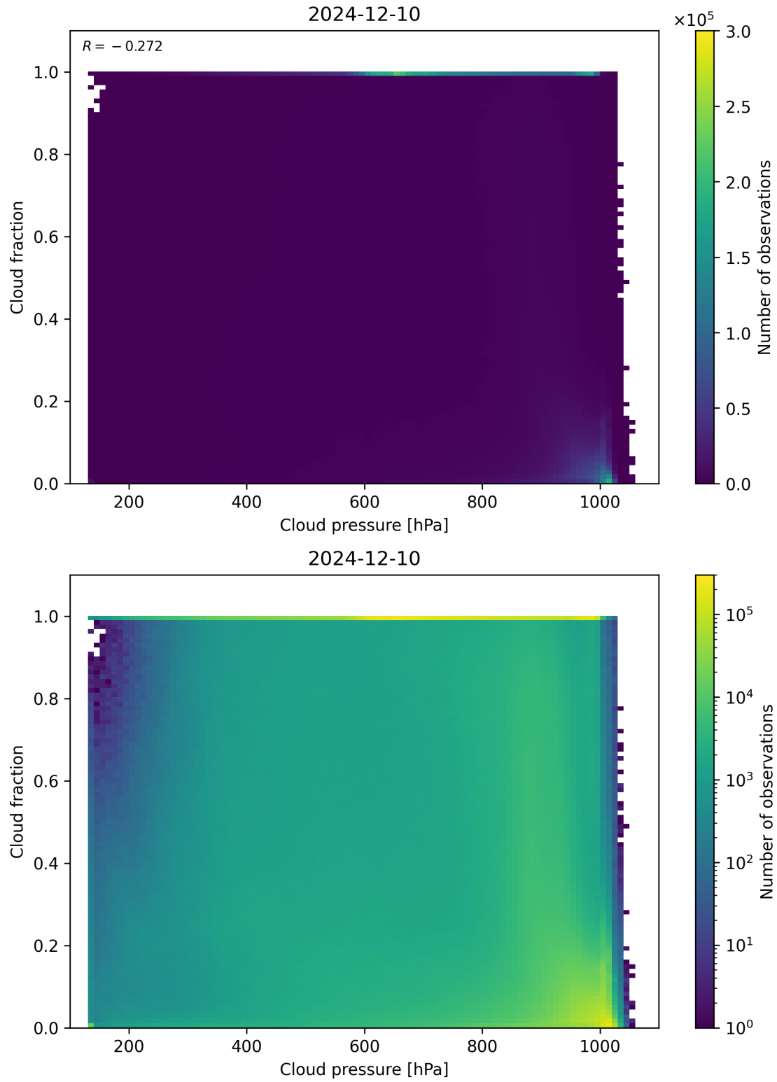
Figure 79: Scatter density plot of “Cloud pressure” against “Cloud fraction” for 2024-12-09 to 2024-12-11.
