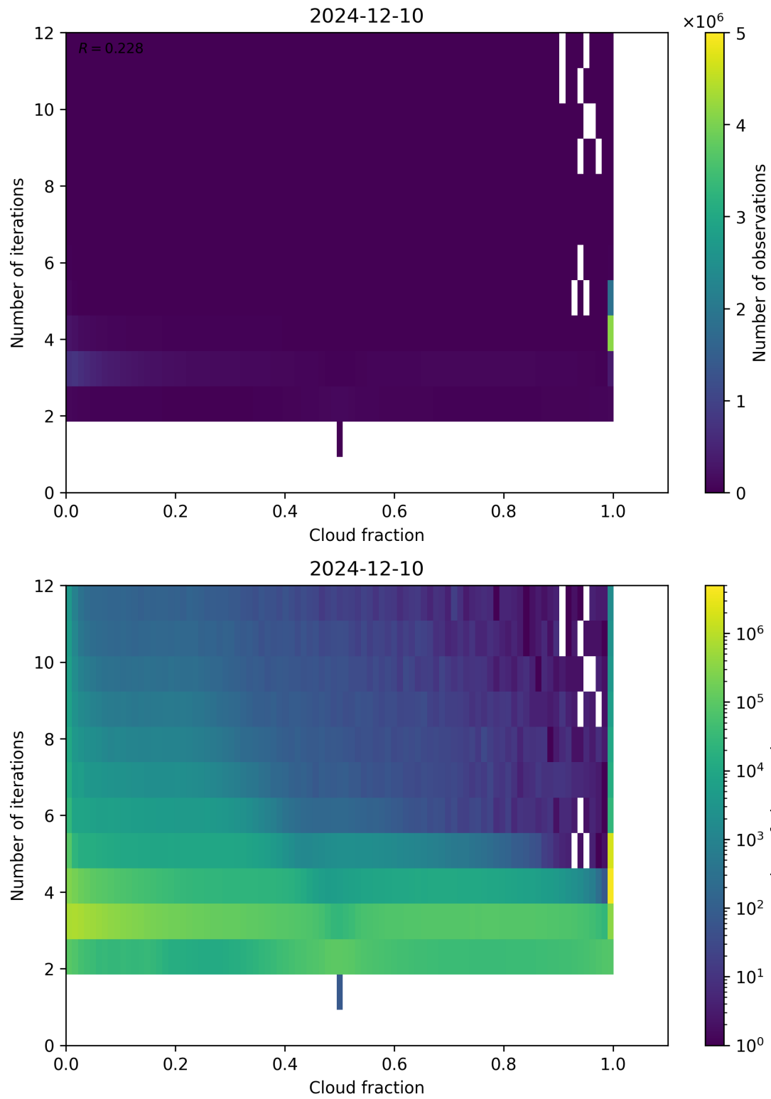
Figure 73: Scatter density plot of “Cloud fraction” against “Number of iterations” for 2024-12-09 to 2024-12-11.
