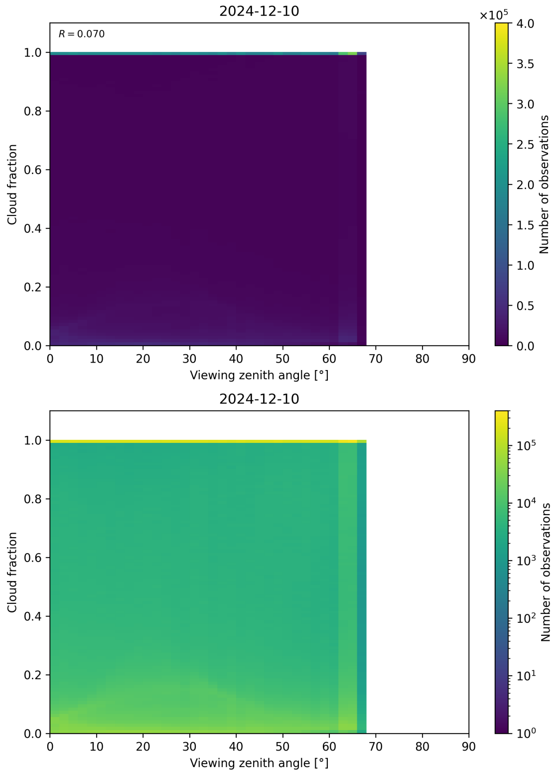
Figure 120: Scatter density plot of “Viewing zenith angle” against “Cloud fraction” for 2024-12-09 to 2024-12-11.
