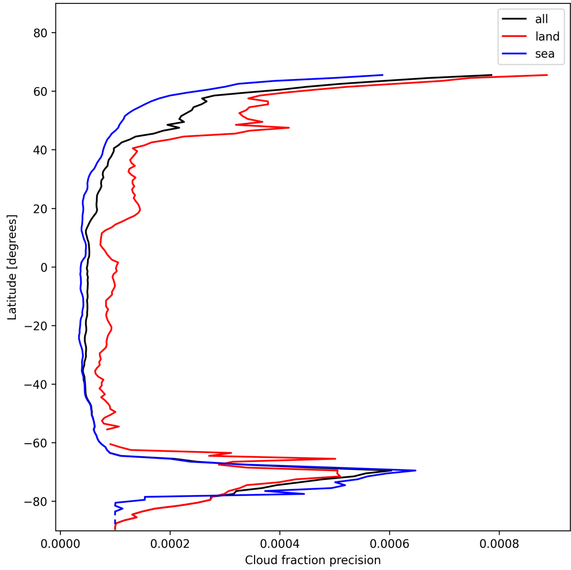
Figure 16: Zonal average of “Cloud fraction precision” for 2024-12-09 to 2024-12-11.
