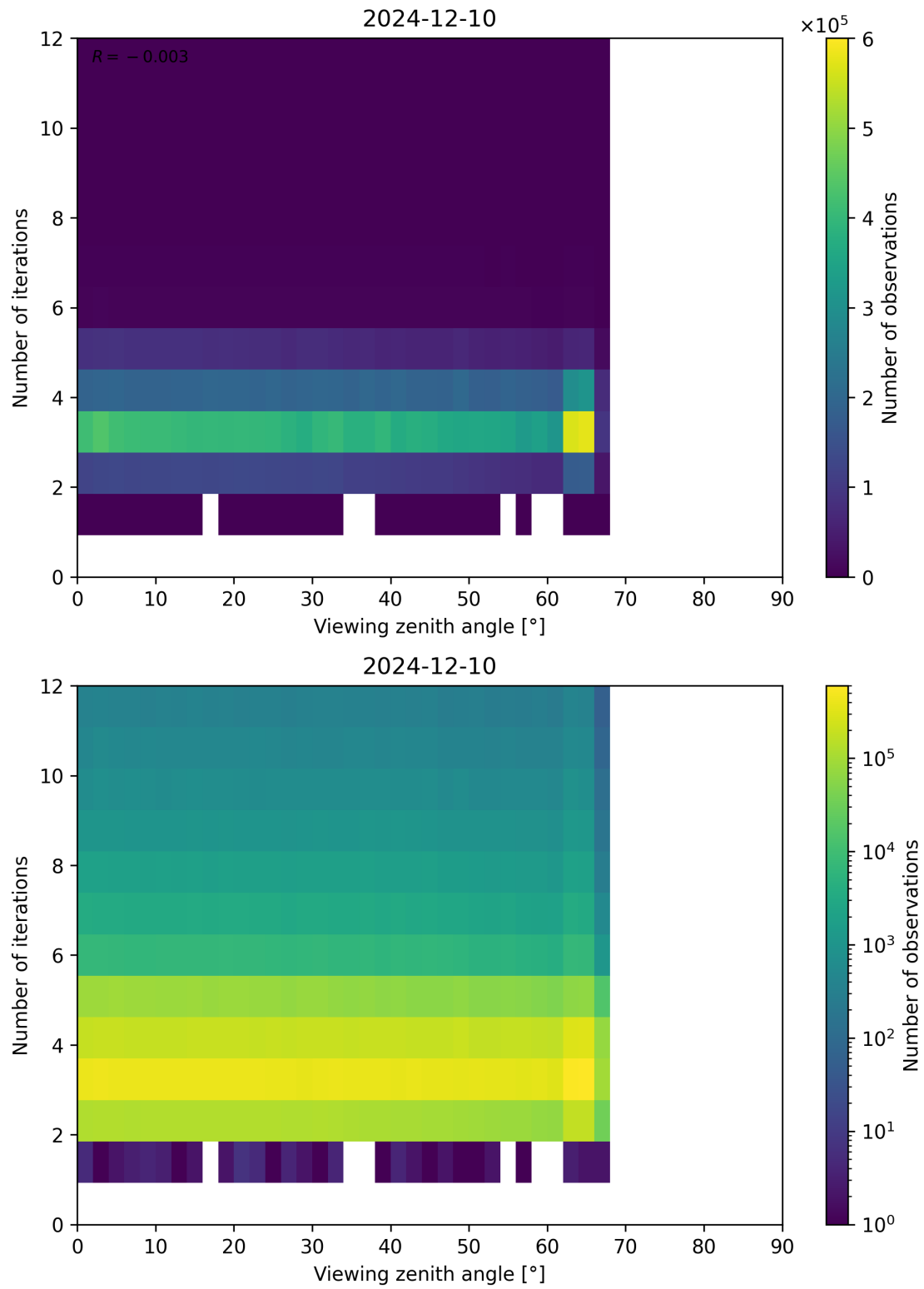
Figure 124: Scatter density plot of “Viewing zenith angle” against “Number of iterations” for 2024-12-09 to 2024-12-11.
