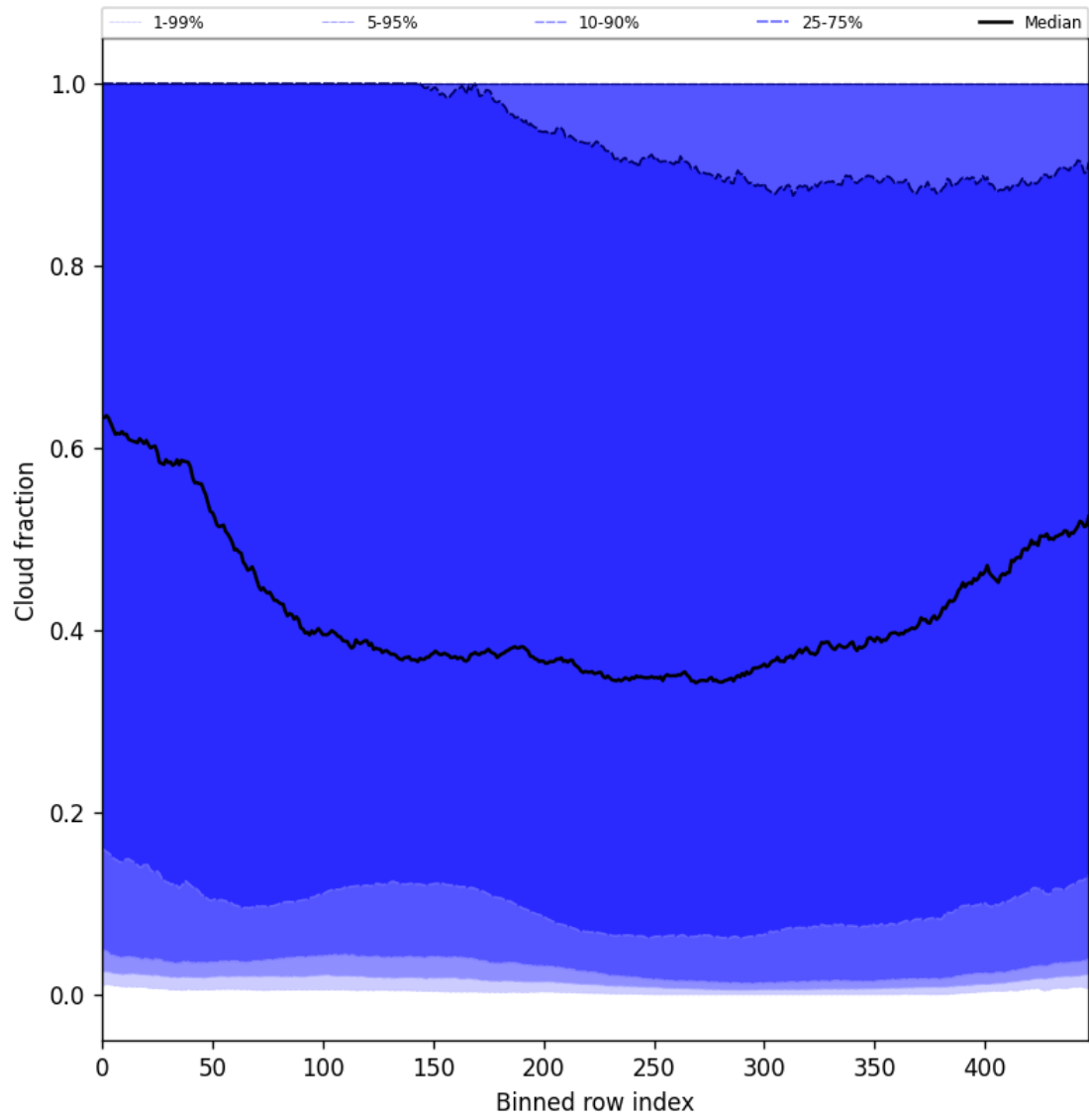
Figure 49: Along track statistics of “Cloud fraction” for 2024-12-09 to 2024-12-11
