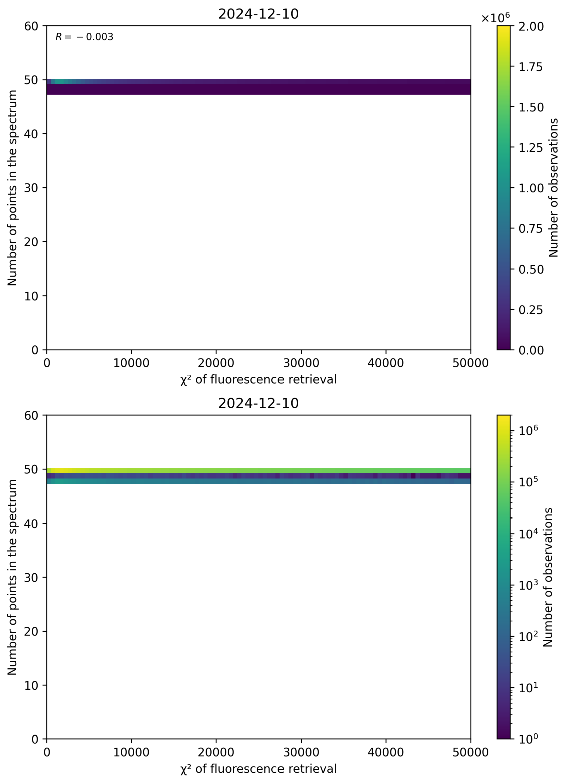
Figure 68: Scatter density plot of “ \chi^2 of fluorescence retrieval” against “Number of points in the spectrum” for 2024-12-09 to 2024-12-11.
