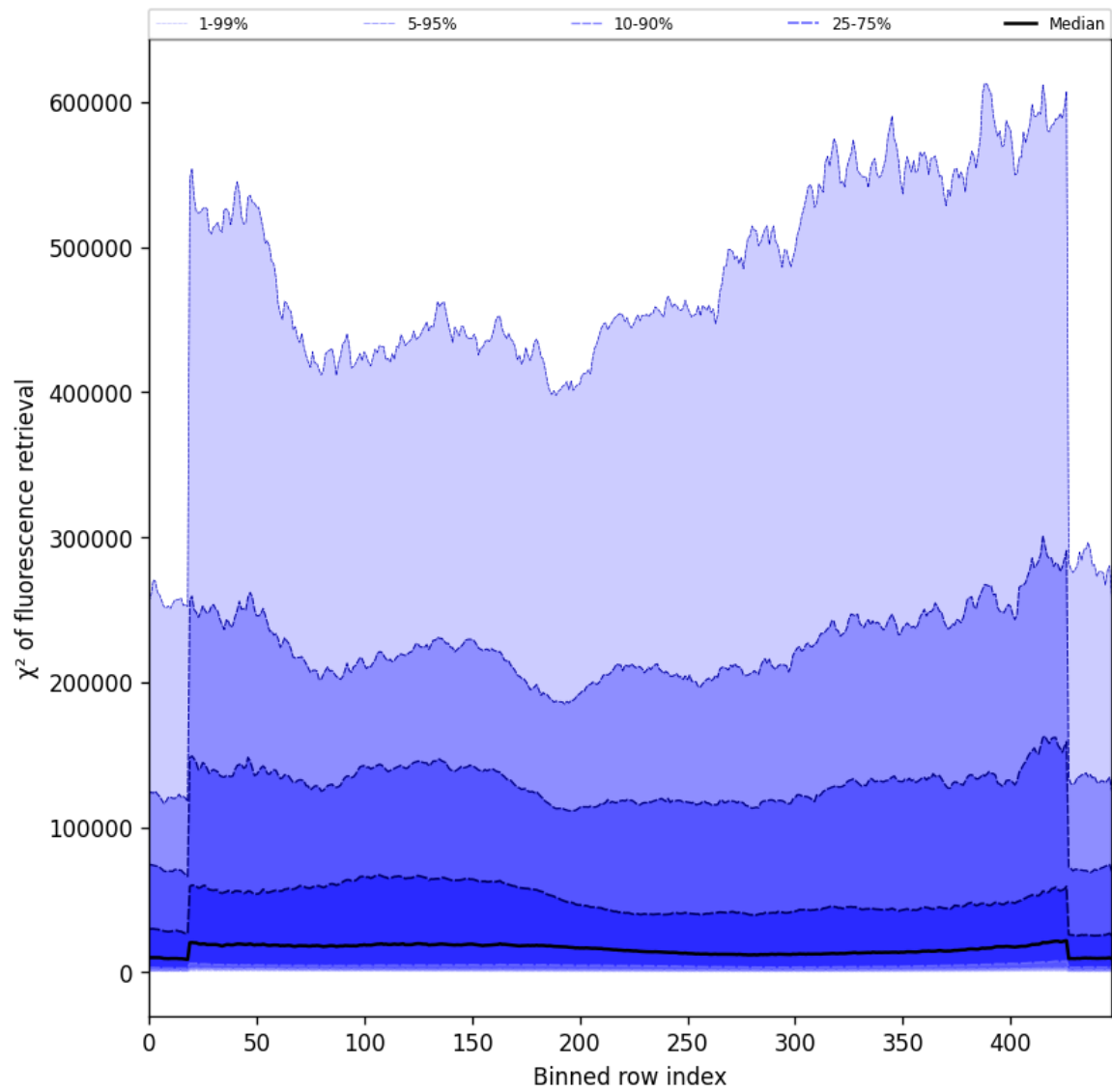
Figure 59: Along track statistics of “ \chi^2 of fluorescence retrieval” for 2024-12-09 to 2024-12-11
