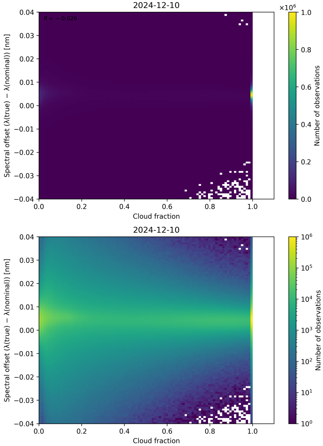
Figure 76: Scatter density plot of “Cloud fraction” against “Spectral offset ( \lambda_{\text{true}} - \lambda_{\text{nominal}} )” for 2024-12-09 to 2024-12-11.
