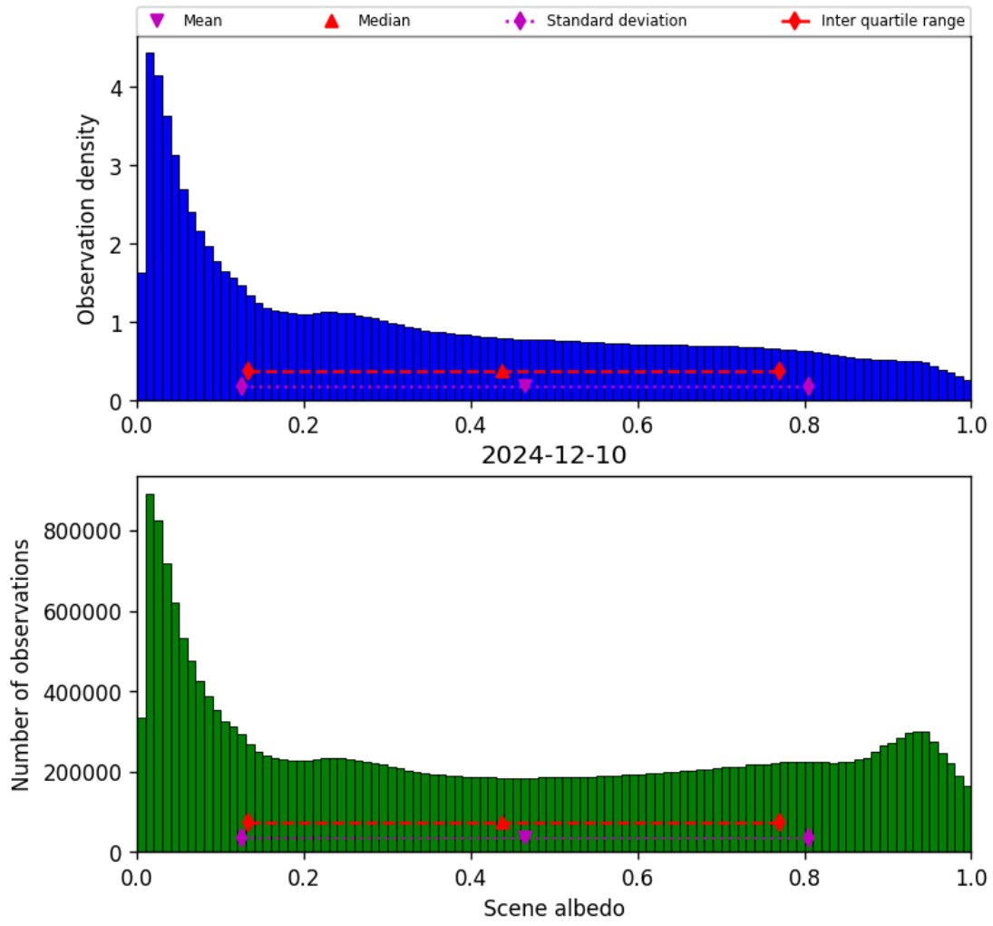
Figure 34: Histogram of “Scene albedo” for 2024-12-09 to 2024-12-11
