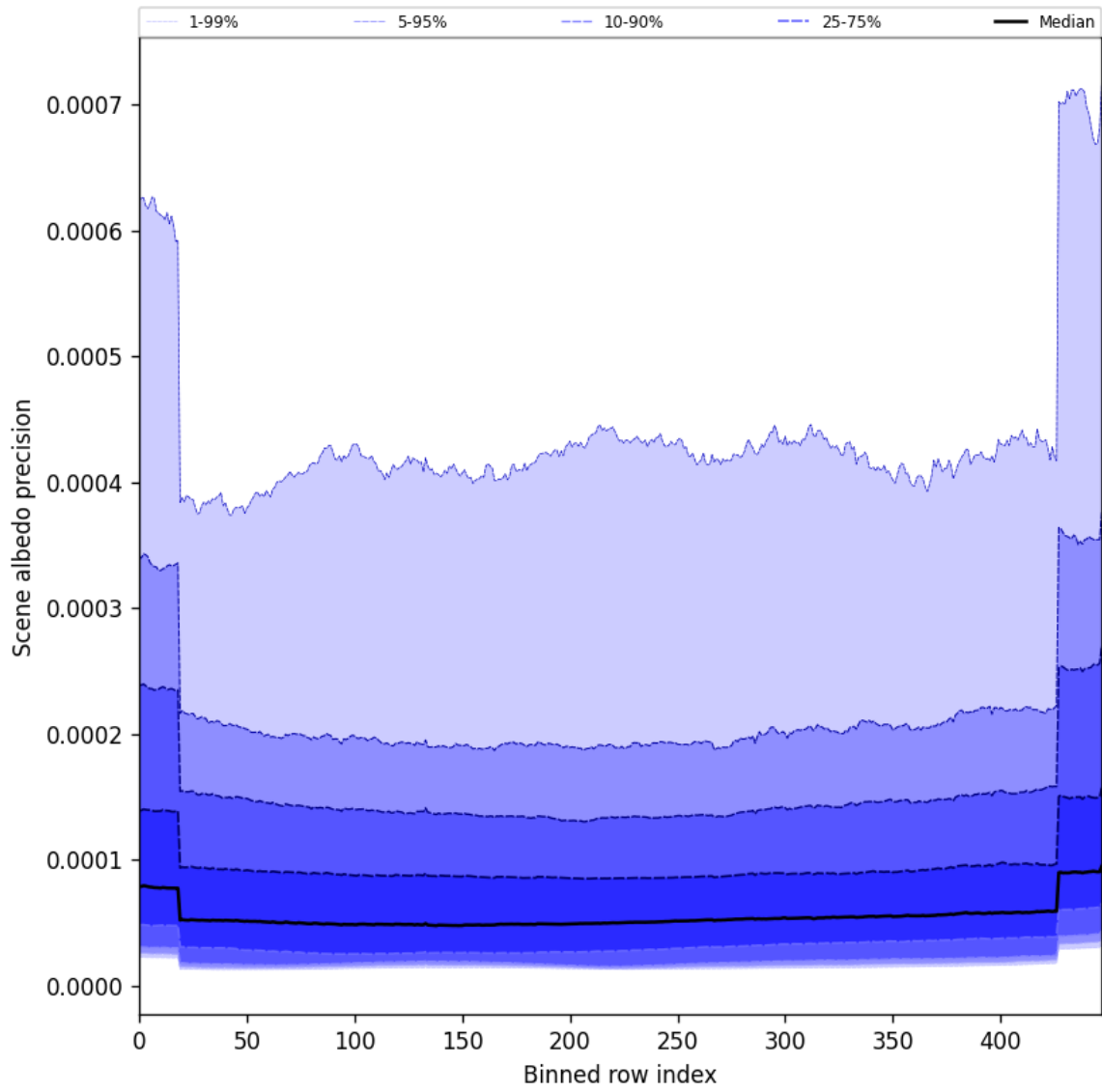
Figure 52: Along track statistics of “Scene albedo precision” for 2024-12-09 to 2024-12-11
