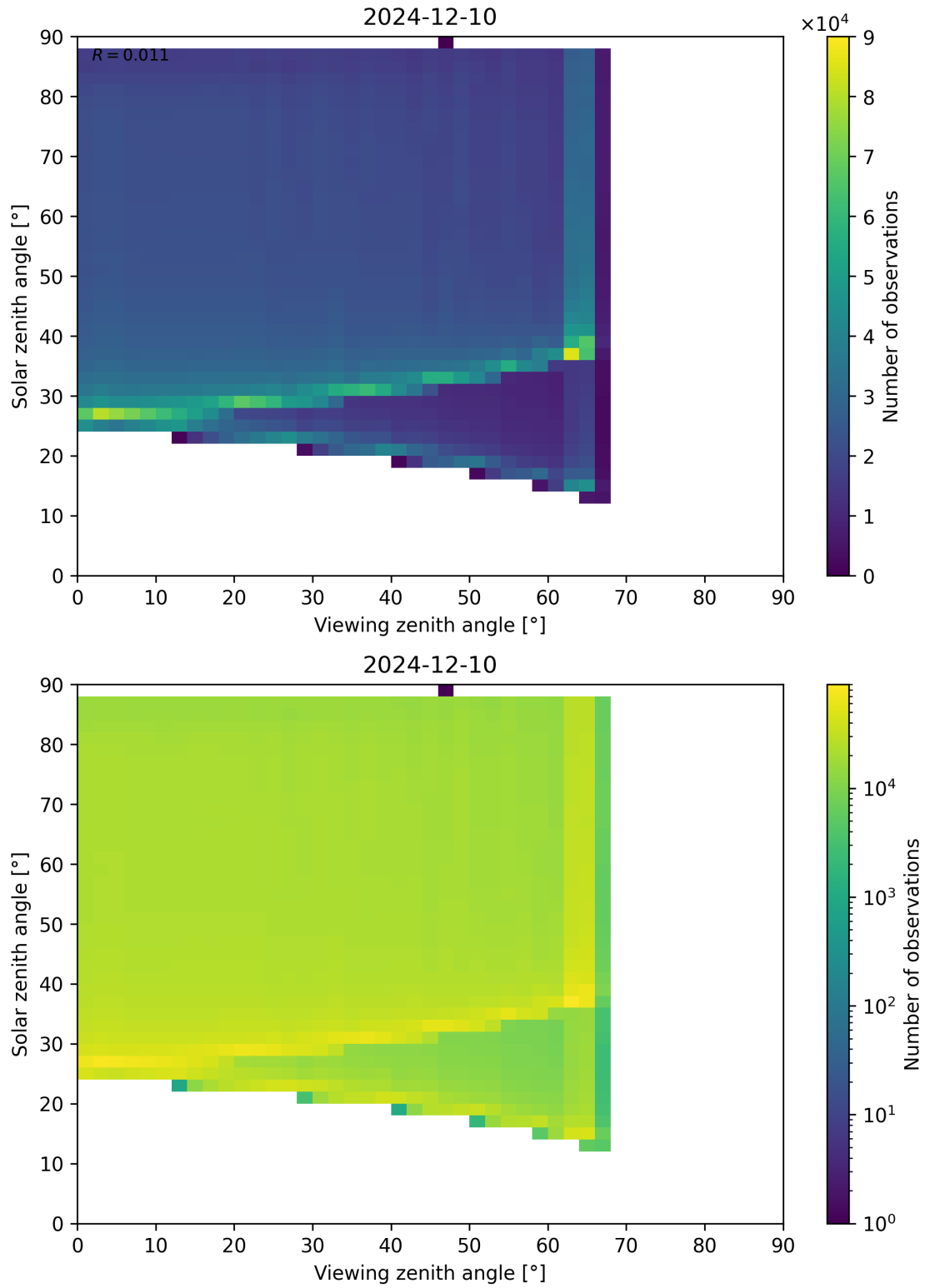
Figure 127: Scatter density plot of “Viewing zenith angle” against “Solar zenith angle” for 2024-12-09 to 2024-12-11.
