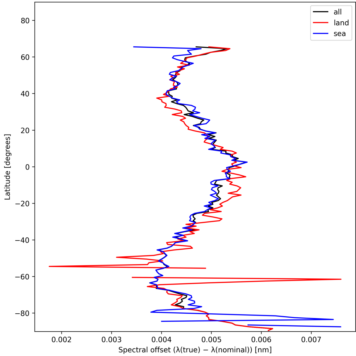
Figure 28: Zonal average of “Spectral offset ( \lambda_{\text{true}} - \lambda_{\text{nominal}} )” for 2024-12-09 to 2024-12-11.
