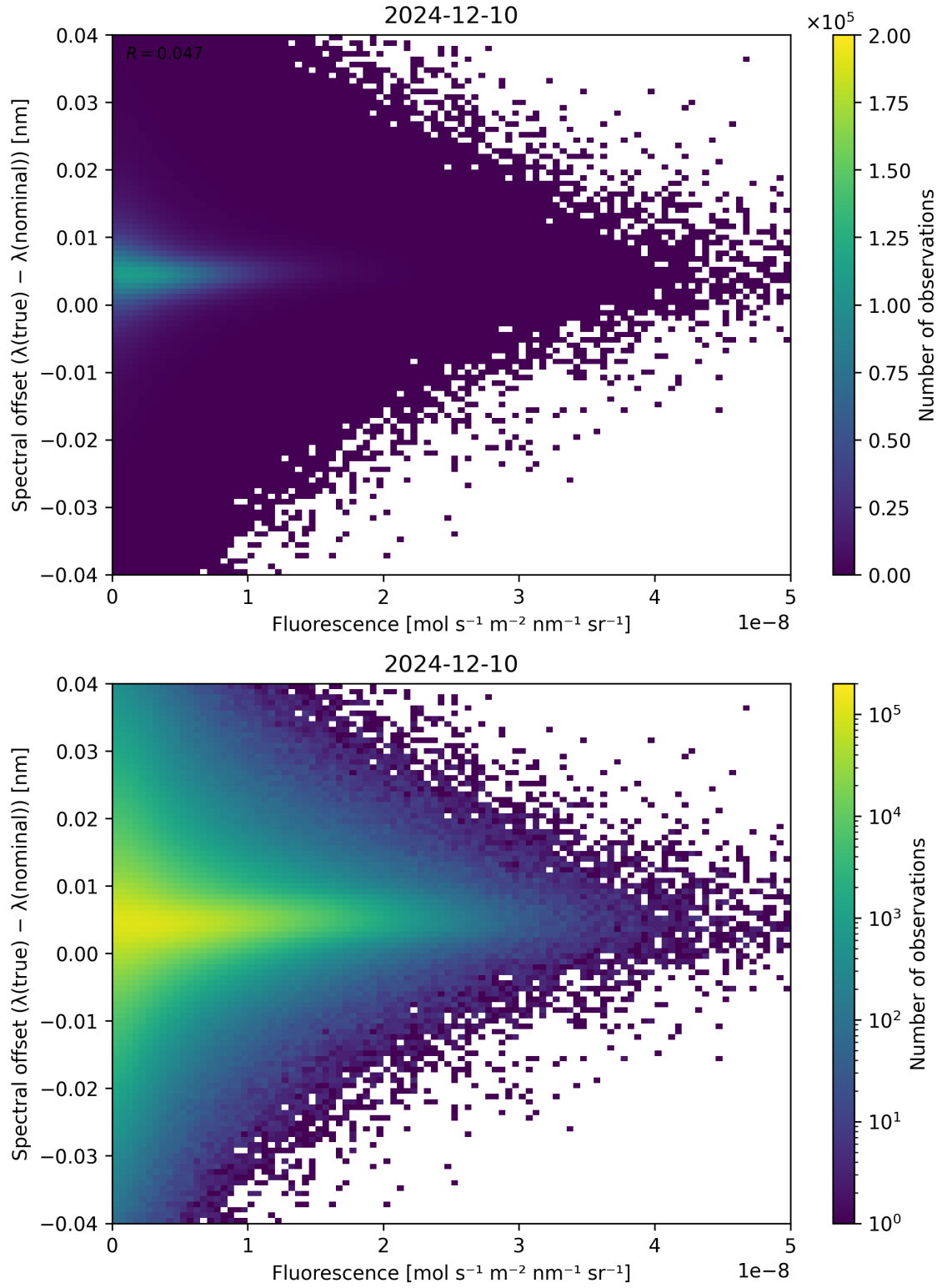
Figure 87: Scatter density plot of “Fluorescence” against “Spectral offset ( \lambda_{\text{true}} - \lambda_{\text{nominal}} )” for 2024-12-09 to 2024-12-11.
