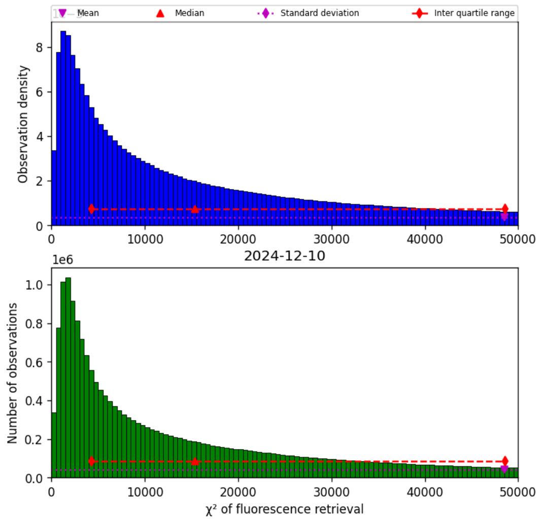
Figure 42: Histogram of “ \chi^2 of fluorescence retrieval” for 2024-12-09 to 2024-12-11
