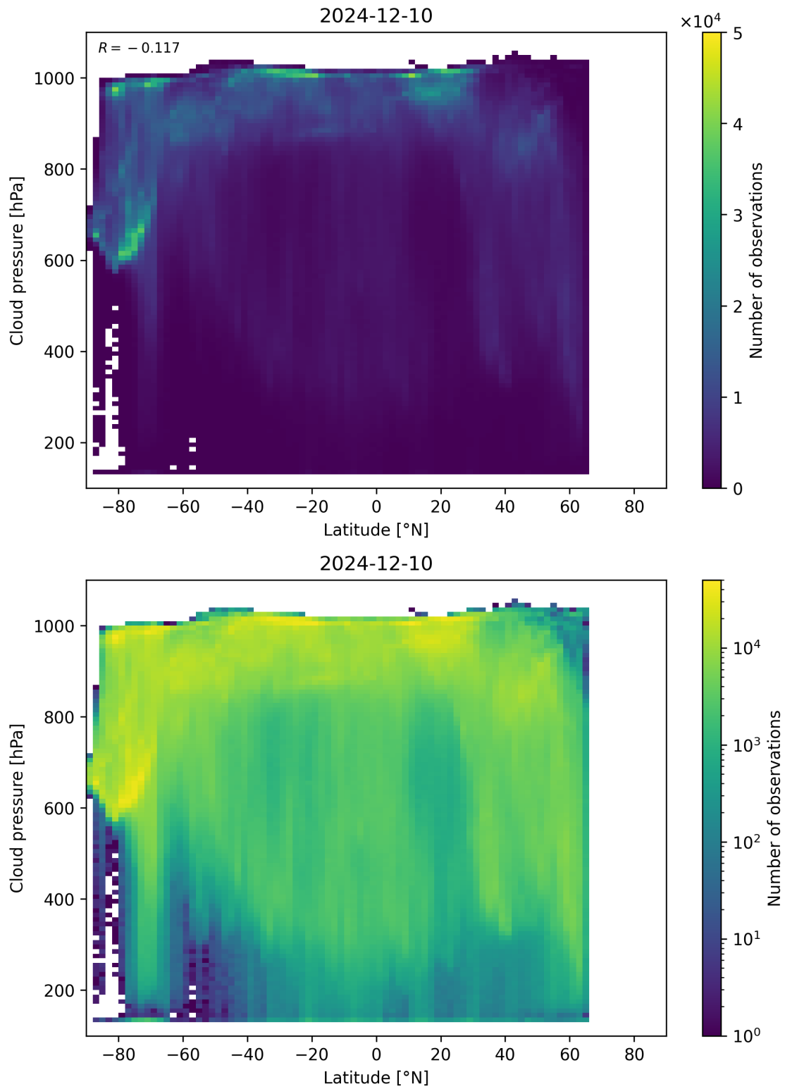
Figure 91: Scatter density plot of “Latitude” against “Cloud pressure” for 2024-12-09 to 2024-12-11.
