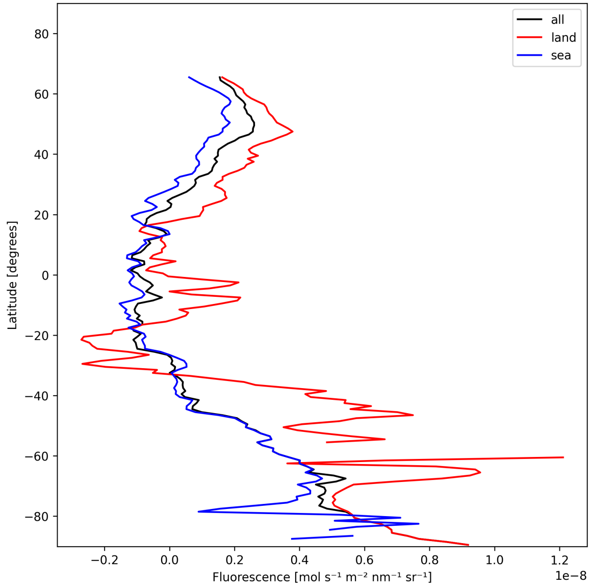
Figure 23: Zonal average of “Fluorescence” for 2024-12-09 to 2024-12-11.
