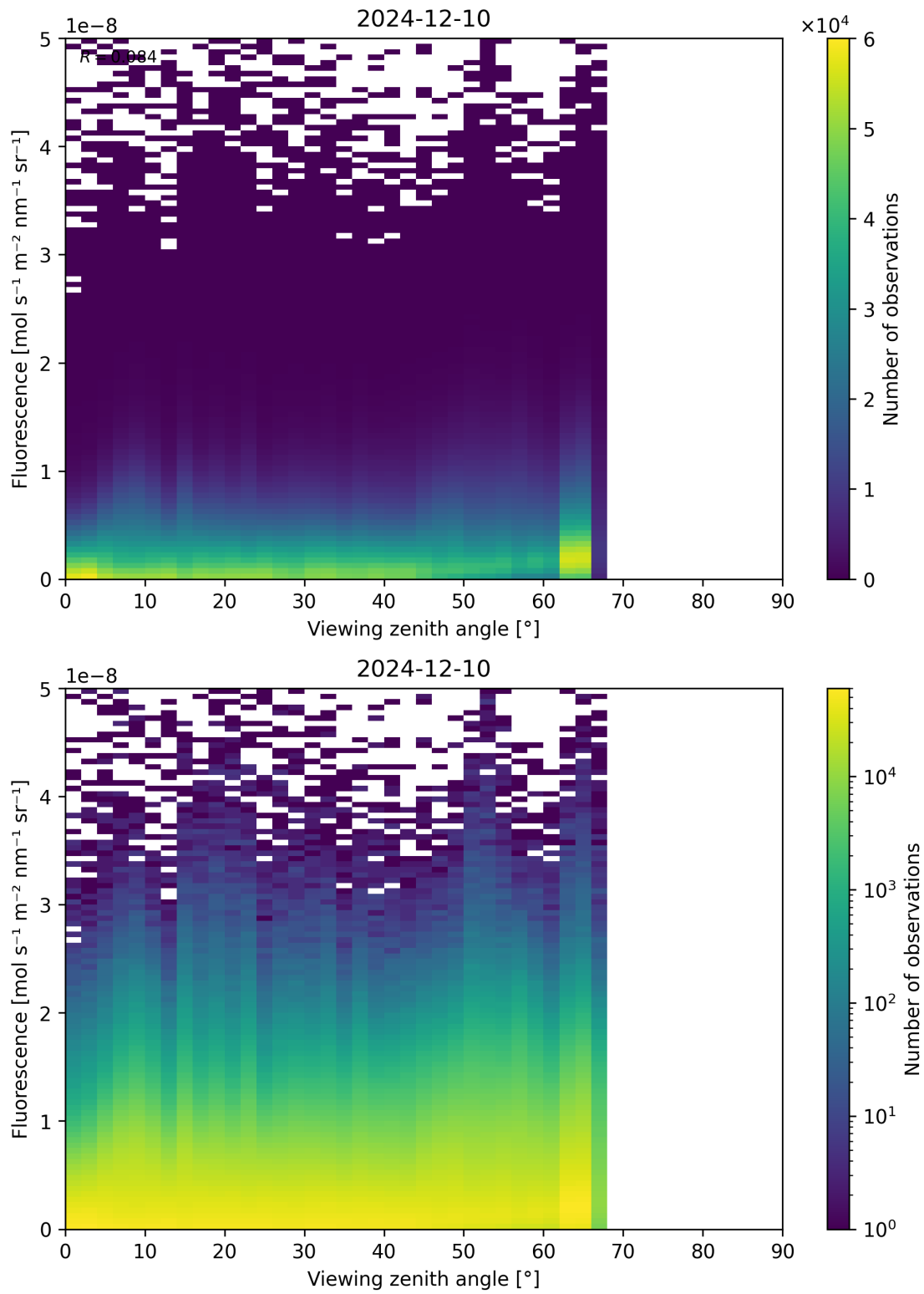
Figure 122: Scatter density plot of “Viewing zenith angle” against “Fluorescence” for 2024-12-09 to 2024-12-11.
