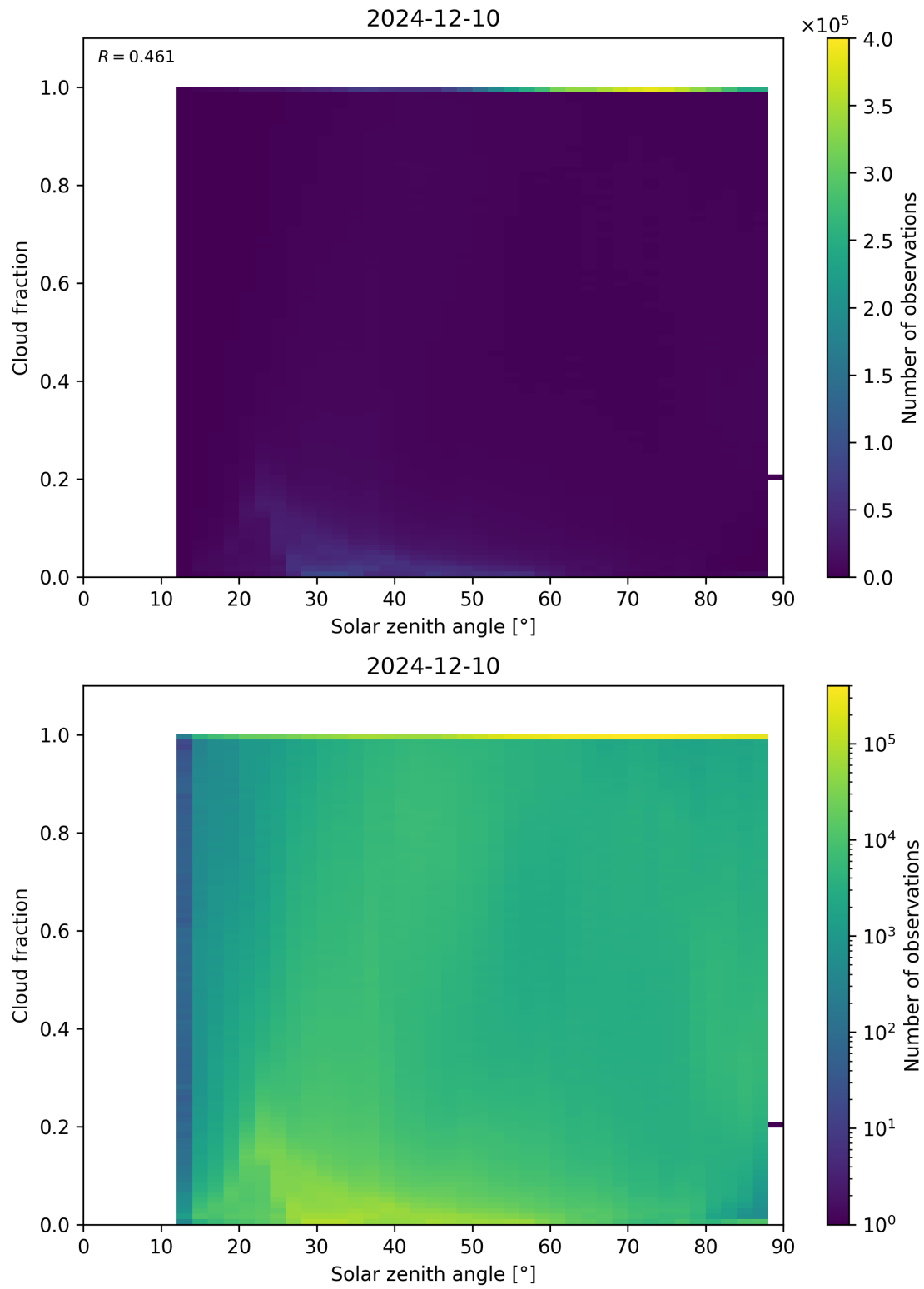
Figure 110: Scatter density plot of “Solar zenith angle” against “Cloud fraction” for 2024-12-09 to 2024-12-11.
