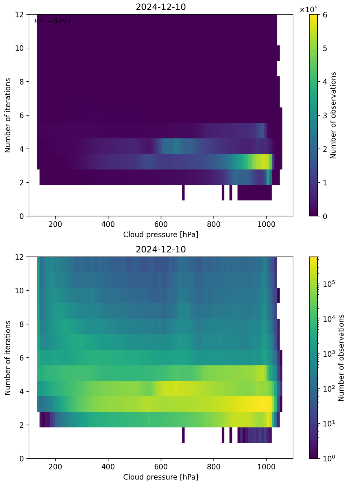
Figure 81: Scatter density plot of “Cloud pressure” against “Number of iterations” for 2024-12-09 to 2024-12-11.
