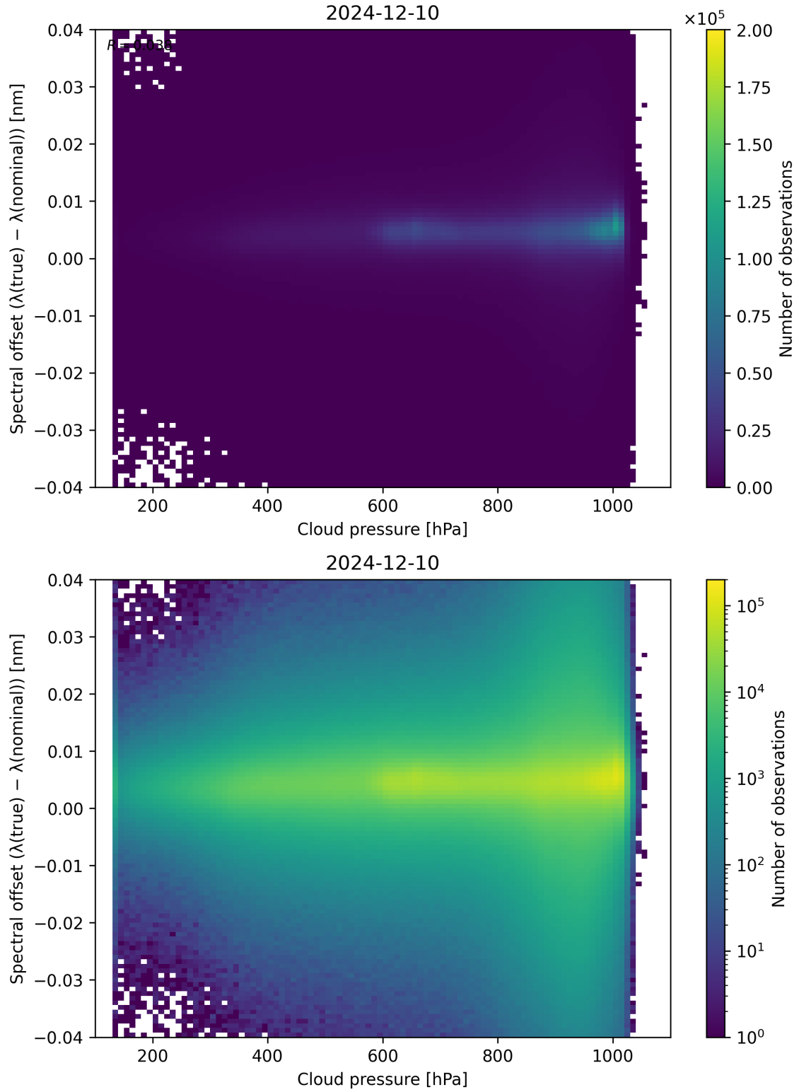
Figure 84: Scatter density plot of “Cloud pressure” against “Spectral offset ( \lambda_{\text{true}} - \lambda_{\text{nominal}} )” for 2024-12-09 to 2024-12-11.
