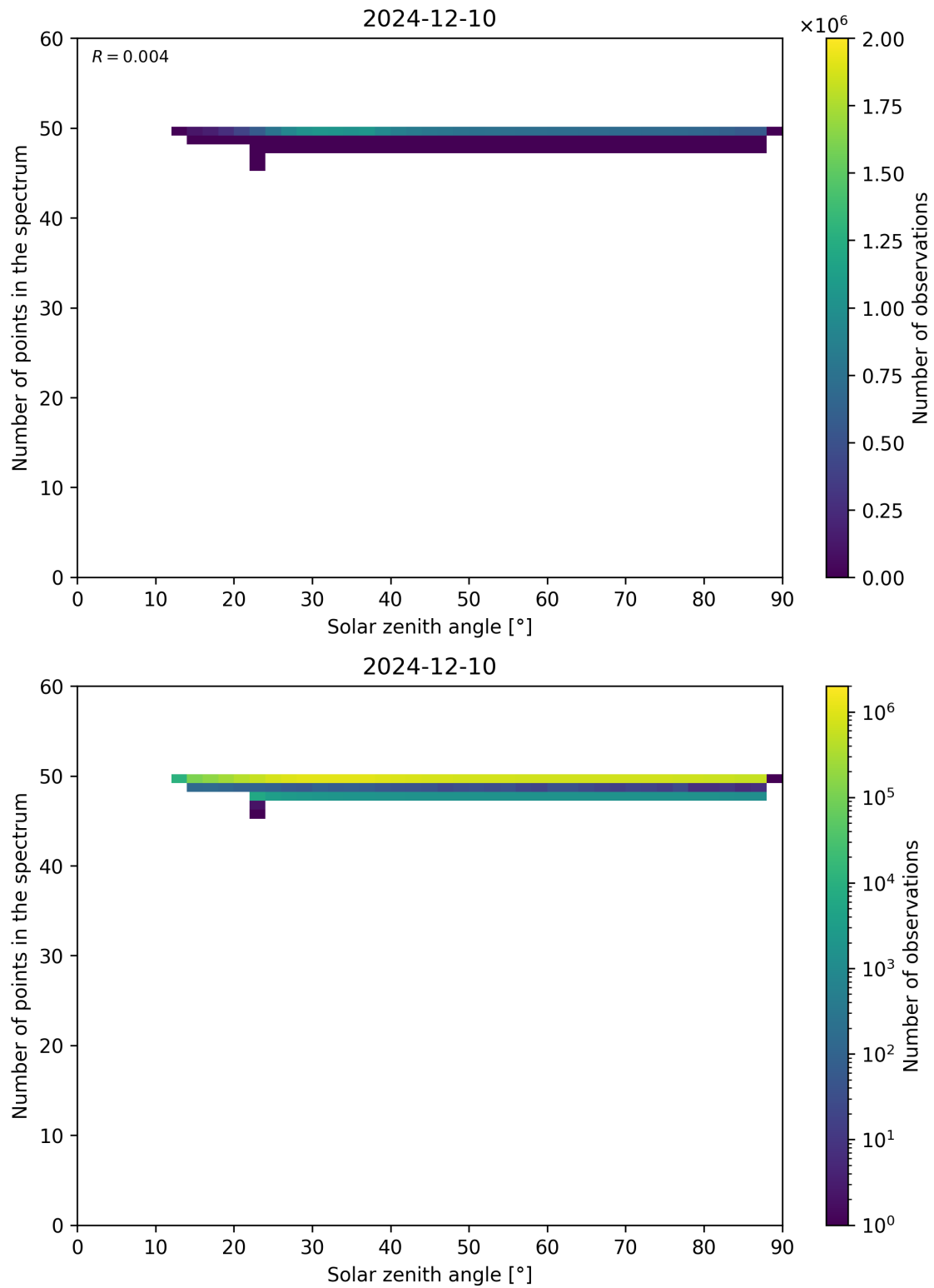
Figure 115: Scatter density plot of “Solar zenith angle” against “Number of points in the spectrum” for 2024-12-09 to 2024-12-11.
