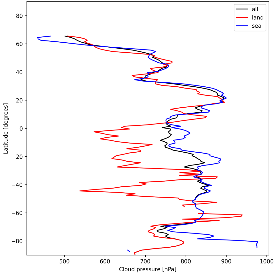
Figure 13: Zonal average of “Cloud pressure” for 2024-12-09 to 2024-12-11.
