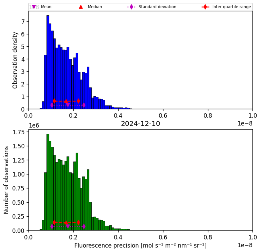
Figure 41: Histogram of “Fluorescence precision” for 2024-12-09 to 2024-12-11
