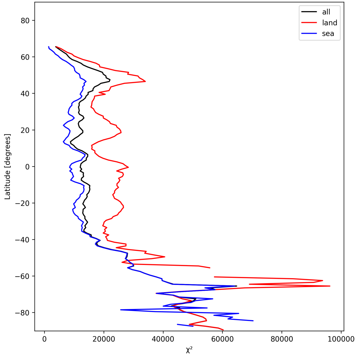
Figure 21: Zonal average of “ \chi^2 ” for 2024-12-09 to 2024-12-11.
