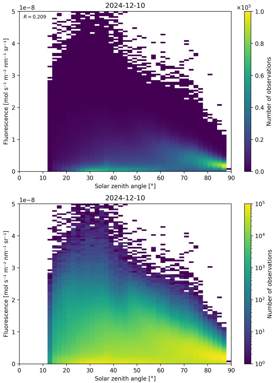
Figure 112: Scatter density plot of “Solar zenith angle” against “Fluorescence” for 2024-12-09 to 2024-12-11.
