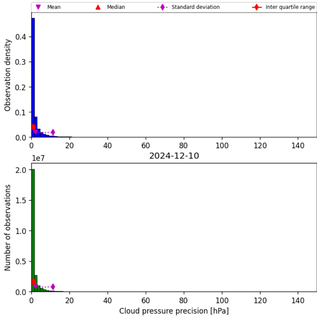
Figure 31: Histogram of “Cloud pressure precision” for 2024-12-09 to 2024-12-11
