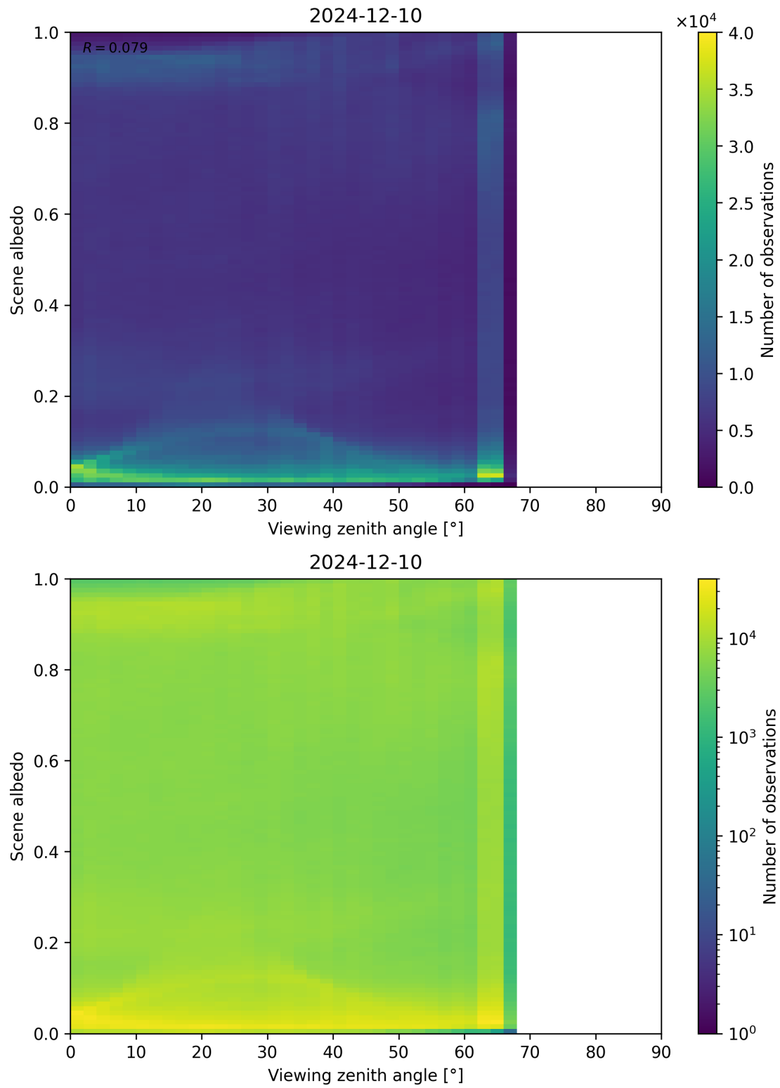
Figure 126: Scatter density plot of “Viewing zenith angle” against “Scene albedo” for 2024-12-09 to 2024-12-11.
