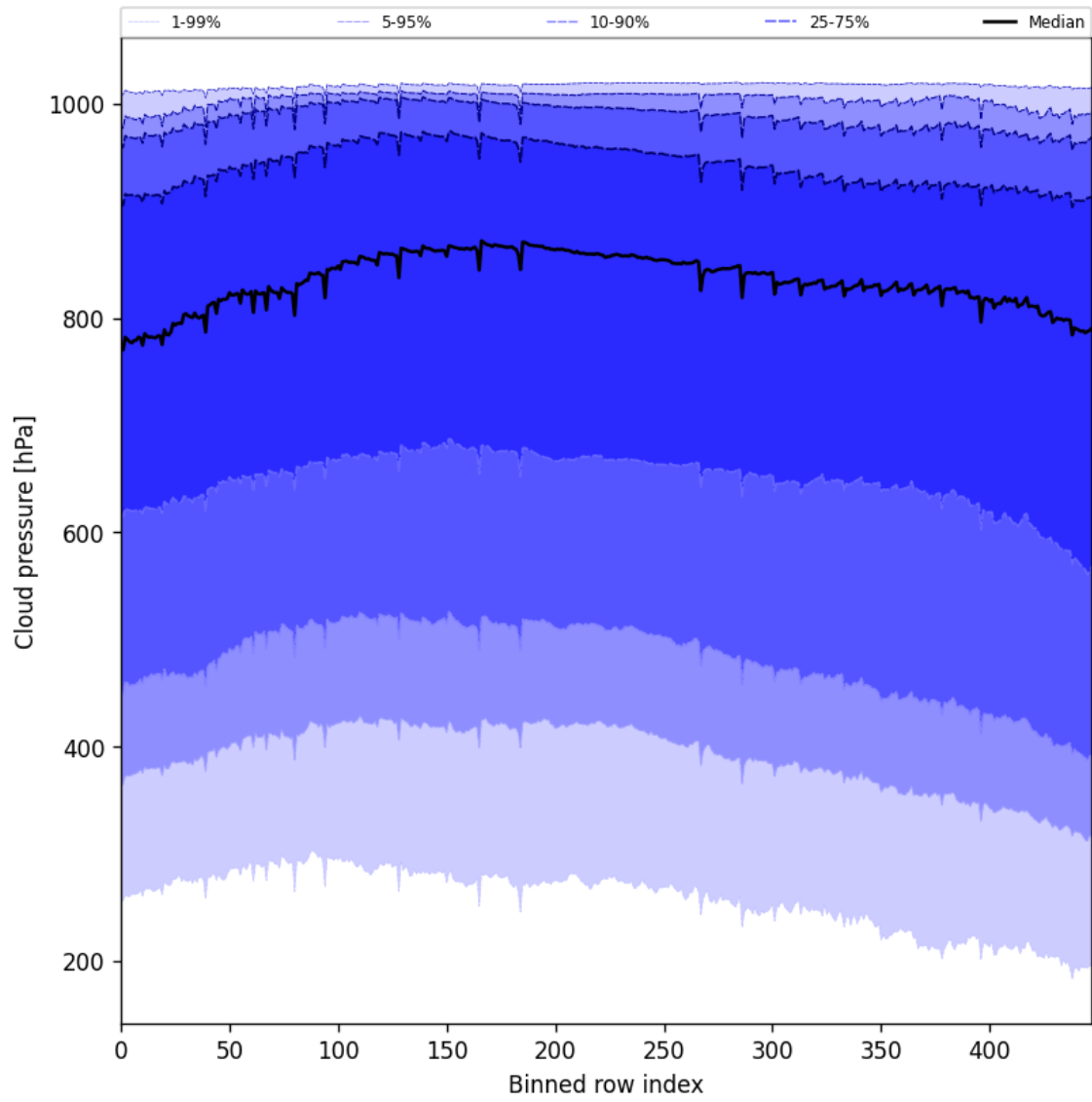
Figure 47: Along track statistics of “Cloud pressure” for 2024-12-09 to 2024-12-11
