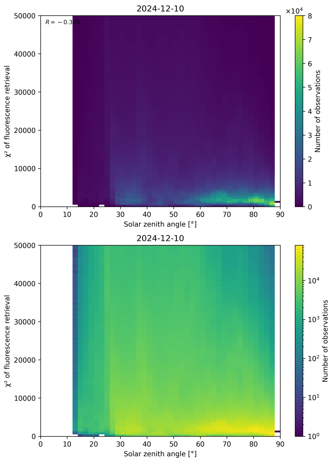
Figure 109: Scatter density plot of “Solar zenith angle” against “ \chi^2 of fluorescence retrieval” for 2024-12-09 to 2024-12-11.
