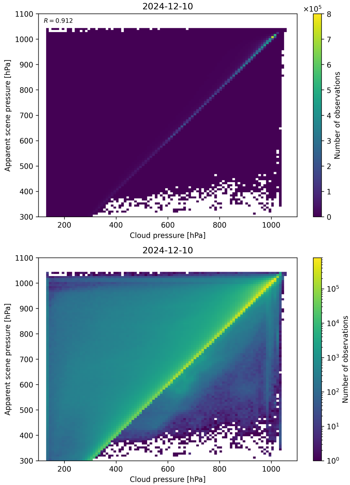
Figure 77: Scatter density plot of “Cloud pressure” against “Apparent scene pressure” for 2024-12-09 to 2024-12-11.
