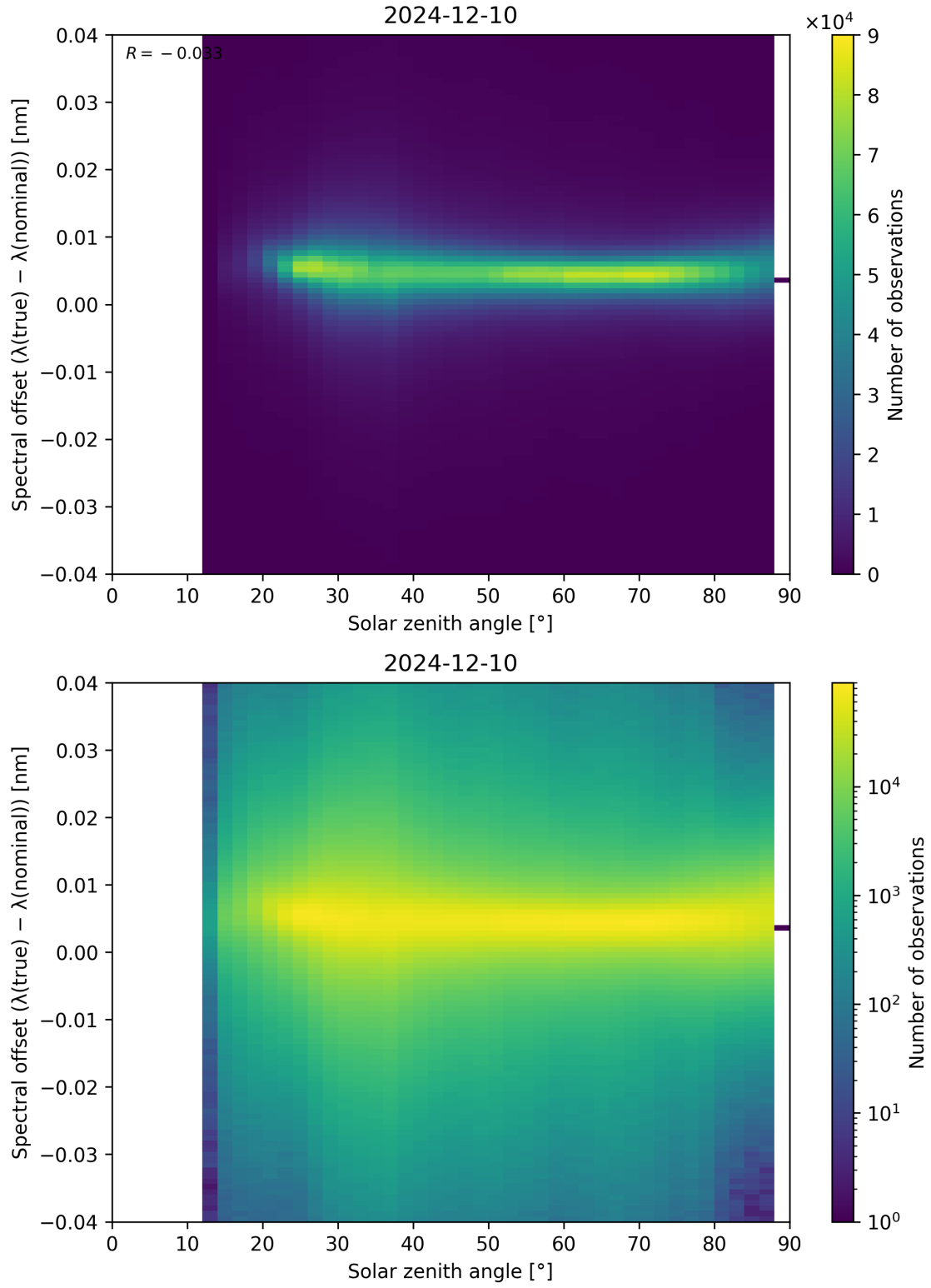
Figure 117: Scatter density plot of “Solar zenith angle” against “Spectral offset ( \lambda_{\text{true}} - \lambda_{\text{nominal}} )” for 2024-12-09 to 2024-12-11.
