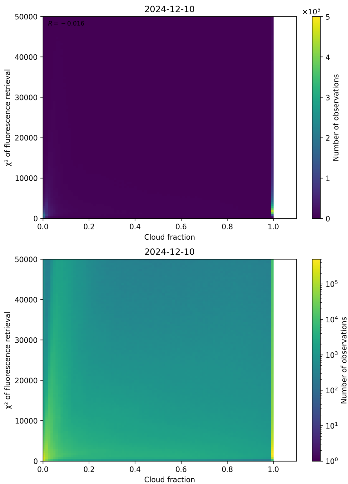
Figure 71: Scatter density plot of “Cloud fraction” against “ \chi^2 of fluorescence retrieval” for 2024-12-09 to 2024-12-11.
