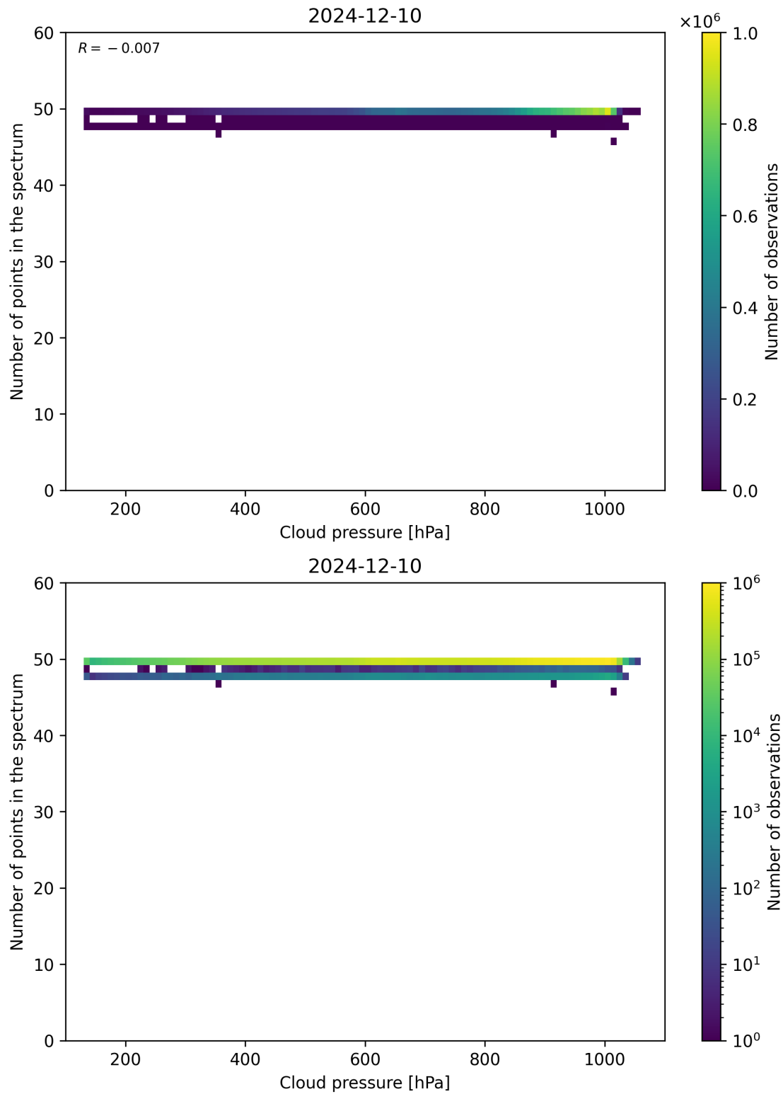
Figure 82: Scatter density plot of “Cloud pressure” against “Number of points in the spectrum” for 2024-12-09 to 2024-12-11.
