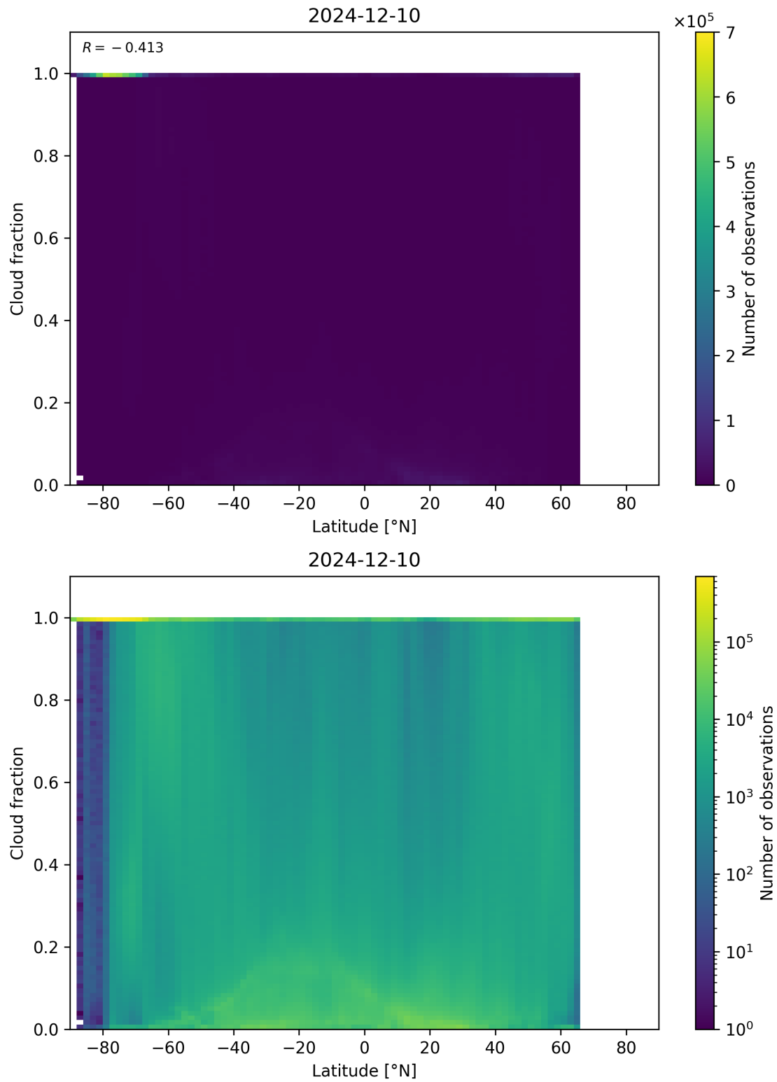
Figure 90: Scatter density plot of “Latitude” against “Cloud fraction” for 2024-12-09 to 2024-12-11.
