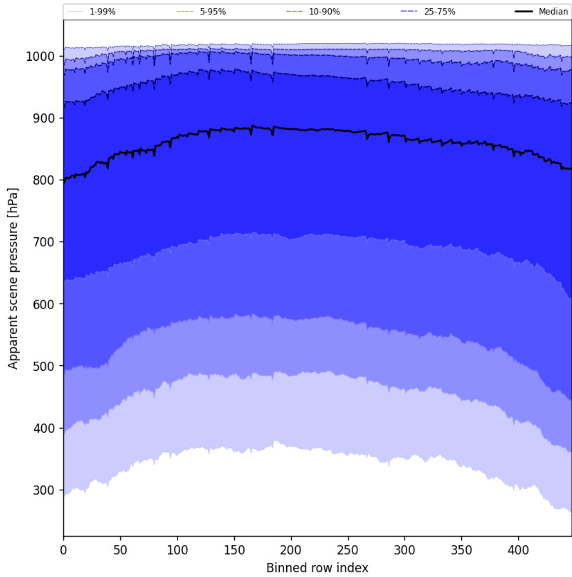
Figure 53: Along track statistics of “Apparent scene pressure” for 2024-12-09 to 2024-12-11
