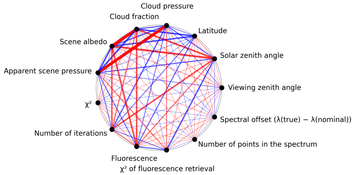
Figure 1: Map of correlation graph for 2024-12-09 to 2024-12-11.
