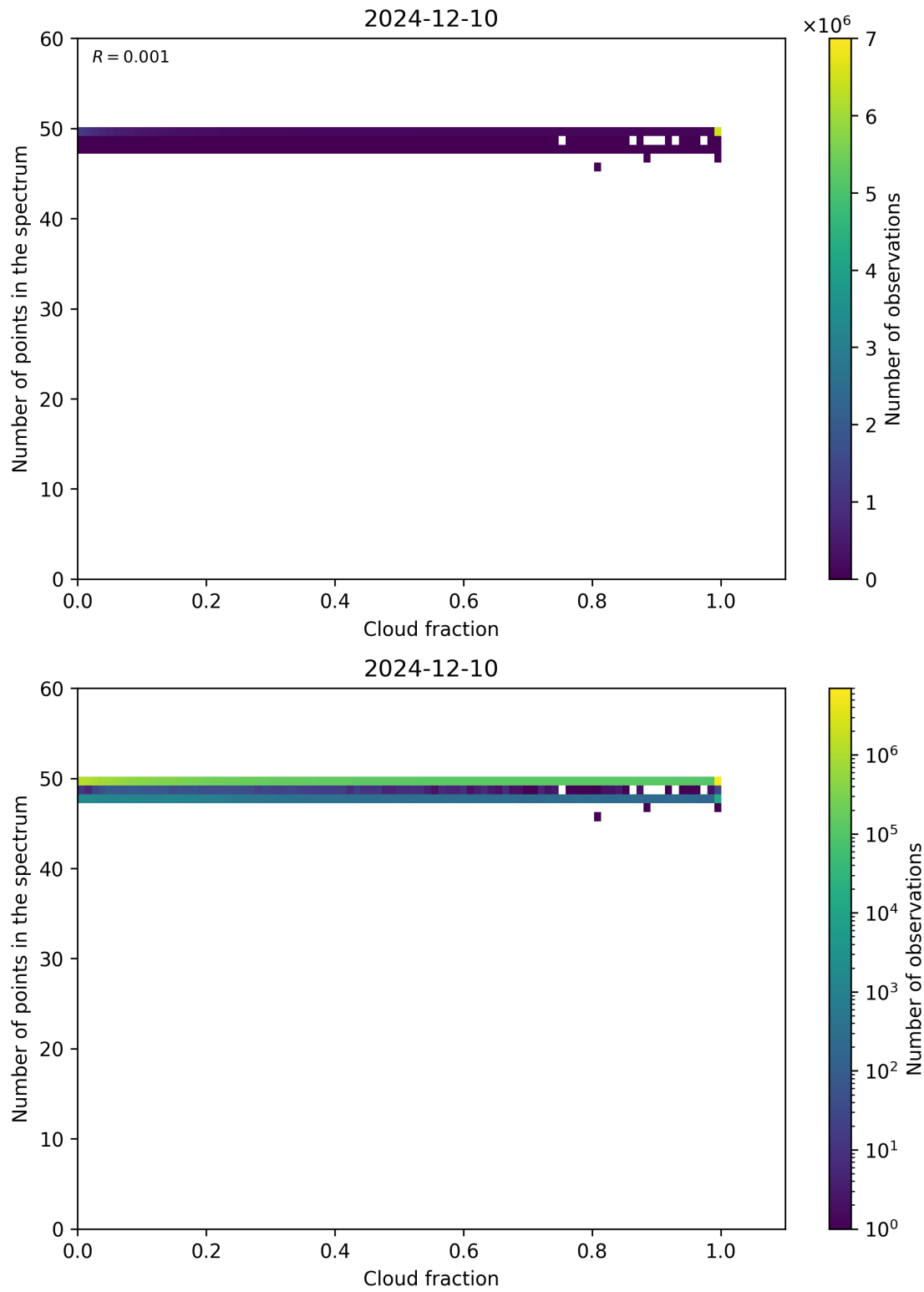
Figure 74: Scatter density plot of “Cloud fraction” against “Number of points in the spectrum” for 2024-12-09 to 2024-12-11.
