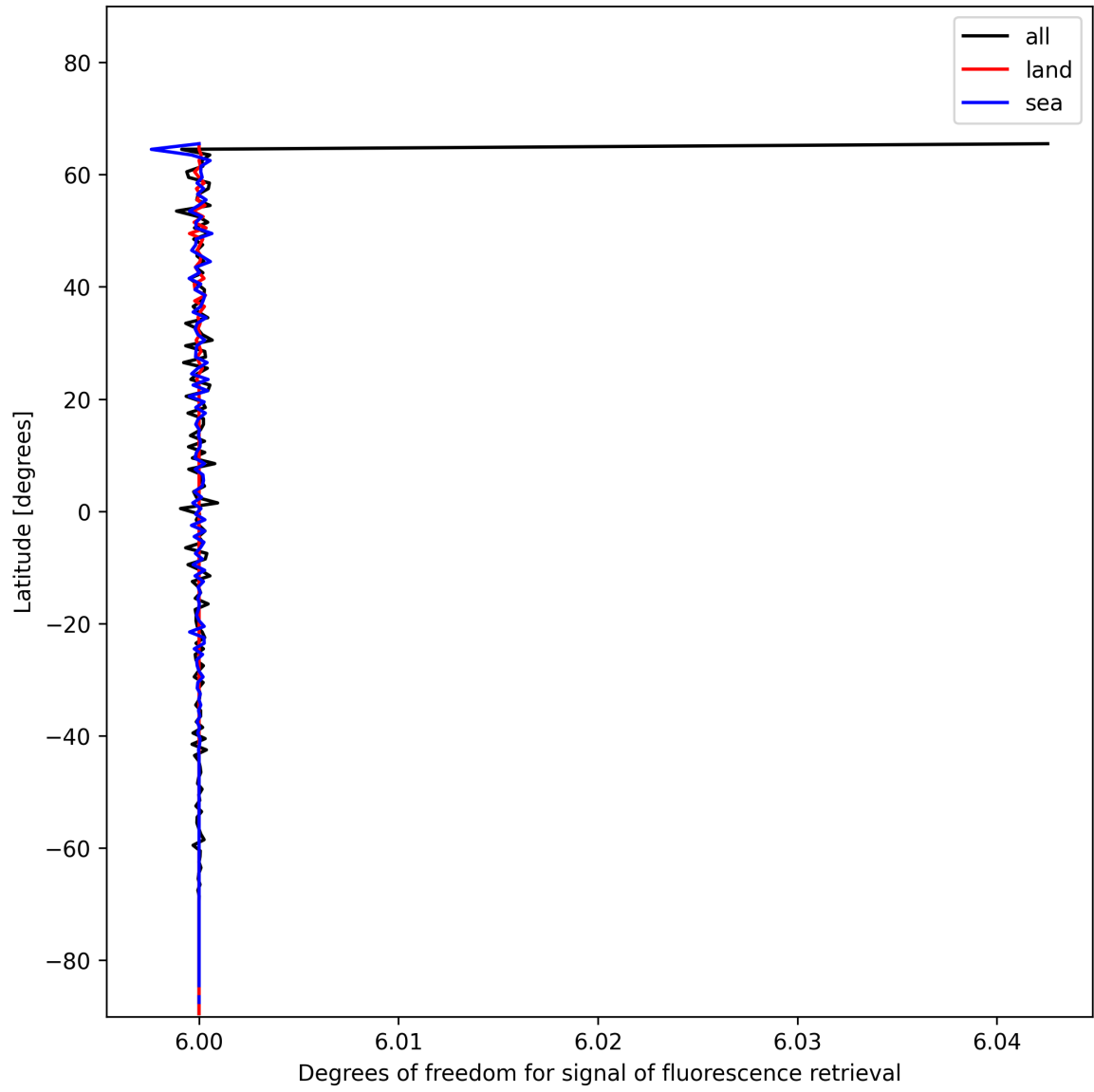
Figure 26: Zonal average of “Degrees of freedom for signal of fluorescence retrieval” for 2024-12-09 to 2024-12-11.
