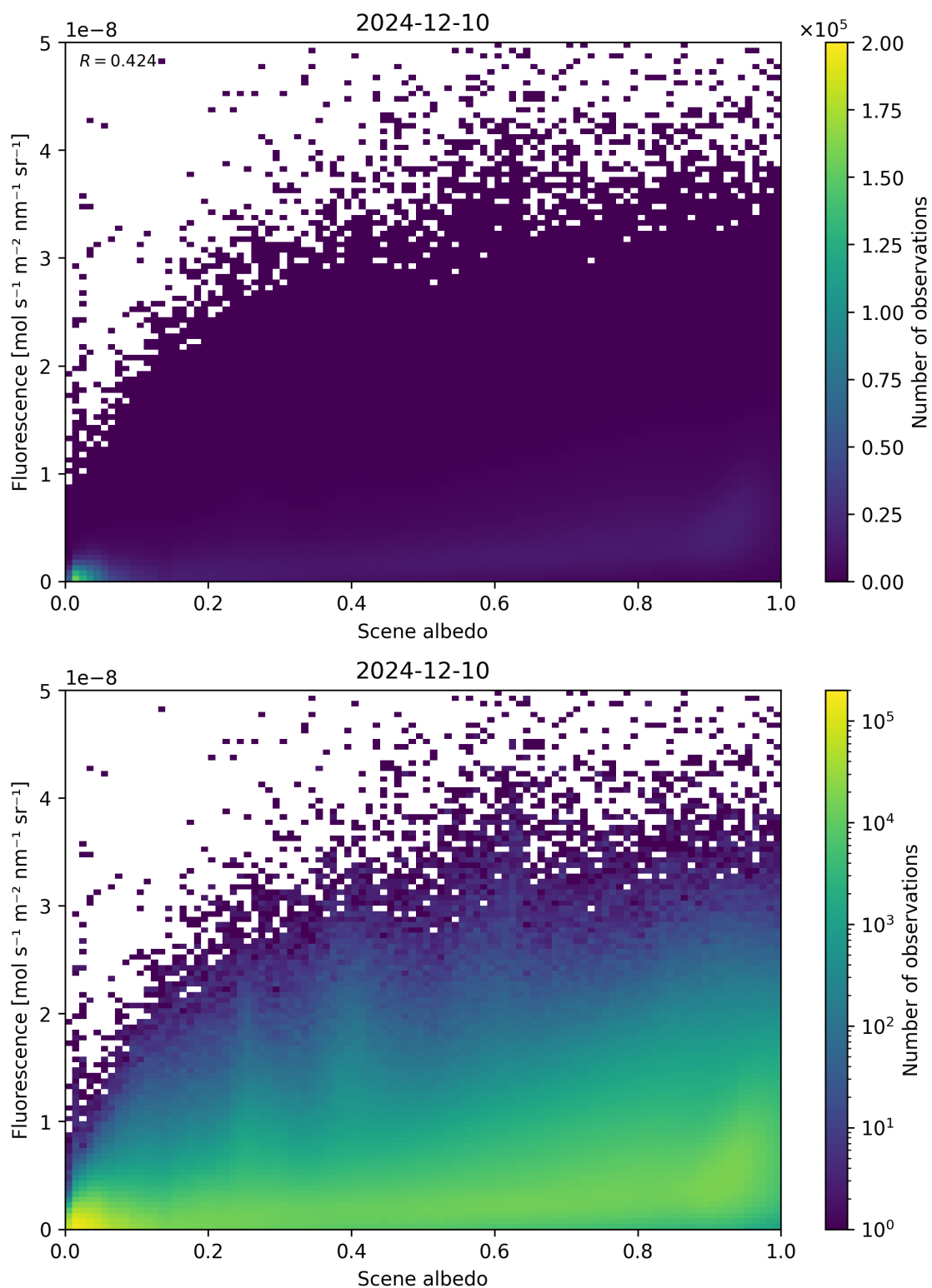
Figure 104: Scatter density plot of “Scene albedo” against “Fluorescence” for 2024-12-09 to 2024-12-11.
