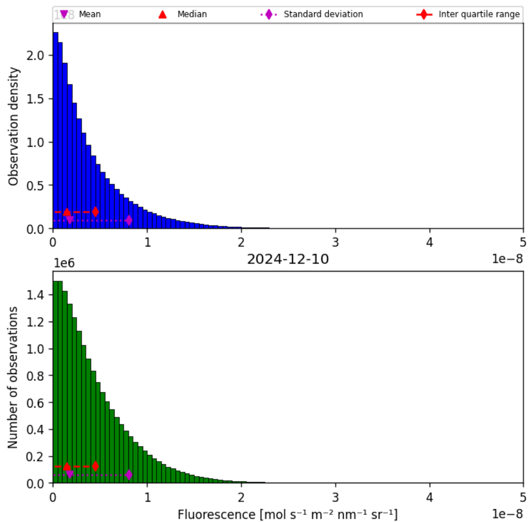
Figure 40: Histogram of “Fluorescence” for 2024-12-09 to 2024-12-11
