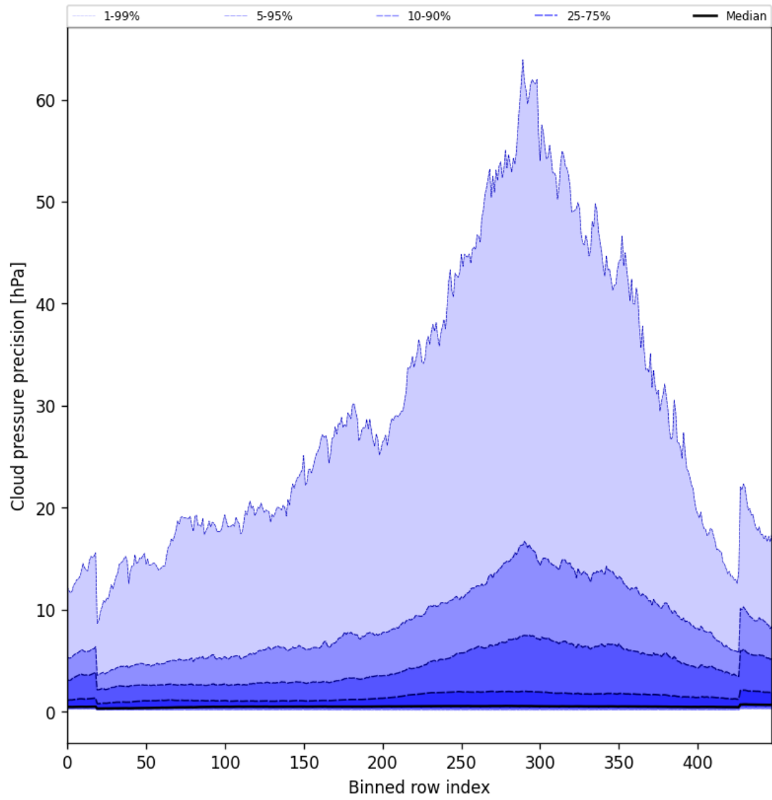
Figure 48: Along track statistics of “Cloud pressure precision” for 2024-12-09 to 2024-12-11
