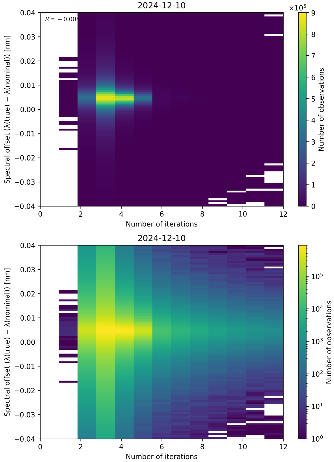
Figure 100: Scatter density plot of “Number of iterations” against “Spectral offset ( \lambda_{\text{true}} - \lambda_{\text{nominal}} )” for 2024-12-09 to 2024-12-11.
