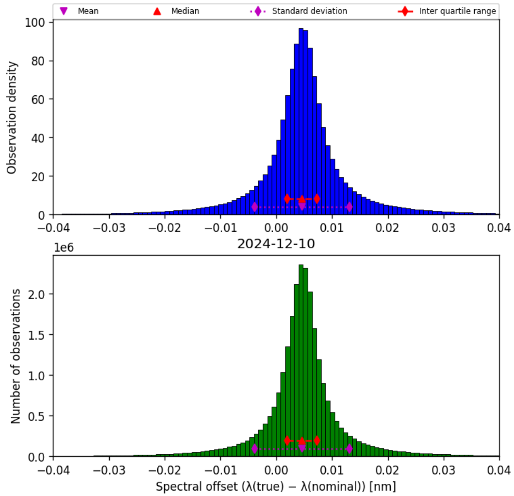
Figure 45: Histogram of “Spectral offset ( \lambda_{\text{true}} - \lambda_{\text{nominal}} )” for 2024-12-09 to 2024-12-11
