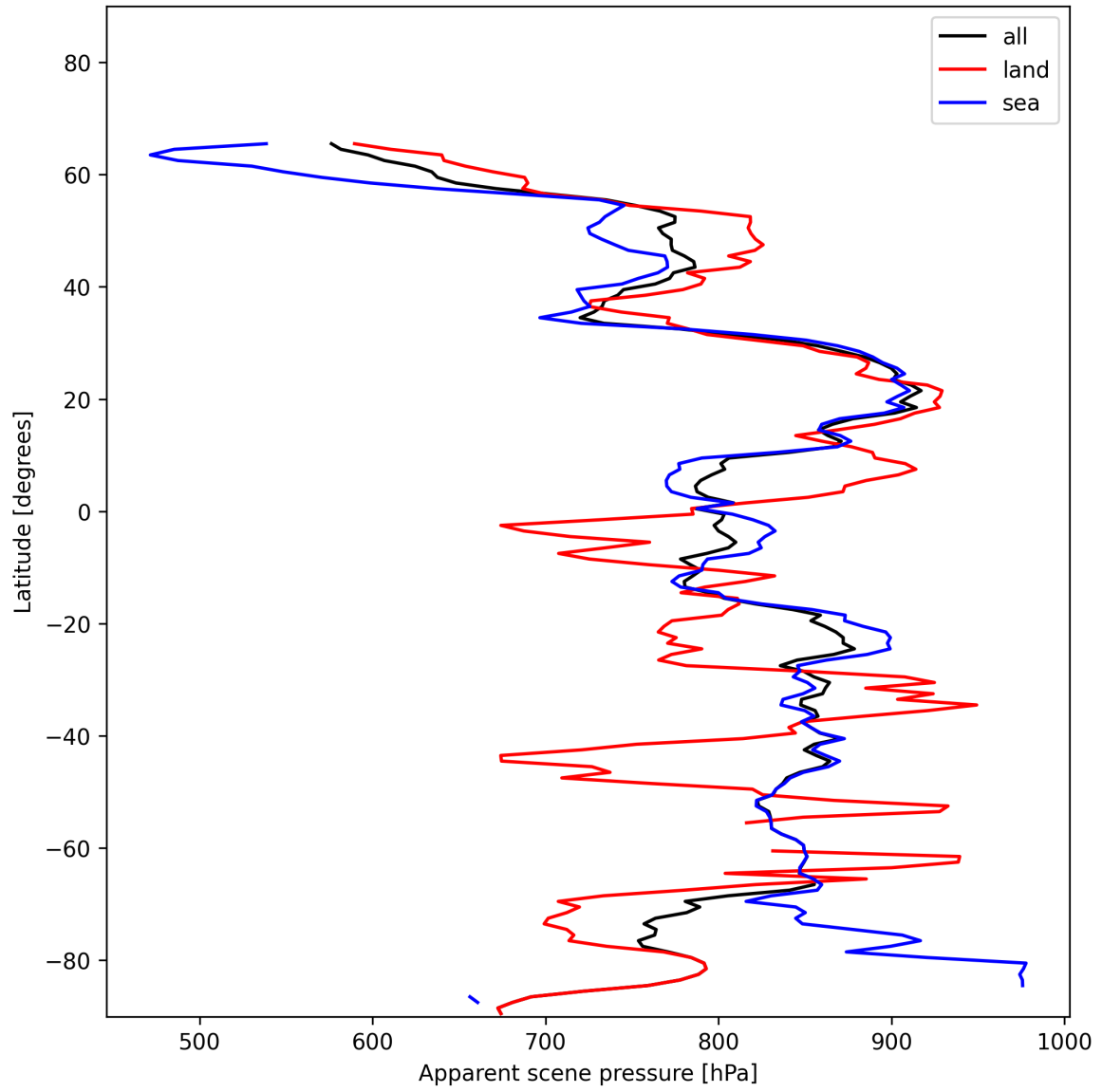
Figure 19: Zonal average of “Apparent scene pressure” for 2024-12-09 to 2024-12-11.
