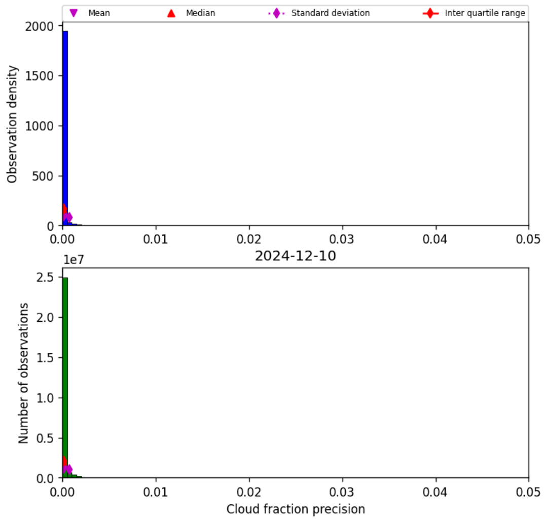
Figure 33: Histogram of “Cloud fraction precision” for 2024-12-09 to 2024-12-11
