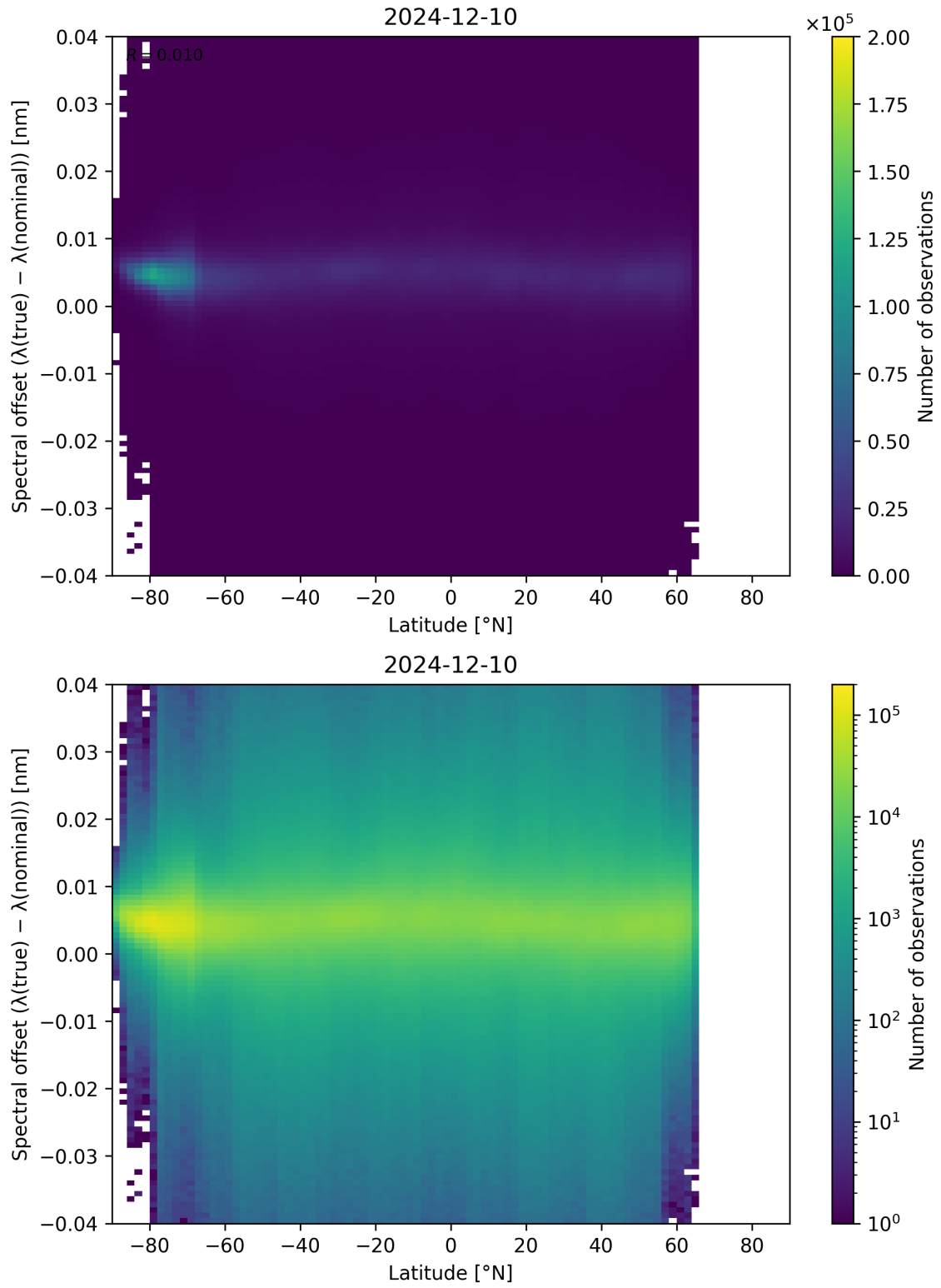
Figure 96: Scatter density plot of “Latitude” against “Spectral offset ( \lambda_{\text{true}} - \lambda_{\text{nominal}} )” for 2024-12-09 to 2024-12-11.
