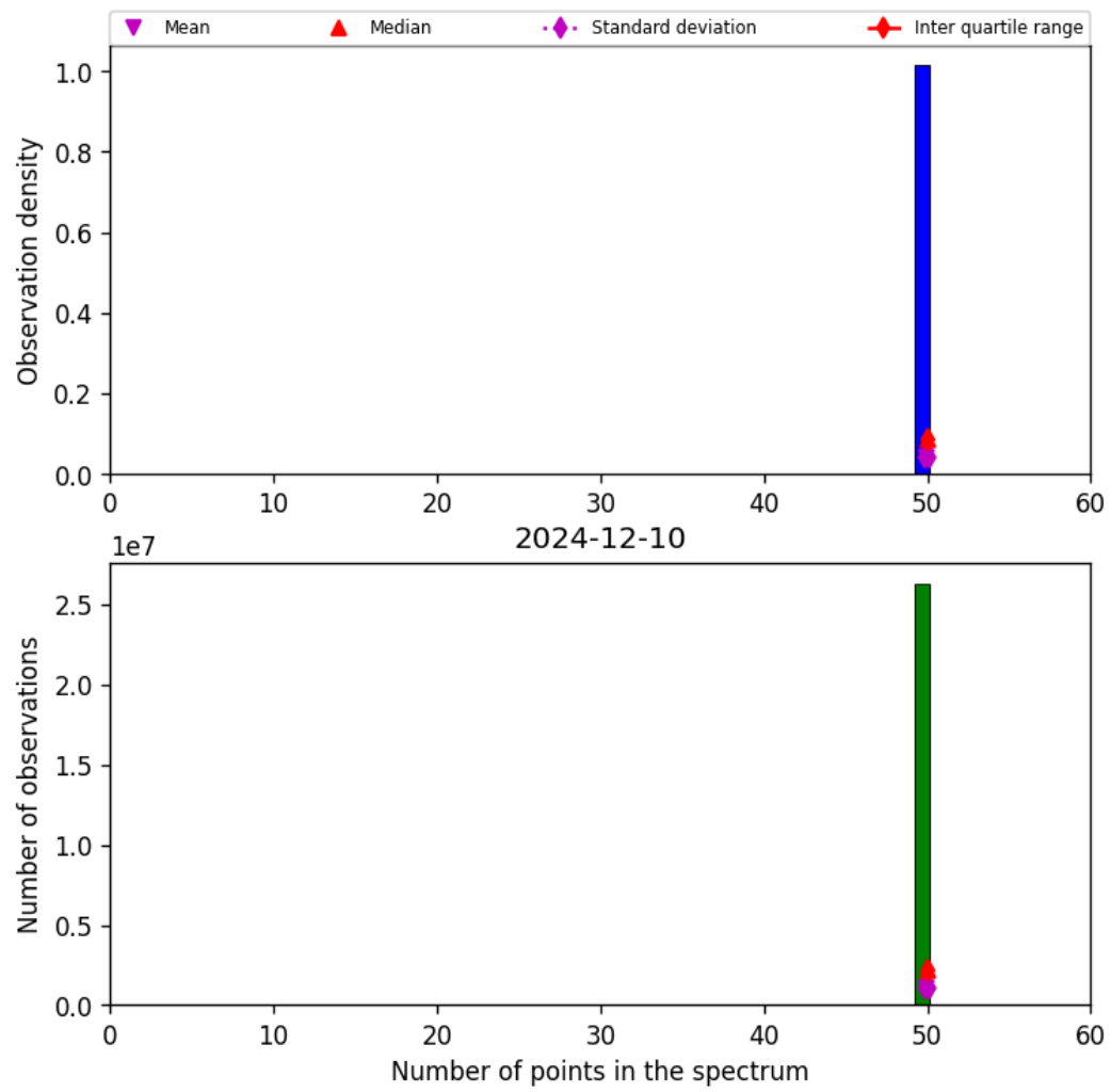
Figure 44: Histogram of “Number of points in the spectrum” for 2024-12-09 to 2024-12-11
