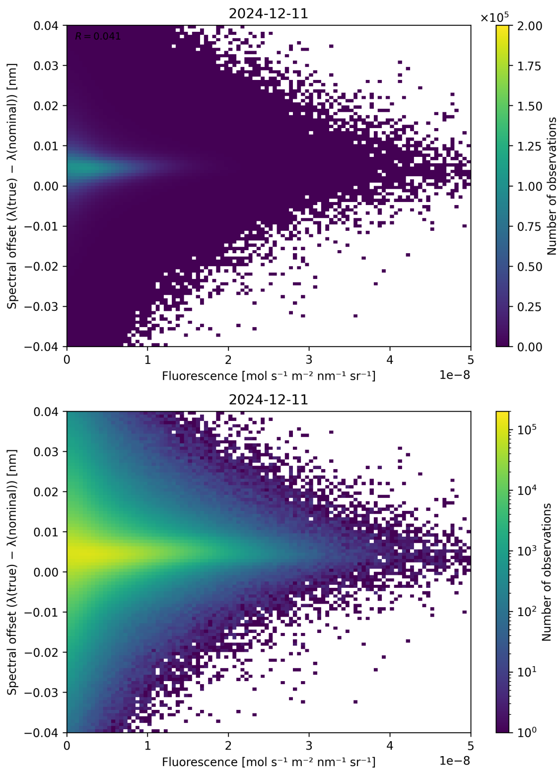
Figure 87: Scatter density plot of “Fluorescence” against “Spectral offset ( \lambda_{\text{true}} - \lambda_{\text{nominal}} )” for 2024-12-11 to 2024-12-12.
