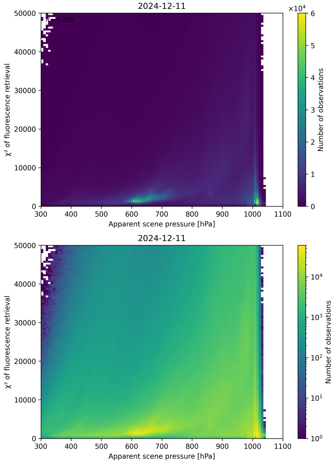
Figure 63: Scatter density plot of “Apparent scene pressure” against “ \chi^2 of fluorescence retrieval” for 2024-12-11 to 2024-12-12.
