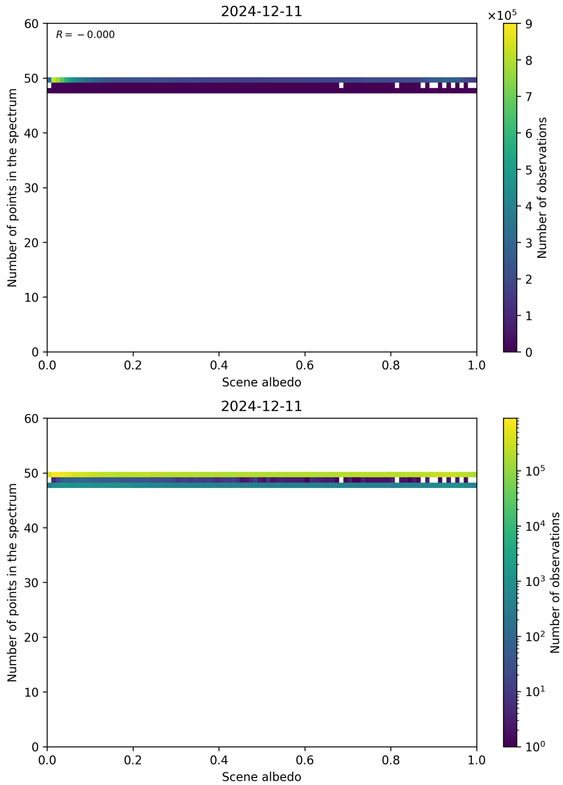
Figure 106: Scatter density plot of “Scene albedo” against “Number of points in the spectrum” for 2024-12-11 to 2024-12-12.
