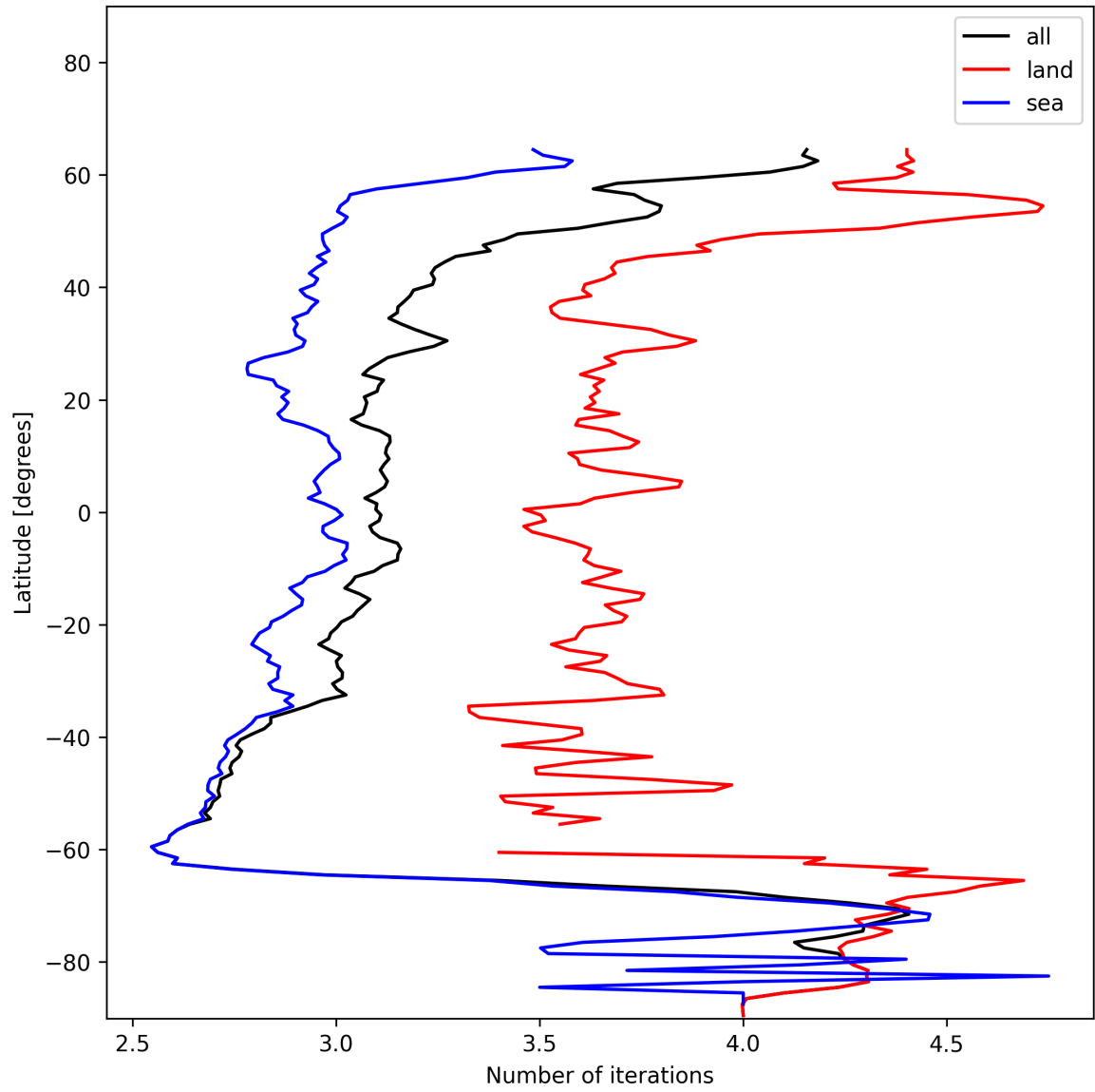
Figure 22: Zonal average of “Number of iterations” for 2024-12-11 to 2024-12-12.
