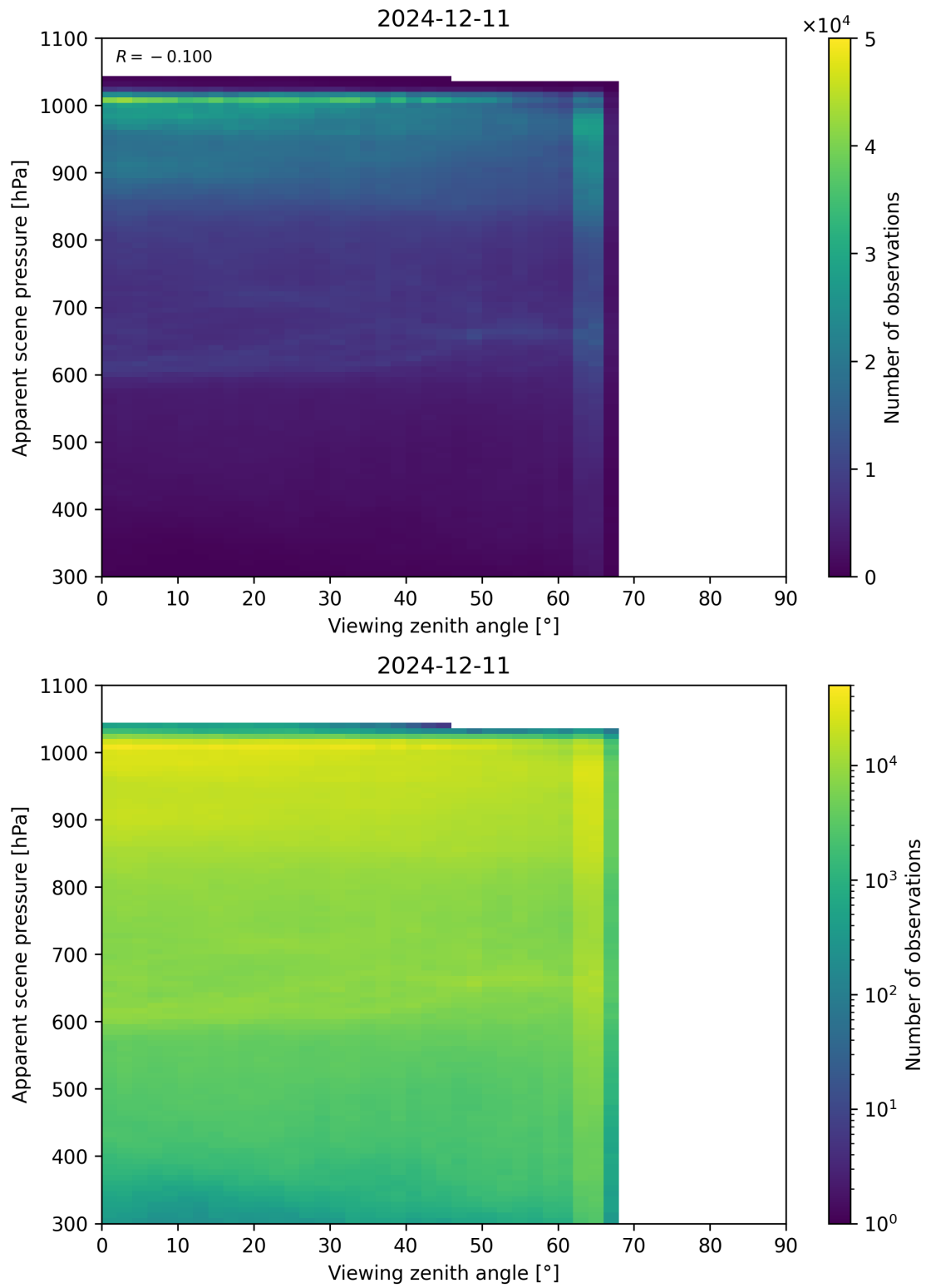
Figure 118: Scatter density plot of “Viewing zenith angle” against “Apparent scene pressure” for 2024-12-11 to 2024-12-12.
