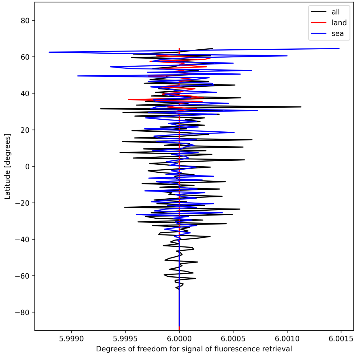
Figure 26: Zonal average of “Degrees of freedom for signal of fluorescence retrieval” for 2024-12-11 to 2024-12-12.
