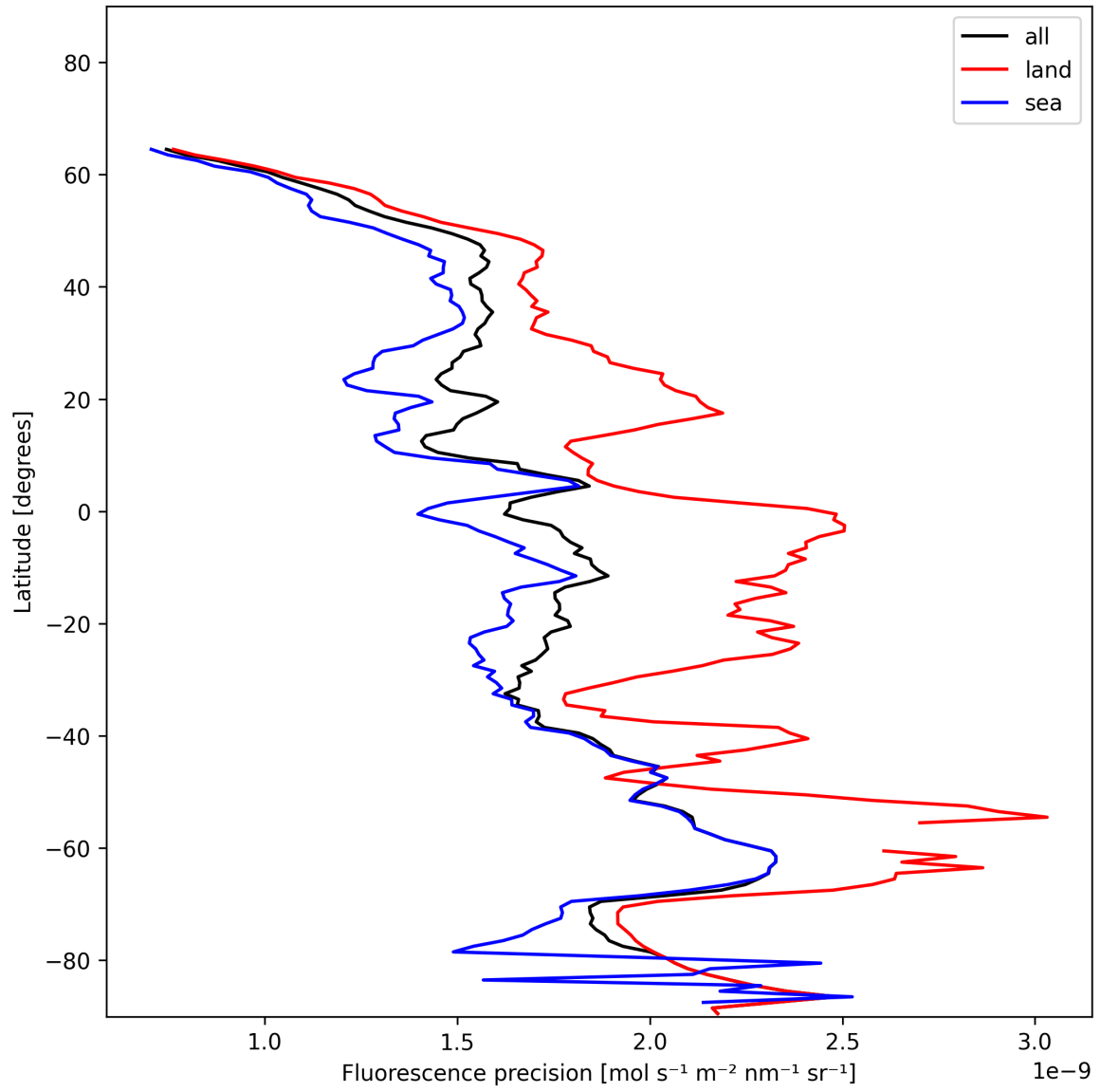
Figure 24: Zonal average of “Fluorescence precision” for 2024-12-11 to 2024-12-12.
