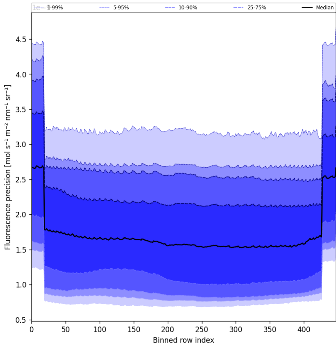
Figure 58: Along track statistics of “Fluorescence precision” for 2024-12-11 to 2024-12-12
