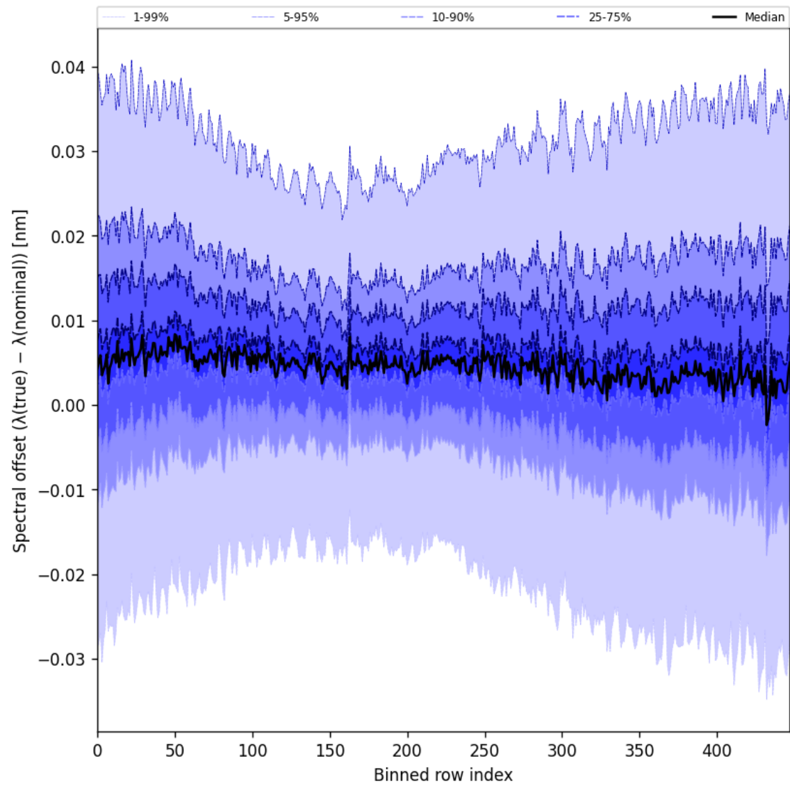
Figure 62: Along track statistics of “Spectral offset ( \lambda_{\text{true}} - \lambda_{\text{nominal}} )” for 2024-12-11 to 2024-12-12
