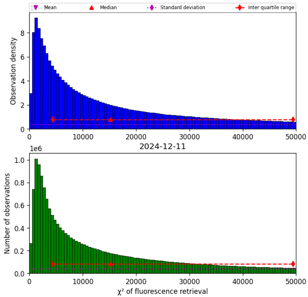
Figure 42: Histogram of “ \chi^2 of fluorescence retrieval” for 2024-12-11 to 2024-12-12
