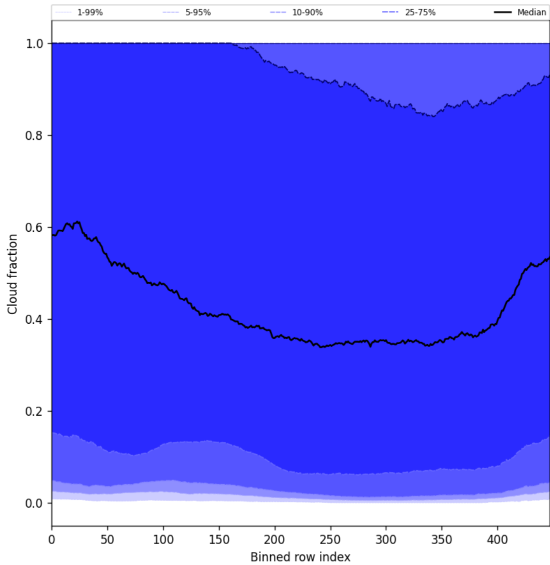
Figure 49: Along track statistics of “Cloud fraction” for 2024-12-11 to 2024-12-12
