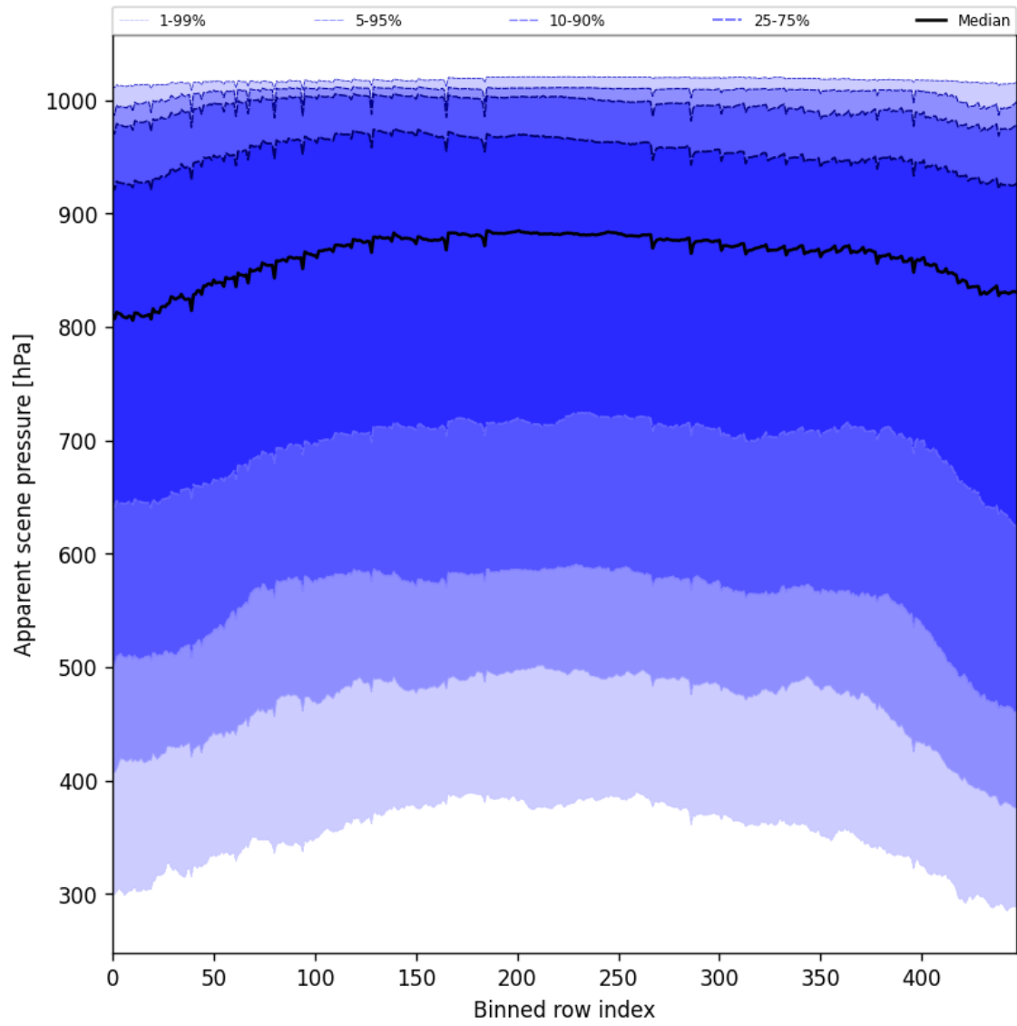
Figure 53: Along track statistics of “Apparent scene pressure” for 2024-12-11 to 2024-12-12
