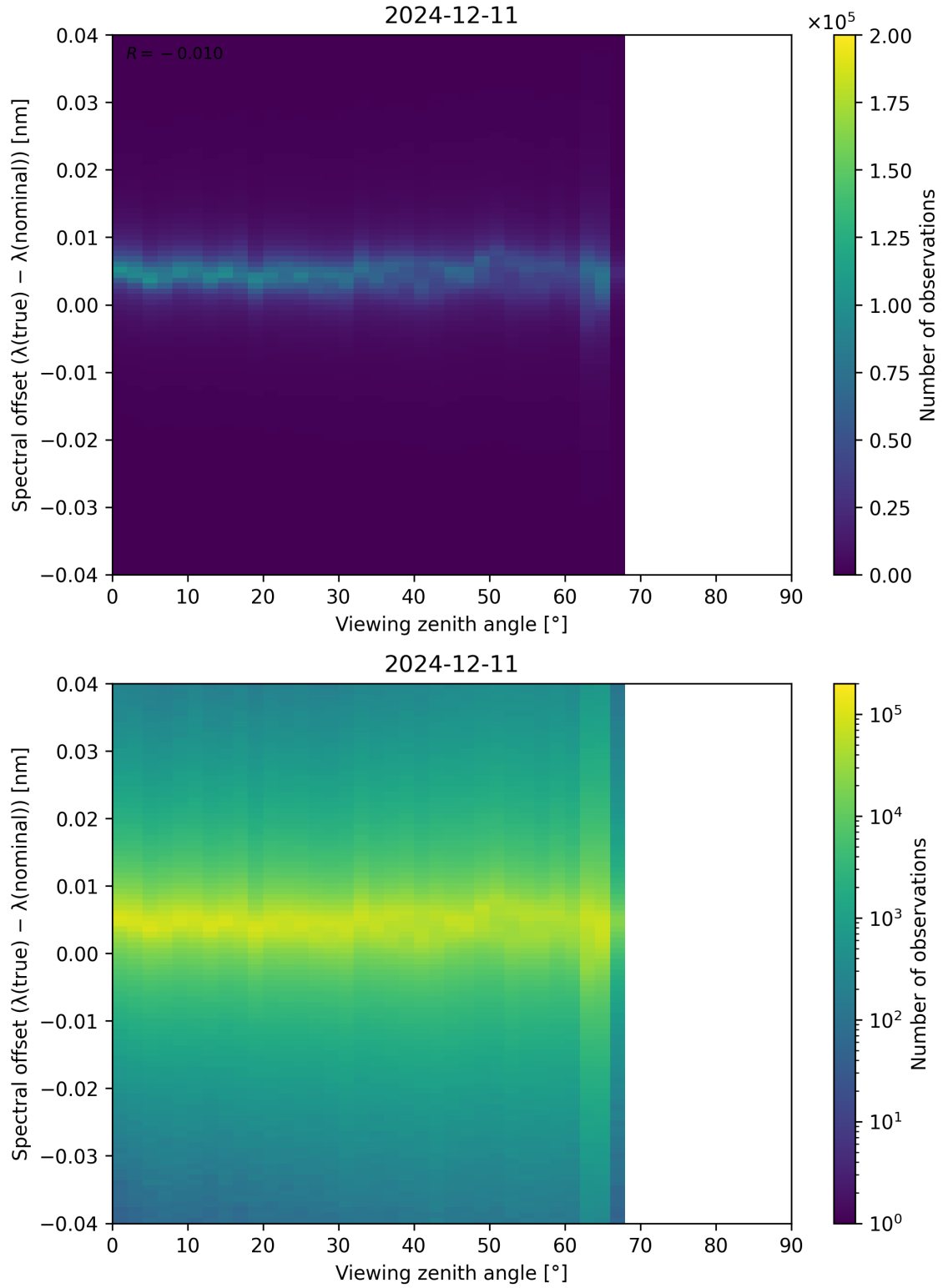
Figure 128: Scatter density plot of “Viewing zenith angle” against “Spectral offset ( \lambda_{\text{true}} - \lambda_{\text{nominal}} )” for 2024-12-11 to 2024-12-12.
