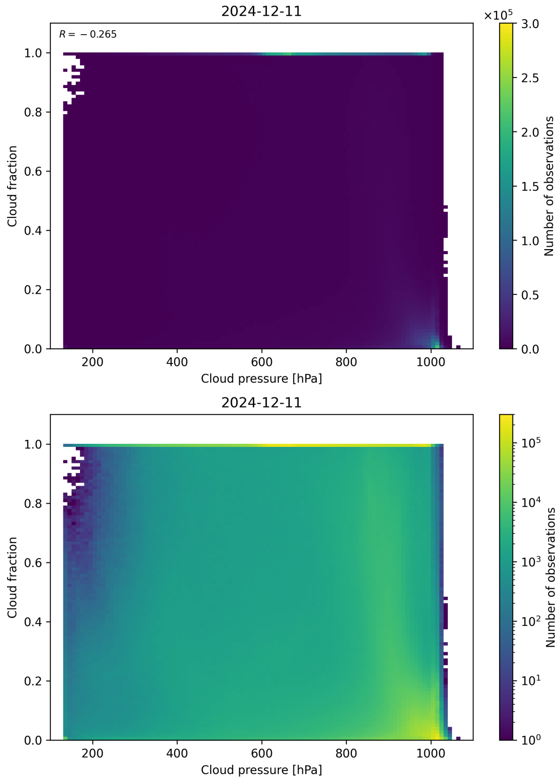
Figure 79: Scatter density plot of “Cloud pressure” against “Cloud fraction” for 2024-12-11 to 2024-12-12.
