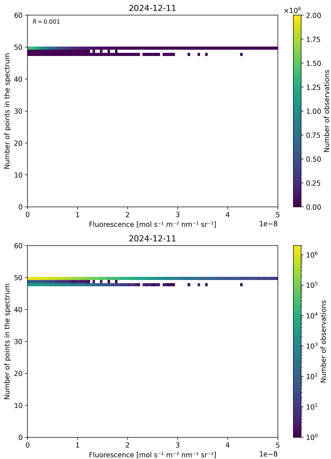
Figure 86: Scatter density plot of “Fluorescence” against “Number of points in the spectrum” for 2024-12-11 to 2024-12-12.
