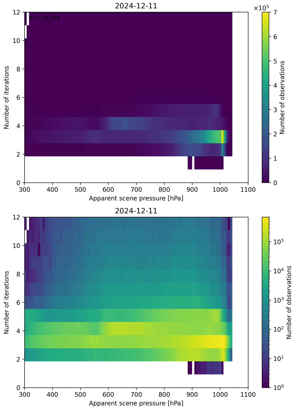
Figure 65: Scatter density plot of “Apparent scene pressure” against “Number of iterations” for 2024-12-11 to 2024-12-12.
