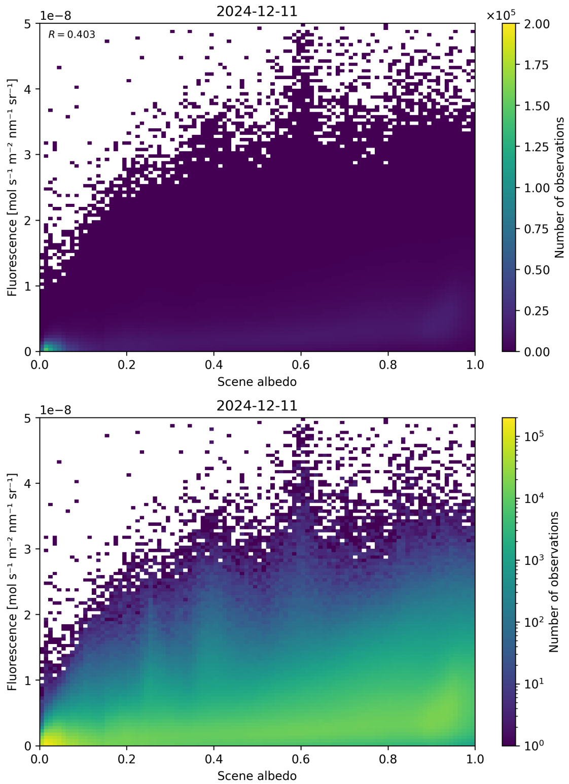
Figure 104: Scatter density plot of “Scene albedo” against “Fluorescence” for 2024-12-11 to 2024-12-12.
