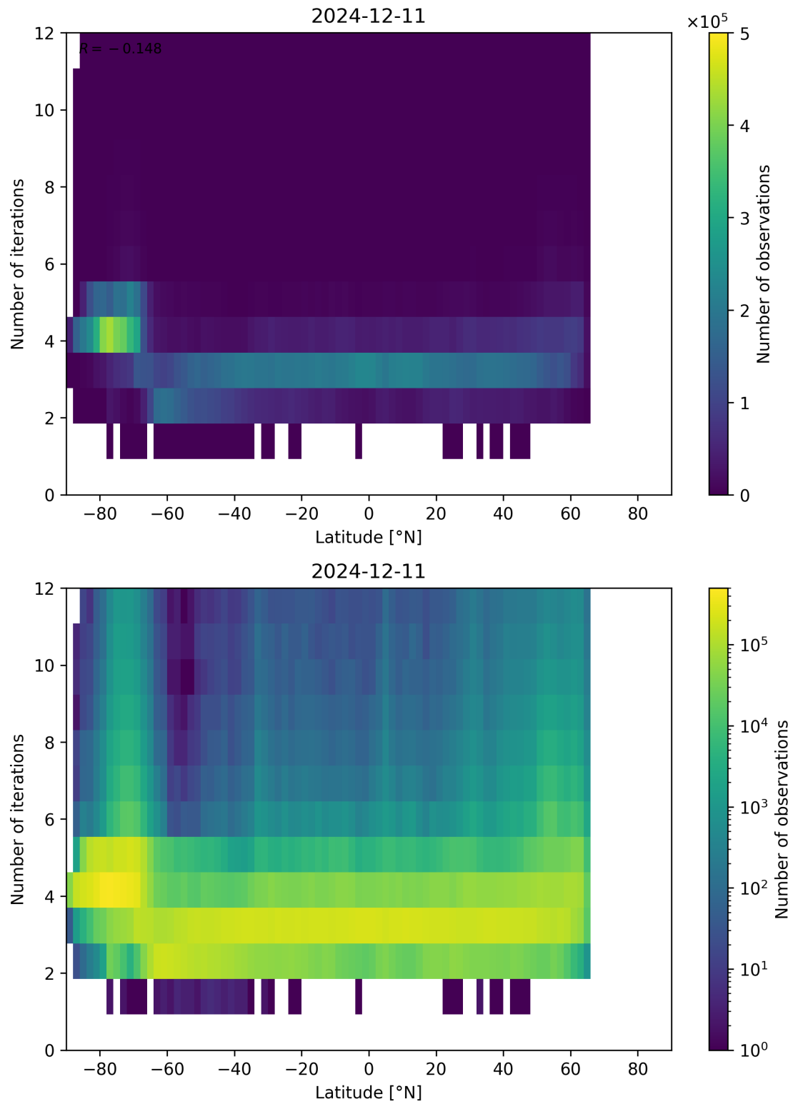
Figure 93: Scatter density plot of “Latitude” against “Number of iterations” for 2024-12-11 to 2024-12-12.
