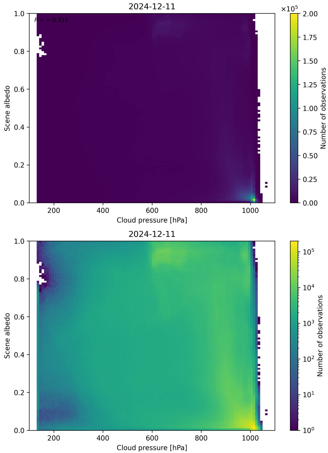
Figure 83: Scatter density plot of “Cloud pressure” against “Scene albedo” for 2024-12-11 to 2024-12-12.
