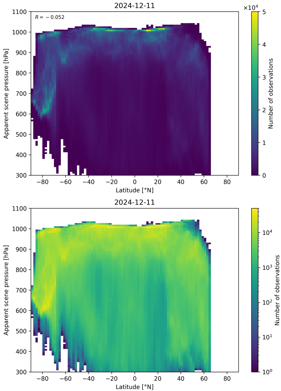
Figure 88: Scatter density plot of “Latitude” against “Apparent scene pressure” for 2024-12-11 to 2024-12-12.
