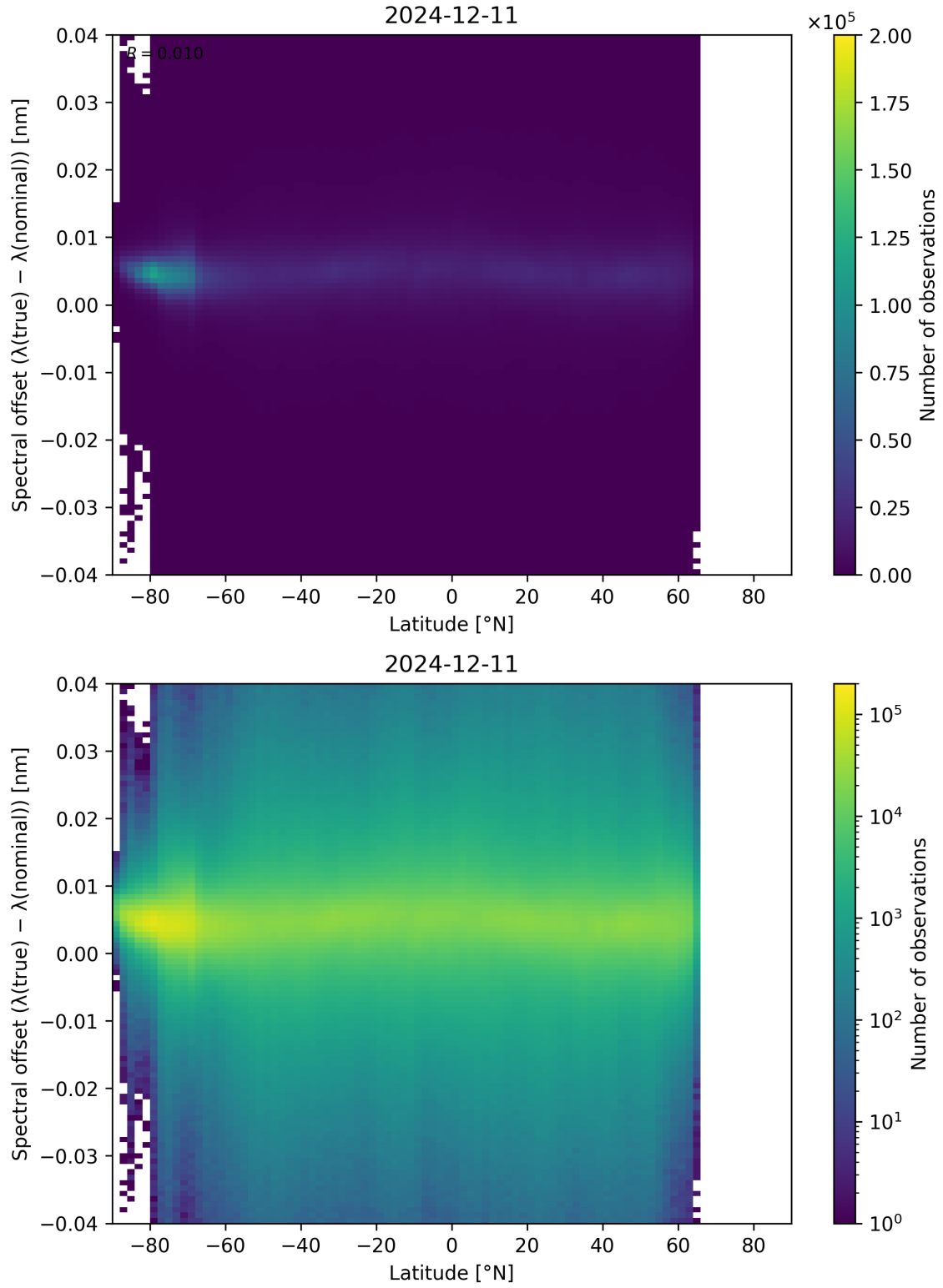
Figure 96: Scatter density plot of “Latitude” against “Spectral offset ( \lambda_{\text{true}} - \lambda_{\text{nominal}} )” for 2024-12-11 to 2024-12-12.
