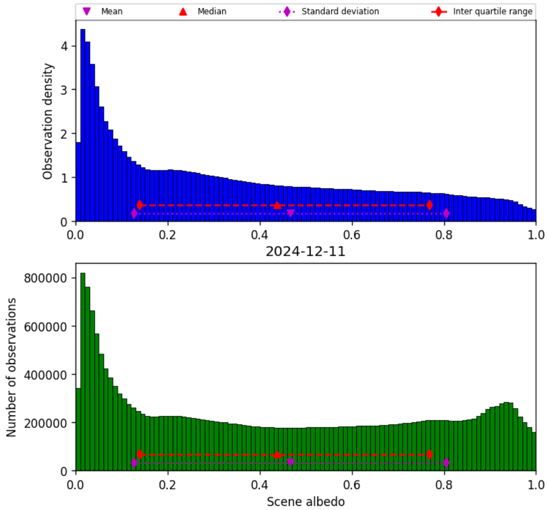
Figure 34: Histogram of “Scene albedo” for 2024-12-11 to 2024-12-12
