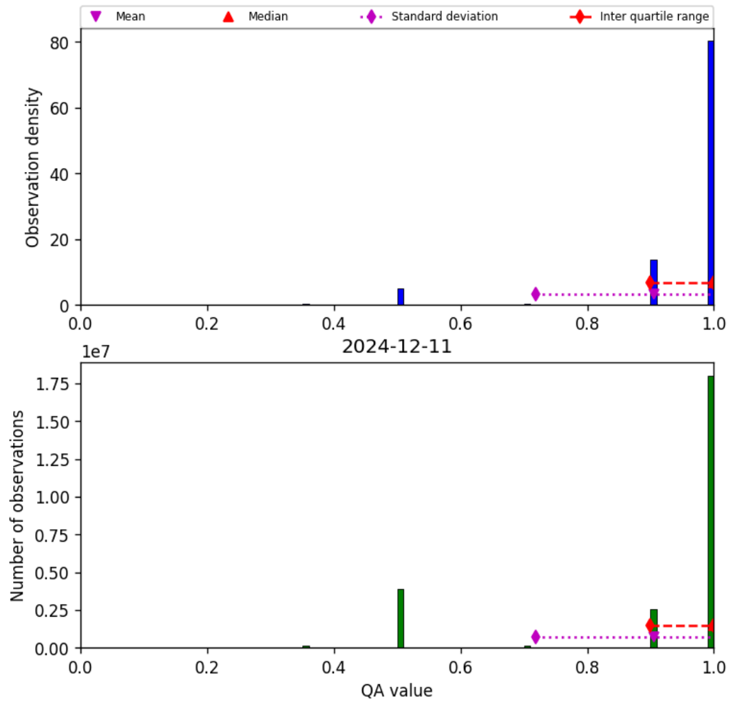
Figure 29: Histogram of “QA value” for 2024-12-11 to 2024-12-12
