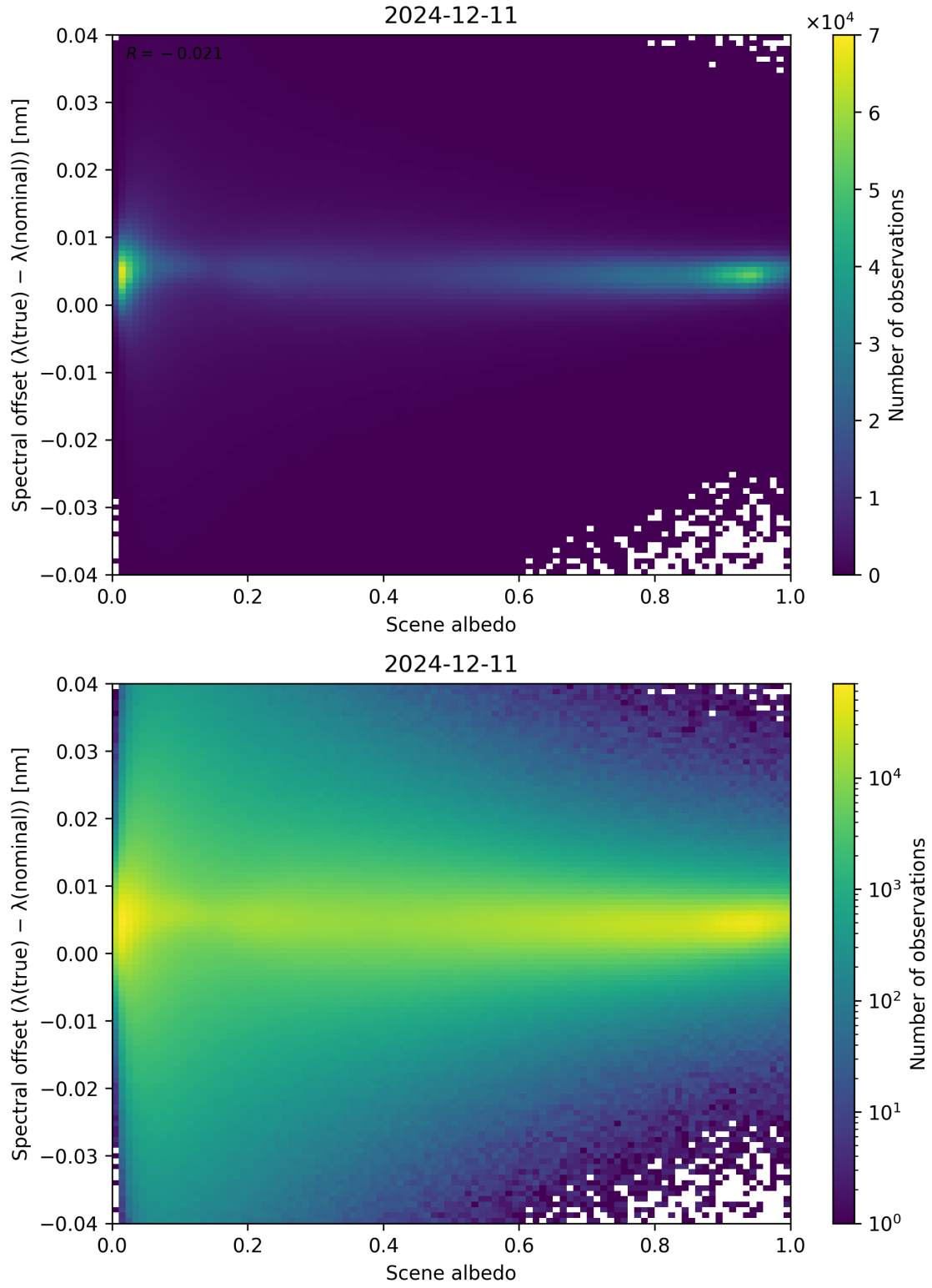
Figure 107: Scatter density plot of “Scene albedo” against “Spectral offset ( \lambda_{\text{true}} - \lambda_{\text{nominal}} )” for 2024-12-11 to 2024-12-12.
