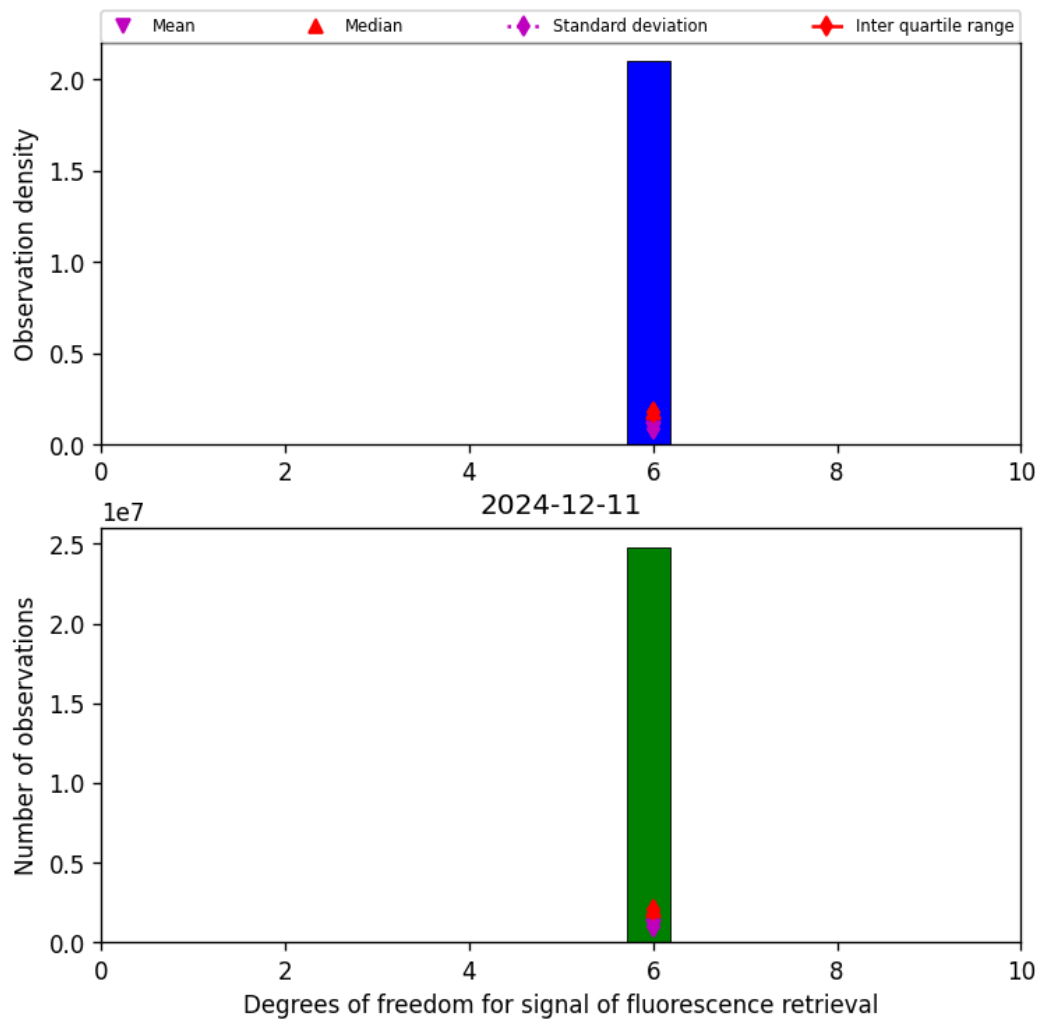
Figure 43: Histogram of “Degrees of freedom for signal of fluorescence retrieval” for 2024-12-11 to 2024-12-12
