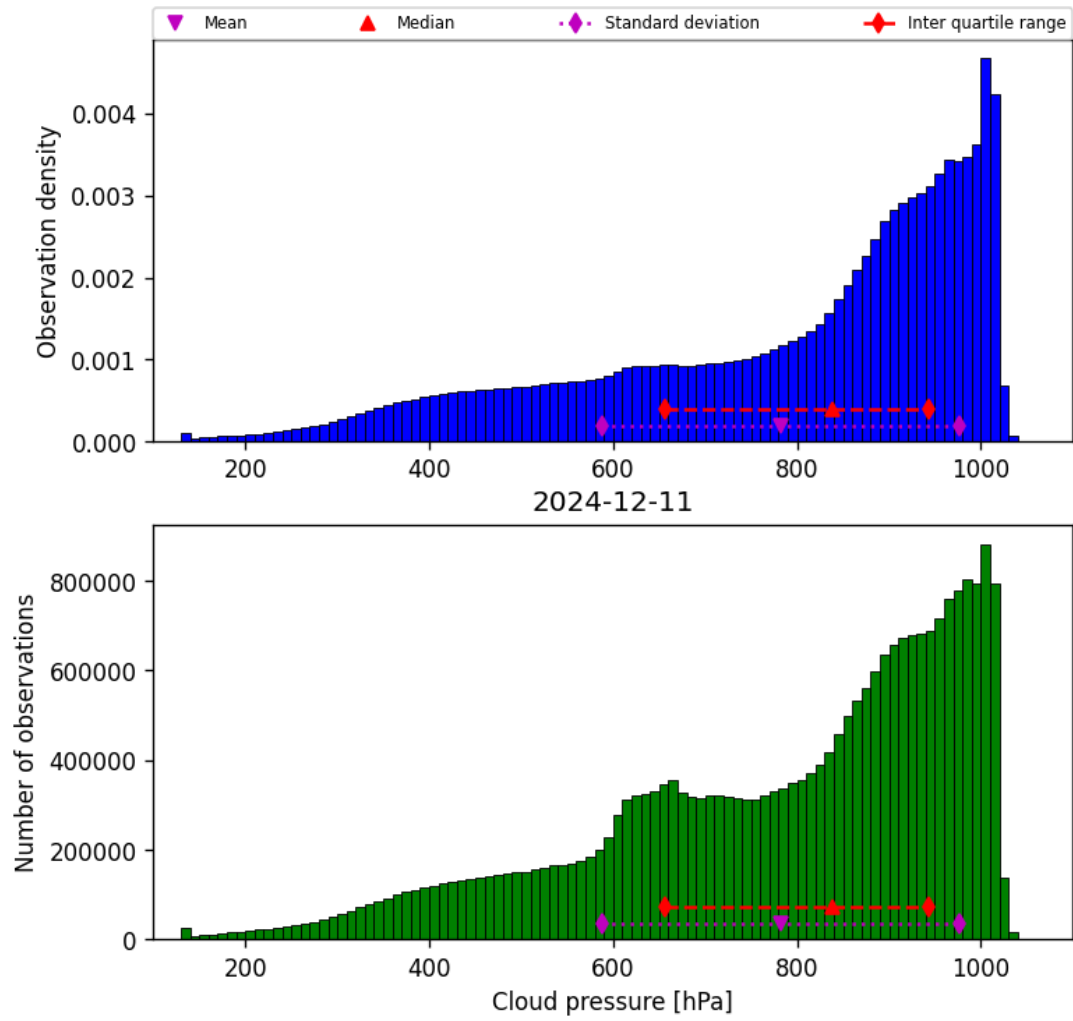
Figure 30: Histogram of “Cloud pressure” for 2024-12-11 to 2024-12-12
