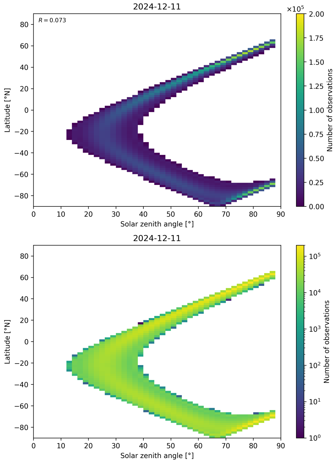
Figure 113: Scatter density plot of “Solar zenith angle” against “Latitude” for 2024-12-11 to 2024-12-12.
