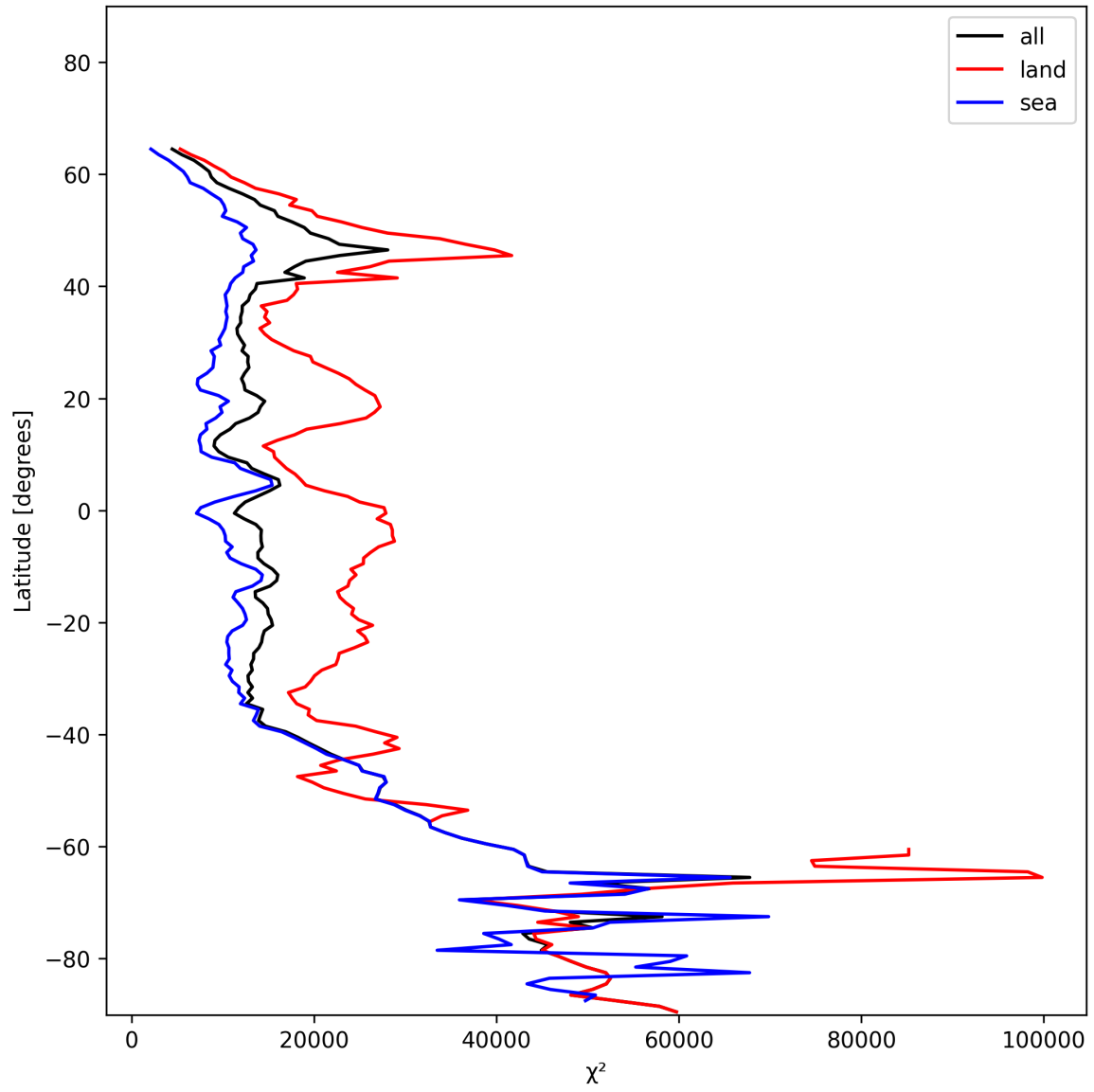
Figure 21: Zonal average of “ \chi^2 ” for 2024-12-11 to 2024-12-12.
