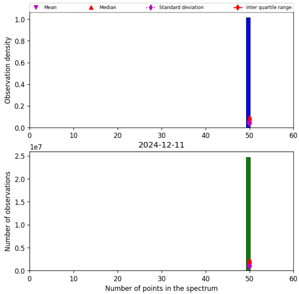
Figure 44: Histogram of “Number of points in the spectrum” for 2024-12-11 to 2024-12-12
