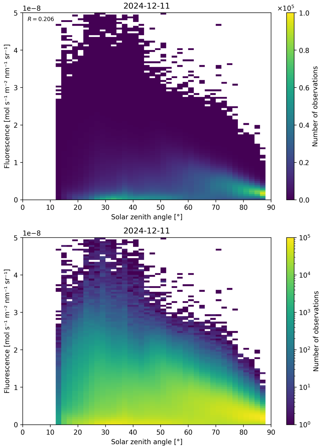
Figure 112: Scatter density plot of “Solar zenith angle” against “Fluorescence” for 2024-12-11 to 2024-12-12.
