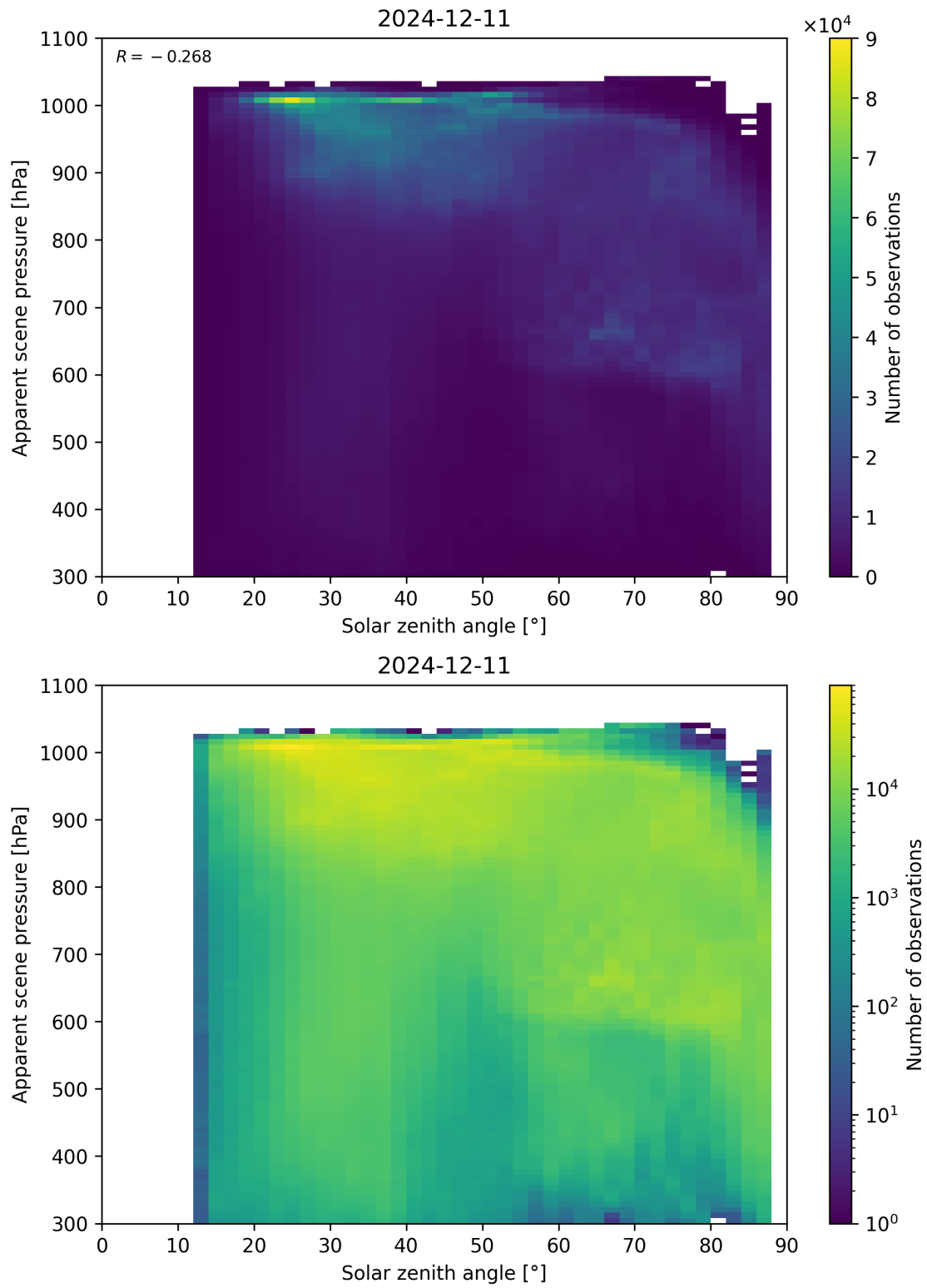
Figure 108: Scatter density plot of “Solar zenith angle” against “Apparent scene pressure” for 2024-12-11 to 2024-12-12.
