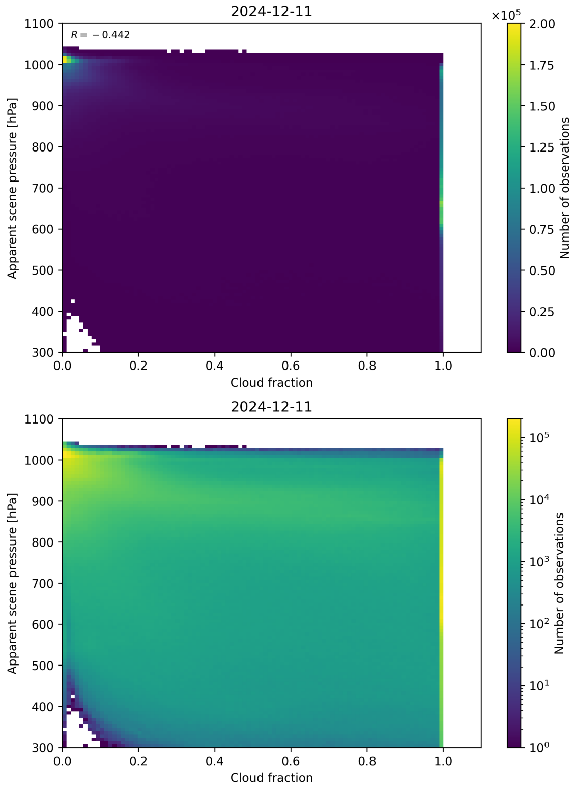
Figure 70: Scatter density plot of “Cloud fraction” against “Apparent scene pressure” for 2024-12-11 to 2024-12-12.
