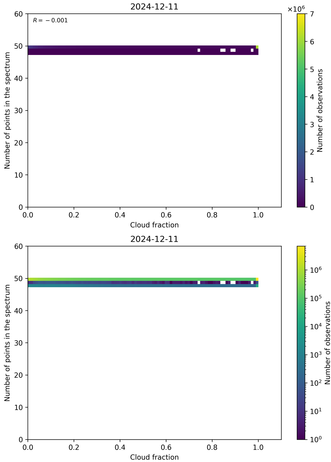
Figure 74: Scatter density plot of “Cloud fraction” against “Number of points in the spectrum” for 2024-12-11 to 2024-12-12.
