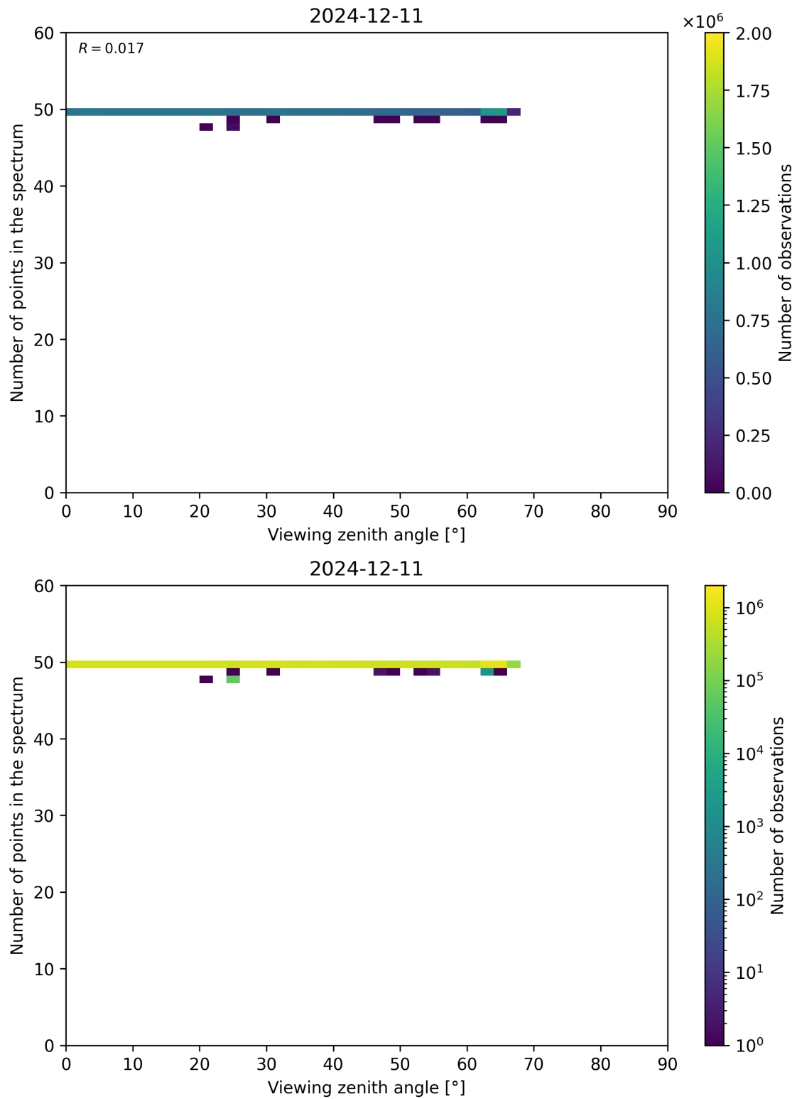
Figure 125: Scatter density plot of “Viewing zenith angle” against “Number of points in the spectrum” for 2024-12-11 to 2024-12-12.
