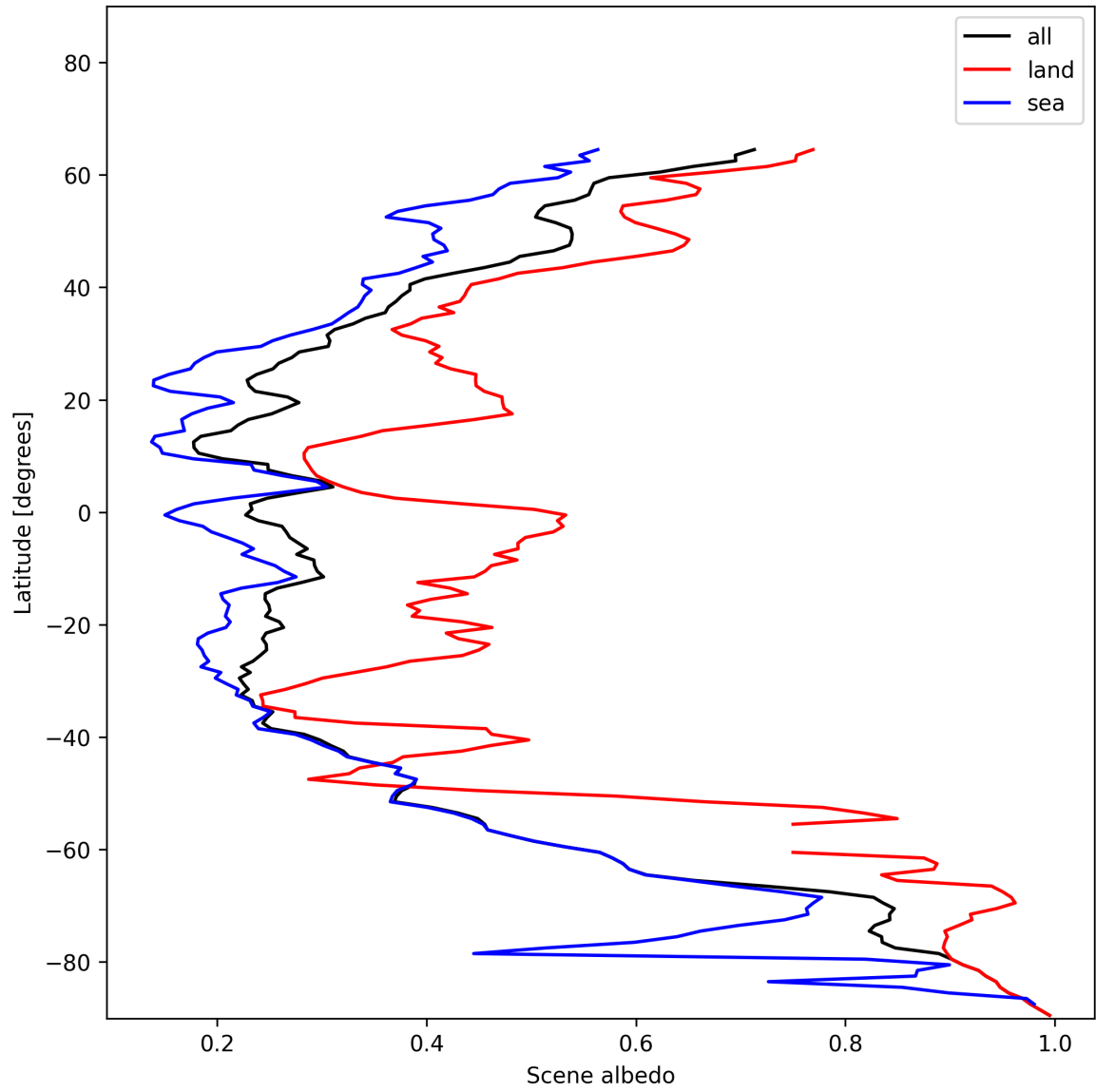
Figure 17: Zonal average of “Scene albedo” for 2024-12-11 to 2024-12-12.
