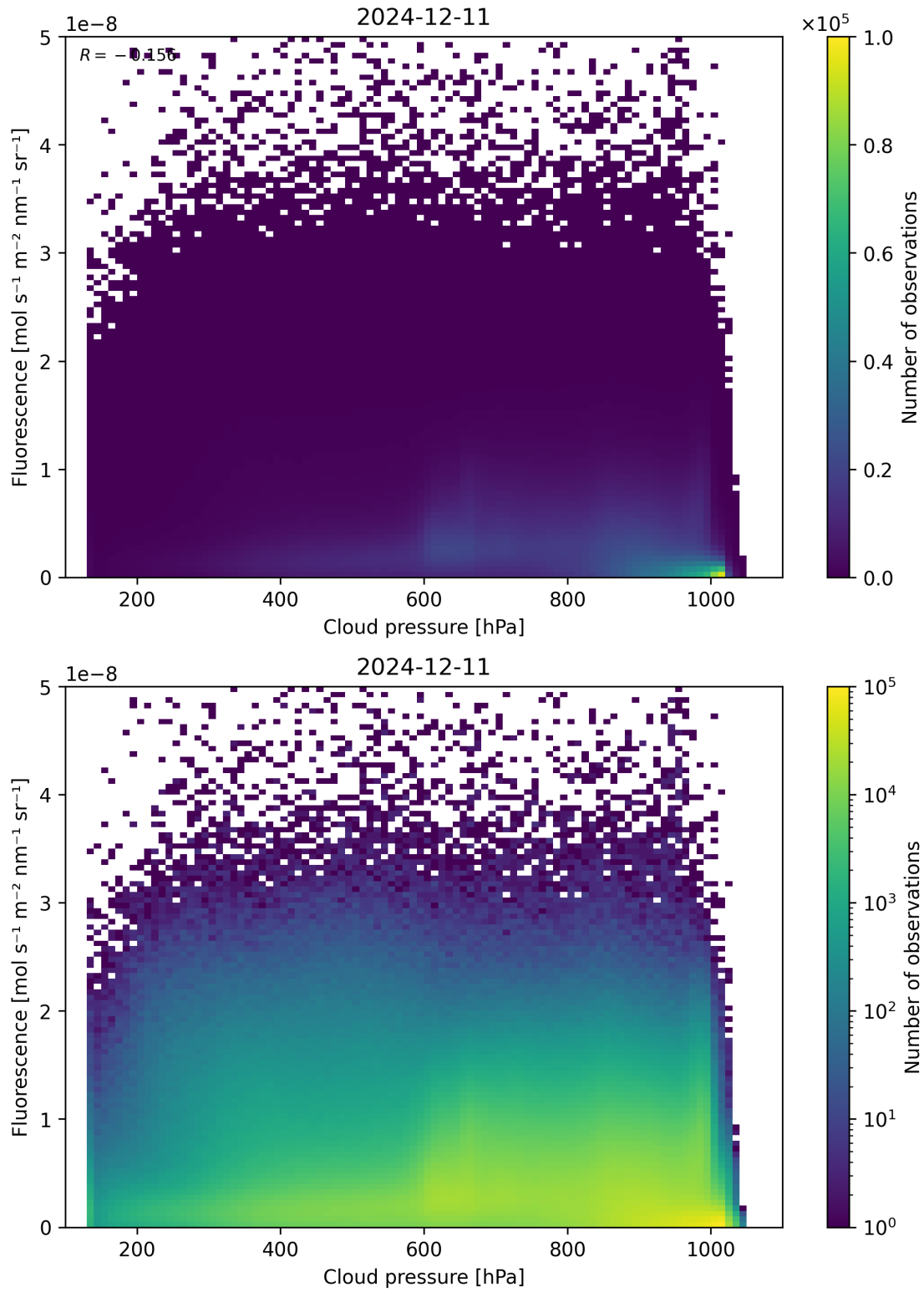
Figure 80: Scatter density plot of “Cloud pressure” against “Fluorescence” for 2024-12-11 to 2024-12-12.
