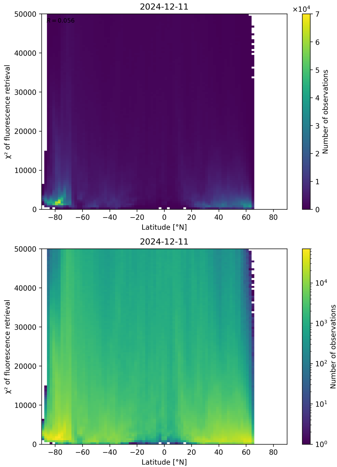
Figure 89: Scatter density plot of “Latitude” against “ \chi^2 of fluorescence retrieval” for 2024-12-11 to 2024-12-12.
