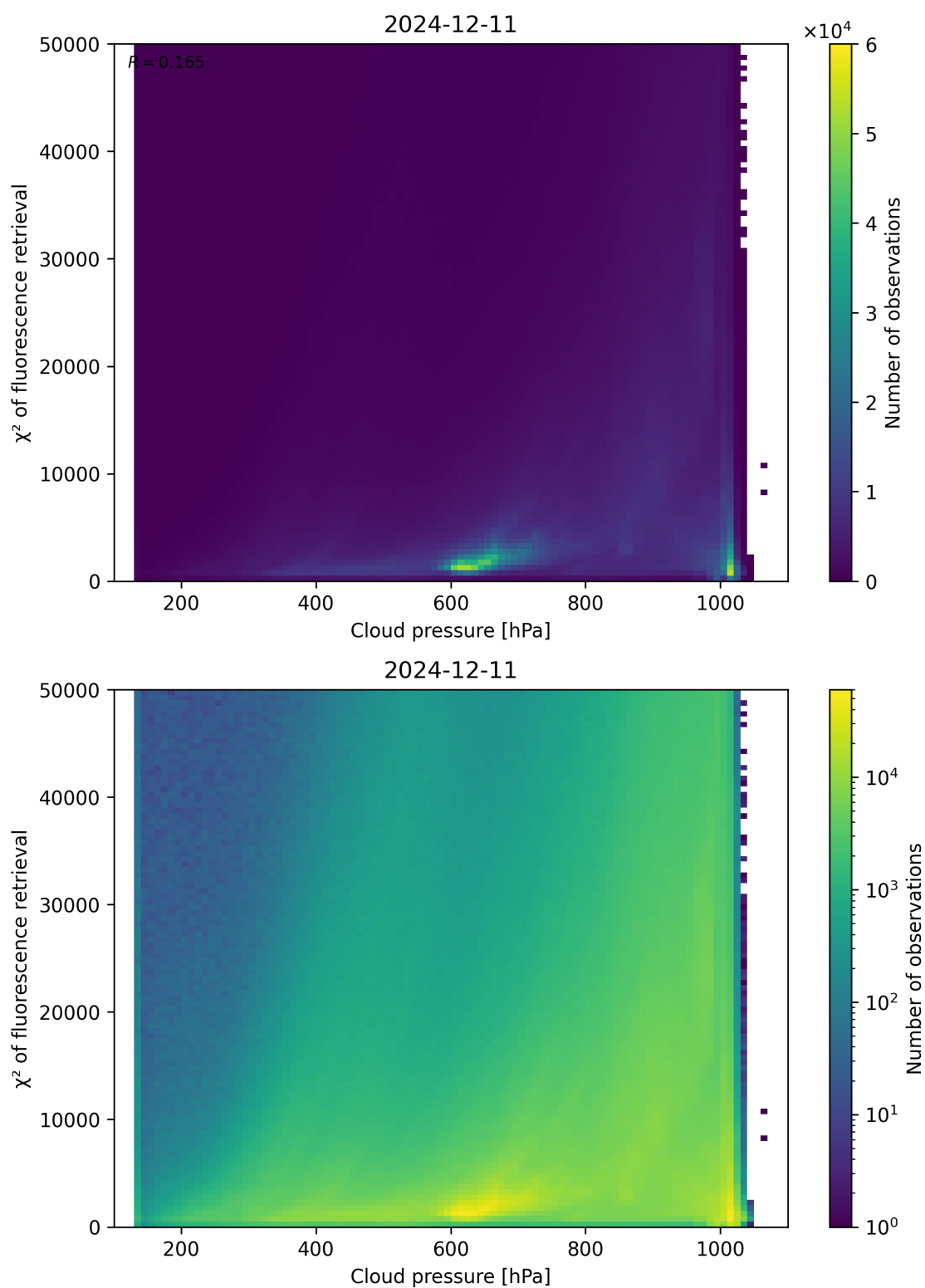
Figure 78: Scatter density plot of “Cloud pressure” against “ \chi^2 of fluorescence retrieval” for 2024-12-11 to 2024-12-12.
