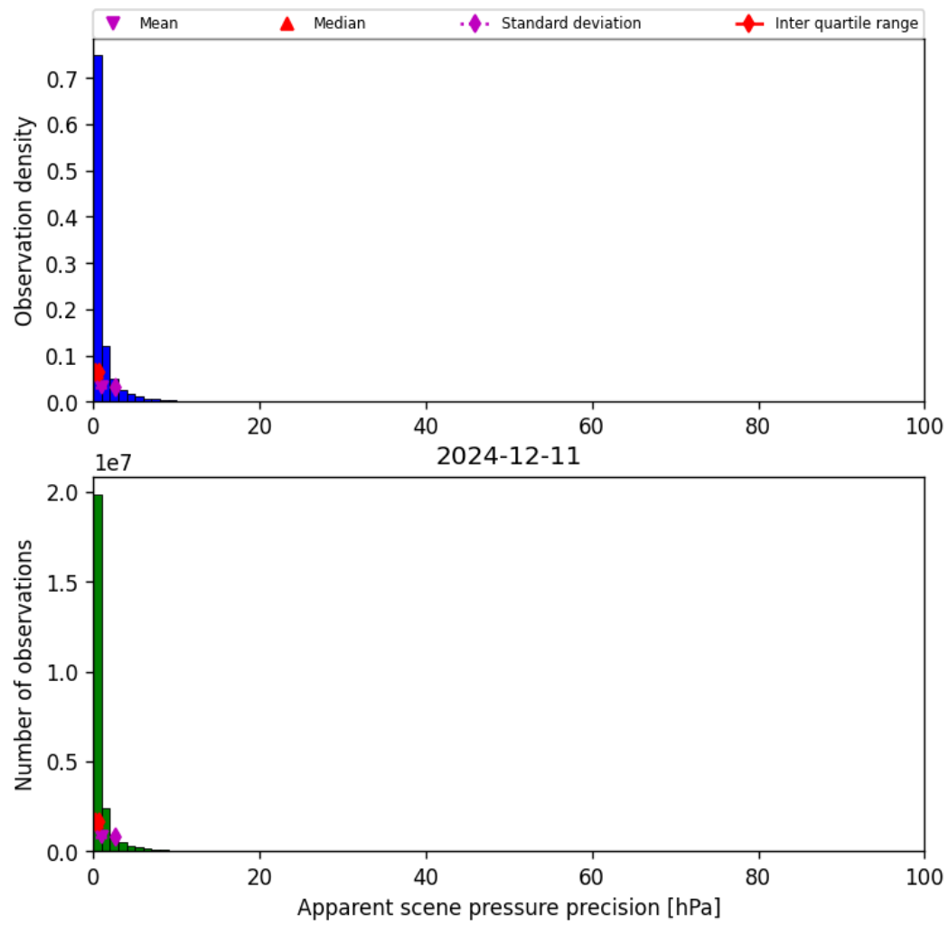
Figure 37: Histogram of “Apparent scene pressure precision” for 2024-12-11 to 2024-12-12
