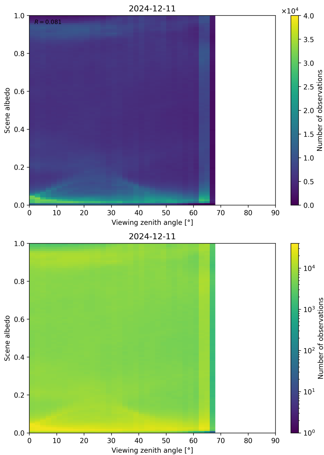
Figure 126: Scatter density plot of “Viewing zenith angle” against “Scene albedo” for 2024-12-11 to 2024-12-12.
