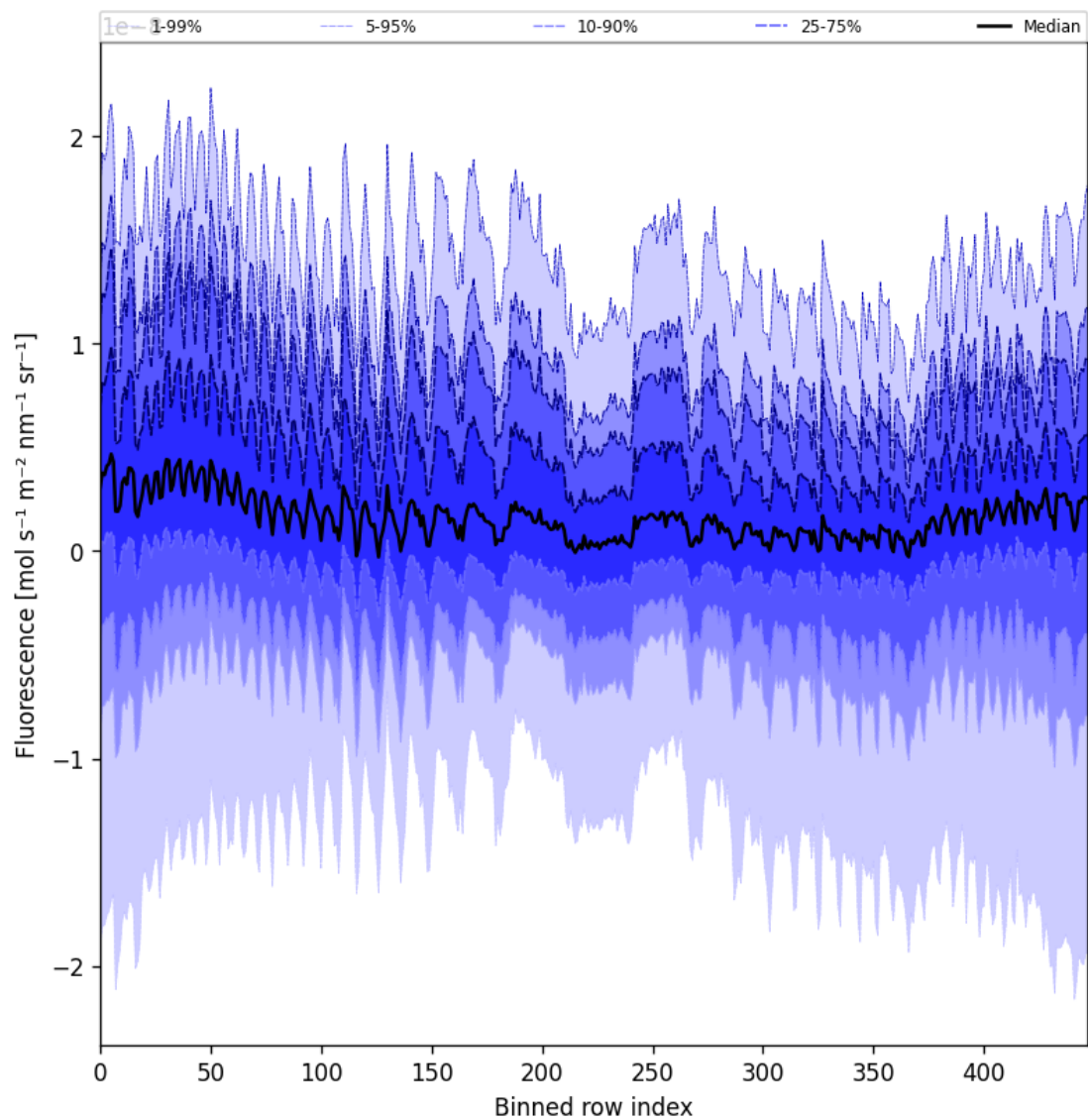
Figure 57: Along track statistics of “Fluorescence” for 2024-12-11 to 2024-12-12
