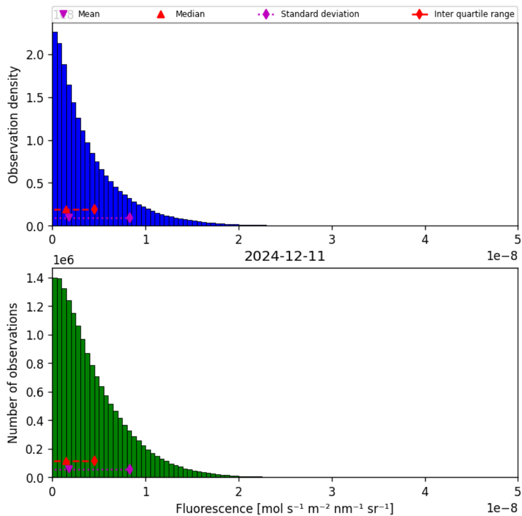
Figure 40: Histogram of “Fluorescence” for 2024-12-11 to 2024-12-12
