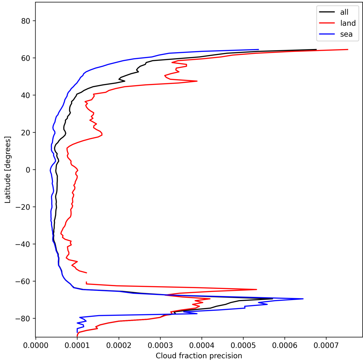
Figure 16: Zonal average of “Cloud fraction precision” for 2024-12-11 to 2024-12-12.
