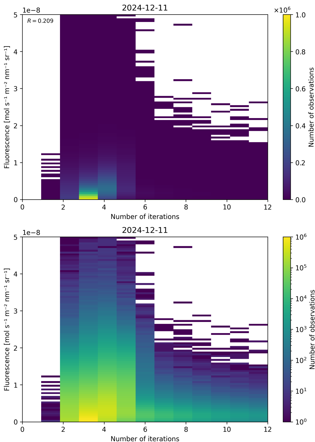
Figure 98: Scatter density plot of “Number of iterations” against “Fluorescence” for 2024-12-11 to 2024-12-12.
