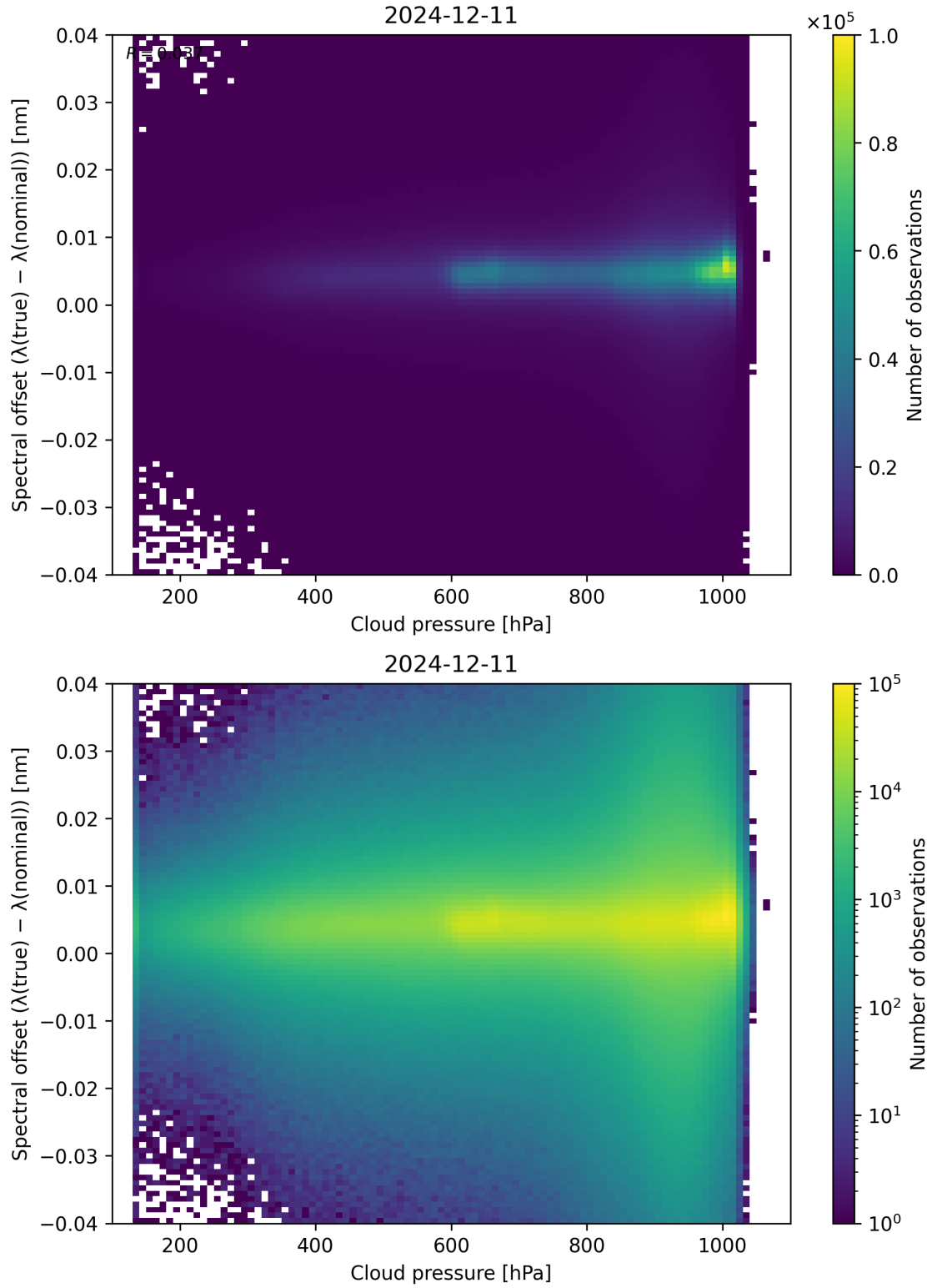
Figure 84: Scatter density plot of “Cloud pressure” against “Spectral offset ( \lambda_{\text{true}} - \lambda_{\text{nominal}} )” for 2024-12-11 to 2024-12-12.
