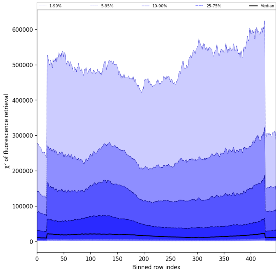
Figure 59: Along track statistics of “ \chi^2 of fluorescence retrieval” for 2024-12-11 to 2024-12-12
