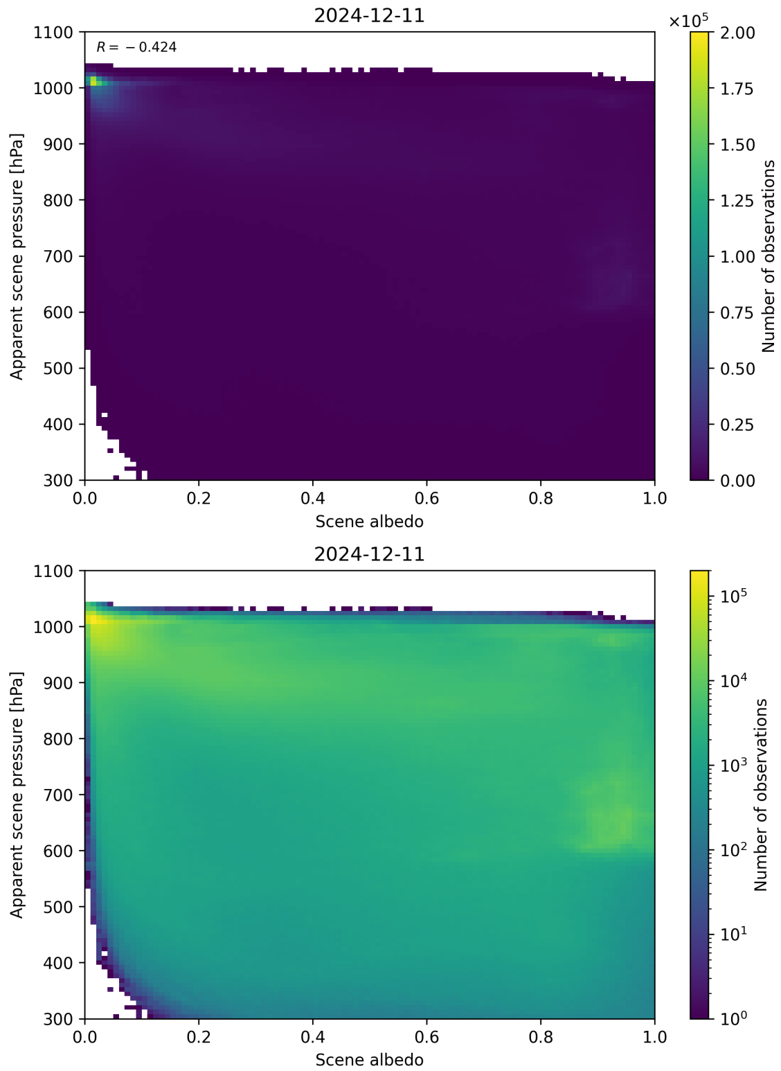
Figure 102: Scatter density plot of “Scene albedo” against “Apparent scene pressure” for 2024-12-11 to 2024-12-12.
