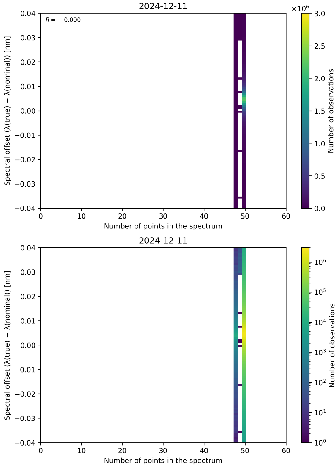
Figure 101: Scatter density plot of “Number of points in the spectrum” against “Spectral offset ( \lambda_{\text{true}} - \lambda_{\text{nominal}} )” for 2024-12-11 to 2024-12-12.
