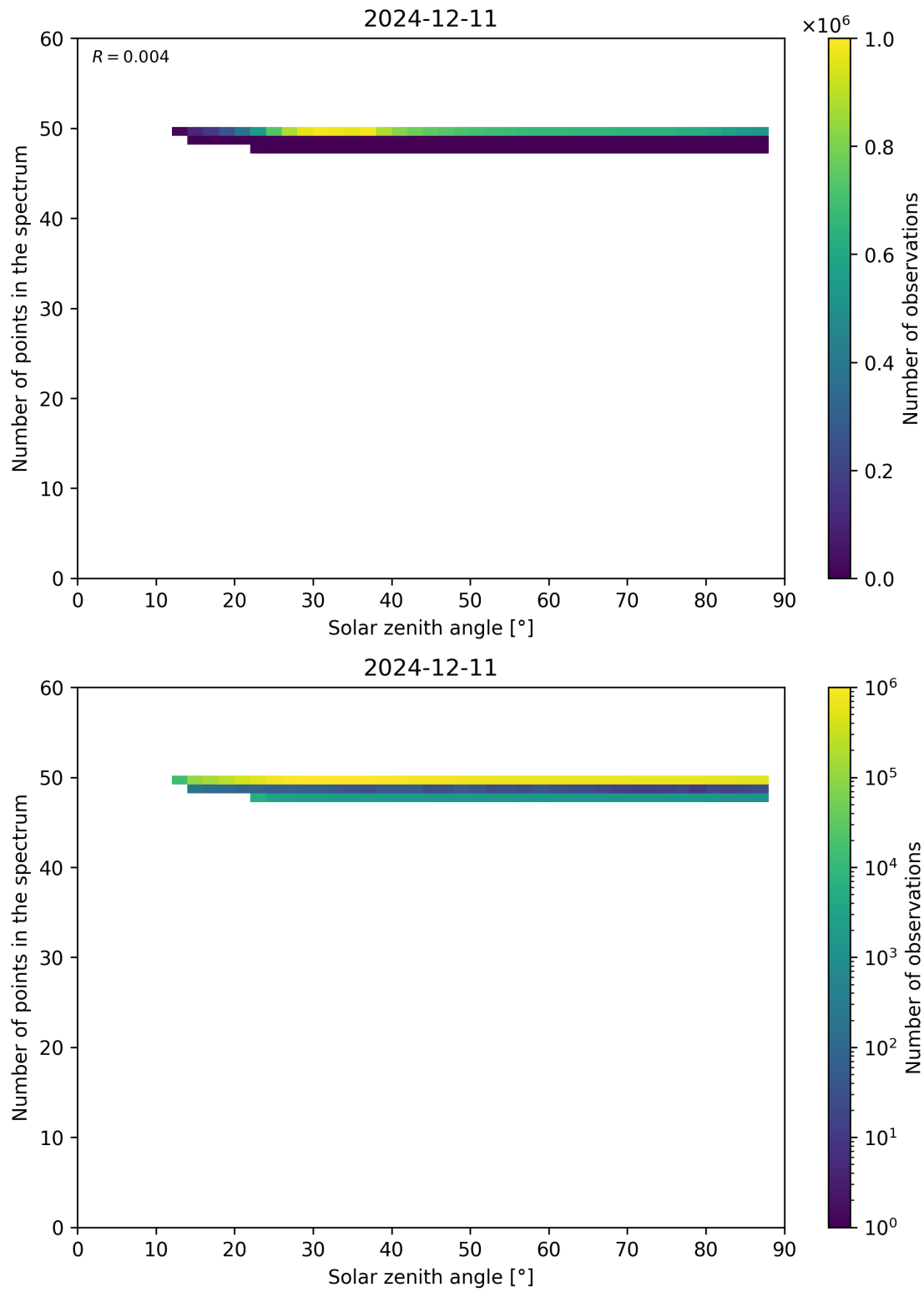
Figure 115: Scatter density plot of “Solar zenith angle” against “Number of points in the spectrum” for 2024-12-11 to 2024-12-12.
