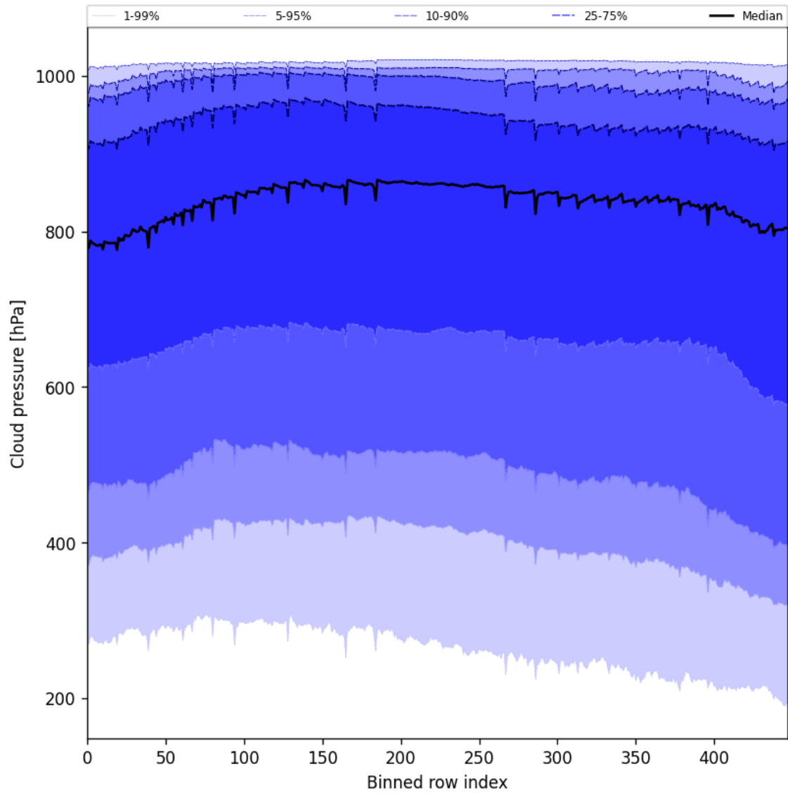
Figure 47: Along track statistics of “Cloud pressure” for 2024-12-11 to 2024-12-12
