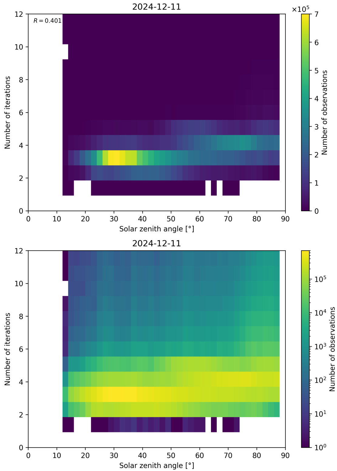
Figure 114: Scatter density plot of “Solar zenith angle” against “Number of iterations” for 2024-12-11 to 2024-12-12.
