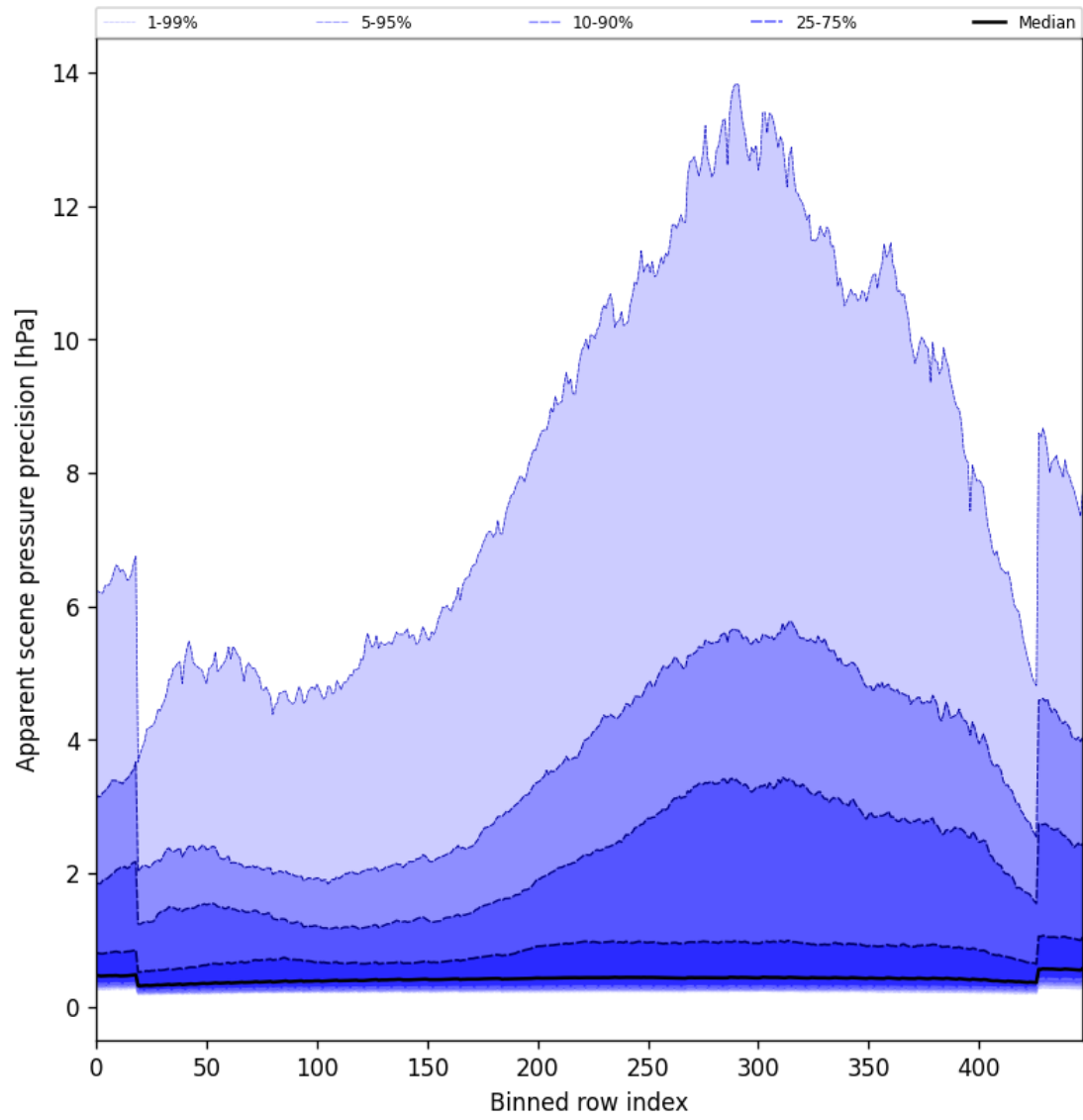
Figure 54: Along track statistics of “Apparent scene pressure precision” for 2024-12-11 to 2024-12-12
