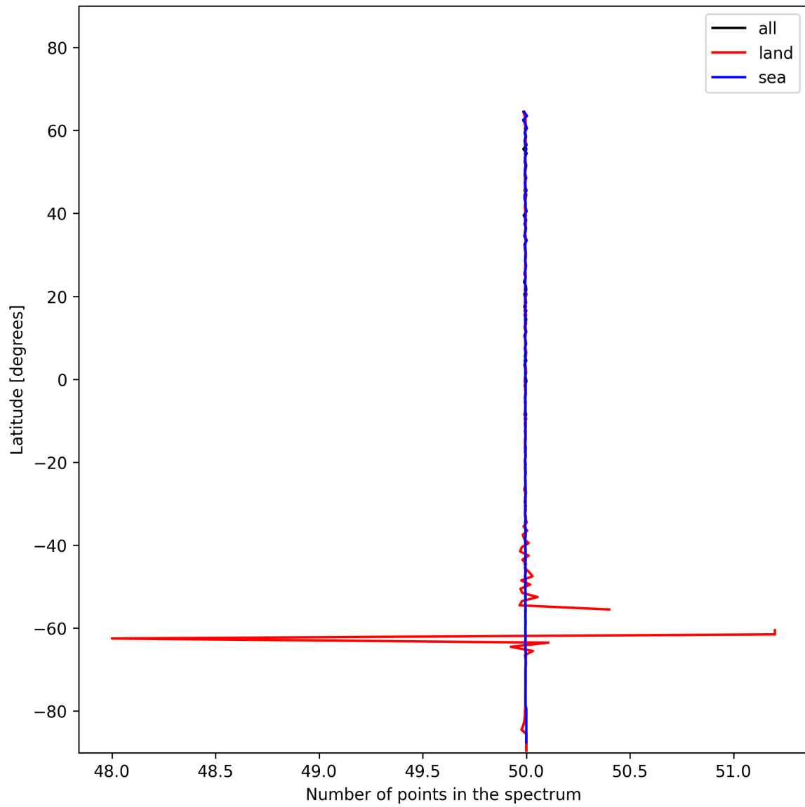
Figure 27: Zonal average of “Number of points in the spectrum” for 2024-12-11 to 2024-12-12.
