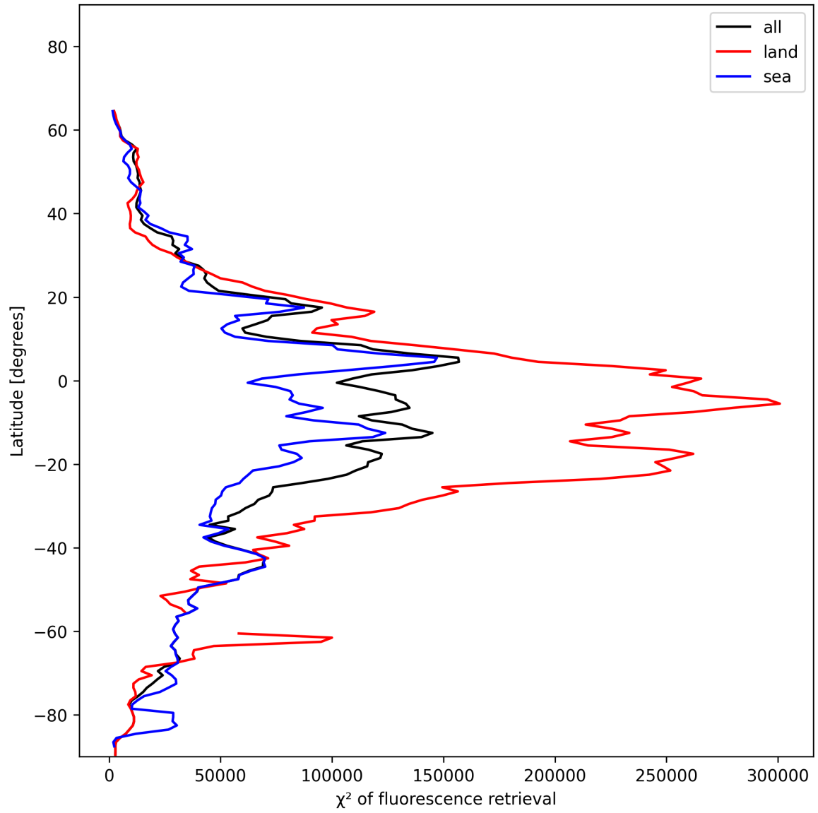
Figure 25: Zonal average of “ \chi^2 of fluorescence retrieval” for 2024-12-11 to 2024-12-12.
