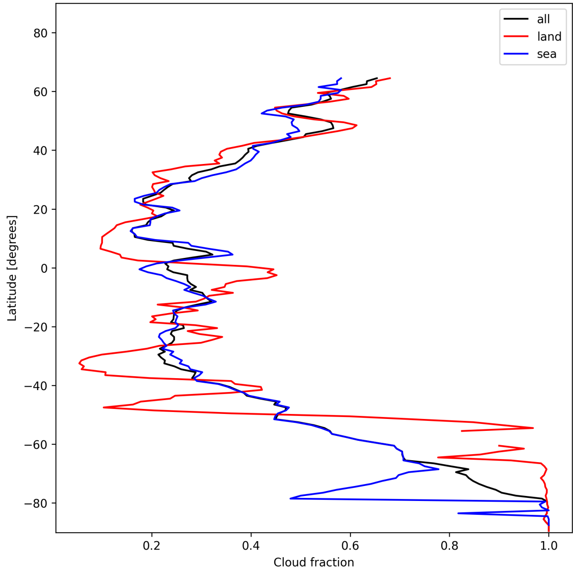
Figure 15: Zonal average of “Cloud fraction” for 2024-12-11 to 2024-12-12.
