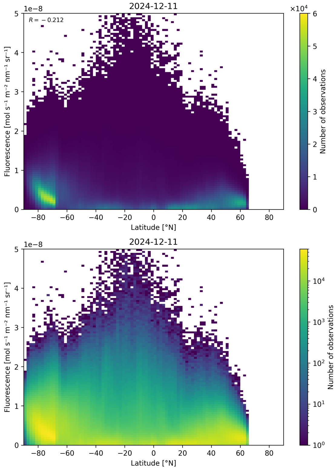
Figure 92: Scatter density plot of “Latitude” against “Fluorescence” for 2024-12-11 to 2024-12-12.
