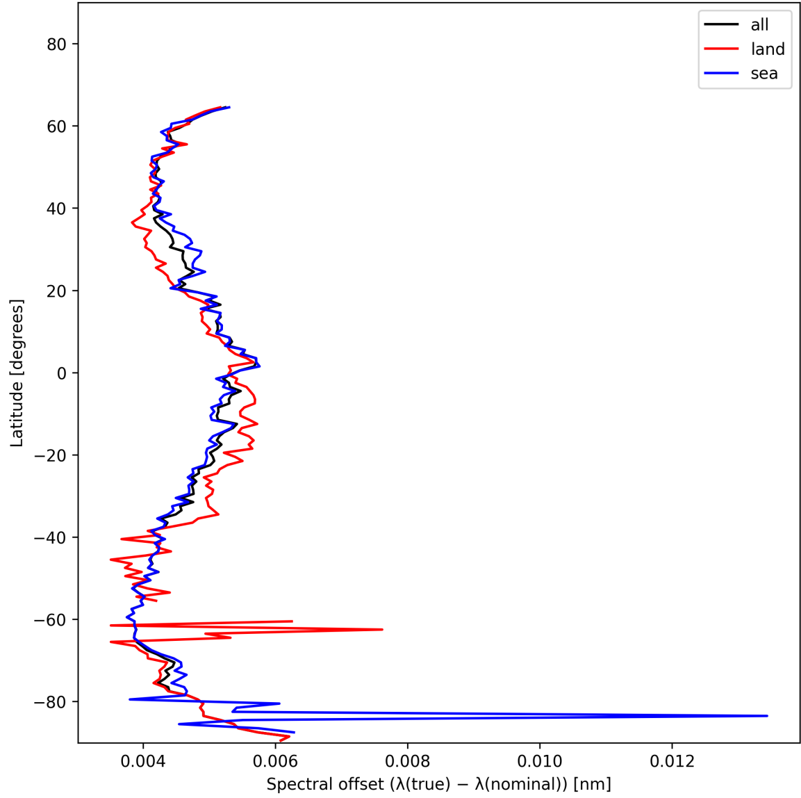
Figure 28: Zonal average of “Spectral offset ( \lambda_{\text{true}} - \lambda_{\text{nominal}} )” for 2024-12-11 to 2024-12-12.
