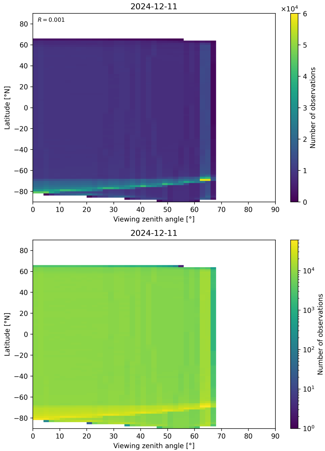
Figure 123: Scatter density plot of “Viewing zenith angle” against “Latitude” for 2024-12-11 to 2024-12-12.
