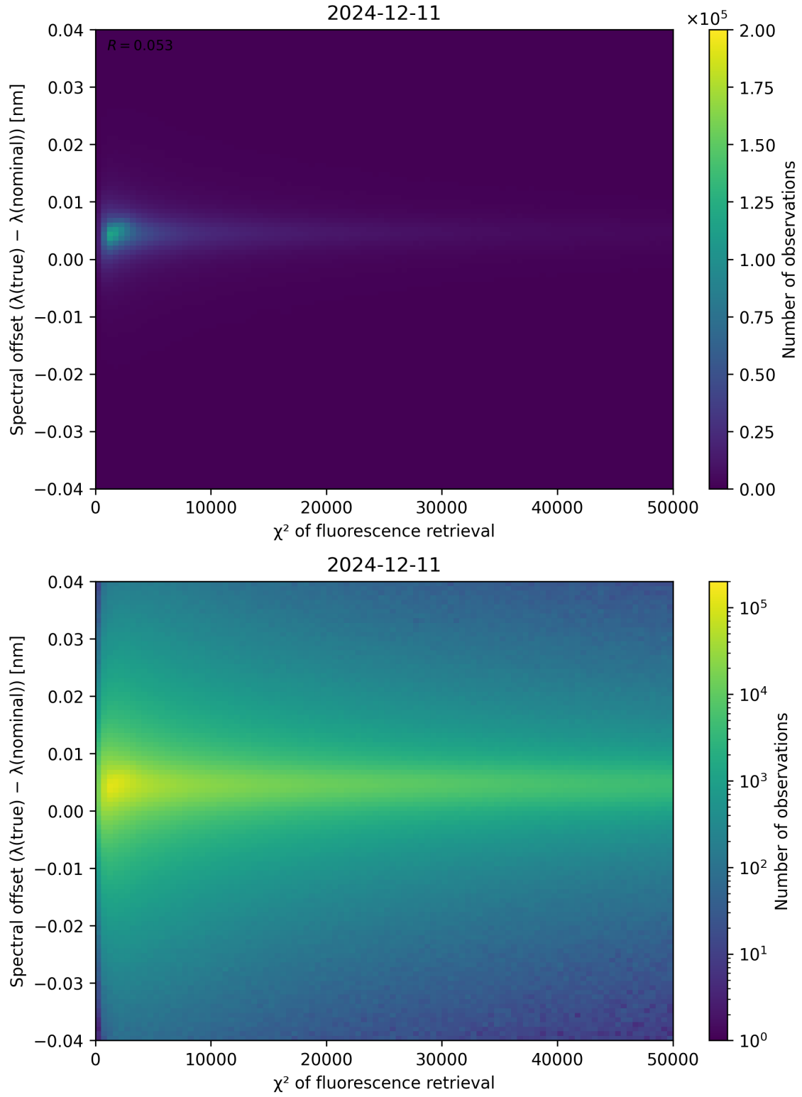
Figure 69: Scatter density plot of “ \chi^2 of fluorescence retrieval” against “Spectral offset ( \lambda_{\text{true}} - \lambda_{\text{nominal}} )” for 2024-12-11 to 2024-12-12.
