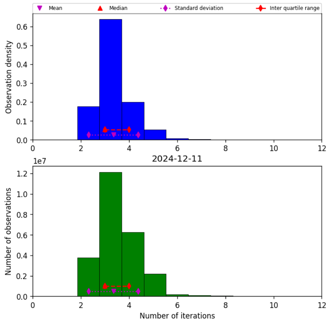
Figure 39: Histogram of “Number of iterations” for 2024-12-11 to 2024-12-12
