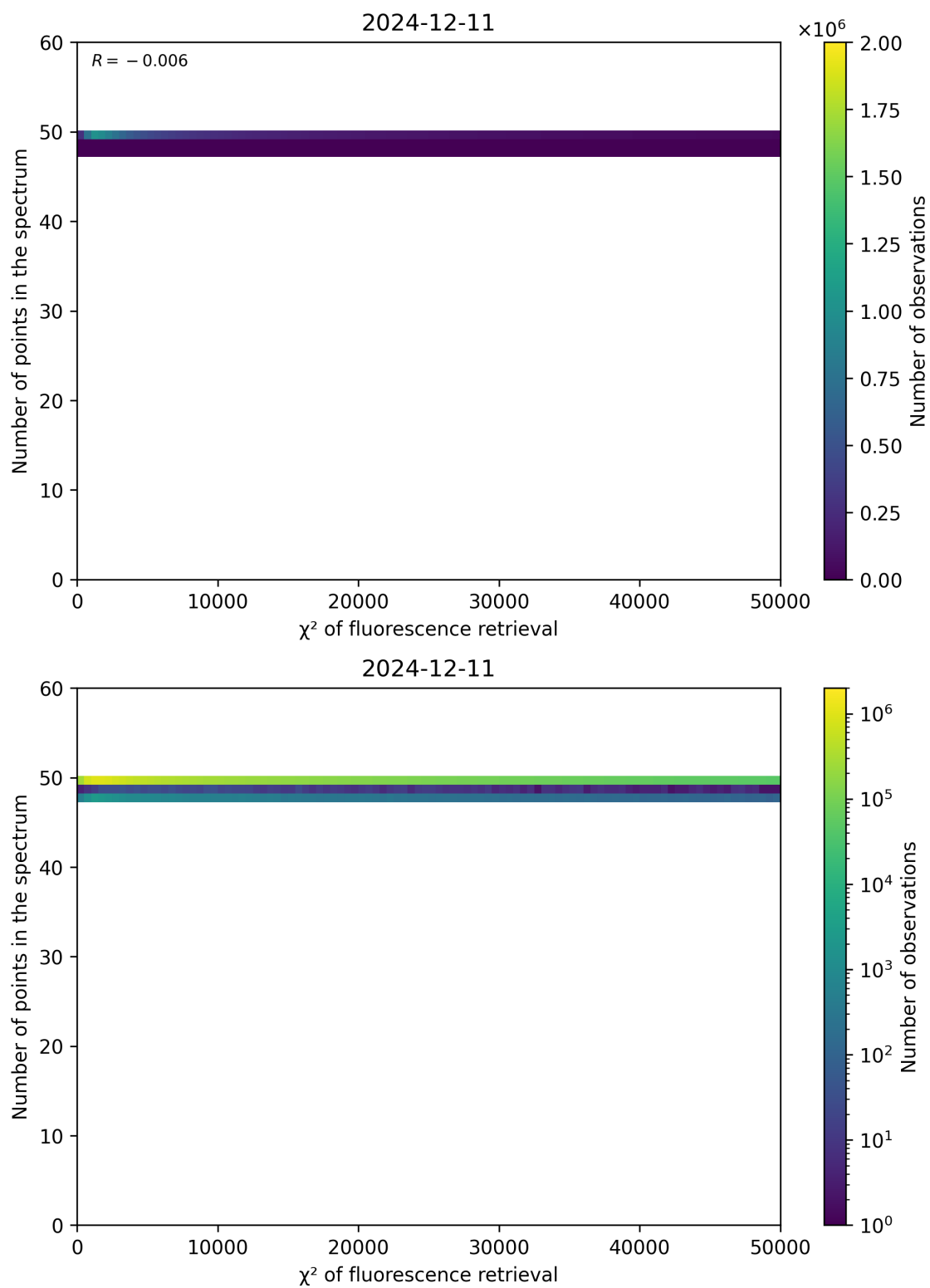
Figure 68: Scatter density plot of “ \chi^2 of fluorescence retrieval” against “Number of points in the spectrum” for 2024-12-11 to 2024-12-12.
