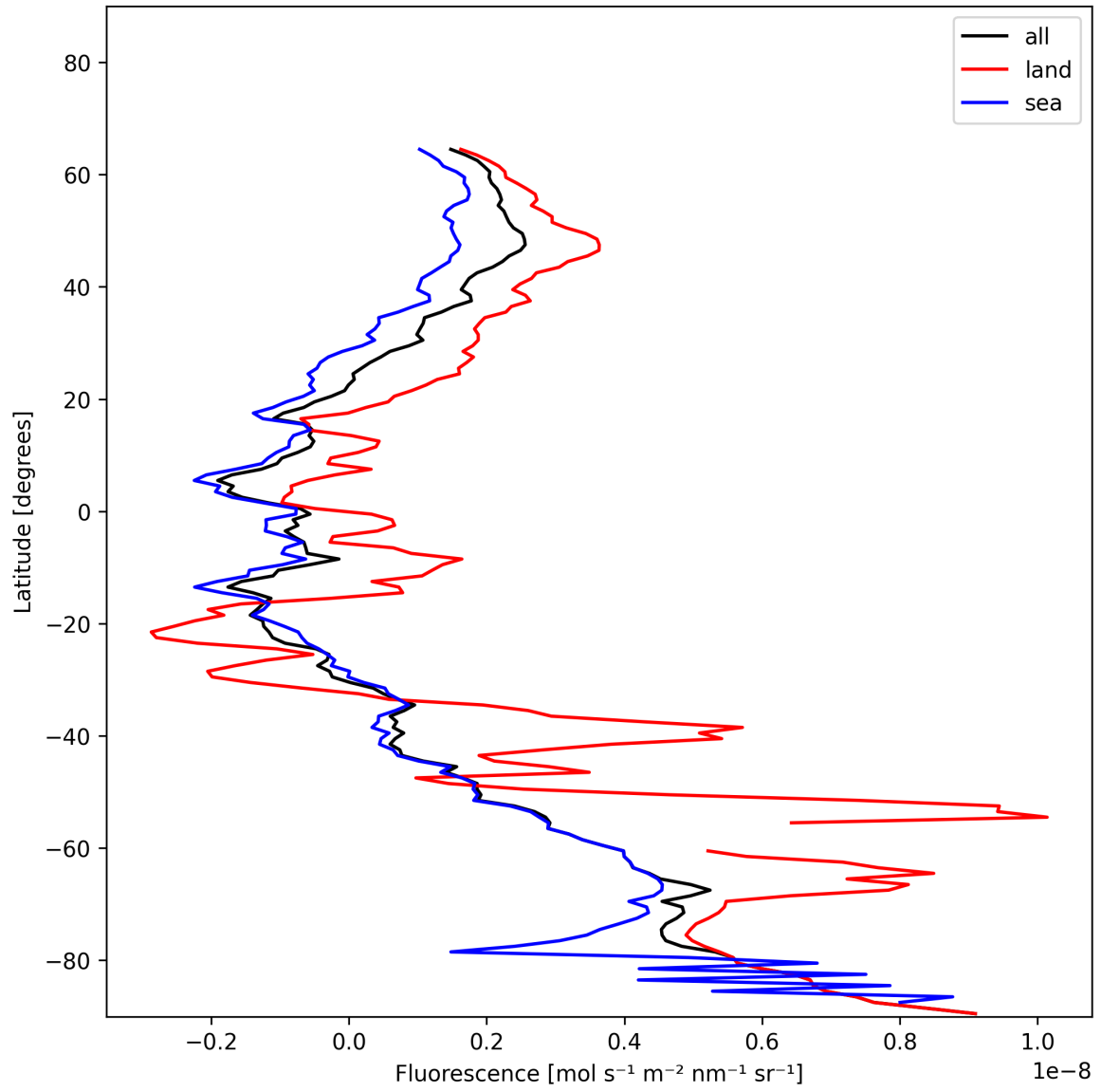
Figure 23: Zonal average of “Fluorescence” for 2024-12-11 to 2024-12-12.
