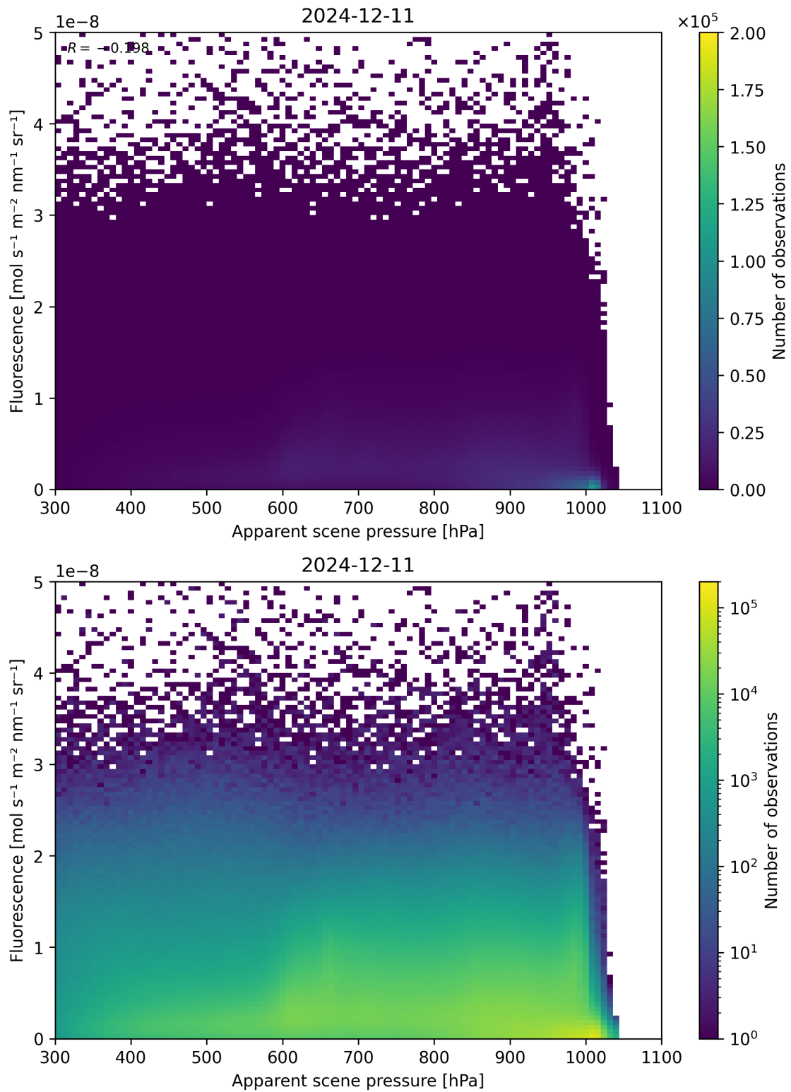
Figure 64: Scatter density plot of “Apparent scene pressure” against “Fluorescence” for 2024-12-11 to 2024-12-12.
