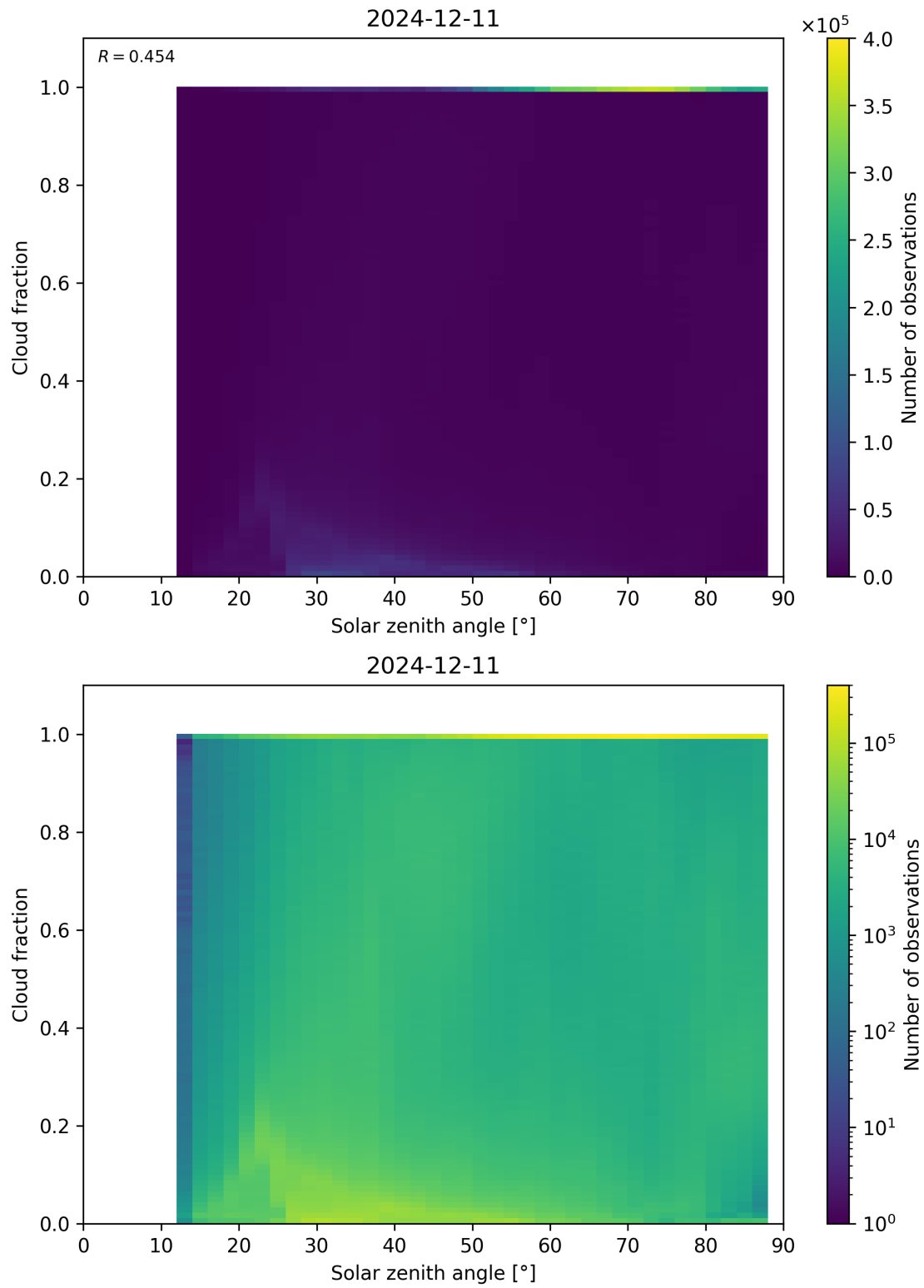
Figure 110: Scatter density plot of “Solar zenith angle” against “Cloud fraction” for 2024-12-11 to 2024-12-12.
