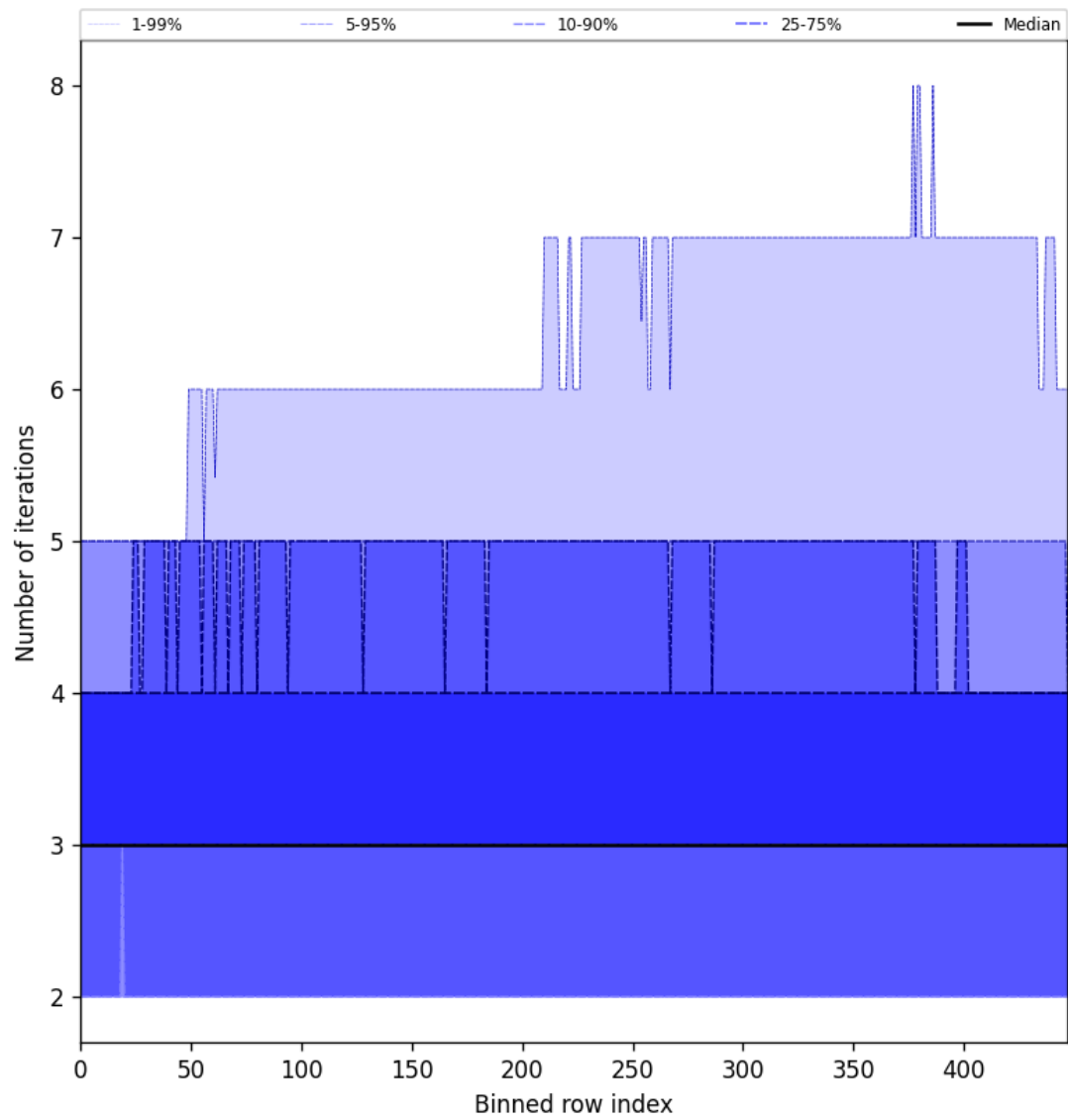
Figure 56: Along track statistics of “Number of iterations” for 2024-12-11 to 2024-12-12
