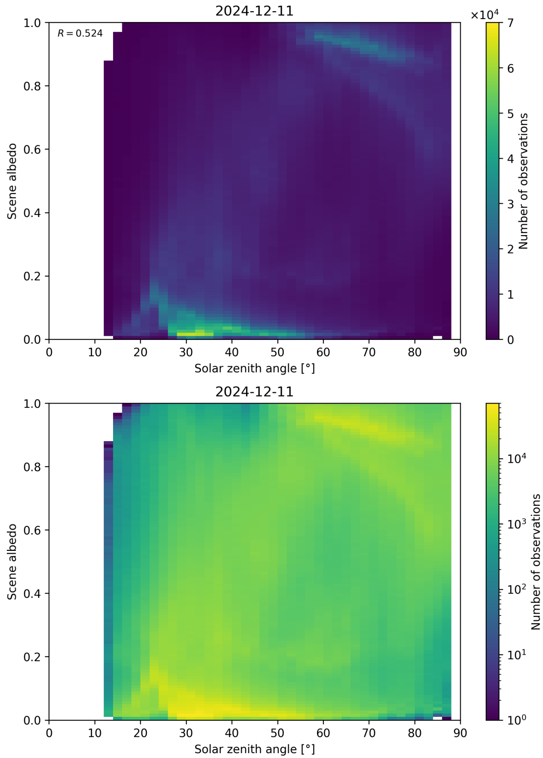
Figure 116: Scatter density plot of “Solar zenith angle” against “Scene albedo” for 2024-12-11 to 2024-12-12.
