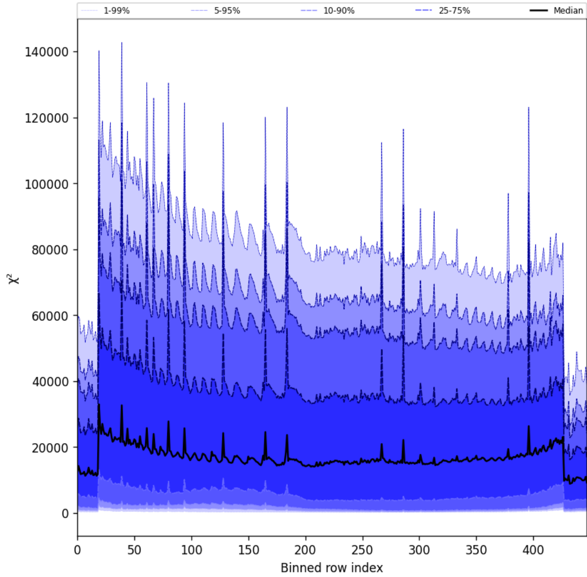
Figure 55: Along track statistics of “ \chi^2 ” for 2024-12-11 to 2024-12-12
