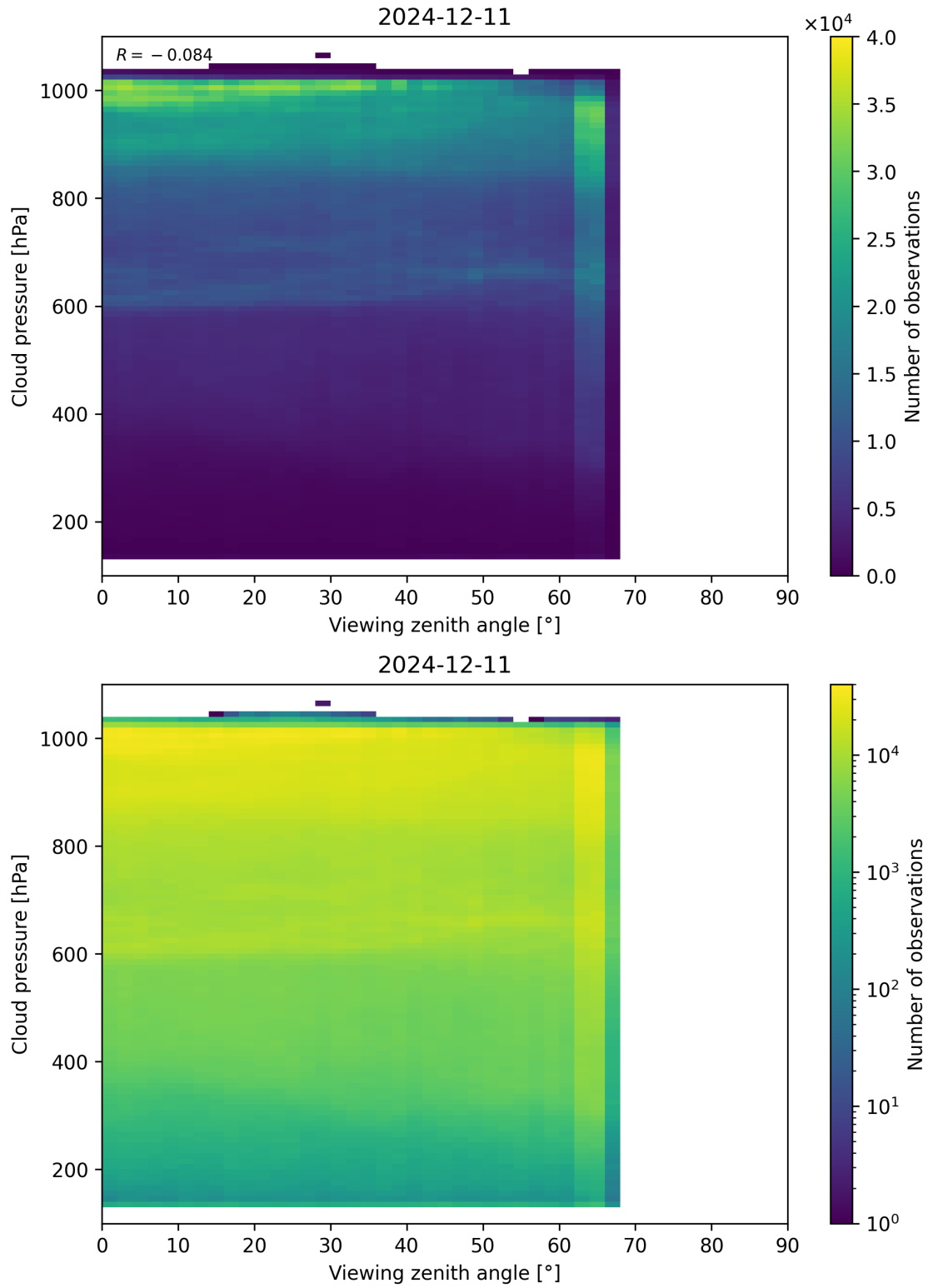
Figure 121: Scatter density plot of “Viewing zenith angle” against “Cloud pressure” for 2024-12-11 to 2024-12-12.
