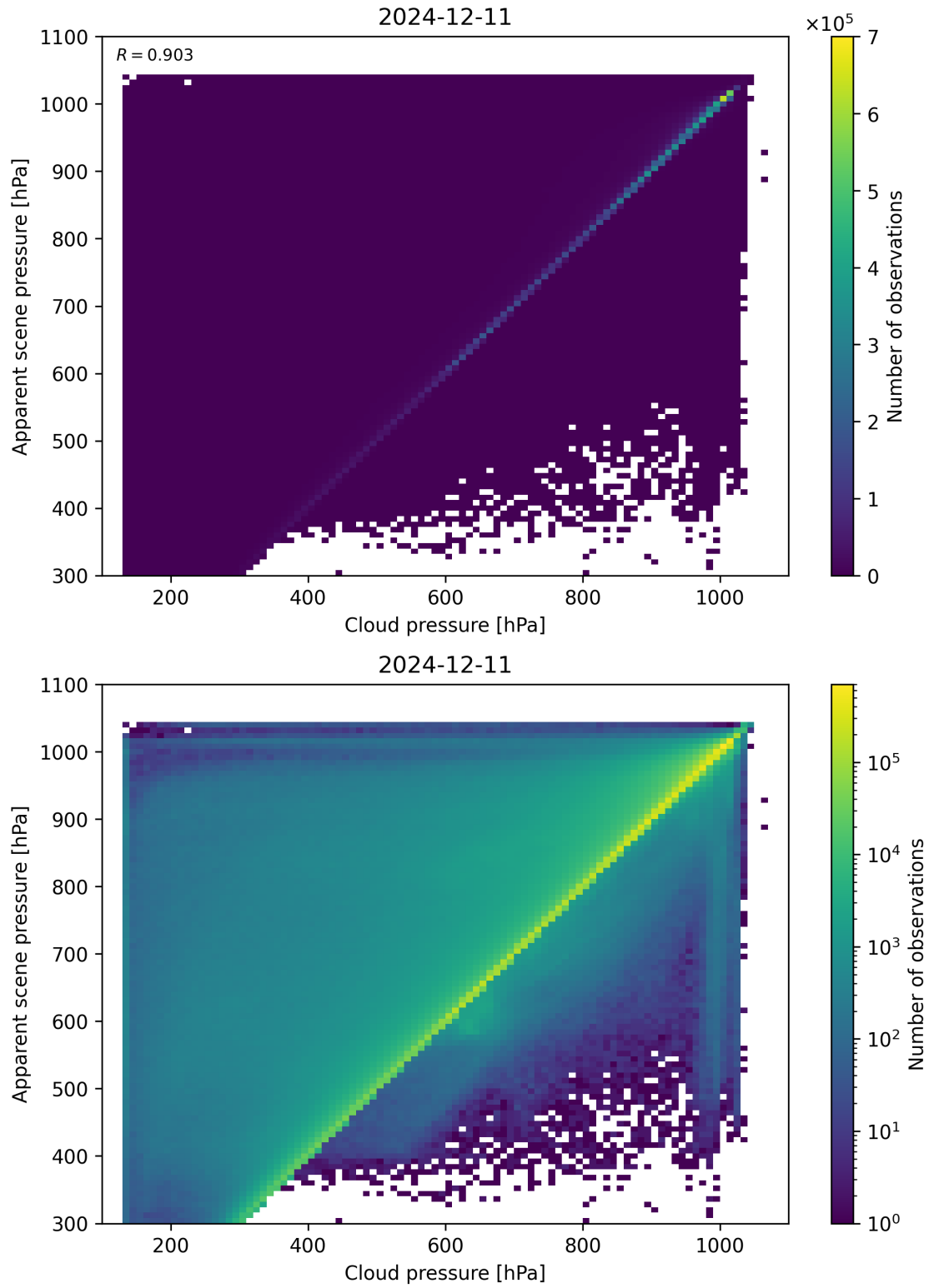
Figure 77: Scatter density plot of “Cloud pressure” against “Apparent scene pressure” for 2024-12-11 to 2024-12-12.
