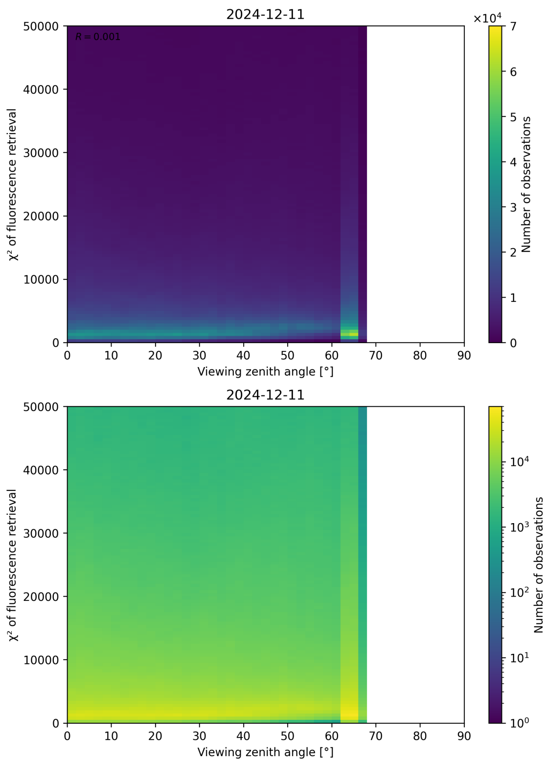
Figure 119: Scatter density plot of “Viewing zenith angle” against “ \chi^2 of fluorescence retrieval” for 2024-12-11 to 2024-12-12.
