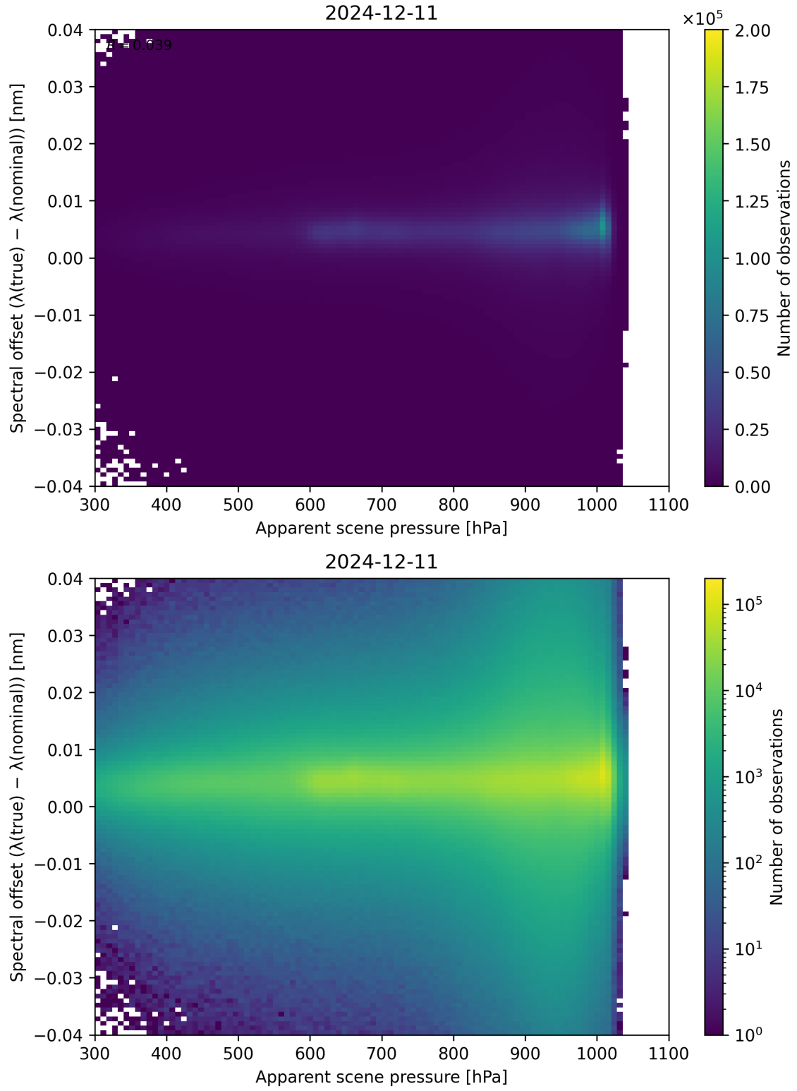
Figure 67: Scatter density plot of “Apparent scene pressure” against “Spectral offset ( \lambda_{\text{true}} - \lambda_{\text{nominal}} )” for 2024-12-11 to 2024-12-12.
