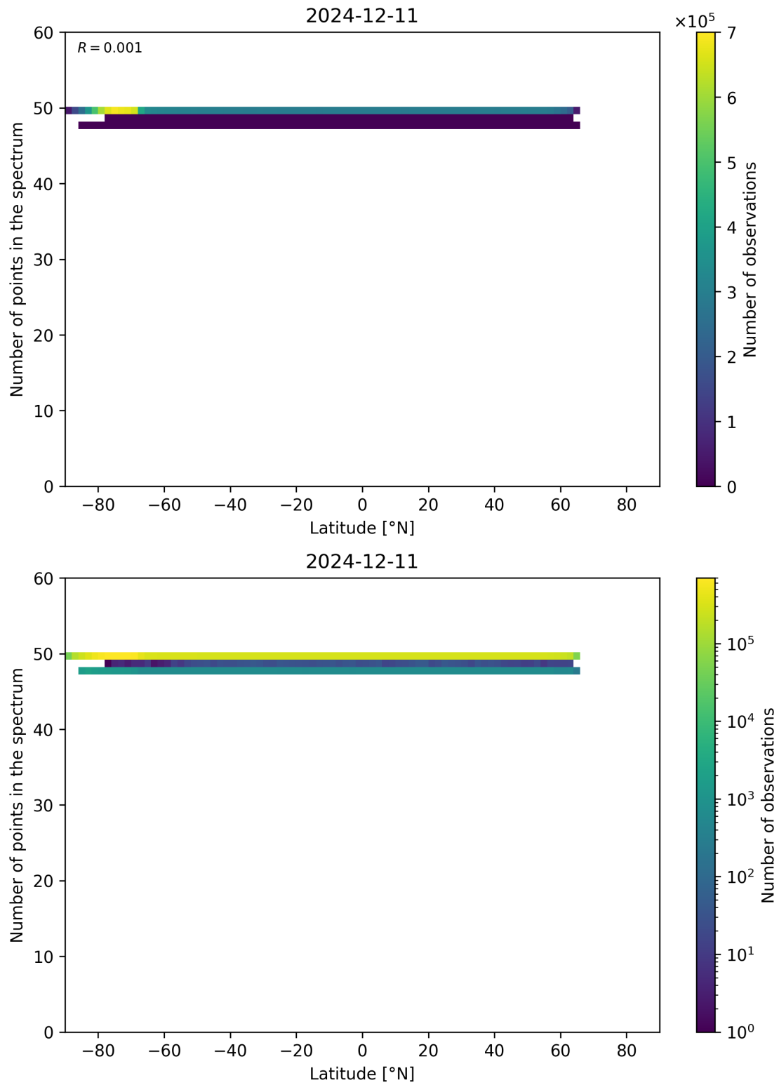
Figure 94: Scatter density plot of “Latitude” against “Number of points in the spectrum” for 2024-12-11 to 2024-12-12.
