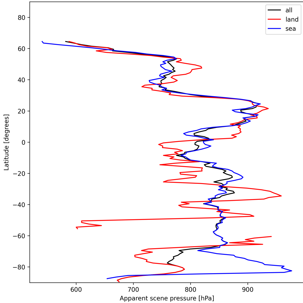
Figure 19: Zonal average of “Apparent scene pressure” for 2024-12-11 to 2024-12-12.
