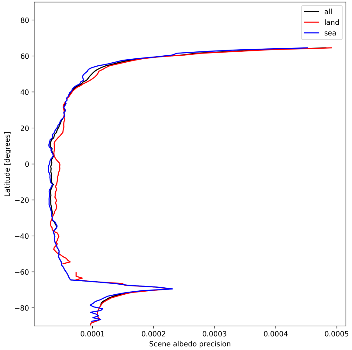
Figure 18: Zonal average of “Scene albedo precision” for 2024-12-11 to 2024-12-12.
