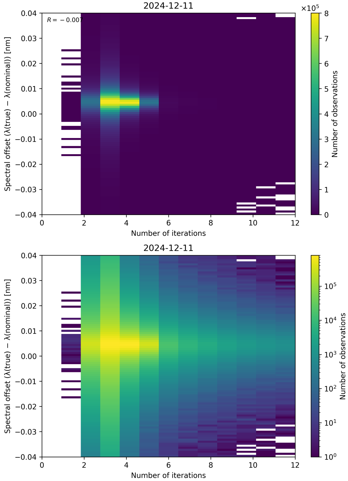
Figure 100: Scatter density plot of “Number of iterations” against “Spectral offset ( \lambda_{\text{true}} - \lambda_{\text{nominal}} )” for 2024-12-11 to 2024-12-12.
