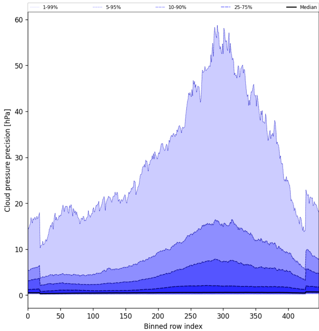
Figure 48: Along track statistics of “Cloud pressure precision” for 2024-12-11 to 2024-12-12
