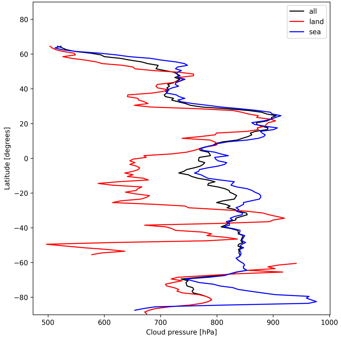
Figure 13: Zonal average of “Cloud pressure” for 2024-12-11 to 2024-12-12.
