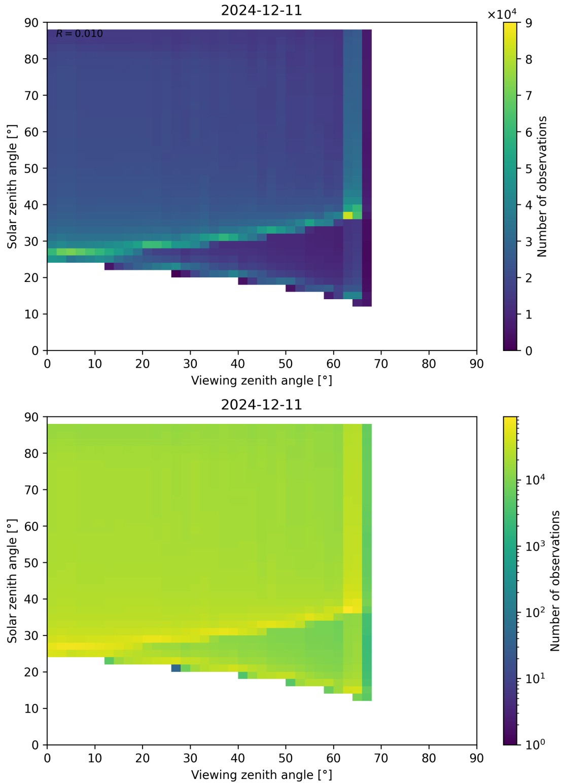
Figure 127: Scatter density plot of “Viewing zenith angle” against “Solar zenith angle” for 2024-12-11 to 2024-12-12.
