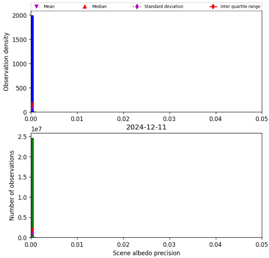
Figure 35: Histogram of “Scene albedo precision” for 2024-12-11 to 2024-12-12
