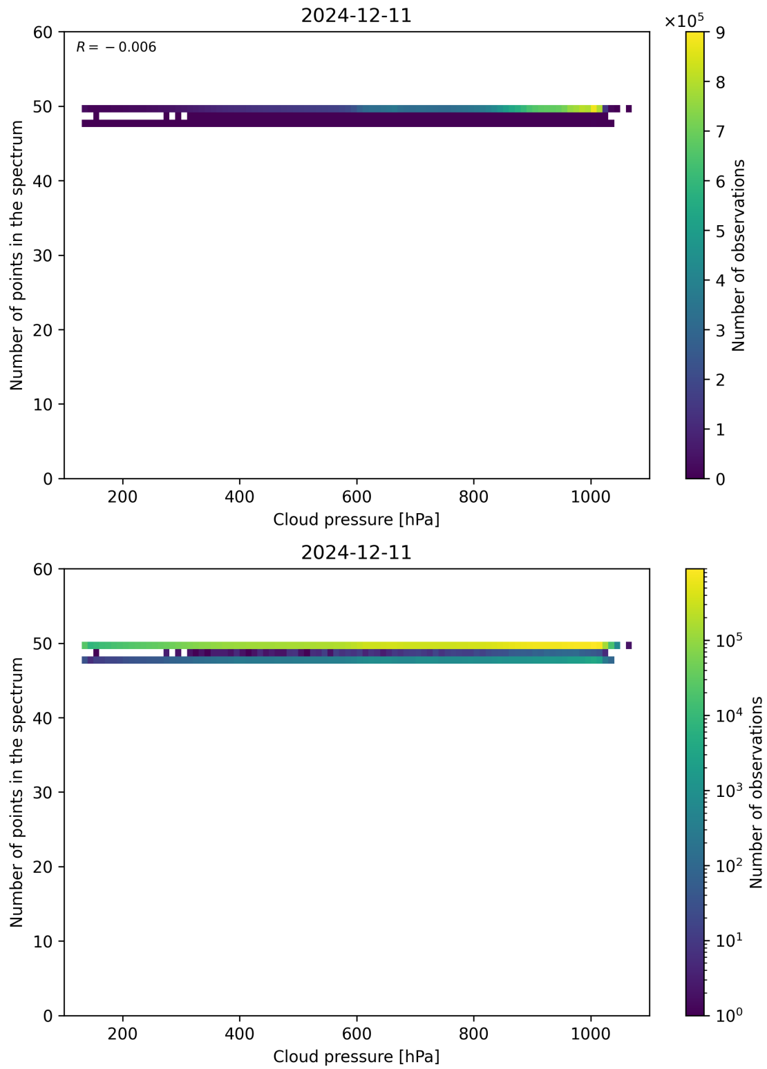
Figure 82: Scatter density plot of “Cloud pressure” against “Number of points in the spectrum” for 2024-12-11 to 2024-12-12.
