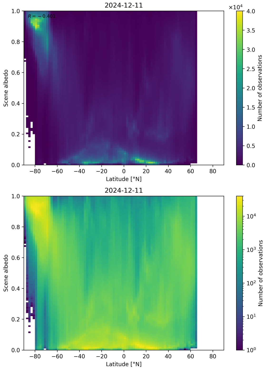
Figure 95: Scatter density plot of “Latitude” against “Scene albedo” for 2024-12-11 to 2024-12-12.
