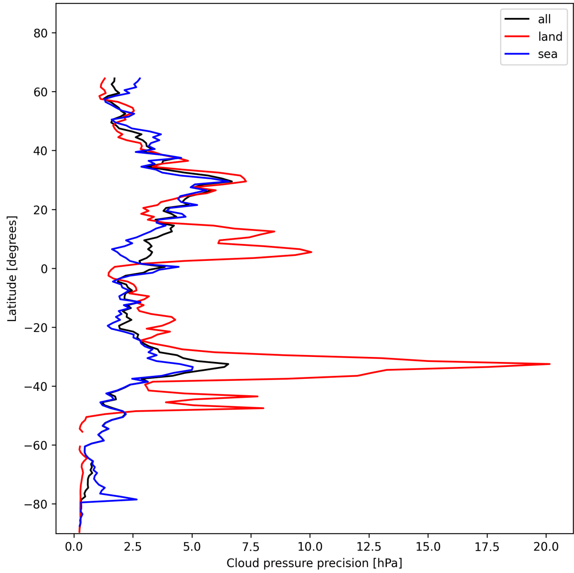
Figure 14: Zonal average of “Cloud pressure precision” for 2024-12-11 to 2024-12-12.
