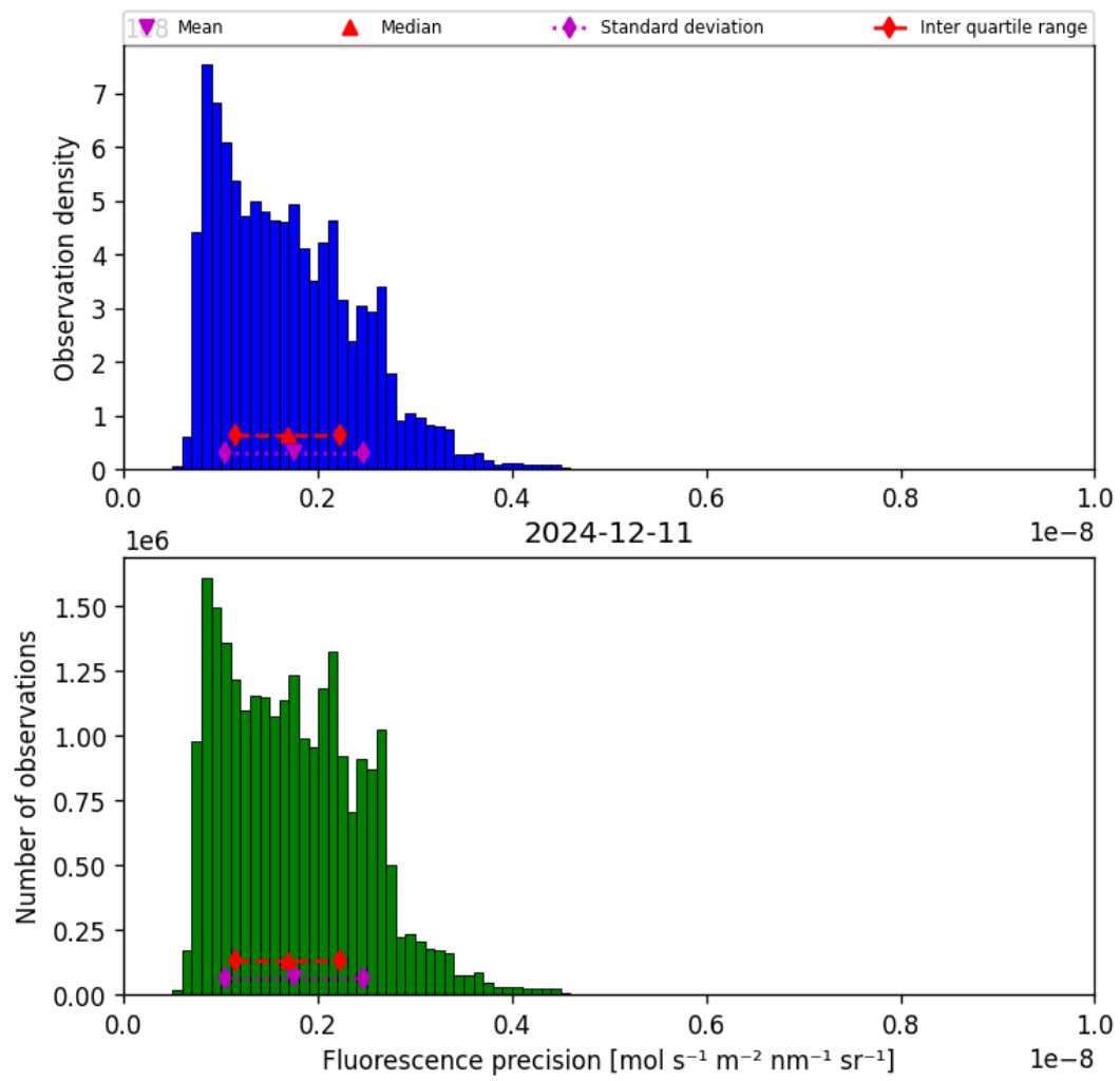
Figure 41: Histogram of “Fluorescence precision” for 2024-12-11 to 2024-12-12
