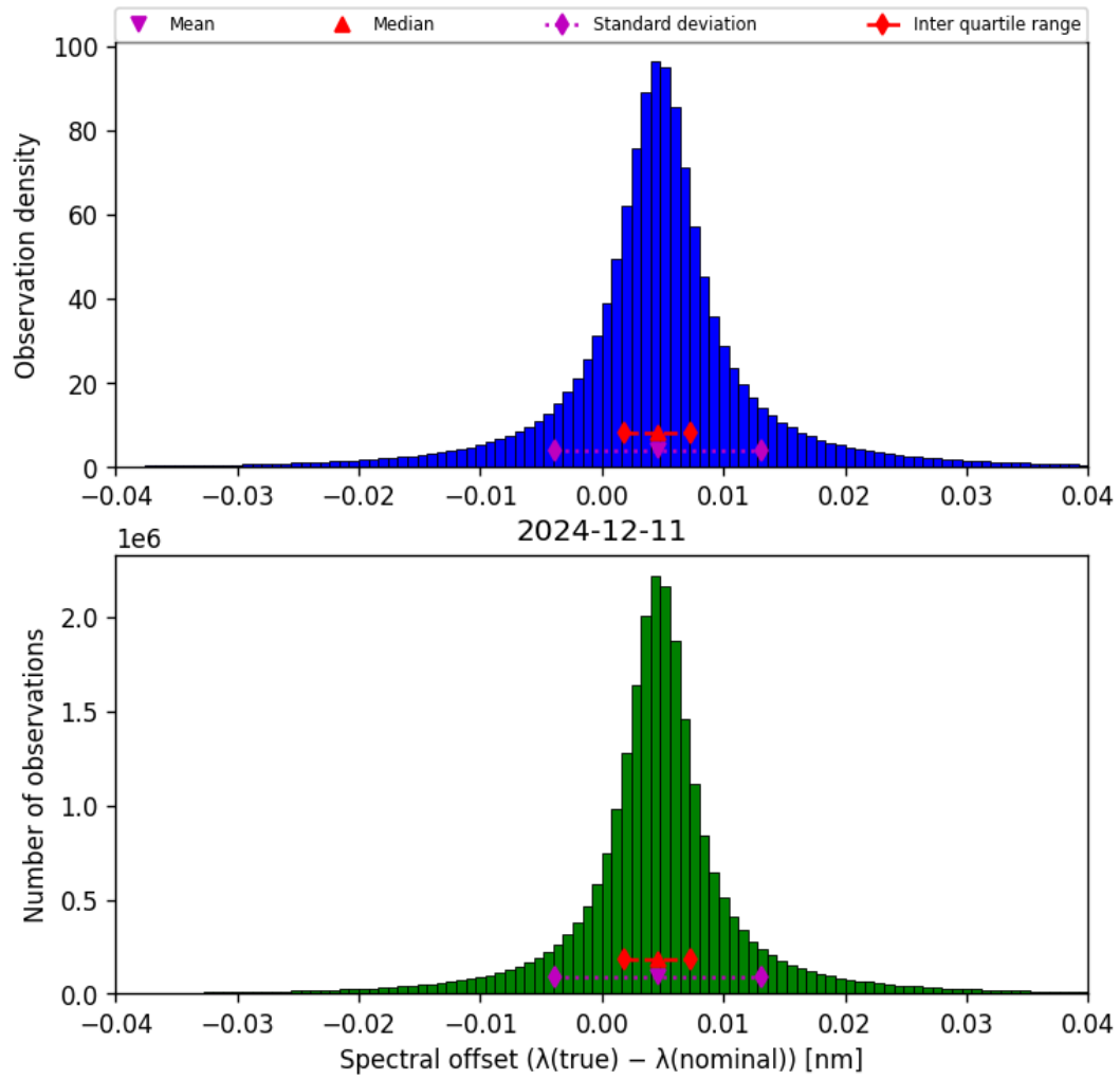
Figure 45: Histogram of “Spectral offset ( \lambda_{\text{true}} - \lambda_{\text{nominal}} )” for 2024-12-11 to 2024-12-12
