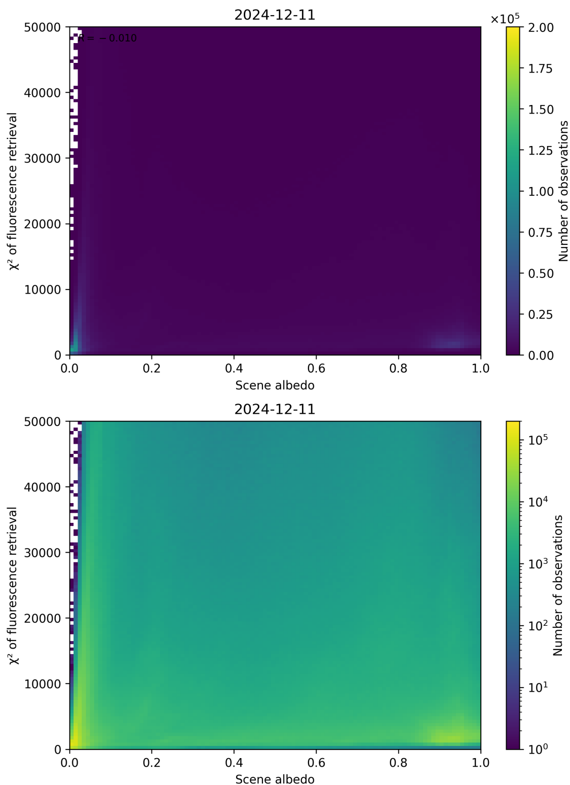
Figure 103: Scatter density plot of “Scene albedo” against “ \chi^2 of fluorescence retrieval” for 2024-12-11 to 2024-12-12.
