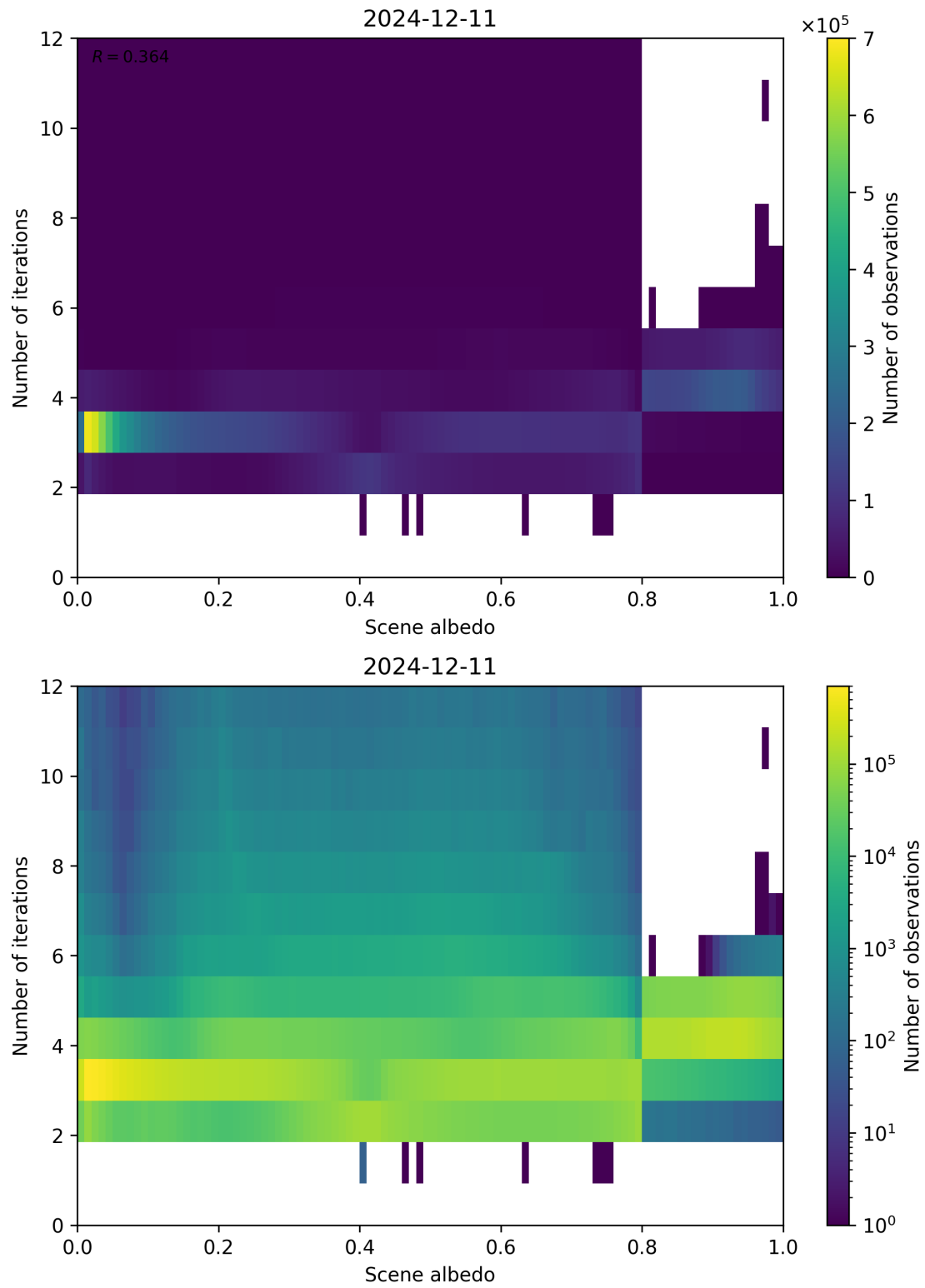
Figure 105: Scatter density plot of “Scene albedo” against “Number of iterations” for 2024-12-11 to 2024-12-12.
