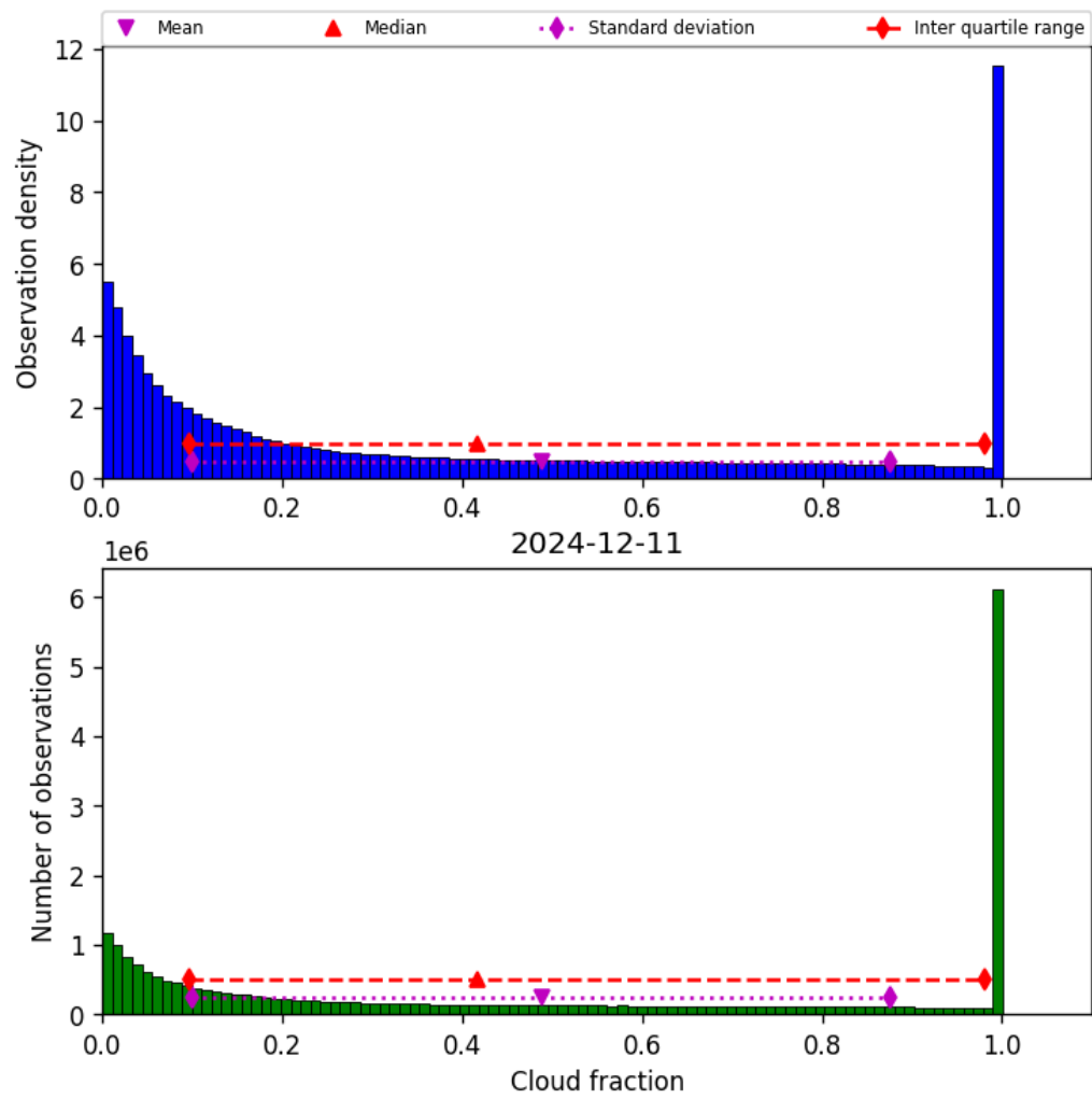
Figure 32: Histogram of “Cloud fraction” for 2024-12-11 to 2024-12-12
