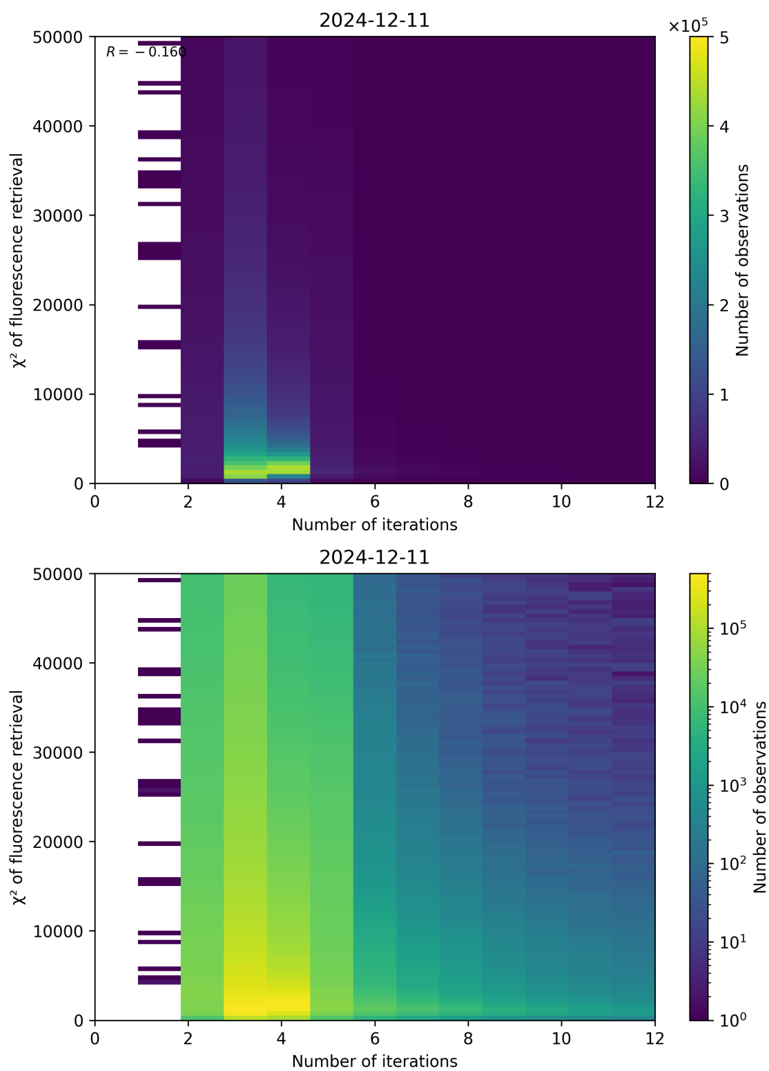
Figure 97: Scatter density plot of “Number of iterations” against “ \chi^2 of fluorescence retrieval” for 2024-12-11 to 2024-12-12.
