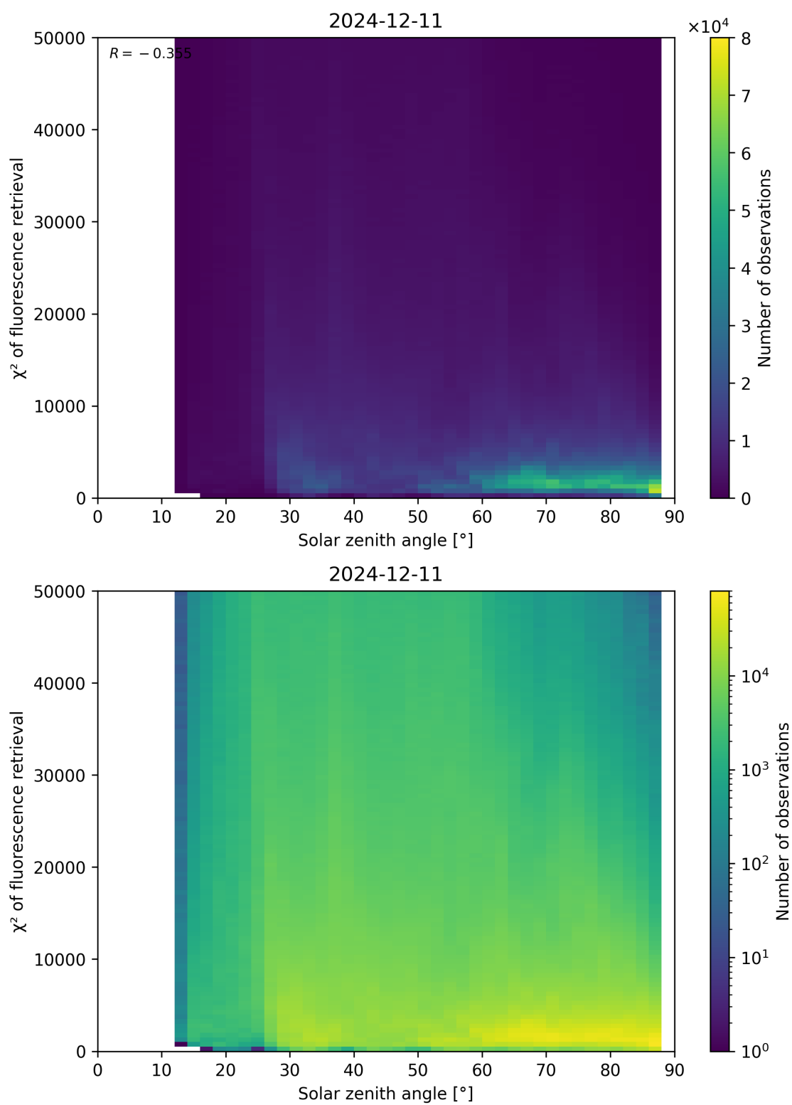
Figure 109: Scatter density plot of “Solar zenith angle” against “ \chi^2 of fluorescence retrieval” for 2024-12-11 to 2024-12-12.
