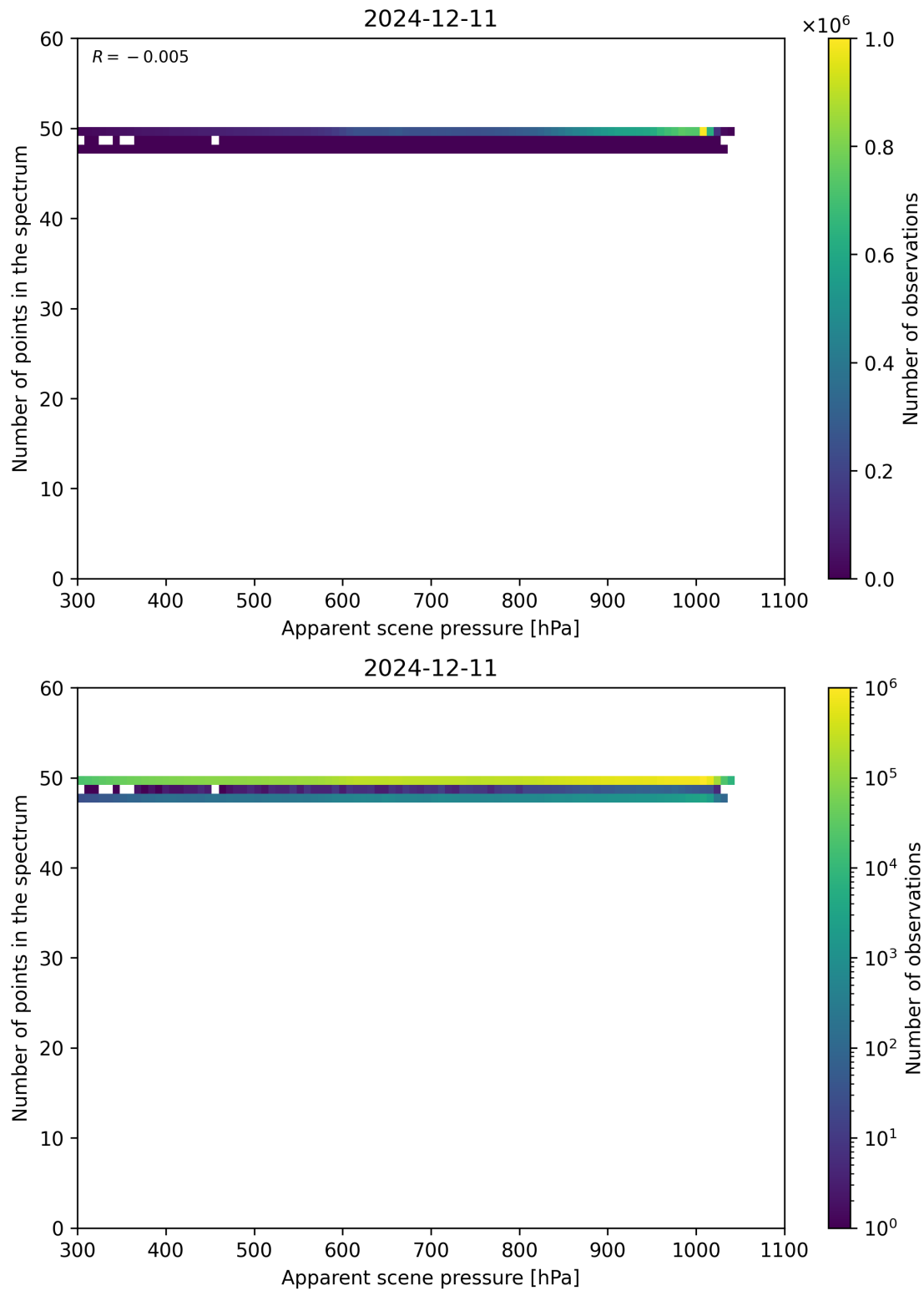
Figure 66: Scatter density plot of “Apparent scene pressure” against “Number of points in the spectrum” for 2024-12-11 to 2024-12-12.
