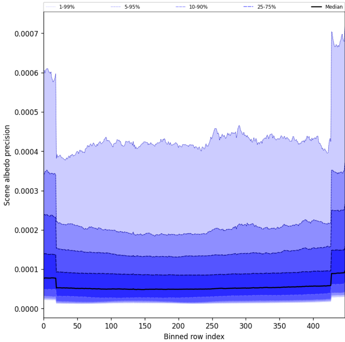
Figure 52: Along track statistics of “Scene albedo precision” for 2024-12-11 to 2024-12-12
