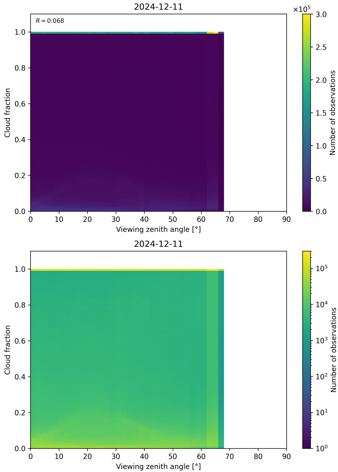
Figure 120: Scatter density plot of “Viewing zenith angle” against “Cloud fraction” for 2024-12-11 to 2024-12-12.
