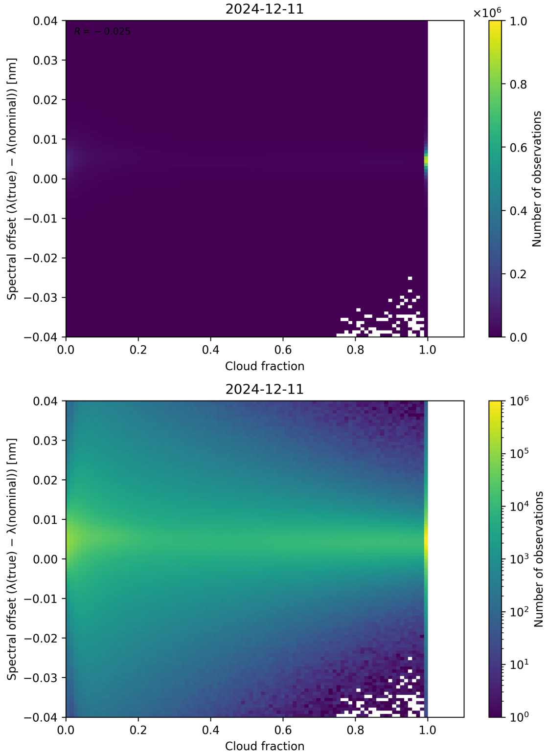
Figure 76: Scatter density plot of “Cloud fraction” against “Spectral offset ( \lambda_{\text{true}} - \lambda_{\text{nominal}} )” for 2024-12-11 to 2024-12-12.
