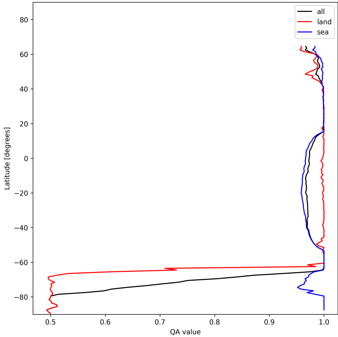
Figure 12: Zonal average of “QA value” for 2024-12-11 to 2024-12-12.
