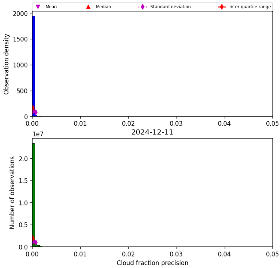
Figure 33: Histogram of “Cloud fraction precision” for 2024-12-11 to 2024-12-12
