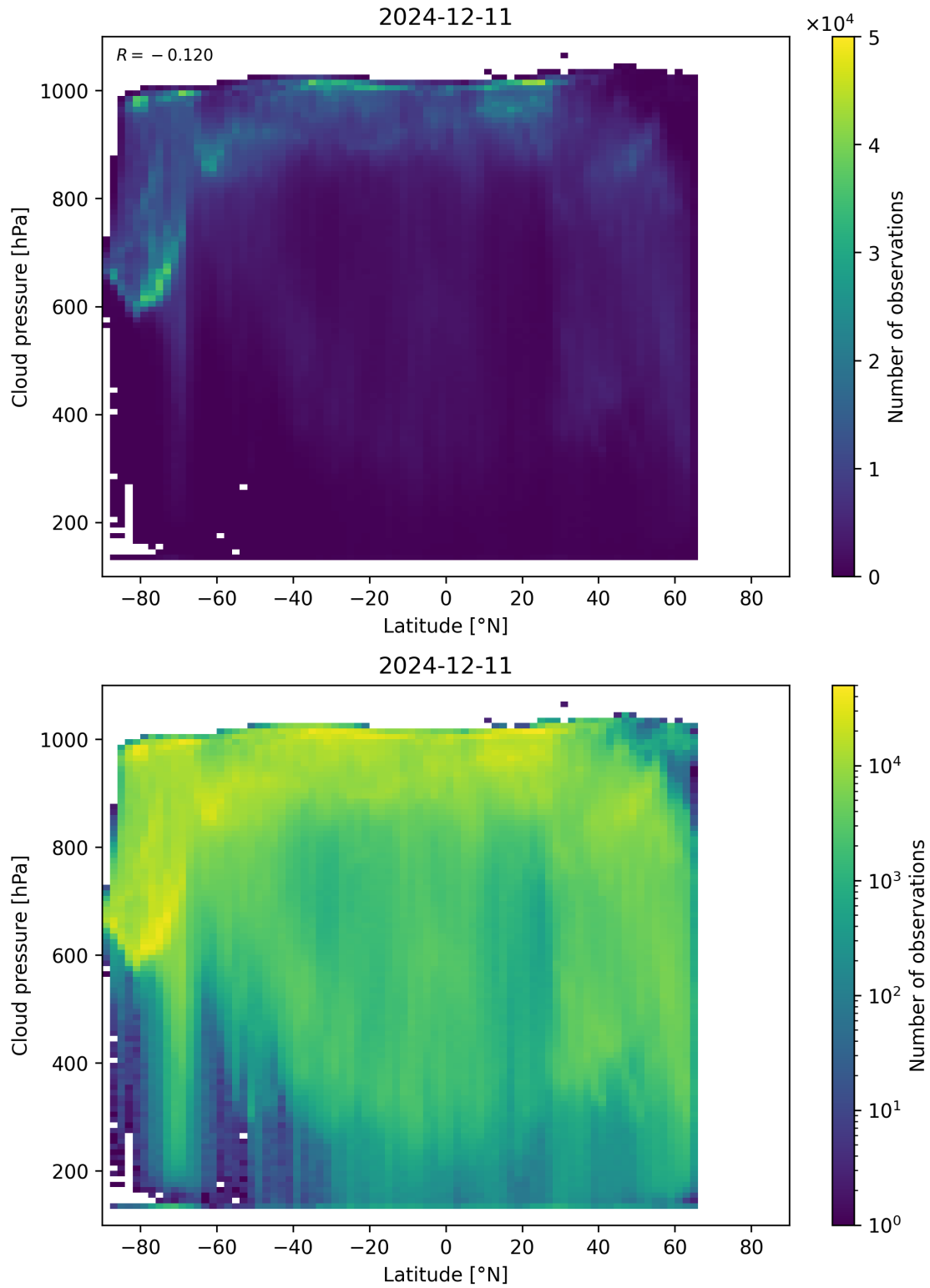
Figure 91: Scatter density plot of “Latitude” against “Cloud pressure” for 2024-12-11 to 2024-12-12.
