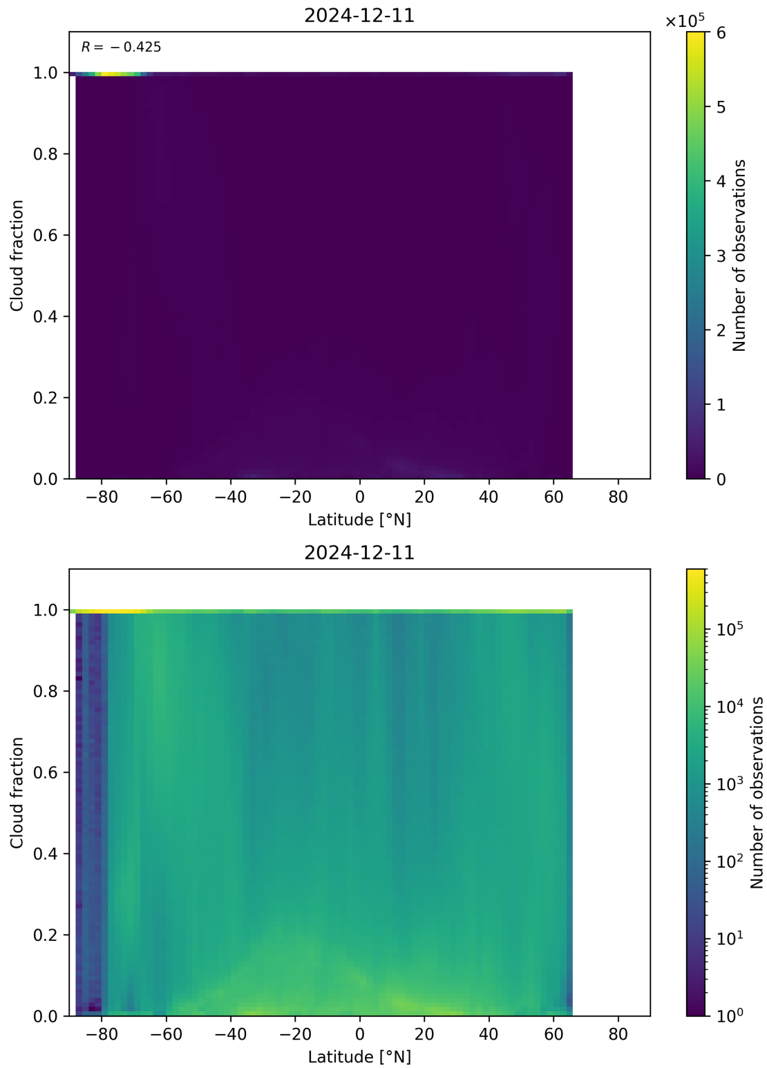
Figure 90: Scatter density plot of “Latitude” against “Cloud fraction” for 2024-12-11 to 2024-12-12.
