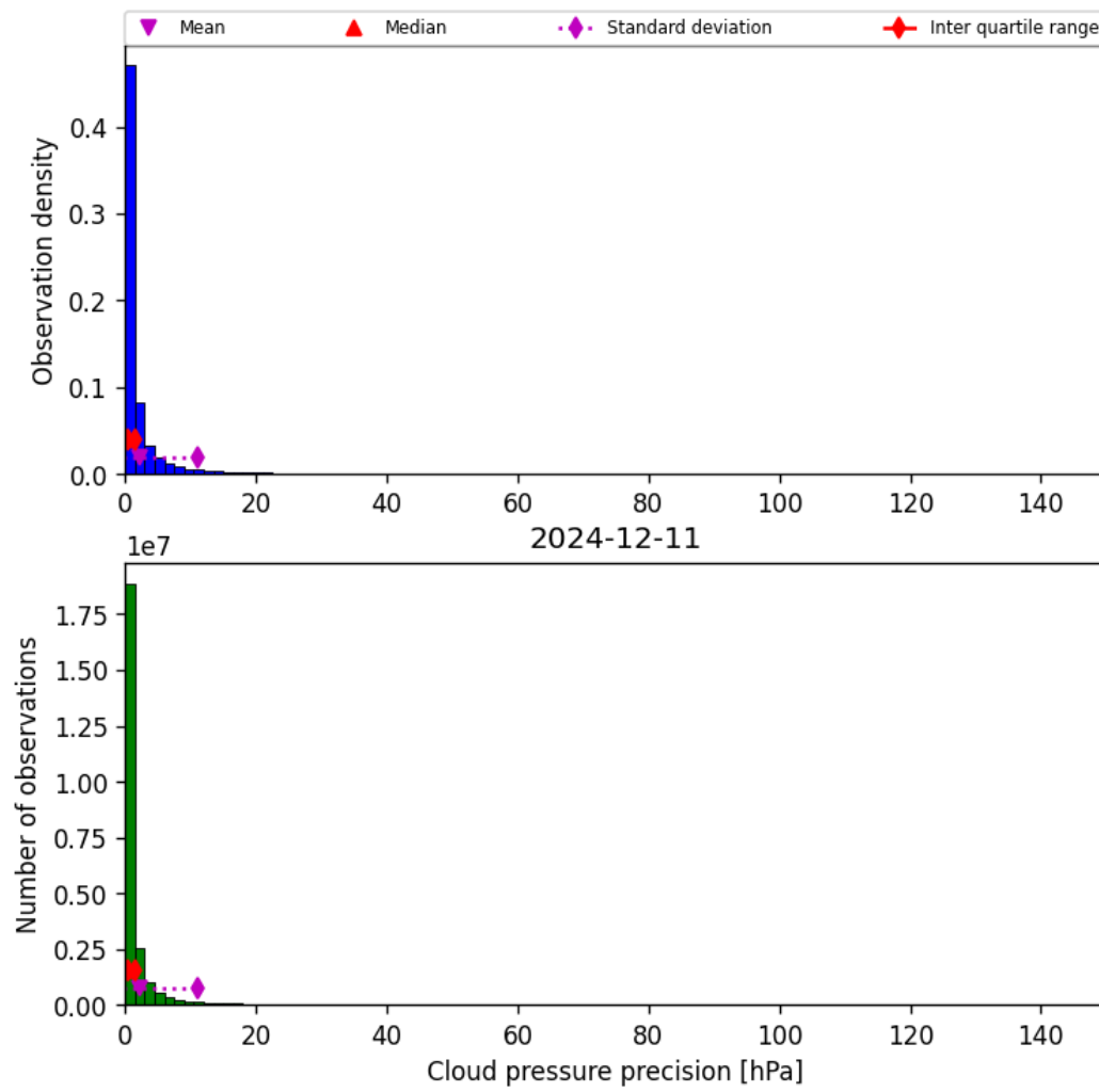
Figure 31: Histogram of “Cloud pressure precision” for 2024-12-11 to 2024-12-12
