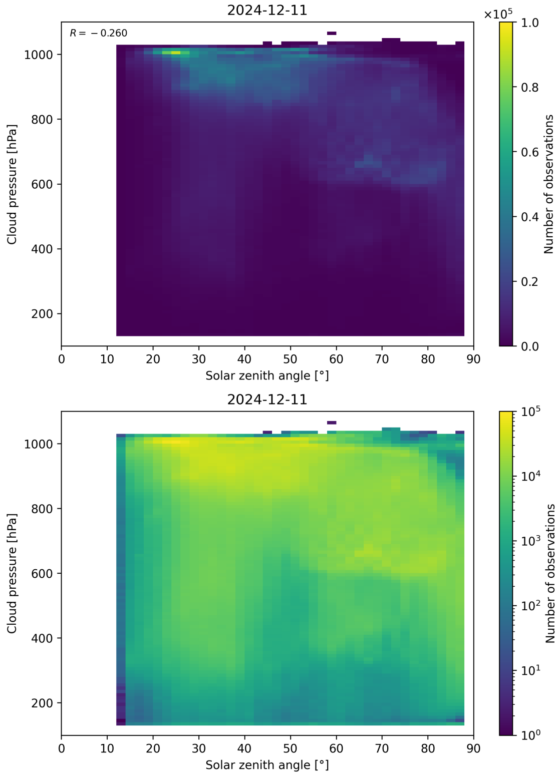
Figure 111: Scatter density plot of “Solar zenith angle” against “Cloud pressure” for 2024-12-11 to 2024-12-12.
