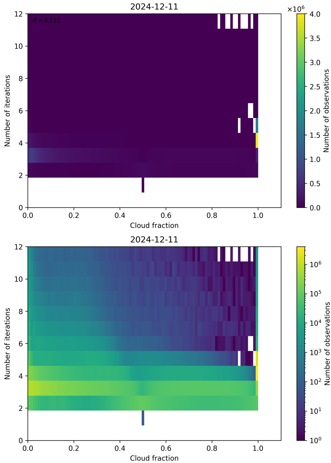
Figure 73: Scatter density plot of “Cloud fraction” against “Number of iterations” for 2024-12-11 to 2024-12-12.
