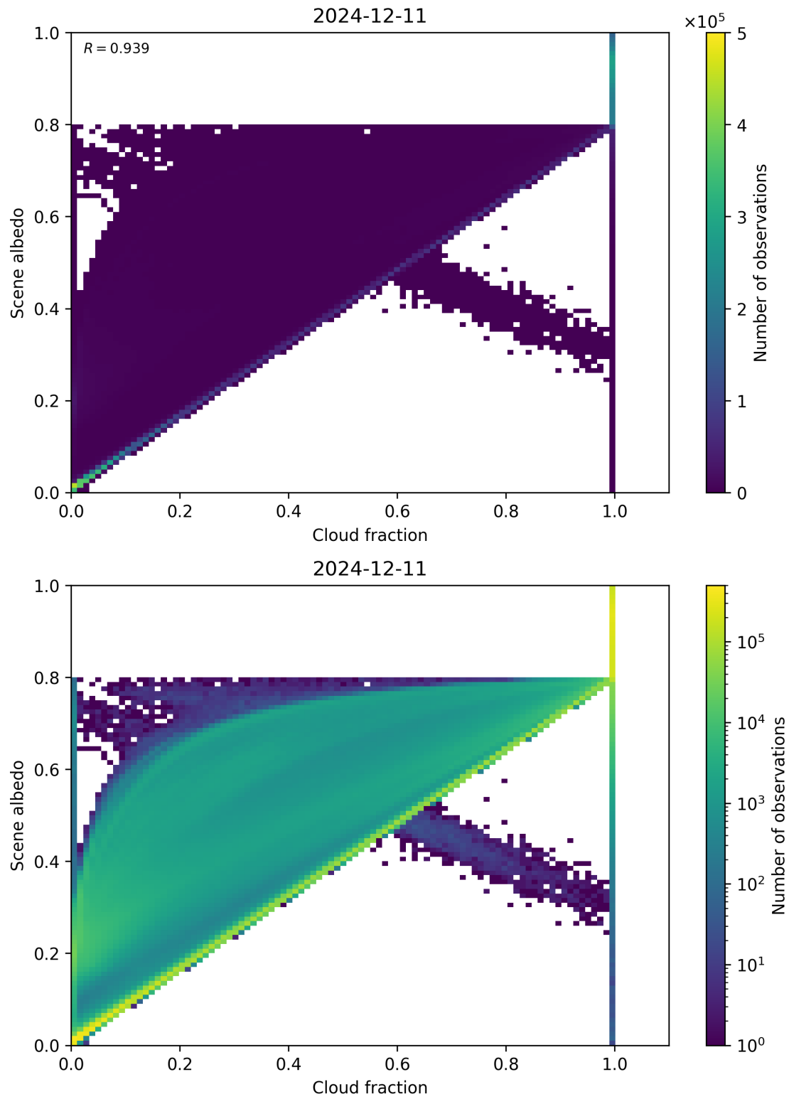
Figure 75: Scatter density plot of “Cloud fraction” against “Scene albedo” for 2024-12-11 to 2024-12-12.
