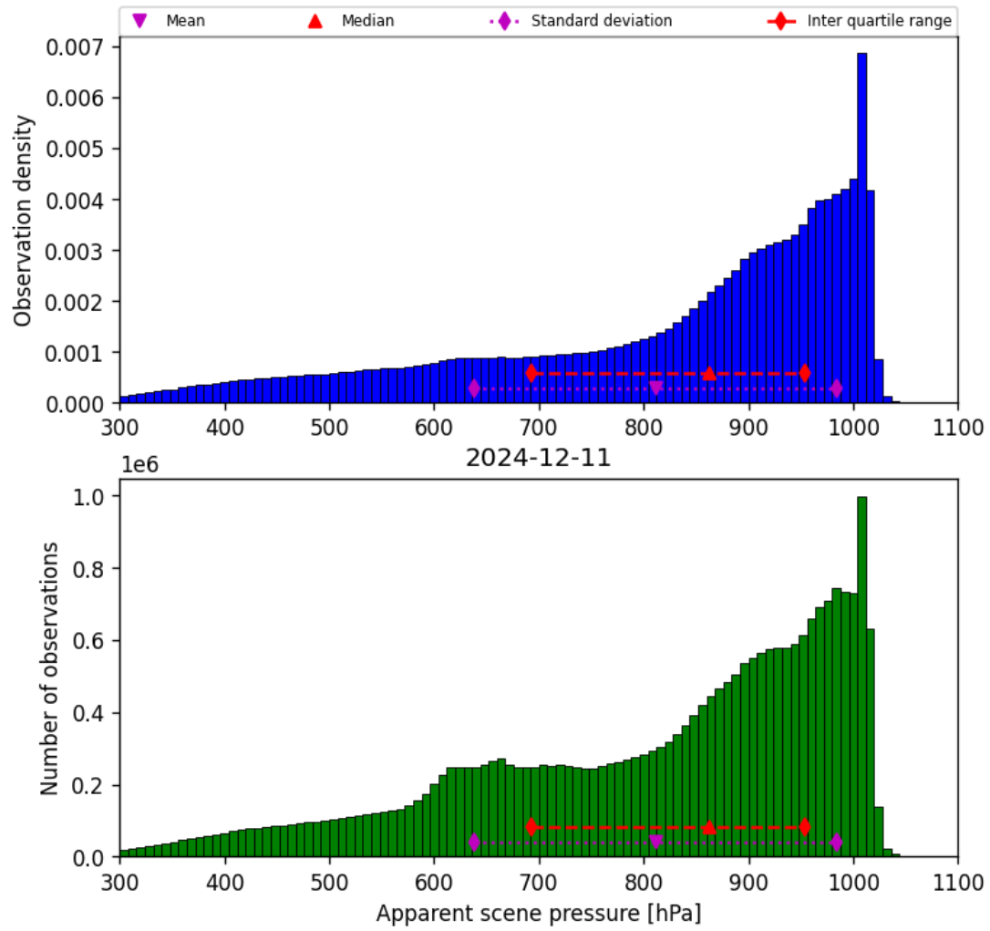
Figure 36: Histogram of “Apparent scene pressure” for 2024-12-11 to 2024-12-12
