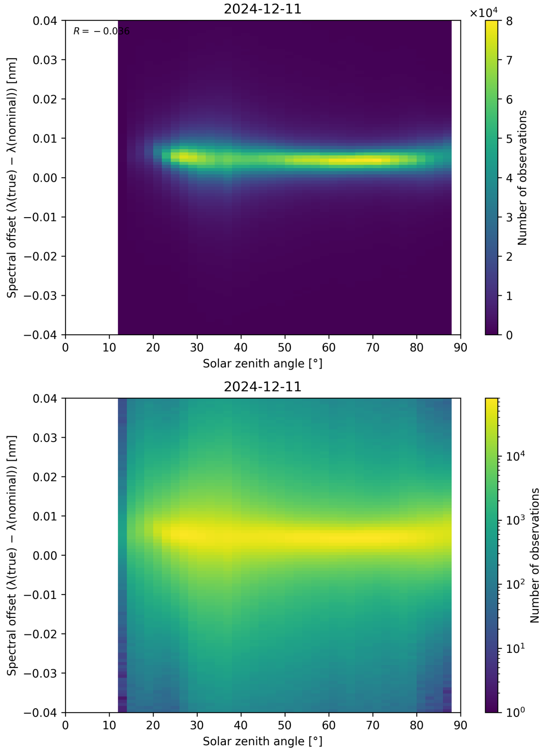
Figure 117: Scatter density plot of “Solar zenith angle” against “Spectral offset ( \lambda_{\text{true}} - \lambda_{\text{nominal}} )” for 2024-12-11 to 2024-12-12.
