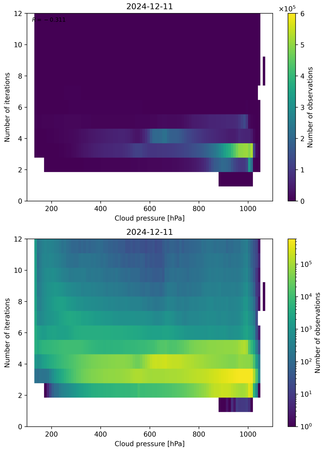
Figure 81: Scatter density plot of “Cloud pressure” against “Number of iterations” for 2024-12-11 to 2024-12-12.
