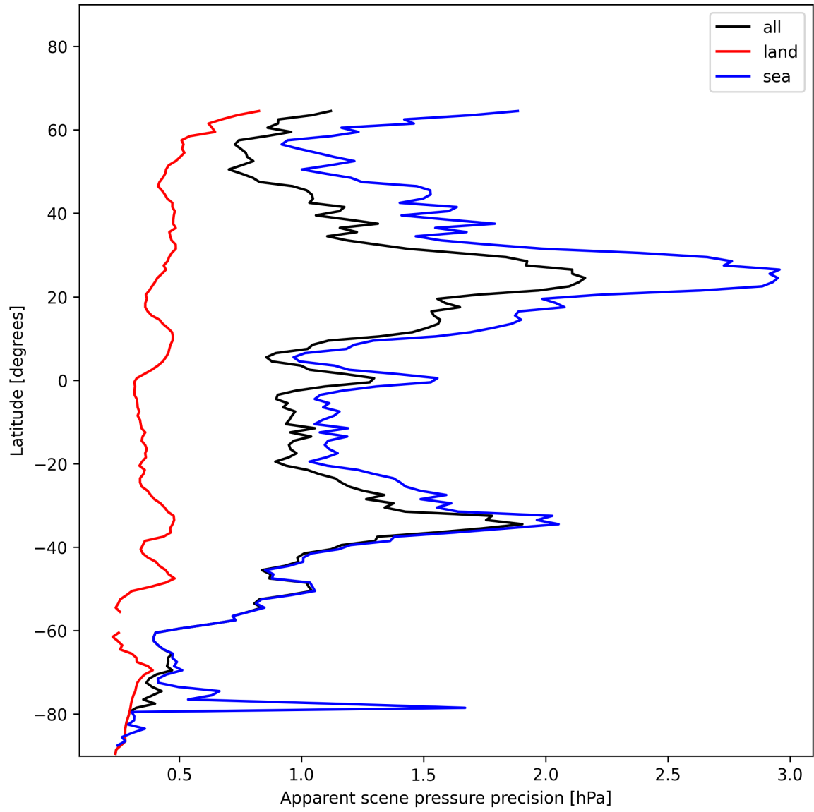
Figure 20: Zonal average of “Apparent scene pressure precision” for 2024-12-11 to 2024-12-12.
