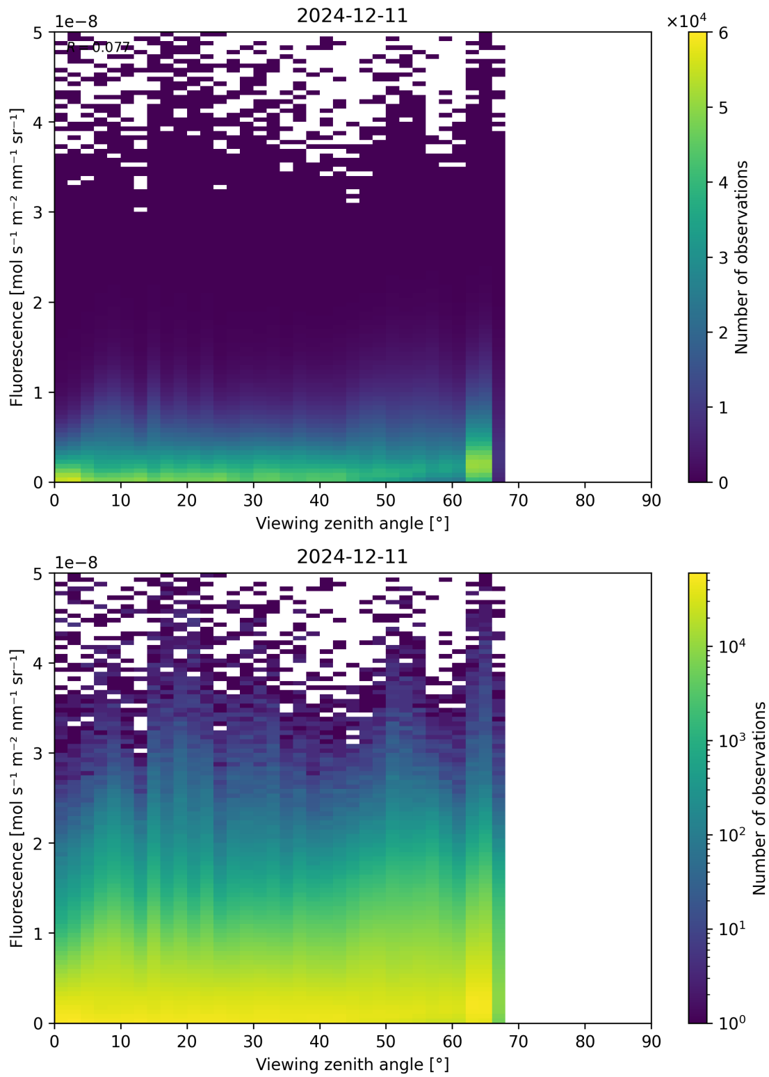
Figure 122: Scatter density plot of “Viewing zenith angle” against “Fluorescence” for 2024-12-11 to 2024-12-12.
