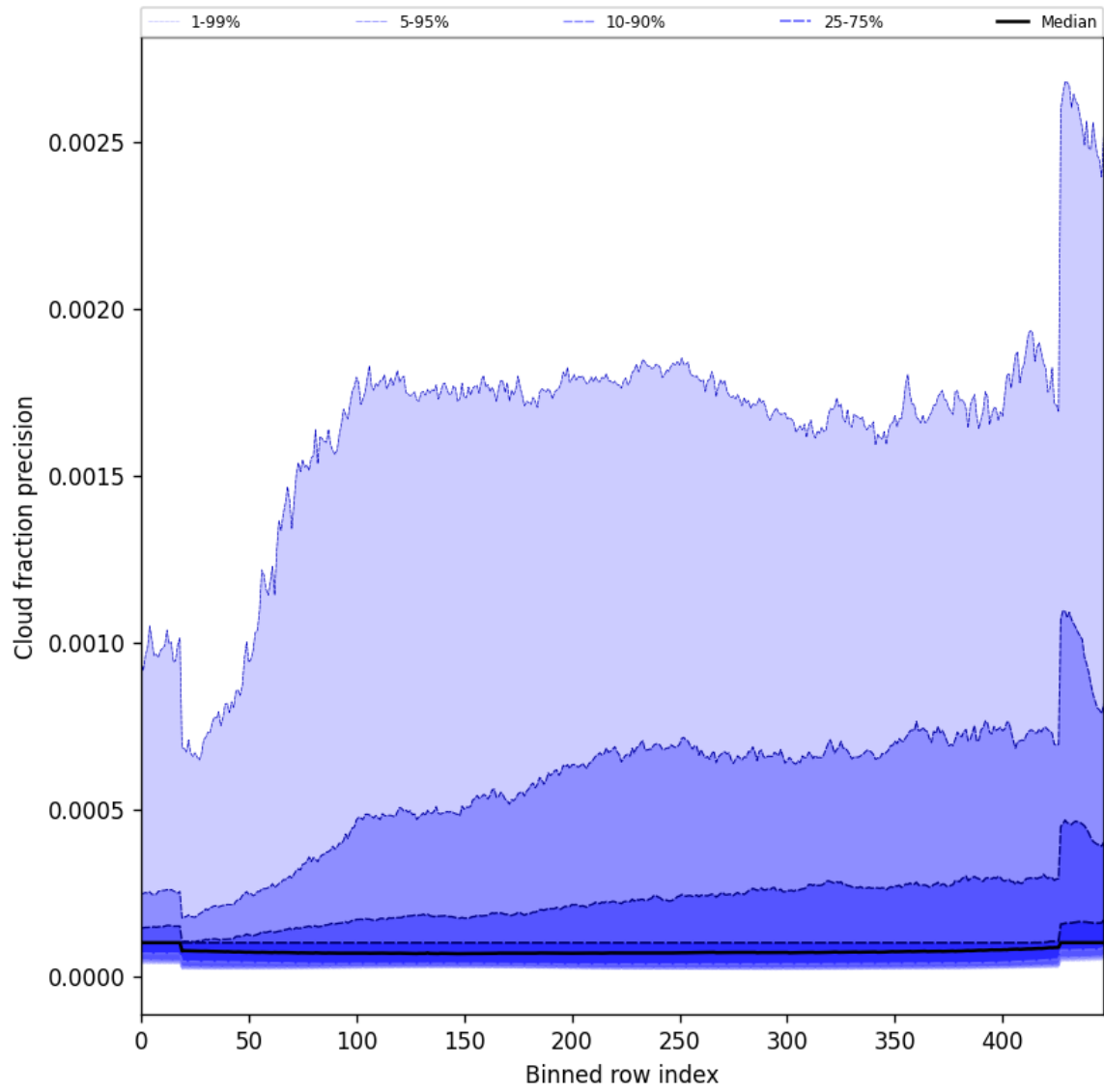
Figure 50: Along track statistics of “Cloud fraction precision” for 2024-12-11 to 2024-12-12
