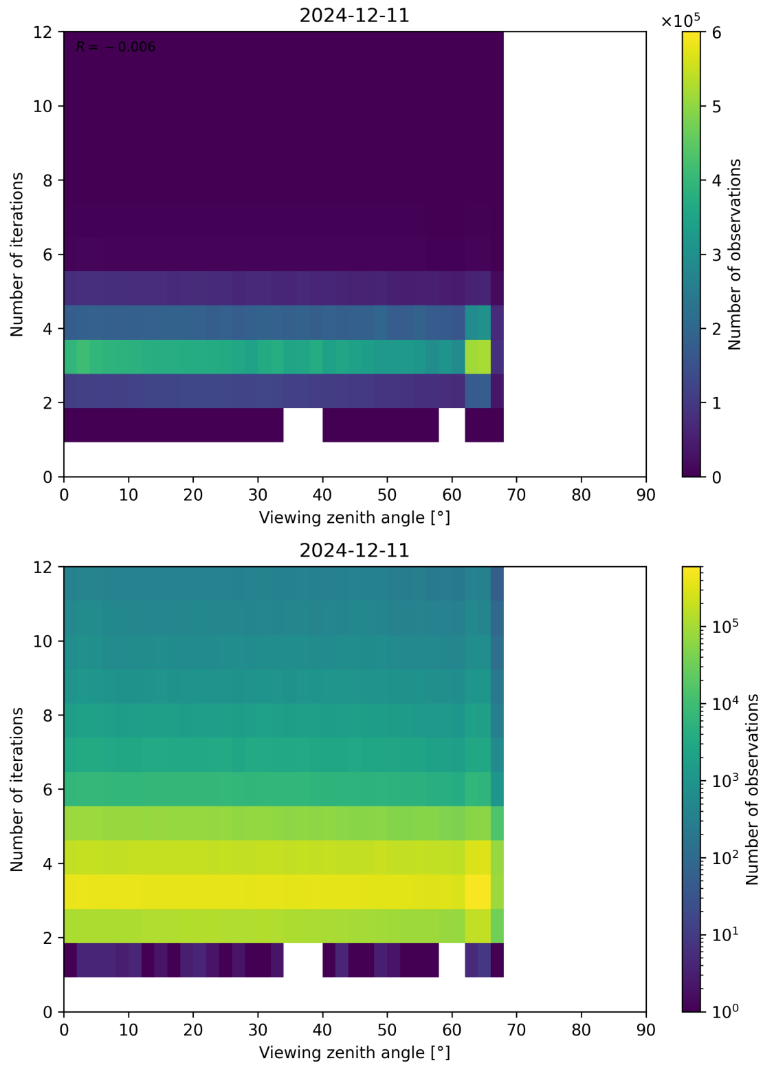
Figure 124: Scatter density plot of “Viewing zenith angle” against “Number of iterations” for 2024-12-11 to 2024-12-12.
