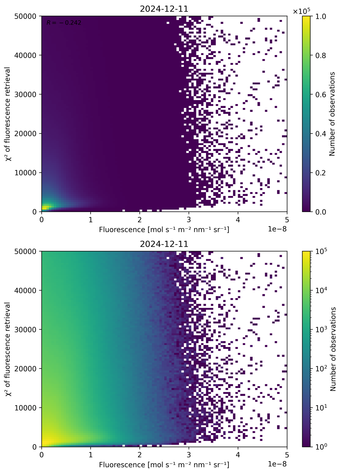
Figure 85: Scatter density plot of “Fluorescence” against “ \chi^2 of fluorescence retrieval” for 2024-12-11 to 2024-12-12.
