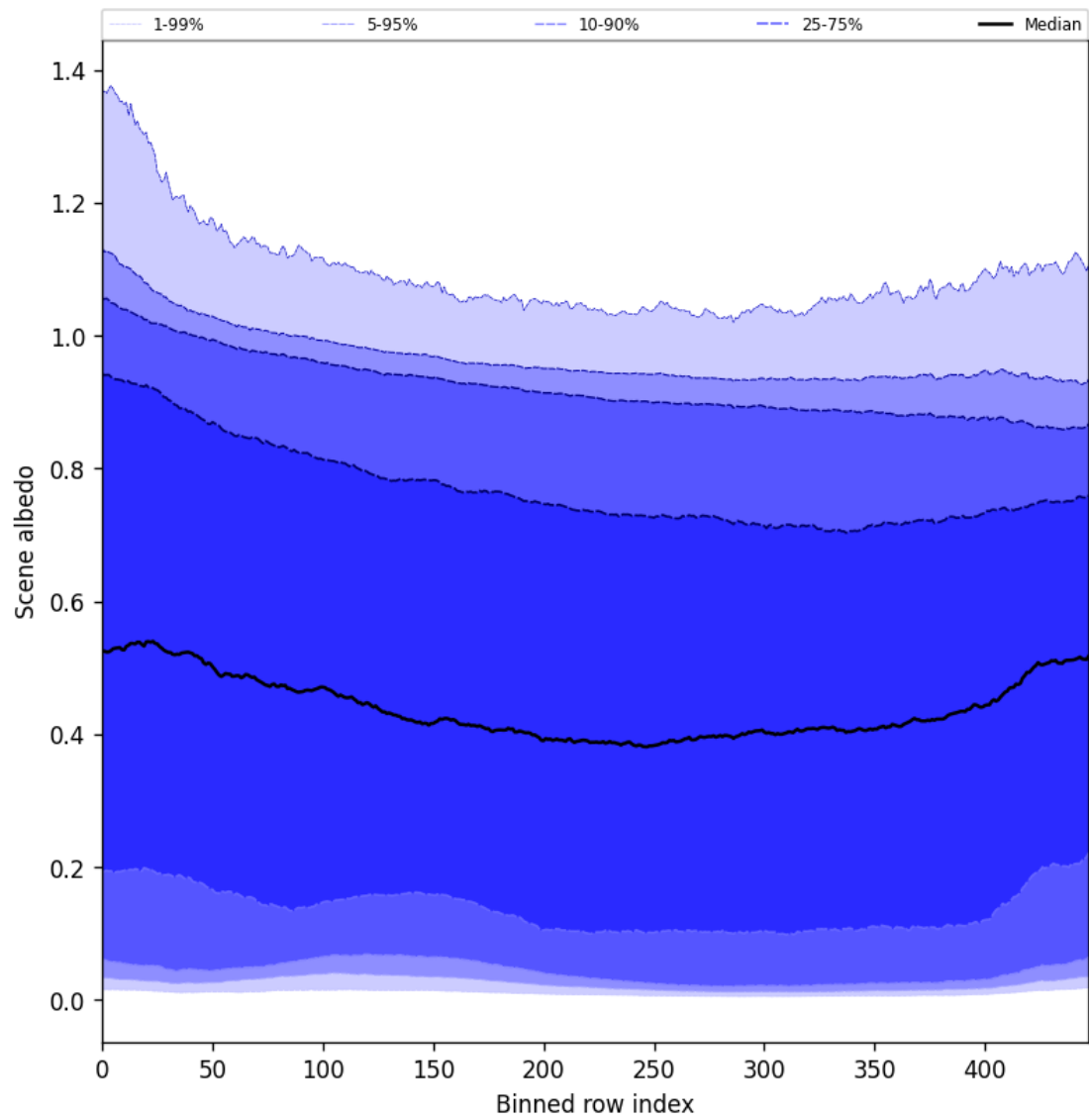
Figure 51: Along track statistics of “Scene albedo” for 2024-12-11 to 2024-12-12
