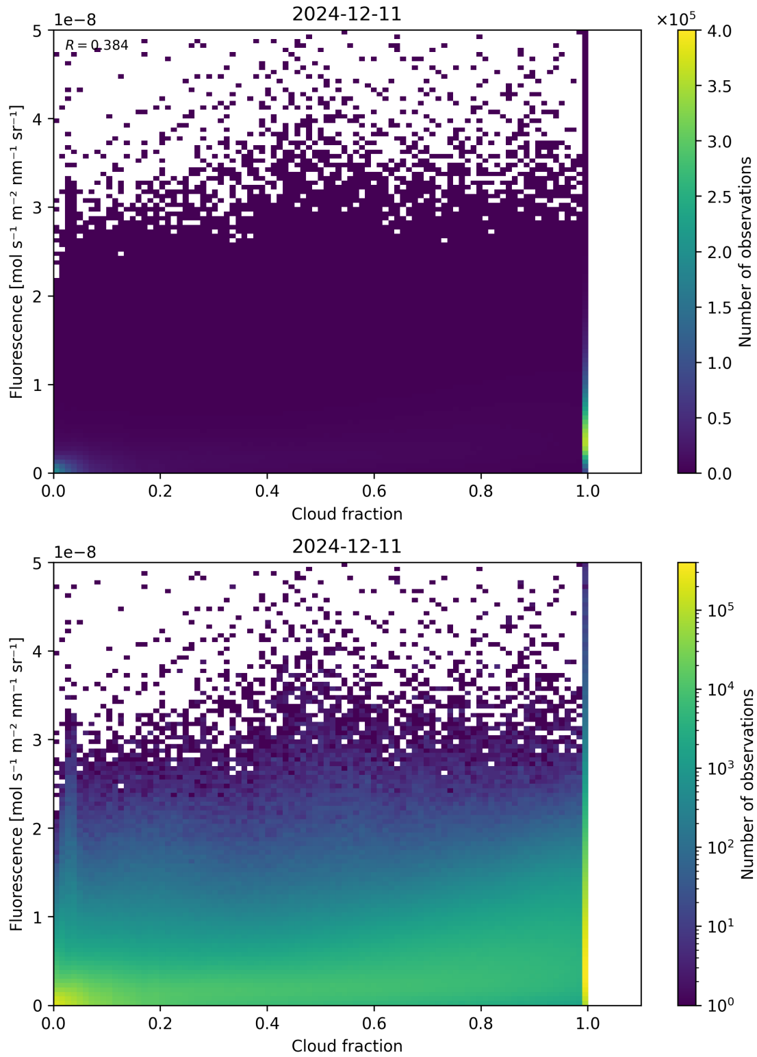
Figure 72: Scatter density plot of “Cloud fraction” against “Fluorescence” for 2024-12-11 to 2024-12-12.
