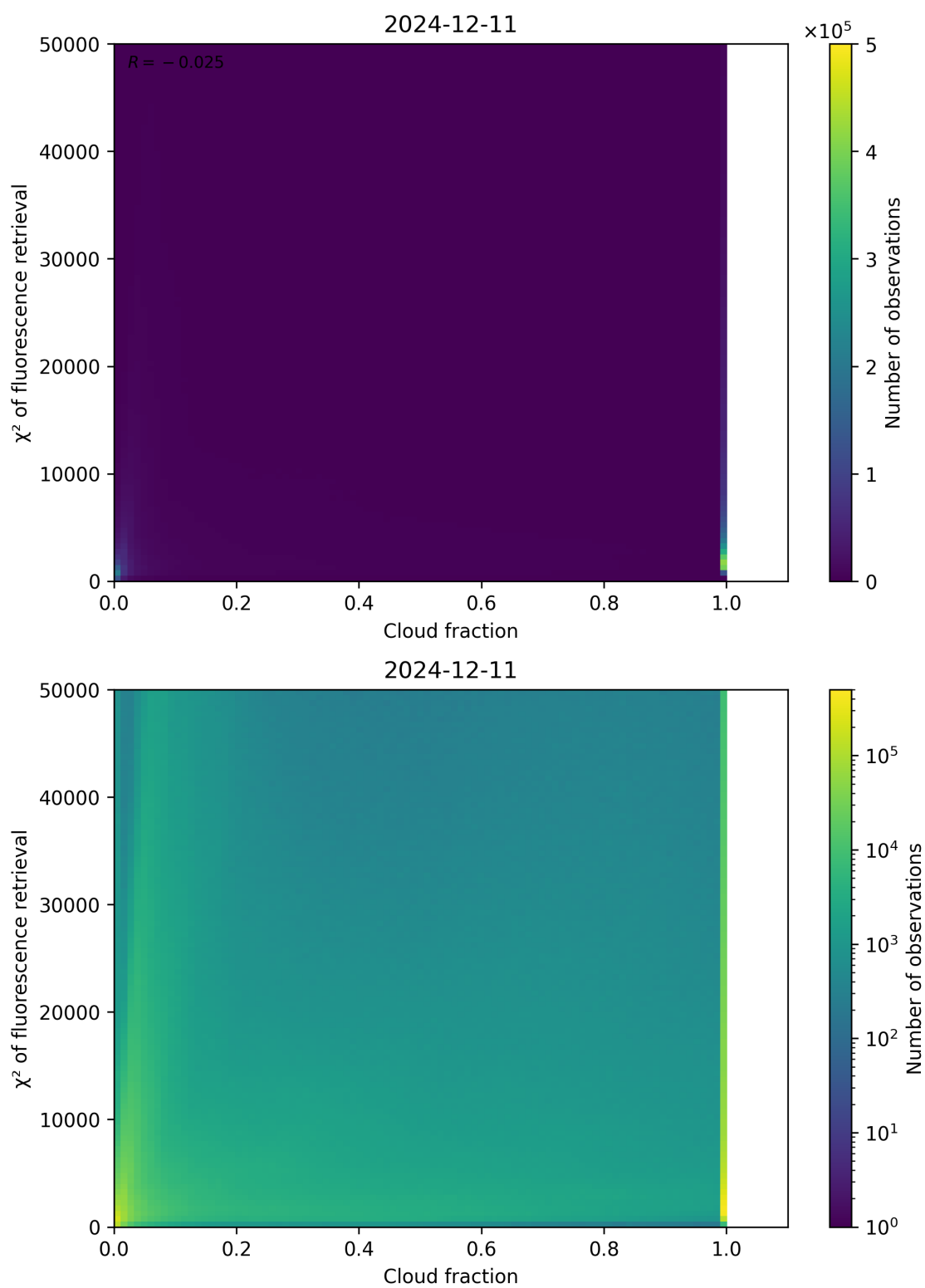
Figure 71: Scatter density plot of “Cloud fraction” against “ \chi^2 of fluorescence retrieval” for 2024-12-11 to 2024-12-12.
