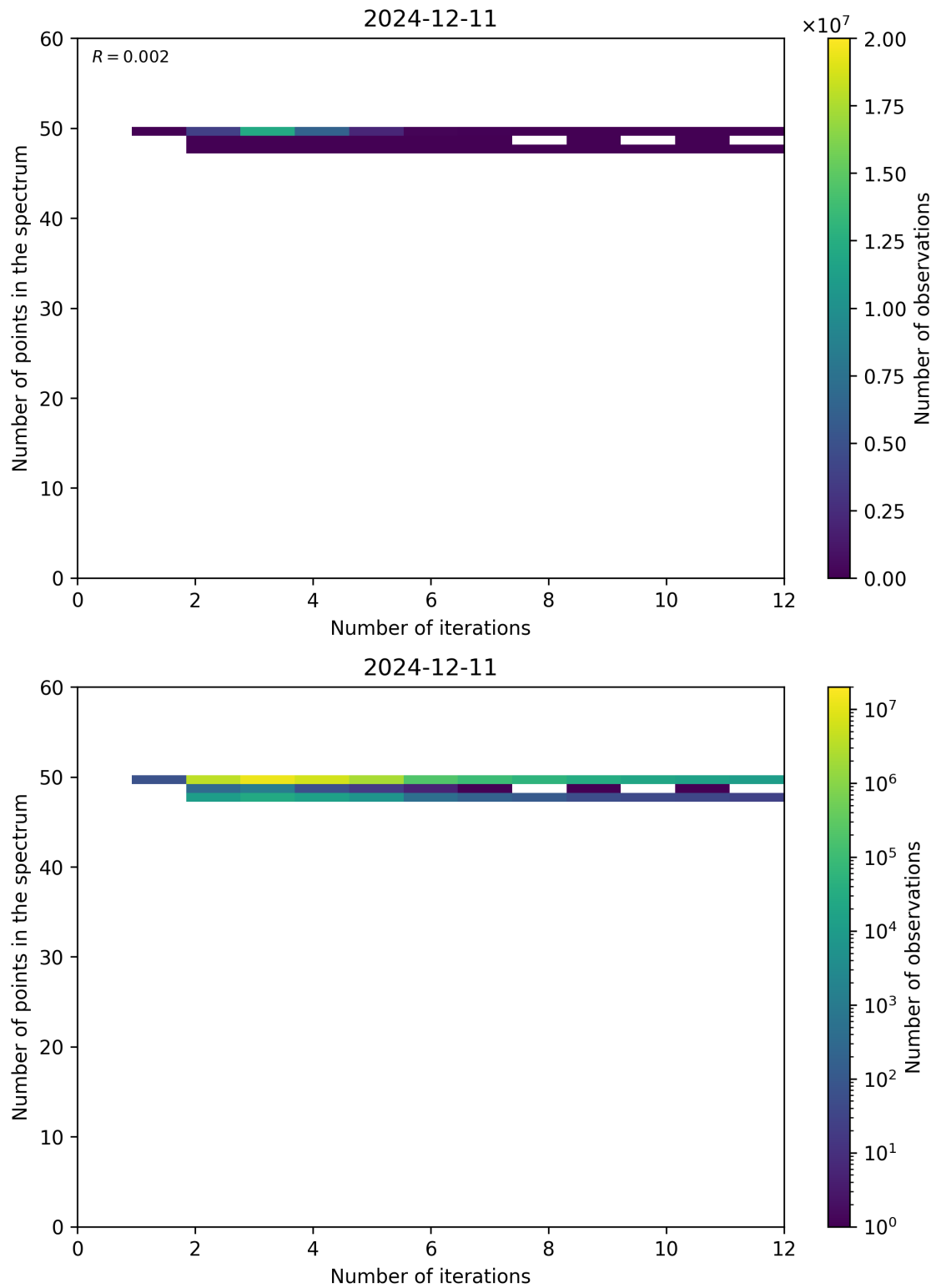
Figure 99: Scatter density plot of “Number of iterations” against “Number of points in the spectrum” for 2024-12-11 to 2024-12-12.
