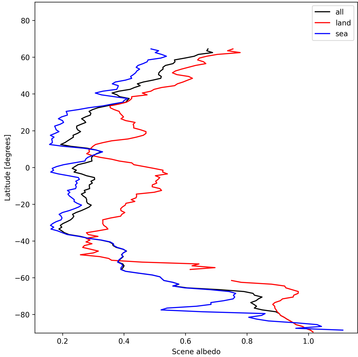
Figure 17: Zonal average of “Scene albedo” for 2024-12-12 to 2024-12-14.
