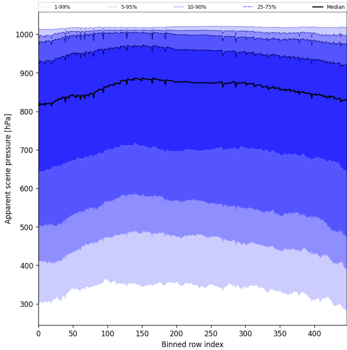
Figure 53: Along track statistics of “Apparent scene pressure” for 2024-12-12 to 2024-12-14
