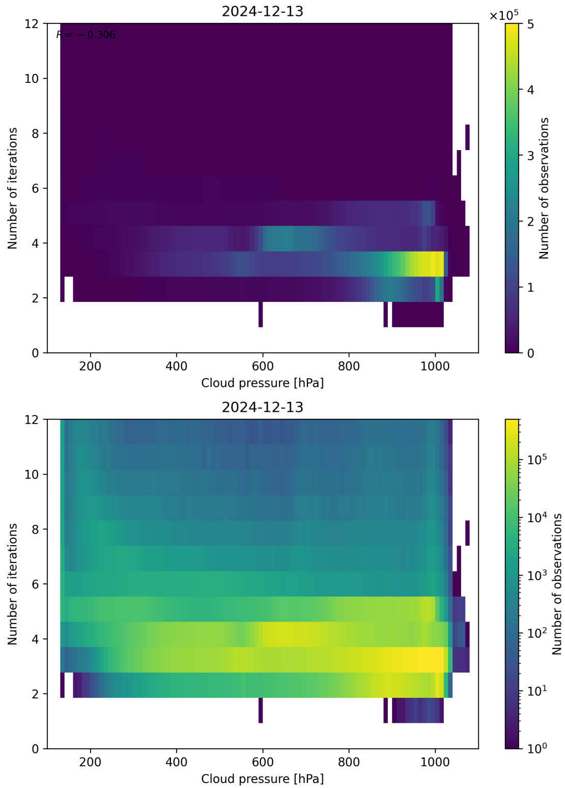
Figure 81: Scatter density plot of “Cloud pressure” against “Number of iterations” for 2024-12-12 to 2024-12-14.
