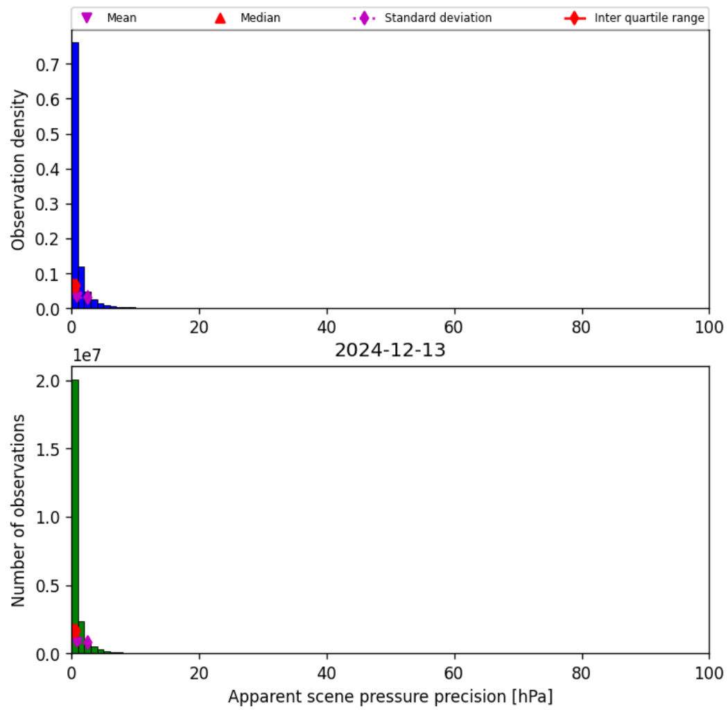
Figure 37: Histogram of “Apparent scene pressure precision” for 2024-12-12 to 2024-12-14
