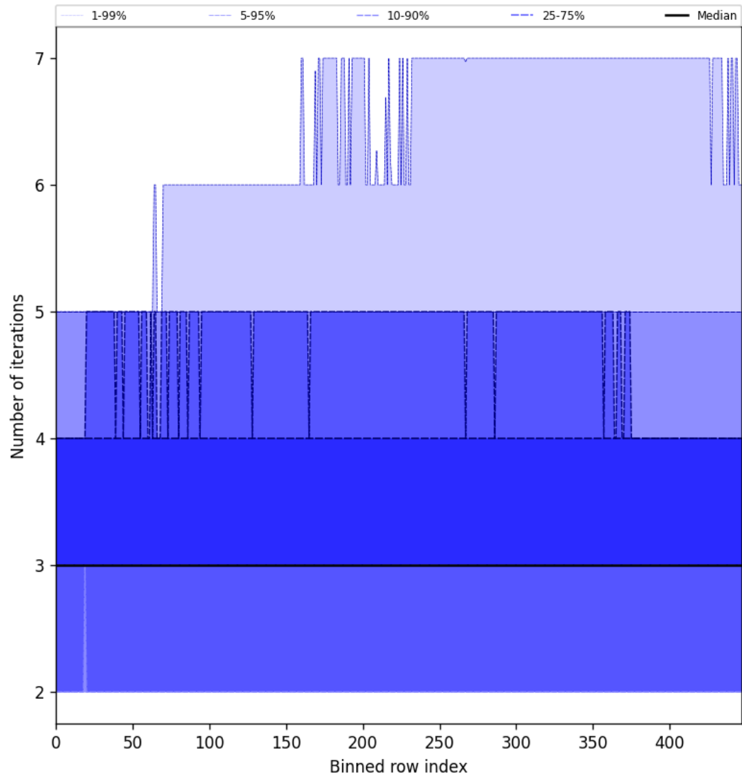
Figure 56: Along track statistics of “Number of iterations” for 2024-12-12 to 2024-12-14
