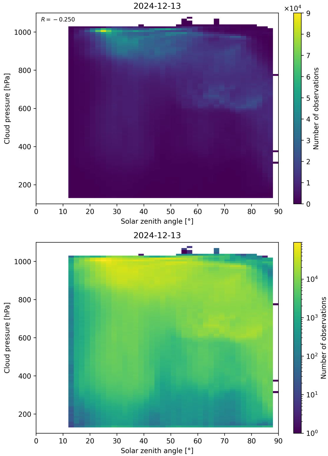
Figure 111: Scatter density plot of “Solar zenith angle” against “Cloud pressure” for 2024-12-12 to 2024-12-14.
