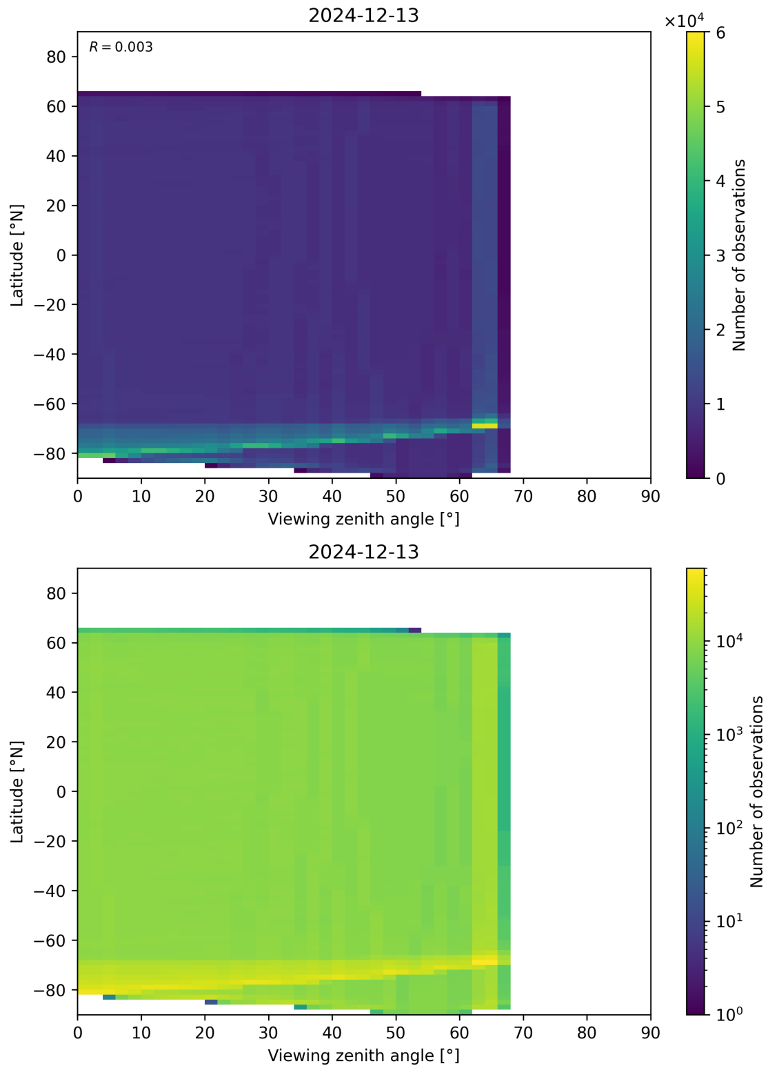
Figure 123: Scatter density plot of “Viewing zenith angle” against “Latitude” for 2024-12-12 to 2024-12-14.
