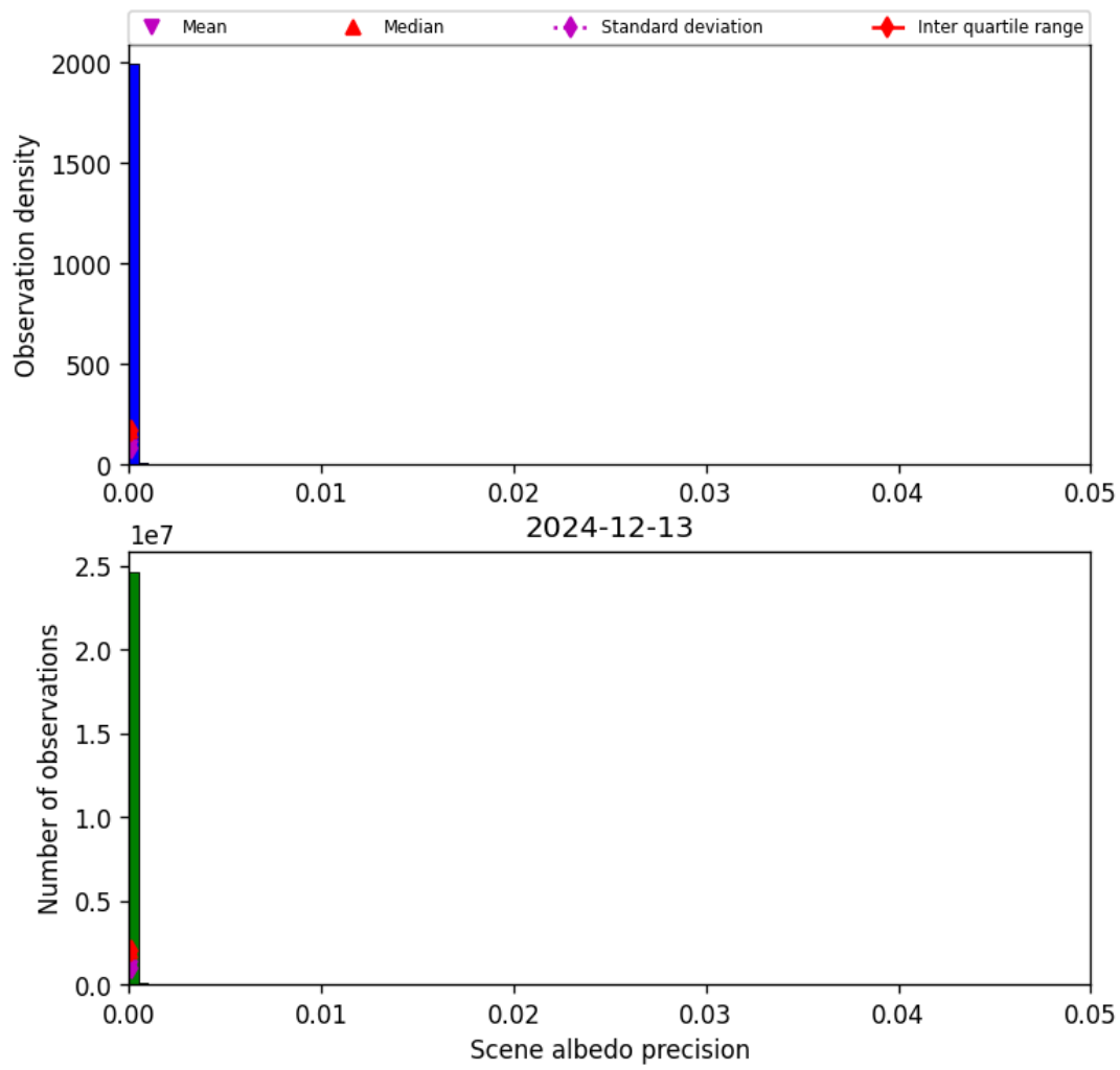
Figure 35: Histogram of “Scene albedo precision” for 2024-12-12 to 2024-12-14
