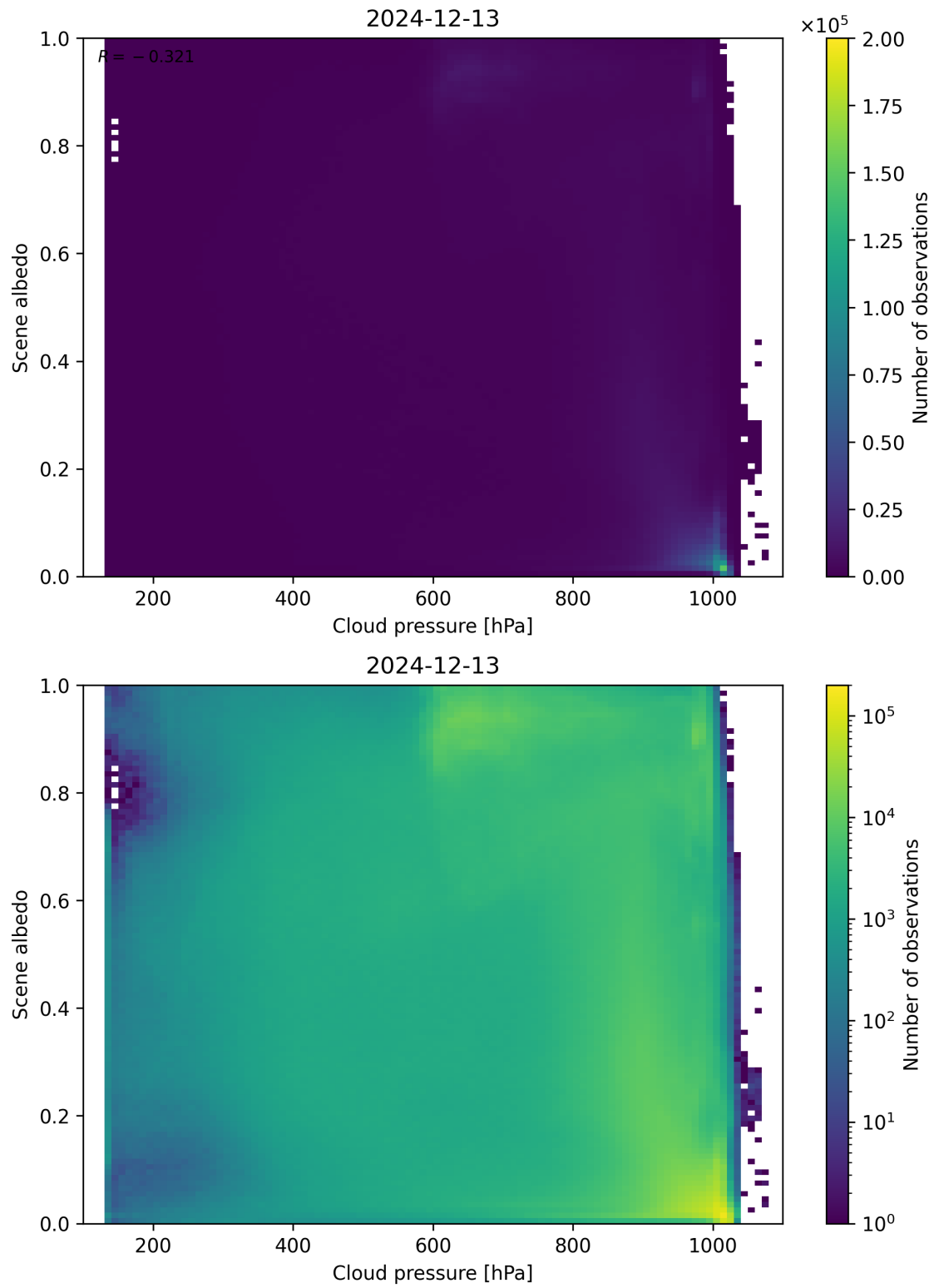
Figure 83: Scatter density plot of “Cloud pressure” against “Scene albedo” for 2024-12-12 to 2024-12-14.
