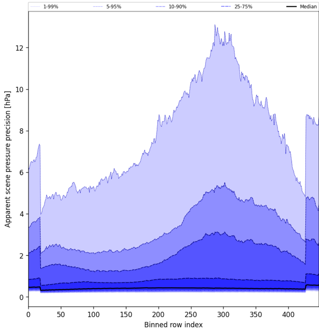
Figure 54: Along track statistics of “Apparent scene pressure precision” for 2024-12-12 to 2024-12-14
