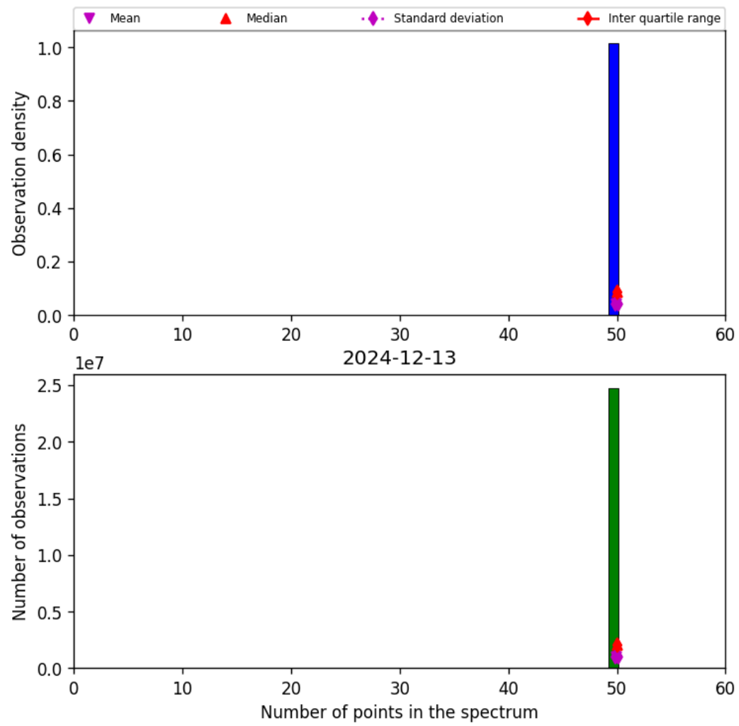
Figure 44: Histogram of “Number of points in the spectrum” for 2024-12-12 to 2024-12-14
