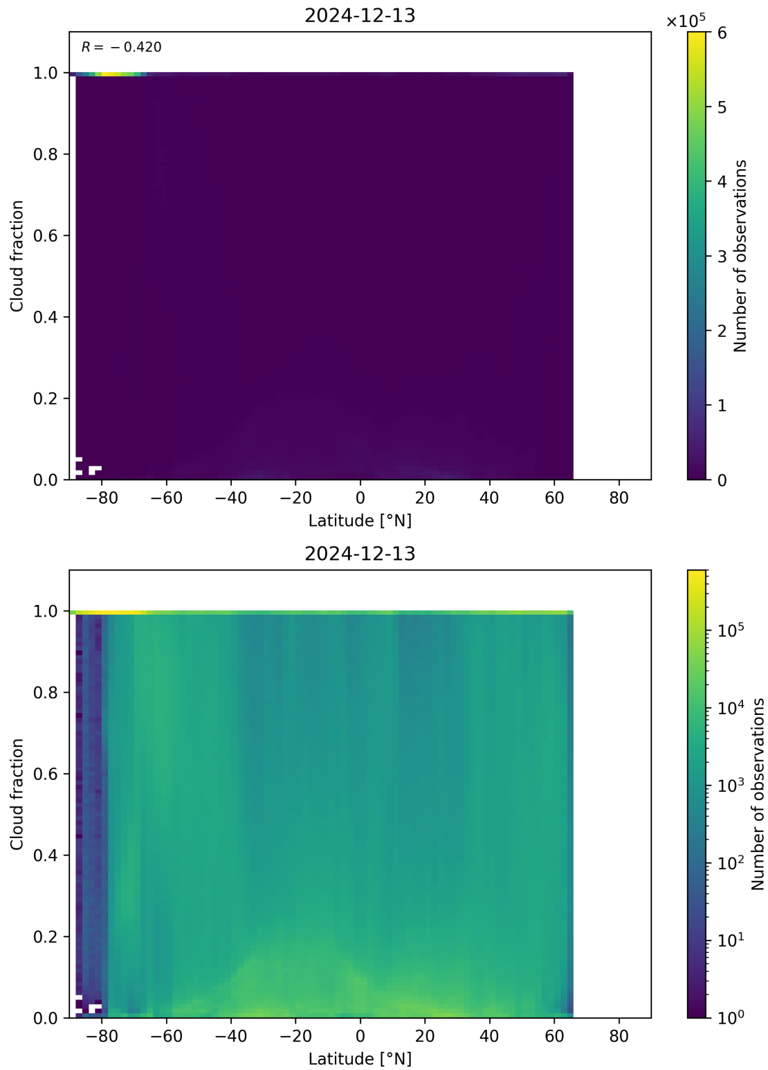
Figure 90: Scatter density plot of “Latitude” against “Cloud fraction” for 2024-12-12 to 2024-12-14.
