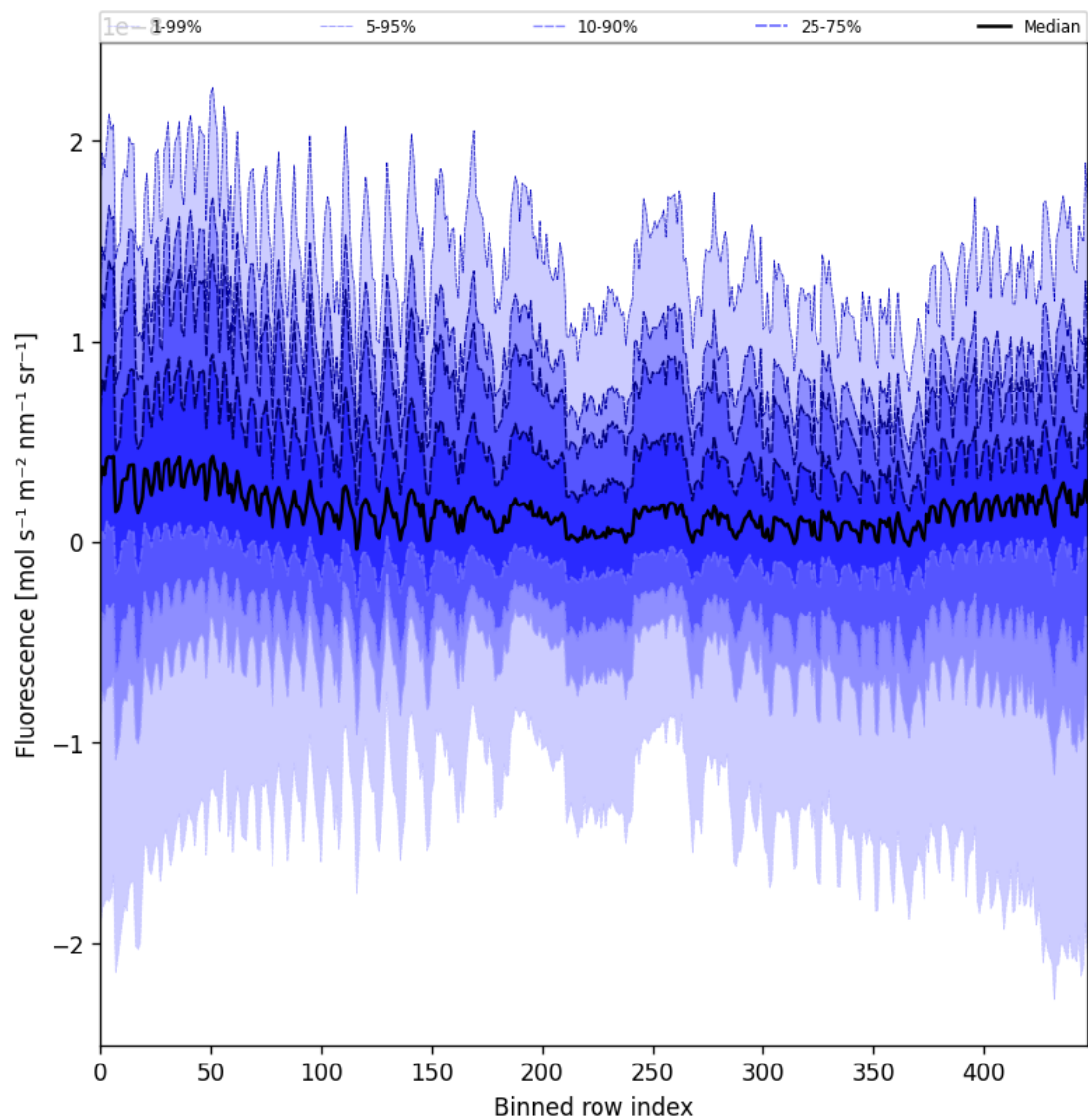
Figure 57: Along track statistics of “Fluorescence” for 2024-12-12 to 2024-12-14
