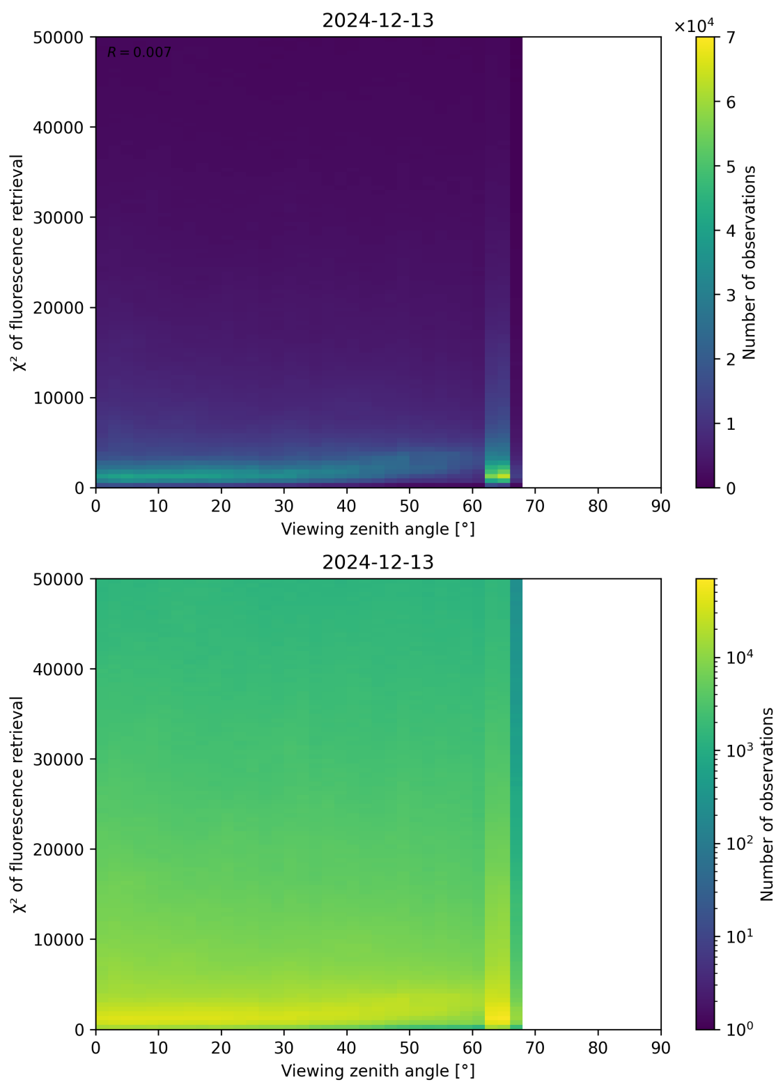
Figure 119: Scatter density plot of “Viewing zenith angle” against “ \chi^2 of fluorescence retrieval” for 2024-12-12 to 2024-12-14.
