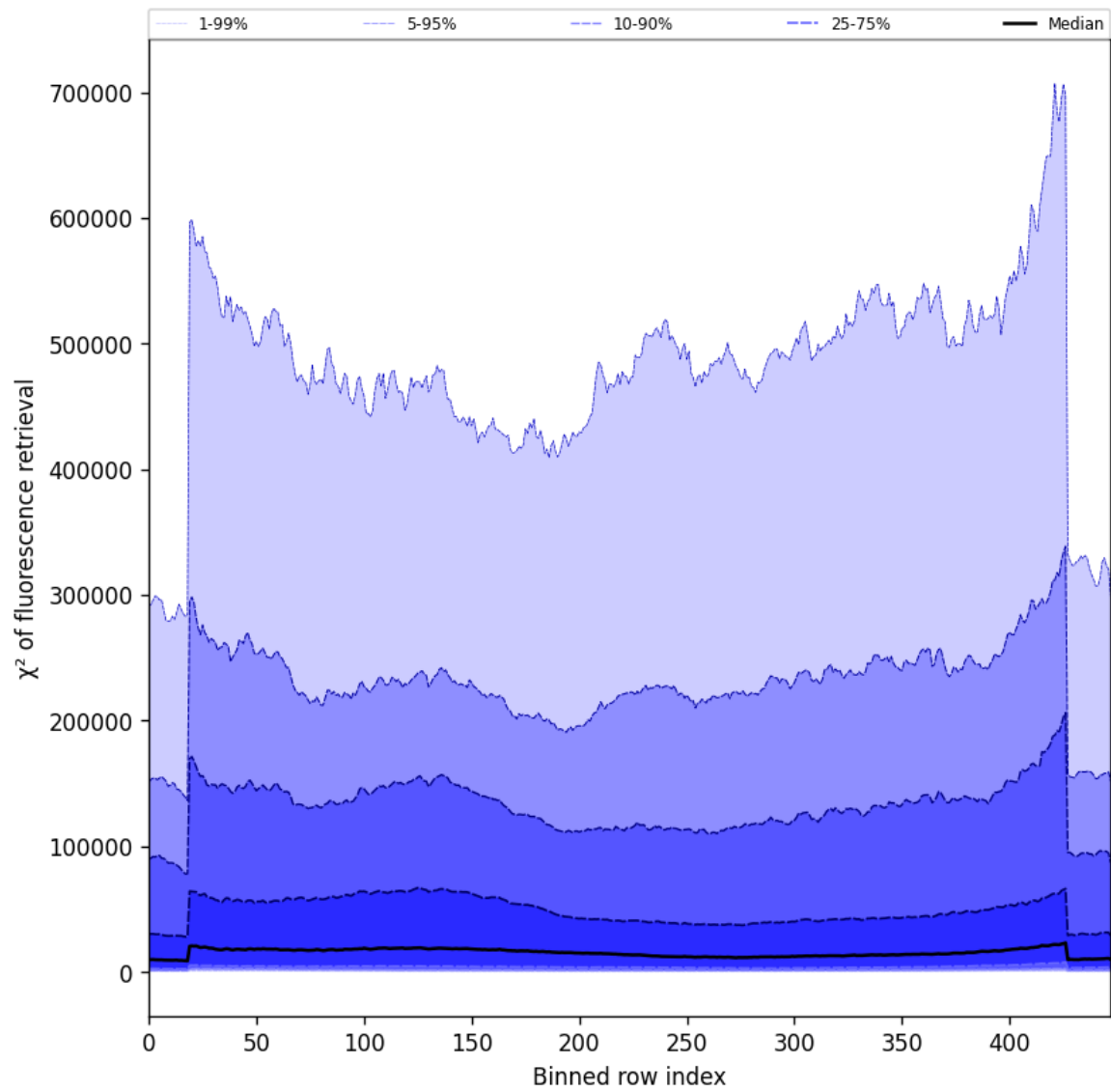
Figure 59: Along track statistics of “ \chi^2 of fluorescence retrieval” for 2024-12-12 to 2024-12-14
