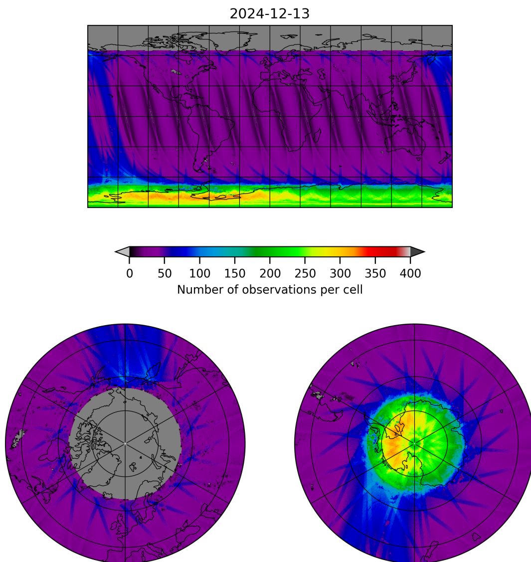
Figure 11: Map of the number of observations for 2024-12-12 to 2024-12-14
