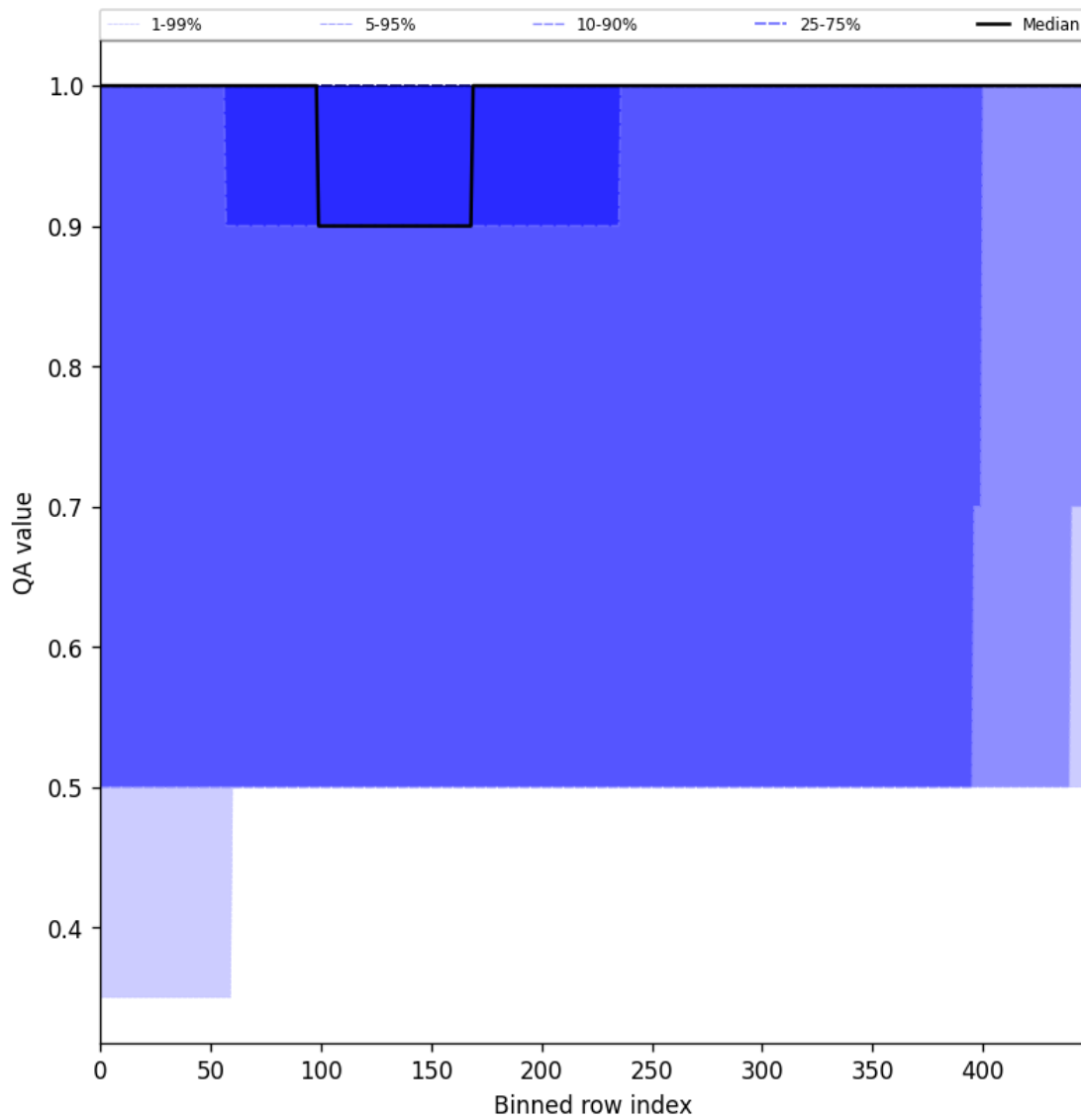
Figure 46: Along track statistics of “QA value” for 2024-12-12 to 2024-12-14
