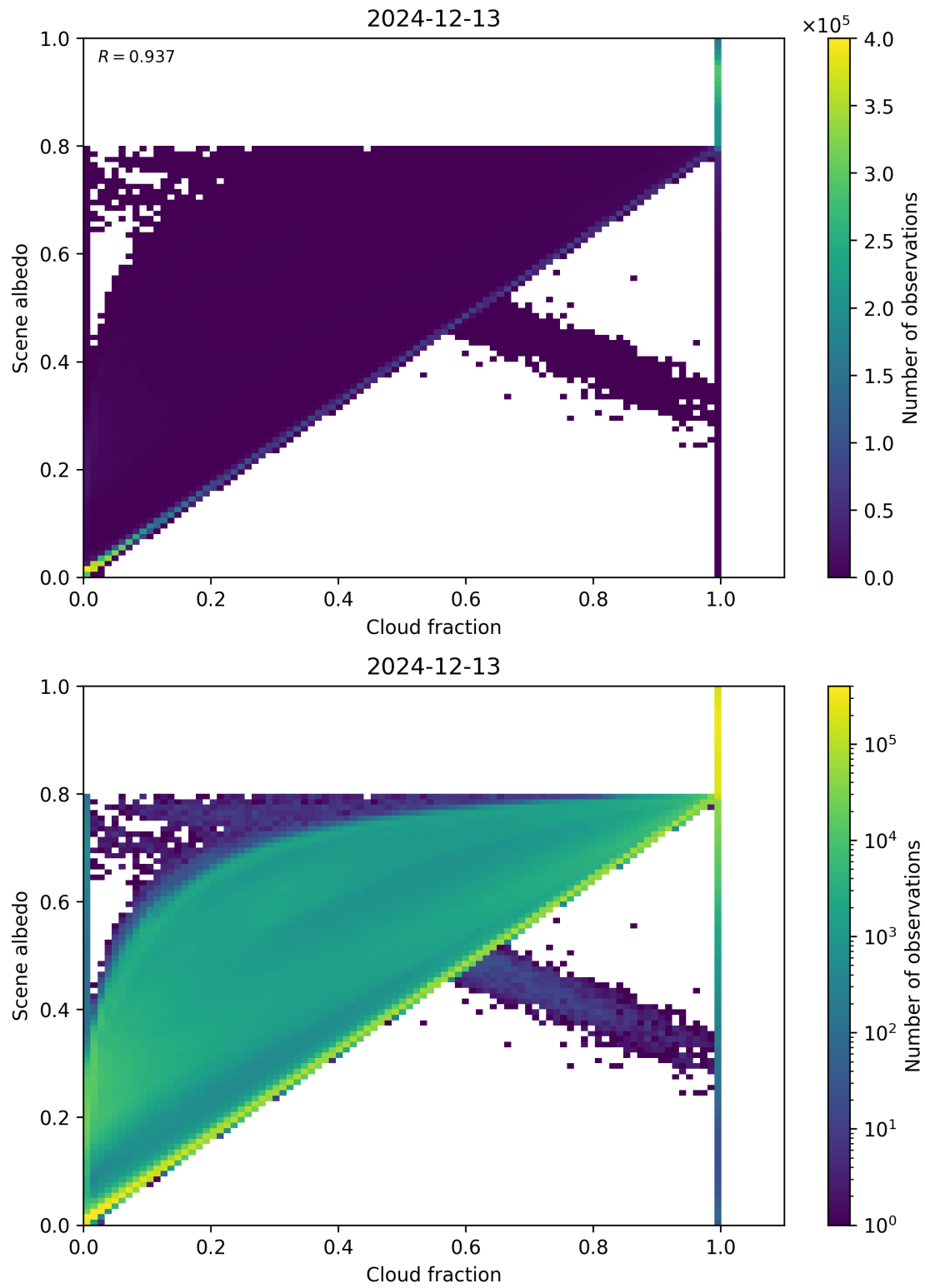
Figure 75: Scatter density plot of “Cloud fraction” against “Scene albedo” for 2024-12-12 to 2024-12-14.
