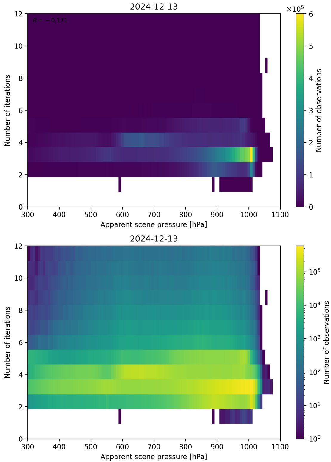
Figure 65: Scatter density plot of “Apparent scene pressure” against “Number of iterations” for 2024-12-12 to 2024-12-14.
