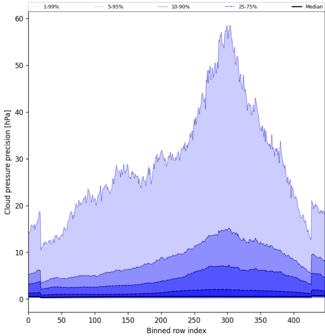
Figure 48: Along track statistics of “Cloud pressure precision” for 2024-12-12 to 2024-12-14
