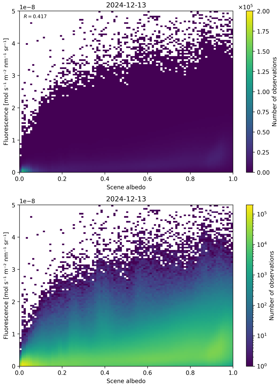
Figure 104: Scatter density plot of “Scene albedo” against “Fluorescence” for 2024-12-12 to 2024-12-14.
