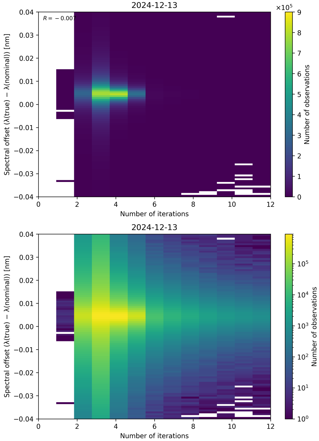
Figure 100: Scatter density plot of “Number of iterations” against “Spectral offset ( \lambda_{\text{true}} - \lambda_{\text{nominal}} )” for 2024-12-12 to 2024-12-14.
