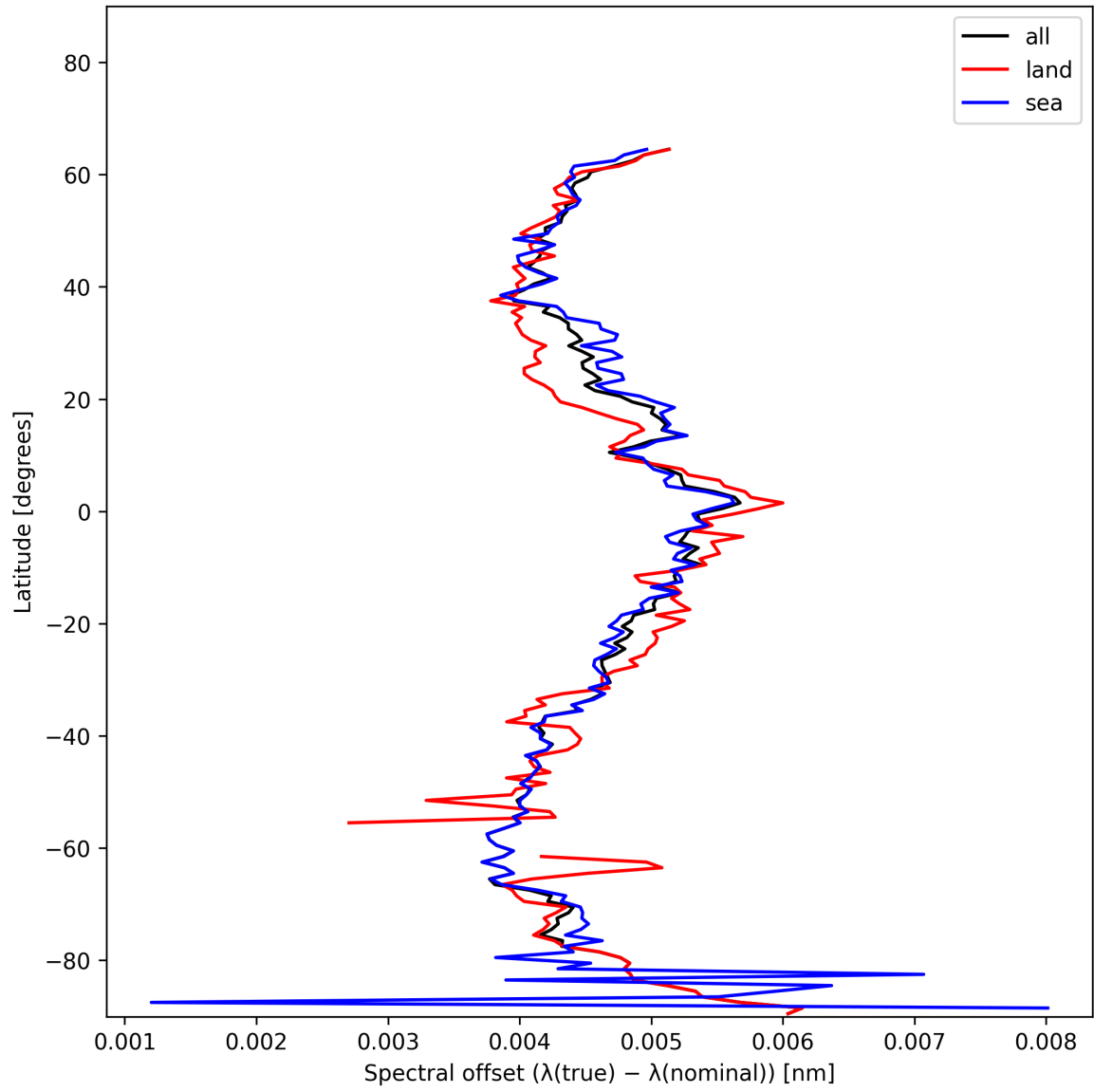
Figure 28: Zonal average of “Spectral offset ( \lambda_{\text{true}} - \lambda_{\text{nominal}} )” for 2024-12-12 to 2024-12-14.
