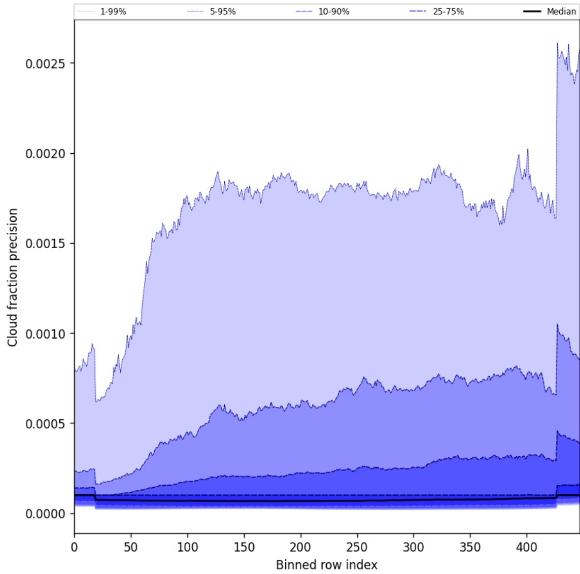
Figure 50: Along track statistics of “Cloud fraction precision” for 2024-12-12 to 2024-12-14
