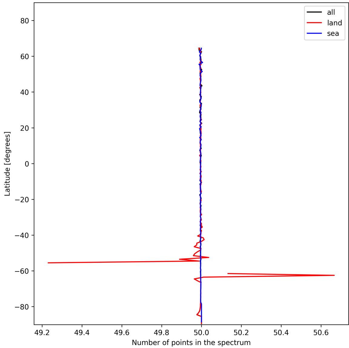
Figure 27: Zonal average of “Number of points in the spectrum” for 2024-12-12 to 2024-12-14.
