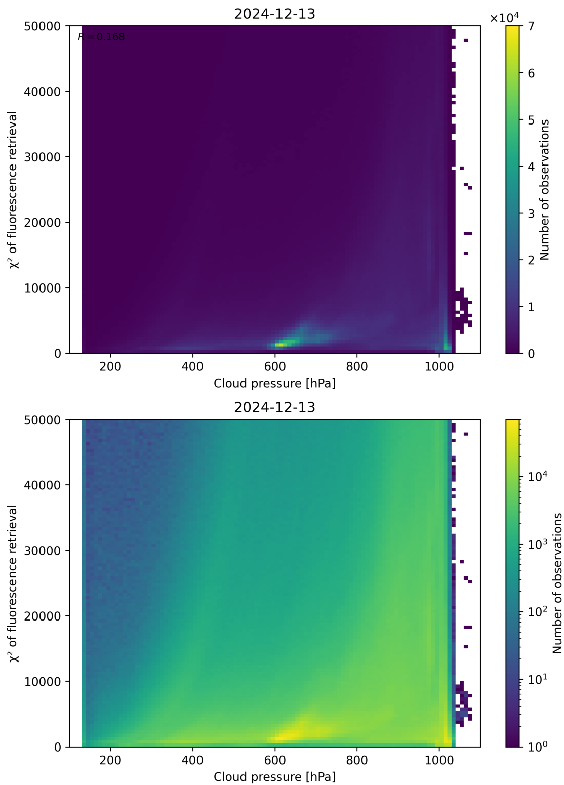
Figure 78: Scatter density plot of “Cloud pressure” against “ \chi^2 of fluorescence retrieval” for 2024-12-12 to 2024-12-14.
