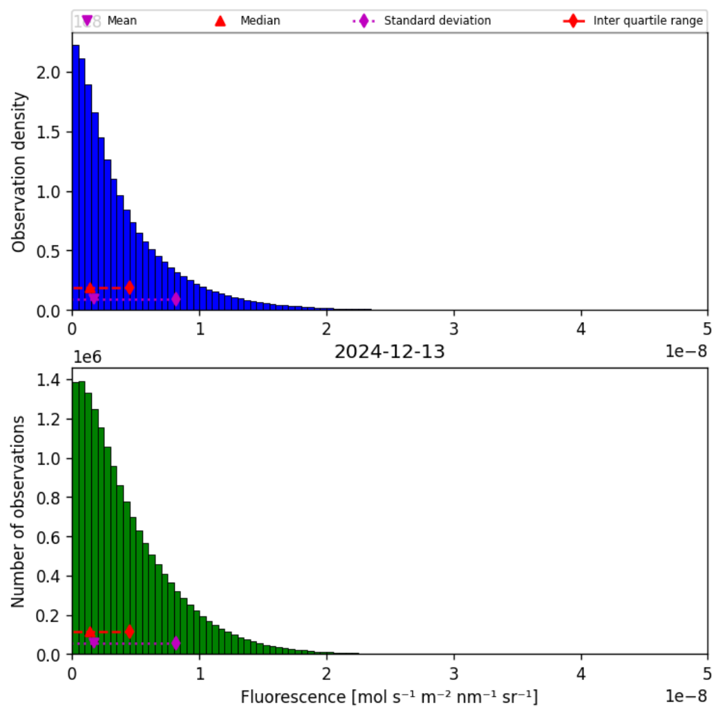
Figure 40: Histogram of “Fluorescence” for 2024-12-12 to 2024-12-14
