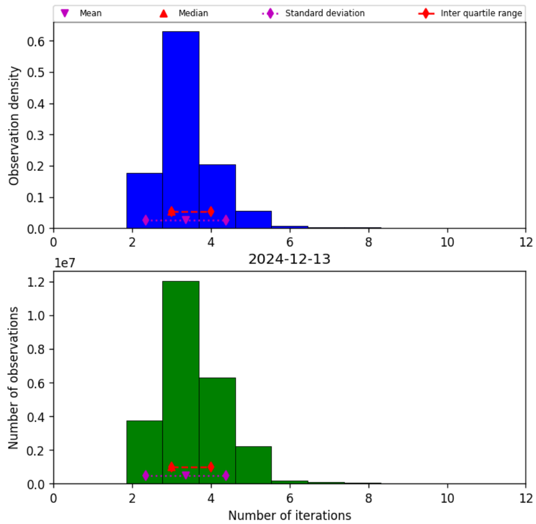
Figure 39: Histogram of “Number of iterations” for 2024-12-12 to 2024-12-14
