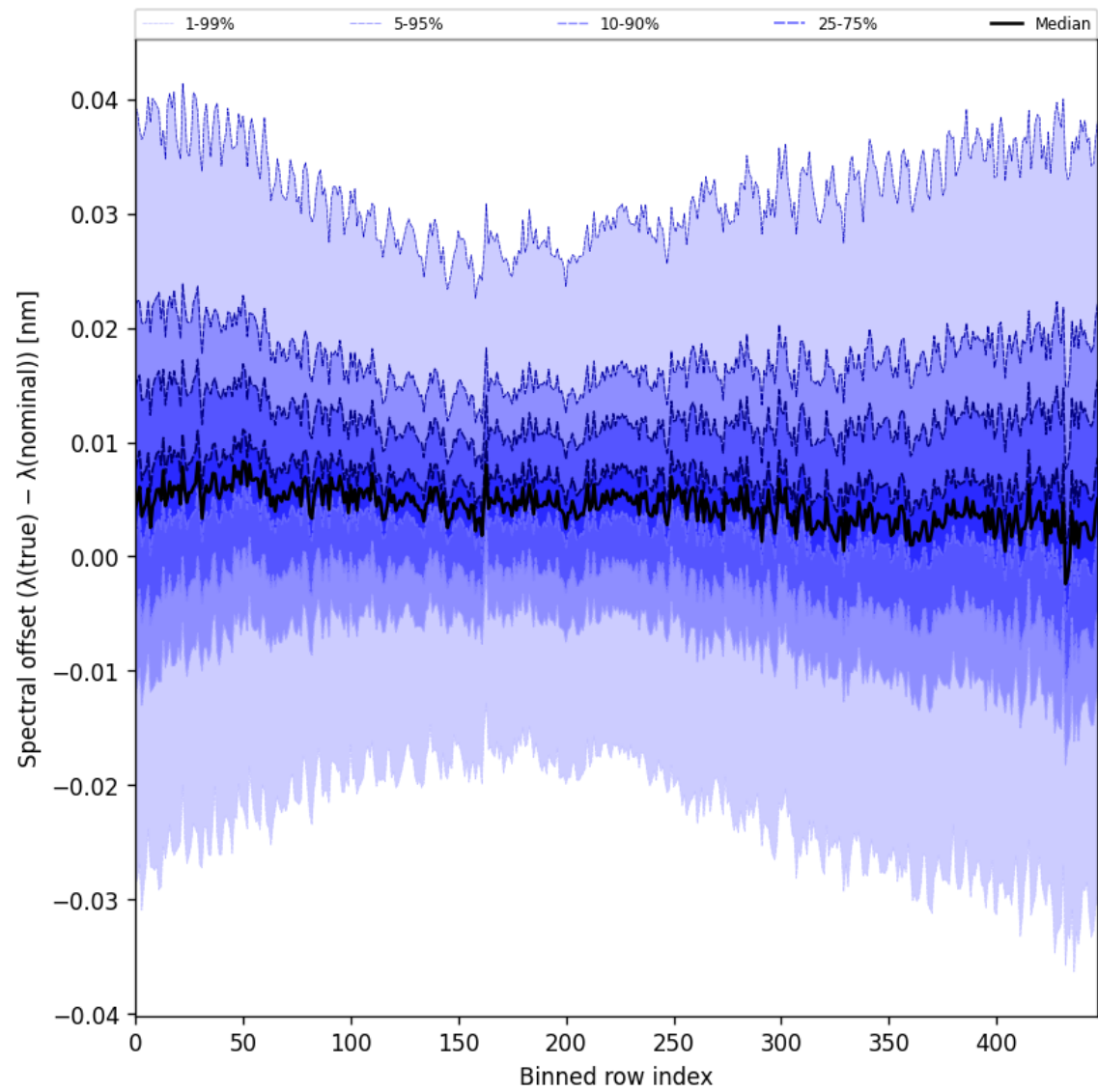
Figure 62: Along track statistics of “Spectral offset ( \lambda_{\text{true}} - \lambda_{\text{nominal}} )” for 2024-12-12 to 2024-12-14
