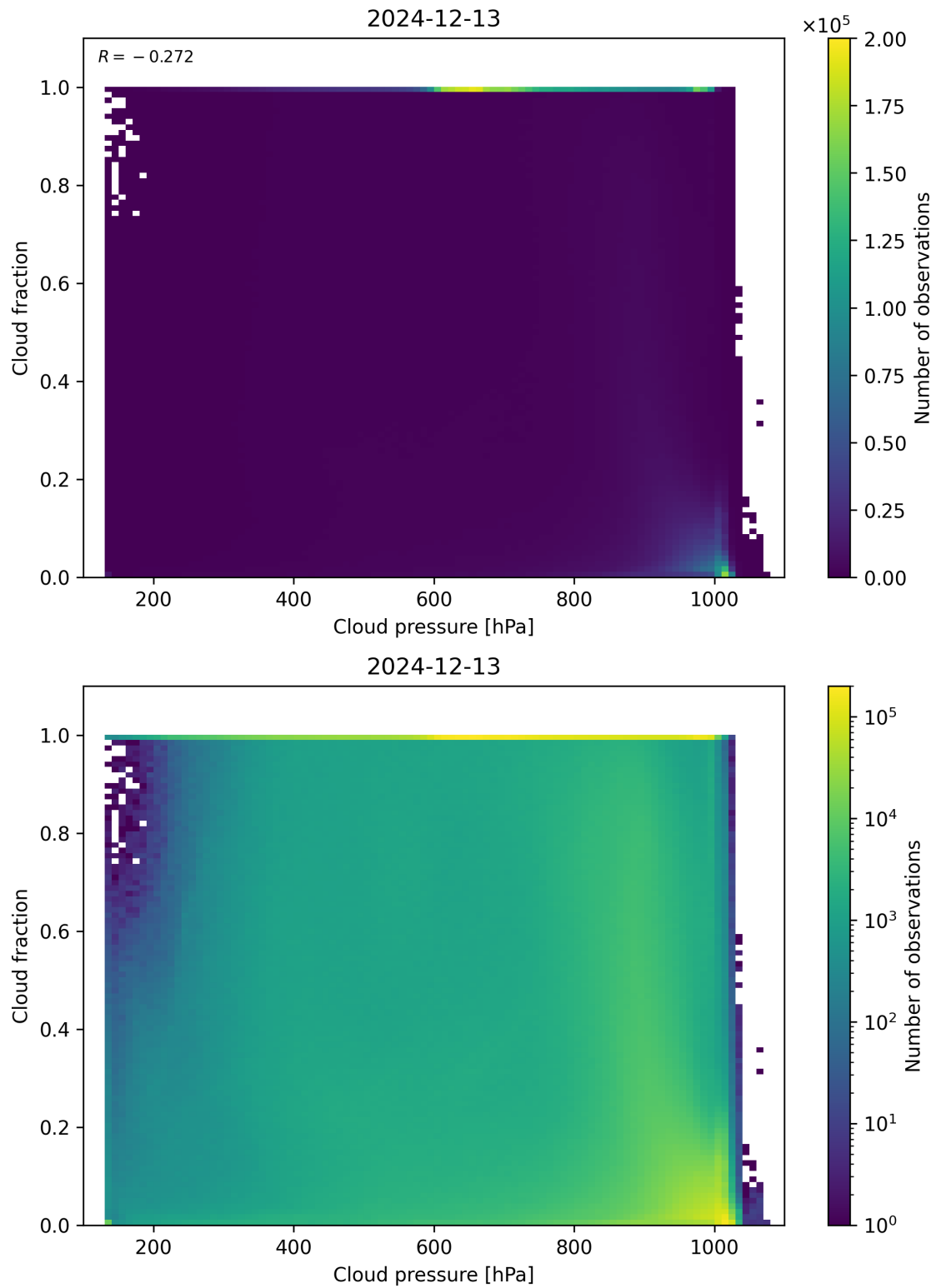
Figure 79: Scatter density plot of “Cloud pressure” against “Cloud fraction” for 2024-12-12 to 2024-12-14.
