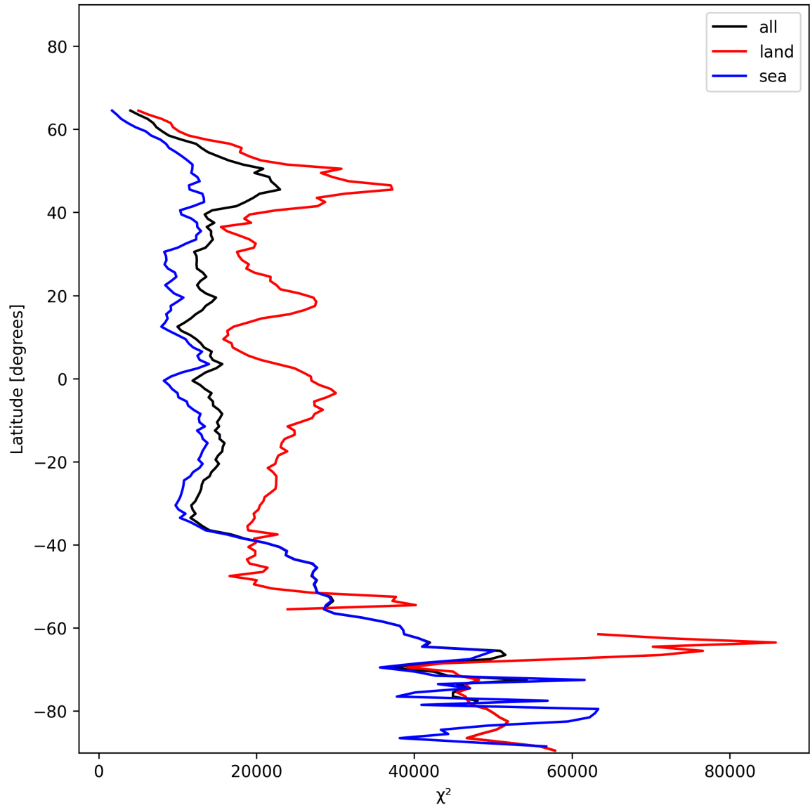
Figure 21: Zonal average of “ \chi^2 ” for 2024-12-12 to 2024-12-14.
