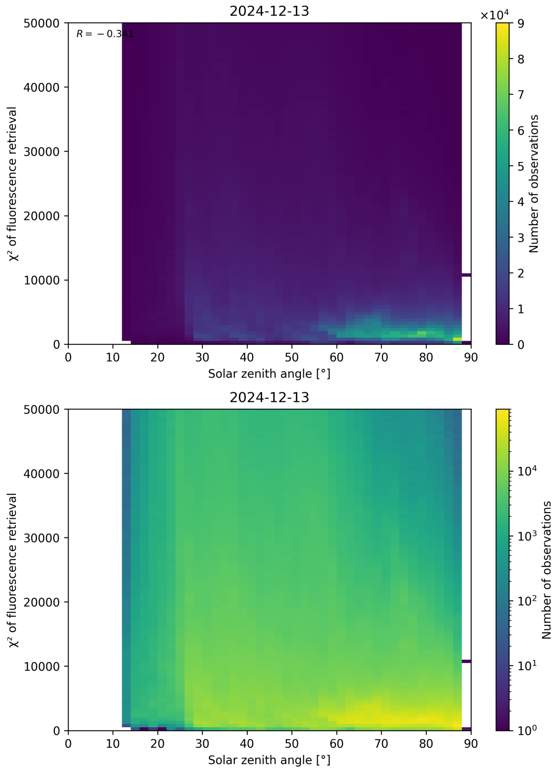
Figure 109: Scatter density plot of “Solar zenith angle” against “ \chi^2 of fluorescence retrieval” for 2024-12-12 to 2024-12-14.
