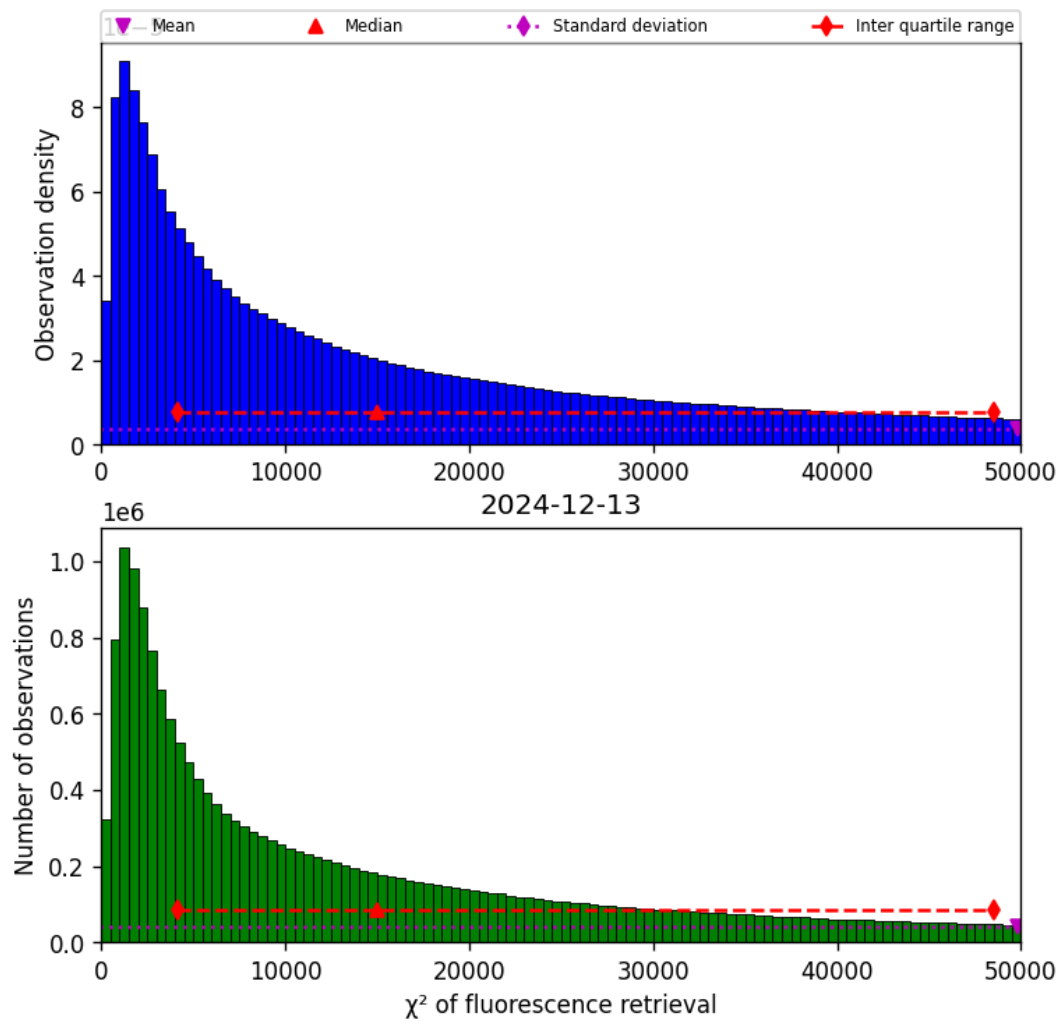
Figure 42: Histogram of “ \chi^2 of fluorescence retrieval” for 2024-12-12 to 2024-12-14
