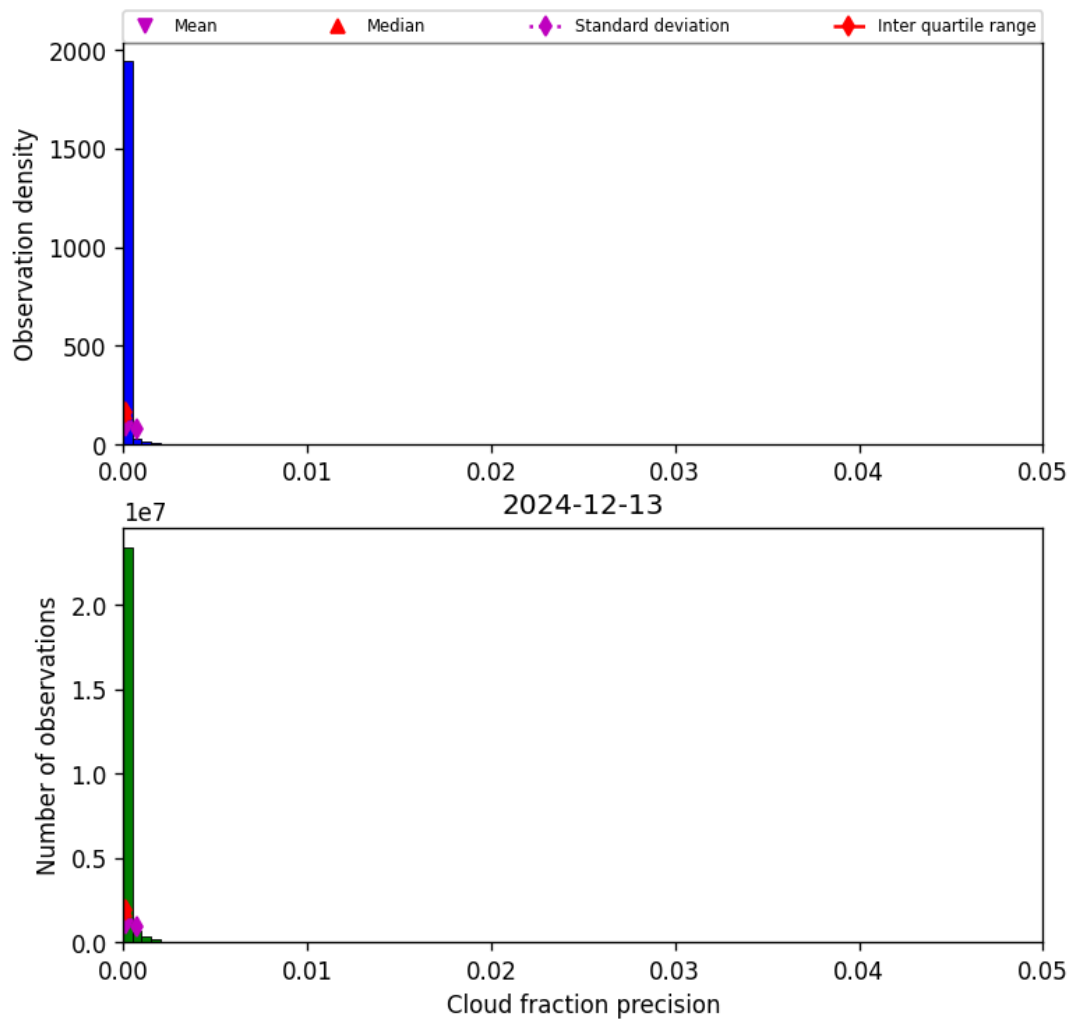
Figure 33: Histogram of “Cloud fraction precision” for 2024-12-12 to 2024-12-14
