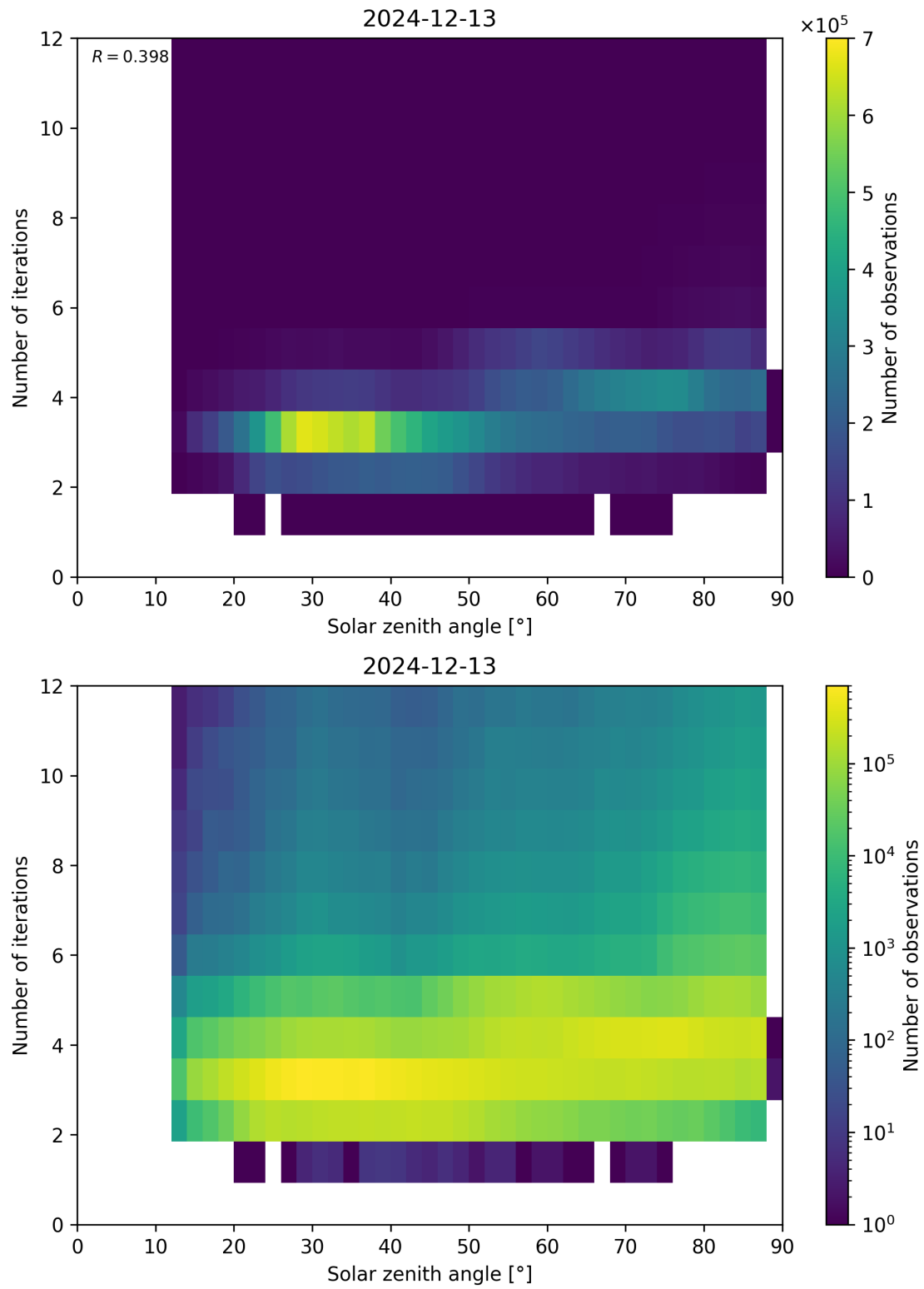
Figure 114: Scatter density plot of “Solar zenith angle” against “Number of iterations” for 2024-12-12 to 2024-12-14.
