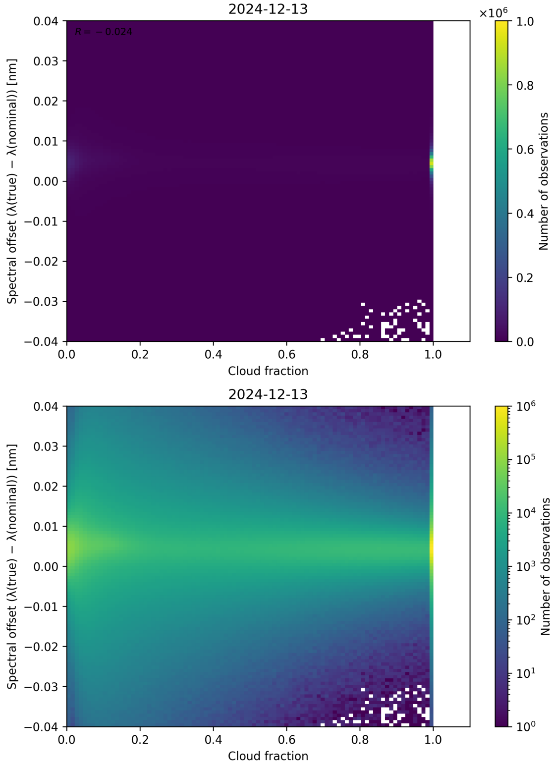
Figure 76: Scatter density plot of “Cloud fraction” against “Spectral offset ( \lambda_{\text{true}} - \lambda_{\text{nominal}} )” for 2024-12-12 to 2024-12-14.
