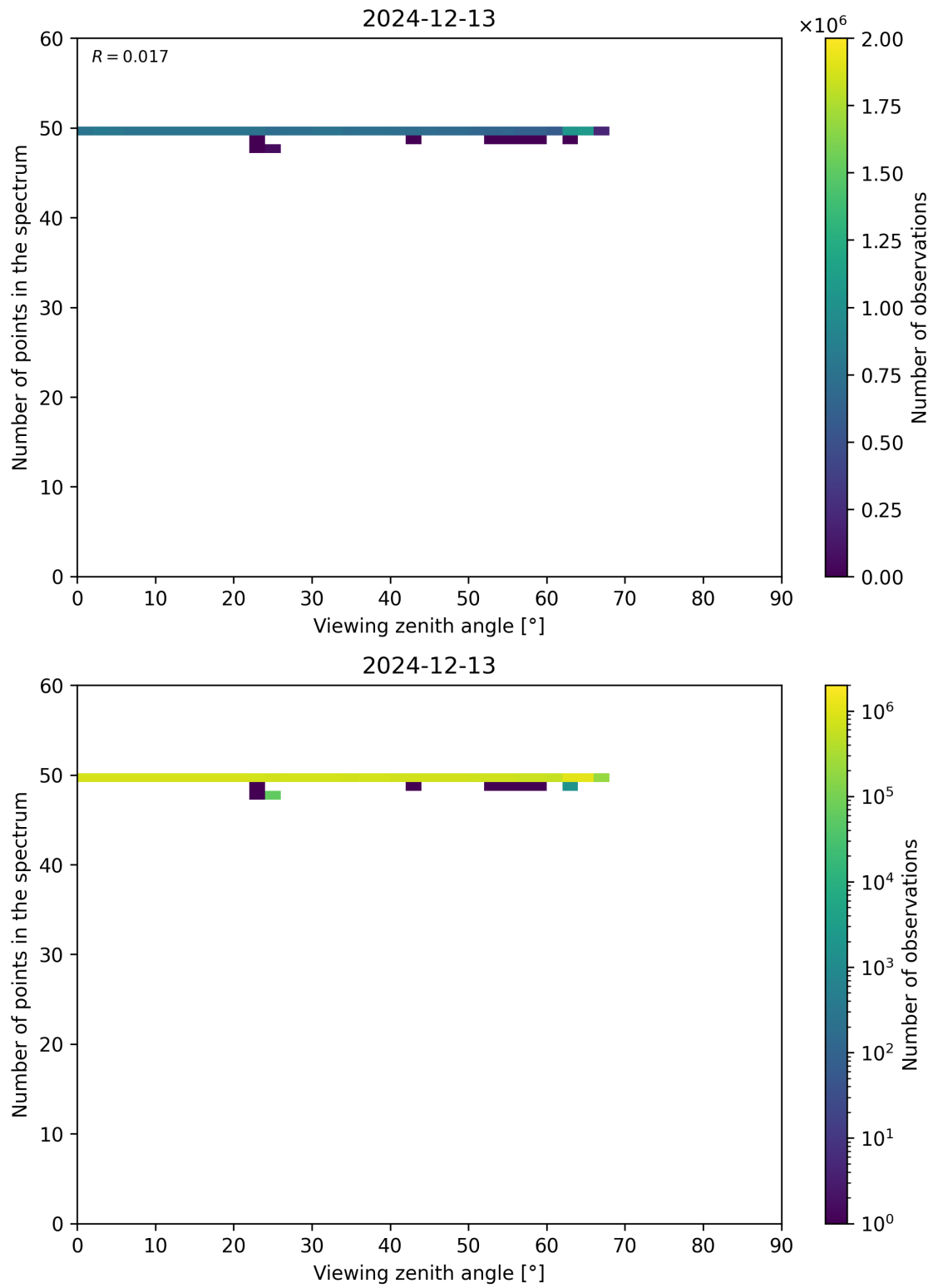
Figure 125: Scatter density plot of “Viewing zenith angle” against “Number of points in the spectrum” for 2024-12-12 to 2024-12-14.
