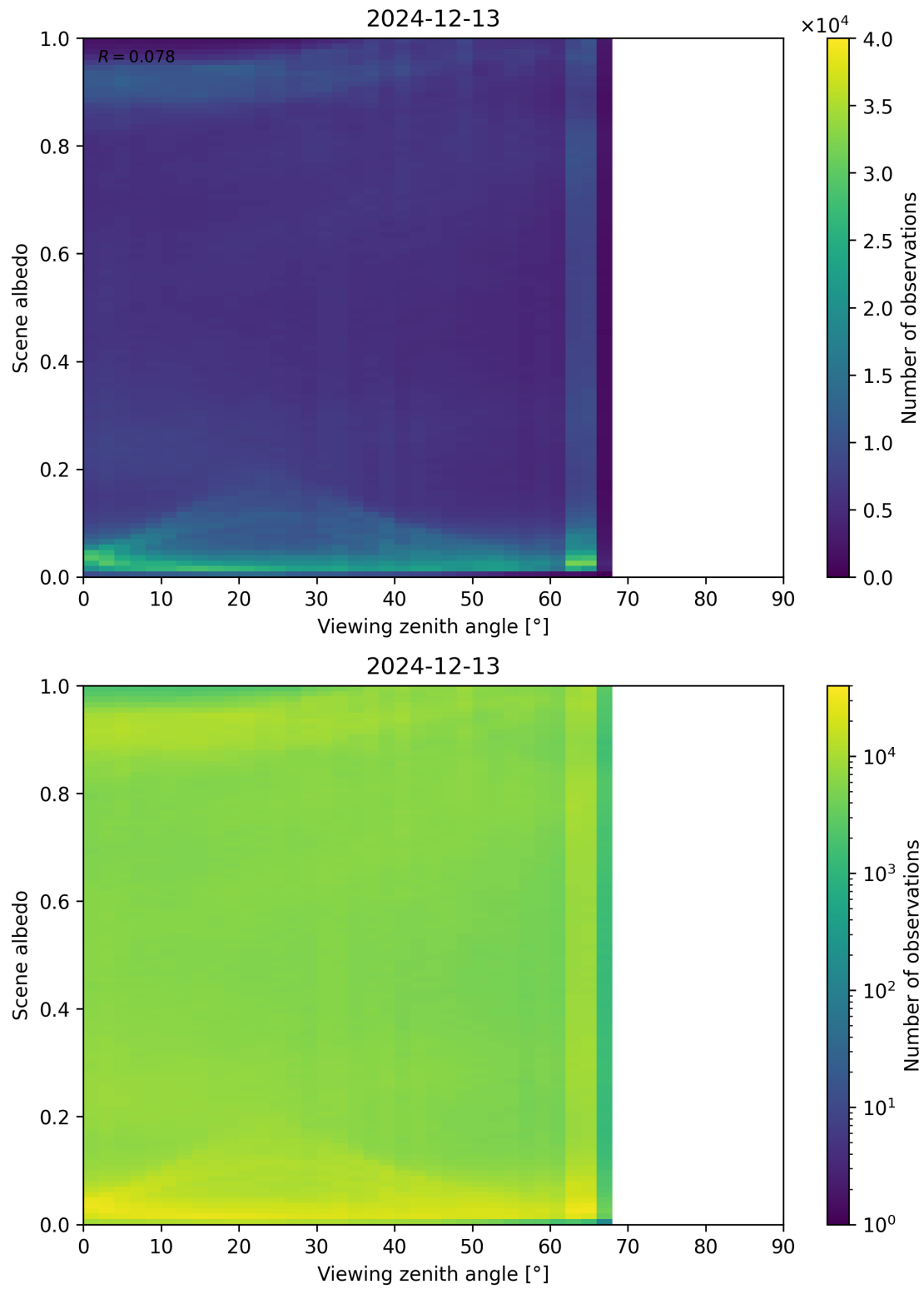
Figure 126: Scatter density plot of “Viewing zenith angle” against “Scene albedo” for 2024-12-12 to 2024-12-14.
