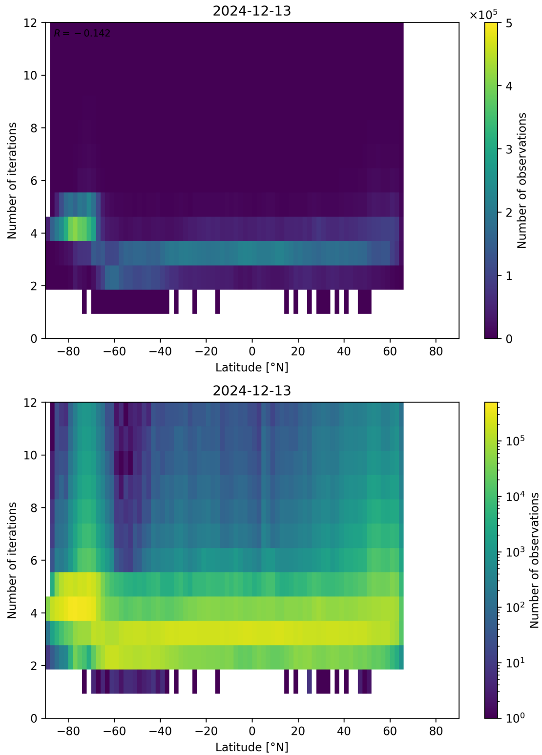
Figure 93: Scatter density plot of “Latitude” against “Number of iterations” for 2024-12-12 to 2024-12-14.
