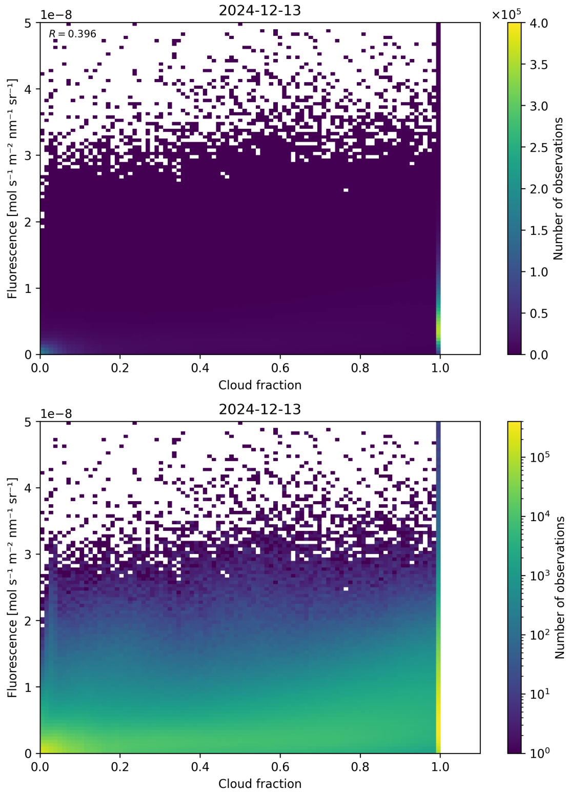
Figure 72: Scatter density plot of “Cloud fraction” against “Fluorescence” for 2024-12-12 to 2024-12-14.
