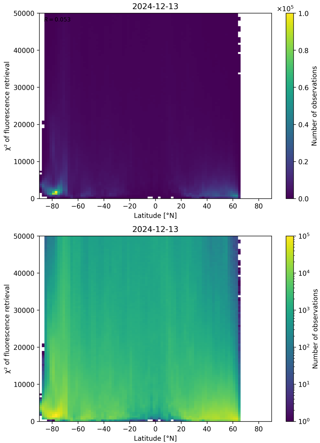
Figure 89: Scatter density plot of “Latitude” against “ \chi^2 of fluorescence retrieval” for 2024-12-12 to 2024-12-14.
