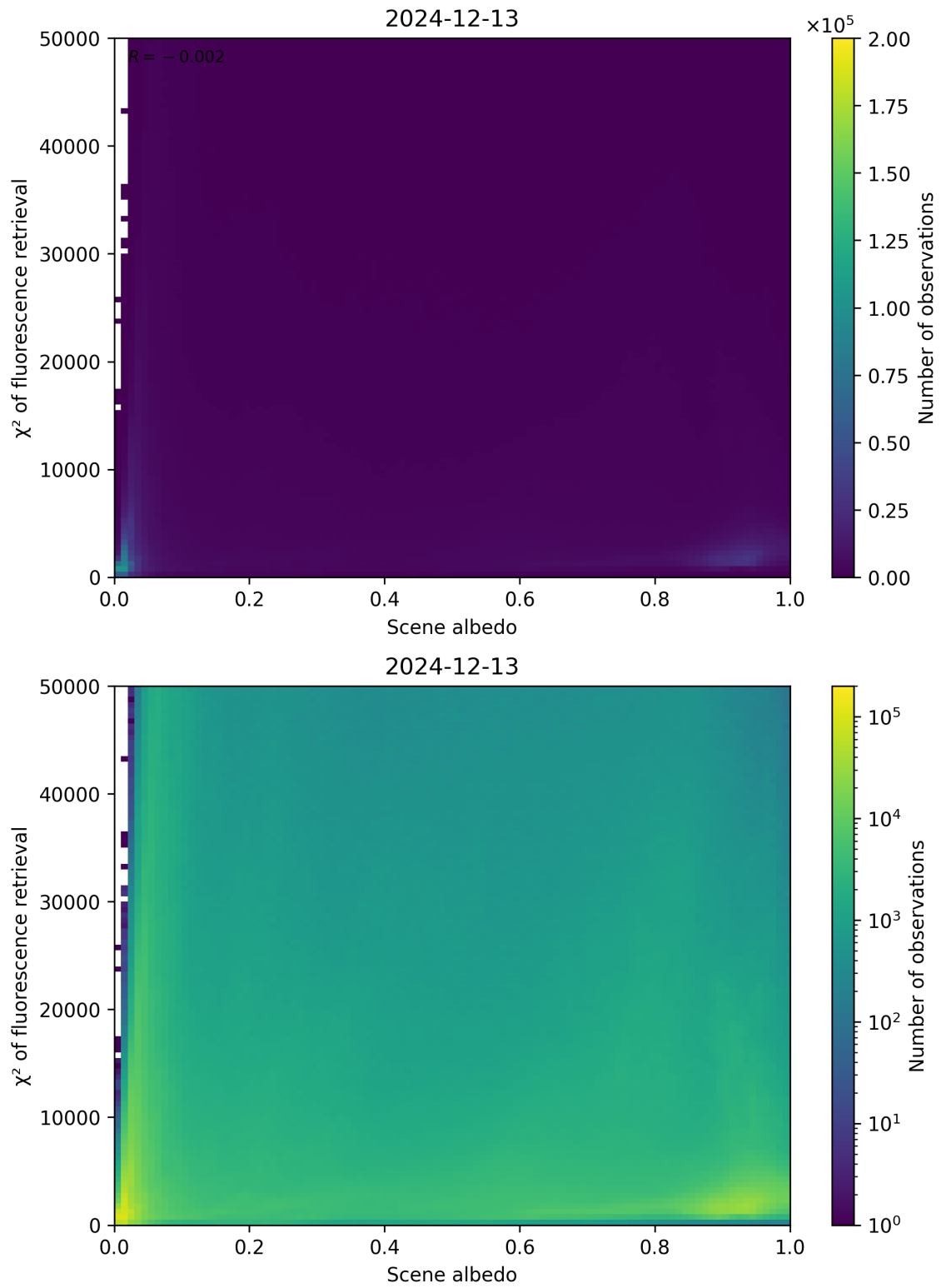
Figure 103: Scatter density plot of “Scene albedo” against “ \chi^2 of fluorescence retrieval” for 2024-12-12 to 2024-12-14.
