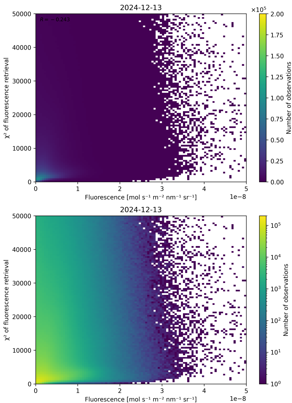
Figure 85: Scatter density plot of “Fluorescence” against “ \chi^2 of fluorescence retrieval” for 2024-12-12 to 2024-12-14.
