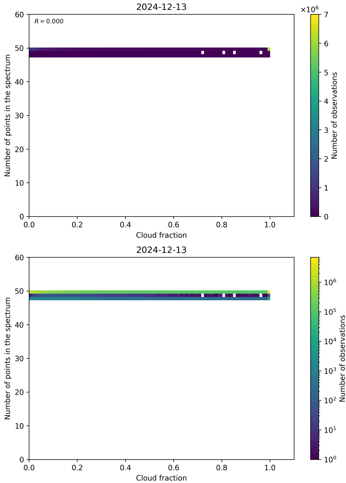
Figure 74: Scatter density plot of “Cloud fraction” against “Number of points in the spectrum” for 2024-12-12 to 2024-12-14.
