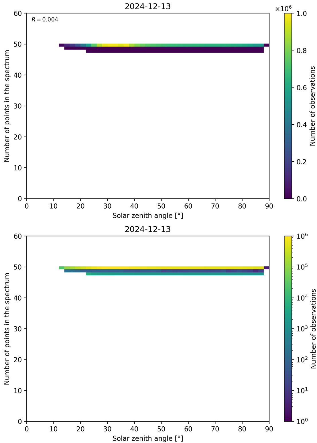
Figure 115: Scatter density plot of “Solar zenith angle” against “Number of points in the spectrum” for 2024-12-12 to 2024-12-14.
