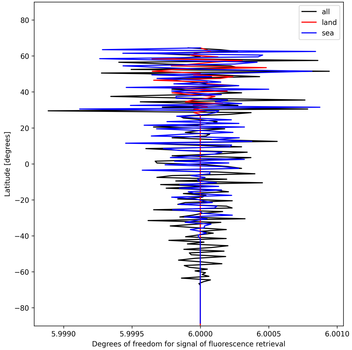
Figure 26: Zonal average of “Degrees of freedom for signal of fluorescence retrieval” for 2024-12-12 to 2024-12-14.
