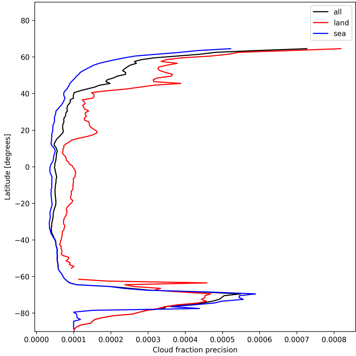
Figure 16: Zonal average of “Cloud fraction precision” for 2024-12-12 to 2024-12-14.
