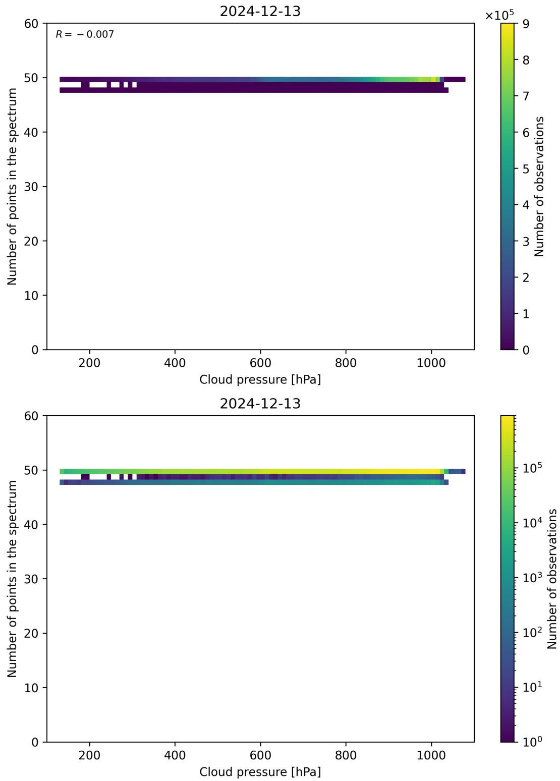
Figure 82: Scatter density plot of “Cloud pressure” against “Number of points in the spectrum” for 2024-12-12 to 2024-12-14.
