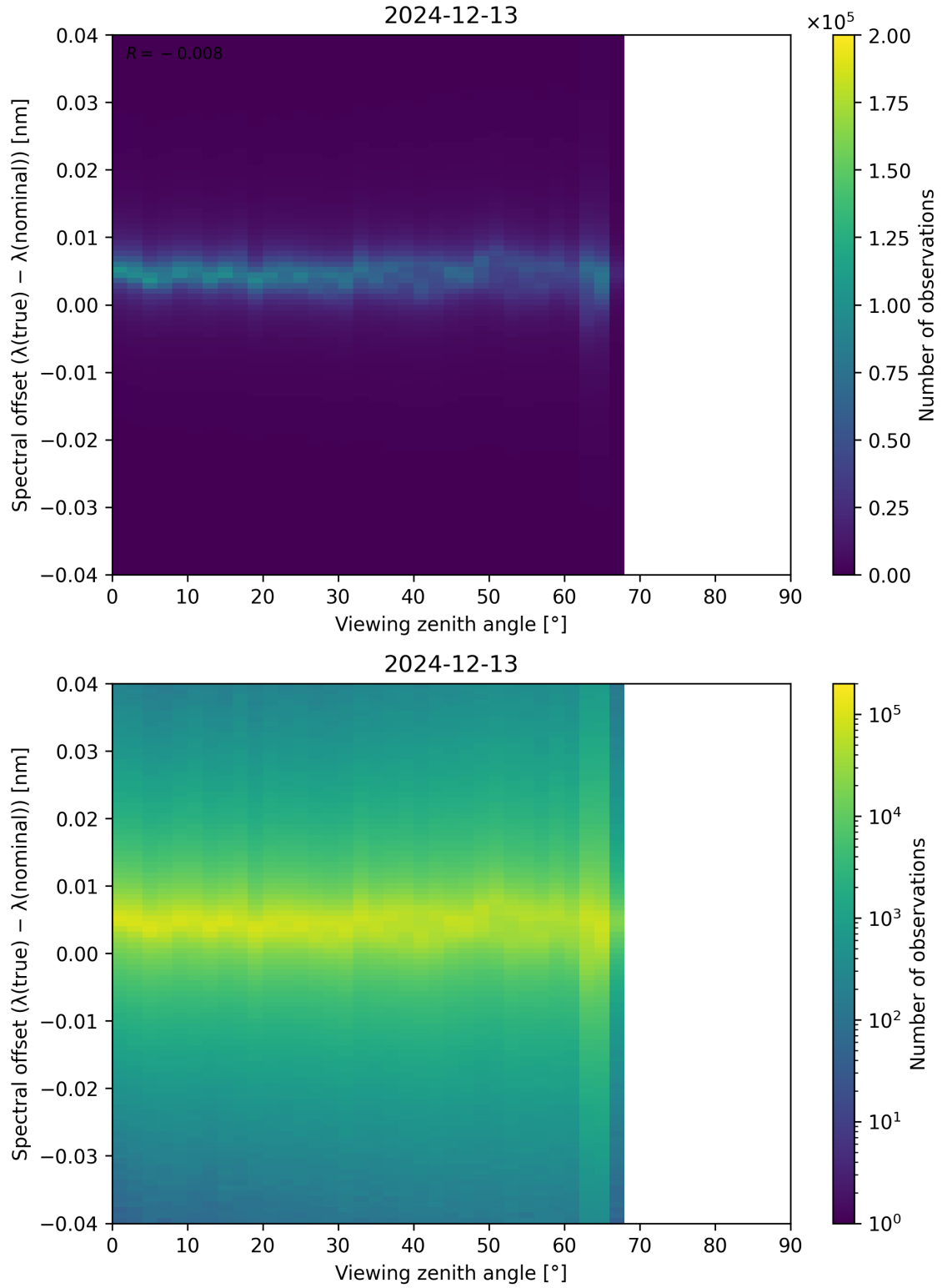
Figure 128: Scatter density plot of “Viewing zenith angle” against “Spectral offset ( \lambda_{\text{true}} - \lambda_{\text{nominal}} )” for 2024-12-12 to 2024-12-14.
