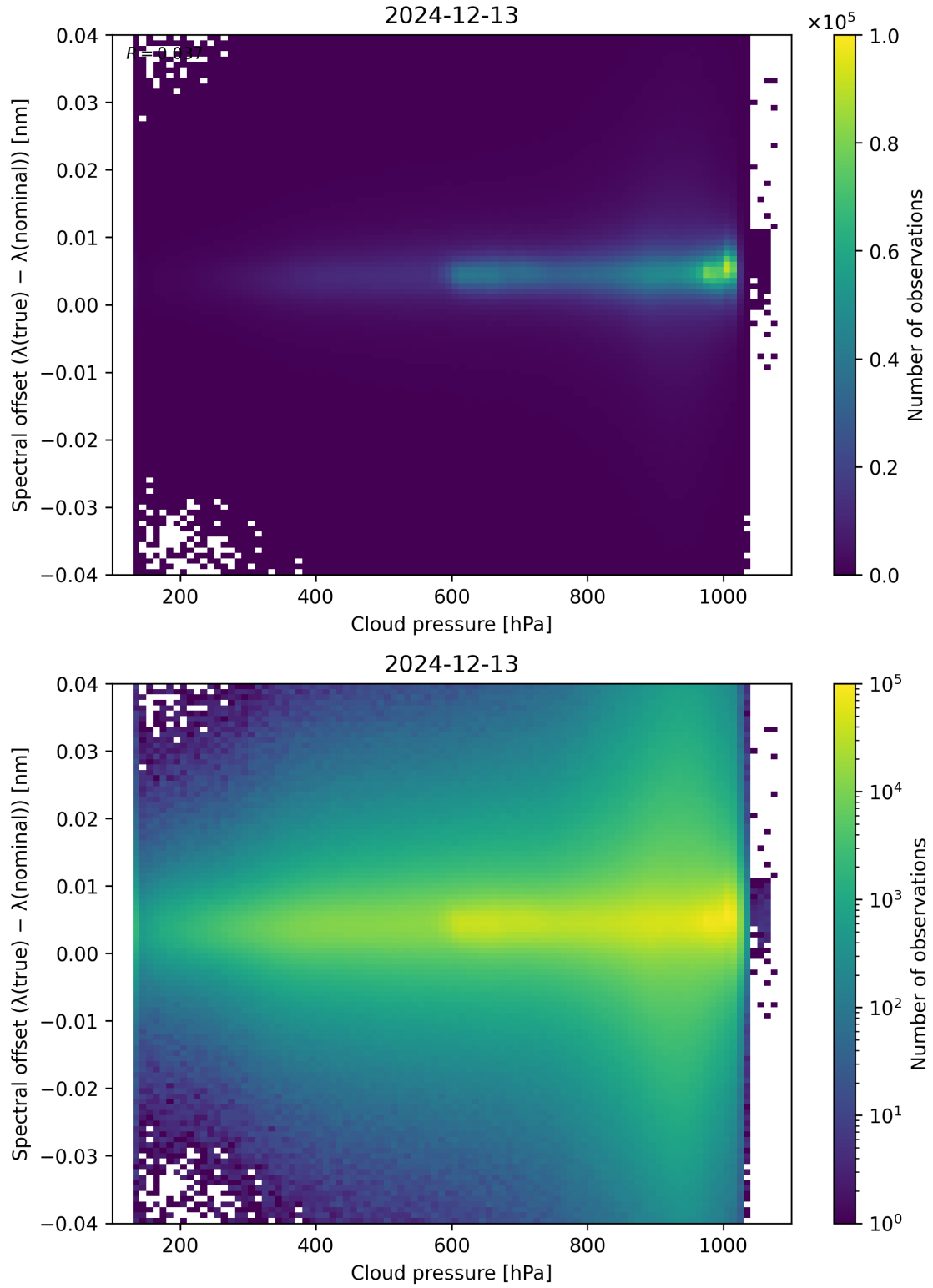
Figure 84: Scatter density plot of “Cloud pressure” against “Spectral offset ( \lambda_{\text{true}} - \lambda_{\text{nominal}} )” for 2024-12-12 to 2024-12-14.
