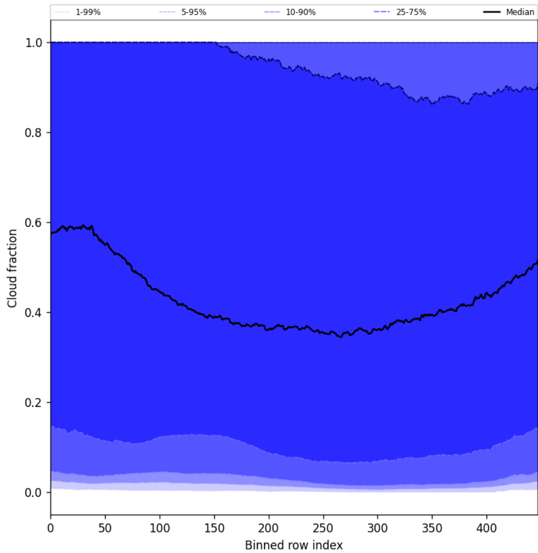
Figure 49: Along track statistics of “Cloud fraction” for 2024-12-12 to 2024-12-14
