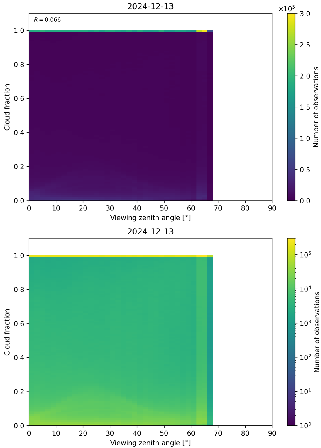
Figure 120: Scatter density plot of “Viewing zenith angle” against “Cloud fraction” for 2024-12-12 to 2024-12-14.
