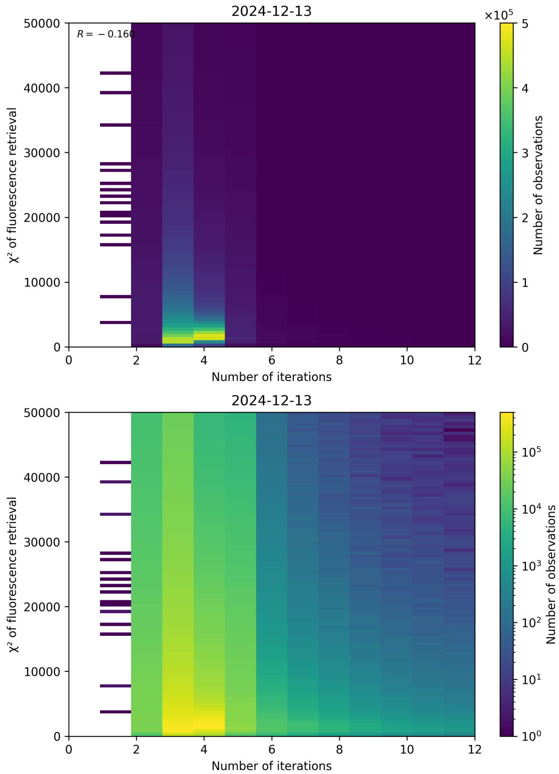
Figure 97: Scatter density plot of “Number of iterations” against “ \chi^2 of fluorescence retrieval” for 2024-12-12 to 2024-12-14.
