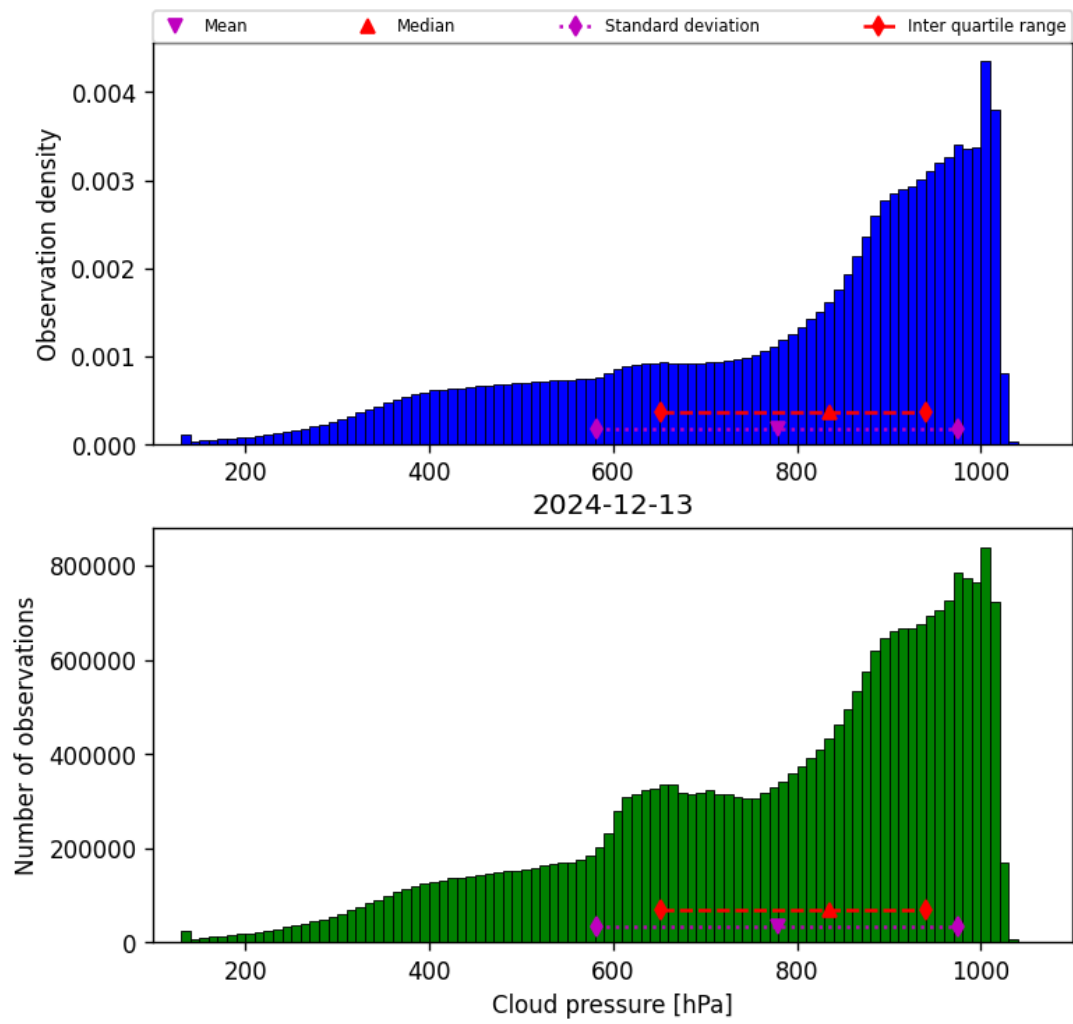
Figure 30: Histogram of “Cloud pressure” for 2024-12-12 to 2024-12-14
