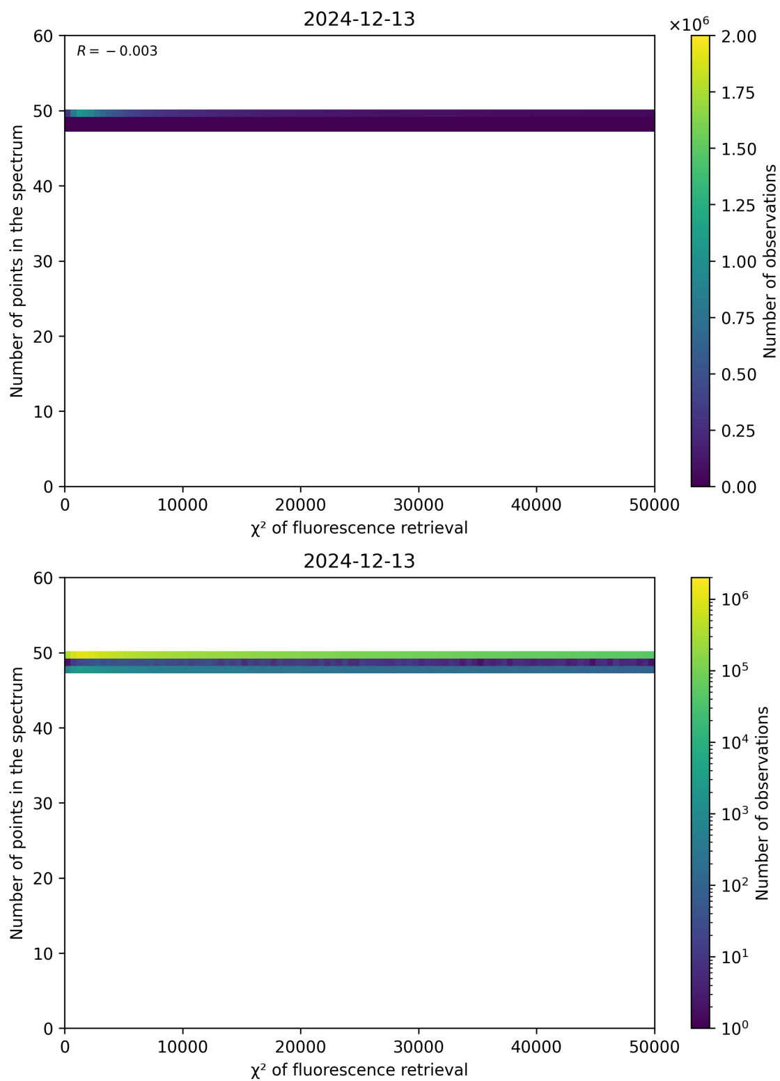
Figure 68: Scatter density plot of “ \chi^2 of fluorescence retrieval” against “Number of points in the spectrum” for 2024-12-12 to 2024-12-14.
