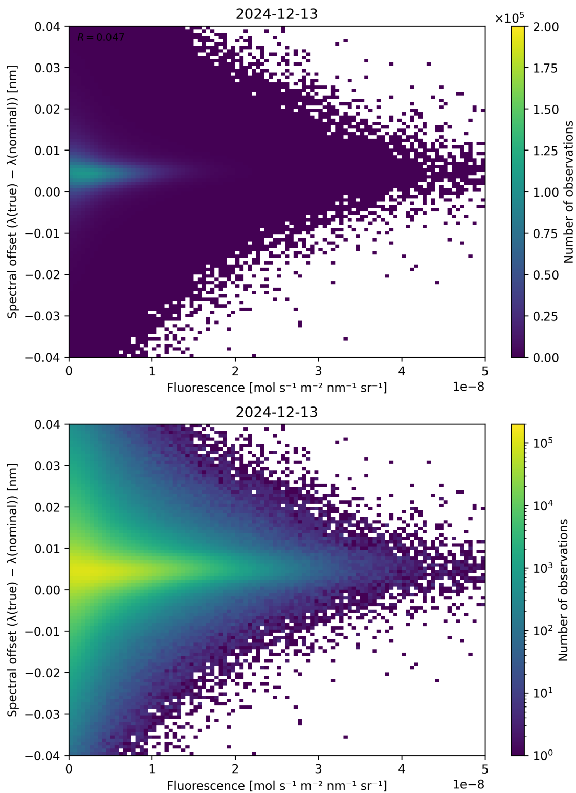
Figure 87: Scatter density plot of “Fluorescence” against “Spectral offset ( \lambda_{\text{true}} - \lambda_{\text{nominal}} )” for 2024-12-12 to 2024-12-14.
