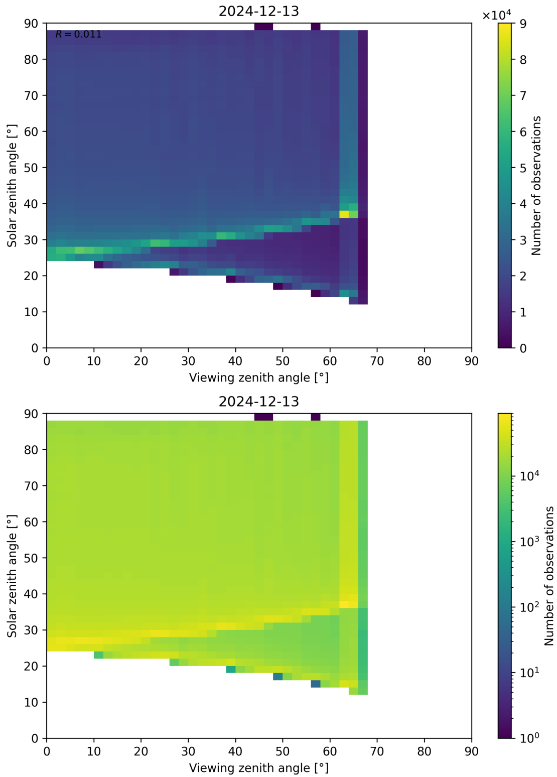
Figure 127: Scatter density plot of “Viewing zenith angle” against “Solar zenith angle” for 2024-12-12 to 2024-12-14.
