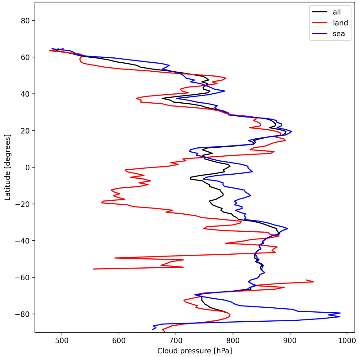
Figure 13: Zonal average of “Cloud pressure” for 2024-12-12 to 2024-12-14.
