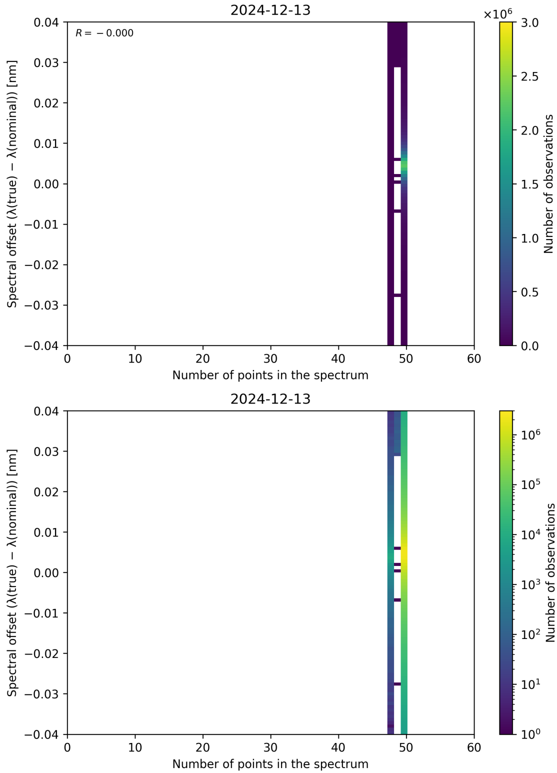
Figure 101: Scatter density plot of “Number of points in the spectrum” against “Spectral offset ( \lambda_{\text{true}} - \lambda_{\text{nominal}} )” for 2024-12-12 to 2024-12-14.
