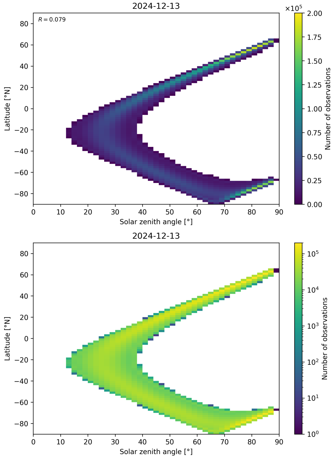
Figure 113: Scatter density plot of “Solar zenith angle” against “Latitude” for 2024-12-12 to 2024-12-14.
