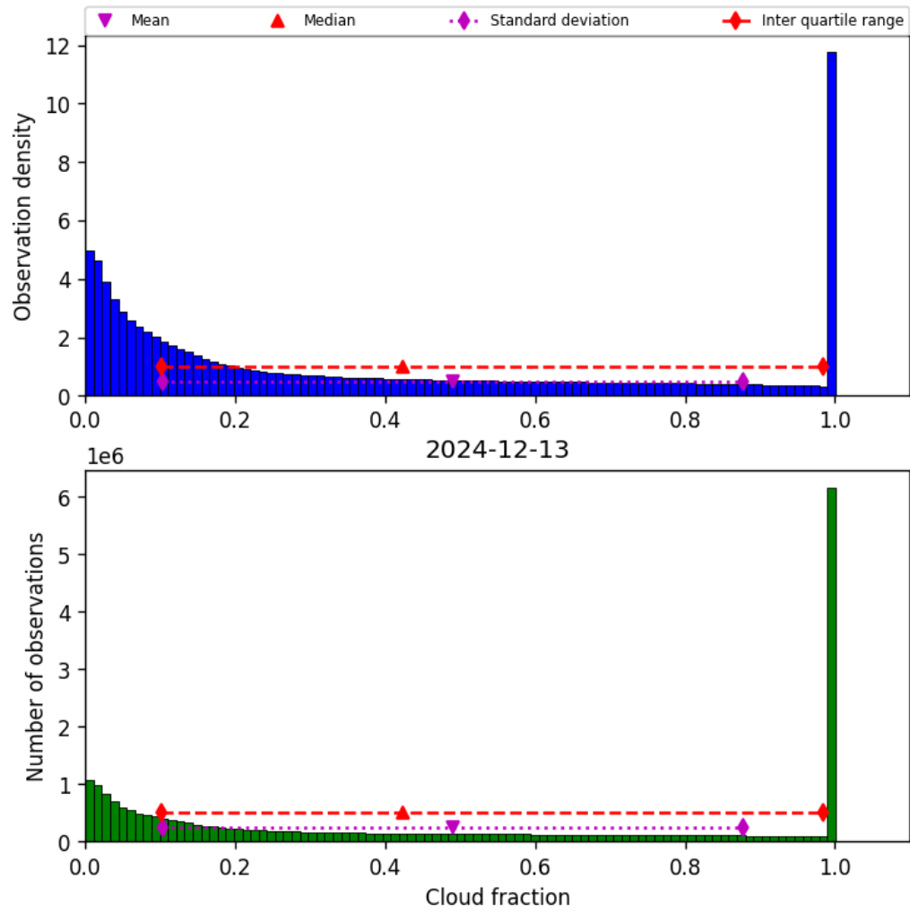
Figure 32: Histogram of “Cloud fraction” for 2024-12-12 to 2024-12-14
