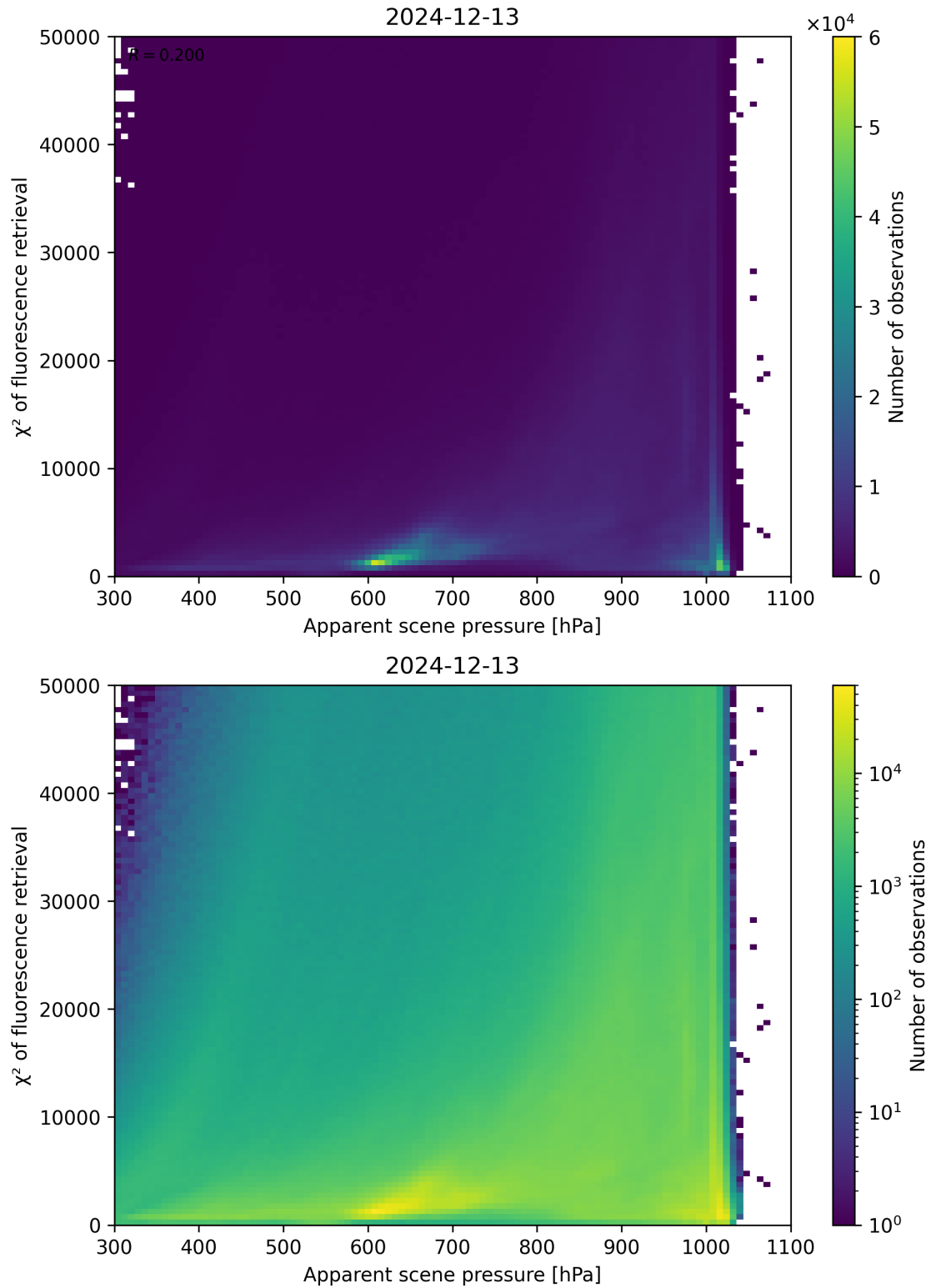
Figure 63: Scatter density plot of “Apparent scene pressure” against “ \chi^2 of fluorescence retrieval” for 2024-12-12 to 2024-12-14.
