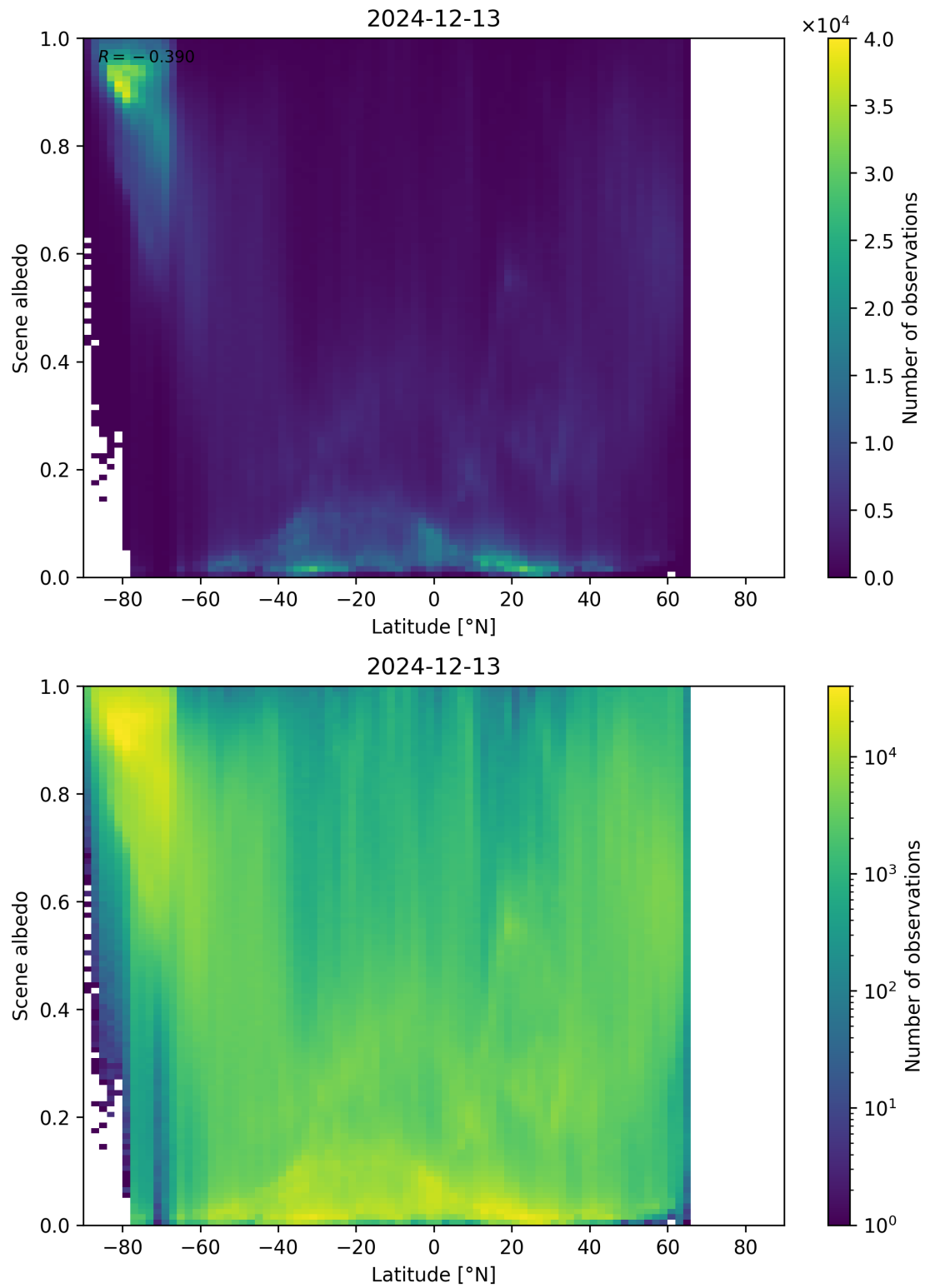
Figure 95: Scatter density plot of “Latitude” against “Scene albedo” for 2024-12-12 to 2024-12-14.
