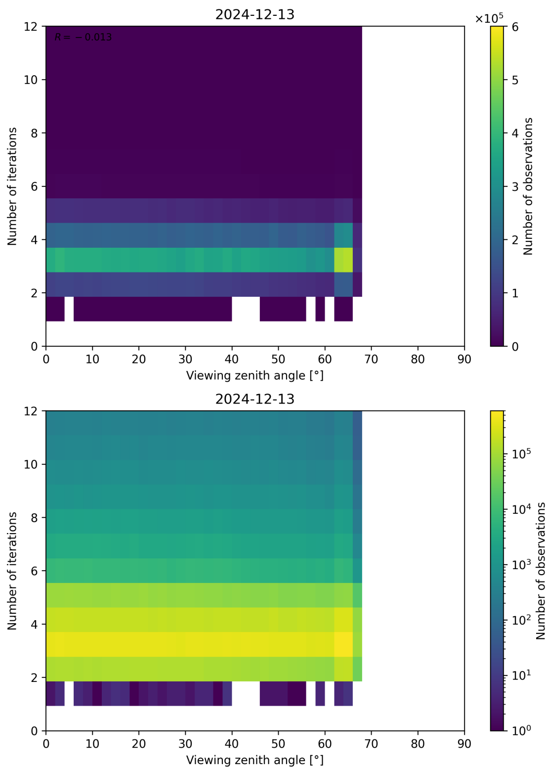
Figure 124: Scatter density plot of “Viewing zenith angle” against “Number of iterations” for 2024-12-12 to 2024-12-14.
