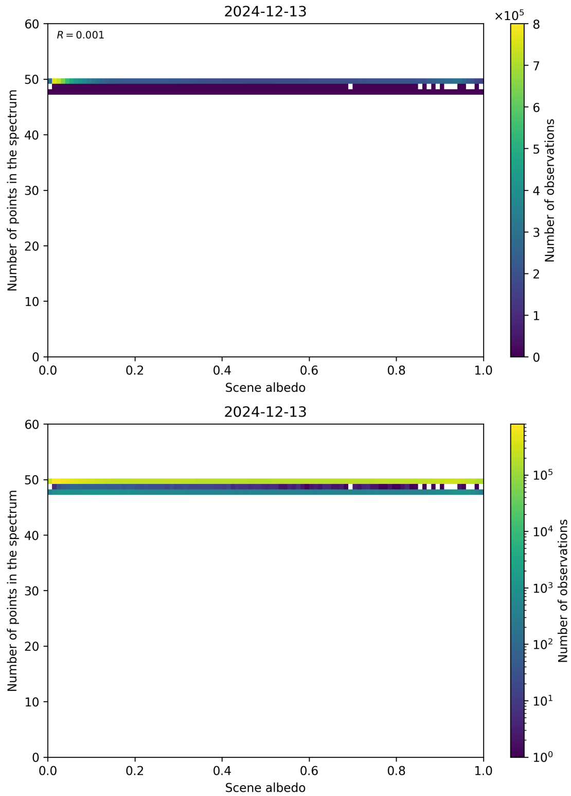
Figure 106: Scatter density plot of “Scene albedo” against “Number of points in the spectrum” for 2024-12-12 to 2024-12-14.
