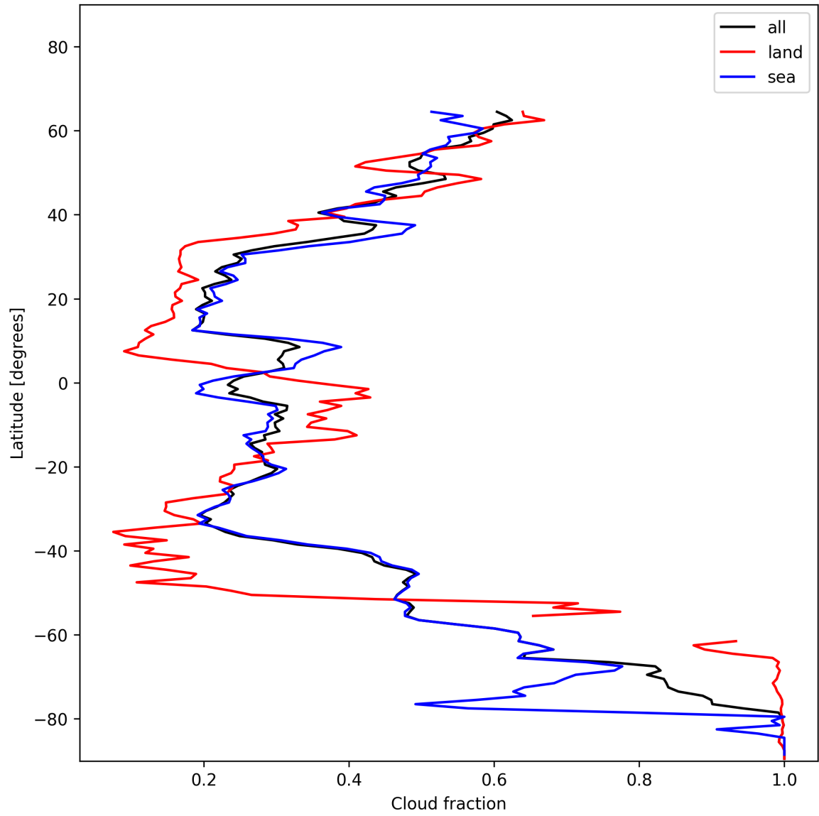
Figure 15: Zonal average of “Cloud fraction” for 2024-12-12 to 2024-12-14.
