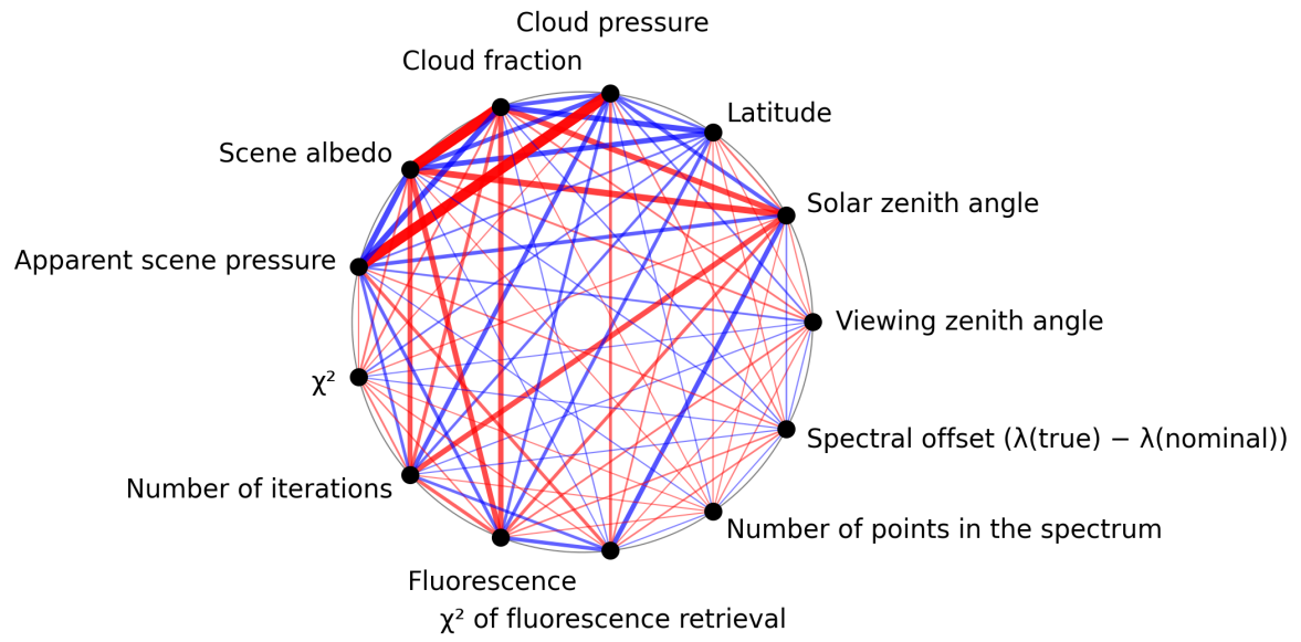
Figure 1: Map of correlation graph for 2024-12-12 to 2024-12-14.
