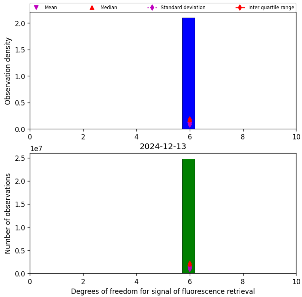
Figure 43: Histogram of "Degrees of freedom for signal of fluorescence retrieval" for 2024-12-12 to 2024-12-14
