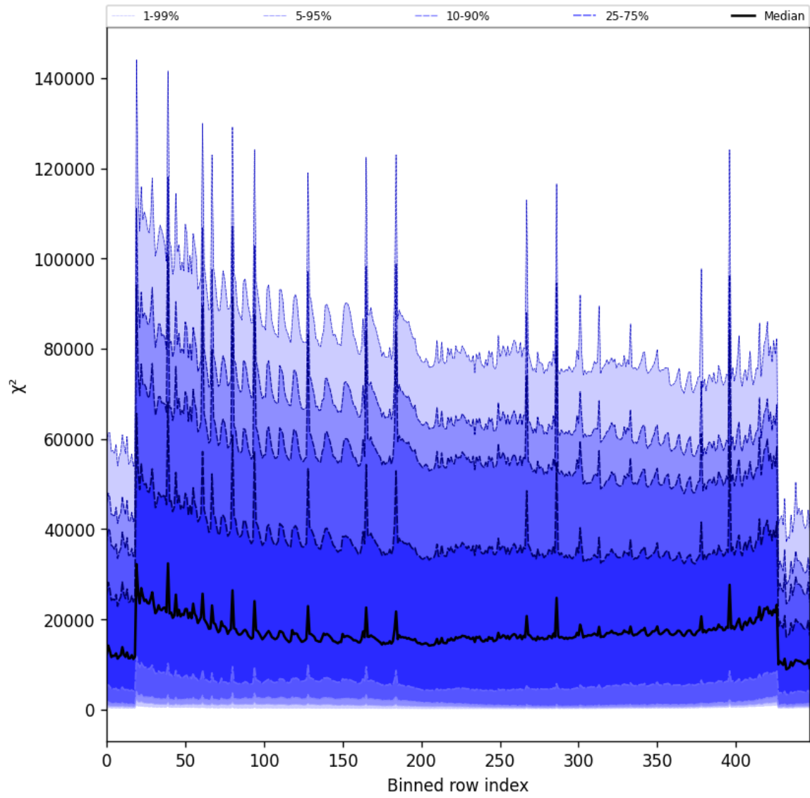
Figure 55: Along track statistics of “ \chi^2 ” for 2024-12-12 to 2024-12-14
