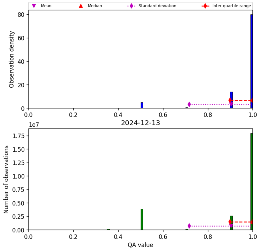
Figure 29: Histogram of “QA value” for 2024-12-12 to 2024-12-14
