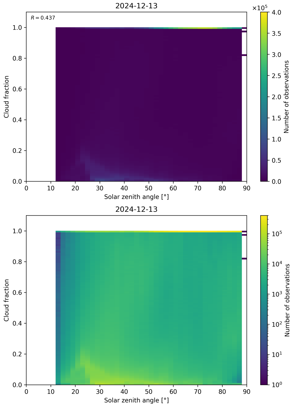
Figure 110: Scatter density plot of “Solar zenith angle” against “Cloud fraction” for 2024-12-12 to 2024-12-14.
