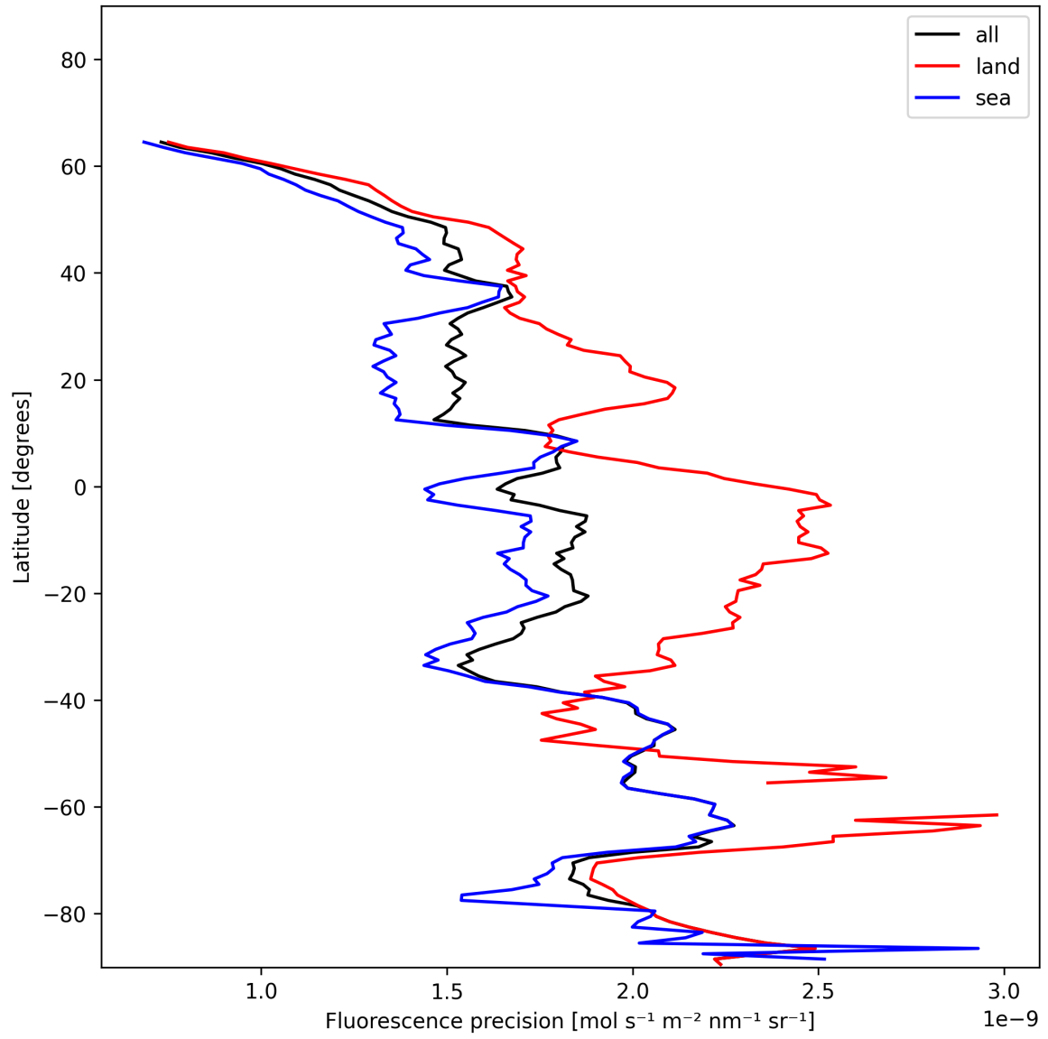
Figure 24: Zonal average of “Fluorescence precision” for 2024-12-12 to 2024-12-14.
