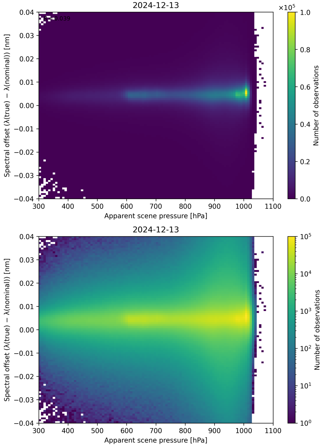
Figure 67: Scatter density plot of “Apparent scene pressure” against “Spectral offset ( \lambda_{\text{true}} - \lambda_{\text{nominal}} )” for 2024-12-12 to 2024-12-14.
