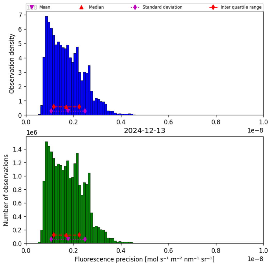
Figure 41: Histogram of “Fluorescence precision” for 2024-12-12 to 2024-12-14
