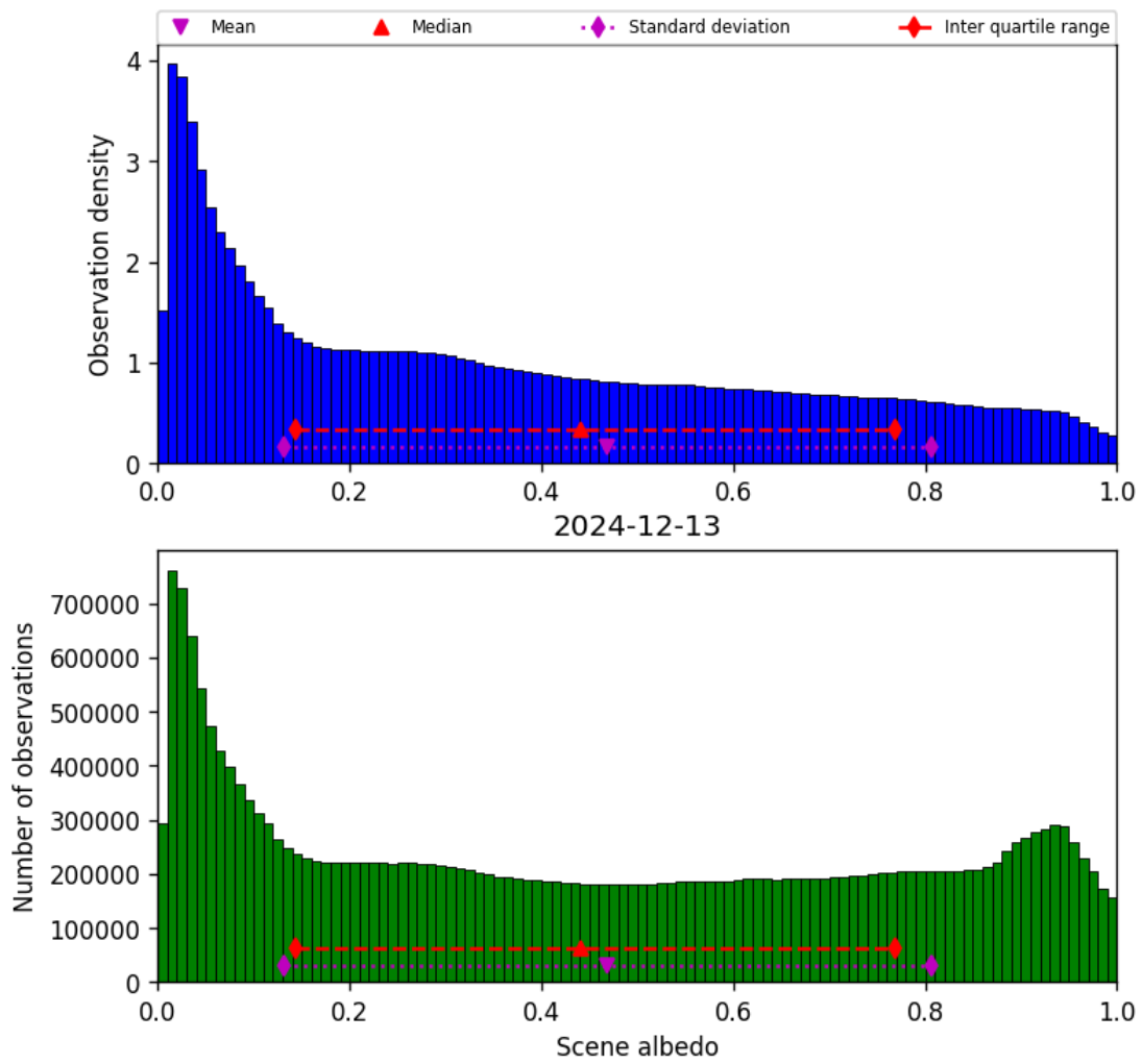
Figure 34: Histogram of “Scene albedo” for 2024-12-12 to 2024-12-14
