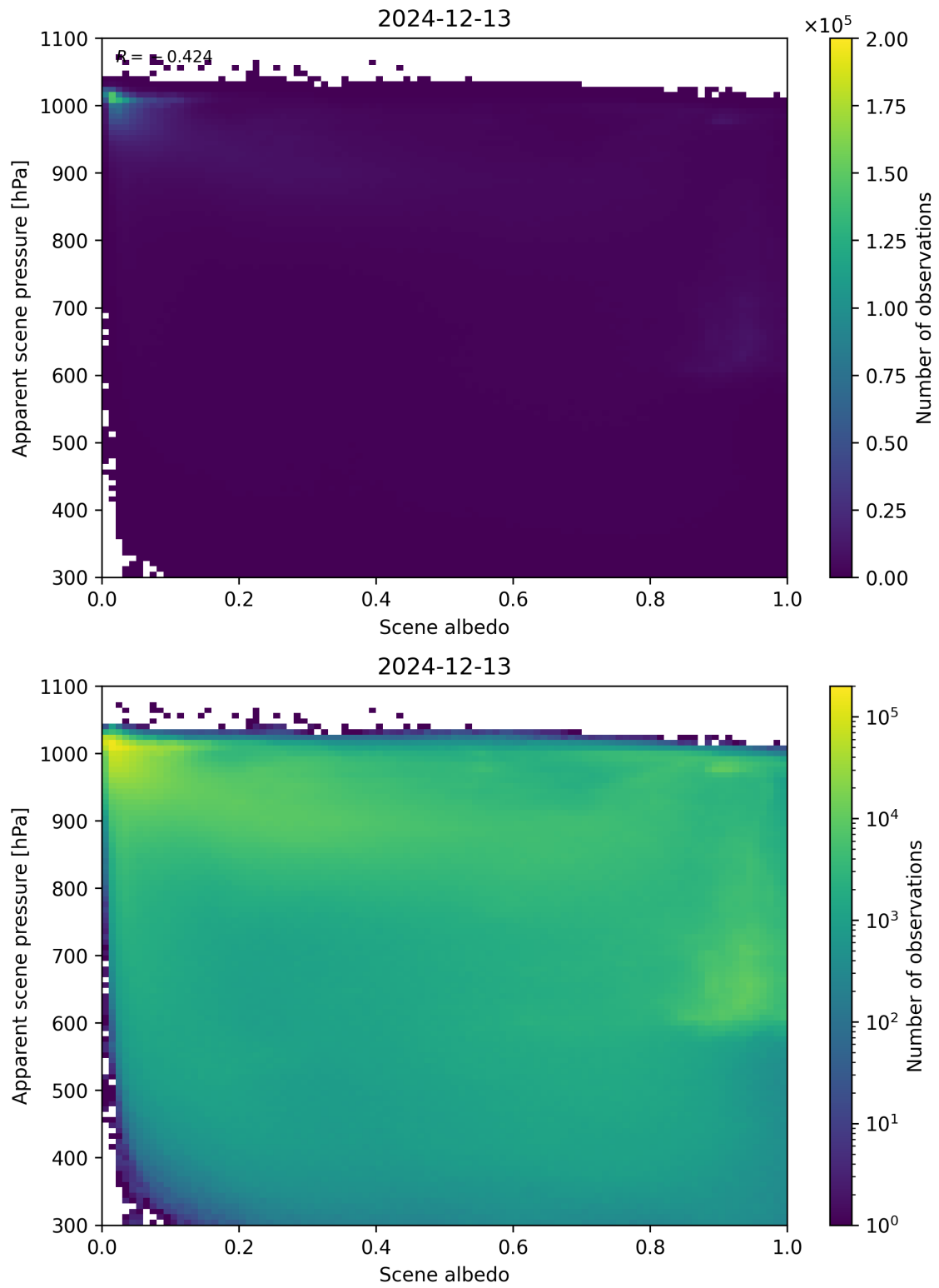
Figure 102: Scatter density plot of “Scene albedo” against “Apparent scene pressure” for 2024-12-12 to 2024-12-14.
