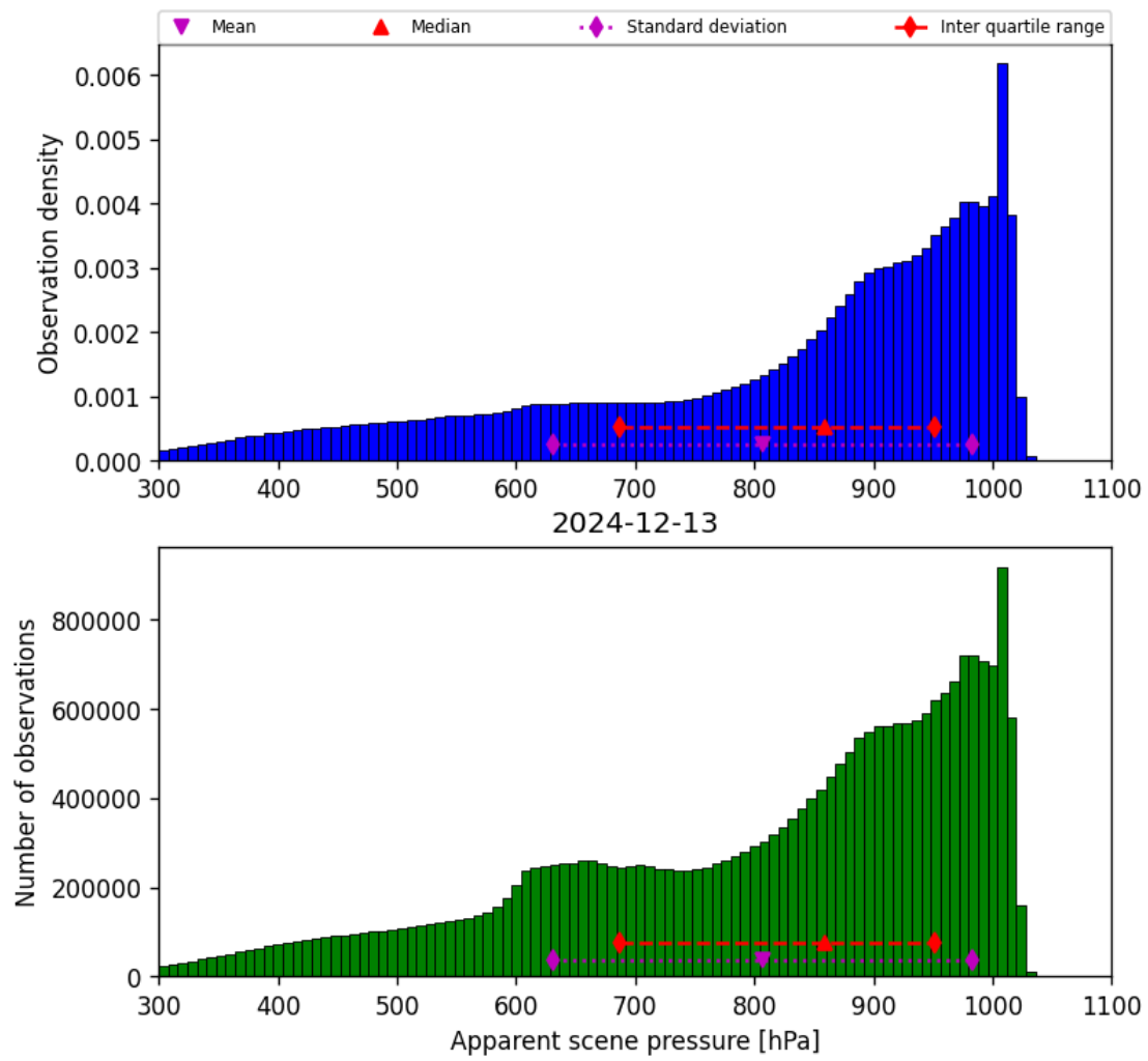
Figure 36: Histogram of “Apparent scene pressure” for 2024-12-12 to 2024-12-14
