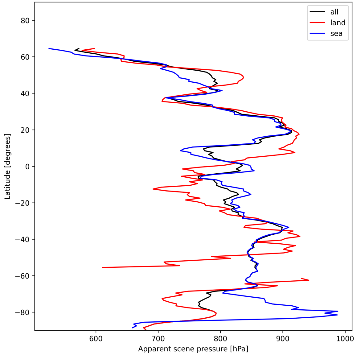
Figure 19: Zonal average of “Apparent scene pressure” for 2024-12-12 to 2024-12-14.
