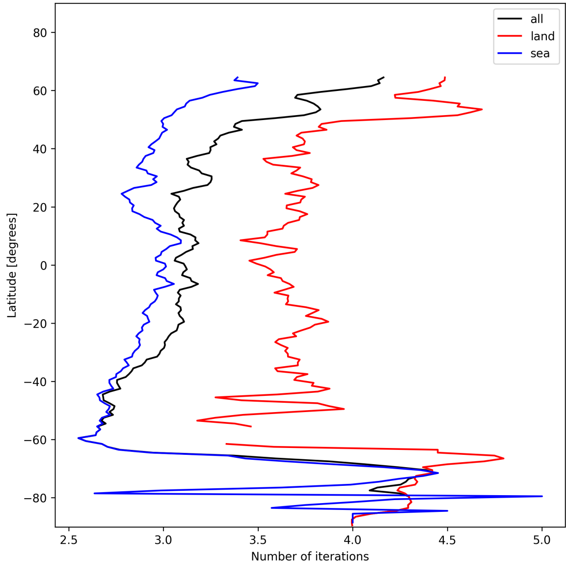
Figure 22: Zonal average of “Number of iterations” for 2024-12-12 to 2024-12-14.
