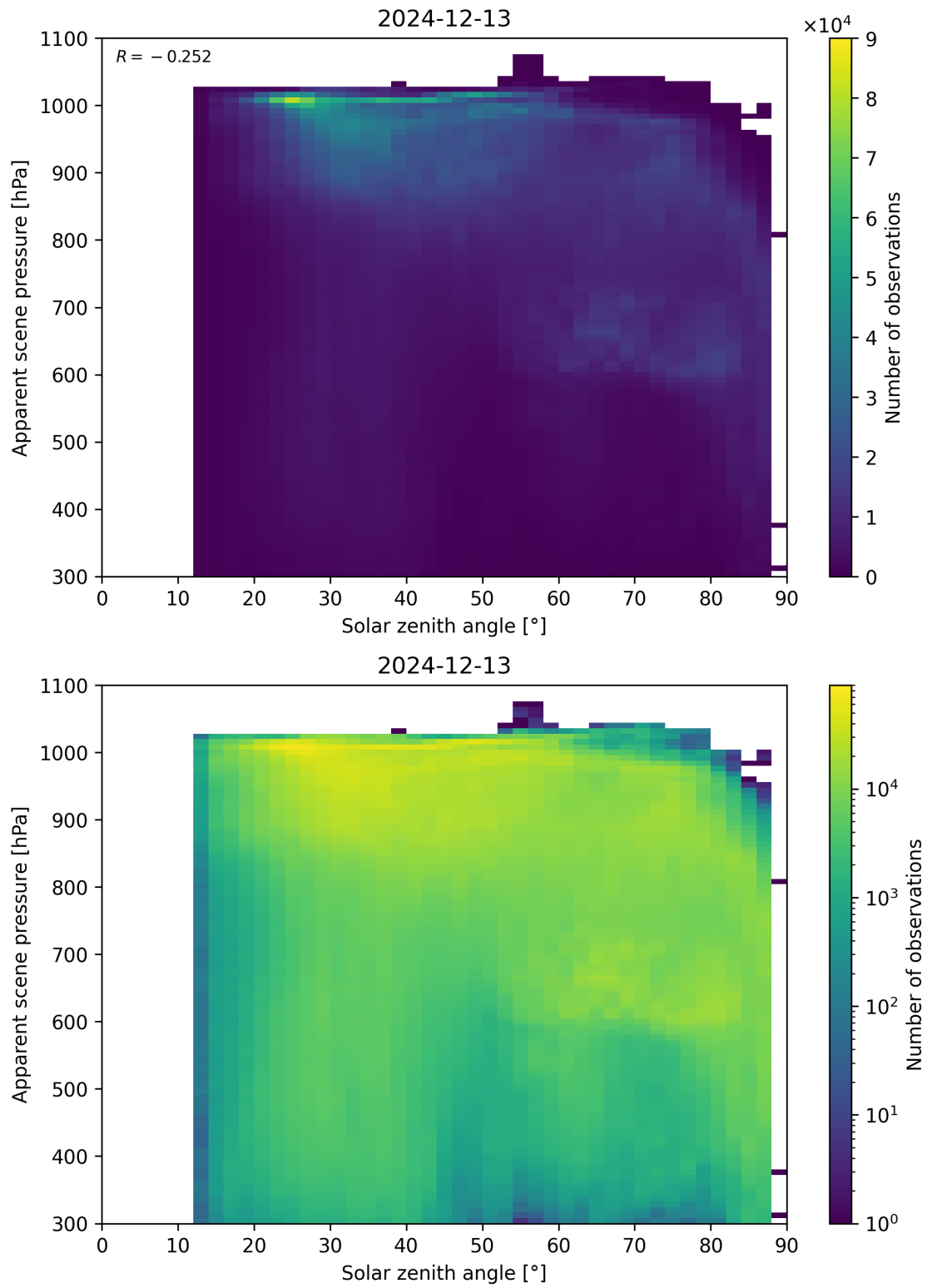
Figure 108: Scatter density plot of “Solar zenith angle” against “Apparent scene pressure” for 2024-12-12 to 2024-12-14.
