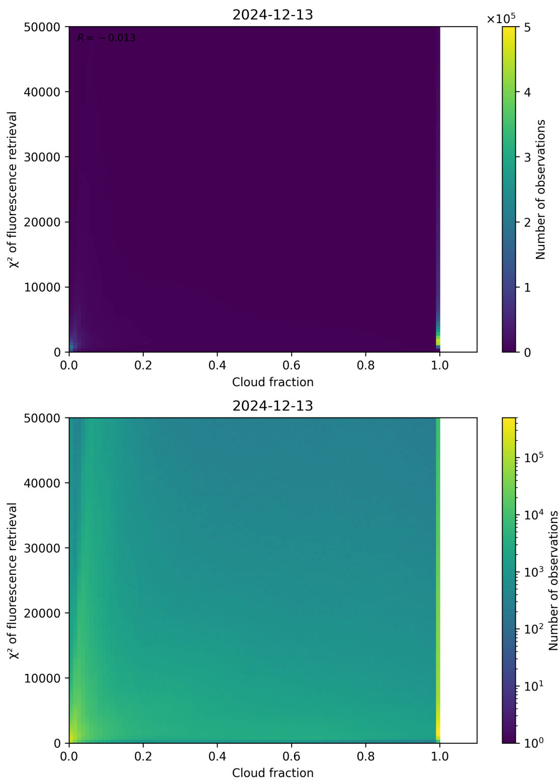
Figure 71: Scatter density plot of “Cloud fraction” against “ \chi^2 of fluorescence retrieval” for 2024-12-12 to 2024-12-14.
