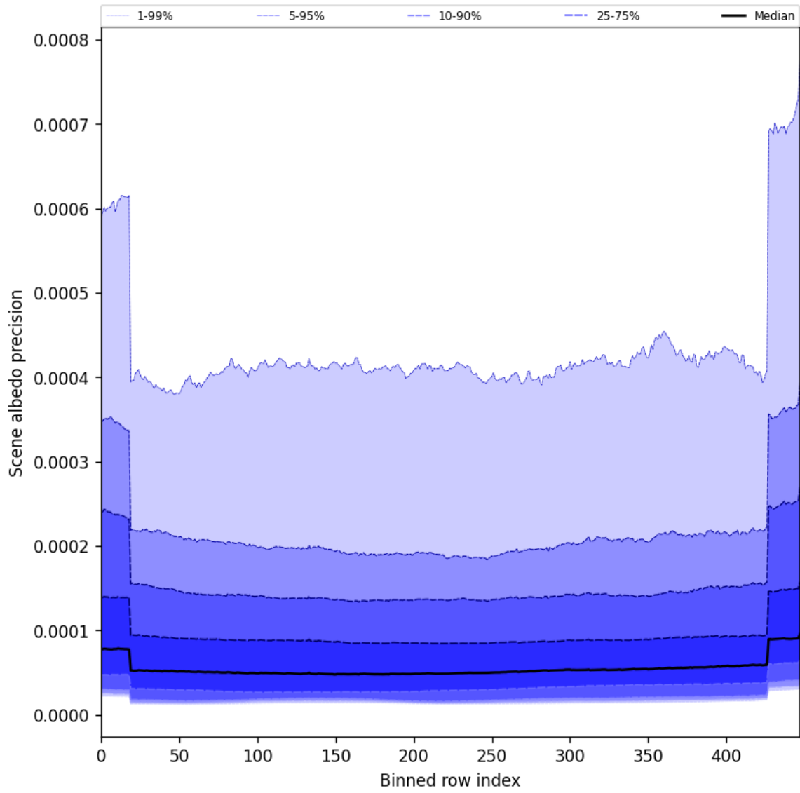
Figure 52: Along track statistics of “Scene albedo precision” for 2024-12-12 to 2024-12-14
