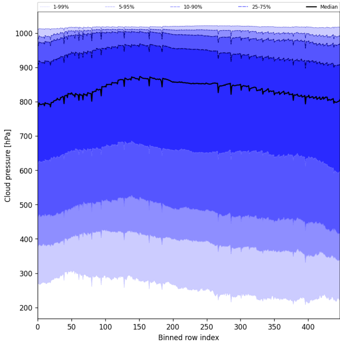
Figure 47: Along track statistics of “Cloud pressure” for 2024-12-12 to 2024-12-14
