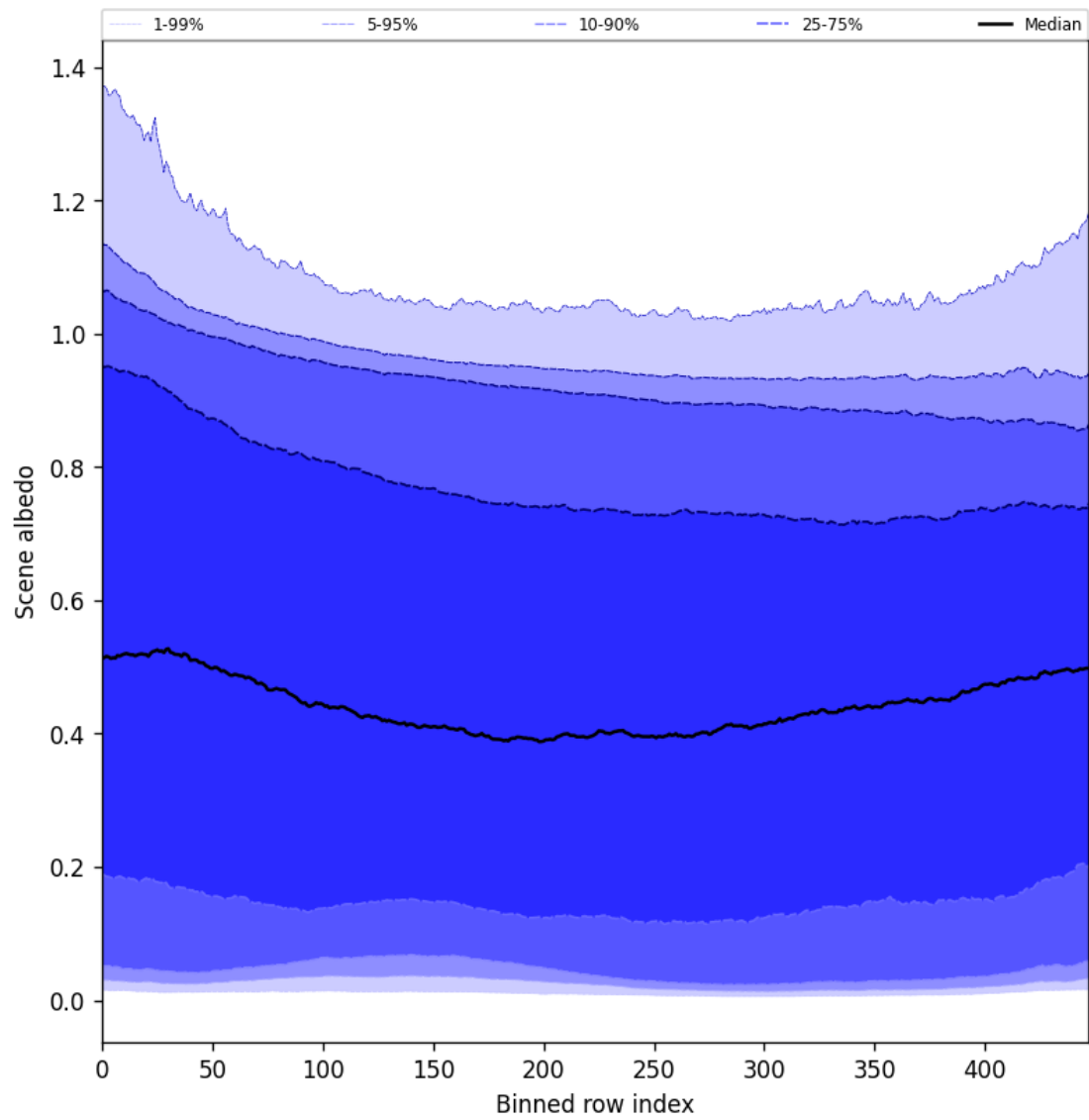
Figure 51: Along track statistics of "Scene albedo" for 2024-12-12 to 2024-12-14
