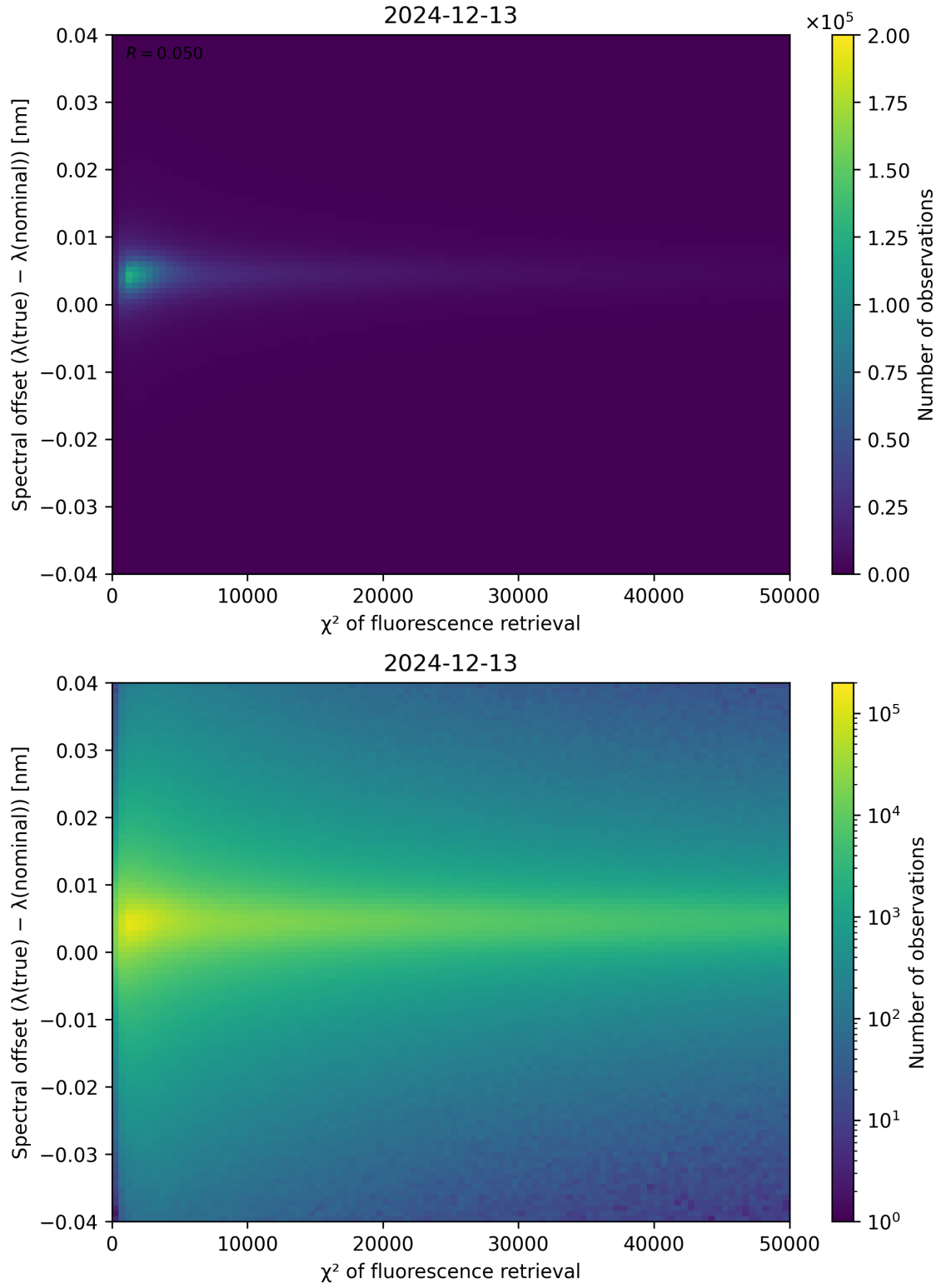
Figure 69: Scatter density plot of “ \chi^2 of fluorescence retrieval” against “Spectral offset ( \lambda_{\text{true}} - \lambda_{\text{nominal}} )” for 2024-12-12 to 2024-12-14.
