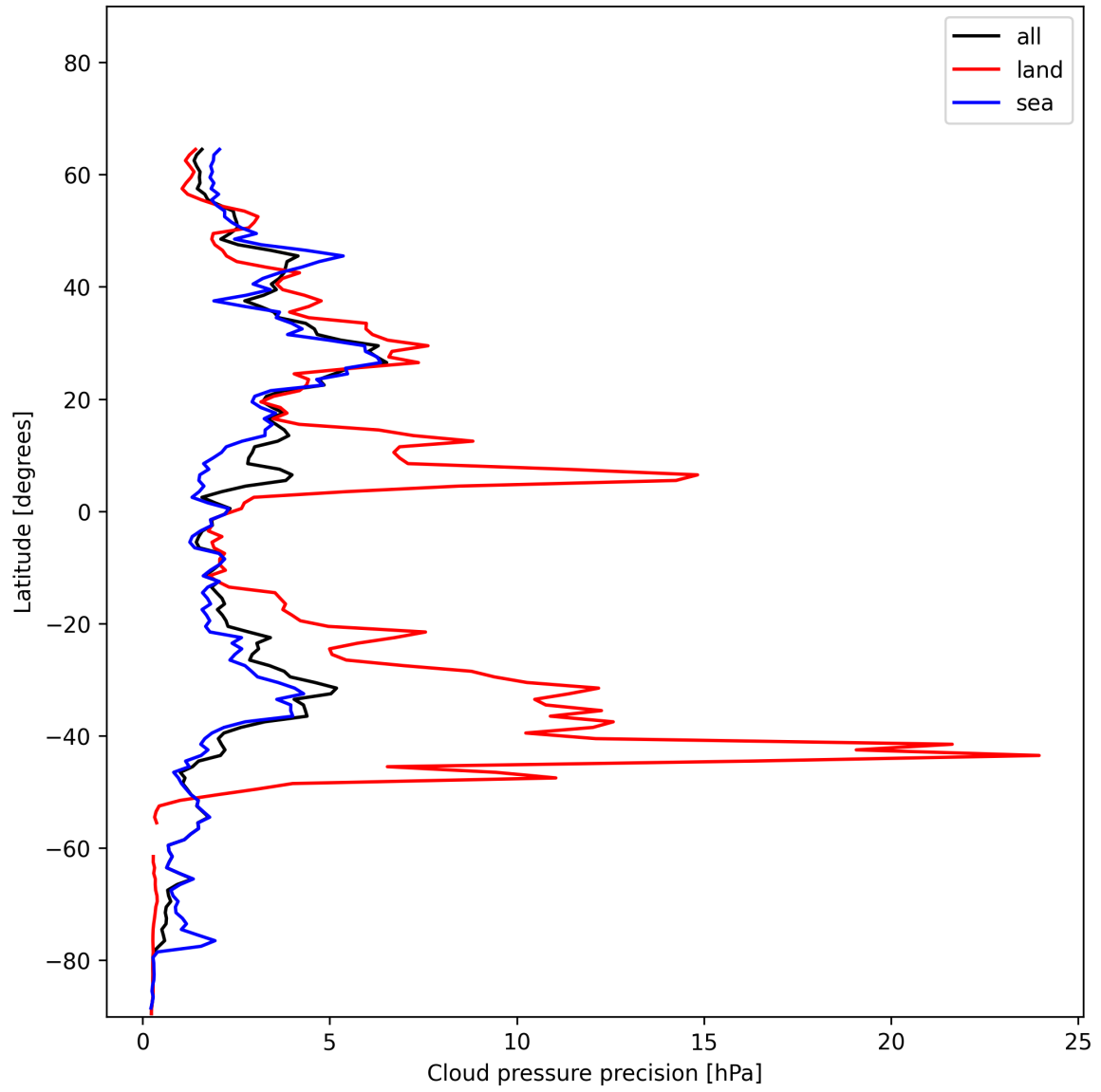
Figure 14: Zonal average of “Cloud pressure precision” for 2024-12-12 to 2024-12-14.
