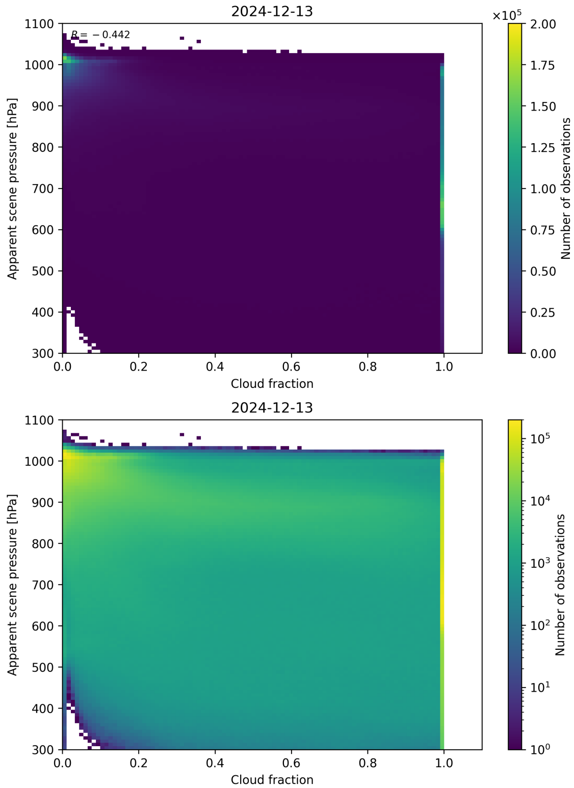
Figure 70: Scatter density plot of “Cloud fraction” against “Apparent scene pressure” for 2024-12-12 to 2024-12-14.
