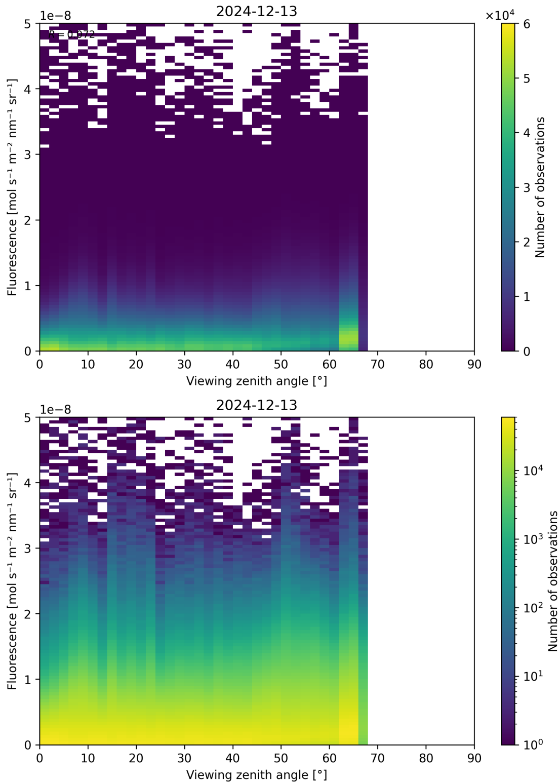
Figure 122: Scatter density plot of “Viewing zenith angle” against “Fluorescence” for 2024-12-12 to 2024-12-14.
