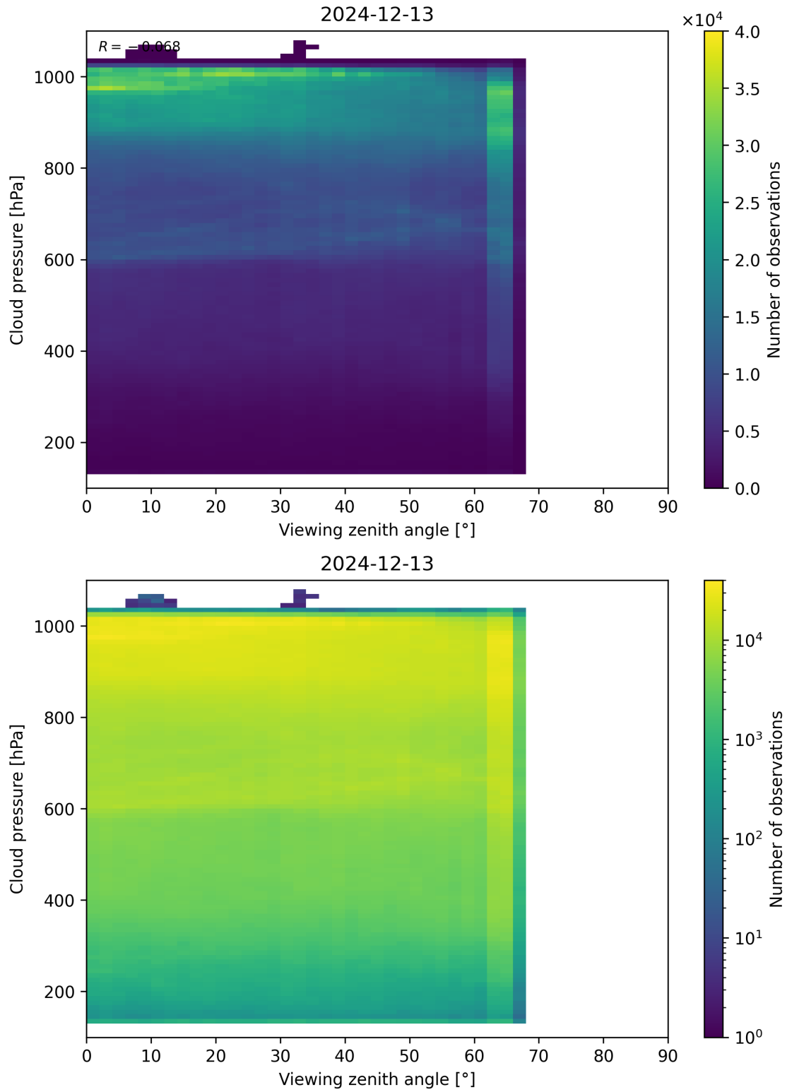
Figure 121: Scatter density plot of “Viewing zenith angle” against “Cloud pressure” for 2024-12-12 to 2024-12-14.
