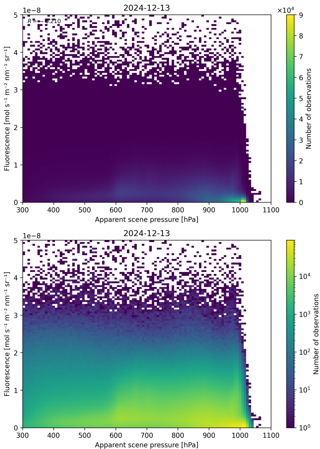
Figure 64: Scatter density plot of “Apparent scene pressure” against “Fluorescence” for 2024-12-12 to 2024-12-14.
