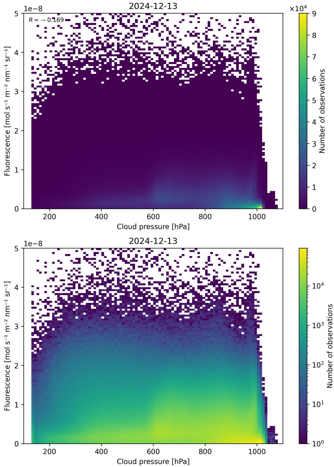
Figure 80: Scatter density plot of “Cloud pressure” against “Fluorescence” for 2024-12-12 to 2024-12-14.
