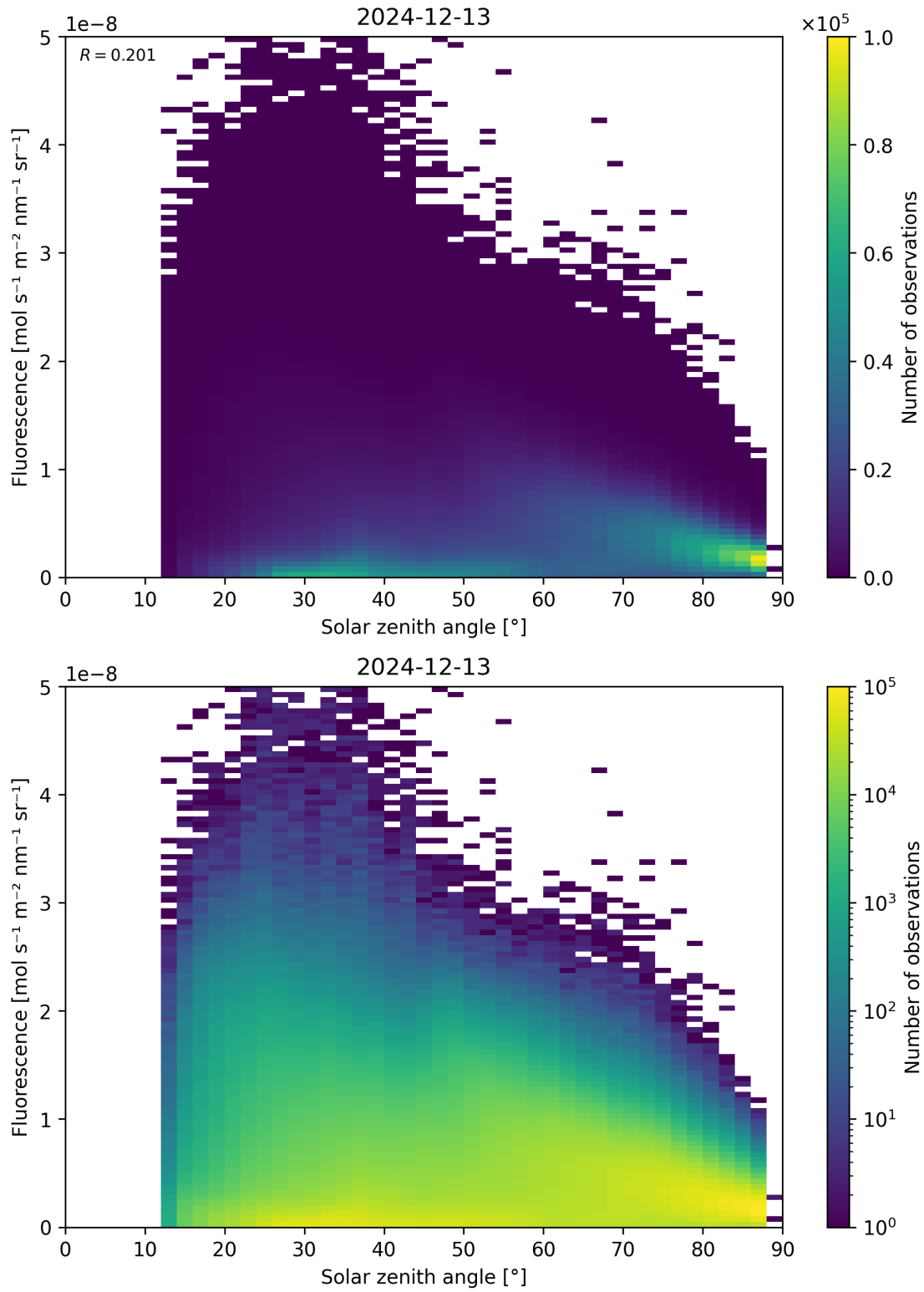
Figure 112: Scatter density plot of “Solar zenith angle” against “Fluorescence” for 2024-12-12 to 2024-12-14.
