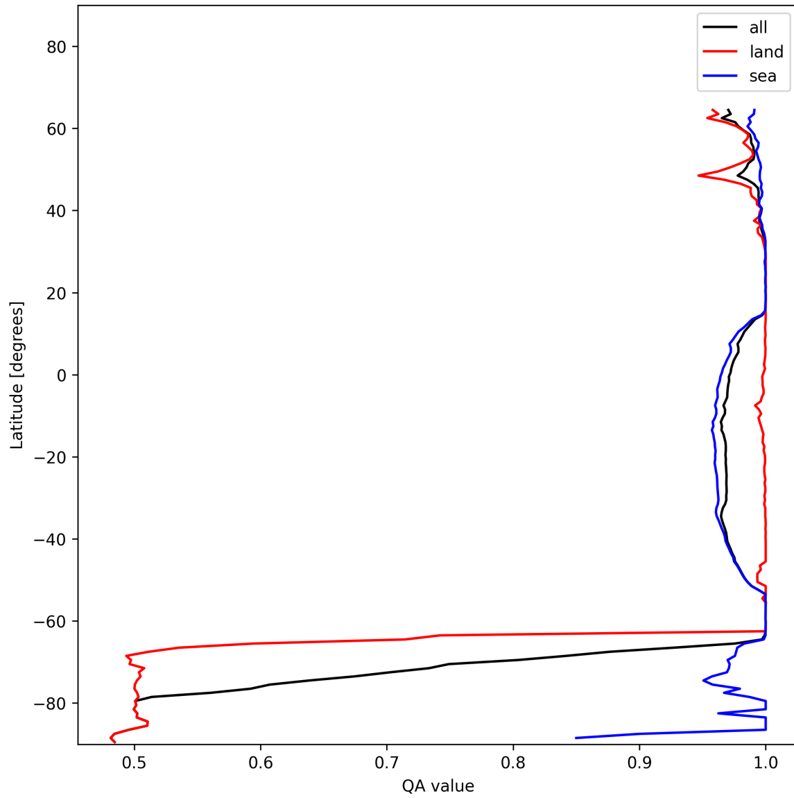
Figure 12: Zonal average of “QA value” for 2024-12-12 to 2024-12-14.
