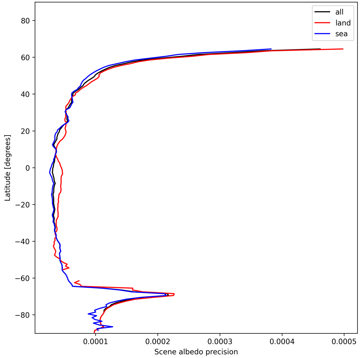
Figure 18: Zonal average of “Scene albedo precision” for 2024-12-12 to 2024-12-14.
