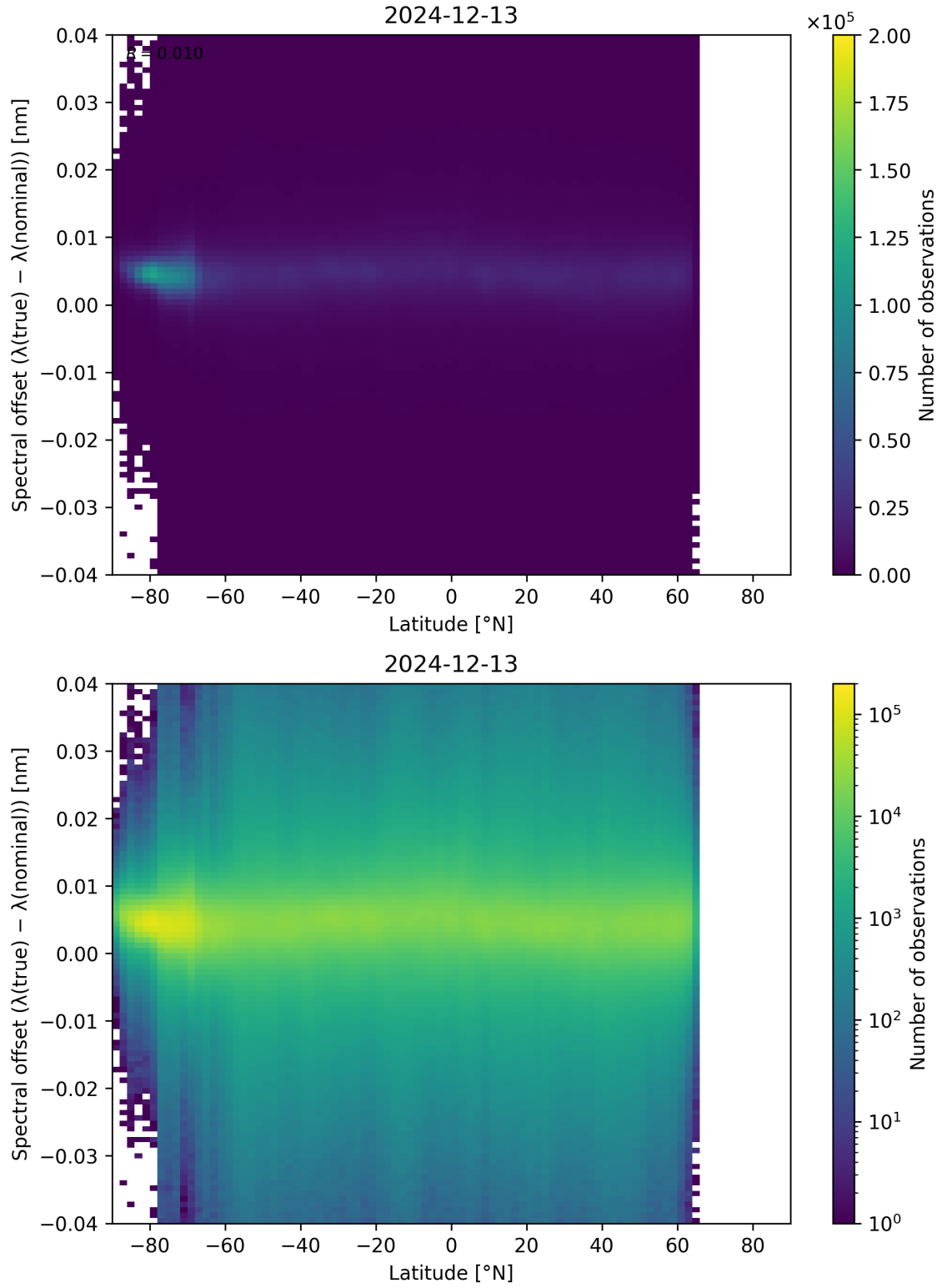
Figure 96: Scatter density plot of “Latitude” against “Spectral offset ( \lambda_{\text{true}} - \lambda_{\text{nominal}} )” for 2024-12-12 to 2024-12-14.
