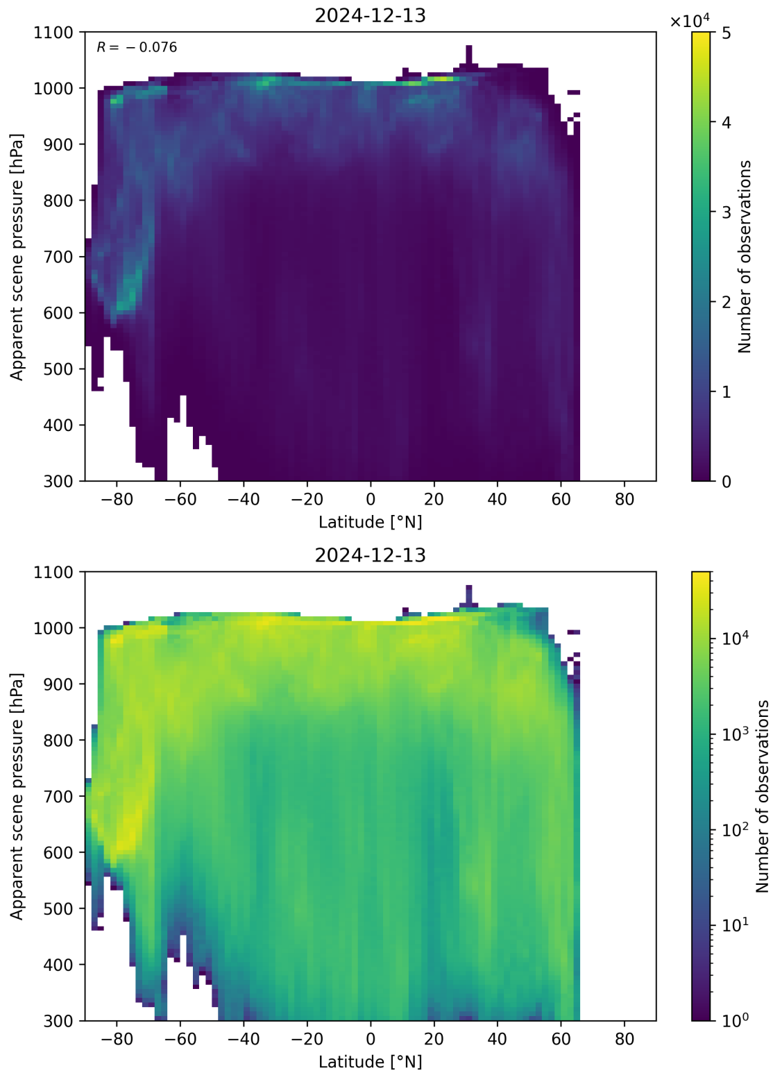
Figure 88: Scatter density plot of “Latitude” against “Apparent scene pressure” for 2024-12-12 to 2024-12-14.
