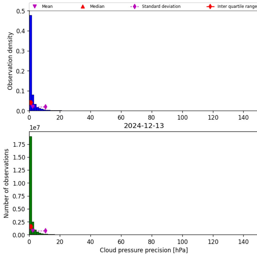
Figure 31: Histogram of “Cloud pressure precision” for 2024-12-12 to 2024-12-14
