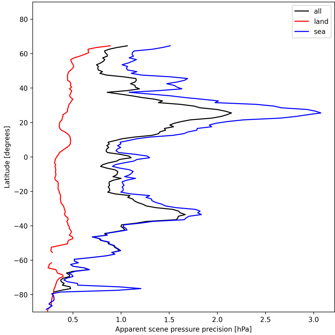
Figure 20: Zonal average of “Apparent scene pressure precision” for 2024-12-12 to 2024-12-14.
