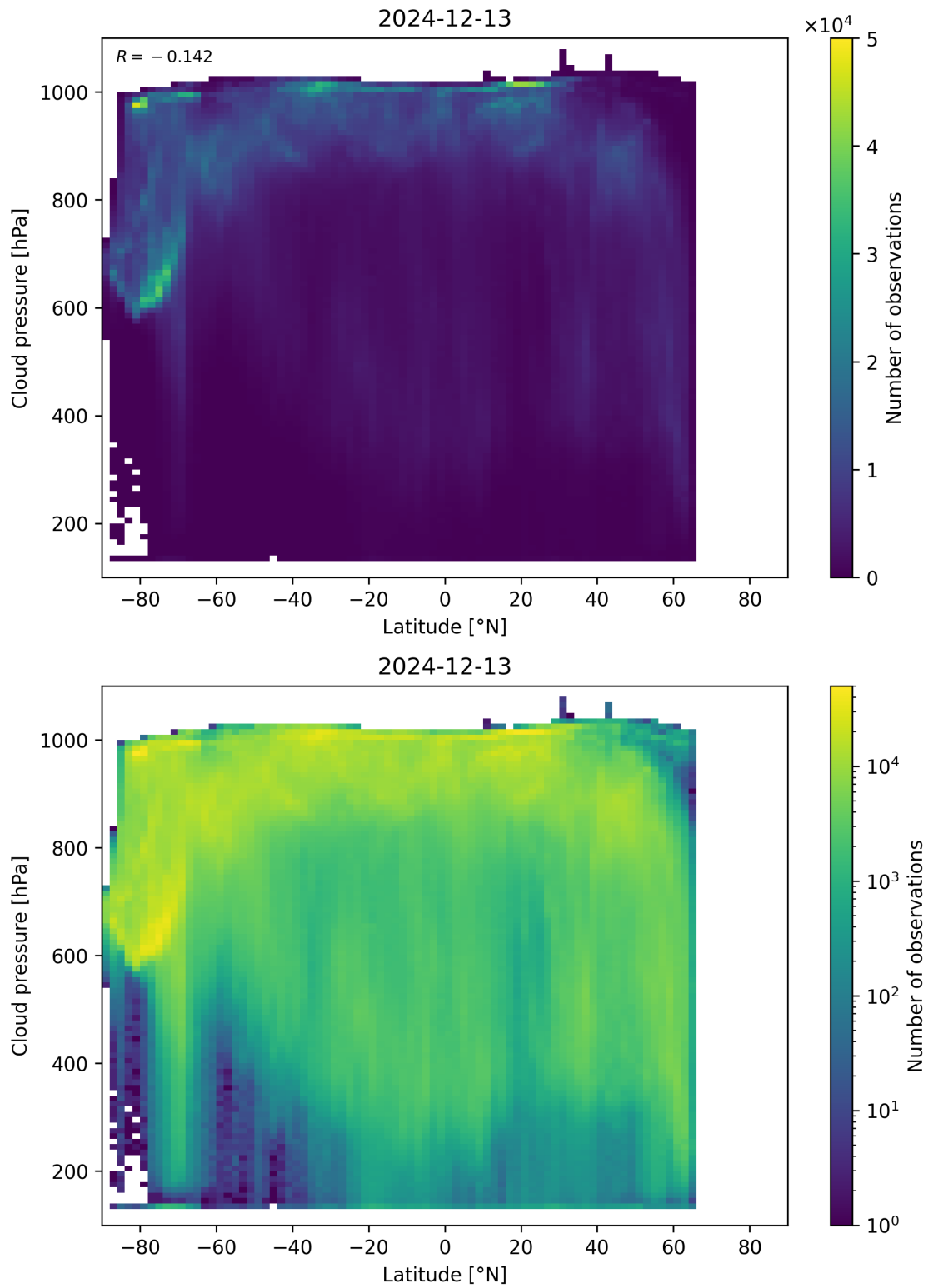
Figure 91: Scatter density plot of “Latitude” against “Cloud pressure” for 2024-12-12 to 2024-12-14.
