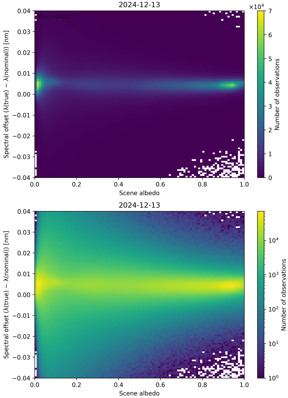
Figure 107: Scatter density plot of “Scene albedo” against “Spectral offset ( \lambda_{\text{true}} - \lambda_{\text{nominal}} )” for 2024-12-12 to 2024-12-14.
