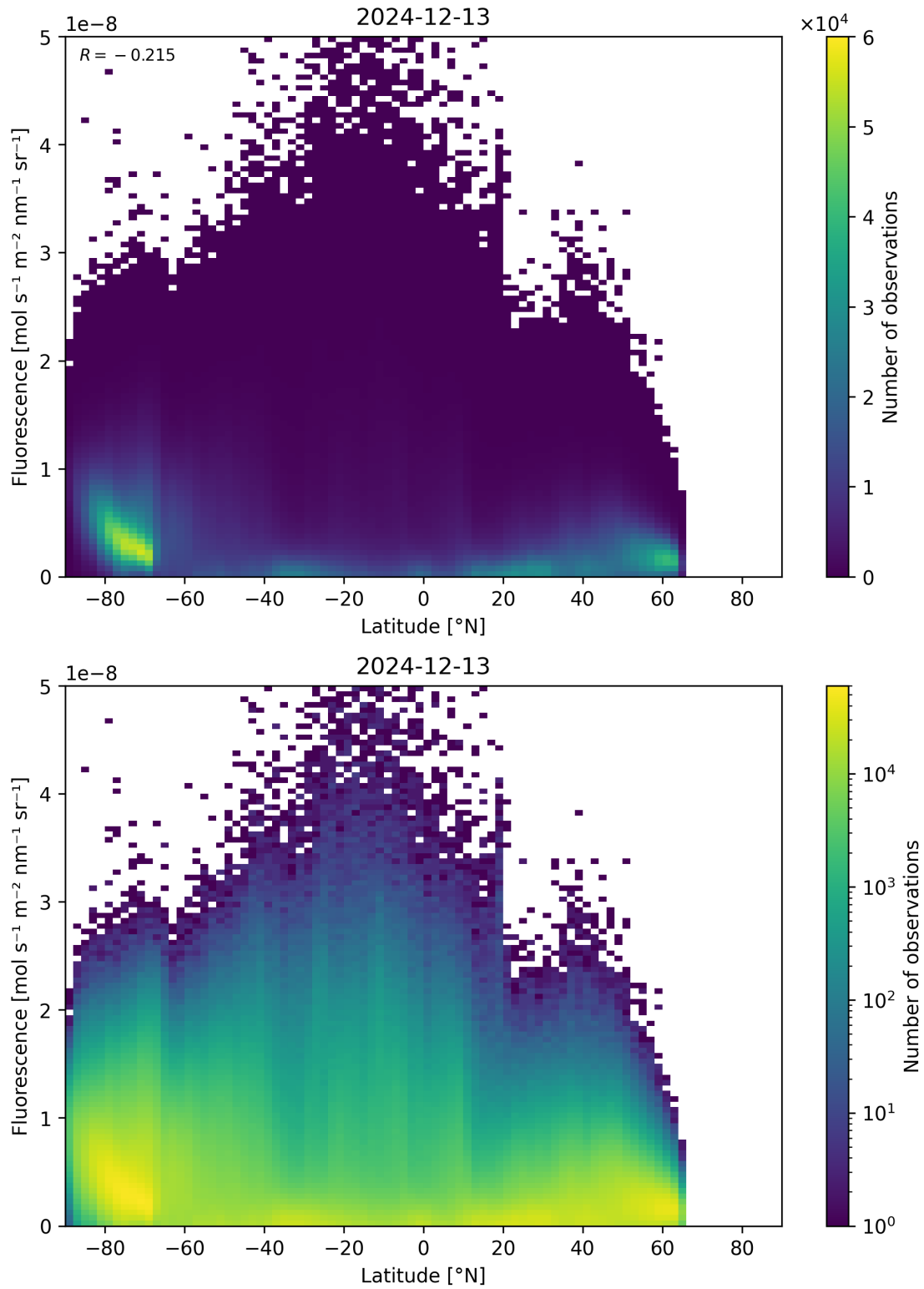
Figure 92: Scatter density plot of “Latitude” against “Fluorescence” for 2024-12-12 to 2024-12-14.
