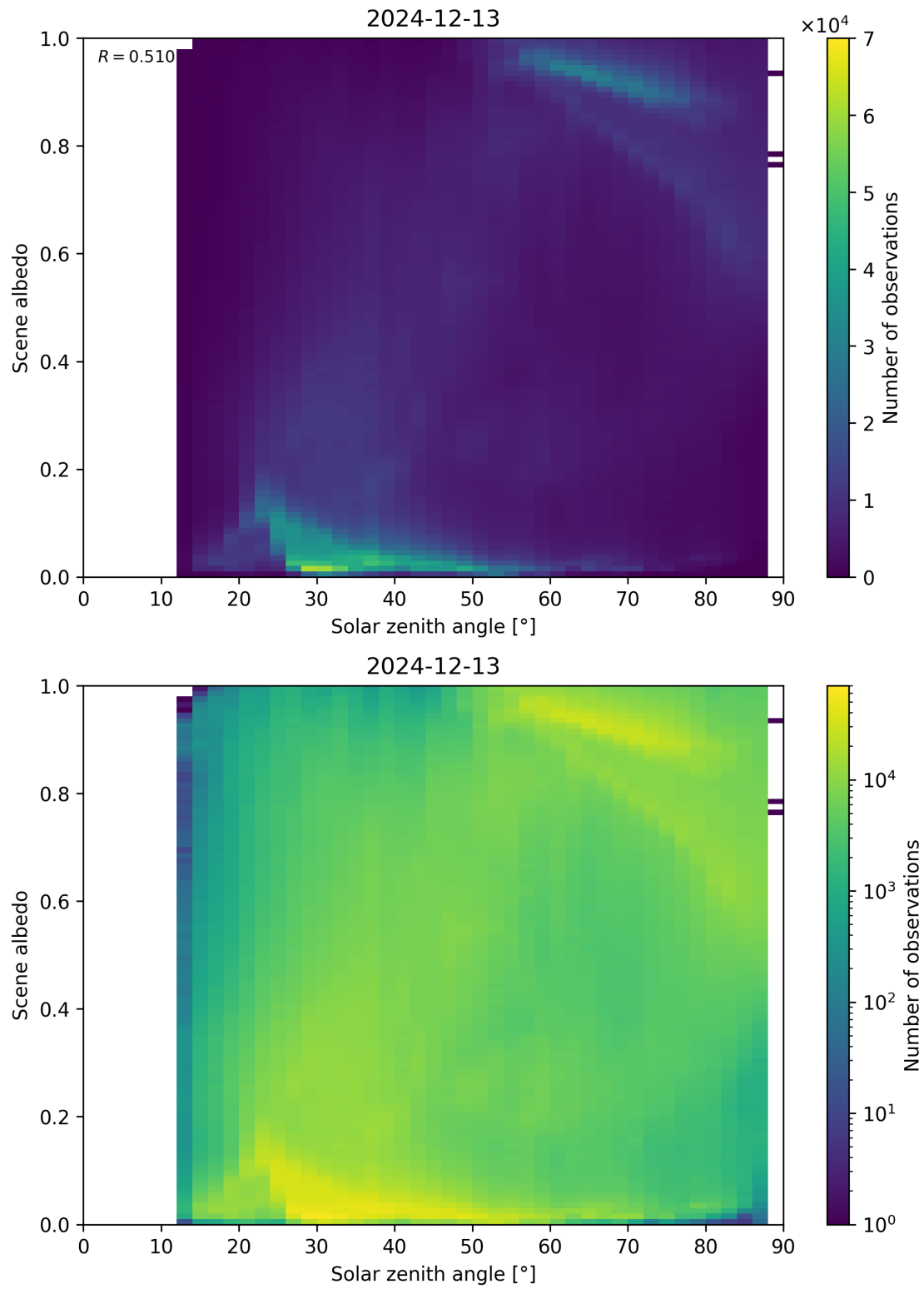
Figure 116: Scatter density plot of “Solar zenith angle” against “Scene albedo” for 2024-12-12 to 2024-12-14.
