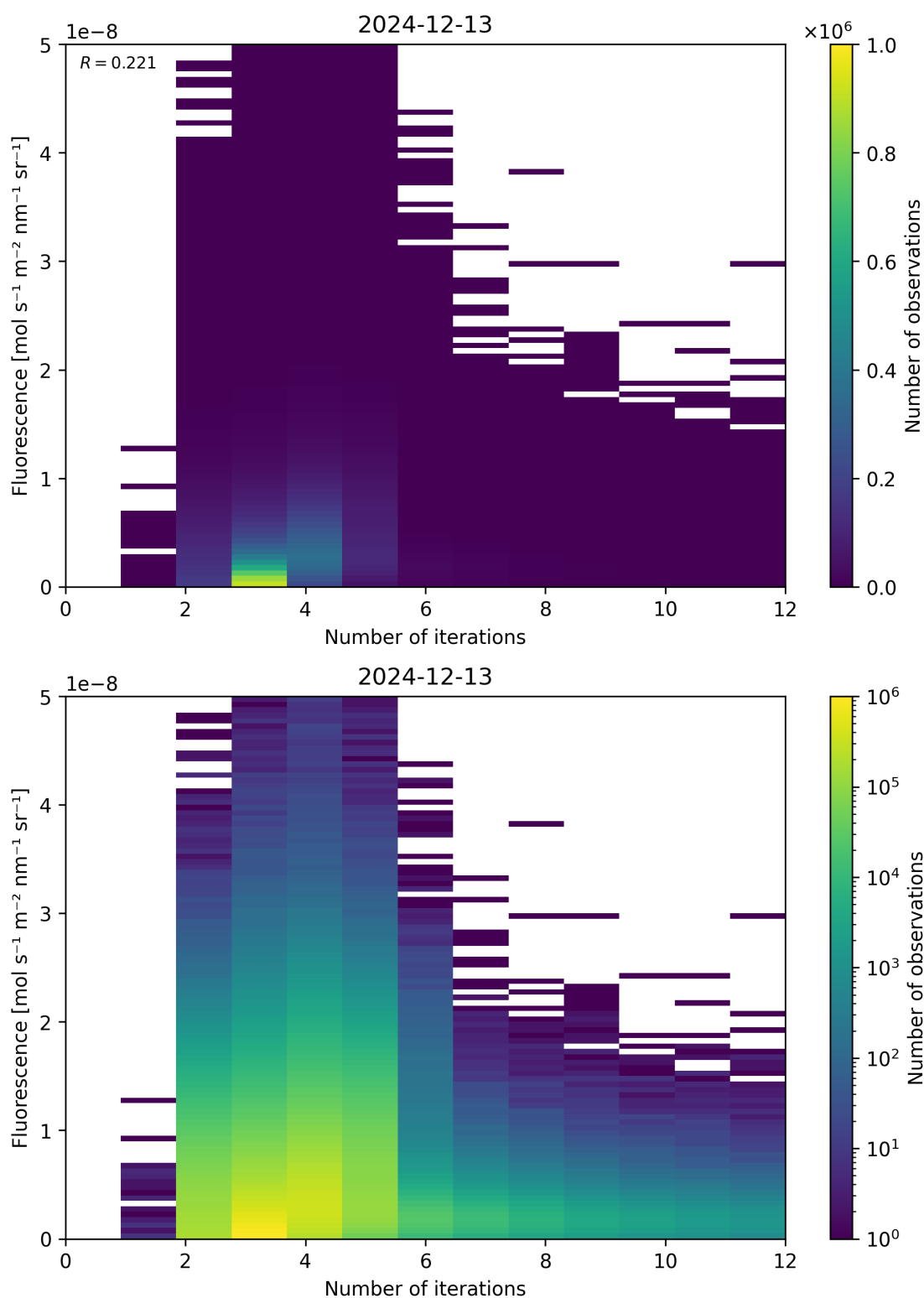
Figure 98: Scatter density plot of “Number of iterations” against “Fluorescence” for 2024-12-12 to 2024-12-14.
