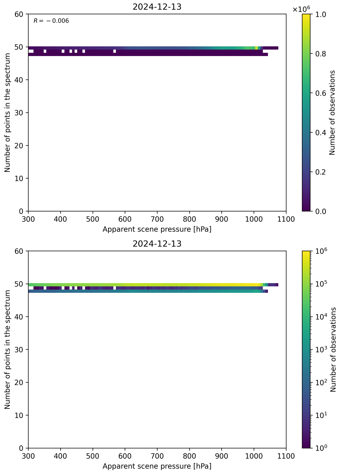
Figure 66: Scatter density plot of “Apparent scene pressure” against “Number of points in the spectrum” for 2024-12-12 to 2024-12-14.
