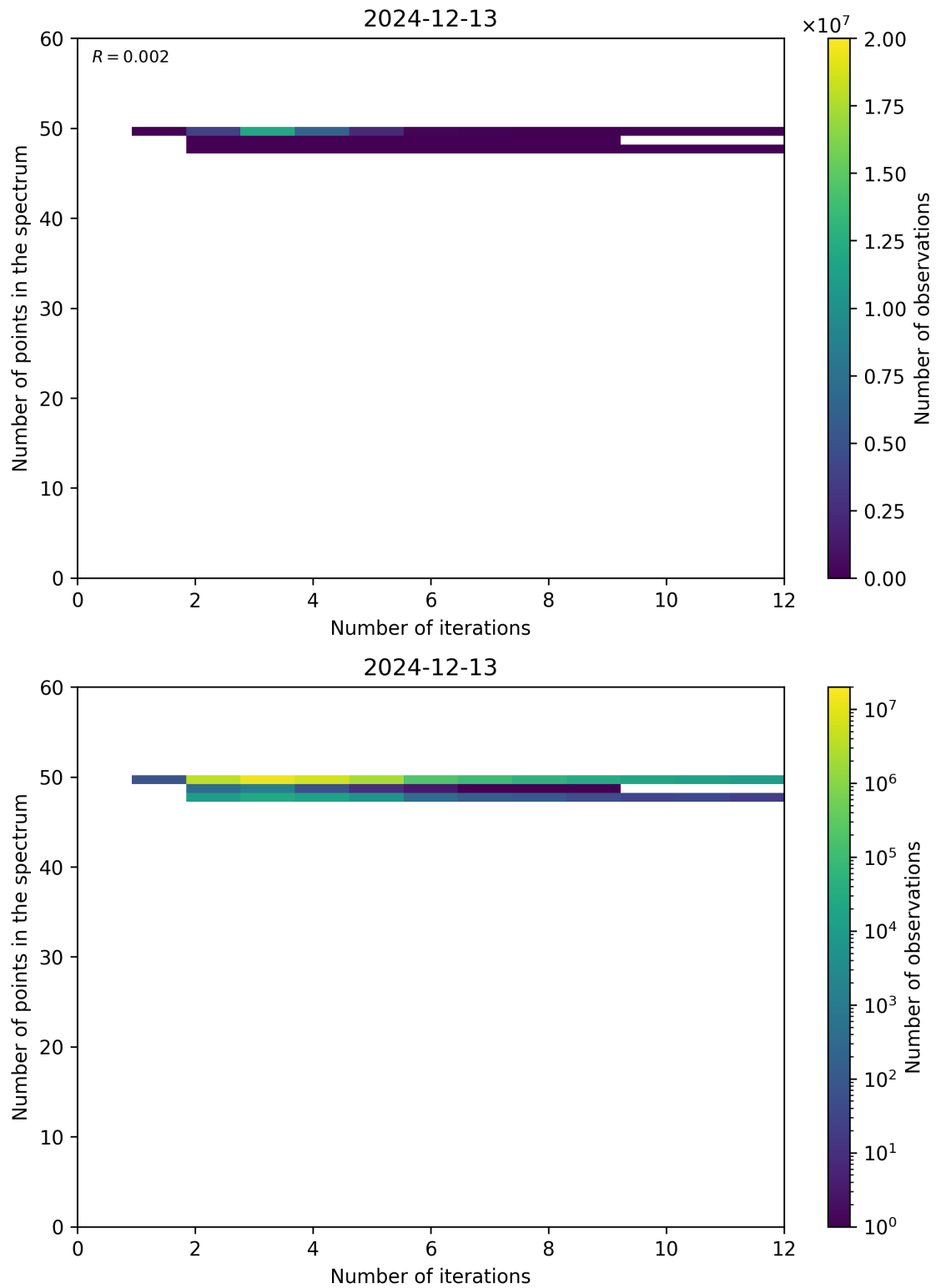
Figure 99: Scatter density plot of “Number of iterations” against “Number of points in the spectrum” for 2024-12-12 to 2024-12-14.
