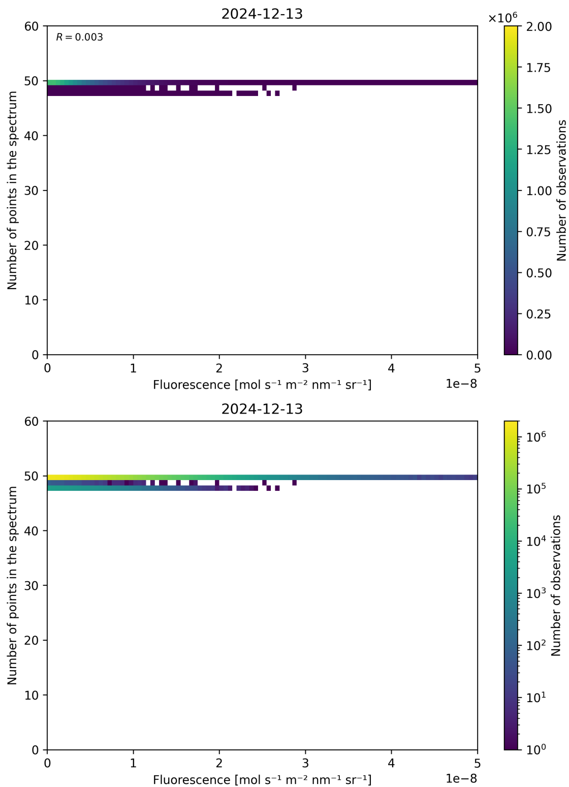
Figure 86: Scatter density plot of “Fluorescence” against “Number of points in the spectrum” for 2024-12-12 to 2024-12-14.
