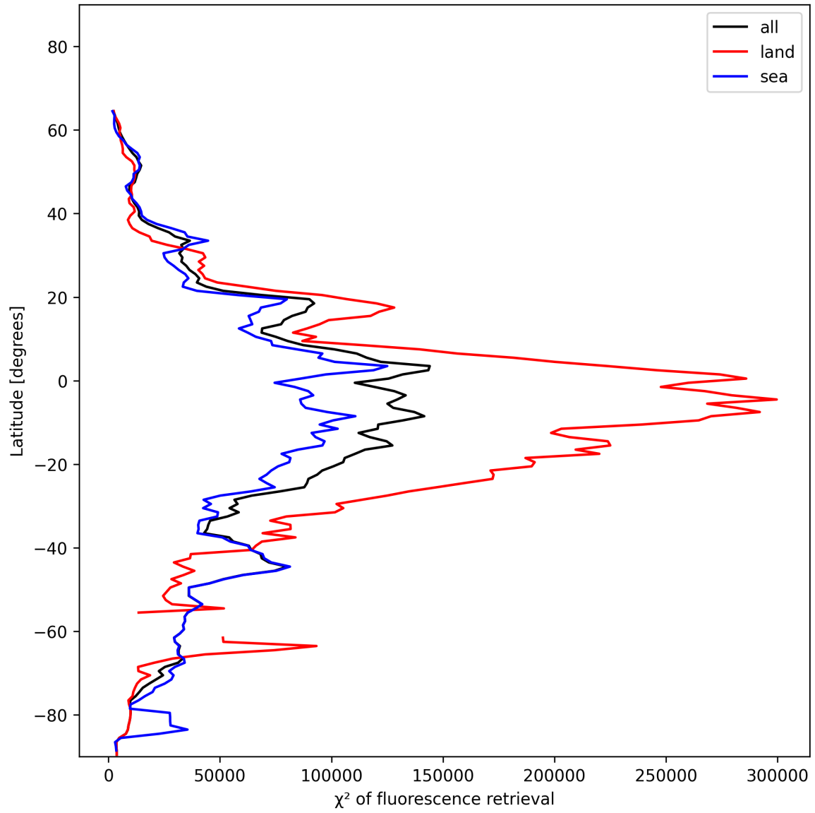
Figure 25: Zonal average of “ \chi^2 of fluorescence retrieval” for 2024-12-12 to 2024-12-14.
