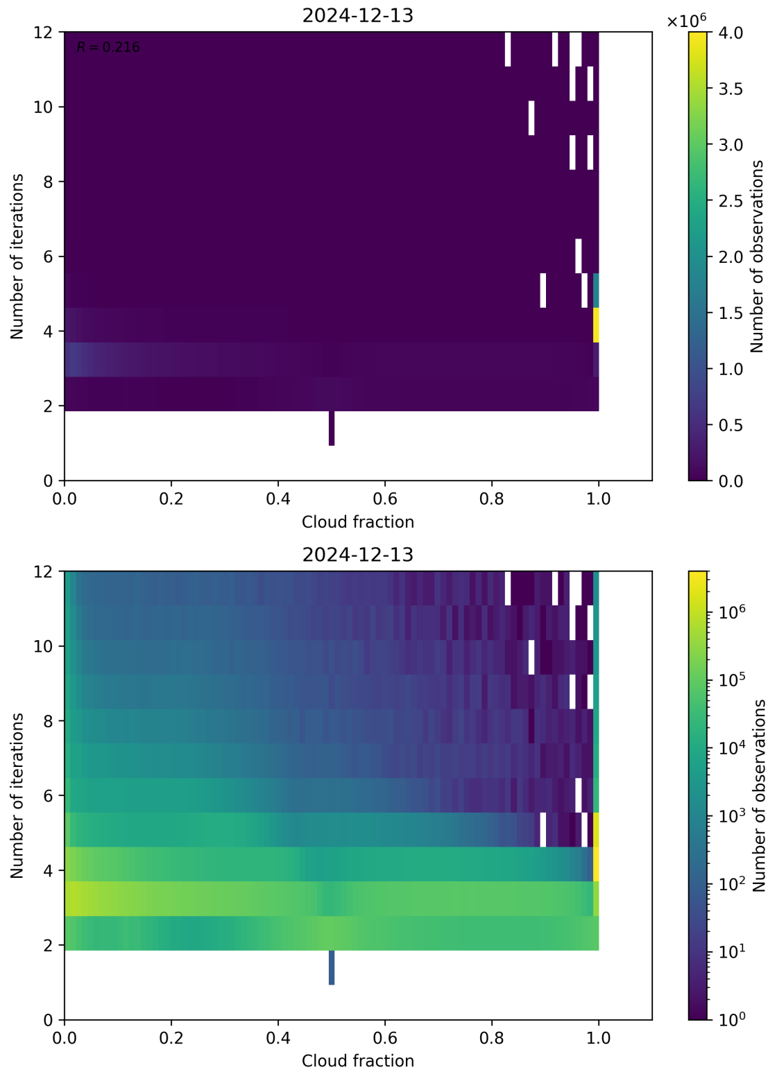
Figure 73: Scatter density plot of “Cloud fraction” against “Number of iterations” for 2024-12-12 to 2024-12-14.
