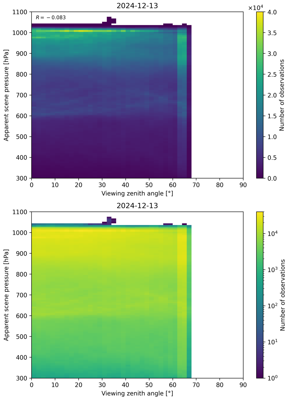
Figure 118: Scatter density plot of “Viewing zenith angle” against “Apparent scene pressure” for 2024-12-12 to 2024-12-14.
