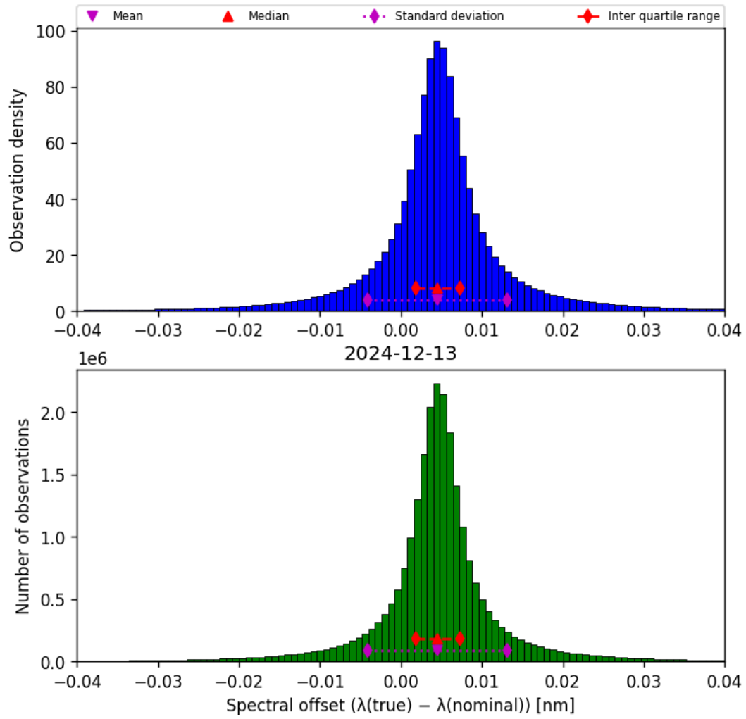
Figure 45: Histogram of “Spectral offset ( \lambda_{\text{true}} - \lambda_{\text{nominal}} )” for 2024-12-12 to 2024-12-14
