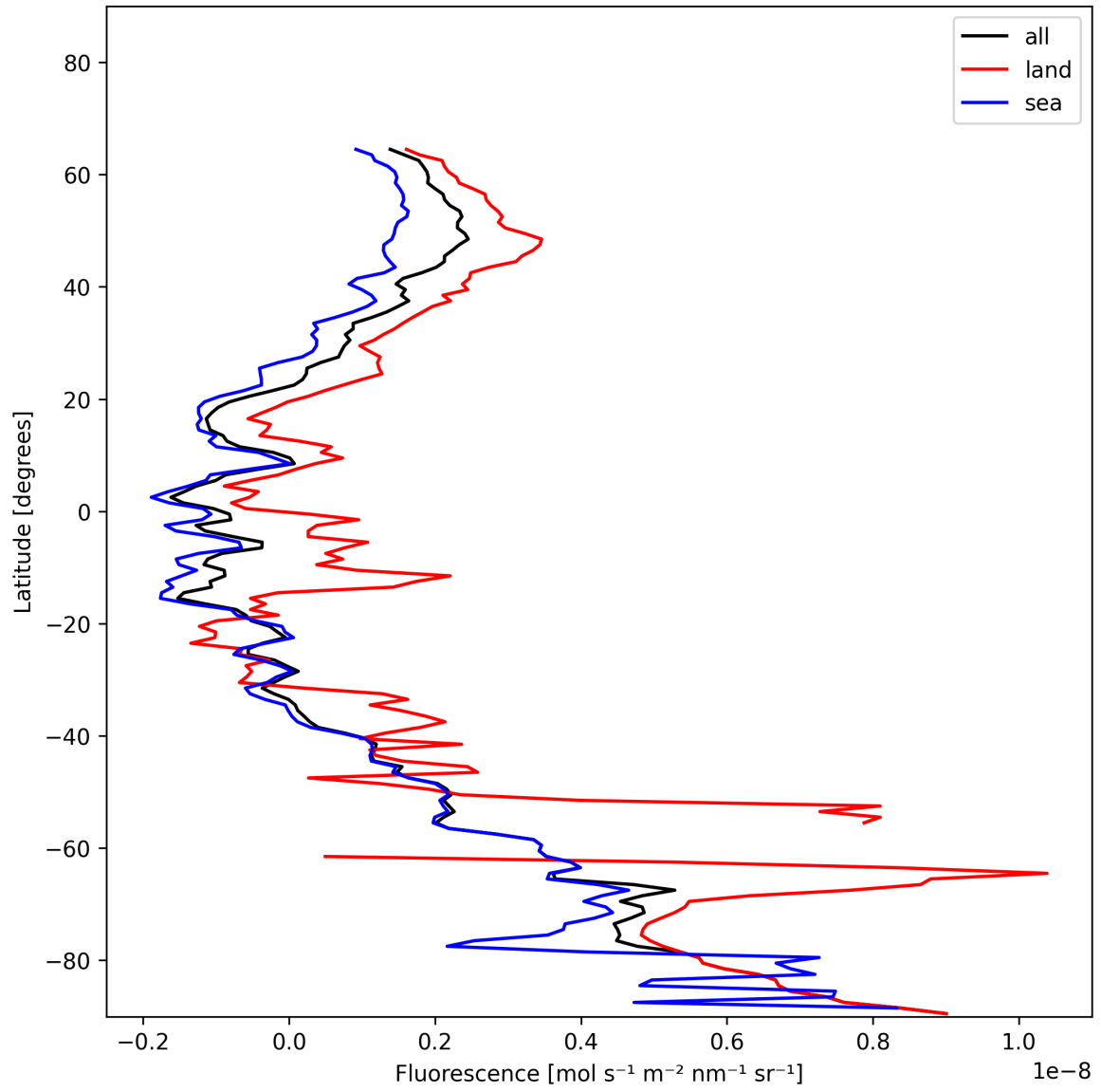
Figure 23: Zonal average of “Fluorescence” for 2024-12-12 to 2024-12-14.
