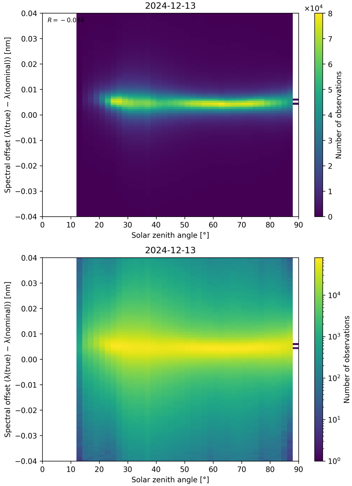
Figure 117: Scatter density plot of “Solar zenith angle” against “Spectral offset ( \lambda_{\text{true}} - \lambda_{\text{nominal}} )” for 2024-12-12 to 2024-12-14.
