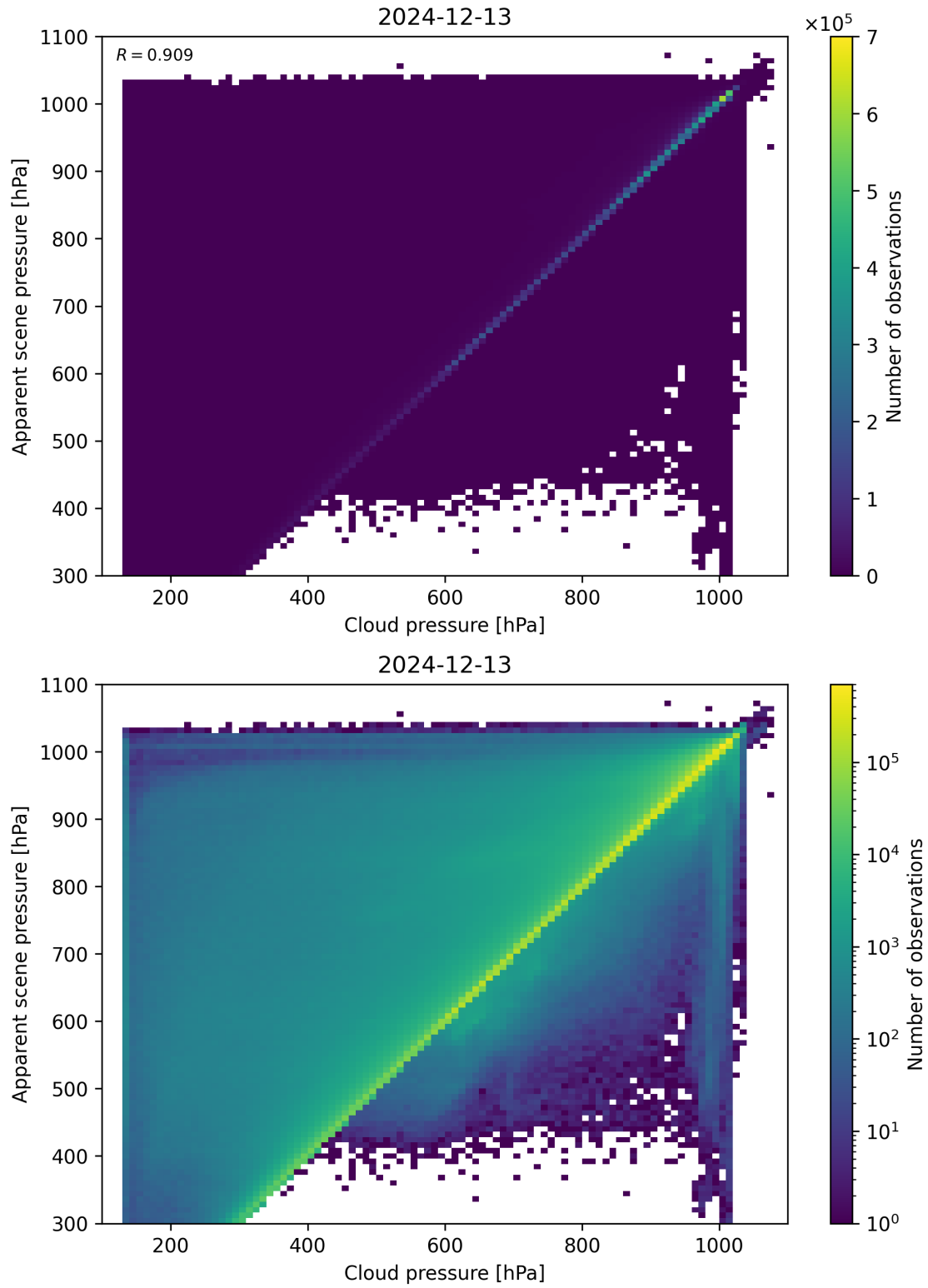
Figure 77: Scatter density plot of “Cloud pressure” against “Apparent scene pressure” for 2024-12-12 to 2024-12-14.
