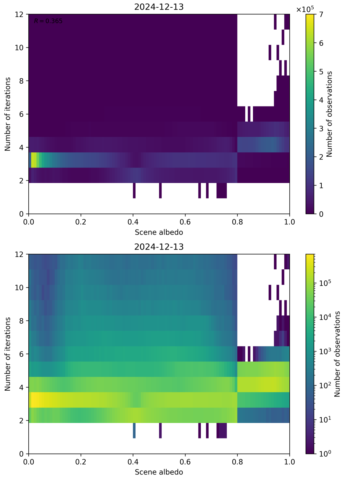
Figure 105: Scatter density plot of “Scene albedo” against “Number of iterations” for 2024-12-12 to 2024-12-14.
