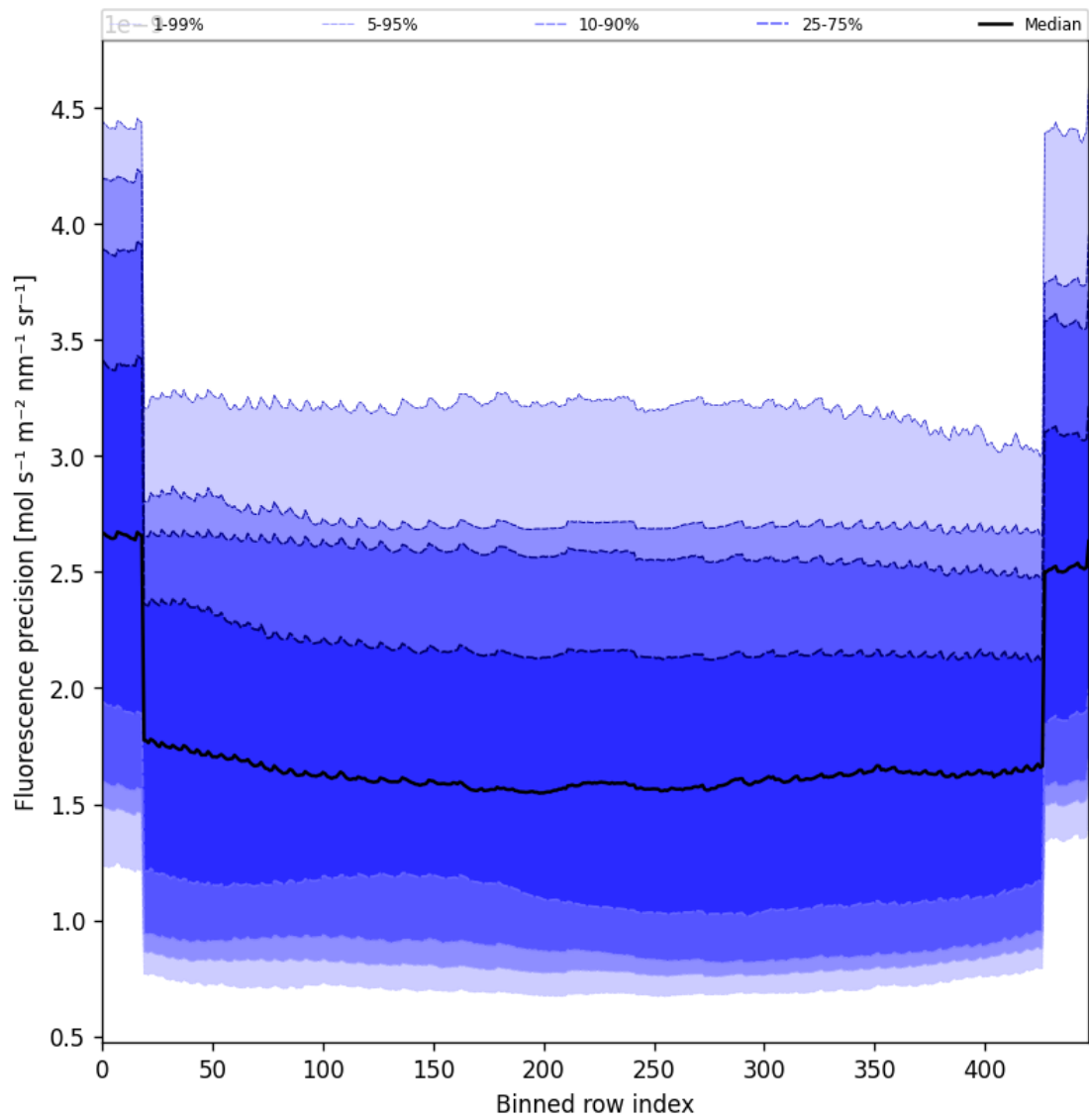
Figure 58: Along track statistics of “Fluorescence precision” for 2024-12-12 to 2024-12-14
