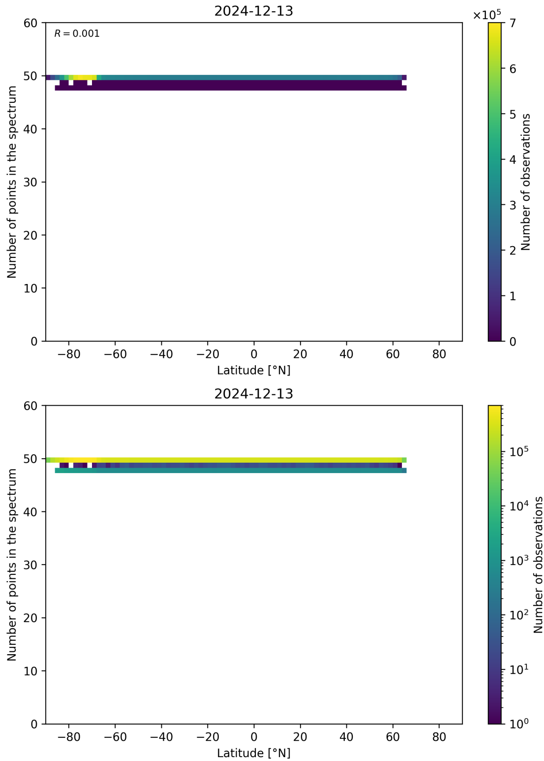
Figure 94: Scatter density plot of “Latitude” against “Number of points in the spectrum” for 2024-12-12 to 2024-12-14.
