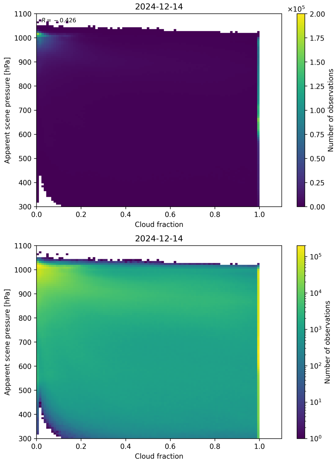
Figure 70: Scatter density plot of “Cloud fraction” against “Apparent scene pressure” for 2024-12-13 to 2024-12-15.
