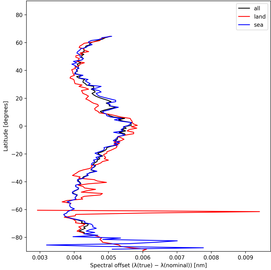
Figure 28: Zonal average of “Spectral offset ( \lambda_{\text{true}} - \lambda_{\text{nominal}} )” for 2024-12-13 to 2024-12-15.
