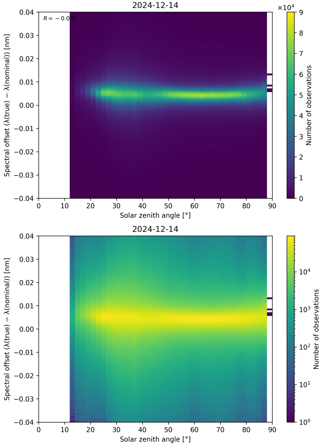
Figure 117: Scatter density plot of “Solar zenith angle” against “Spectral offset ( \lambda_{\text{true}} - \lambda_{\text{nominal}} )” for 2024-12-13 to 2024-12-15.
