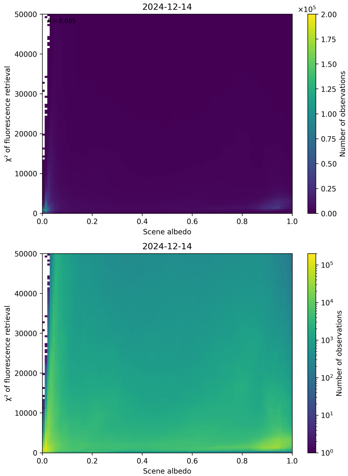
Figure 103: Scatter density plot of “Scene albedo” against “ \chi^2 of fluorescence retrieval” for 2024-12-13 to 2024-12-15.
