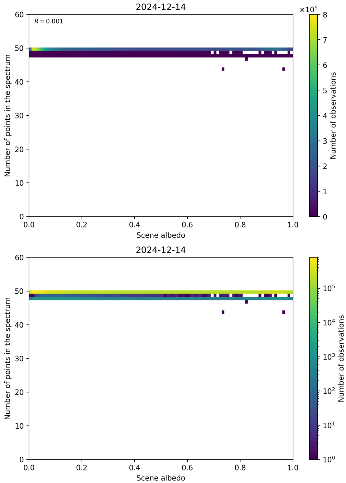
Figure 106: Scatter density plot of “Scene albedo” against “Number of points in the spectrum” for 2024-12-13 to 2024-12-15.
