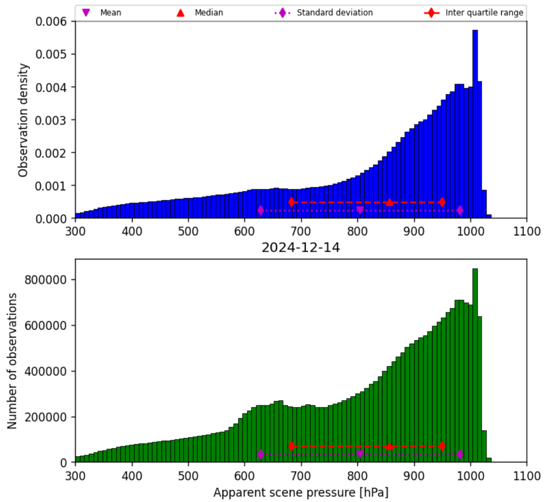
Figure 36: Histogram of “Apparent scene pressure” for 2024-12-13 to 2024-12-15
