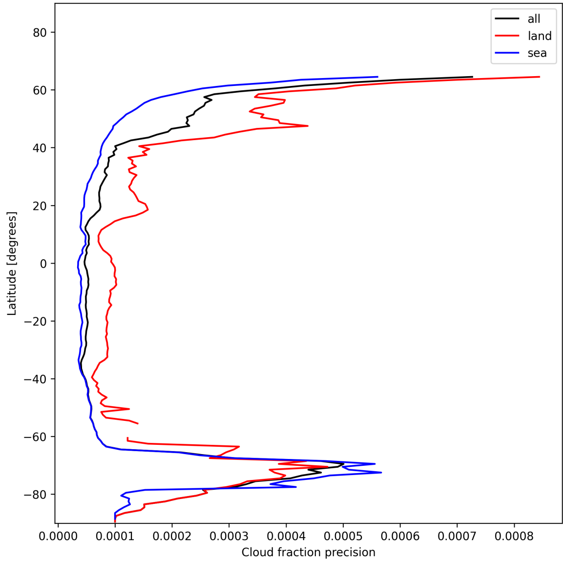
Figure 16: Zonal average of “Cloud fraction precision” for 2024-12-13 to 2024-12-15.
