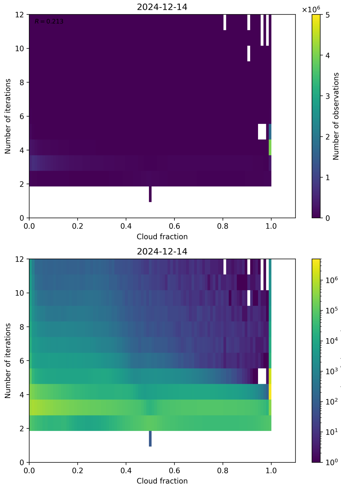
Figure 73: Scatter density plot of “Cloud fraction” against “Number of iterations” for 2024-12-13 to 2024-12-15.
