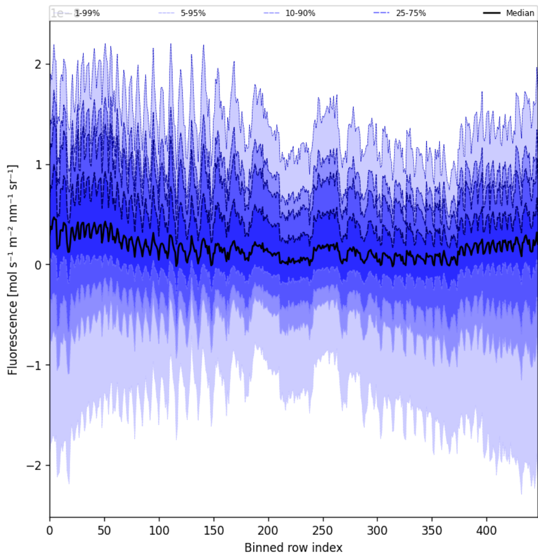
Figure 57: Along track statistics of “Fluorescence” for 2024-12-13 to 2024-12-15
