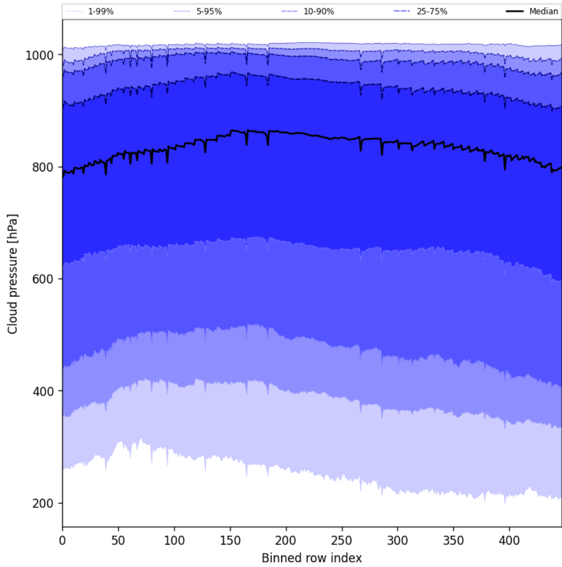
Figure 47: Along track statistics of “Cloud pressure” for 2024-12-13 to 2024-12-15
