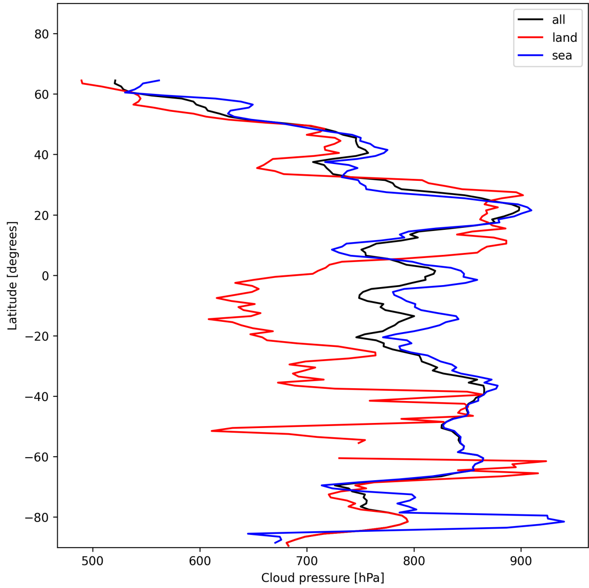
Figure 13: Zonal average of “Cloud pressure” for 2024-12-13 to 2024-12-15.
