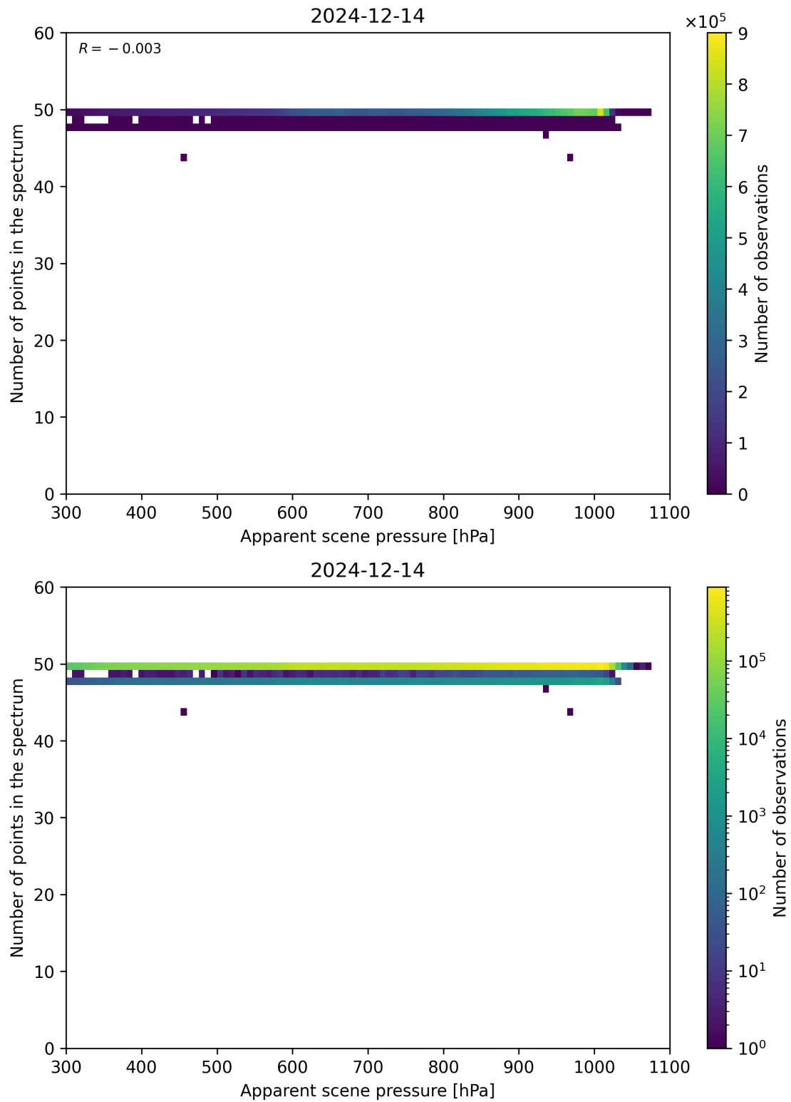
Figure 66: Scatter density plot of “Apparent scene pressure” against “Number of points in the spectrum” for 2024-12-13 to 2024-12-15.
