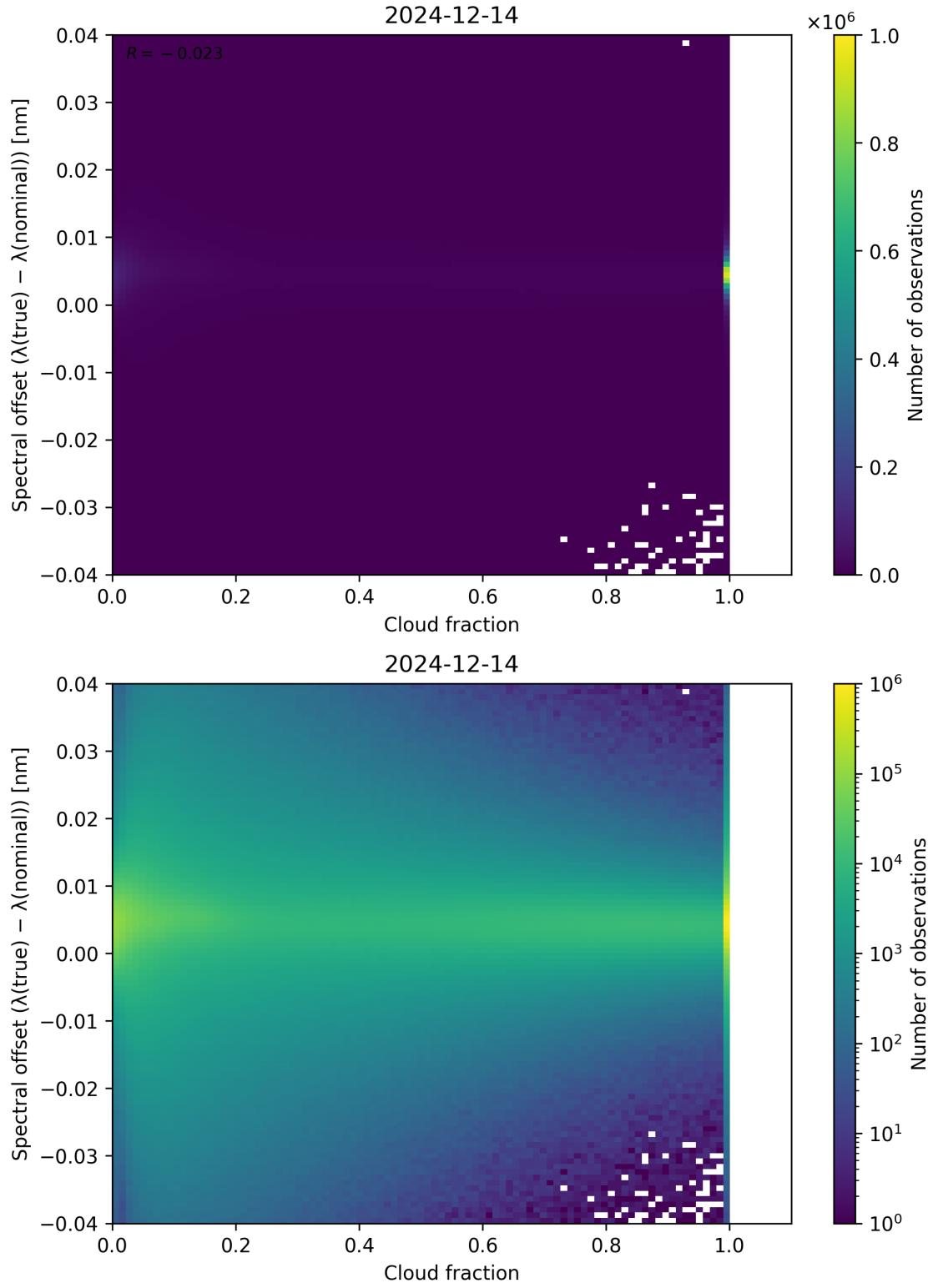
Figure 76: Scatter density plot of “Cloud fraction” against “Spectral offset ( \lambda_{\text{true}} - \lambda_{\text{nominal}} )” for 2024-12-13 to 2024-12-15.
