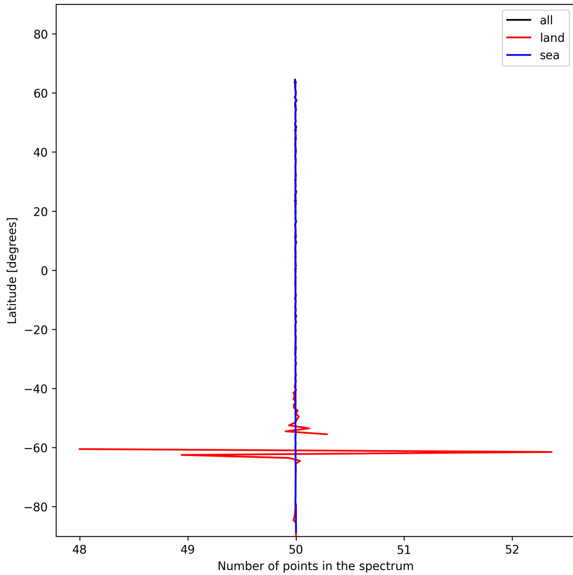
Figure 27: Zonal average of “Number of points in the spectrum” for 2024-12-13 to 2024-12-15.
