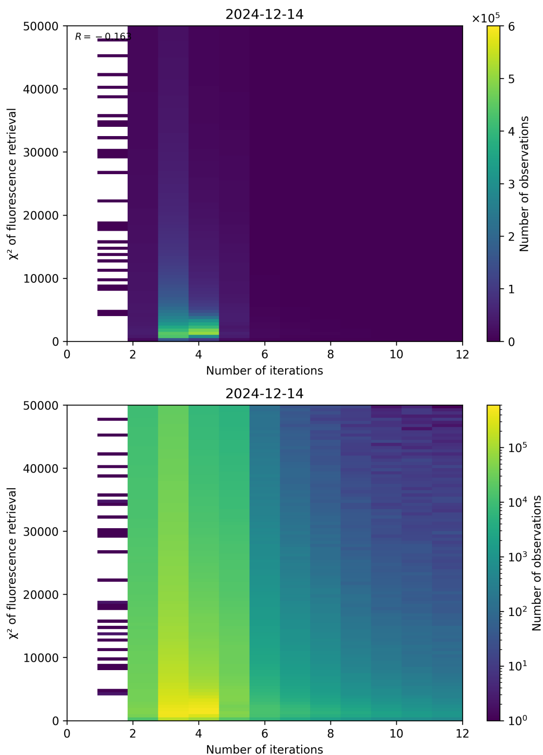
Figure 97: Scatter density plot of “Number of iterations” against “ \chi^2 of fluorescence retrieval” for 2024-12-13 to 2024-12-15.
