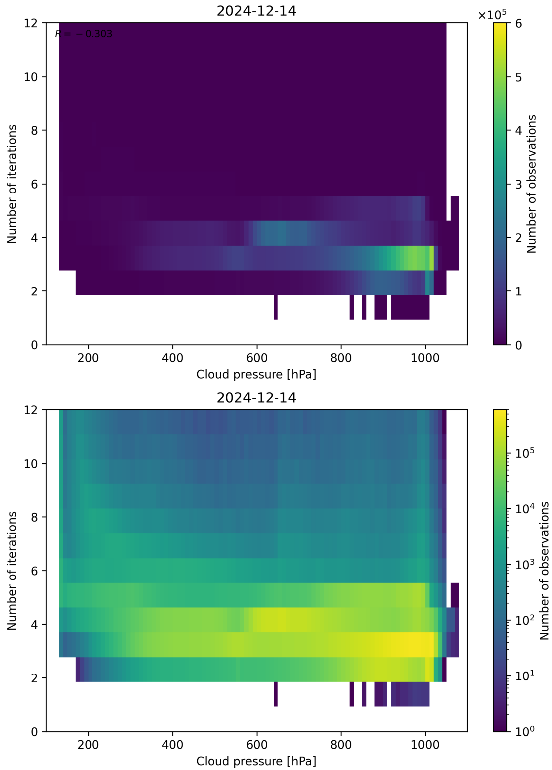
Figure 81: Scatter density plot of “Cloud pressure” against “Number of iterations” for 2024-12-13 to 2024-12-15.
