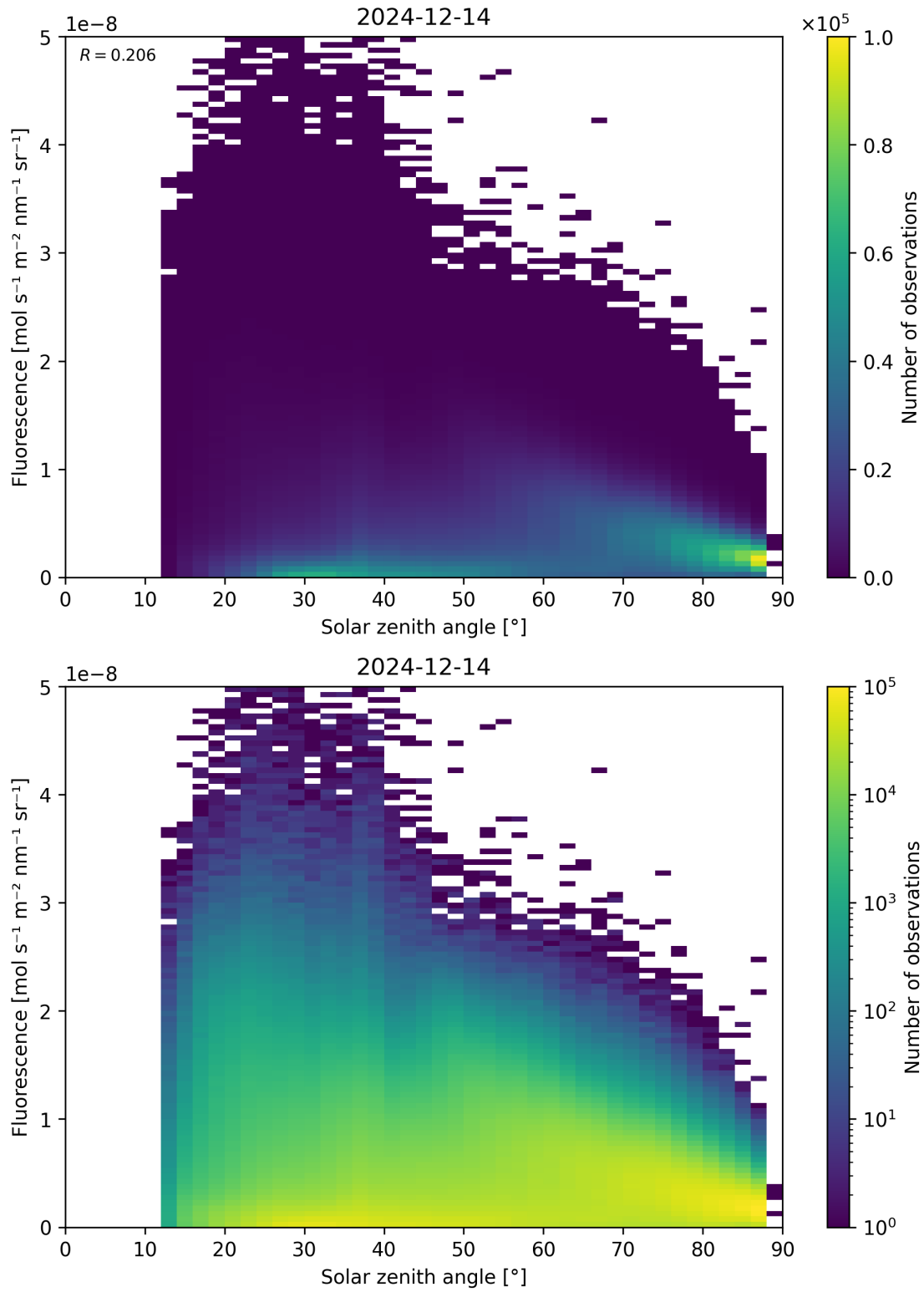
Figure 112: Scatter density plot of “Solar zenith angle” against “Fluorescence” for 2024-12-13 to 2024-12-15.
