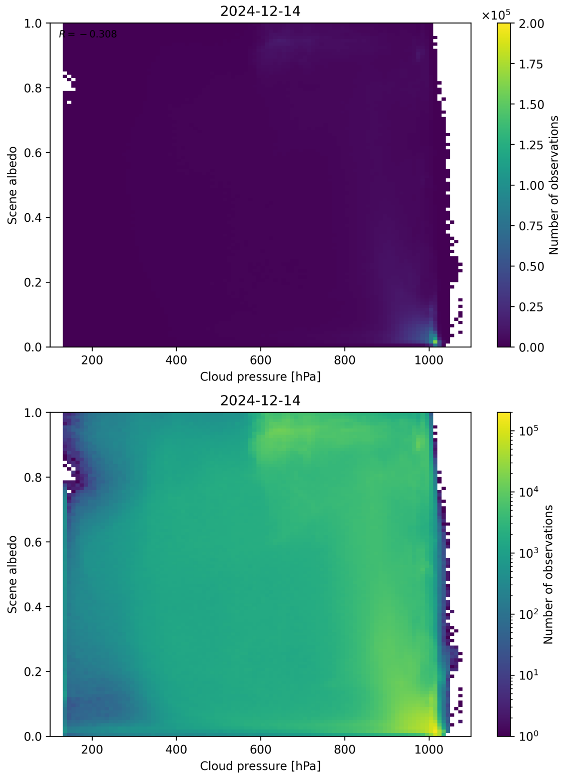
Figure 83: Scatter density plot of “Cloud pressure” against “Scene albedo” for 2024-12-13 to 2024-12-15.
