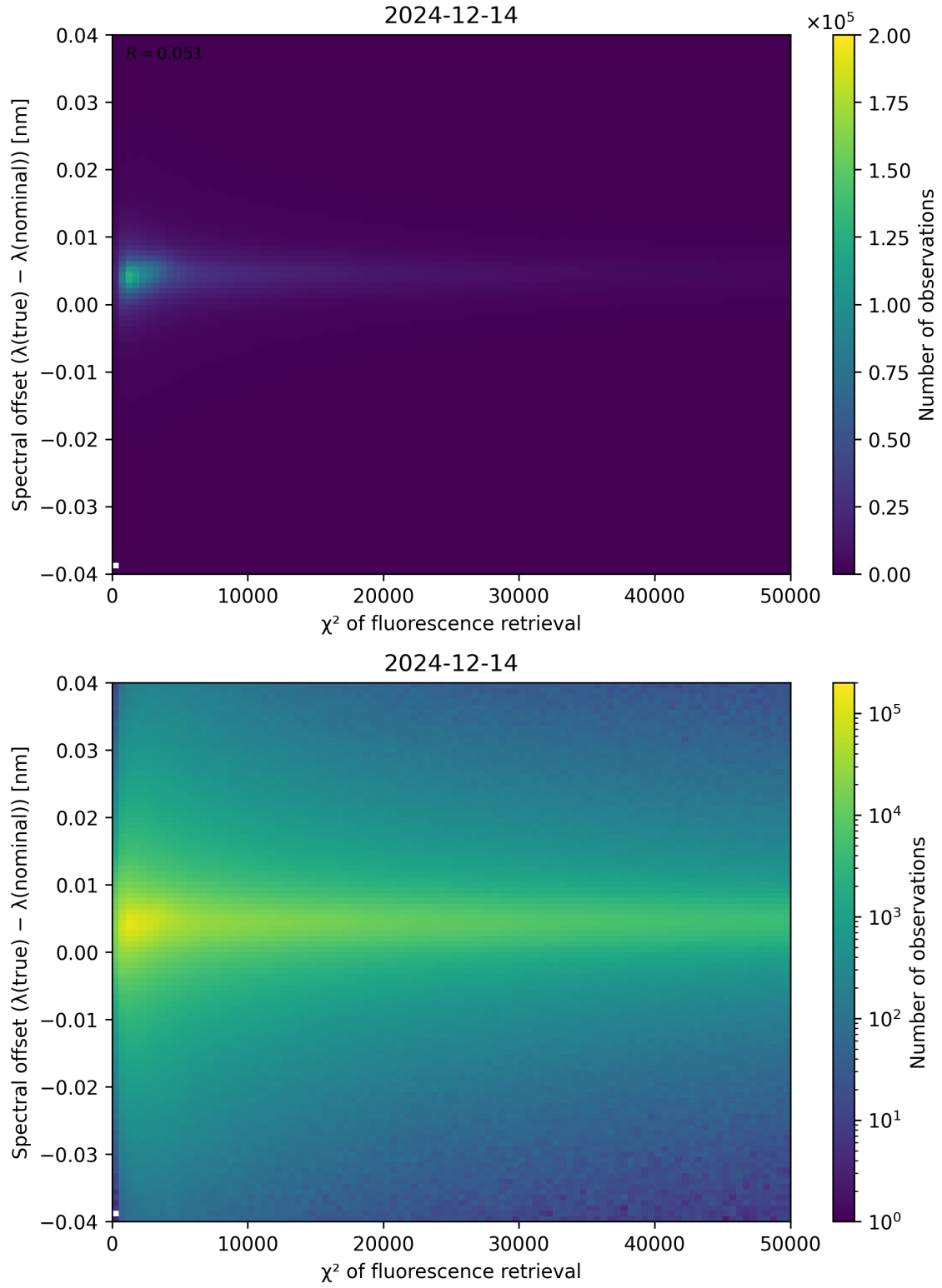
Figure 69: Scatter density plot of “ \chi^2 of fluorescence retrieval” against “Spectral offset ( \lambda_{\text{true}} - \lambda_{\text{nominal}} )” for 2024-12-13 to 2024-12-15.
