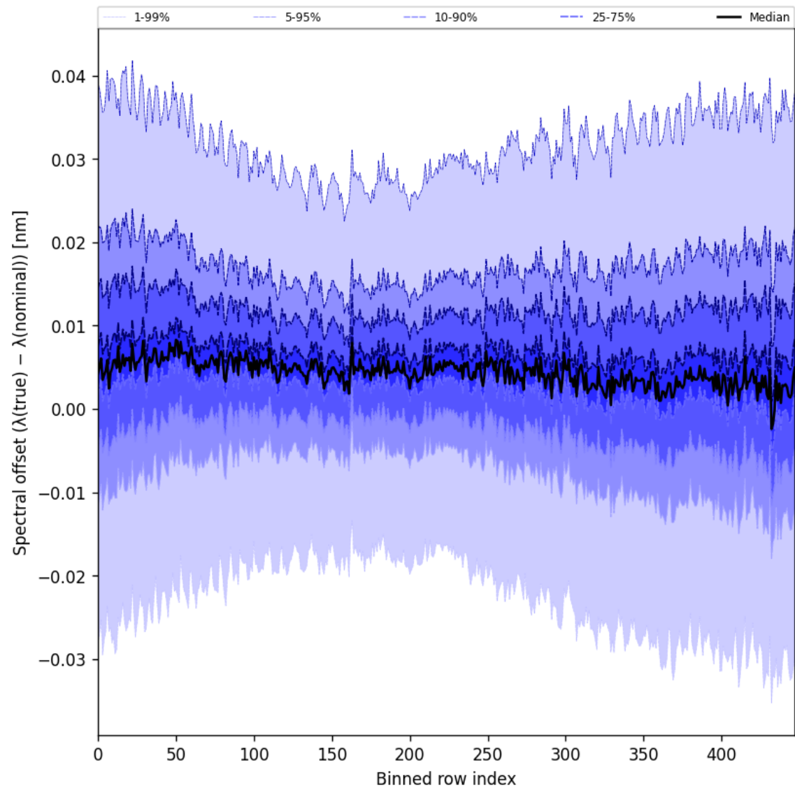
Figure 62: Along track statistics of “Spectral offset ( \lambda_{\text{true}} - \lambda_{\text{nominal}} )” for 2024-12-13 to 2024-12-15
