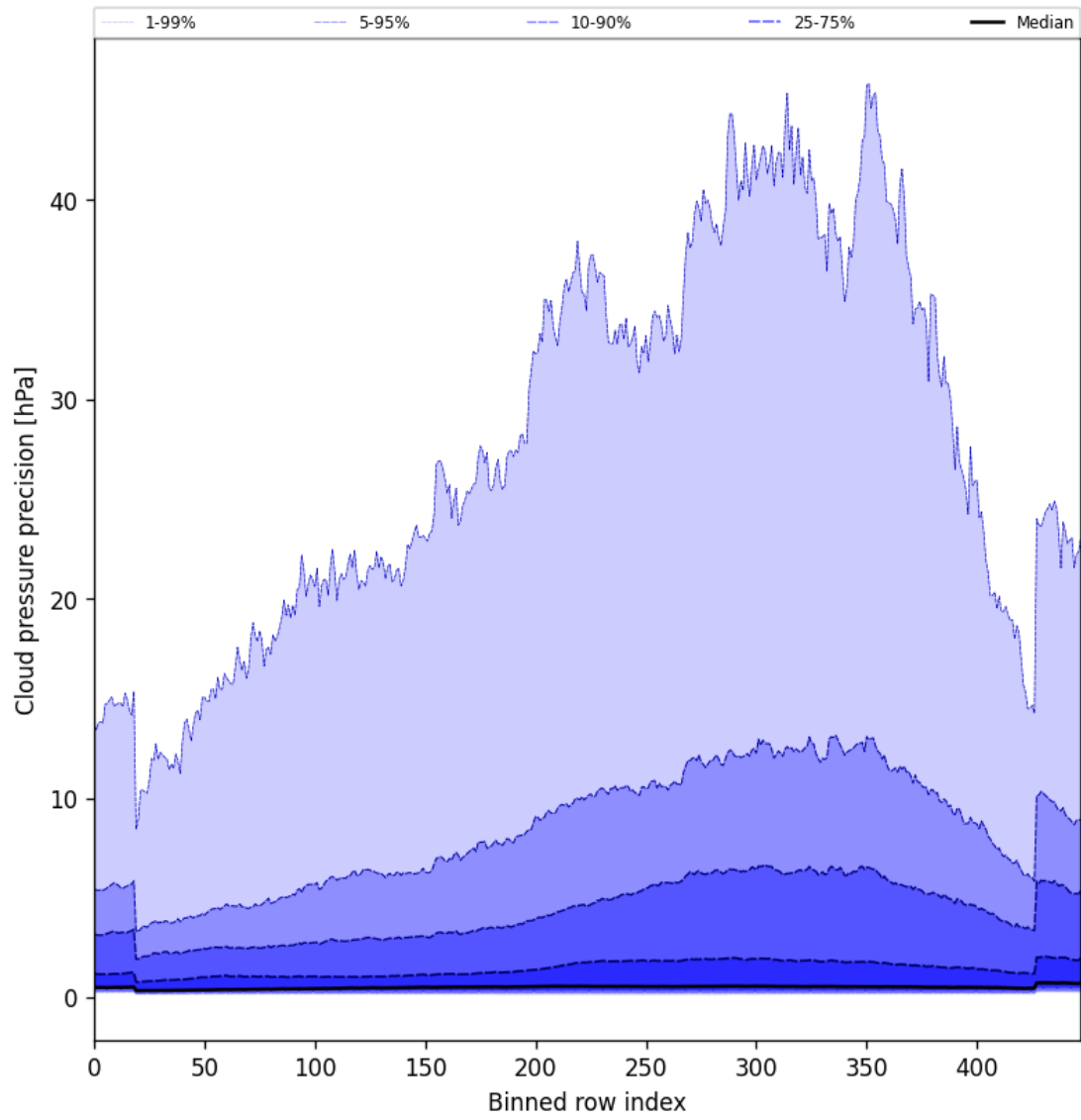
Figure 48: Along track statistics of “Cloud pressure precision” for 2024-12-13 to 2024-12-15
