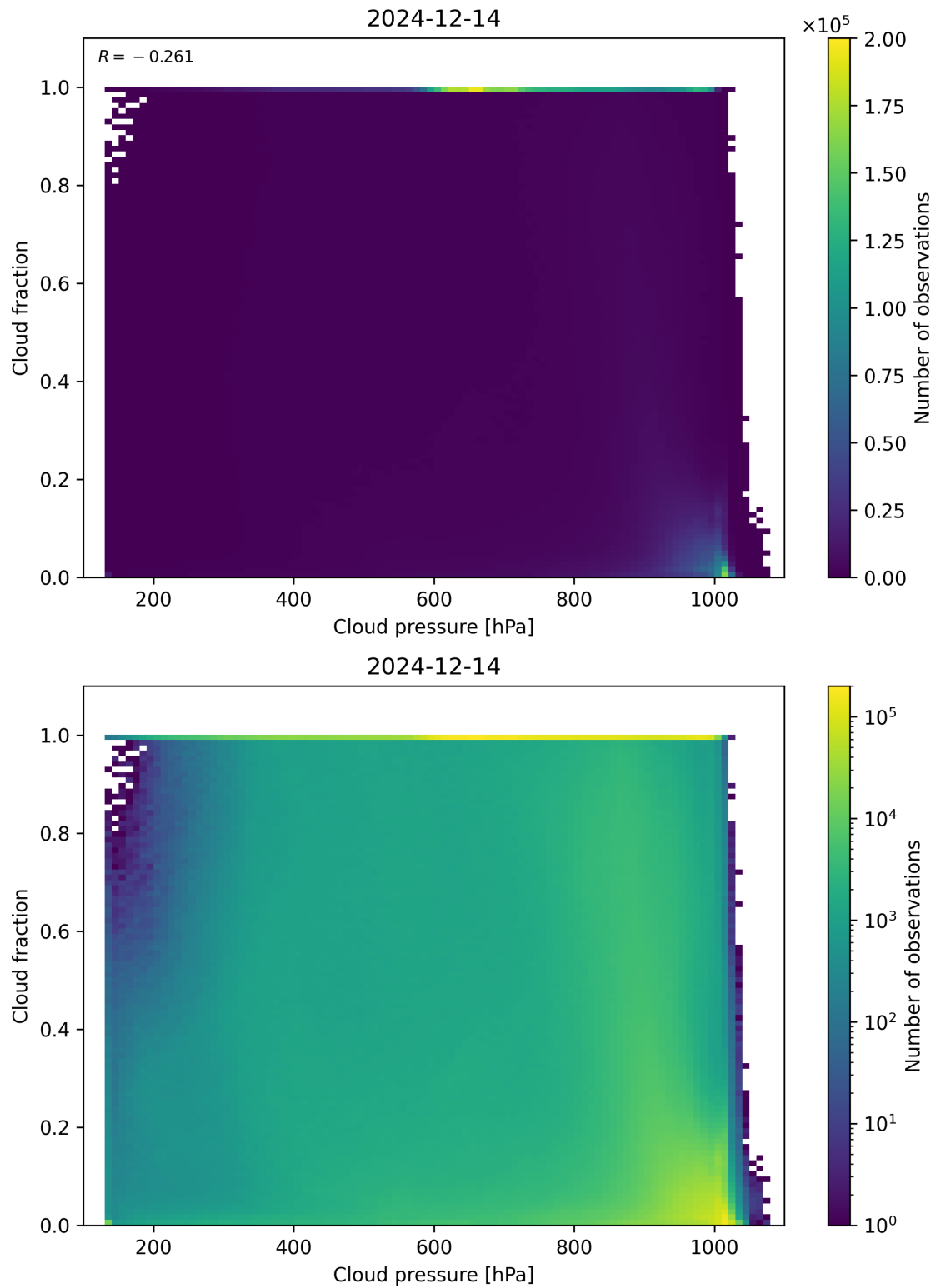
Figure 79: Scatter density plot of “Cloud pressure” against “Cloud fraction” for 2024-12-13 to 2024-12-15.
