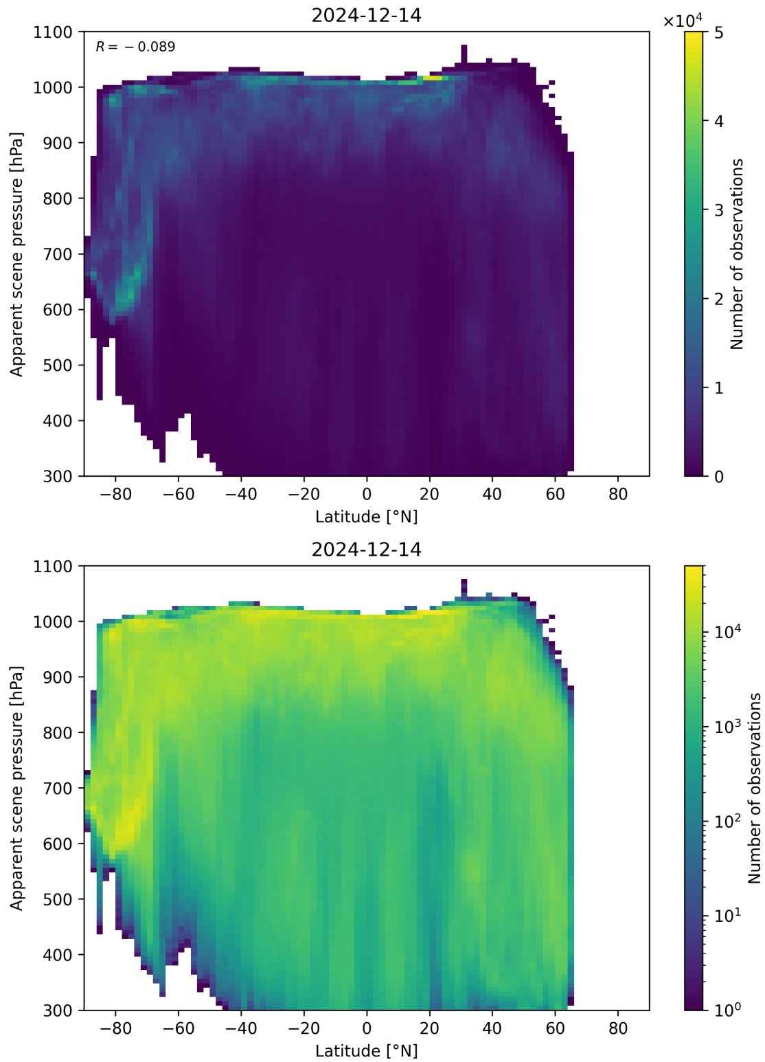
Figure 88: Scatter density plot of “Latitude” against “Apparent scene pressure” for 2024-12-13 to 2024-12-15.
