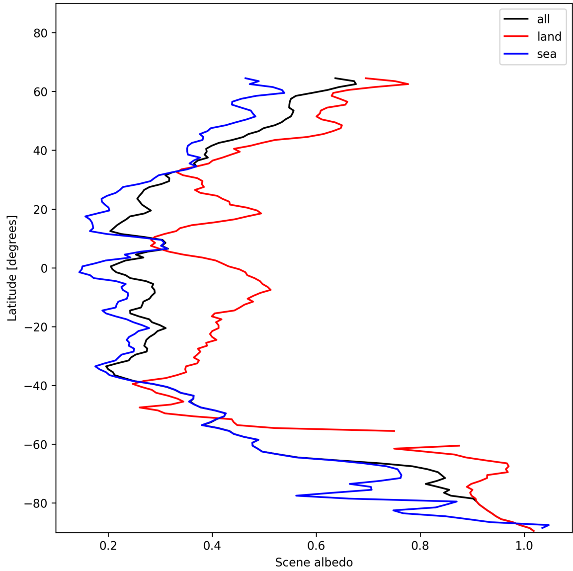
Figure 17: Zonal average of "Scene albedo" for 2024-12-13 to 2024-12-15.
