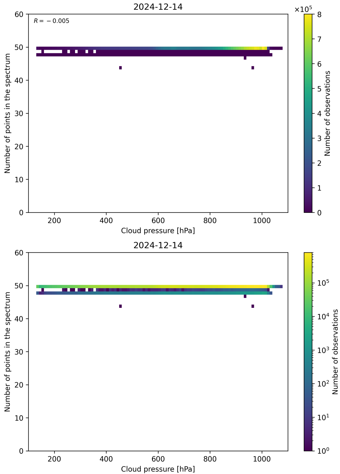
Figure 82: Scatter density plot of “Cloud pressure” against “Number of points in the spectrum” for 2024-12-13 to 2024-12-15.
