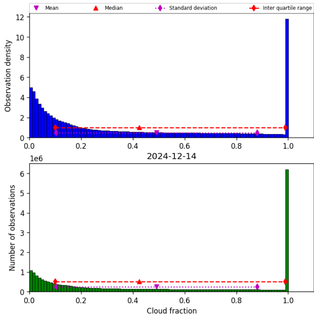
Figure 32: Histogram of “Cloud fraction” for 2024-12-13 to 2024-12-15
