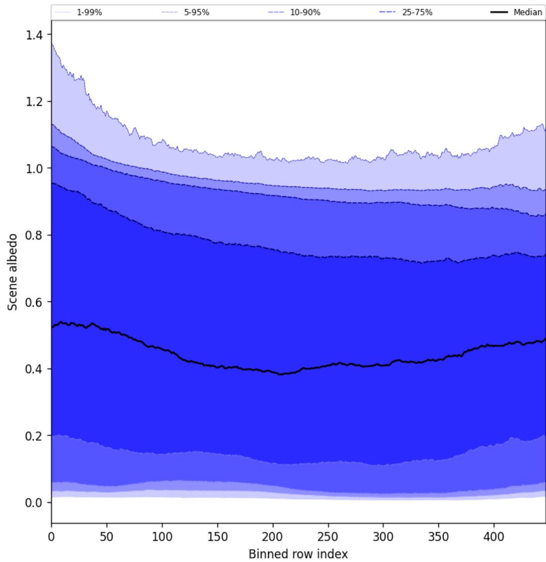
Figure 51: Along track statistics of "Scene albedo" for 2024-12-13 to 2024-12-15
