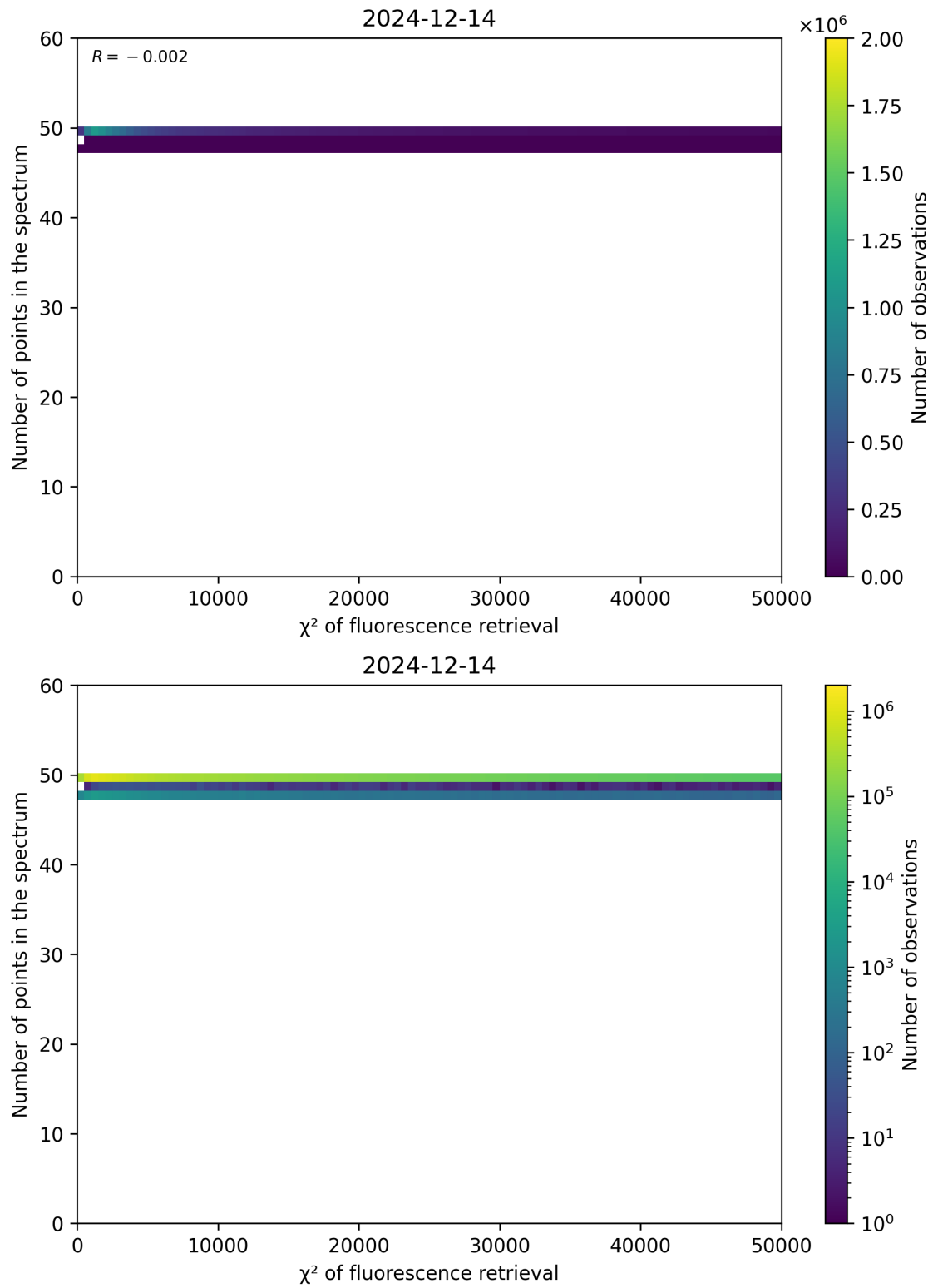
Figure 68: Scatter density plot of “ \chi^2 of fluorescence retrieval” against “Number of points in the spectrum” for 2024-12-13 to 2024-12-15.
