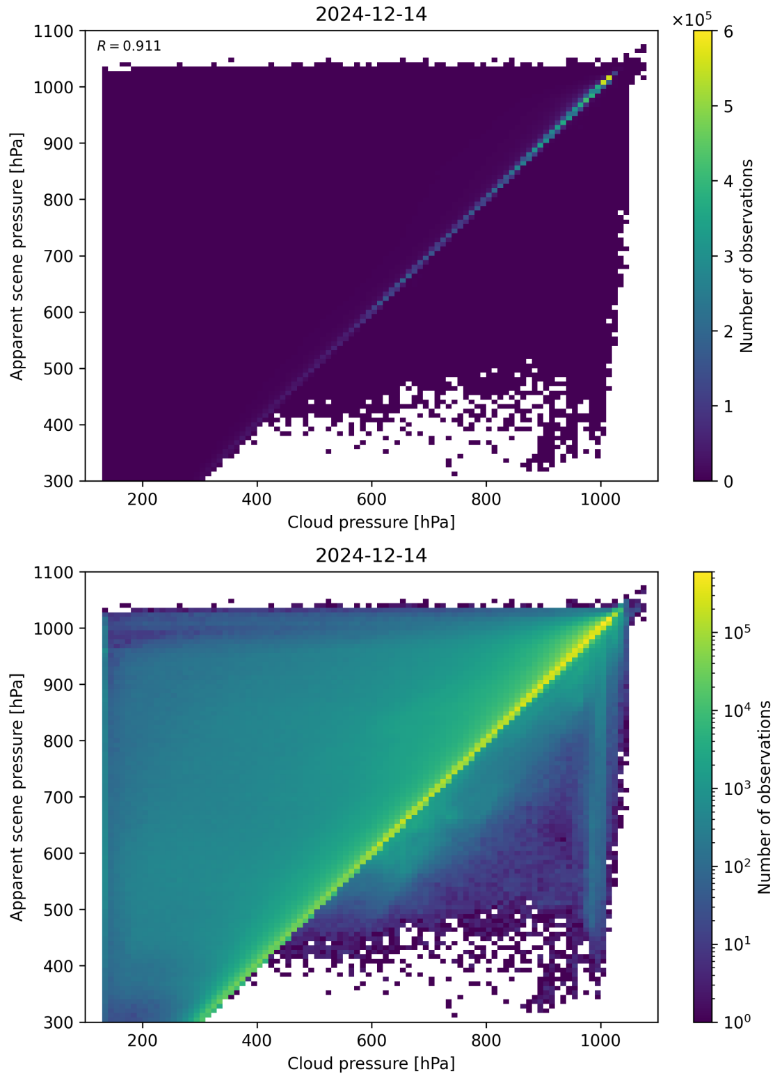
Figure 77: Scatter density plot of “Cloud pressure” against “Apparent scene pressure” for 2024-12-13 to 2024-12-15.
