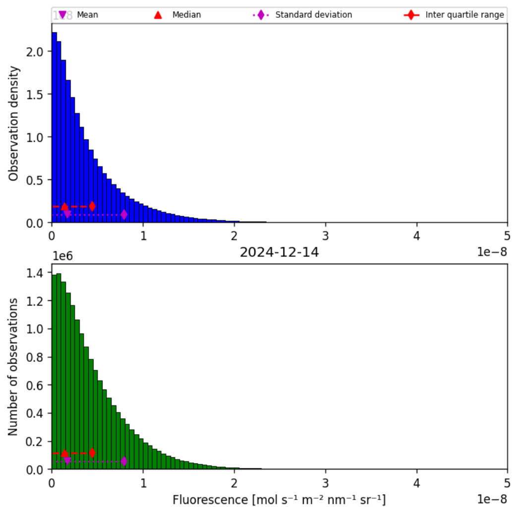
Figure 40: Histogram of “Fluorescence” for 2024-12-13 to 2024-12-15
