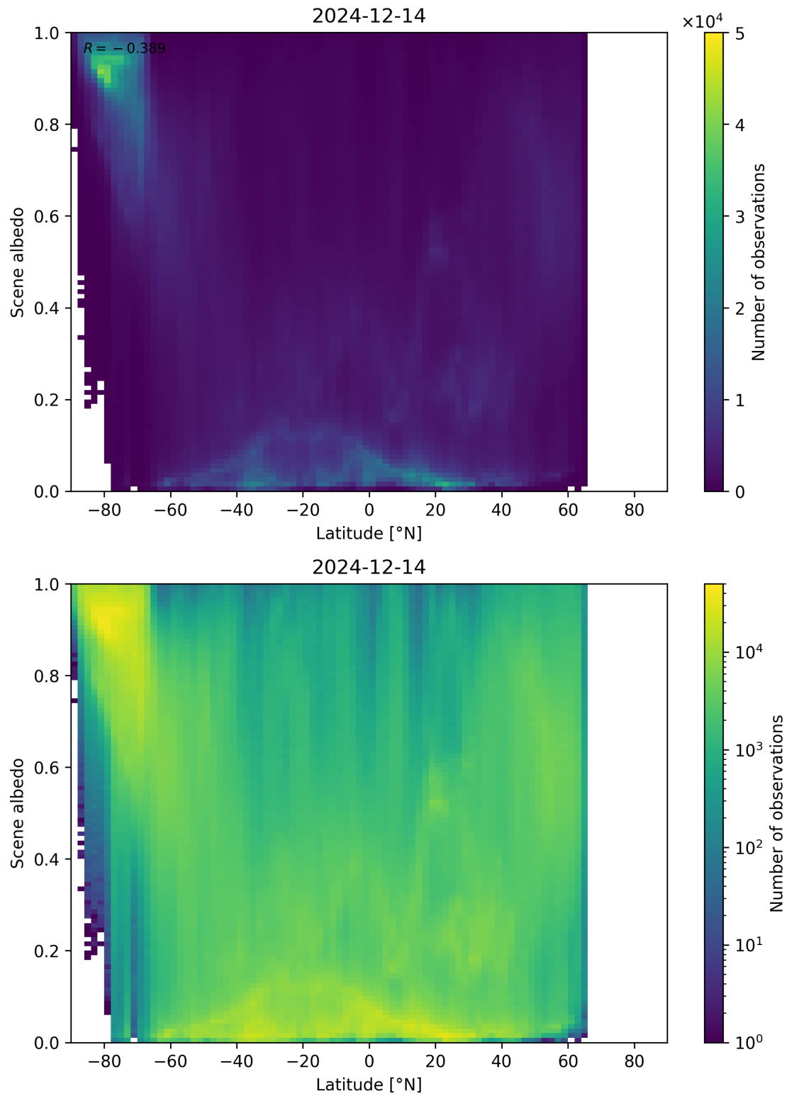
Figure 95: Scatter density plot of “Latitude” against “Scene albedo” for 2024-12-13 to 2024-12-15.
