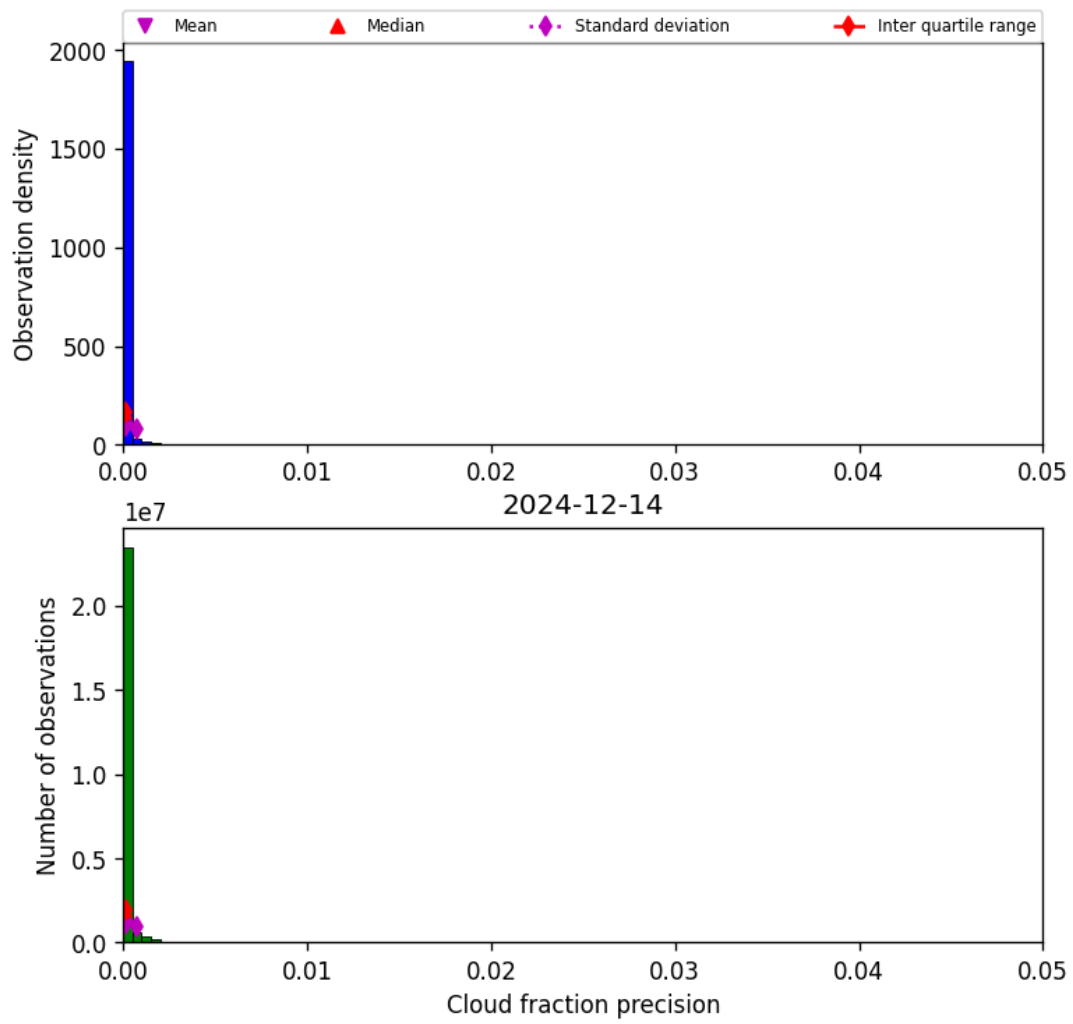
Figure 33: Histogram of “Cloud fraction precision” for 2024-12-13 to 2024-12-15
