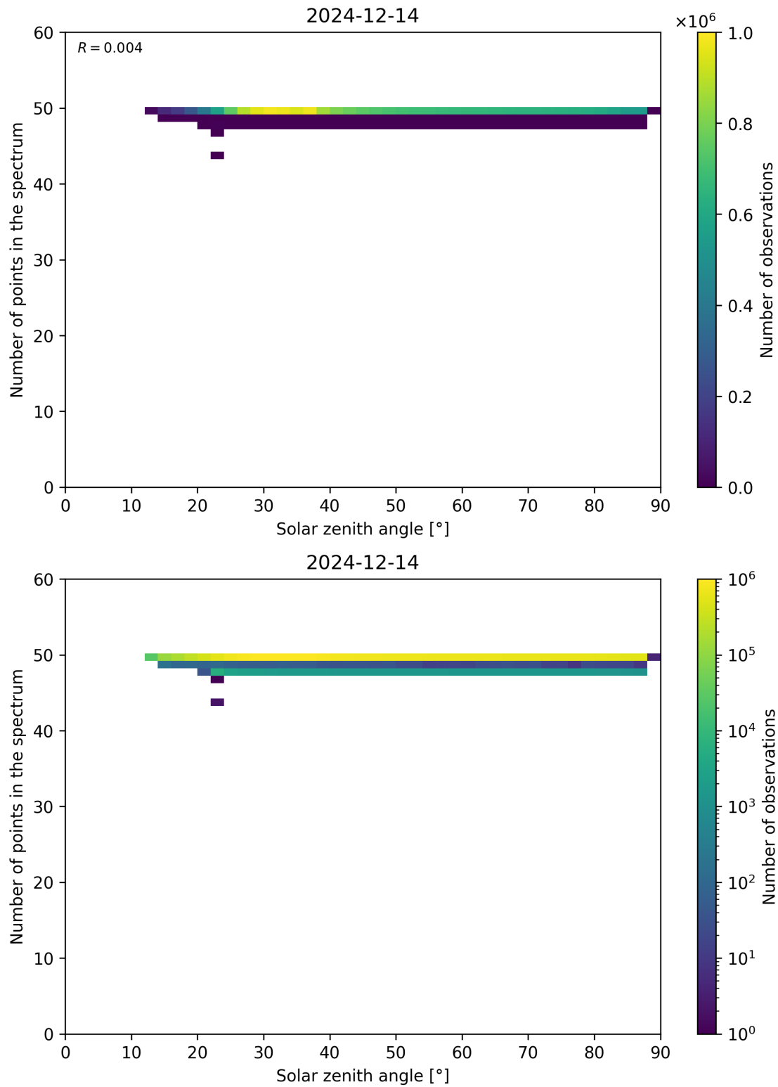
Figure 115: Scatter density plot of “Solar zenith angle” against “Number of points in the spectrum” for 2024-12-13 to 2024-12-15.
