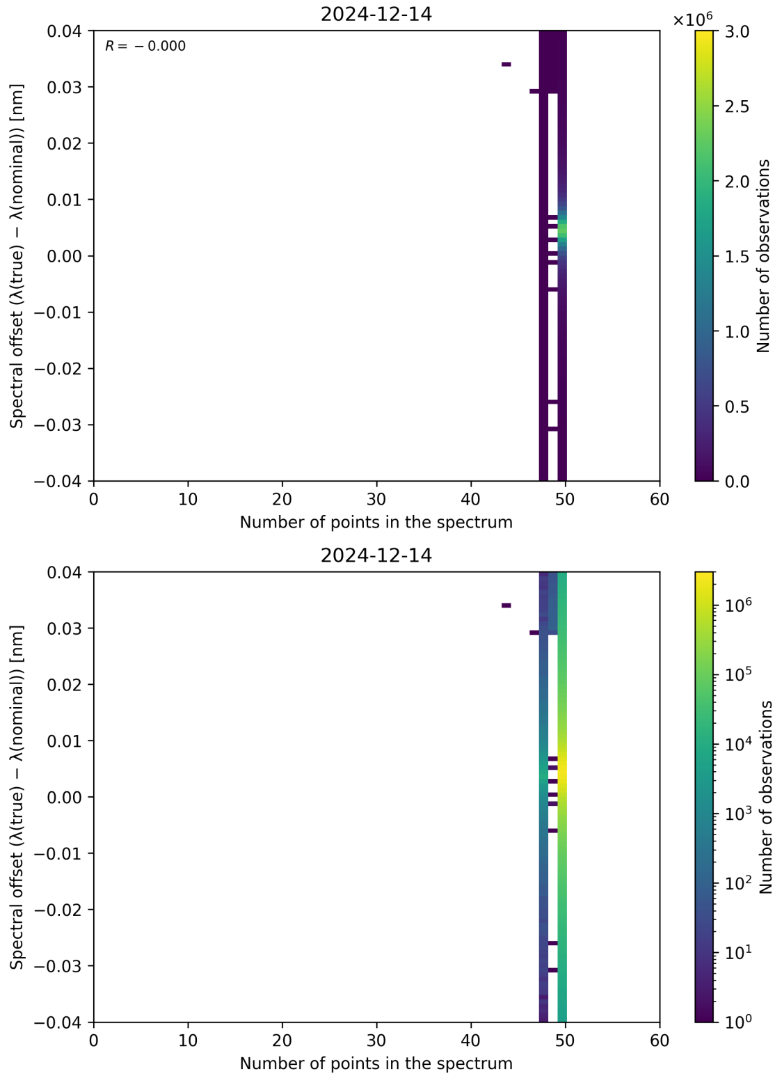
Figure 101: Scatter density plot of “Number of points in the spectrum” against “Spectral offset ( \lambda_{\text{true}} - \lambda_{\text{nominal}} )” for 2024-12-13 to 2024-12-15.
