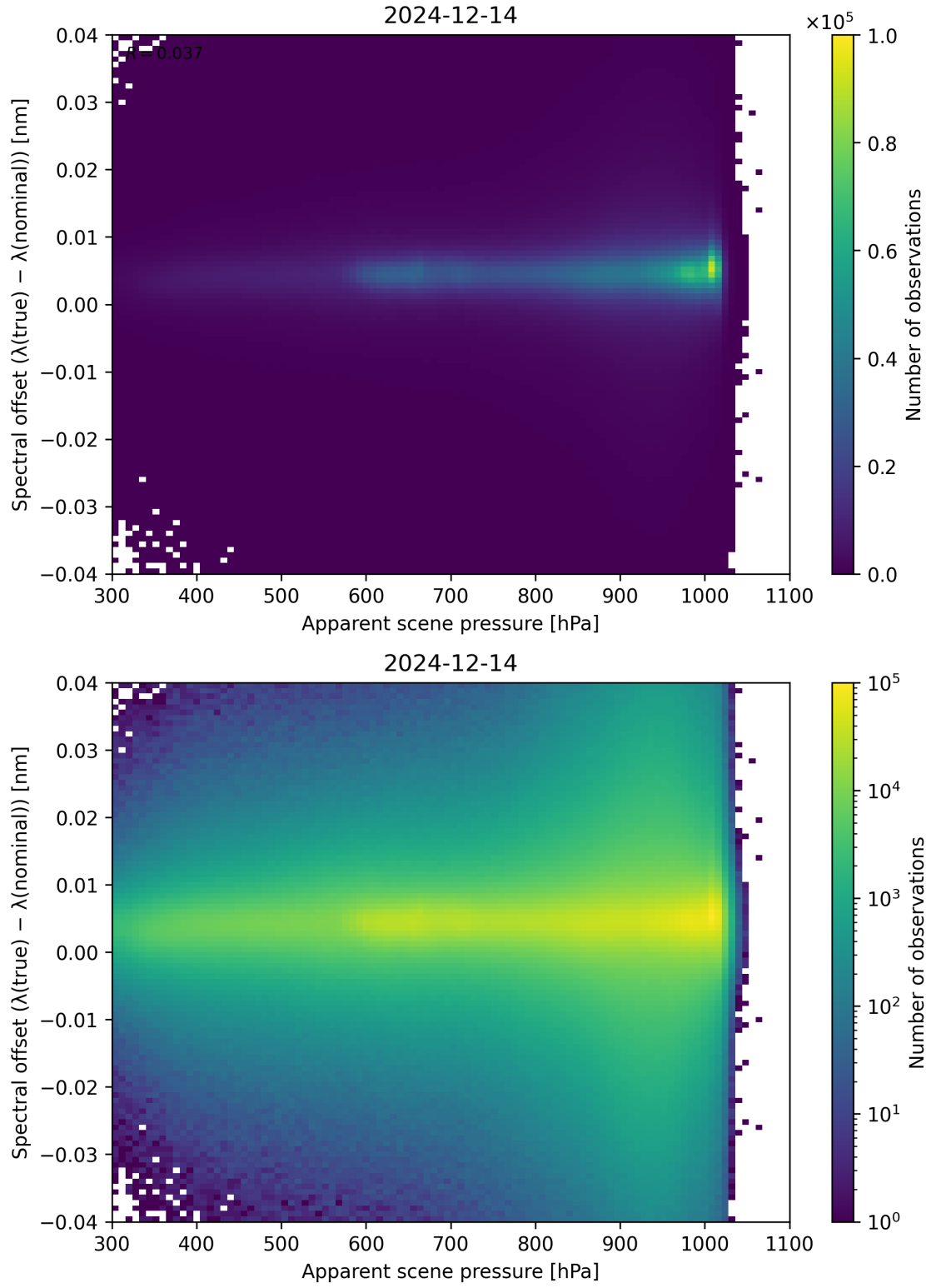
Figure 67: Scatter density plot of “Apparent scene pressure” against “Spectral offset ( \lambda_{\text{true}} - \lambda_{\text{nominal}} )” for 2024-12-13 to 2024-12-15.
