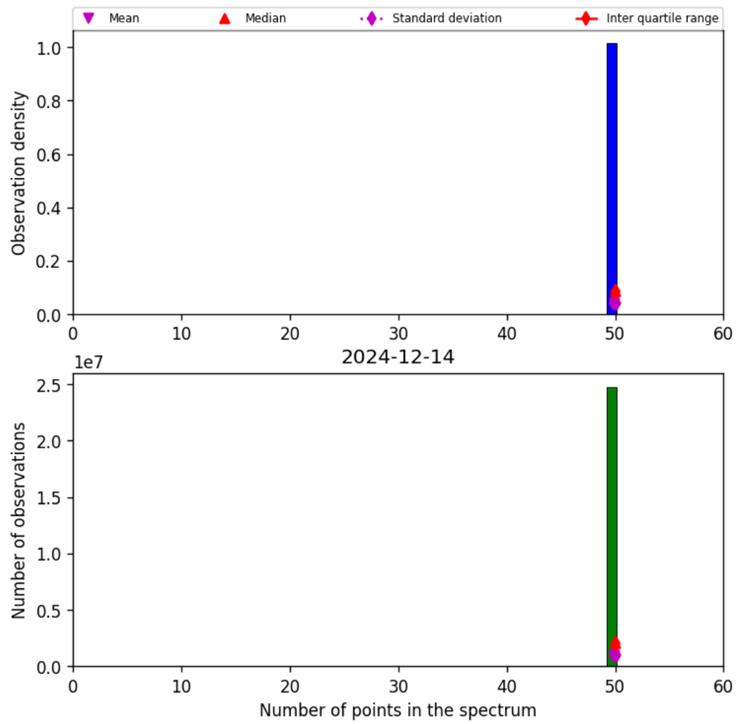
Figure 44: Histogram of “Number of points in the spectrum” for 2024-12-13 to 2024-12-15
