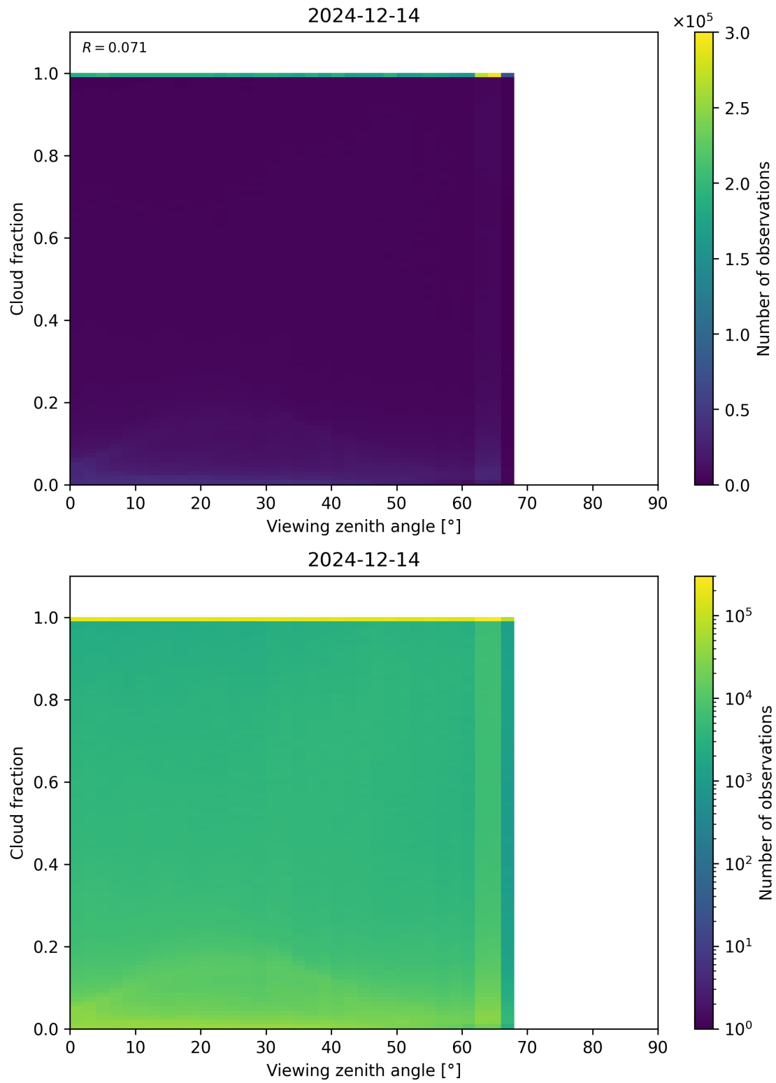
Figure 120: Scatter density plot of “Viewing zenith angle” against “Cloud fraction” for 2024-12-13 to 2024-12-15.
