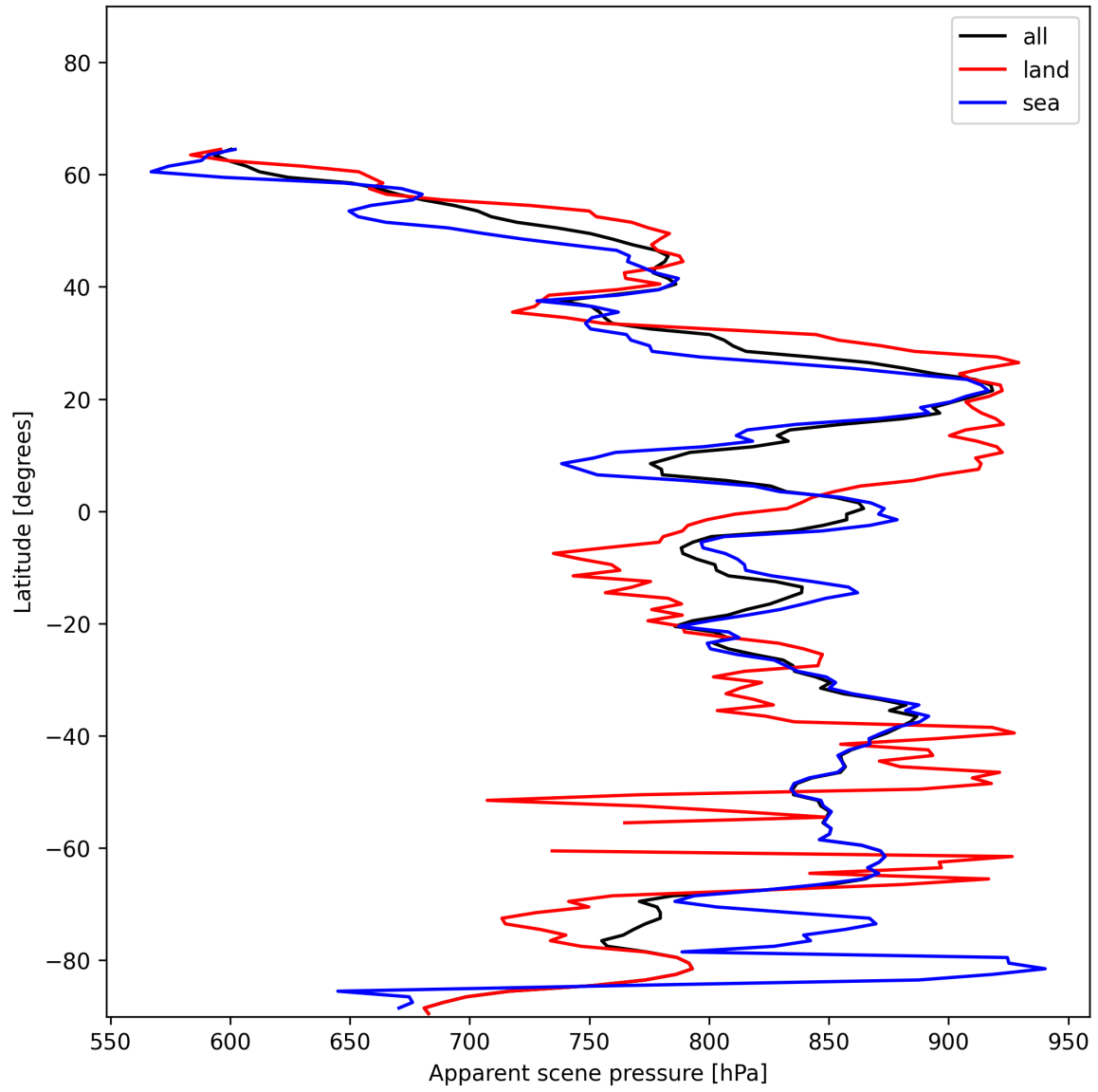
Figure 19: Zonal average of “Apparent scene pressure” for 2024-12-13 to 2024-12-15.
