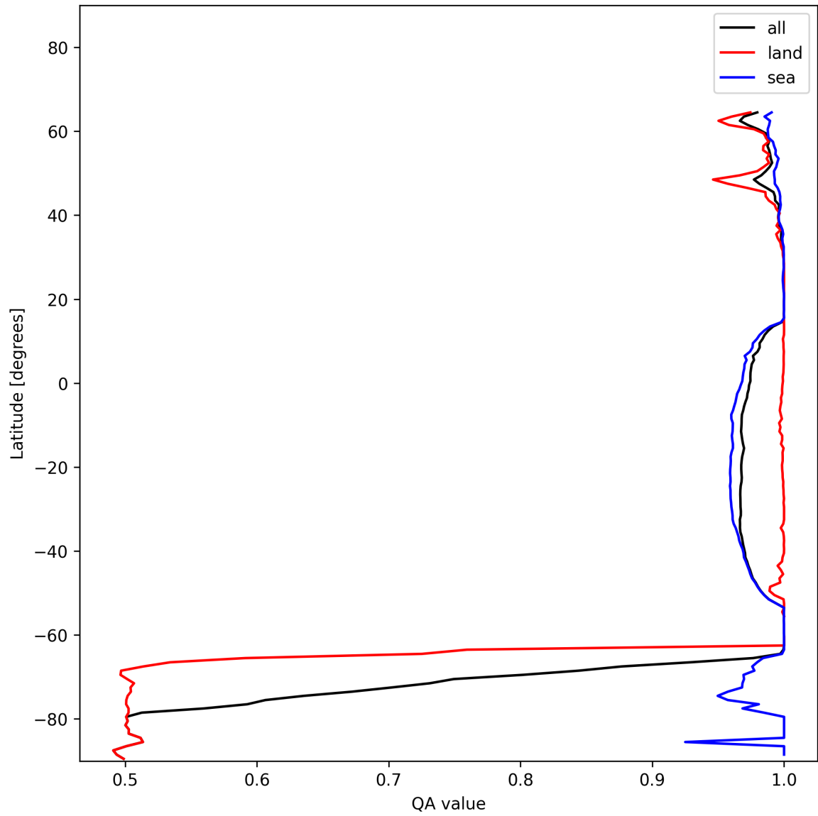
Figure 12: Zonal average of “QA value” for 2024-12-13 to 2024-12-15.
