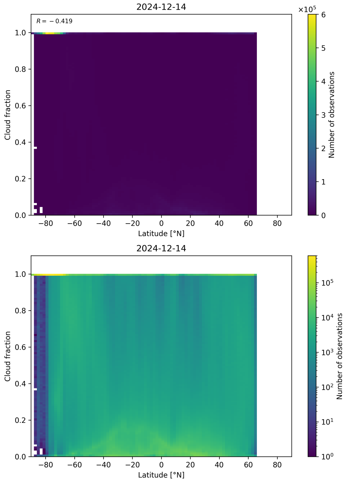
Figure 90: Scatter density plot of “Latitude” against “Cloud fraction” for 2024-12-13 to 2024-12-15.
