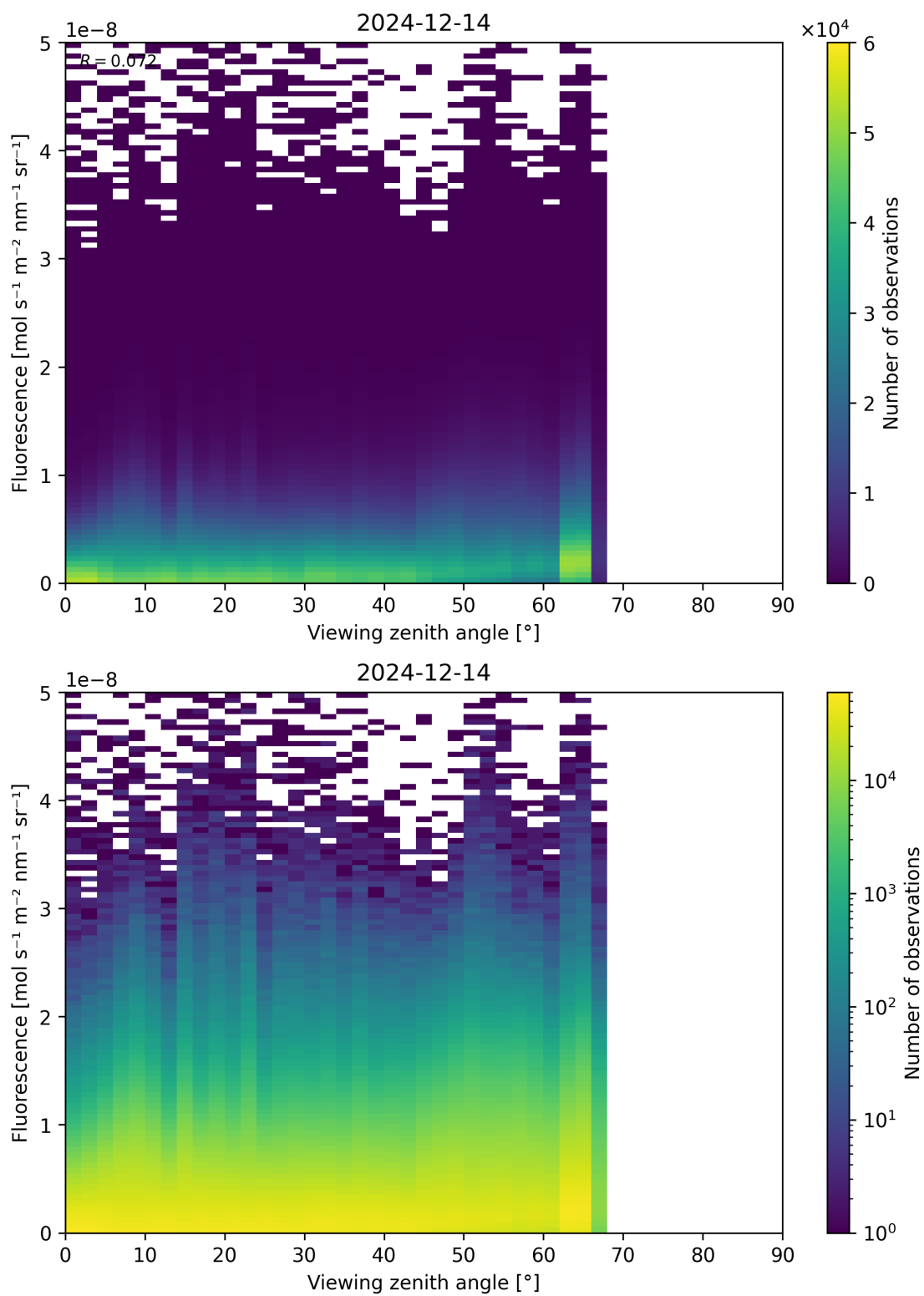
Figure 122: Scatter density plot of “Viewing zenith angle” against “Fluorescence” for 2024-12-13 to 2024-12-15.
