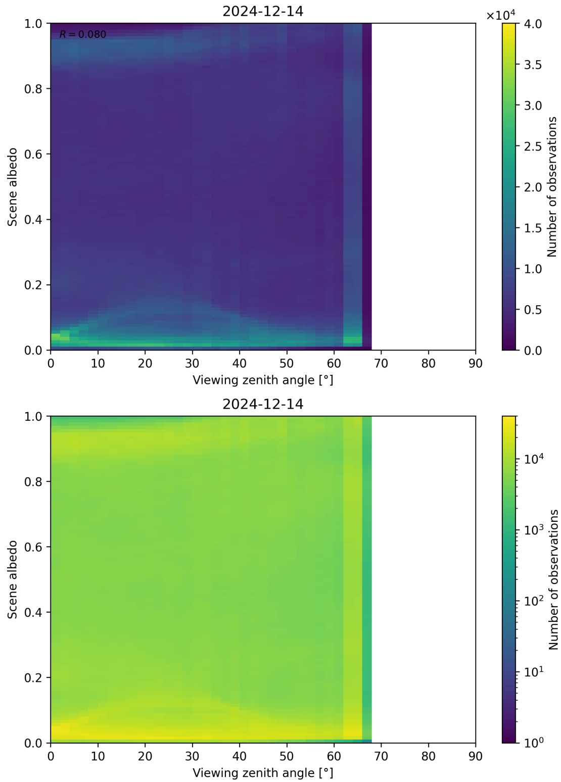
Figure 126: Scatter density plot of “Viewing zenith angle” against “Scene albedo” for 2024-12-13 to 2024-12-15.
