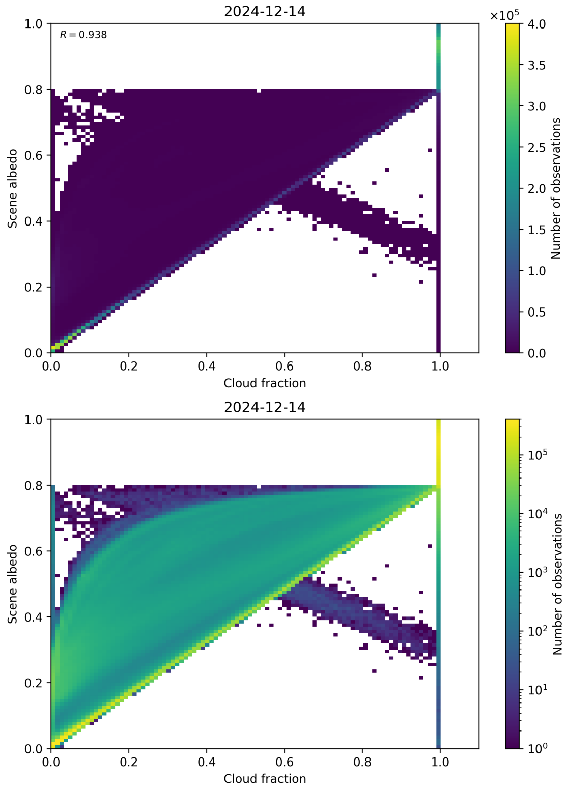
Figure 75: Scatter density plot of “Cloud fraction” against “Scene albedo” for 2024-12-13 to 2024-12-15.
