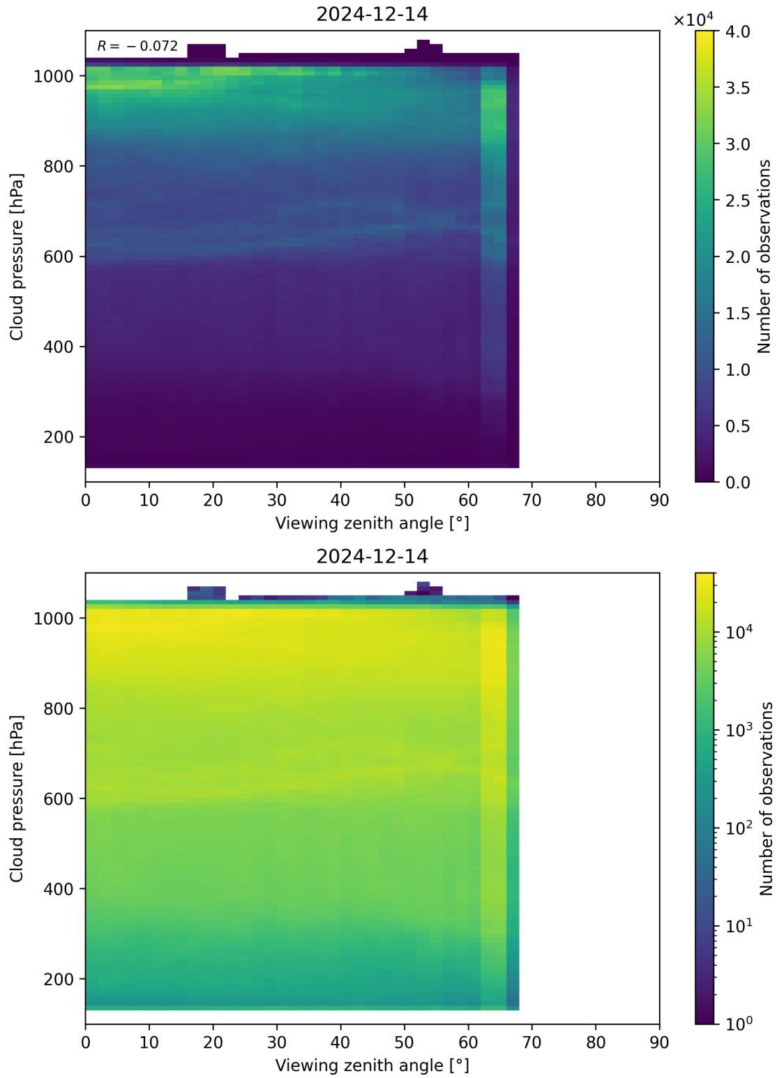
Figure 121: Scatter density plot of “Viewing zenith angle” against “Cloud pressure” for 2024-12-13 to 2024-12-15.
