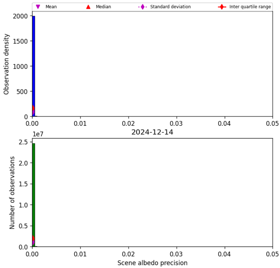
Figure 35: Histogram of “Scene albedo precision” for 2024-12-13 to 2024-12-15
