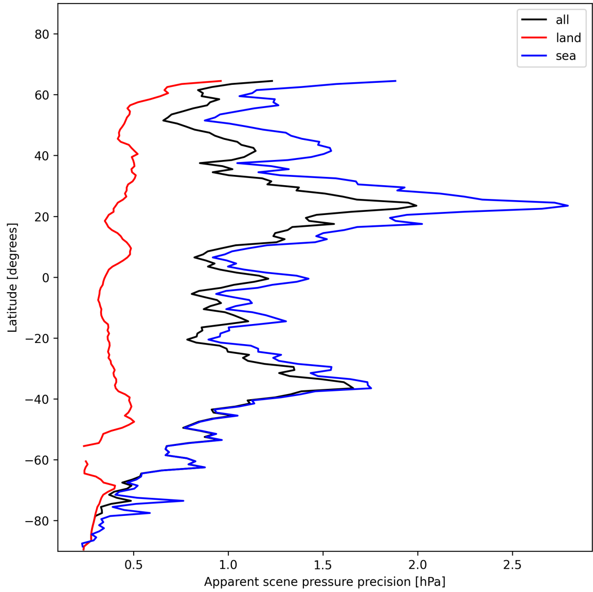
Figure 20: Zonal average of “Apparent scene pressure precision” for 2024-12-13 to 2024-12-15.
