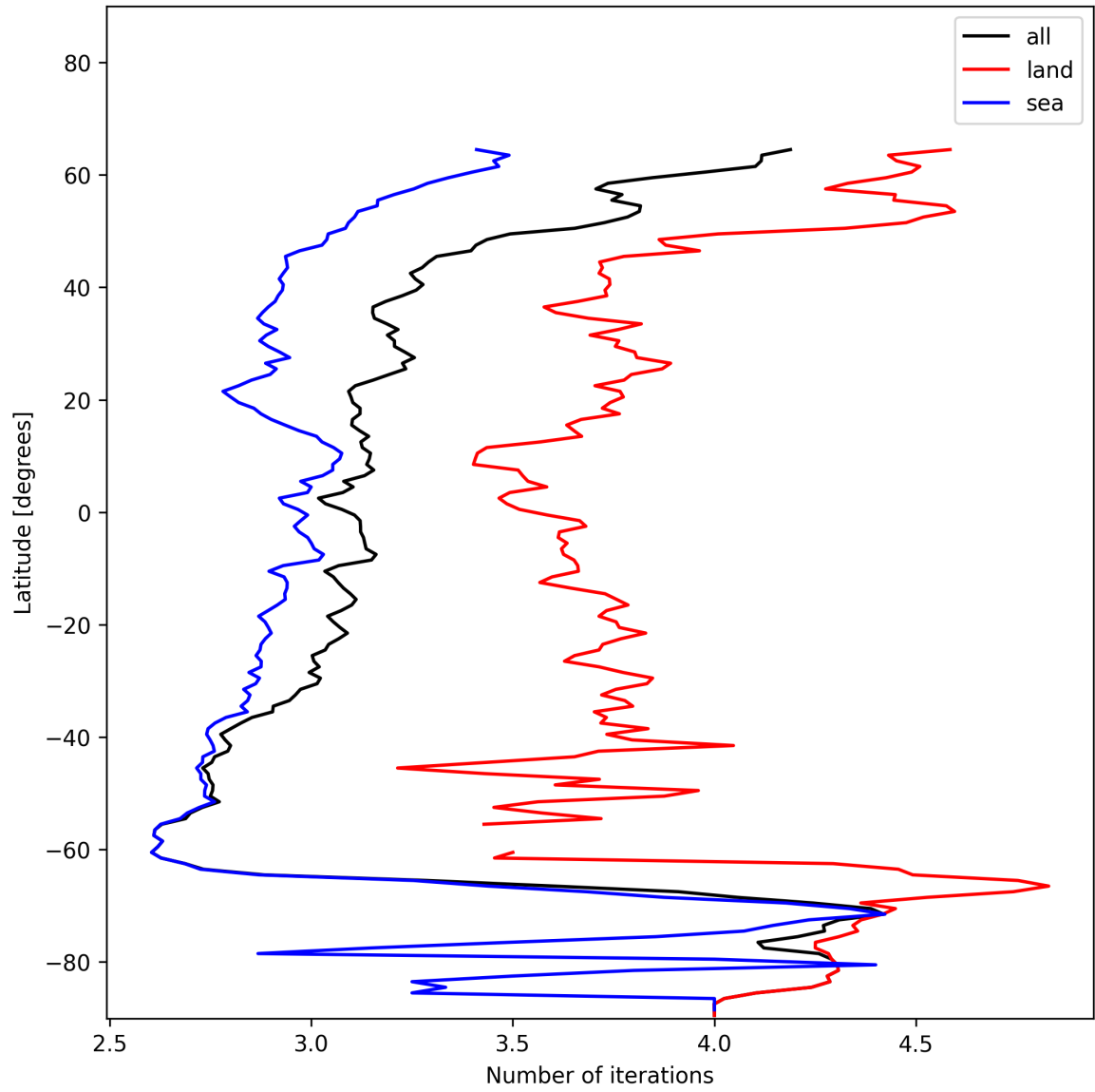
Figure 22: Zonal average of “Number of iterations” for 2024-12-13 to 2024-12-15.
