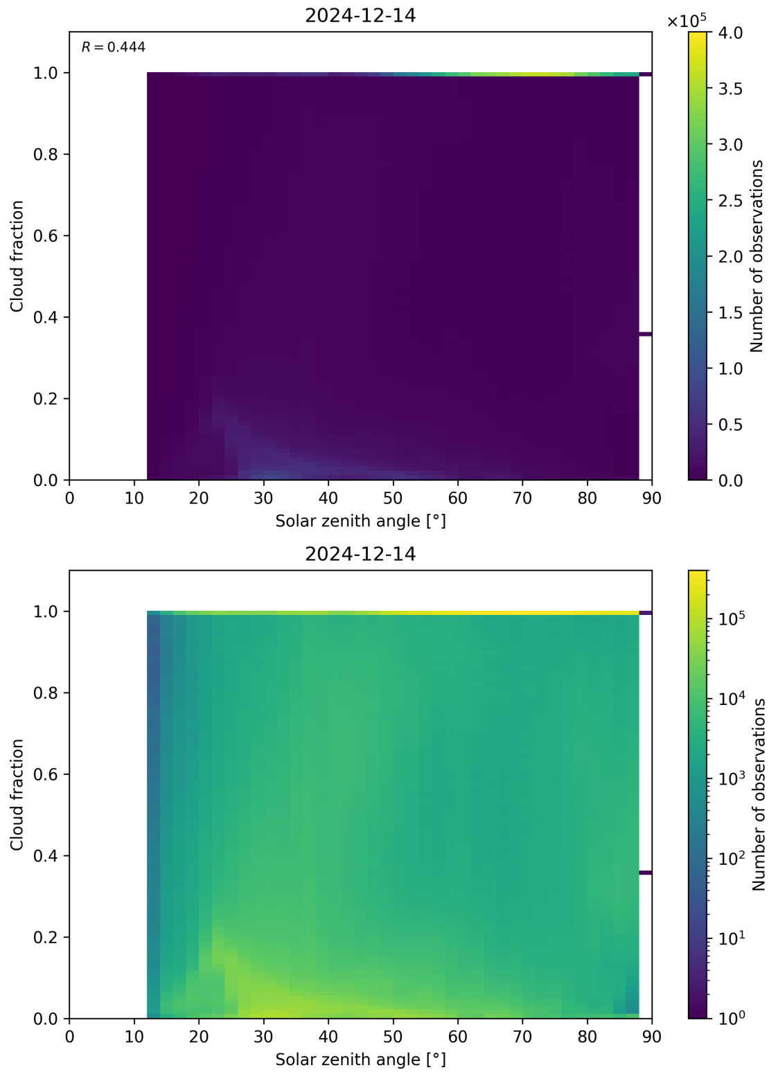
Figure 110: Scatter density plot of “Solar zenith angle” against “Cloud fraction” for 2024-12-13 to 2024-12-15.
