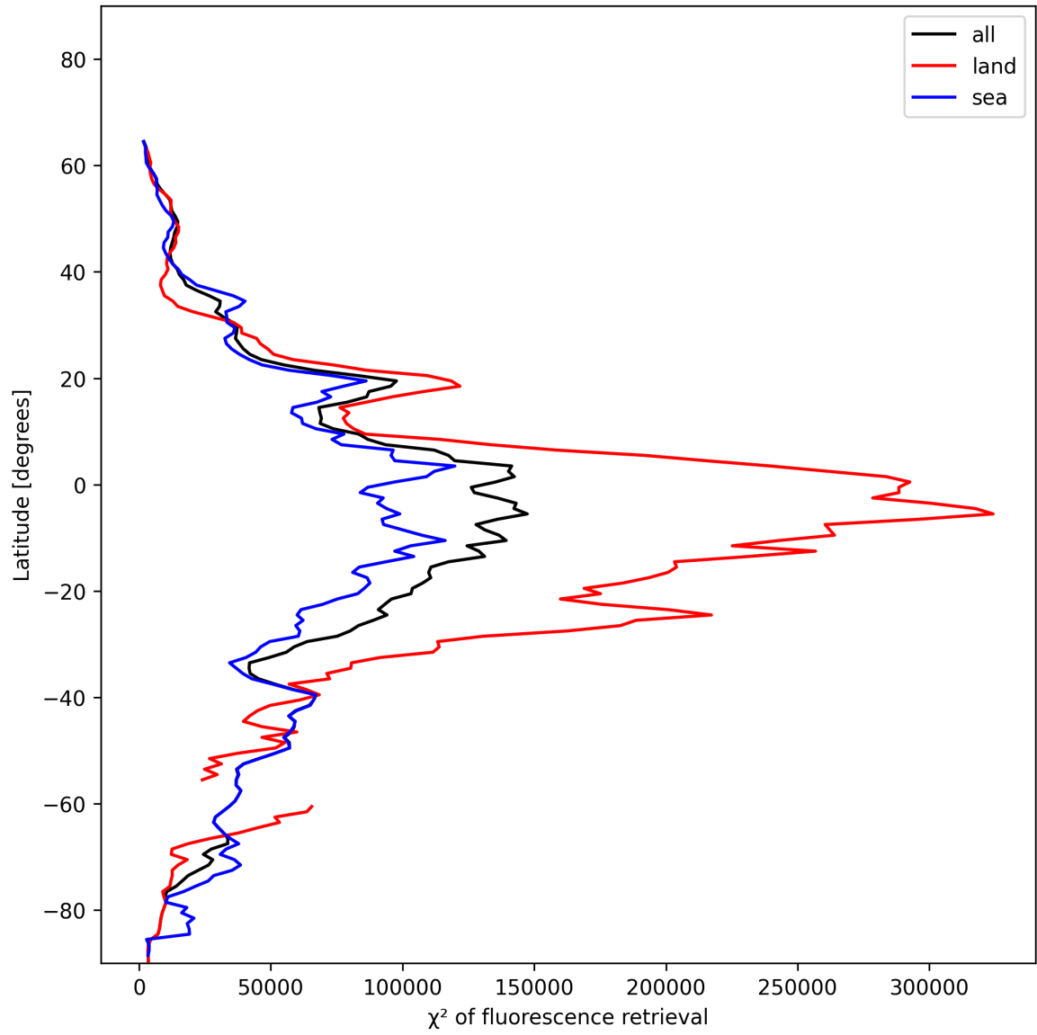
Figure 25: Zonal average of “ \chi^2 of fluorescence retrieval” for 2024-12-13 to 2024-12-15.
