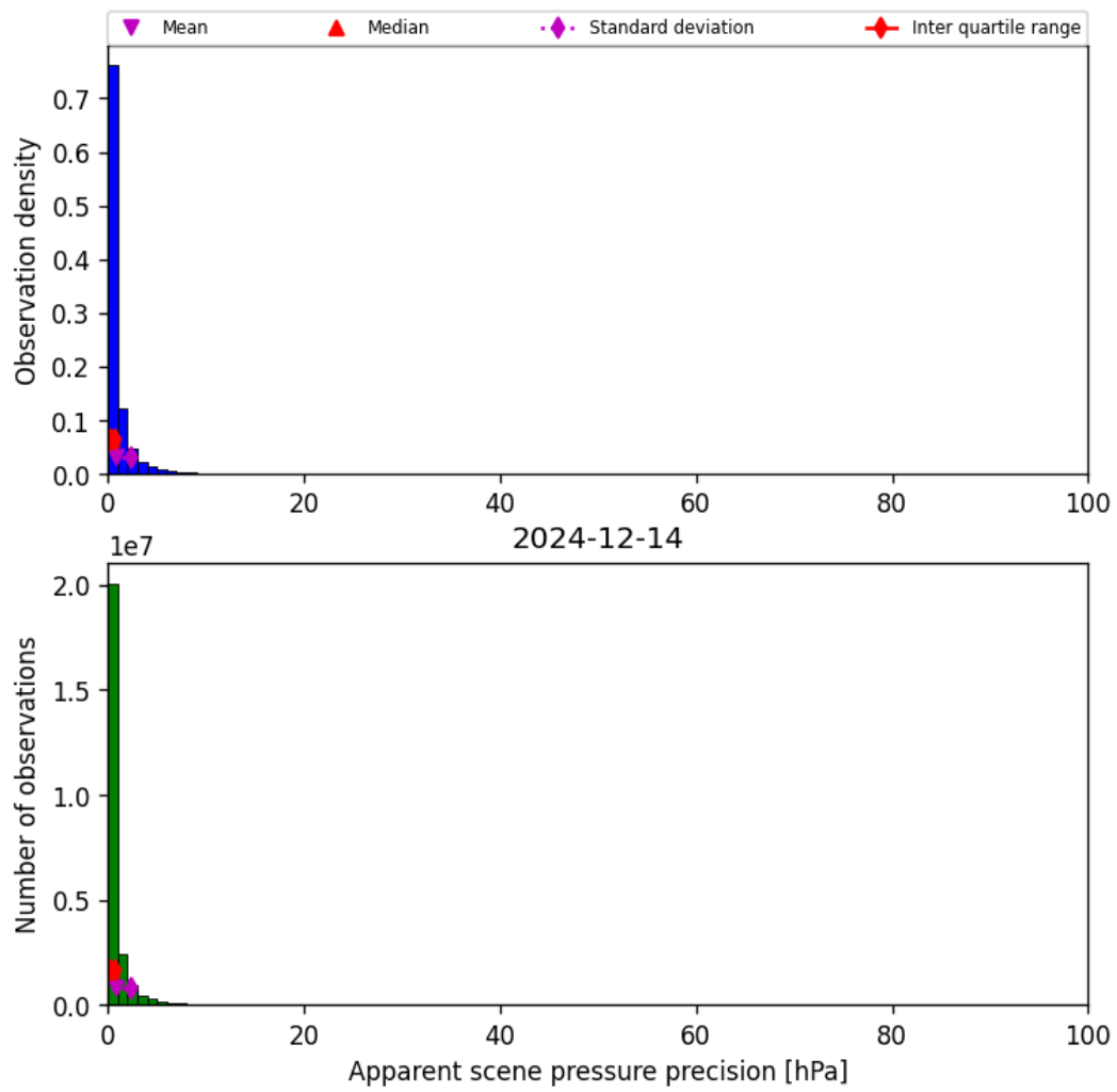
Figure 37: Histogram of “Apparent scene pressure precision” for 2024-12-13 to 2024-12-15
