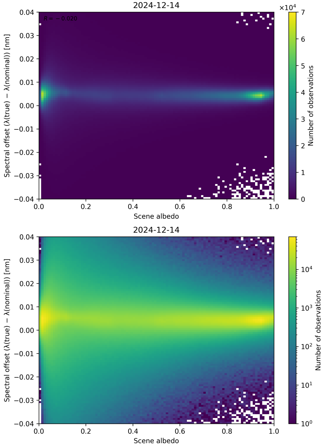
Figure 107: Scatter density plot of “Scene albedo” against “Spectral offset ( \lambda_{\text{true}} - \lambda_{\text{nominal}} )” for 2024-12-13 to 2024-12-15.
