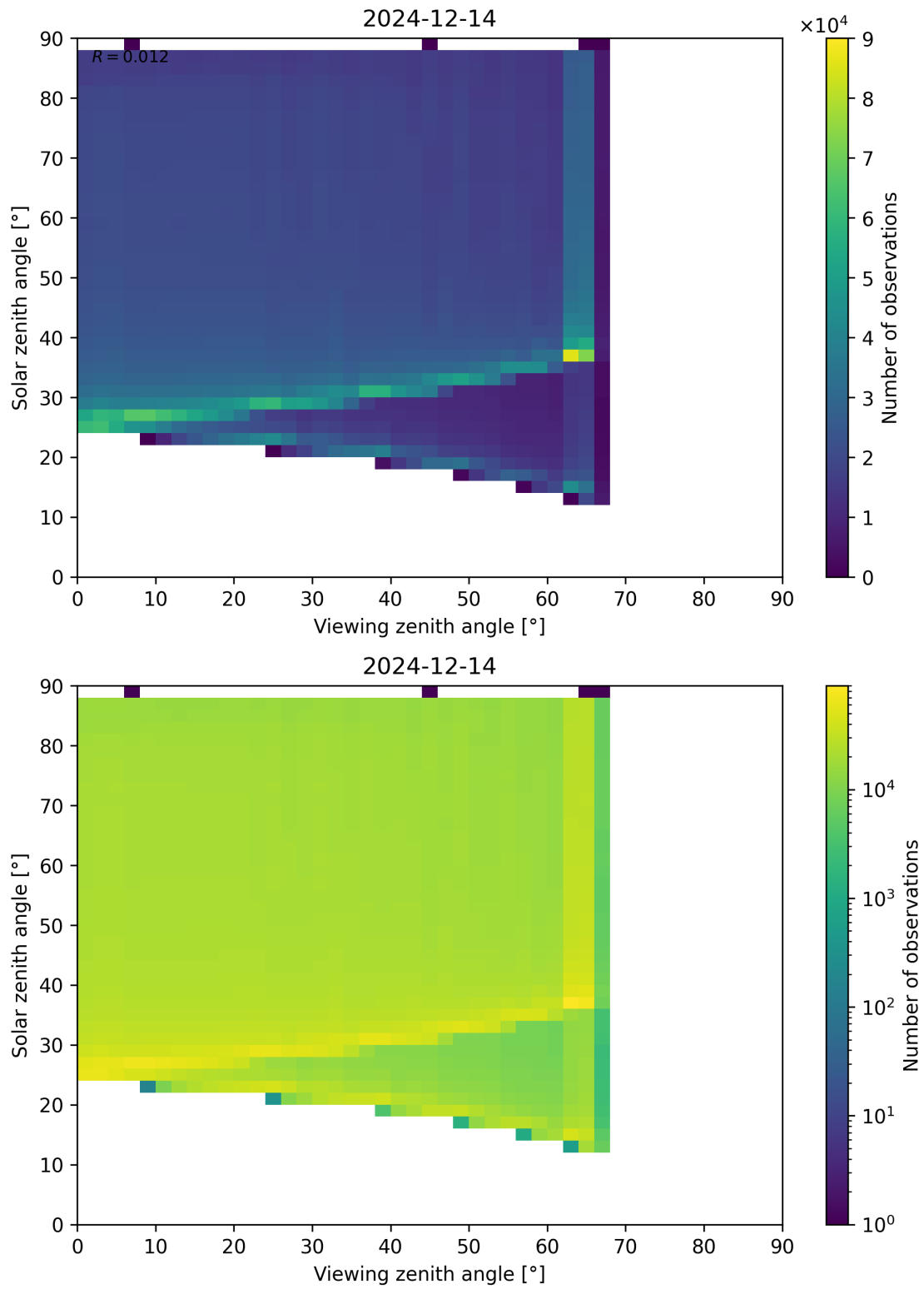
Figure 127: Scatter density plot of “Viewing zenith angle” against “Solar zenith angle” for 2024-12-13 to 2024-12-15.
