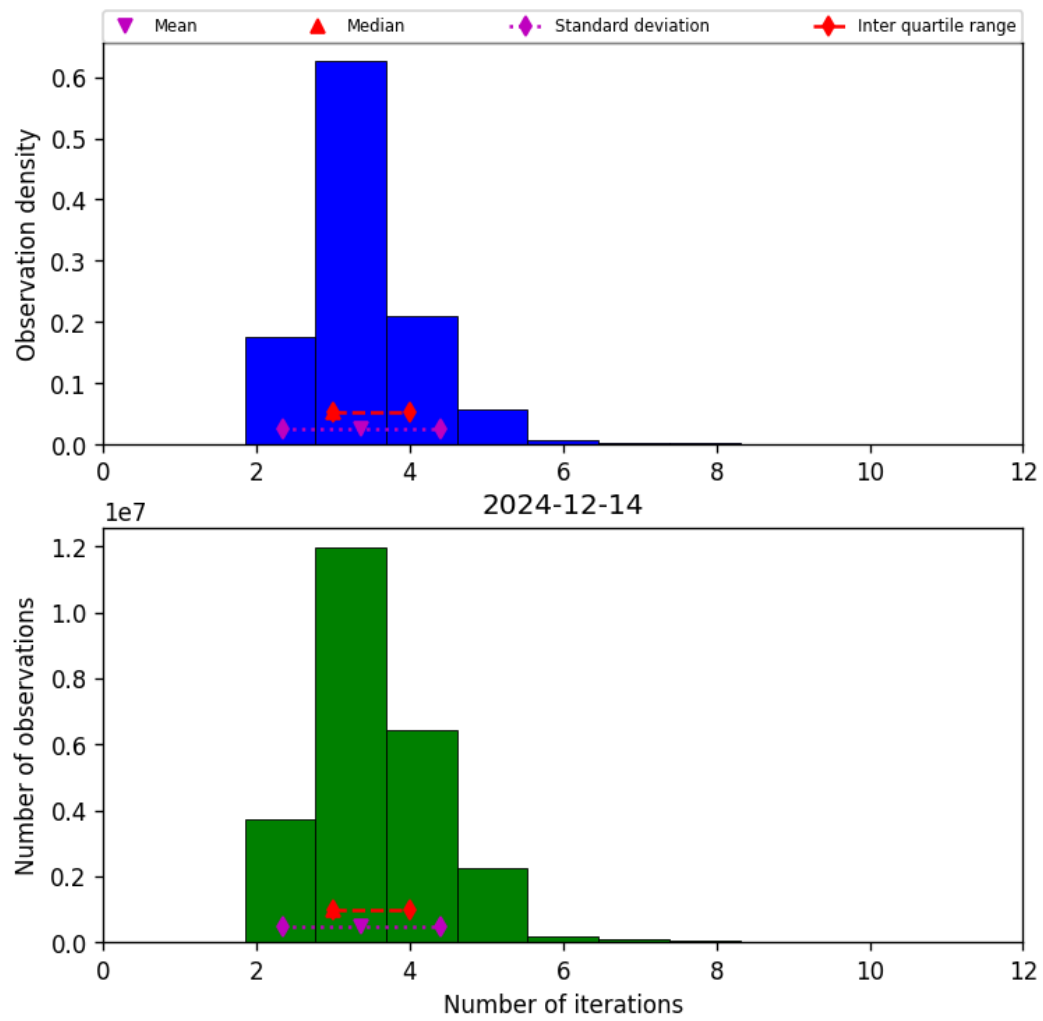
Figure 39: Histogram of “Number of iterations” for 2024-12-13 to 2024-12-15
