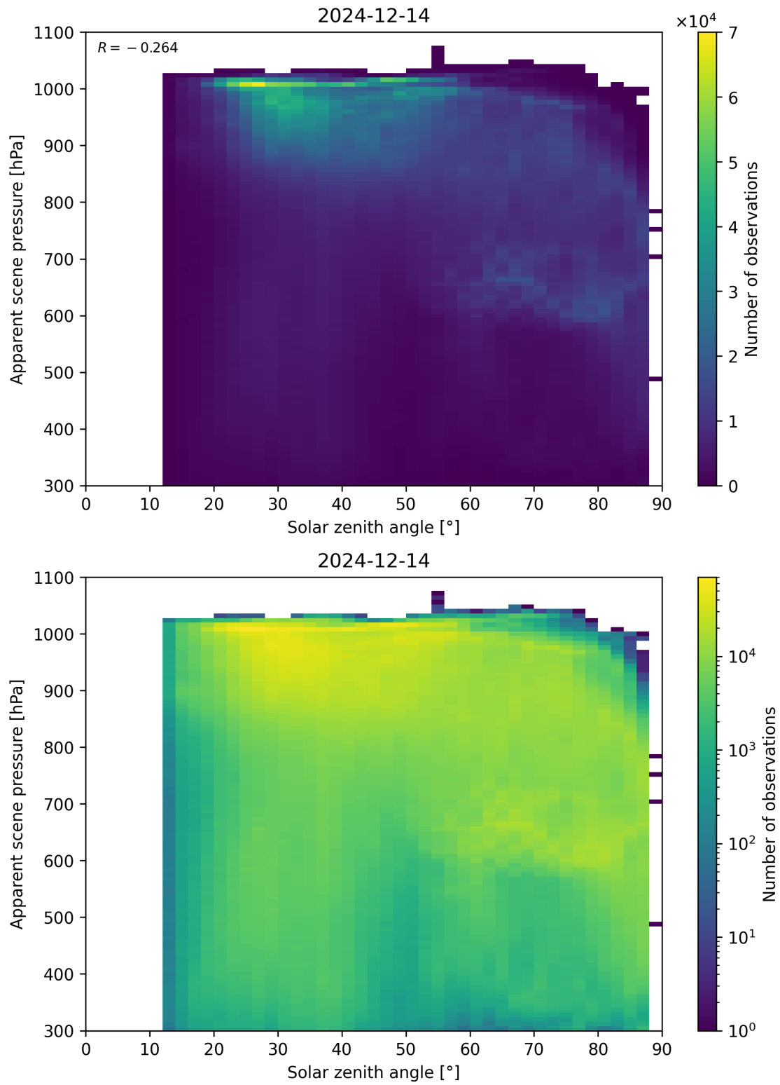
Figure 108: Scatter density plot of “Solar zenith angle” against “Apparent scene pressure” for 2024-12-13 to 2024-12-15.
