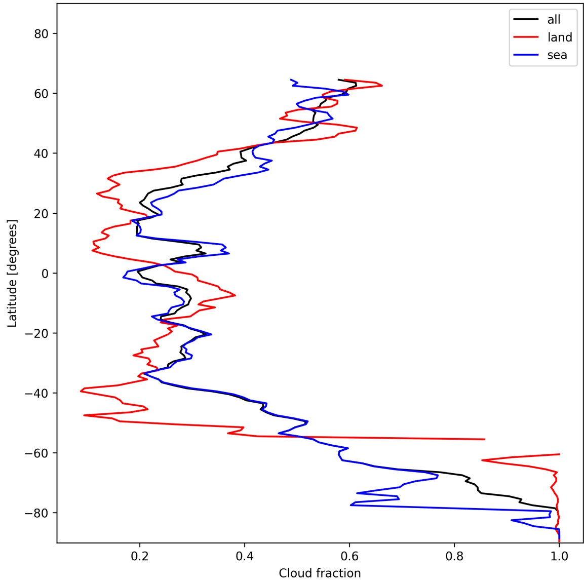
Figure 15: Zonal average of “Cloud fraction” for 2024-12-13 to 2024-12-15.
