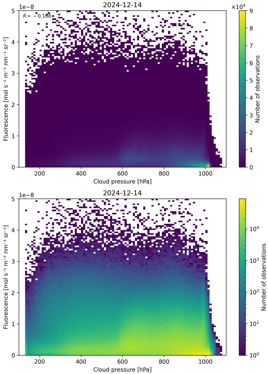
Figure 80: Scatter density plot of “Cloud pressure” against “Fluorescence” for 2024-12-13 to 2024-12-15.
