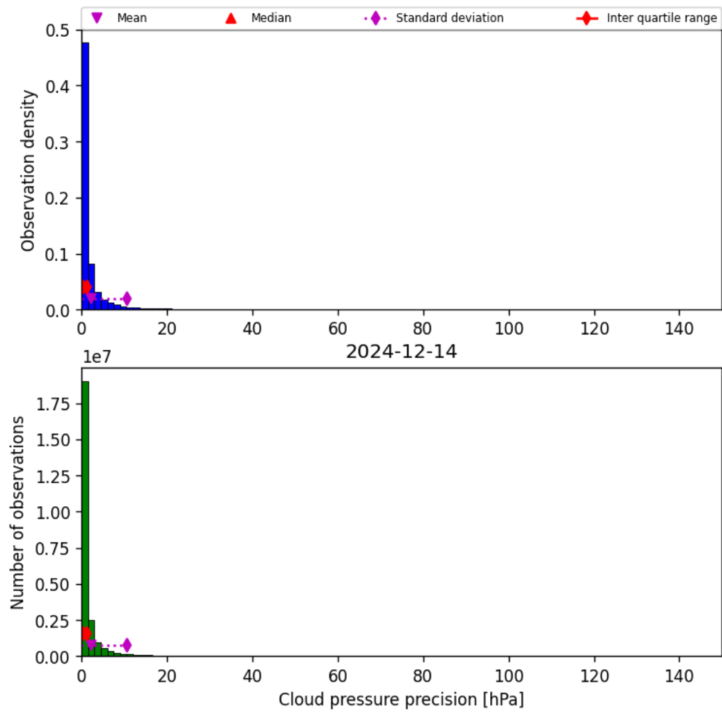
Figure 31: Histogram of “Cloud pressure precision” for 2024-12-13 to 2024-12-15
