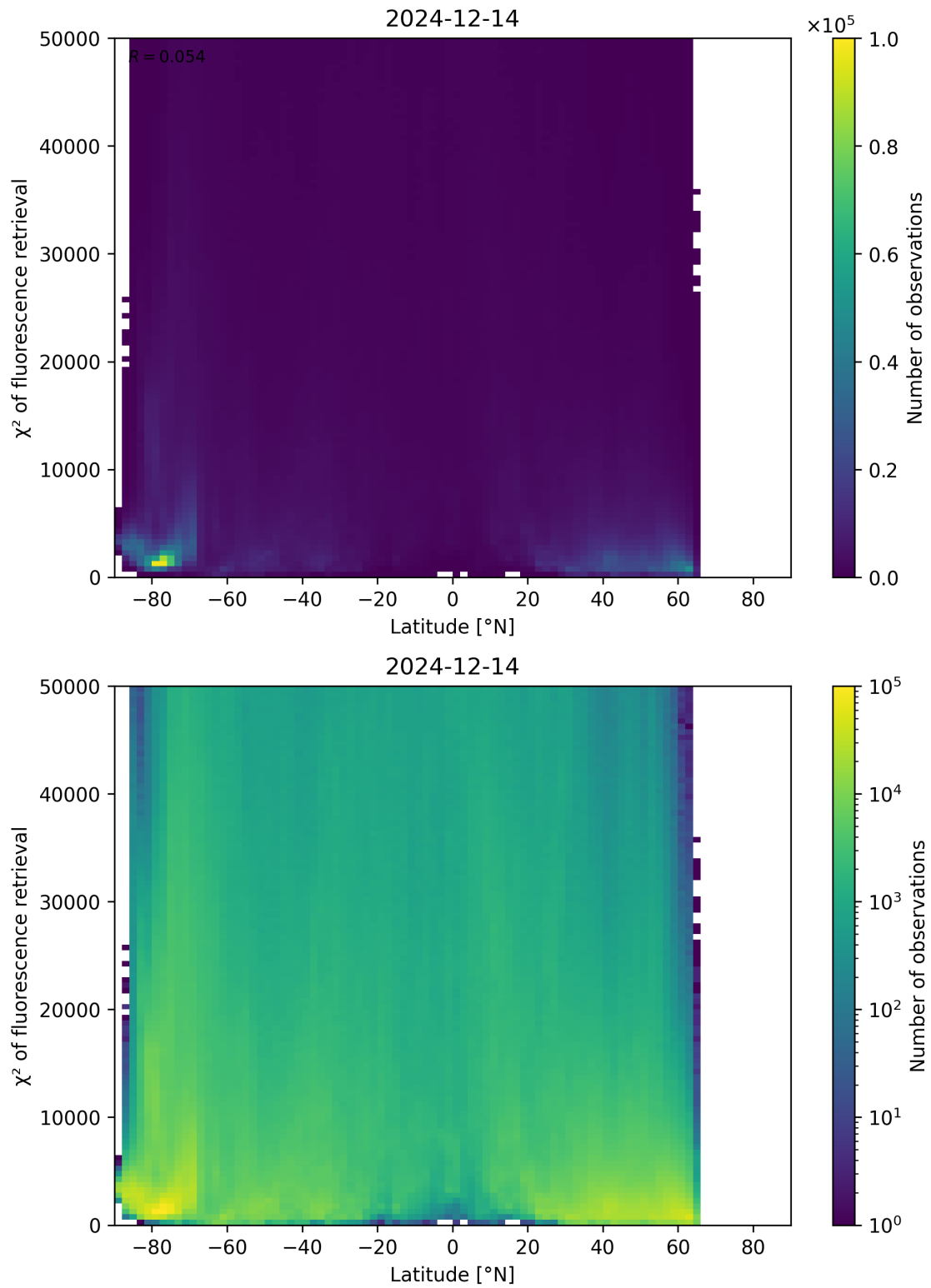
Figure 89: Scatter density plot of “Latitude” against “ \chi^2 of fluorescence retrieval” for 2024-12-13 to 2024-12-15.
