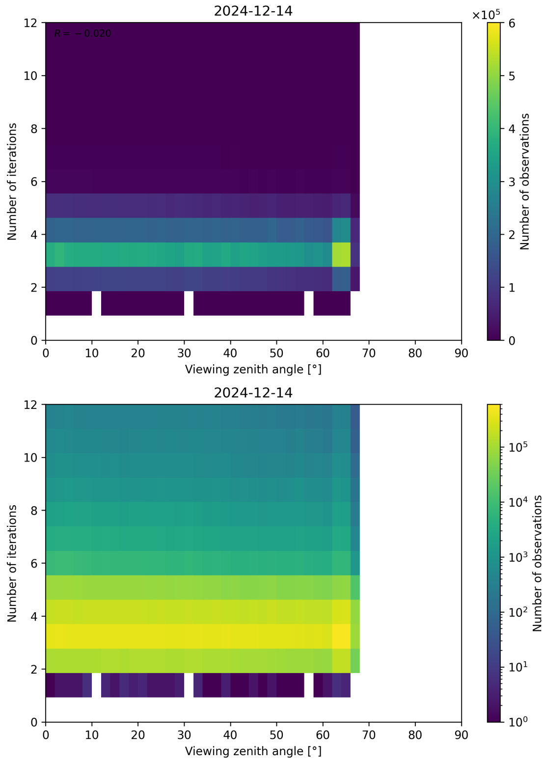
Figure 124: Scatter density plot of “Viewing zenith angle” against “Number of iterations” for 2024-12-13 to 2024-12-15.
