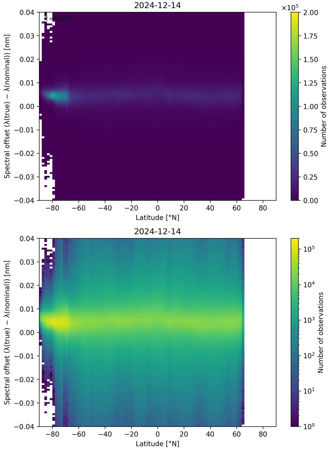
Figure 96: Scatter density plot of “Latitude” against “Spectral offset ( \lambda_{\text{true}} - \lambda_{\text{nominal}} )” for 2024-12-13 to 2024-12-15.
