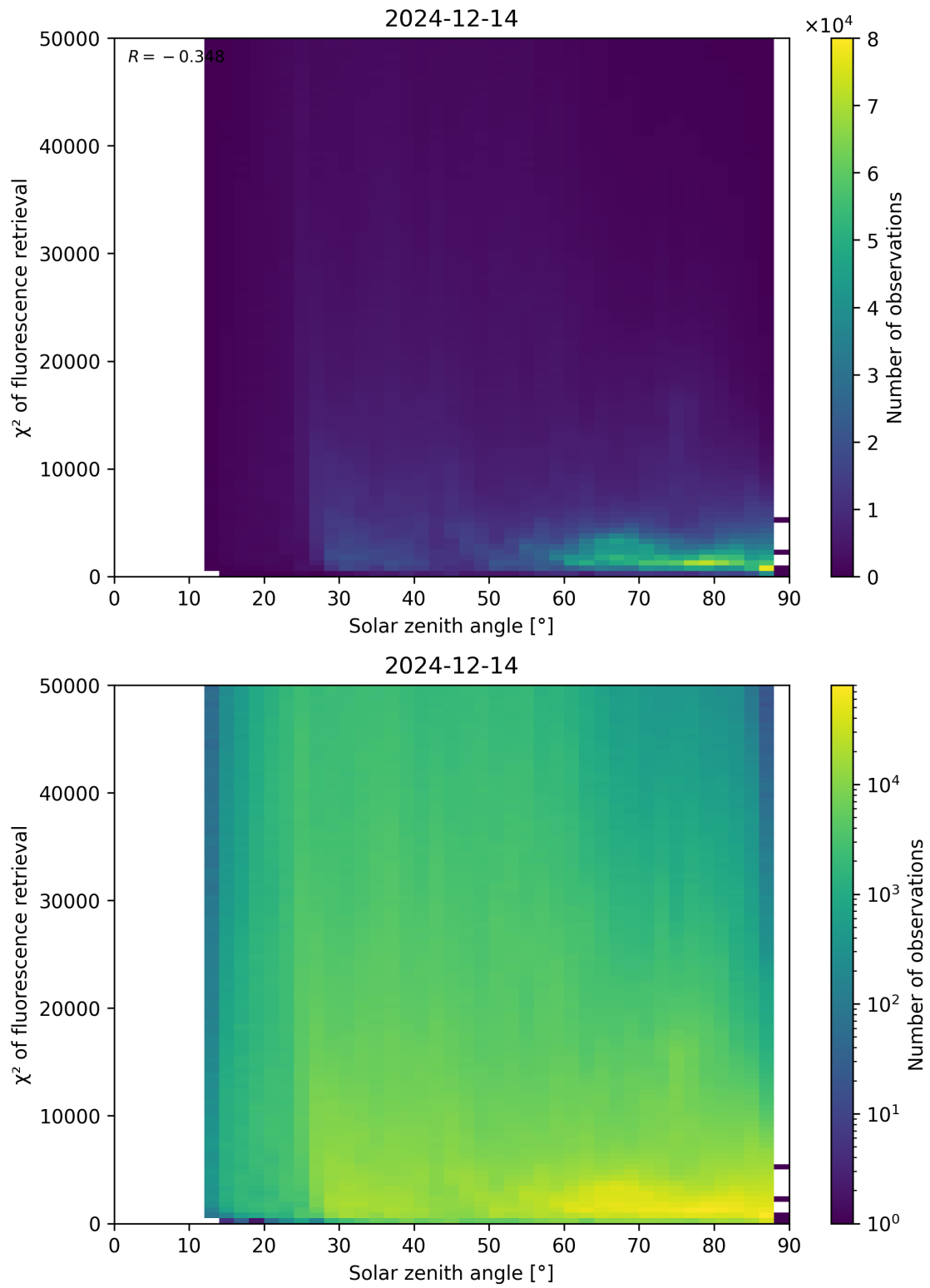
Figure 109: Scatter density plot of “Solar zenith angle” against “ \chi^2 of fluorescence retrieval” for 2024-12-13 to 2024-12-15.
