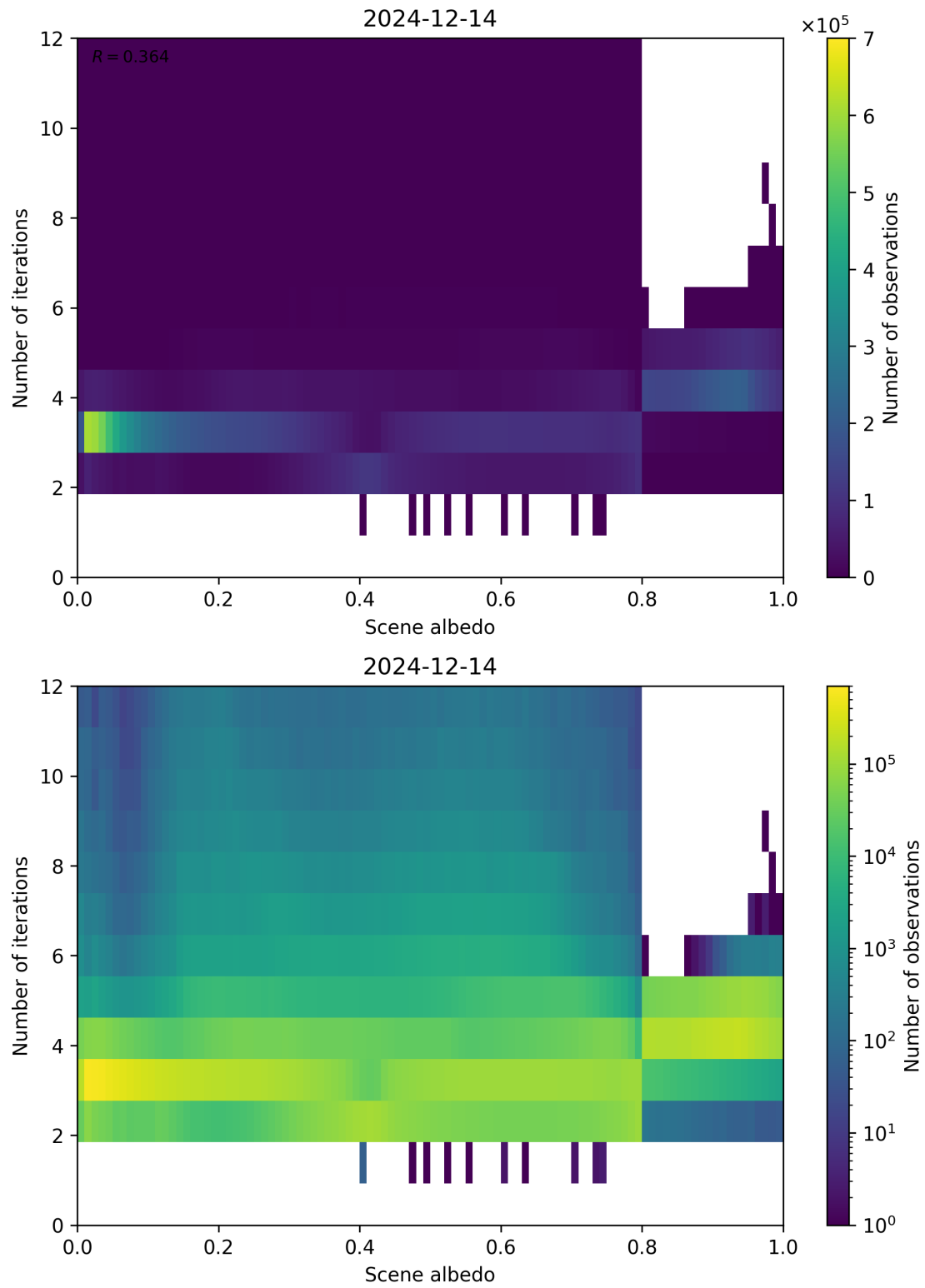
Figure 105: Scatter density plot of “Scene albedo” against “Number of iterations” for 2024-12-13 to 2024-12-15.
