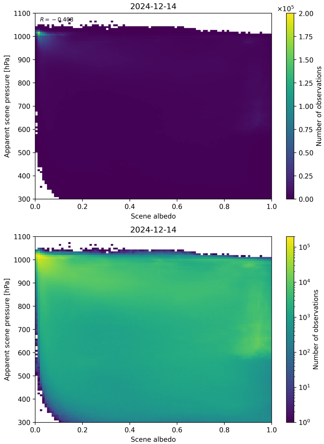
Figure 102: Scatter density plot of “Scene albedo” against “Apparent scene pressure” for 2024-12-13 to 2024-12-15.
