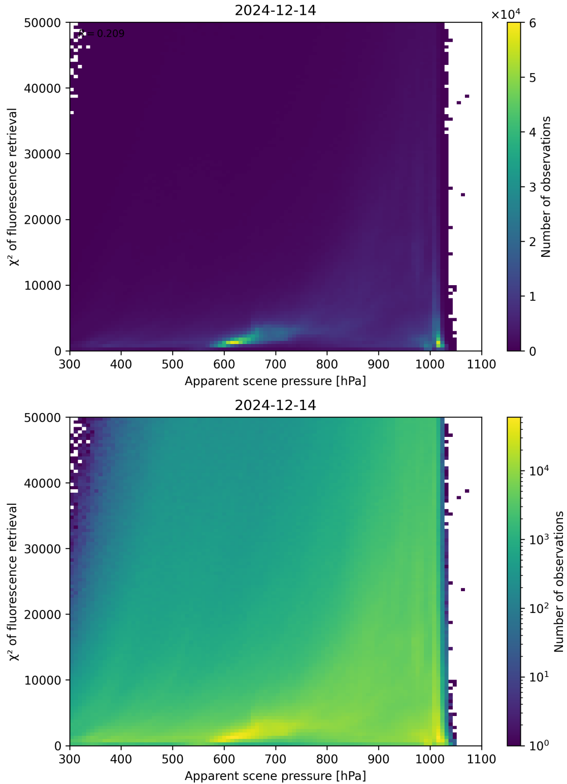
Figure 63: Scatter density plot of “Apparent scene pressure” against “ \chi^2 of fluorescence retrieval” for 2024-12-13 to 2024-12-15.
