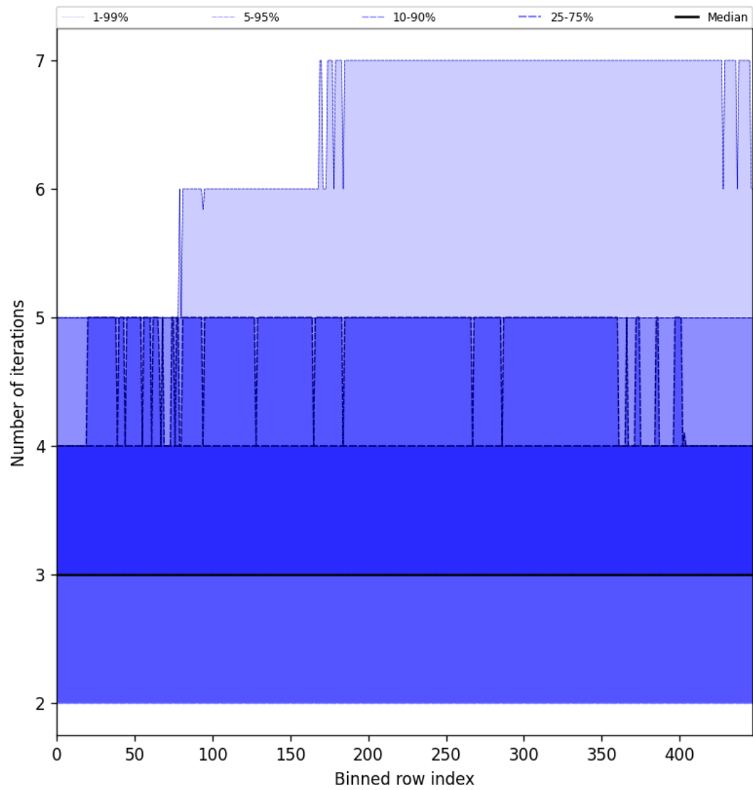
Figure 56: Along track statistics of “Number of iterations” for 2024-12-13 to 2024-12-15
