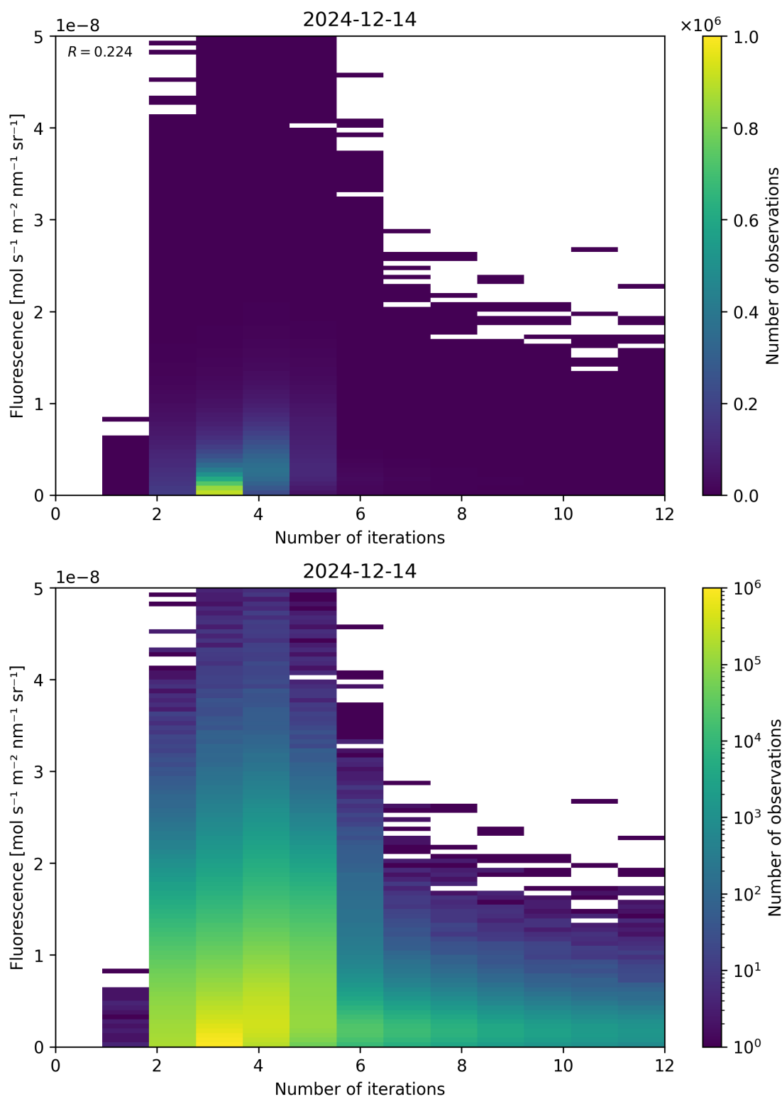
Figure 98: Scatter density plot of “Number of iterations” against “Fluorescence” for 2024-12-13 to 2024-12-15.
