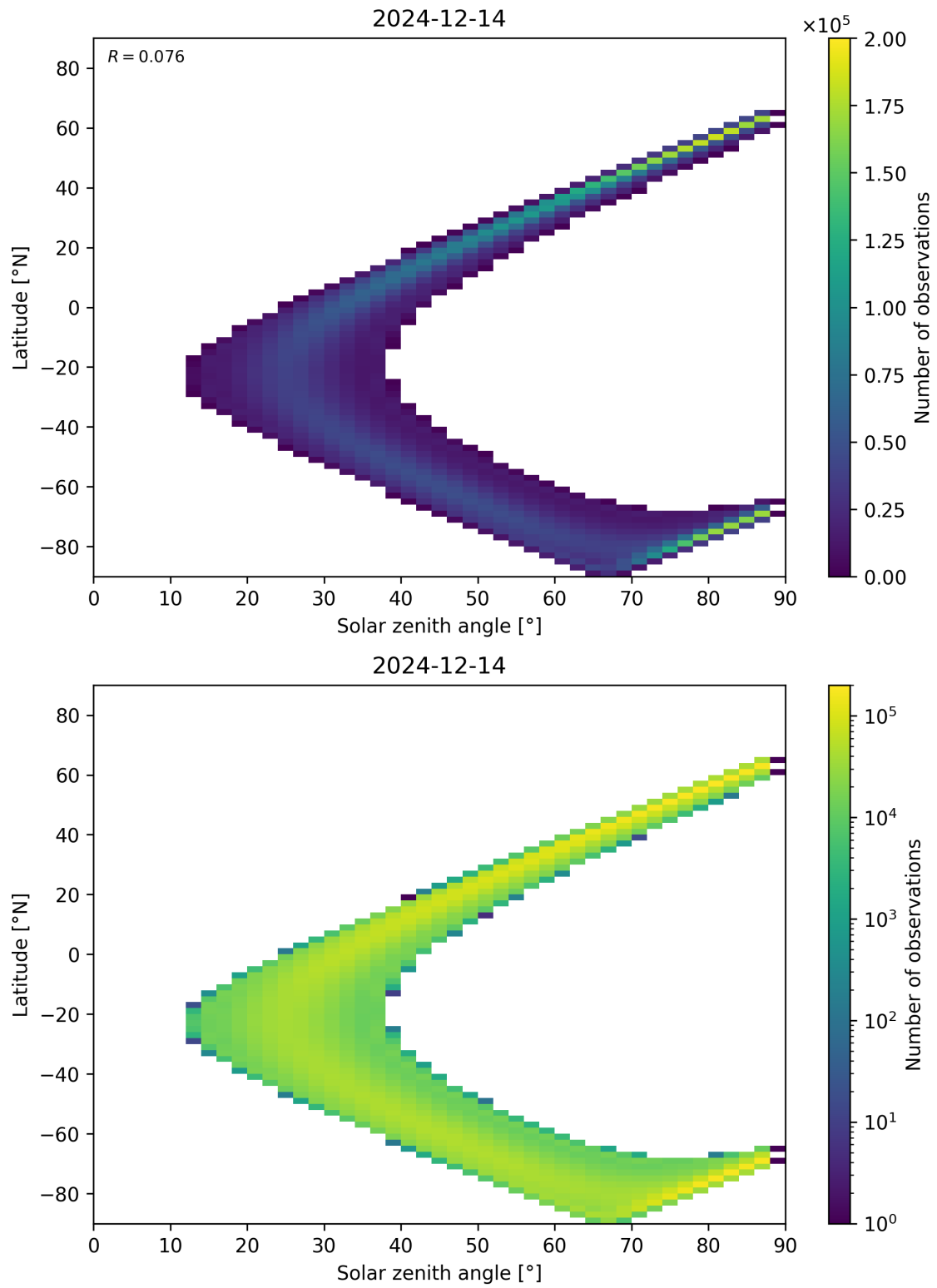
Figure 113: Scatter density plot of “Solar zenith angle” against “Latitude” for 2024-12-13 to 2024-12-15.
