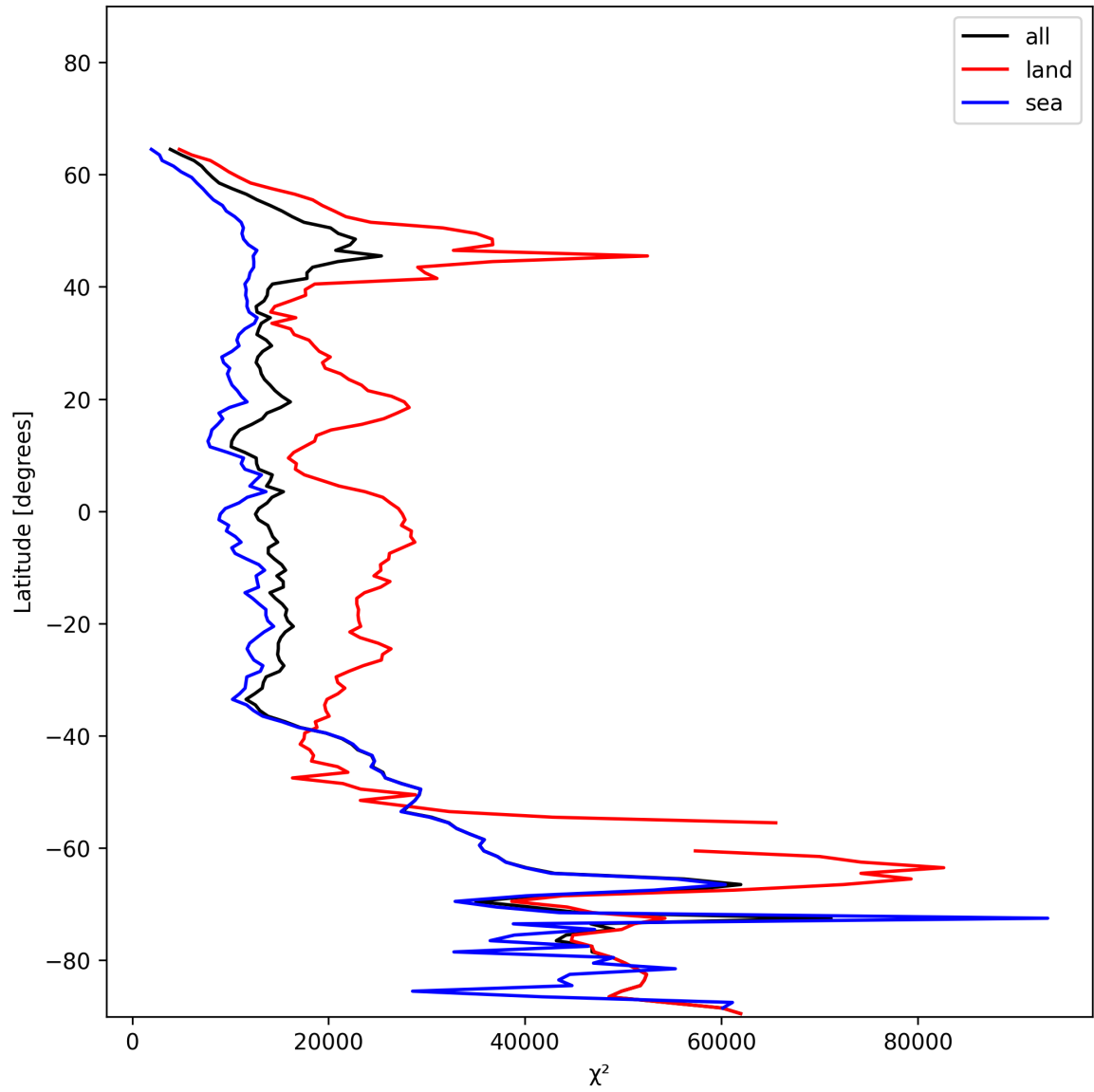
Figure 21: Zonal average of “ \chi^2 ” for 2024-12-13 to 2024-12-15.
