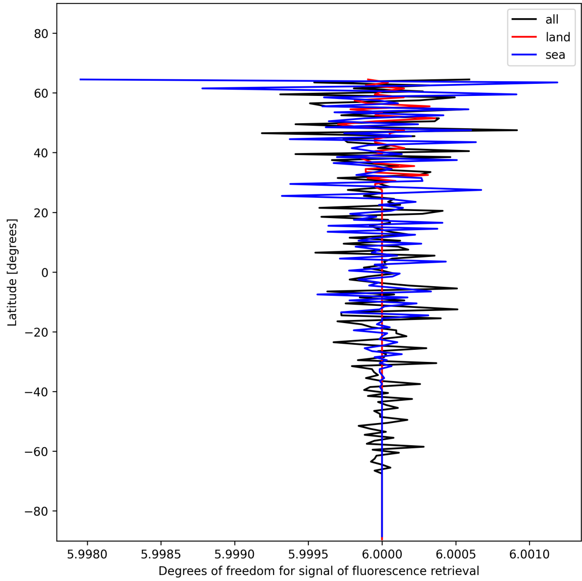
Figure 26: Zonal average of “Degrees of freedom for signal of fluorescence retrieval” for 2024-12-13 to 2024-12-15.
