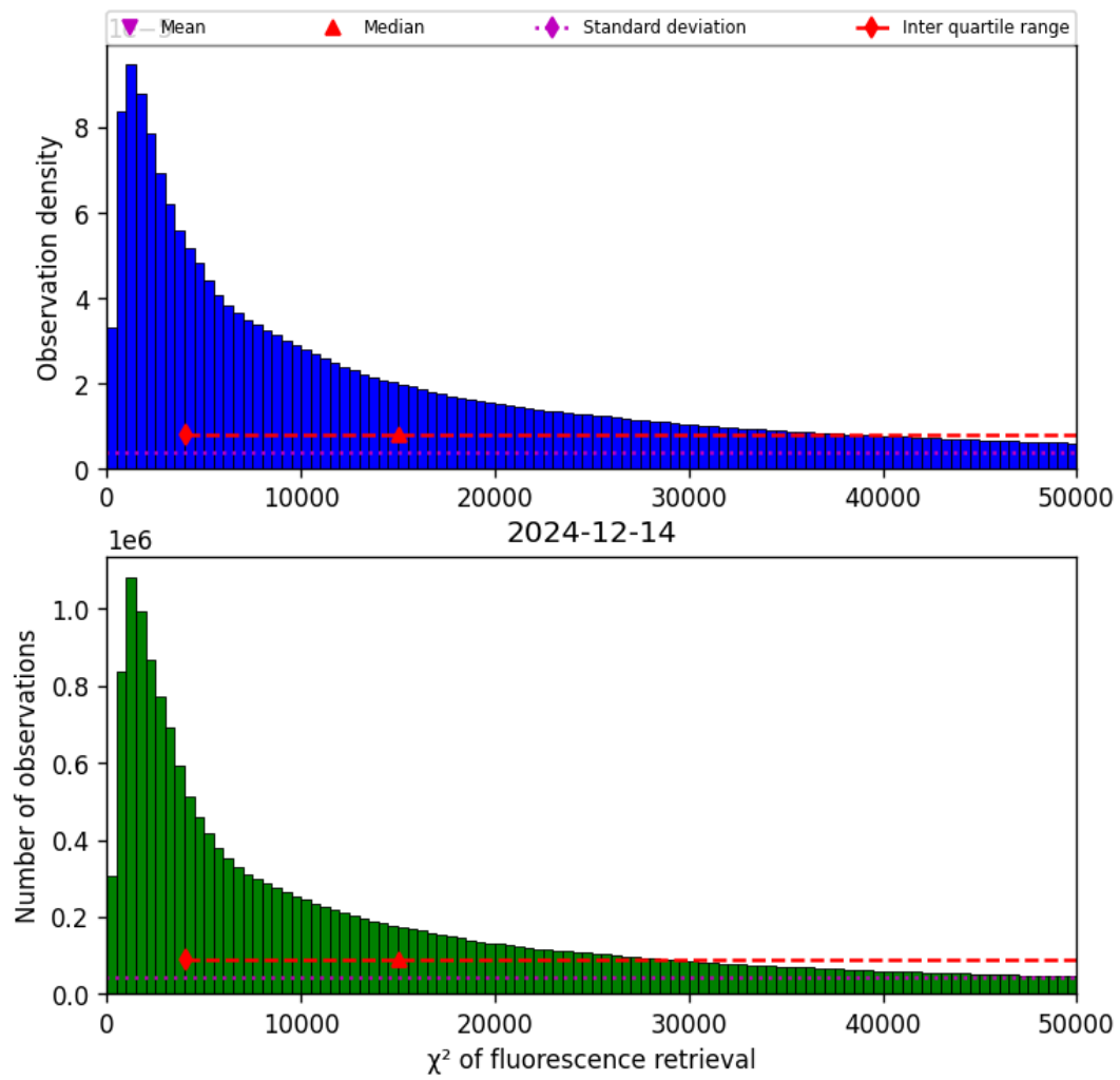
Figure 42: Histogram of “ \chi^2 of fluorescence retrieval” for 2024-12-13 to 2024-12-15
