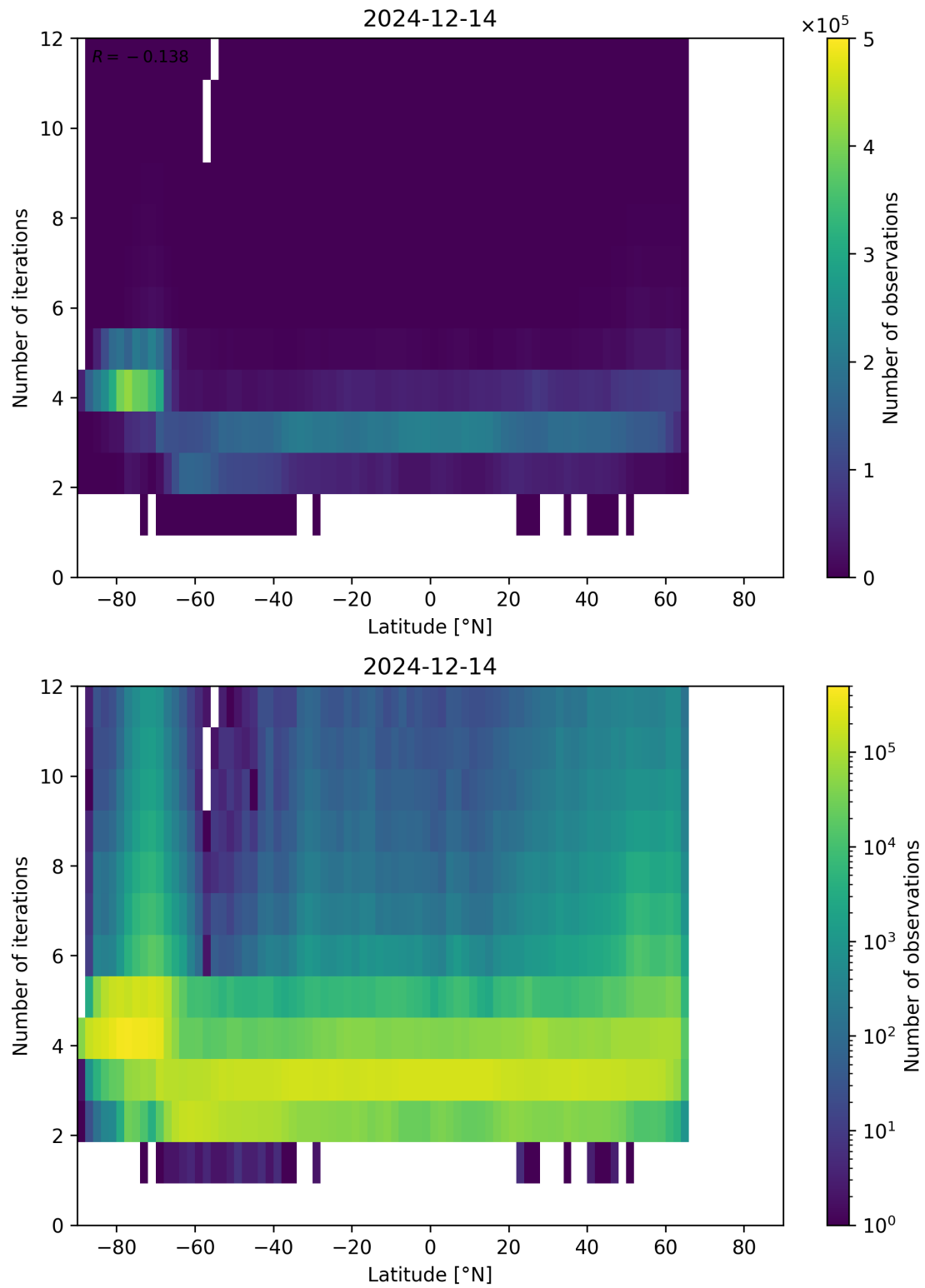
Figure 93: Scatter density plot of “Latitude” against “Number of iterations” for 2024-12-13 to 2024-12-15.
