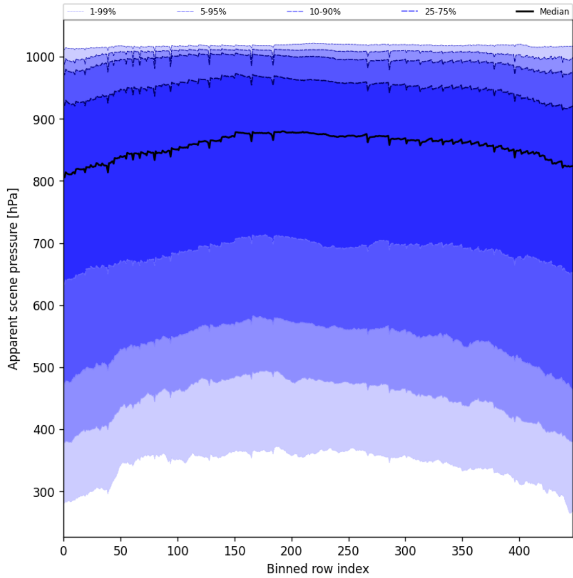
Figure 53: Along track statistics of “Apparent scene pressure” for 2024-12-13 to 2024-12-15
