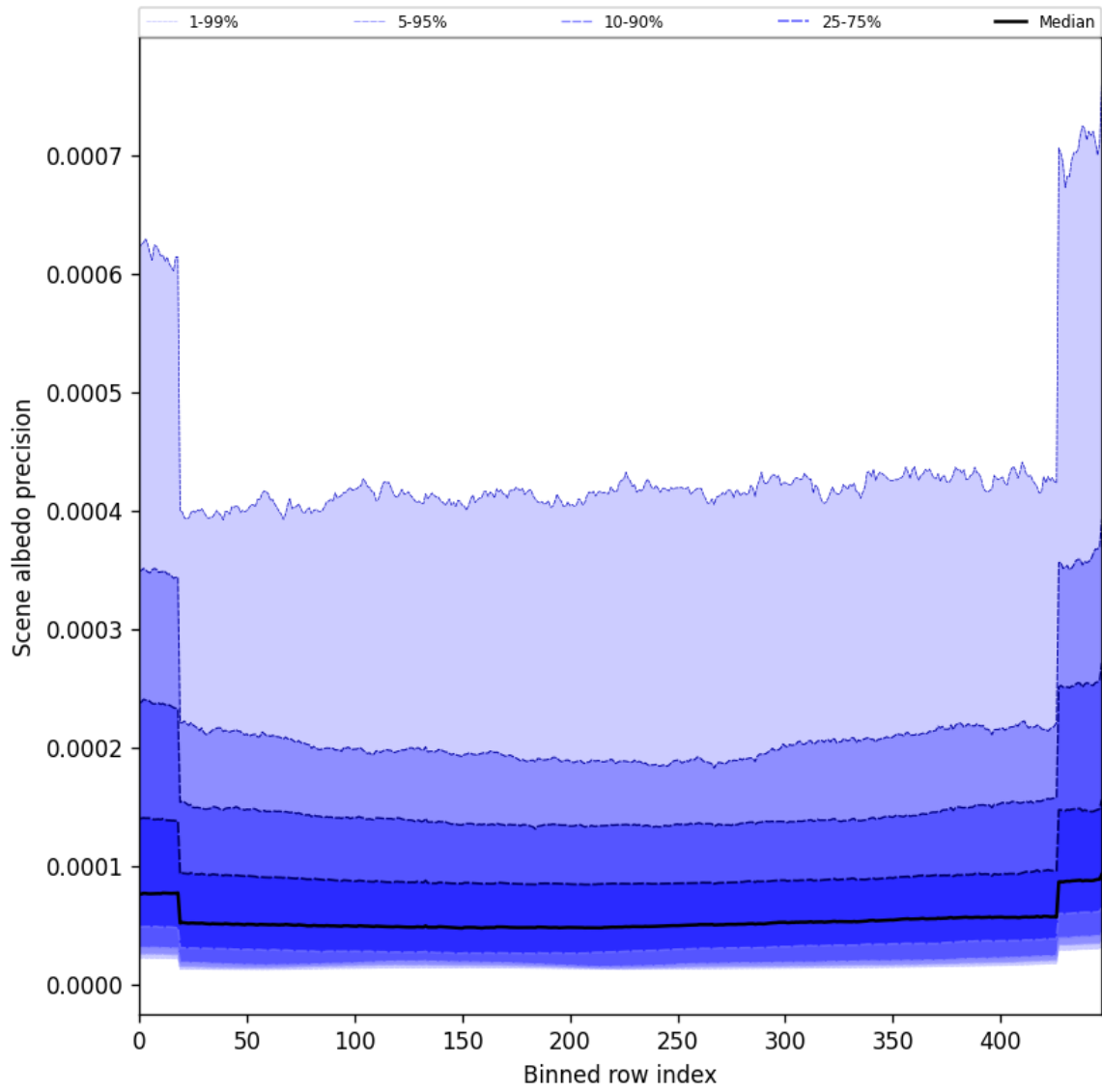
Figure 52: Along track statistics of “Scene albedo precision” for 2024-12-13 to 2024-12-15
