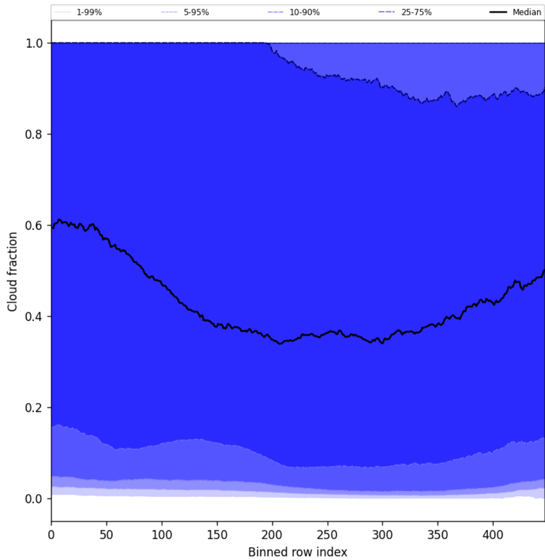
Figure 49: Along track statistics of “Cloud fraction” for 2024-12-13 to 2024-12-15
