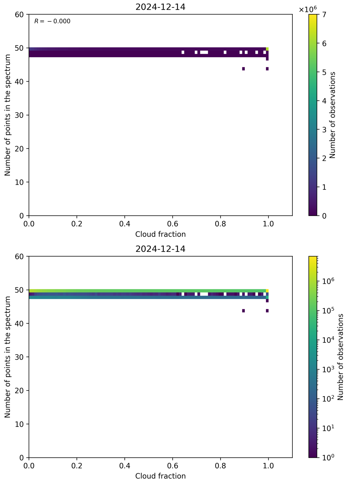
Figure 74: Scatter density plot of “Cloud fraction” against “Number of points in the spectrum” for 2024-12-13 to 2024-12-15.
