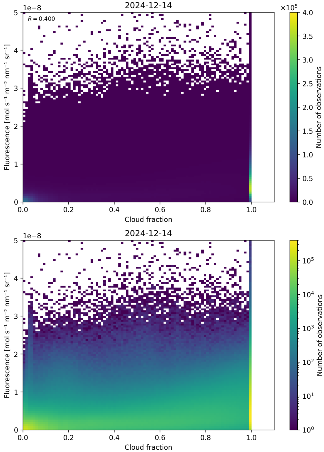
Figure 72: Scatter density plot of “Cloud fraction” against “Fluorescence” for 2024-12-13 to 2024-12-15.
