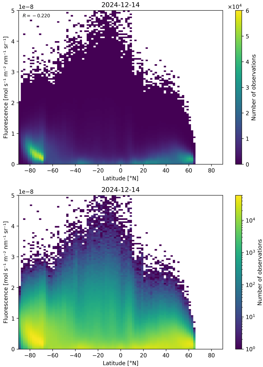
Figure 92: Scatter density plot of “Latitude” against “Fluorescence” for 2024-12-13 to 2024-12-15.
