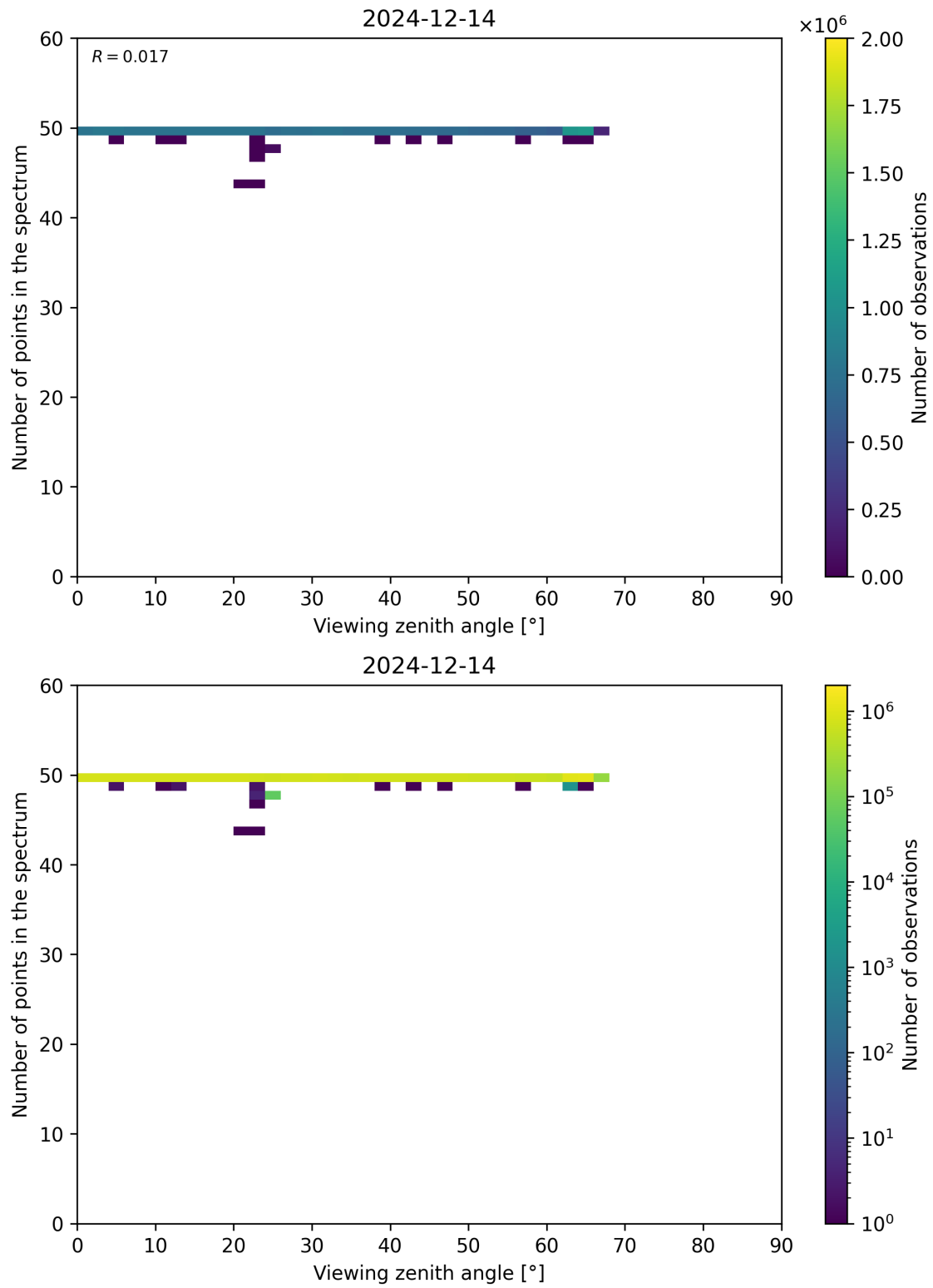
Figure 125: Scatter density plot of “Viewing zenith angle” against “Number of points in the spectrum” for 2024-12-13 to 2024-12-15.
