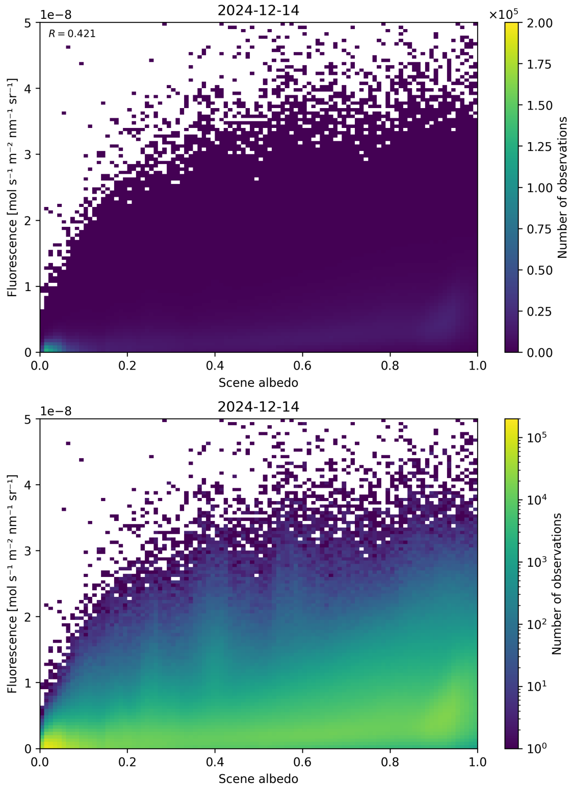
Figure 104: Scatter density plot of “Scene albedo” against “Fluorescence” for 2024-12-13 to 2024-12-15.
