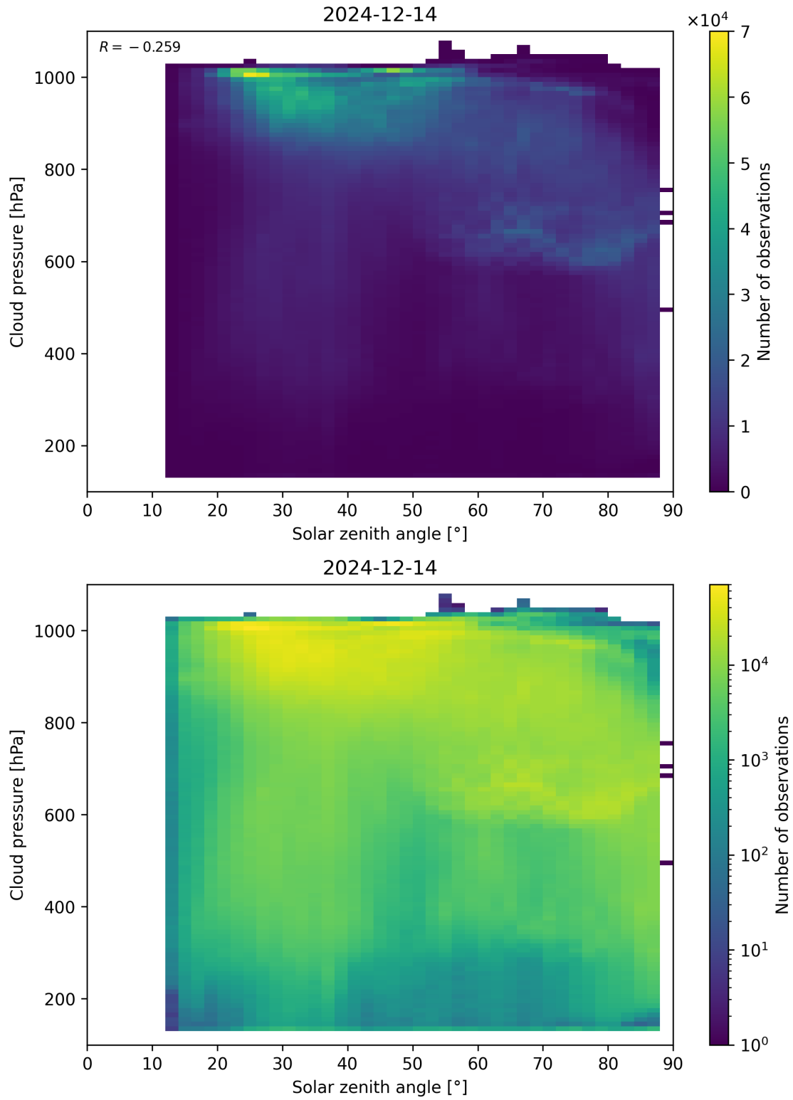
Figure 111: Scatter density plot of “Solar zenith angle” against “Cloud pressure” for 2024-12-13 to 2024-12-15.
