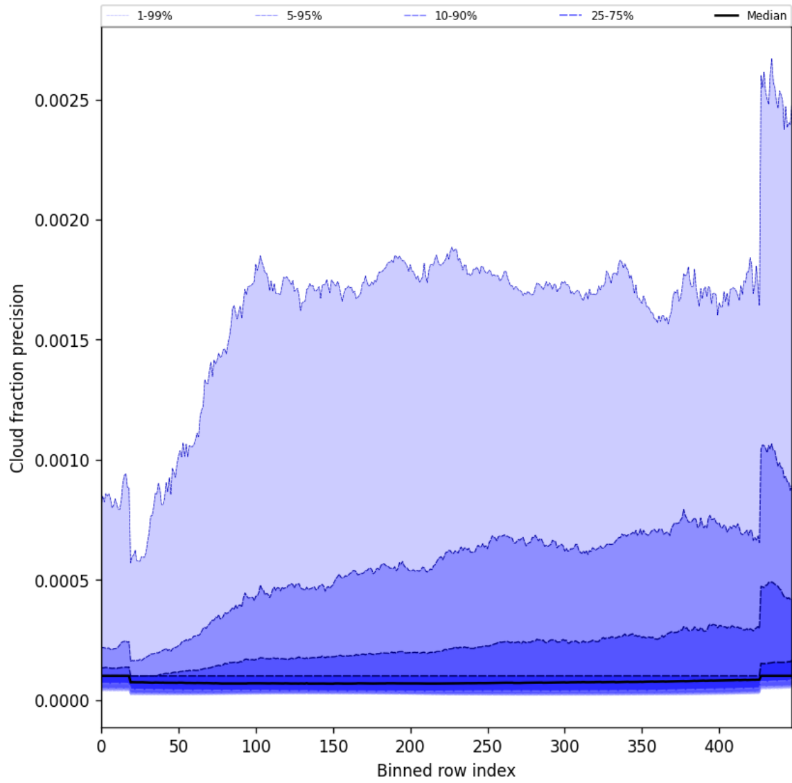
Figure 50: Along track statistics of “Cloud fraction precision” for 2024-12-13 to 2024-12-15
