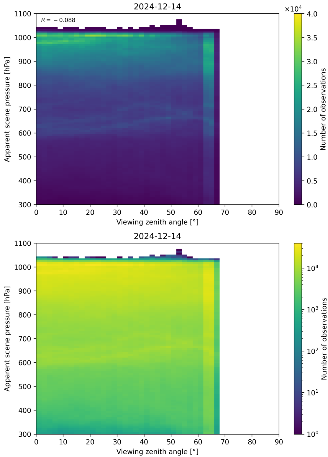
Figure 118: Scatter density plot of “Viewing zenith angle” against “Apparent scene pressure” for 2024-12-13 to 2024-12-15.
