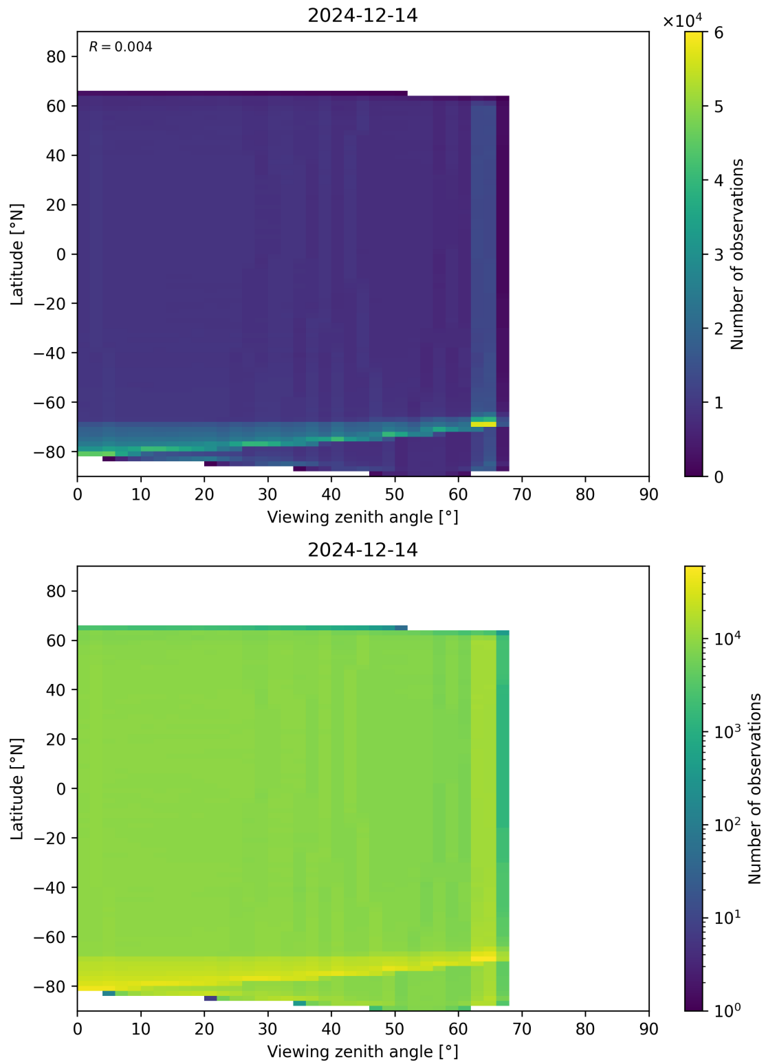
Figure 123: Scatter density plot of “Viewing zenith angle” against “Latitude” for 2024-12-13 to 2024-12-15.
