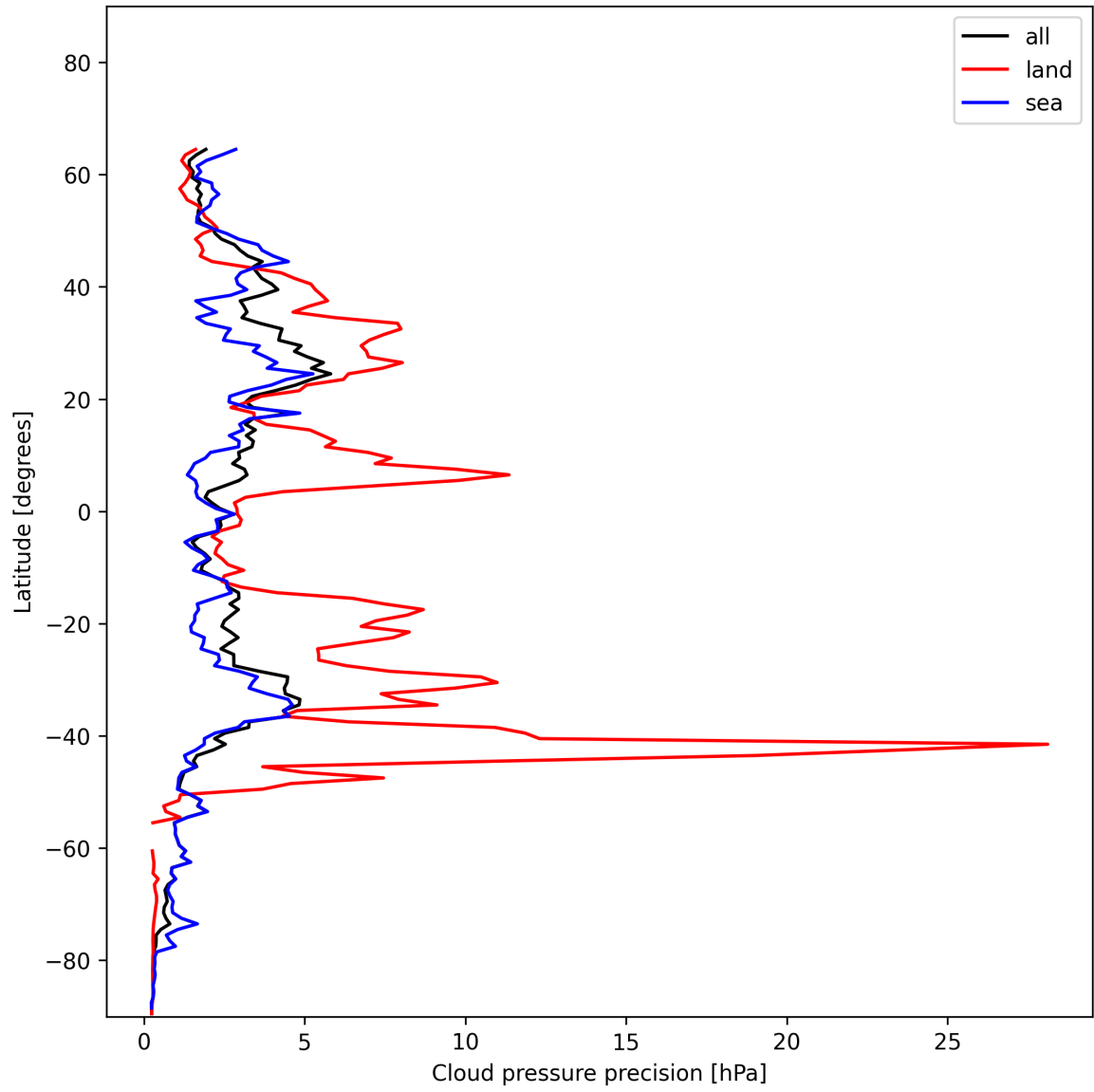
Figure 14: Zonal average of “Cloud pressure precision” for 2024-12-13 to 2024-12-15.
