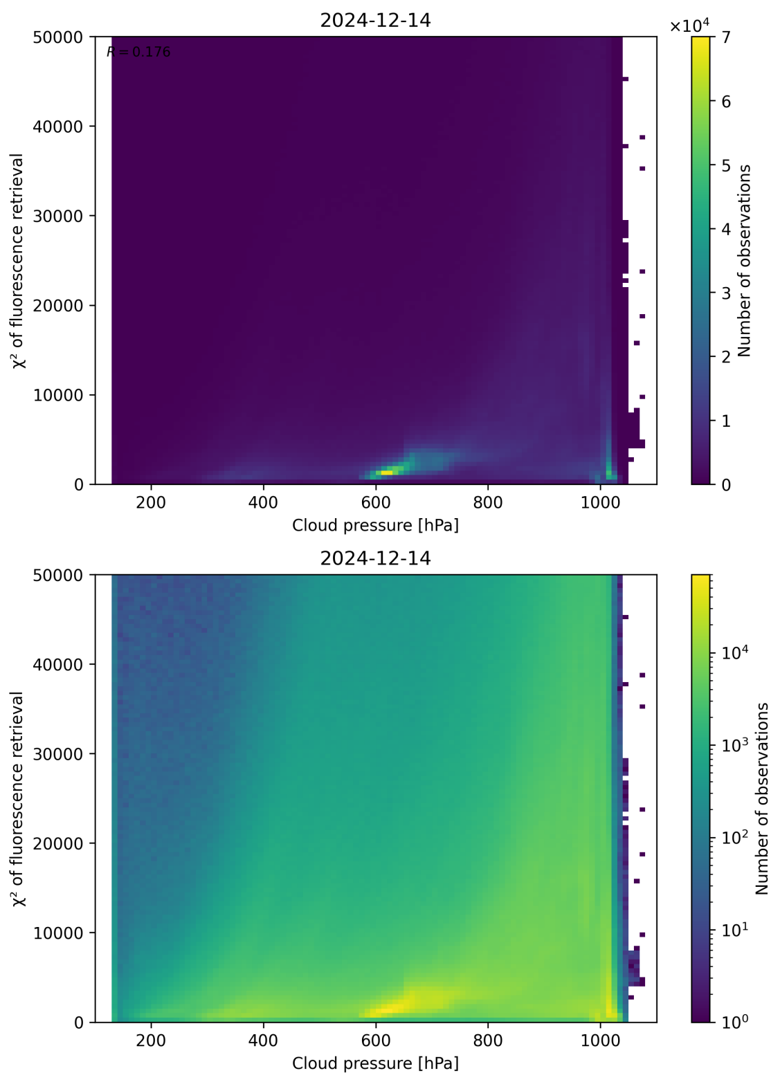
Figure 78: Scatter density plot of “Cloud pressure” against “ \chi^2 of fluorescence retrieval” for 2024-12-13 to 2024-12-15.
