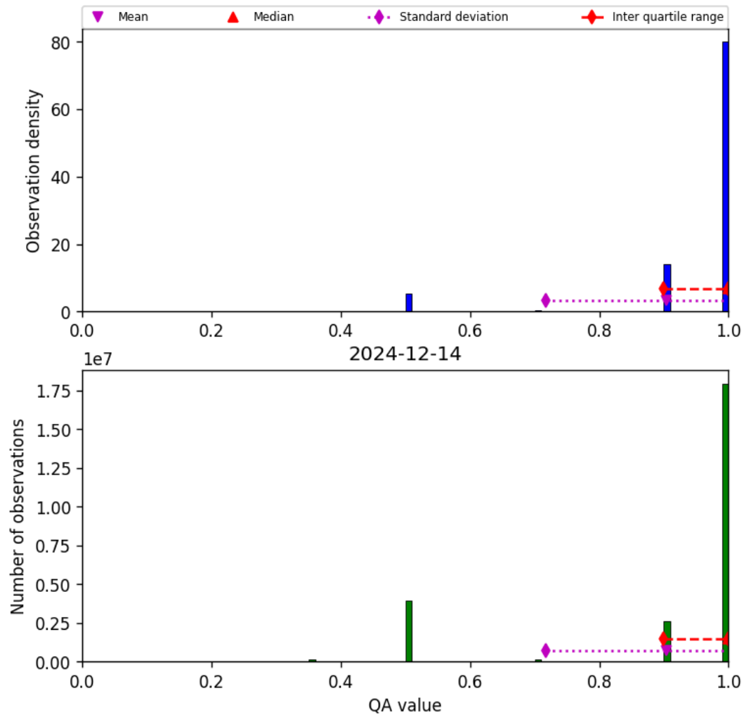
Figure 29: Histogram of “QA value” for 2024-12-13 to 2024-12-15
