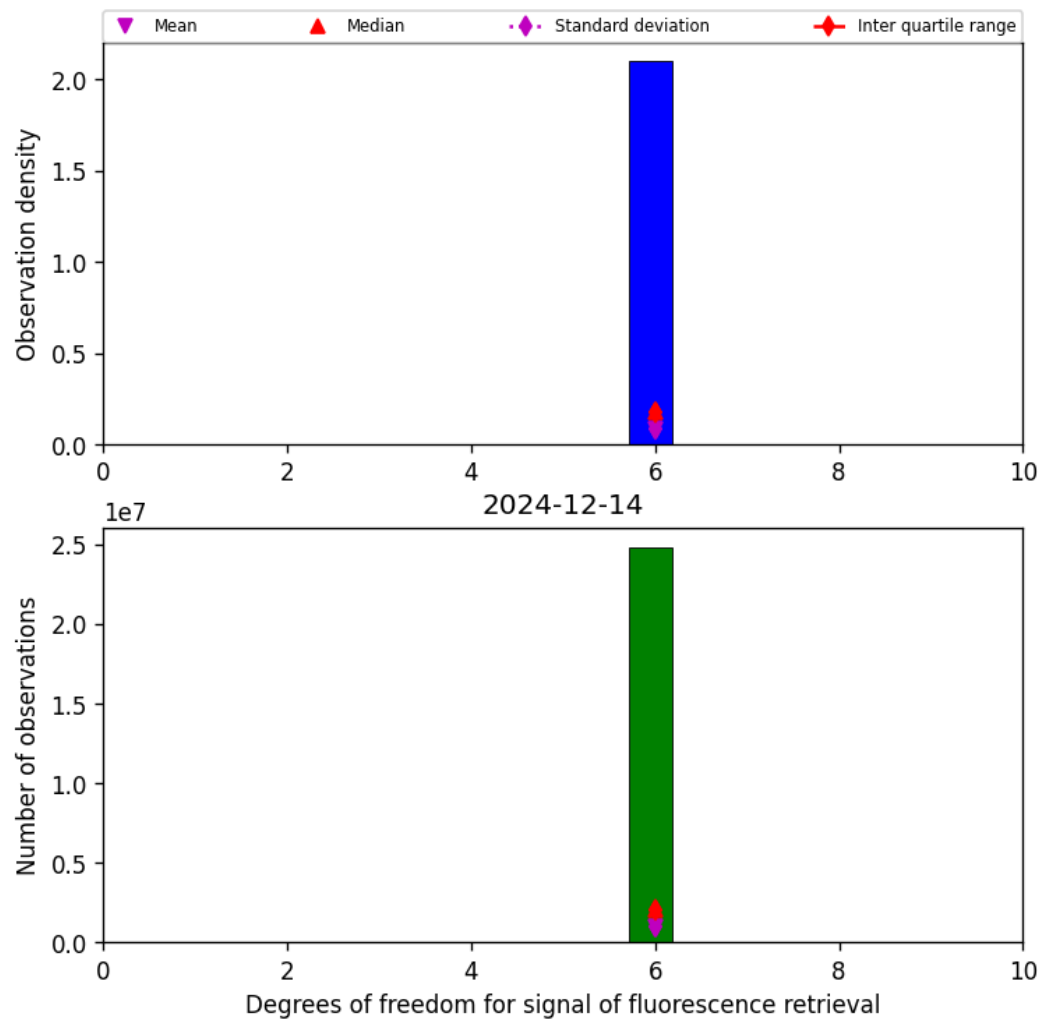
Figure 43: Histogram of “Degrees of freedom for signal of fluorescence retrieval” for 2024-12-13 to 2024-12-15
