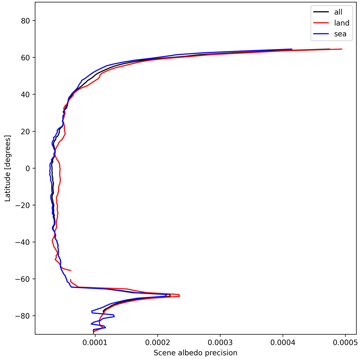
Figure 18: Zonal average of “Scene albedo precision” for 2024-12-13 to 2024-12-15.
