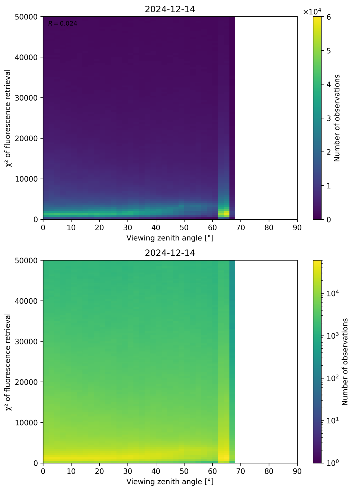
Figure 119: Scatter density plot of “Viewing zenith angle” against “ \chi^2 of fluorescence retrieval” for 2024-12-13 to 2024-12-15.
