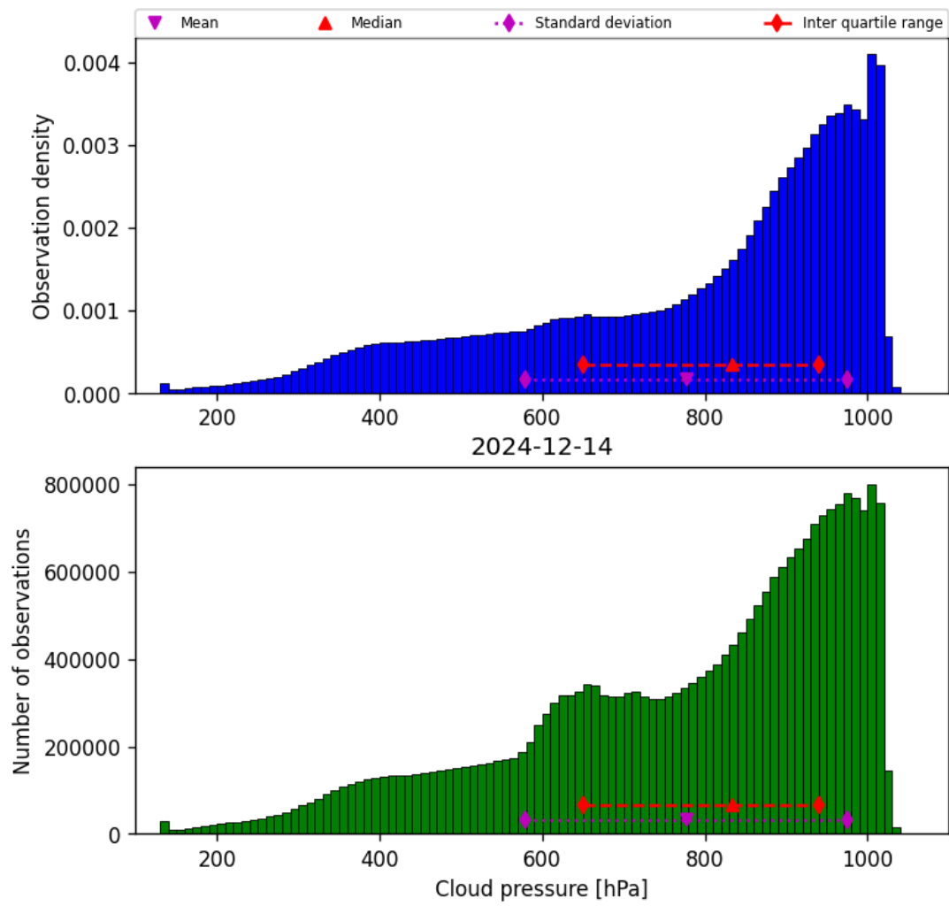
Figure 30: Histogram of “Cloud pressure” for 2024-12-13 to 2024-12-15
