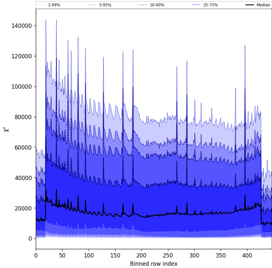
Figure 55: Along track statistics of “ \chi^2 ” for 2024-12-13 to 2024-12-15
