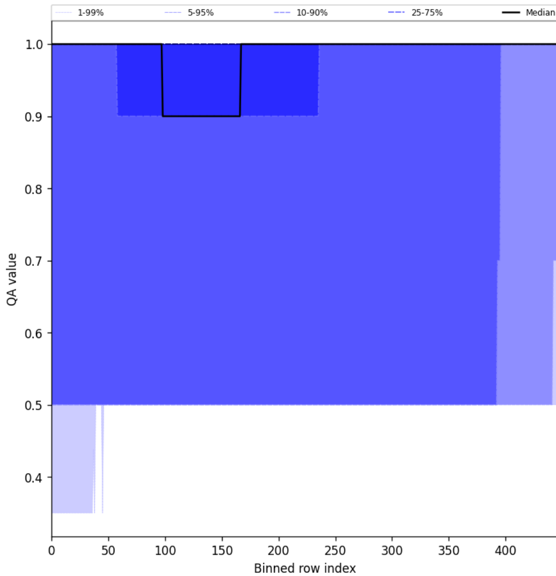
Figure 46: Along track statistics of “QA value” for 2024-12-13 to 2024-12-15
