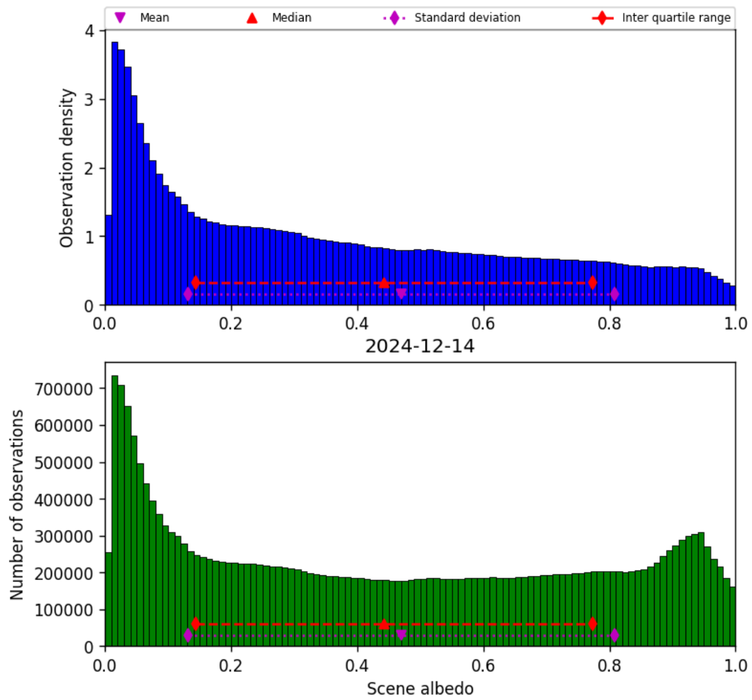
Figure 34: Histogram of “Scene albedo” for 2024-12-13 to 2024-12-15
