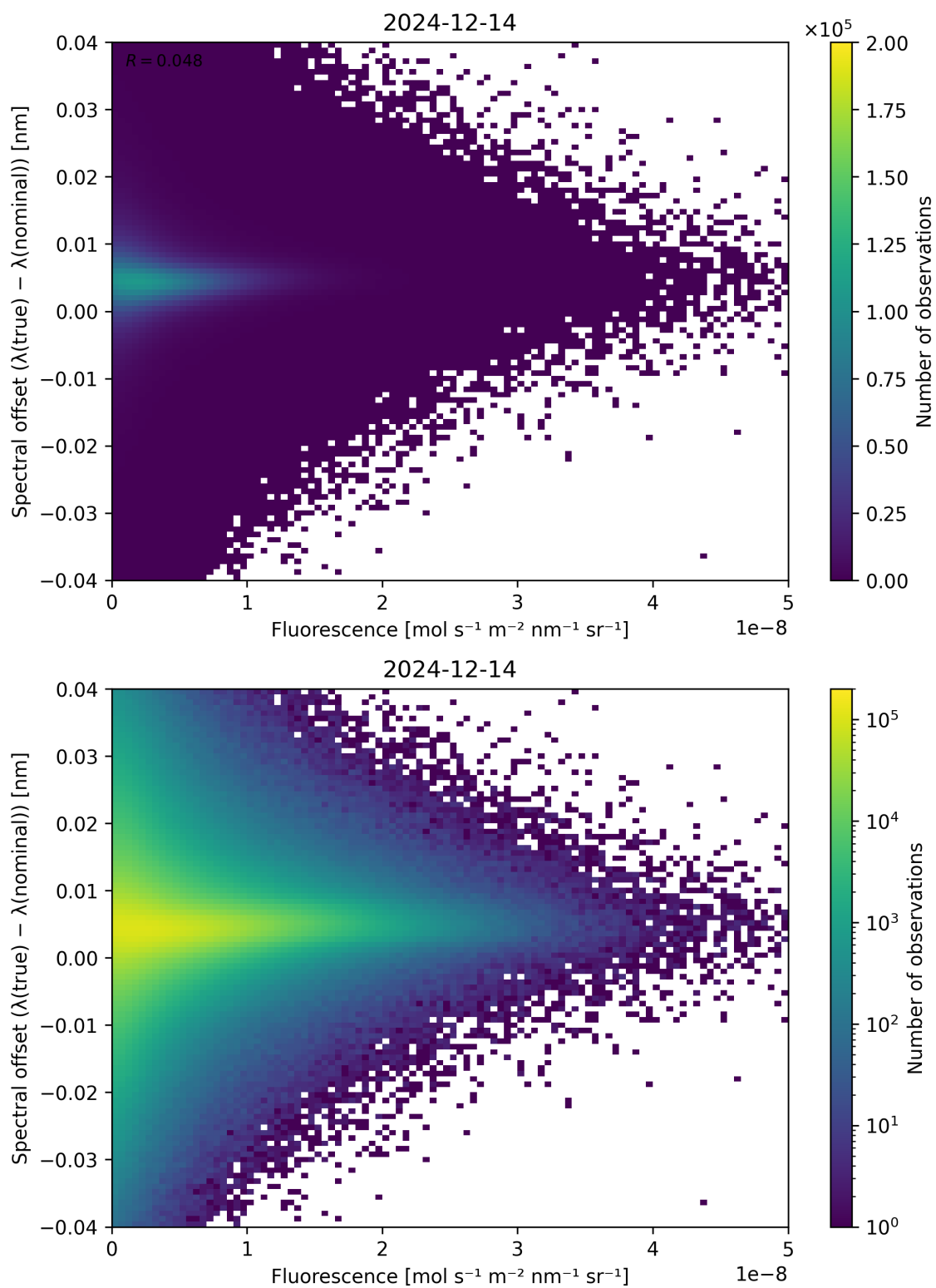
Figure 87: Scatter density plot of “Fluorescence” against “Spectral offset ( \lambda_{\text{true}} - \lambda_{\text{nominal}} )” for 2024-12-13 to 2024-12-15.
