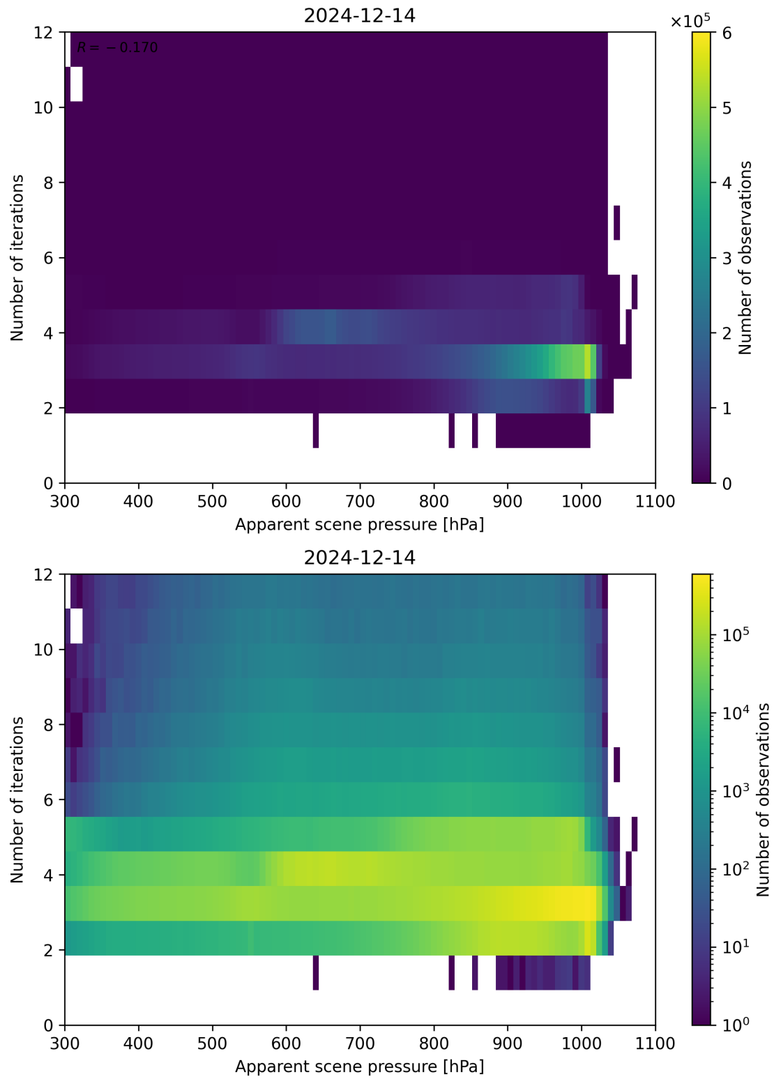
Figure 65: Scatter density plot of “Apparent scene pressure” against “Number of iterations” for 2024-12-13 to 2024-12-15.
