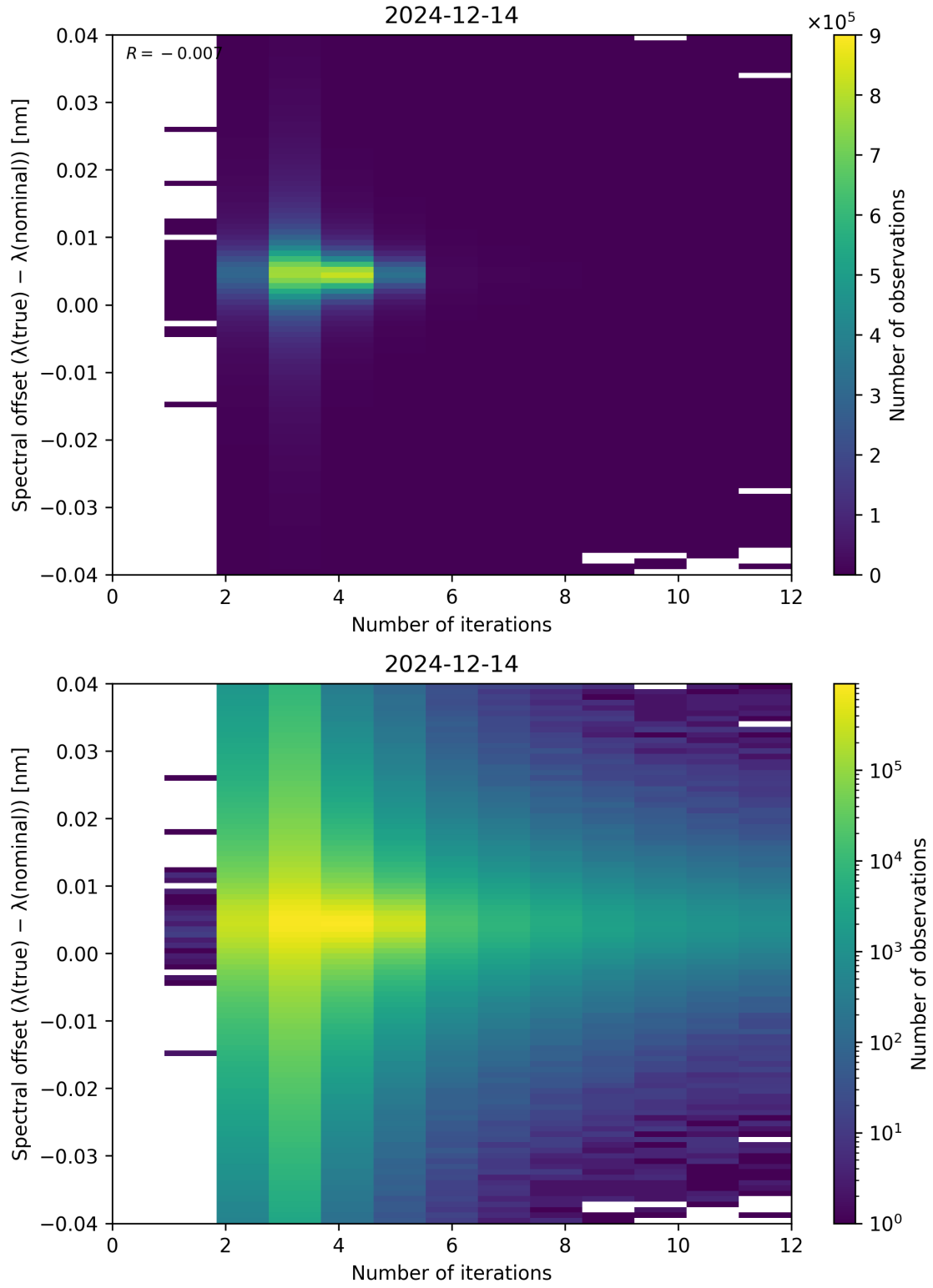
Figure 100: Scatter density plot of “Number of iterations” against “Spectral offset ( \lambda_{\text{true}} - \lambda_{\text{nominal}} )” for 2024-12-13 to 2024-12-15.
