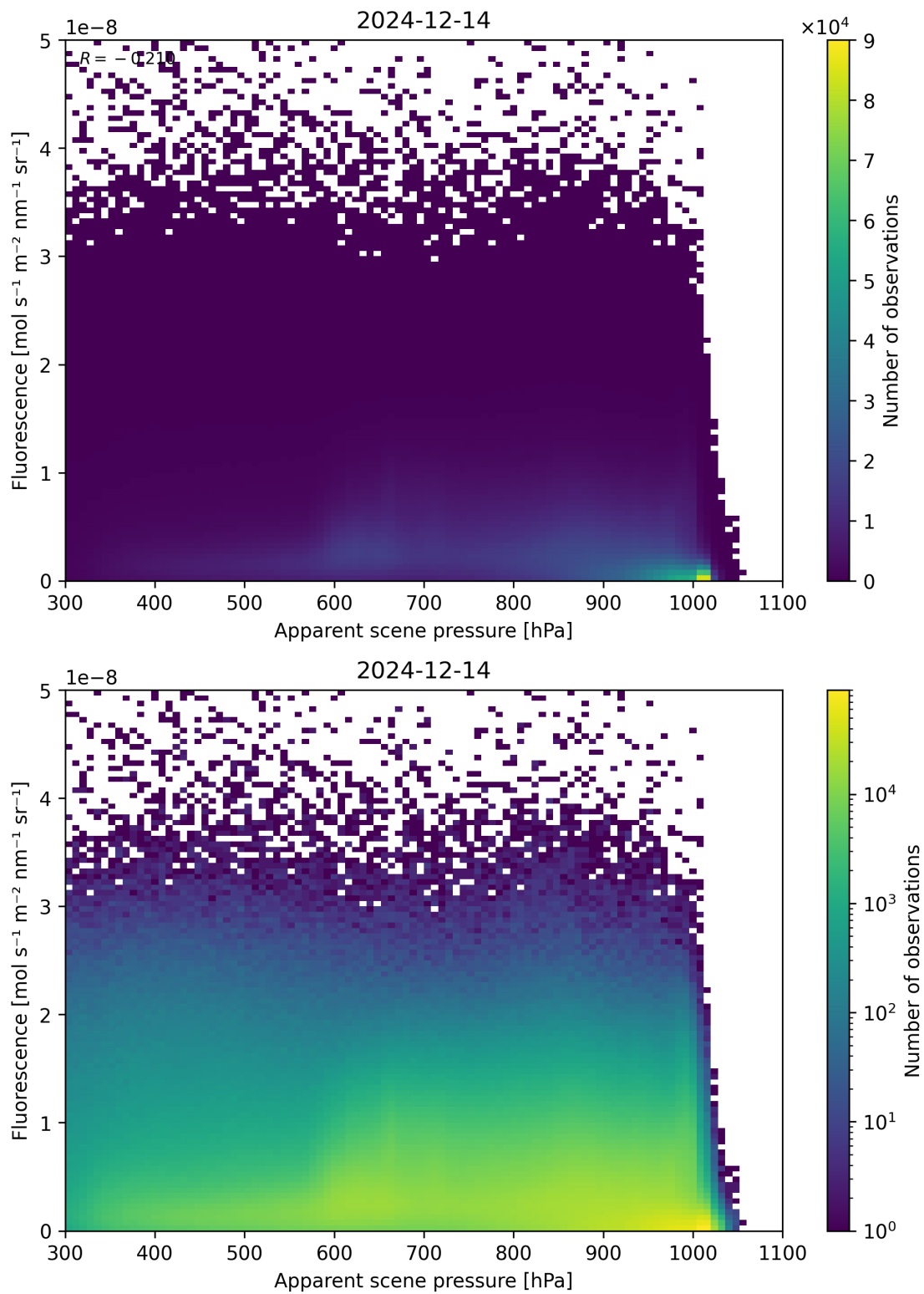
Figure 64: Scatter density plot of “Apparent scene pressure” against “Fluorescence” for 2024-12-13 to 2024-12-15.
