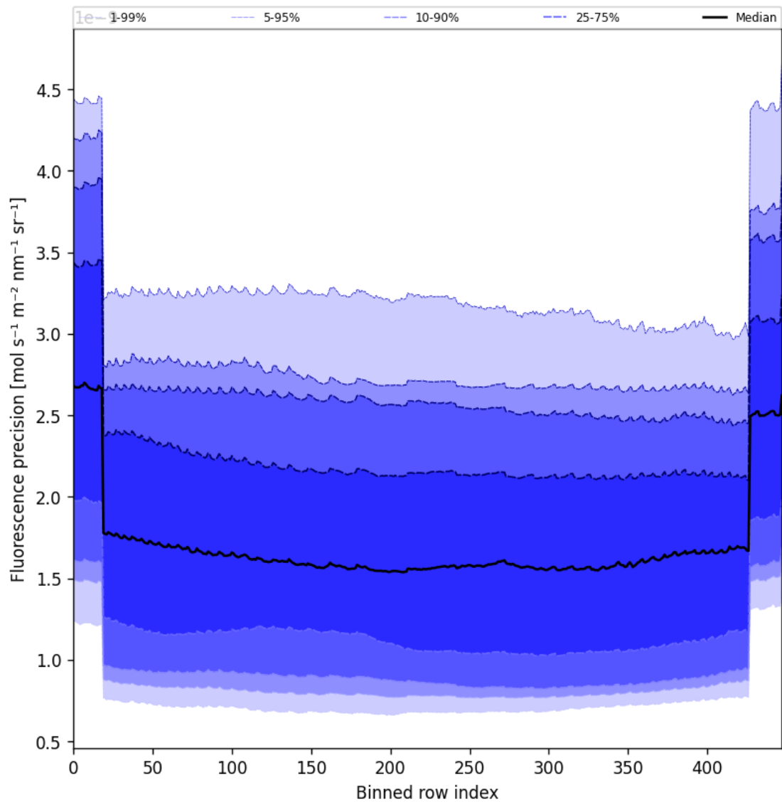
Figure 58: Along track statistics of “Fluorescence precision” for 2024-12-13 to 2024-12-15
