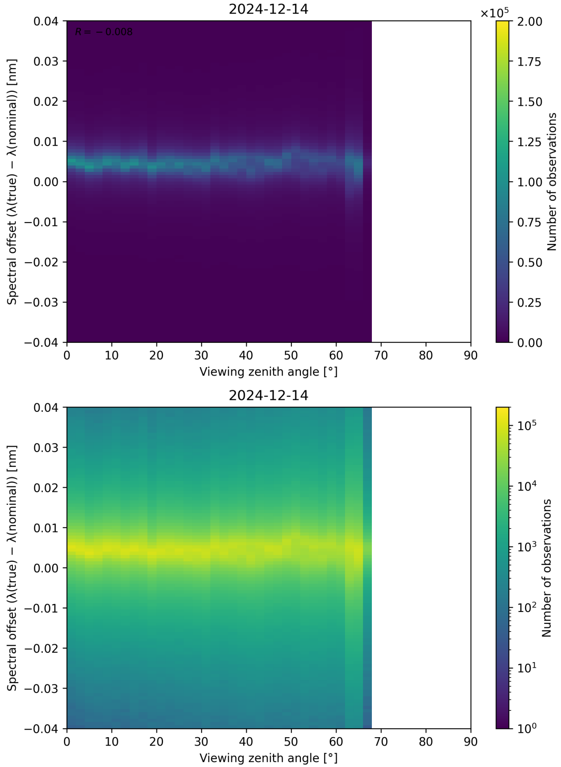
Figure 128: Scatter density plot of “Viewing zenith angle” against “Spectral offset ( \lambda_{\text{true}} - \lambda_{\text{nominal}} )” for 2024-12-13 to 2024-12-15.
