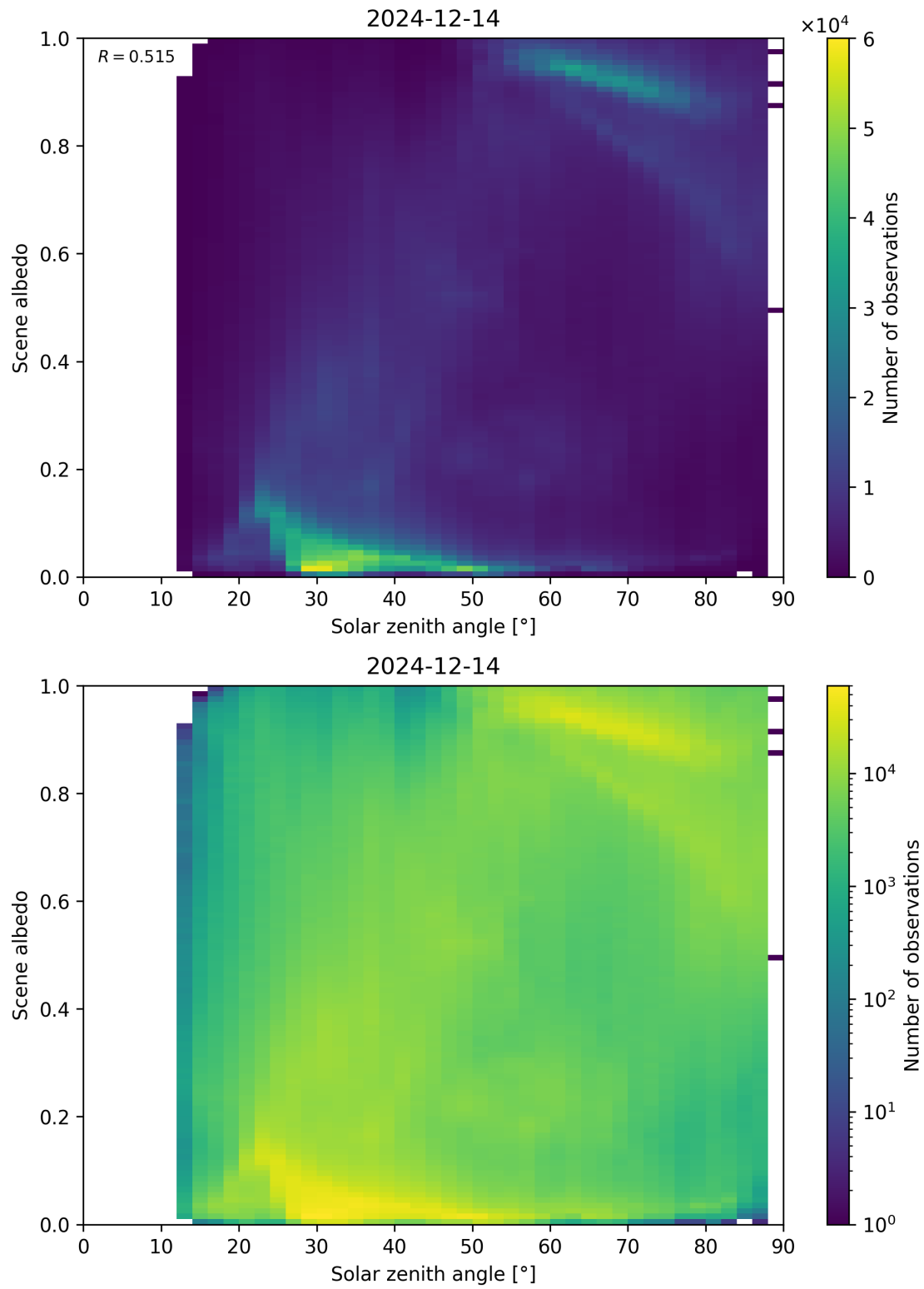
Figure 116: Scatter density plot of “Solar zenith angle” against “Scene albedo” for 2024-12-13 to 2024-12-15.
