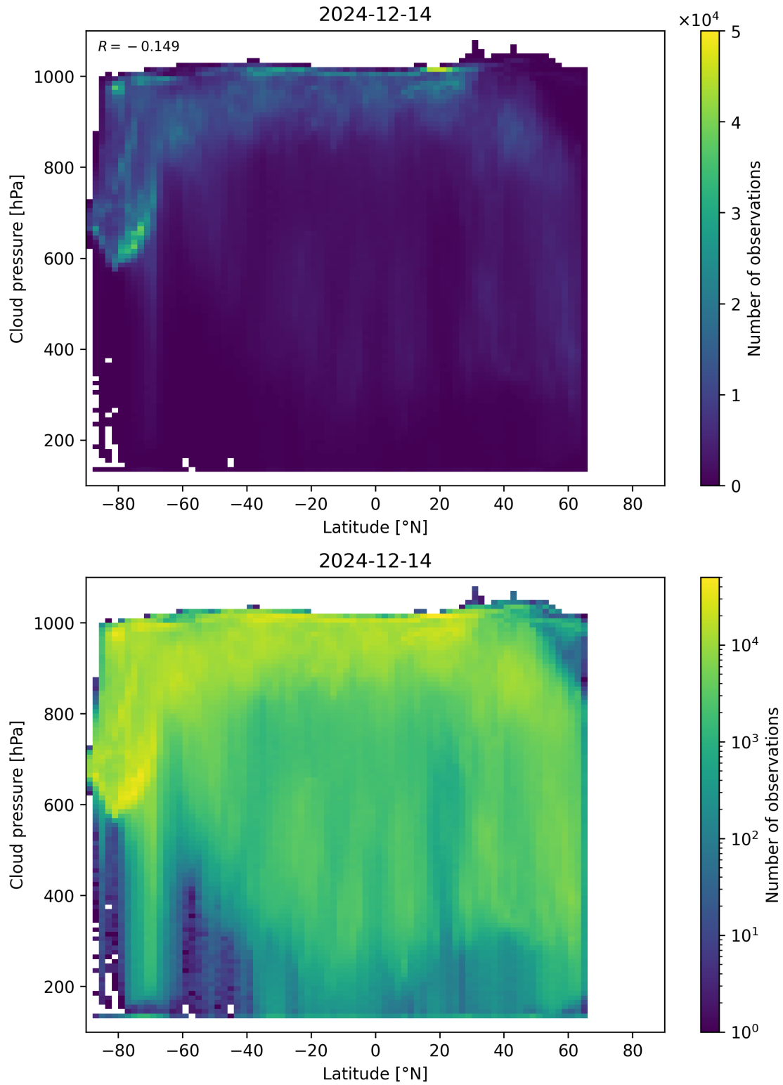
Figure 91: Scatter density plot of “Latitude” against “Cloud pressure” for 2024-12-13 to 2024-12-15.
