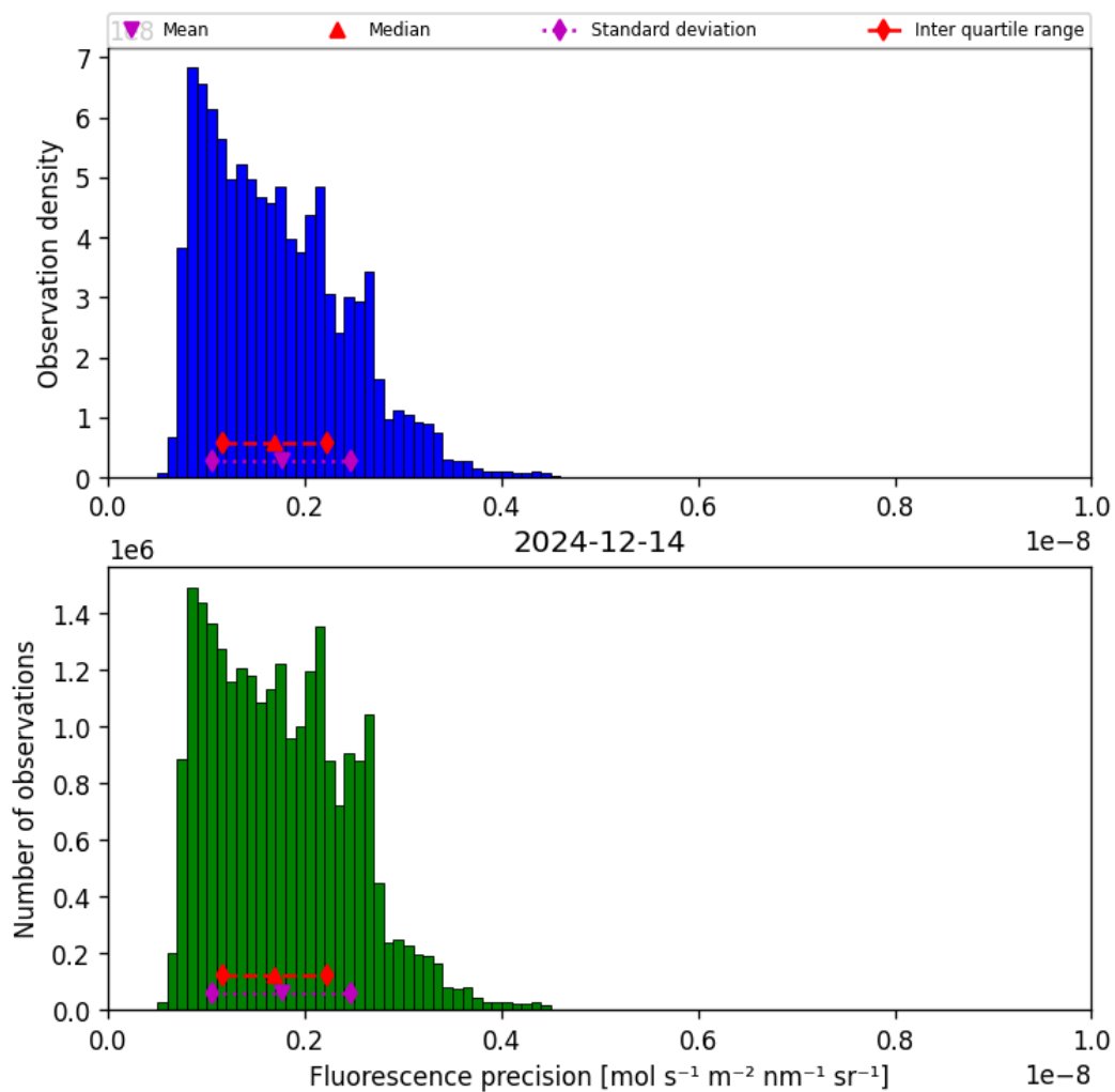
Figure 41: Histogram of “Fluorescence precision” for 2024-12-13 to 2024-12-15
