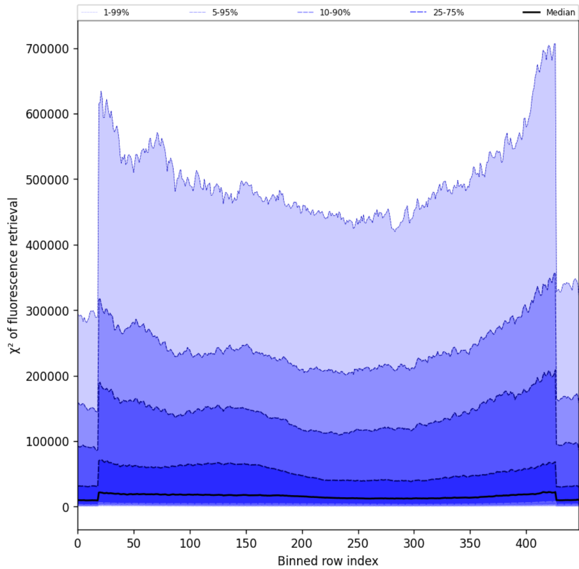
Figure 59: Along track statistics of “ \chi^2 of fluorescence retrieval” for 2024-12-13 to 2024-12-15
