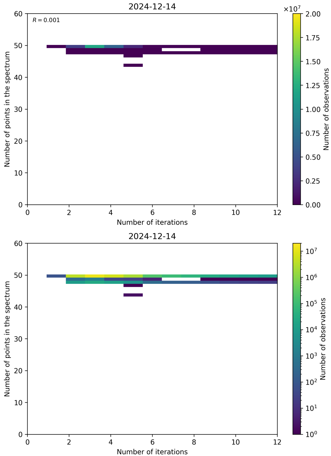
Figure 99: Scatter density plot of “Number of iterations” against “Number of points in the spectrum” for 2024-12-13 to 2024-12-15.
