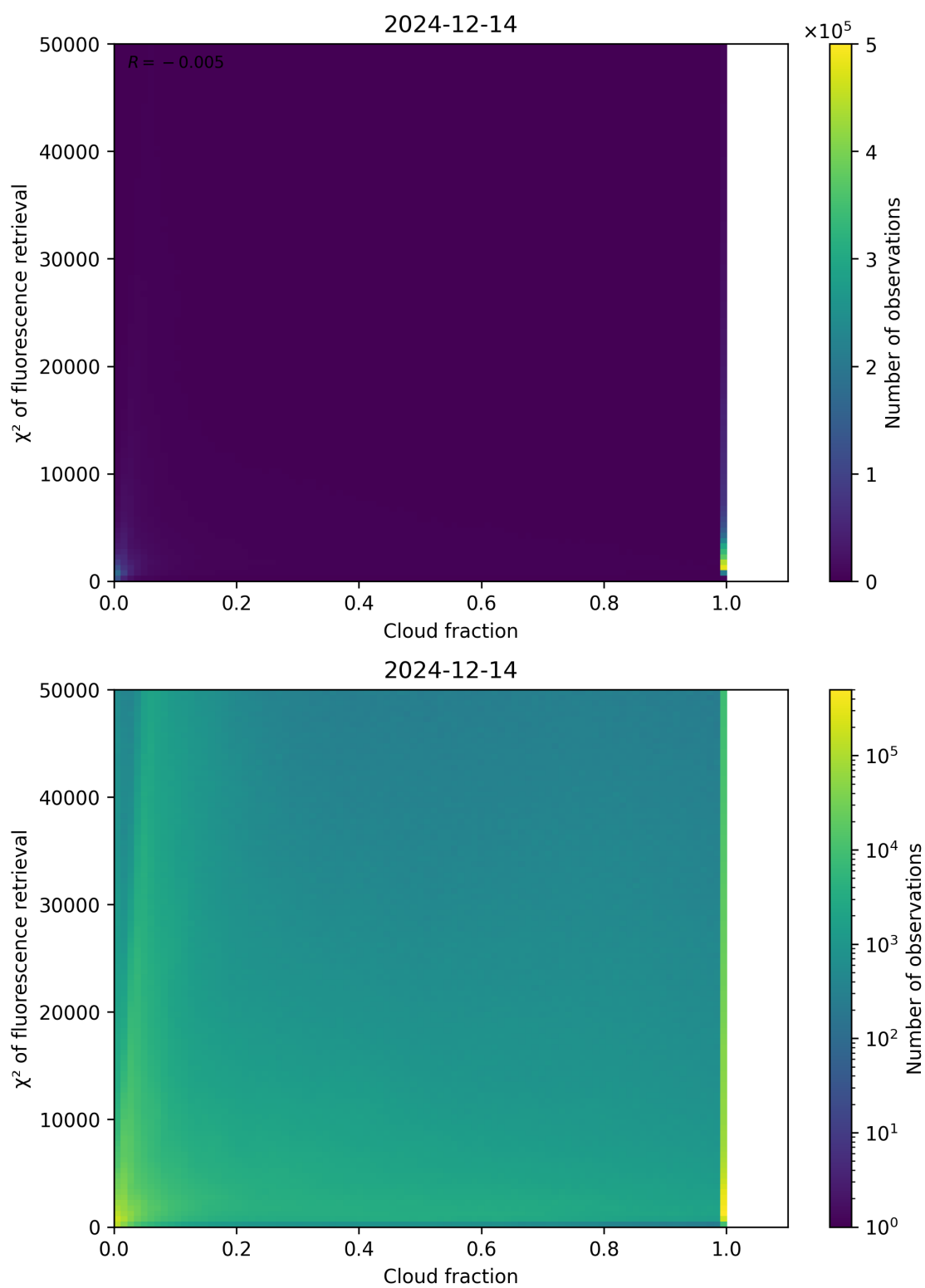
Figure 71: Scatter density plot of “Cloud fraction” against “ \chi^2 of fluorescence retrieval” for 2024-12-13 to 2024-12-15.
