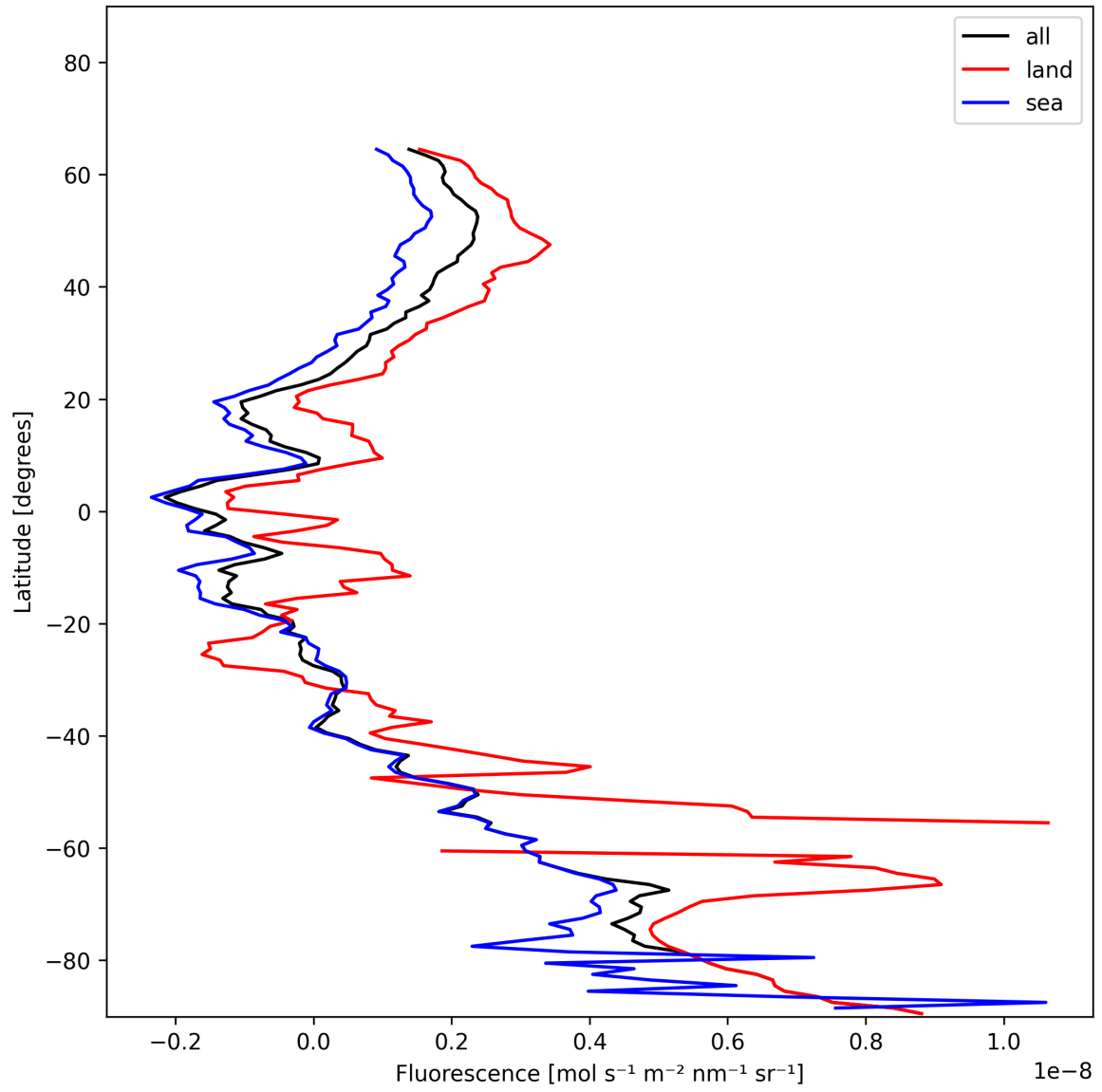
Figure 23: Zonal average of “Fluorescence” for 2024-12-13 to 2024-12-15.
