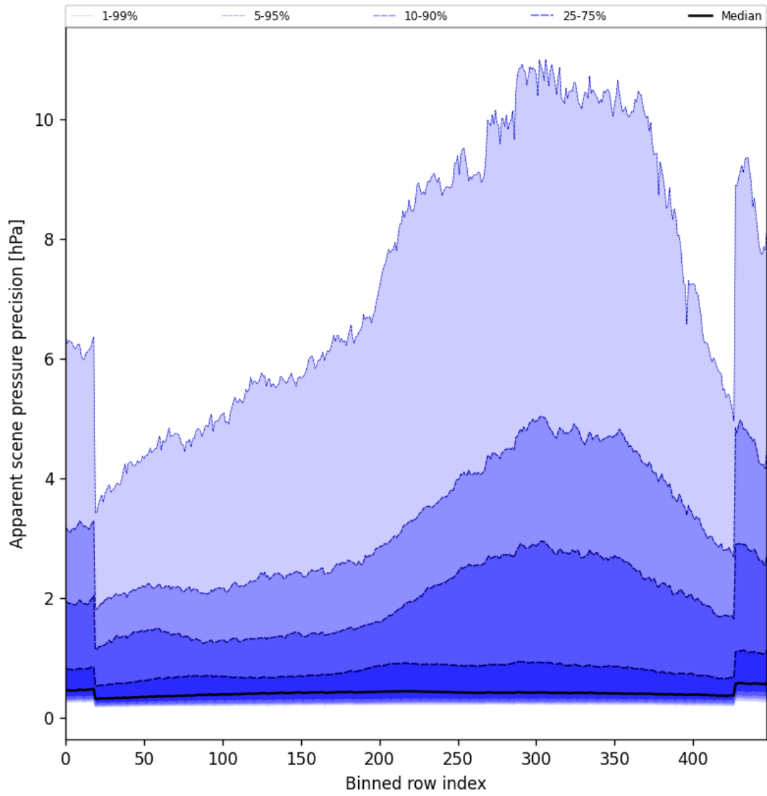
Figure 54: Along track statistics of “Apparent scene pressure precision” for 2024-12-13 to 2024-12-15
