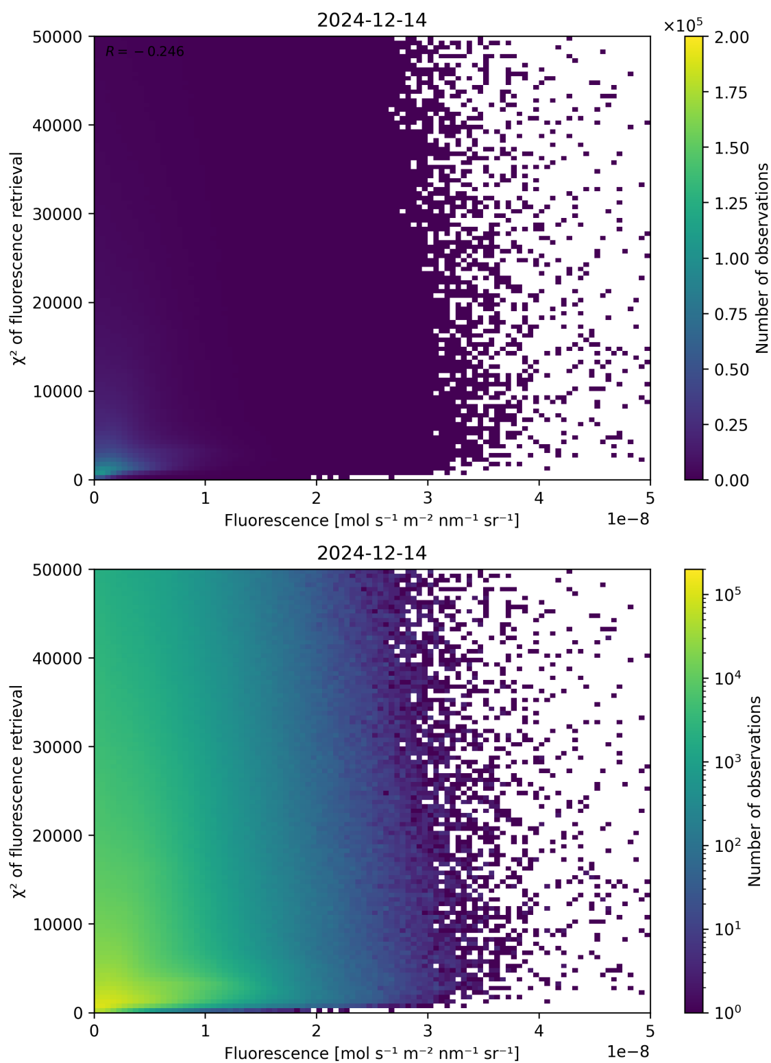
Figure 85: Scatter density plot of “Fluorescence” against “ \chi^2 of fluorescence retrieval” for 2024-12-13 to 2024-12-15.
