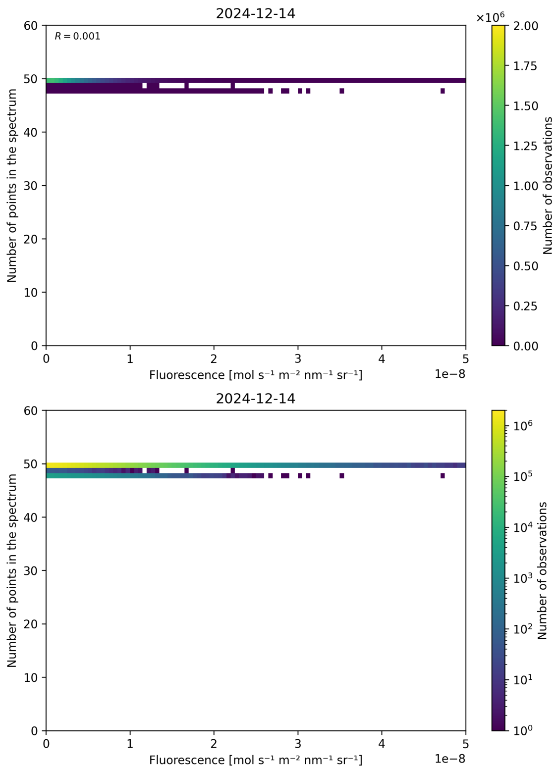
Figure 86: Scatter density plot of “Fluorescence” against “Number of points in the spectrum” for 2024-12-13 to 2024-12-15.
