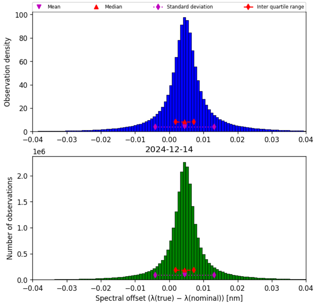
Figure 45: Histogram of “Spectral offset ( \lambda_{\text{true}} - \lambda_{\text{nominal}} )” for 2024-12-13 to 2024-12-15
