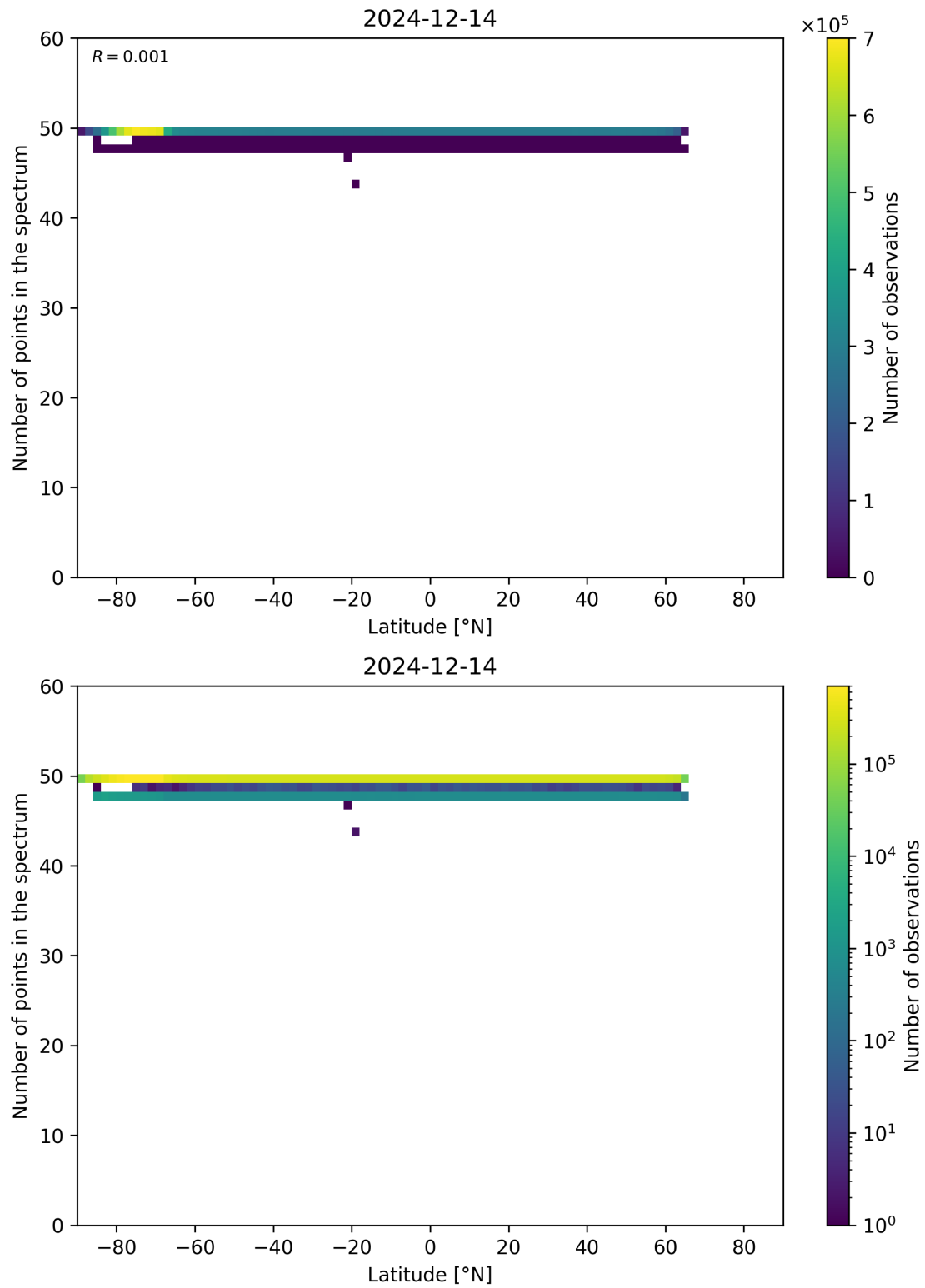
Figure 94: Scatter density plot of “Latitude” against “Number of points in the spectrum” for 2024-12-13 to 2024-12-15.
