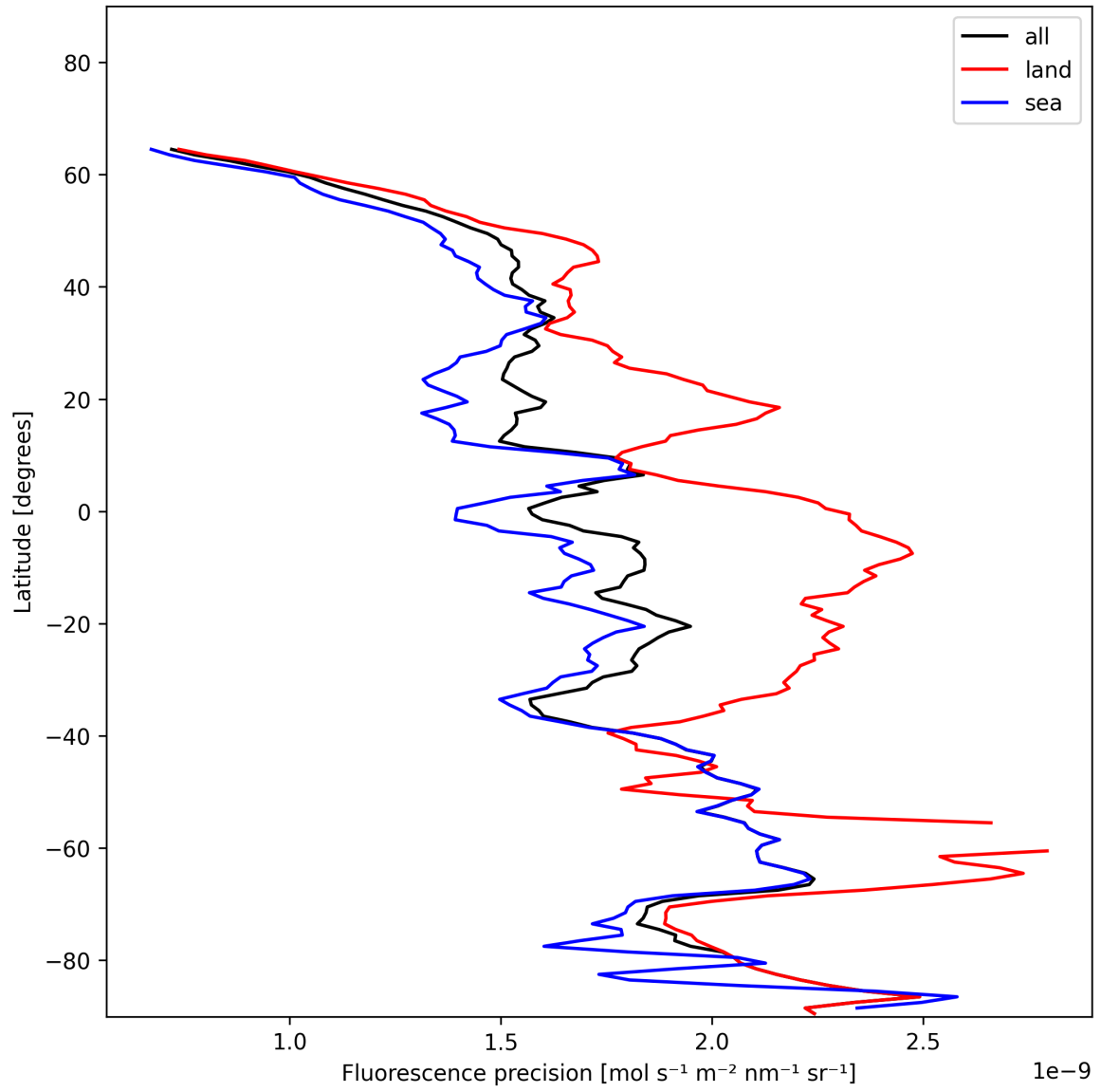
Figure 24: Zonal average of “Fluorescence precision” for 2024-12-13 to 2024-12-15.
