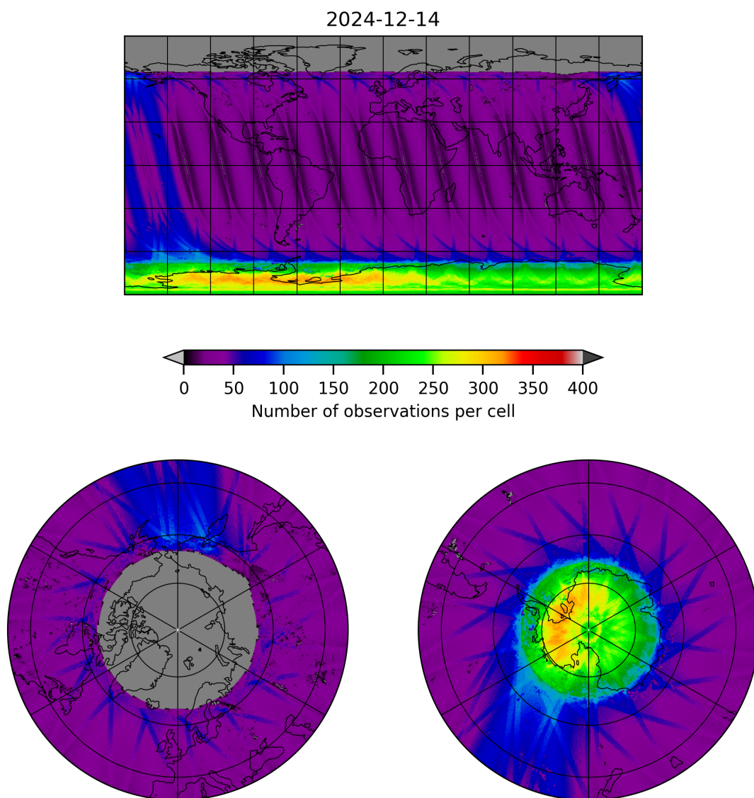
Figure 11: Map of the number of observations for 2024-12-13 to 2024-12-15
