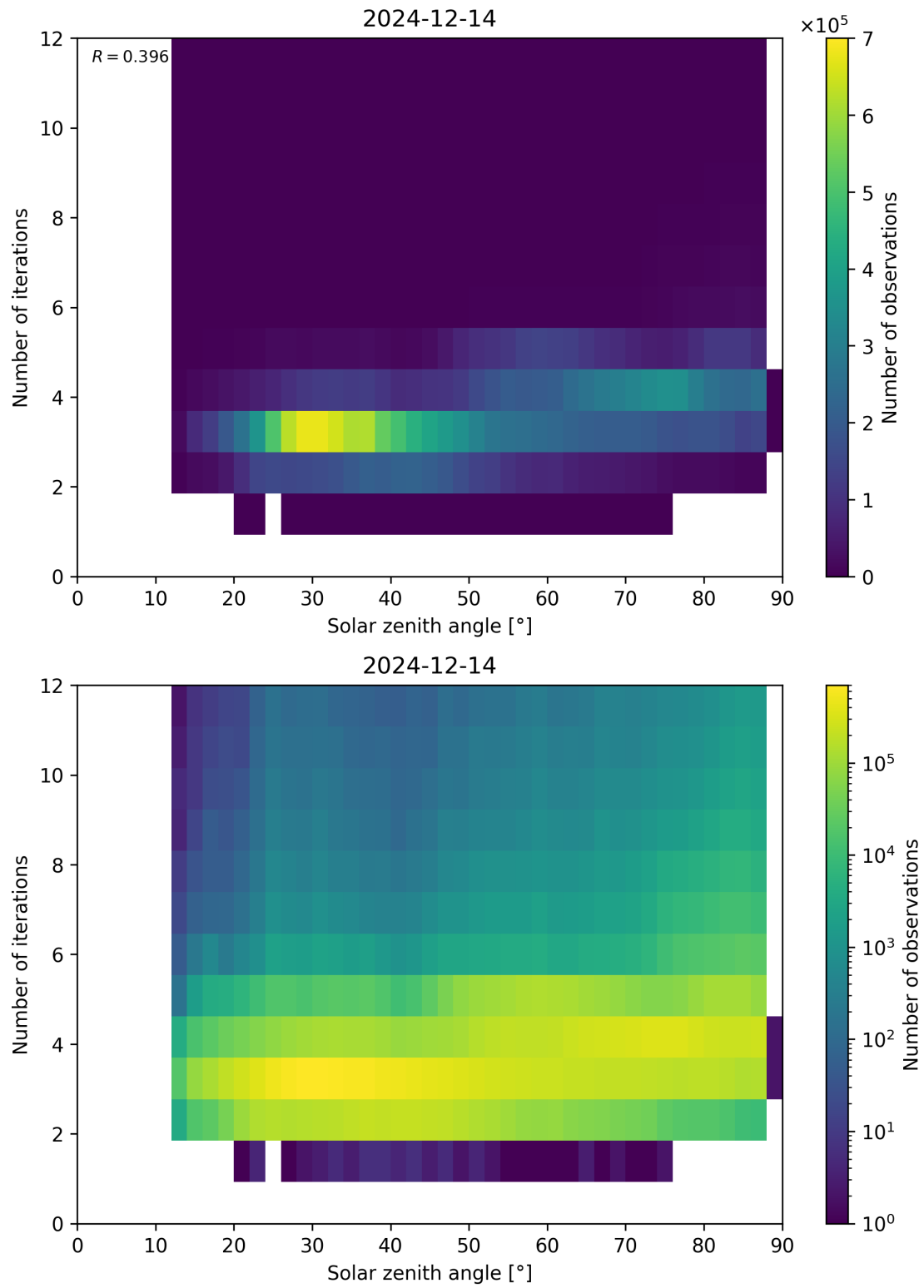
Figure 114: Scatter density plot of “Solar zenith angle” against “Number of iterations” for 2024-12-13 to 2024-12-15.
