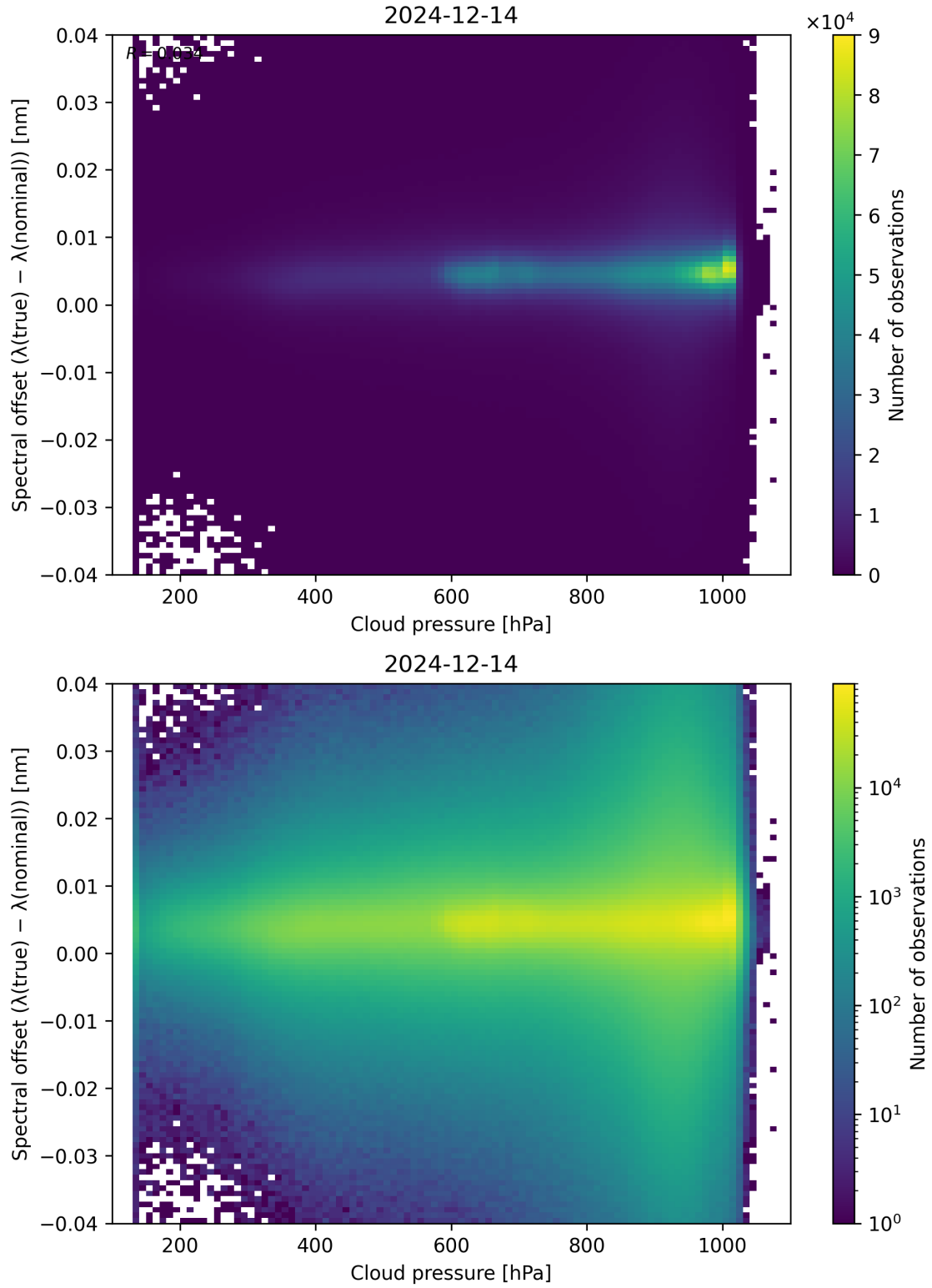
Figure 84: Scatter density plot of “Cloud pressure” against “Spectral offset ( \lambda_{\text{true}} - \lambda_{\text{nominal}} )” for 2024-12-13 to 2024-12-15.
