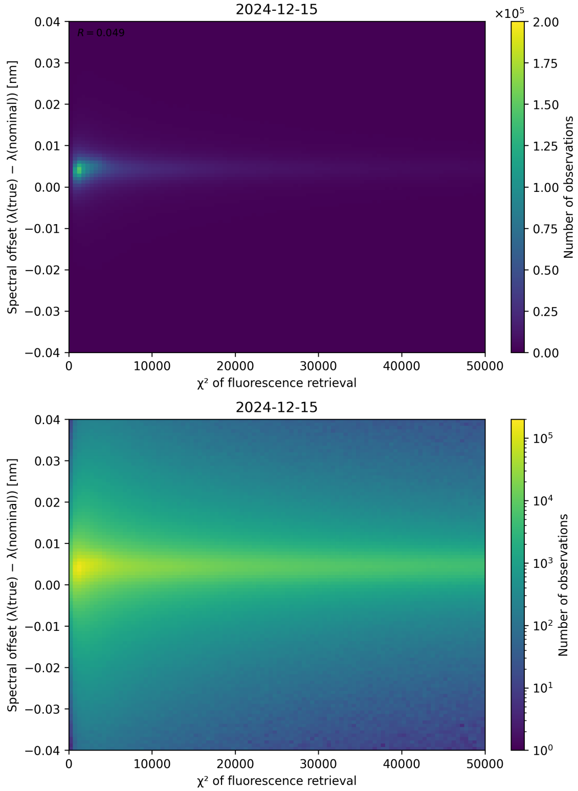
Figure 69: Scatter density plot of “ \chi^2 of fluorescence retrieval” against “Spectral offset ( \lambda_{\text{true}} - \lambda_{\text{nominal}} )” for 2024-12-14 to 2024-12-16.
