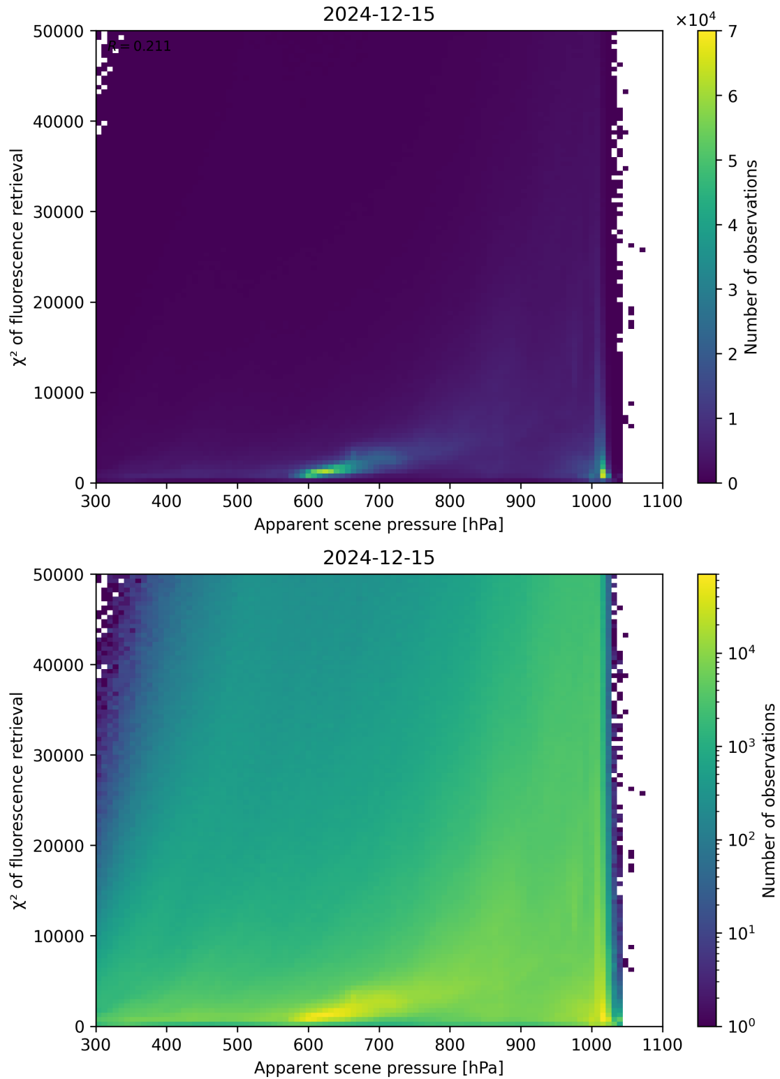
Figure 63: Scatter density plot of “Apparent scene pressure” against “ \chi^2 of fluorescence retrieval” for 2024-12-14 to 2024-12-16.
