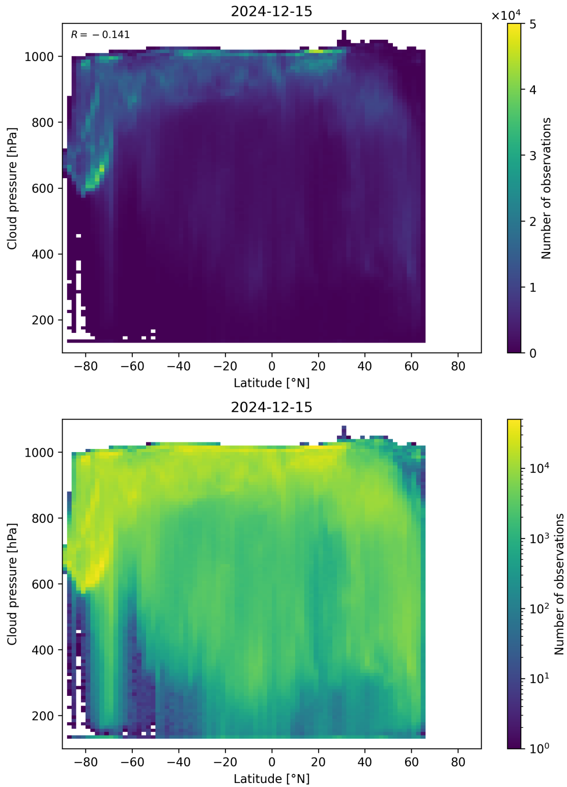
Figure 91: Scatter density plot of “Latitude” against “Cloud pressure” for 2024-12-14 to 2024-12-16.
