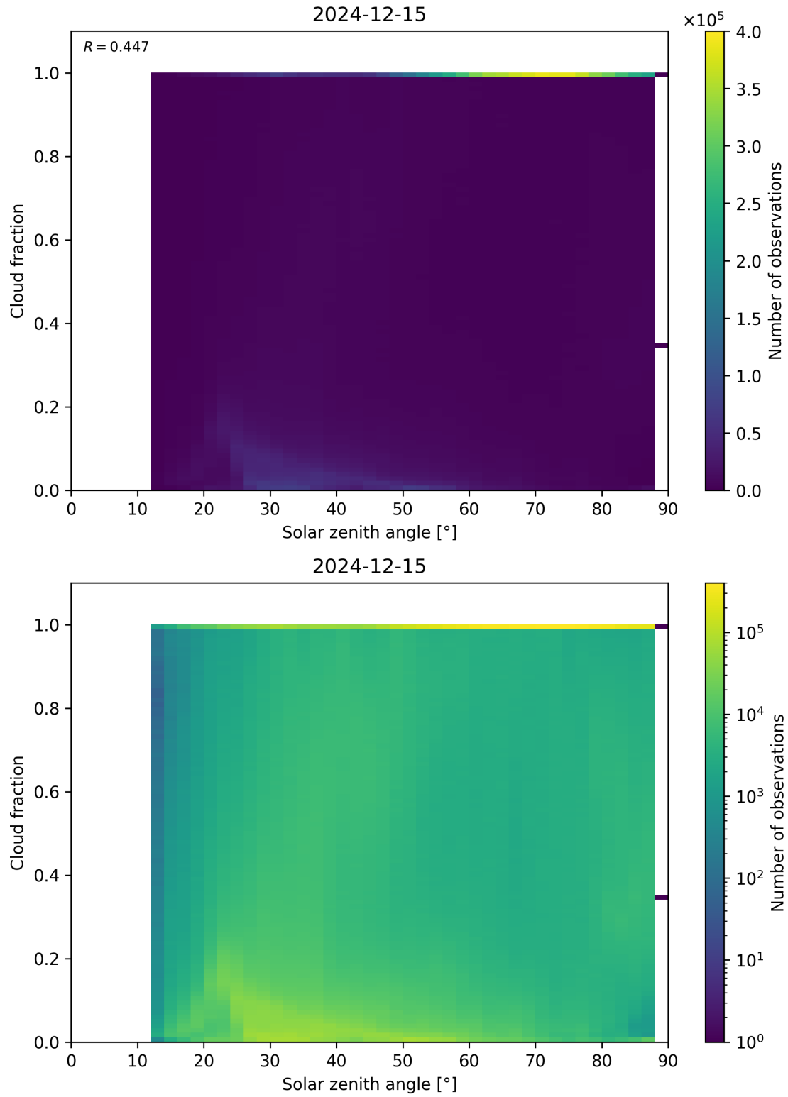
Figure 110: Scatter density plot of “Solar zenith angle” against “Cloud fraction” for 2024-12-14 to 2024-12-16.
