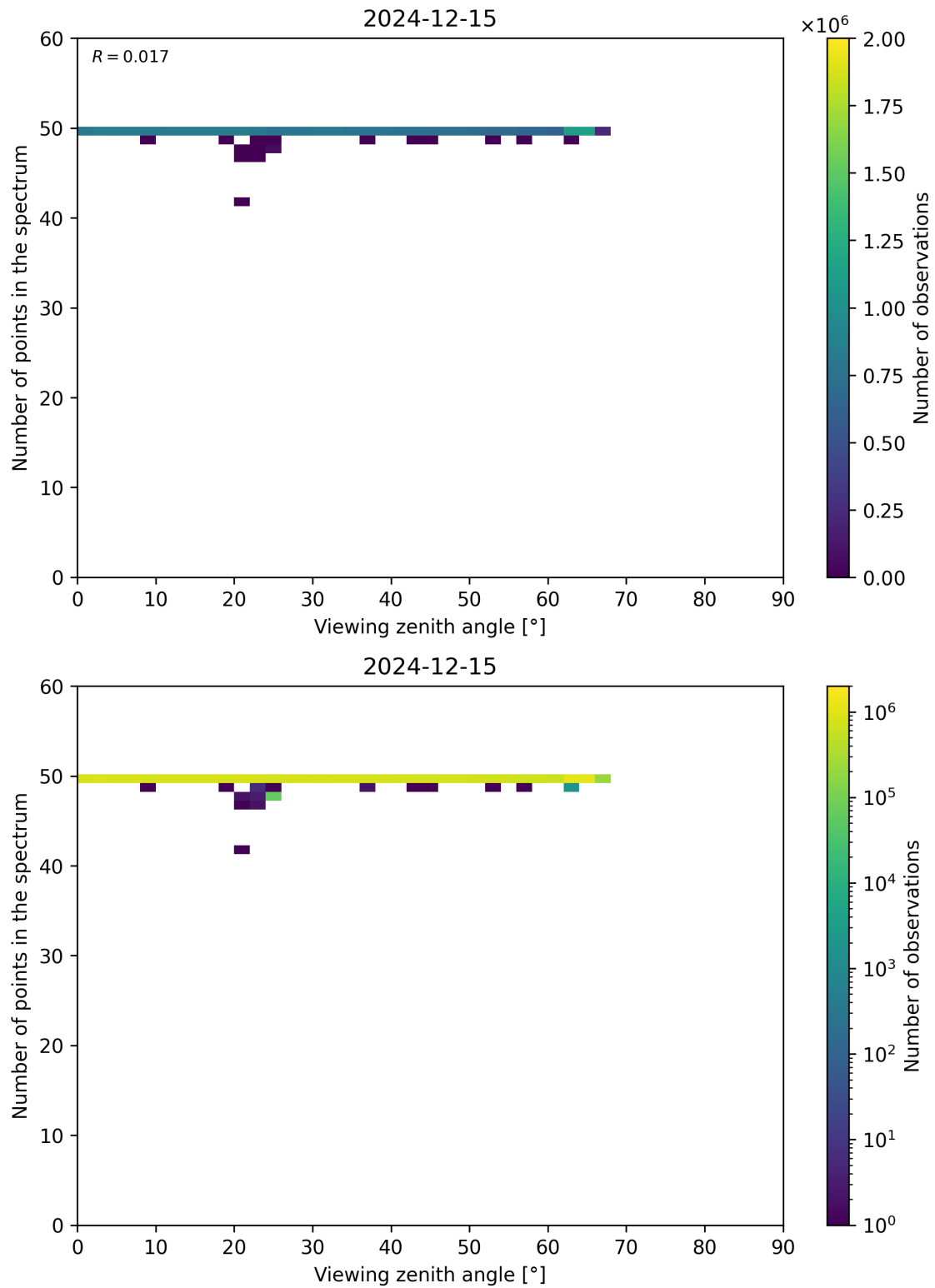
Figure 125: Scatter density plot of “Viewing zenith angle” against “Number of points in the spectrum” for 2024-12-14 to 2024-12-16.
