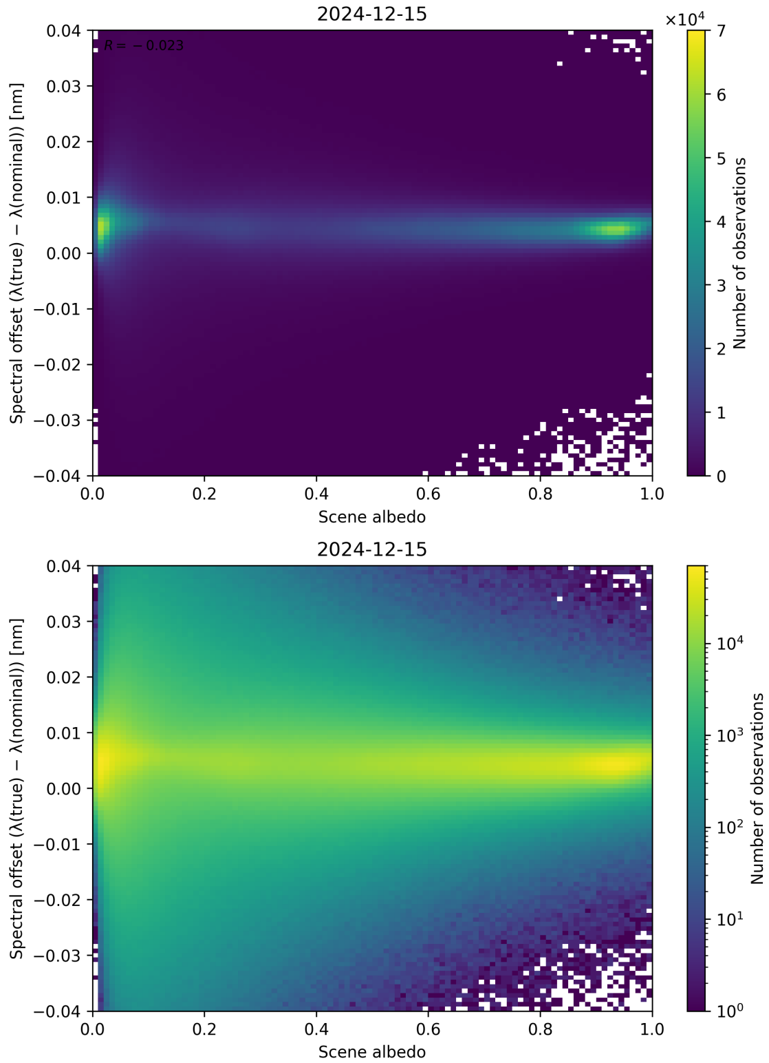
Figure 107: Scatter density plot of “Scene albedo” against “Spectral offset ( \lambda_{\text{true}} - \lambda_{\text{nominal}} )” for 2024-12-14 to 2024-12-16.
