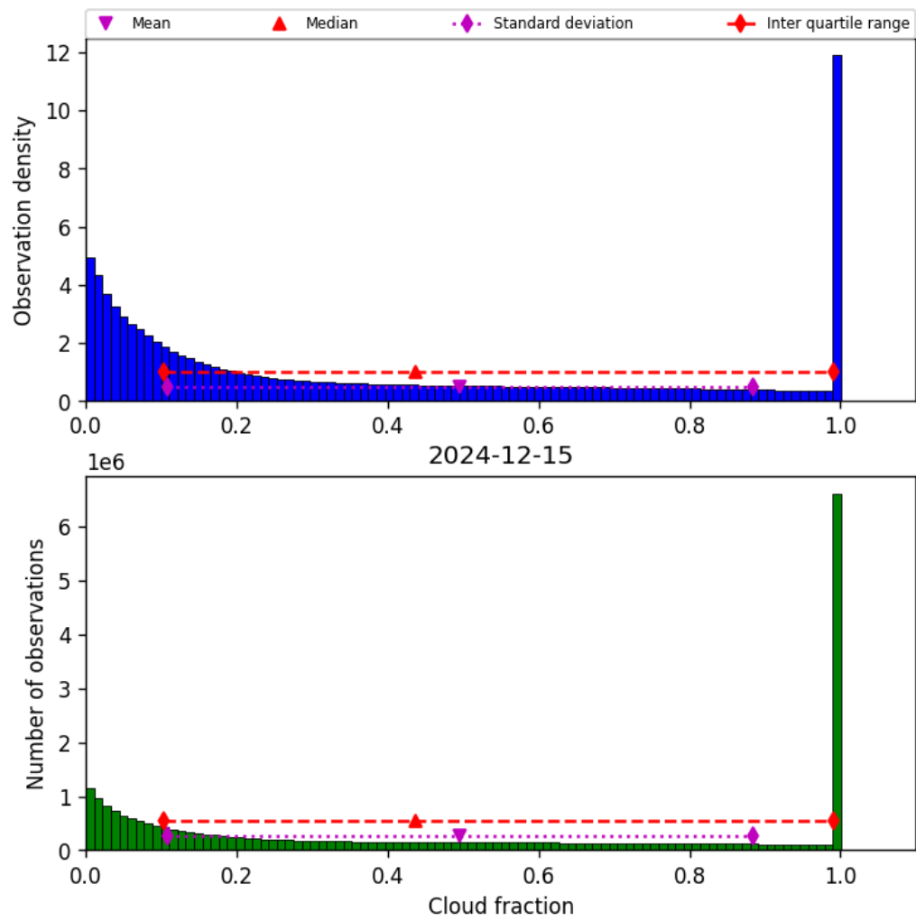
Figure 32: Histogram of "Cloud fraction" for 2024-12-14 to 2024-12-16
