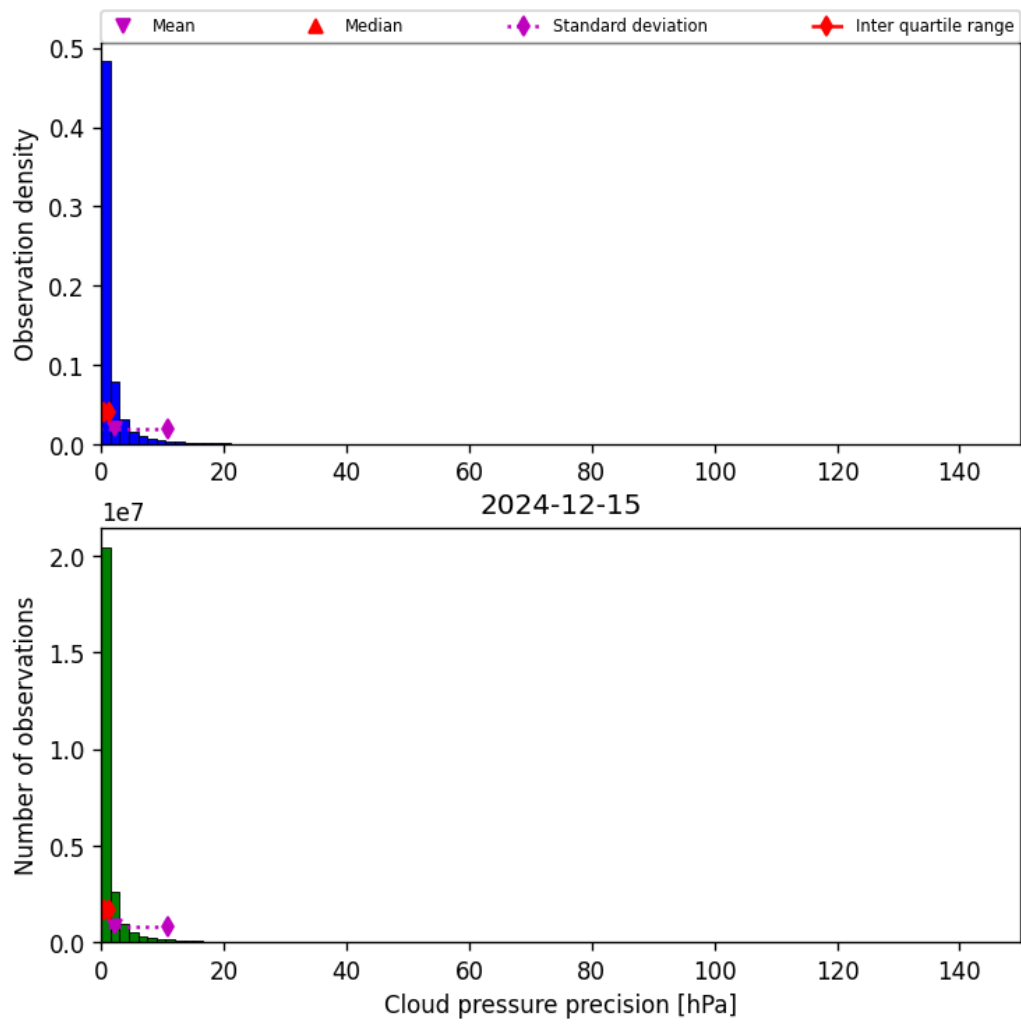
Figure 31: Histogram of “Cloud pressure precision” for 2024-12-14 to 2024-12-16
