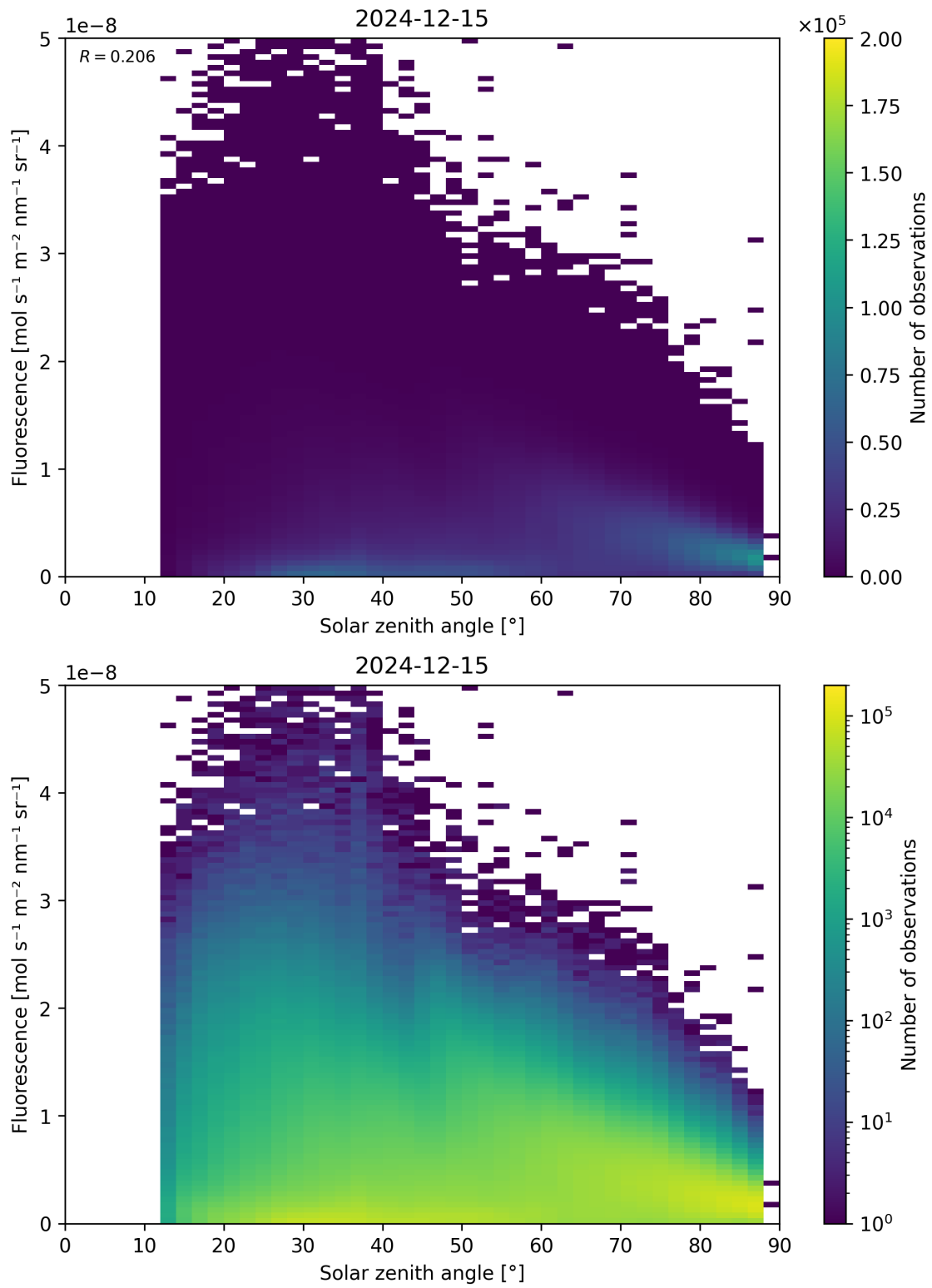
Figure 112: Scatter density plot of “Solar zenith angle” against “Fluorescence” for 2024-12-14 to 2024-12-16.
