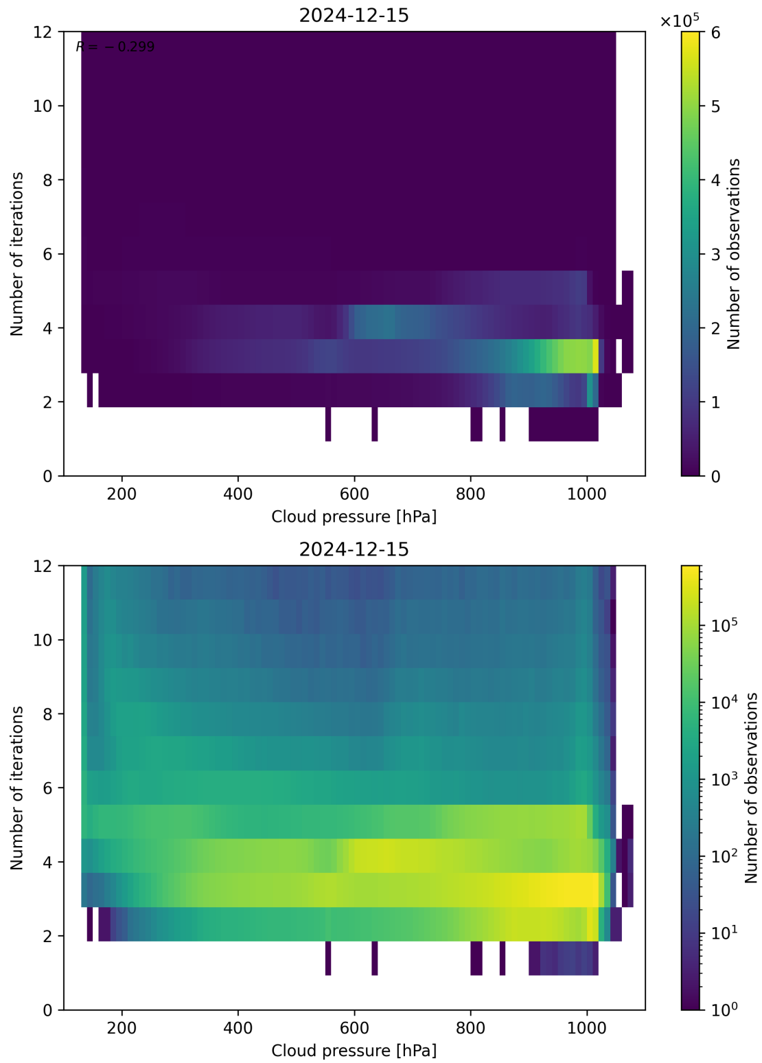
Figure 81: Scatter density plot of “Cloud pressure” against “Number of iterations” for 2024-12-14 to 2024-12-16.
