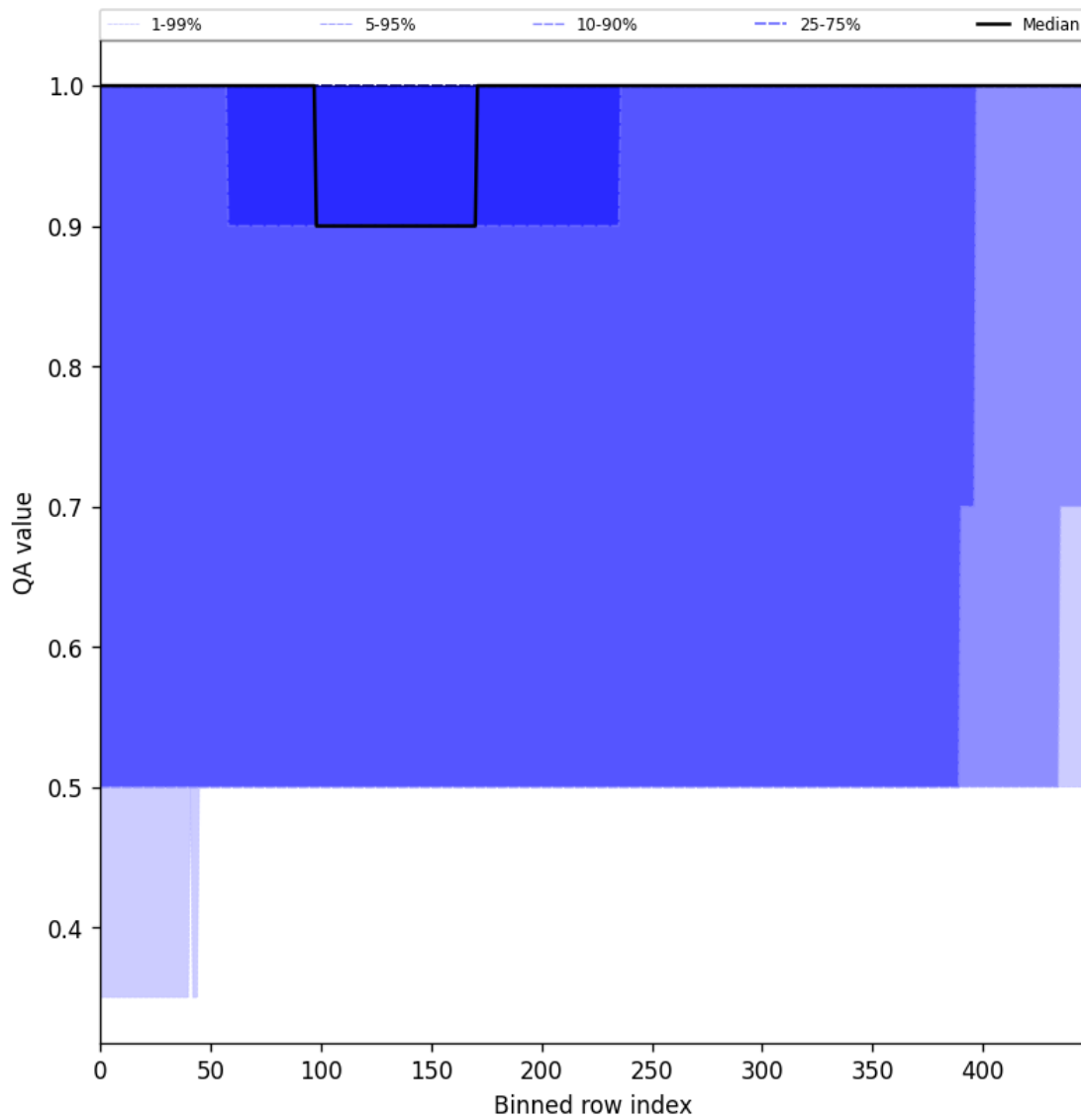
Figure 46: Along track statistics of “QA value” for 2024-12-14 to 2024-12-16
