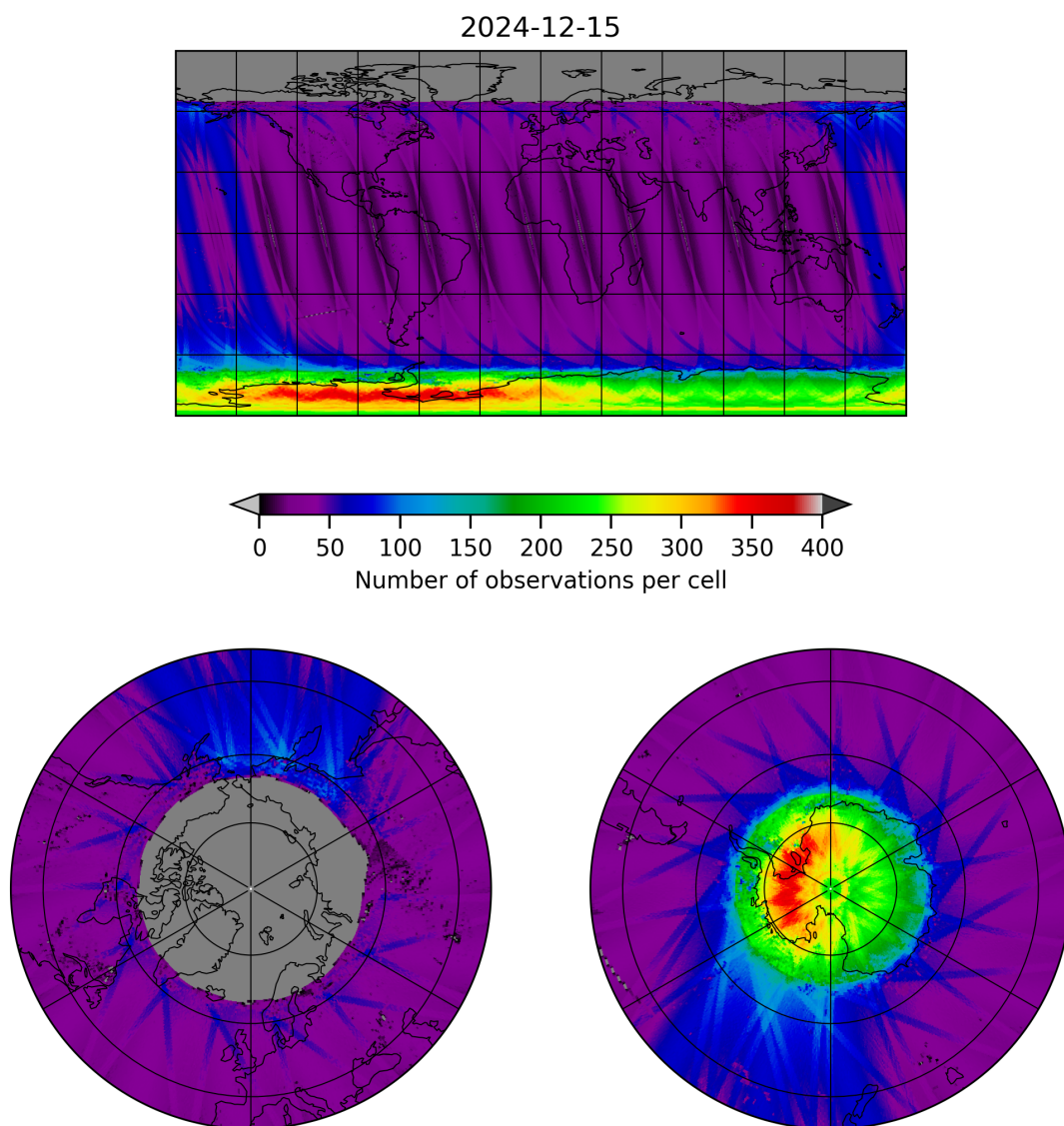
Figure 11: Map of the number of observations for 2024-12-14 to 2024-12-16
