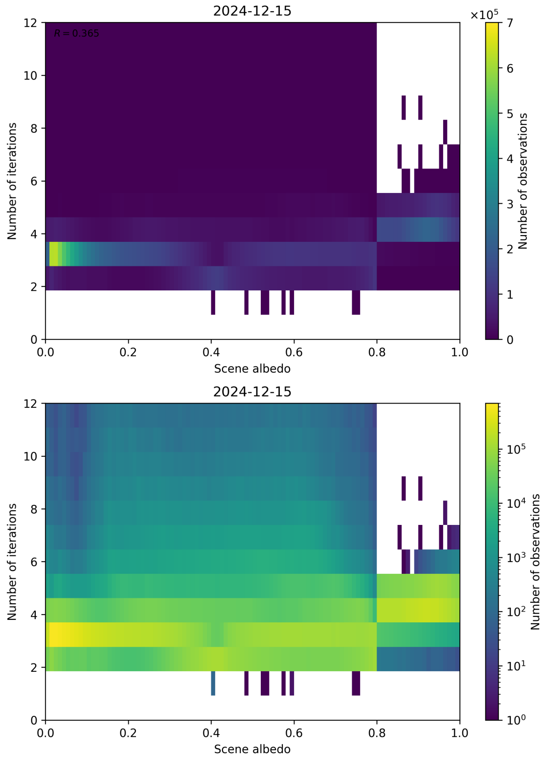
Figure 105: Scatter density plot of “Scene albedo” against “Number of iterations” for 2024-12-14 to 2024-12-16.
