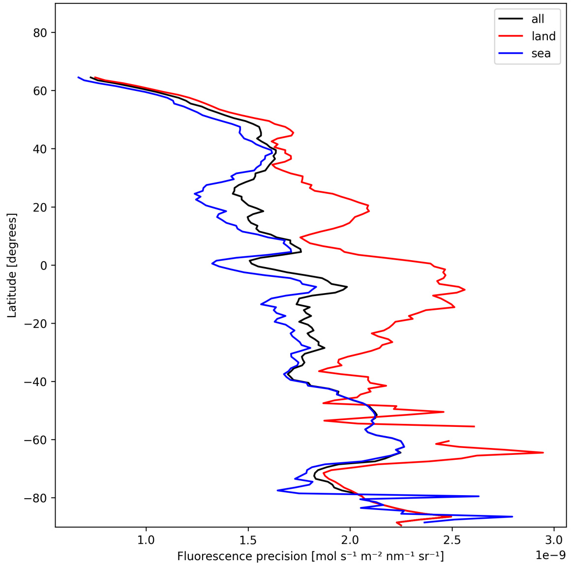
Figure 24: Zonal average of “Fluorescence precision” for 2024-12-14 to 2024-12-16.
