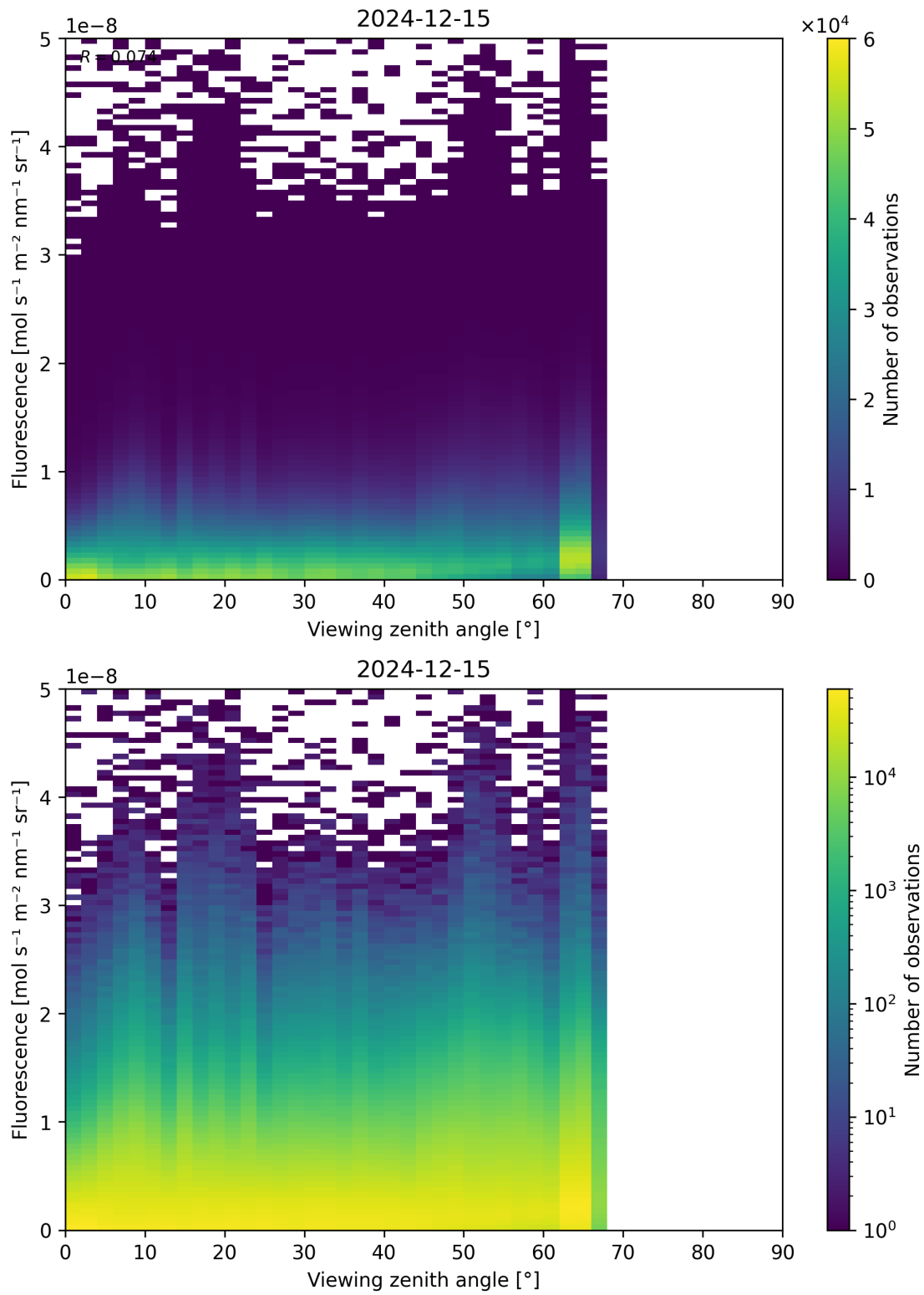
Figure 122: Scatter density plot of “Viewing zenith angle” against “Fluorescence” for 2024-12-14 to 2024-12-16.
