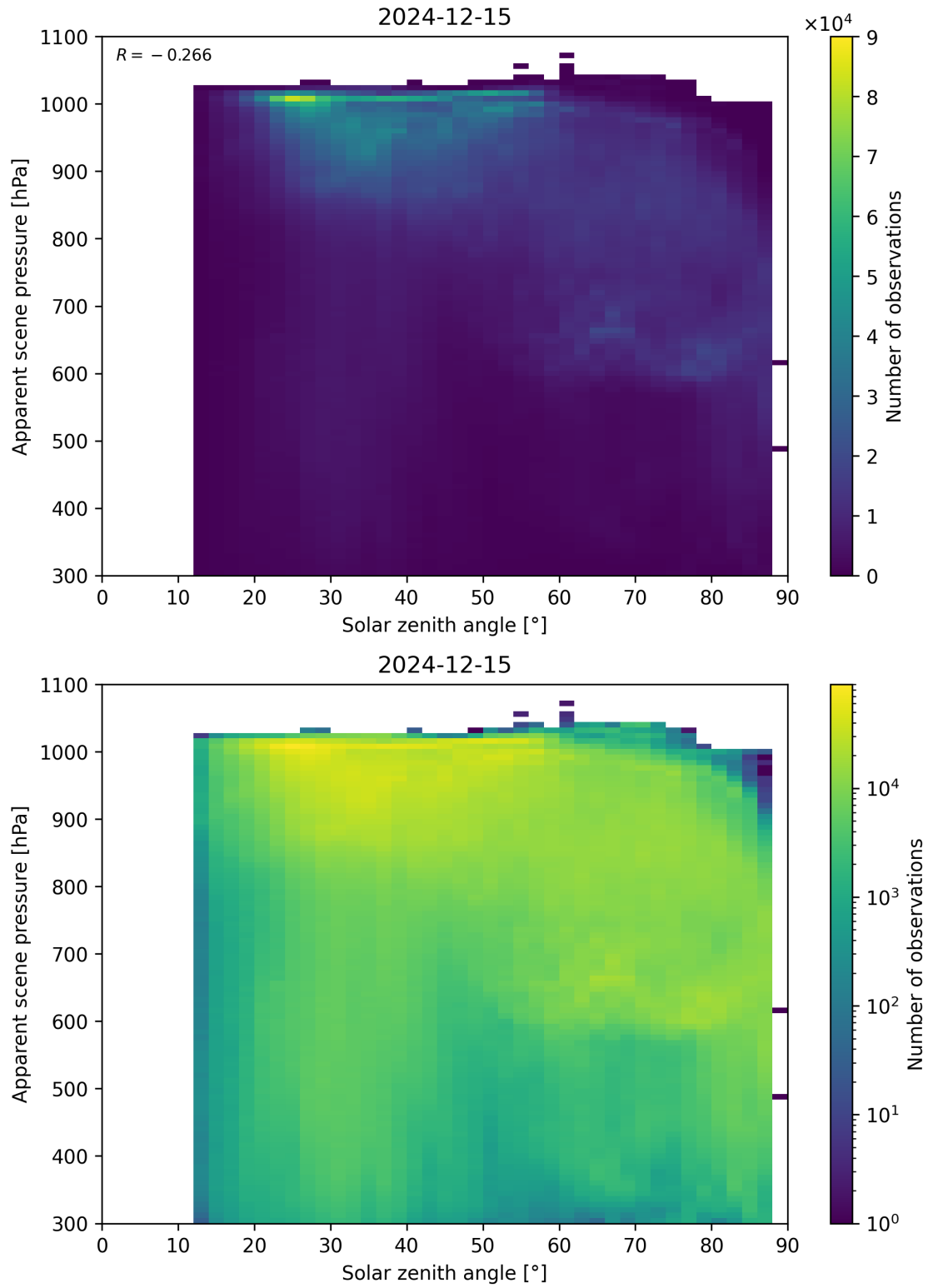
Figure 108: Scatter density plot of “Solar zenith angle” against “Apparent scene pressure” for 2024-12-14 to 2024-12-16.
