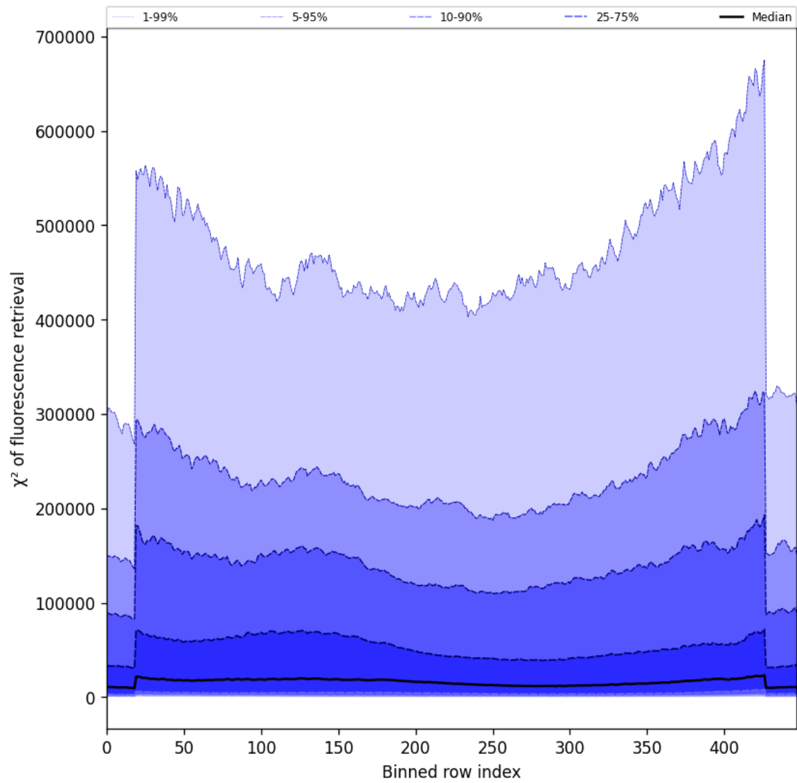
Figure 59: Along track statistics of “ \chi^2 of fluorescence retrieval” for 2024-12-14 to 2024-12-16
