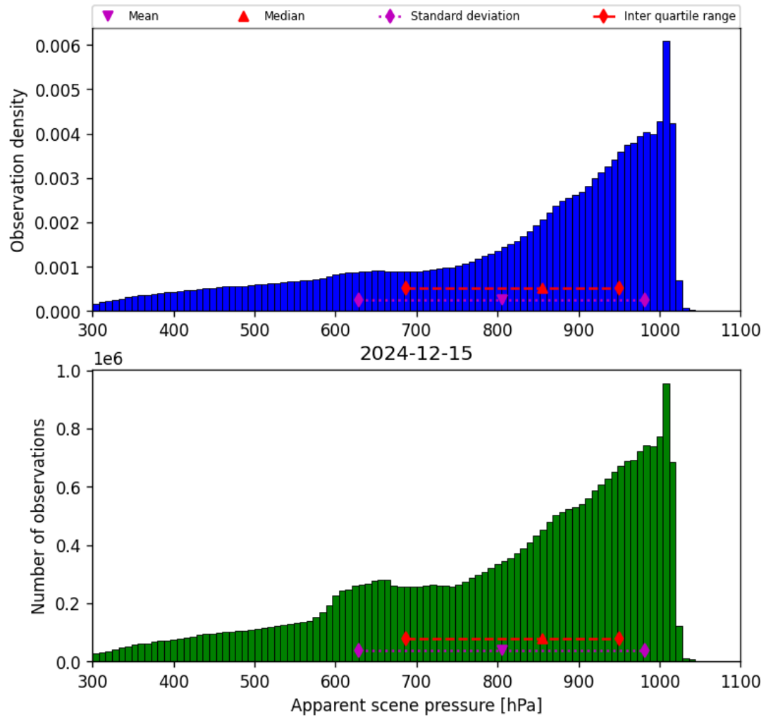
Figure 36: Histogram of “Apparent scene pressure” for 2024-12-14 to 2024-12-16
