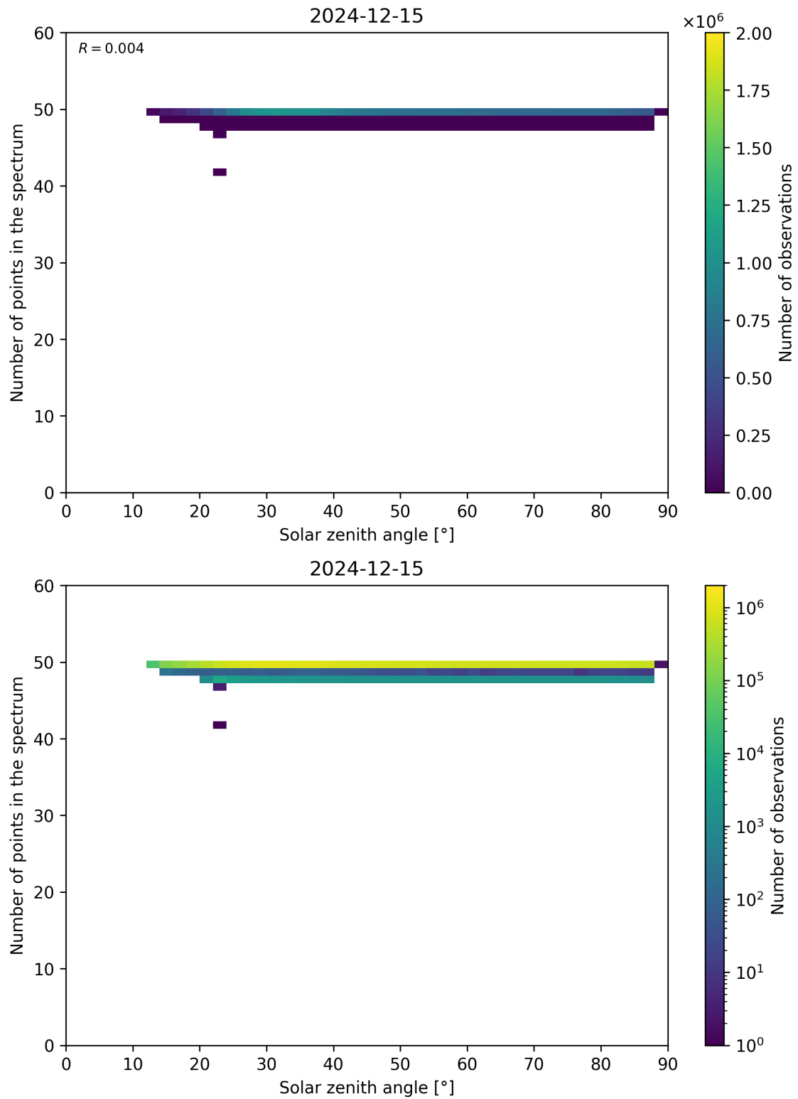
Figure 115: Scatter density plot of “Solar zenith angle” against “Number of points in the spectrum” for 2024-12-14 to 2024-12-16.
