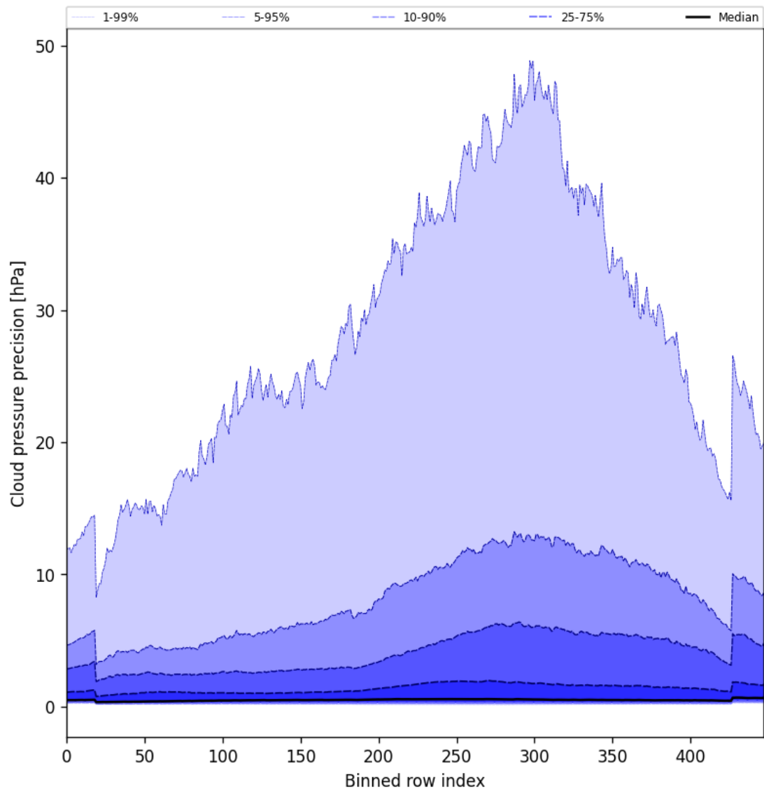
Figure 48: Along track statistics of “Cloud pressure precision” for 2024-12-14 to 2024-12-16
