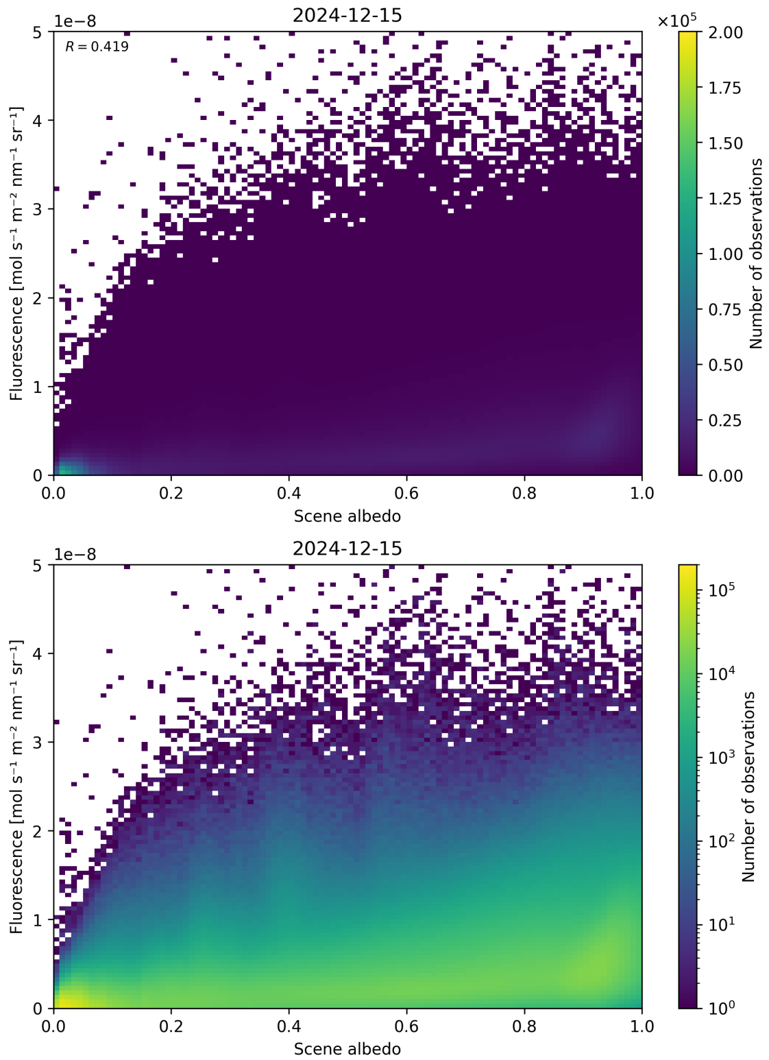
Figure 104: Scatter density plot of “Scene albedo” against “Fluorescence” for 2024-12-14 to 2024-12-16.
