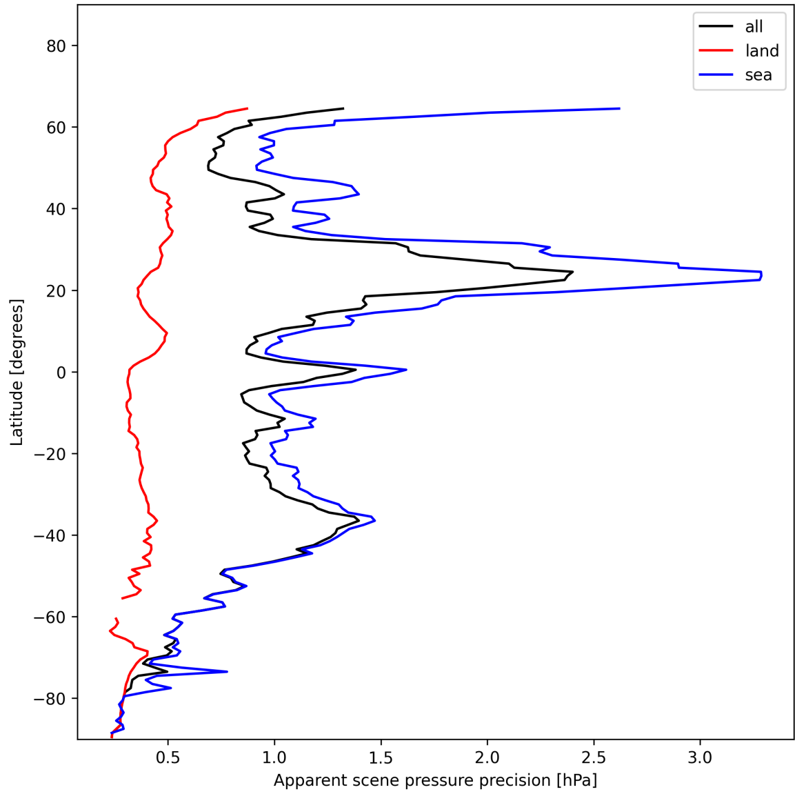
Figure 20: Zonal average of “Apparent scene pressure precision” for 2024-12-14 to 2024-12-16.
