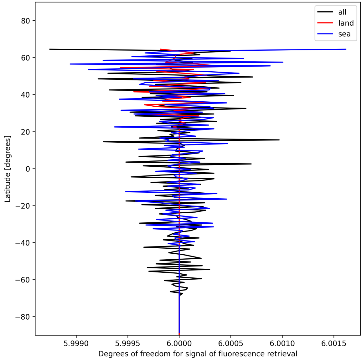
Figure 26: Zonal average of “Degrees of freedom for signal of fluorescence retrieval” for 2024-12-14 to 2024-12-16.
