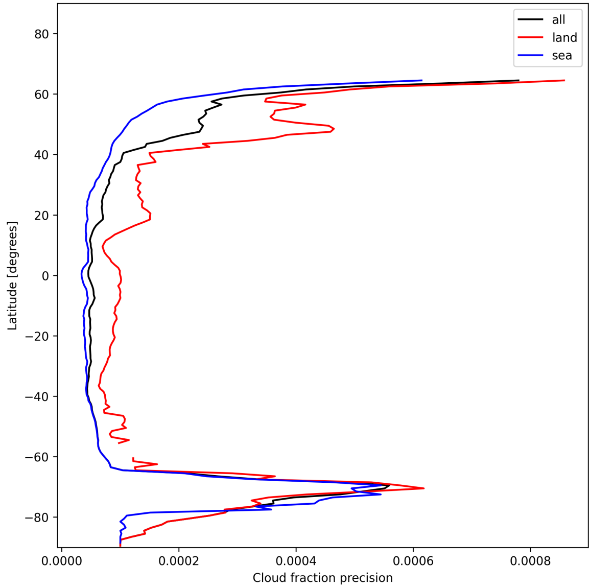
Figure 16: Zonal average of “Cloud fraction precision” for 2024-12-14 to 2024-12-16.
