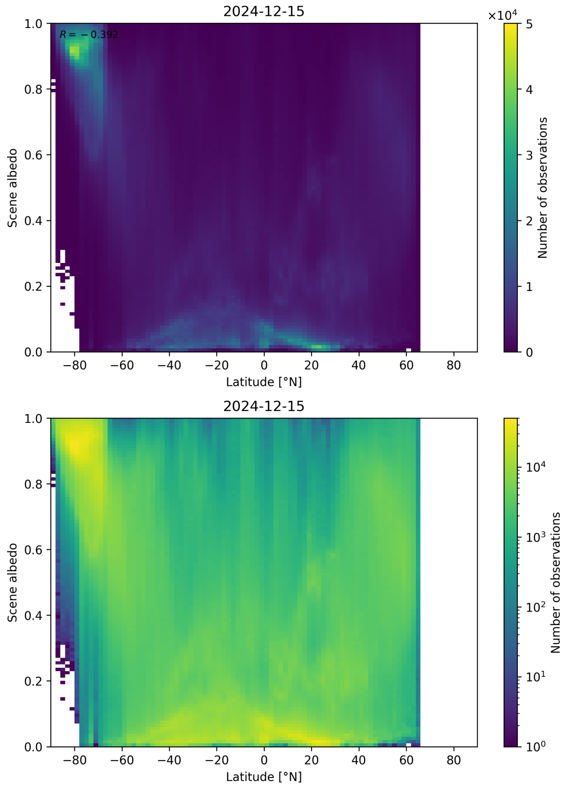
Figure 95: Scatter density plot of “Latitude” against “Scene albedo” for 2024-12-14 to 2024-12-16.
