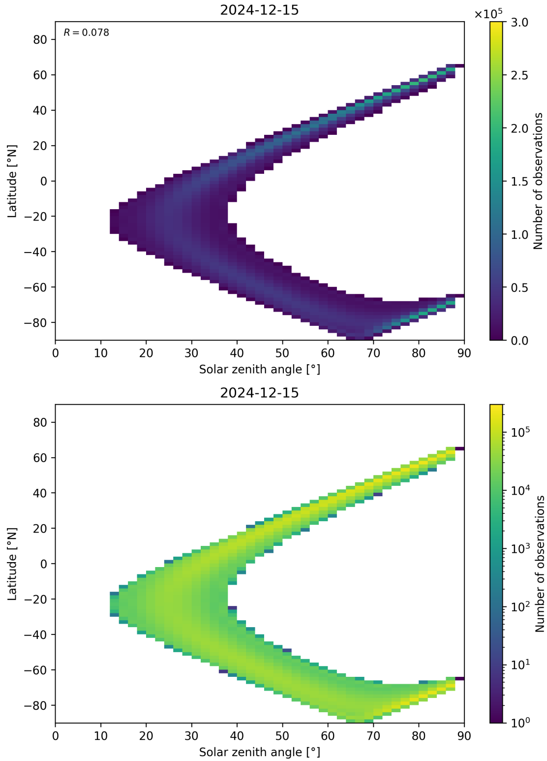
Figure 113: Scatter density plot of “Solar zenith angle” against “Latitude” for 2024-12-14 to 2024-12-16.
