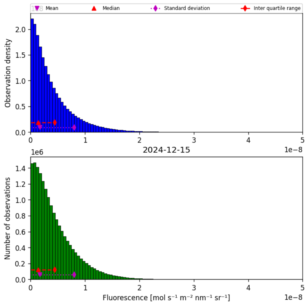
Figure 40: Histogram of “Fluorescence” for 2024-12-14 to 2024-12-16
