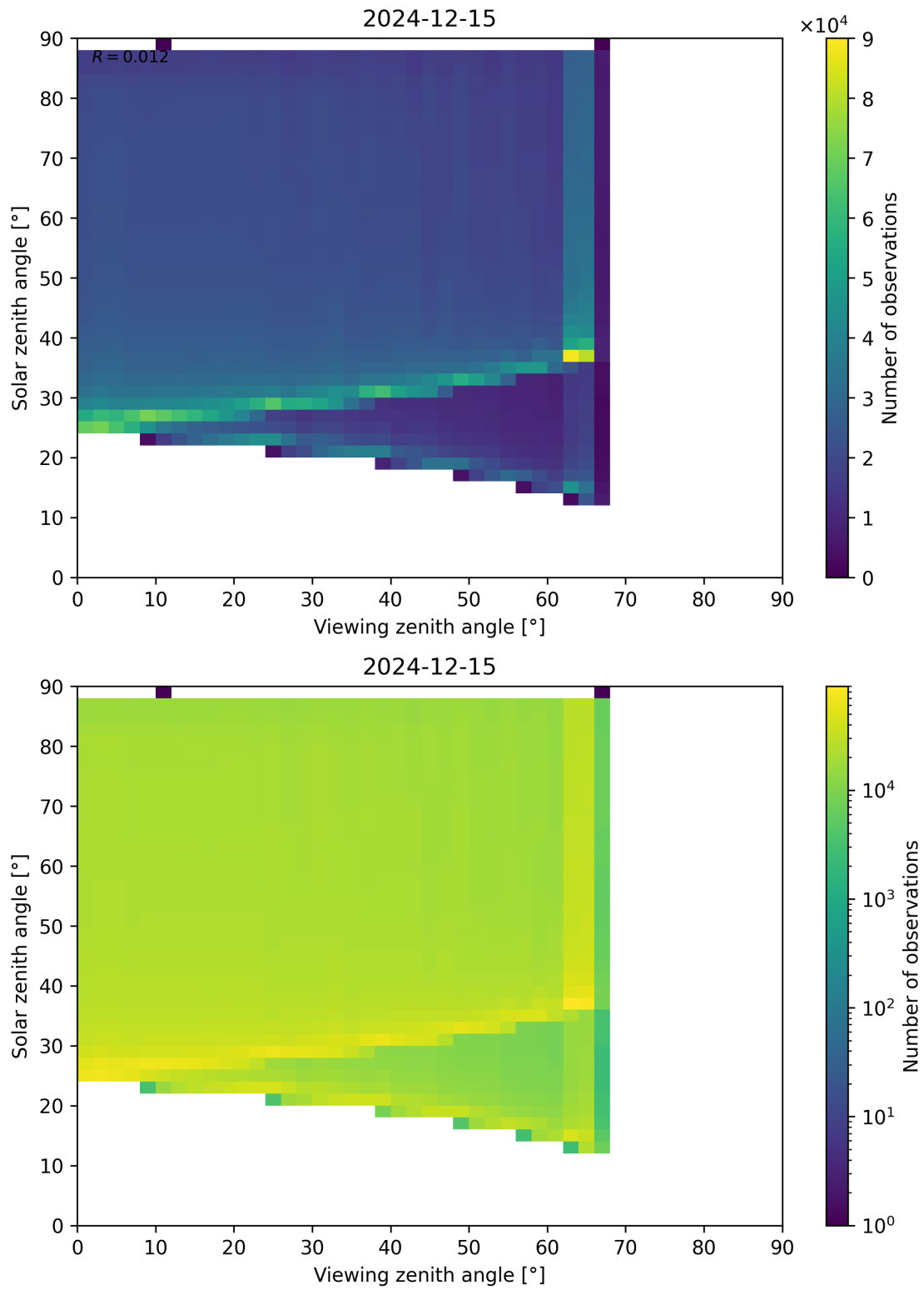
Figure 127: Scatter density plot of “Viewing zenith angle” against “Solar zenith angle” for 2024-12-14 to 2024-12-16.
