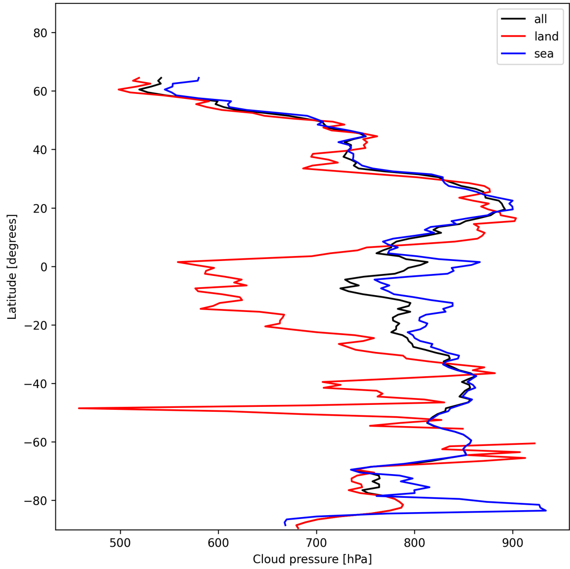
Figure 13: Zonal average of “Cloud pressure” for 2024-12-14 to 2024-12-16.
