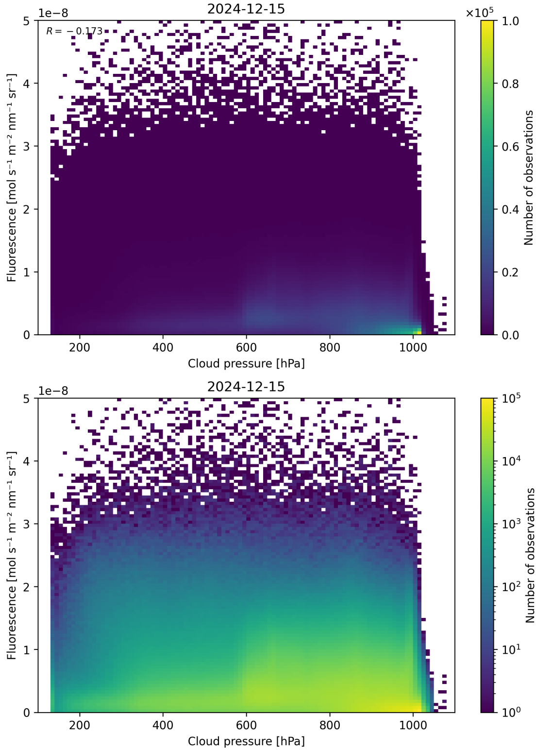
Figure 80: Scatter density plot of “Cloud pressure” against “Fluorescence” for 2024-12-14 to 2024-12-16.
