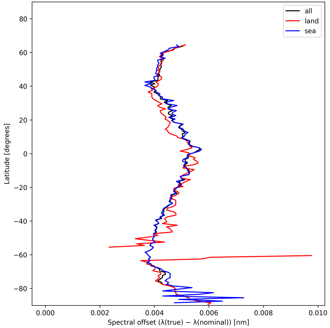
Figure 28: Zonal average of “Spectral offset ( \lambda_{\text{true}} - \lambda_{\text{nominal}} )” for 2024-12-14 to 2024-12-16.
