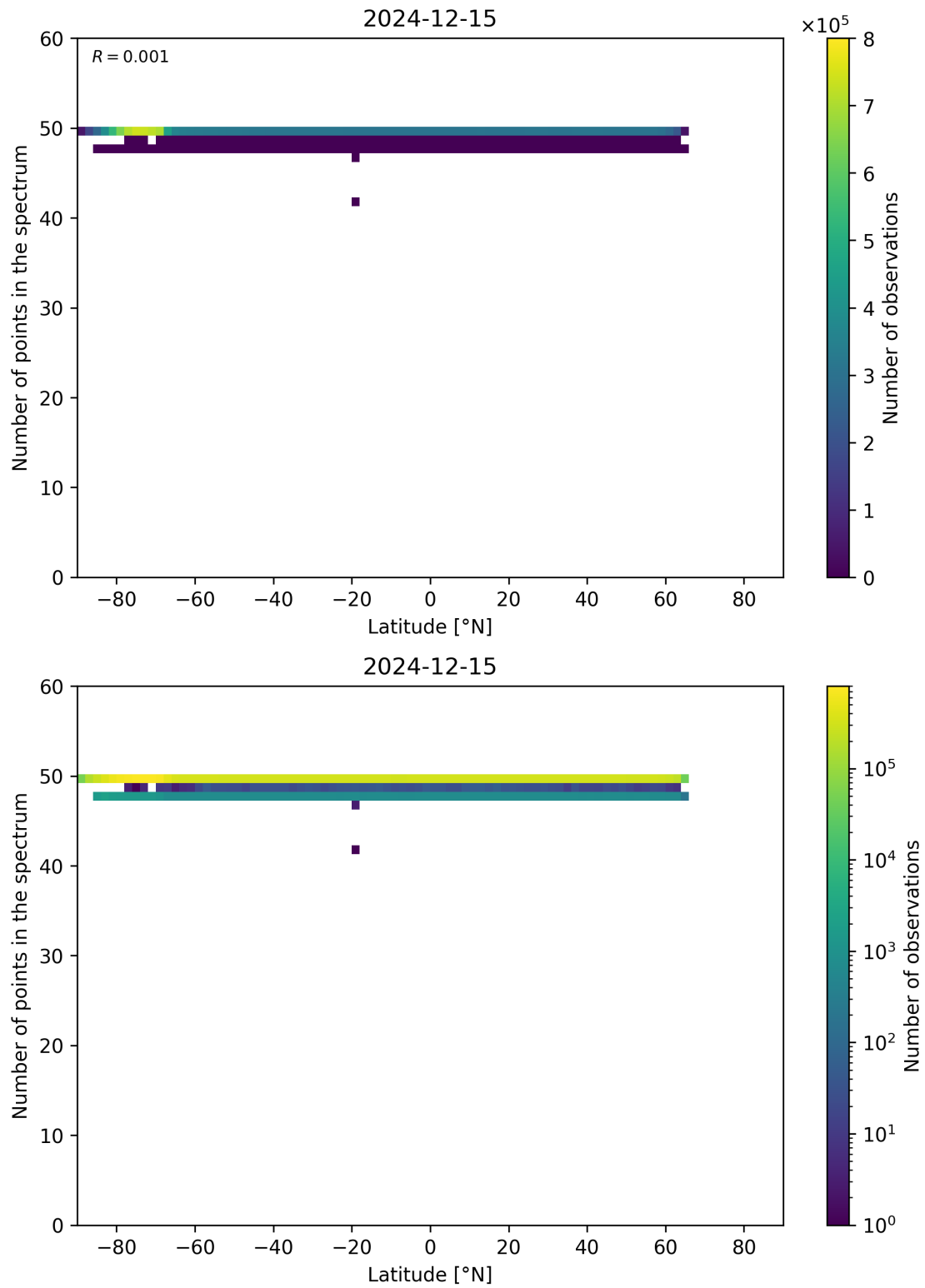
Figure 94: Scatter density plot of “Latitude” against “Number of points in the spectrum” for 2024-12-14 to 2024-12-16.
