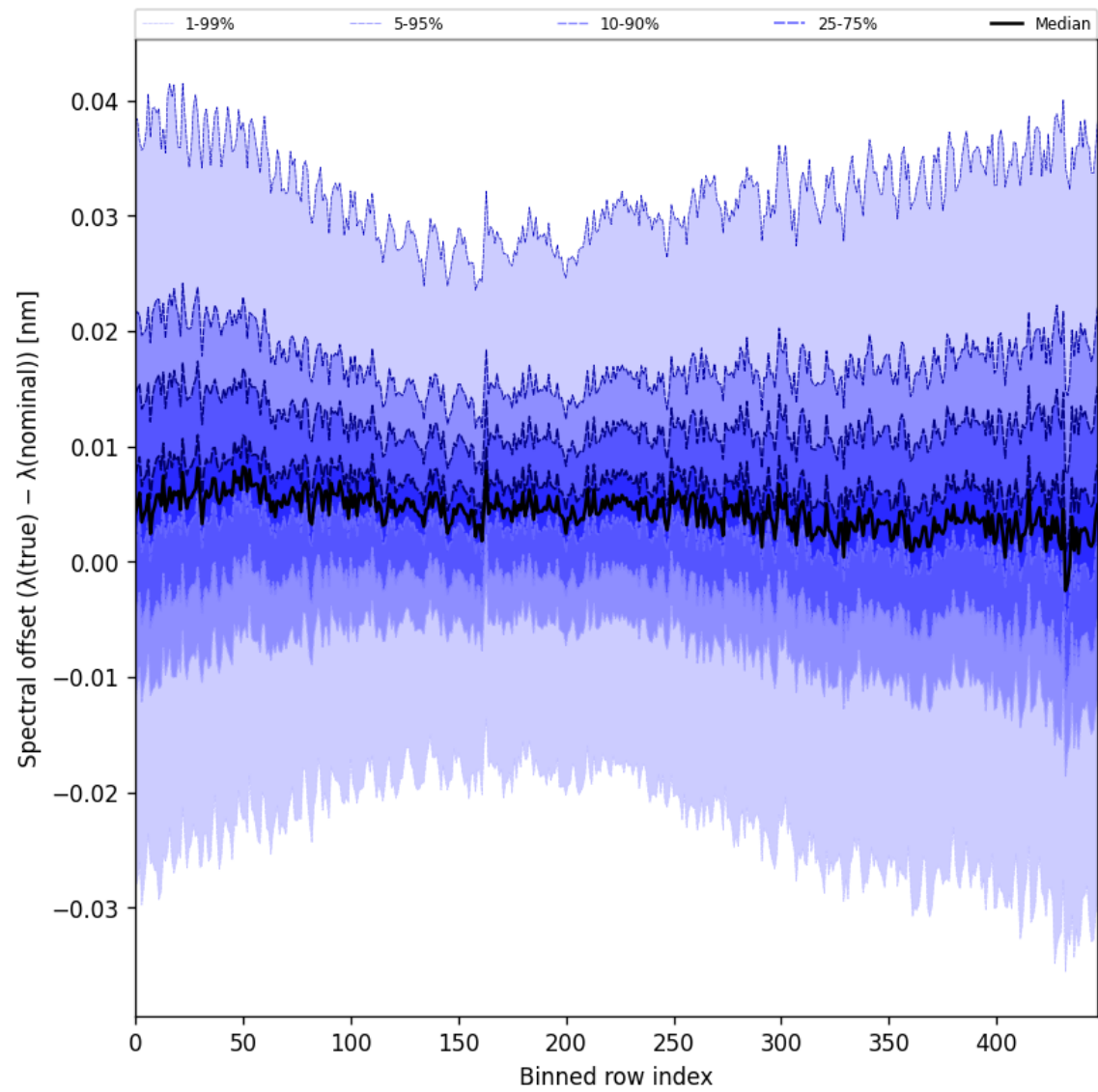
Figure 62: Along track statistics of “Spectral offset ( \lambda_{\text{true}} - \lambda_{\text{nominal}} )” for 2024-12-14 to 2024-12-16
