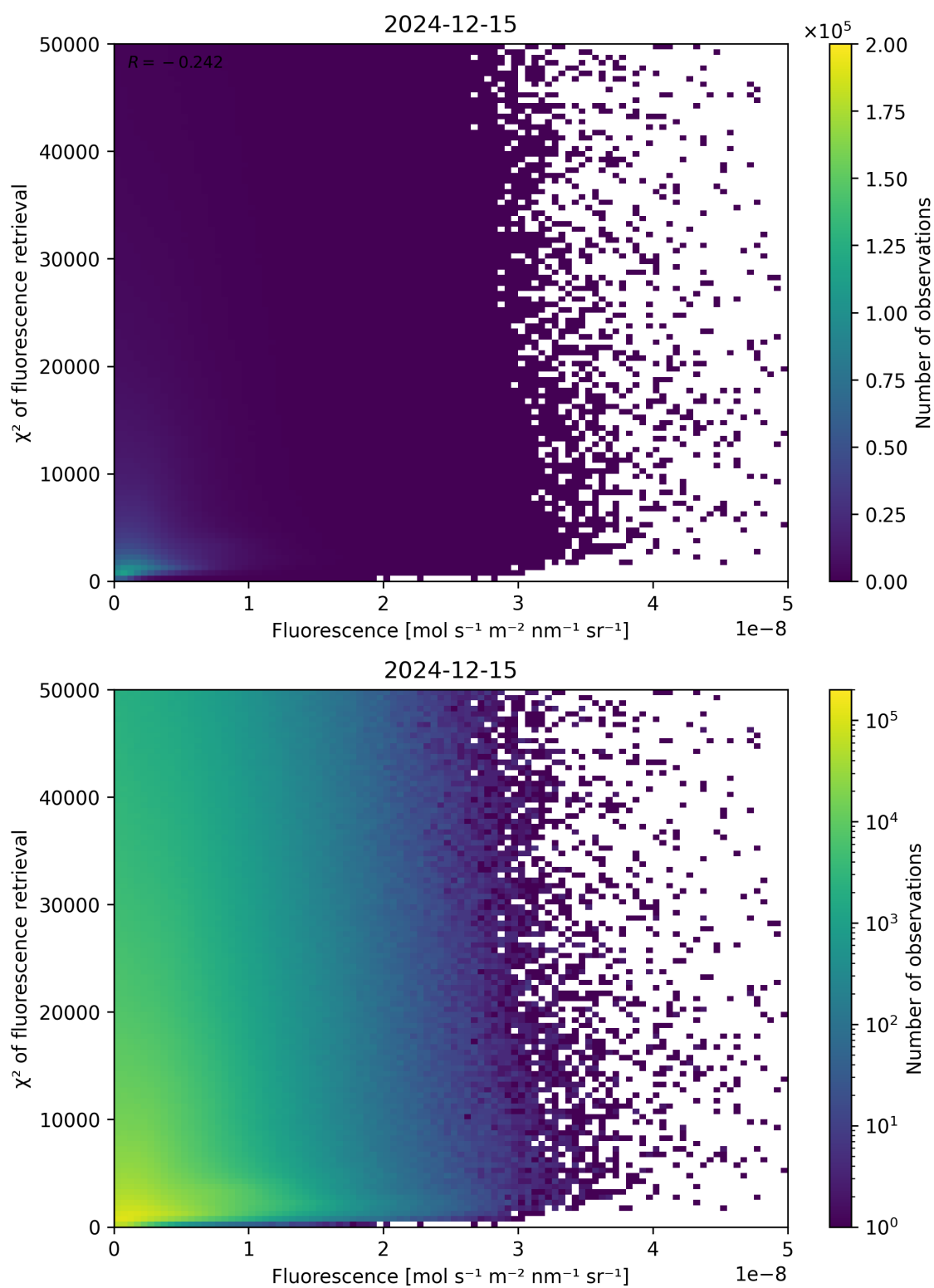
Figure 85: Scatter density plot of “Fluorescence” against “ \chi^2 of fluorescence retrieval” for 2024-12-14 to 2024-12-16.
