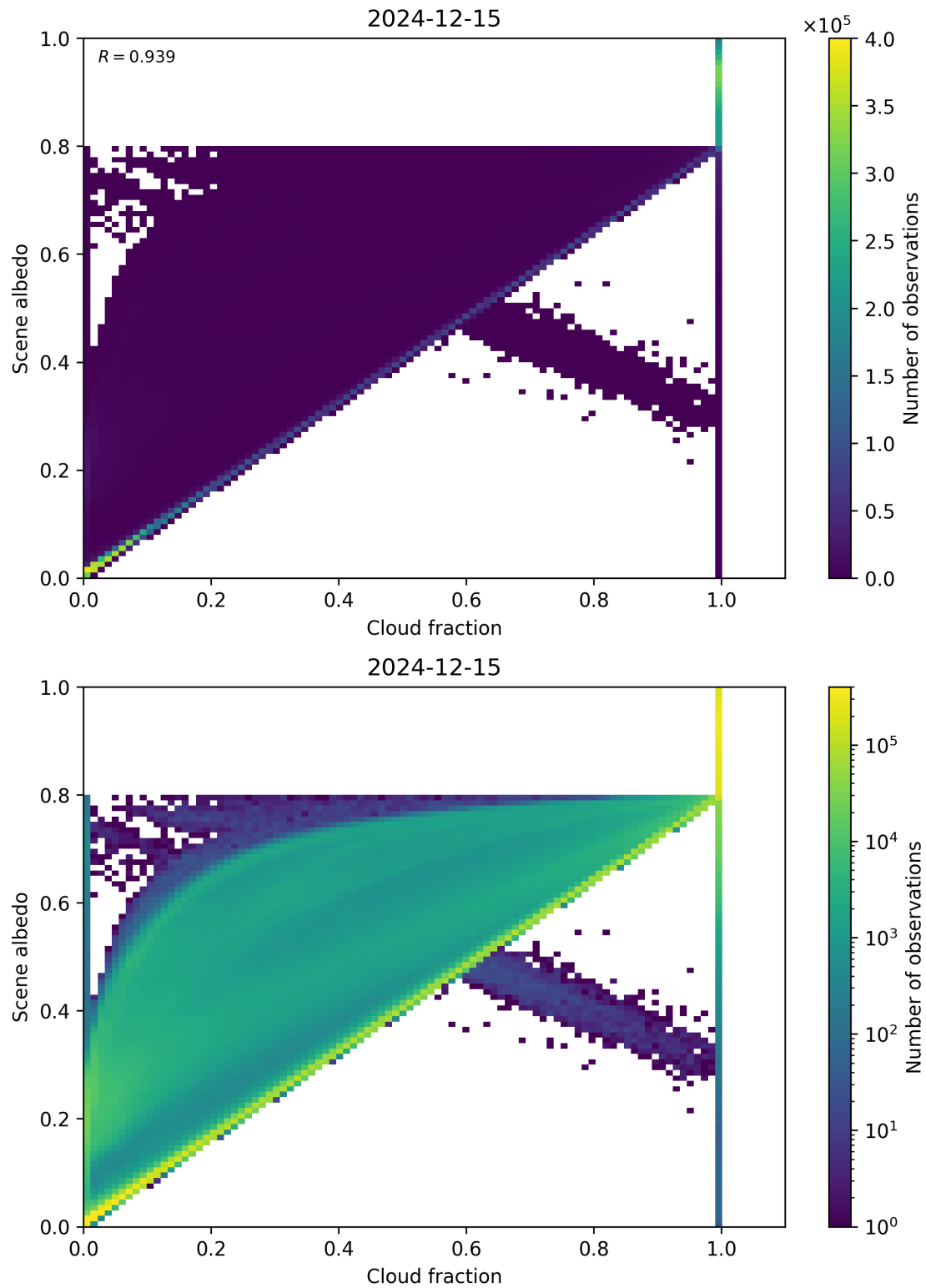
Figure 75: Scatter density plot of “Cloud fraction” against “Scene albedo” for 2024-12-14 to 2024-12-16.
