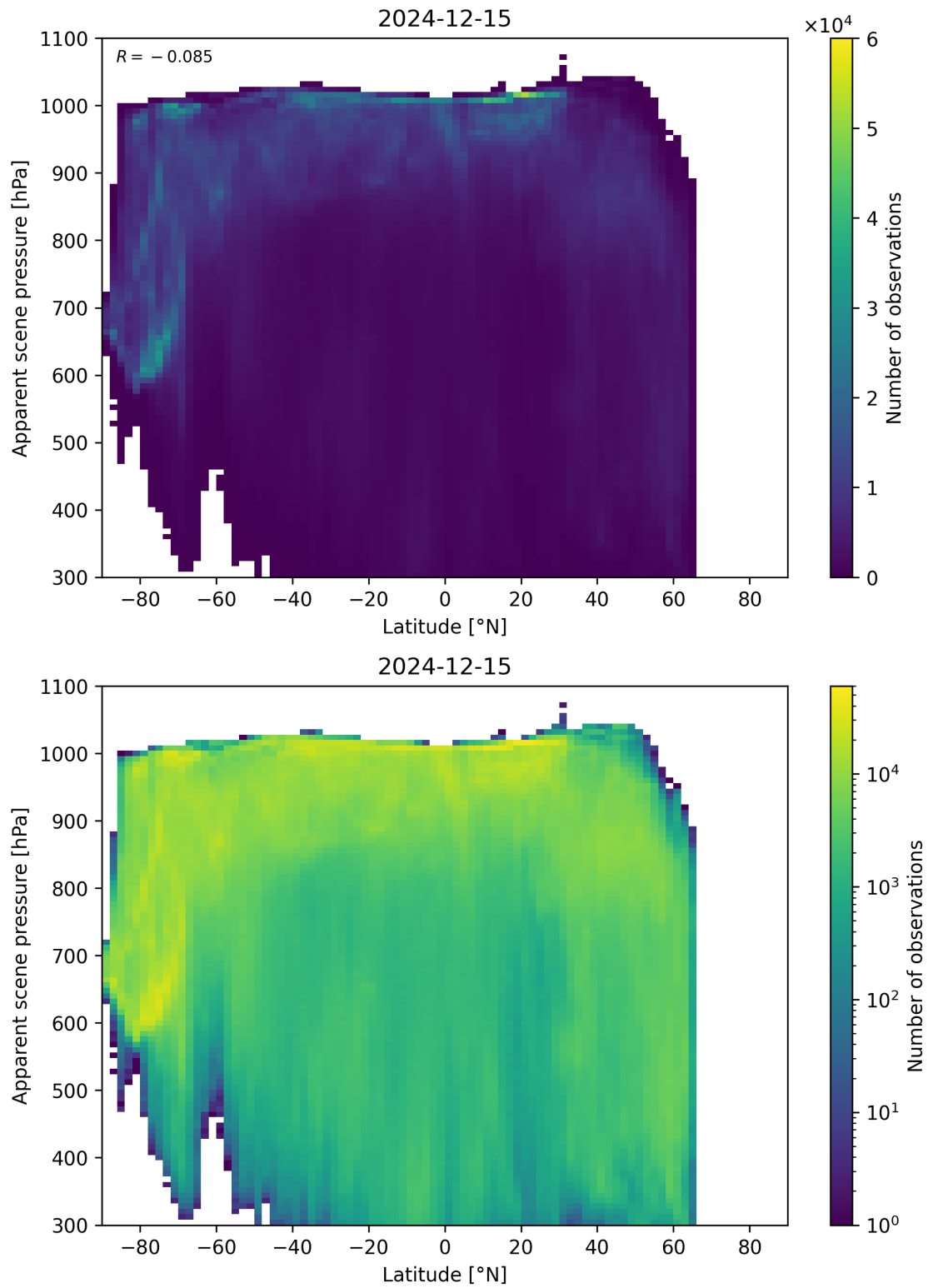
Figure 88: Scatter density plot of “Latitude” against “Apparent scene pressure” for 2024-12-14 to 2024-12-16.
