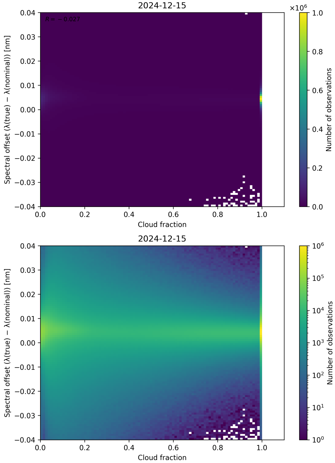
Figure 76: Scatter density plot of “Cloud fraction” against “Spectral offset ( \lambda_{\text{true}} - \lambda_{\text{nominal}} )” for 2024-12-14 to 2024-12-16.
