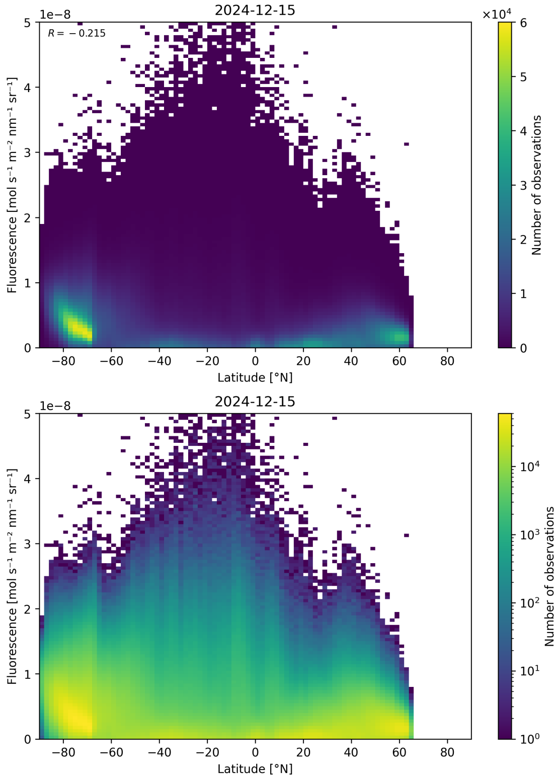
Figure 92: Scatter density plot of “Latitude” against “Fluorescence” for 2024-12-14 to 2024-12-16.
