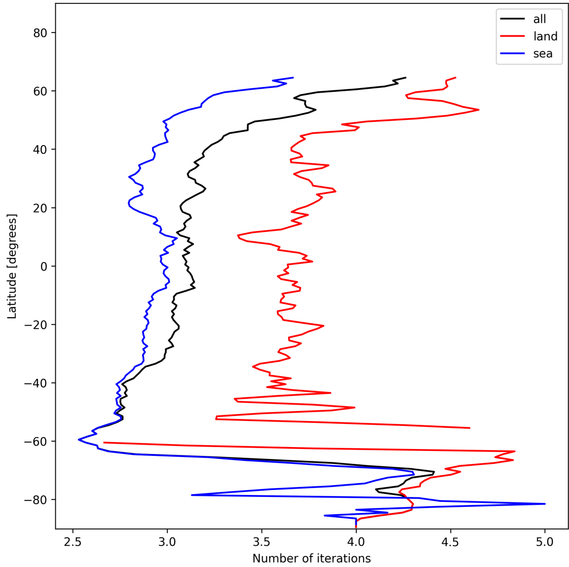
Figure 22: Zonal average of “Number of iterations” for 2024-12-14 to 2024-12-16.
