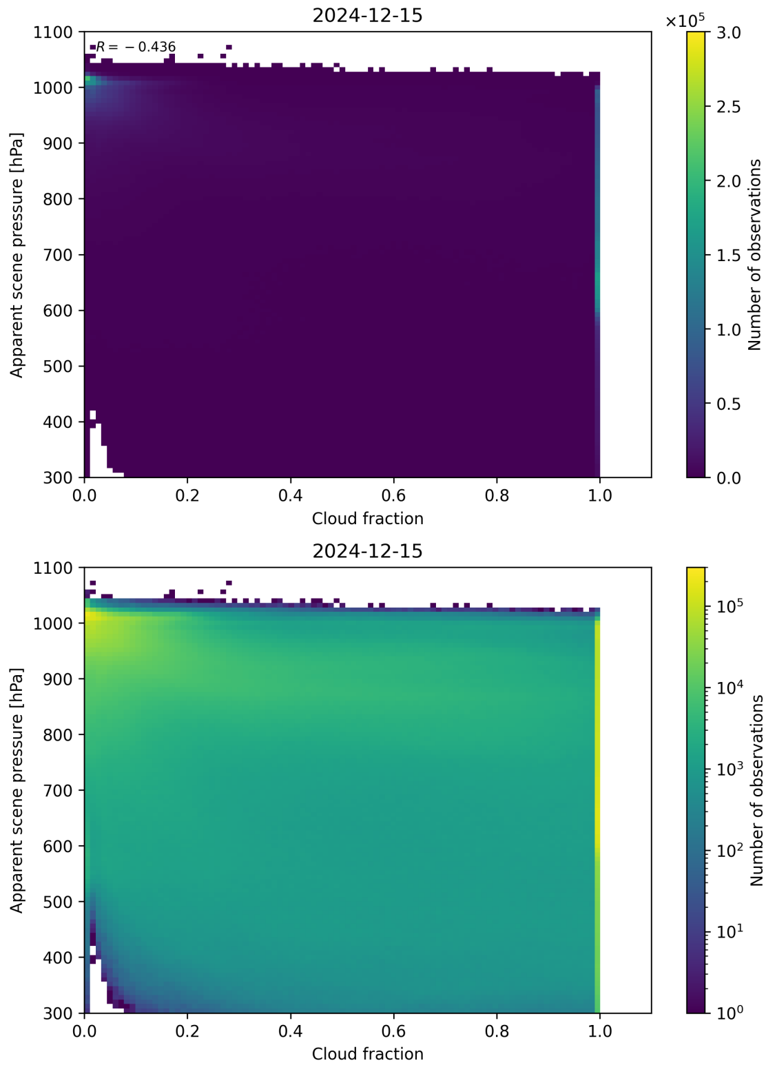
Figure 70: Scatter density plot of “Cloud fraction” against “Apparent scene pressure” for 2024-12-14 to 2024-12-16.
