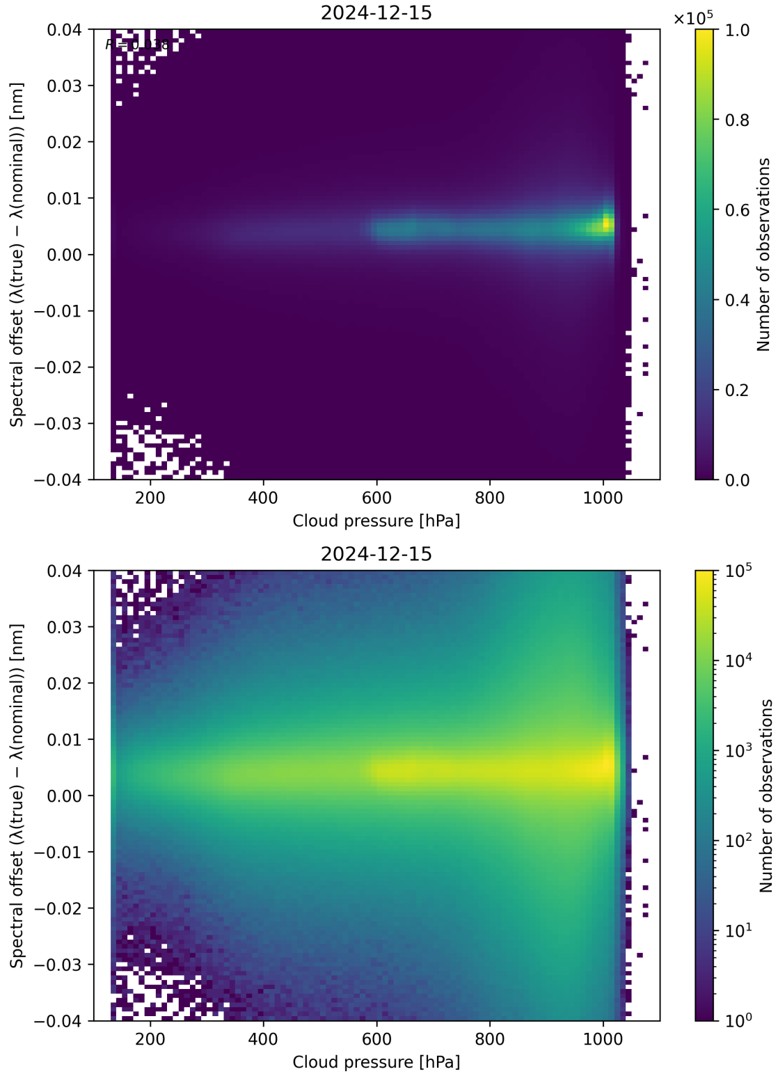
Figure 84: Scatter density plot of “Cloud pressure” against “Spectral offset ( \lambda_{\text{true}} - \lambda_{\text{nominal}} )” for 2024-12-14 to 2024-12-16.
