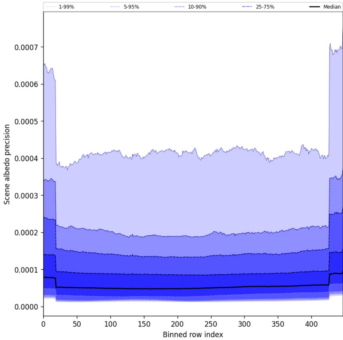
Figure 52: Along track statistics of “Scene albedo precision” for 2024-12-14 to 2024-12-16
