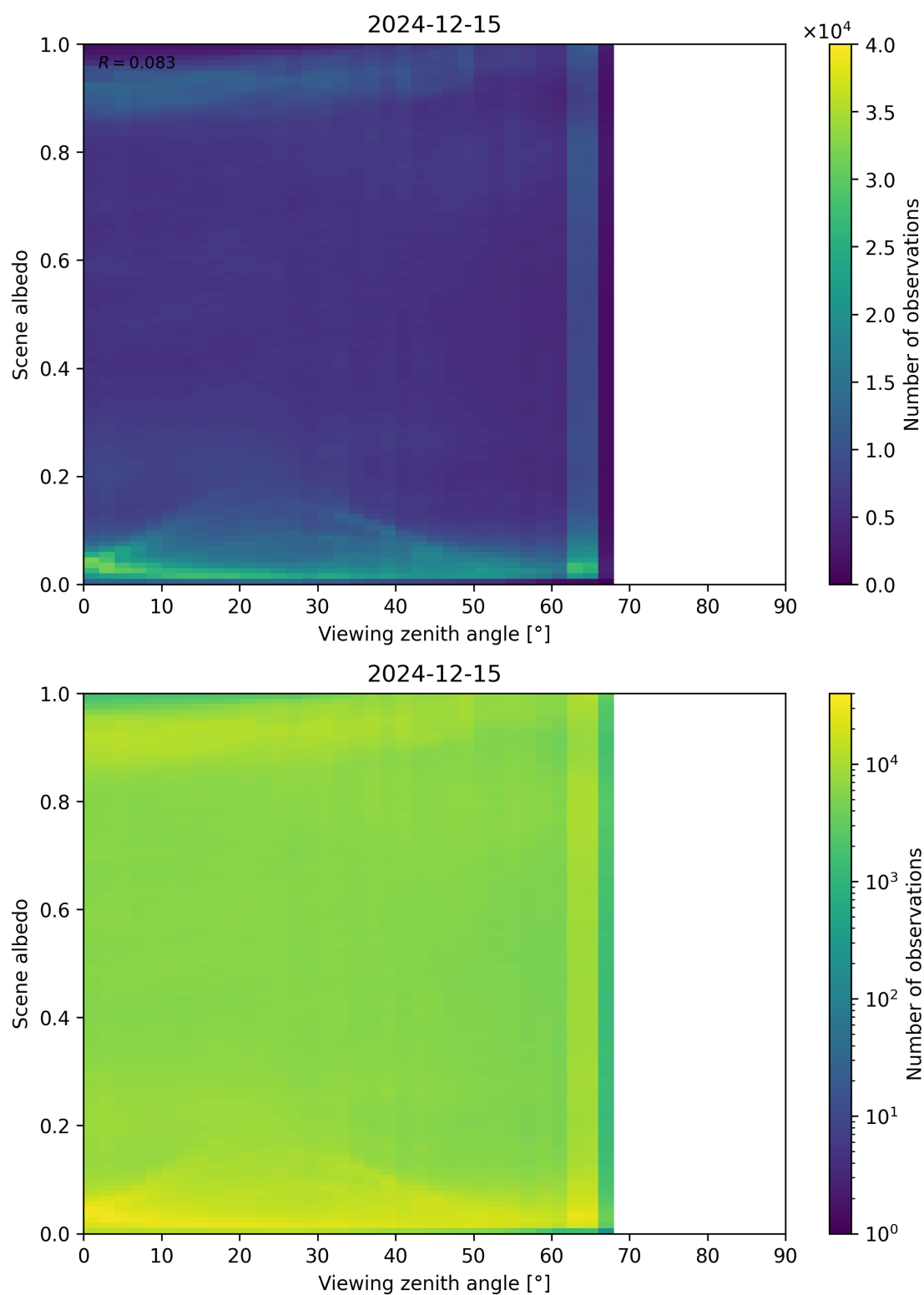
Figure 126: Scatter density plot of “Viewing zenith angle” against “Scene albedo” for 2024-12-14 to 2024-12-16.
