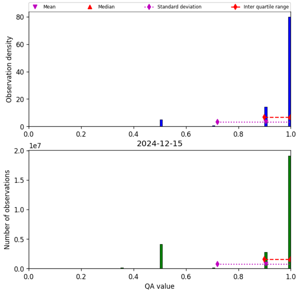
Figure 29: Histogram of “QA value” for 2024-12-14 to 2024-12-16
