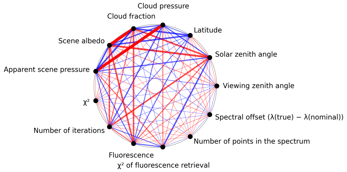
Figure 1: Map of correlation graph for 2024-12-14 to 2024-12-16.
