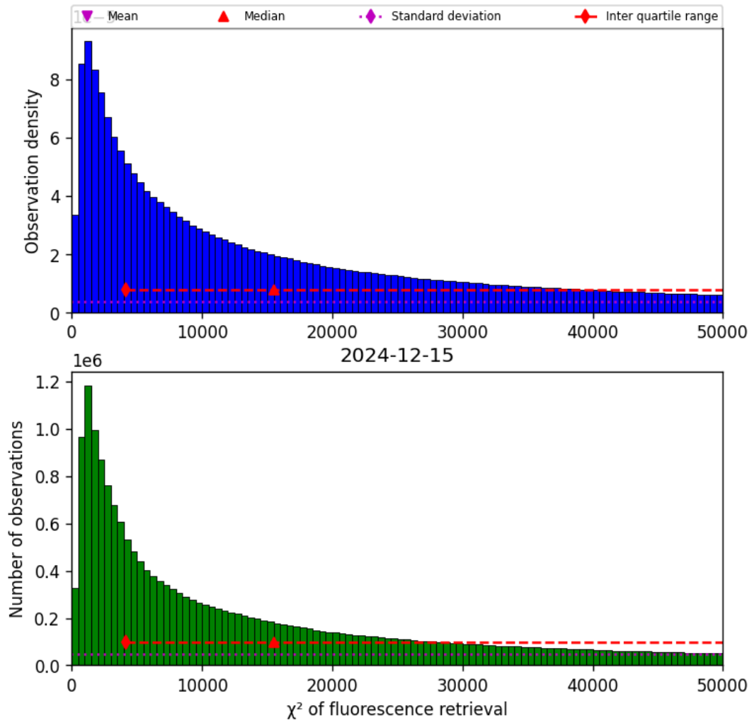
Figure 42: Histogram of “ \chi^2 of fluorescence retrieval” for 2024-12-14 to 2024-12-16
