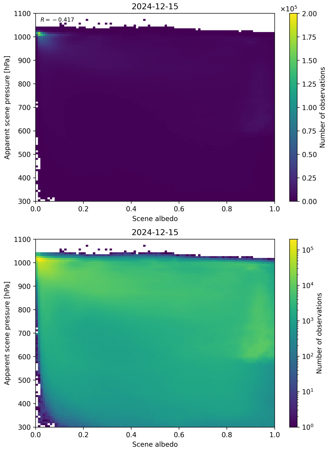
Figure 102: Scatter density plot of “Scene albedo” against “Apparent scene pressure” for 2024-12-14 to 2024-12-16.
