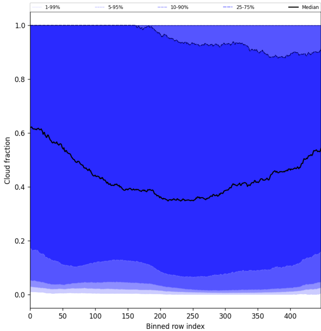
Figure 49: Along track statistics of “Cloud fraction” for 2024-12-14 to 2024-12-16
