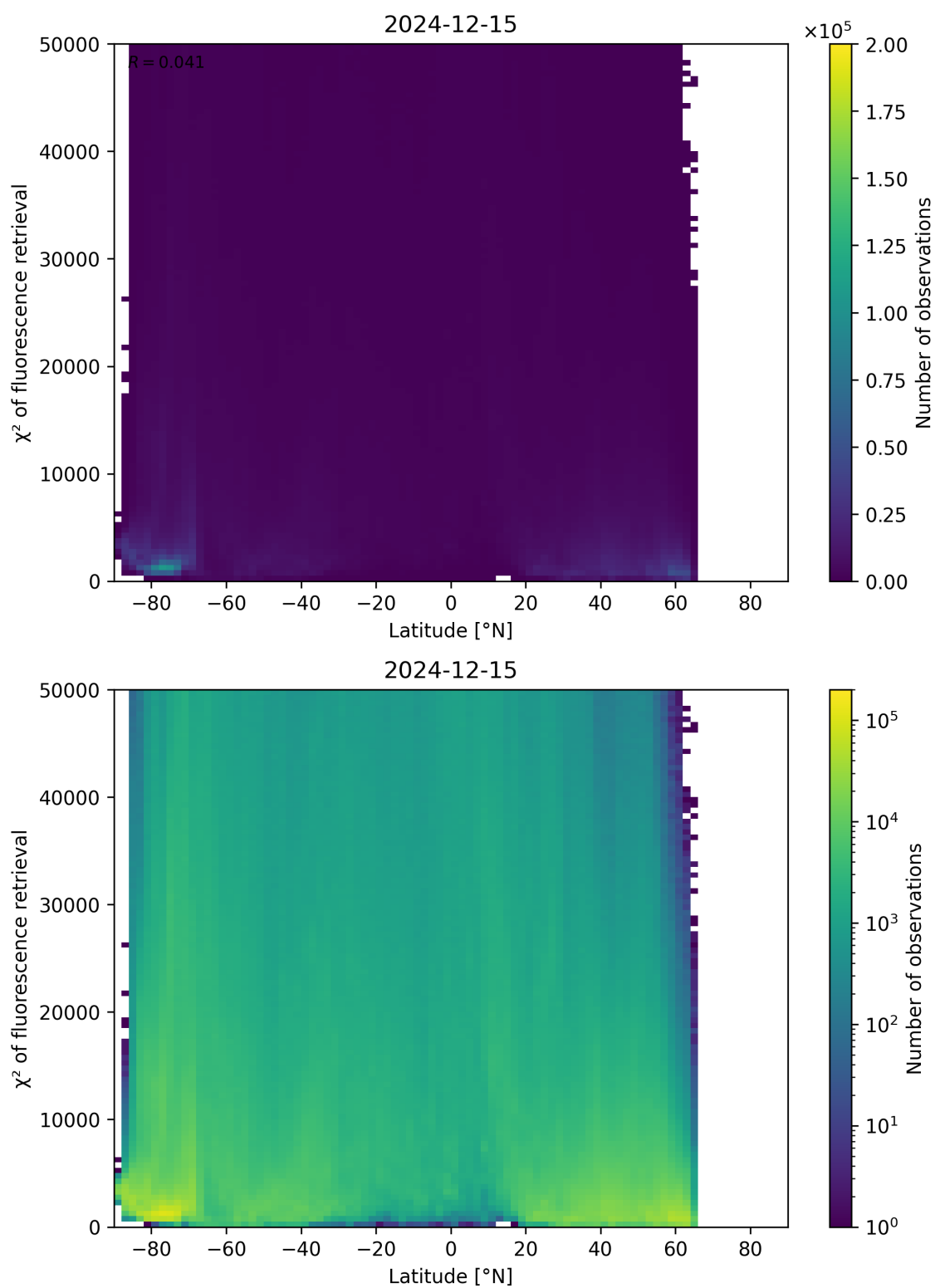
Figure 89: Scatter density plot of “Latitude” against “ \chi^2 of fluorescence retrieval” for 2024-12-14 to 2024-12-16.
