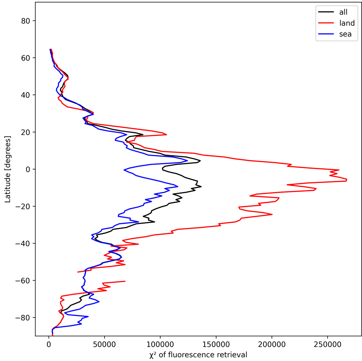
Figure 25: Zonal average of “ \chi^2 of fluorescence retrieval” for 2024-12-14 to 2024-12-16.
