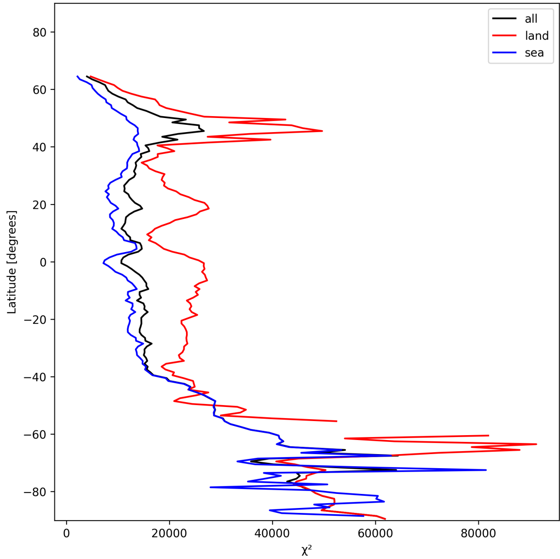
Figure 21: Zonal average of “ \chi^2 ” for 2024-12-14 to 2024-12-16.
