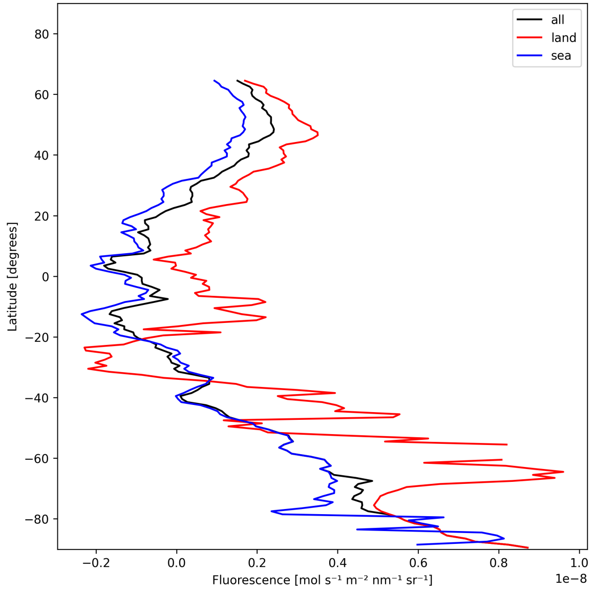
Figure 23: Zonal average of “Fluorescence” for 2024-12-14 to 2024-12-16.
