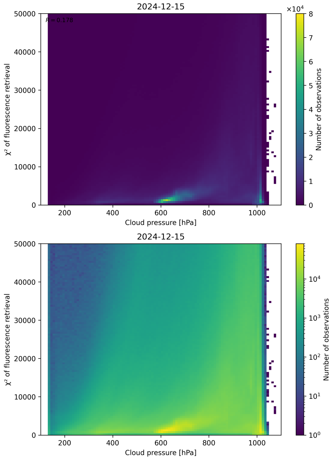
Figure 78: Scatter density plot of “Cloud pressure” against “ \chi^2 of fluorescence retrieval” for 2024-12-14 to 2024-12-16.
