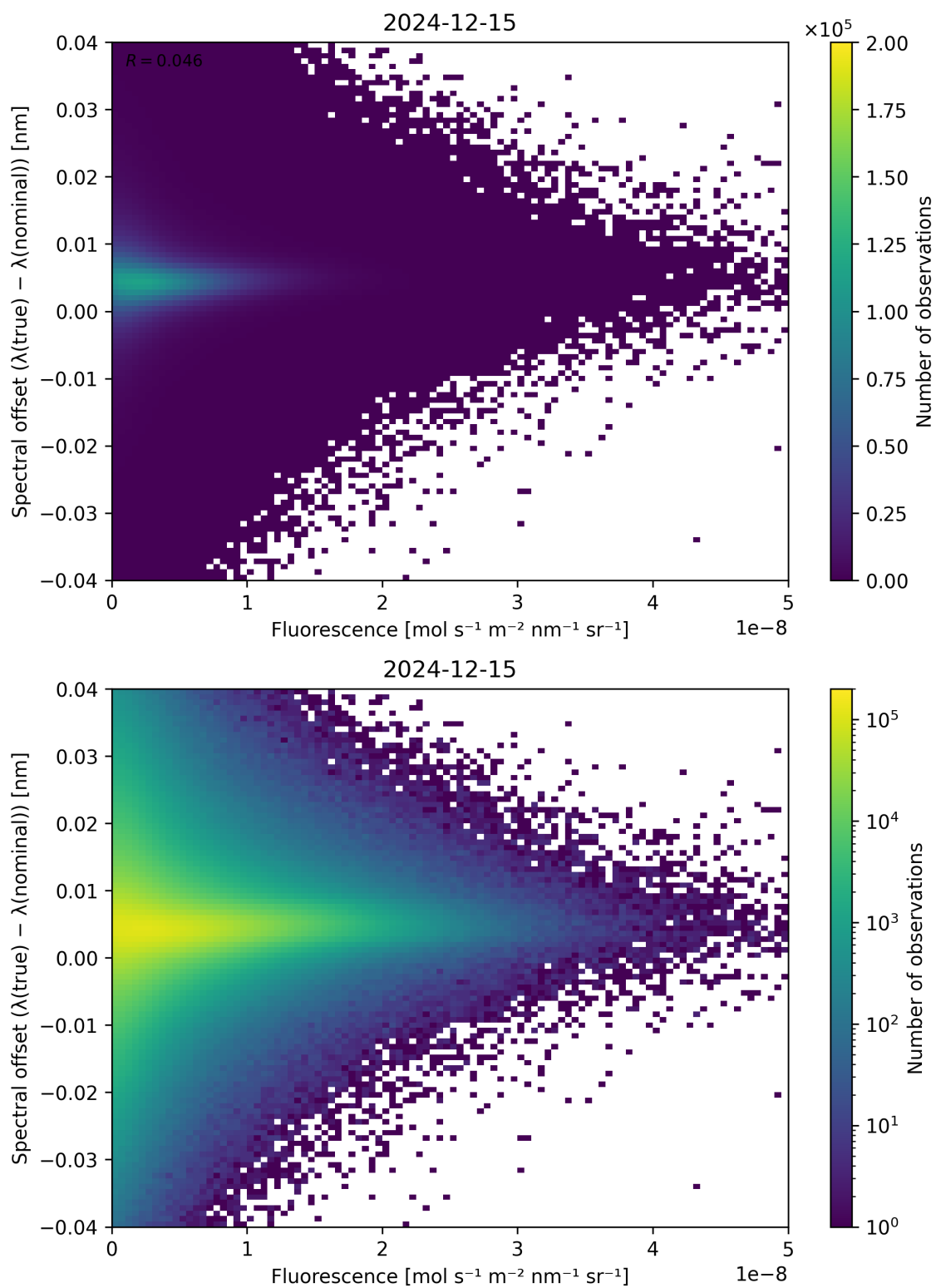
Figure 87: Scatter density plot of “Fluorescence” against “Spectral offset ( \lambda_{\text{true}} - \lambda_{\text{nominal}} )” for 2024-12-14 to 2024-12-16.
