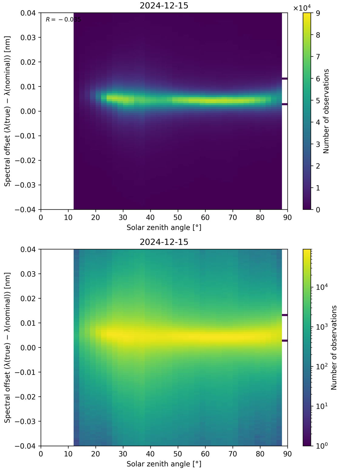
Figure 117: Scatter density plot of “Solar zenith angle” against “Spectral offset ( \lambda_{\text{true}} - \lambda_{\text{nominal}} )” for 2024-12-14 to 2024-12-16.
