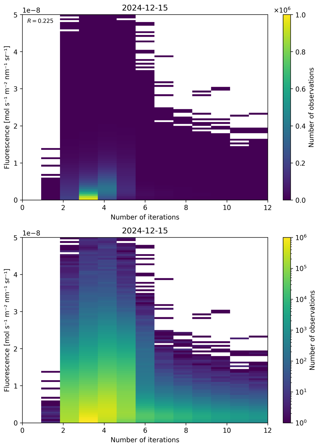
Figure 98: Scatter density plot of “Number of iterations” against “Fluorescence” for 2024-12-14 to 2024-12-16.
