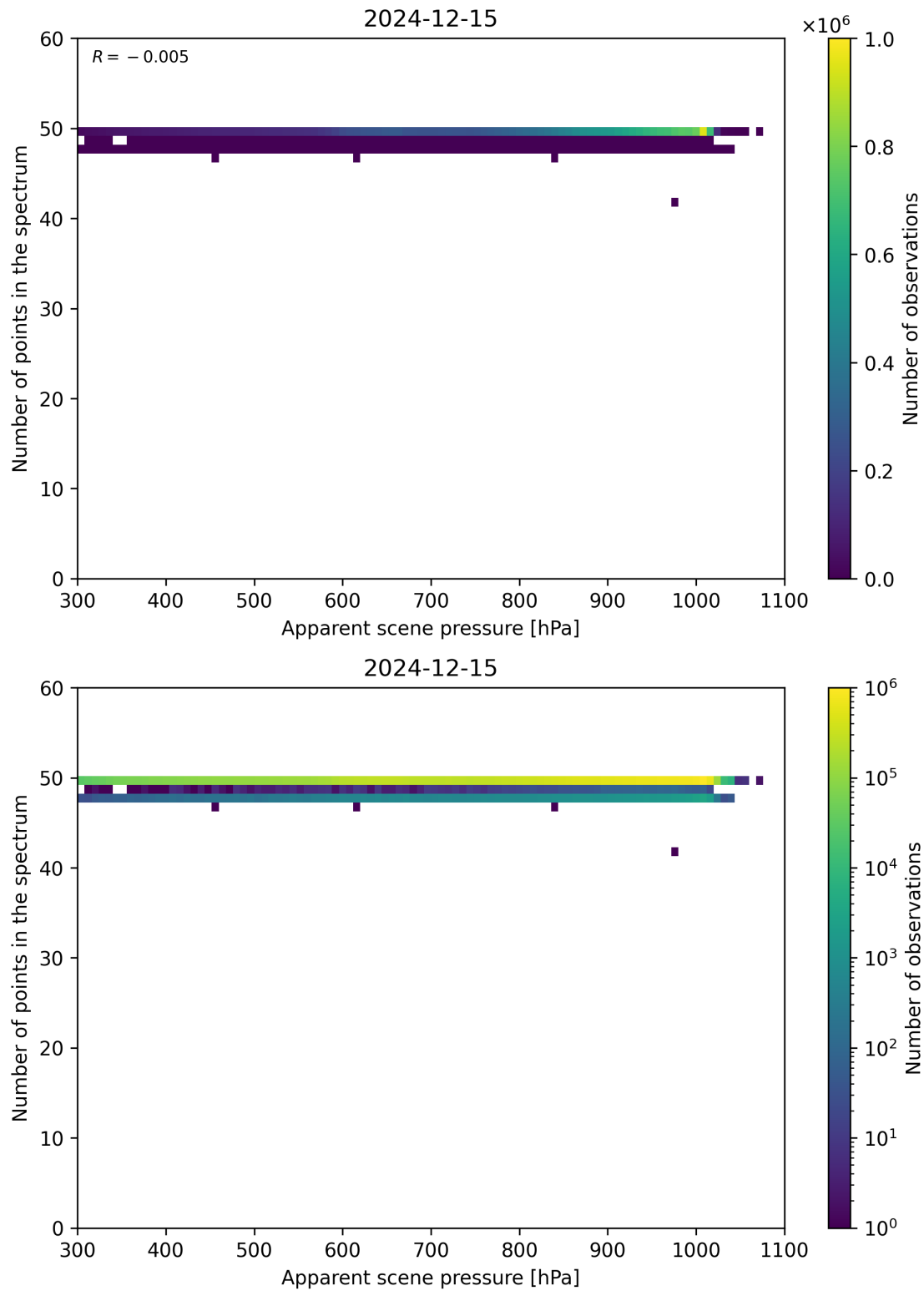
Figure 66: Scatter density plot of “Apparent scene pressure” against “Number of points in the spectrum” for 2024-12-14 to 2024-12-16.
