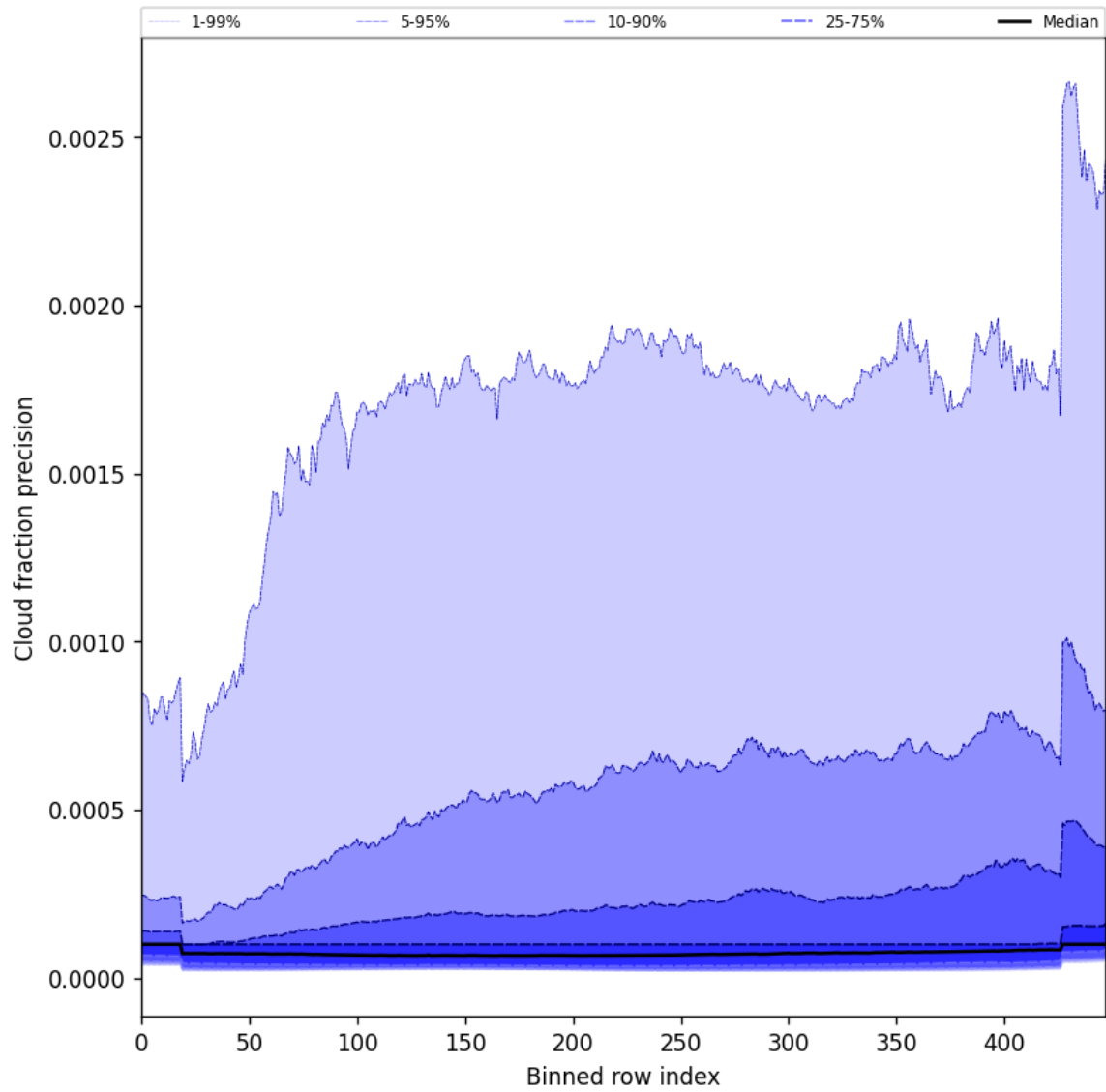
Figure 50: Along track statistics of “Cloud fraction precision” for 2024-12-14 to 2024-12-16
