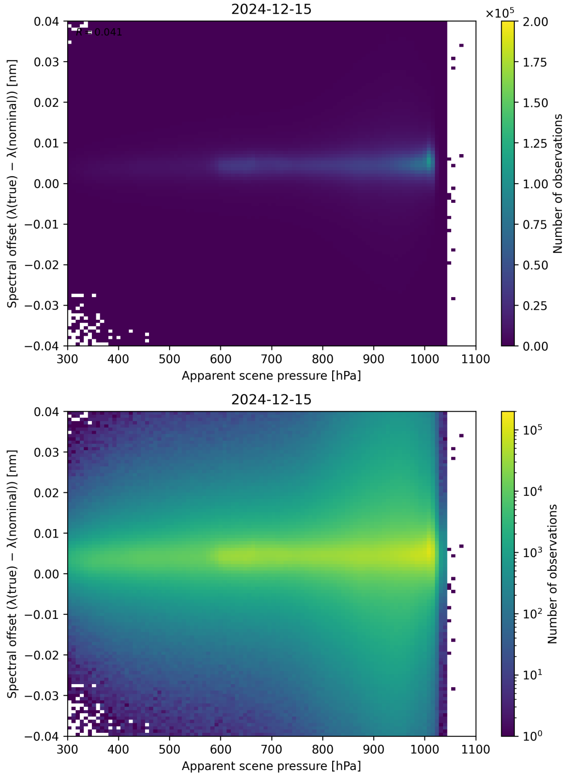
Figure 67: Scatter density plot of “Apparent scene pressure” against “Spectral offset ( \lambda_{\text{true}} - \lambda_{\text{nominal}} )” for 2024-12-14 to 2024-12-16.
