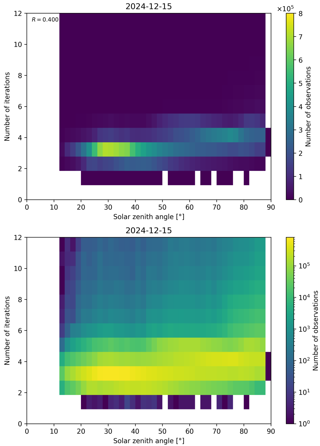
Figure 114: Scatter density plot of “Solar zenith angle” against “Number of iterations” for 2024-12-14 to 2024-12-16.
