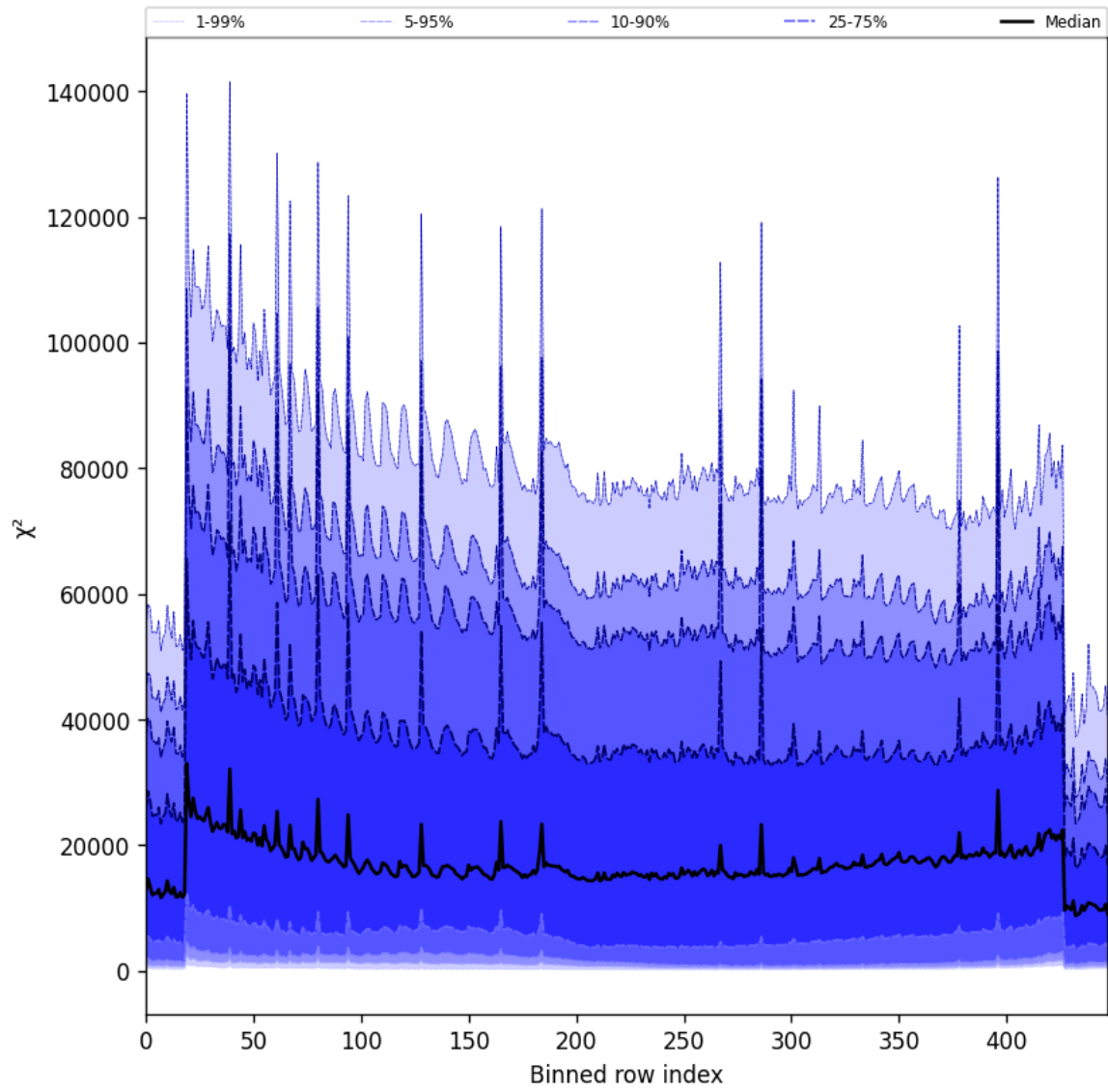
Figure 55: Along track statistics of “ \chi^2 ” for 2024-12-14 to 2024-12-16
