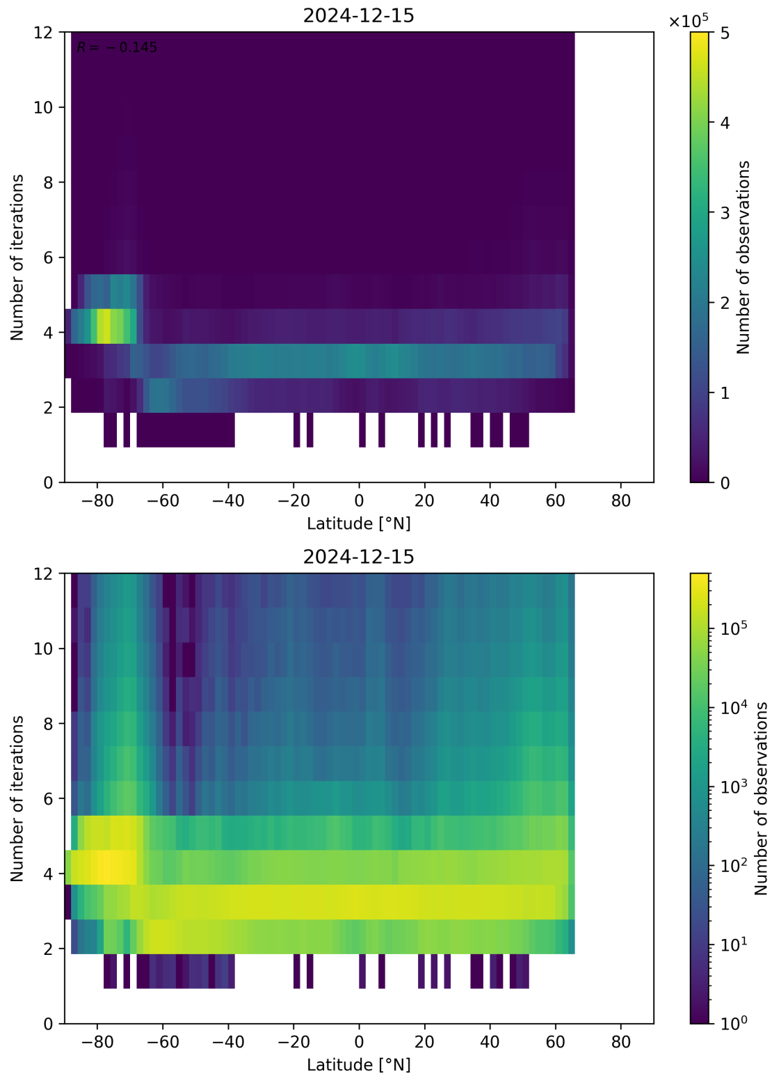
Figure 93: Scatter density plot of “Latitude” against “Number of iterations” for 2024-12-14 to 2024-12-16.
