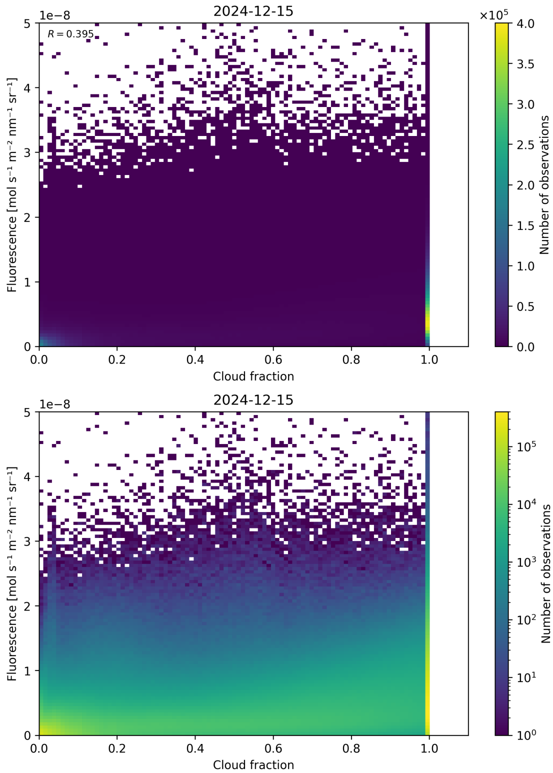
Figure 72: Scatter density plot of “Cloud fraction” against “Fluorescence” for 2024-12-14 to 2024-12-16.
