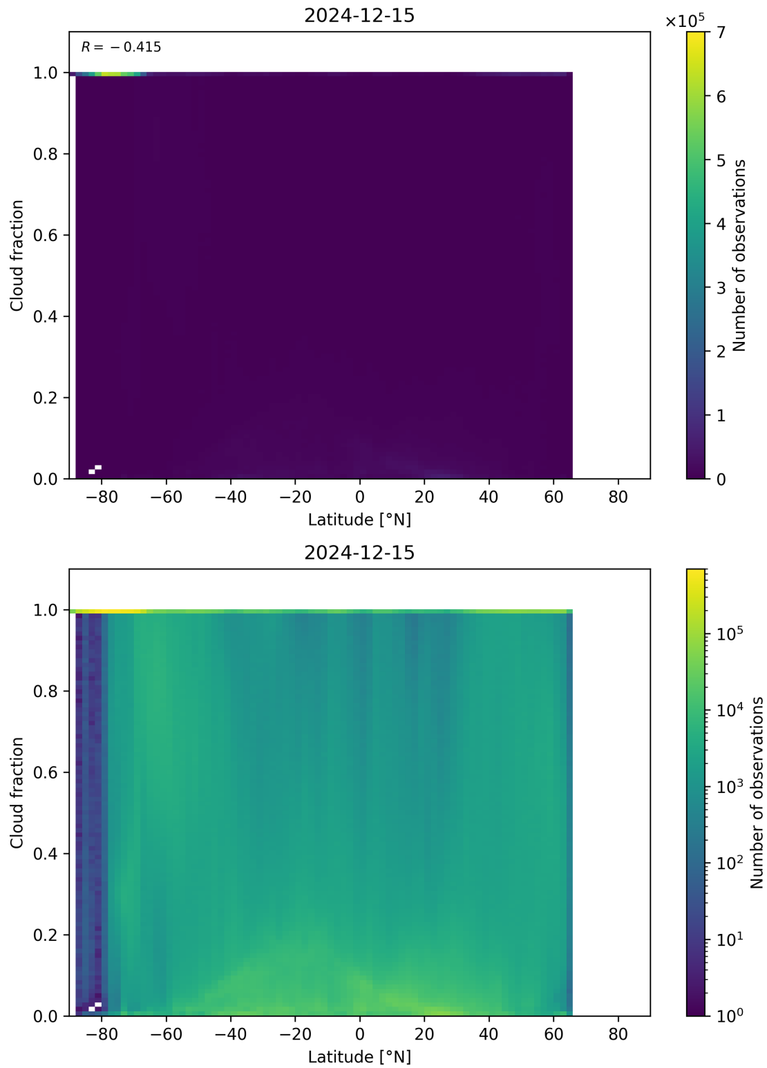
Figure 90: Scatter density plot of “Latitude” against “Cloud fraction” for 2024-12-14 to 2024-12-16.
