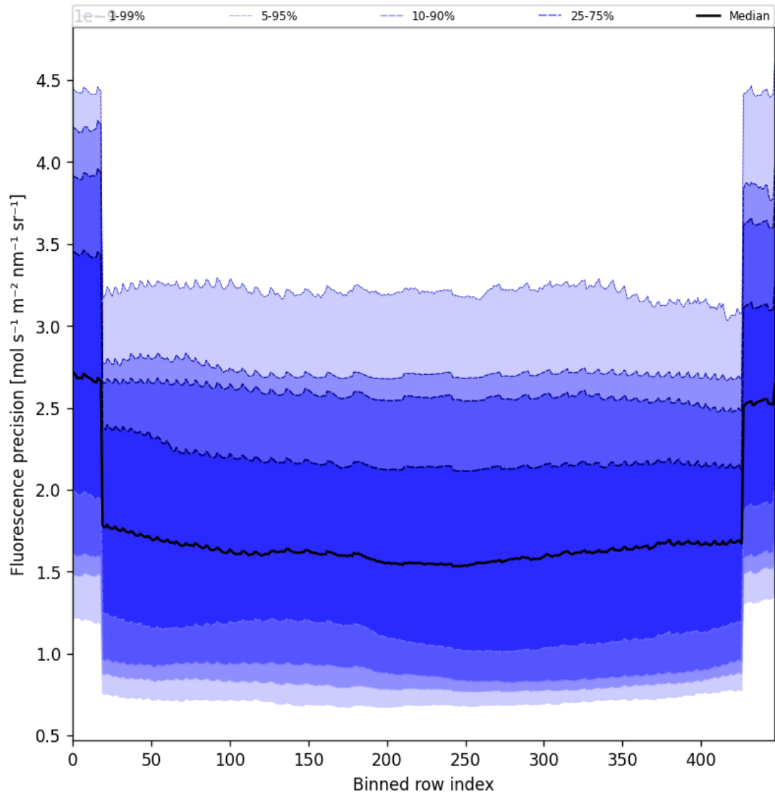
Figure 58: Along track statistics of “Fluorescence precision” for 2024-12-14 to 2024-12-16
