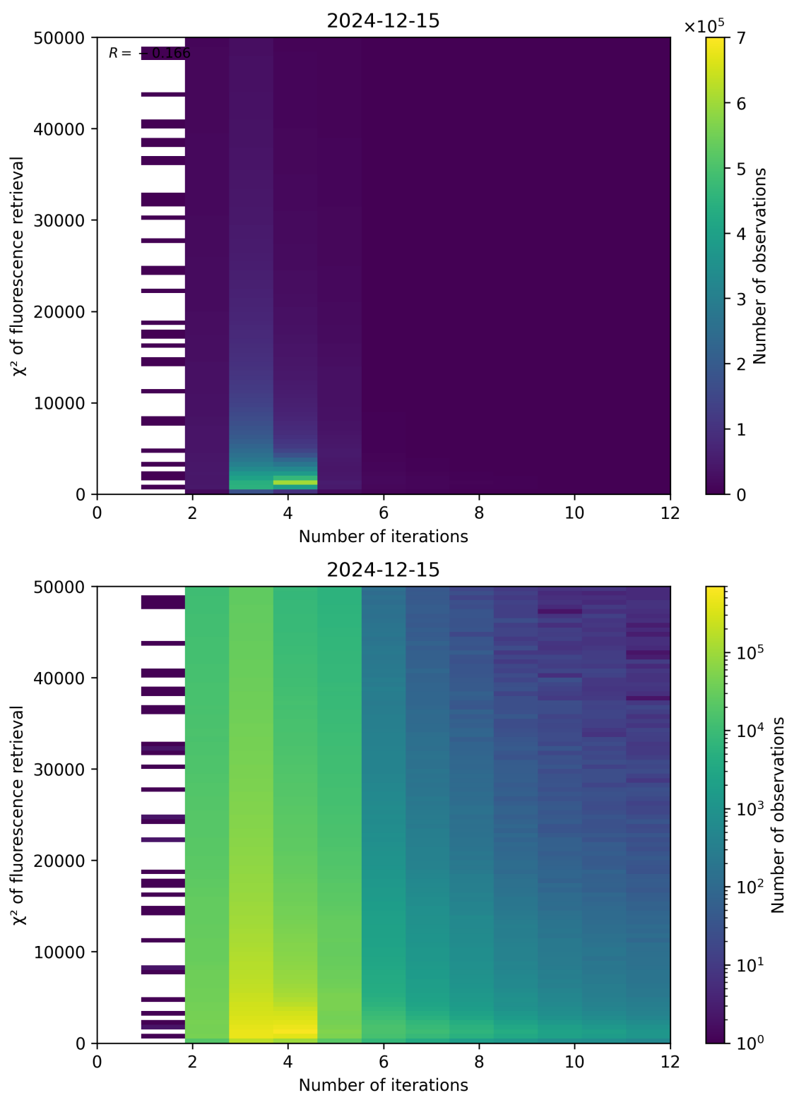
Figure 97: Scatter density plot of “Number of iterations” against “ \chi^2 of fluorescence retrieval” for 2024-12-14 to 2024-12-16.
