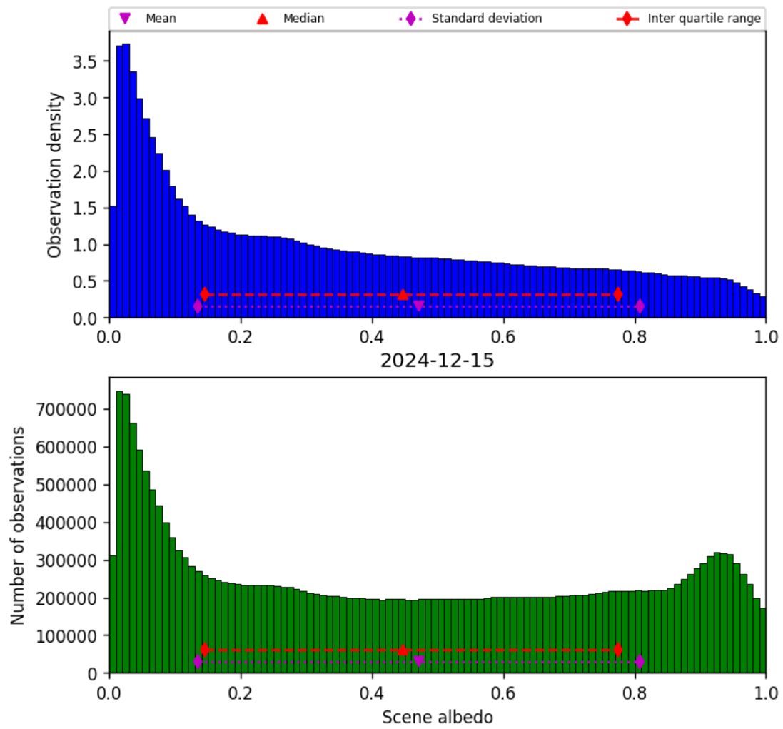
Figure 34: Histogram of “Scene albedo” for 2024-12-14 to 2024-12-16
