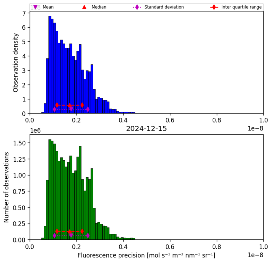
Figure 41: Histogram of “Fluorescence precision” for 2024-12-14 to 2024-12-16
