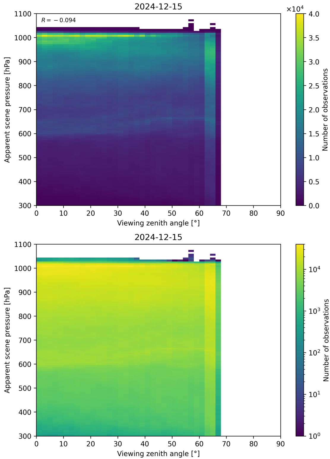
Figure 118: Scatter density plot of “Viewing zenith angle” against “Apparent scene pressure” for 2024-12-14 to 2024-12-16.
