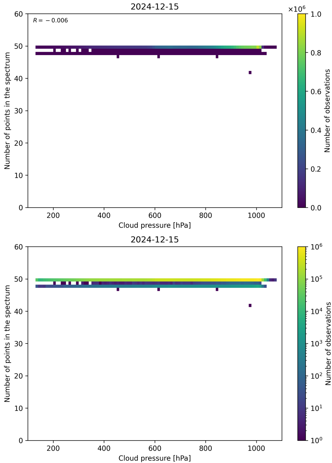
Figure 82: Scatter density plot of “Cloud pressure” against “Number of points in the spectrum” for 2024-12-14 to 2024-12-16.
