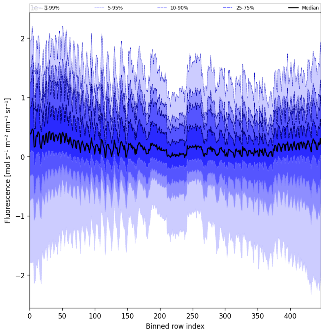
Figure 57: Along track statistics of “Fluorescence” for 2024-12-14 to 2024-12-16
