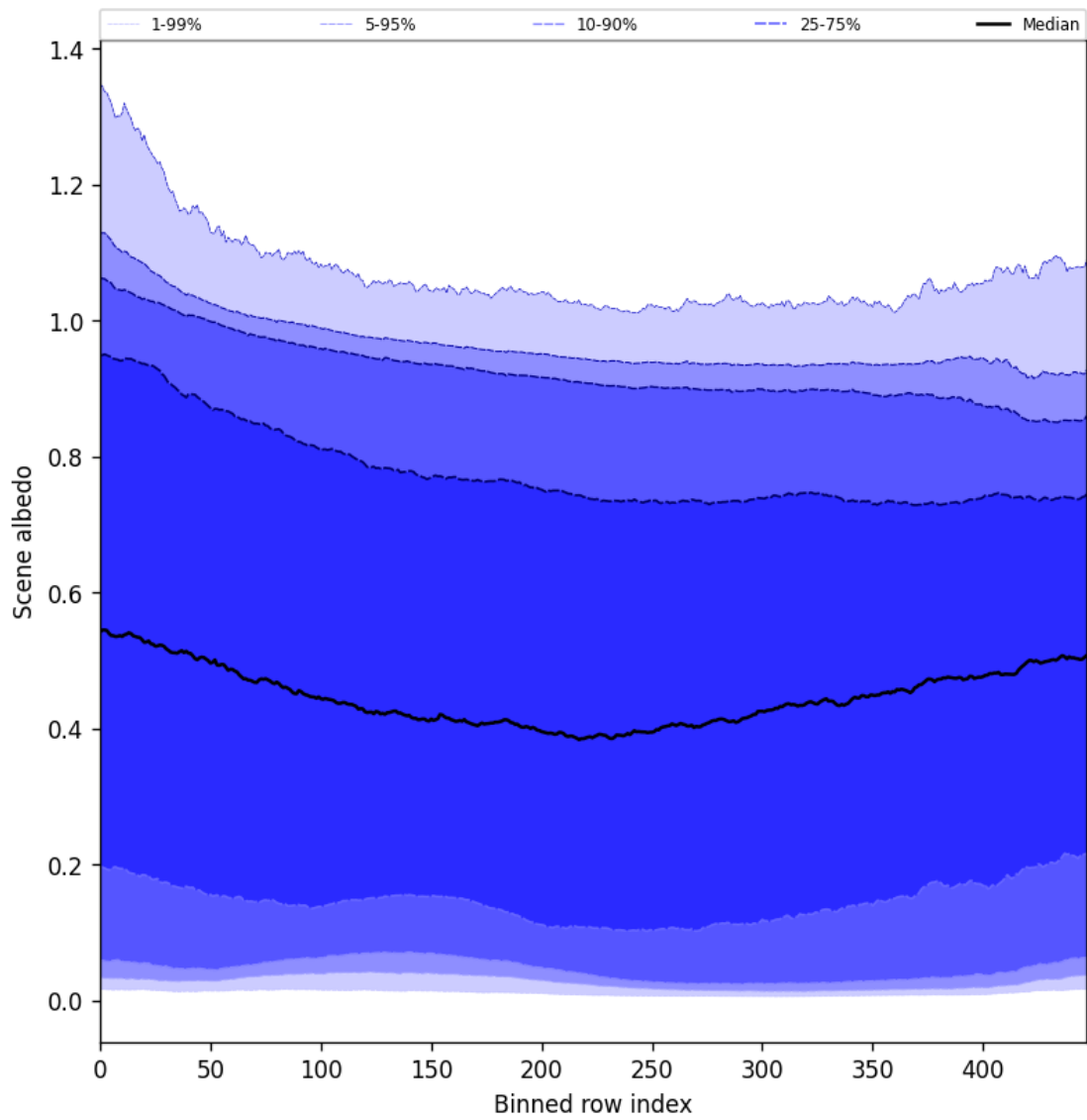
Figure 51: Along track statistics of “Scene albedo” for 2024-12-14 to 2024-12-16
