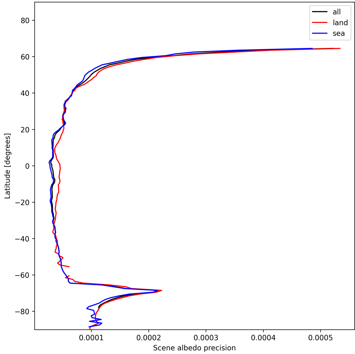
Figure 18: Zonal average of “Scene albedo precision” for 2024-12-14 to 2024-12-16.
