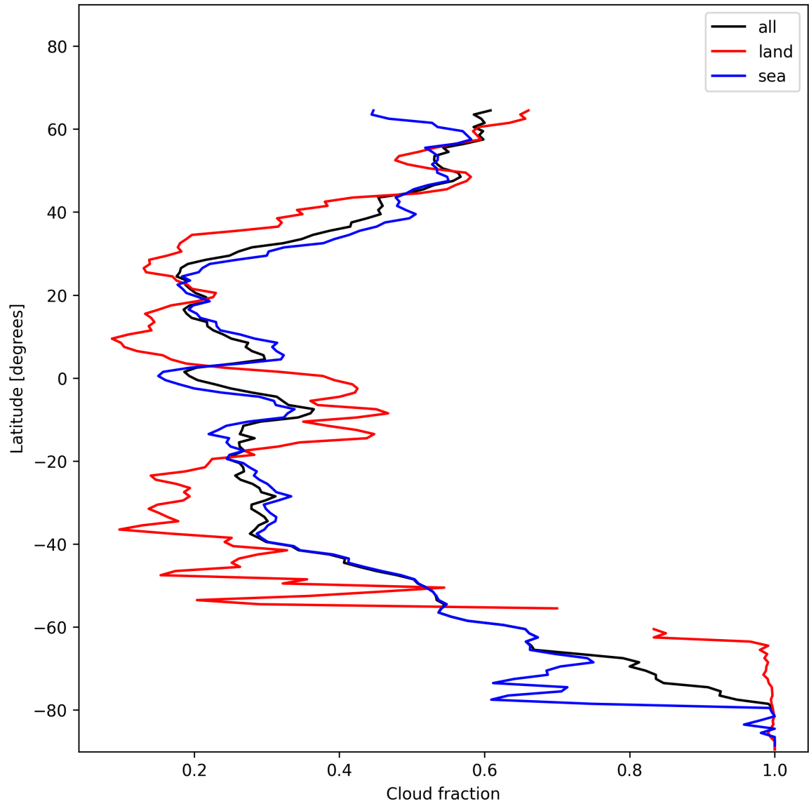
Figure 15: Zonal average of “Cloud fraction” for 2024-12-14 to 2024-12-16.
