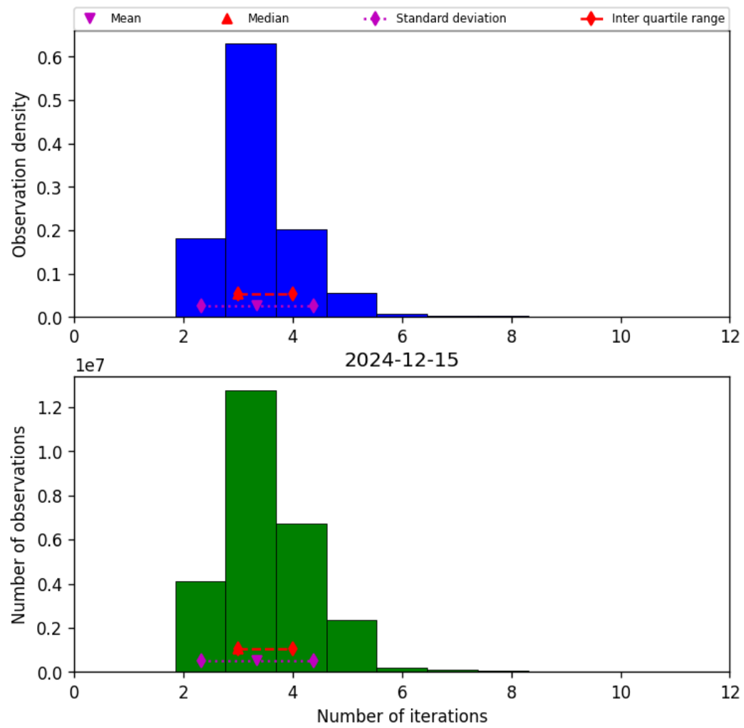
Figure 39: Histogram of “Number of iterations” for 2024-12-14 to 2024-12-16
