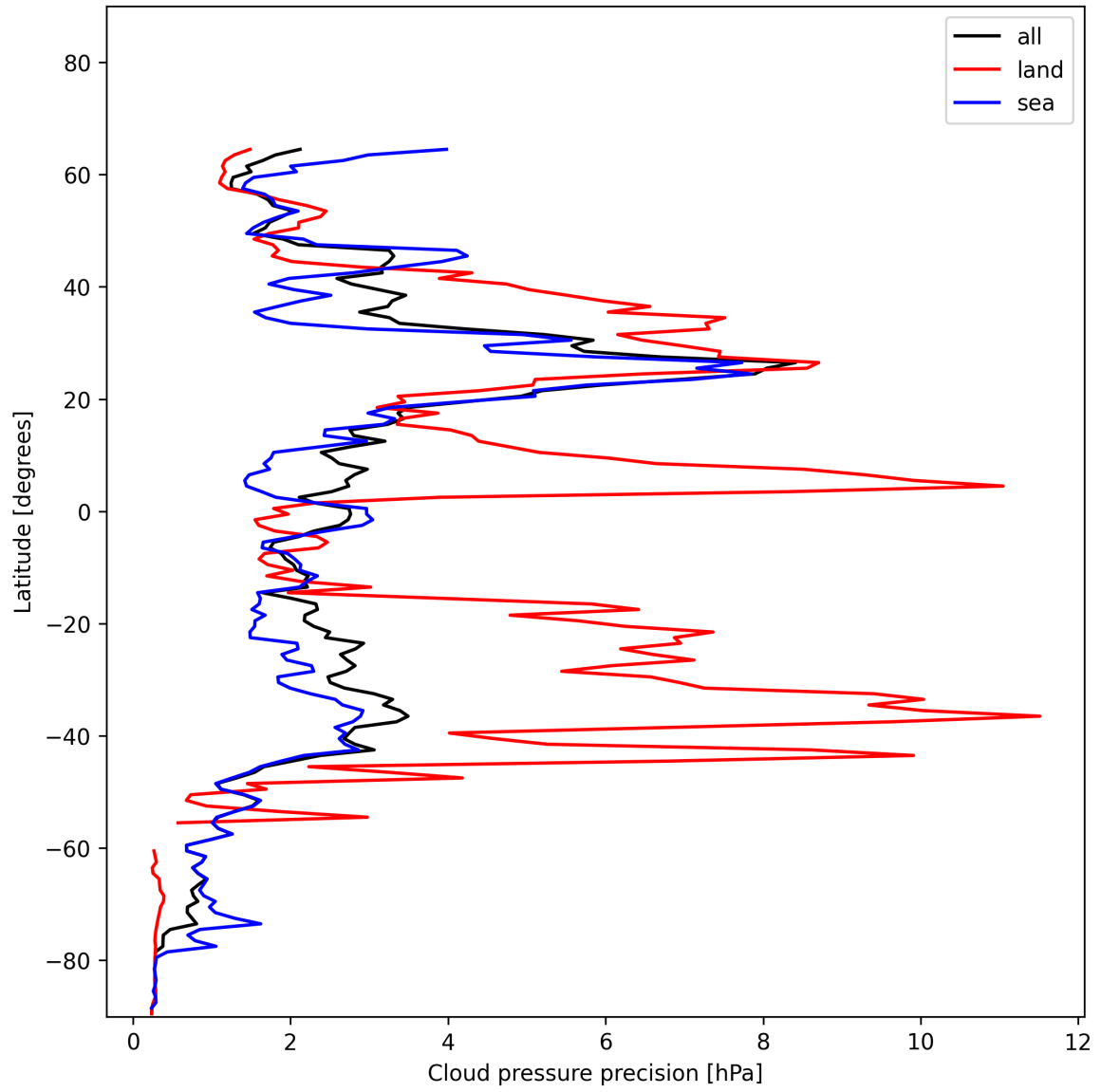
Figure 14: Zonal average of “Cloud pressure precision” for 2024-12-14 to 2024-12-16.
