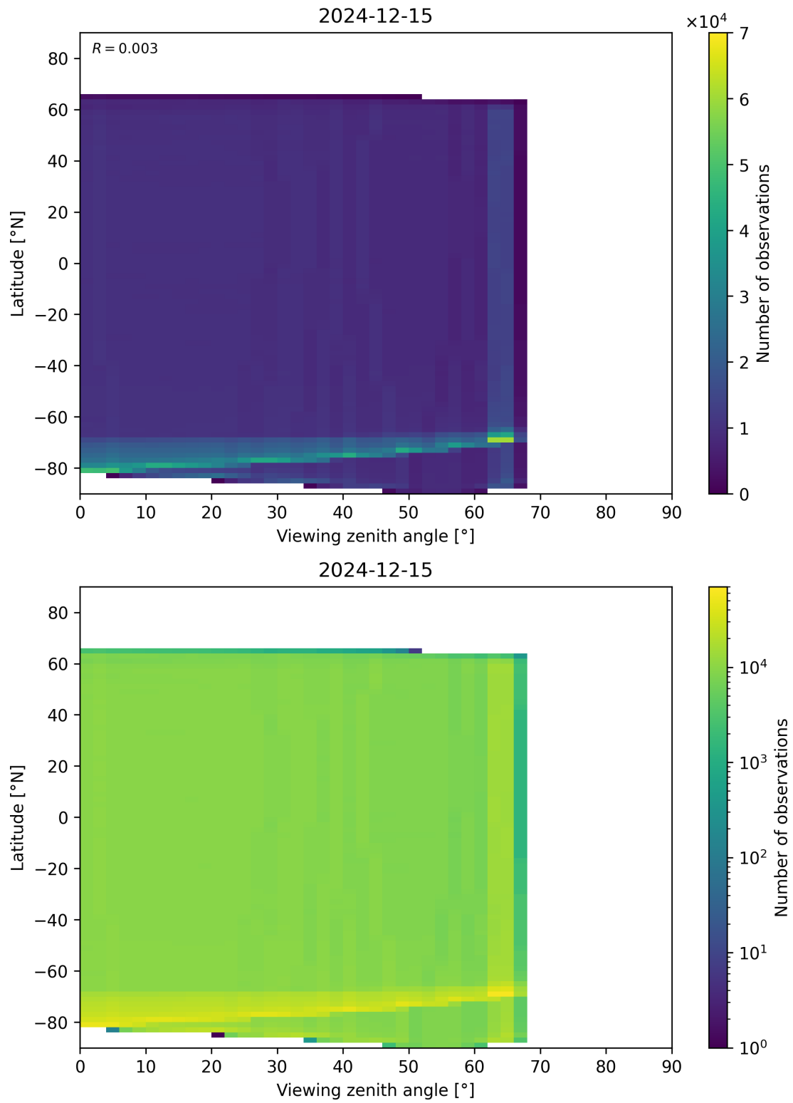
Figure 123: Scatter density plot of “Viewing zenith angle” against “Latitude” for 2024-12-14 to 2024-12-16.
