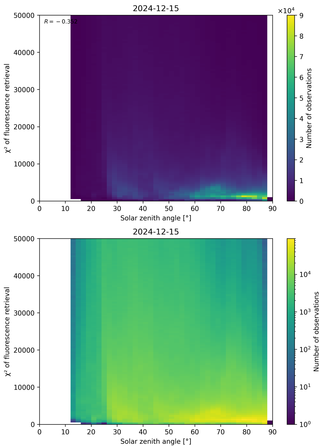
Figure 109: Scatter density plot of “Solar zenith angle” against “ \chi^2 of fluorescence retrieval” for 2024-12-14 to 2024-12-16.
