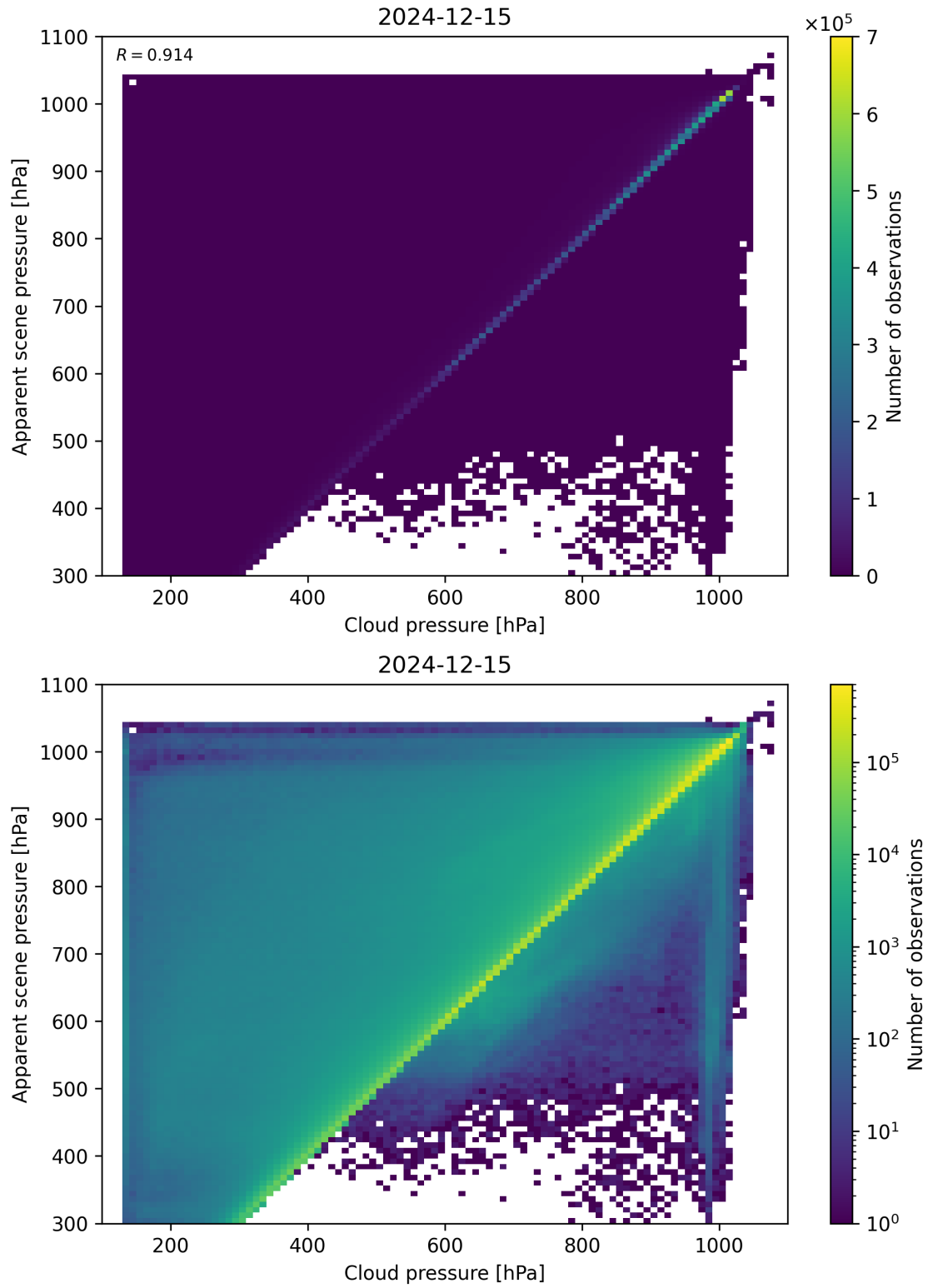
Figure 77: Scatter density plot of “Cloud pressure” against “Apparent scene pressure” for 2024-12-14 to 2024-12-16.
