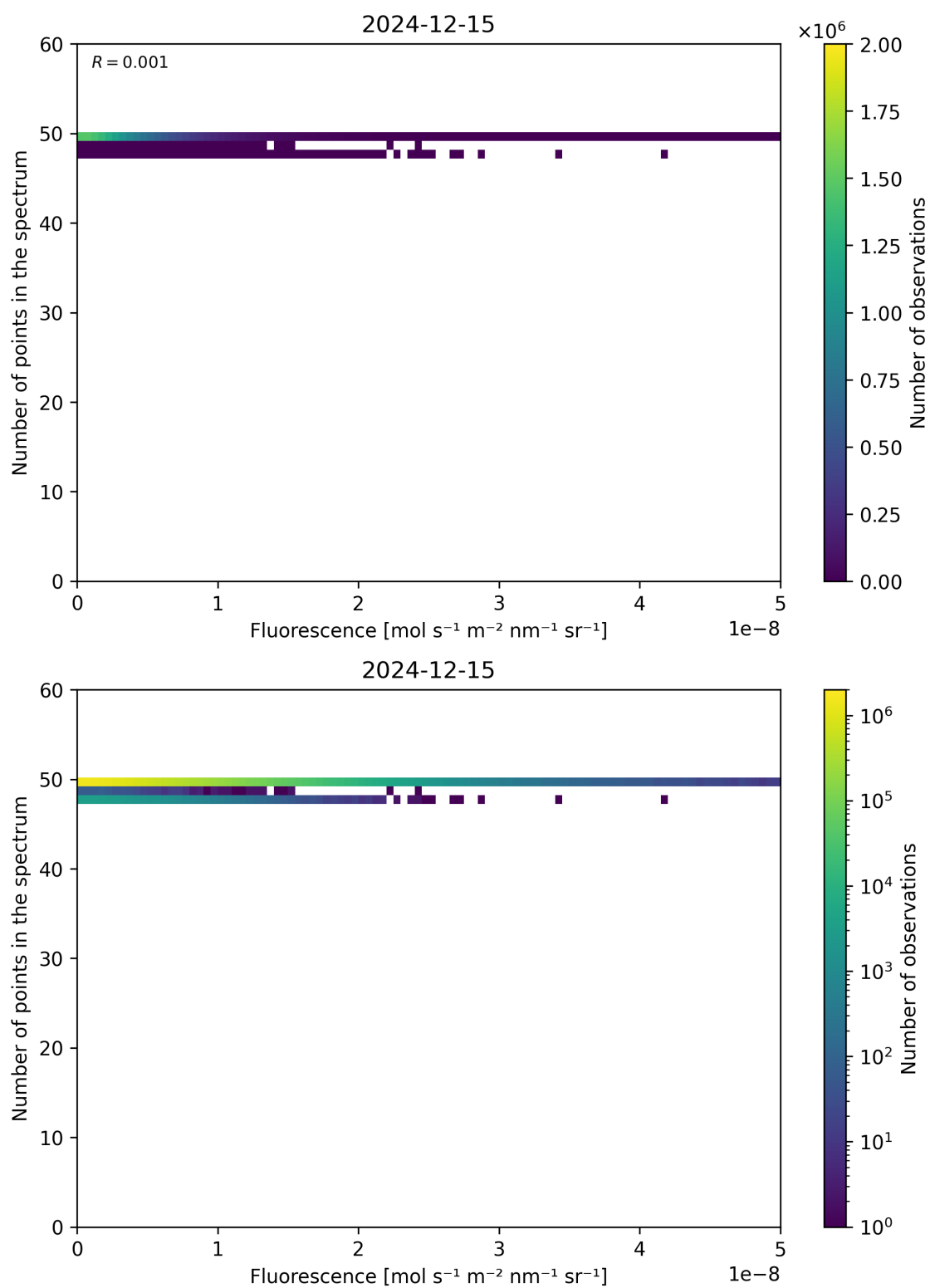
Figure 86: Scatter density plot of “Fluorescence” against “Number of points in the spectrum” for 2024-12-14 to 2024-12-16.
