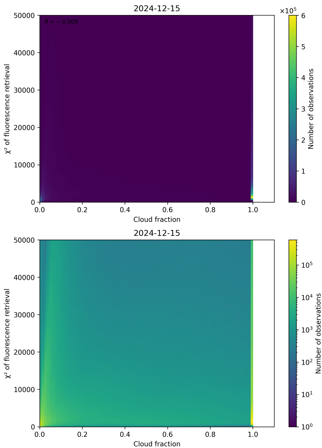
Figure 71: Scatter density plot of “Cloud fraction” against “ \chi^2 of fluorescence retrieval” for 2024-12-14 to 2024-12-16.
