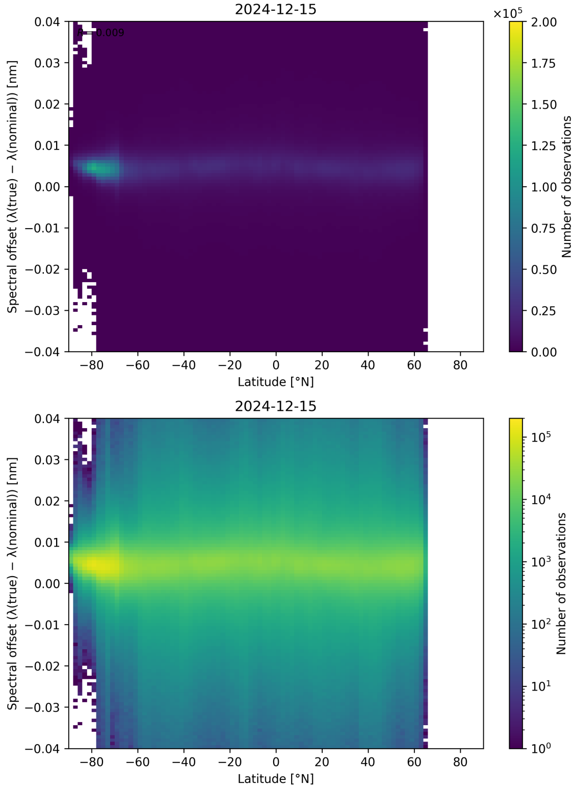
Figure 96: Scatter density plot of “Latitude” against “Spectral offset ( \lambda_{\text{true}} - \lambda_{\text{nominal}} )” for 2024-12-14 to 2024-12-16.
