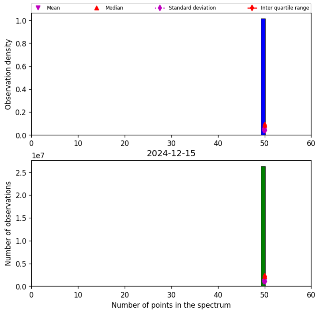
Figure 44: Histogram of “Number of points in the spectrum” for 2024-12-14 to 2024-12-16
