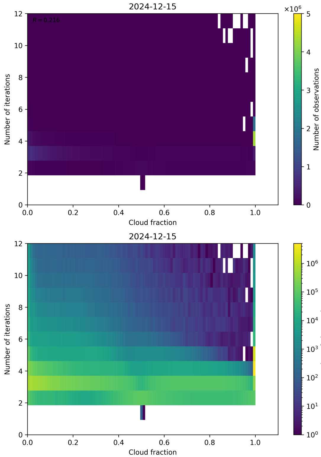
Figure 73: Scatter density plot of “Cloud fraction” against “Number of iterations” for 2024-12-14 to 2024-12-16.
