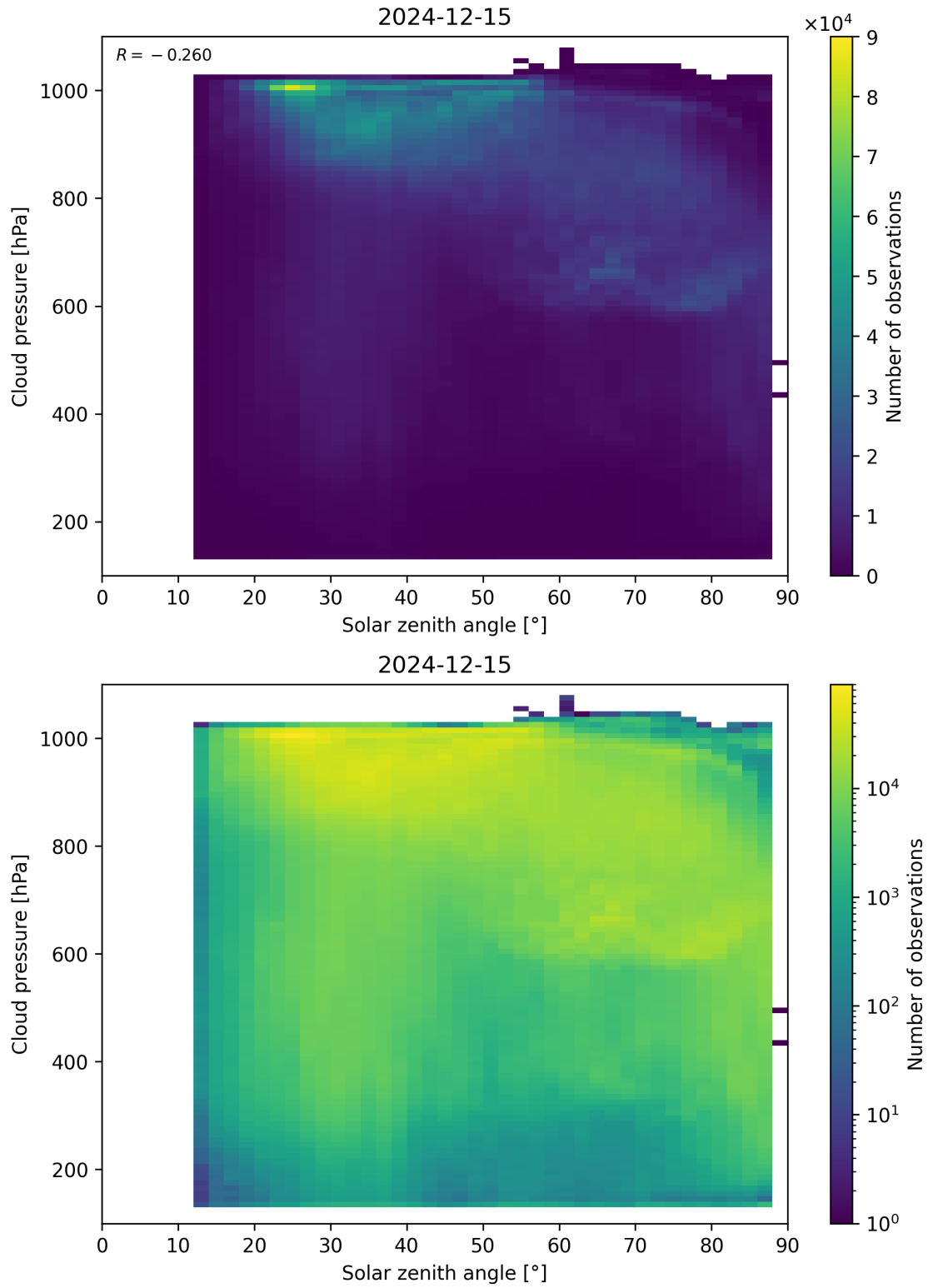
Figure 111: Scatter density plot of “Solar zenith angle” against “Cloud pressure” for 2024-12-14 to 2024-12-16.
