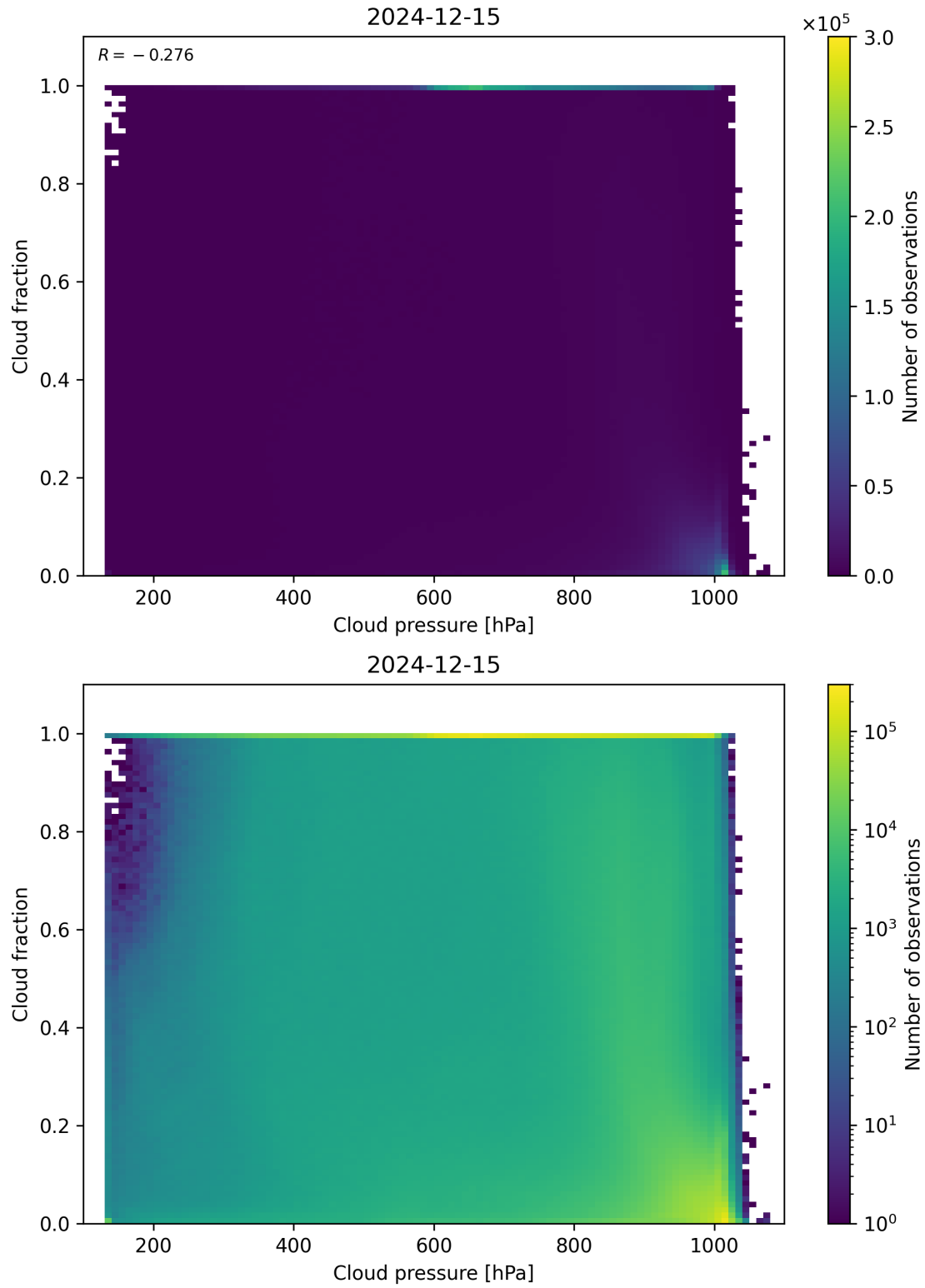
Figure 79: Scatter density plot of “Cloud pressure” against “Cloud fraction” for 2024-12-14 to 2024-12-16.
