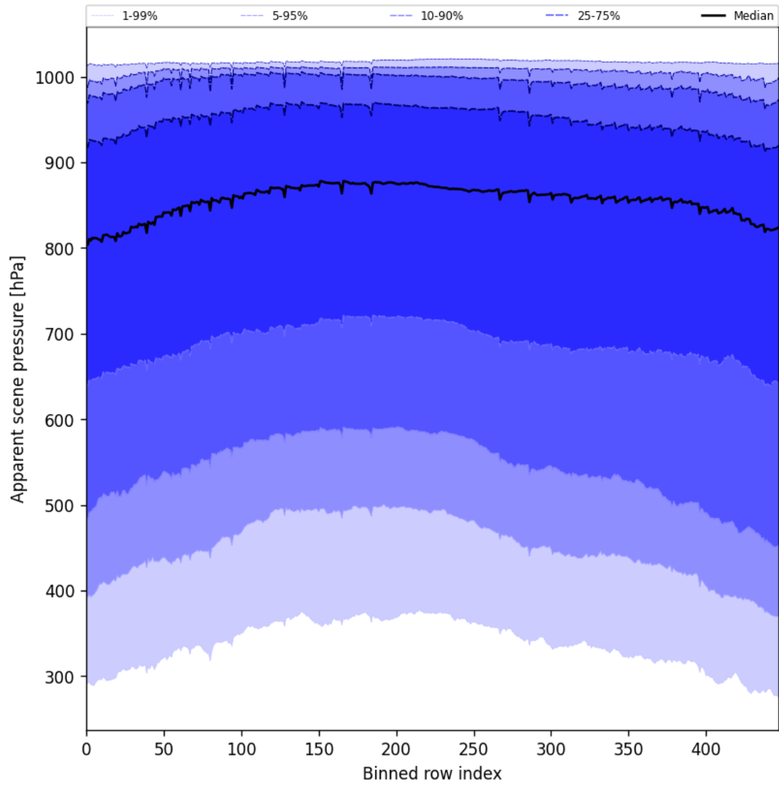
Figure 53: Along track statistics of “Apparent scene pressure” for 2024-12-14 to 2024-12-16
