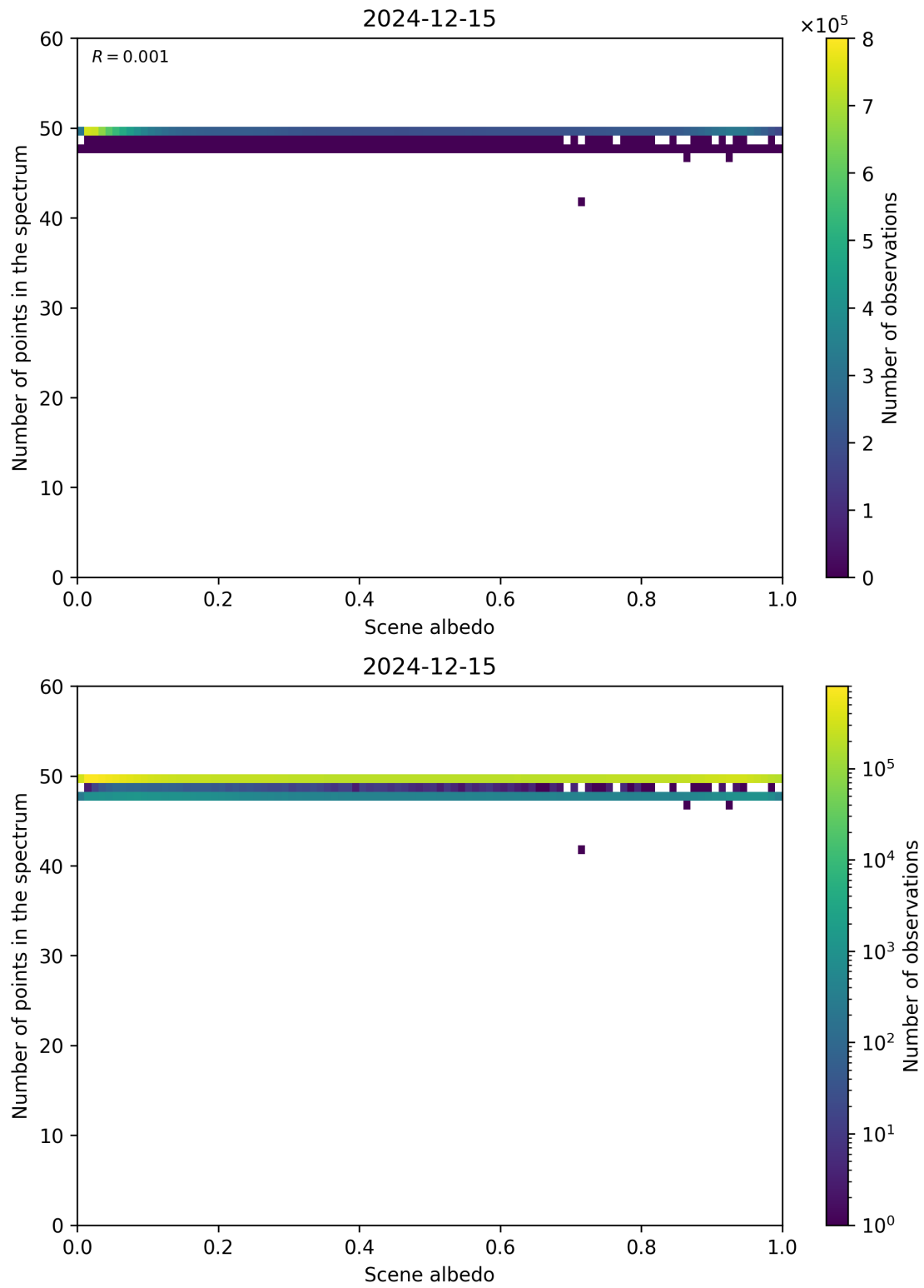
Figure 106: Scatter density plot of “Scene albedo” against “Number of points in the spectrum” for 2024-12-14 to 2024-12-16.
