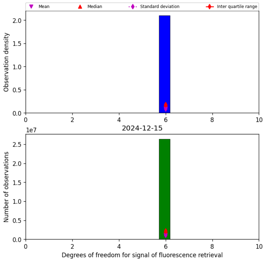
Figure 43: Histogram of “Degrees of freedom for signal of fluorescence retrieval” for 2024-12-14 to 2024-12-16
