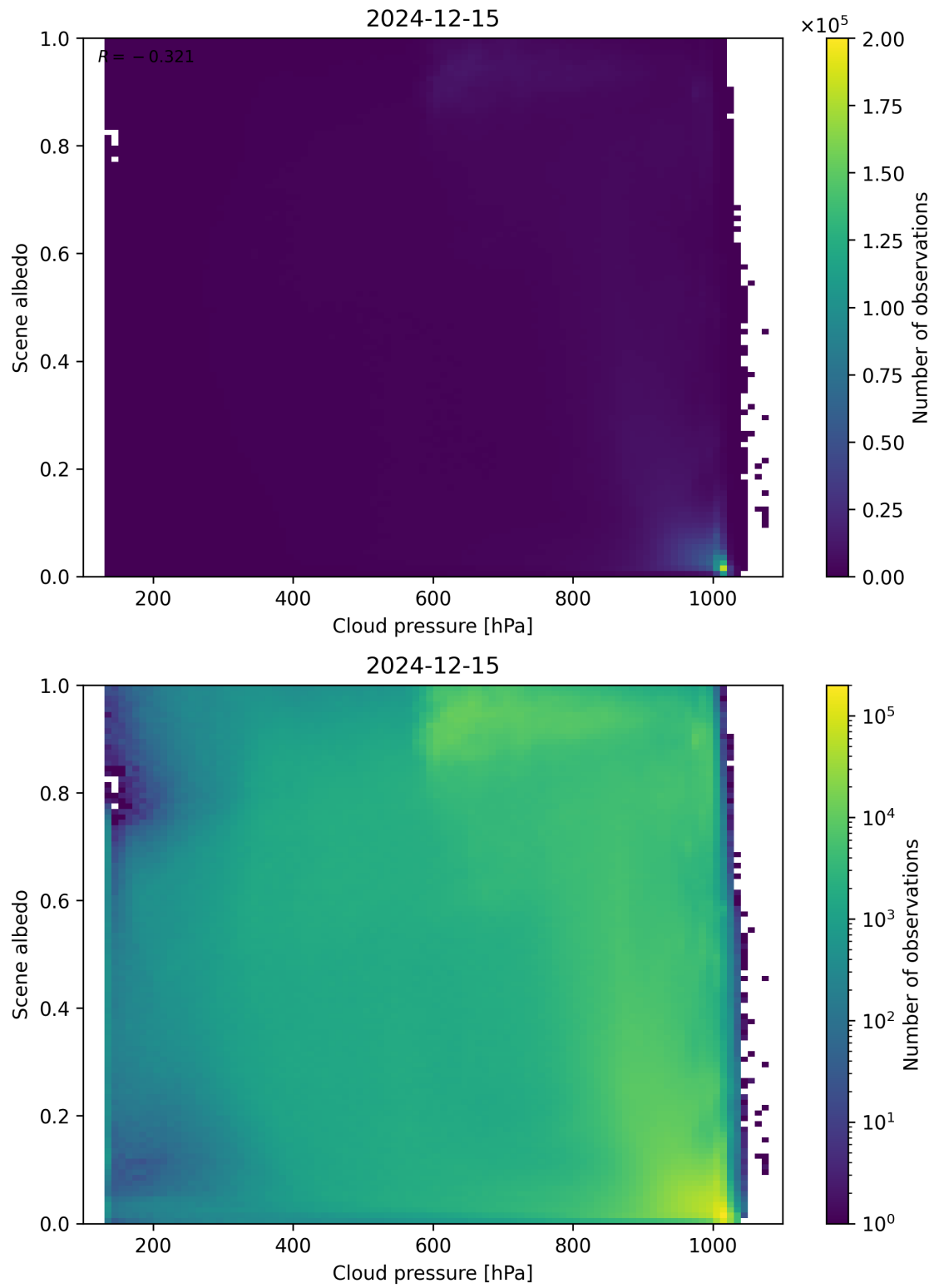
Figure 83: Scatter density plot of “Cloud pressure” against “Scene albedo” for 2024-12-14 to 2024-12-16.
