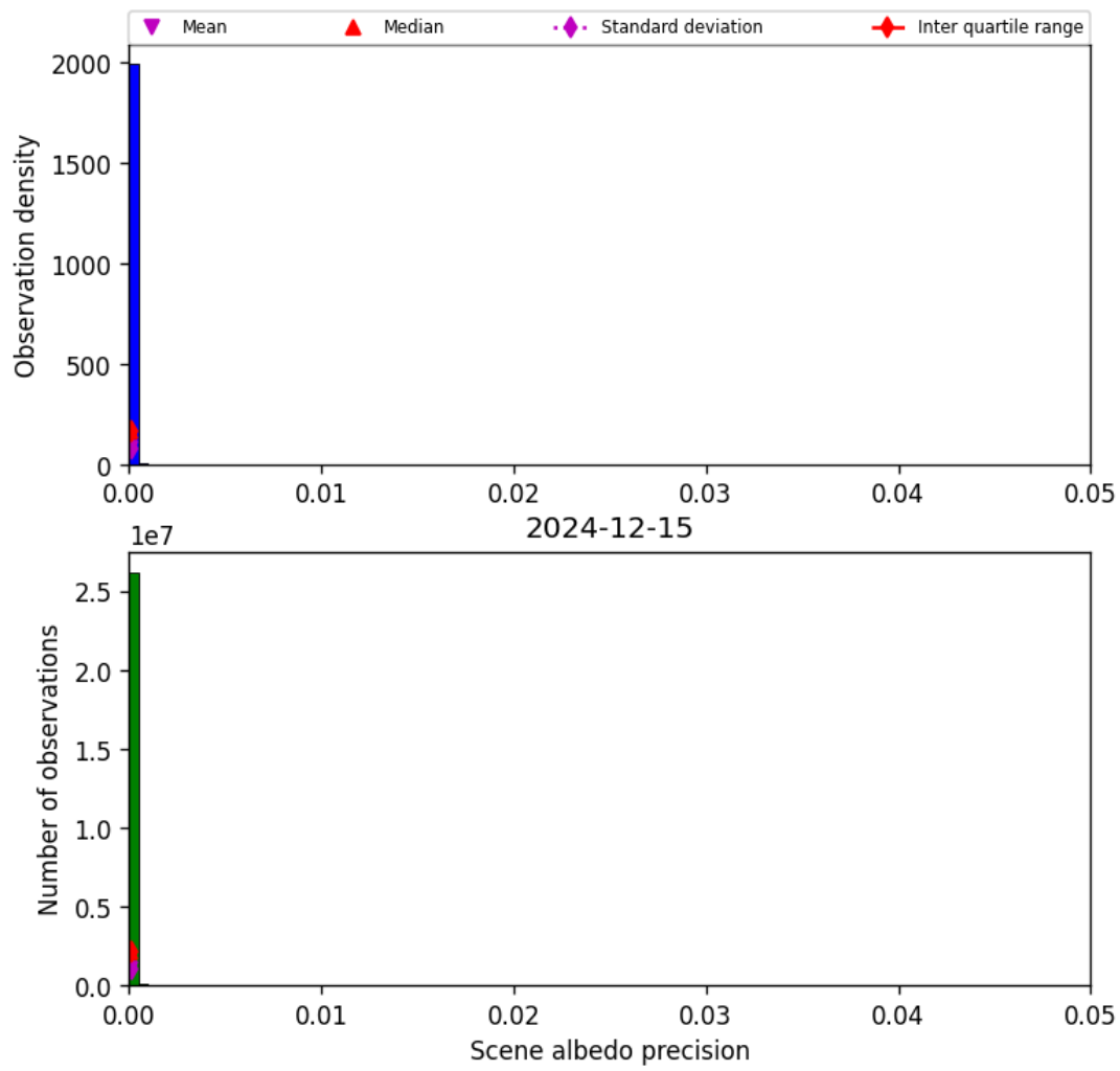
Figure 35: Histogram of “Scene albedo precision” for 2024-12-14 to 2024-12-16
