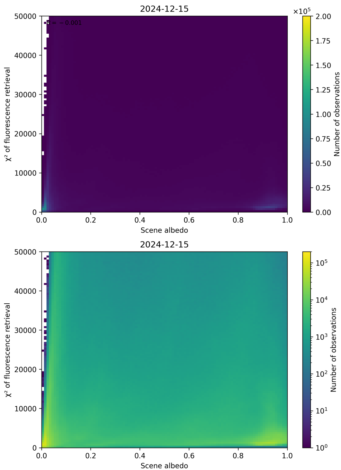
Figure 103: Scatter density plot of “Scene albedo” against “ \chi^2 of fluorescence retrieval” for 2024-12-14 to 2024-12-16.
