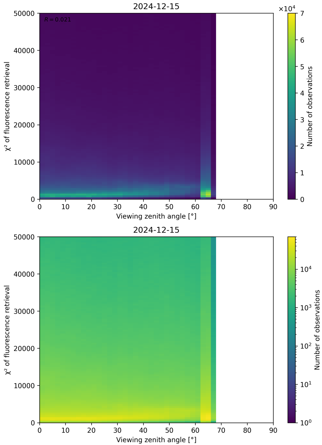
Figure 119: Scatter density plot of “Viewing zenith angle” against “ \chi^2 of fluorescence retrieval” for 2024-12-14 to 2024-12-16.
