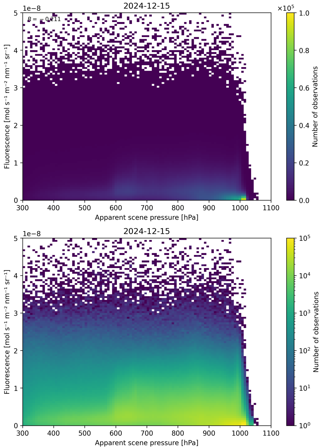
Figure 64: Scatter density plot of “Apparent scene pressure” against “Fluorescence” for 2024-12-14 to 2024-12-16.
