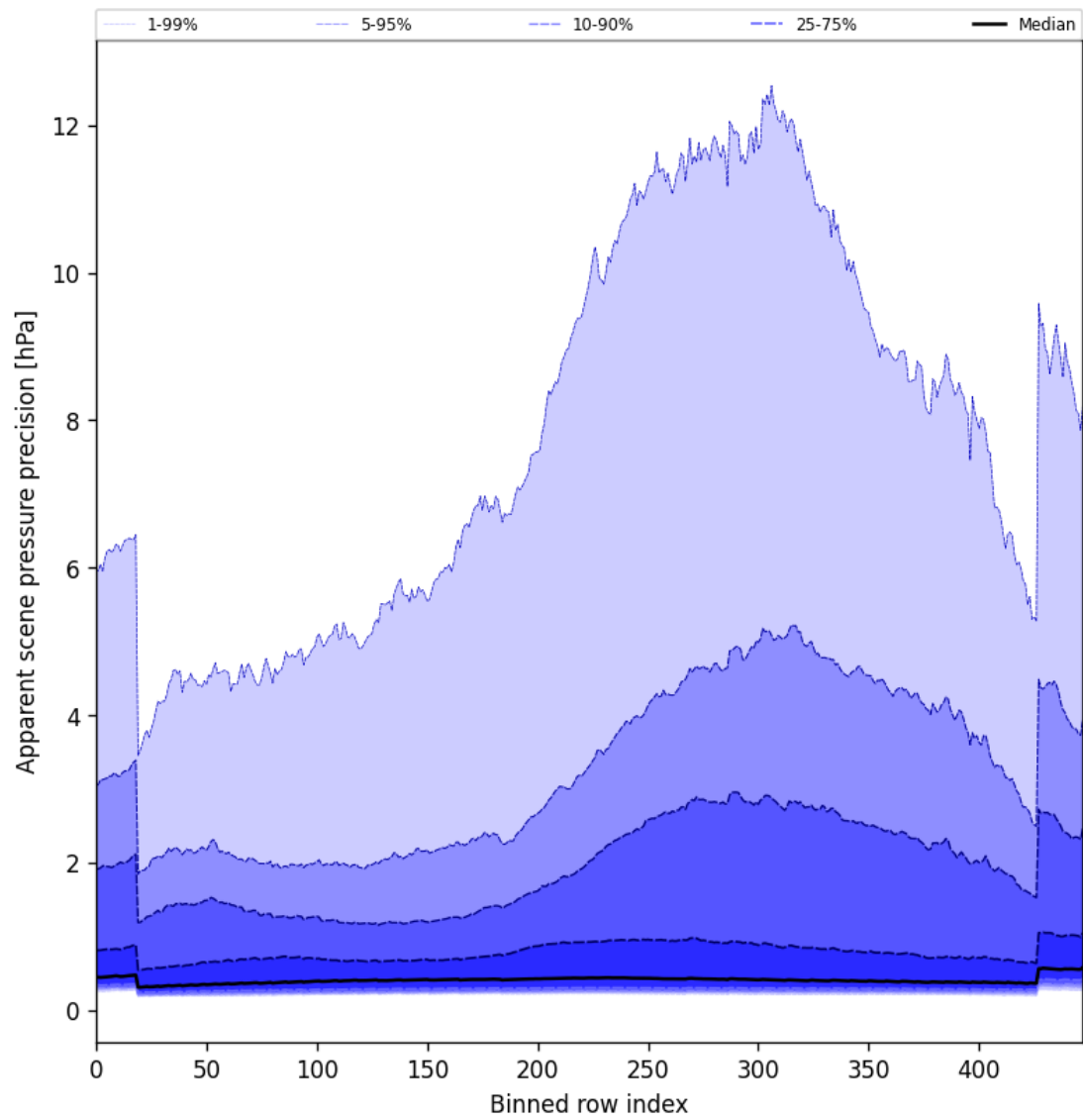
Figure 54: Along track statistics of “Apparent scene pressure precision” for 2024-12-14 to 2024-12-16
