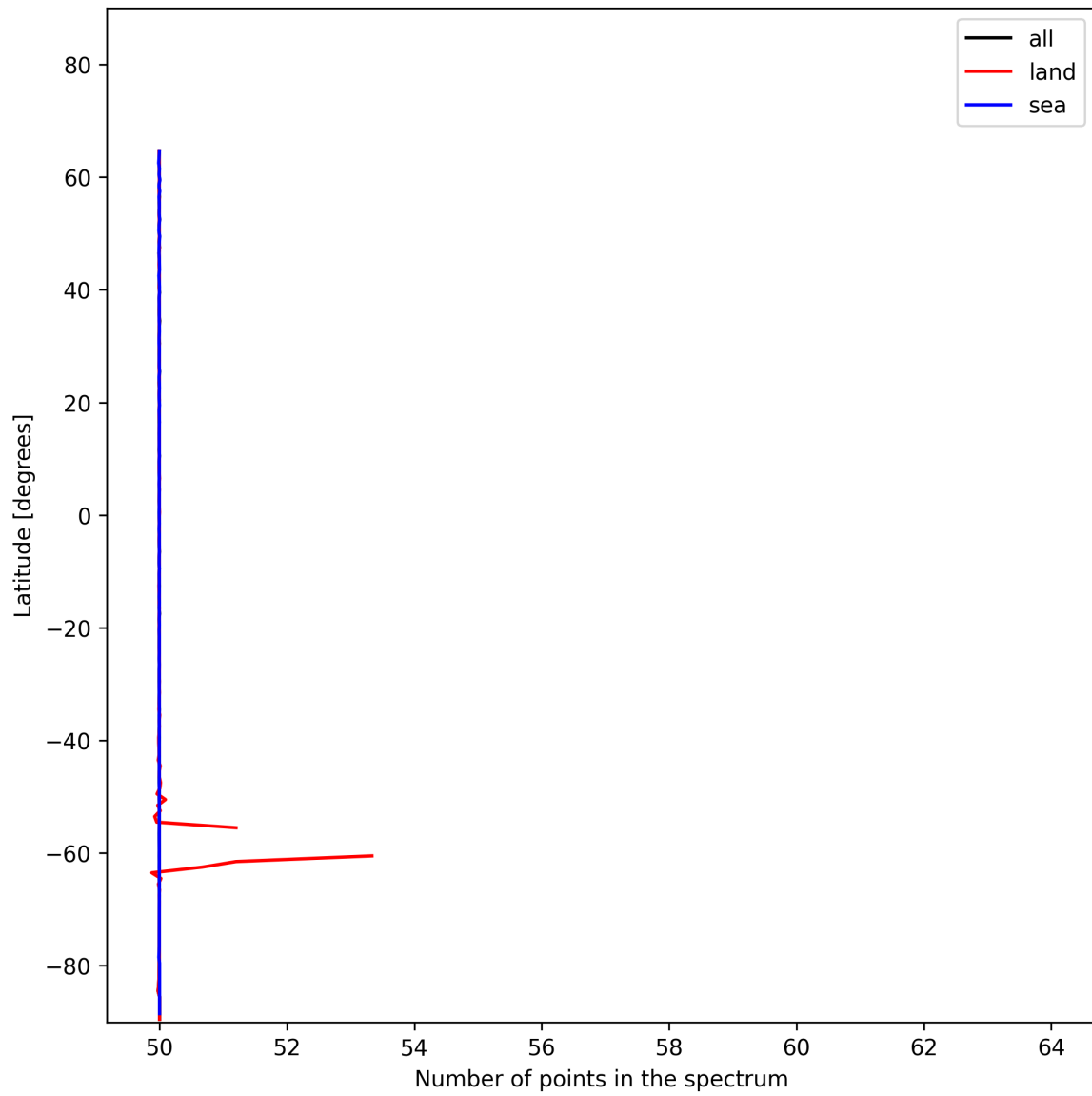
Figure 27: Zonal average of “Number of points in the spectrum” for 2024-12-14 to 2024-12-16.
