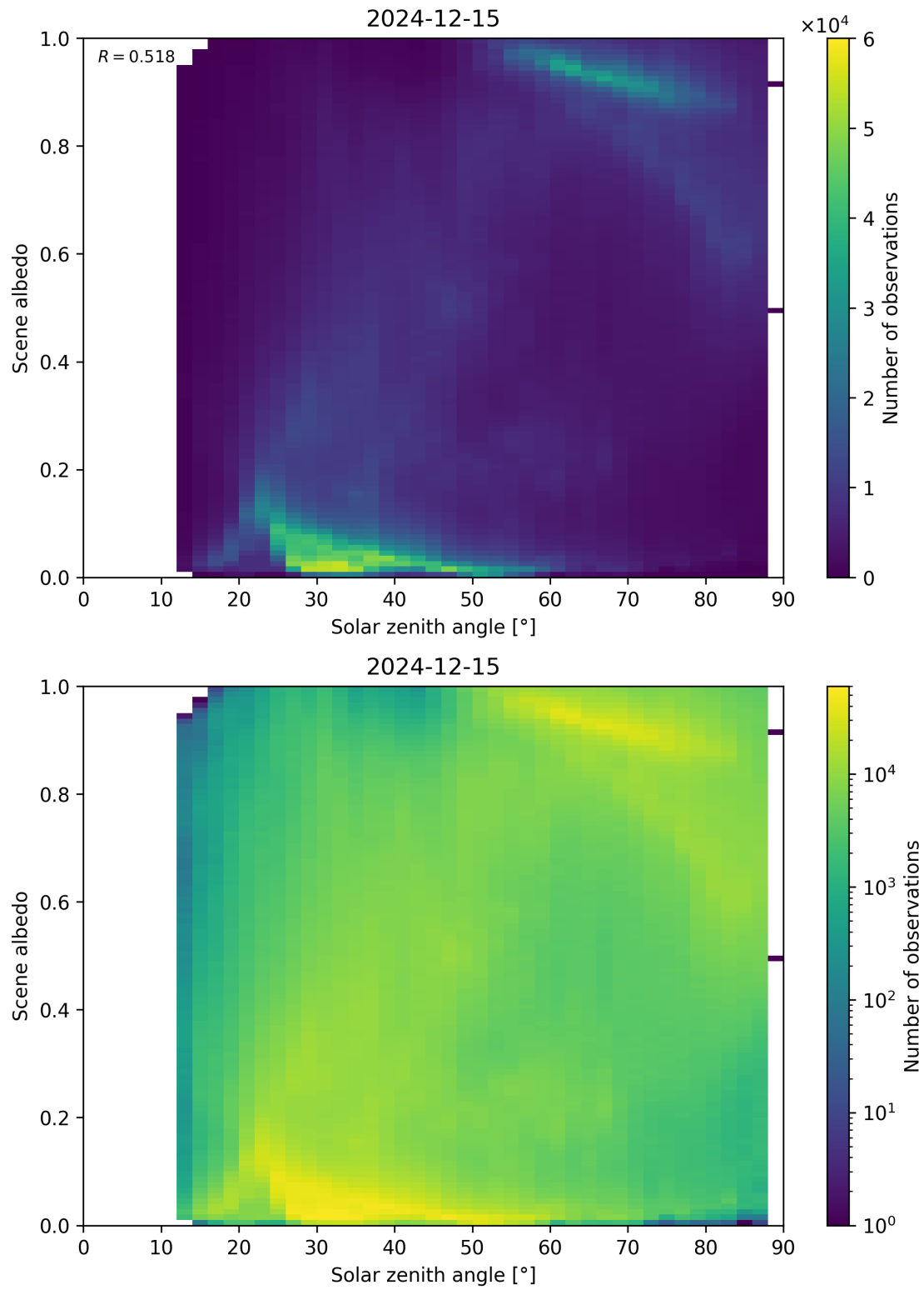
Figure 116: Scatter density plot of “Solar zenith angle” against “Scene albedo” for 2024-12-14 to 2024-12-16.
