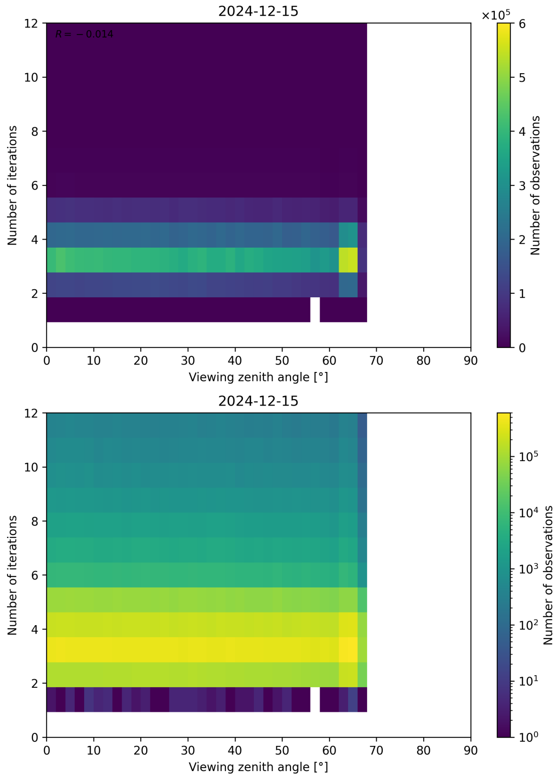
Figure 124: Scatter density plot of “Viewing zenith angle” against “Number of iterations” for 2024-12-14 to 2024-12-16.
