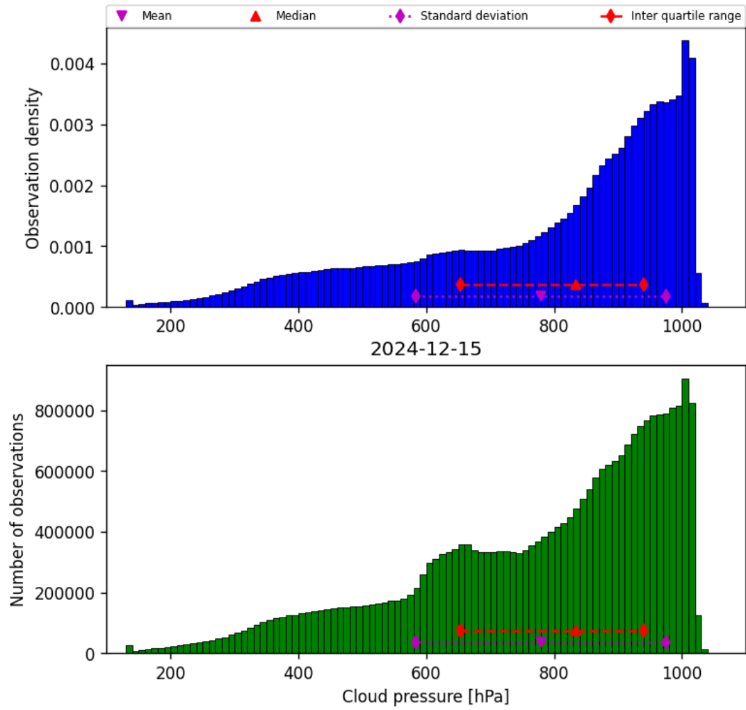
Figure 30: Histogram of “Cloud pressure” for 2024-12-14 to 2024-12-16
