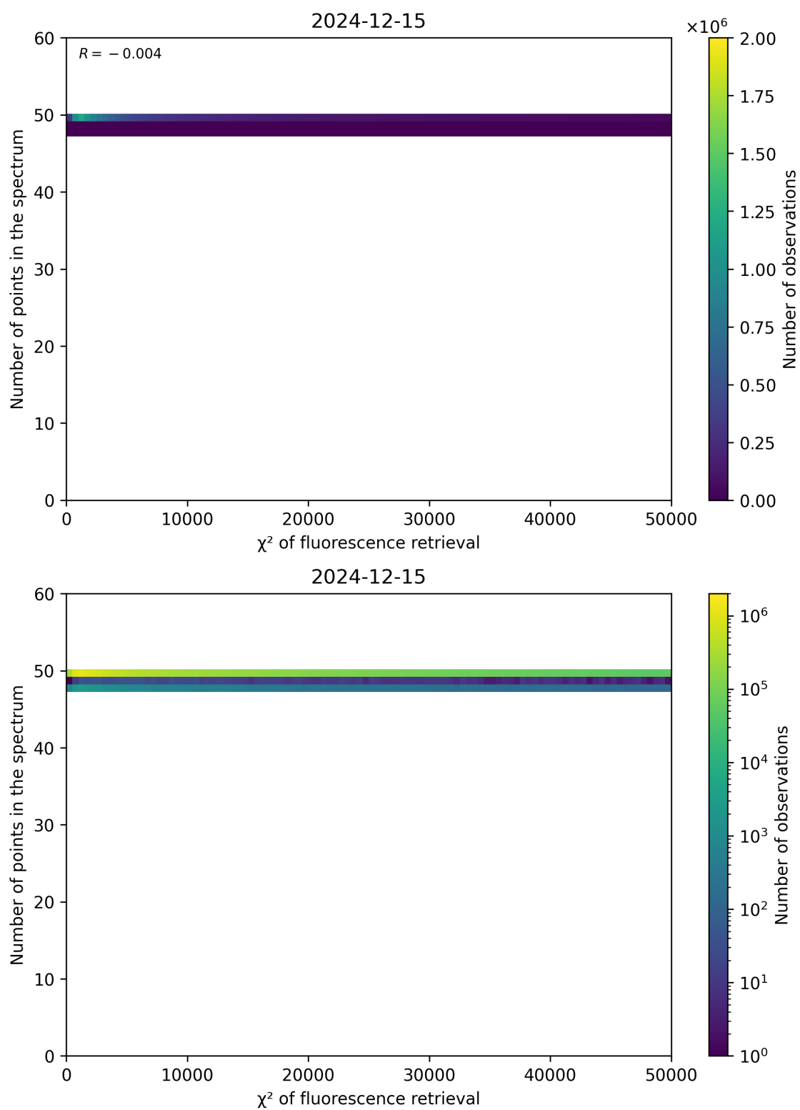
Figure 68: Scatter density plot of “ \chi^2 of fluorescence retrieval” against “Number of points in the spectrum” for 2024-12-14 to 2024-12-16.
