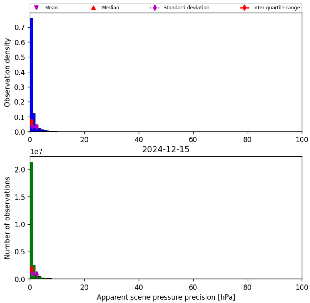
Figure 37: Histogram of “Apparent scene pressure precision” for 2024-12-14 to 2024-12-16
