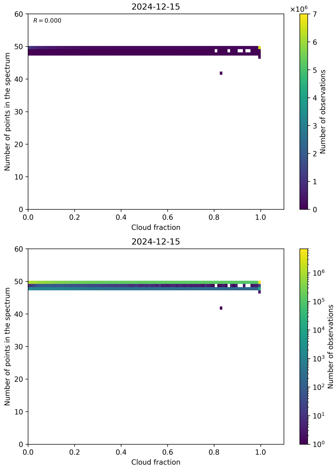
Figure 74: Scatter density plot of “Cloud fraction” against “Number of points in the spectrum” for 2024-12-14 to 2024-12-16.
