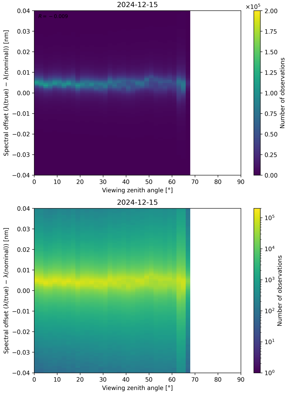
Figure 128: Scatter density plot of “Viewing zenith angle” against “Spectral offset ( \lambda_{\text{true}} - \lambda_{\text{nominal}} )” for 2024-12-14 to 2024-12-16.
