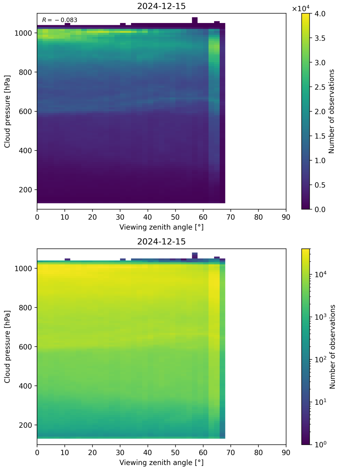
Figure 121: Scatter density plot of “Viewing zenith angle” against “Cloud pressure” for 2024-12-14 to 2024-12-16.
