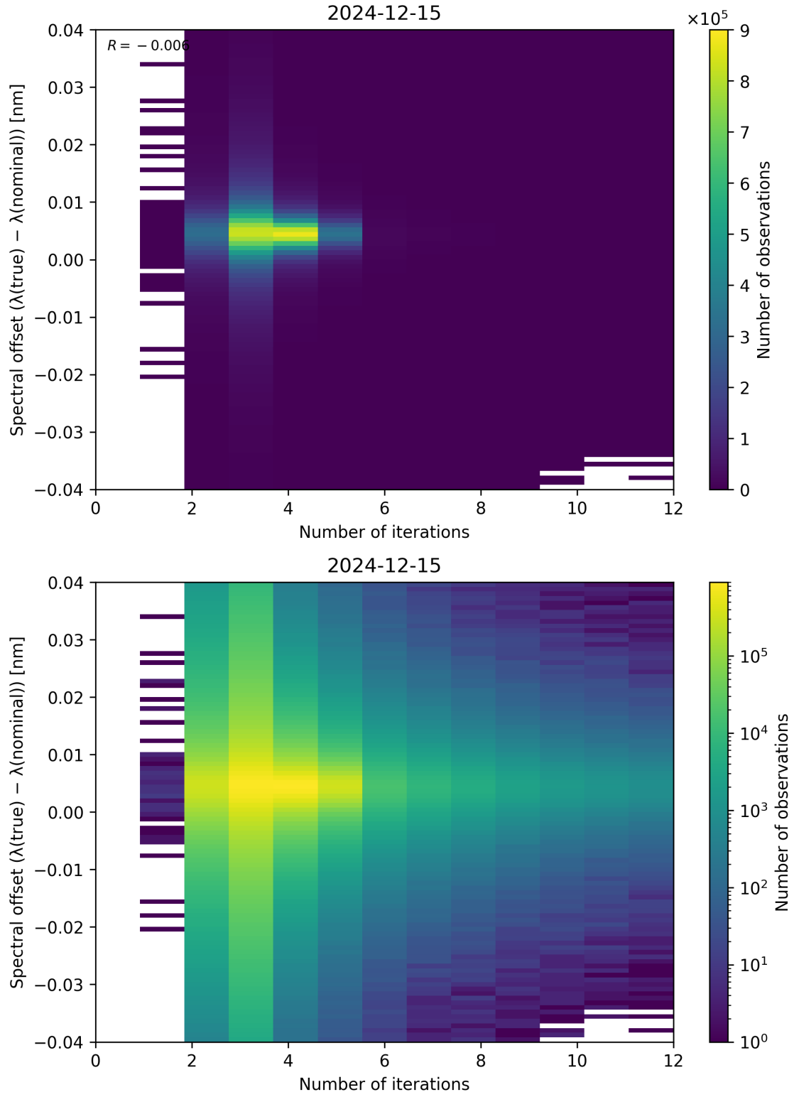
Figure 100: Scatter density plot of “Number of iterations” against “Spectral offset ( \lambda_{\text{true}} - \lambda_{\text{nominal}} )” for 2024-12-14 to 2024-12-16.
