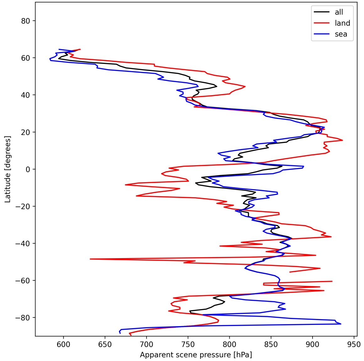
Figure 19: Zonal average of “Apparent scene pressure” for 2024-12-14 to 2024-12-16.
