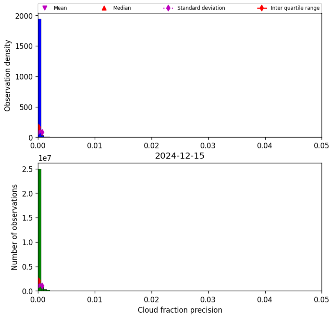
Figure 33: Histogram of “Cloud fraction precision” for 2024-12-14 to 2024-12-16
