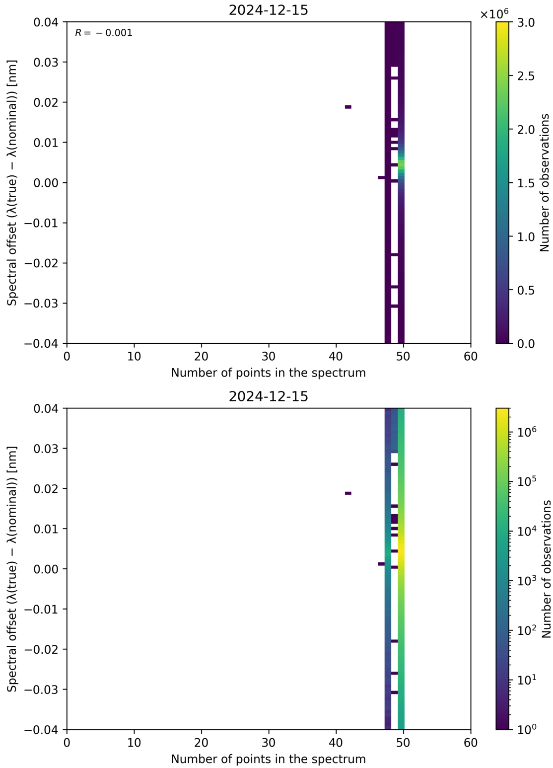
Figure 101: Scatter density plot of “Number of points in the spectrum” against “Spectral offset ( \lambda_{\text{true}} - \lambda_{\text{nominal}} )” for 2024-12-14 to 2024-12-16.
