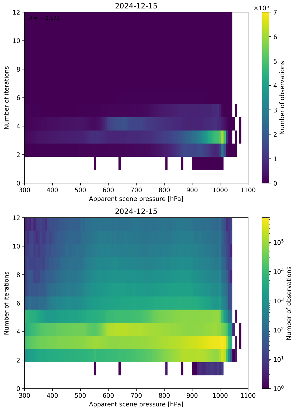
Figure 65: Scatter density plot of “Apparent scene pressure” against “Number of iterations” for 2024-12-14 to 2024-12-16.
