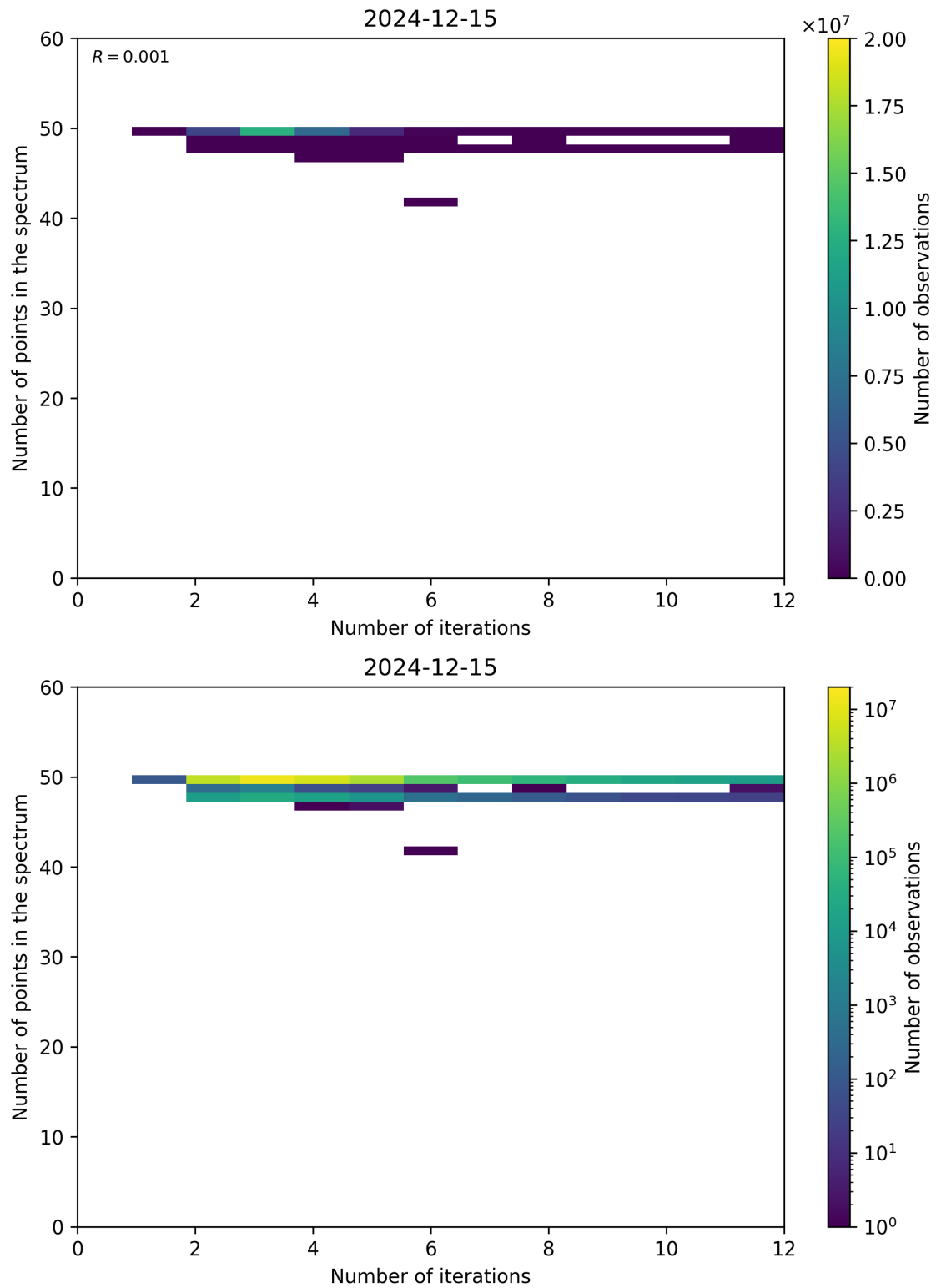
Figure 99: Scatter density plot of “Number of iterations” against “Number of points in the spectrum” for 2024-12-14 to 2024-12-16.
