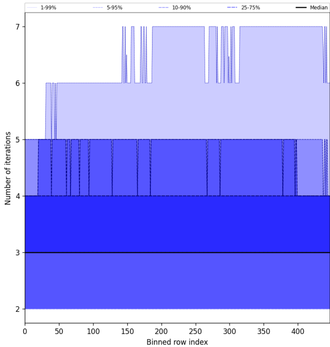
Figure 56: Along track statistics of “Number of iterations” for 2024-12-14 to 2024-12-16
