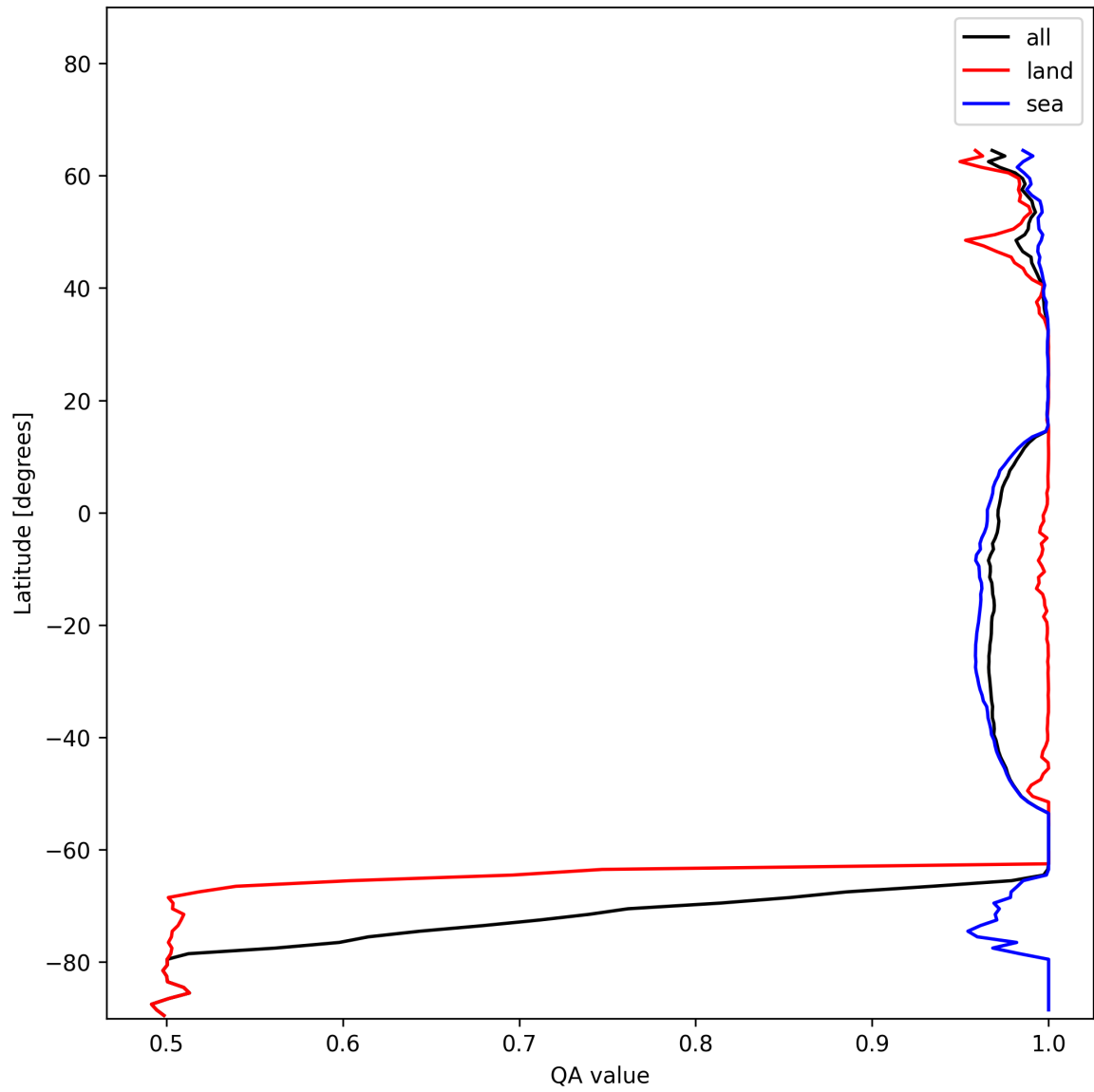
Figure 12: Zonal average of “QA value” for 2024-12-14 to 2024-12-16.
