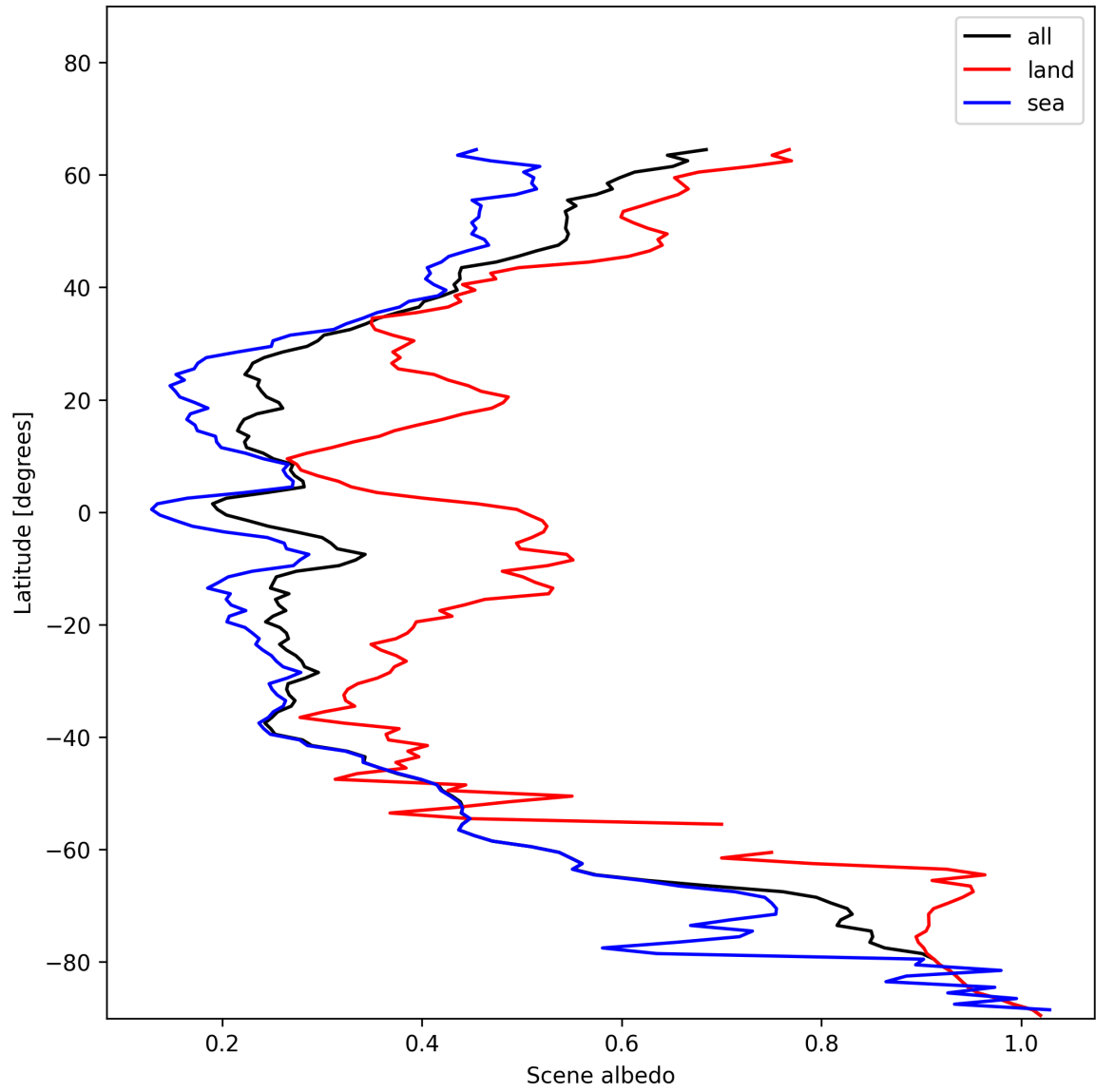
Figure 17: Zonal average of “Scene albedo” for 2024-12-14 to 2024-12-16.
