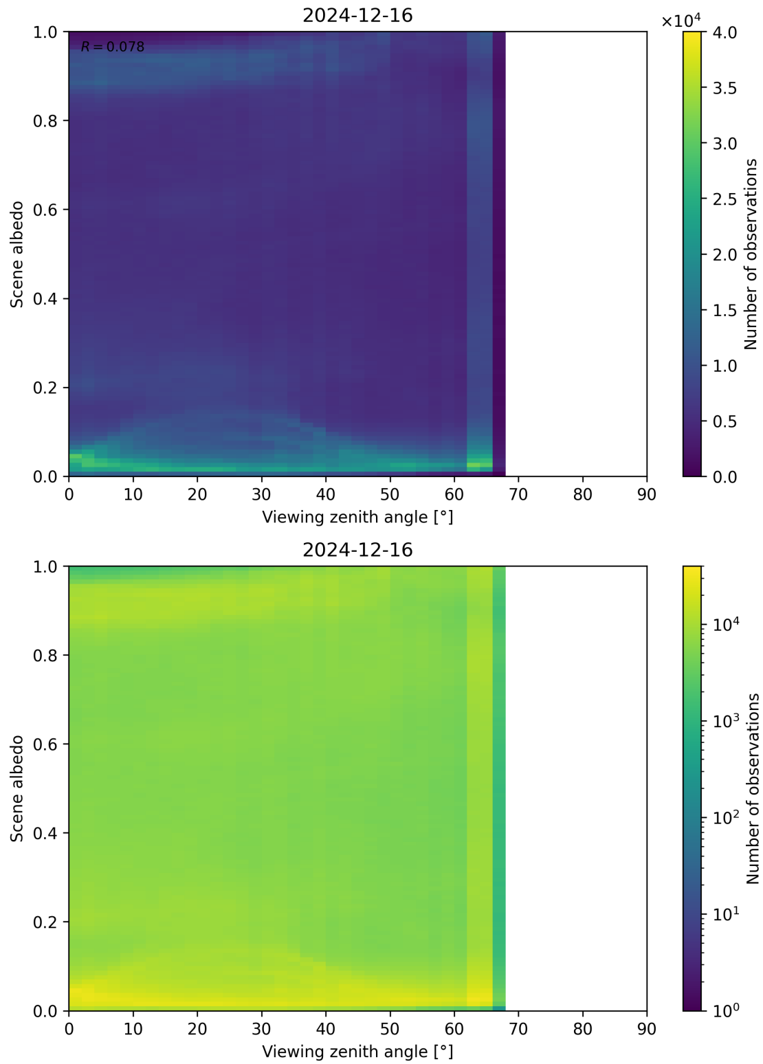
Figure 126: Scatter density plot of “Viewing zenith angle” against “Scene albedo” for 2024-12-16 to 2024-12-17.
