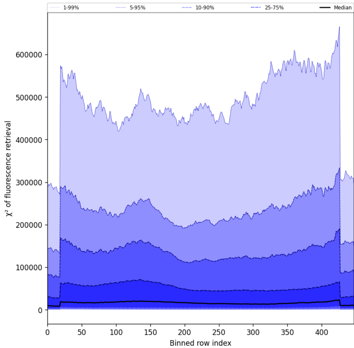
Figure 59: Along track statistics of “ \chi^2 of fluorescence retrieval” for 2024-12-16 to 2024-12-17
