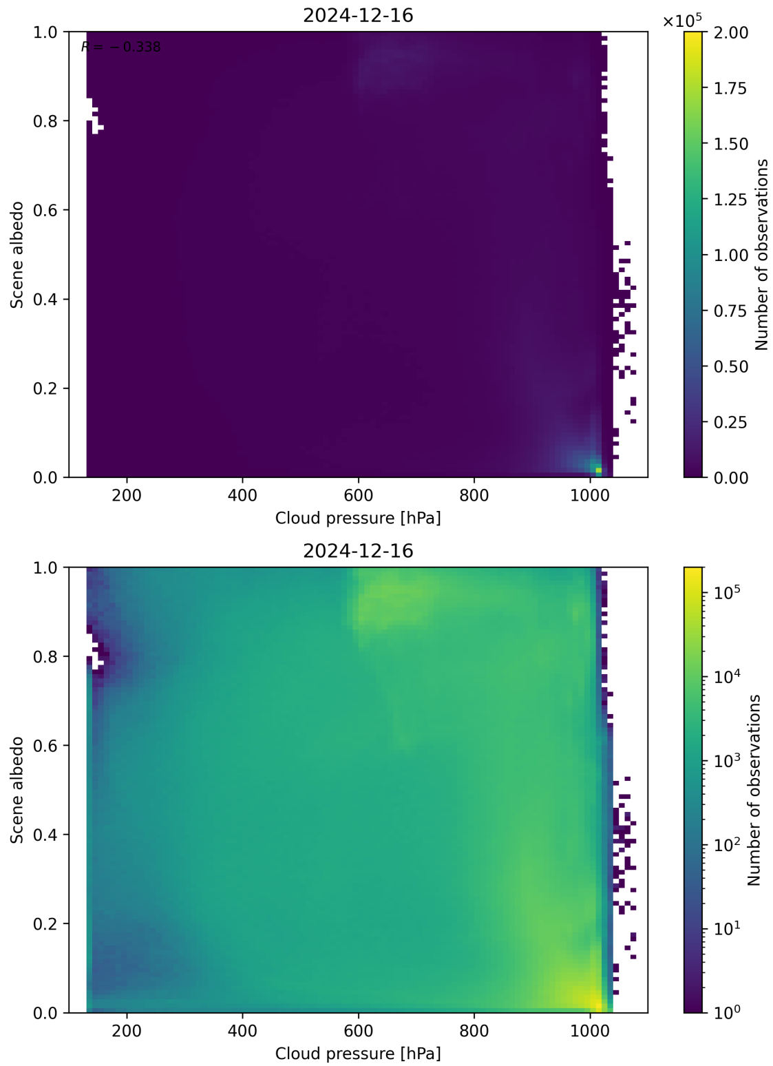
Figure 83: Scatter density plot of “Cloud pressure” against “Scene albedo” for 2024-12-16 to 2024-12-17.
