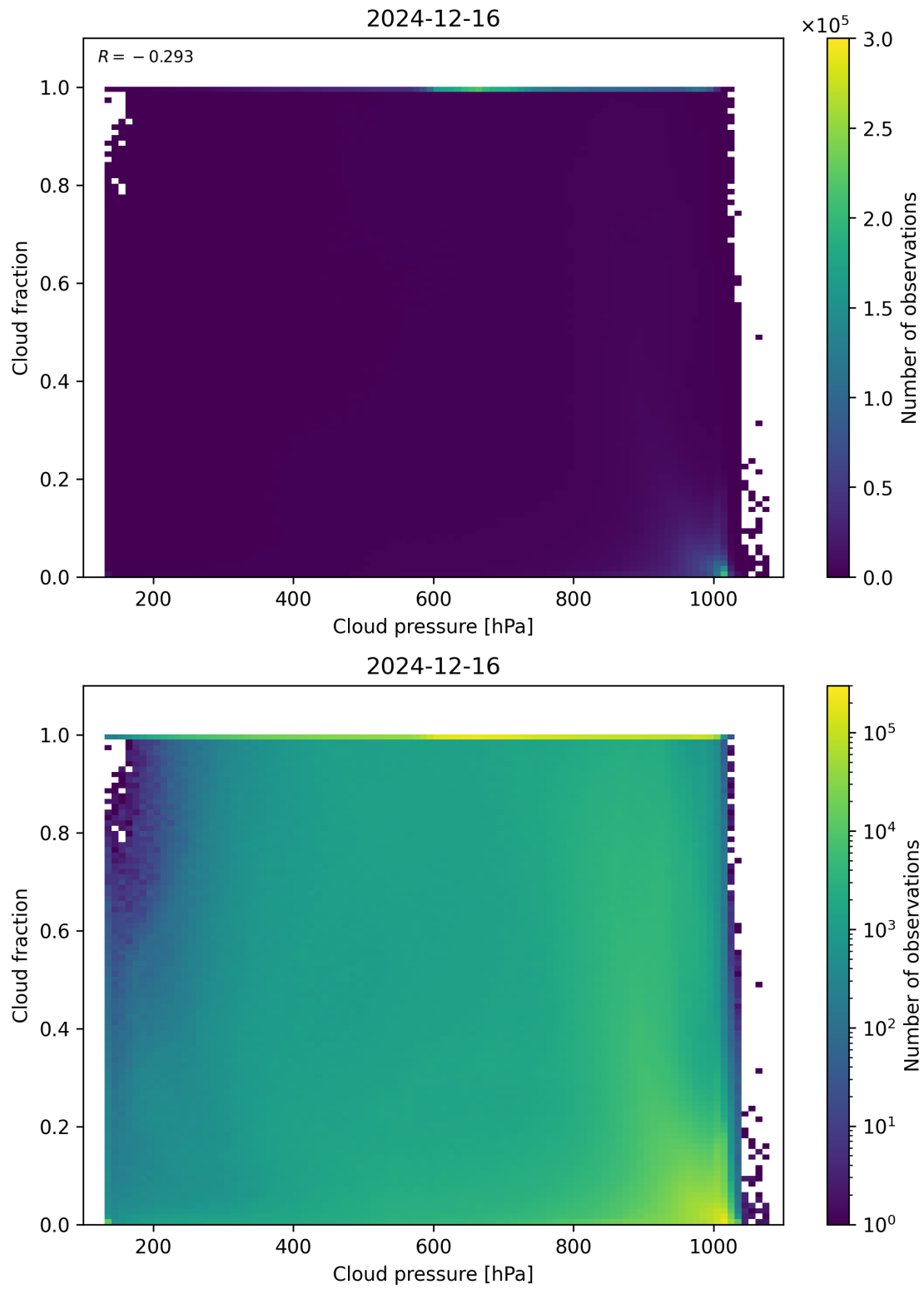
Figure 79: Scatter density plot of “Cloud pressure” against “Cloud fraction” for 2024-12-16 to 2024-12-17.
