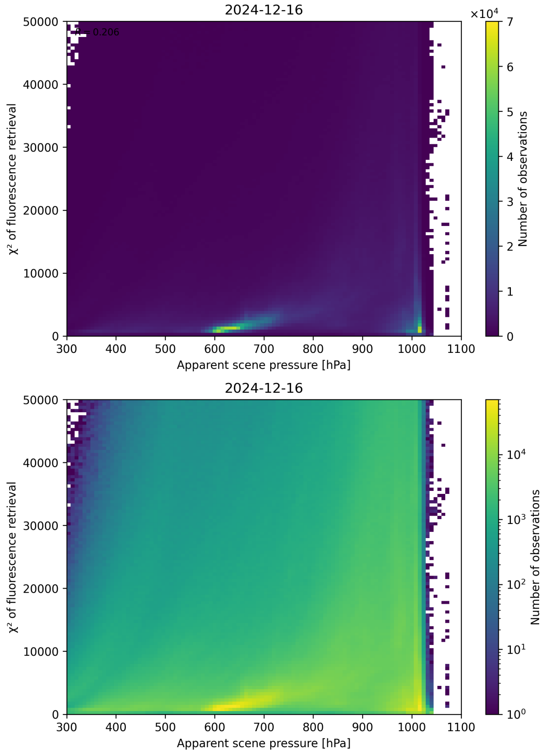
Figure 63: Scatter density plot of “Apparent scene pressure” against “ \chi^2 of fluorescence retrieval” for 2024-12-16 to 2024-12-17.
