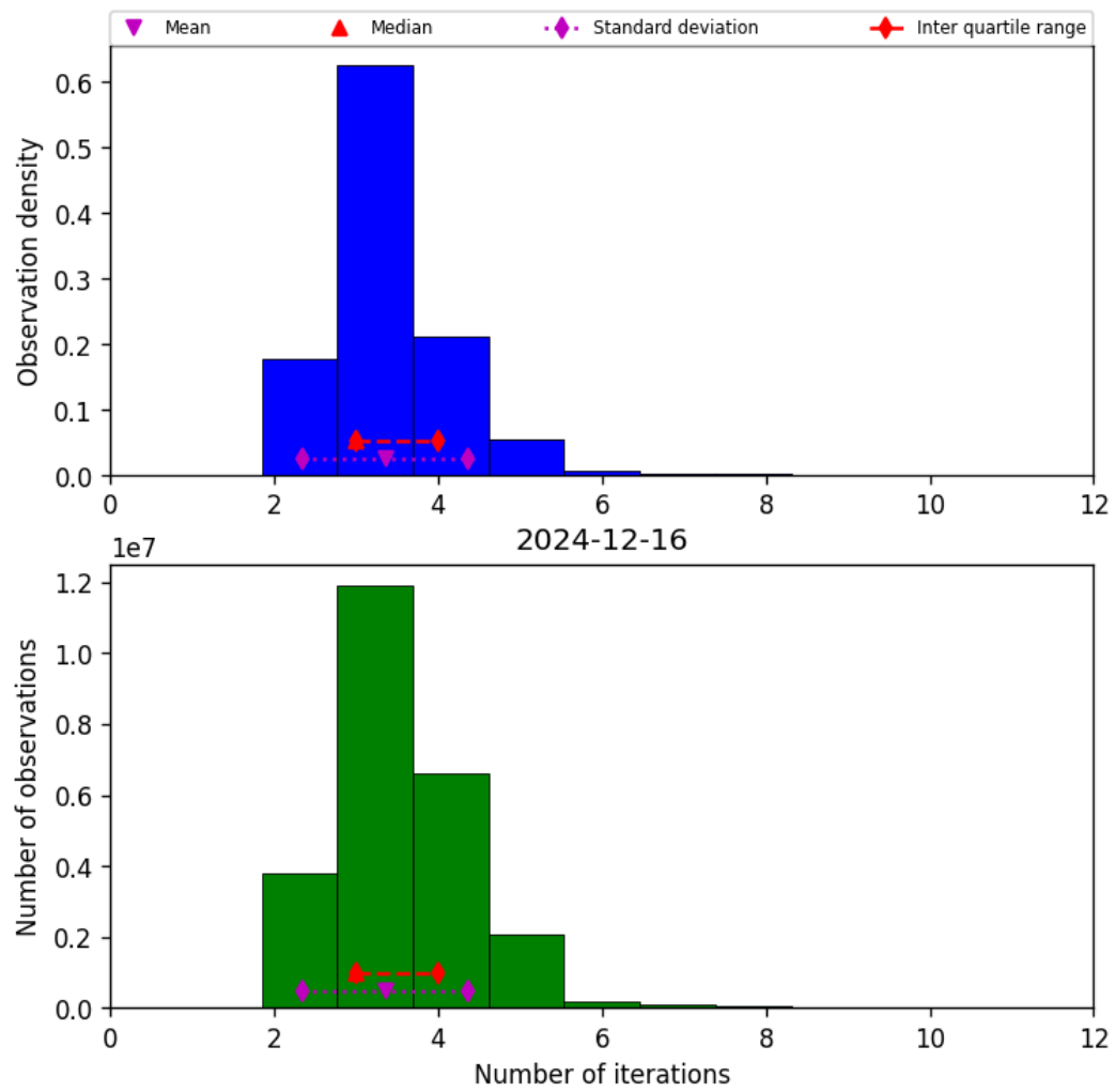
Figure 39: Histogram of “Number of iterations” for 2024-12-16 to 2024-12-17
