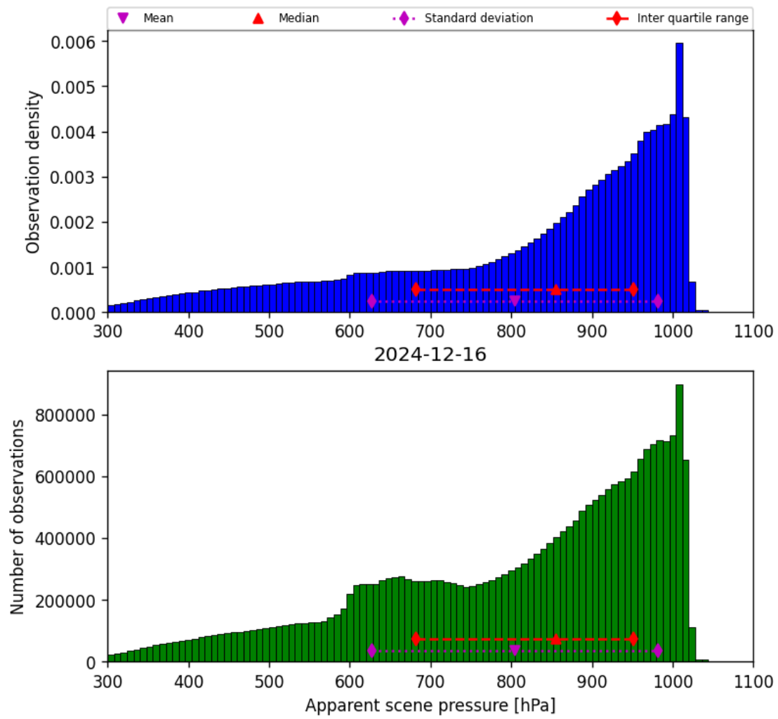
Figure 36: Histogram of “Apparent scene pressure” for 2024-12-16 to 2024-12-17
