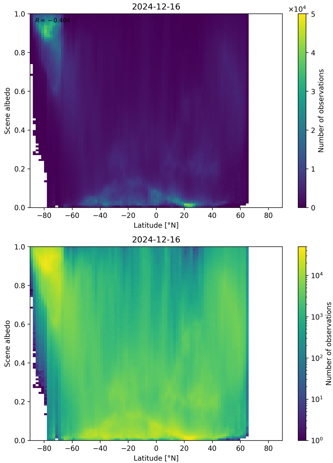
Figure 95: Scatter density plot of “Latitude” against “Scene albedo” for 2024-12-16 to 2024-12-17.
