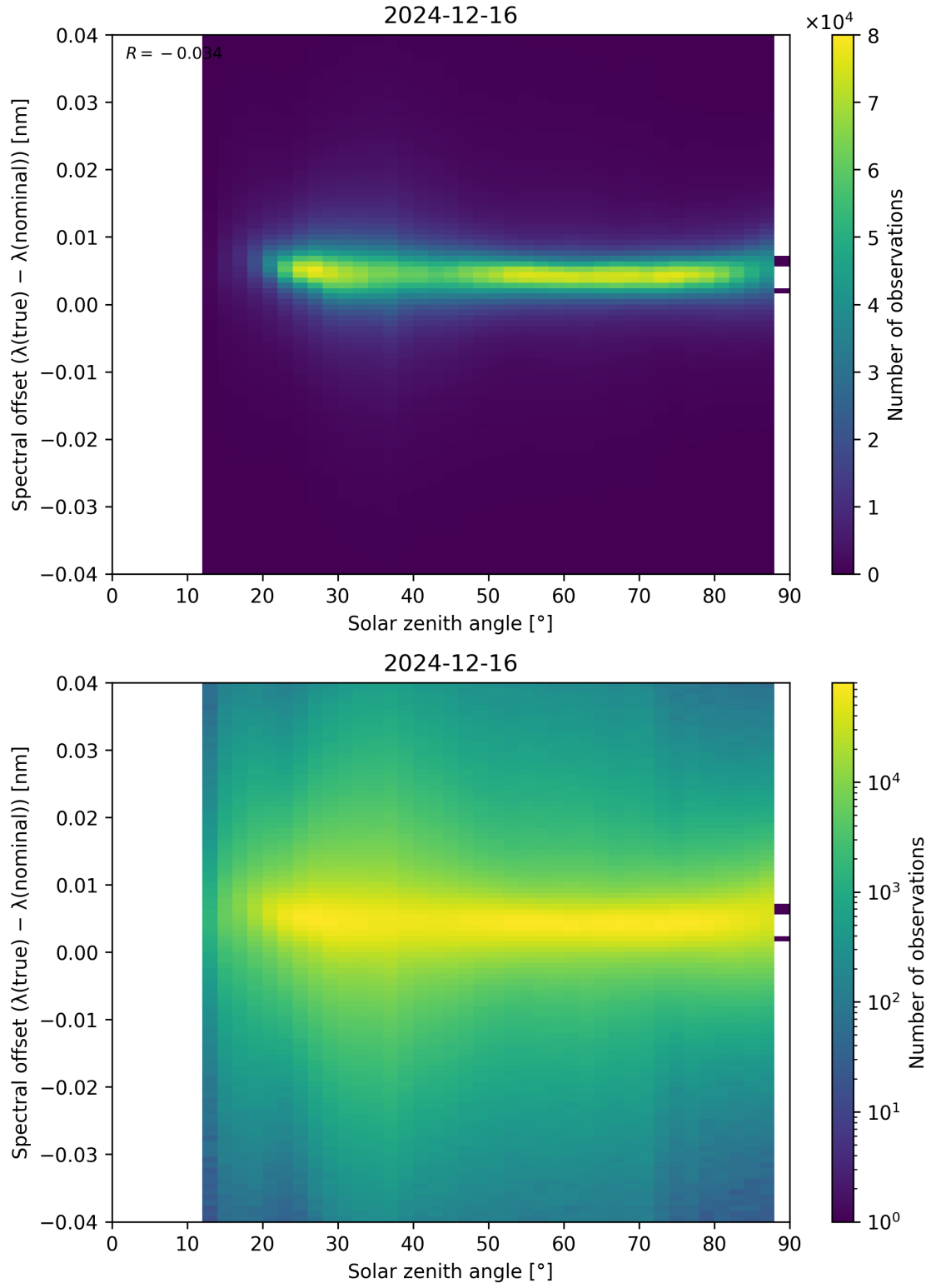
Figure 117: Scatter density plot of “Solar zenith angle” against “Spectral offset ( \lambda_{\text{true}} - \lambda_{\text{nominal}} )” for 2024-12-16 to 2024-12-17.
