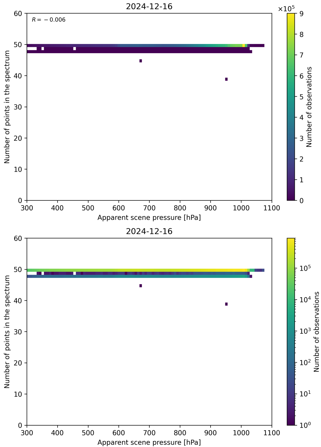
Figure 66: Scatter density plot of “Apparent scene pressure” against “Number of points in the spectrum” for 2024-12-16 to 2024-12-17.
