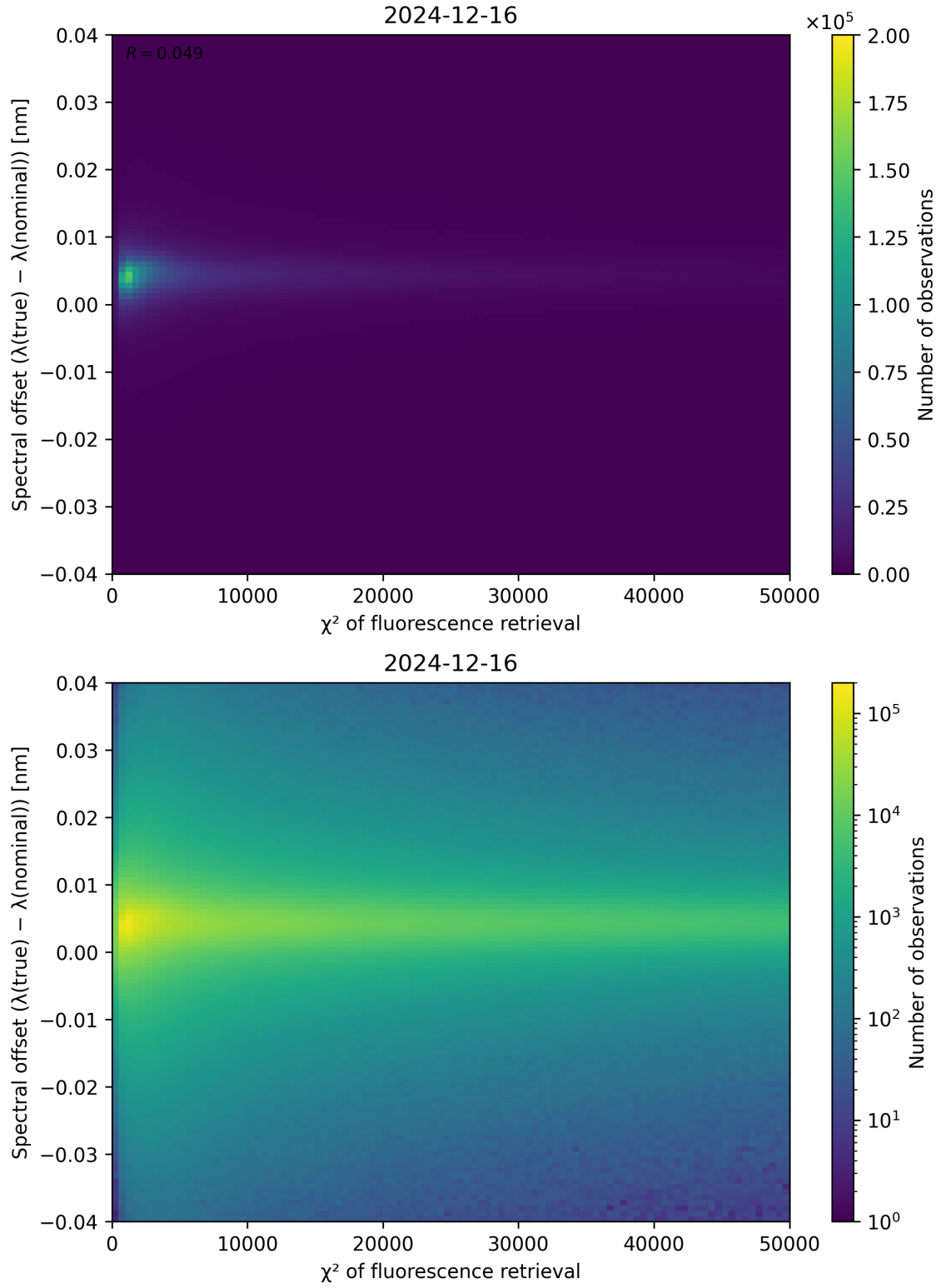
Figure 69: Scatter density plot of “ \chi^2 of fluorescence retrieval” against “Spectral offset ( \lambda_{\text{true}} - \lambda_{\text{nominal}} )” for 2024-12-16 to 2024-12-17.
