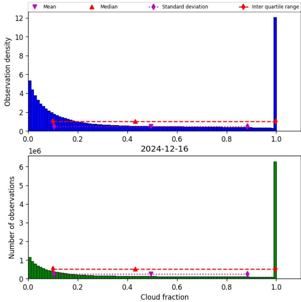
Figure 32: Histogram of “Cloud fraction” for 2024-12-16 to 2024-12-17
