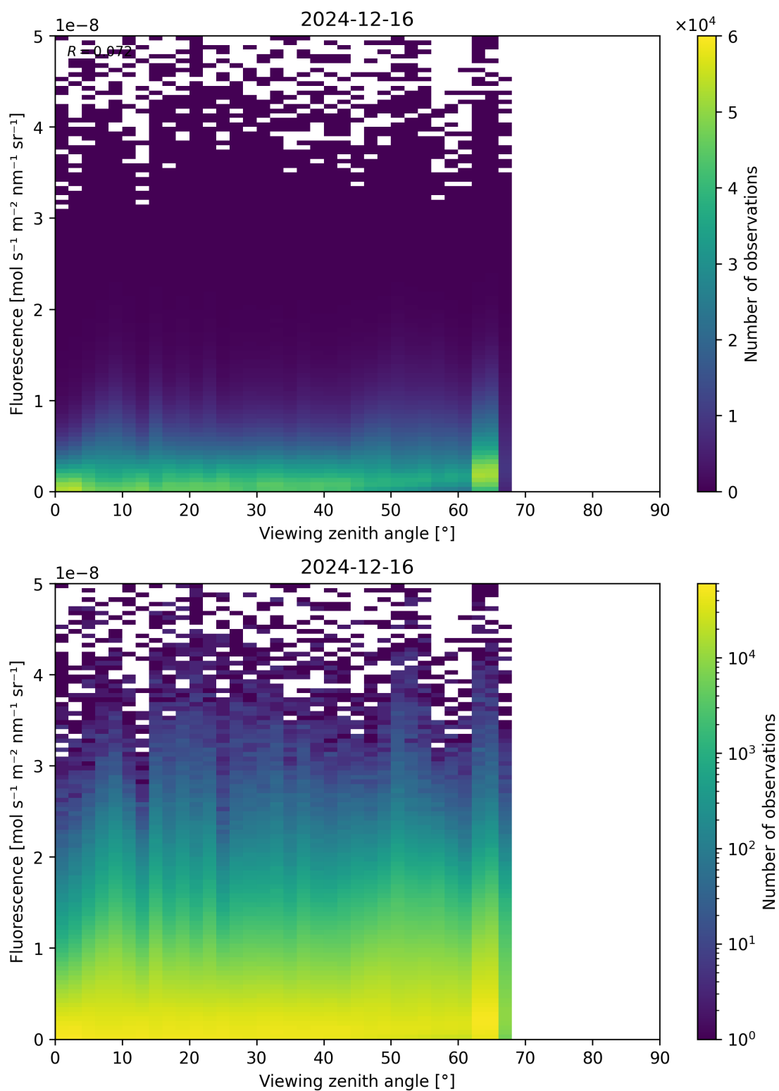
Figure 122: Scatter density plot of “Viewing zenith angle” against “Fluorescence” for 2024-12-16 to 2024-12-17.
