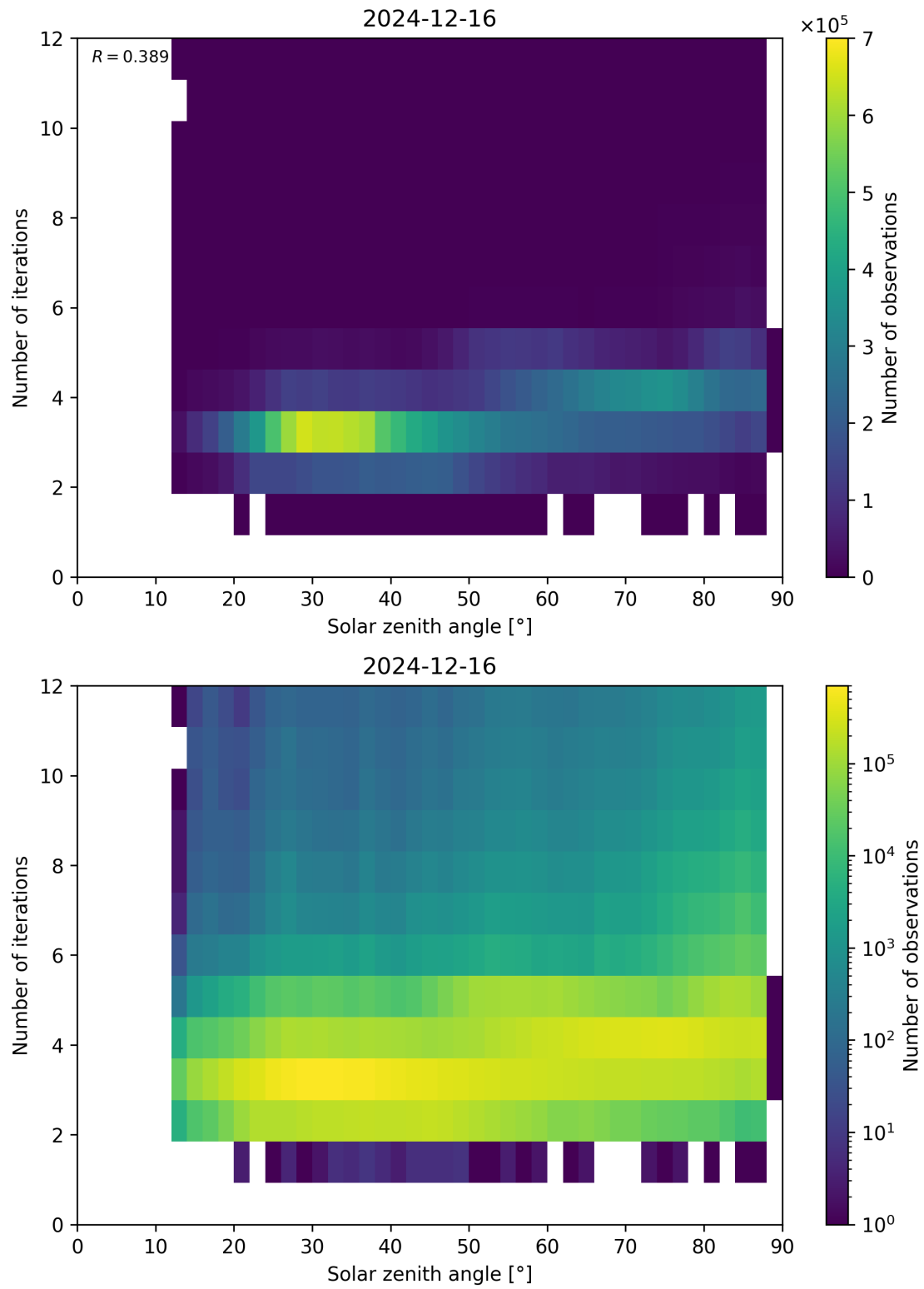
Figure 114: Scatter density plot of “Solar zenith angle” against “Number of iterations” for 2024-12-16 to 2024-12-17.
