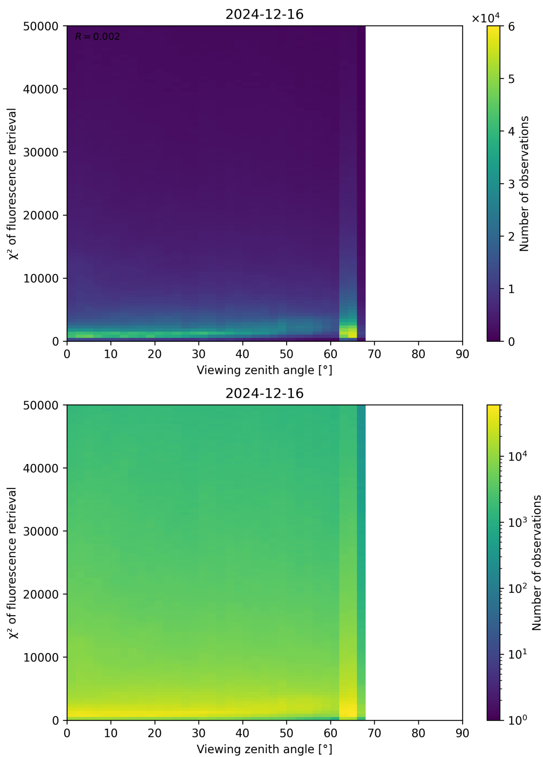
Figure 119: Scatter density plot of “Viewing zenith angle” against “ \chi^2 of fluorescence retrieval” for 2024-12-16 to 2024-12-17.
