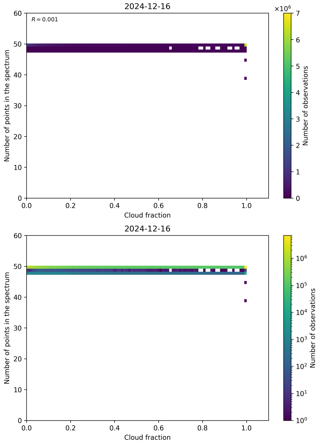
Figure 74: Scatter density plot of “Cloud fraction” against “Number of points in the spectrum” for 2024-12-16 to 2024-12-17.
