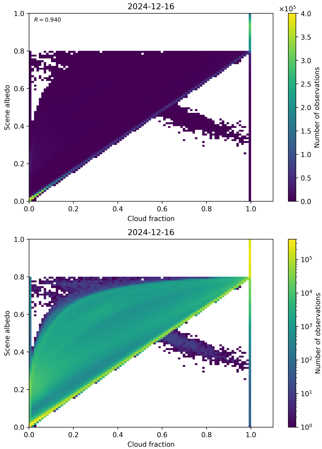
Figure 75: Scatter density plot of “Cloud fraction” against “Scene albedo” for 2024-12-16 to 2024-12-17.
