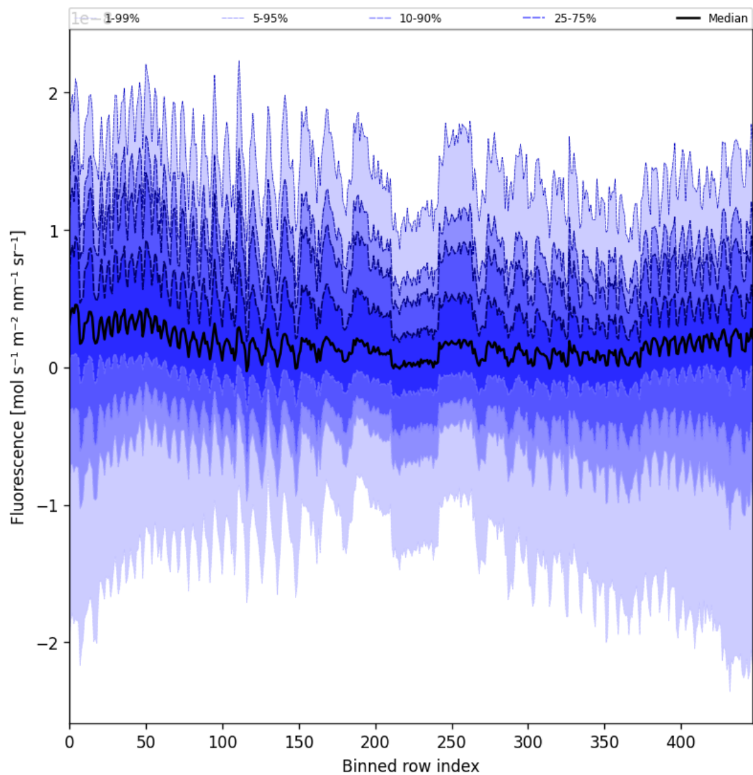
Figure 57: Along track statistics of “Fluorescence” for 2024-12-16 to 2024-12-17
