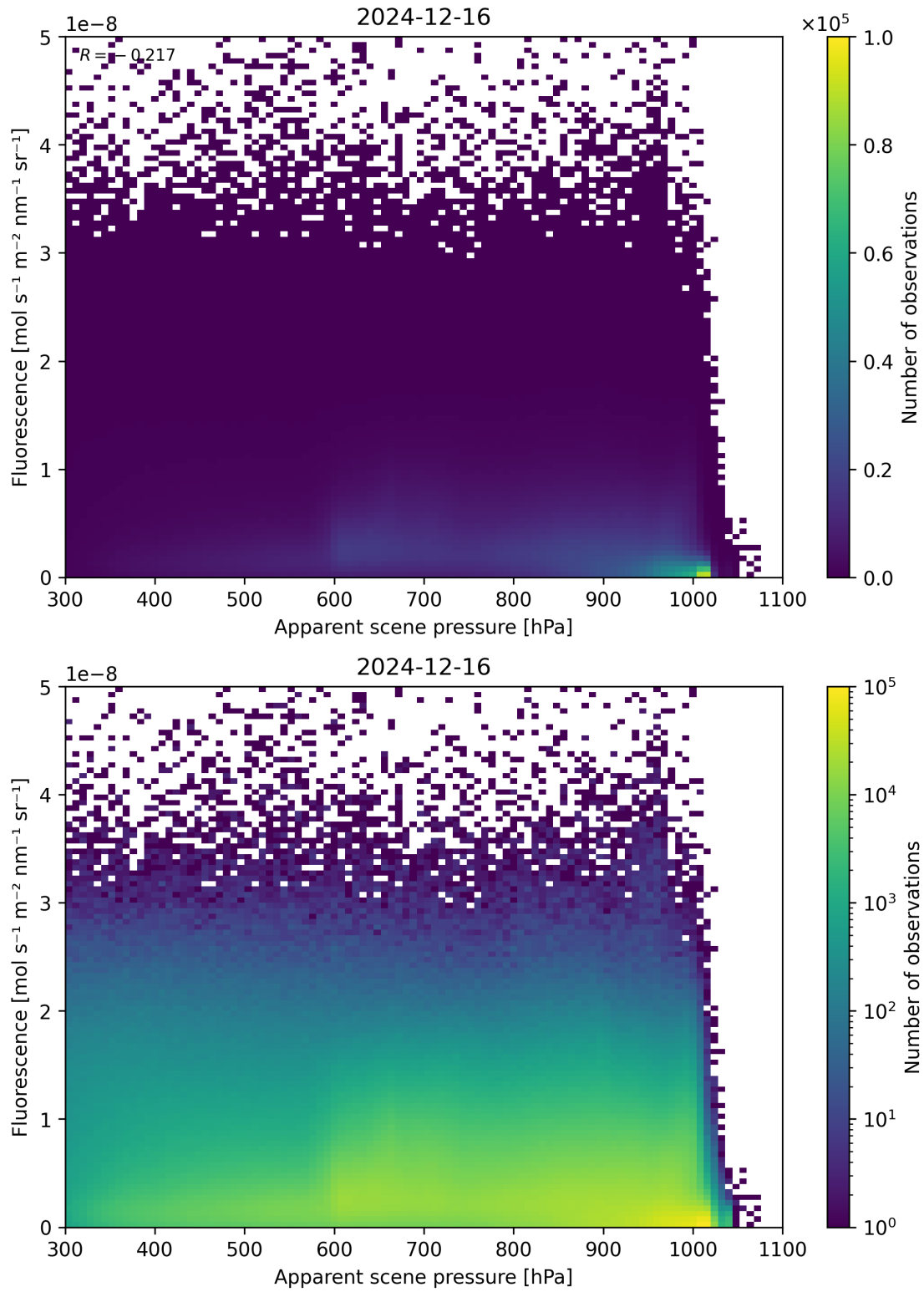
Figure 64: Scatter density plot of “Apparent scene pressure” against “Fluorescence” for 2024-12-16 to 2024-12-17.
