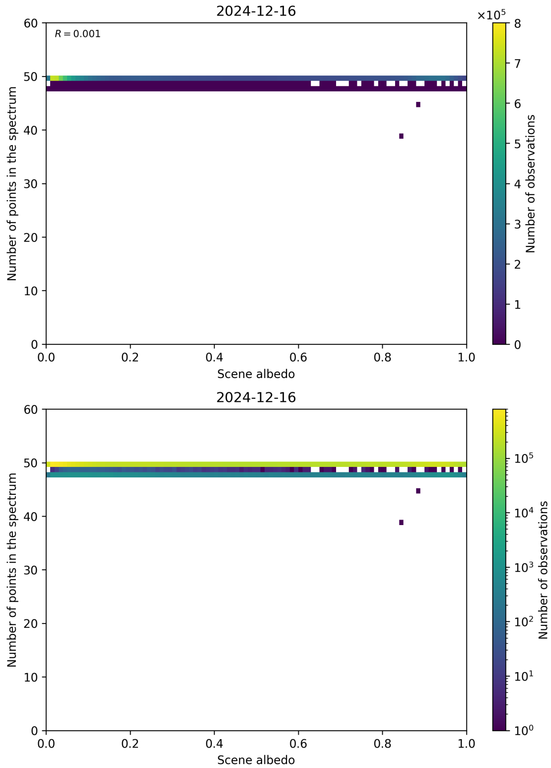
Figure 106: Scatter density plot of “Scene albedo” against “Number of points in the spectrum” for 2024-12-16 to 2024-12-17.
