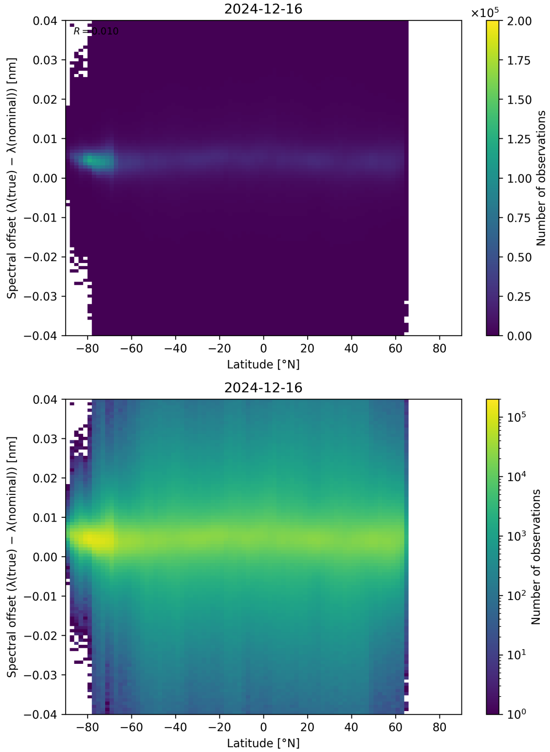
Figure 96: Scatter density plot of “Latitude” against “Spectral offset ( \lambda_{\text{true}} - \lambda_{\text{nominal}} )” for 2024-12-16 to 2024-12-17.
