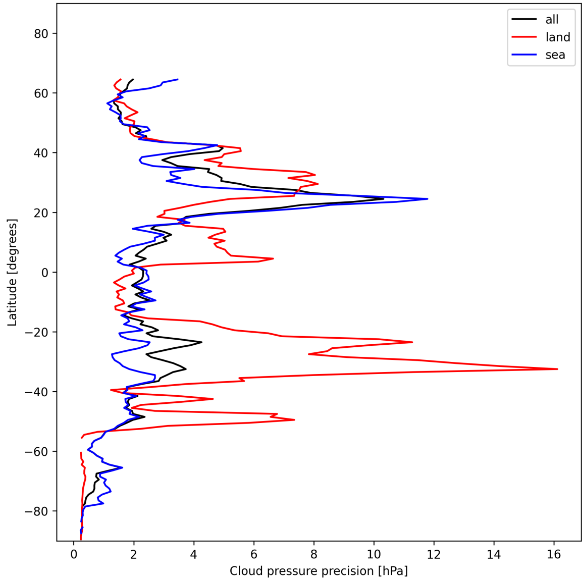
Figure 14: Zonal average of “Cloud pressure precision” for 2024-12-16 to 2024-12-17.
