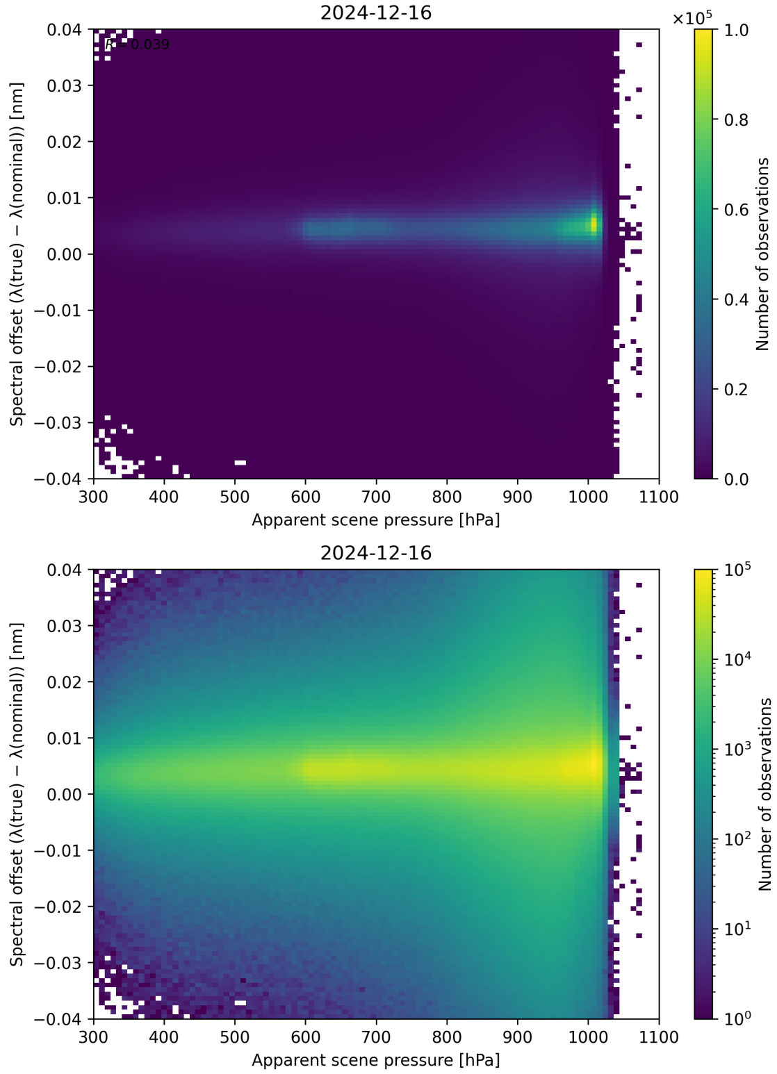
Figure 67: Scatter density plot of “Apparent scene pressure” against “Spectral offset ( \lambda_{\text{true}} - \lambda_{\text{nominal}} )” for 2024-12-16 to 2024-12-17.
