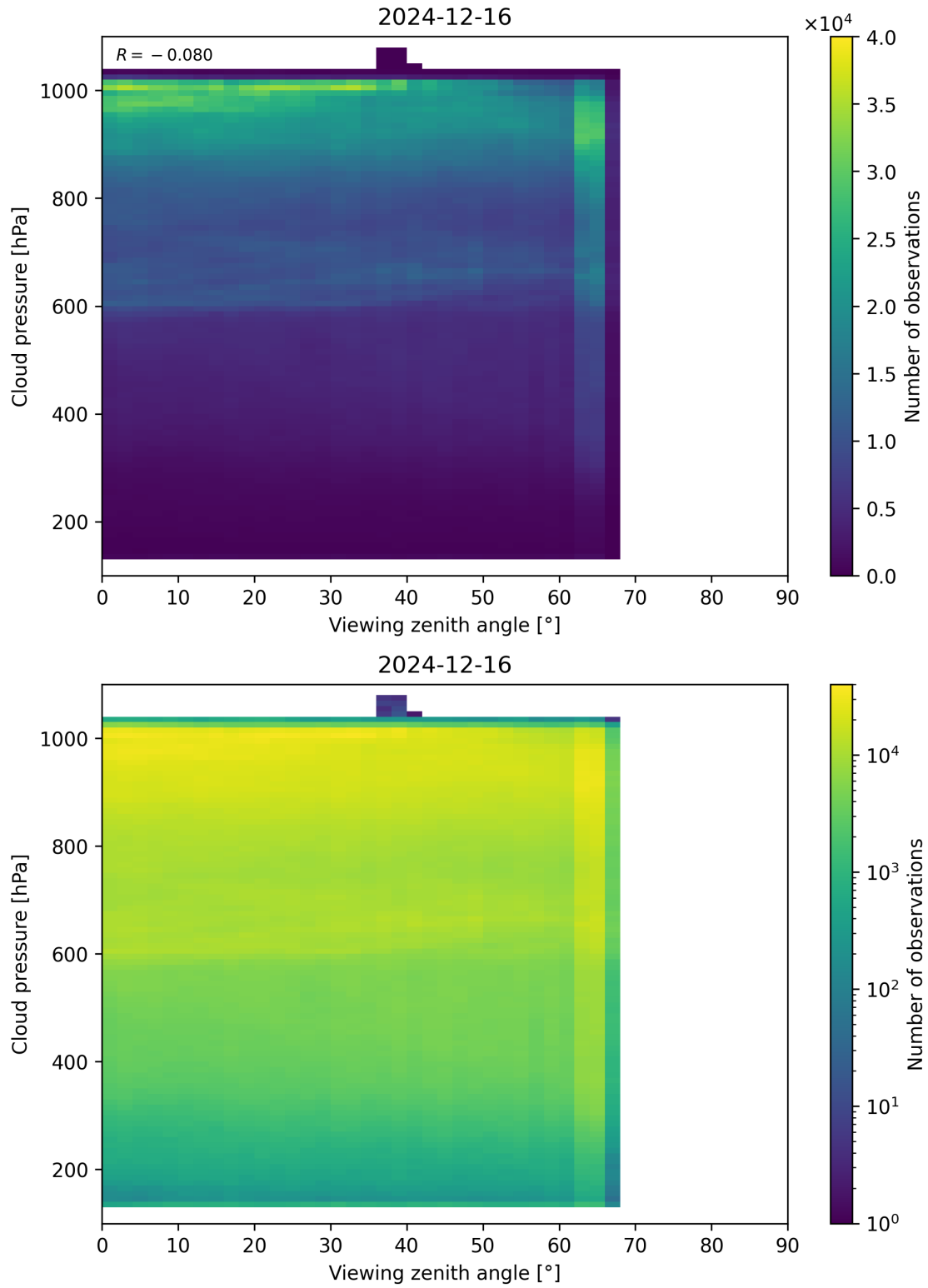
Figure 121: Scatter density plot of “Viewing zenith angle” against “Cloud pressure” for 2024-12-16 to 2024-12-17.
