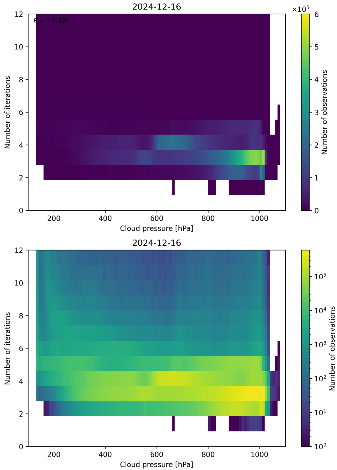
Figure 81: Scatter density plot of “Cloud pressure” against “Number of iterations” for 2024-12-16 to 2024-12-17.
