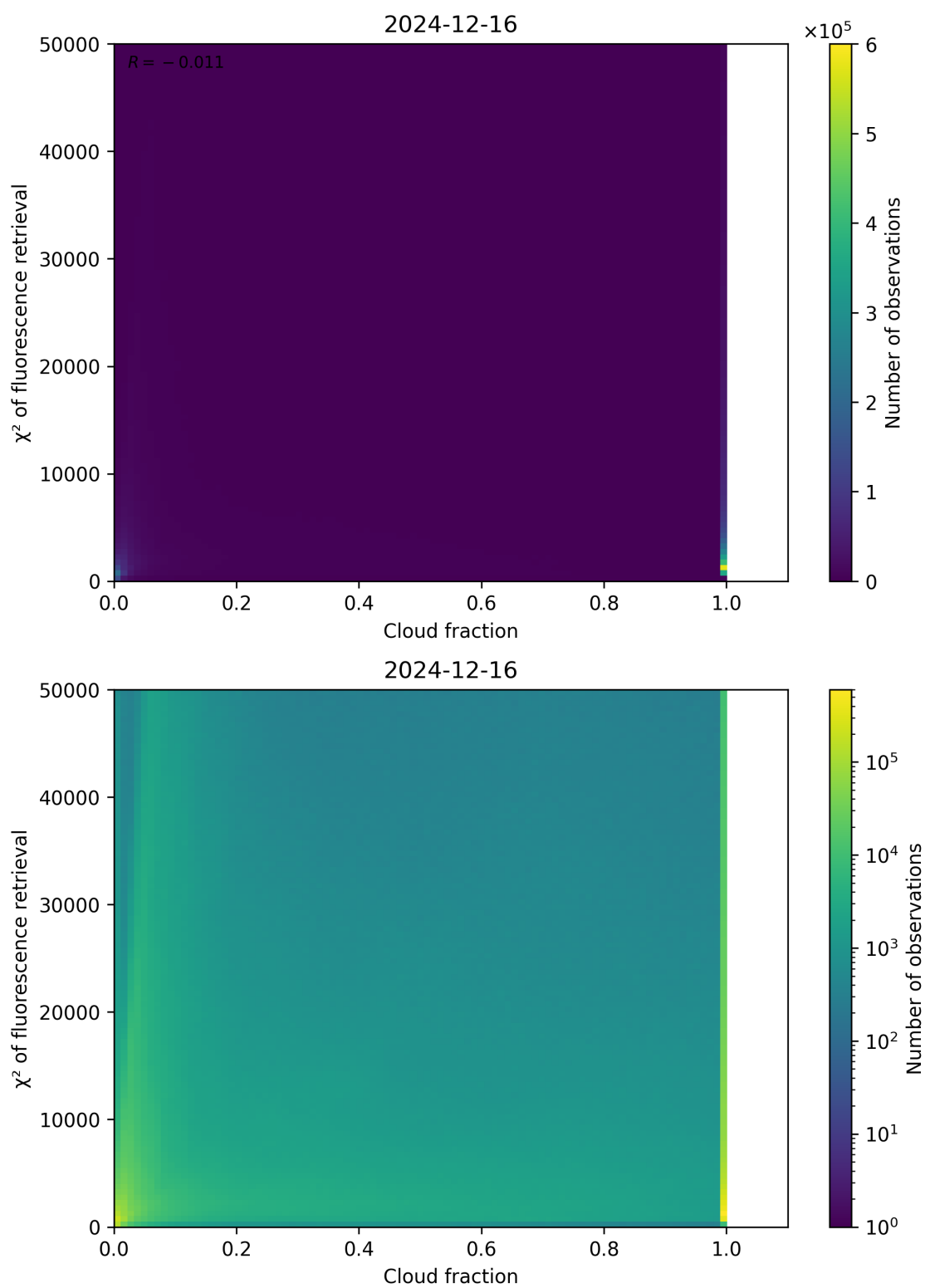
Figure 71: Scatter density plot of “Cloud fraction” against “ \chi^2 of fluorescence retrieval” for 2024-12-16 to 2024-12-17.
