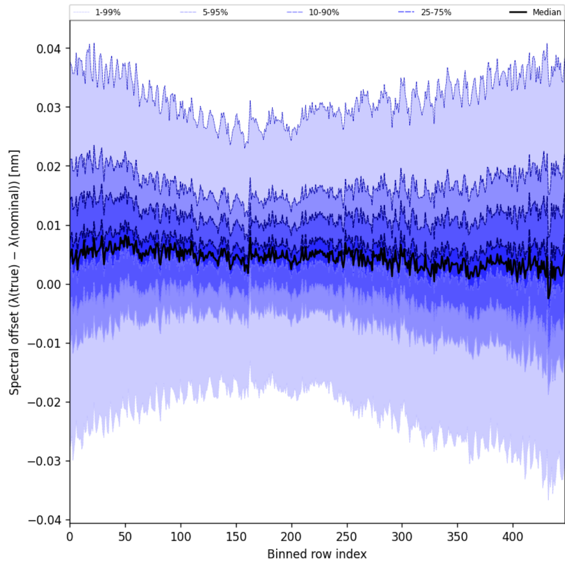
Figure 62: Along track statistics of “Spectral offset ( \lambda_{\text{true}} - \lambda_{\text{nominal}} )” for 2024-12-16 to 2024-12-17
