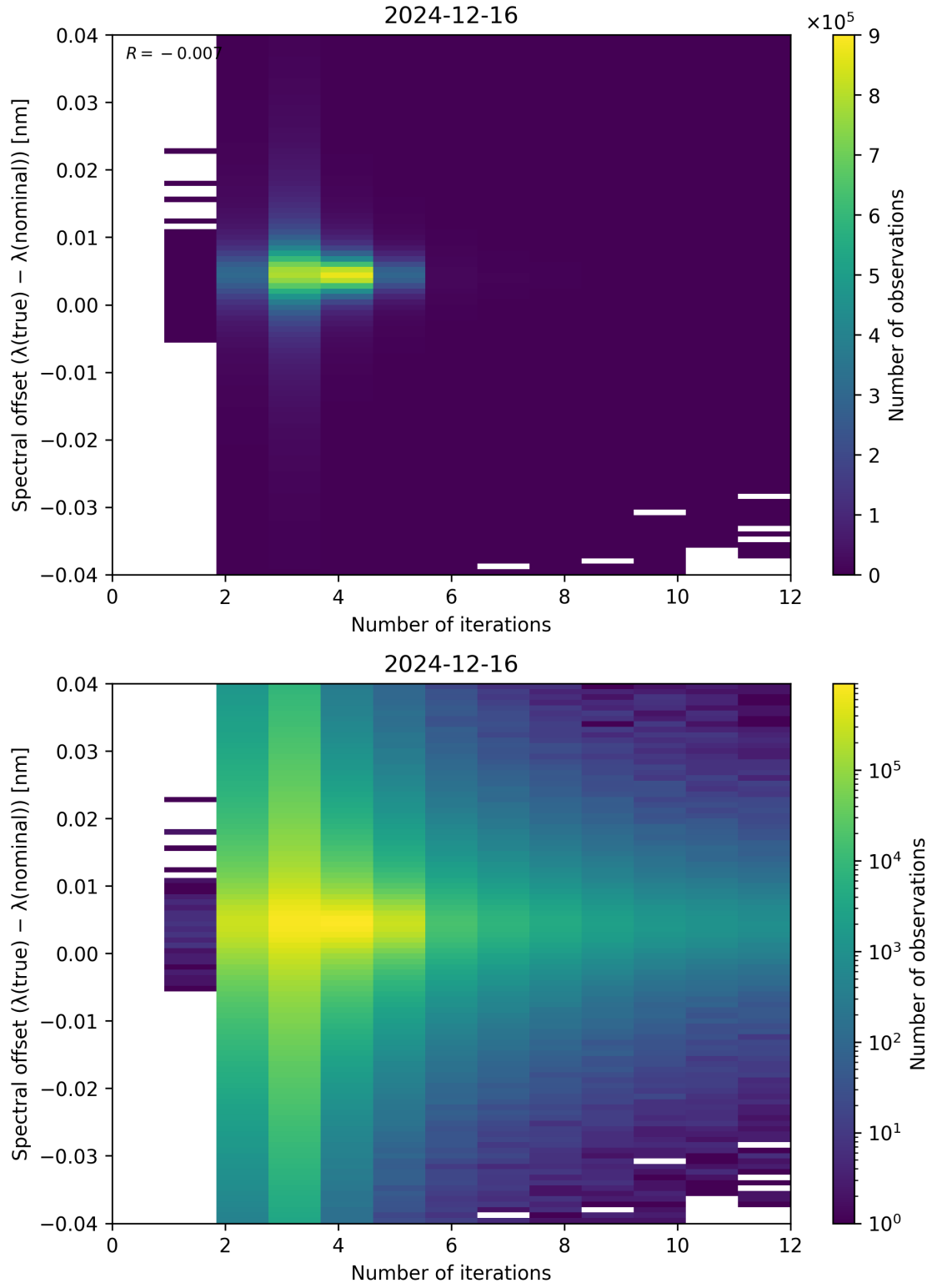
Figure 100: Scatter density plot of “Number of iterations” against “Spectral offset ( \lambda_{\text{true}} - \lambda_{\text{nominal}} )” for 2024-12-16 to 2024-12-17.
