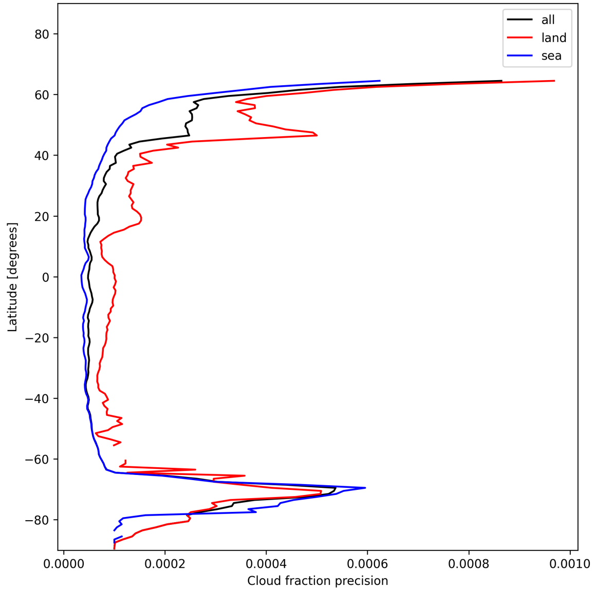
Figure 16: Zonal average of “Cloud fraction precision” for 2024-12-16 to 2024-12-17.
