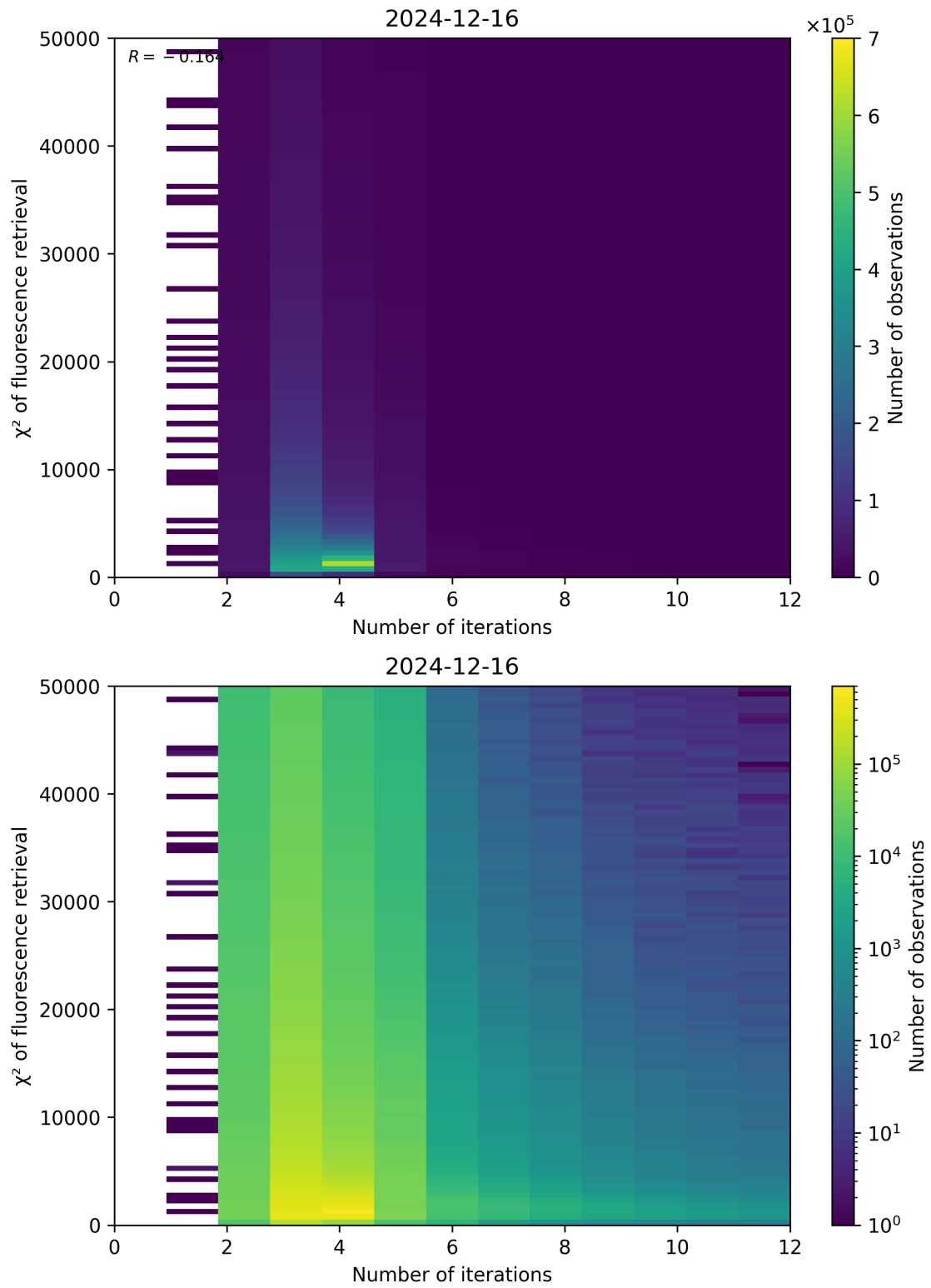
Figure 97: Scatter density plot of “Number of iterations” against “ \chi^2 of fluorescence retrieval” for 2024-12-16 to 2024-12-17.
