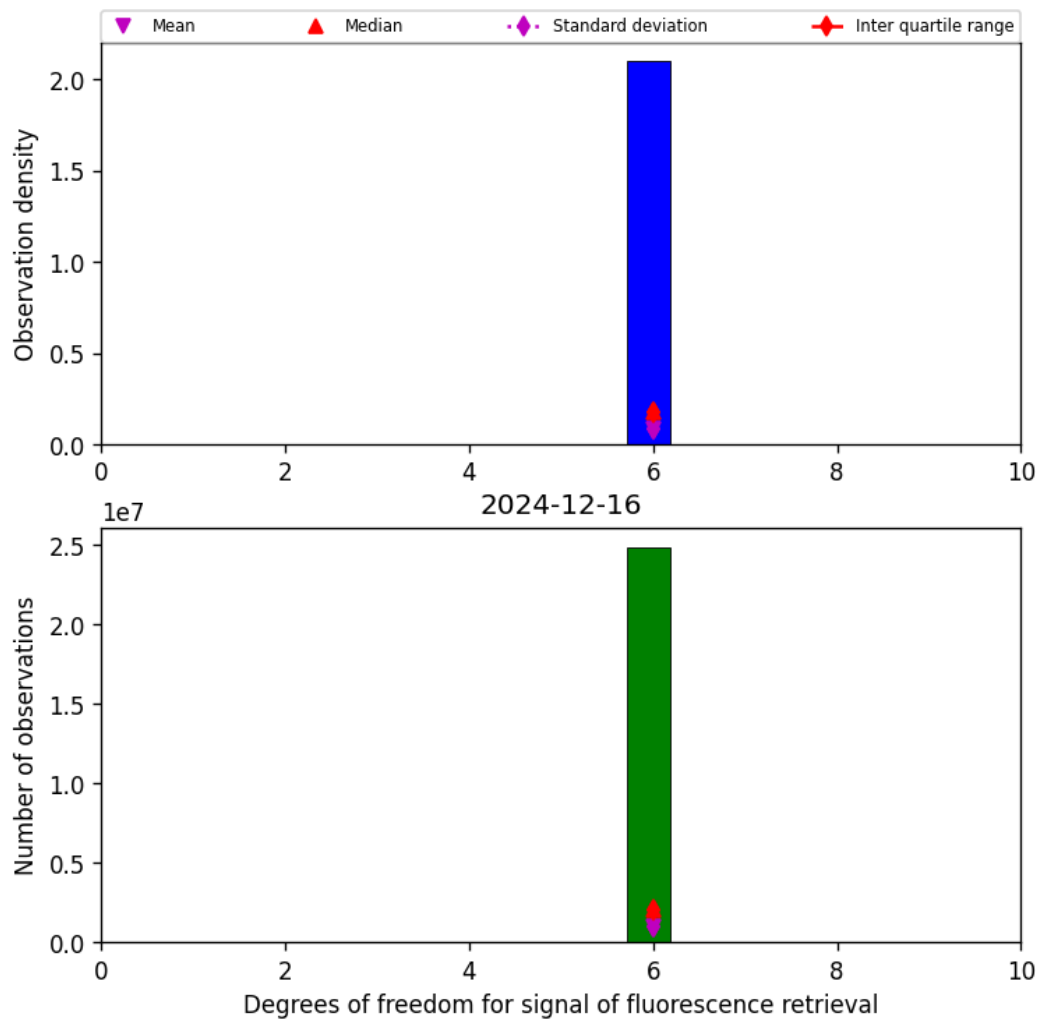
Figure 43: Histogram of “Degrees of freedom for signal of fluorescence retrieval” for 2024-12-16 to 2024-12-17
