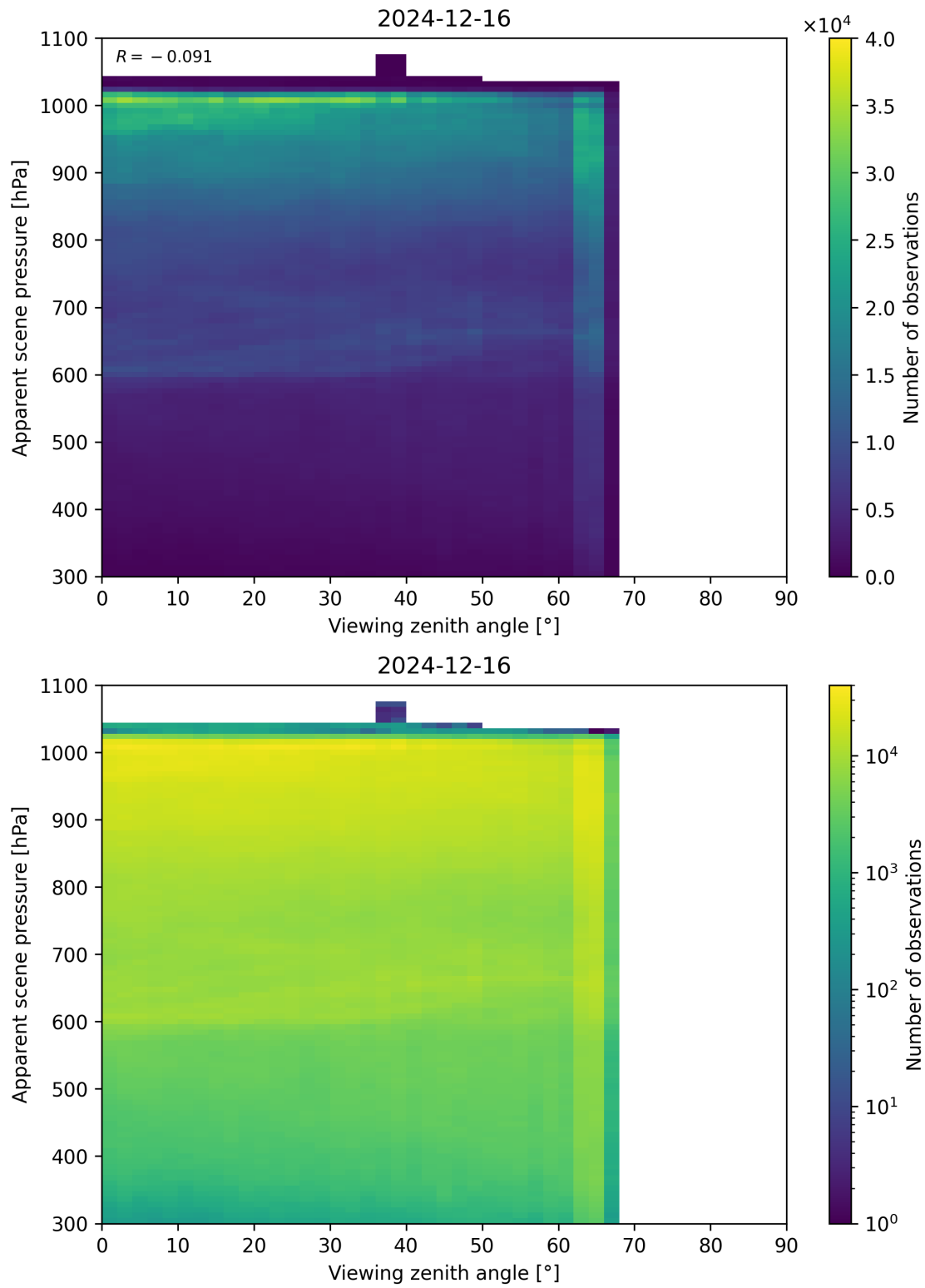
Figure 118: Scatter density plot of “Viewing zenith angle” against “Apparent scene pressure” for 2024-12-16 to 2024-12-17.
