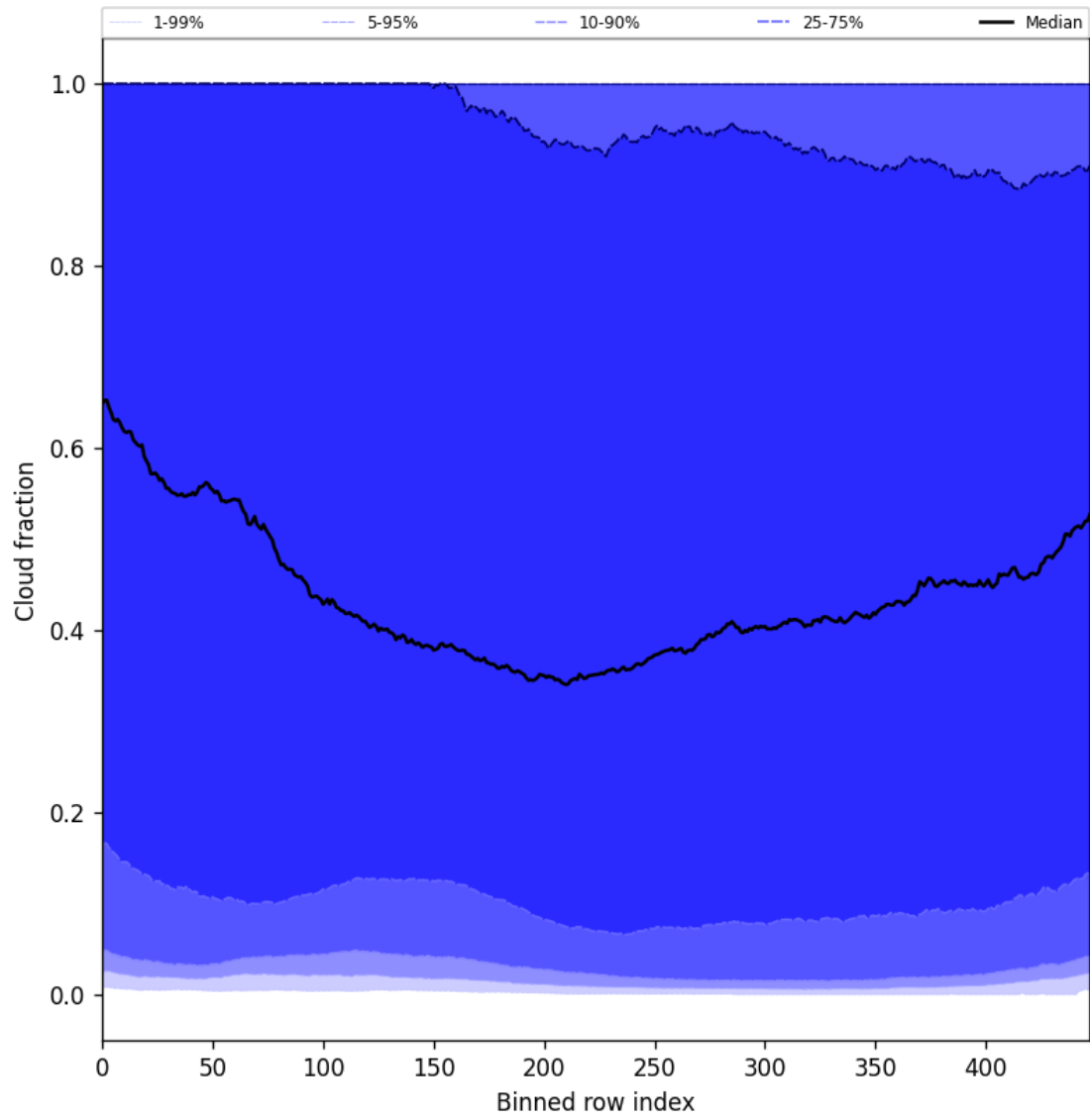
Figure 49: Along track statistics of “Cloud fraction” for 2024-12-16 to 2024-12-17
