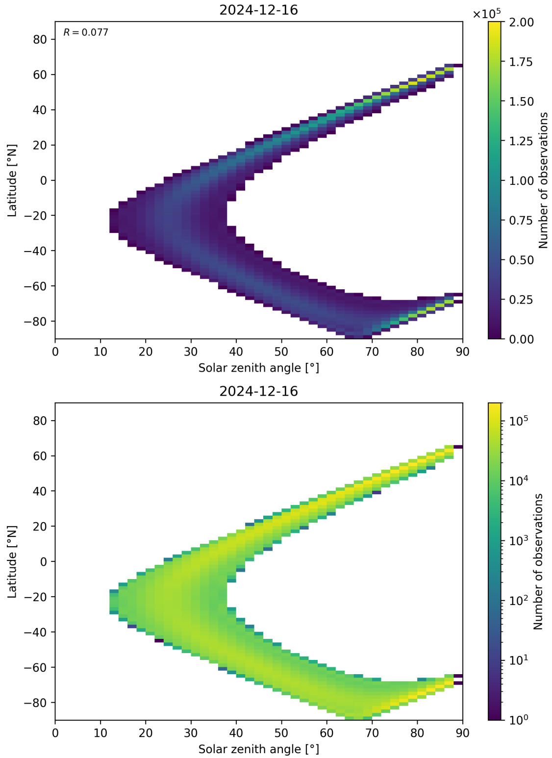
Figure 113: Scatter density plot of “Solar zenith angle” against “Latitude” for 2024-12-16 to 2024-12-17.
