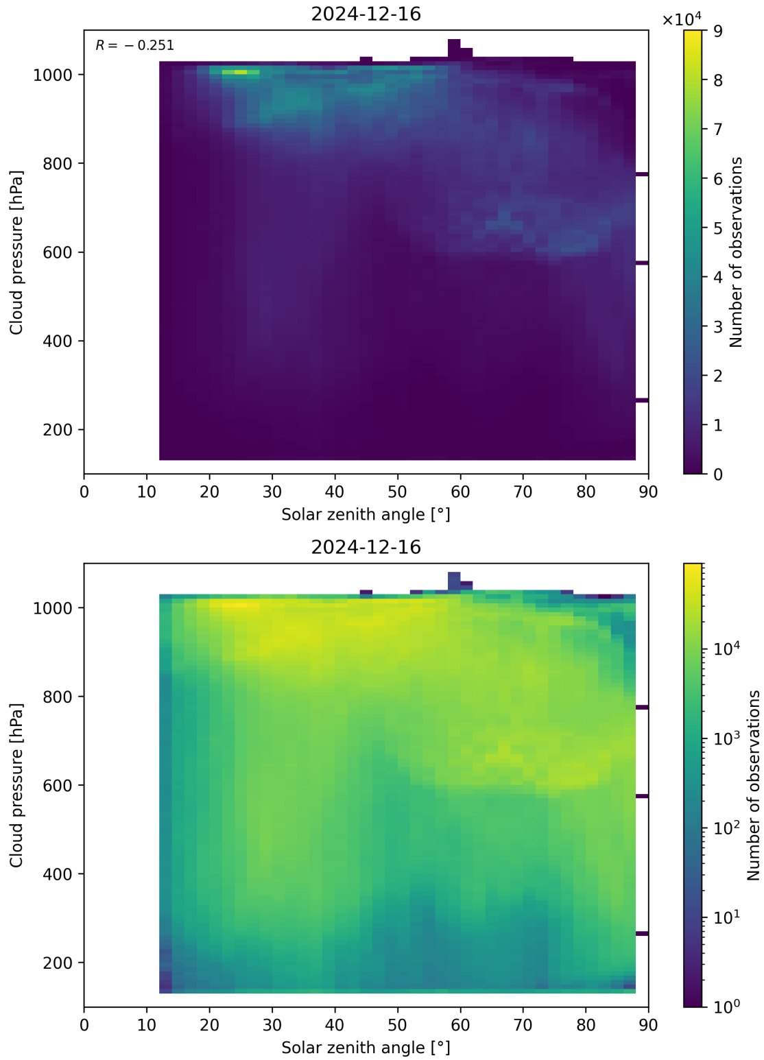
Figure 111: Scatter density plot of “Solar zenith angle” against “Cloud pressure” for 2024-12-16 to 2024-12-17.
