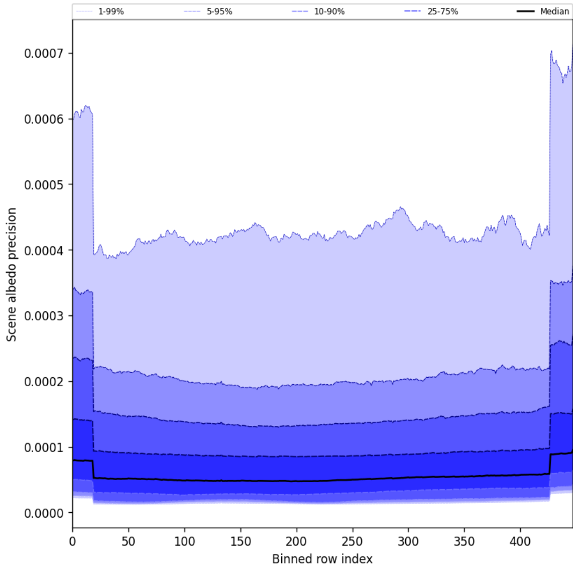
Figure 52: Along track statistics of “Scene albedo precision” for 2024-12-16 to 2024-12-17
