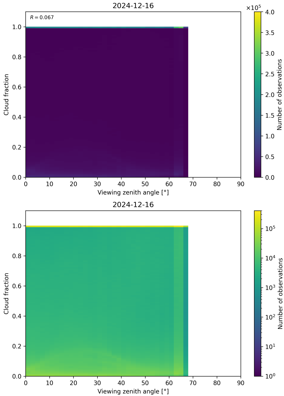
Figure 120: Scatter density plot of “Viewing zenith angle” against “Cloud fraction” for 2024-12-16 to 2024-12-17.
