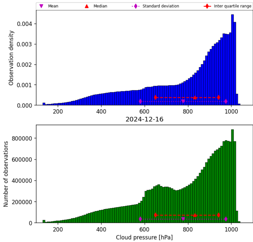
Figure 30: Histogram of “Cloud pressure” for 2024-12-16 to 2024-12-17
