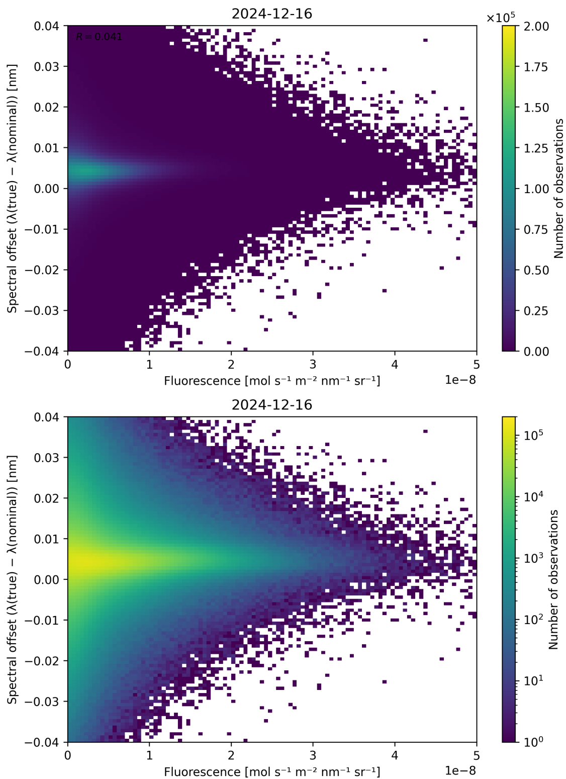
Figure 87: Scatter density plot of “Fluorescence” against “Spectral offset ( \lambda_{\text{true}} - \lambda_{\text{nominal}} )” for 2024-12-16 to 2024-12-17.
