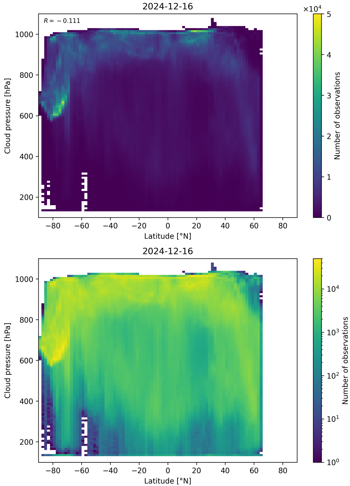
Figure 91: Scatter density plot of “Latitude” against “Cloud pressure” for 2024-12-16 to 2024-12-17.
