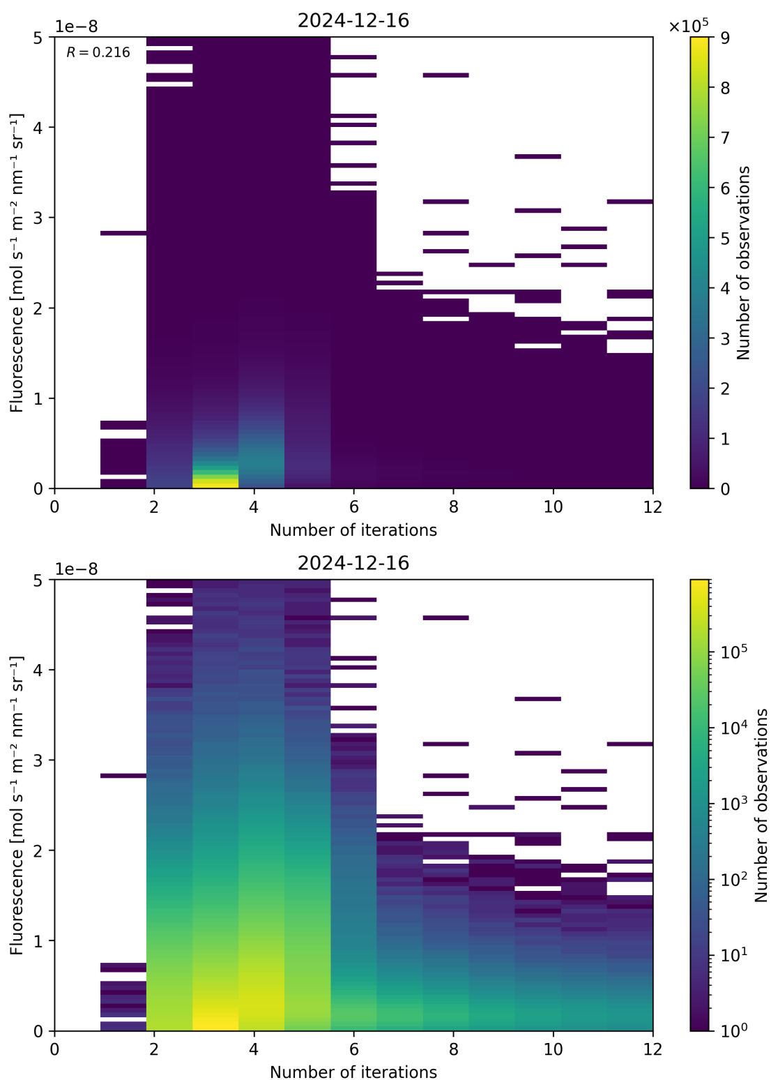
Figure 98: Scatter density plot of “Number of iterations” against “Fluorescence” for 2024-12-16 to 2024-12-17.
