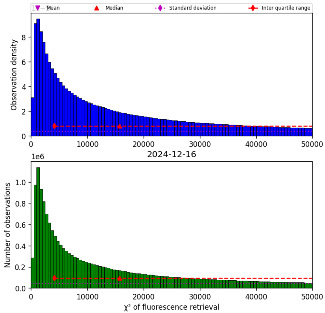
Figure 42: Histogram of “ \chi^2 of fluorescence retrieval” for 2024-12-16 to 2024-12-17
