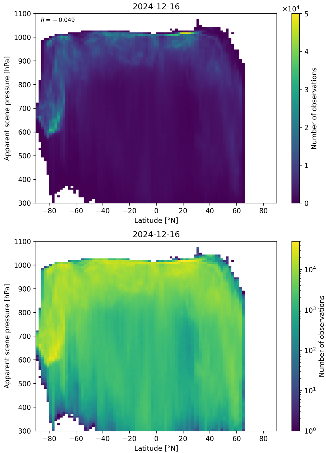
Figure 88: Scatter density plot of “Latitude” against “Apparent scene pressure” for 2024-12-16 to 2024-12-17.
