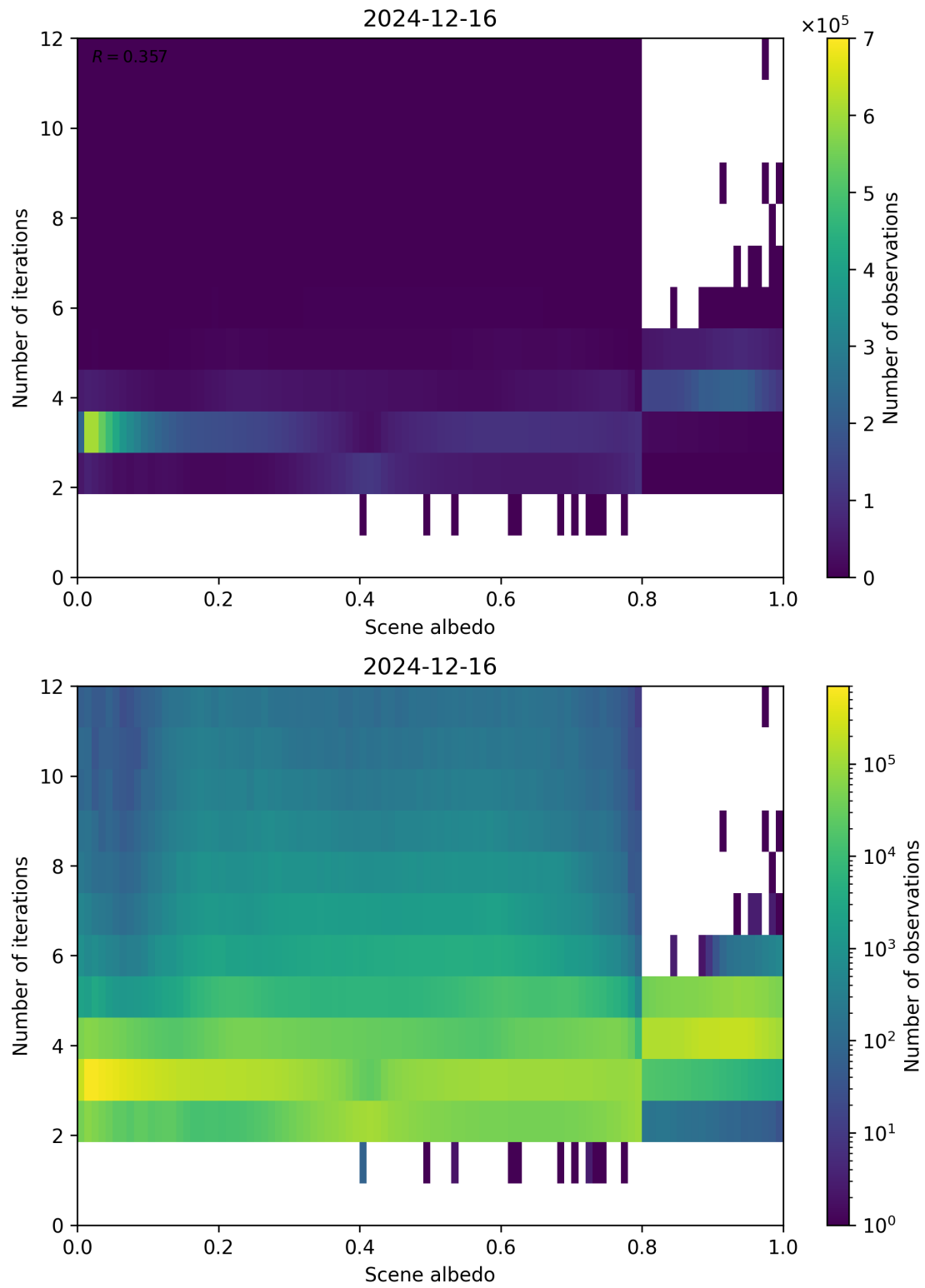
Figure 105: Scatter density plot of “Scene albedo” against “Number of iterations” for 2024-12-16 to 2024-12-17.
