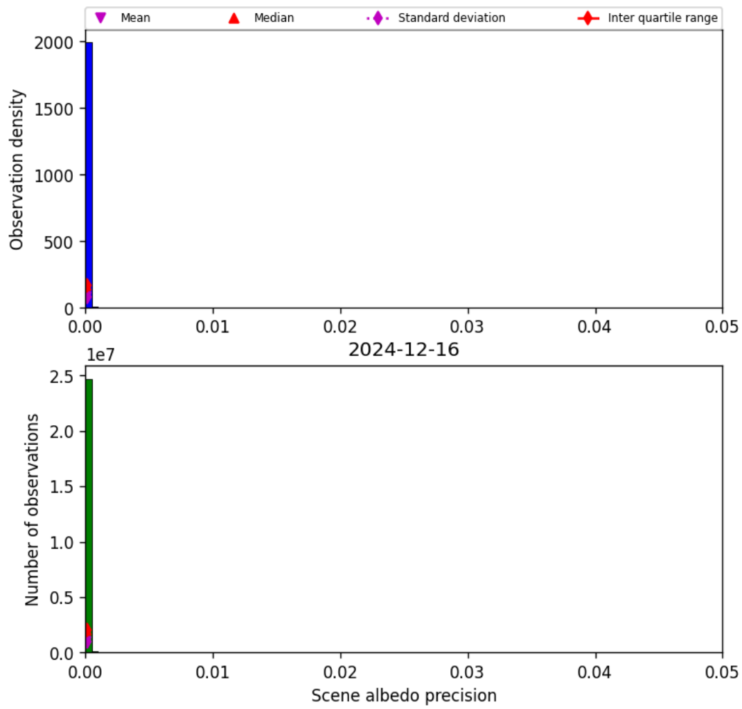
Figure 35: Histogram of “Scene albedo precision” for 2024-12-16 to 2024-12-17
