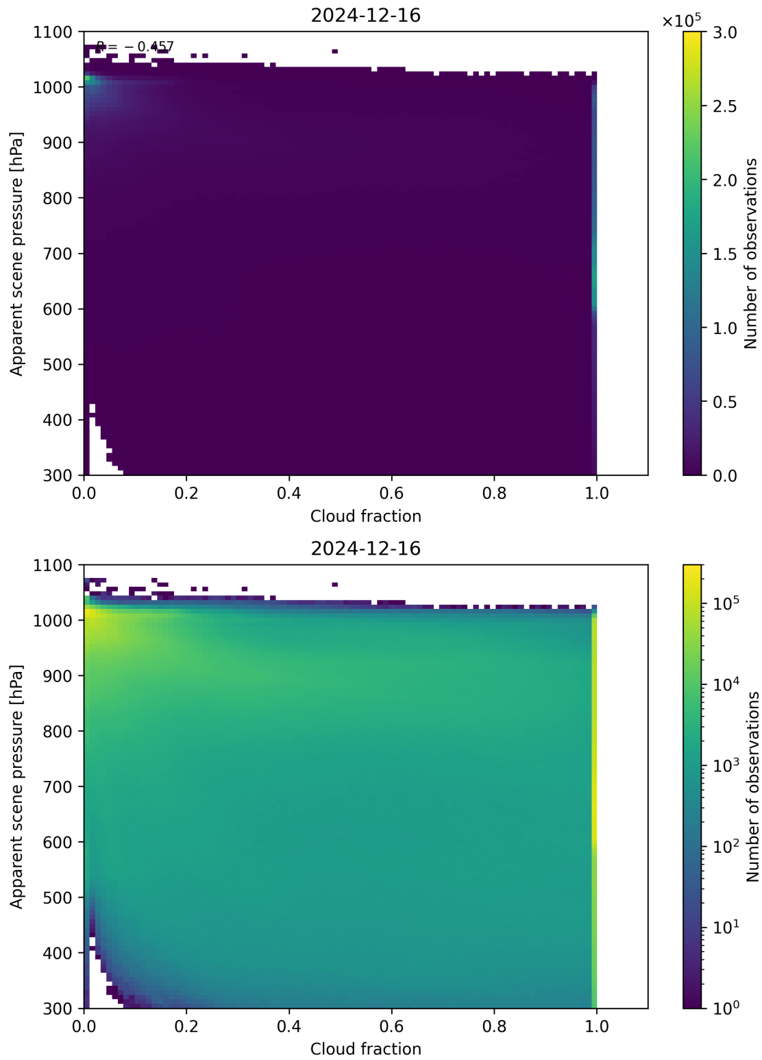
Figure 70: Scatter density plot of “Cloud fraction” against “Apparent scene pressure” for 2024-12-16 to 2024-12-17.
