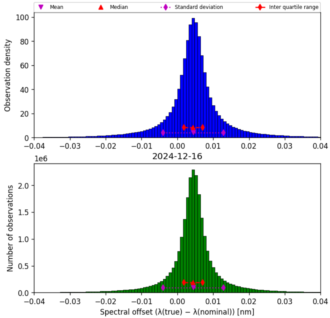
Figure 45: Histogram of “Spectral offset ( \lambda_{\text{true}} - \lambda_{\text{nominal}} )” for 2024-12-16 to 2024-12-17
