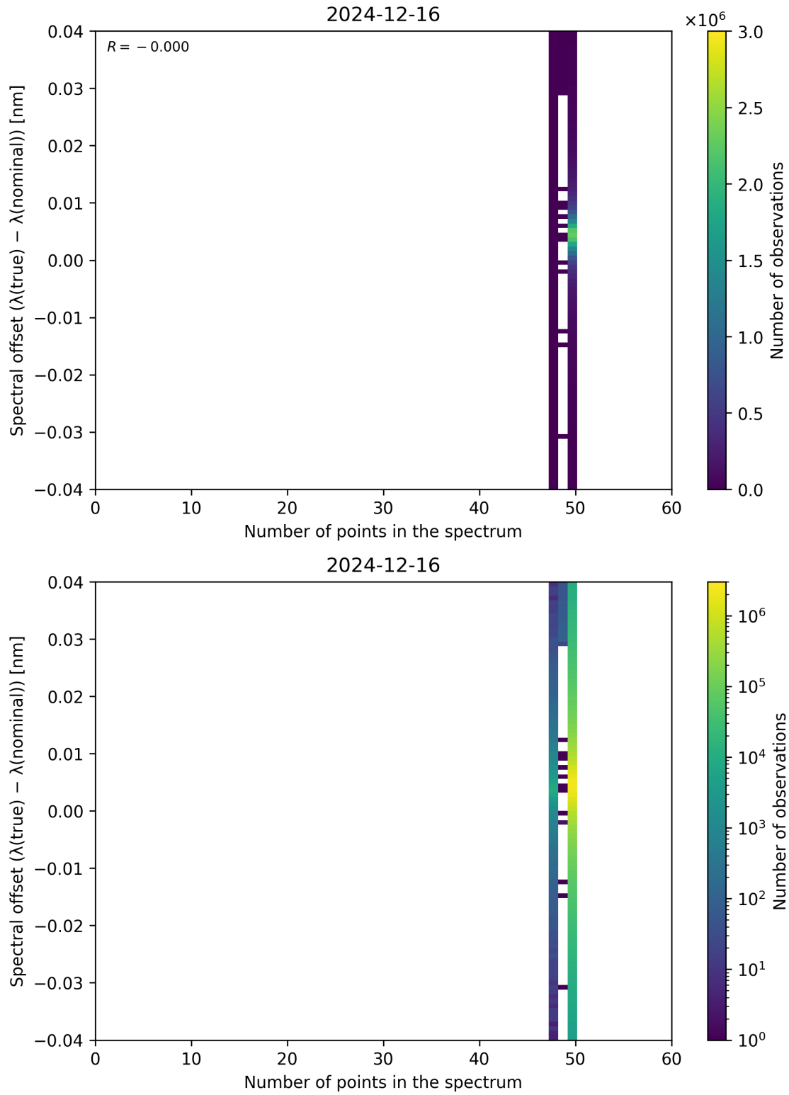
Figure 101: Scatter density plot of “Number of points in the spectrum” against “Spectral offset ( \lambda_{\text{true}} - \lambda_{\text{nominal}} )” for 2024-12-16 to 2024-12-17.
