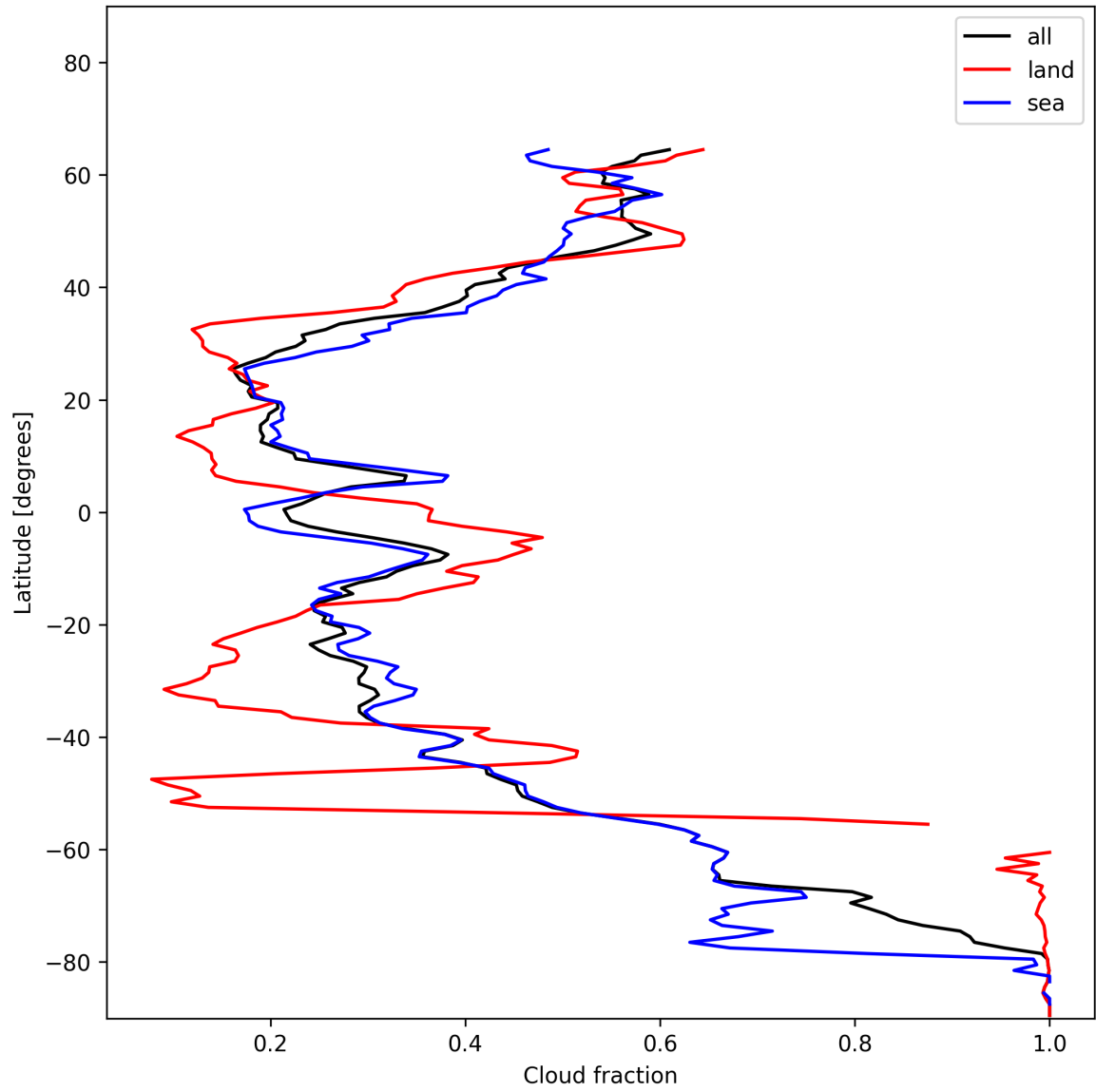
Figure 15: Zonal average of “Cloud fraction” for 2024-12-16 to 2024-12-17.
