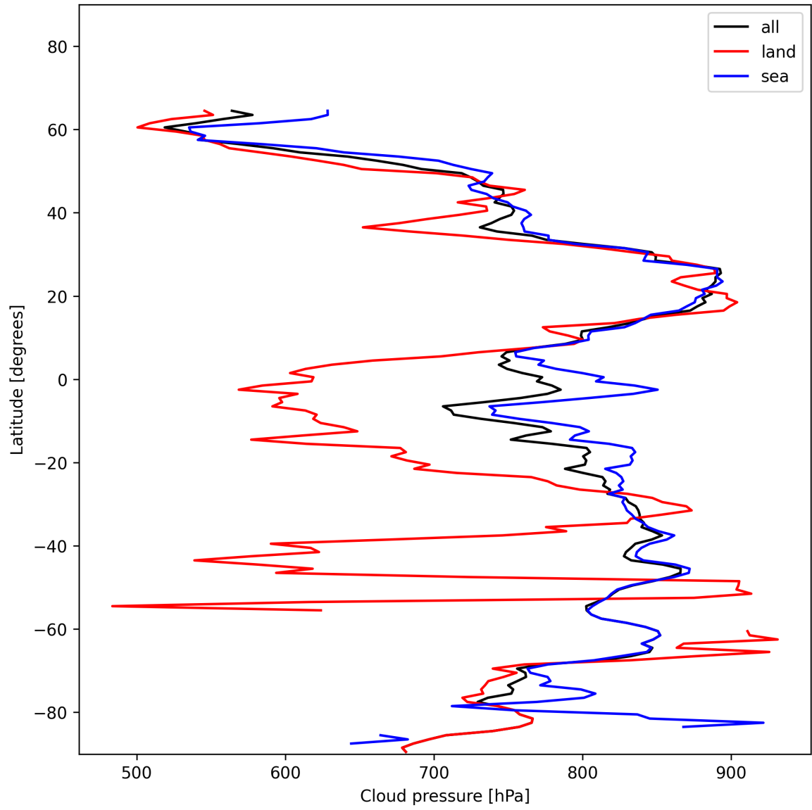
Figure 13: Zonal average of “Cloud pressure” for 2024-12-16 to 2024-12-17.
