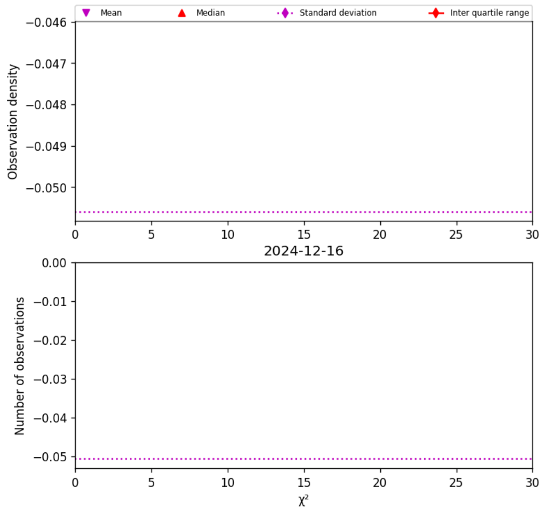
Figure 38: Histogram of " \chi^2 " for 2024-12-16 to 2024-12-17
