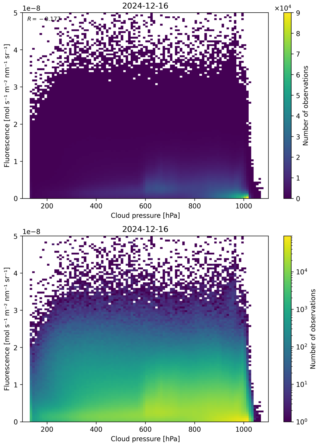
Figure 80: Scatter density plot of “Cloud pressure” against “Fluorescence” for 2024-12-16 to 2024-12-17.
