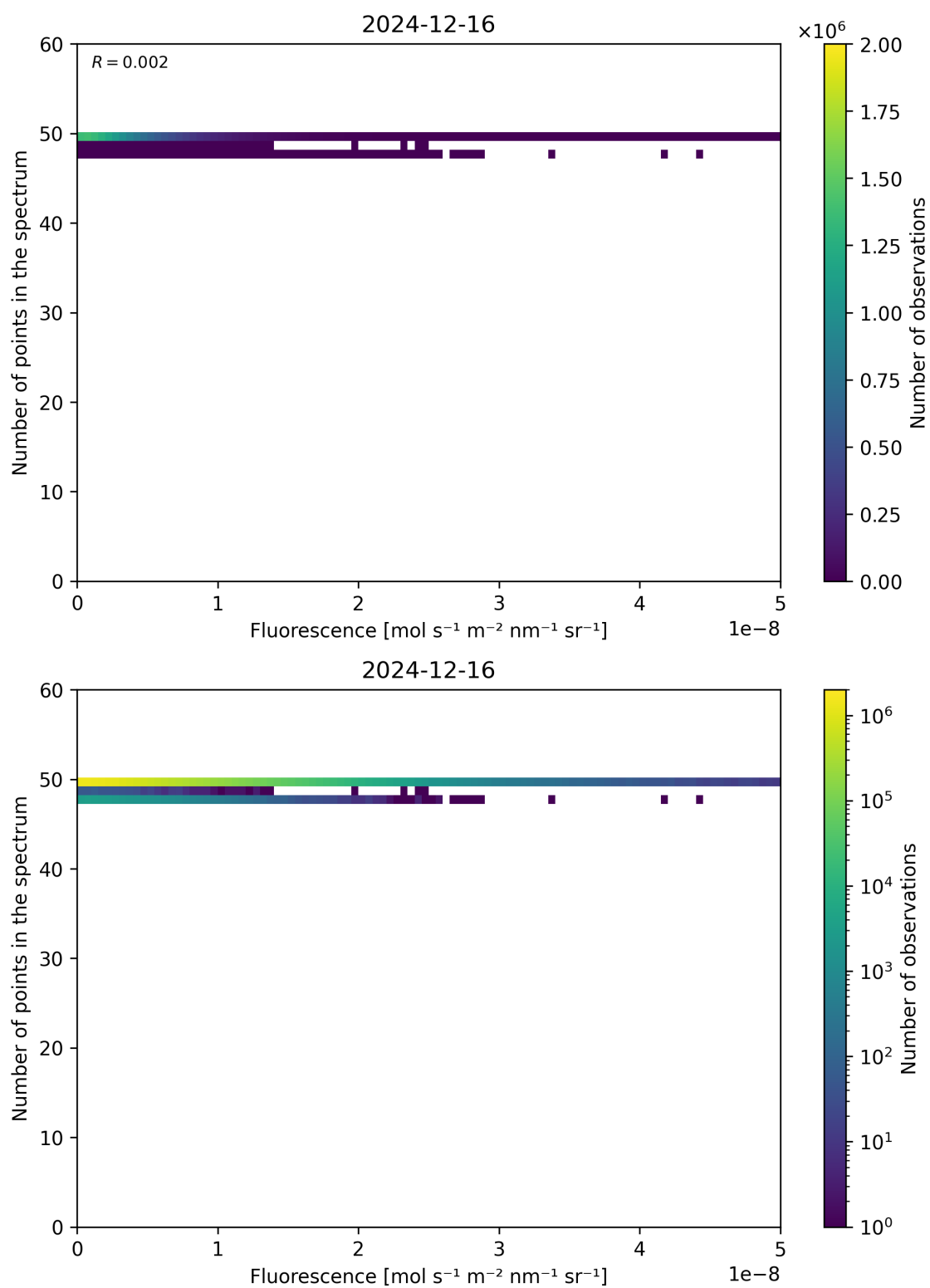
Figure 86: Scatter density plot of “Fluorescence” against “Number of points in the spectrum” for 2024-12-16 to 2024-12-17.
