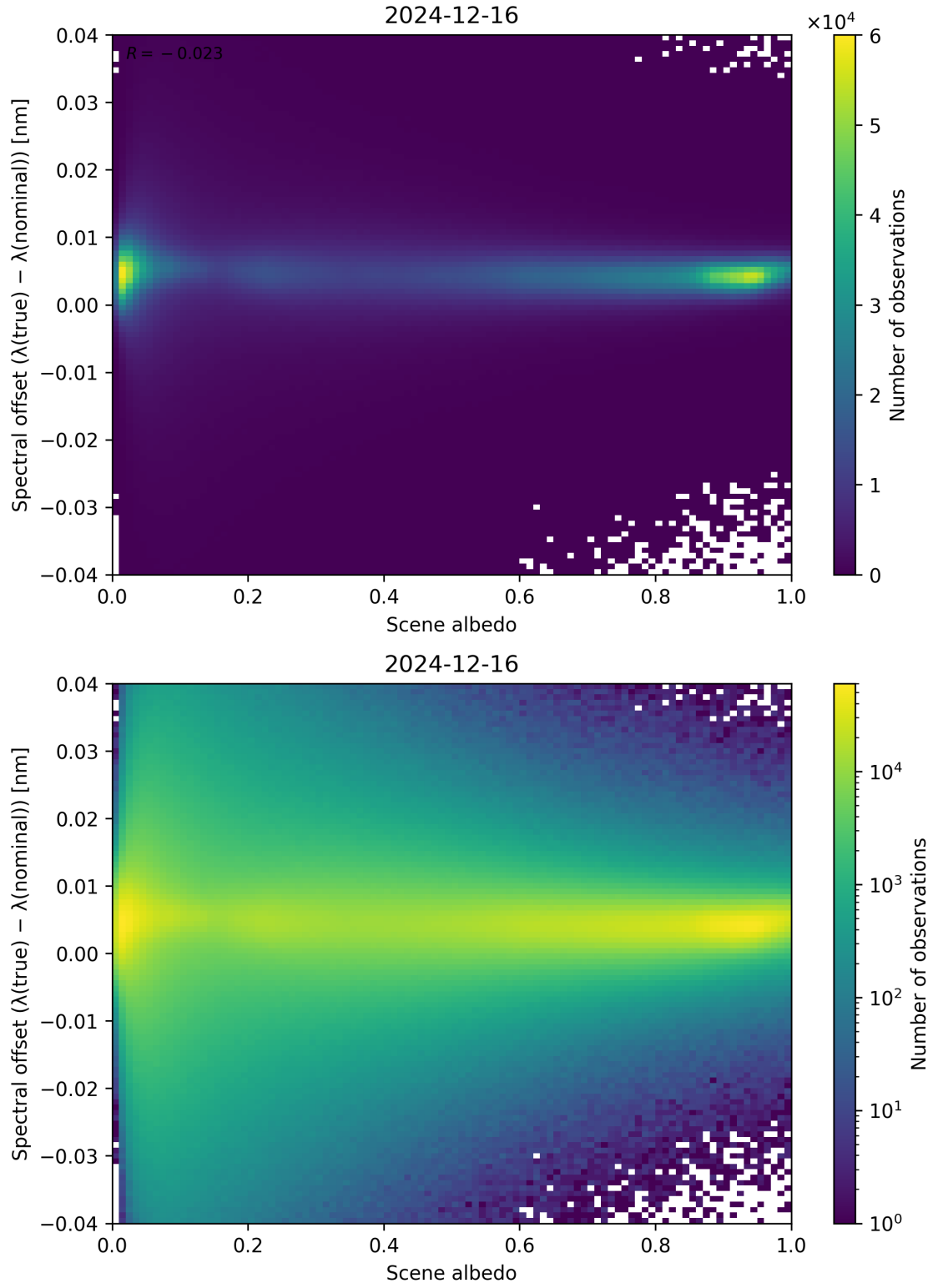
Figure 107: Scatter density plot of “Scene albedo” against “Spectral offset ( \lambda_{\text{true}} - \lambda_{\text{nominal}} )” for 2024-12-16 to 2024-12-17.
