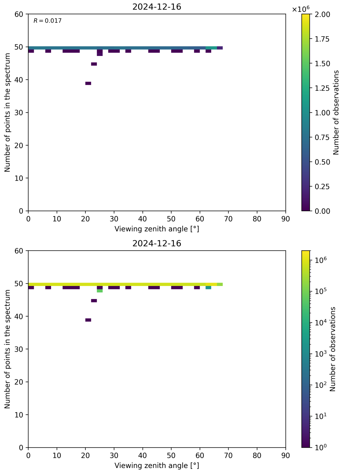
Figure 125: Scatter density plot of “Viewing zenith angle” against “Number of points in the spectrum” for 2024-12-16 to 2024-12-17.
