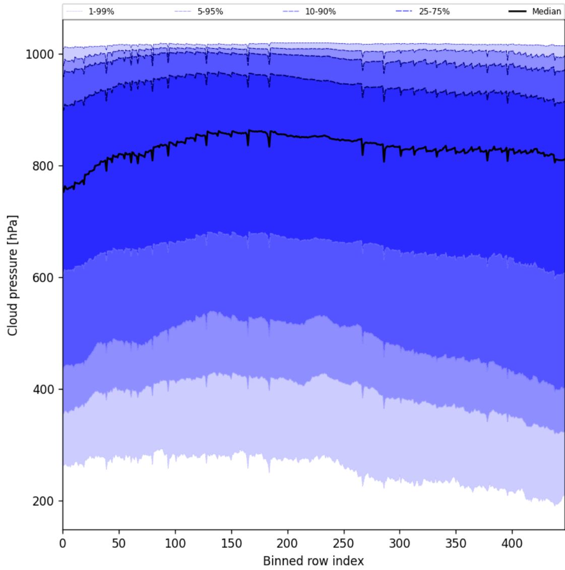
Figure 47: Along track statistics of “Cloud pressure” for 2024-12-16 to 2024-12-17
