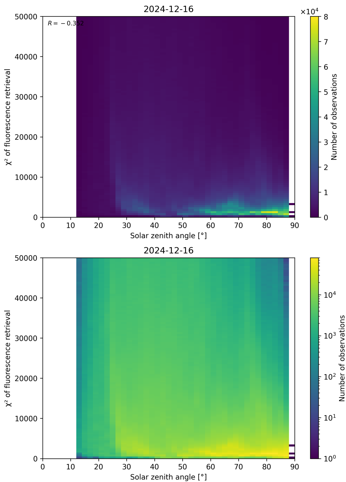
Figure 109: Scatter density plot of “Solar zenith angle” against “ \chi^2 of fluorescence retrieval” for 2024-12-16 to 2024-12-17.
