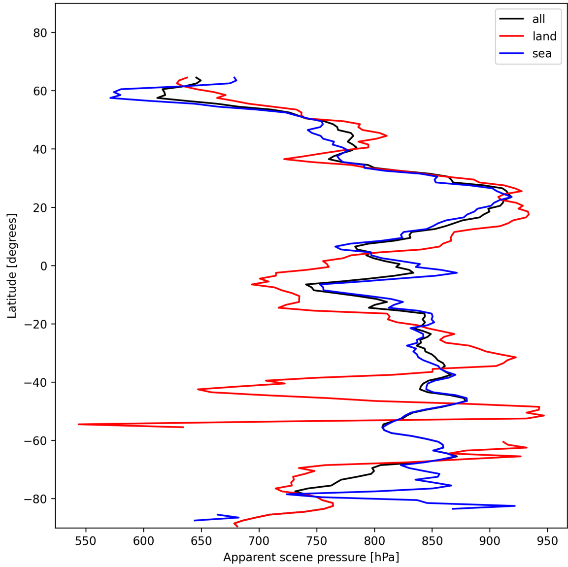
Figure 19: Zonal average of “Apparent scene pressure” for 2024-12-16 to 2024-12-17.
