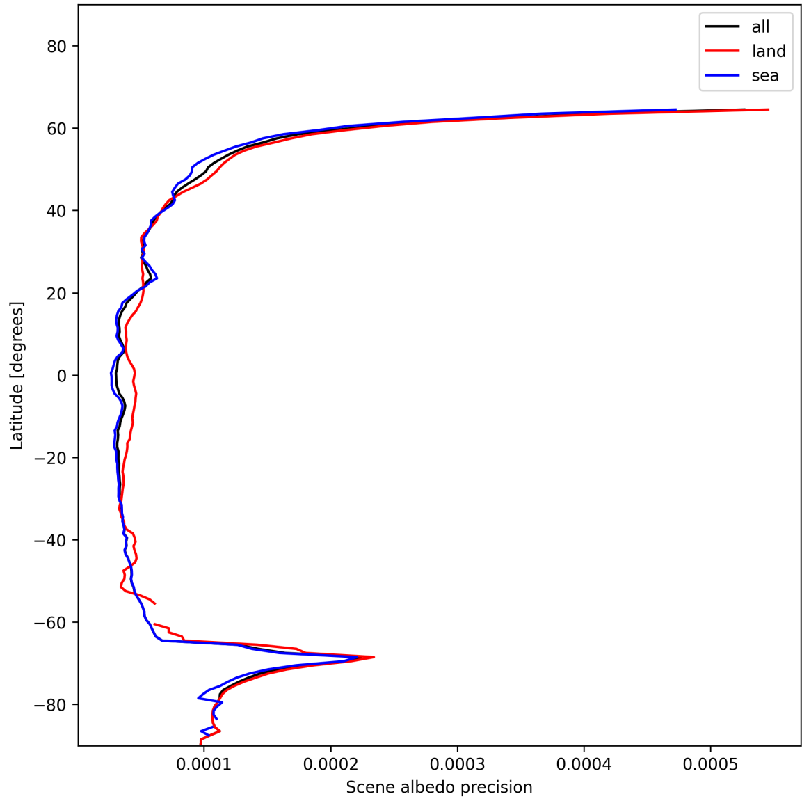
Figure 18: Zonal average of “Scene albedo precision” for 2024-12-16 to 2024-12-17.
