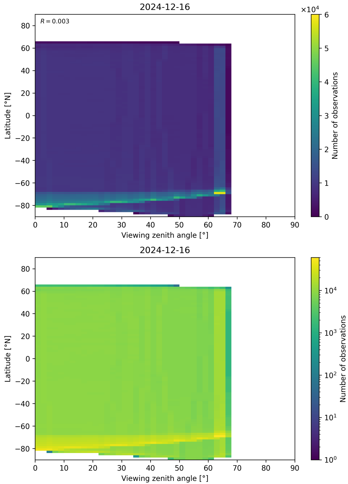
Figure 123: Scatter density plot of “Viewing zenith angle” against “Latitude” for 2024-12-16 to 2024-12-17.
