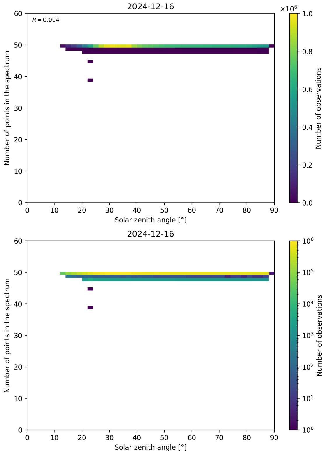
Figure 115: Scatter density plot of “Solar zenith angle” against “Number of points in the spectrum” for 2024-12-16 to 2024-12-17.
