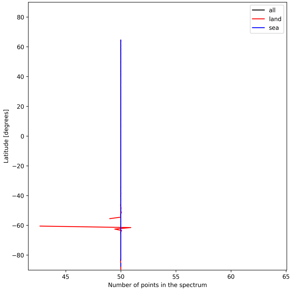
Figure 27: Zonal average of “Number of points in the spectrum” for 2024-12-16 to 2024-12-17.
