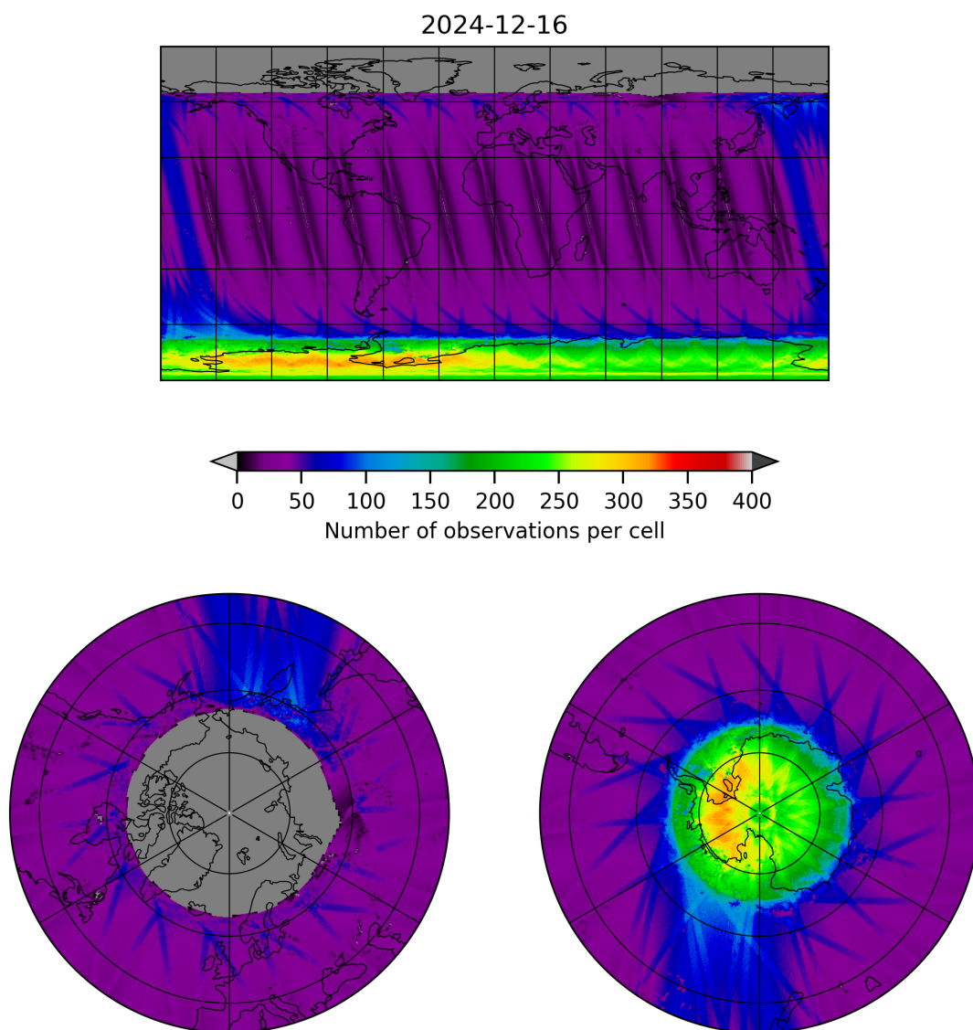
Figure 11: Map of the number of observations for 2024-12-16 to 2024-12-17
