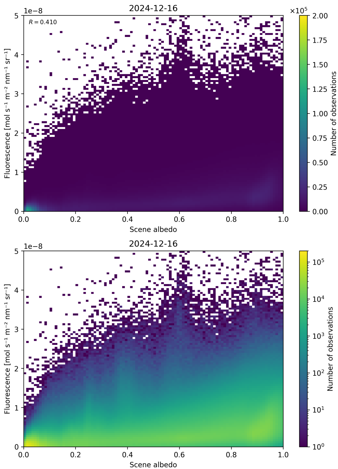
Figure 104: Scatter density plot of “Scene albedo” against “Fluorescence” for 2024-12-16 to 2024-12-17.
