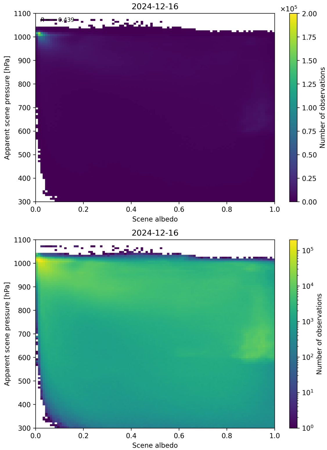
Figure 102: Scatter density plot of “Scene albedo” against “Apparent scene pressure” for 2024-12-16 to 2024-12-17.
