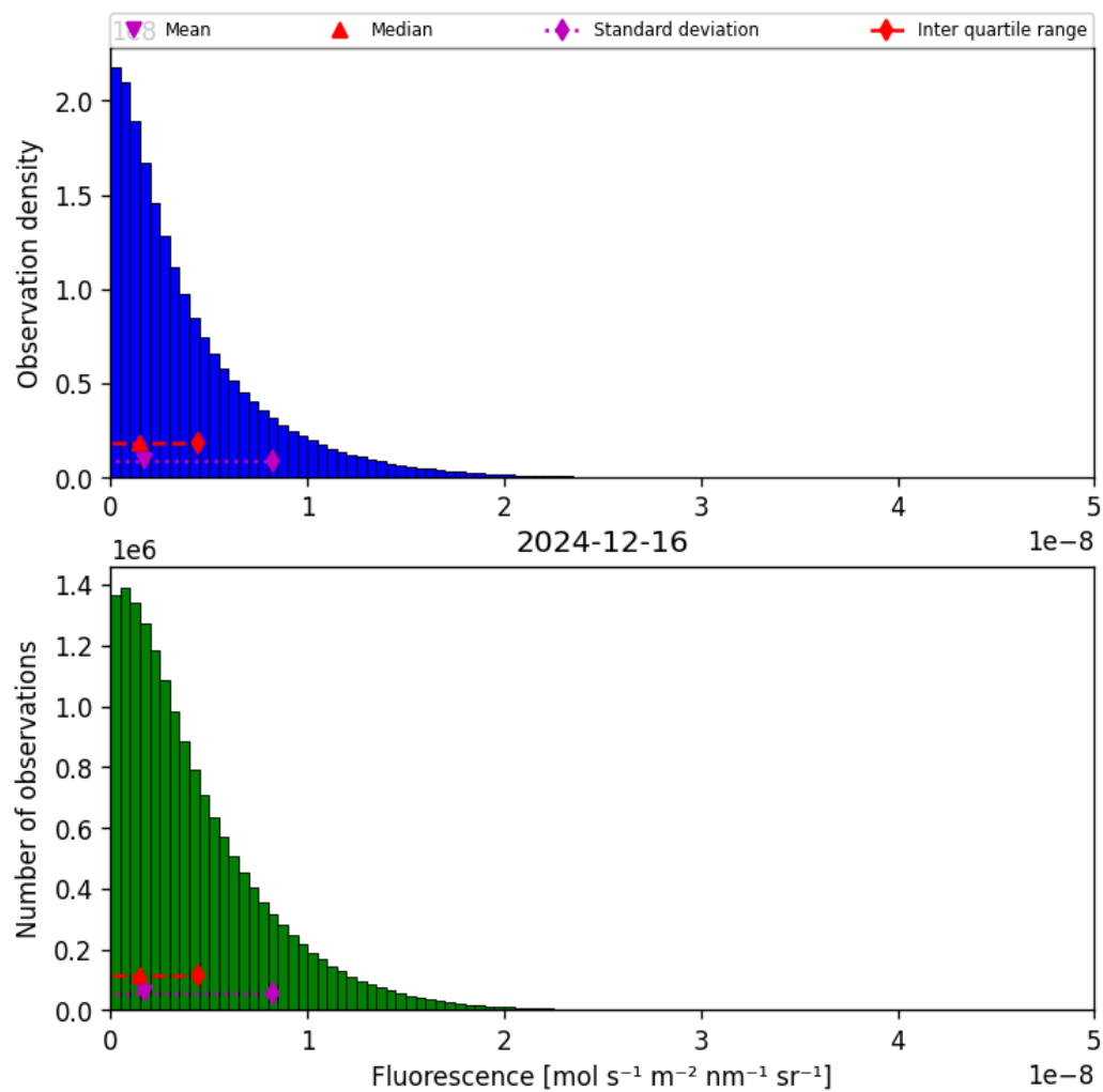
Figure 40: Histogram of “Fluorescence” for 2024-12-16 to 2024-12-17
