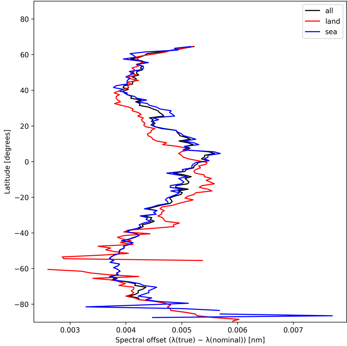
Figure 28: Zonal average of “Spectral offset ( \lambda_{\text{true}} - \lambda_{\text{nominal}} )” for 2024-12-16 to 2024-12-17.
