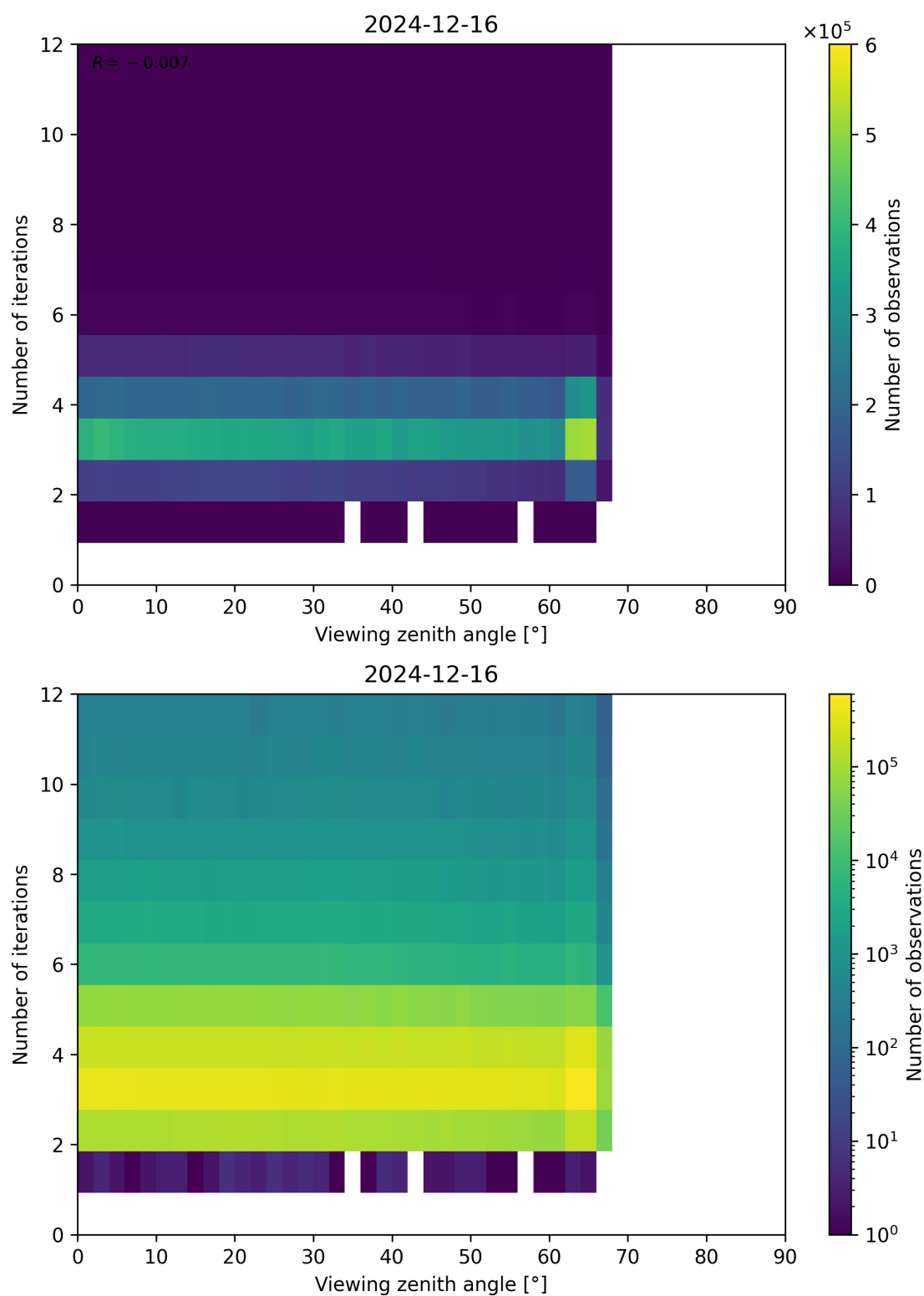
Figure 124: Scatter density plot of “Viewing zenith angle” against “Number of iterations” for 2024-12-16 to 2024-12-17.
