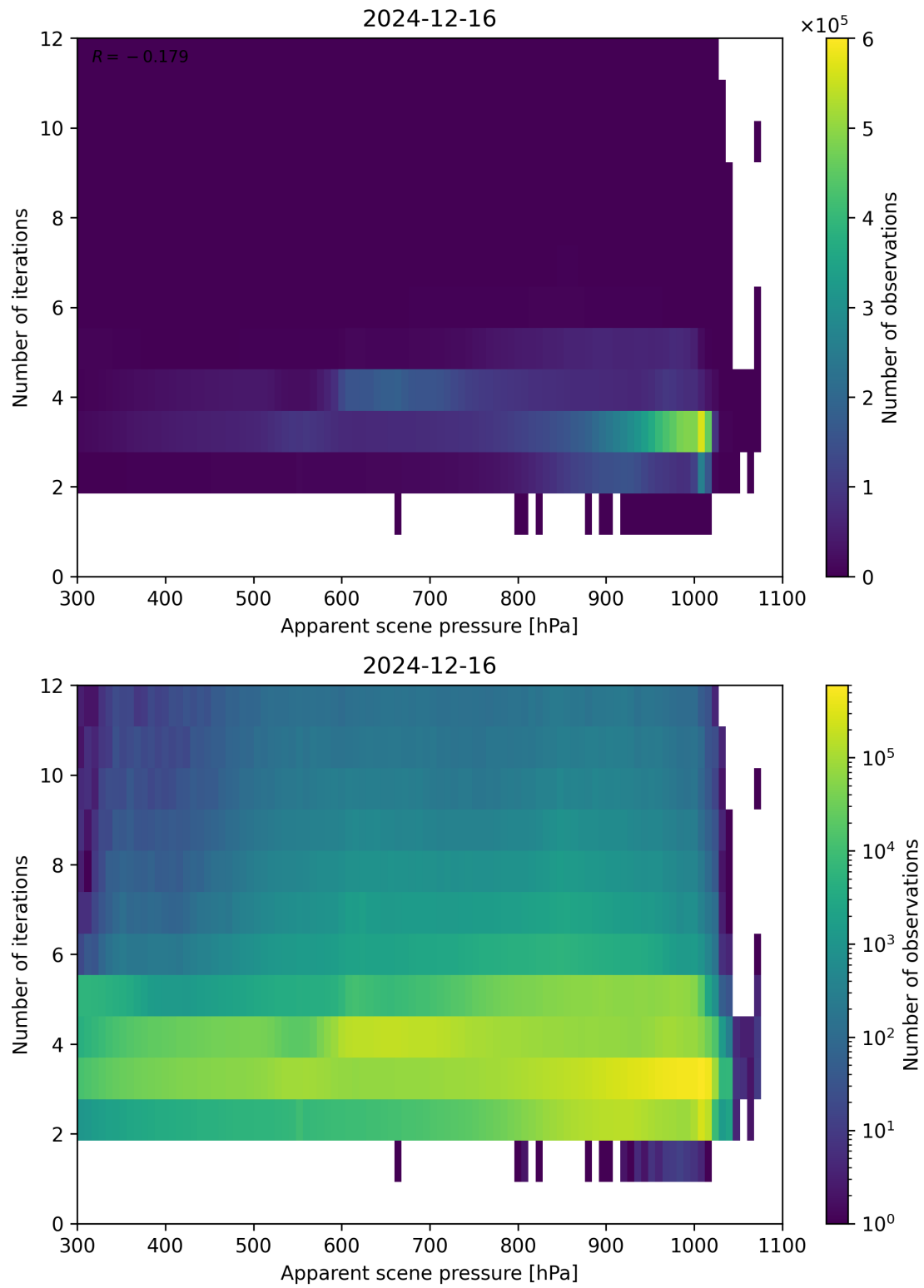
Figure 65: Scatter density plot of “Apparent scene pressure” against “Number of iterations” for 2024-12-16 to 2024-12-17.
