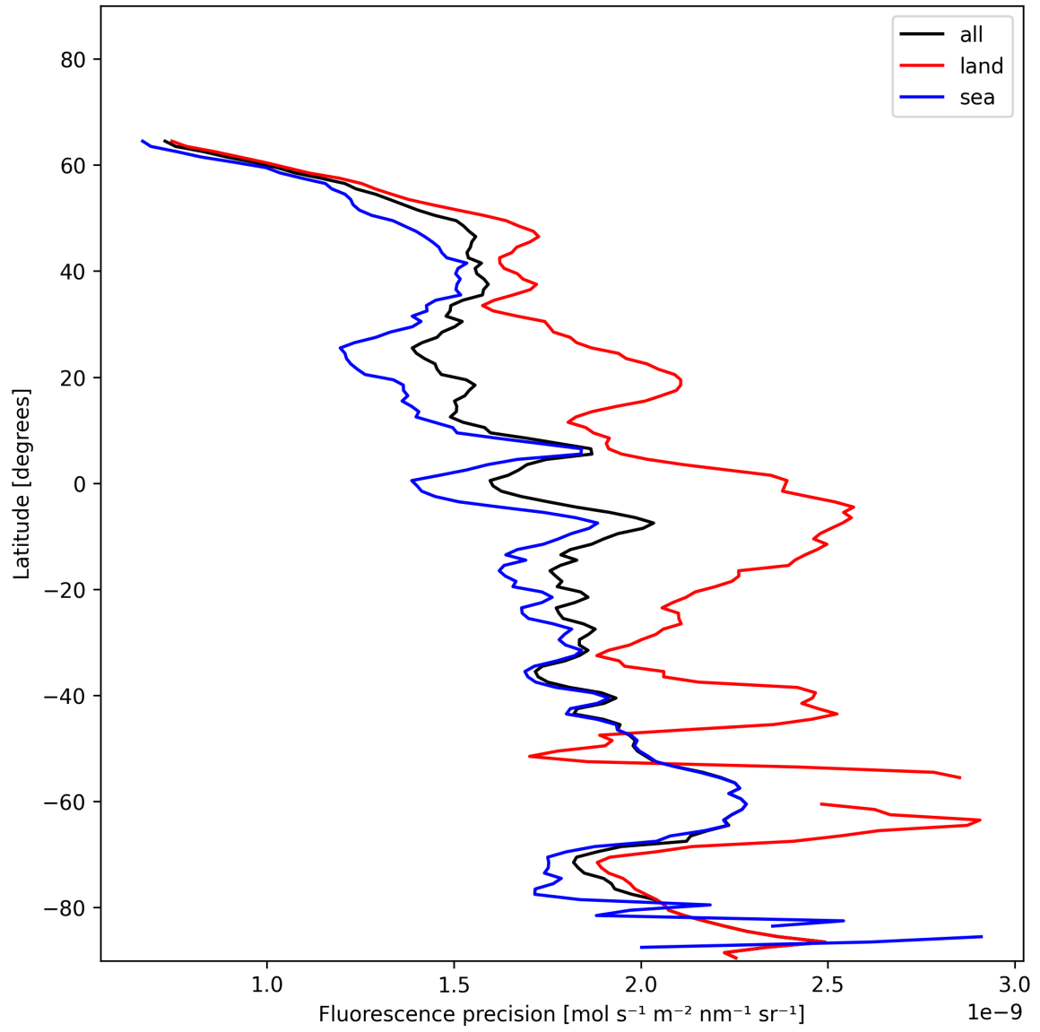
Figure 24: Zonal average of “Fluorescence precision” for 2024-12-16 to 2024-12-17.
