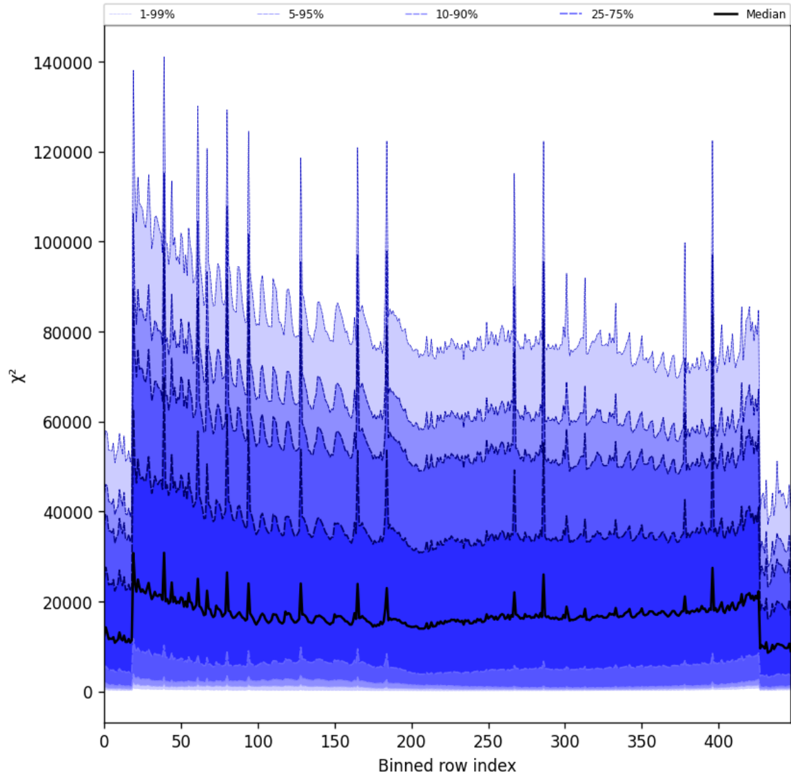
Figure 55: Along track statistics of “ \chi^2 ” for 2024-12-16 to 2024-12-17
