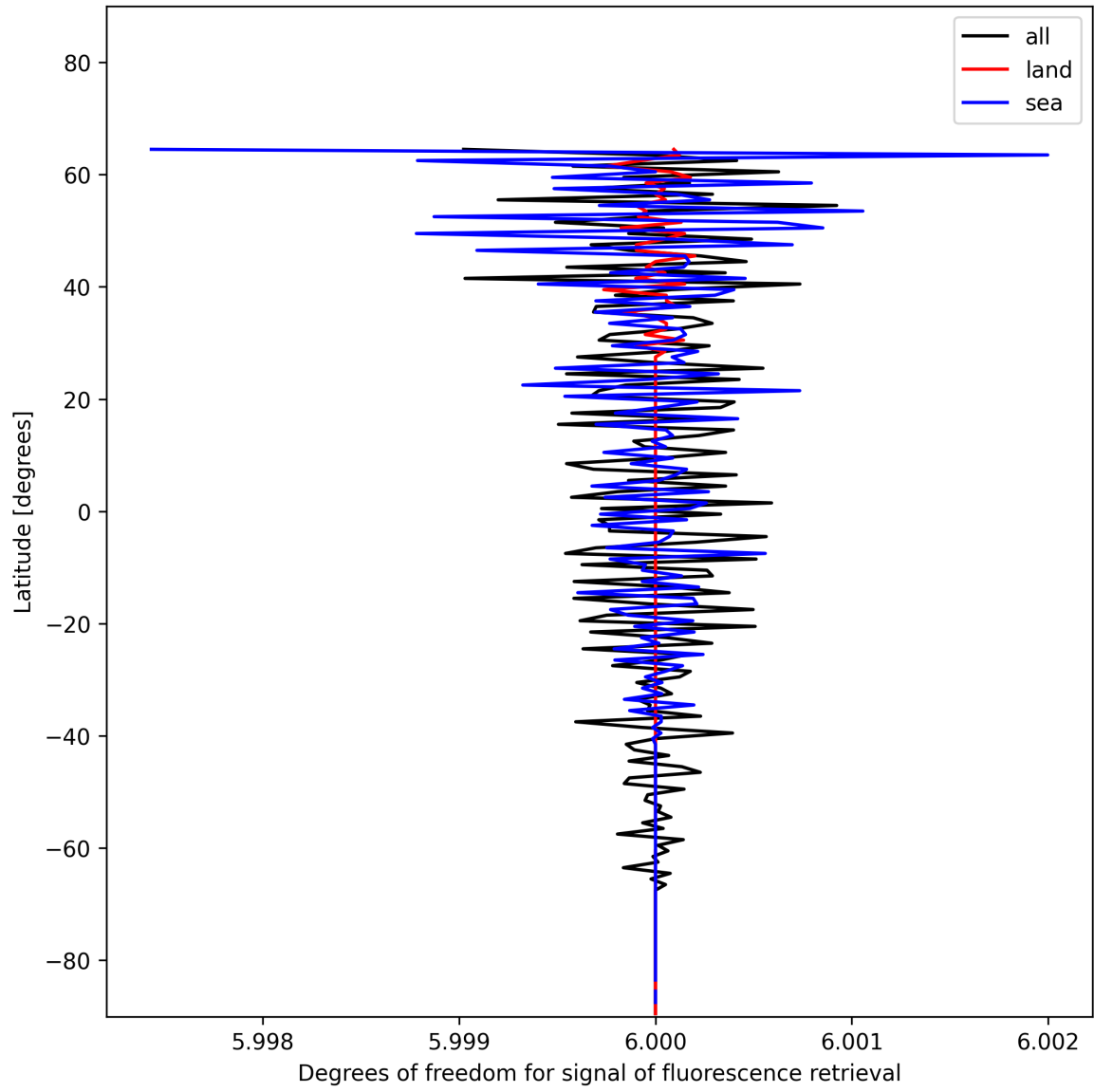
Figure 26: Zonal average of “Degrees of freedom for signal of fluorescence retrieval” for 2024-12-16 to 2024-12-17.
