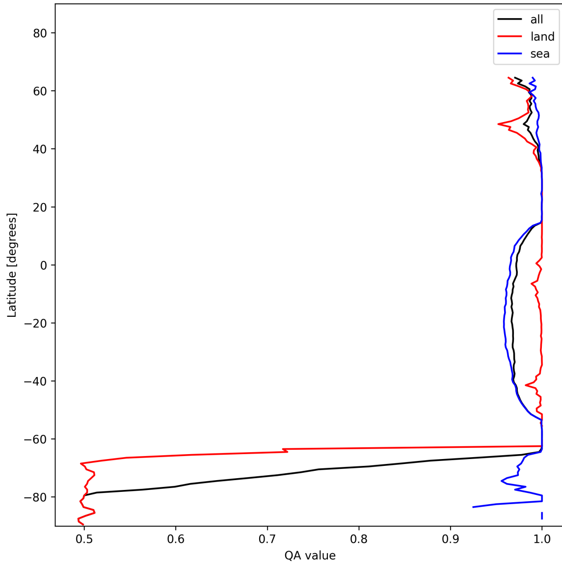
Figure 12: Zonal average of “QA value” for 2024-12-16 to 2024-12-17.
