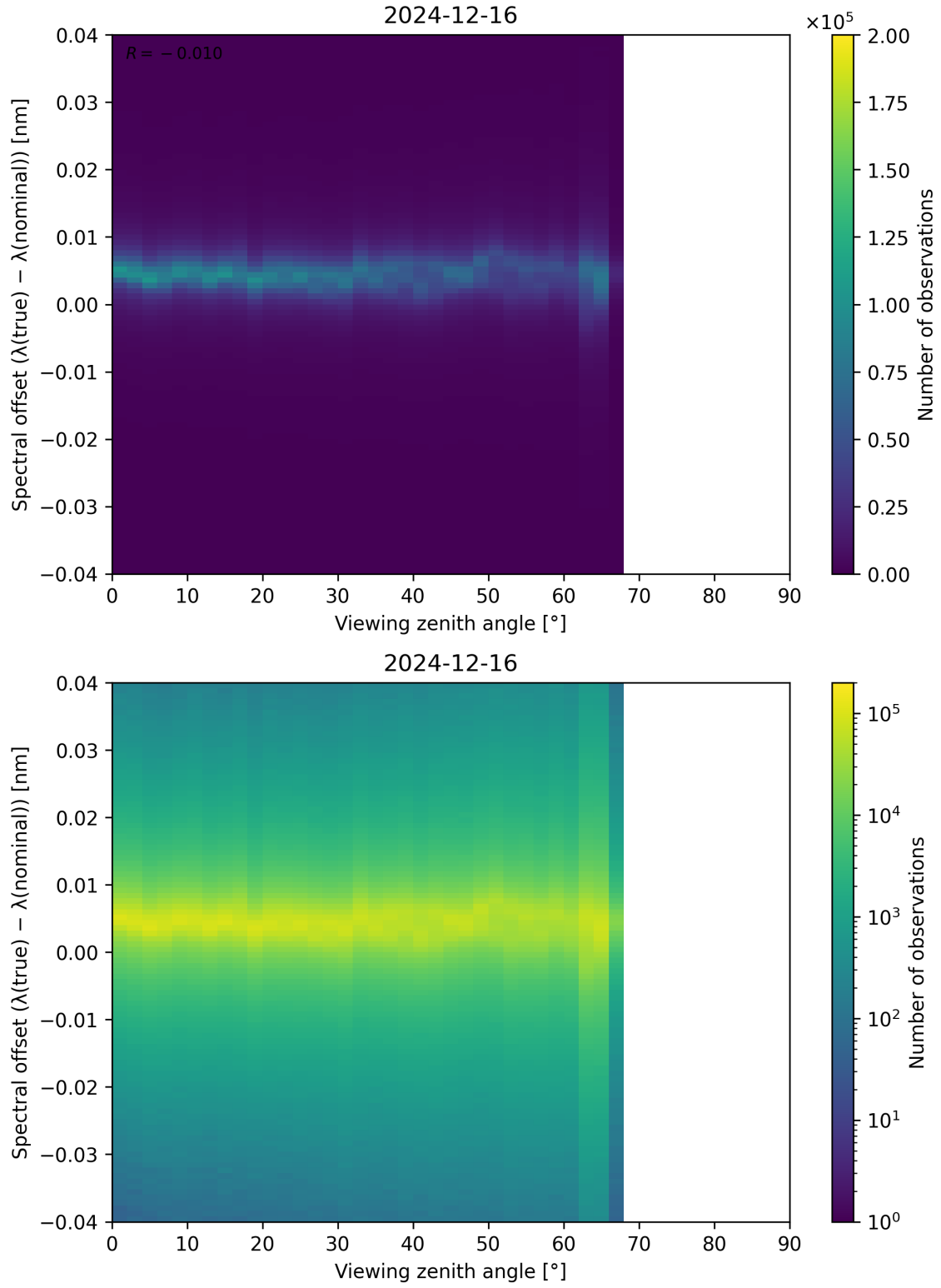
Figure 128: Scatter density plot of “Viewing zenith angle” against “Spectral offset ( \lambda_{\text{true}} - \lambda_{\text{nominal}} )” for 2024-12-16 to 2024-12-17.
