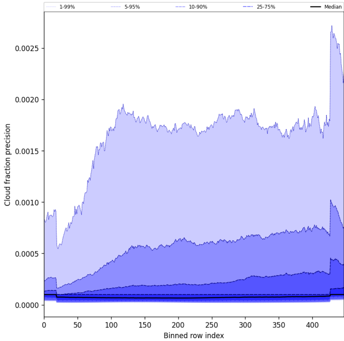
Figure 50: Along track statistics of “Cloud fraction precision” for 2024-12-16 to 2024-12-17
