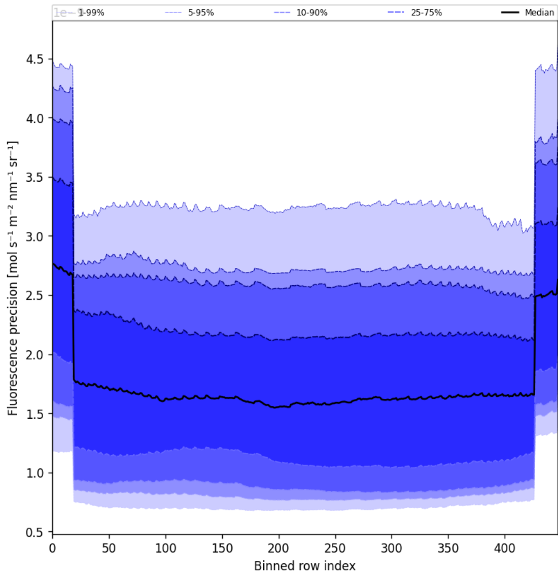
Figure 58: Along track statistics of “Fluorescence precision” for 2024-12-16 to 2024-12-17
