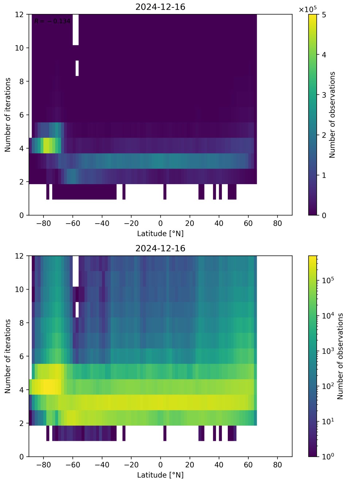
Figure 93: Scatter density plot of “Latitude” against “Number of iterations” for 2024-12-16 to 2024-12-17.
