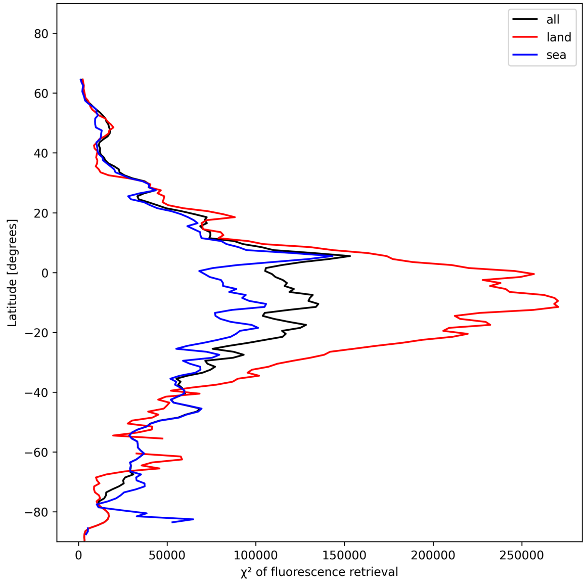
Figure 25: Zonal average of “ \chi^2 of fluorescence retrieval” for 2024-12-16 to 2024-12-17.
