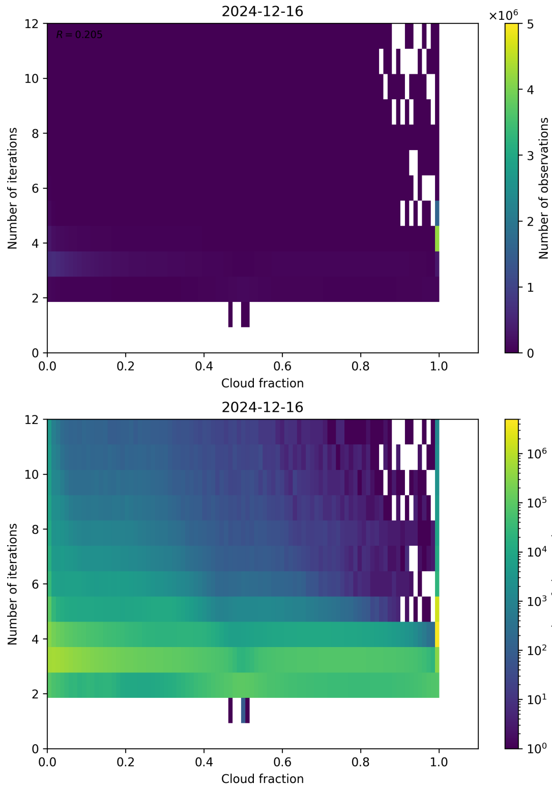
Figure 73: Scatter density plot of “Cloud fraction” against “Number of iterations” for 2024-12-16 to 2024-12-17.
