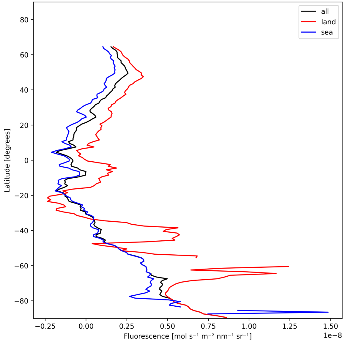
Figure 23: Zonal average of “Fluorescence” for 2024-12-16 to 2024-12-17.
