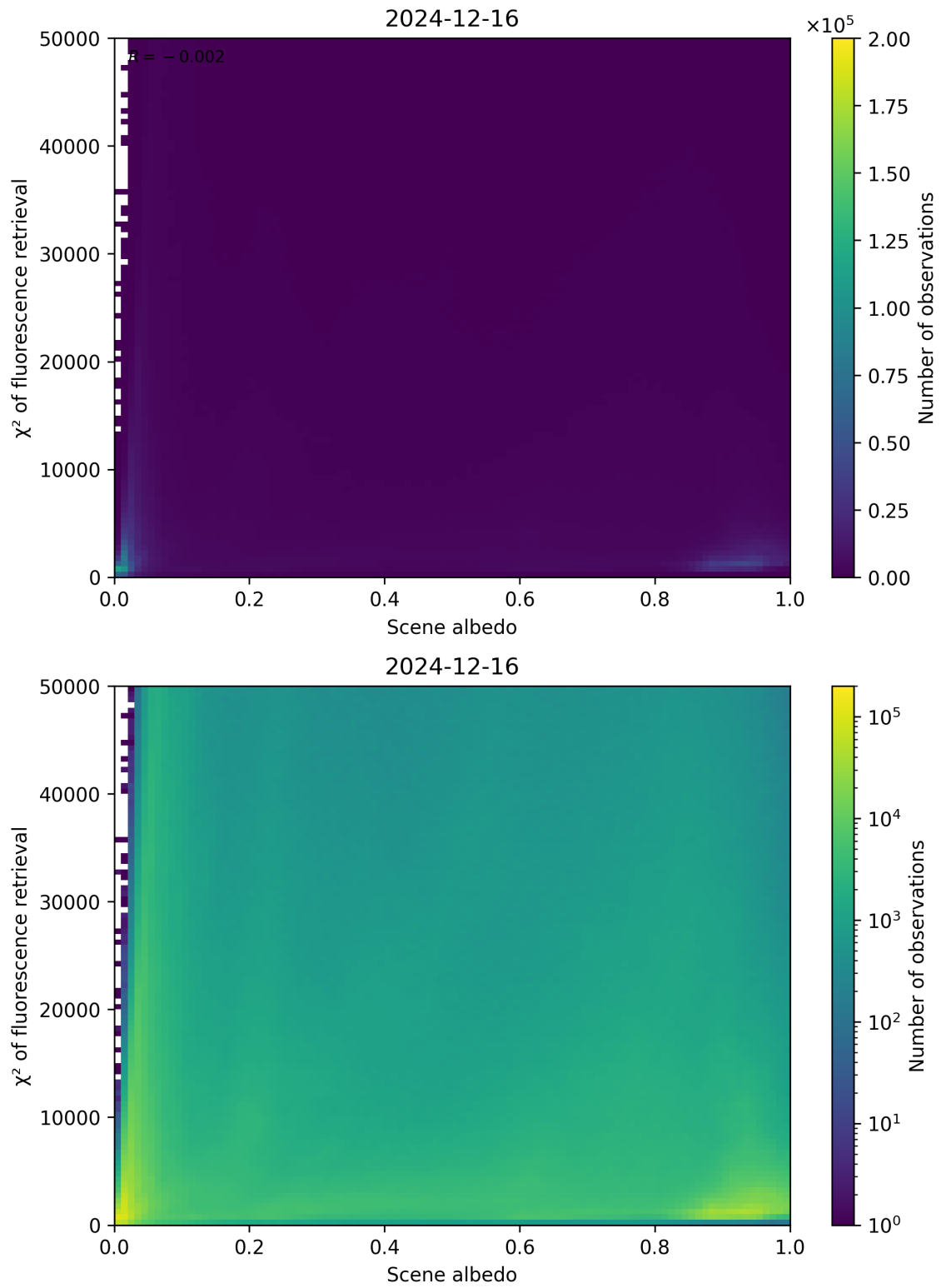
Figure 103: Scatter density plot of “Scene albedo” against “ \chi^2 of fluorescence retrieval” for 2024-12-16 to 2024-12-17.
