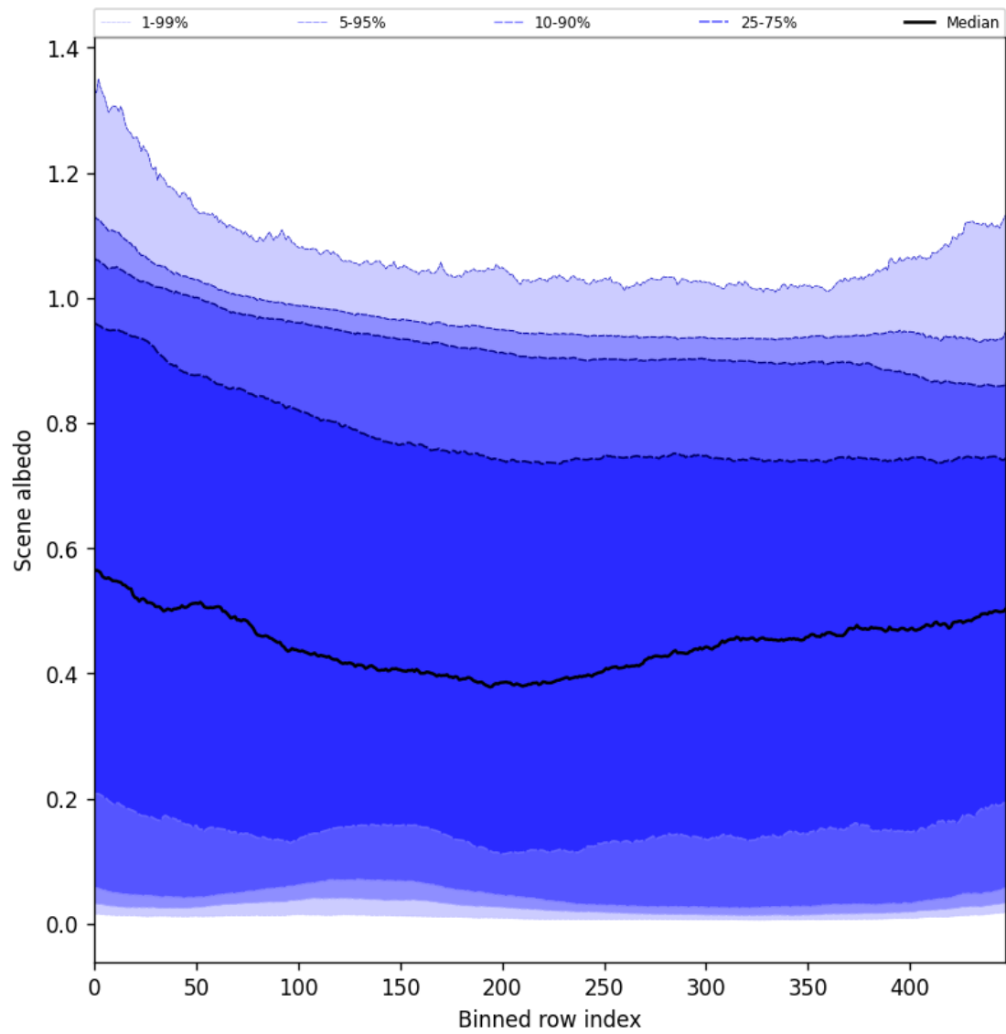
Figure 51: Along track statistics of “Scene albedo” for 2024-12-16 to 2024-12-17
