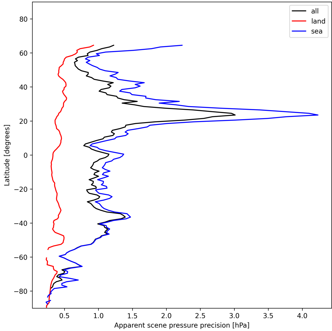
Figure 20: Zonal average of “Apparent scene pressure precision” for 2024-12-16 to 2024-12-17.
