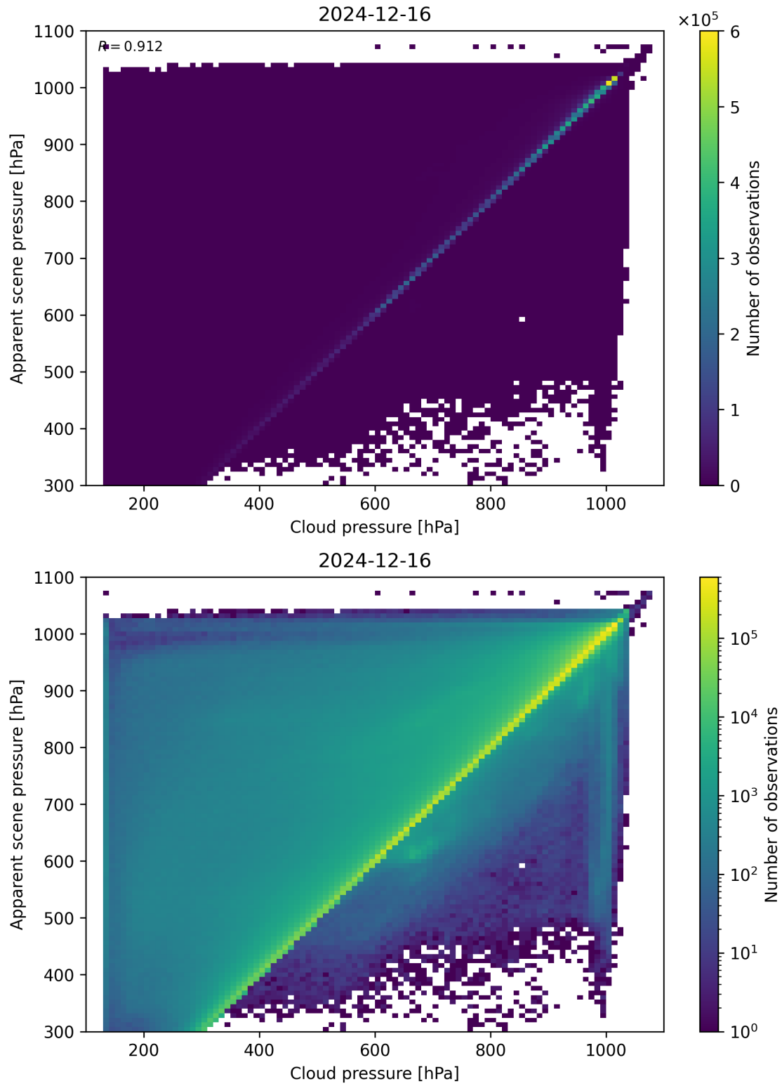
Figure 77: Scatter density plot of “Cloud pressure” against “Apparent scene pressure” for 2024-12-16 to 2024-12-17.
