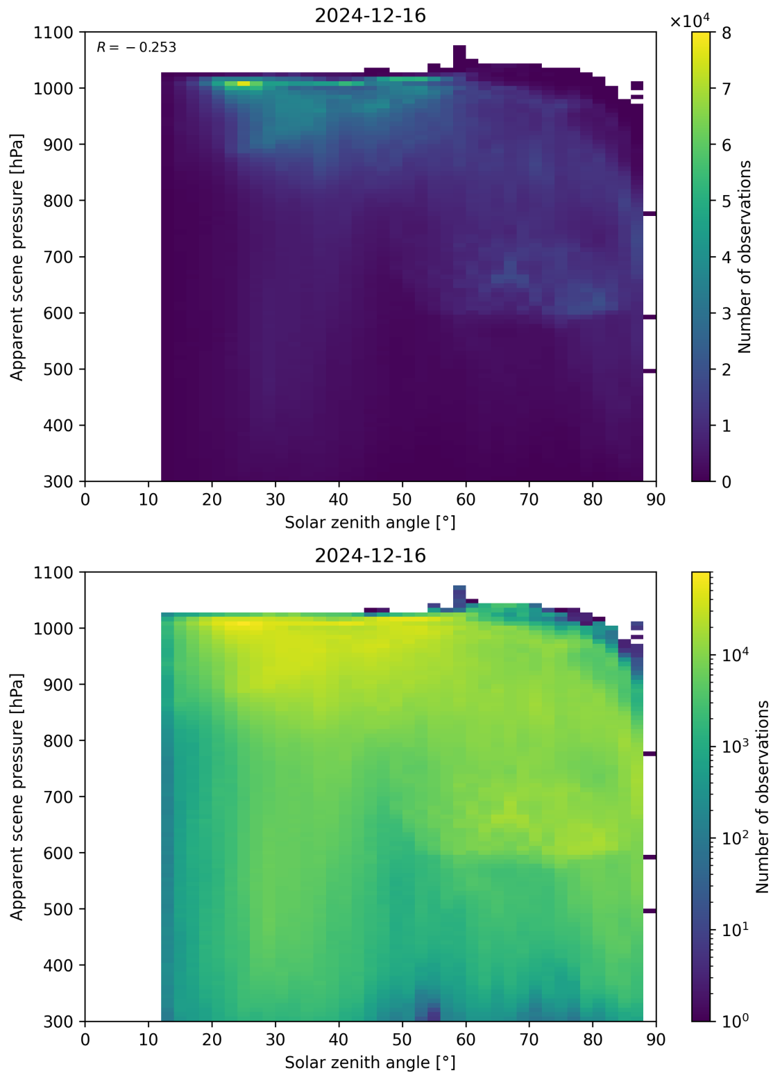
Figure 108: Scatter density plot of “Solar zenith angle” against “Apparent scene pressure” for 2024-12-16 to 2024-12-17.
