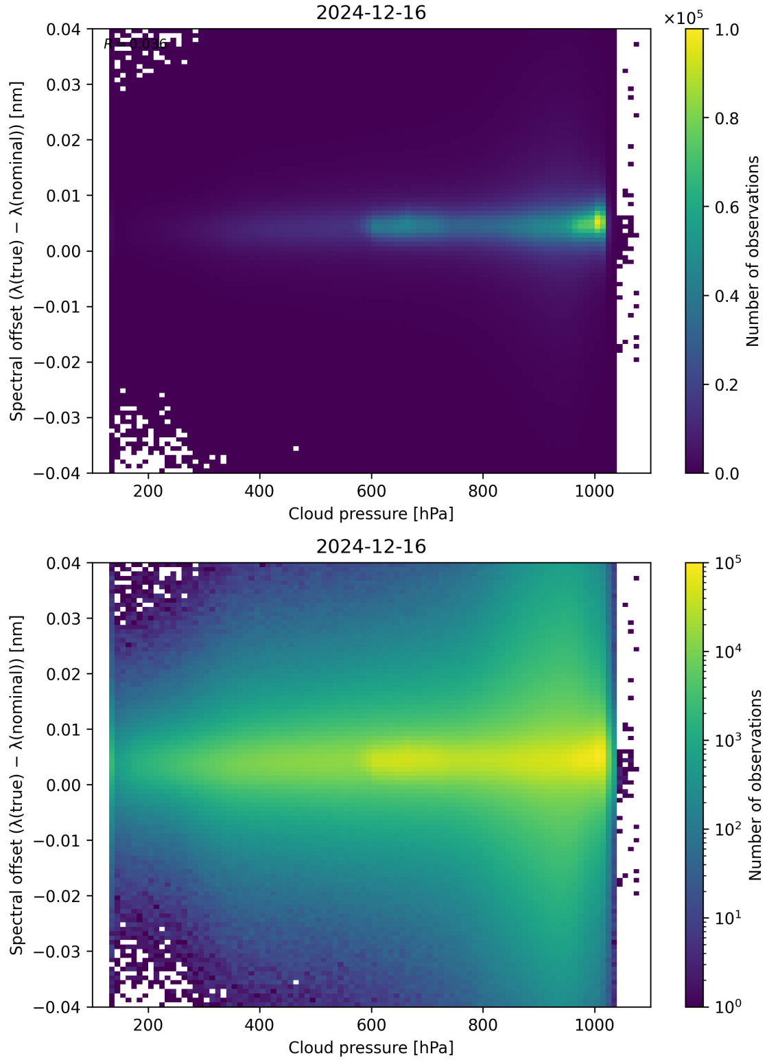
Figure 84: Scatter density plot of “Cloud pressure” against “Spectral offset ( \lambda_{\text{true}} - \lambda_{\text{nominal}} )” for 2024-12-16 to 2024-12-17.
