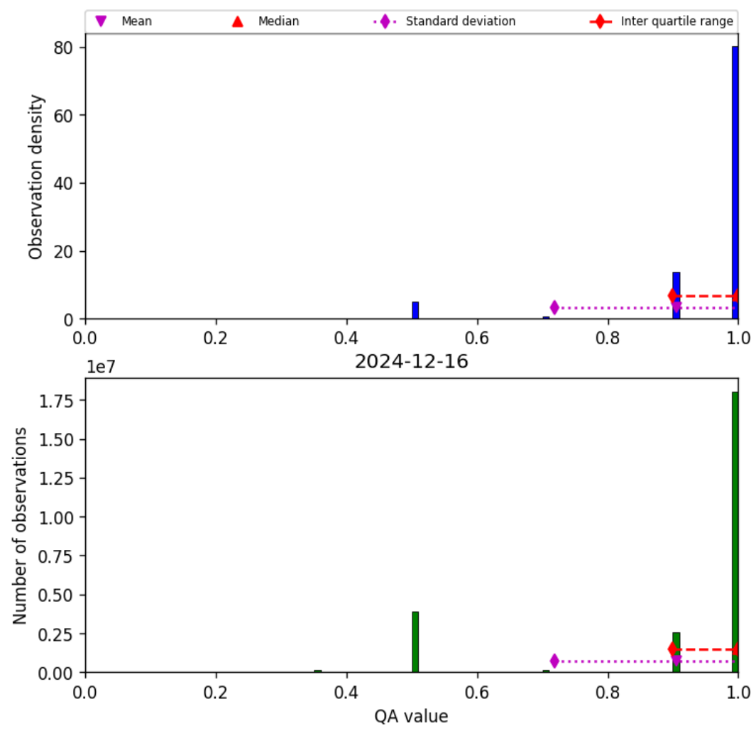
Figure 29: Histogram of “QA value” for 2024-12-16 to 2024-12-17
