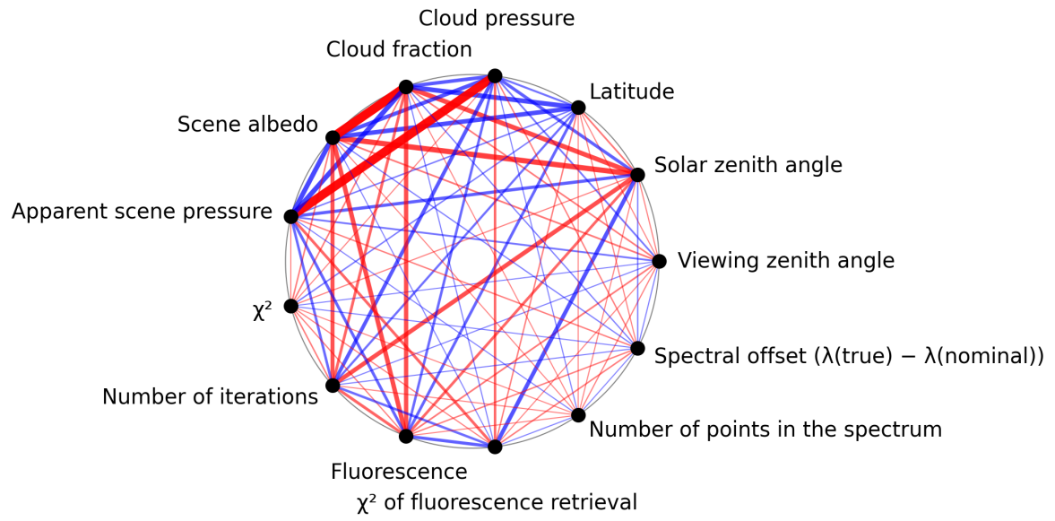
Figure 1: Map of correlation graph for 2024-12-16 to 2024-12-17.
