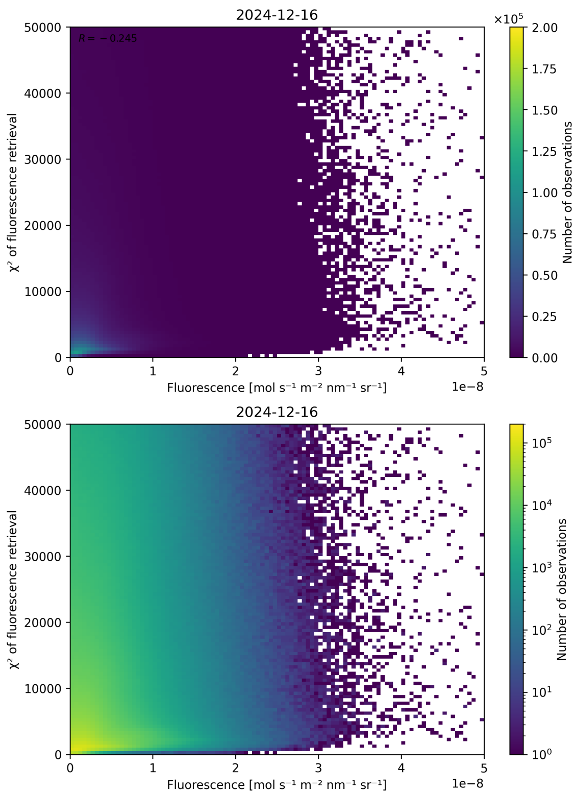
Figure 85: Scatter density plot of “Fluorescence” against “ \chi^2 of fluorescence retrieval” for 2024-12-16 to 2024-12-17.
