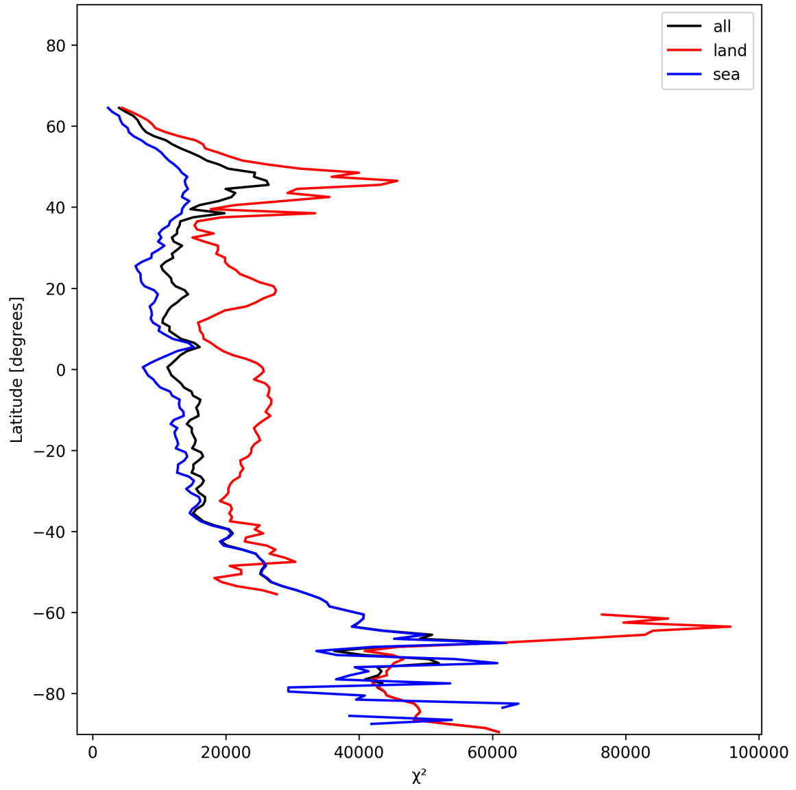
Figure 21: Zonal average of “ \chi^2 ” for 2024-12-16 to 2024-12-17.
