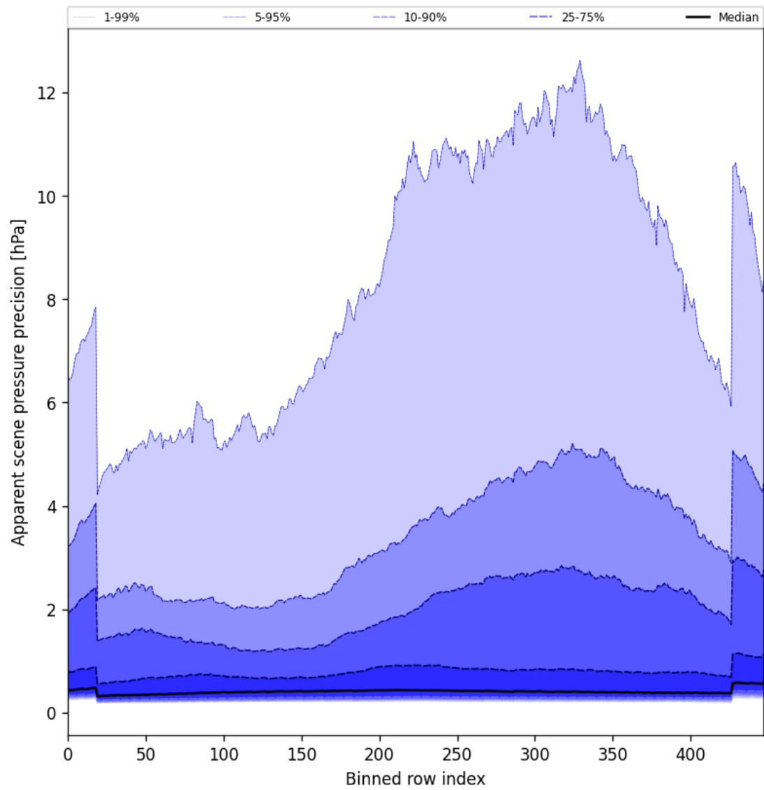
Figure 54: Along track statistics of “Apparent scene pressure precision” for 2024-12-16 to 2024-12-17
