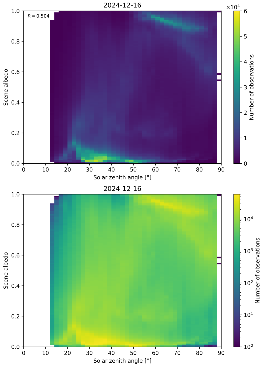
Figure 116: Scatter density plot of “Solar zenith angle” against “Scene albedo” for 2024-12-16 to 2024-12-17.
