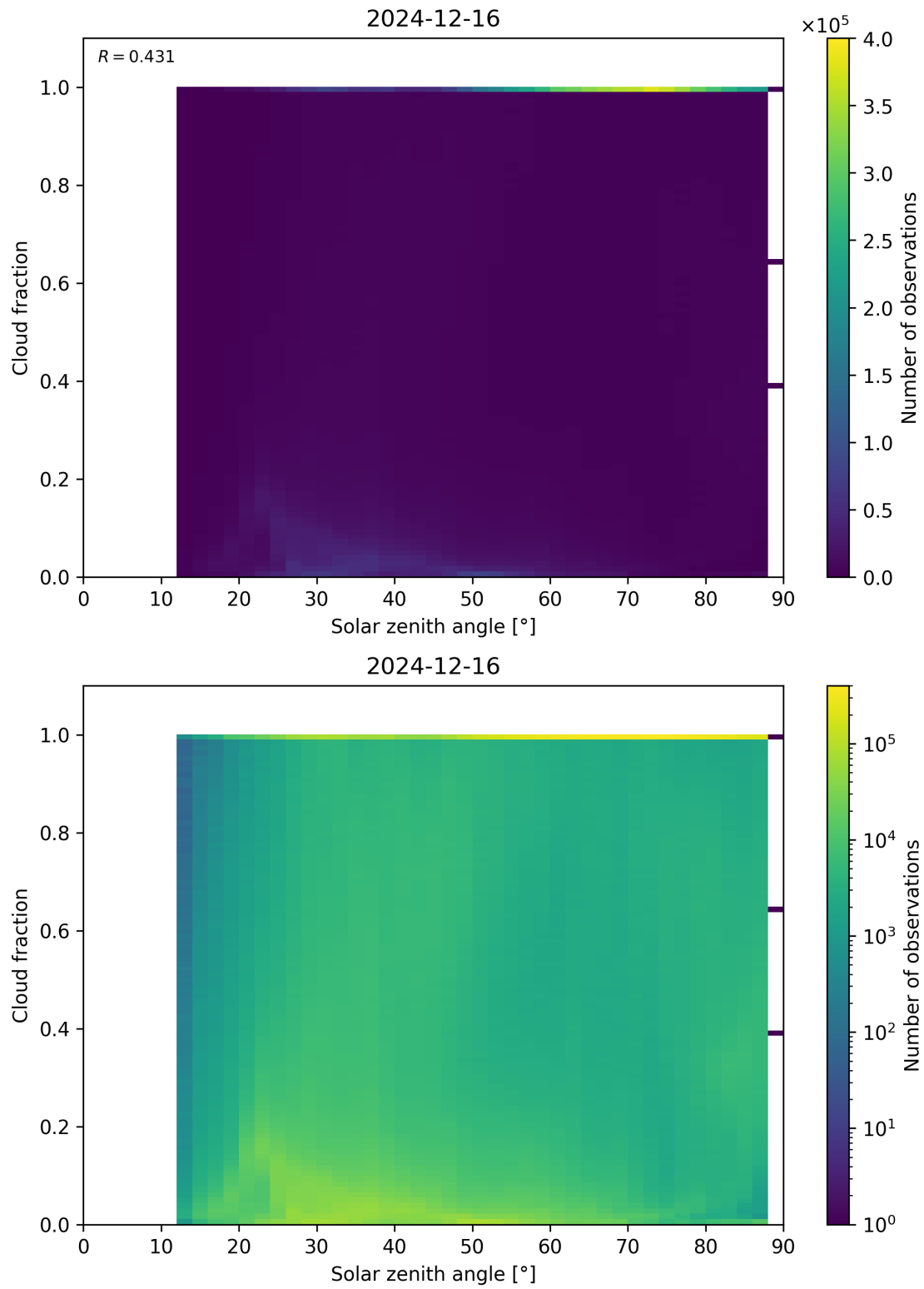
Figure 110: Scatter density plot of “Solar zenith angle” against “Cloud fraction” for 2024-12-16 to 2024-12-17.
