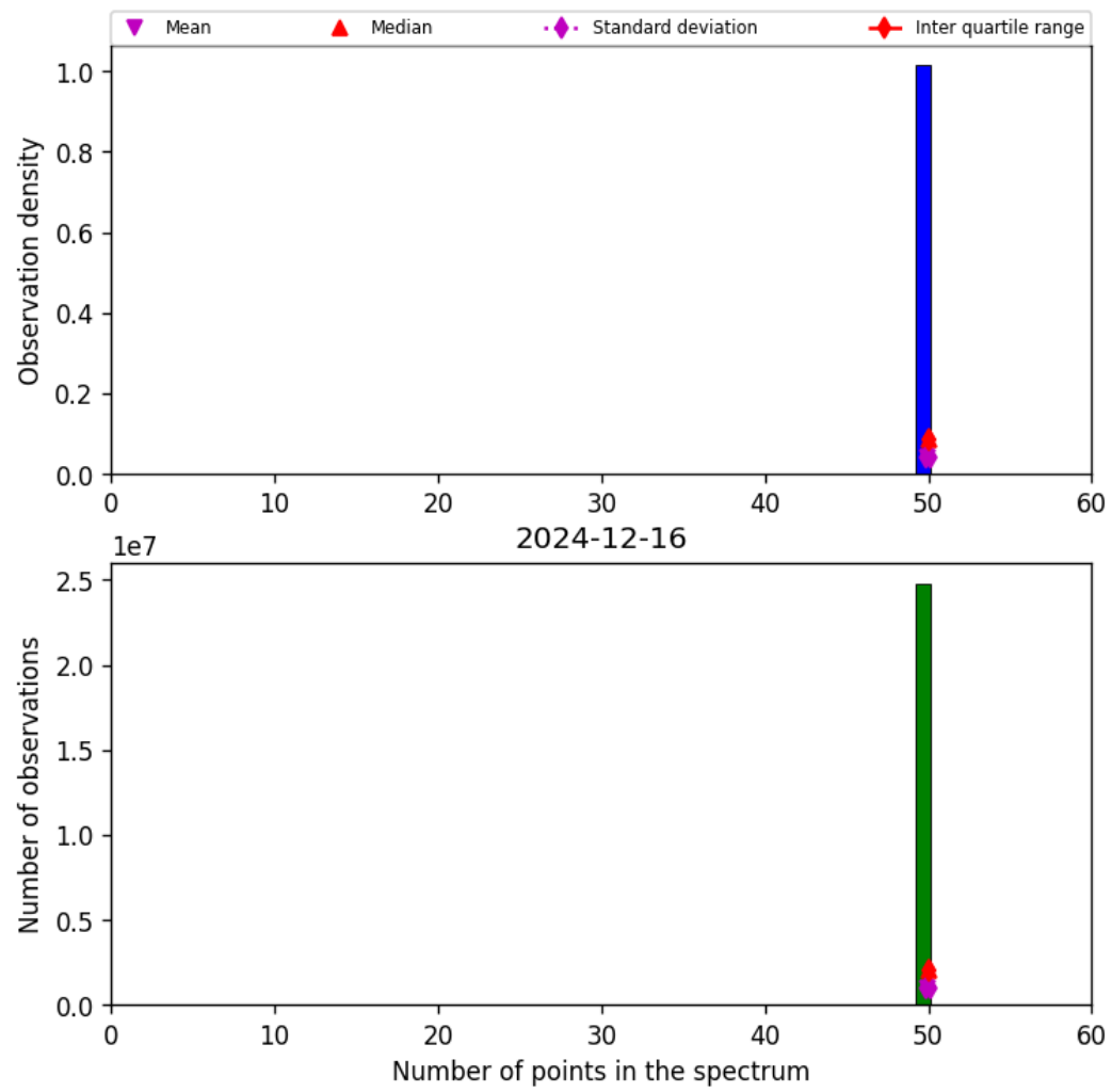
Figure 44: Histogram of “Number of points in the spectrum” for 2024-12-16 to 2024-12-17
