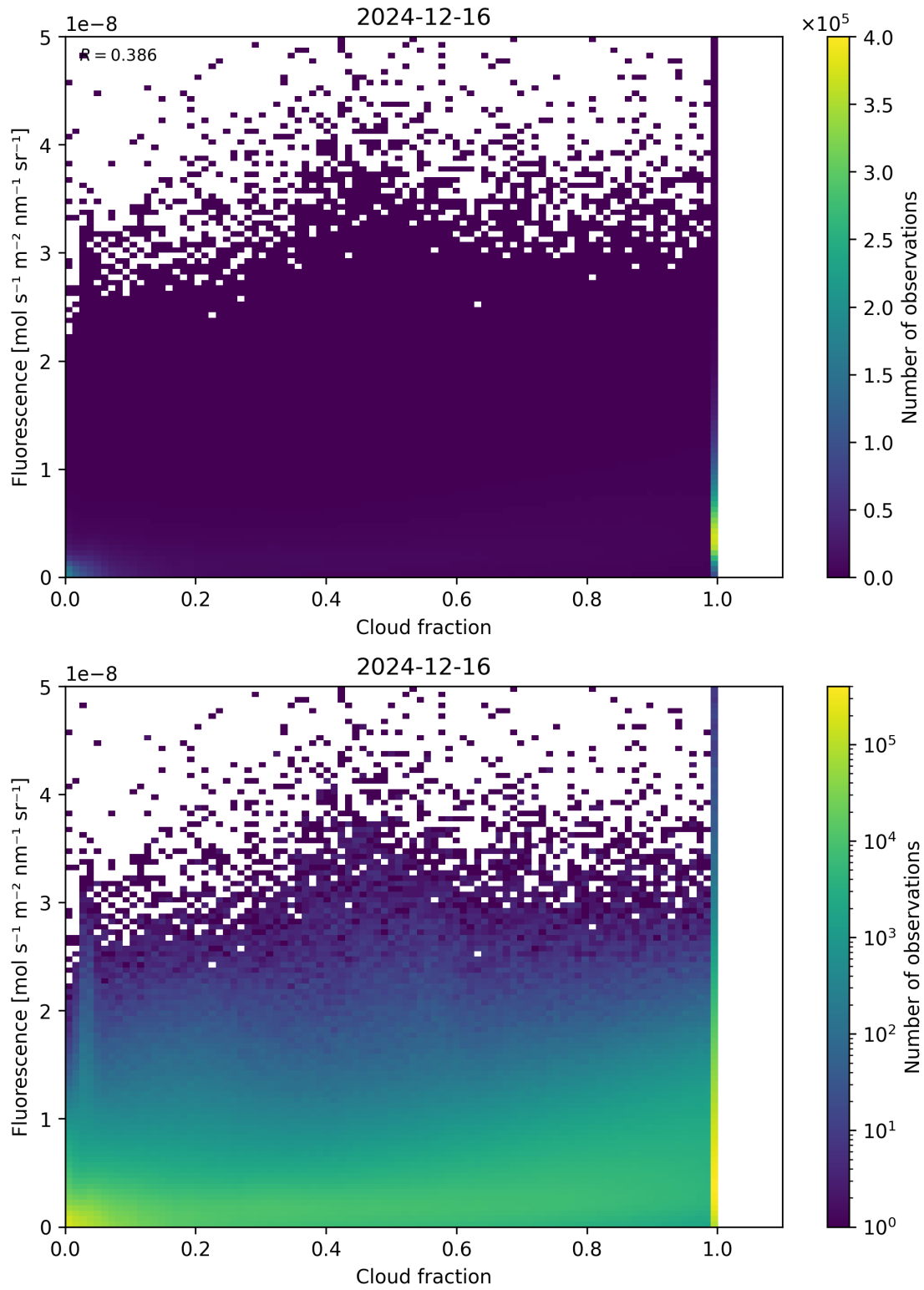
Figure 72: Scatter density plot of “Cloud fraction” against “Fluorescence” for 2024-12-16 to 2024-12-17.
