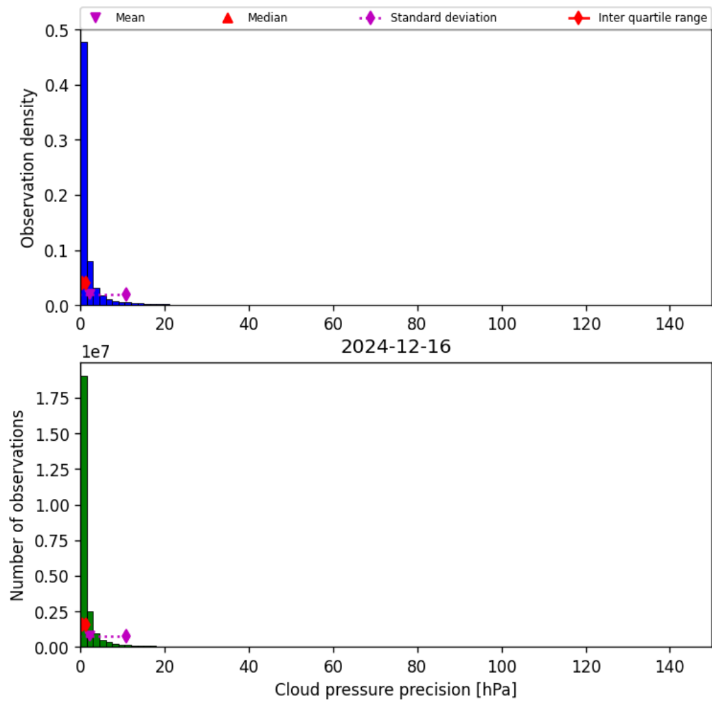
Figure 31: Histogram of “Cloud pressure precision” for 2024-12-16 to 2024-12-17
