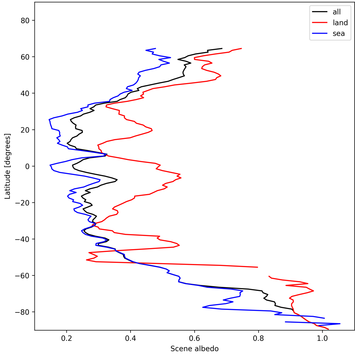
Figure 17: Zonal average of “Scene albedo” for 2024-12-16 to 2024-12-17.
