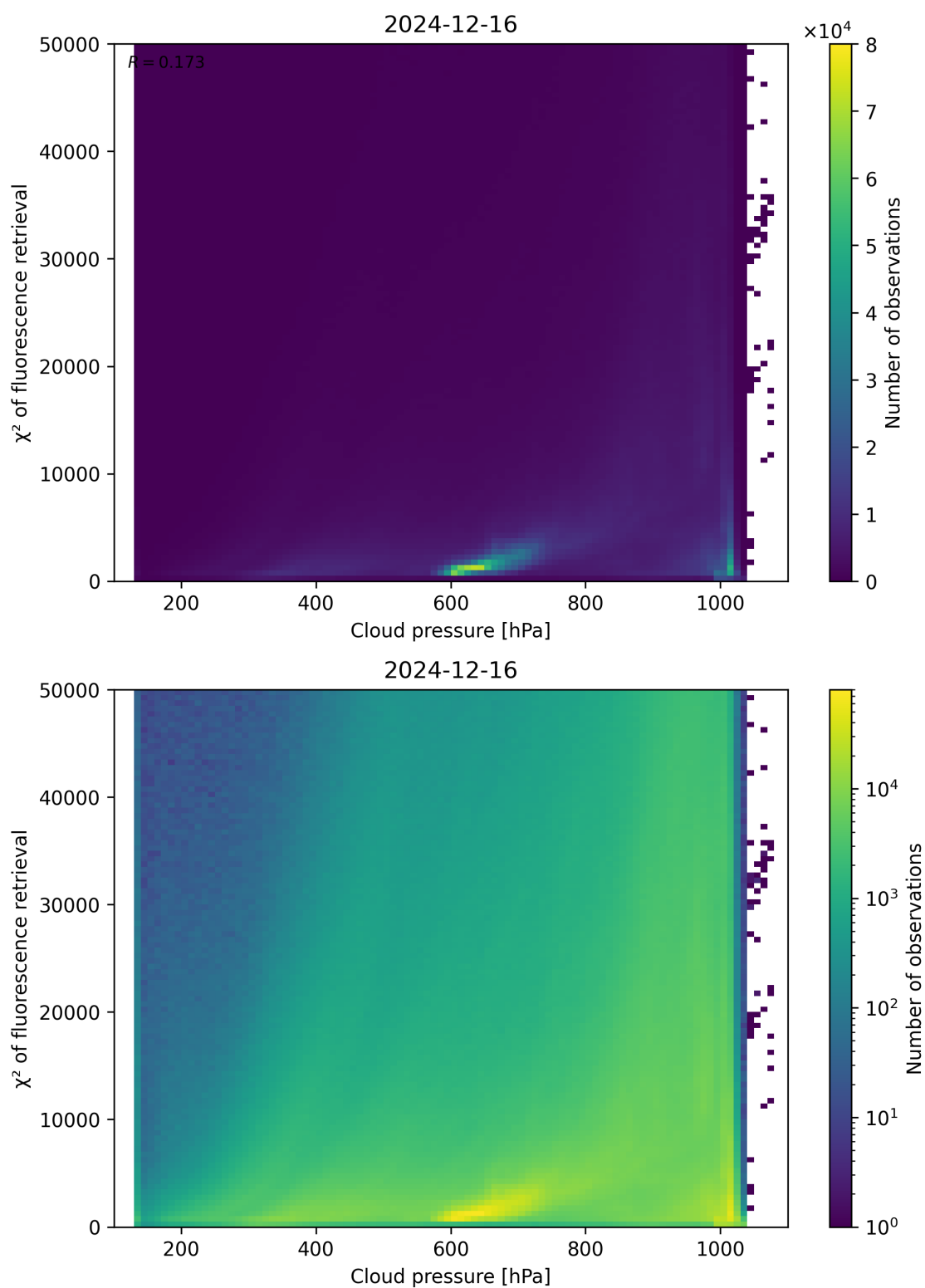
Figure 78: Scatter density plot of “Cloud pressure” against “ \chi^2 of fluorescence retrieval” for 2024-12-16 to 2024-12-17.
