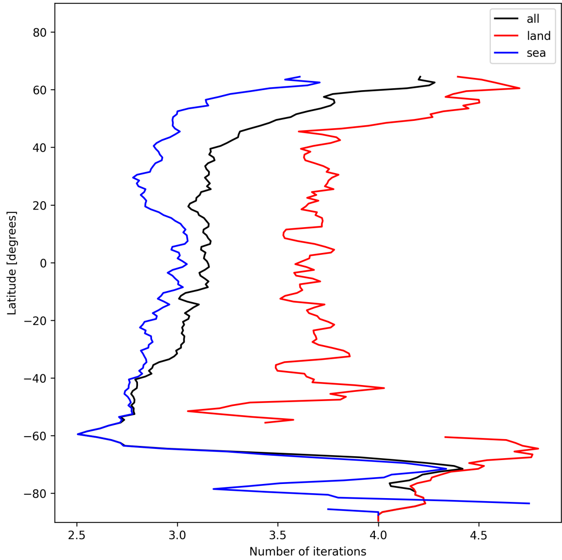
Figure 22: Zonal average of “Number of iterations” for 2024-12-16 to 2024-12-17.
