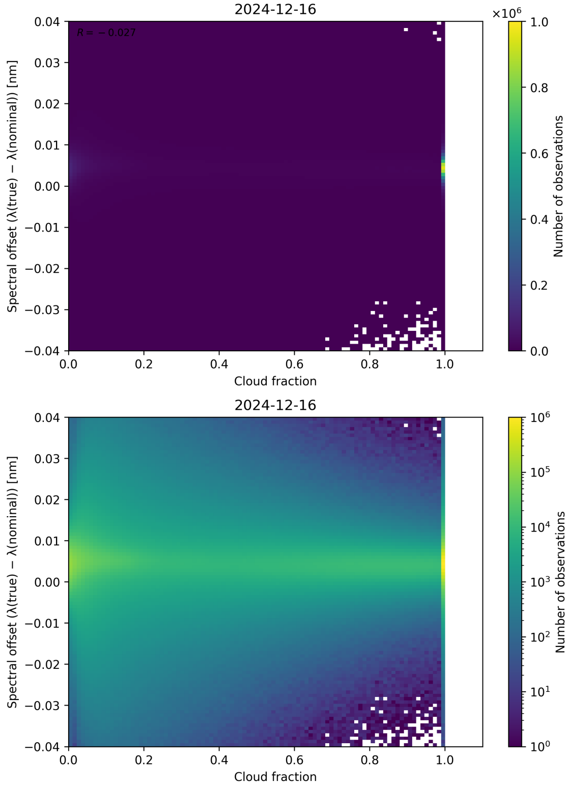
Figure 76: Scatter density plot of “Cloud fraction” against “Spectral offset ( \lambda_{\text{true}} - \lambda_{\text{nominal}} )” for 2024-12-16 to 2024-12-17.
