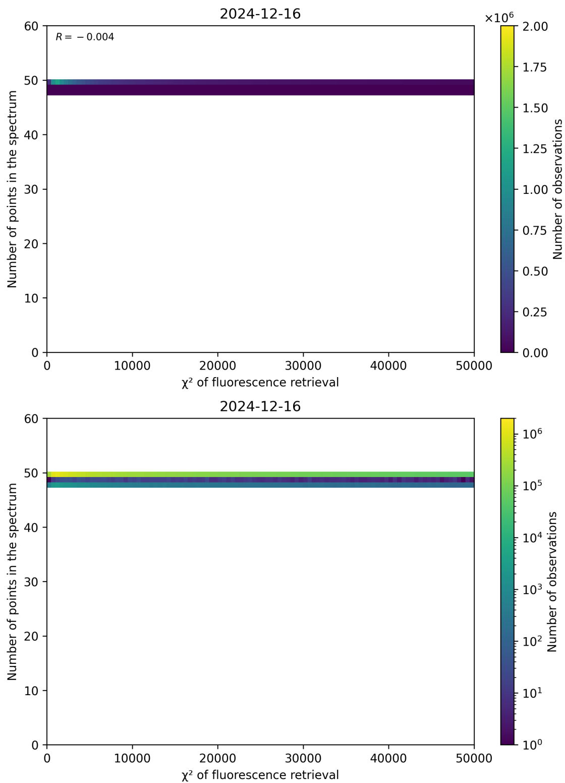
Figure 68: Scatter density plot of “ \chi^2 of fluorescence retrieval” against “Number of points in the spectrum” for 2024-12-16 to 2024-12-17.
