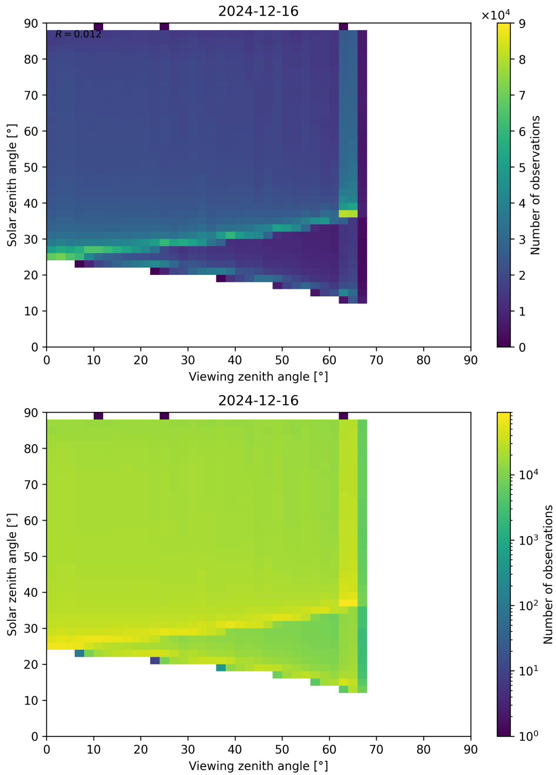
Figure 127: Scatter density plot of “Viewing zenith angle” against “Solar zenith angle” for 2024-12-16 to 2024-12-17.
