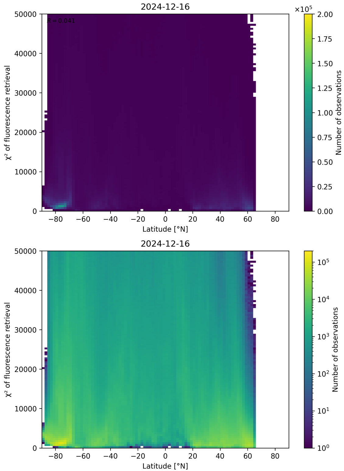
Figure 89: Scatter density plot of “Latitude” against “ \chi^2 of fluorescence retrieval” for 2024-12-16 to 2024-12-17.
