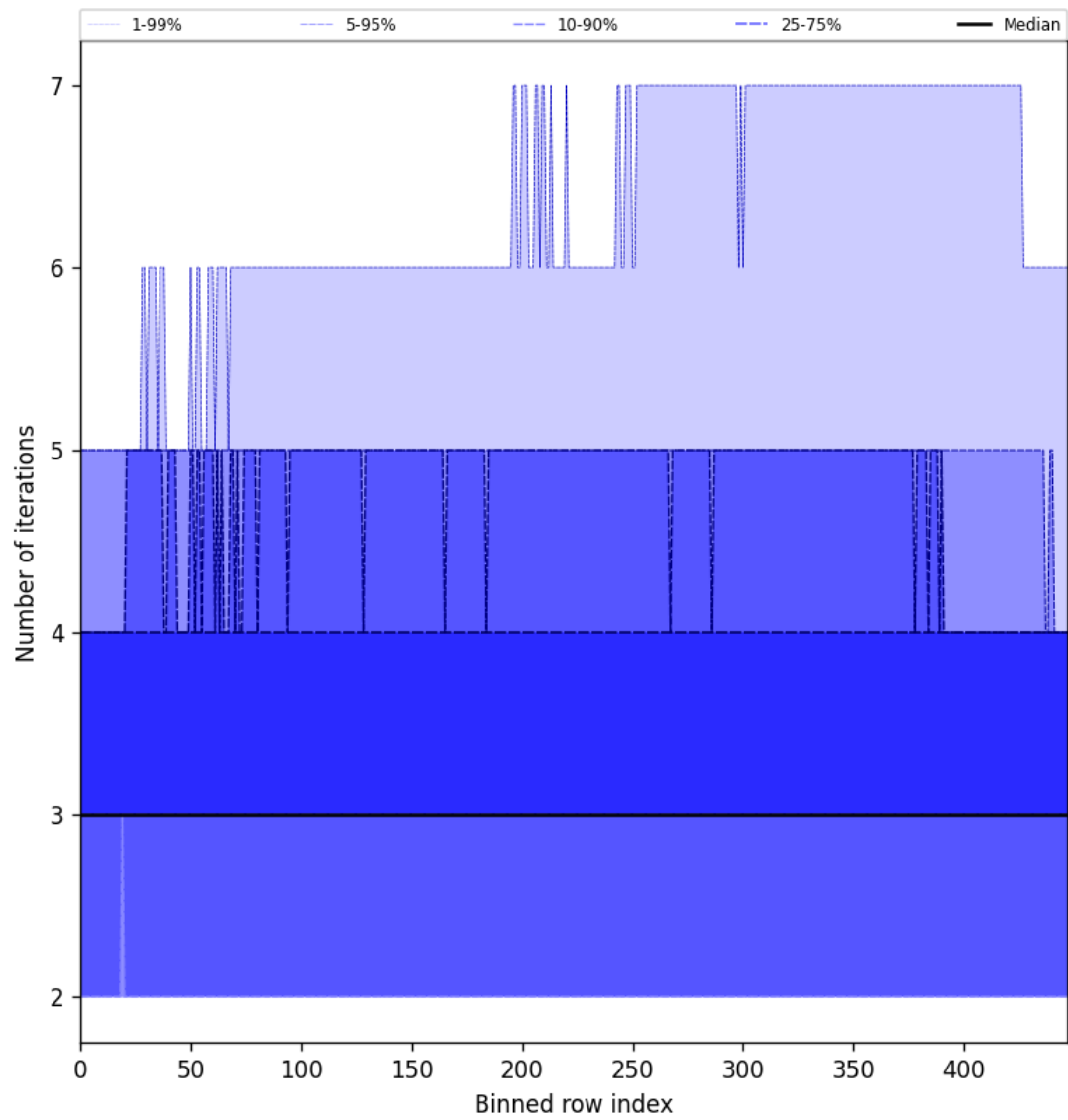
Figure 56: Along track statistics of “Number of iterations” for 2024-12-16 to 2024-12-17
