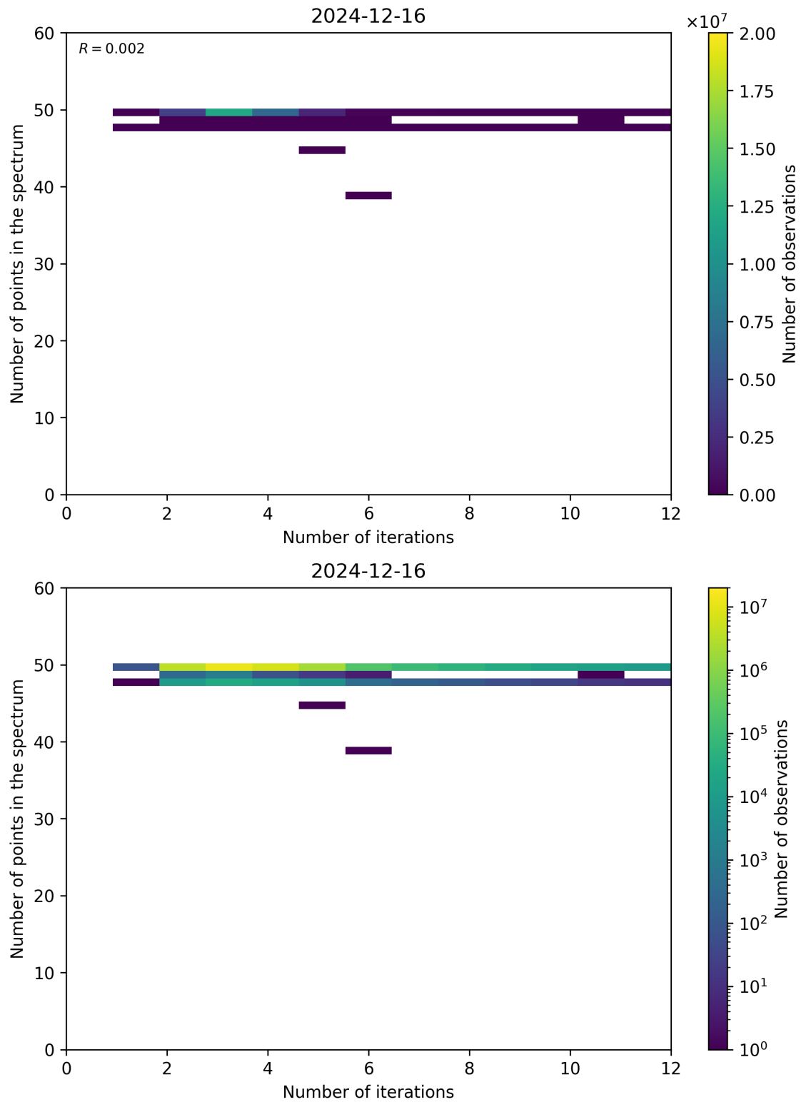
Figure 99: Scatter density plot of “Number of iterations” against “Number of points in the spectrum” for 2024-12-16 to 2024-12-17.
