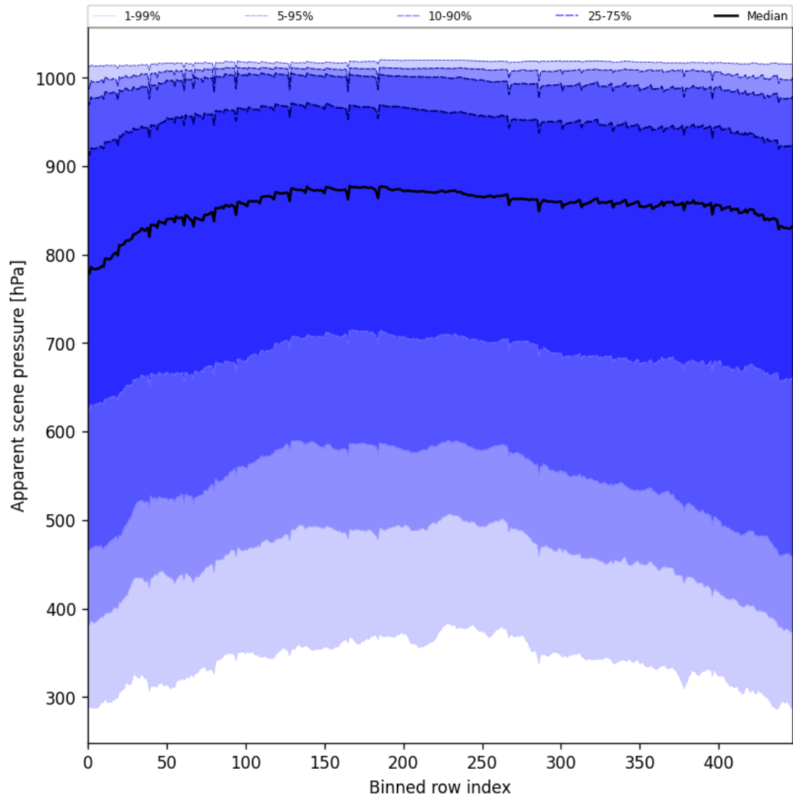
Figure 53: Along track statistics of “Apparent scene pressure” for 2024-12-16 to 2024-12-17
