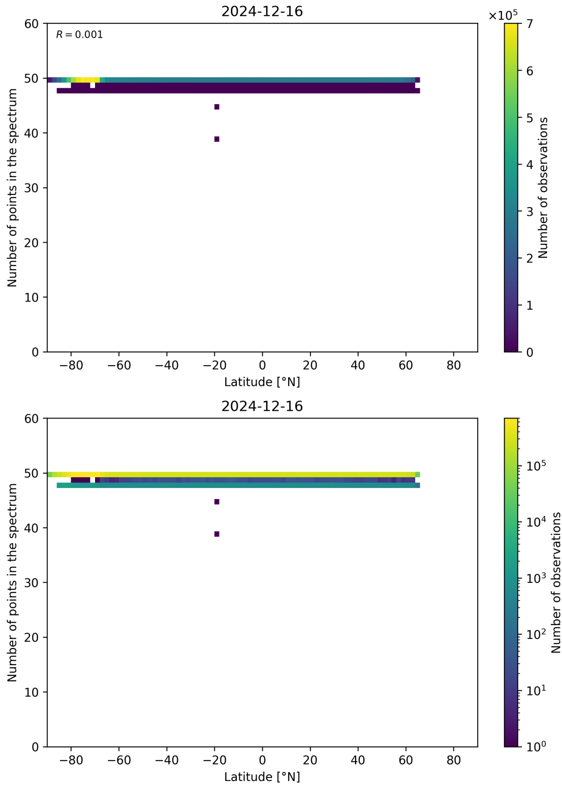
Figure 94: Scatter density plot of “Latitude” against “Number of points in the spectrum” for 2024-12-16 to 2024-12-17.
