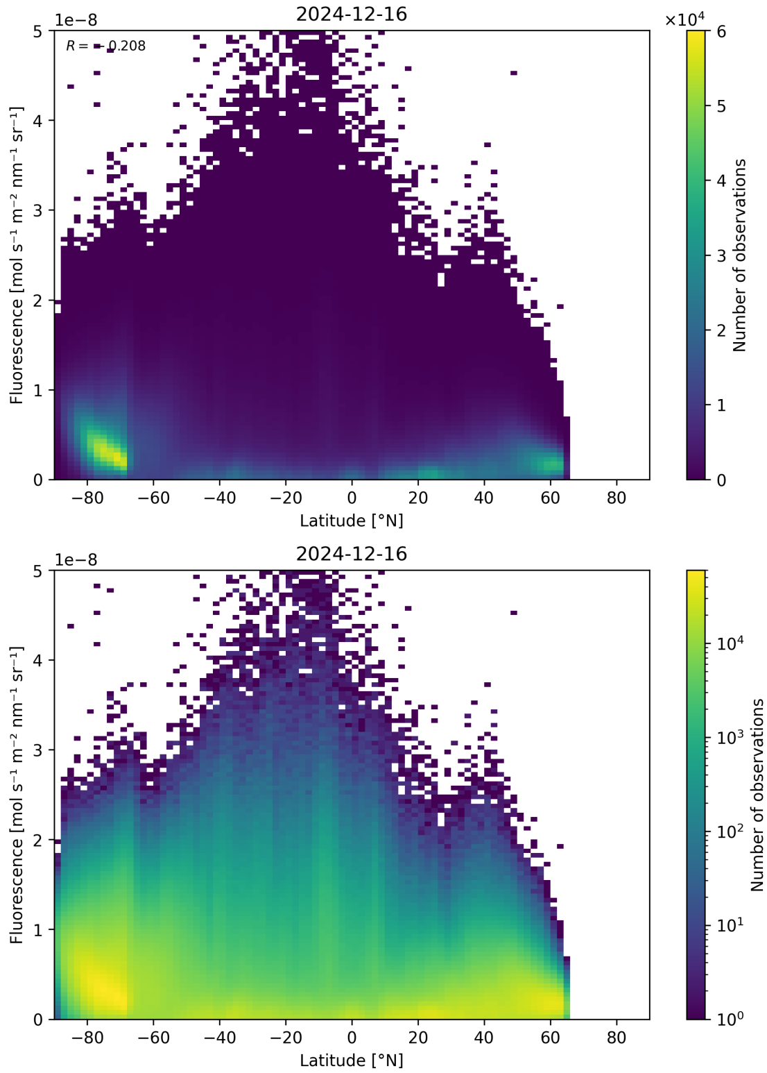
Figure 92: Scatter density plot of “Latitude” against “Fluorescence” for 2024-12-16 to 2024-12-17.
