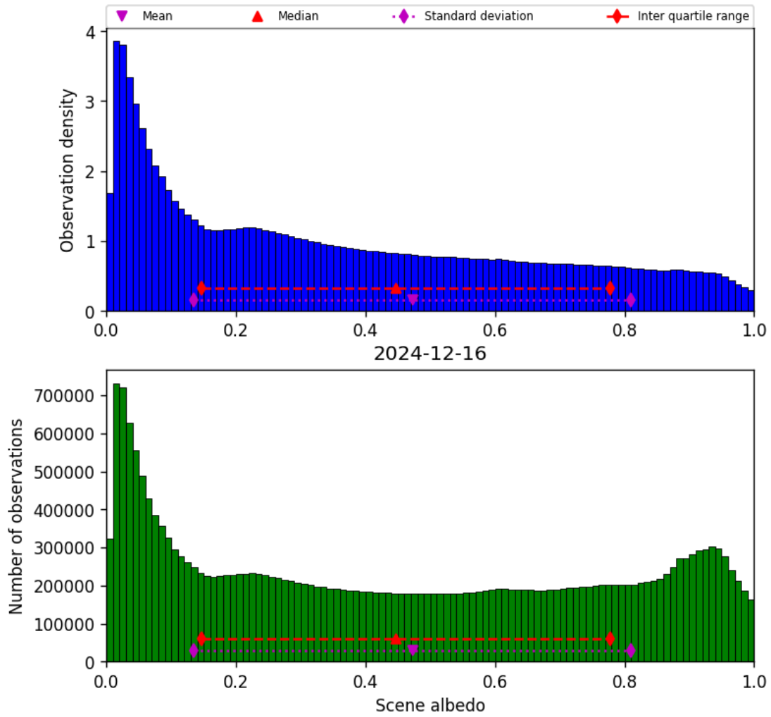
Figure 34: Histogram of “Scene albedo” for 2024-12-16 to 2024-12-17
