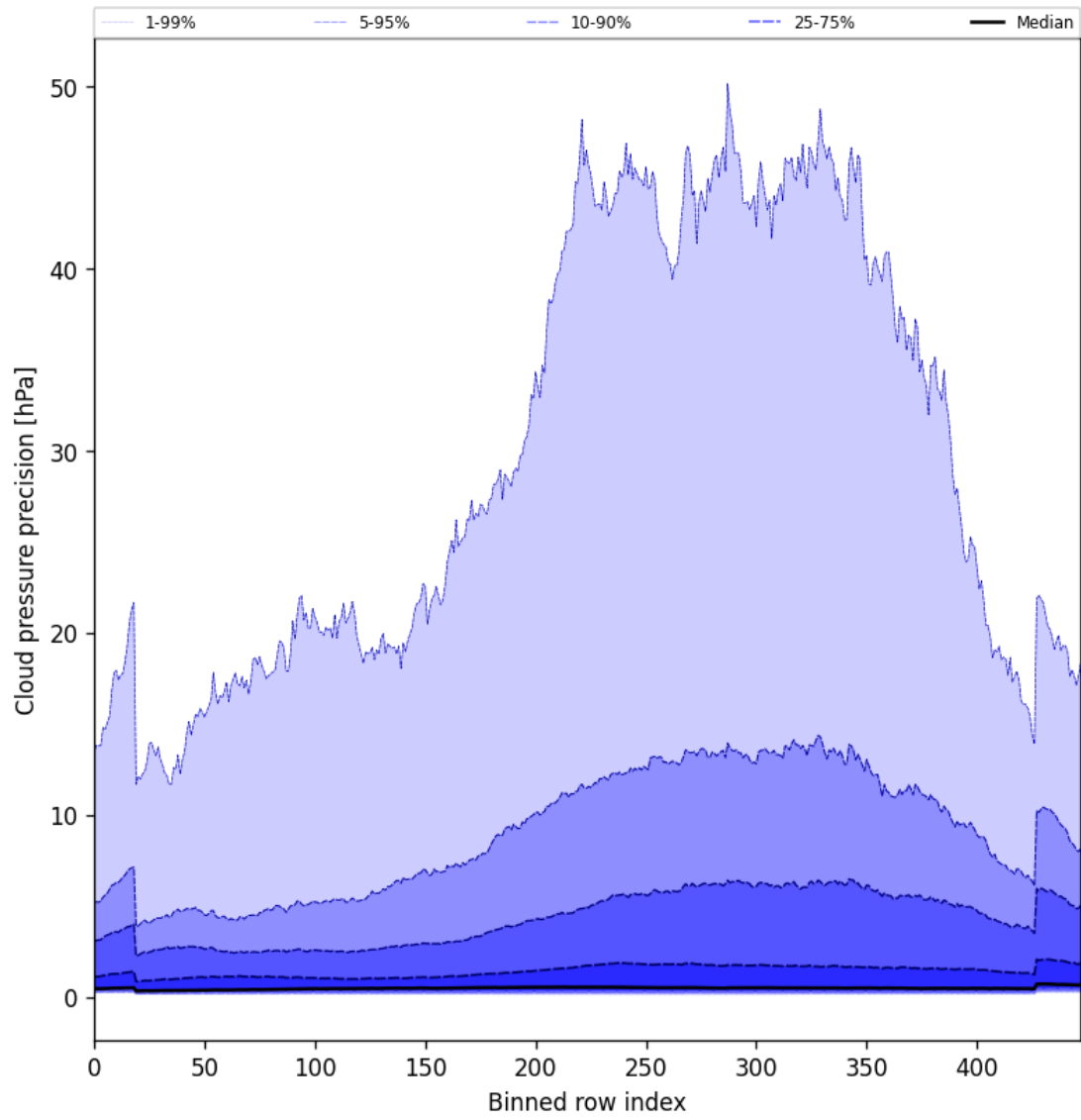
Figure 48: Along track statistics of “Cloud pressure precision” for 2024-12-16 to 2024-12-17
