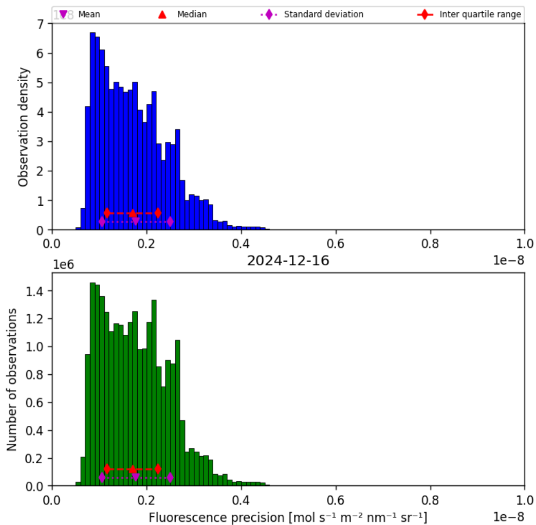
Figure 41: Histogram of “Fluorescence precision” for 2024-12-16 to 2024-12-17
