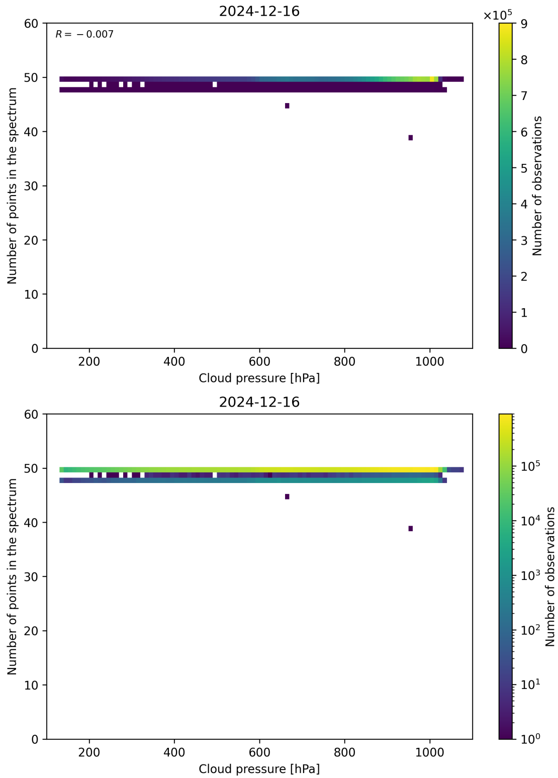
Figure 82: Scatter density plot of “Cloud pressure” against “Number of points in the spectrum” for 2024-12-16 to 2024-12-17.
