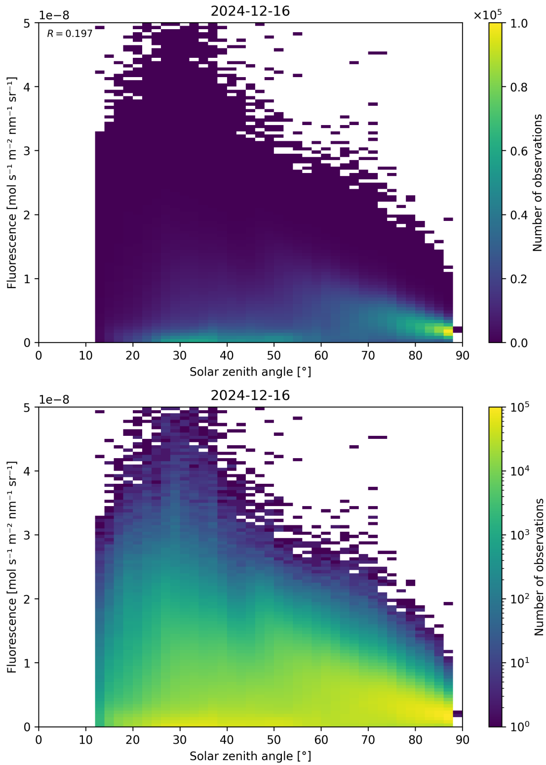
Figure 112: Scatter density plot of “Solar zenith angle” against “Fluorescence” for 2024-12-16 to 2024-12-17.
