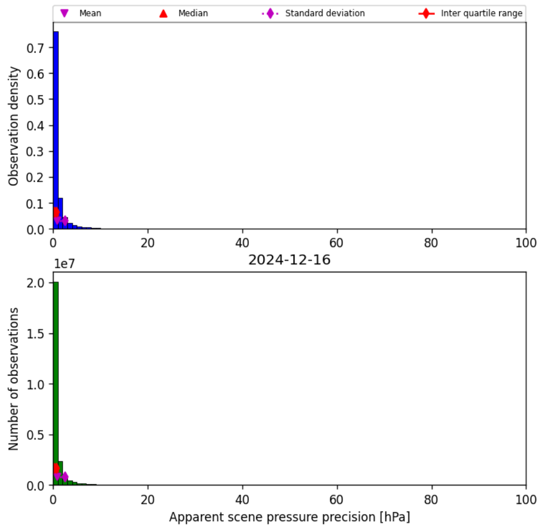
Figure 37: Histogram of “Apparent scene pressure precision” for 2024-12-16 to 2024-12-17
