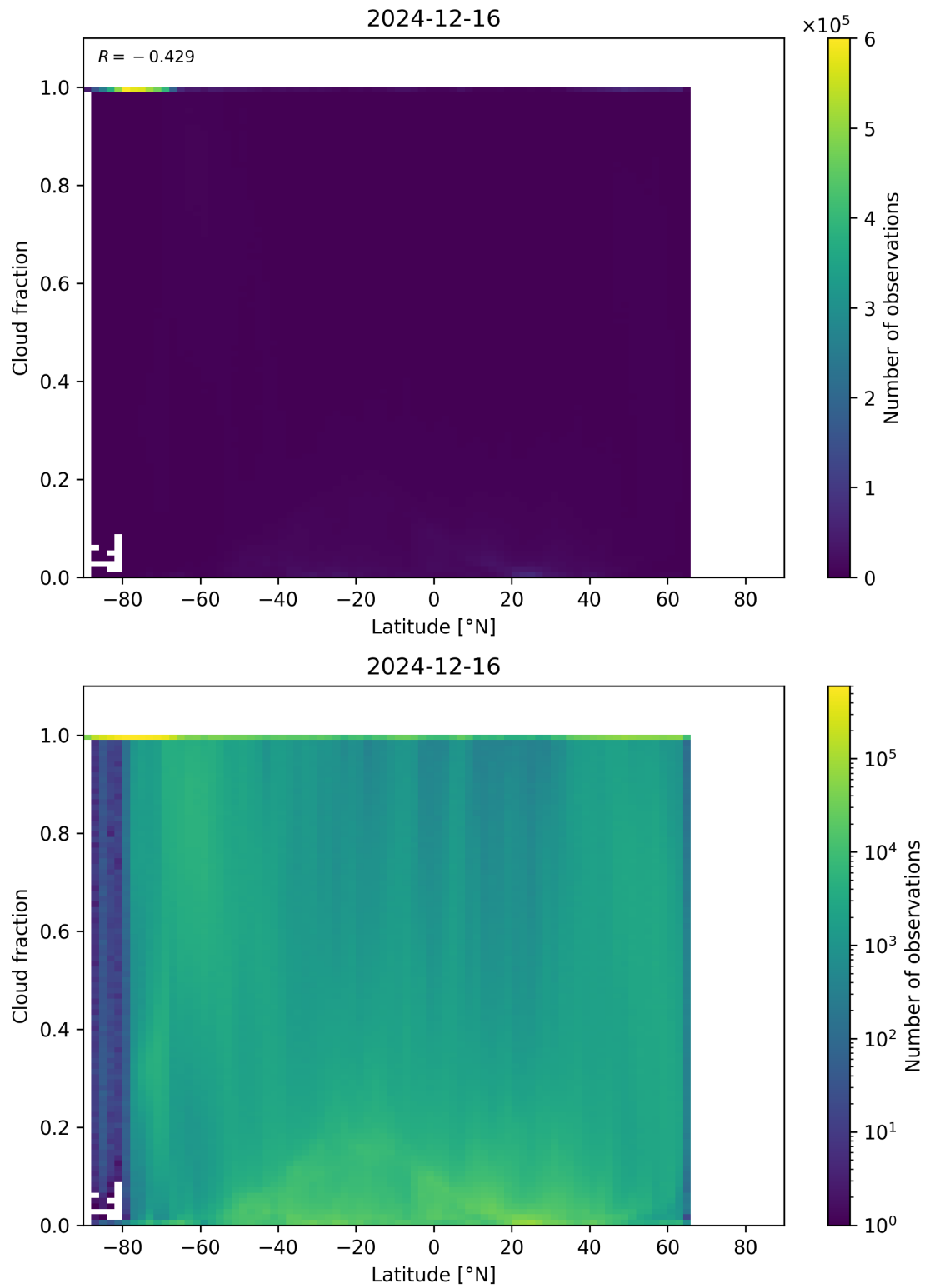
Figure 90: Scatter density plot of “Latitude” against “Cloud fraction” for 2024-12-16 to 2024-12-17.
