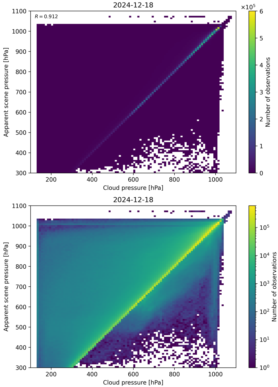
Figure 77: Scatter density plot of “Cloud pressure” against “Apparent scene pressure” for 2024-12-17 to 2024-12-19.
