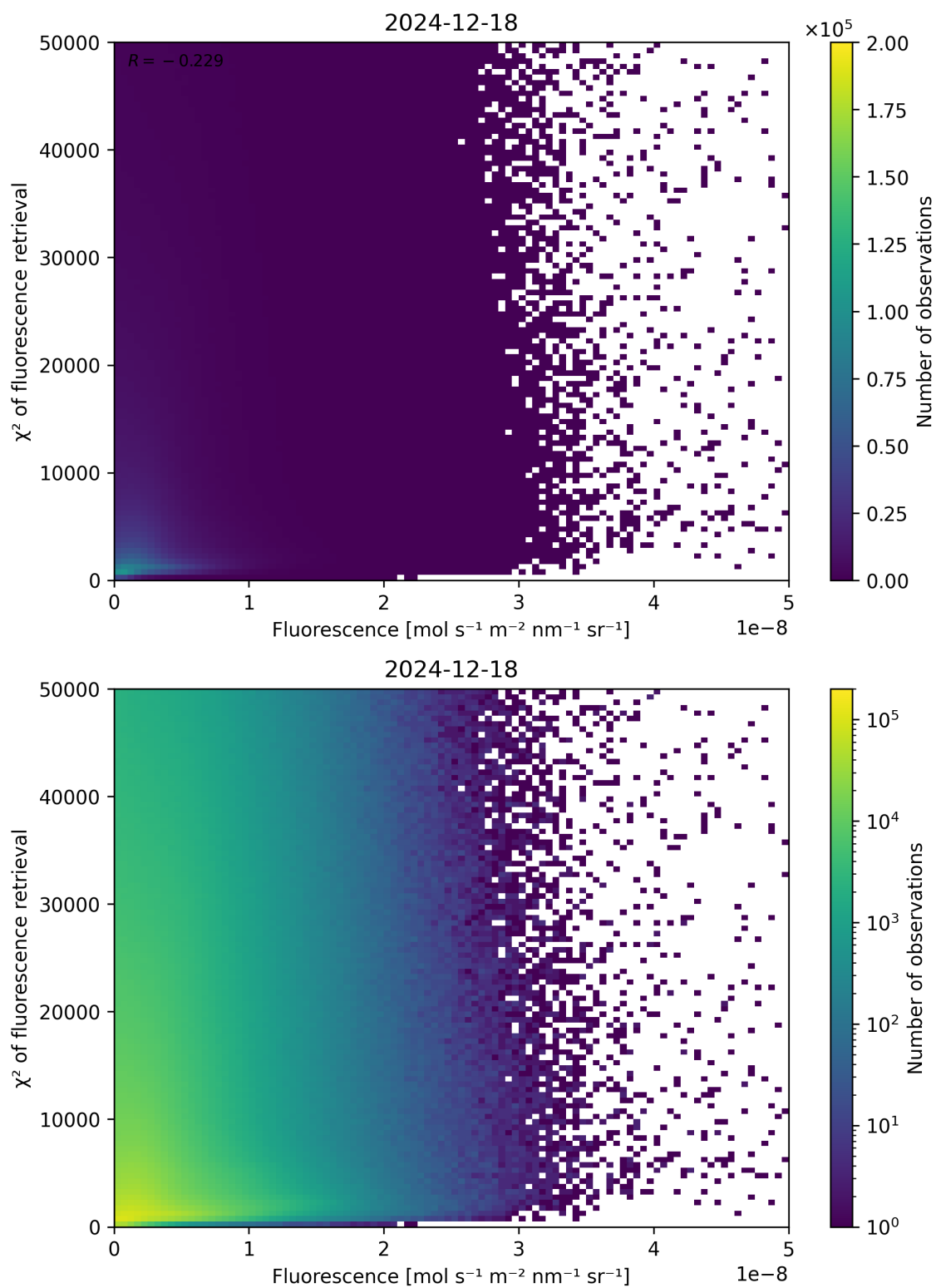
Figure 85: Scatter density plot of “Fluorescence” against “ \chi^2 of fluorescence retrieval” for 2024-12-17 to 2024-12-19.
