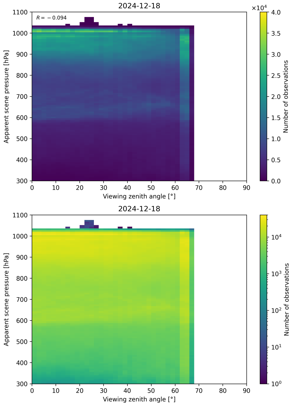
Figure 118: Scatter density plot of “Viewing zenith angle” against “Apparent scene pressure” for 2024-12-17 to 2024-12-19.
