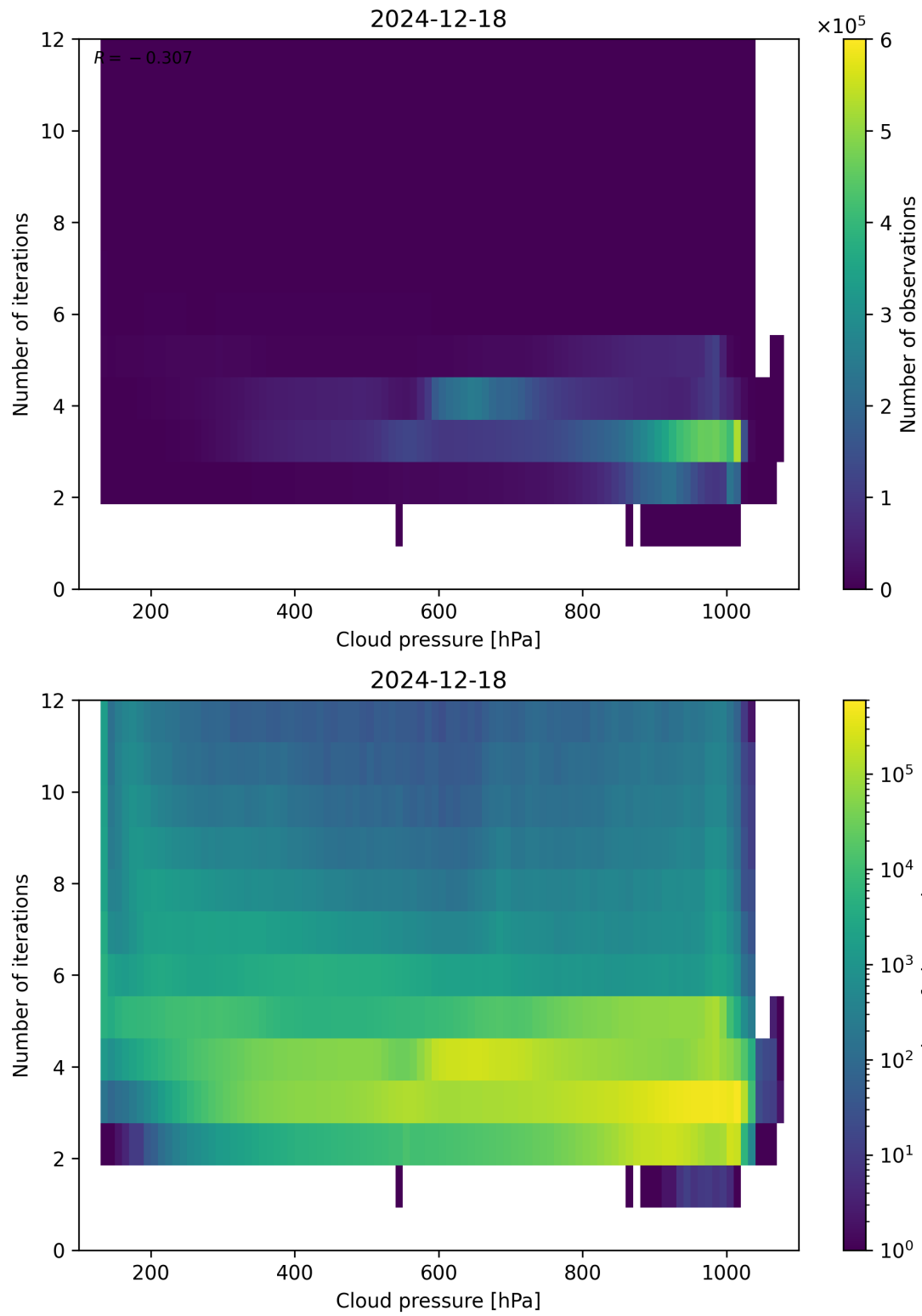
Figure 81: Scatter density plot of “Cloud pressure” against “Number of iterations” for 2024-12-17 to 2024-12-19.
