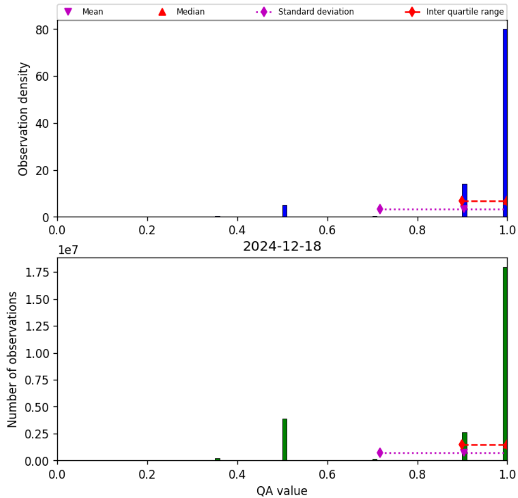
Figure 29: Histogram of “QA value” for 2024-12-17 to 2024-12-19
