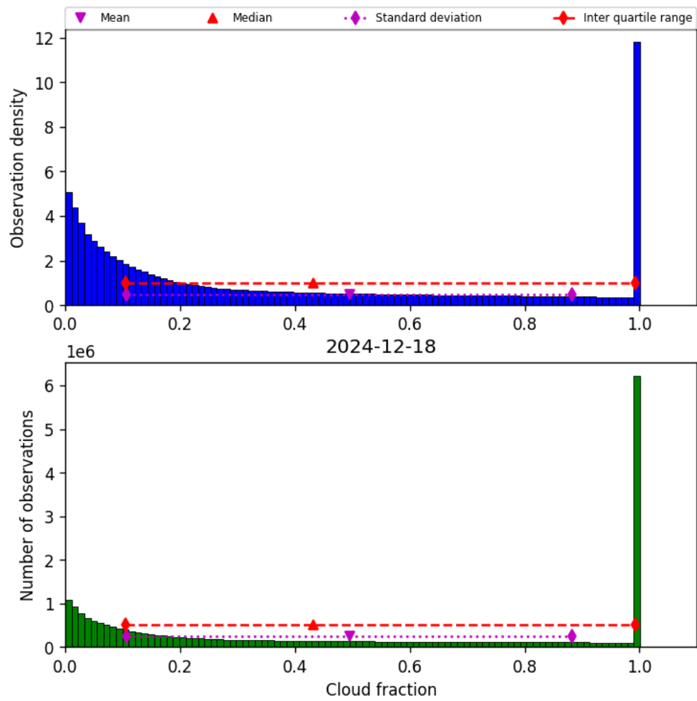
Figure 32: Histogram of “Cloud fraction” for 2024-12-17 to 2024-12-19
