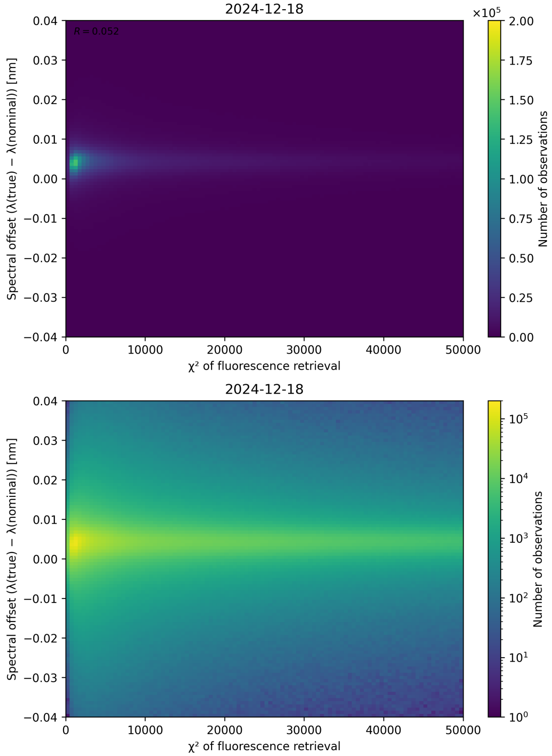
Figure 69: Scatter density plot of “ \chi^2 of fluorescence retrieval” against “Spectral offset ( \lambda_{\text{true}} - \lambda_{\text{nominal}} )” for 2024-12-17 to 2024-12-19.
