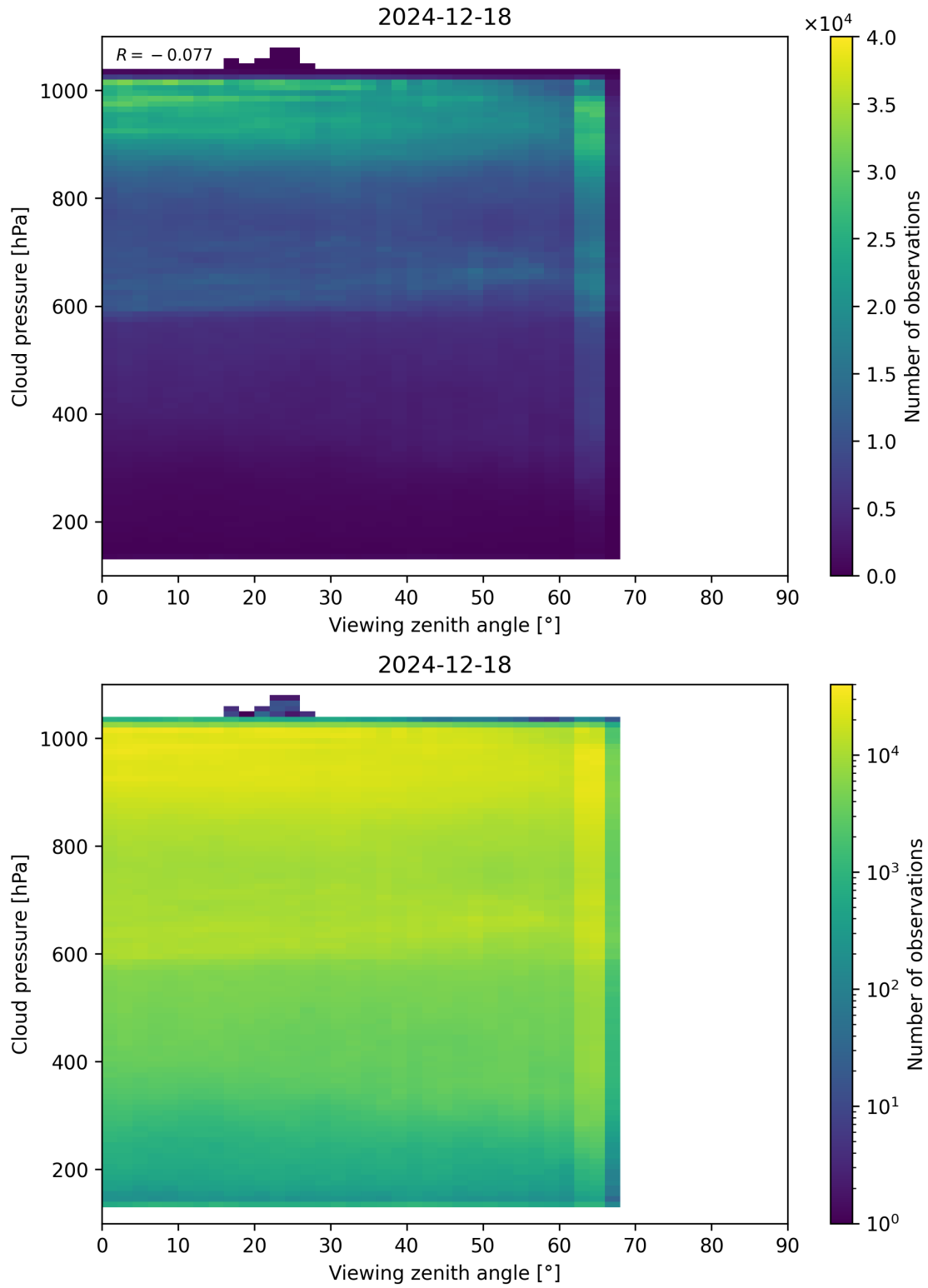
Figure 121: Scatter density plot of “Viewing zenith angle” against “Cloud pressure” for 2024-12-17 to 2024-12-19.
