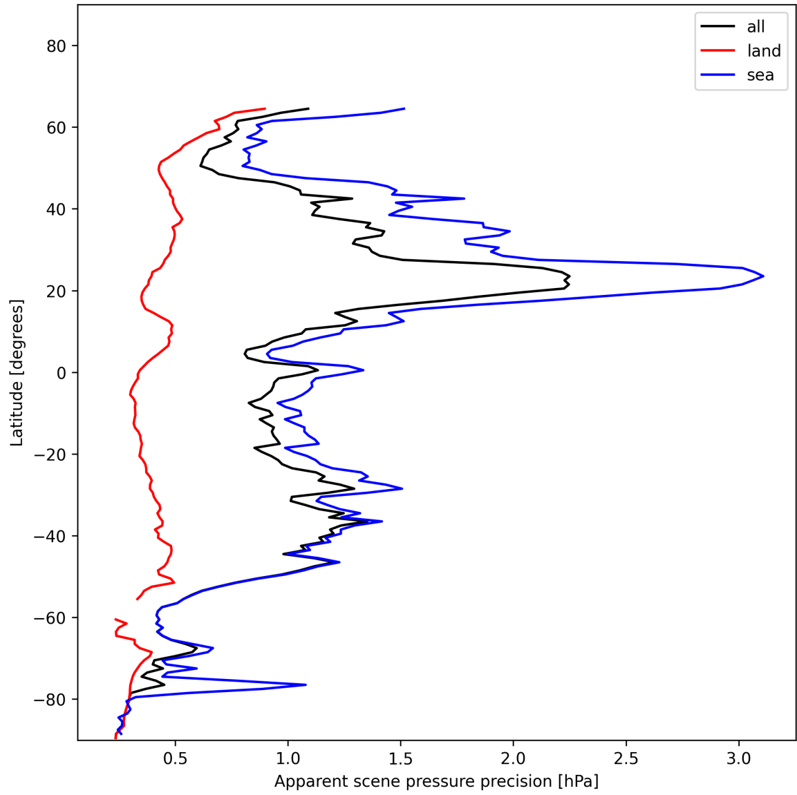
Figure 20: Zonal average of “Apparent scene pressure precision” for 2024-12-17 to 2024-12-19.
