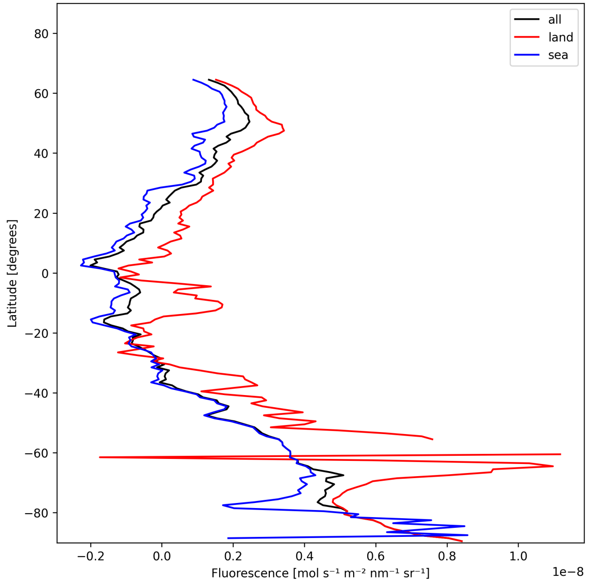
Figure 23: Zonal average of “Fluorescence” for 2024-12-17 to 2024-12-19.
