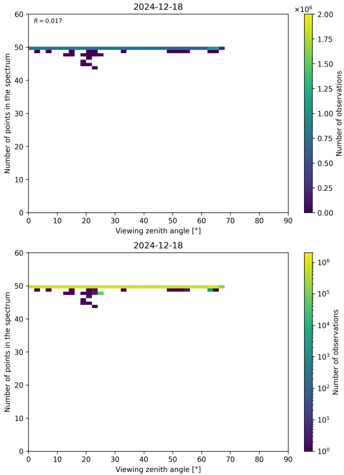
Figure 125: Scatter density plot of “Viewing zenith angle” against “Number of points in the spectrum” for 2024-12-17 to 2024-12-19.
