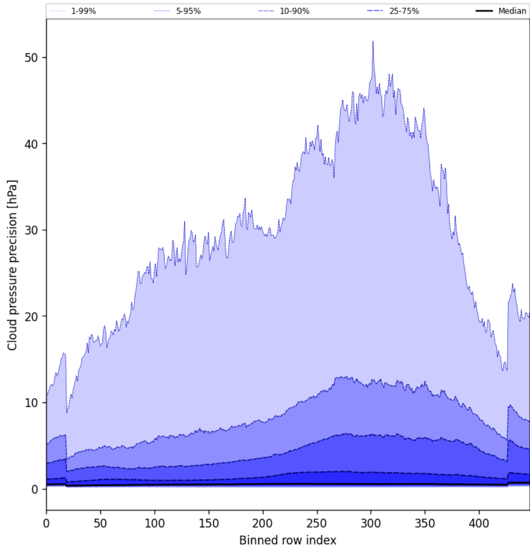
Figure 48: Along track statistics of “Cloud pressure precision” for 2024-12-17 to 2024-12-19
