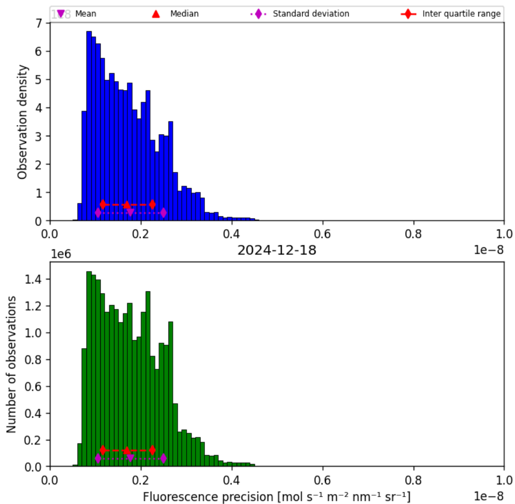
Figure 41: Histogram of “Fluorescence precision” for 2024-12-17 to 2024-12-19
