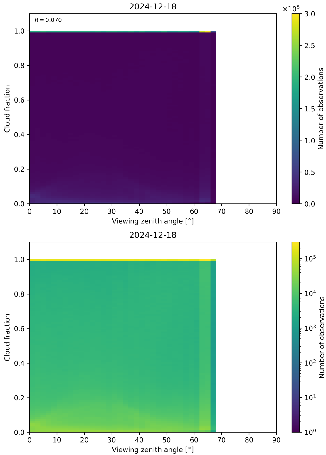
Figure 120: Scatter density plot of “Viewing zenith angle” against “Cloud fraction” for 2024-12-17 to 2024-12-19.
