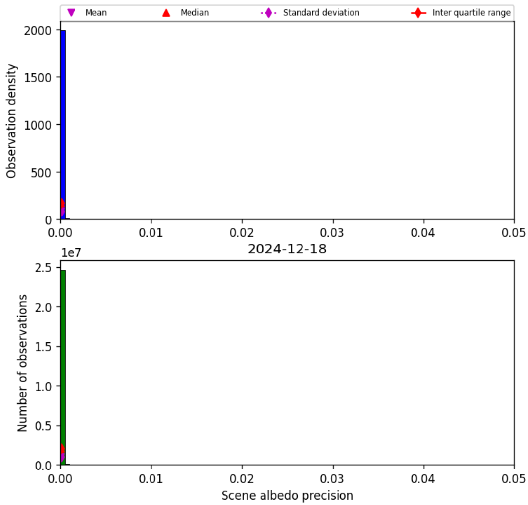
Figure 35: Histogram of “Scene albedo precision” for 2024-12-17 to 2024-12-19
