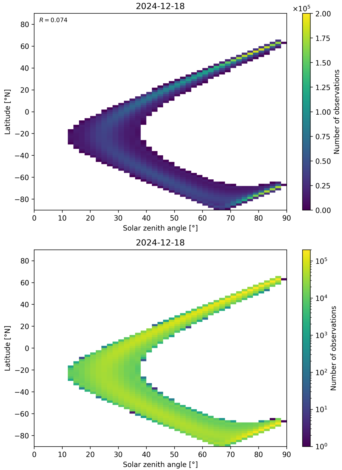
Figure 113: Scatter density plot of “Solar zenith angle” against “Latitude” for 2024-12-17 to 2024-12-19.
