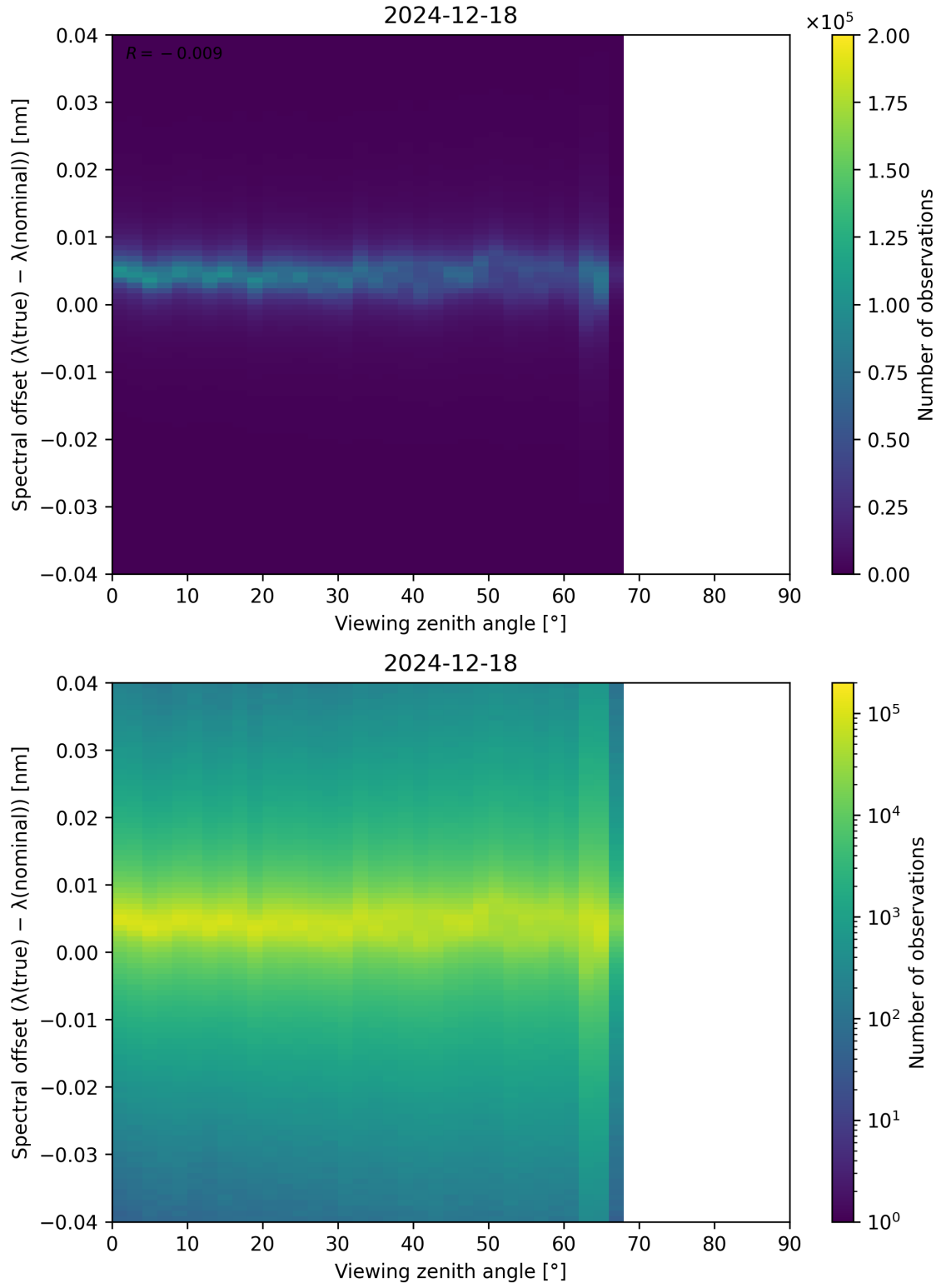
Figure 128: Scatter density plot of “Viewing zenith angle” against “Spectral offset ( \lambda_{\text{true}} - \lambda_{\text{nominal}} )” for 2024-12-17 to 2024-12-19.
