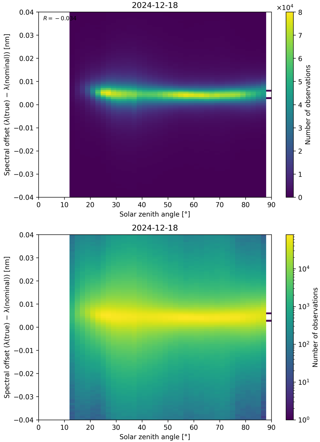
Figure 117: Scatter density plot of “Solar zenith angle” against “Spectral offset ( \lambda_{\text{true}} - \lambda_{\text{nominal}} )” for 2024-12-17 to 2024-12-19.
