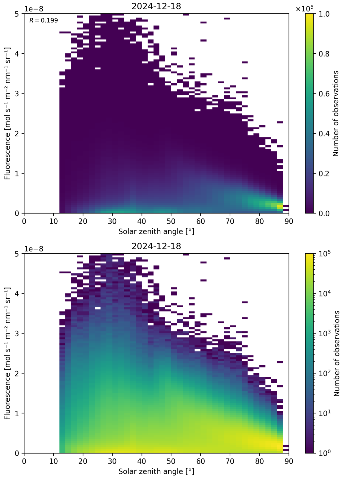
Figure 112: Scatter density plot of “Solar zenith angle” against “Fluorescence” for 2024-12-17 to 2024-12-19.
