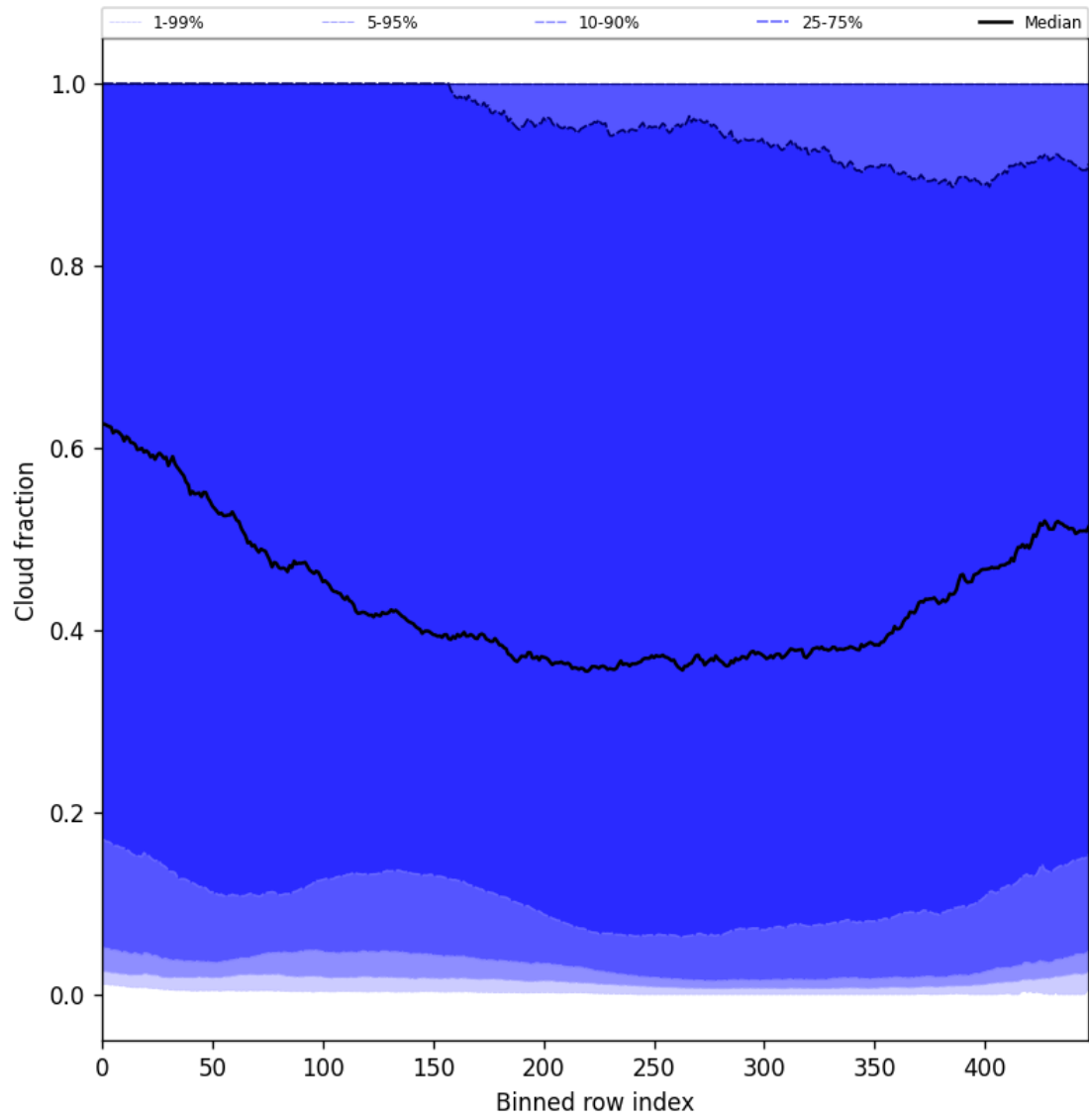
Figure 49: Along track statistics of “Cloud fraction” for 2024-12-17 to 2024-12-19
