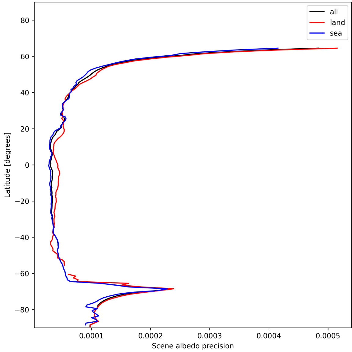
Figure 18: Zonal average of “Scene albedo precision” for 2024-12-17 to 2024-12-19.
