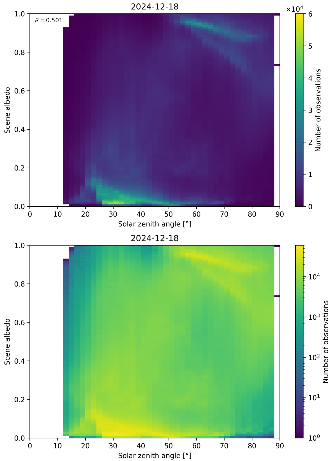
Figure 116: Scatter density plot of “Solar zenith angle” against “Scene albedo” for 2024-12-17 to 2024-12-19.
