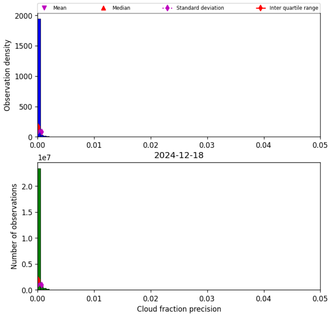
Figure 33: Histogram of “Cloud fraction precision” for 2024-12-17 to 2024-12-19
