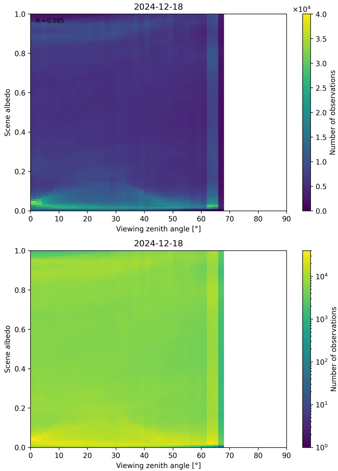
Figure 126: Scatter density plot of “Viewing zenith angle” against “Scene albedo” for 2024-12-17 to 2024-12-19.
