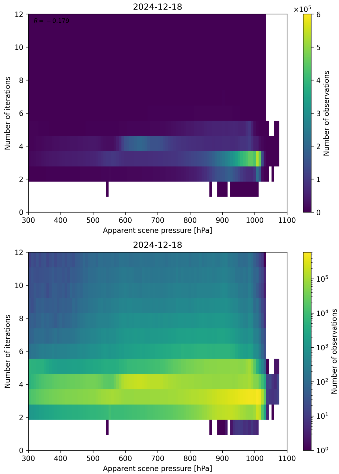
Figure 65: Scatter density plot of “Apparent scene pressure” against “Number of iterations” for 2024-12-17 to 2024-12-19.
