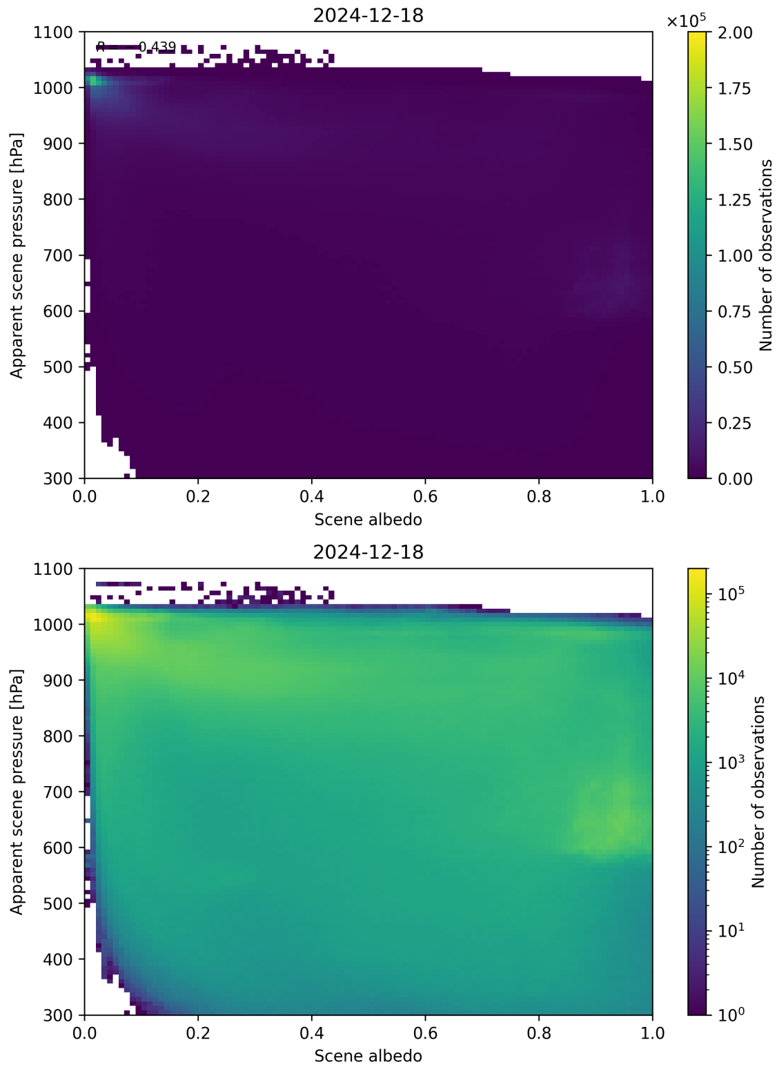
Figure 102: Scatter density plot of “Scene albedo” against “Apparent scene pressure” for 2024-12-17 to 2024-12-19.
