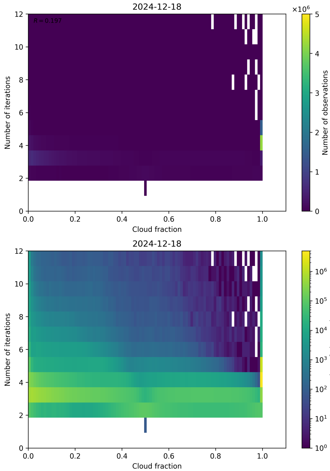
Figure 73: Scatter density plot of “Cloud fraction” against “Number of iterations” for 2024-12-17 to 2024-12-19.
