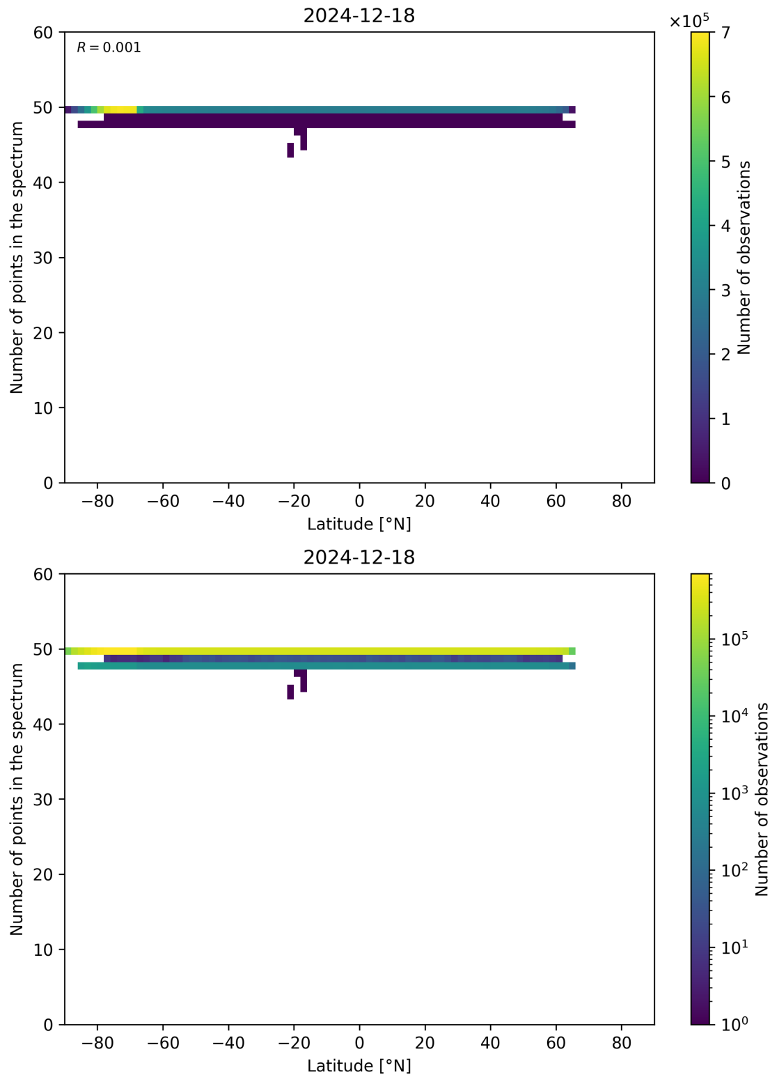
Figure 94: Scatter density plot of “Latitude” against “Number of points in the spectrum” for 2024-12-17 to 2024-12-19.
