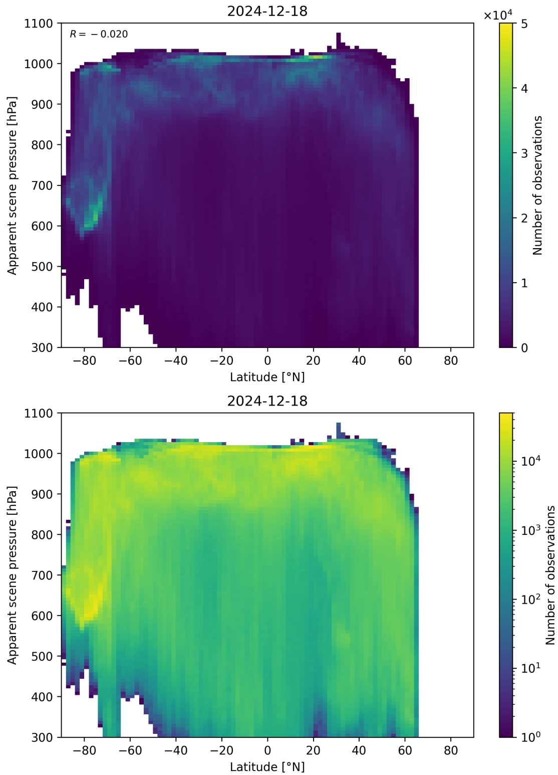
Figure 88: Scatter density plot of “Latitude” against “Apparent scene pressure” for 2024-12-17 to 2024-12-19.
