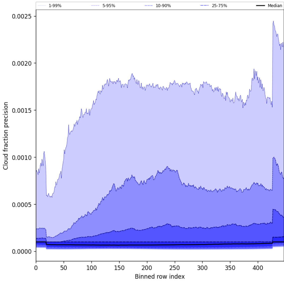
Figure 50: Along track statistics of “Cloud fraction precision” for 2024-12-17 to 2024-12-19
