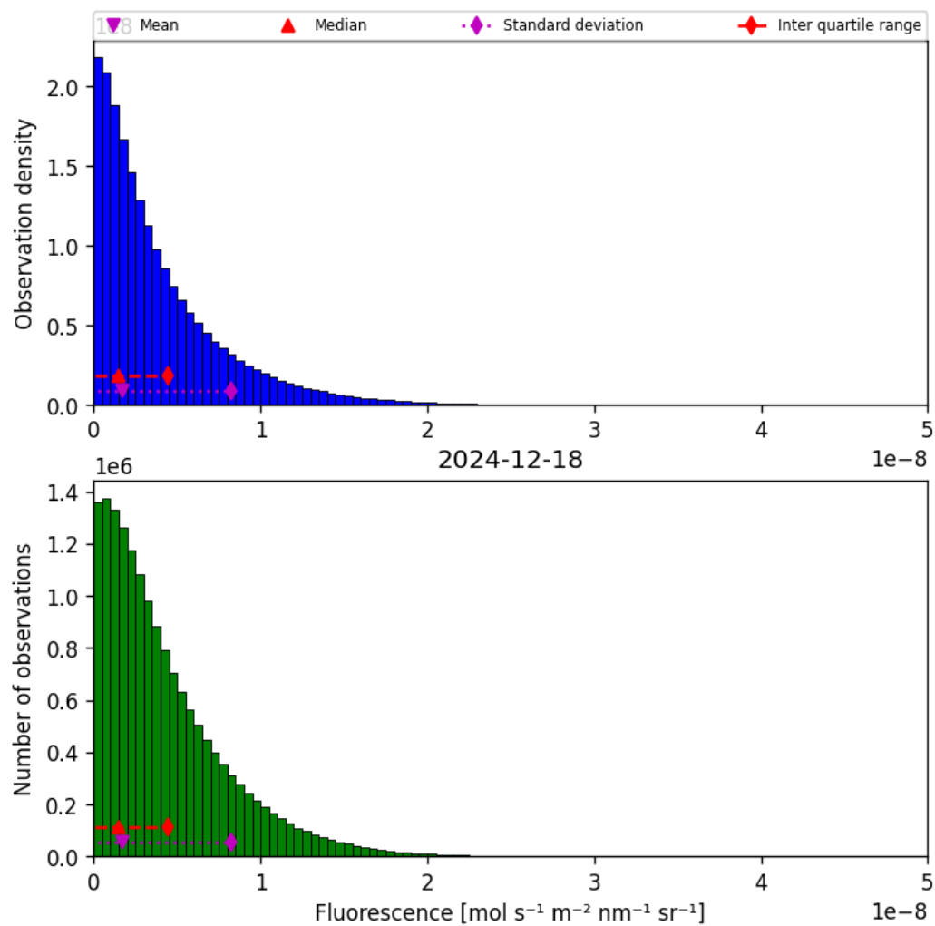
Figure 40: Histogram of “Fluorescence” for 2024-12-17 to 2024-12-19
