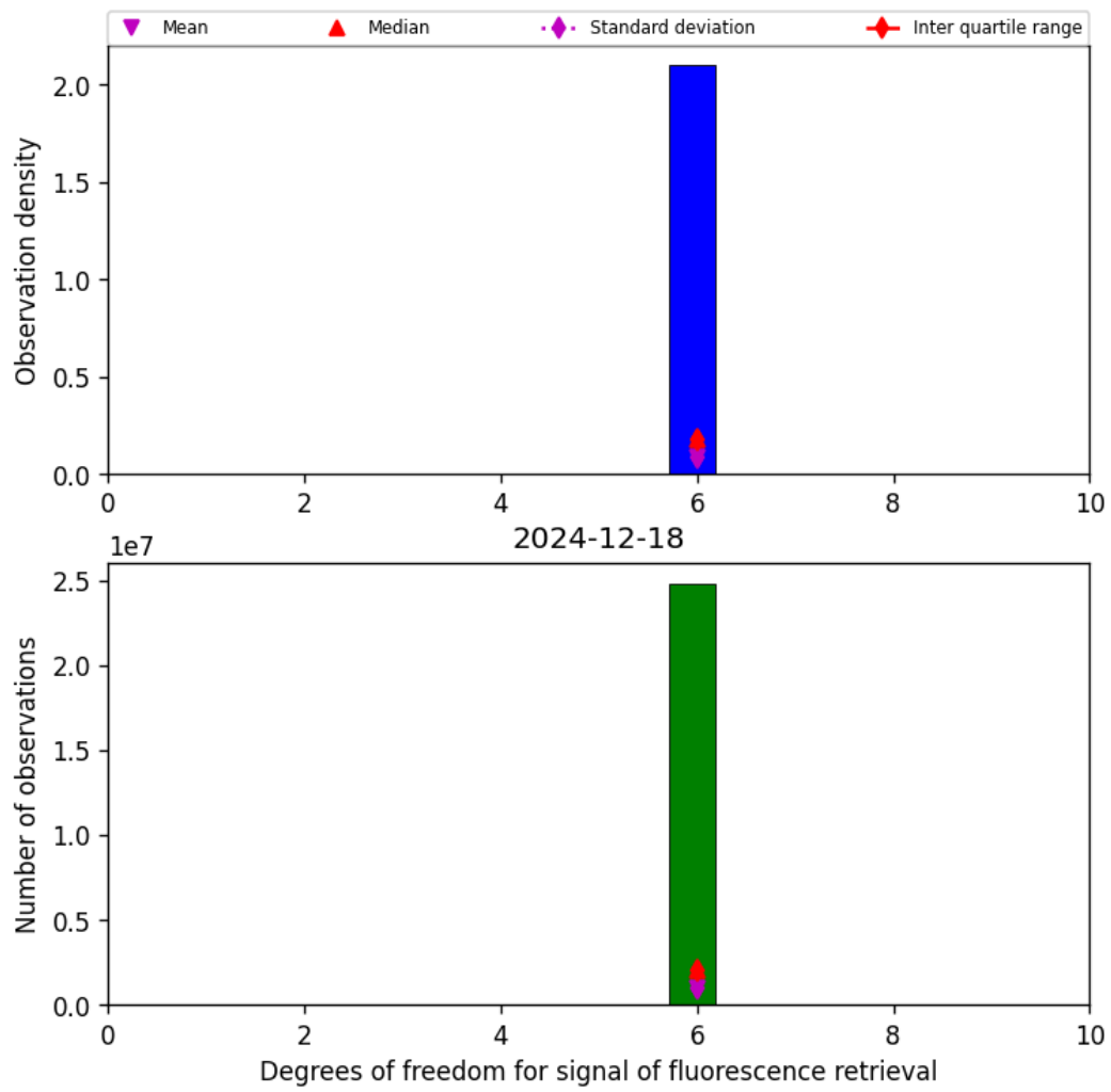
Figure 43: Histogram of “Degrees of freedom for signal of fluorescence retrieval” for 2024-12-17 to 2024-12-19
