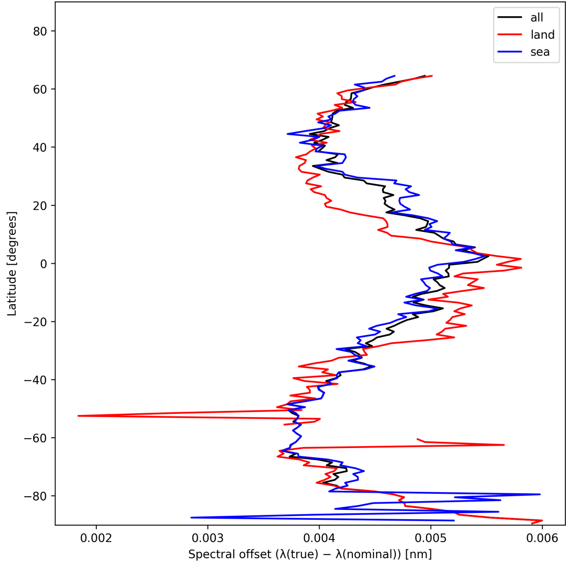
Figure 28: Zonal average of “Spectral offset ( \lambda_{\text{true}} - \lambda_{\text{nominal}} )” for 2024-12-17 to 2024-12-19.
