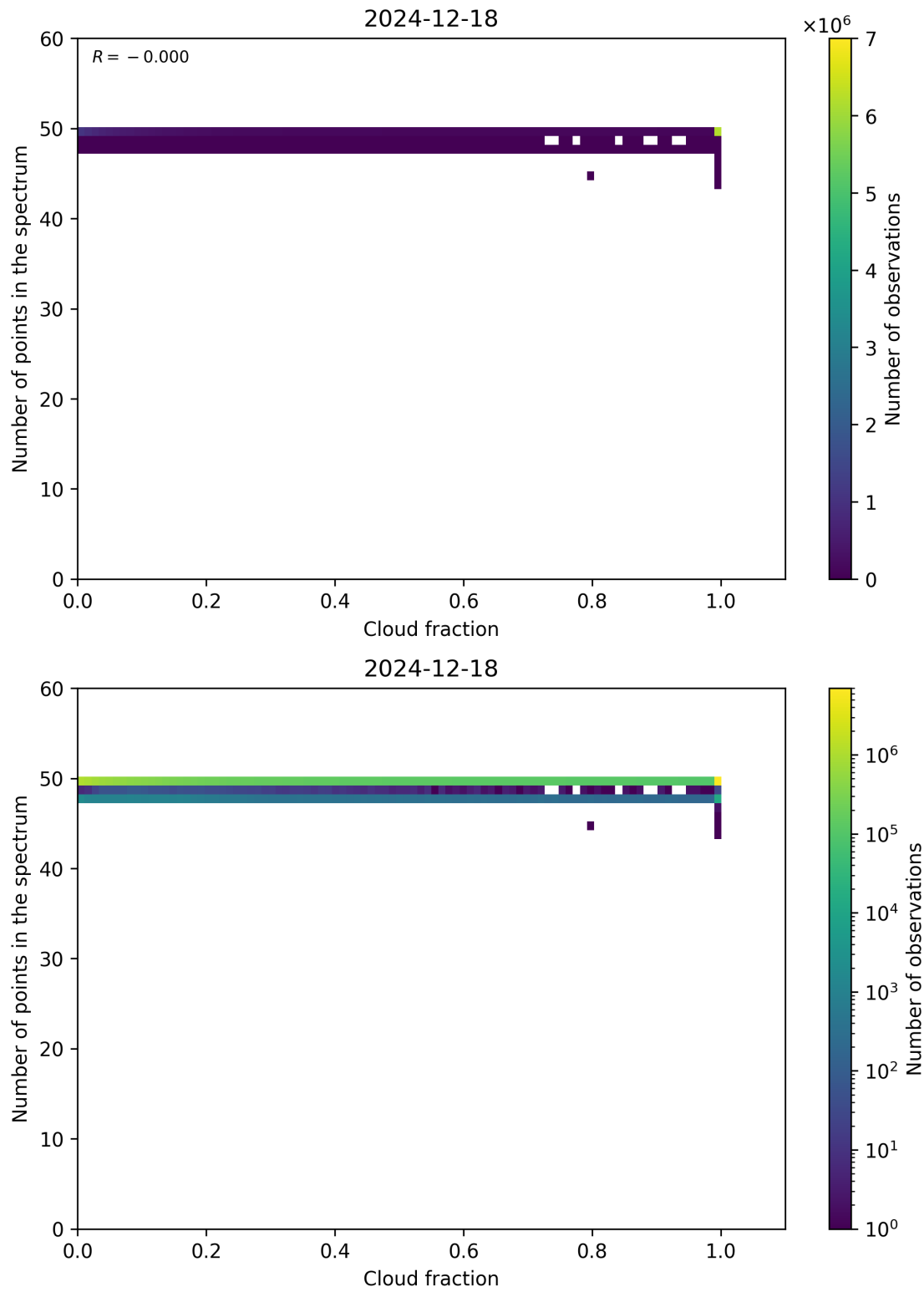
Figure 74: Scatter density plot of “Cloud fraction” against “Number of points in the spectrum” for 2024-12-17 to 2024-12-19.
