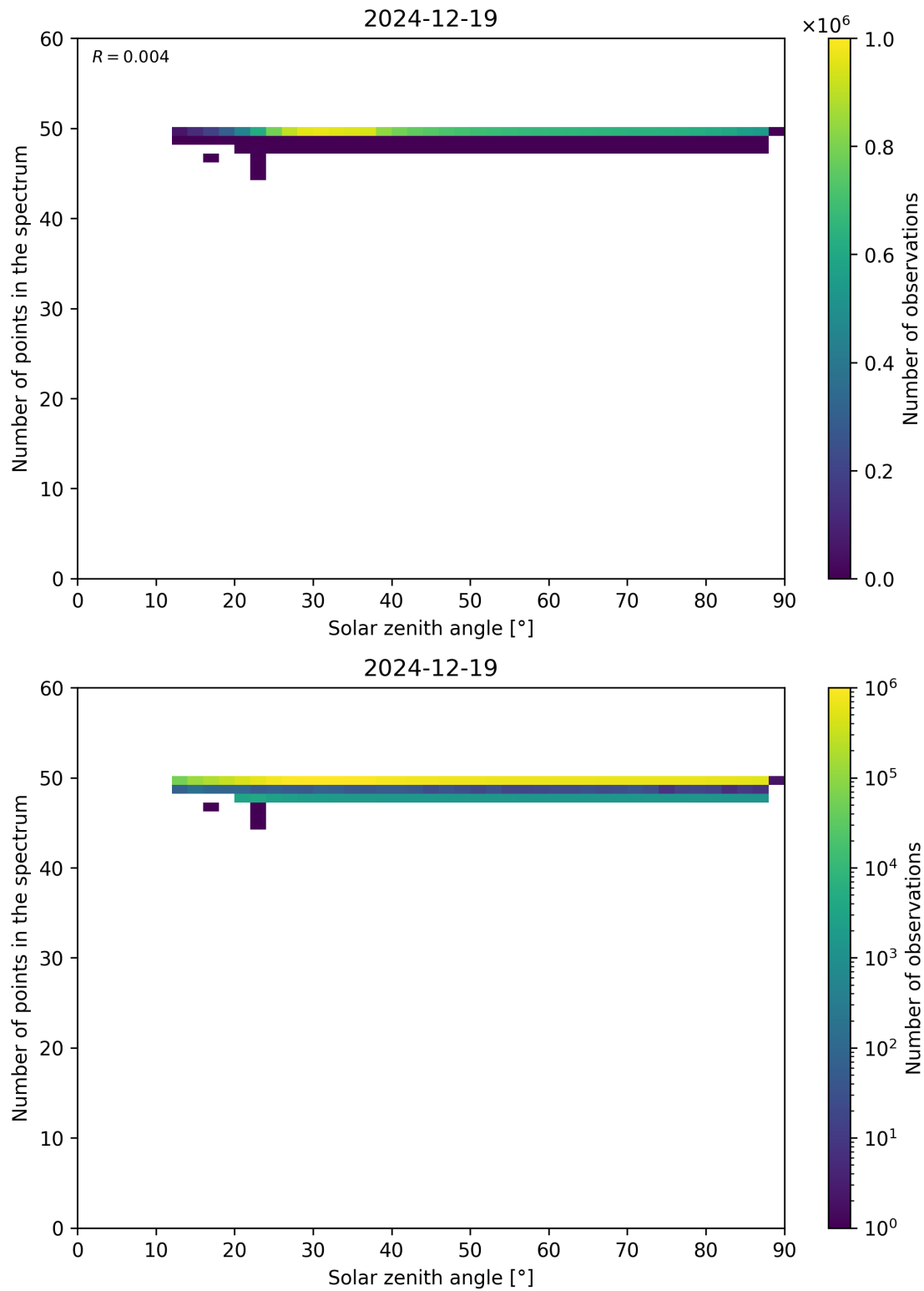
Figure 115: Scatter density plot of “Solar zenith angle” against “Number of points in the spectrum” for 2024-12-18 to 2024-12-20.
