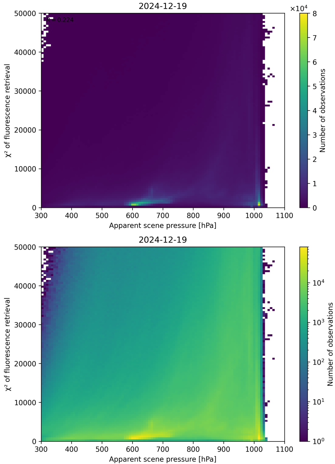
Figure 63: Scatter density plot of “Apparent scene pressure” against “ \chi^2 of fluorescence retrieval” for 2024-12-18 to 2024-12-20.
