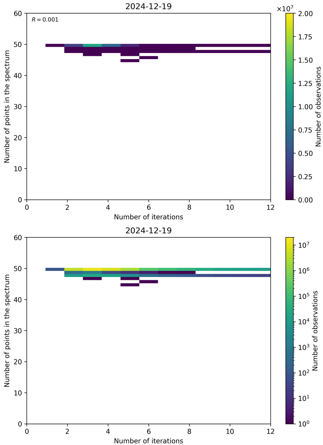
Figure 99: Scatter density plot of “Number of iterations” against “Number of points in the spectrum” for 2024-12-18 to 2024-12-20.
