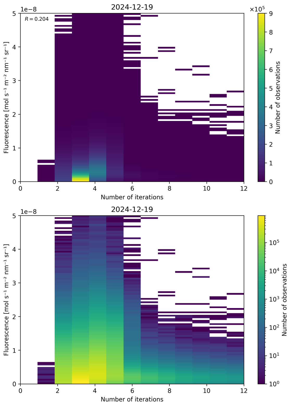
Figure 98: Scatter density plot of “Number of iterations” against “Fluorescence” for 2024-12-18 to 2024-12-20.
