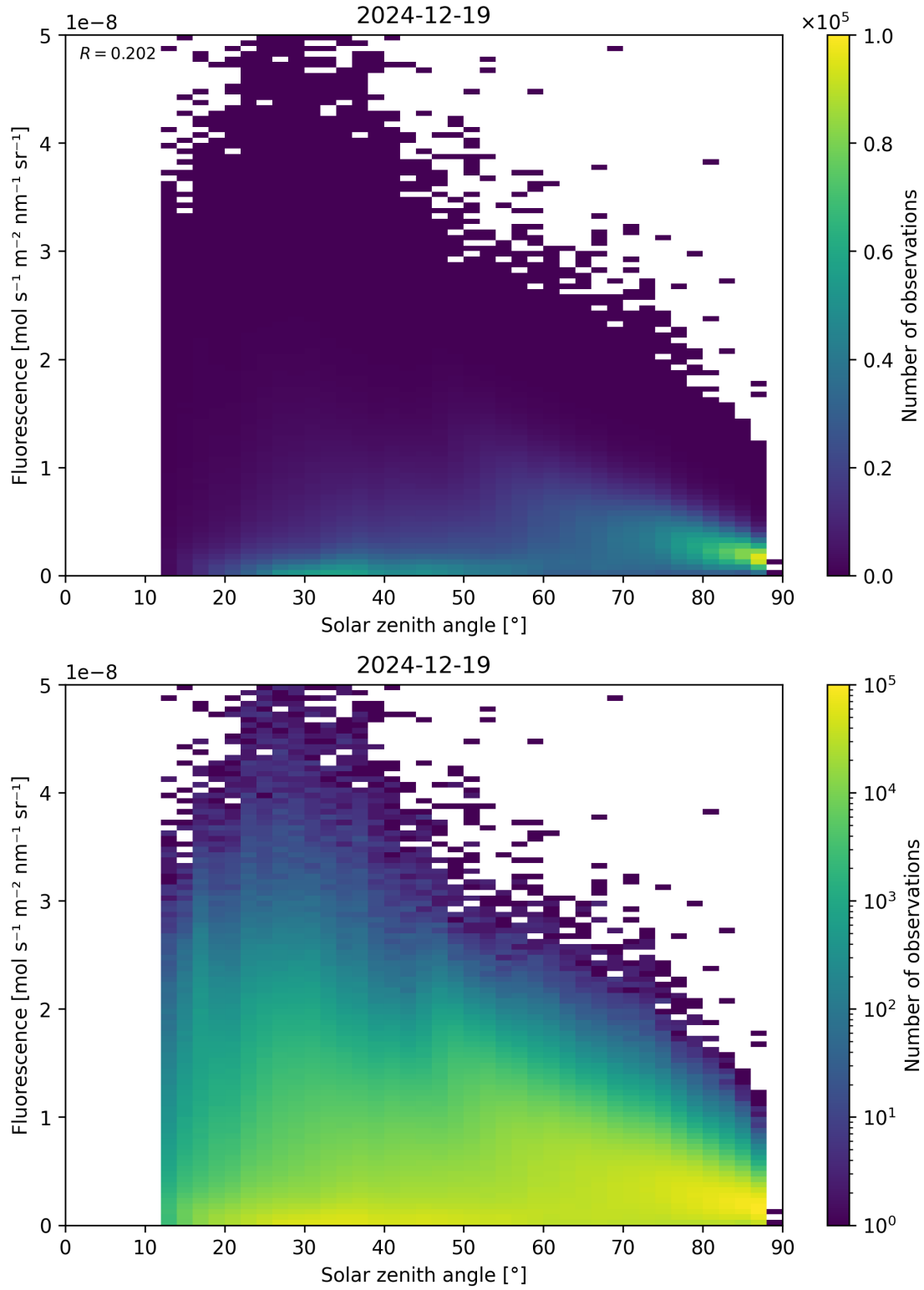
Figure 112: Scatter density plot of “Solar zenith angle” against “Fluorescence” for 2024-12-18 to 2024-12-20.
