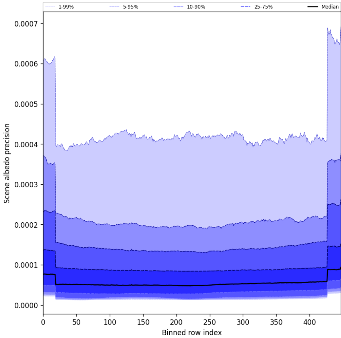
Figure 52: Along track statistics of “Scene albedo precision” for 2024-12-18 to 2024-12-20
