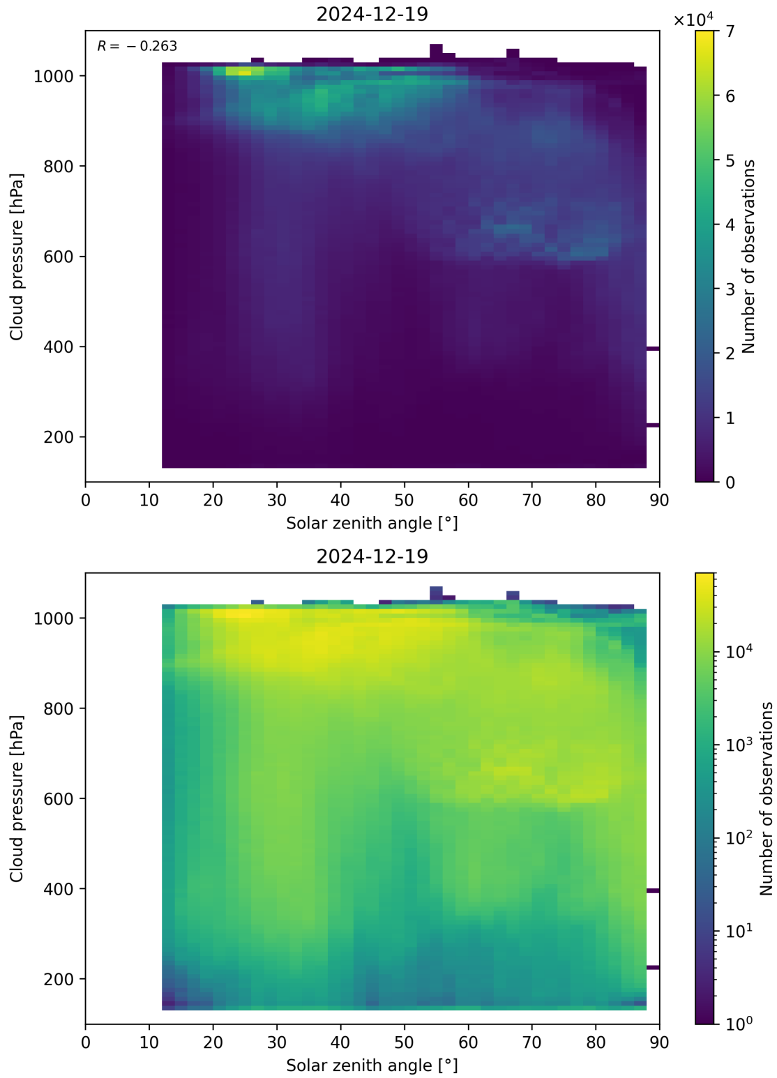
Figure 111: Scatter density plot of “Solar zenith angle” against “Cloud pressure” for 2024-12-18 to 2024-12-20.
