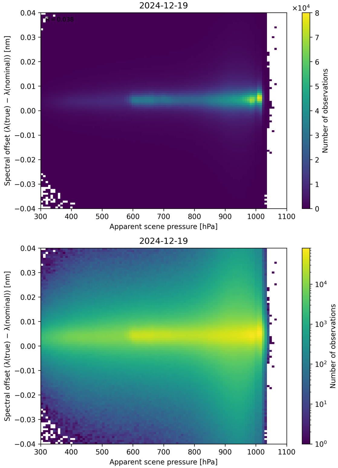
Figure 67: Scatter density plot of “Apparent scene pressure” against “Spectral offset ( \lambda_{\text{true}} - \lambda_{\text{nominal}} )” for 2024-12-18 to 2024-12-20.
