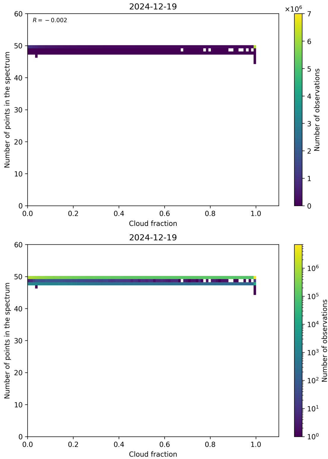
Figure 74: Scatter density plot of “Cloud fraction” against “Number of points in the spectrum” for 2024-12-18 to 2024-12-20.
