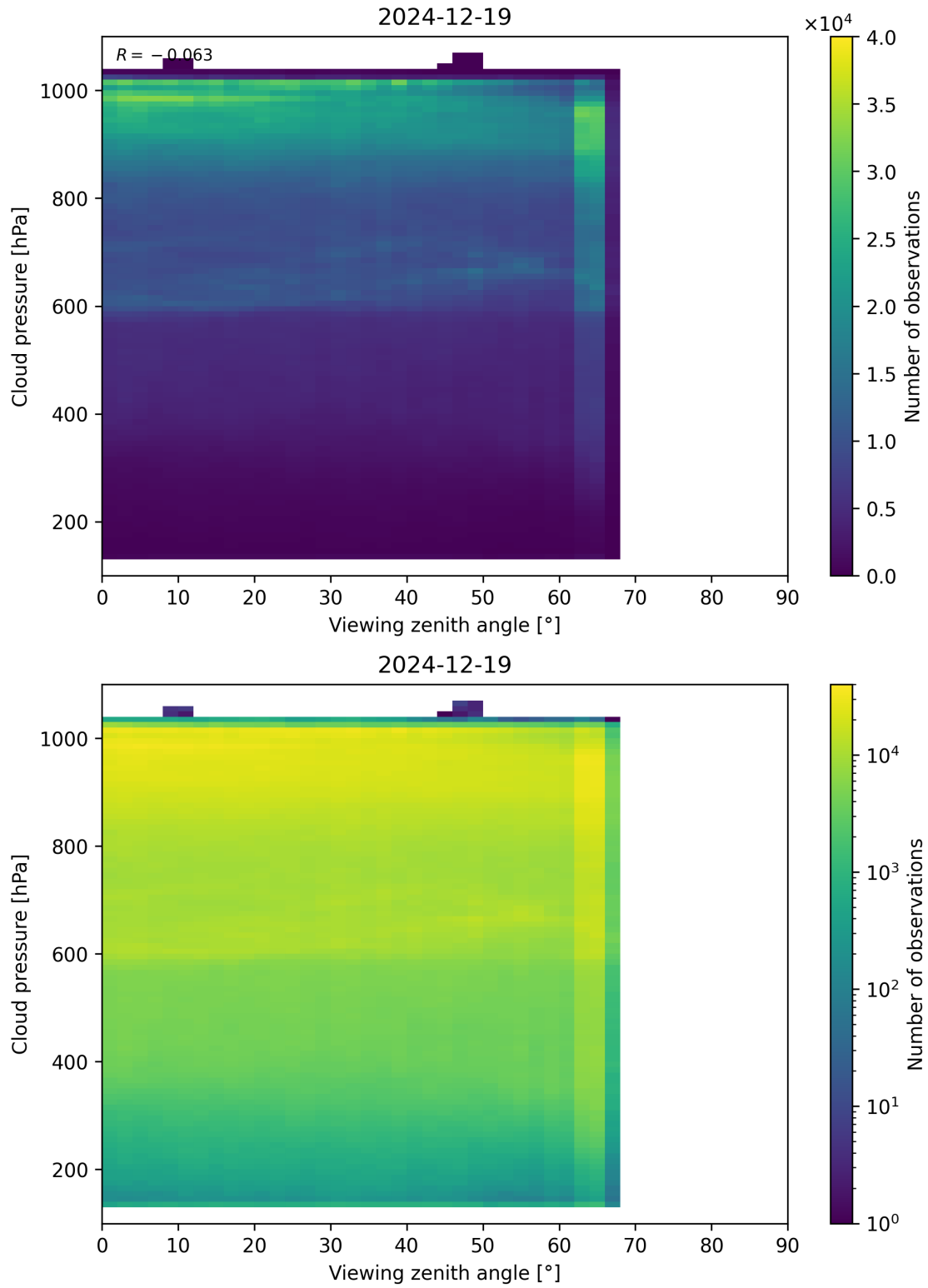
Figure 121: Scatter density plot of “Viewing zenith angle” against “Cloud pressure” for 2024-12-18 to 2024-12-20.
