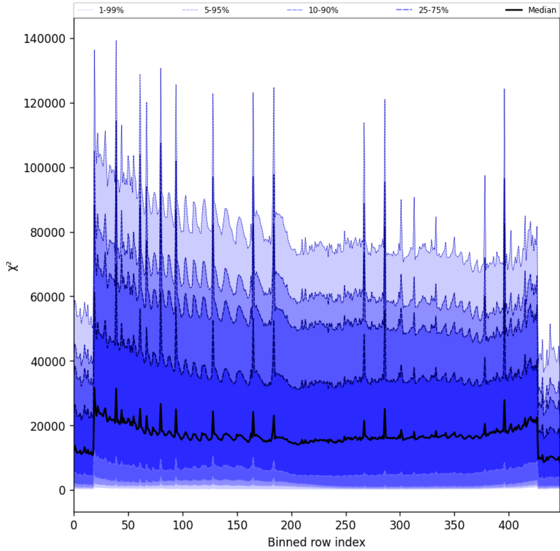
Figure 55: Along track statistics of “ \chi^2 ” for 2024-12-18 to 2024-12-20
