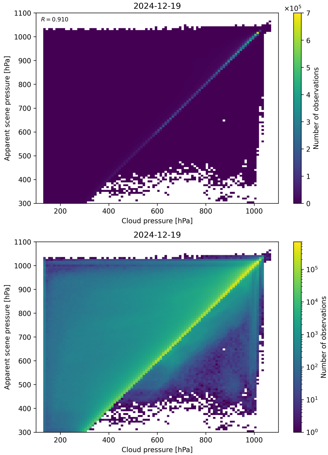
Figure 77: Scatter density plot of “Cloud pressure” against “Apparent scene pressure” for 2024-12-18 to 2024-12-20.
