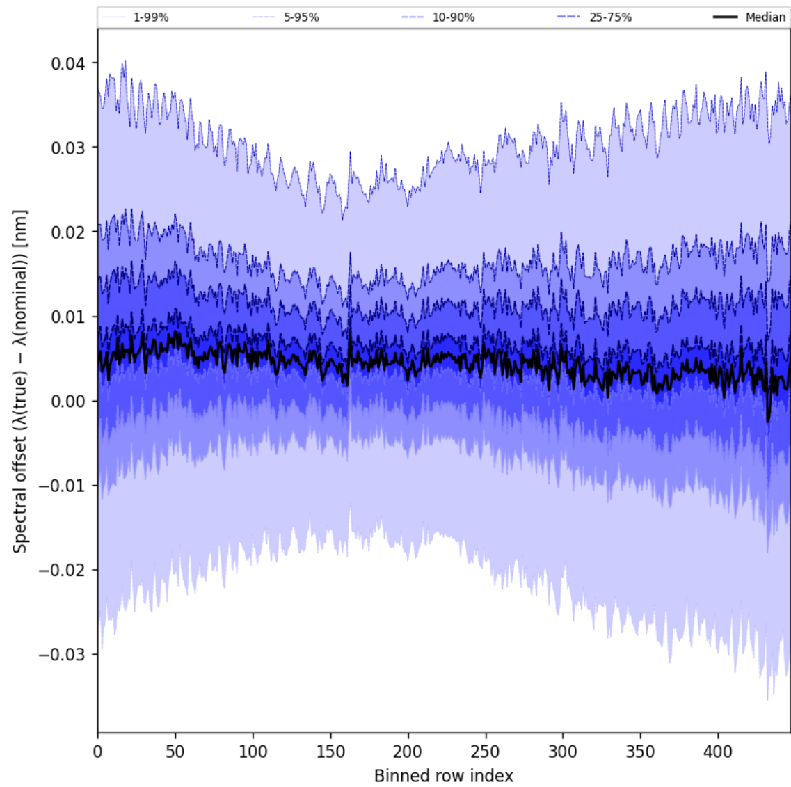
Figure 62: Along track statistics of “Spectral offset ( \lambda_{\text{true}} - \lambda_{\text{nominal}} )” for 2024-12-18 to 2024-12-20
