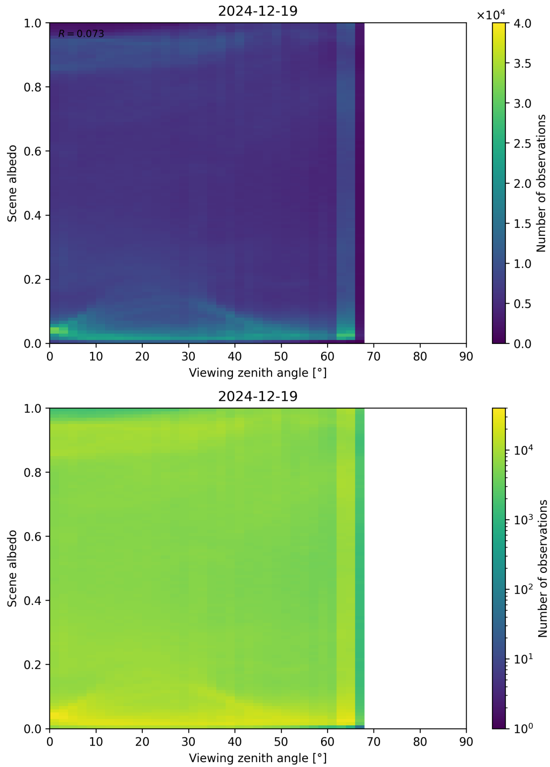
Figure 126: Scatter density plot of “Viewing zenith angle” against “Scene albedo” for 2024-12-18 to 2024-12-20.
