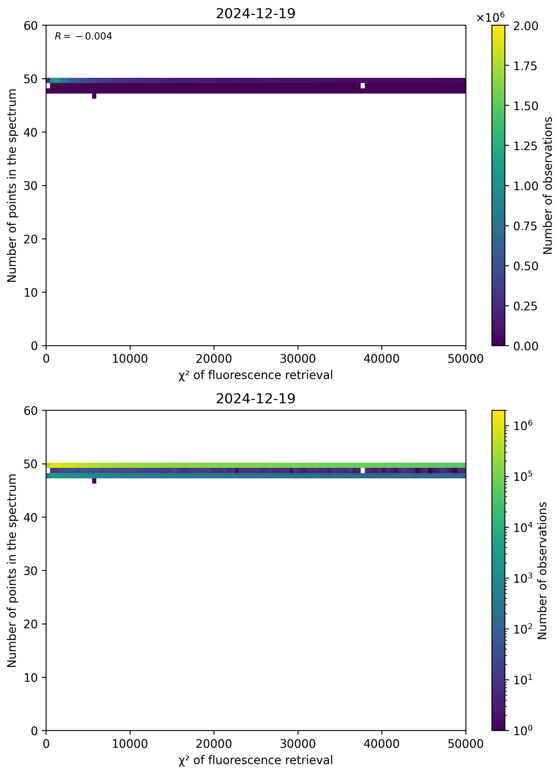
Figure 68: Scatter density plot of “ \chi^2 of fluorescence retrieval” against “Number of points in the spectrum” for 2024-12-18 to 2024-12-20.
