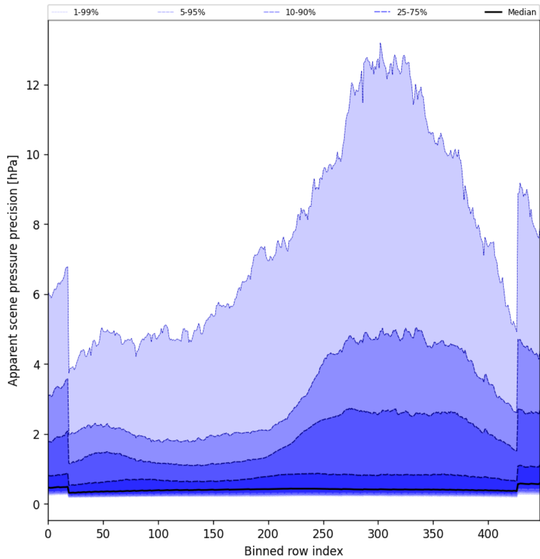
Figure 54: Along track statistics of “Apparent scene pressure precision” for 2024-12-18 to 2024-12-20
