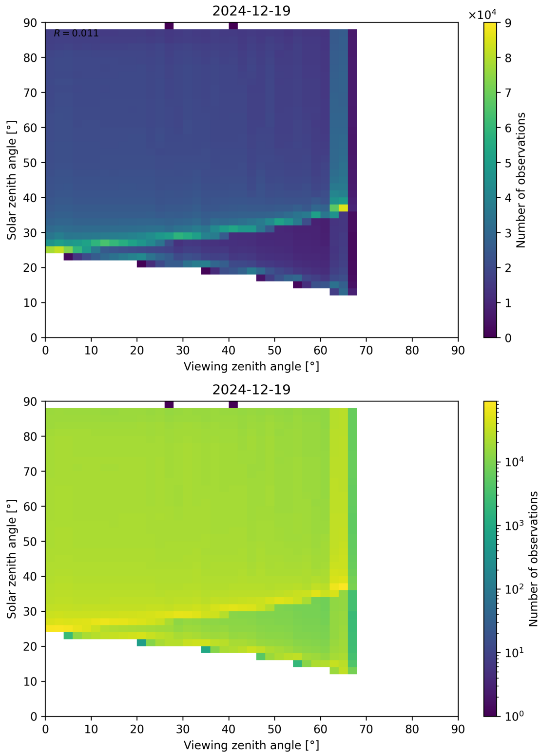
Figure 127: Scatter density plot of “Viewing zenith angle” against “Solar zenith angle” for 2024-12-18 to 2024-12-20.
