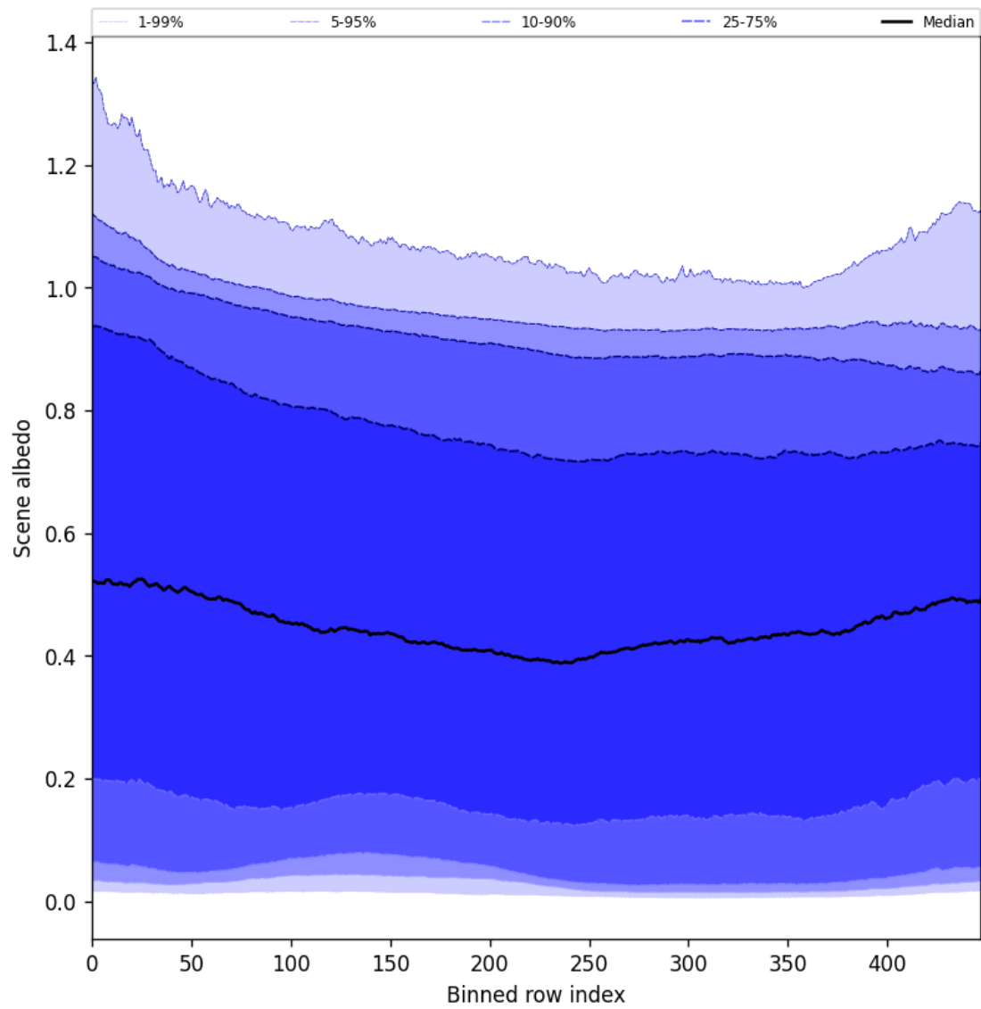
Figure 51: Along track statistics of “Scene albedo” for 2024-12-18 to 2024-12-20
