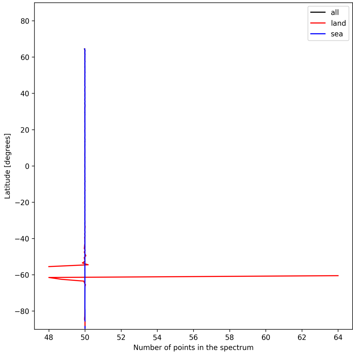
Figure 27: Zonal average of “Number of points in the spectrum” for 2024-12-18 to 2024-12-20.
