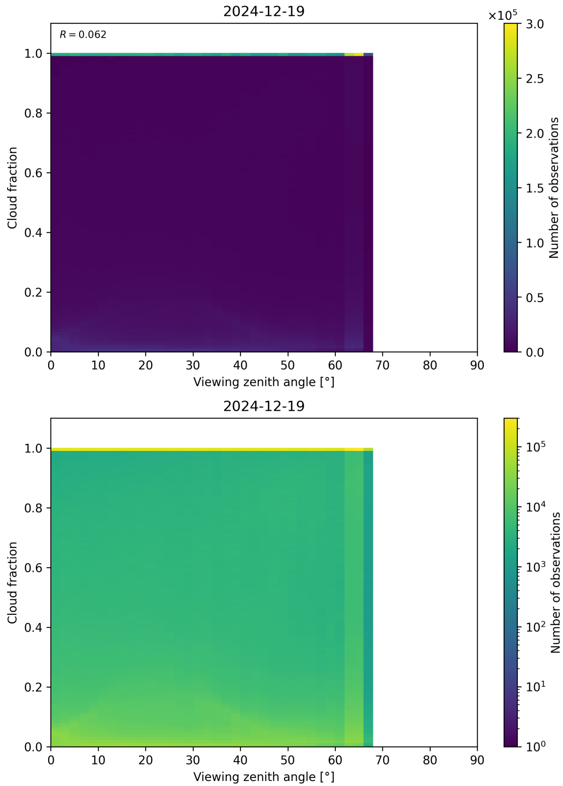
Figure 120: Scatter density plot of “Viewing zenith angle” against “Cloud fraction” for 2024-12-18 to 2024-12-20.
