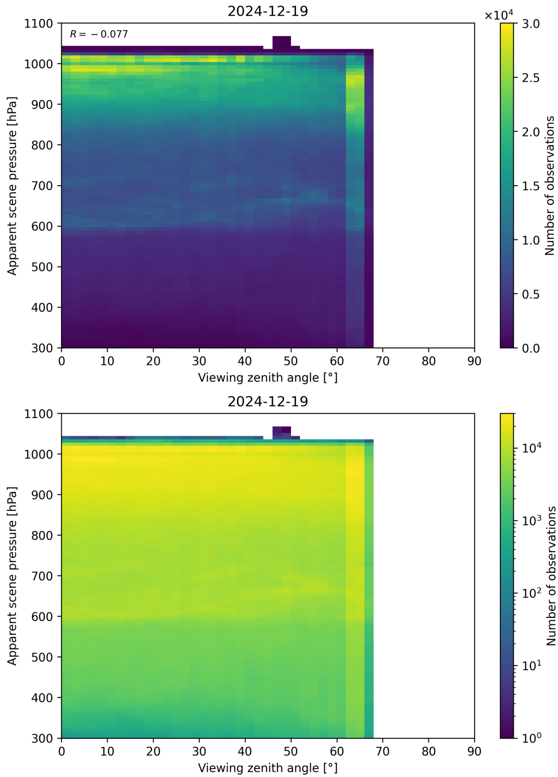
Figure 118: Scatter density plot of “Viewing zenith angle” against “Apparent scene pressure” for 2024-12-18 to 2024-12-20.
