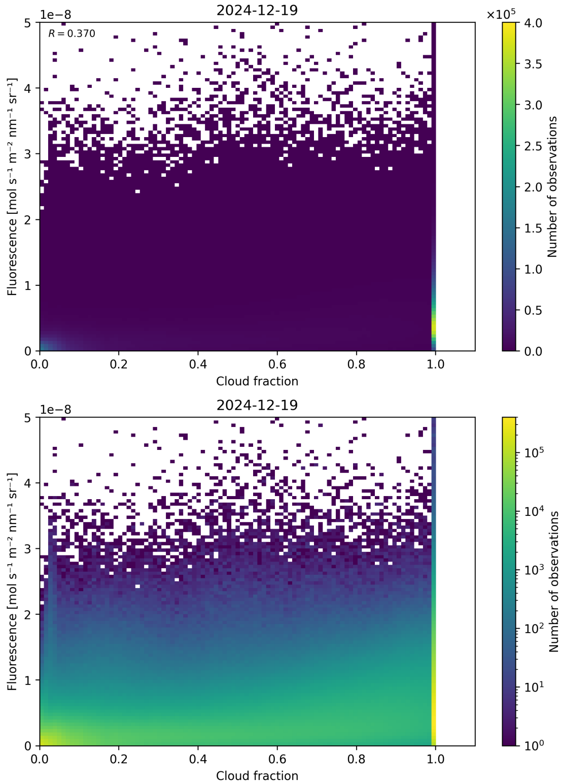
Figure 72: Scatter density plot of “Cloud fraction” against “Fluorescence” for 2024-12-18 to 2024-12-20.
