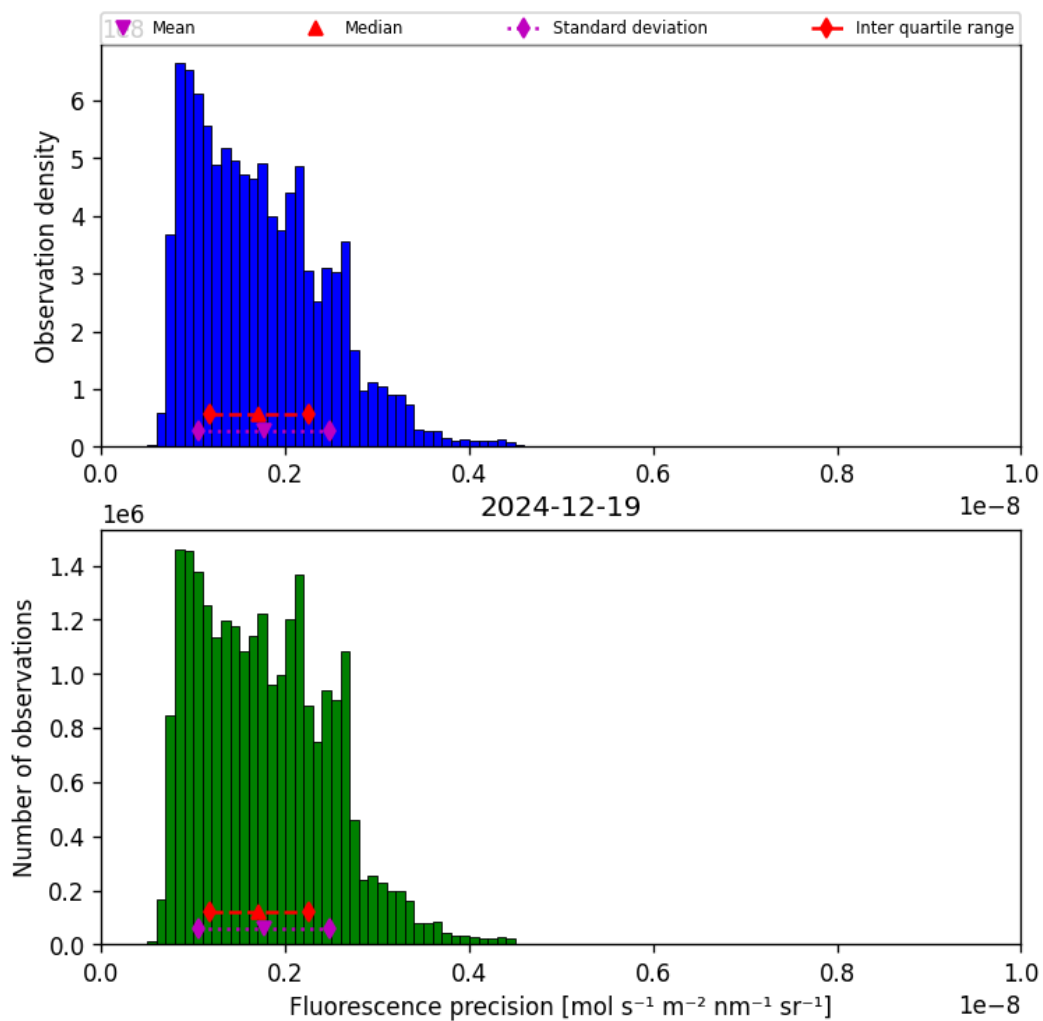
Figure 41: Histogram of “Fluorescence precision” for 2024-12-18 to 2024-12-20
