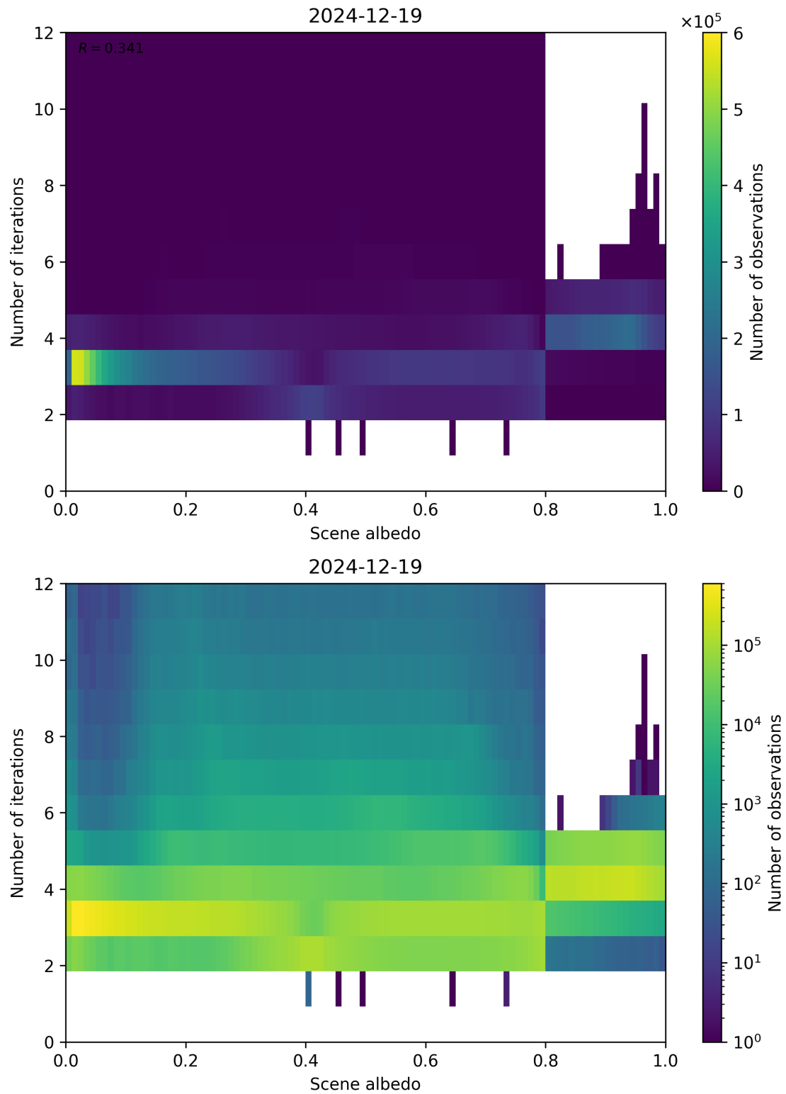
Figure 105: Scatter density plot of “Scene albedo” against “Number of iterations” for 2024-12-18 to 2024-12-20.
