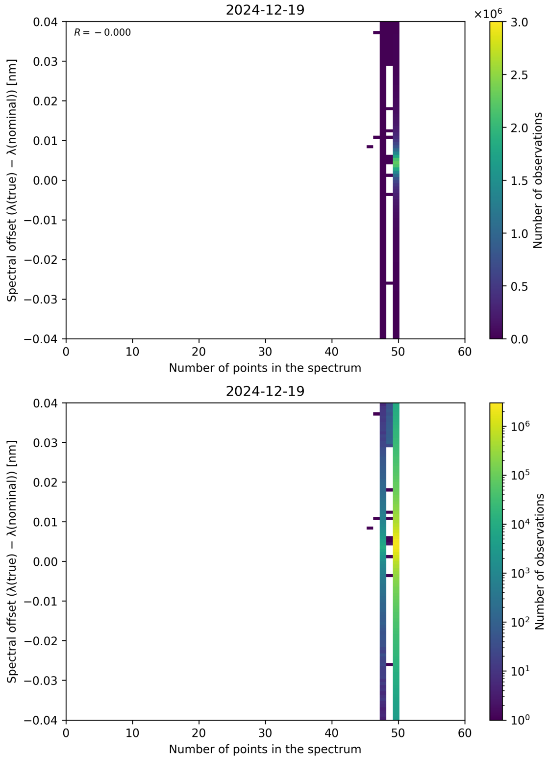
Figure 101: Scatter density plot of “Number of points in the spectrum” against “Spectral offset ( \lambda_{\text{true}} - \lambda_{\text{nominal}} )” for 2024-12-18 to 2024-12-20.
