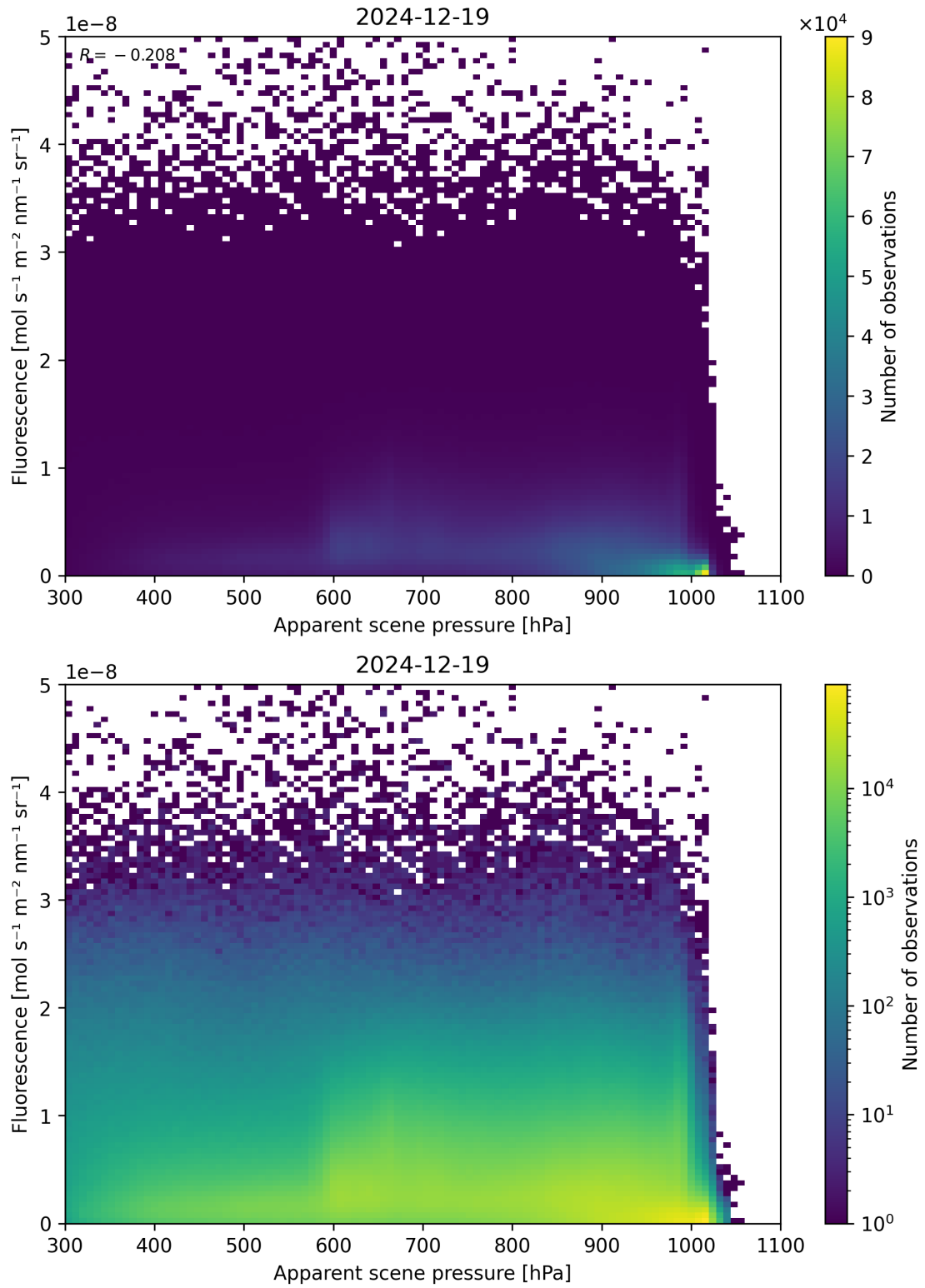
Figure 64: Scatter density plot of “Apparent scene pressure” against “Fluorescence” for 2024-12-18 to 2024-12-20.
