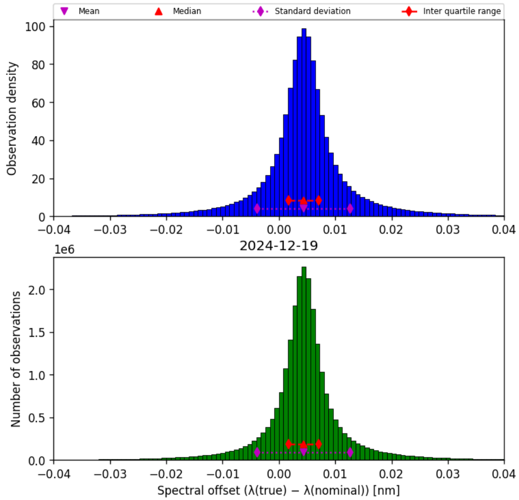
Figure 45: Histogram of “Spectral offset ( \lambda_{\text{true}} - \lambda_{\text{nominal}} )” for 2024-12-18 to 2024-12-20
