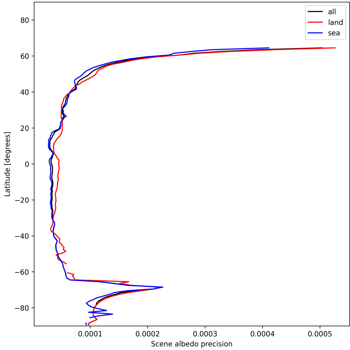
Figure 18: Zonal average of “Scene albedo precision” for 2024-12-18 to 2024-12-20.
