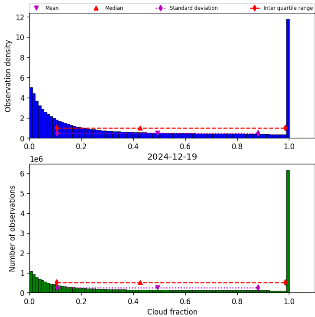
Figure 32: Histogram of “Cloud fraction” for 2024-12-18 to 2024-12-20
