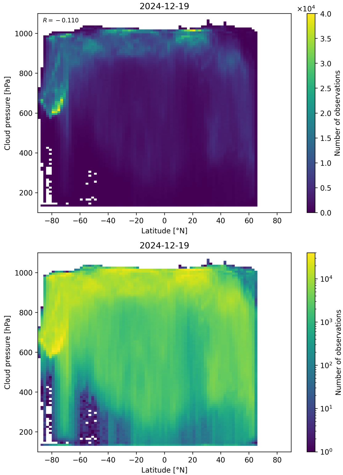
Figure 91: Scatter density plot of “Latitude” against “Cloud pressure” for 2024-12-18 to 2024-12-20.
