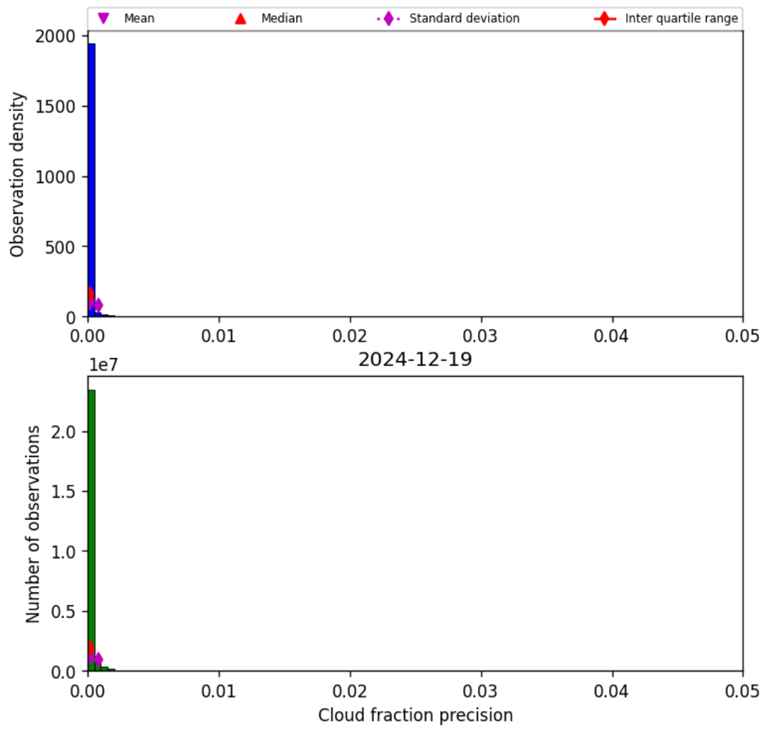
Figure 33: Histogram of “Cloud fraction precision” for 2024-12-18 to 2024-12-20
