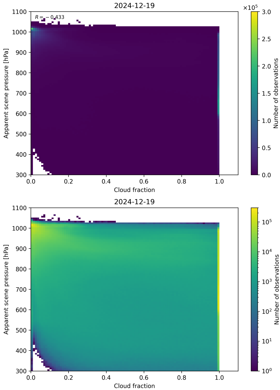
Figure 70: Scatter density plot of “Cloud fraction” against “Apparent scene pressure” for 2024-12-18 to 2024-12-20.
