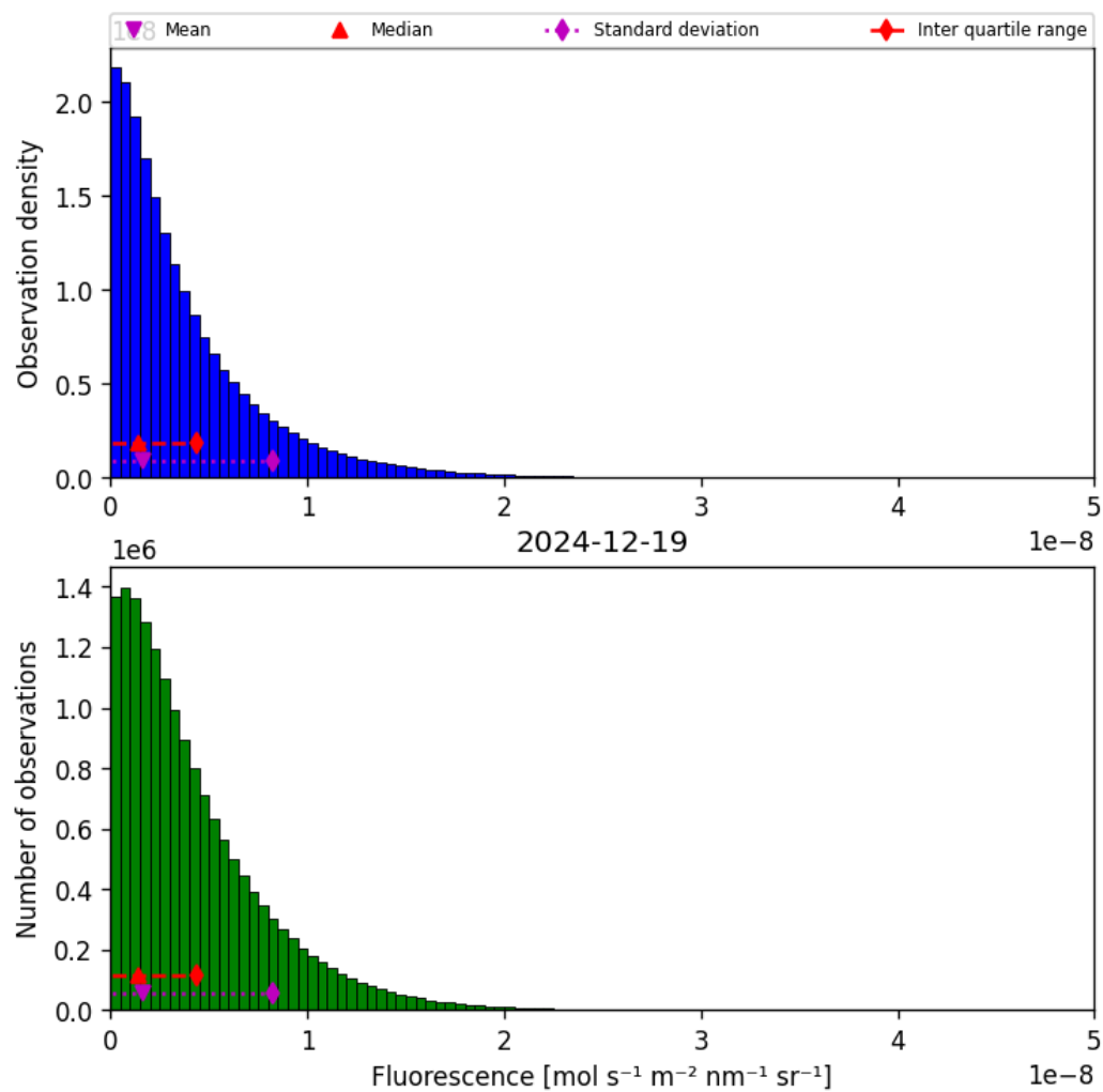
Figure 40: Histogram of “Fluorescence” for 2024-12-18 to 2024-12-20
