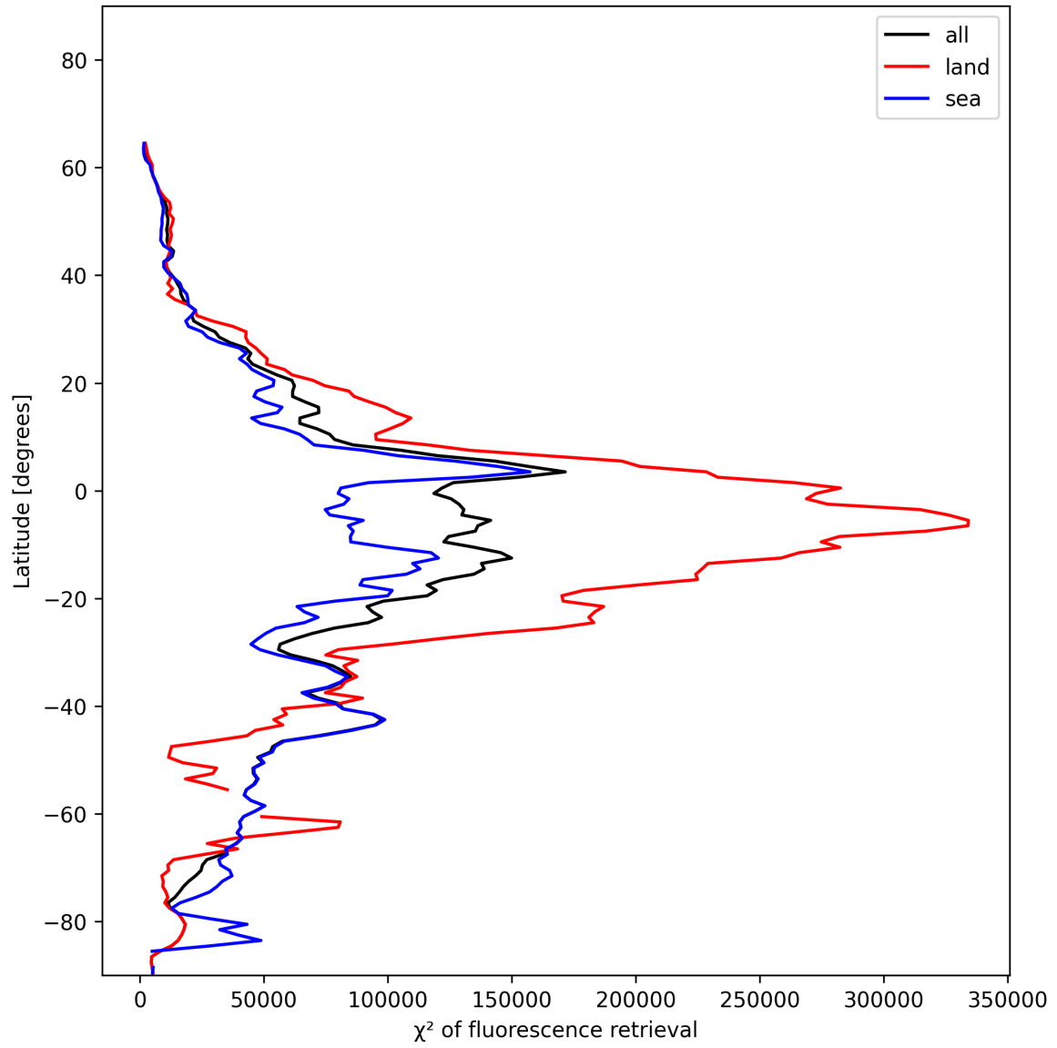
Figure 25: Zonal average of “ \chi^2 of fluorescence retrieval” for 2024-12-18 to 2024-12-20.
