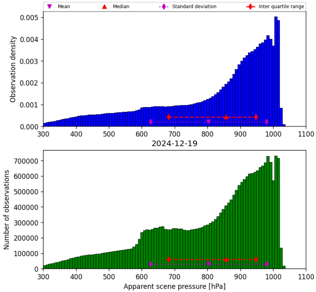
Figure 36: Histogram of “Apparent scene pressure” for 2024-12-18 to 2024-12-20
