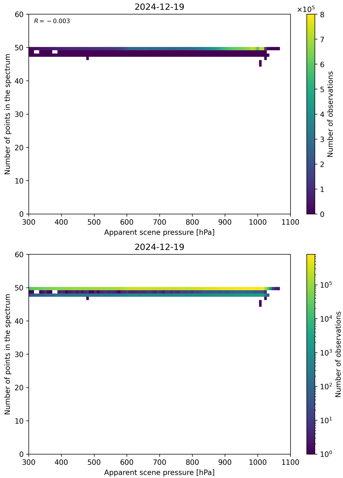
Figure 66: Scatter density plot of “Apparent scene pressure” against “Number of points in the spectrum” for 2024-12-18 to 2024-12-20.
