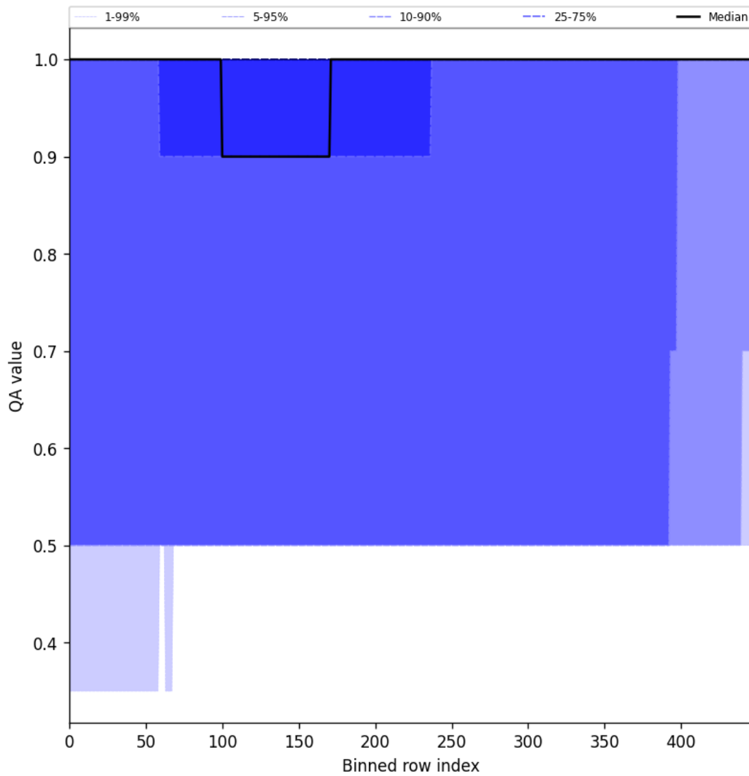
Figure 46: Along track statistics of “QA value” for 2024-12-18 to 2024-12-20
