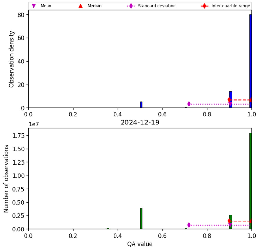
Figure 29: Histogram of “QA value” for 2024-12-18 to 2024-12-20
