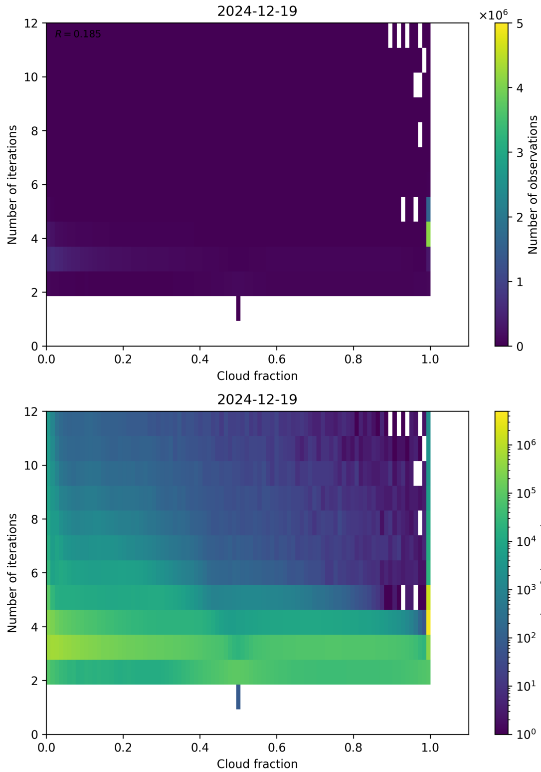
Figure 73: Scatter density plot of “Cloud fraction” against “Number of iterations” for 2024-12-18 to 2024-12-20.
