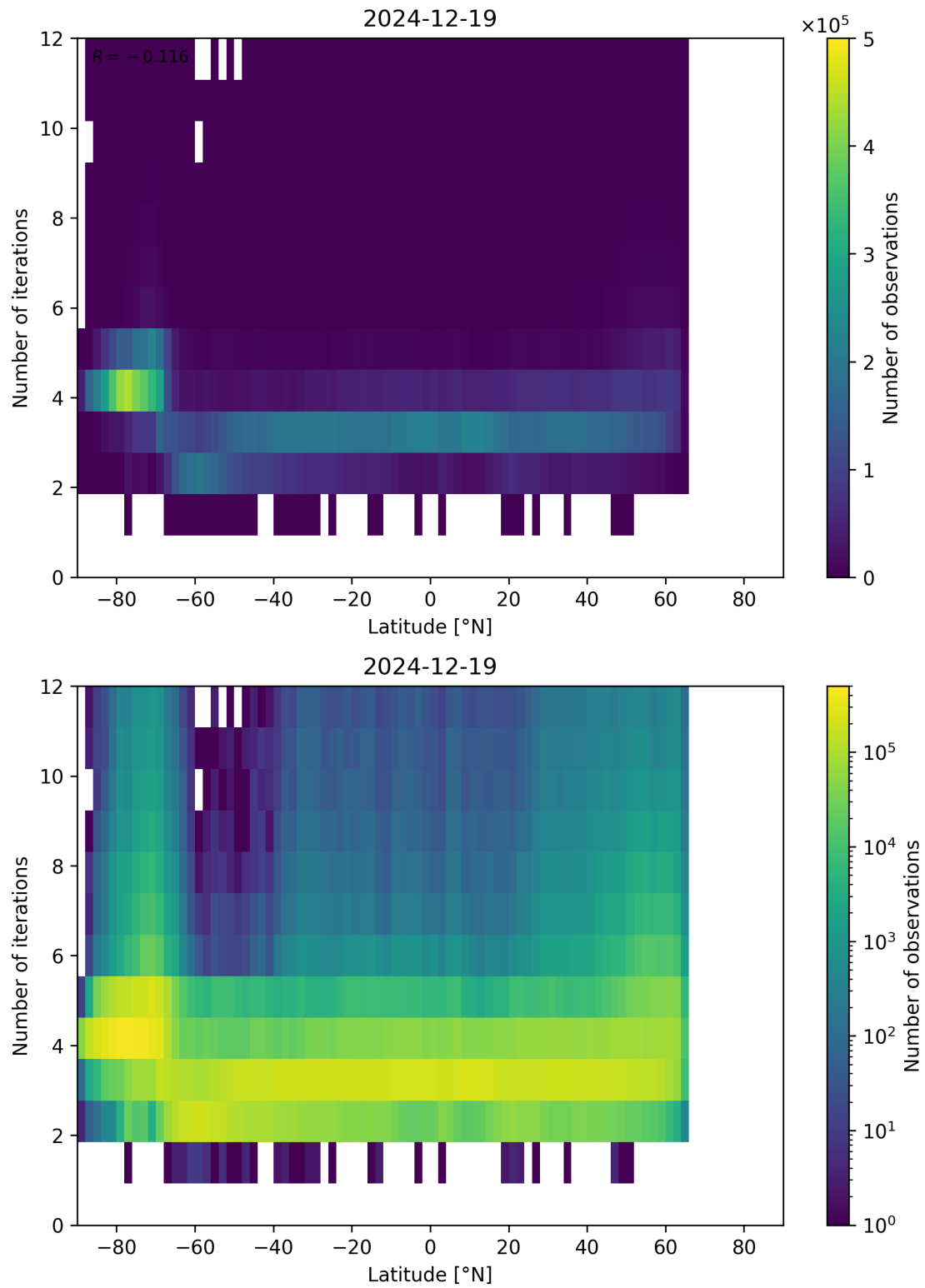
Figure 93: Scatter density plot of “Latitude” against “Number of iterations” for 2024-12-18 to 2024-12-20.
