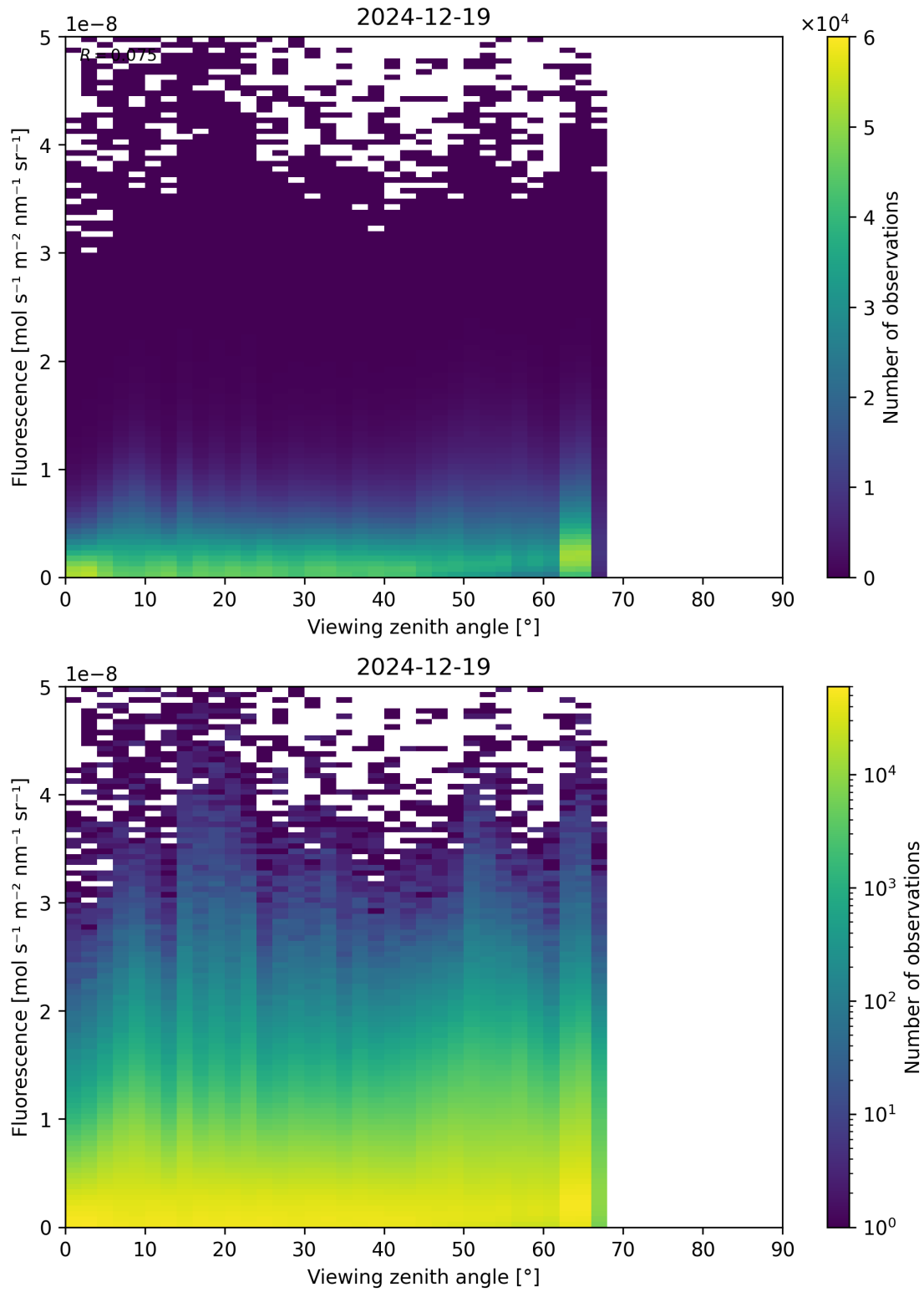
Figure 122: Scatter density plot of “Viewing zenith angle” against “Fluorescence” for 2024-12-18 to 2024-12-20.
