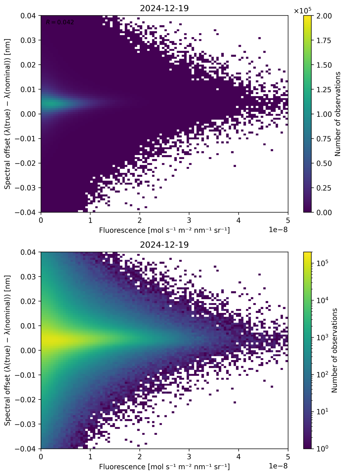
Figure 87: Scatter density plot of “Fluorescence” against “Spectral offset ( \lambda_{\text{true}} - \lambda_{\text{nominal}} )” for 2024-12-18 to 2024-12-20.
