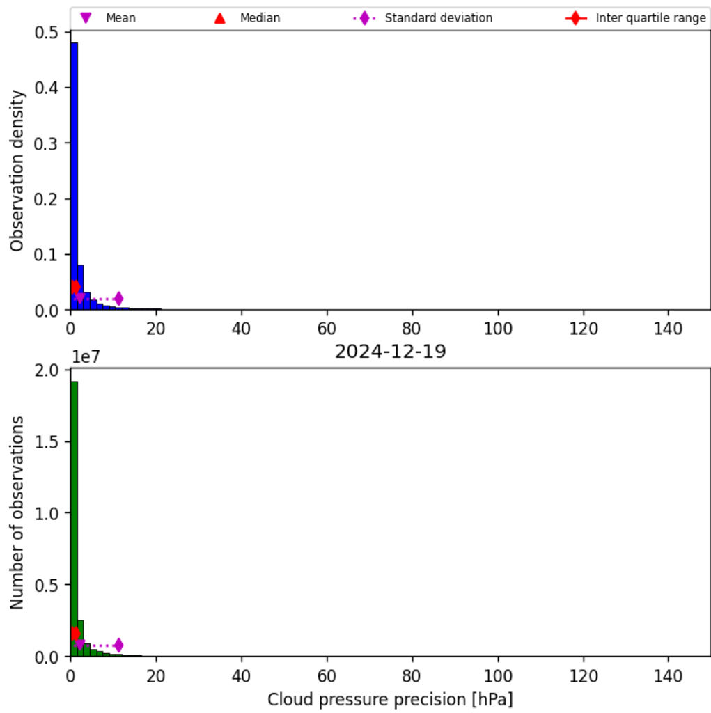
Figure 31: Histogram of “Cloud pressure precision” for 2024-12-18 to 2024-12-20
