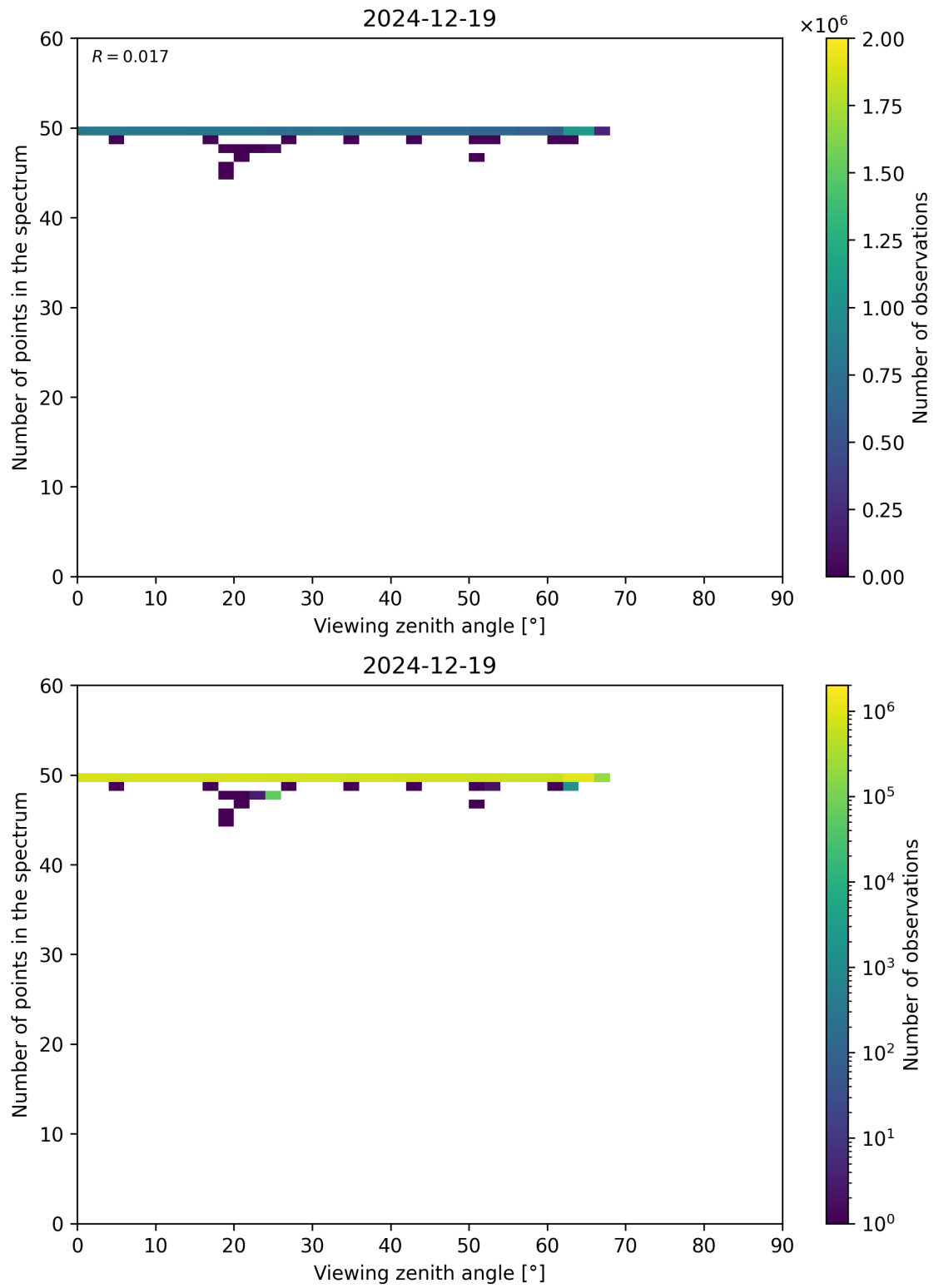
Figure 125: Scatter density plot of “Viewing zenith angle” against “Number of points in the spectrum” for 2024-12-18 to 2024-12-20.
