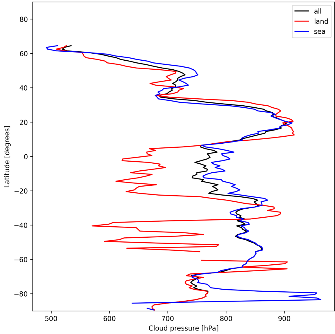
Figure 13: Zonal average of “Cloud pressure” for 2024-12-18 to 2024-12-20.
