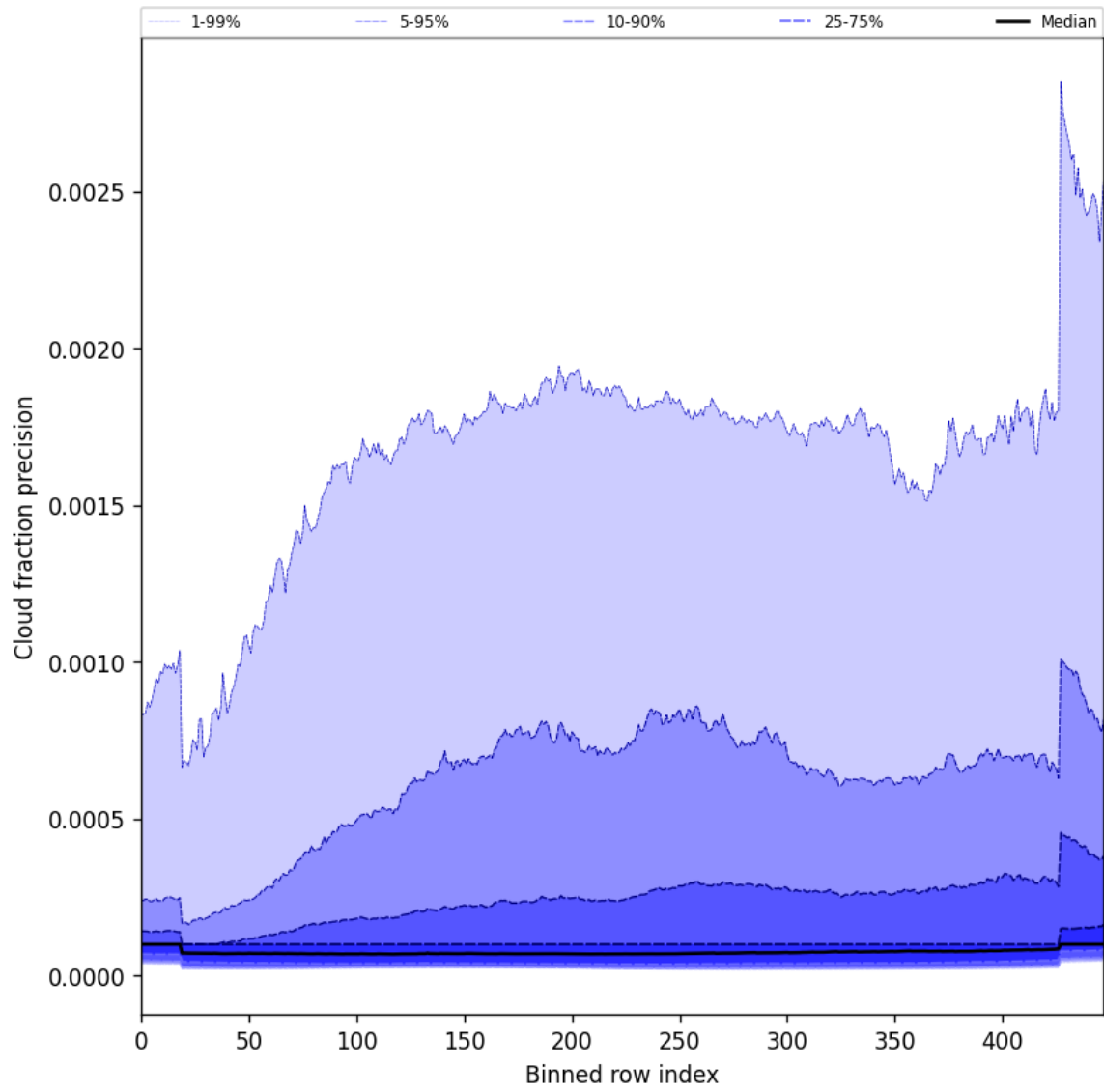
Figure 50: Along track statistics of “Cloud fraction precision” for 2024-12-18 to 2024-12-20
