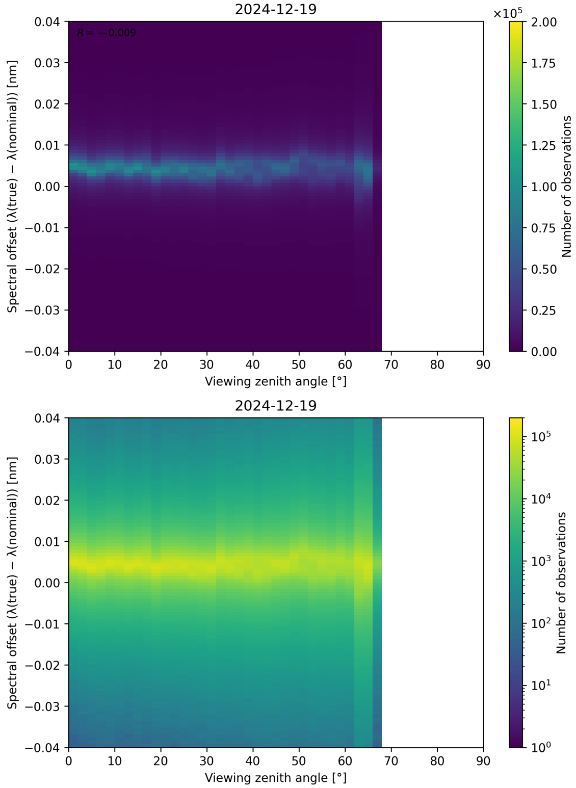
Figure 128: Scatter density plot of “Viewing zenith angle” against “Spectral offset ( \lambda_{\text{true}} - \lambda_{\text{nominal}} )” for 2024-12-18 to 2024-12-20.
