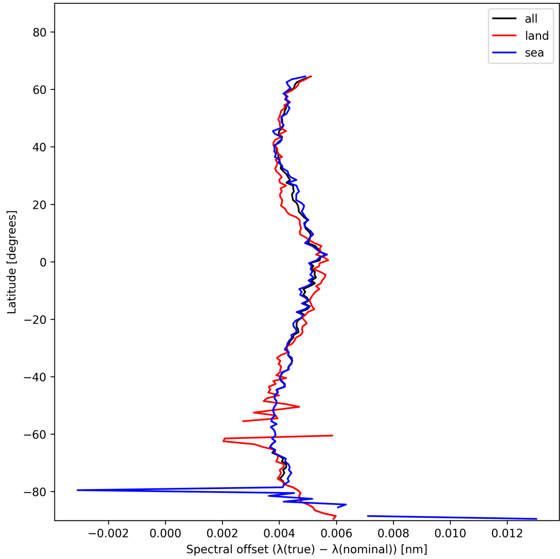
Figure 28: Zonal average of “Spectral offset ( \lambda_{\text{true}} - \lambda_{\text{nominal}} )” for 2024-12-18 to 2024-12-20.
