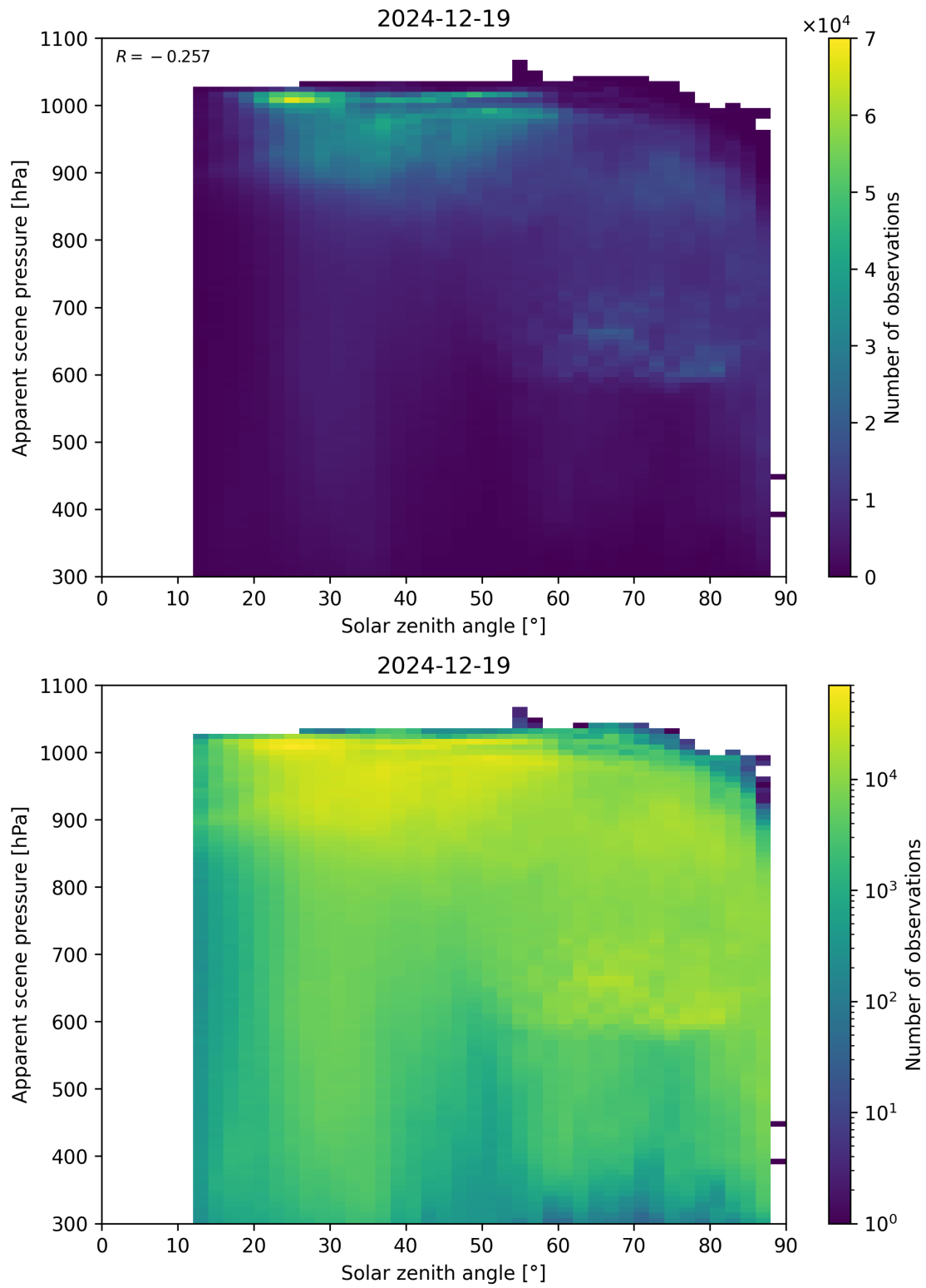
Figure 108: Scatter density plot of “Solar zenith angle” against “Apparent scene pressure” for 2024-12-18 to 2024-12-20.
