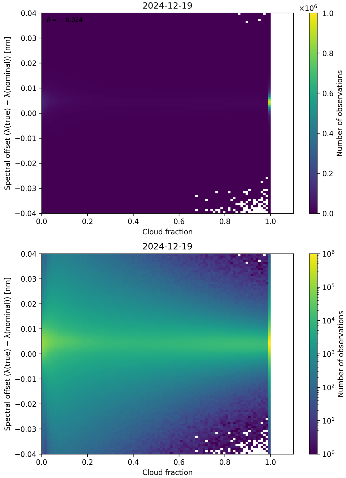
Figure 76: Scatter density plot of “Cloud fraction” against “Spectral offset ( \lambda_{\text{true}} - \lambda_{\text{nominal}} )” for 2024-12-18 to 2024-12-20.
