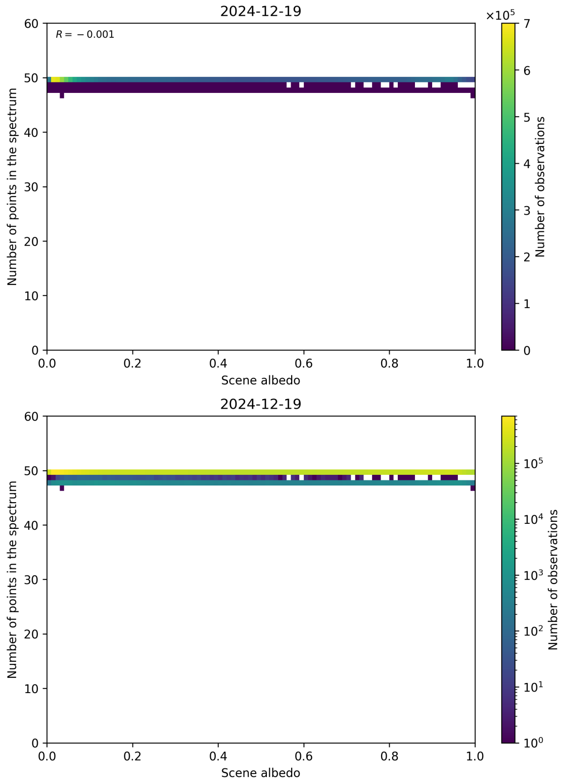
Figure 106: Scatter density plot of “Scene albedo” against “Number of points in the spectrum” for 2024-12-18 to 2024-12-20.
