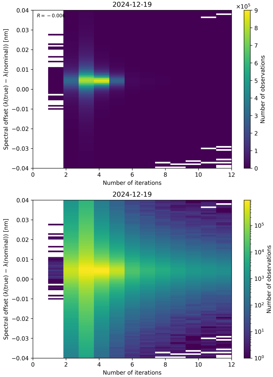
Figure 100: Scatter density plot of “Number of iterations” against “Spectral offset ( \lambda_{\text{true}} - \lambda_{\text{nominal}} )” for 2024-12-18 to 2024-12-20.
