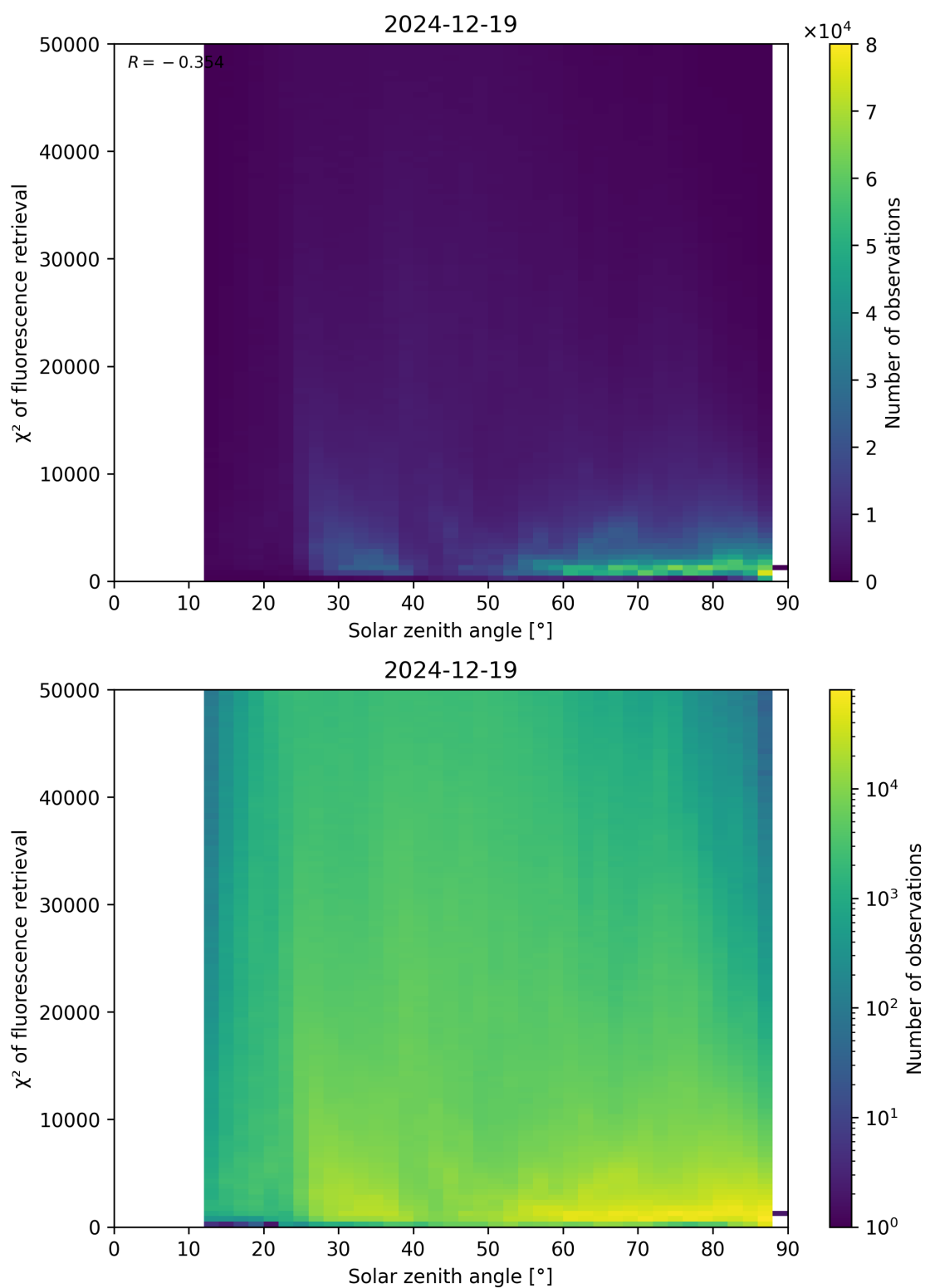
Figure 109: Scatter density plot of “Solar zenith angle” against “ \chi^2 of fluorescence retrieval” for 2024-12-18 to 2024-12-20.
