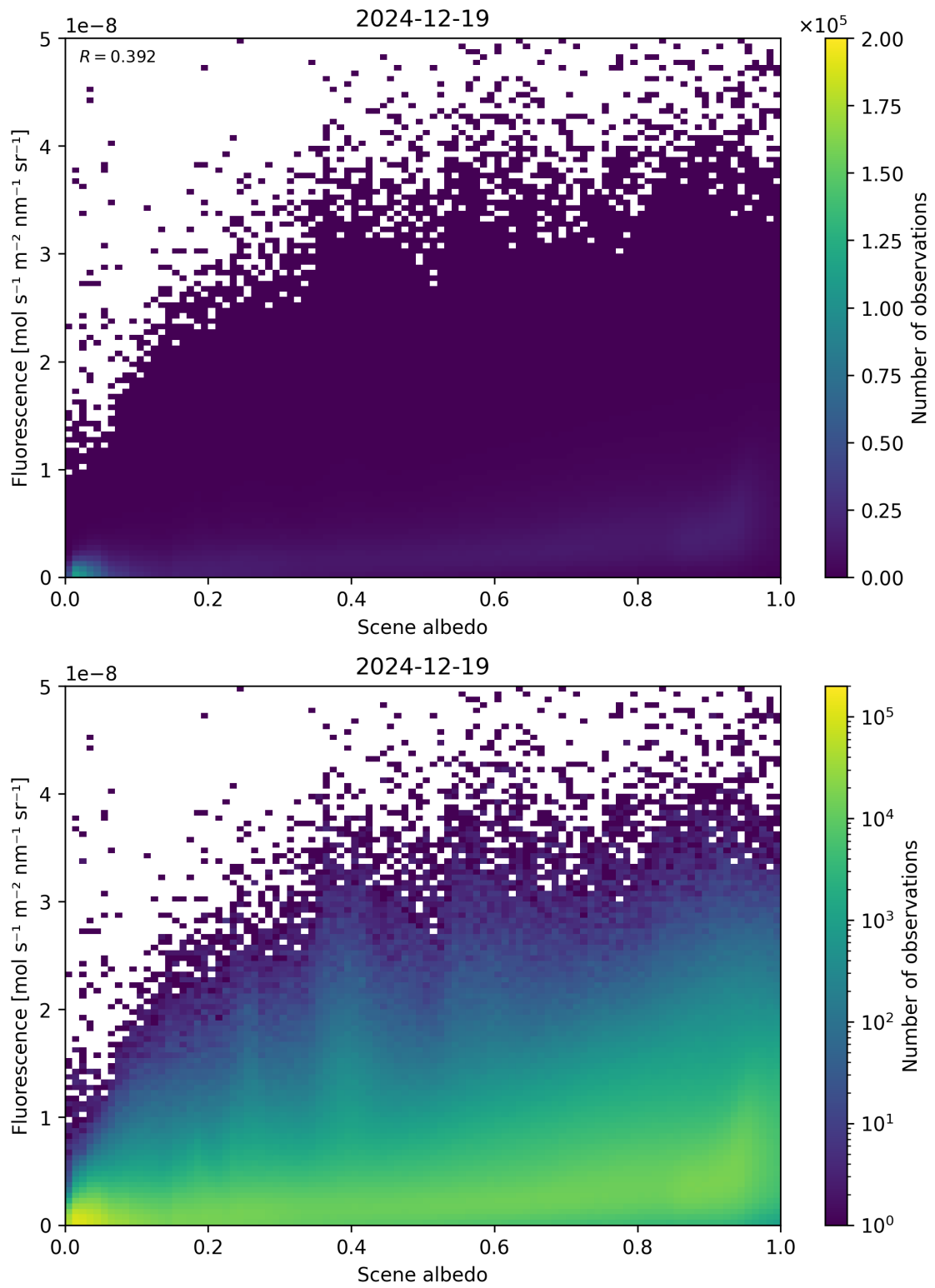
Figure 104: Scatter density plot of “Scene albedo” against “Fluorescence” for 2024-12-18 to 2024-12-20.
