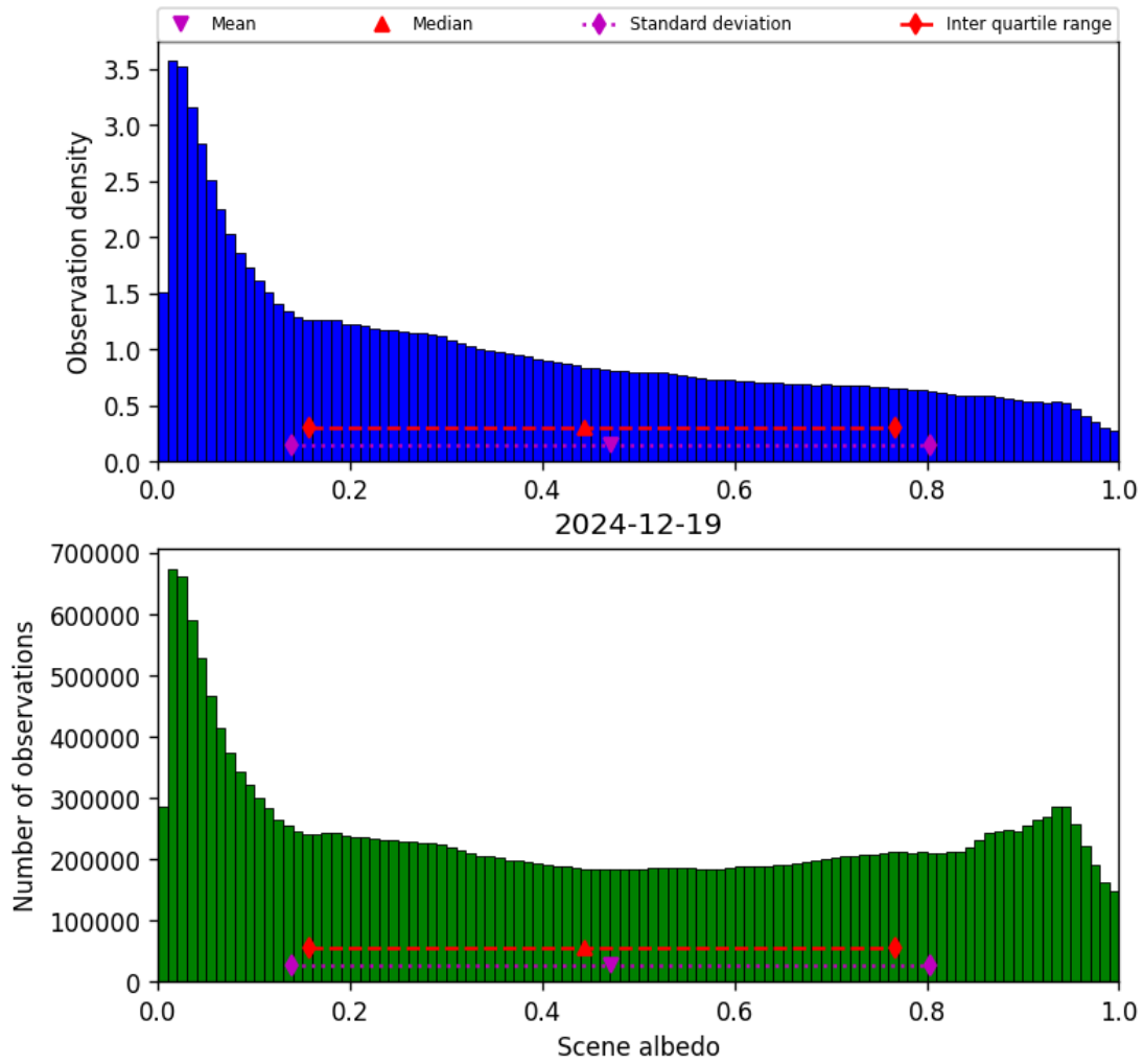
Figure 34: Histogram of “Scene albedo” for 2024-12-18 to 2024-12-20
