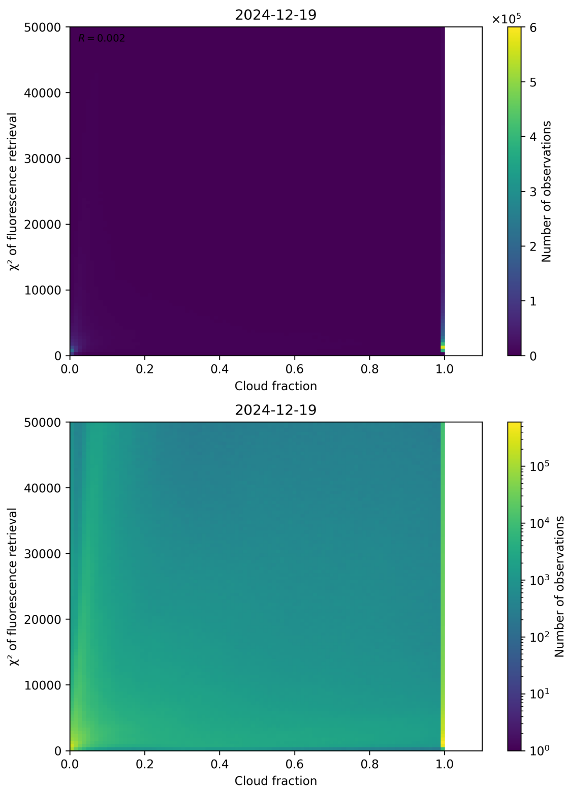
Figure 71: Scatter density plot of “Cloud fraction” against “ \chi^2 of fluorescence retrieval” for 2024-12-18 to 2024-12-20.
