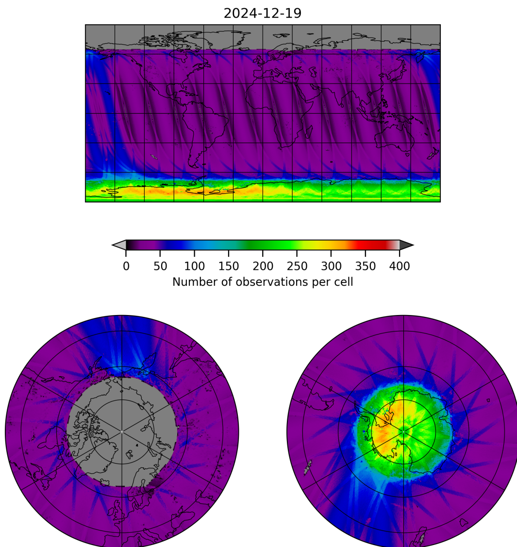
Figure 11: Map of the number of observations for 2024-12-18 to 2024-12-20
