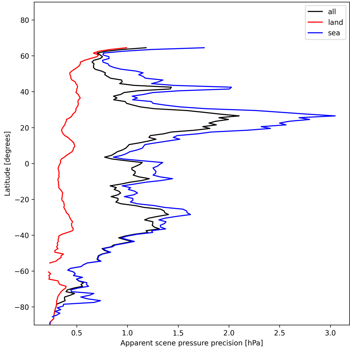
Figure 20: Zonal average of “Apparent scene pressure precision” for 2024-12-18 to 2024-12-20.
