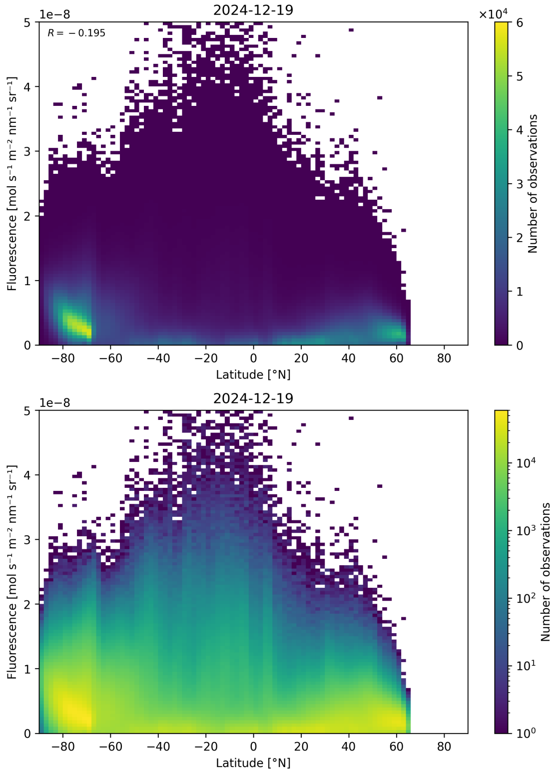
Figure 92: Scatter density plot of “Latitude” against “Fluorescence” for 2024-12-18 to 2024-12-20.
