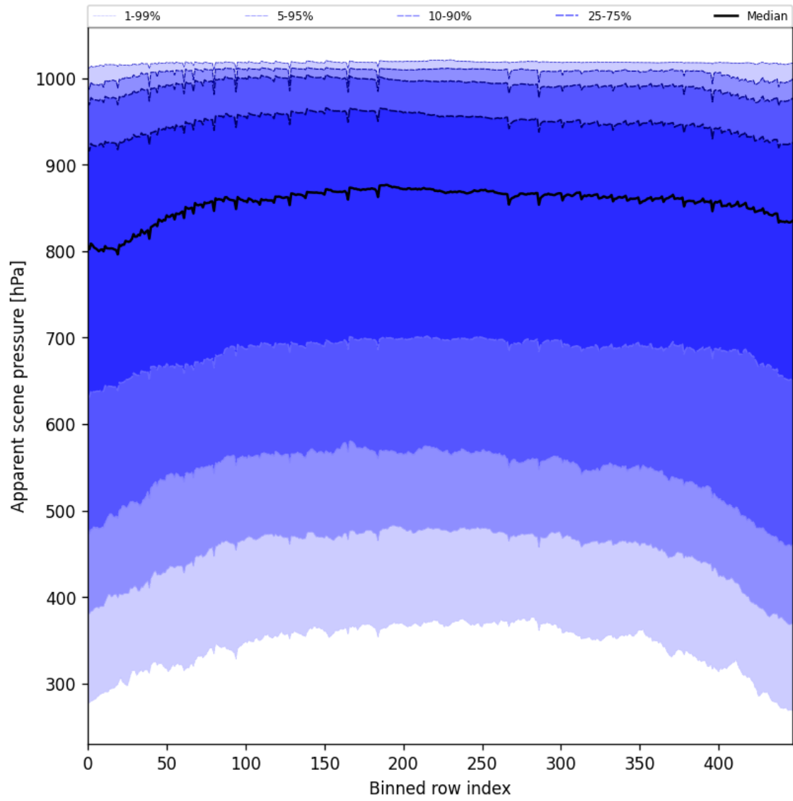
Figure 53: Along track statistics of “Apparent scene pressure” for 2024-12-18 to 2024-12-20
