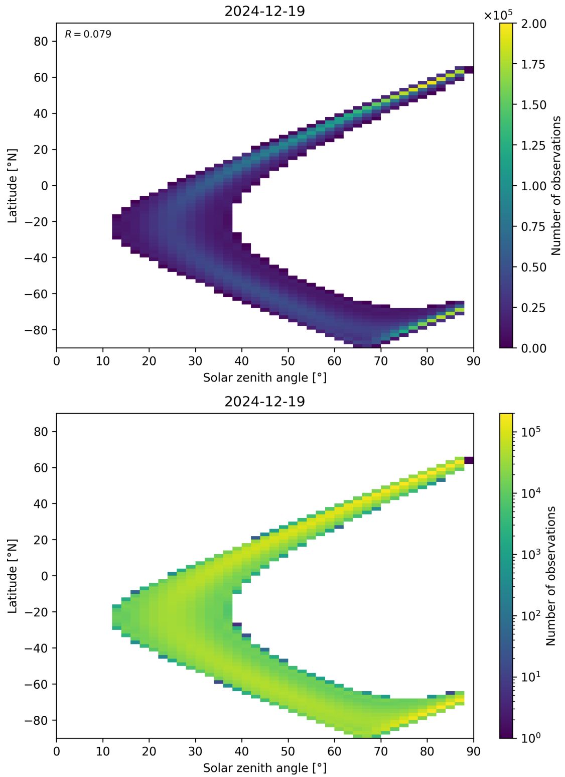
Figure 113: Scatter density plot of “Solar zenith angle” against “Latitude” for 2024-12-18 to 2024-12-20.
