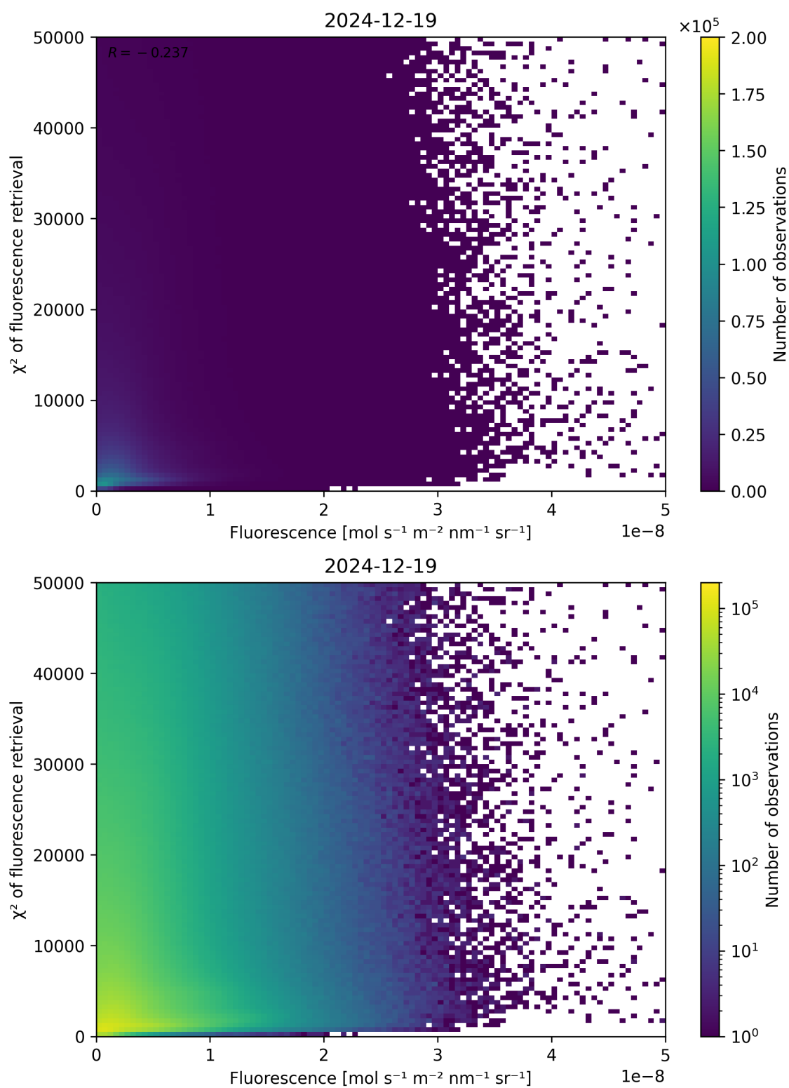
Figure 85: Scatter density plot of “Fluorescence” against “ \chi^2 of fluorescence retrieval” for 2024-12-18 to 2024-12-20.
