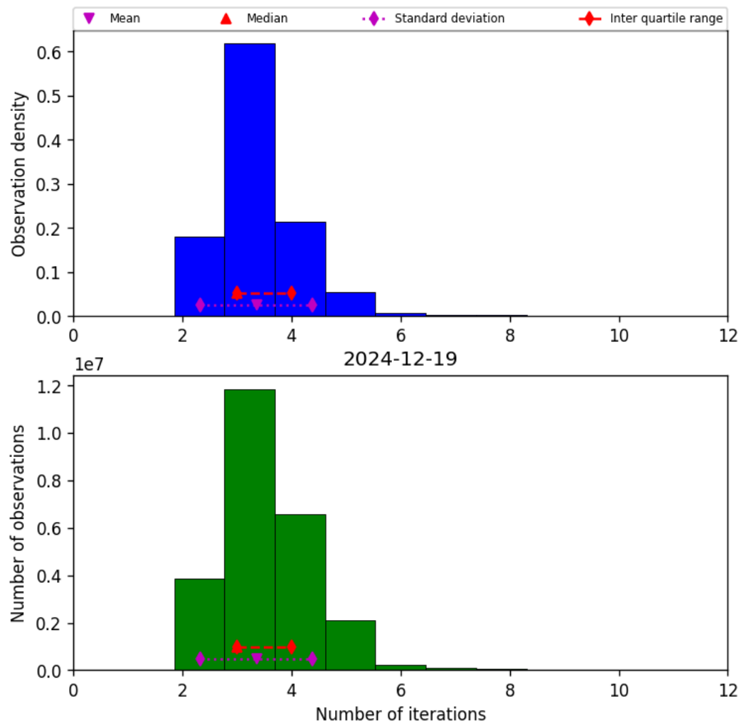
Figure 39: Histogram of “Number of iterations” for 2024-12-18 to 2024-12-20
