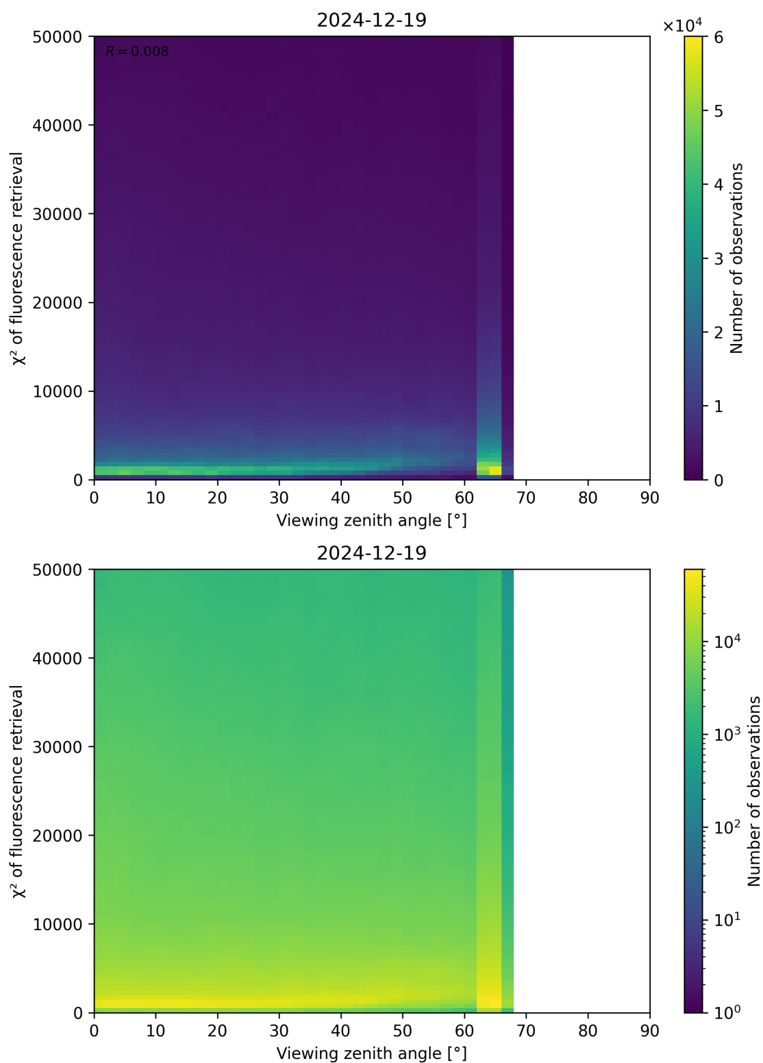
Figure 119: Scatter density plot of “Viewing zenith angle” against “ \chi^2 of fluorescence retrieval” for 2024-12-18 to 2024-12-20.
