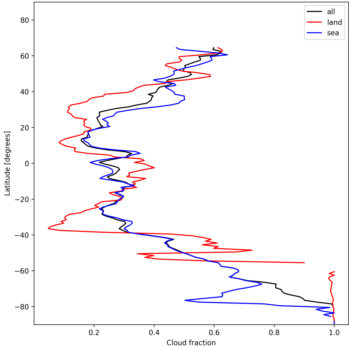
Figure 15: Zonal average of “Cloud fraction” for 2024-12-18 to 2024-12-20.
