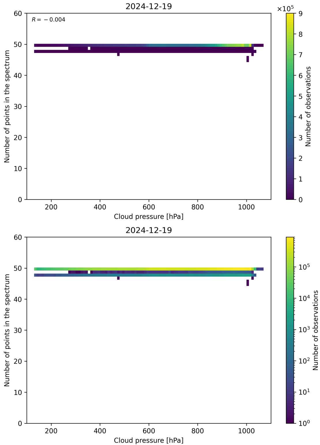
Figure 82: Scatter density plot of “Cloud pressure” against “Number of points in the spectrum” for 2024-12-18 to 2024-12-20.
