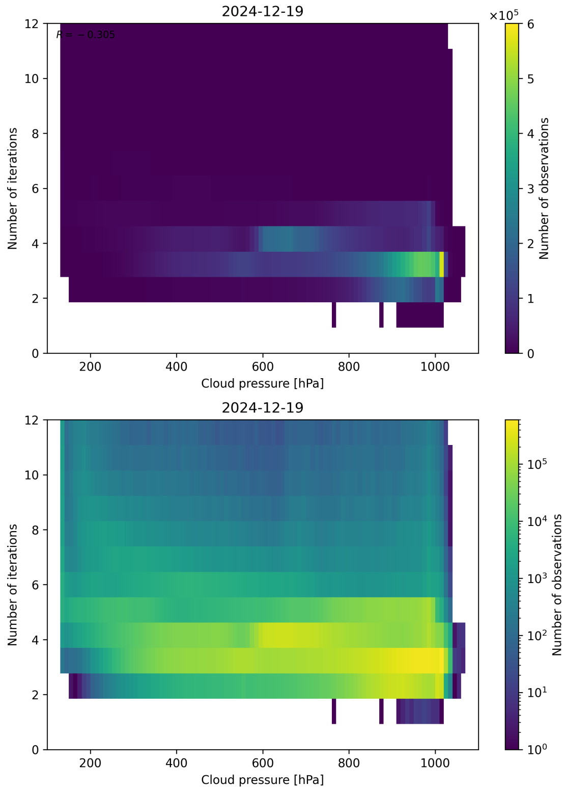
Figure 81: Scatter density plot of “Cloud pressure” against “Number of iterations” for 2024-12-18 to 2024-12-20.
