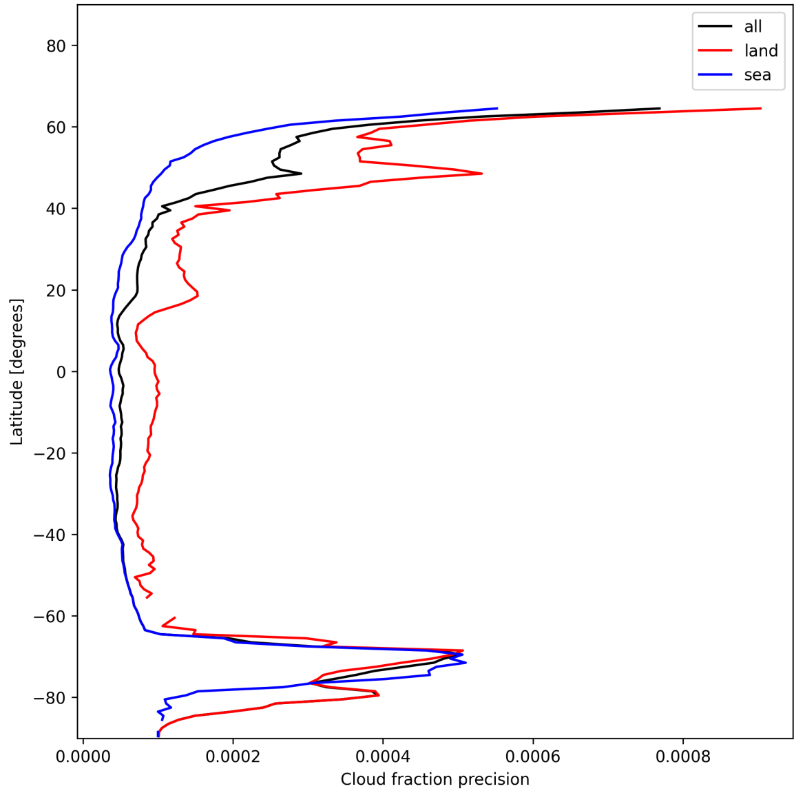
Figure 16: Zonal average of “Cloud fraction precision” for 2024-12-18 to 2024-12-20.
