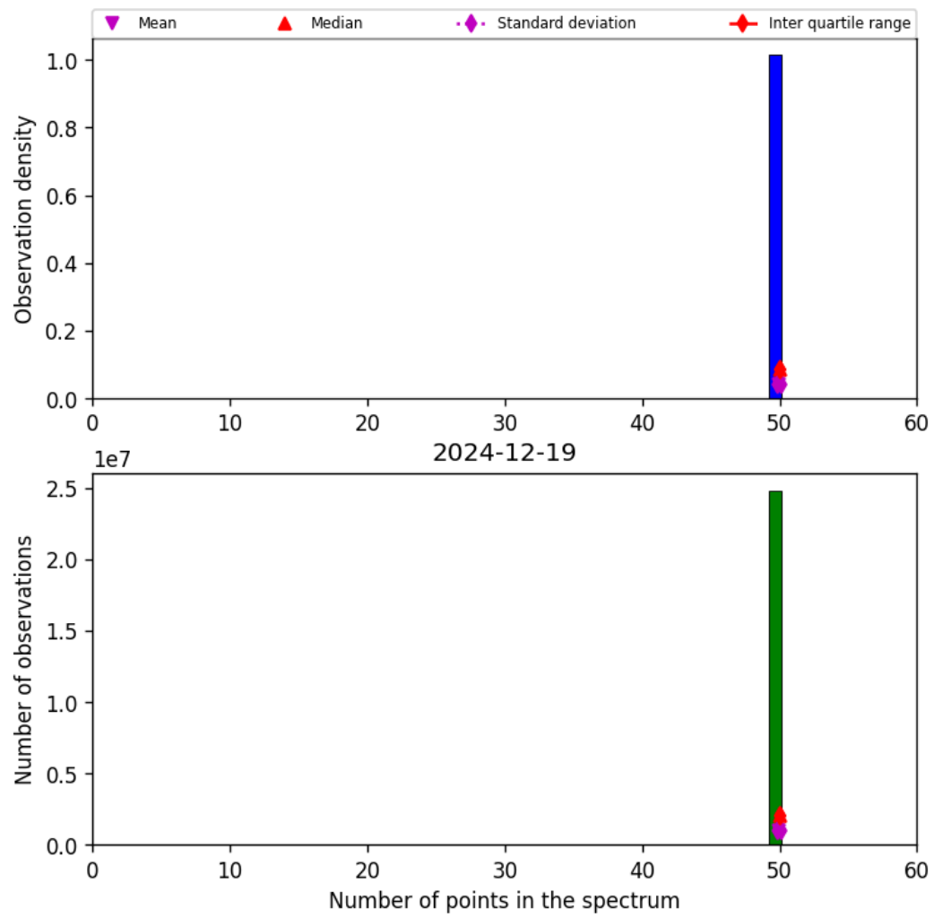
Figure 44: Histogram of “Number of points in the spectrum” for 2024-12-18 to 2024-12-20
