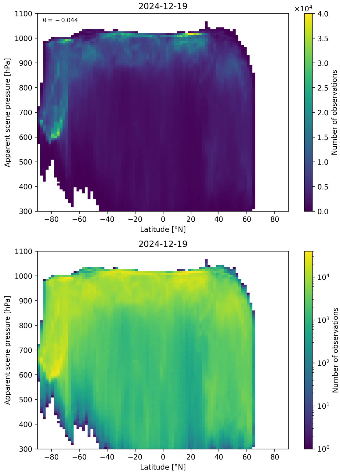
Figure 88: Scatter density plot of “Latitude” against “Apparent scene pressure” for 2024-12-18 to 2024-12-20.
