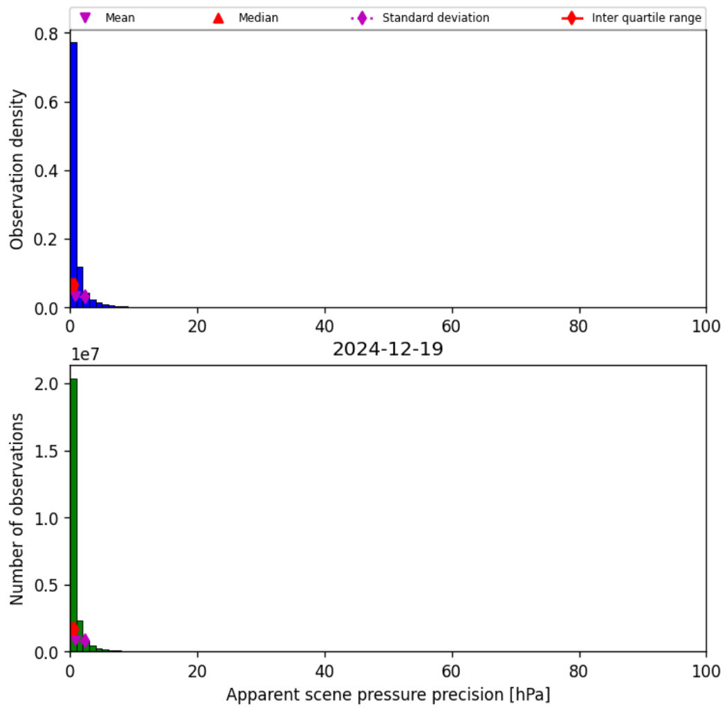
Figure 37: Histogram of “Apparent scene pressure precision” for 2024-12-18 to 2024-12-20
