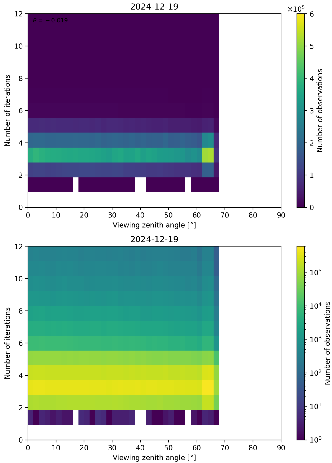
Figure 124: Scatter density plot of “Viewing zenith angle” against “Number of iterations” for 2024-12-18 to 2024-12-20.
