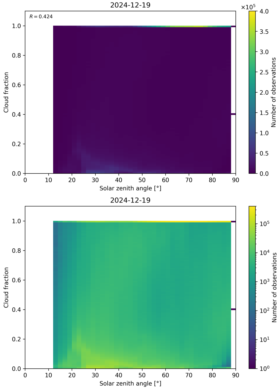
Figure 110: Scatter density plot of “Solar zenith angle” against “Cloud fraction” for 2024-12-18 to 2024-12-20.
