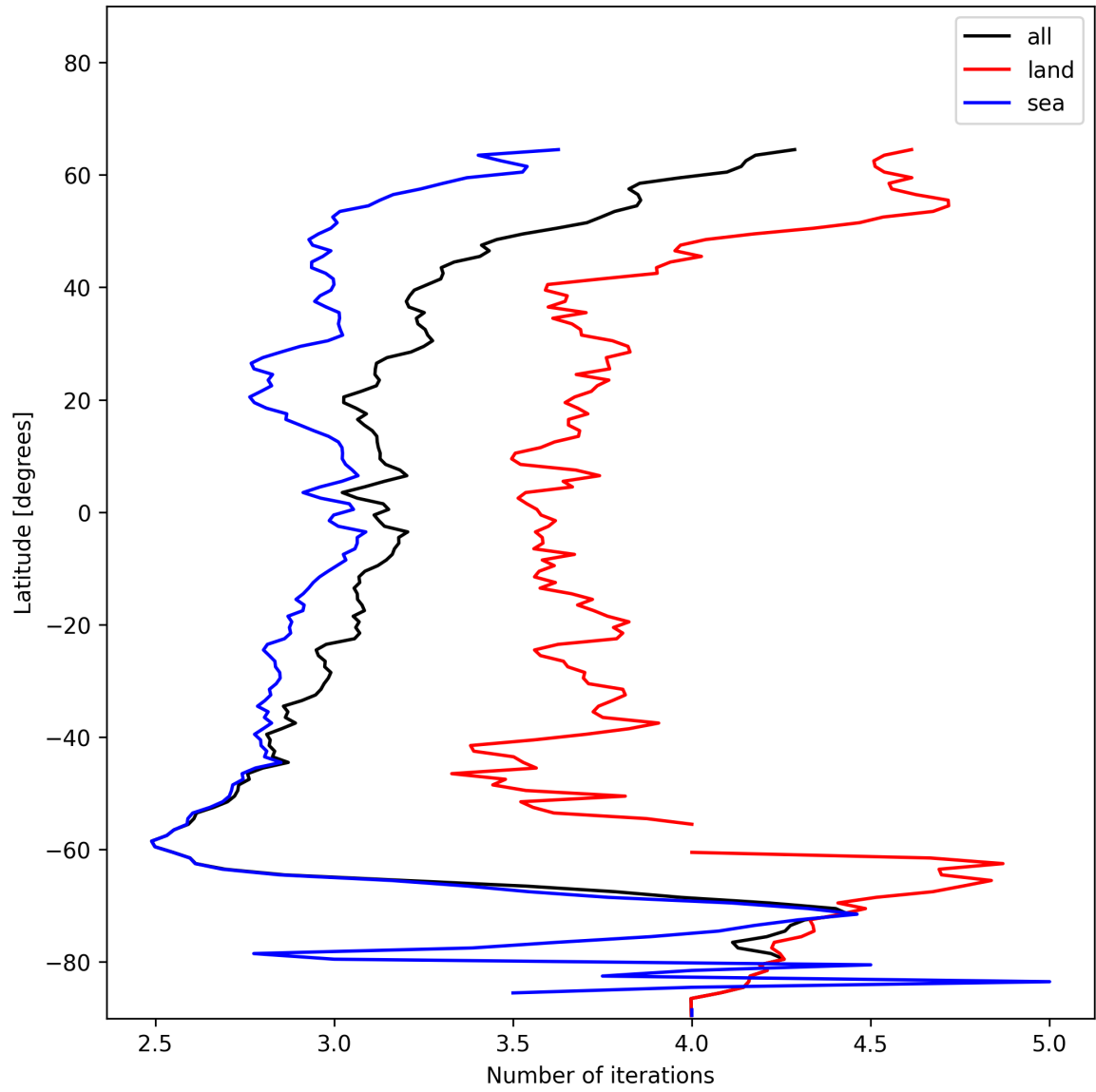
Figure 22: Zonal average of “Number of iterations” for 2024-12-18 to 2024-12-20.
