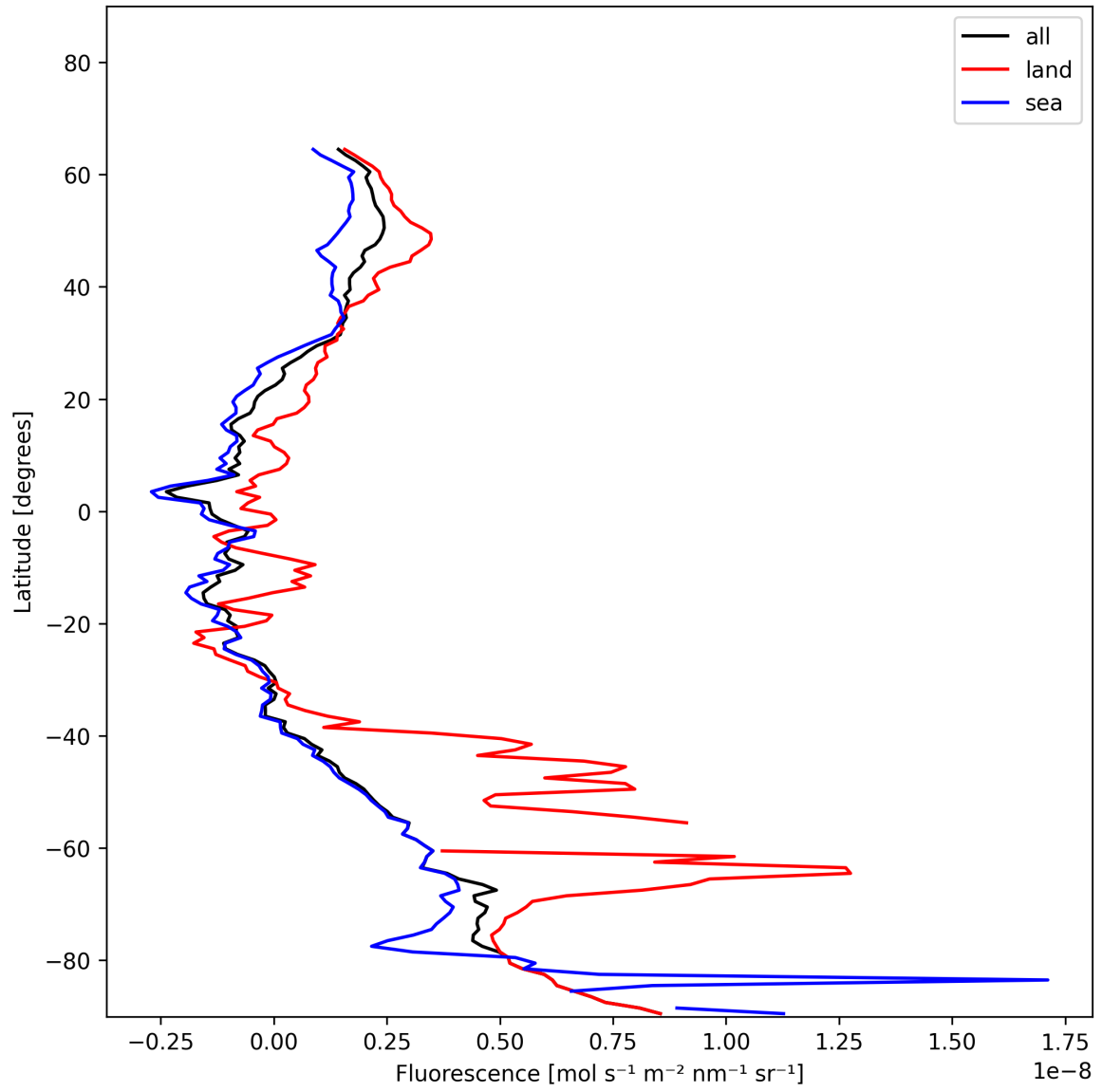
Figure 23: Zonal average of “Fluorescence” for 2024-12-18 to 2024-12-20.
