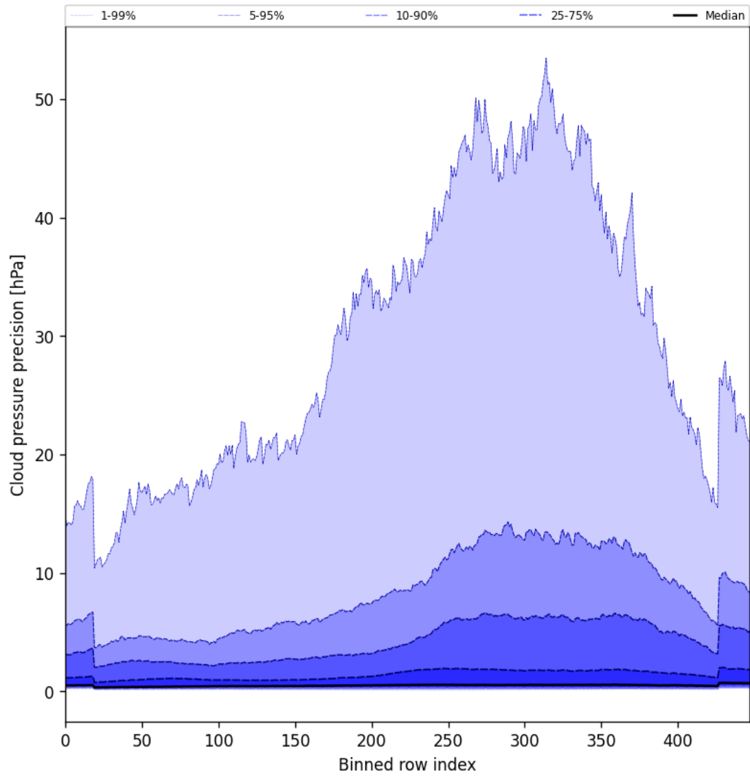
Figure 48: Along track statistics of “Cloud pressure precision” for 2024-12-18 to 2024-12-20
