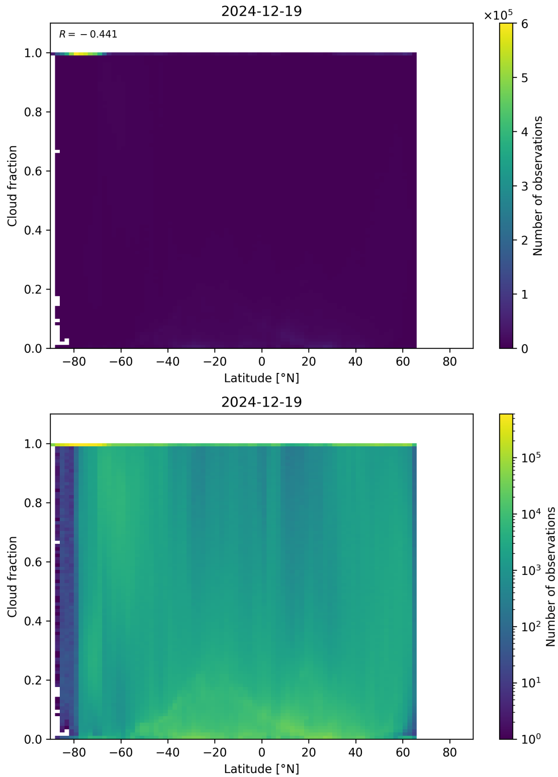
Figure 90: Scatter density plot of “Latitude” against “Cloud fraction” for 2024-12-18 to 2024-12-20.
