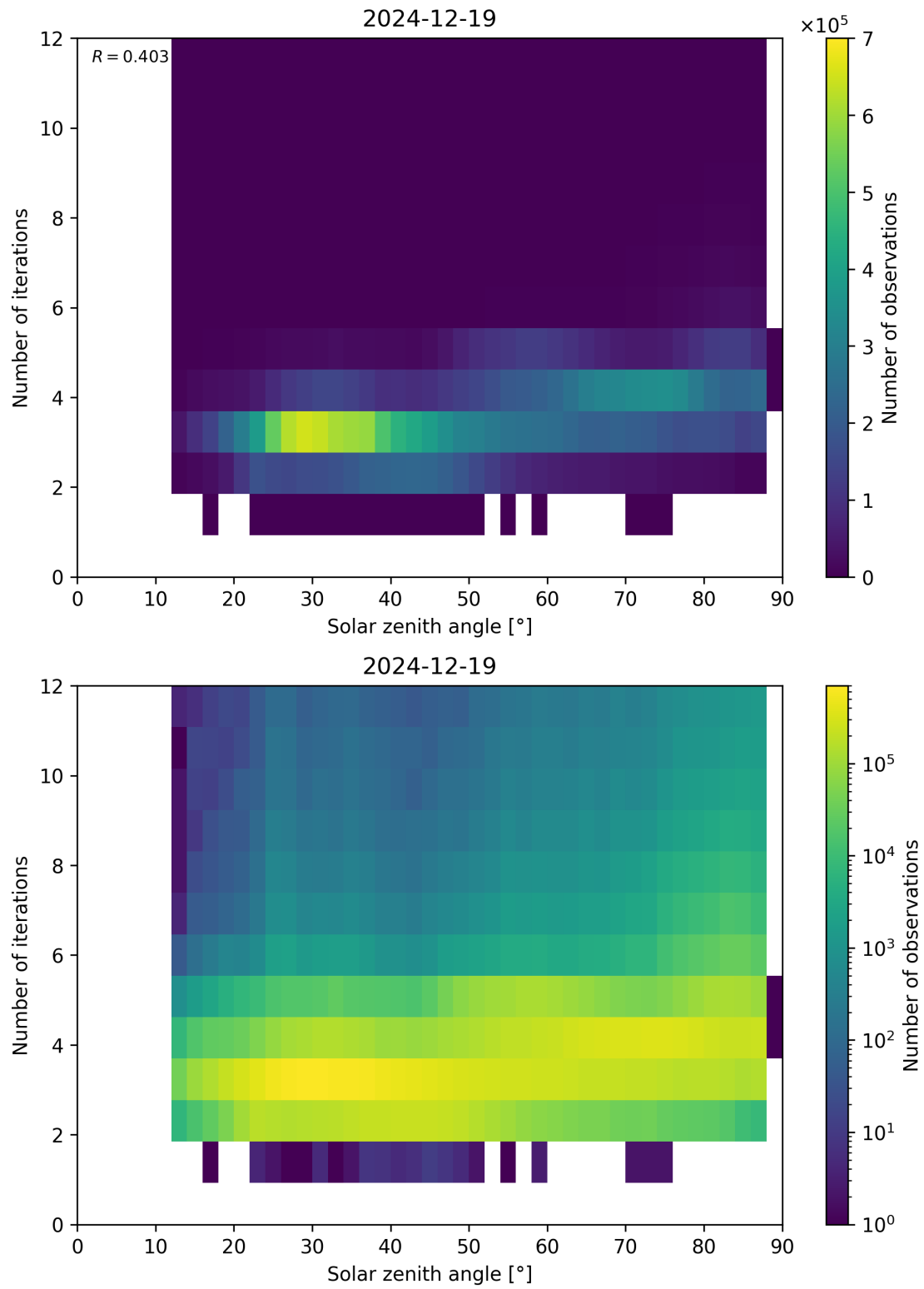
Figure 114: Scatter density plot of “Solar zenith angle” against “Number of iterations” for 2024-12-18 to 2024-12-20.
