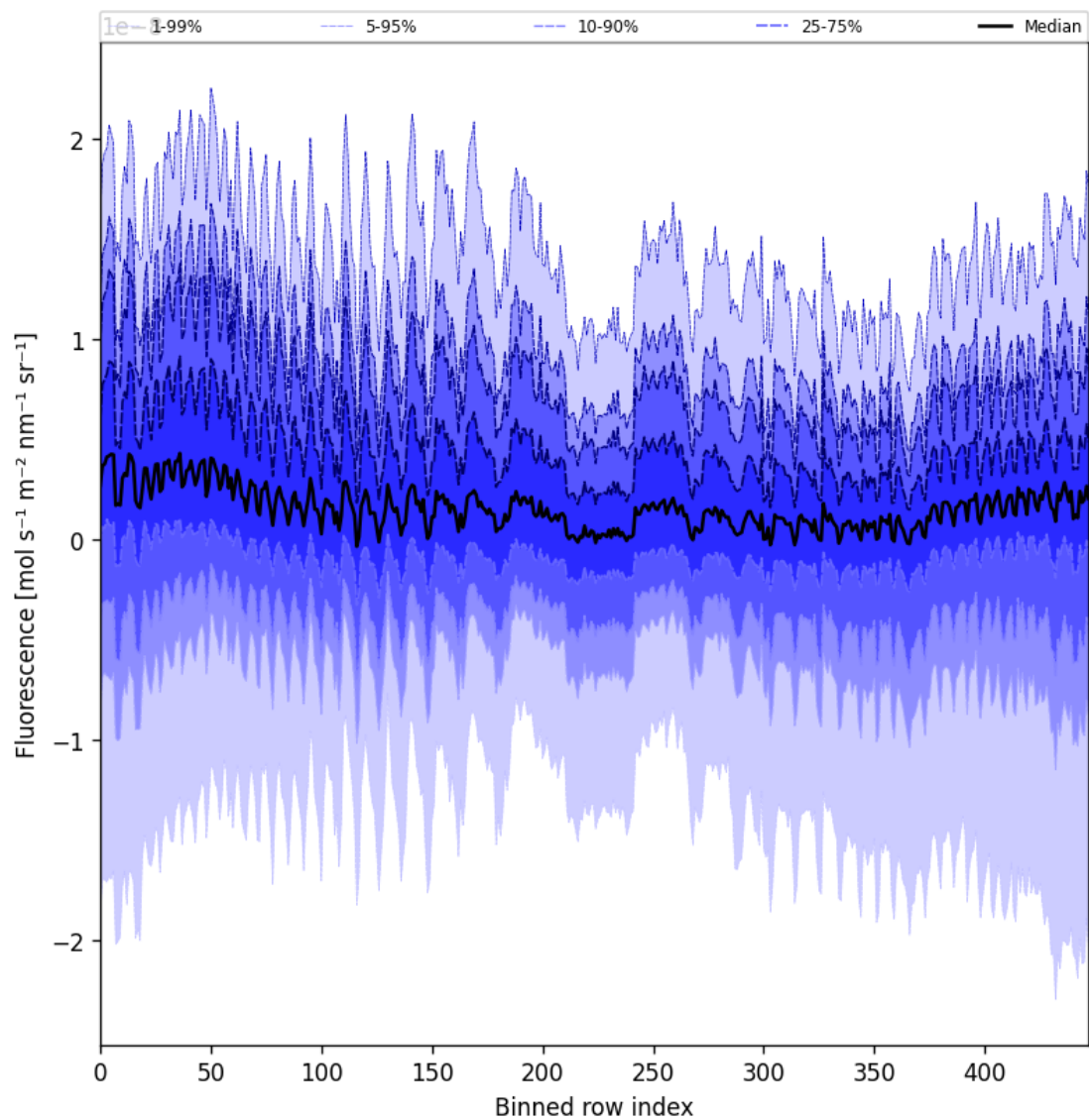
Figure 57: Along track statistics of “Fluorescence” for 2024-12-18 to 2024-12-20
