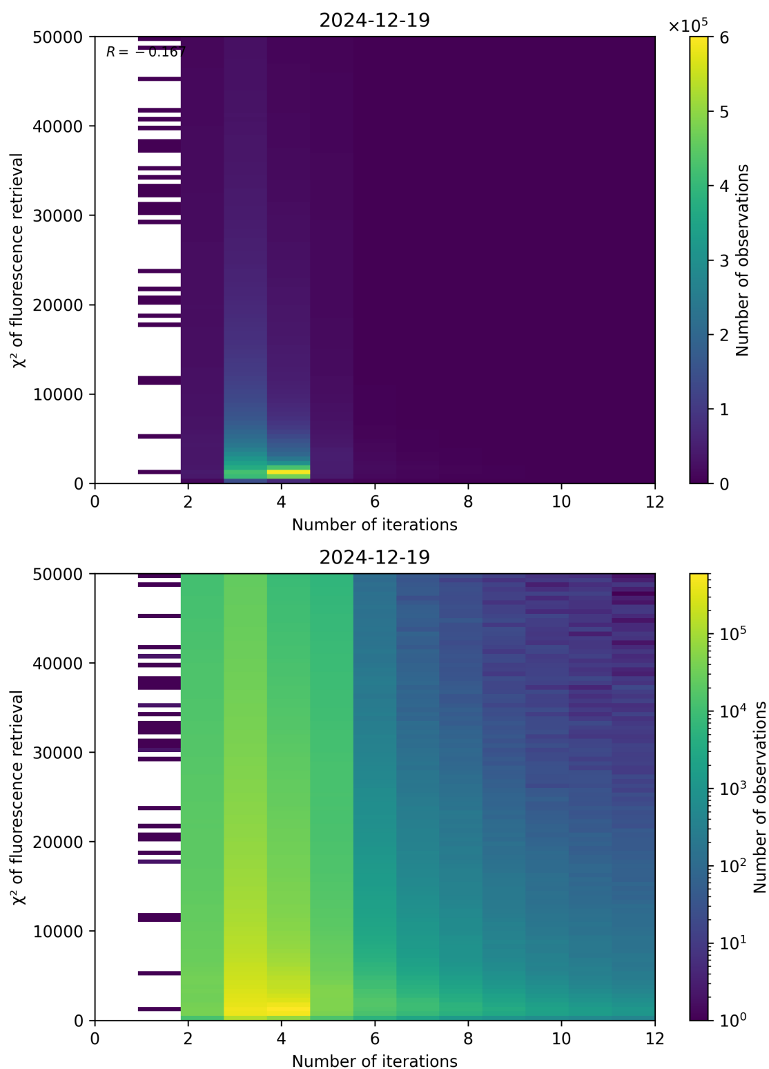
Figure 97: Scatter density plot of “Number of iterations” against “ \chi^2 of fluorescence retrieval” for 2024-12-18 to 2024-12-20.
