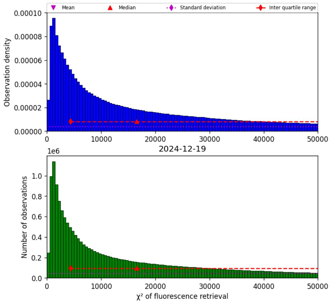
Figure 42: Histogram of “ \chi^2 of fluorescence retrieval” for 2024-12-18 to 2024-12-20
