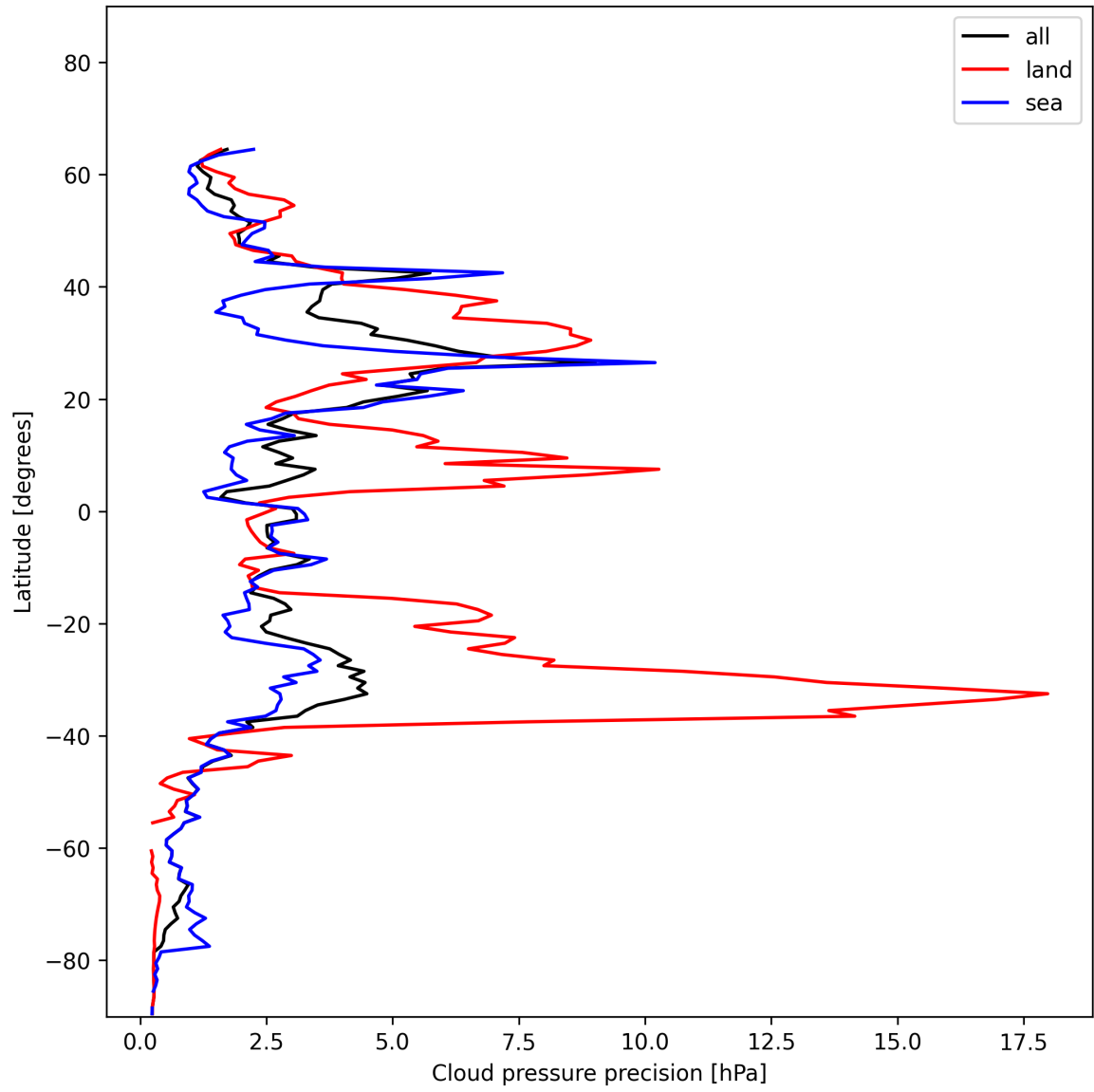
Figure 14: Zonal average of “Cloud pressure precision” for 2024-12-18 to 2024-12-20.
