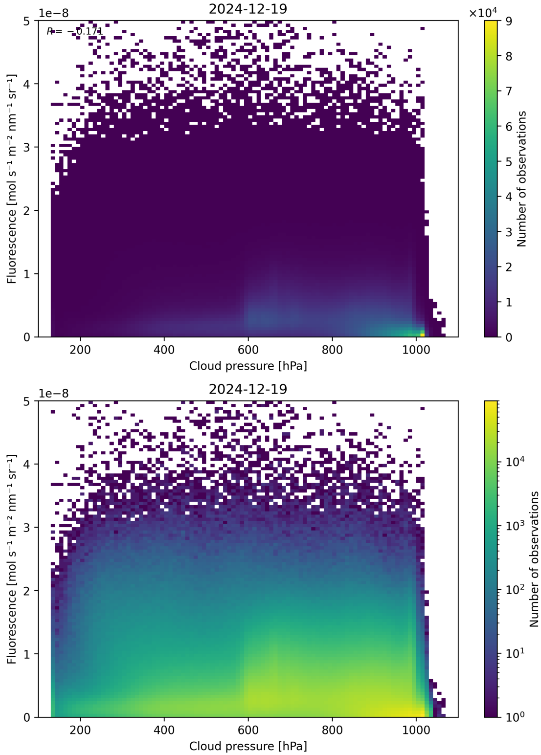
Figure 80: Scatter density plot of “Cloud pressure” against “Fluorescence” for 2024-12-18 to 2024-12-20.
