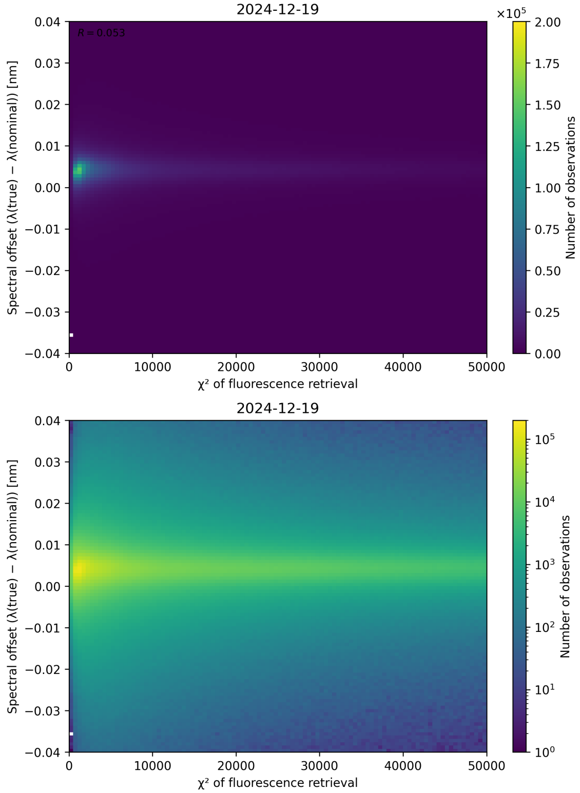
Figure 69: Scatter density plot of “ \chi^2 of fluorescence retrieval” against “Spectral offset ( \lambda_{\text{true}} - \lambda_{\text{nominal}} )” for 2024-12-18 to 2024-12-20.
