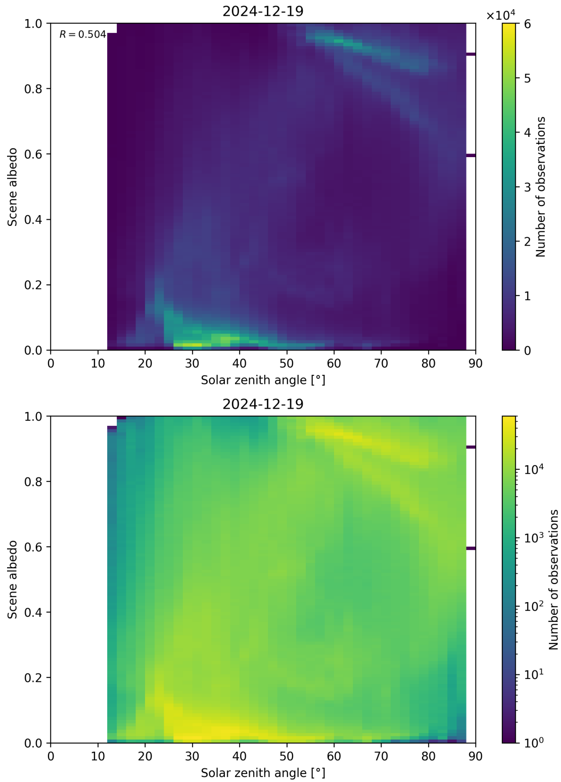
Figure 116: Scatter density plot of “Solar zenith angle” against “Scene albedo” for 2024-12-18 to 2024-12-20.
