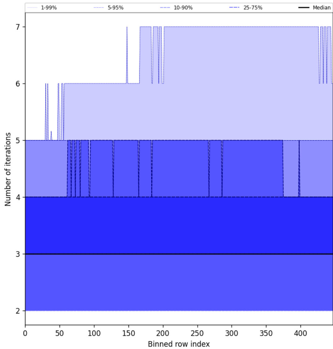
Figure 56: Along track statistics of “Number of iterations” for 2024-12-18 to 2024-12-20
