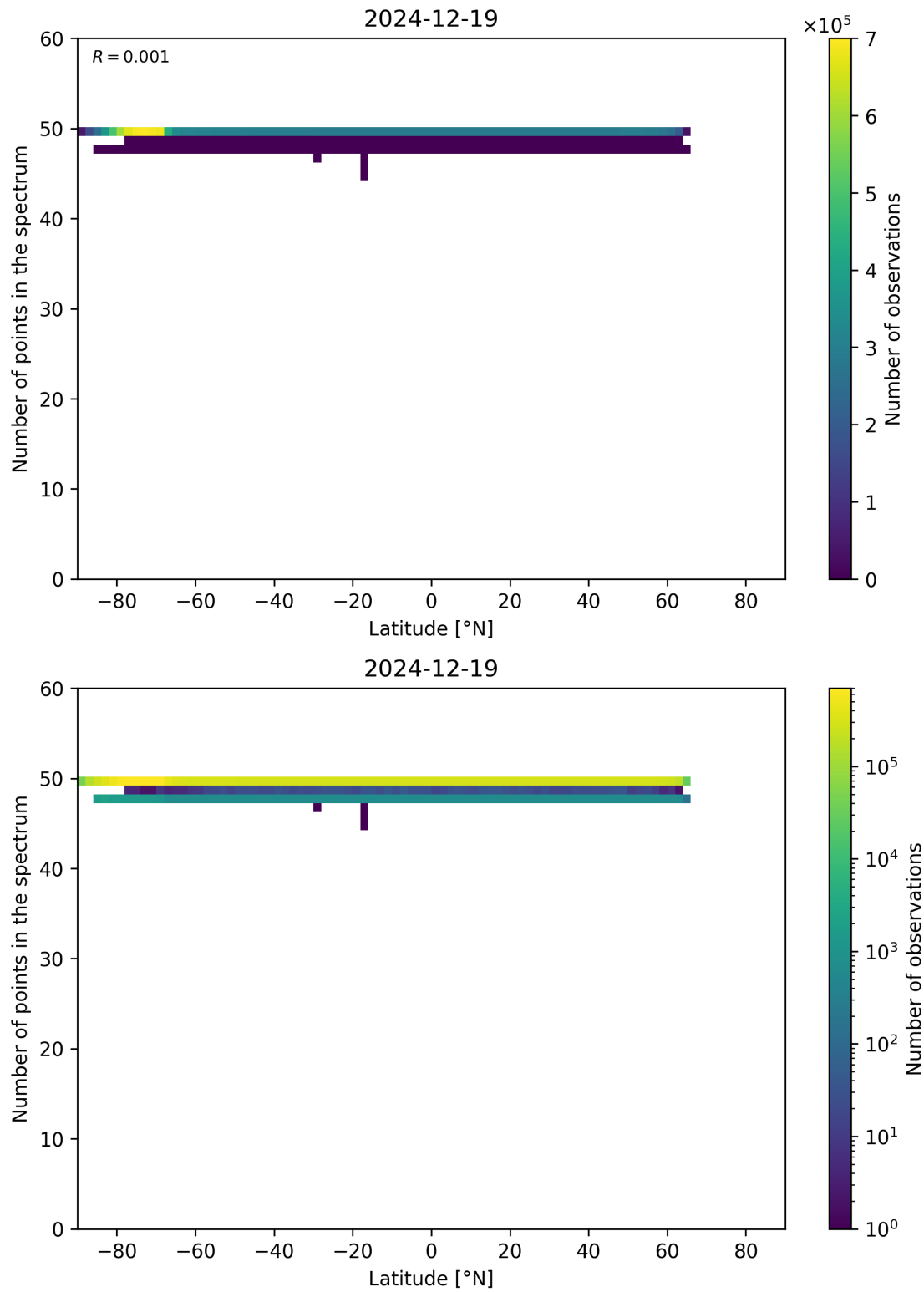
Figure 94: Scatter density plot of “Latitude” against “Number of points in the spectrum” for 2024-12-18 to 2024-12-20.
