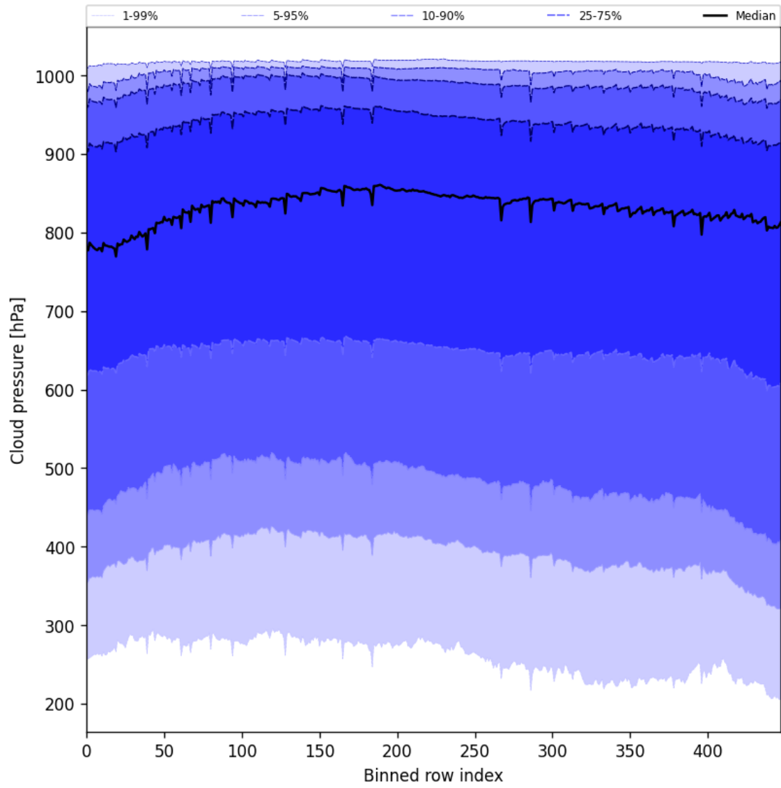
Figure 47: Along track statistics of “Cloud pressure” for 2024-12-18 to 2024-12-20
