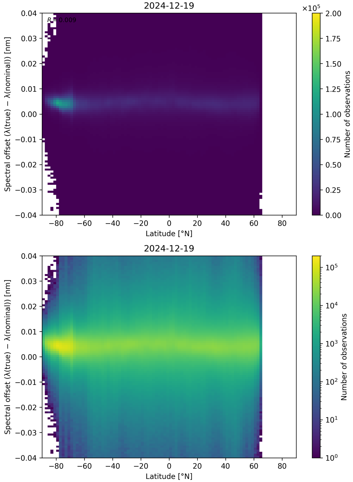
Figure 96: Scatter density plot of “Latitude” against “Spectral offset ( \lambda_{\text{true}} - \lambda_{\text{nominal}} )” for 2024-12-18 to 2024-12-20.
