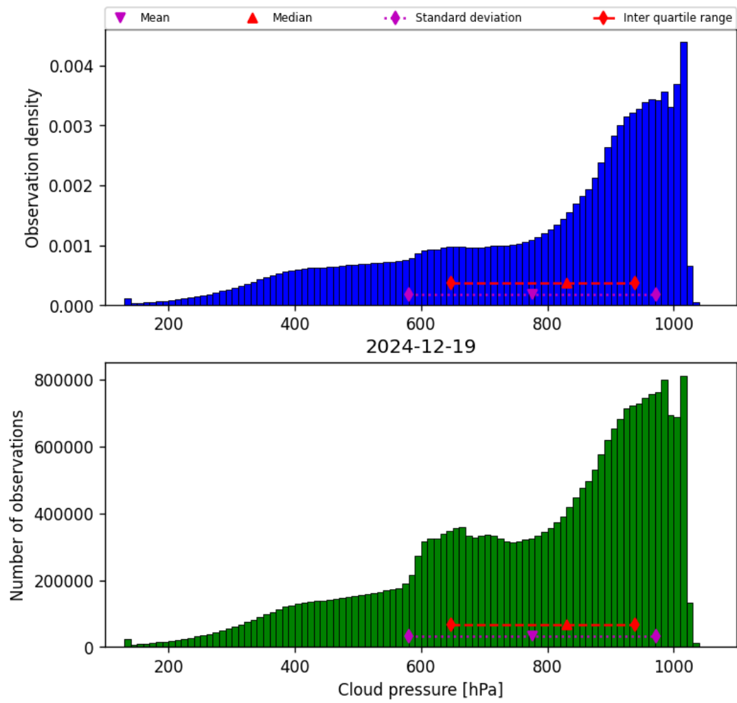
Figure 30: Histogram of “Cloud pressure” for 2024-12-18 to 2024-12-20
