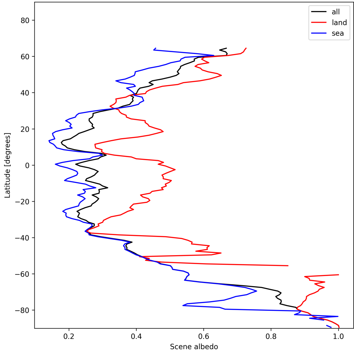
Figure 17: Zonal average of “Scene albedo” for 2024-12-18 to 2024-12-20.
