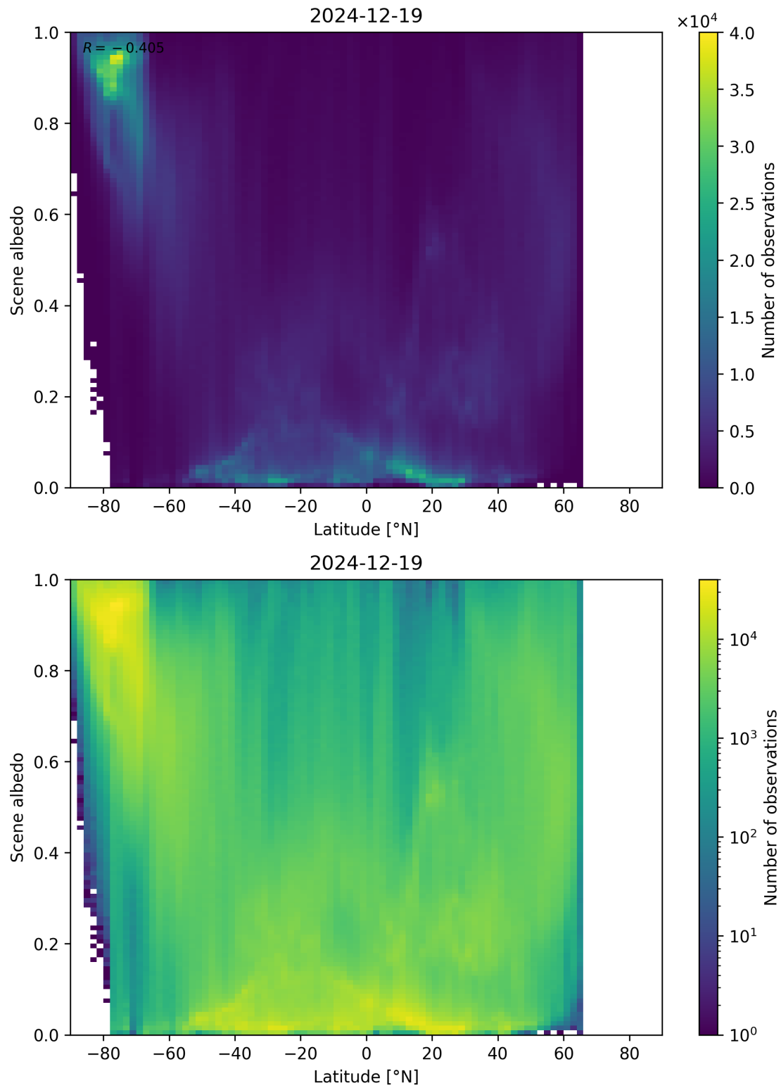
Figure 95: Scatter density plot of “Latitude” against “Scene albedo” for 2024-12-18 to 2024-12-20.
