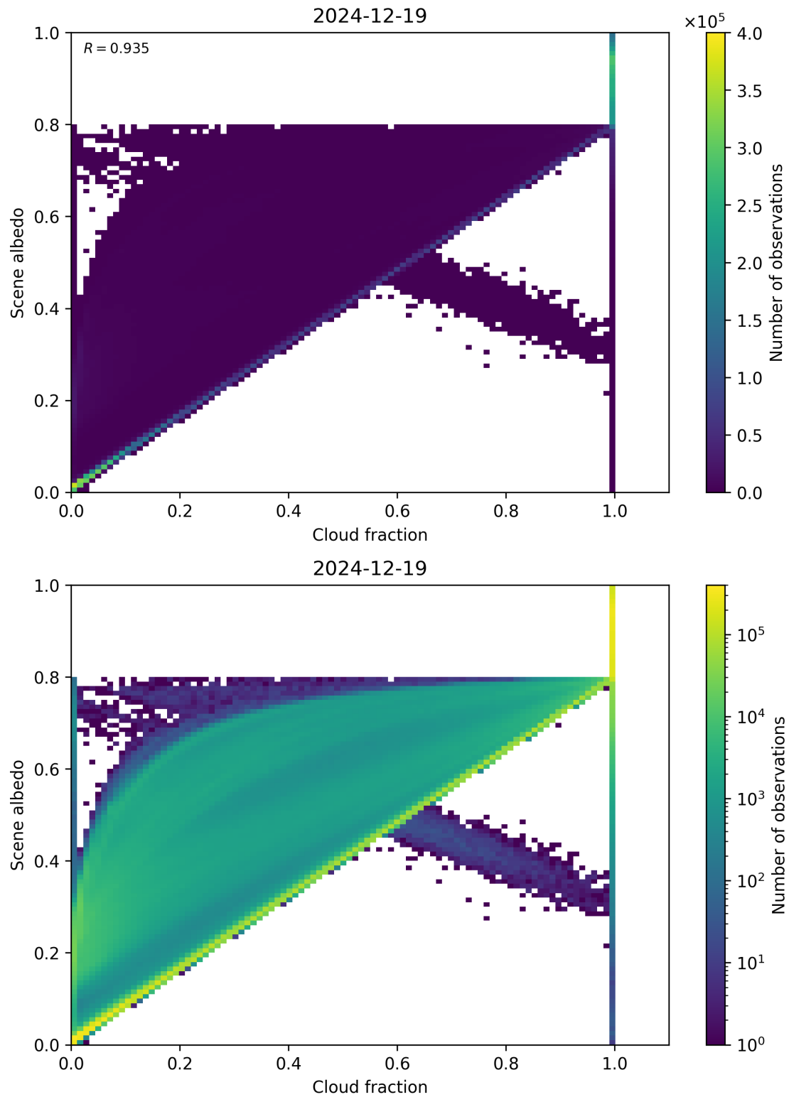
Figure 75: Scatter density plot of “Cloud fraction” against “Scene albedo” for 2024-12-18 to 2024-12-20.
