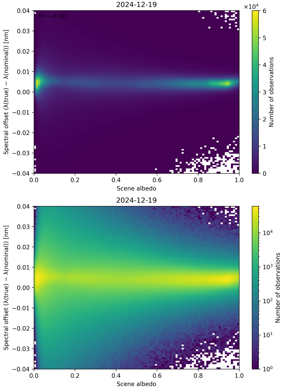
Figure 107: Scatter density plot of “Scene albedo” against “Spectral offset ( \lambda_{\text{true}} - \lambda_{\text{nominal}} )” for 2024-12-18 to 2024-12-20.
