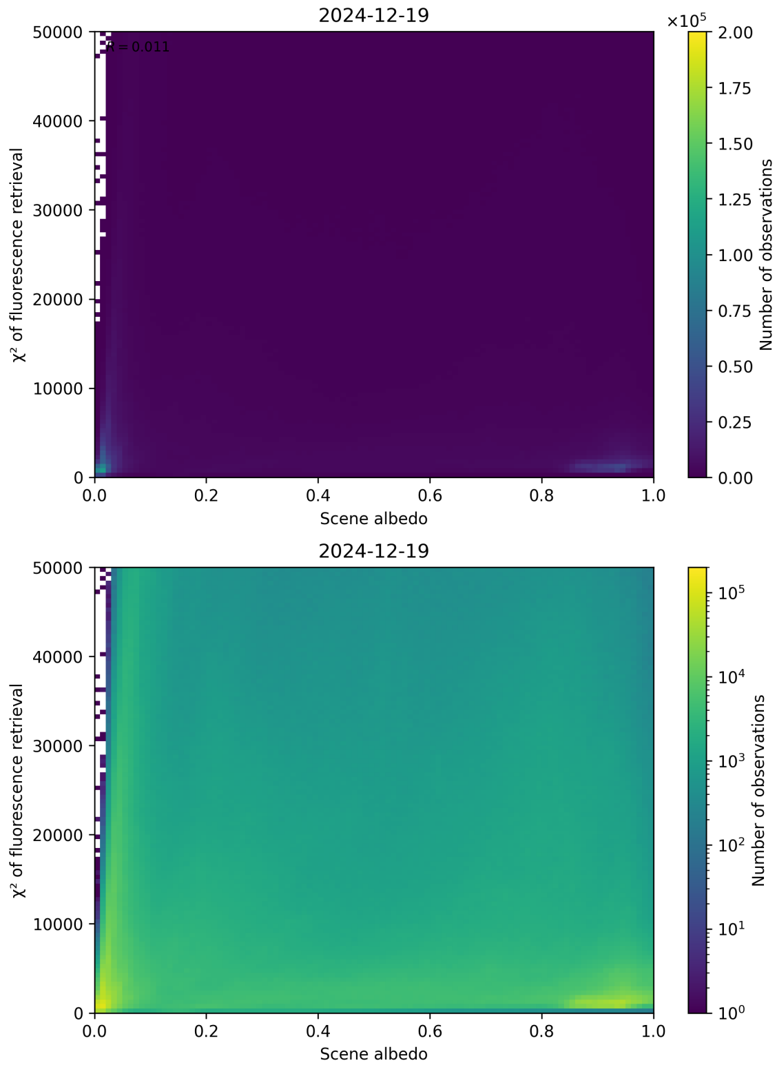
Figure 103: Scatter density plot of “Scene albedo” against “ \chi^2 of fluorescence retrieval” for 2024-12-18 to 2024-12-20.
