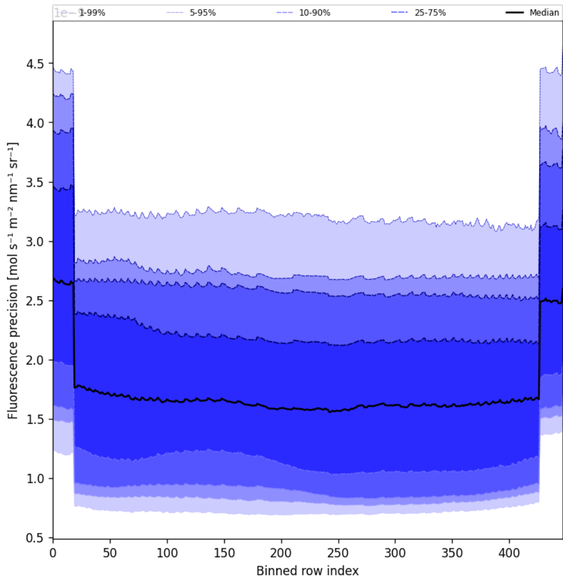
Figure 58: Along track statistics of “Fluorescence precision” for 2024-12-18 to 2024-12-20
