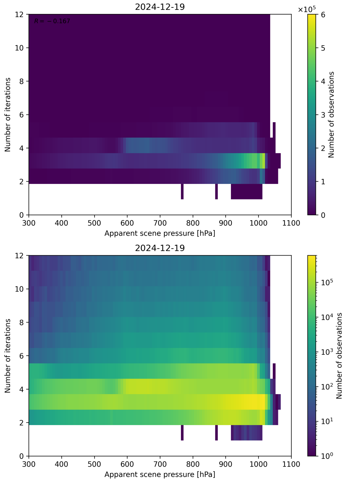
Figure 65: Scatter density plot of “Apparent scene pressure” against “Number of iterations” for 2024-12-18 to 2024-12-20.
