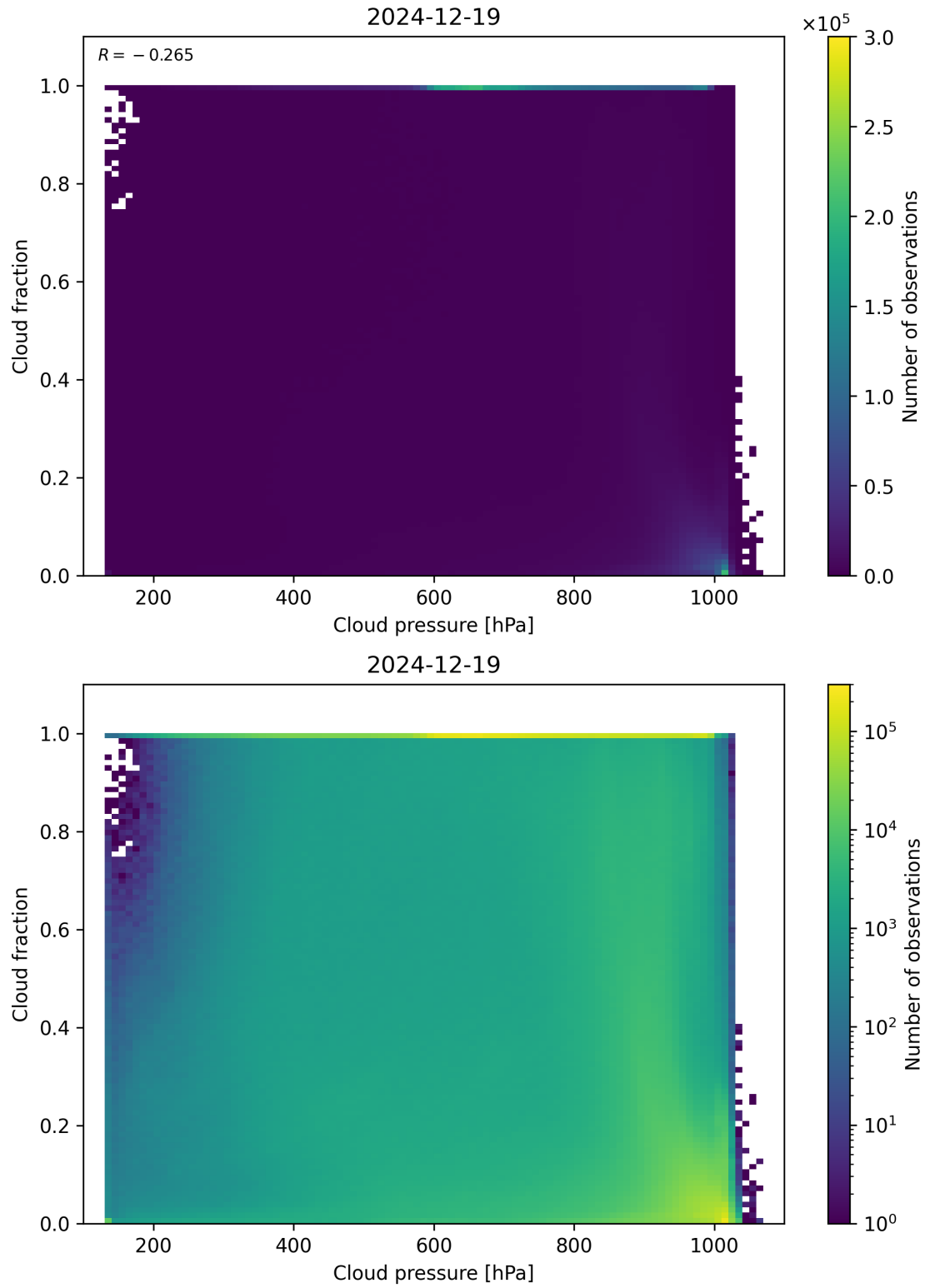
Figure 79: Scatter density plot of “Cloud pressure” against “Cloud fraction” for 2024-12-18 to 2024-12-20.
