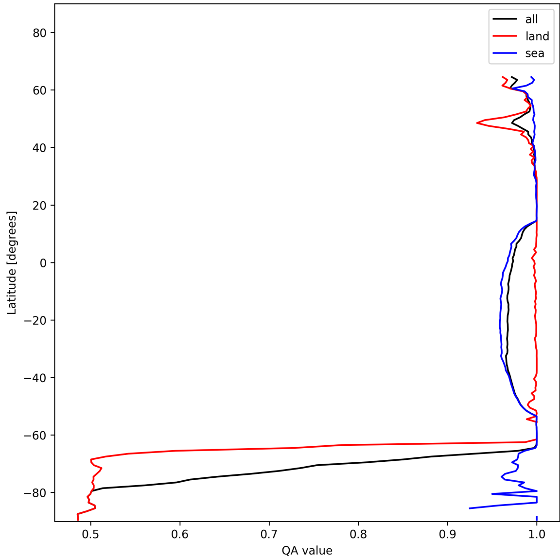
Figure 12: Zonal average of “QA value” for 2024-12-18 to 2024-12-20.
