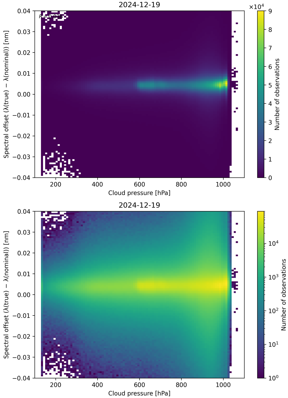
Figure 84: Scatter density plot of “Cloud pressure” against “Spectral offset ( \lambda_{\text{true}} - \lambda_{\text{nominal}} )” for 2024-12-18 to 2024-12-20.
