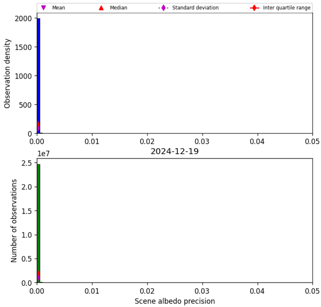
Figure 35: Histogram of “Scene albedo precision” for 2024-12-18 to 2024-12-20
