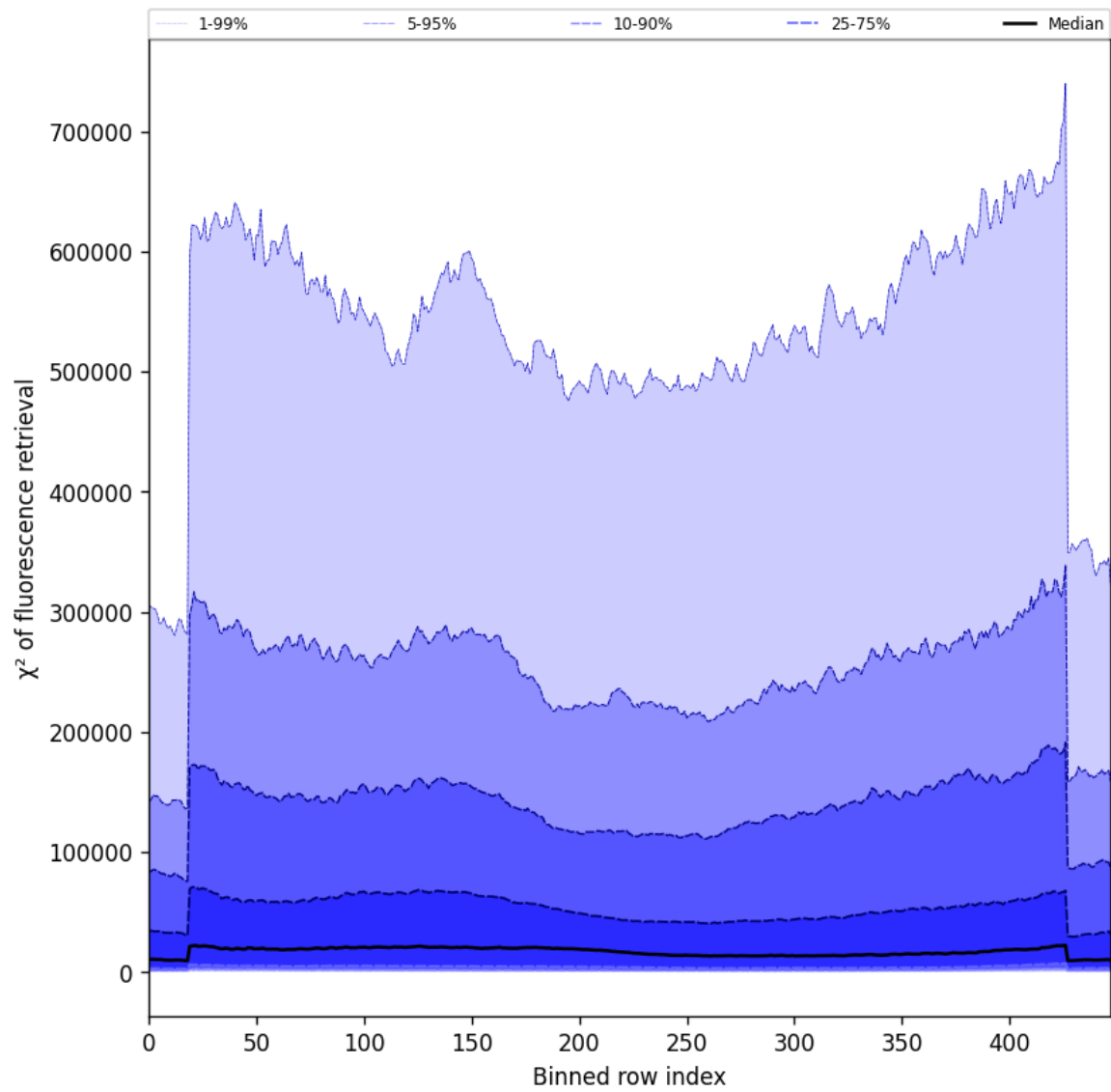
Figure 59: Along track statistics of “ \chi^2 of fluorescence retrieval” for 2024-12-18 to 2024-12-20
