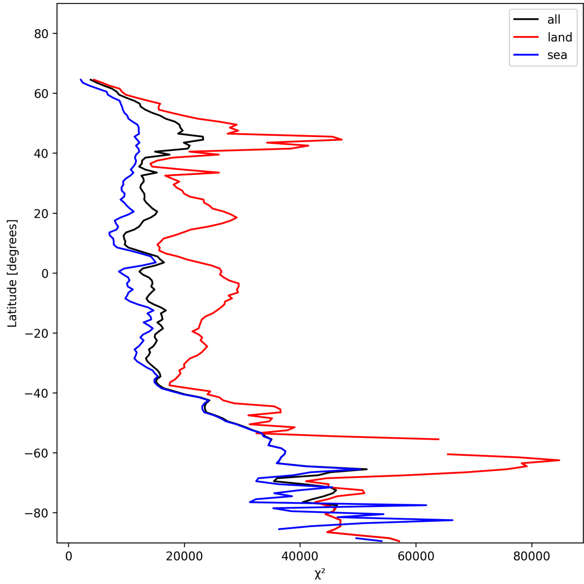
Figure 21: Zonal average of “ \chi^2 ” for 2024-12-18 to 2024-12-20.
