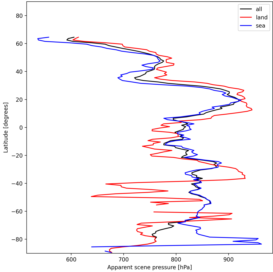
Figure 19: Zonal average of “Apparent scene pressure” for 2024-12-18 to 2024-12-20.
