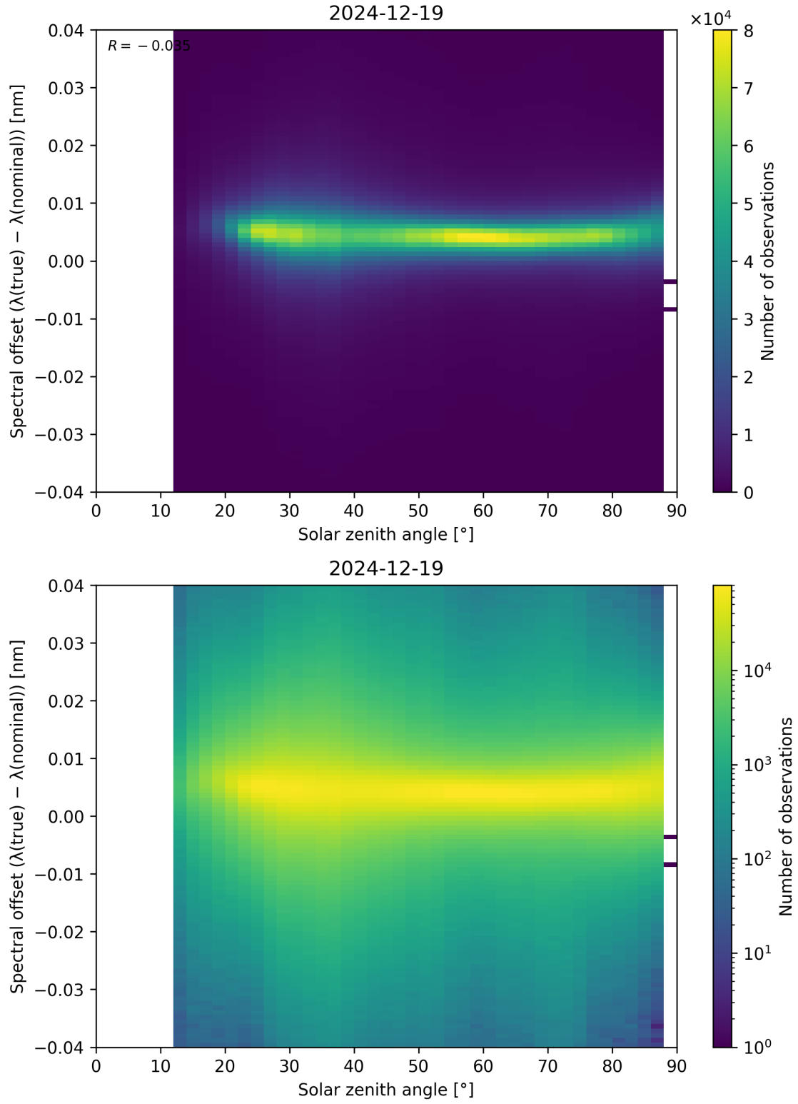
Figure 117: Scatter density plot of “Solar zenith angle” against “Spectral offset ( \lambda_{\text{true}} - \lambda_{\text{nominal}} )” for 2024-12-18 to 2024-12-20.
