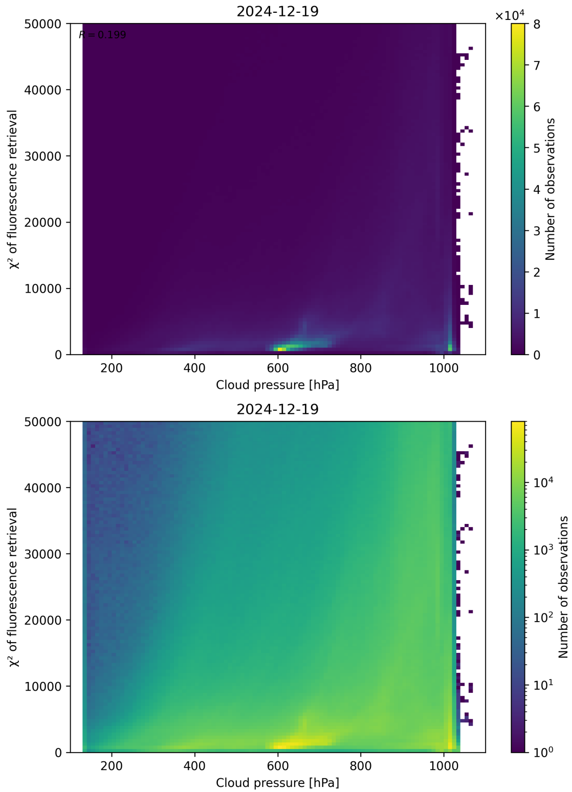
Figure 78: Scatter density plot of “Cloud pressure” against “ \chi^2 of fluorescence retrieval” for 2024-12-18 to 2024-12-20.
