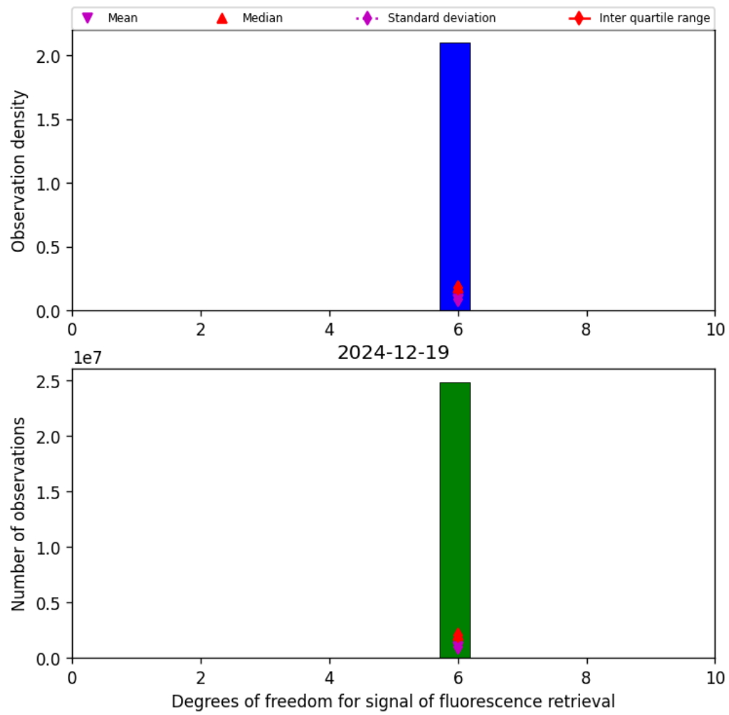
Figure 43: Histogram of “Degrees of freedom for signal of fluorescence retrieval” for 2024-12-18 to 2024-12-20
