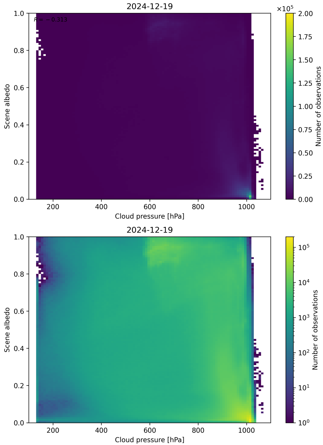
Figure 83: Scatter density plot of “Cloud pressure” against “Scene albedo” for 2024-12-18 to 2024-12-20.
