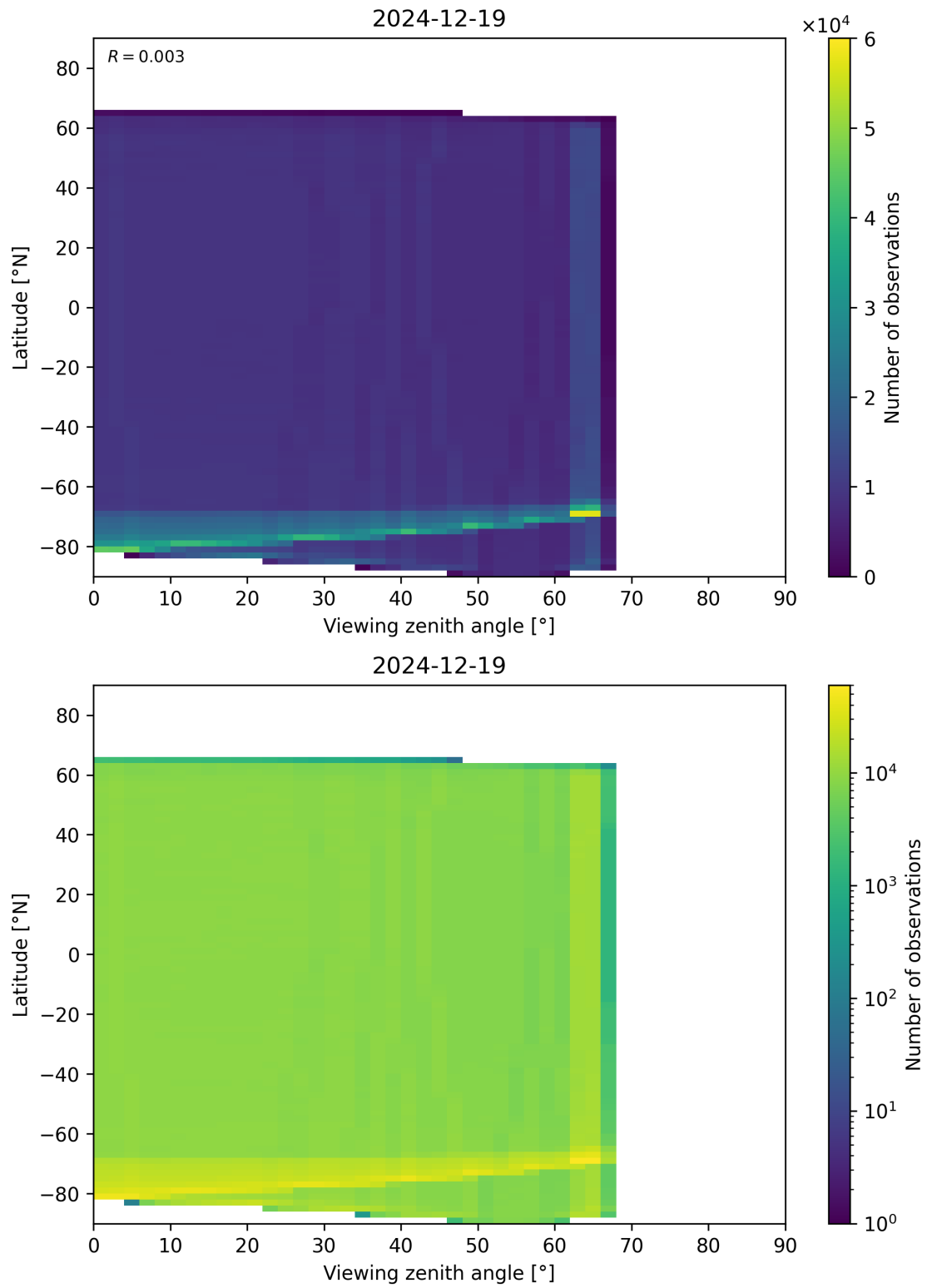
Figure 123: Scatter density plot of “Viewing zenith angle” against “Latitude” for 2024-12-18 to 2024-12-20.
