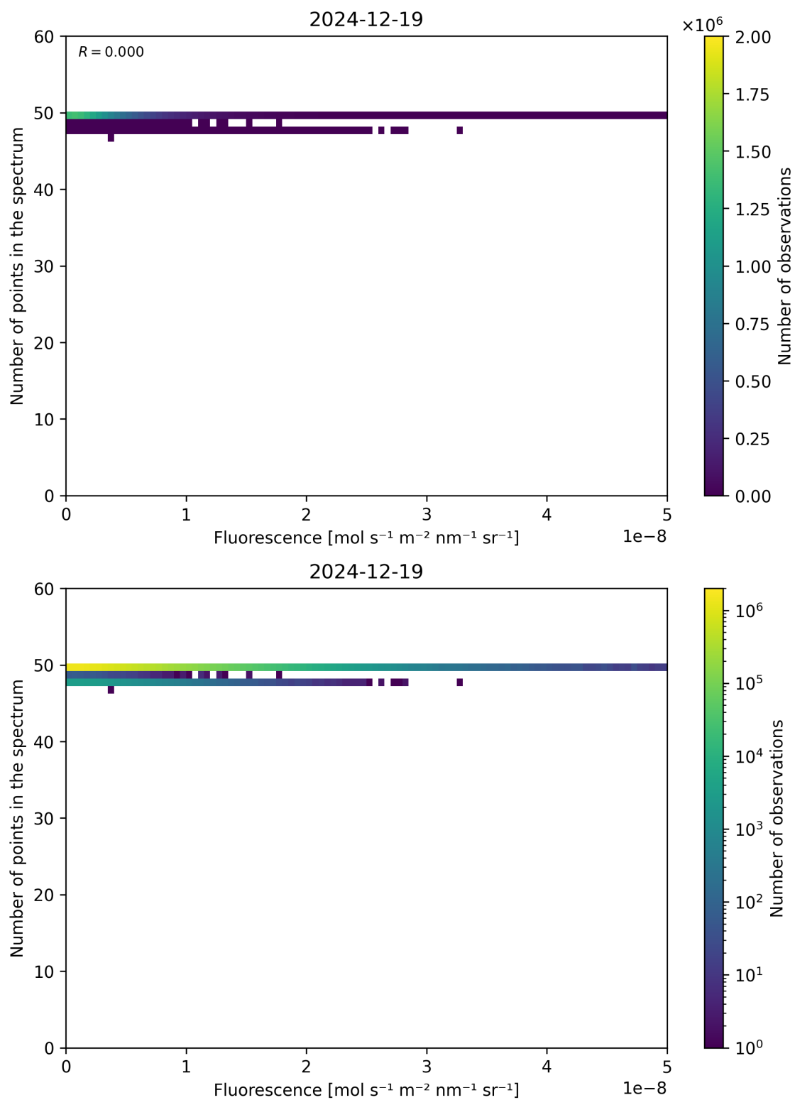
Figure 86: Scatter density plot of “Fluorescence” against “Number of points in the spectrum” for 2024-12-18 to 2024-12-20.
