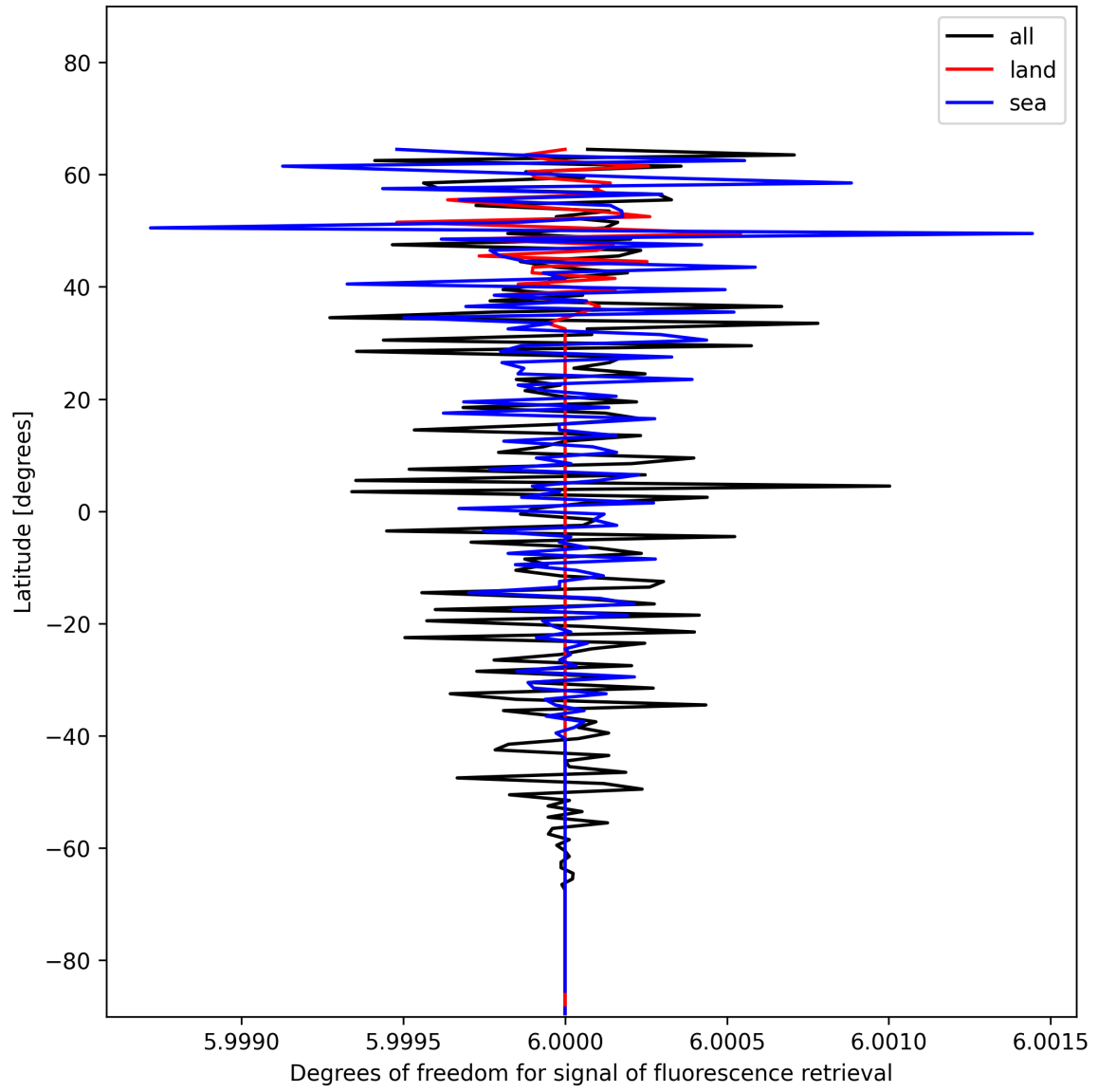
Figure 26: Zonal average of “Degrees of freedom for signal of fluorescence retrieval” for 2024-12-18 to 2024-12-20.
