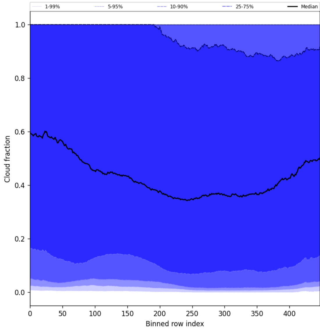
Figure 49: Along track statistics of “Cloud fraction” for 2024-12-18 to 2024-12-20
