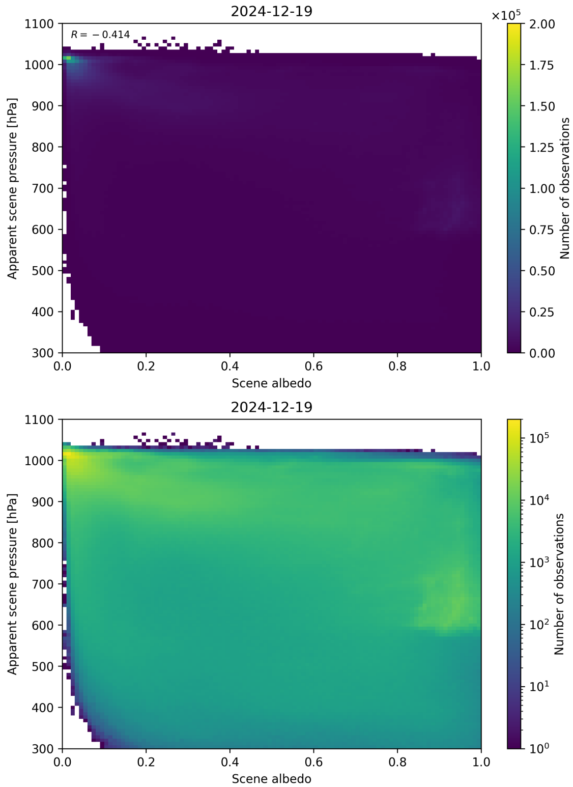
Figure 102: Scatter density plot of “Scene albedo” against “Apparent scene pressure” for 2024-12-18 to 2024-12-20.
