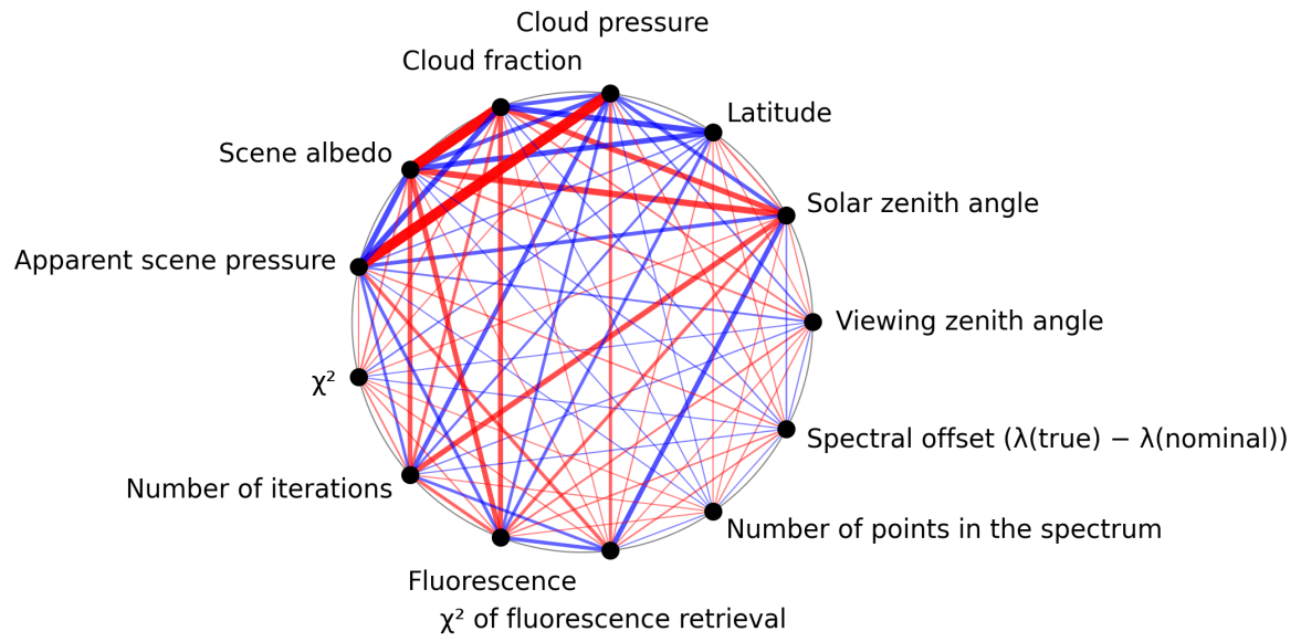
Figure 1: Map of correlation graph for 2024-12-18 to 2024-12-20.
