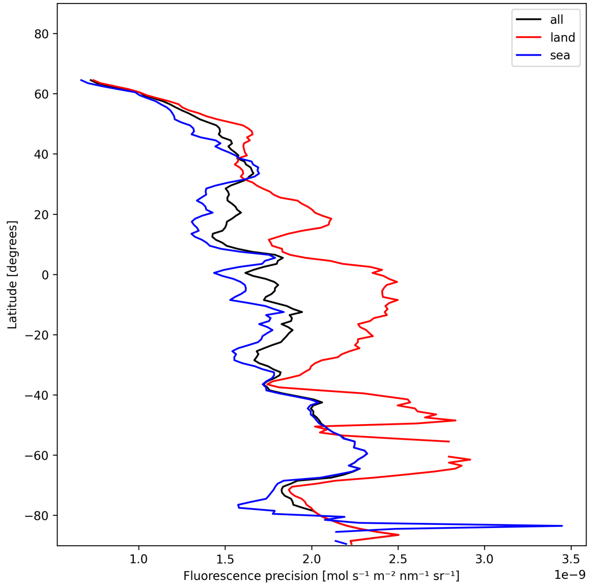
Figure 24: Zonal average of “Fluorescence precision” for 2024-12-18 to 2024-12-20.
