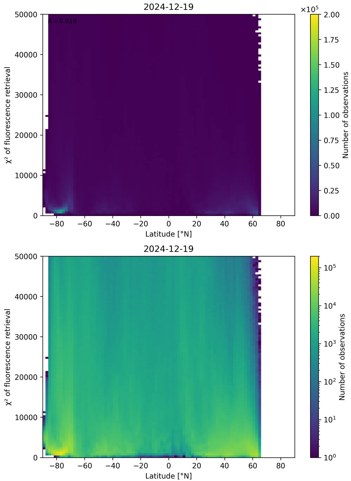
Figure 89: Scatter density plot of “Latitude” against “ \chi^2 of fluorescence retrieval” for 2024-12-18 to 2024-12-20.
