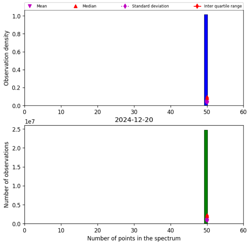
Figure 44: Histogram of “Number of points in the spectrum” for 2024-12-19 to 2024-12-21
