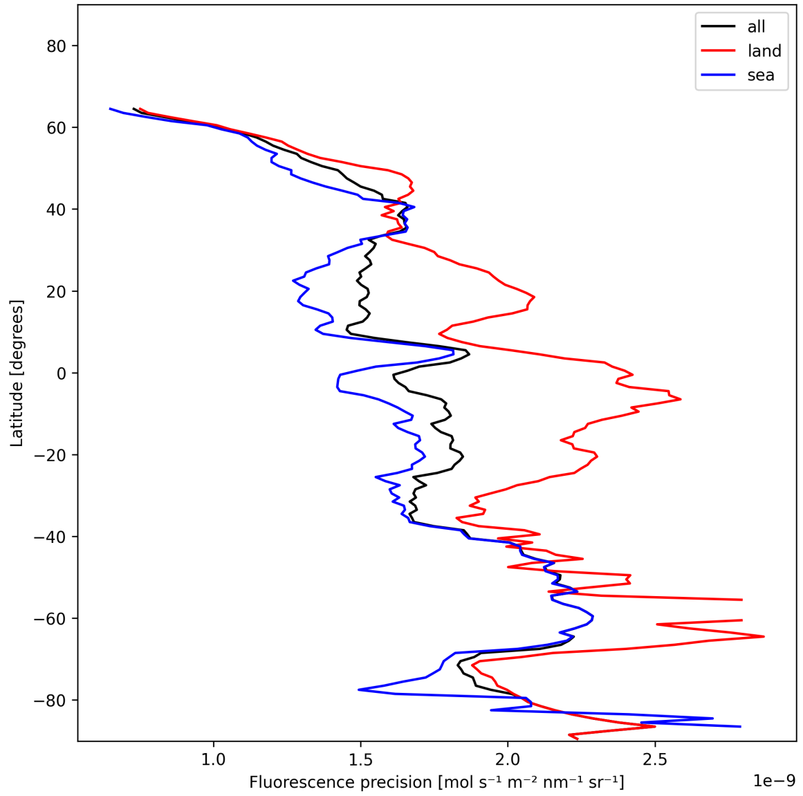
Figure 24: Zonal average of “Fluorescence precision” for 2024-12-19 to 2024-12-21.
