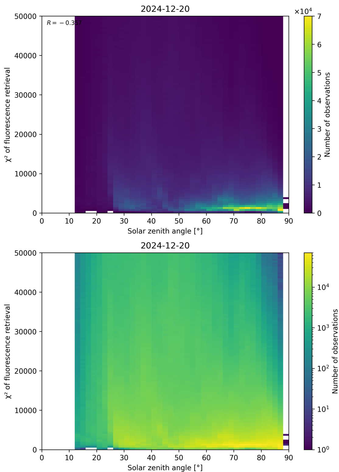
Figure 109: Scatter density plot of “Solar zenith angle” against “ \chi^2 of fluorescence retrieval” for 2024-12-19 to 2024-12-21.
