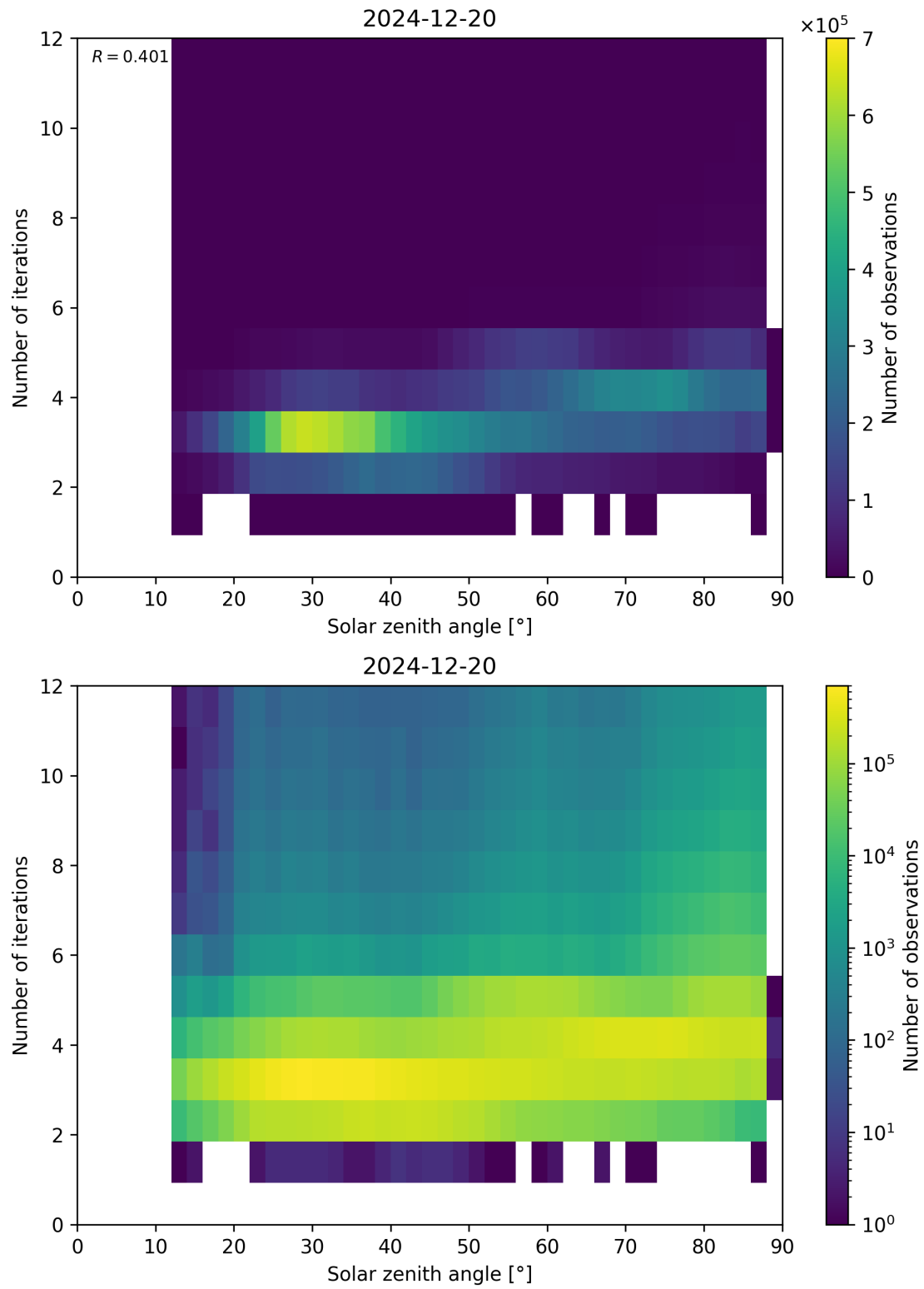
Figure 114: Scatter density plot of “Solar zenith angle” against “Number of iterations” for 2024-12-19 to 2024-12-21.
