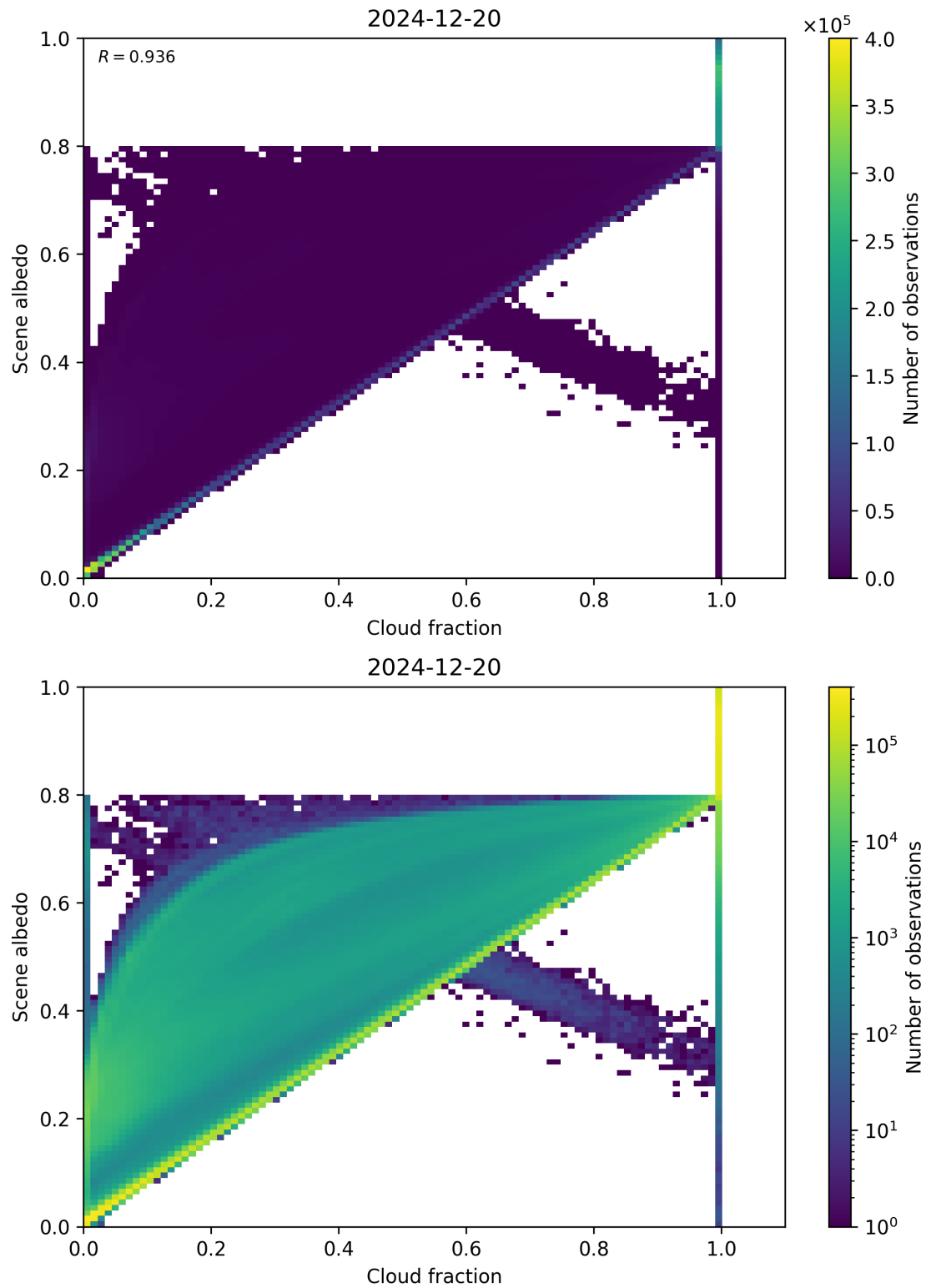
Figure 75: Scatter density plot of “Cloud fraction” against “Scene albedo” for 2024-12-19 to 2024-12-21.
