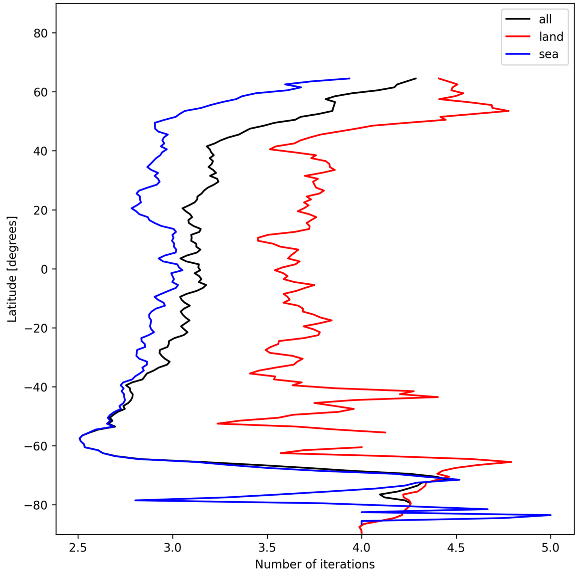
Figure 22: Zonal average of “Number of iterations” for 2024-12-19 to 2024-12-21.
