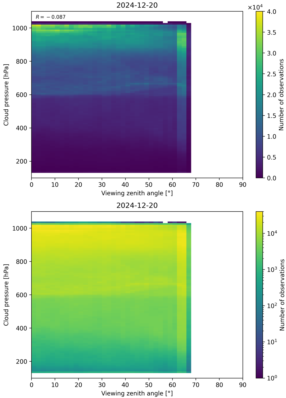
Figure 121: Scatter density plot of “Viewing zenith angle” against “Cloud pressure” for 2024-12-19 to 2024-12-21.
