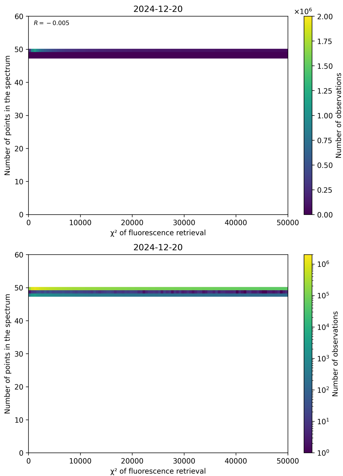
Figure 68: Scatter density plot of “ \chi^2 of fluorescence retrieval” against “Number of points in the spectrum” for 2024-12-19 to 2024-12-21.
