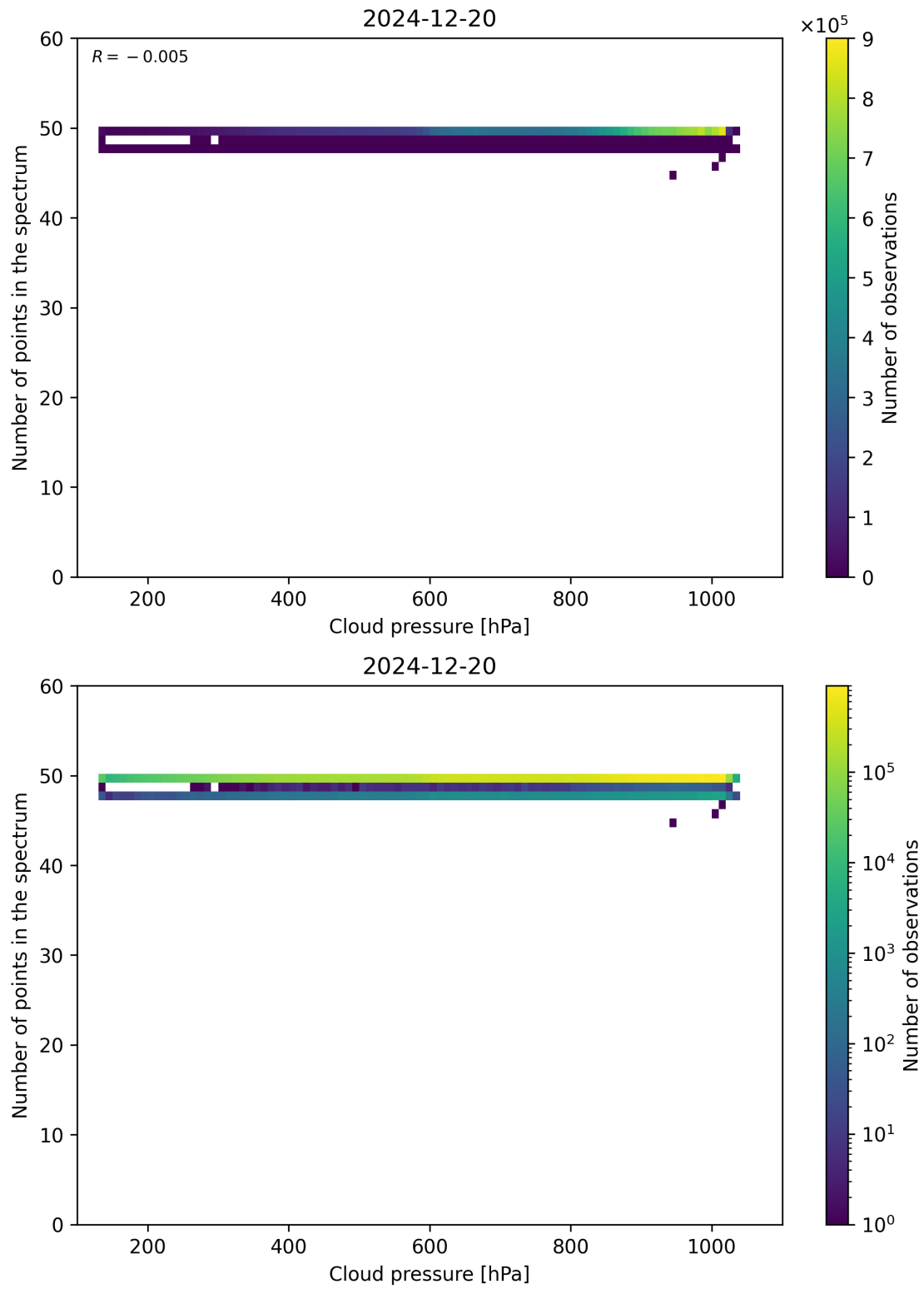
Figure 82: Scatter density plot of “Cloud pressure” against “Number of points in the spectrum” for 2024-12-19 to 2024-12-21.
