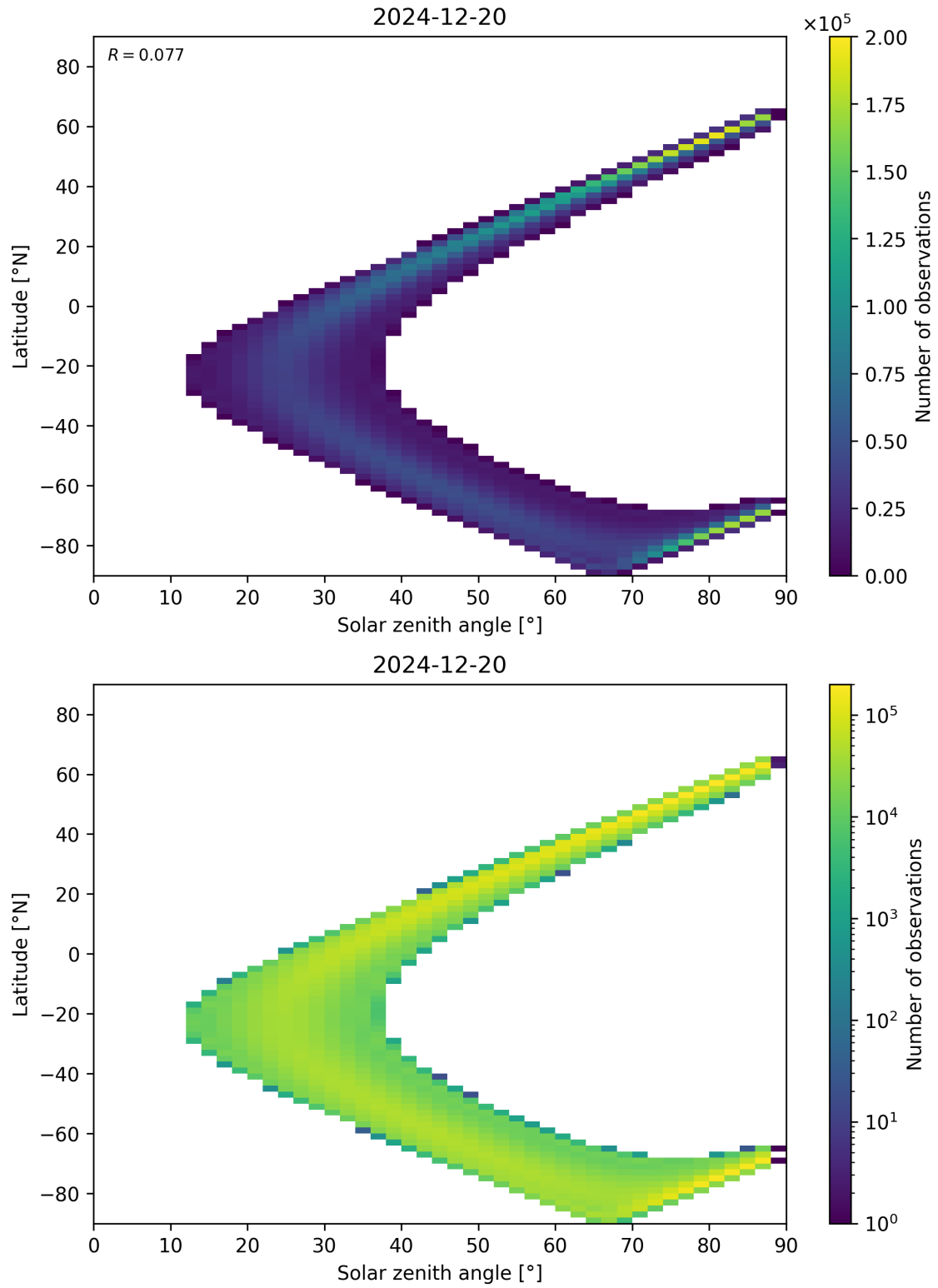
Figure 113: Scatter density plot of “Solar zenith angle” against “Latitude” for 2024-12-19 to 2024-12-21.
