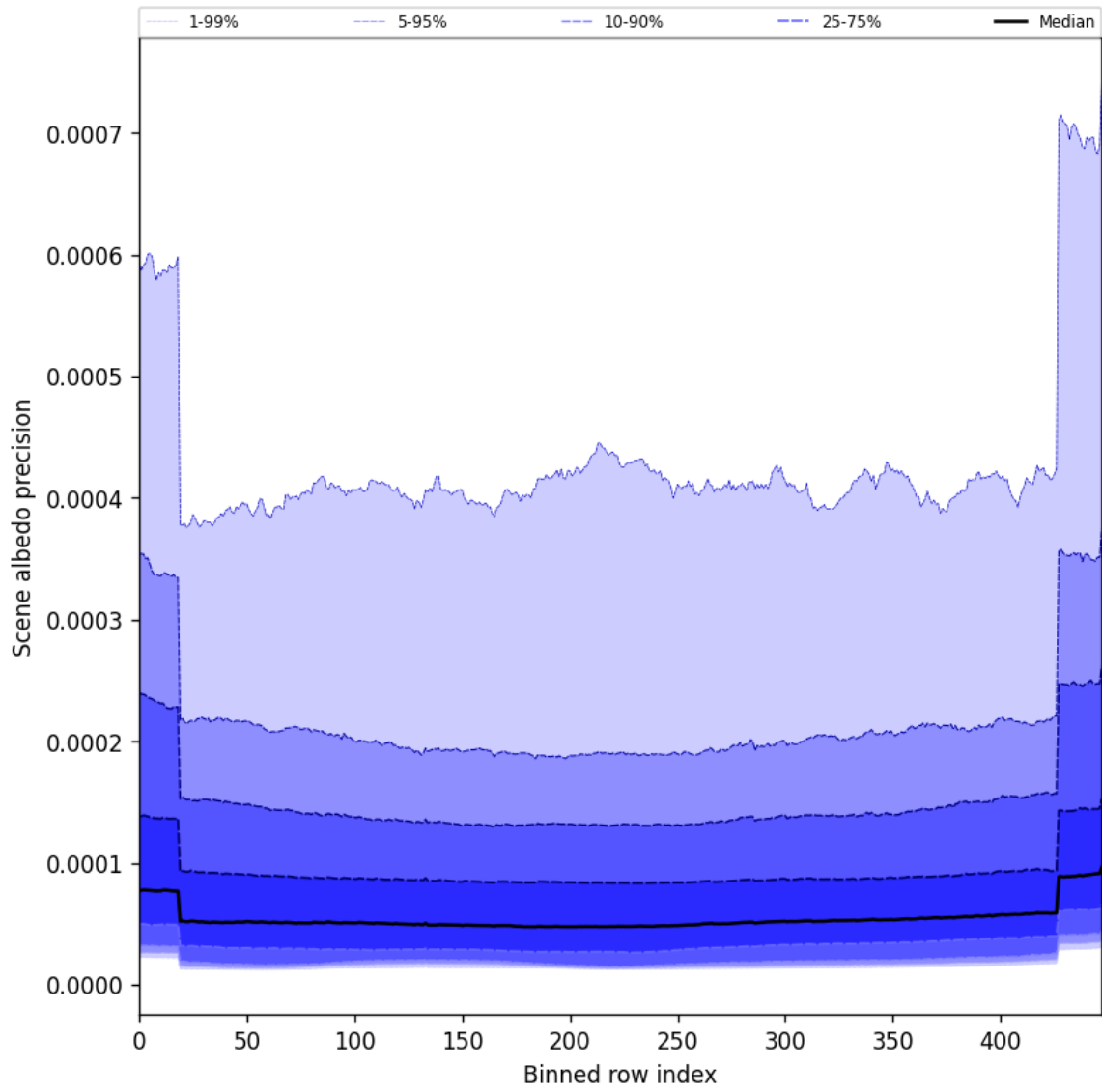
Figure 52: Along track statistics of “Scene albedo precision” for 2024-12-19 to 2024-12-21
