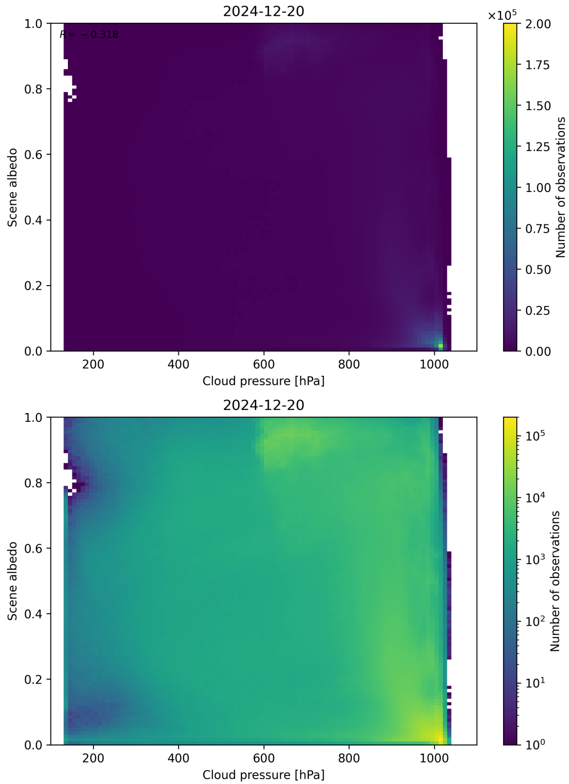
Figure 83: Scatter density plot of “Cloud pressure” against “Scene albedo” for 2024-12-19 to 2024-12-21.
