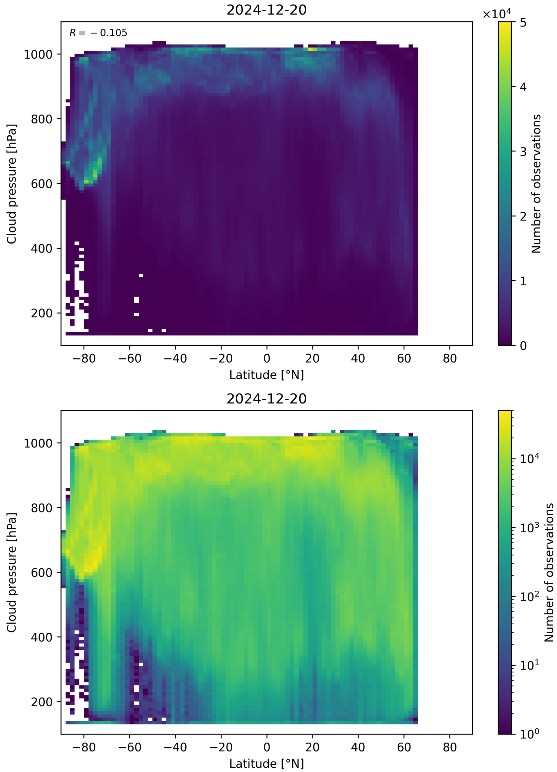
Figure 91: Scatter density plot of “Latitude” against “Cloud pressure” for 2024-12-19 to 2024-12-21.
