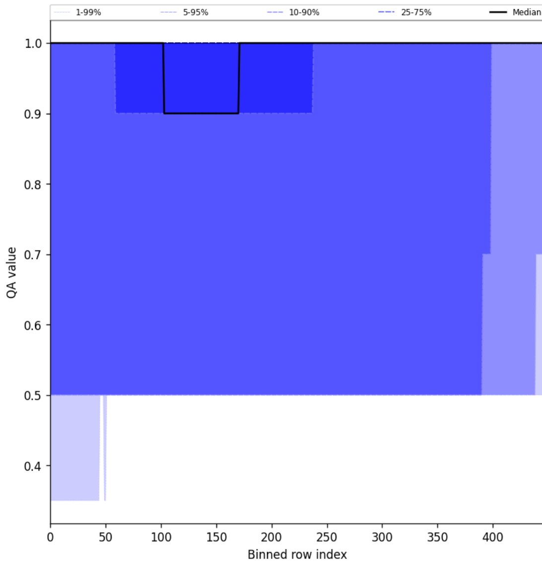
Figure 46: Along track statistics of “QA value” for 2024-12-19 to 2024-12-21
