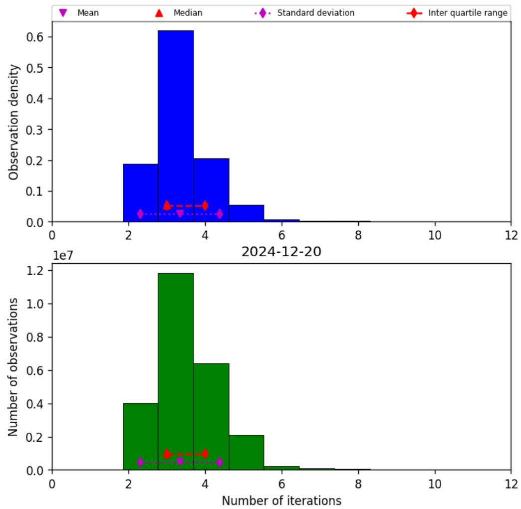
Figure 39: Histogram of “Number of iterations” for 2024-12-19 to 2024-12-21
