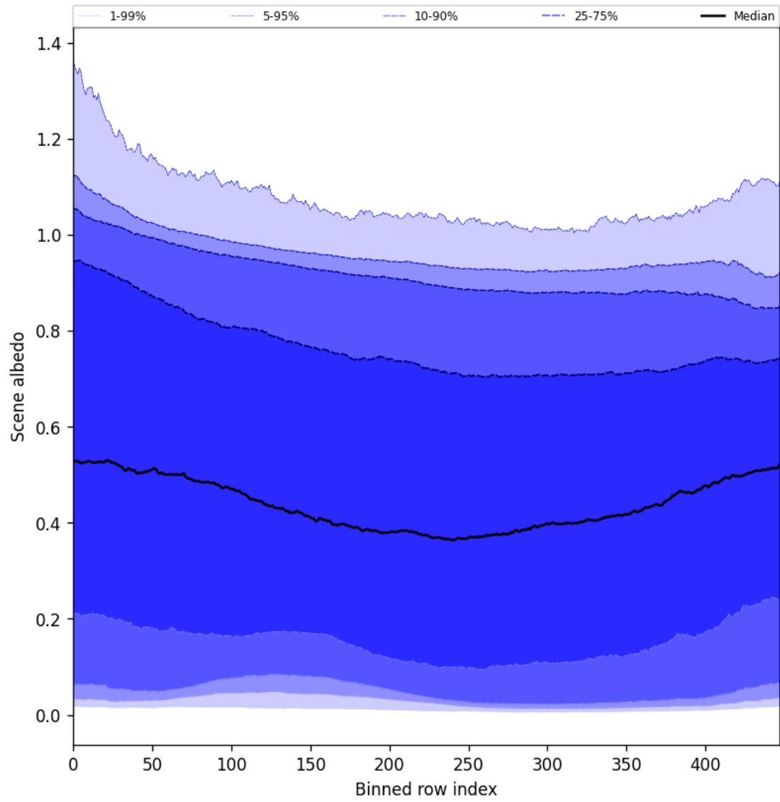
Figure 51: Along track statistics of “Scene albedo” for 2024-12-19 to 2024-12-21
