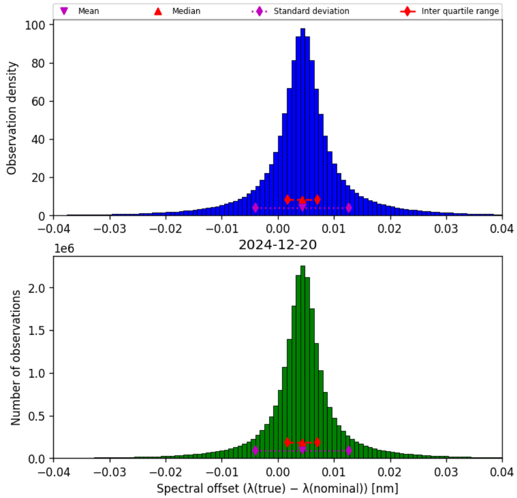
Figure 45: Histogram of “Spectral offset ( \lambda_{\text{true}} - \lambda_{\text{nominal}} )” for 2024-12-19 to 2024-12-21
