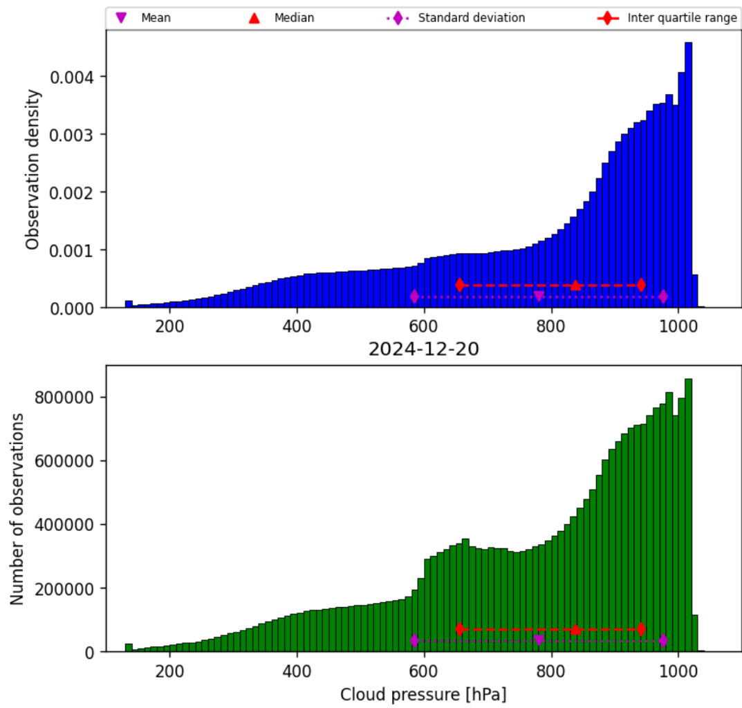
Figure 30: Histogram of “Cloud pressure” for 2024-12-19 to 2024-12-21
