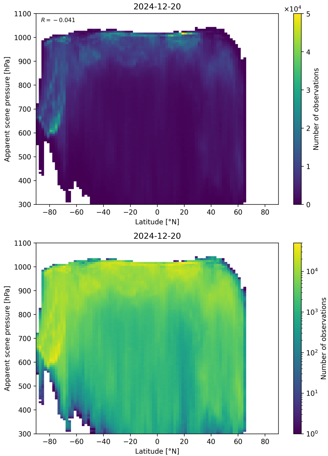
Figure 88: Scatter density plot of “Latitude” against “Apparent scene pressure” for 2024-12-19 to 2024-12-21.
