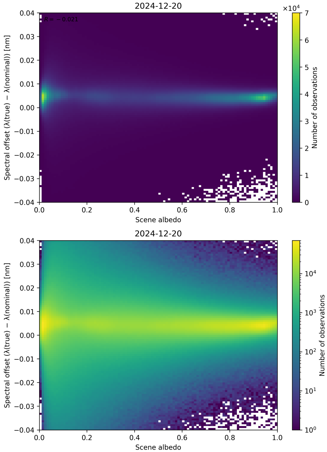
Figure 107: Scatter density plot of “Scene albedo” against “Spectral offset ( \lambda_{\text{true}} - \lambda_{\text{nominal}} )” for 2024-12-19 to 2024-12-21.
