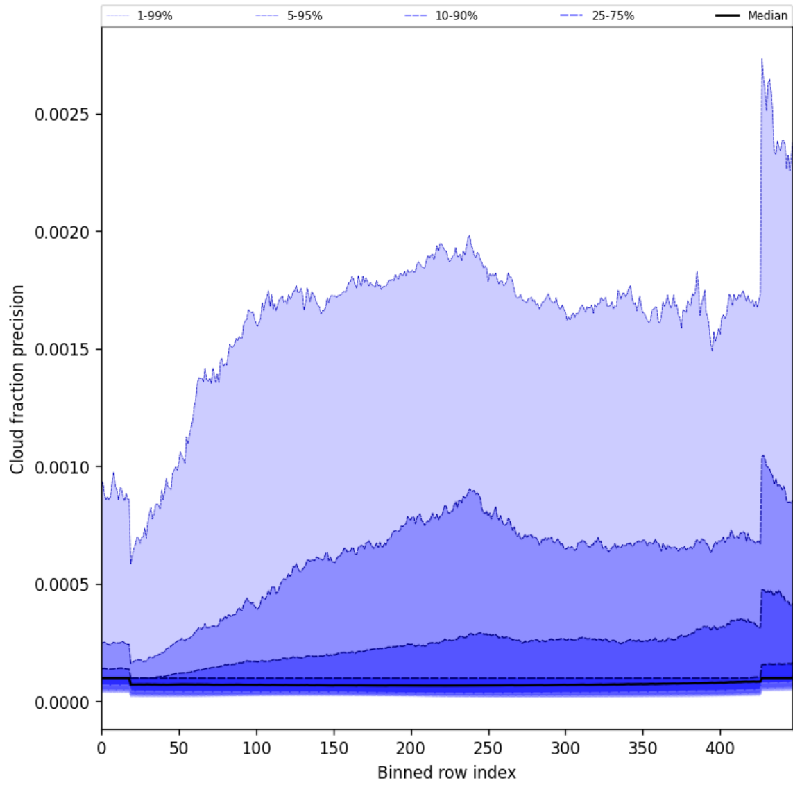
Figure 50: Along track statistics of “Cloud fraction precision” for 2024-12-19 to 2024-12-21
