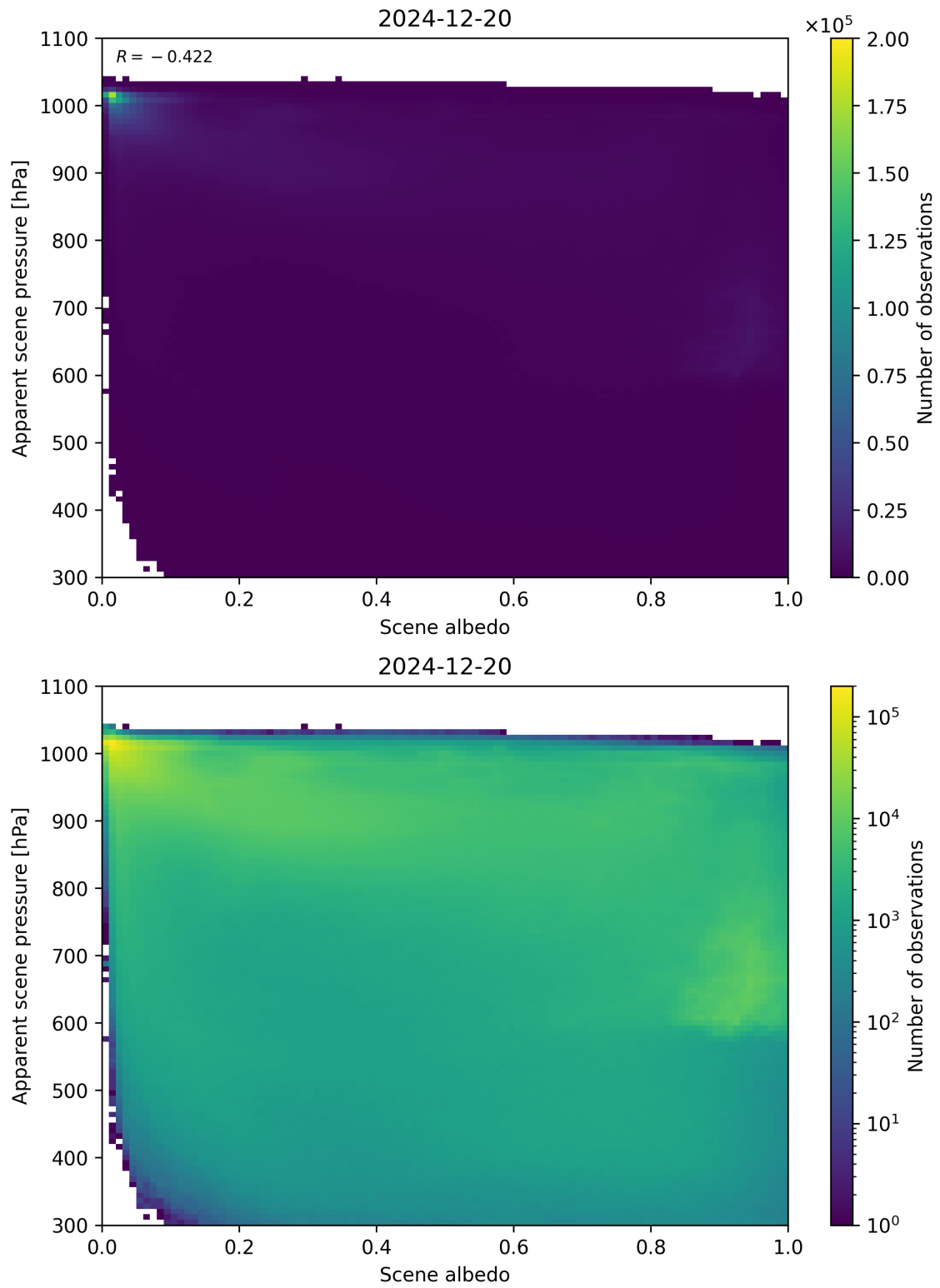
Figure 102: Scatter density plot of “Scene albedo” against “Apparent scene pressure” for 2024-12-19 to 2024-12-21.
