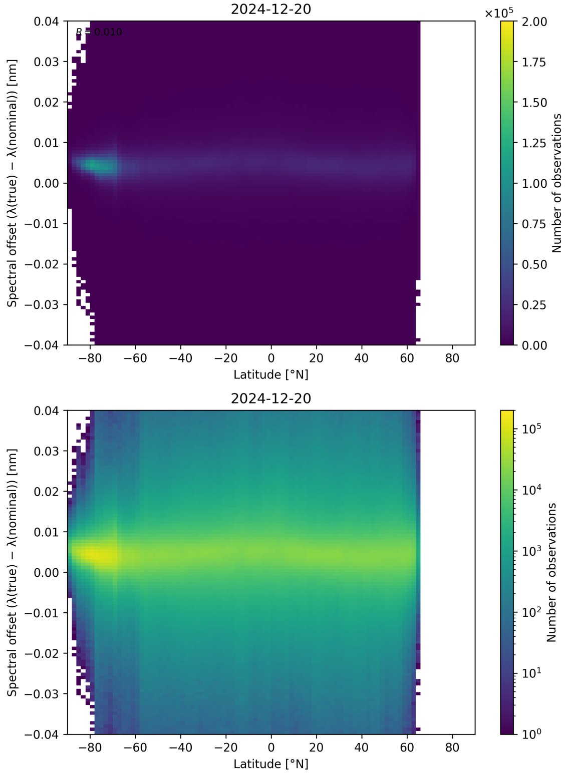
Figure 96: Scatter density plot of “Latitude” against “Spectral offset ( \lambda_{\text{true}} - \lambda_{\text{nominal}} )” for 2024-12-19 to 2024-12-21.
