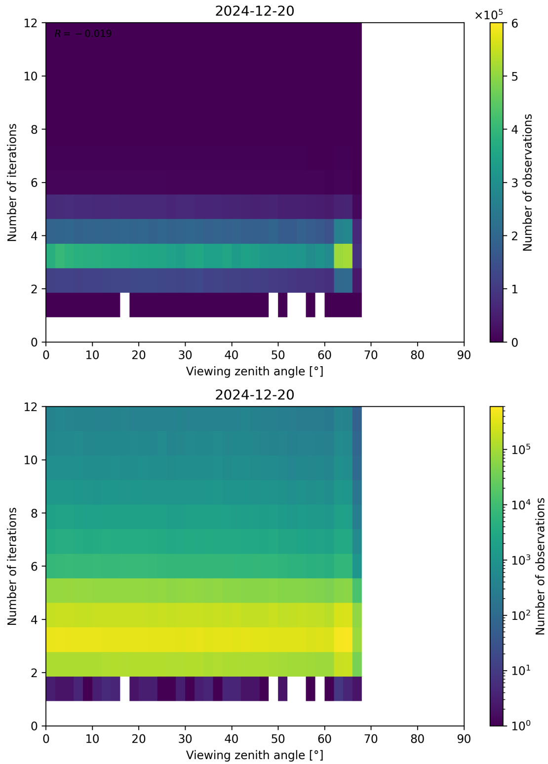
Figure 124: Scatter density plot of “Viewing zenith angle” against “Number of iterations” for 2024-12-19 to 2024-12-21.
