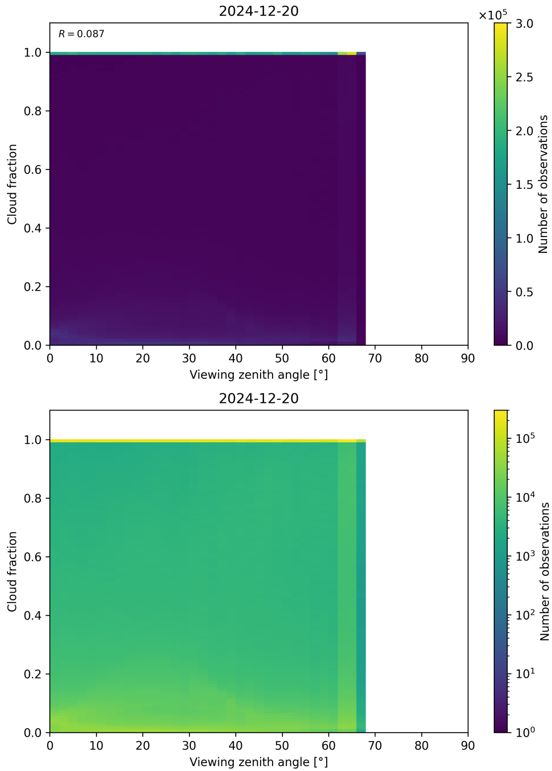
Figure 120: Scatter density plot of “Viewing zenith angle” against “Cloud fraction” for 2024-12-19 to 2024-12-21.
