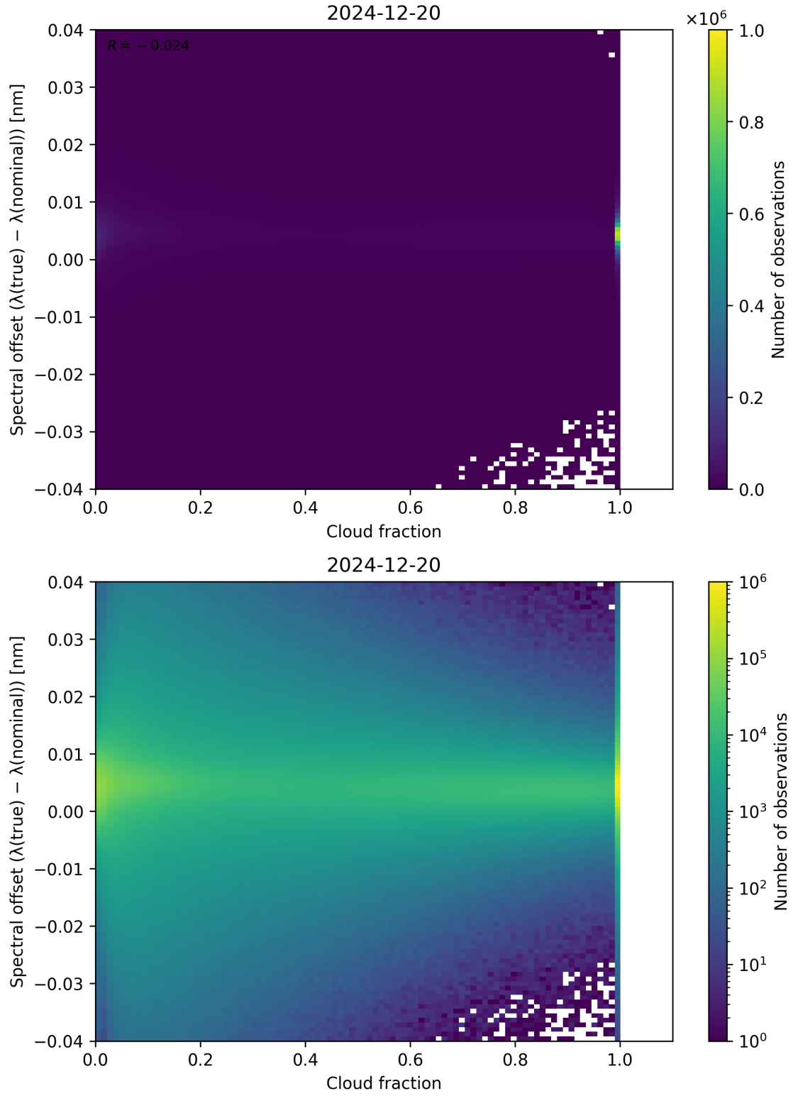
Figure 76: Scatter density plot of “Cloud fraction” against “Spectral offset ( \lambda_{\text{true}} - \lambda_{\text{nominal}} )” for 2024-12-19 to 2024-12-21.
