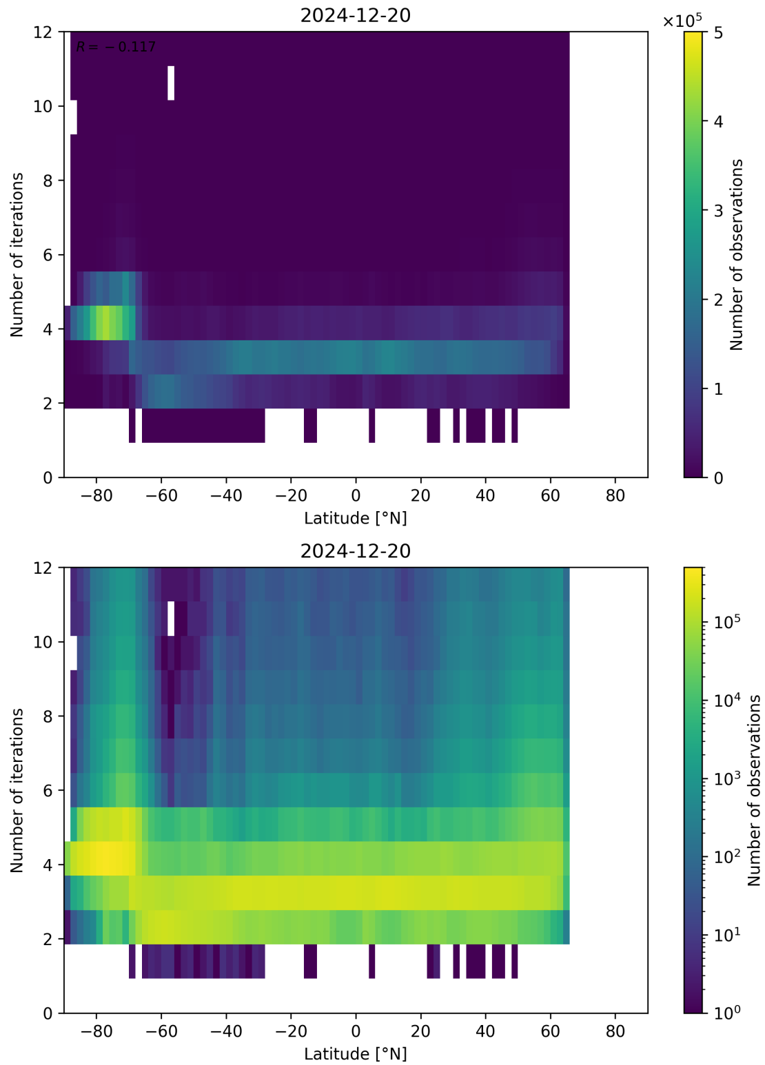
Figure 93: Scatter density plot of “Latitude” against “Number of iterations” for 2024-12-19 to 2024-12-21.
