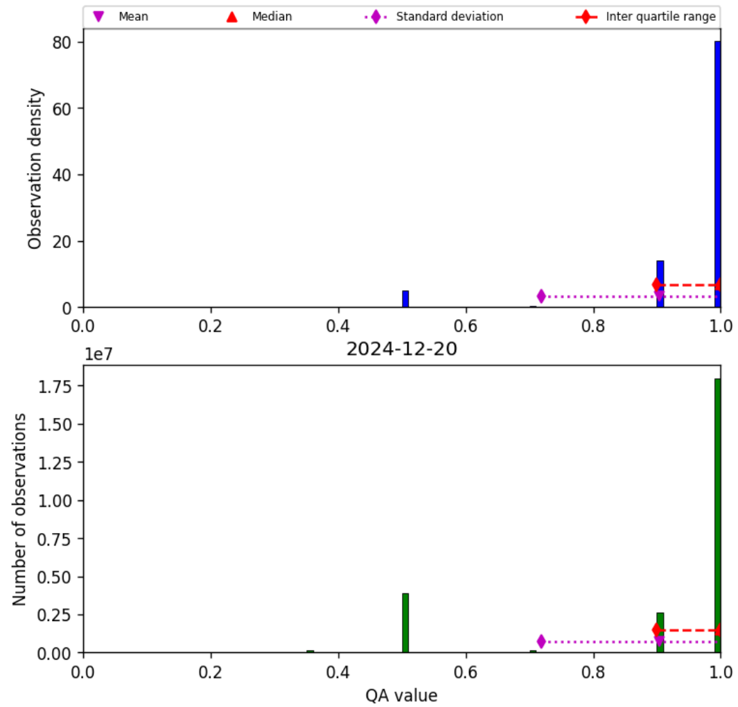
Figure 29: Histogram of “QA value” for 2024-12-19 to 2024-12-21
