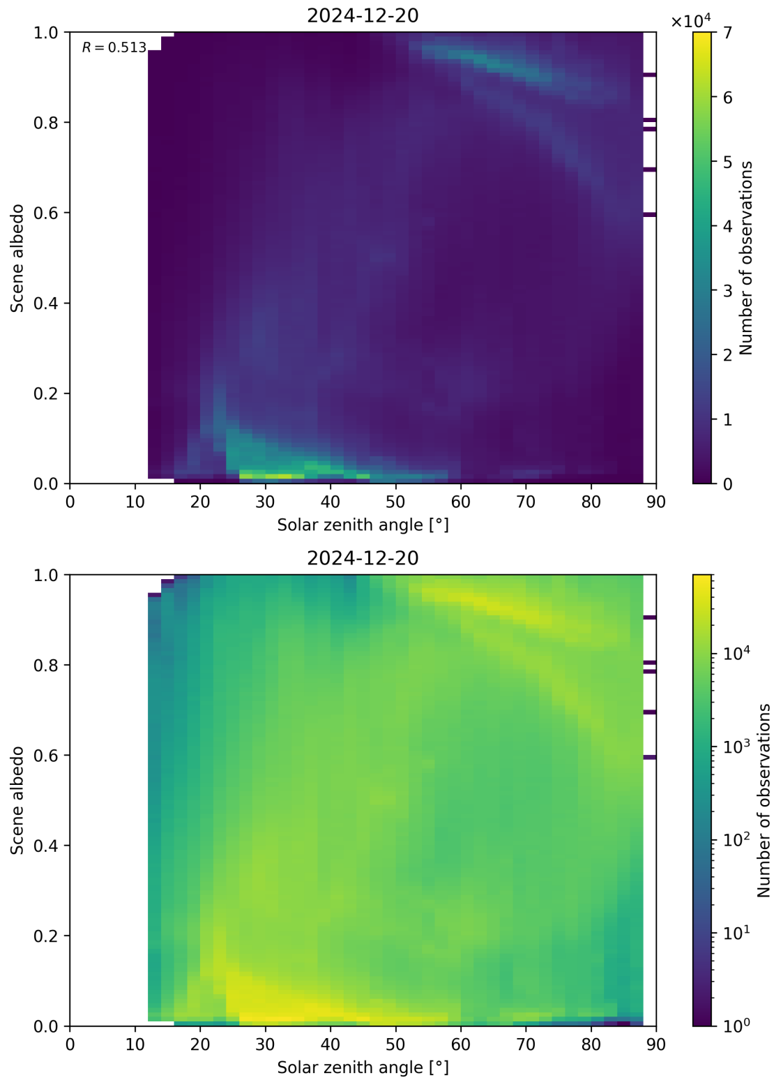
Figure 116: Scatter density plot of “Solar zenith angle” against “Scene albedo” for 2024-12-19 to 2024-12-21.
