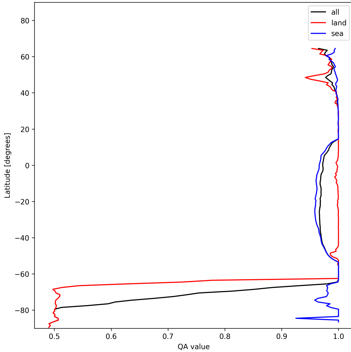
Figure 12: Zonal average of “QA value” for 2024-12-19 to 2024-12-21.
