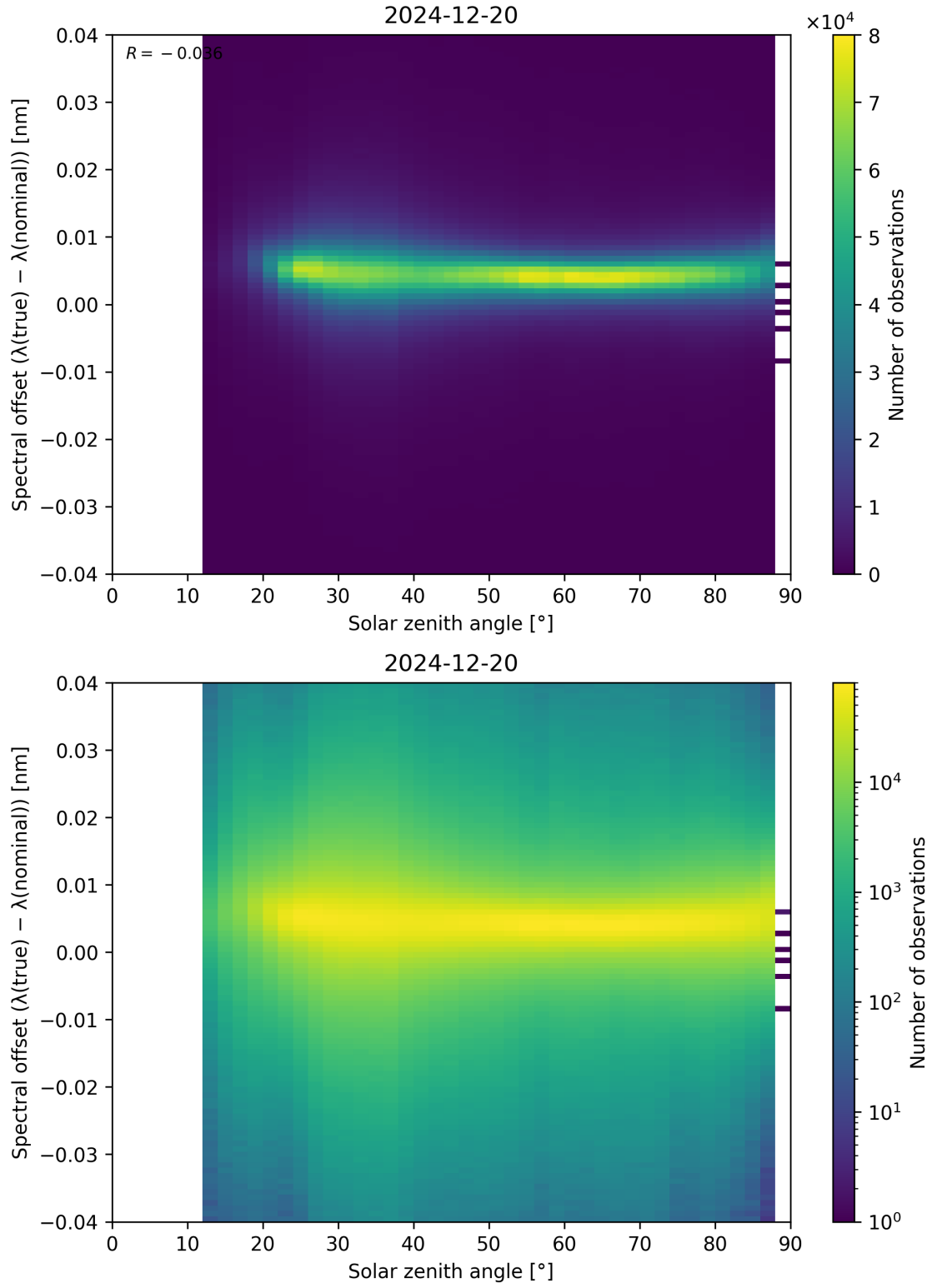
Figure 117: Scatter density plot of “Solar zenith angle” against “Spectral offset ( \lambda_{\text{true}} - \lambda_{\text{nominal}} )” for 2024-12-19 to 2024-12-21.
