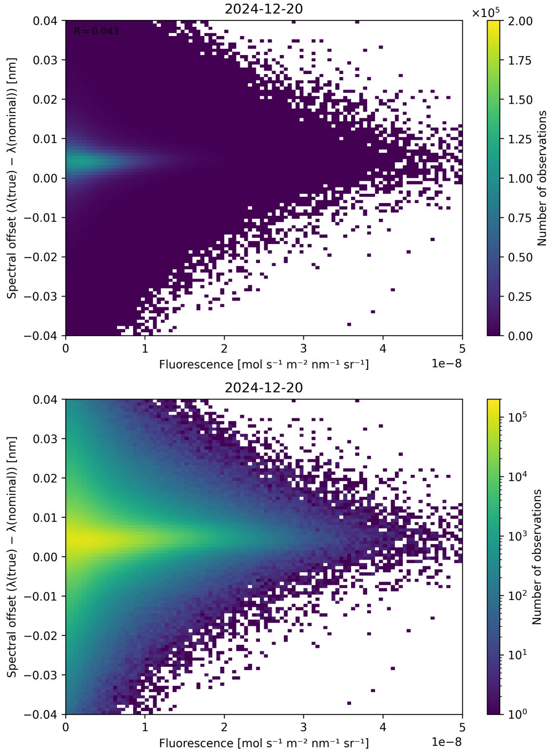
Figure 87: Scatter density plot of “Fluorescence” against “Spectral offset ( \lambda_{\text{true}} - \lambda_{\text{nominal}} )” for 2024-12-19 to 2024-12-21.
