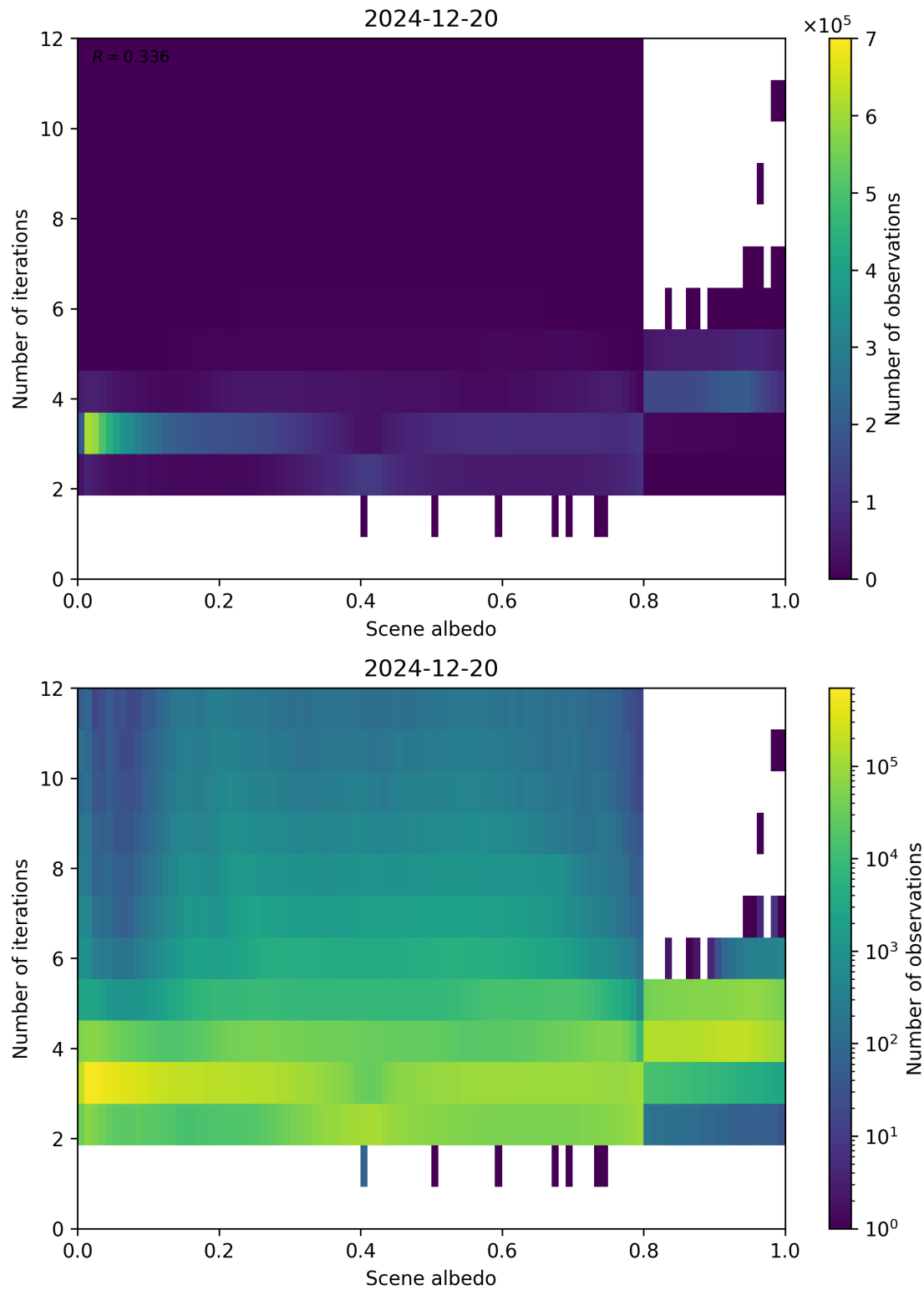
Figure 105: Scatter density plot of “Scene albedo” against “Number of iterations” for 2024-12-19 to 2024-12-21.
