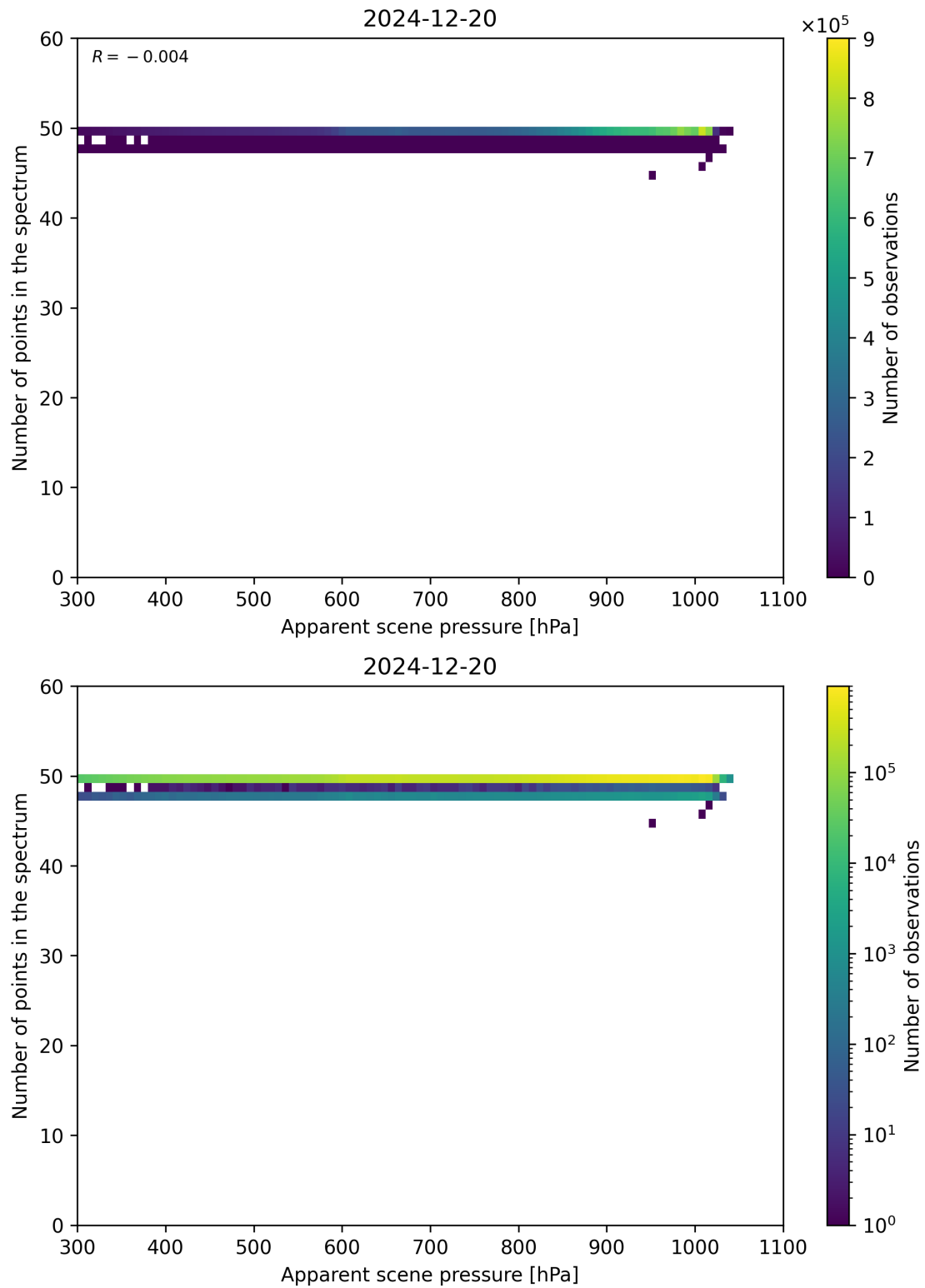
Figure 66: Scatter density plot of “Apparent scene pressure” against “Number of points in the spectrum” for 2024-12-19 to 2024-12-21.
