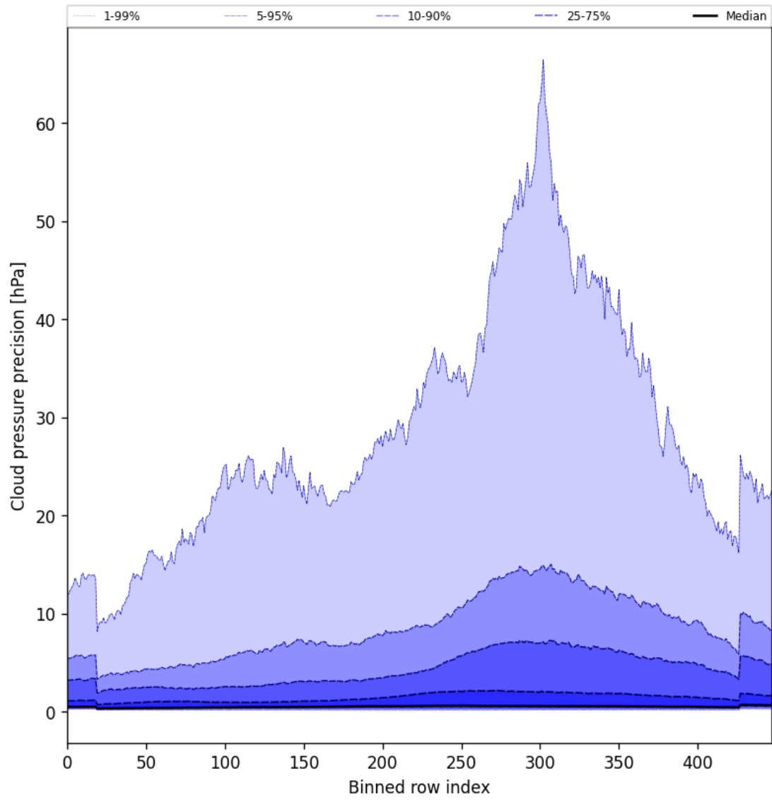
Figure 48: Along track statistics of “Cloud pressure precision” for 2024-12-19 to 2024-12-21
