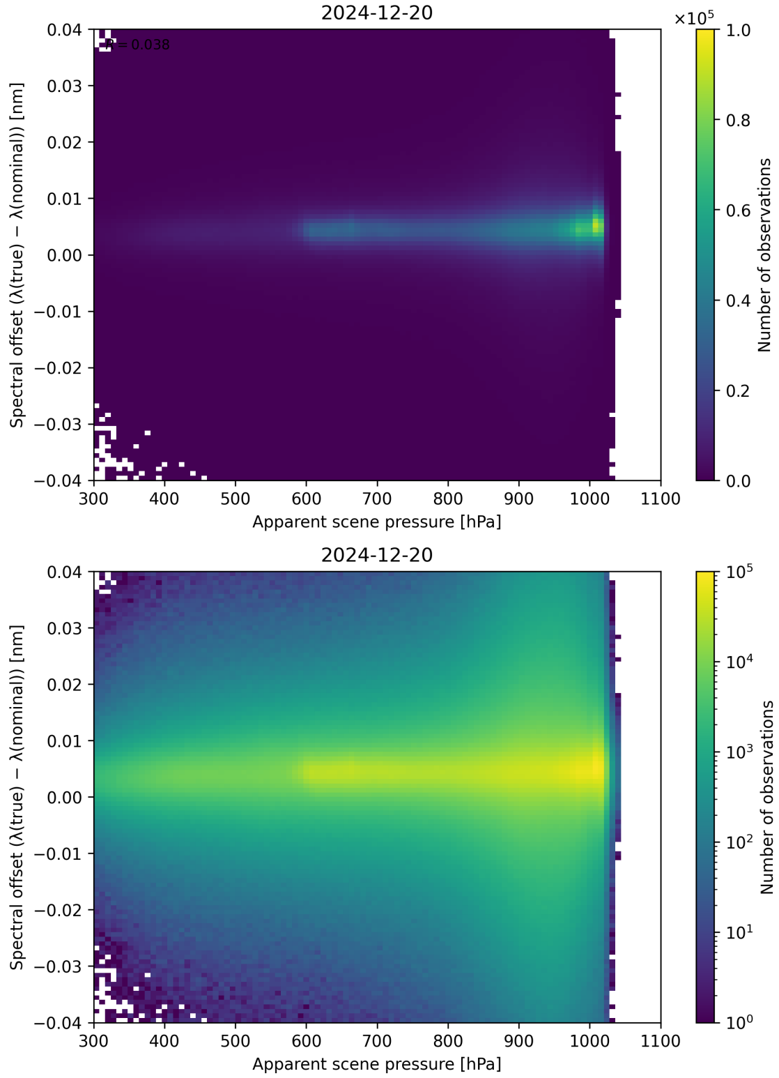
Figure 67: Scatter density plot of “Apparent scene pressure” against “Spectral offset ( \lambda_{\text{true}} - \lambda_{\text{nominal}} )” for 2024-12-19 to 2024-12-21.
