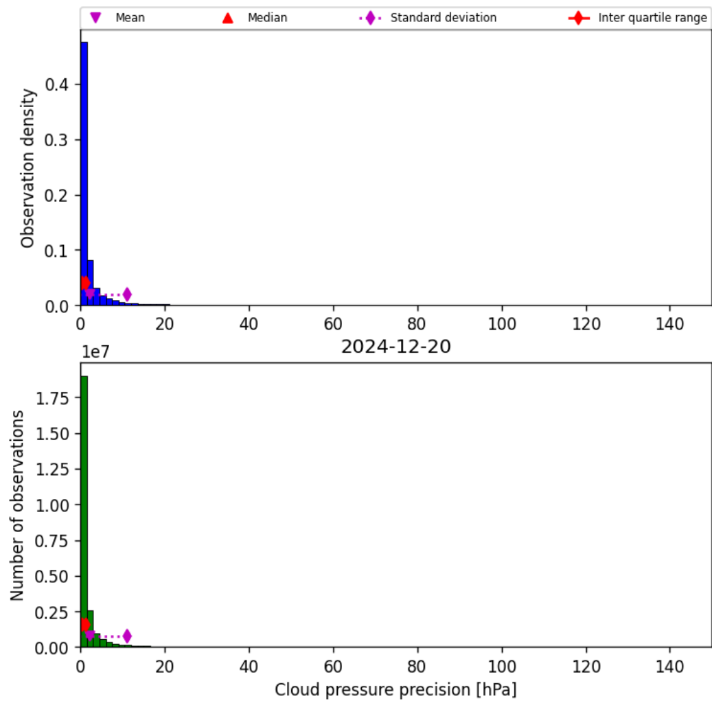
Figure 31: Histogram of “Cloud pressure precision” for 2024-12-19 to 2024-12-21
