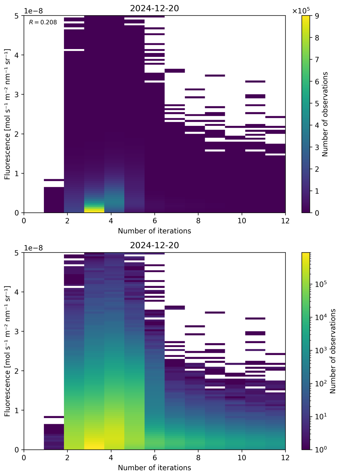
Figure 98: Scatter density plot of “Number of iterations” against “Fluorescence” for 2024-12-19 to 2024-12-21.
