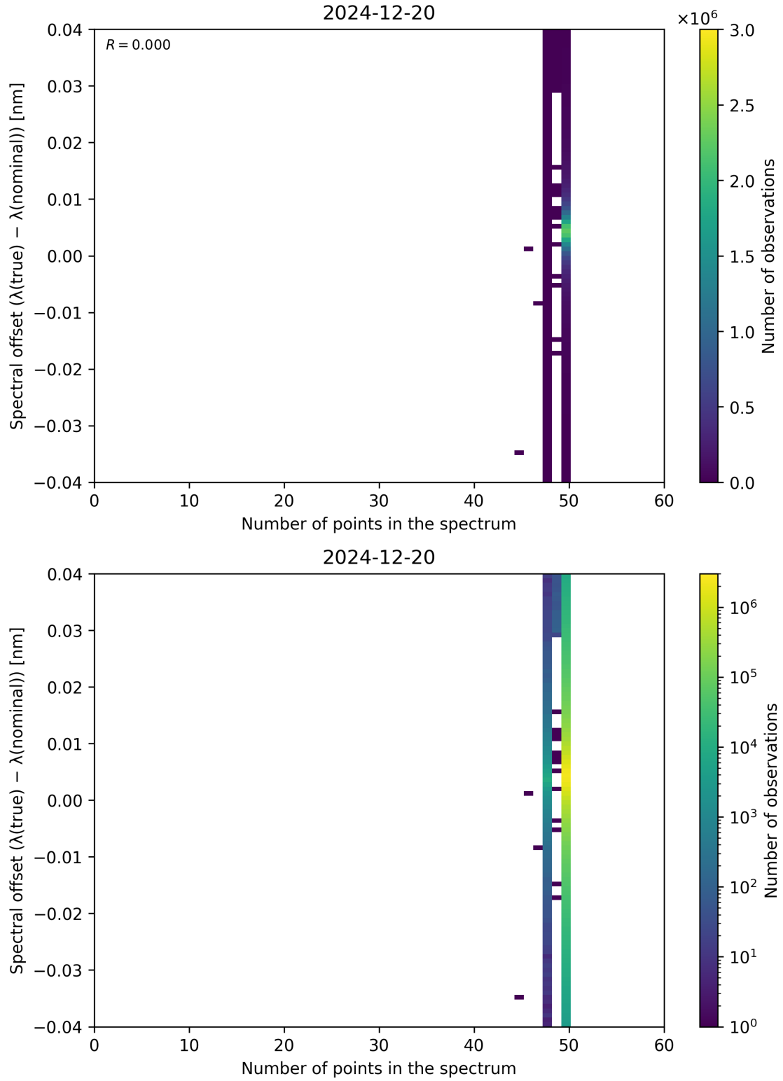
Figure 101: Scatter density plot of “Number of points in the spectrum” against “Spectral offset ( \lambda_{\text{true}} - \lambda_{\text{nominal}} )” for 2024-12-19 to 2024-12-21.
