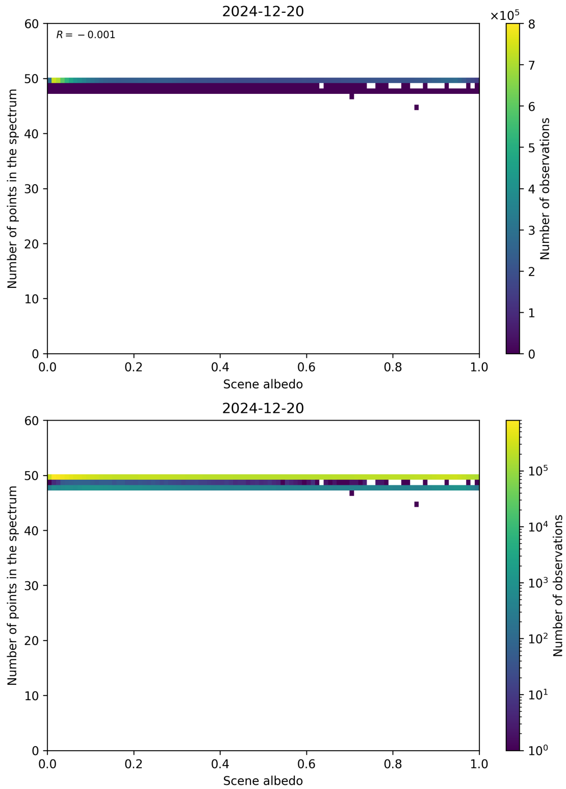
Figure 106: Scatter density plot of “Scene albedo” against “Number of points in the spectrum” for 2024-12-19 to 2024-12-21.
