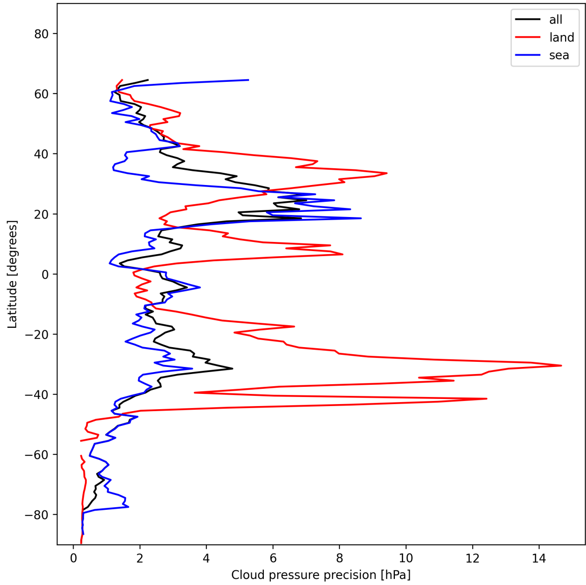
Figure 14: Zonal average of “Cloud pressure precision” for 2024-12-19 to 2024-12-21.
