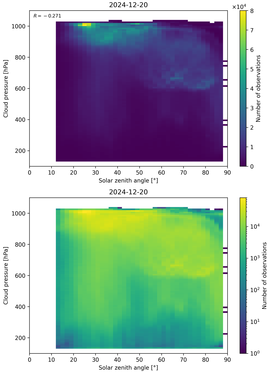
Figure 111: Scatter density plot of “Solar zenith angle” against “Cloud pressure” for 2024-12-19 to 2024-12-21.
