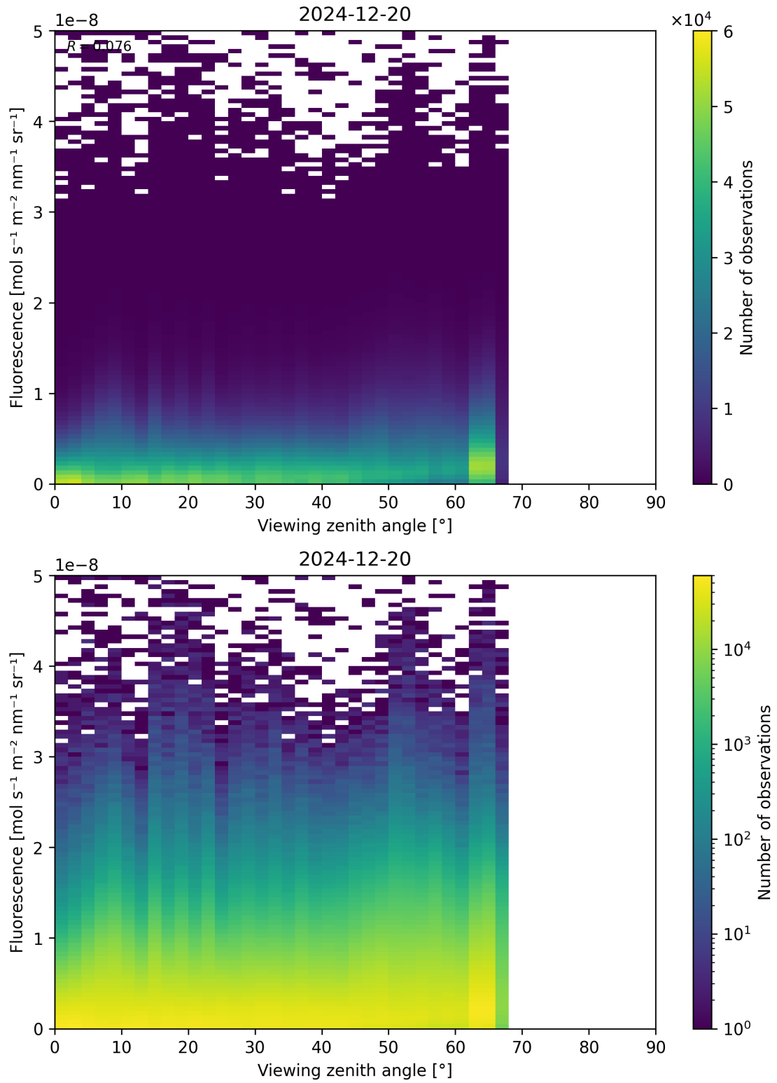
Figure 122: Scatter density plot of “Viewing zenith angle” against “Fluorescence” for 2024-12-19 to 2024-12-21.
