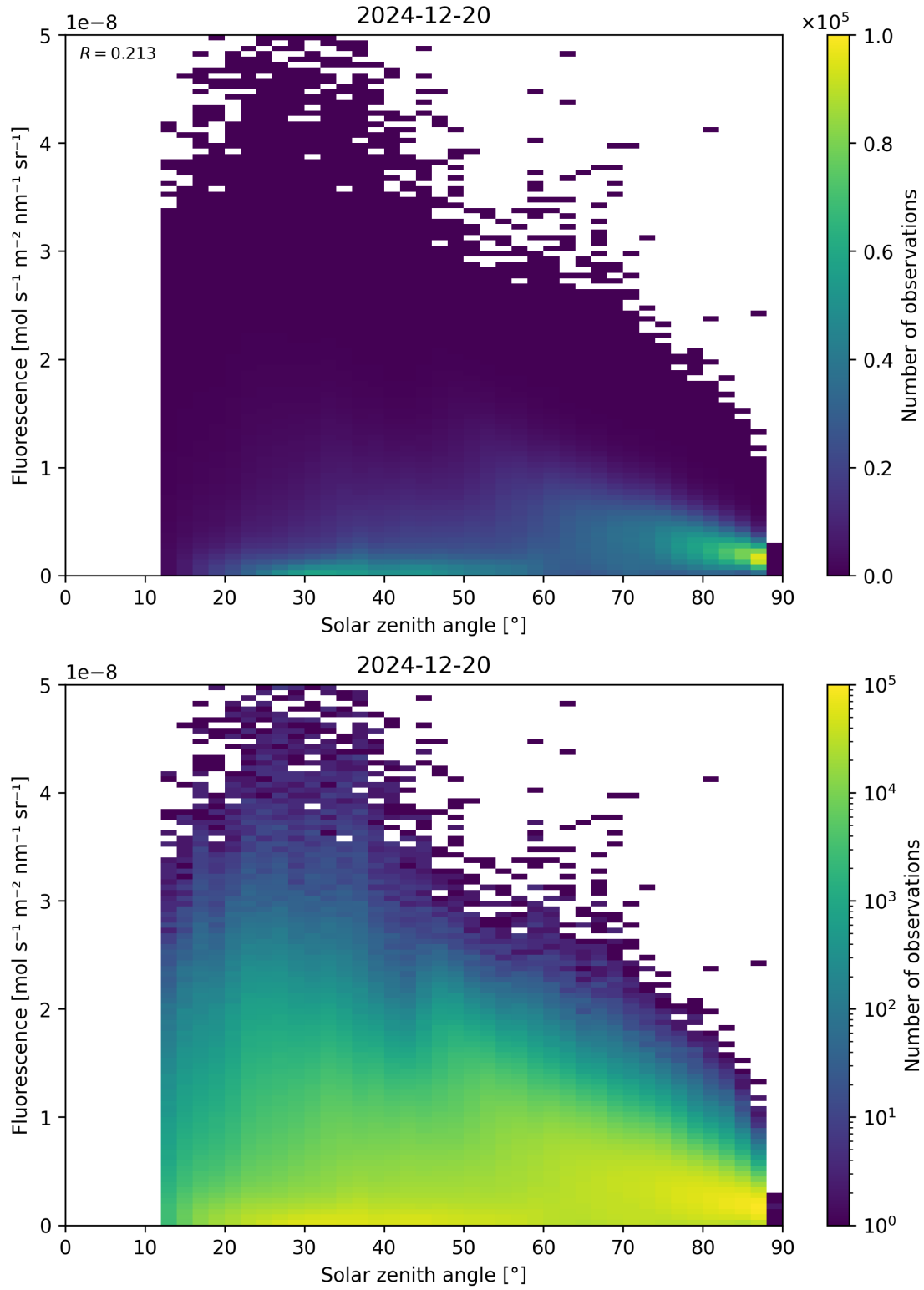
Figure 112: Scatter density plot of “Solar zenith angle” against “Fluorescence” for 2024-12-19 to 2024-12-21.
