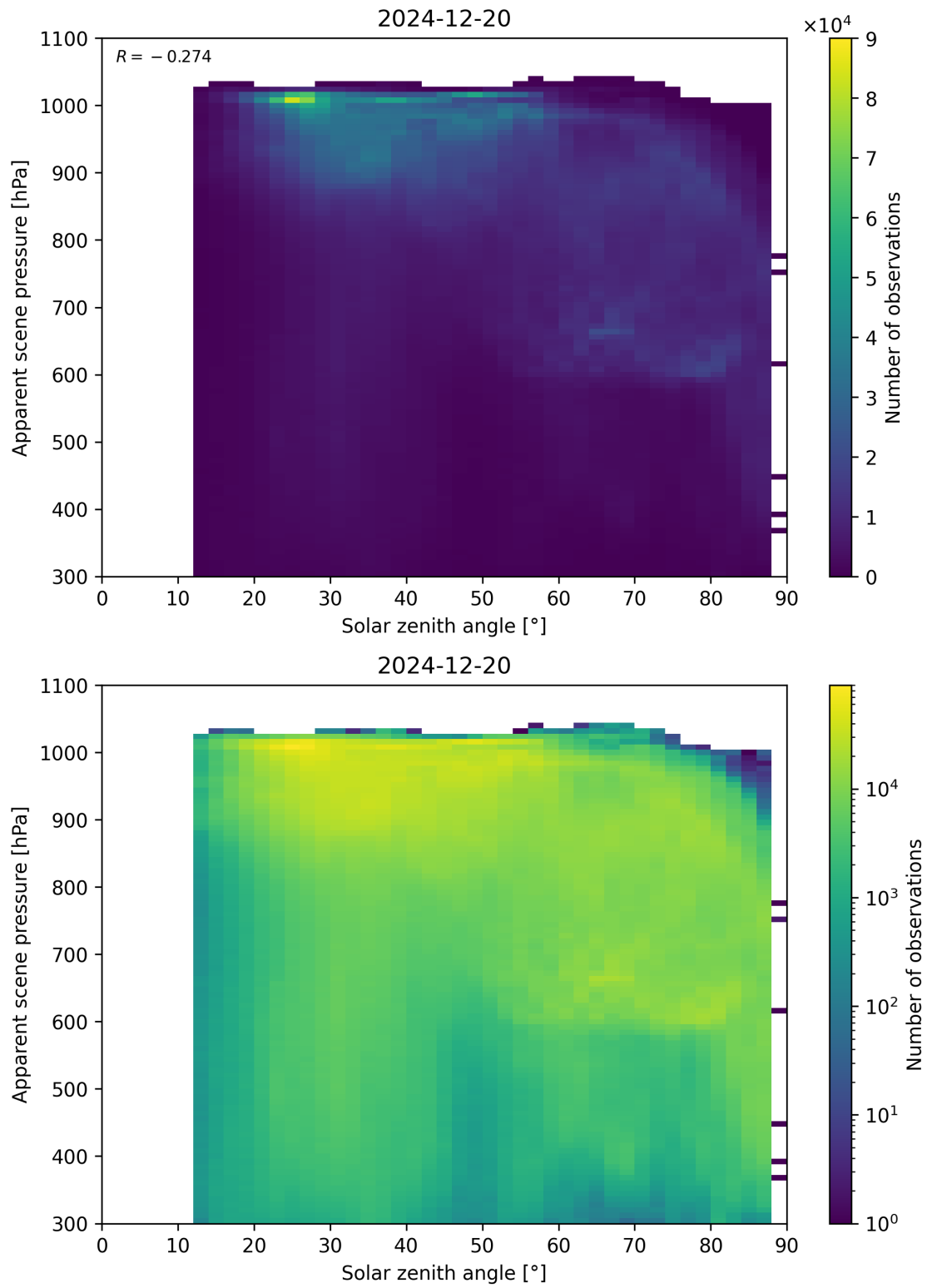
Figure 108: Scatter density plot of “Solar zenith angle” against “Apparent scene pressure” for 2024-12-19 to 2024-12-21.
