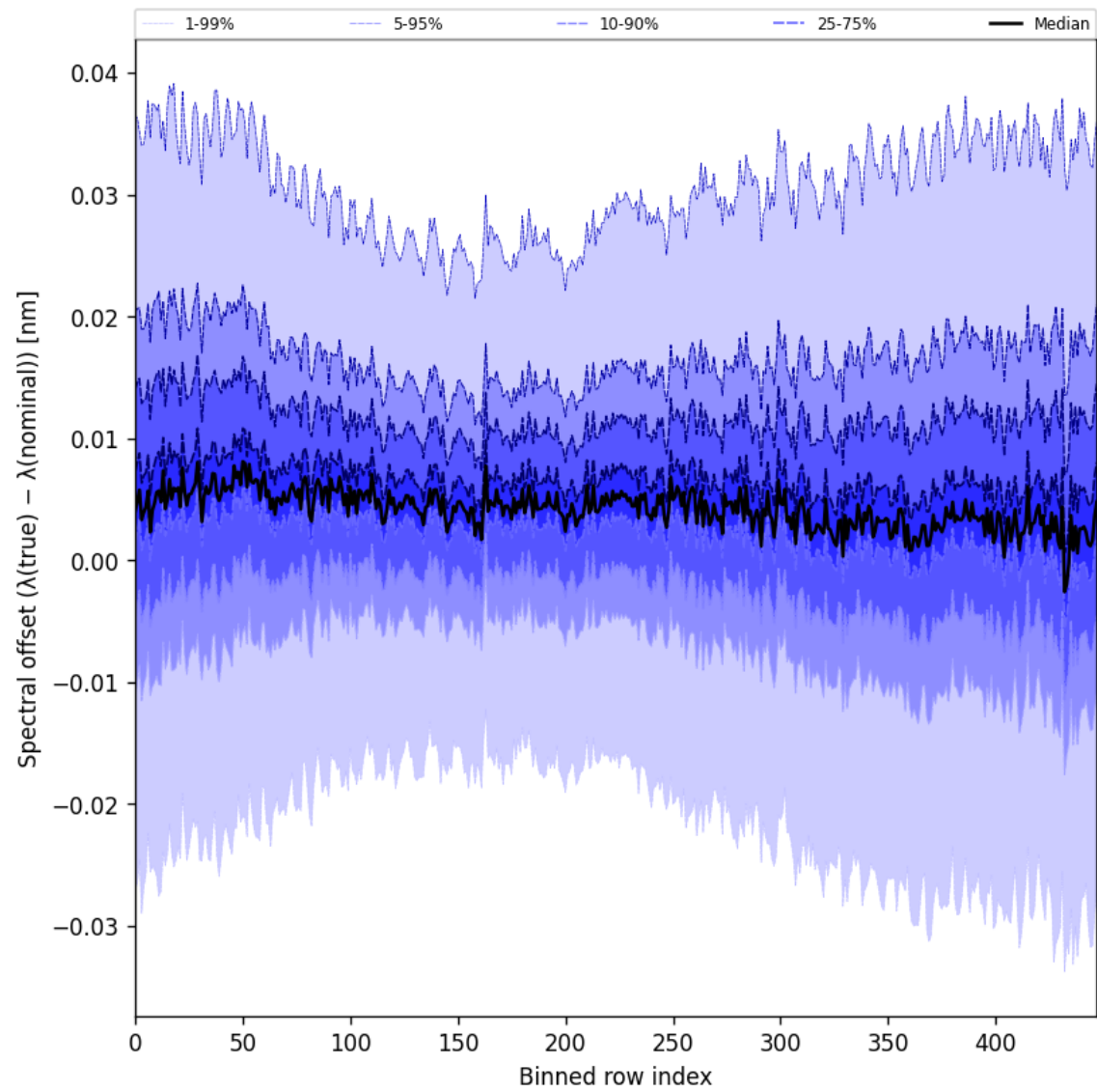
Figure 62: Along track statistics of “Spectral offset ( \lambda_{\text{true}} - \lambda_{\text{nominal}} )” for 2024-12-19 to 2024-12-21
