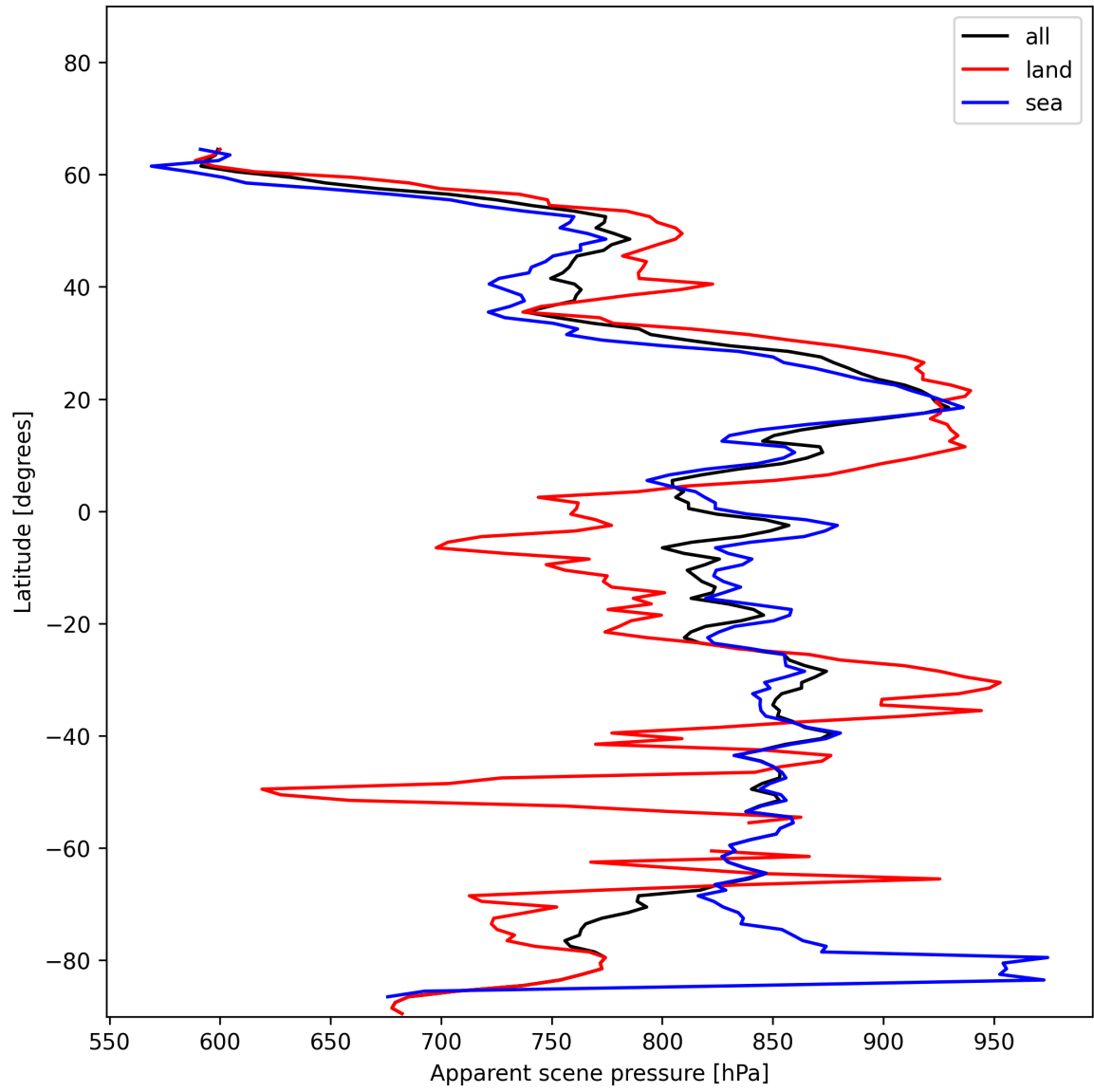
Figure 19: Zonal average of “Apparent scene pressure” for 2024-12-19 to 2024-12-21.
