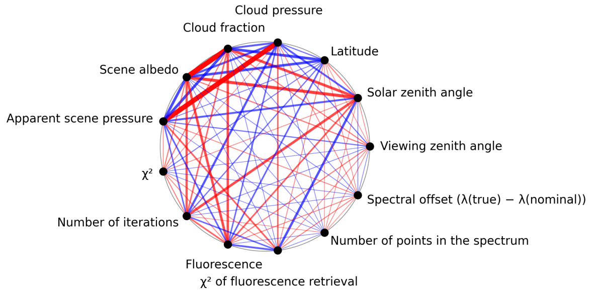
Figure 1: Map of correlation graph for 2024-12-19 to 2024-12-21.
