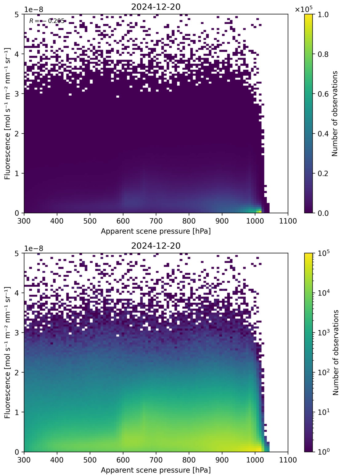
Figure 64: Scatter density plot of “Apparent scene pressure” against “Fluorescence” for 2024-12-19 to 2024-12-21.
