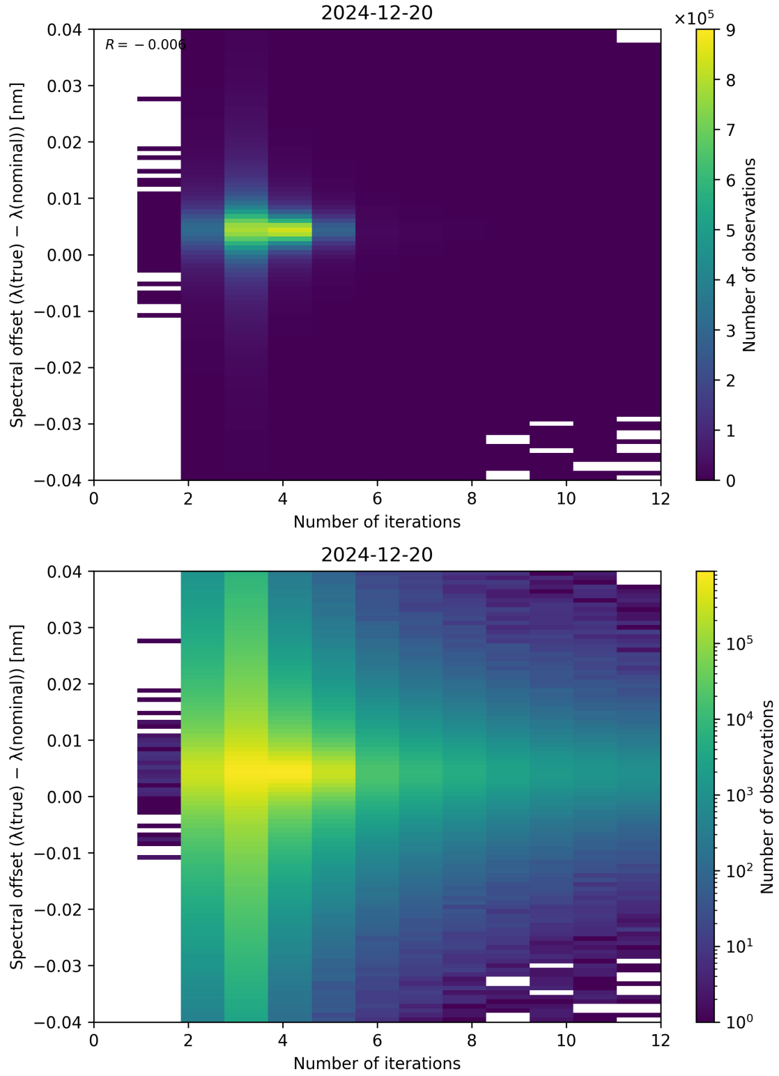
Figure 100: Scatter density plot of “Number of iterations” against “Spectral offset ( \lambda_{\text{true}} - \lambda_{\text{nominal}} )” for 2024-12-19 to 2024-12-21.
