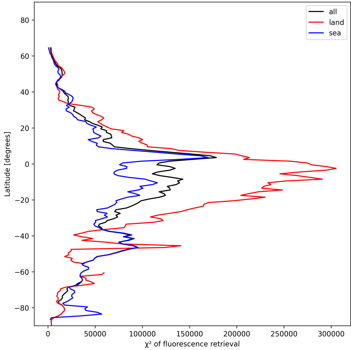
Figure 25: Zonal average of “ \chi^2 of fluorescence retrieval” for 2024-12-19 to 2024-12-21.
