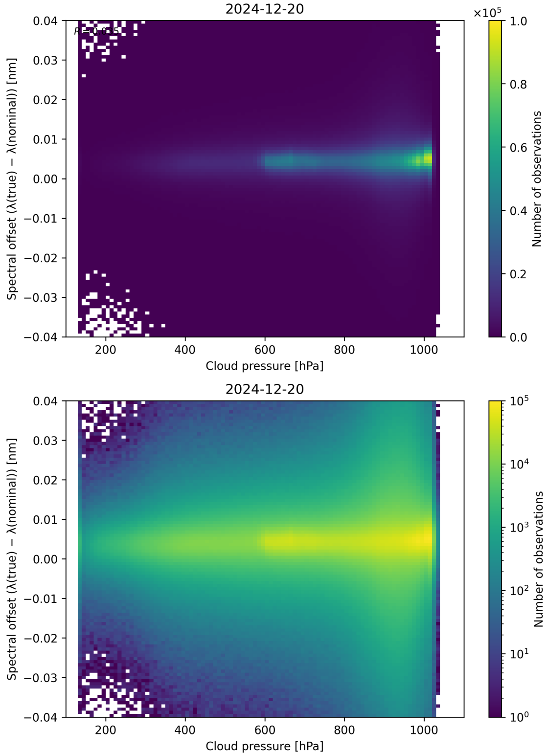
Figure 84: Scatter density plot of “Cloud pressure” against “Spectral offset ( \lambda_{\text{true}} - \lambda_{\text{nominal}} )” for 2024-12-19 to 2024-12-21.
