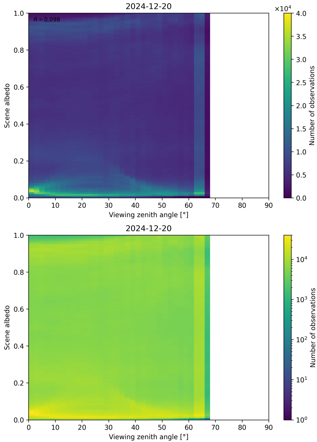
Figure 126: Scatter density plot of “Viewing zenith angle” against “Scene albedo” for 2024-12-19 to 2024-12-21.
