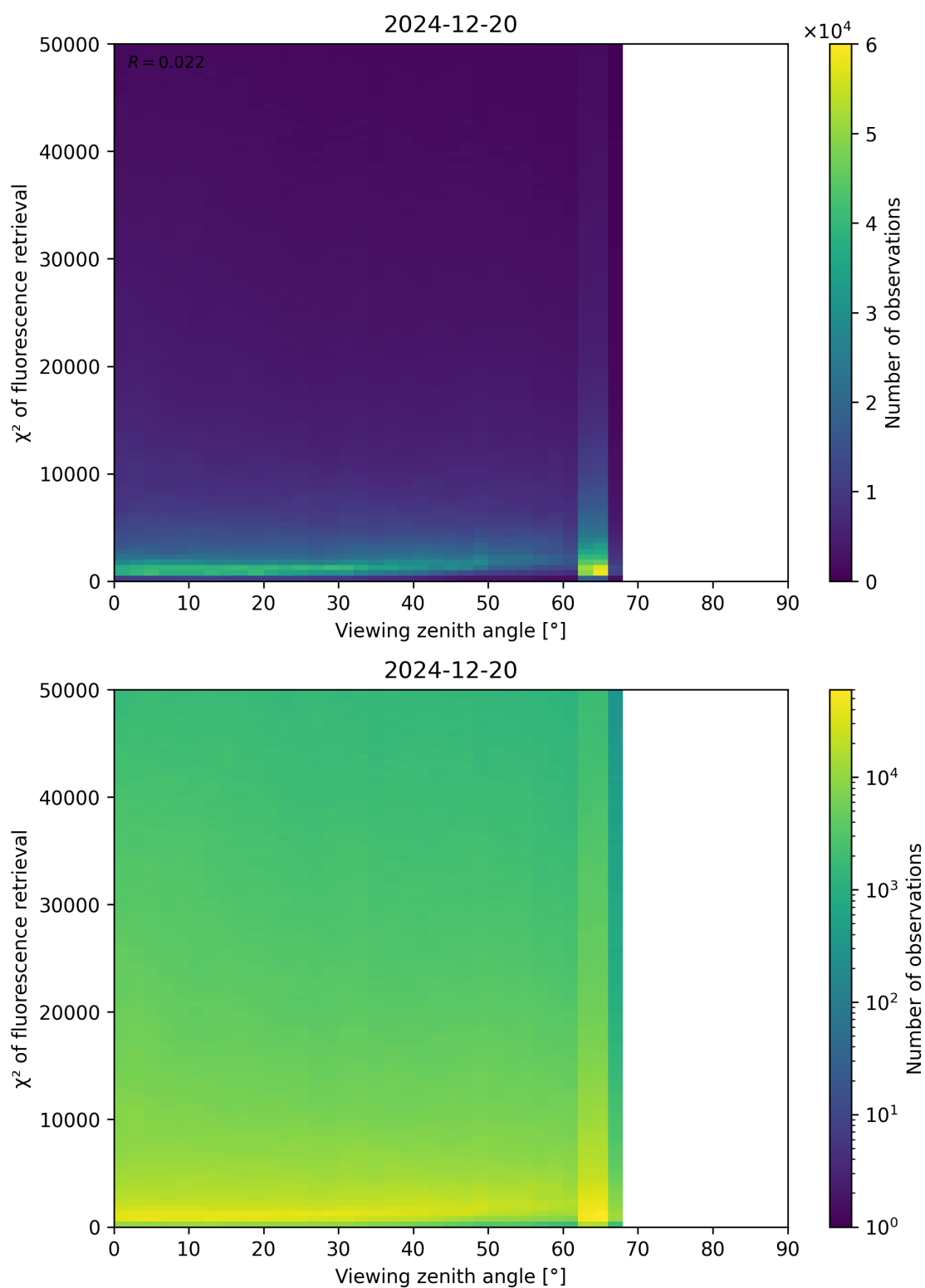
Figure 119: Scatter density plot of “Viewing zenith angle” against “ \chi^2 of fluorescence retrieval” for 2024-12-19 to 2024-12-21.
