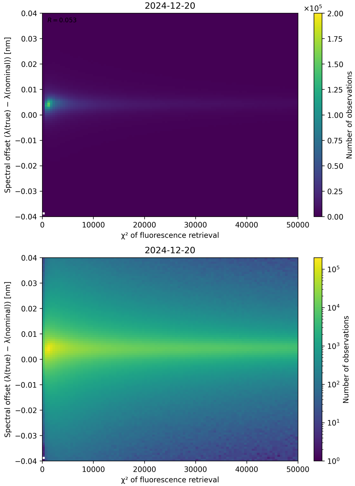
Figure 69: Scatter density plot of “ \chi^2 of fluorescence retrieval” against “Spectral offset ( \lambda_{\text{true}} - \lambda_{\text{nominal}} )” for 2024-12-19 to 2024-12-21.
