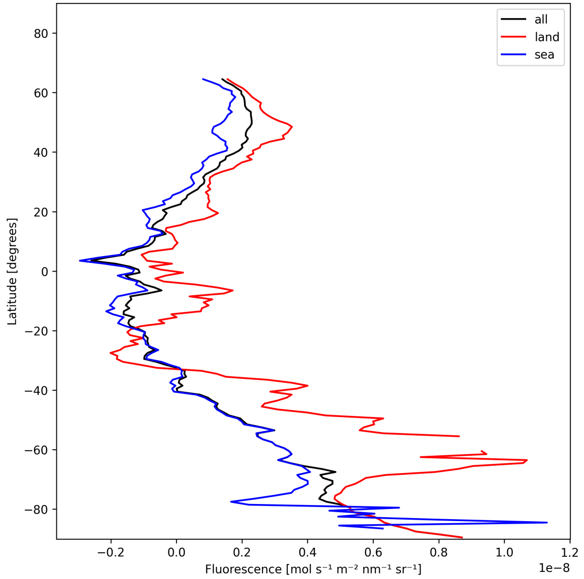
Figure 23: Zonal average of “Fluorescence” for 2024-12-19 to 2024-12-21.
