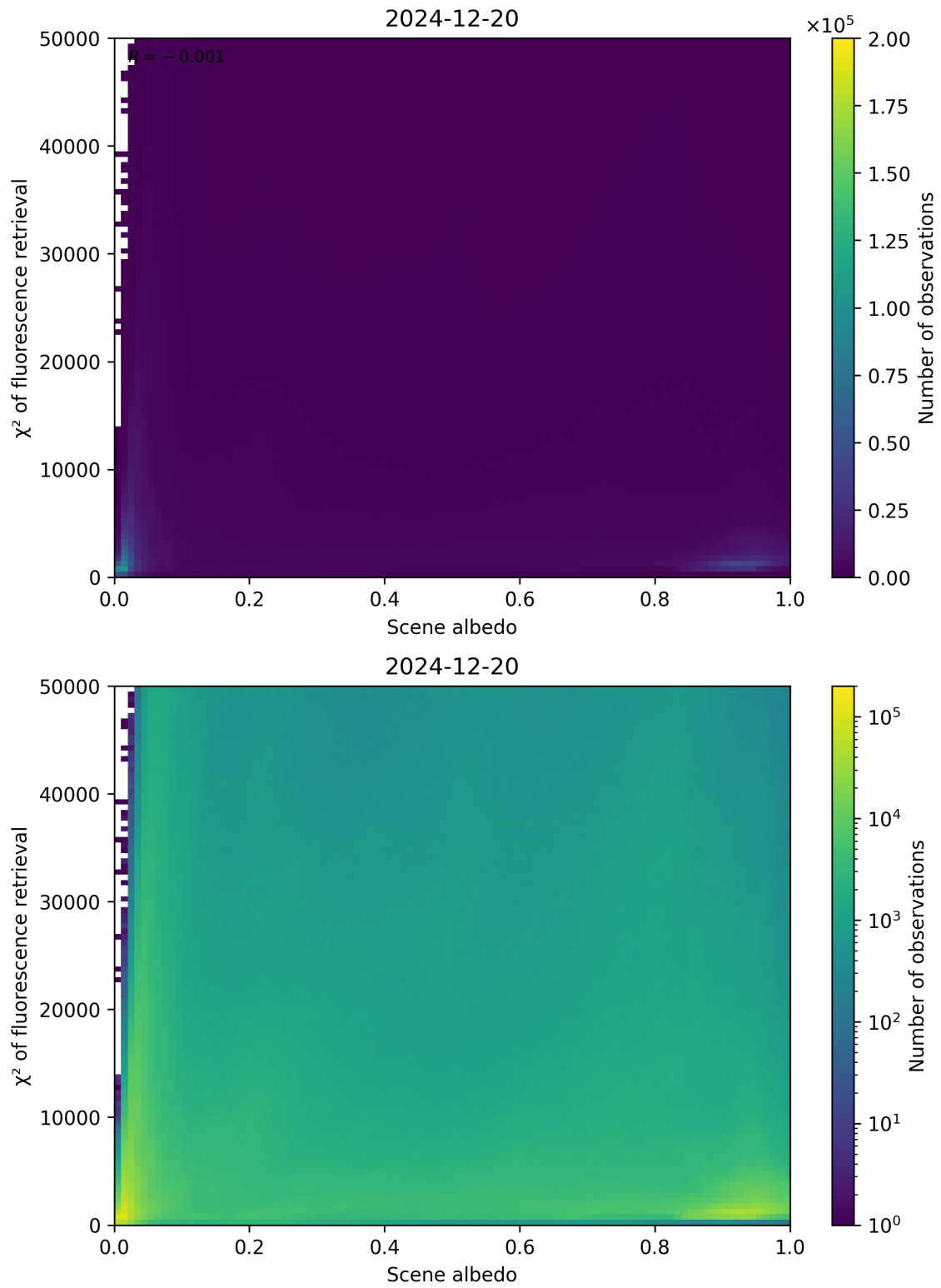
Figure 103: Scatter density plot of “Scene albedo” against “ \chi^2 of fluorescence retrieval” for 2024-12-19 to 2024-12-21.
