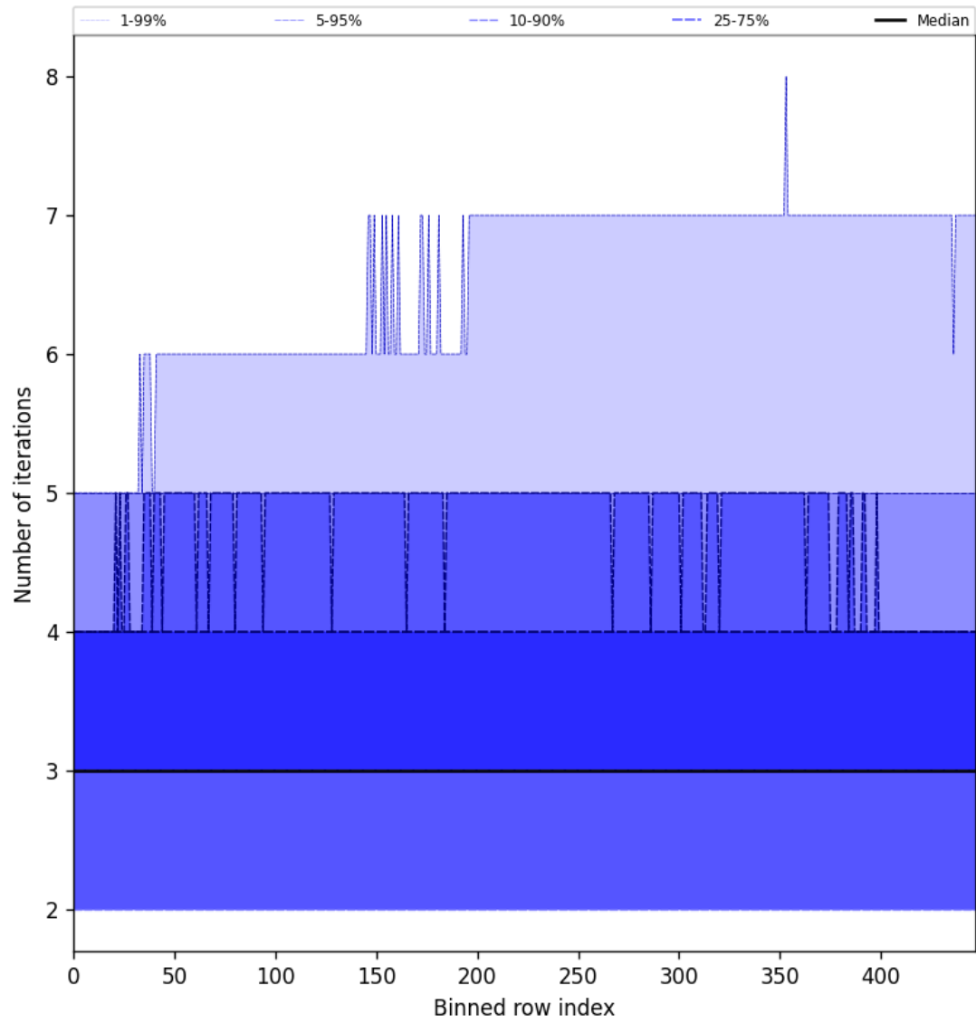
Figure 56: Along track statistics of “Number of iterations” for 2024-12-19 to 2024-12-21
