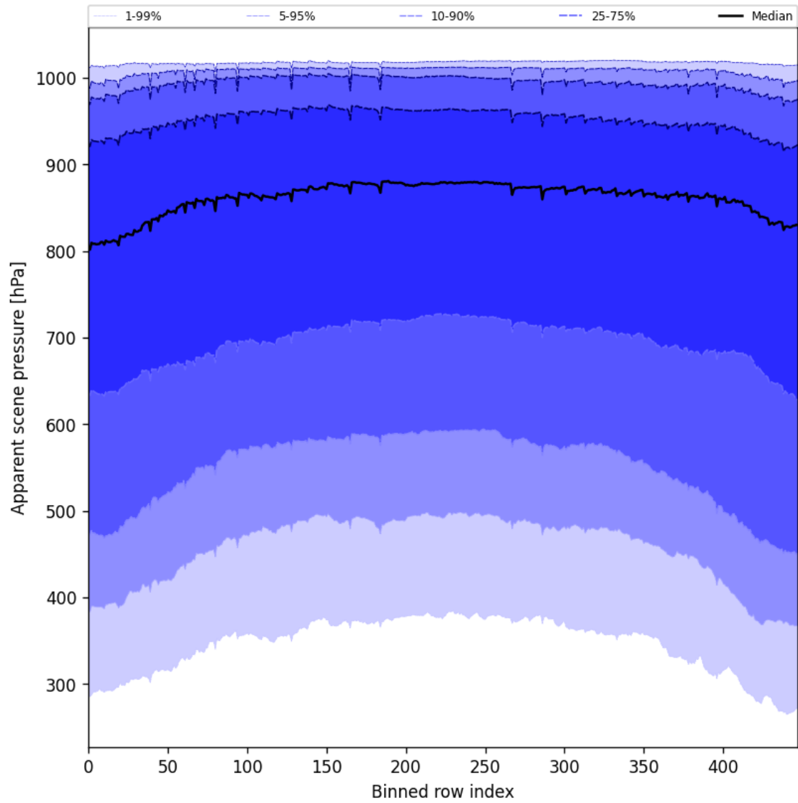
Figure 53: Along track statistics of “Apparent scene pressure” for 2024-12-19 to 2024-12-21
