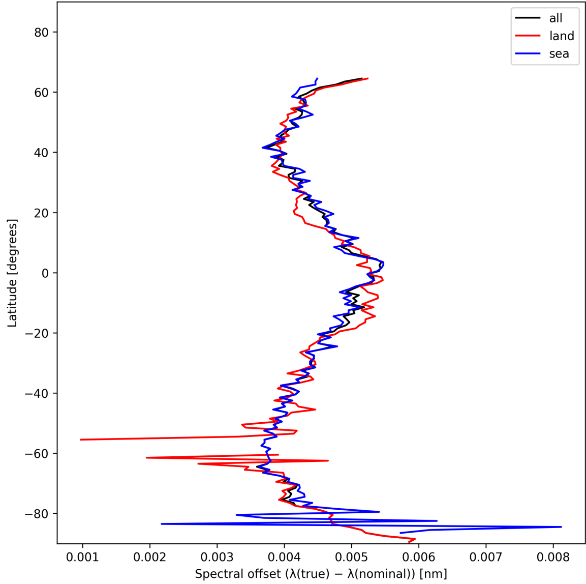
Figure 28: Zonal average of “Spectral offset ( \lambda_{\text{true}} - \lambda_{\text{nominal}} )” for 2024-12-19 to 2024-12-21.
