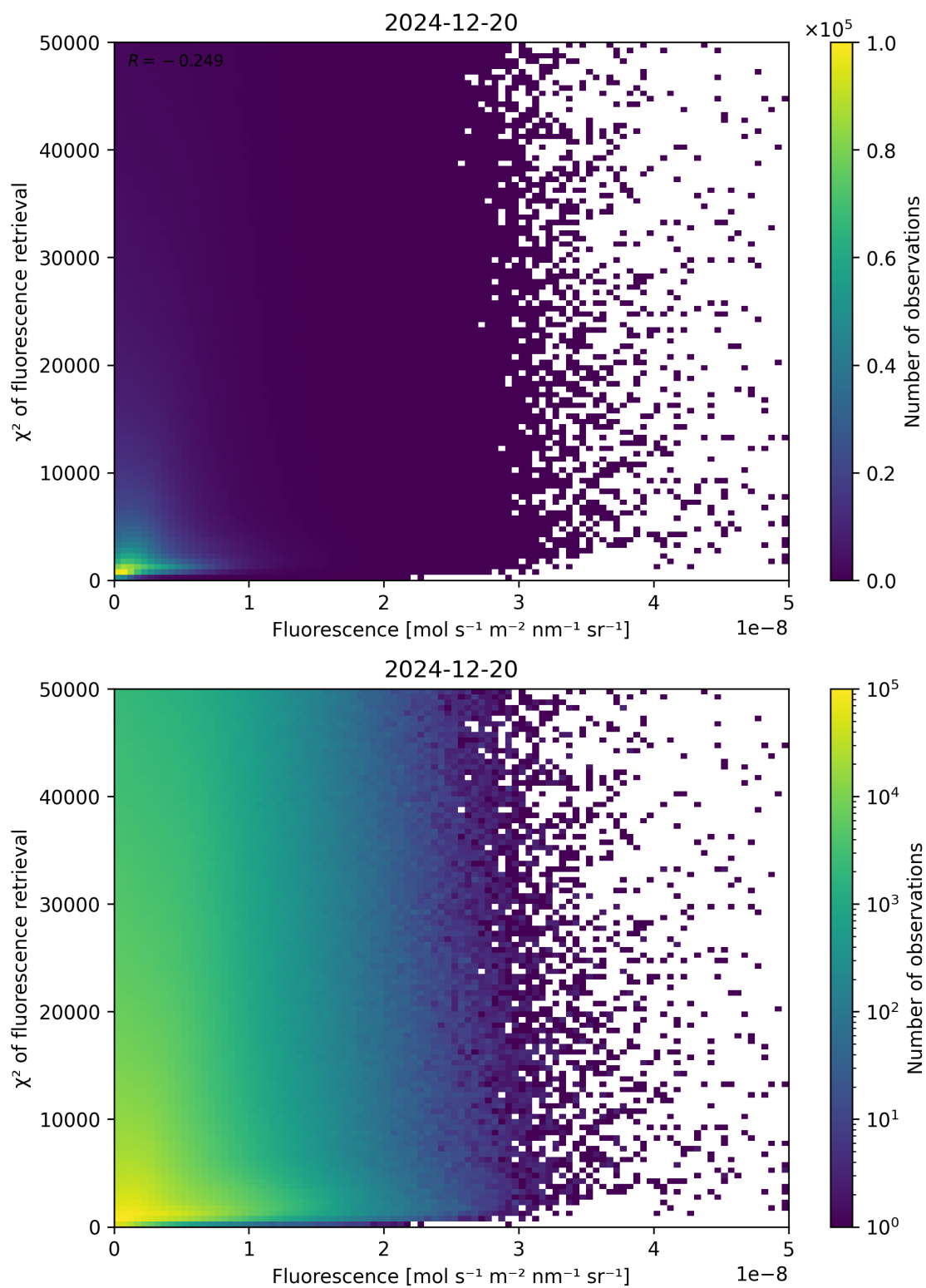
Figure 85: Scatter density plot of “Fluorescence” against “ \chi^2 of fluorescence retrieval” for 2024-12-19 to 2024-12-21.
