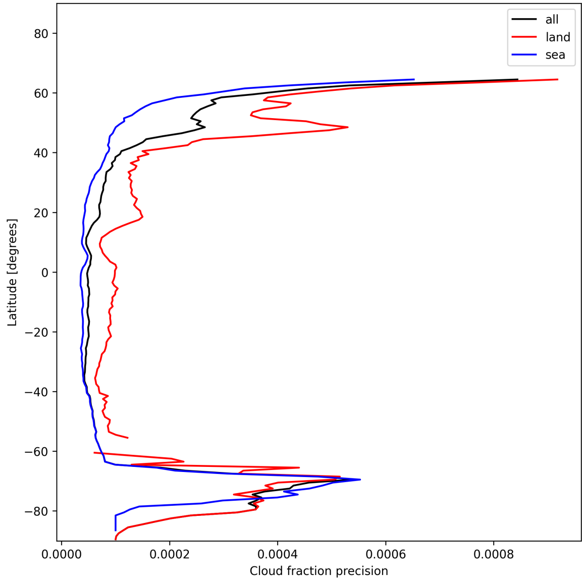
Figure 16: Zonal average of “Cloud fraction precision” for 2024-12-19 to 2024-12-21.
