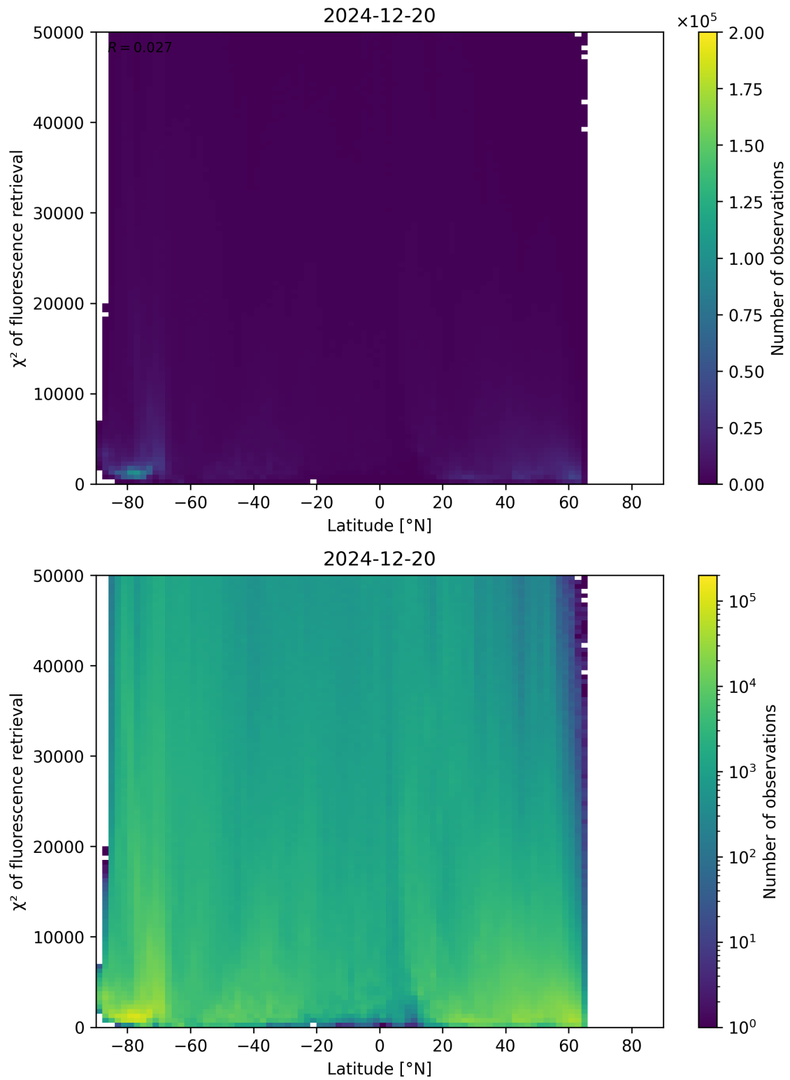
Figure 89: Scatter density plot of “Latitude” against “ \chi^2 of fluorescence retrieval” for 2024-12-19 to 2024-12-21.
