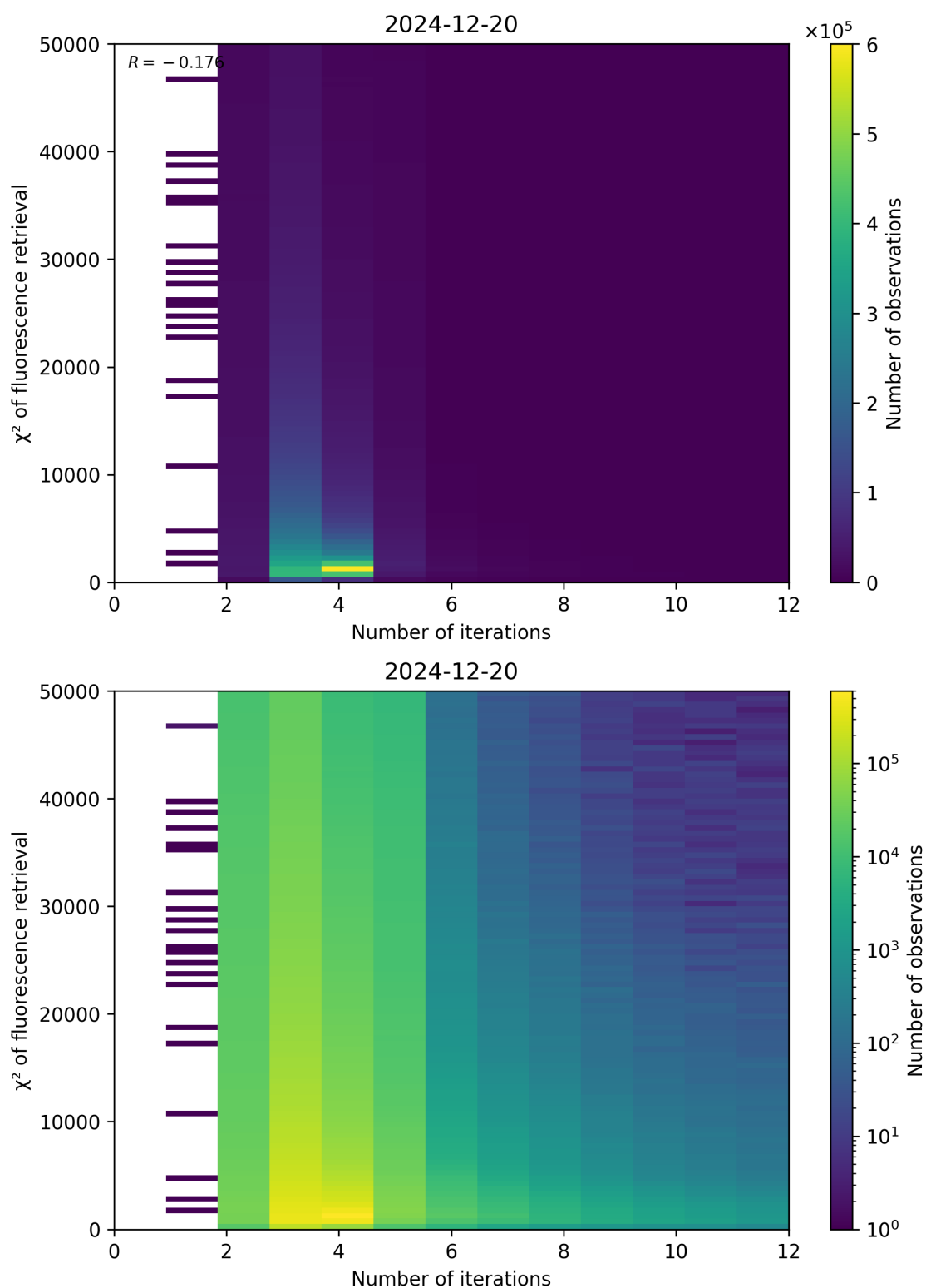
Figure 97: Scatter density plot of “Number of iterations” against “ \chi^2 of fluorescence retrieval” for 2024-12-19 to 2024-12-21.
