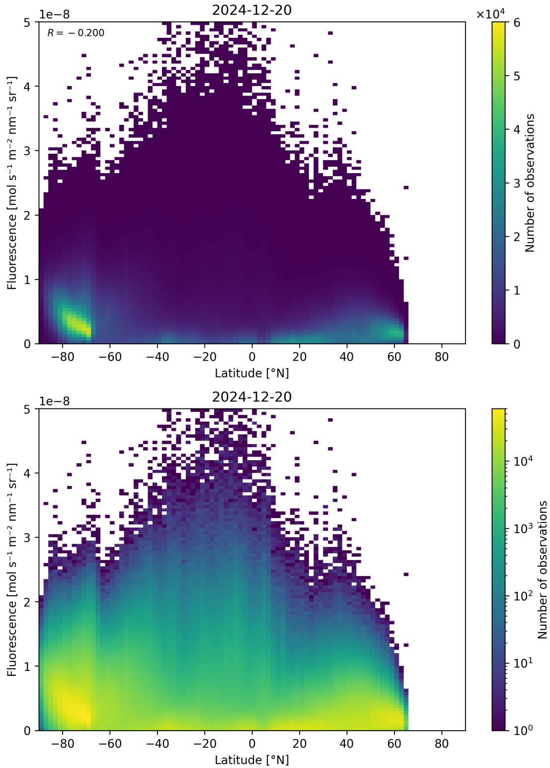
Figure 92: Scatter density plot of “Latitude” against “Fluorescence” for 2024-12-19 to 2024-12-21.
