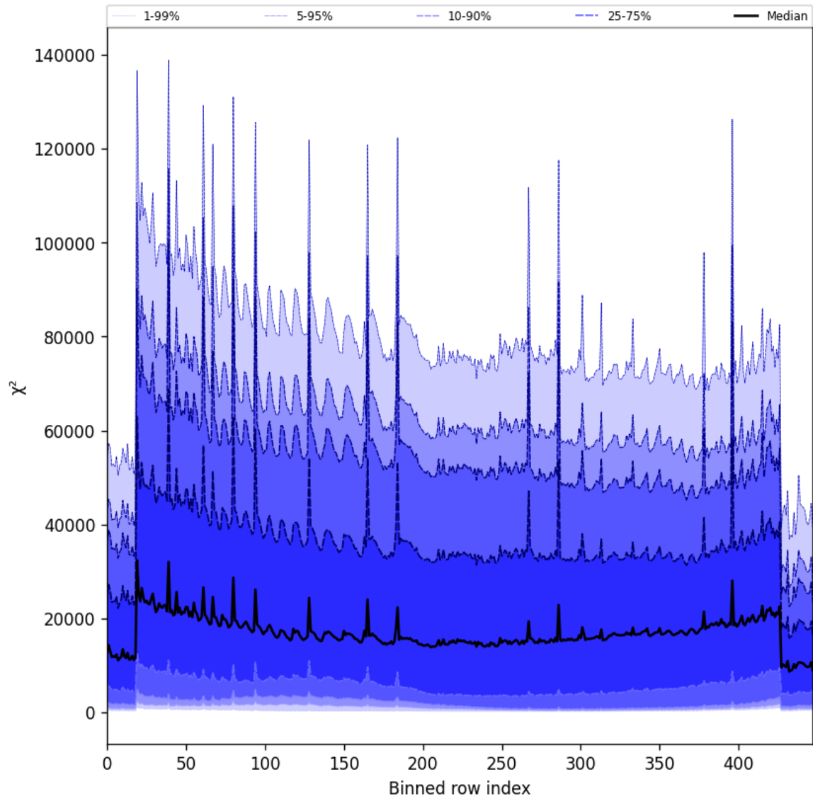
Figure 55: Along track statistics of “ \chi^2 ” for 2024-12-19 to 2024-12-21
