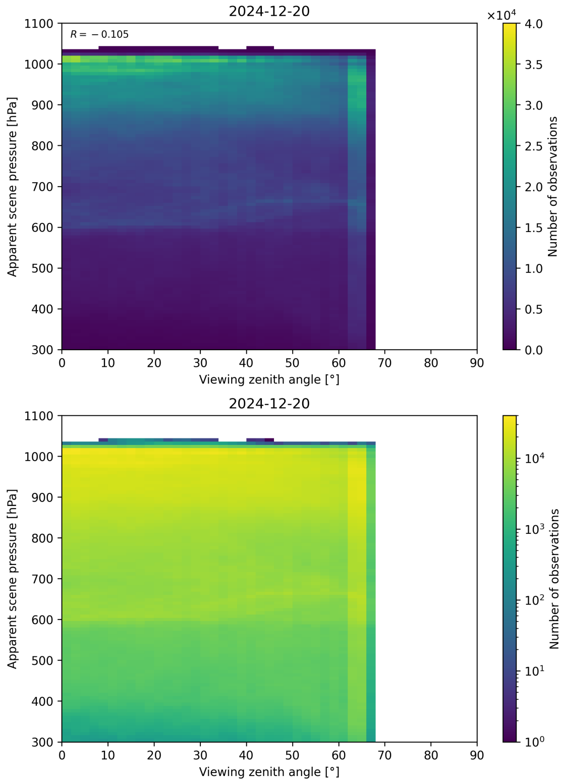
Figure 118: Scatter density plot of “Viewing zenith angle” against “Apparent scene pressure” for 2024-12-19 to 2024-12-21.
