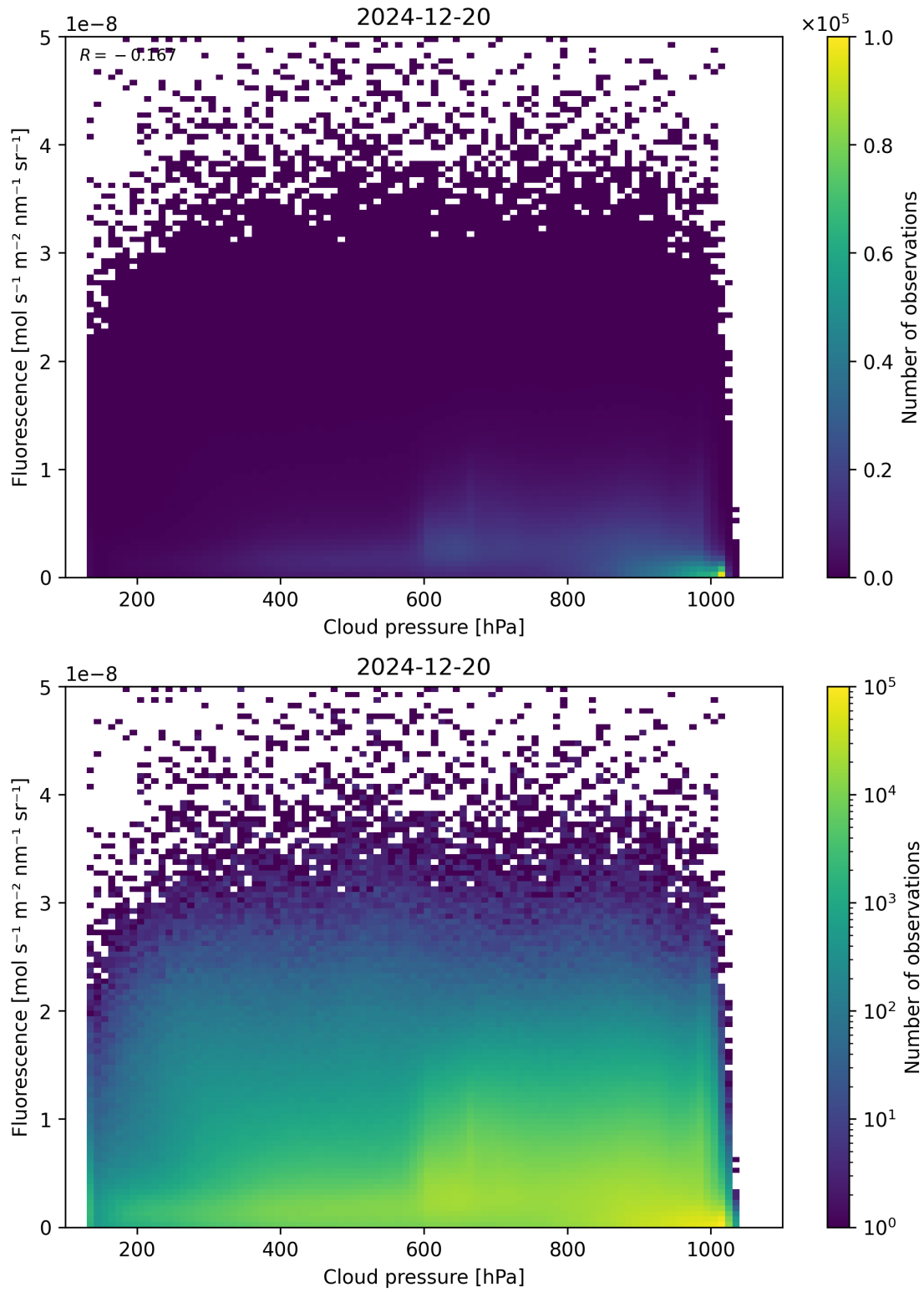
Figure 80: Scatter density plot of “Cloud pressure” against “Fluorescence” for 2024-12-19 to 2024-12-21.
