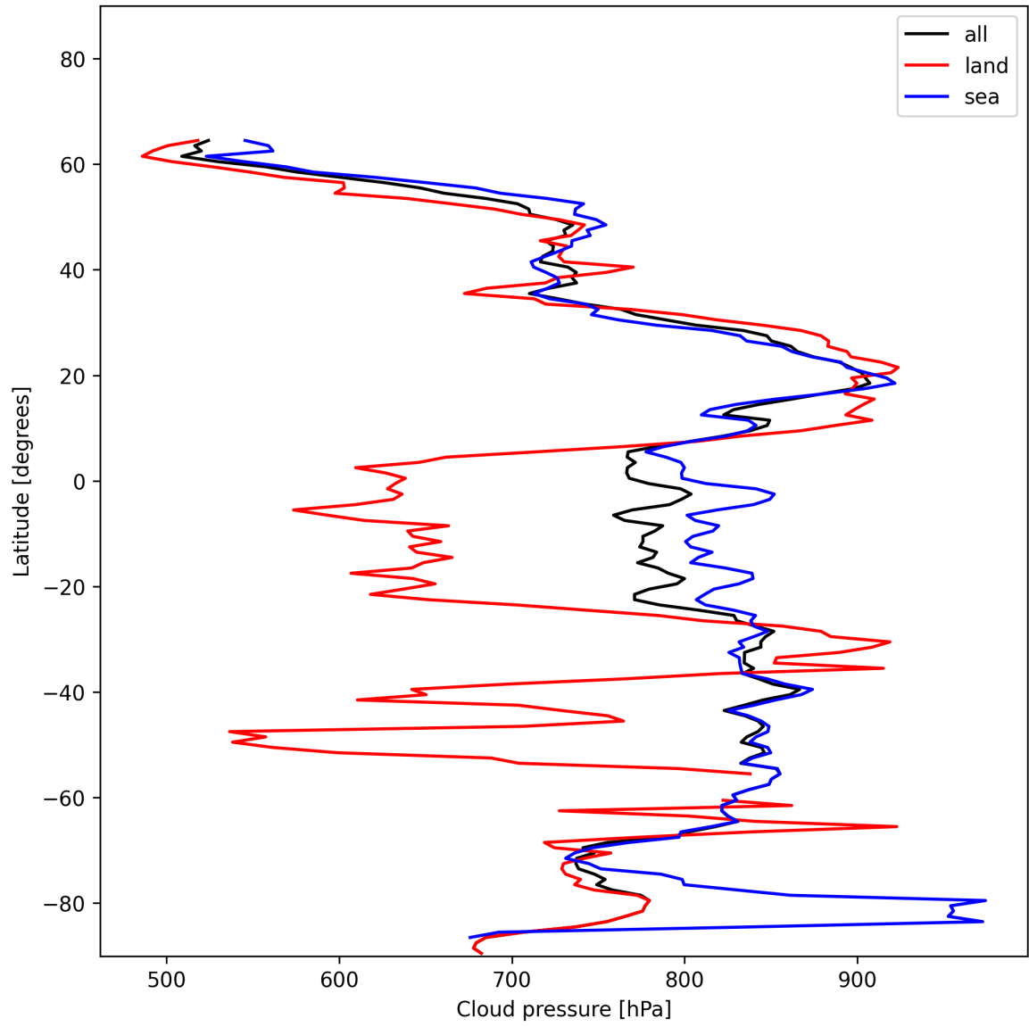
Figure 13: Zonal average of “Cloud pressure” for 2024-12-19 to 2024-12-21.
