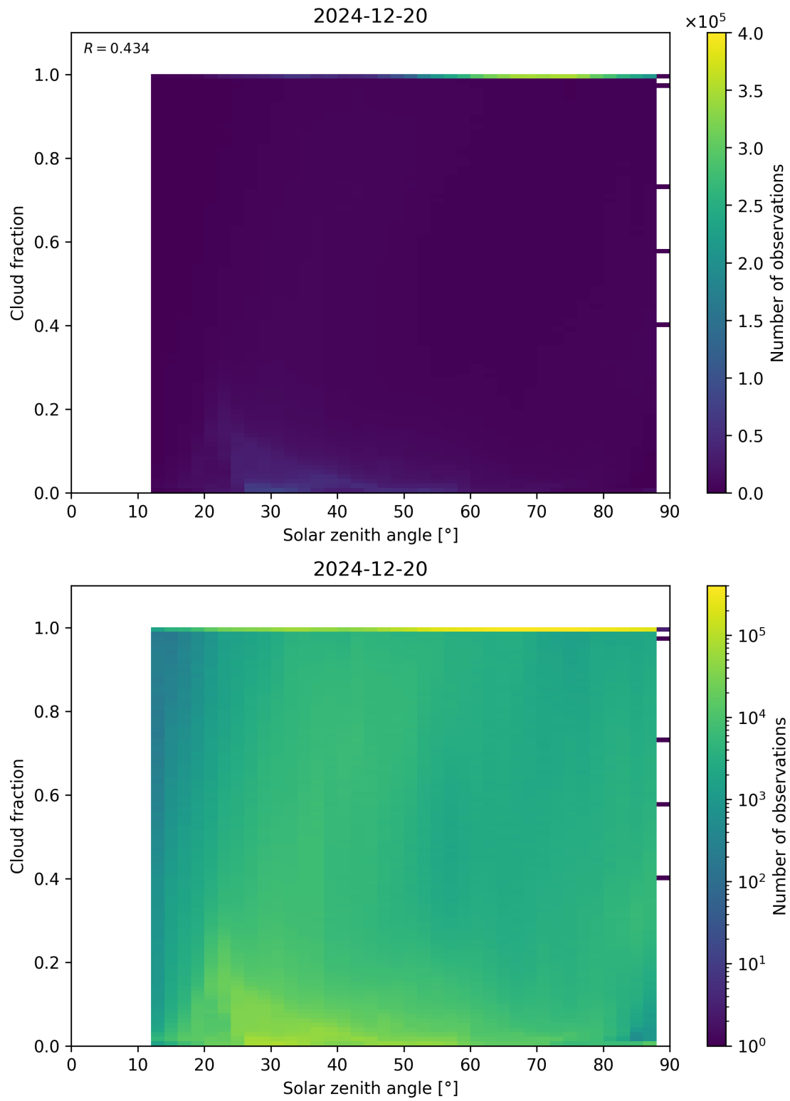
Figure 110: Scatter density plot of “Solar zenith angle” against “Cloud fraction” for 2024-12-19 to 2024-12-21.
