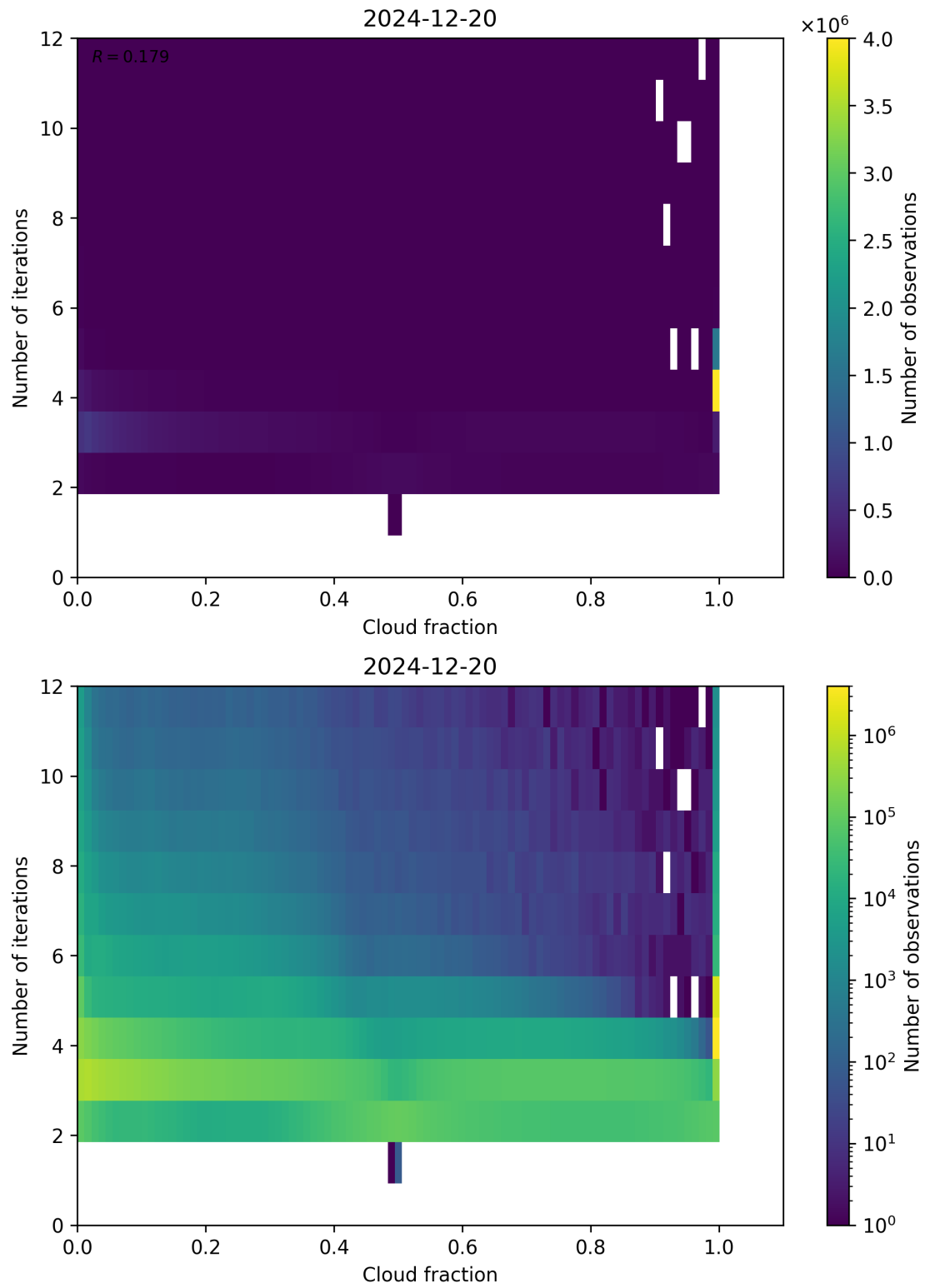
Figure 73: Scatter density plot of “Cloud fraction” against “Number of iterations” for 2024-12-19 to 2024-12-21.
