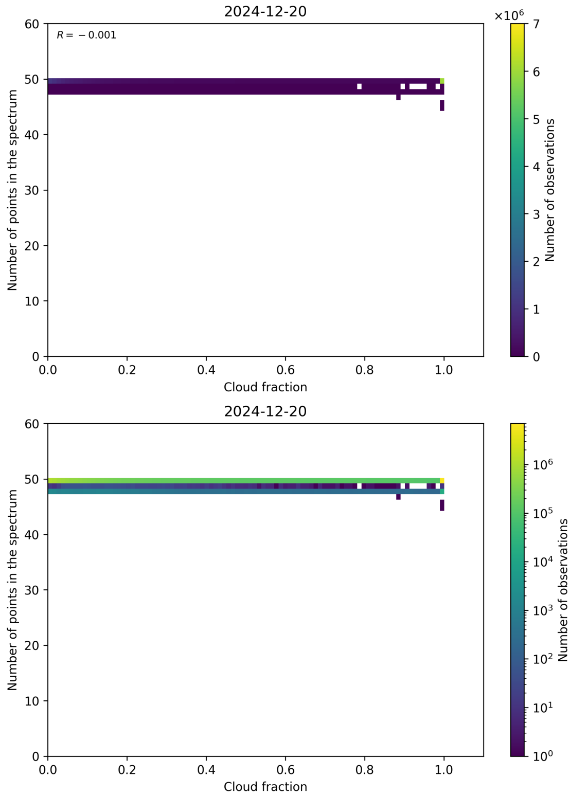
Figure 74: Scatter density plot of “Cloud fraction” against “Number of points in the spectrum” for 2024-12-19 to 2024-12-21.
