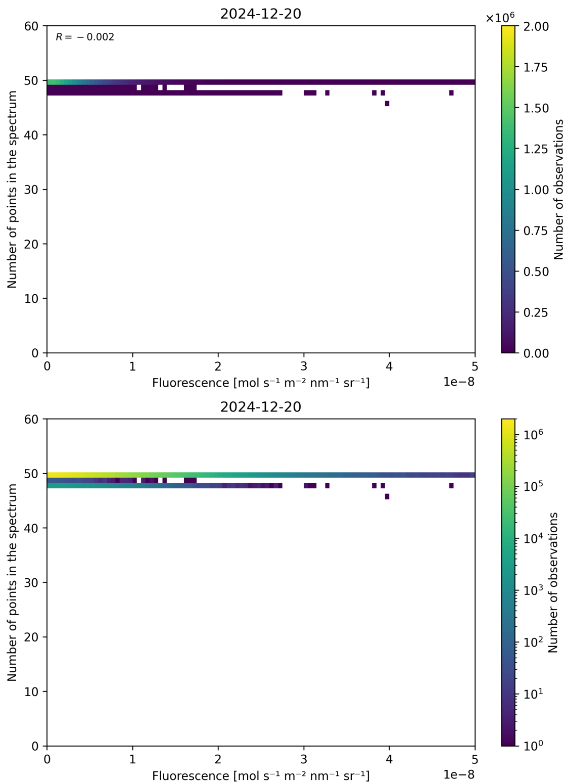
Figure 86: Scatter density plot of “Fluorescence” against “Number of points in the spectrum” for 2024-12-19 to 2024-12-21.
