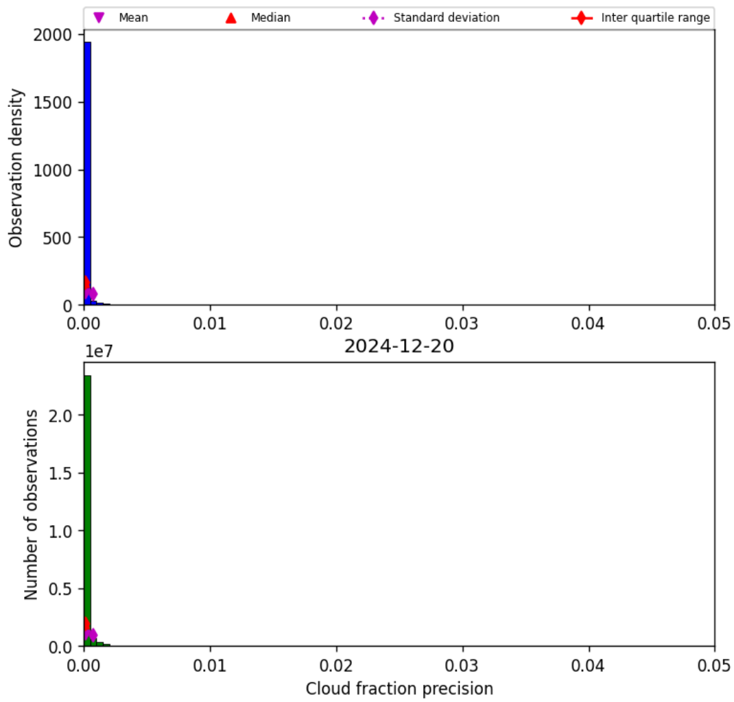
Figure 33: Histogram of “Cloud fraction precision” for 2024-12-19 to 2024-12-21
