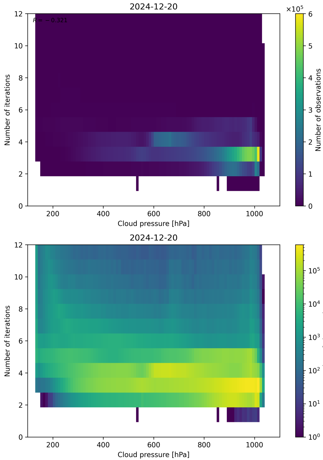
Figure 81: Scatter density plot of “Cloud pressure” against “Number of iterations” for 2024-12-19 to 2024-12-21.
