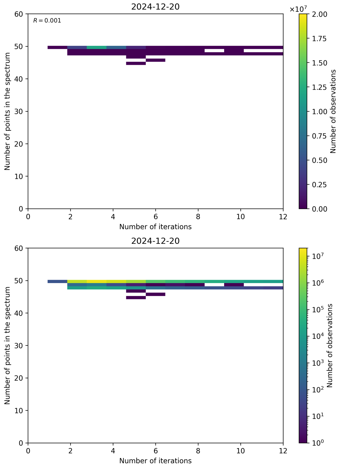
Figure 99: Scatter density plot of “Number of iterations” against “Number of points in the spectrum” for 2024-12-19 to 2024-12-21.
