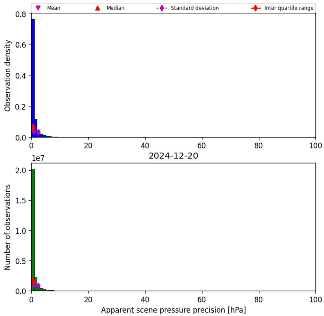
Figure 37: Histogram of “Apparent scene pressure precision” for 2024-12-19 to 2024-12-21
