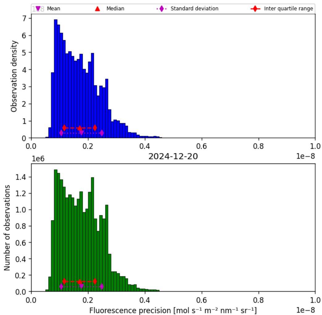
Figure 41: Histogram of “Fluorescence precision” for 2024-12-19 to 2024-12-21
