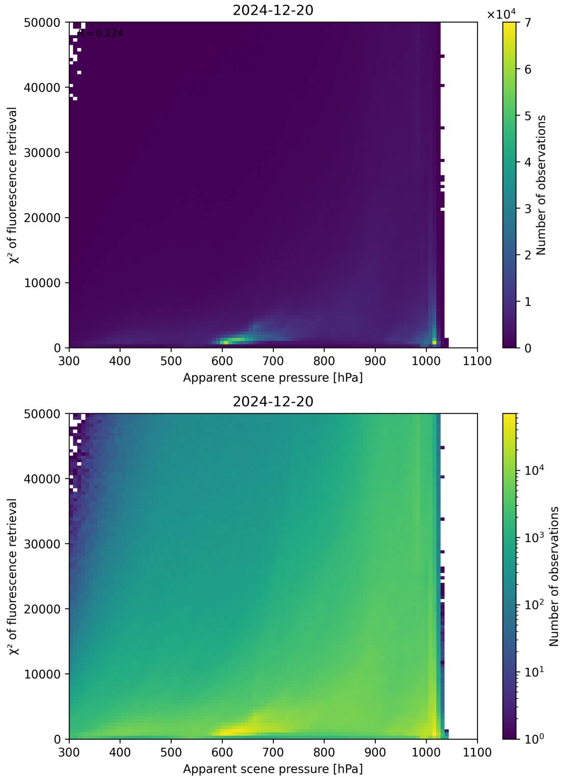
Figure 63: Scatter density plot of “Apparent scene pressure” against “ \chi^2 of fluorescence retrieval” for 2024-12-19 to 2024-12-21.
