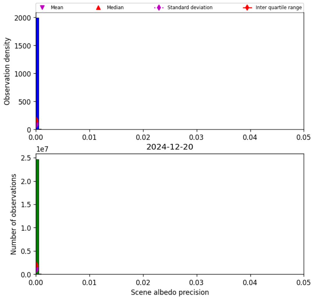
Figure 35: Histogram of “Scene albedo precision” for 2024-12-19 to 2024-12-21
