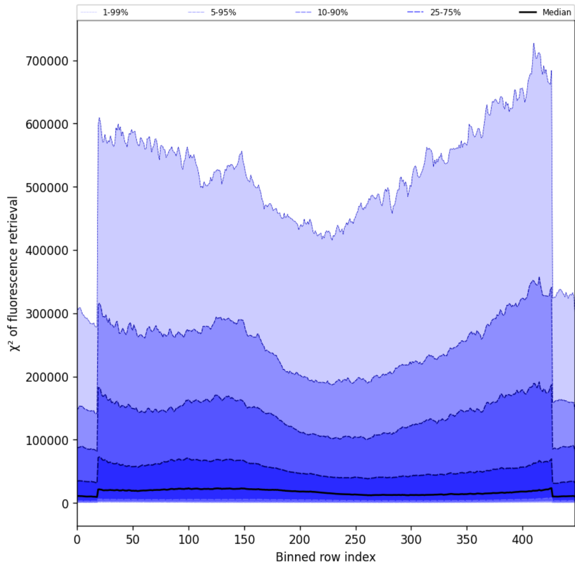
Figure 59: Along track statistics of “ \chi^2 of fluorescence retrieval” for 2024-12-19 to 2024-12-21
