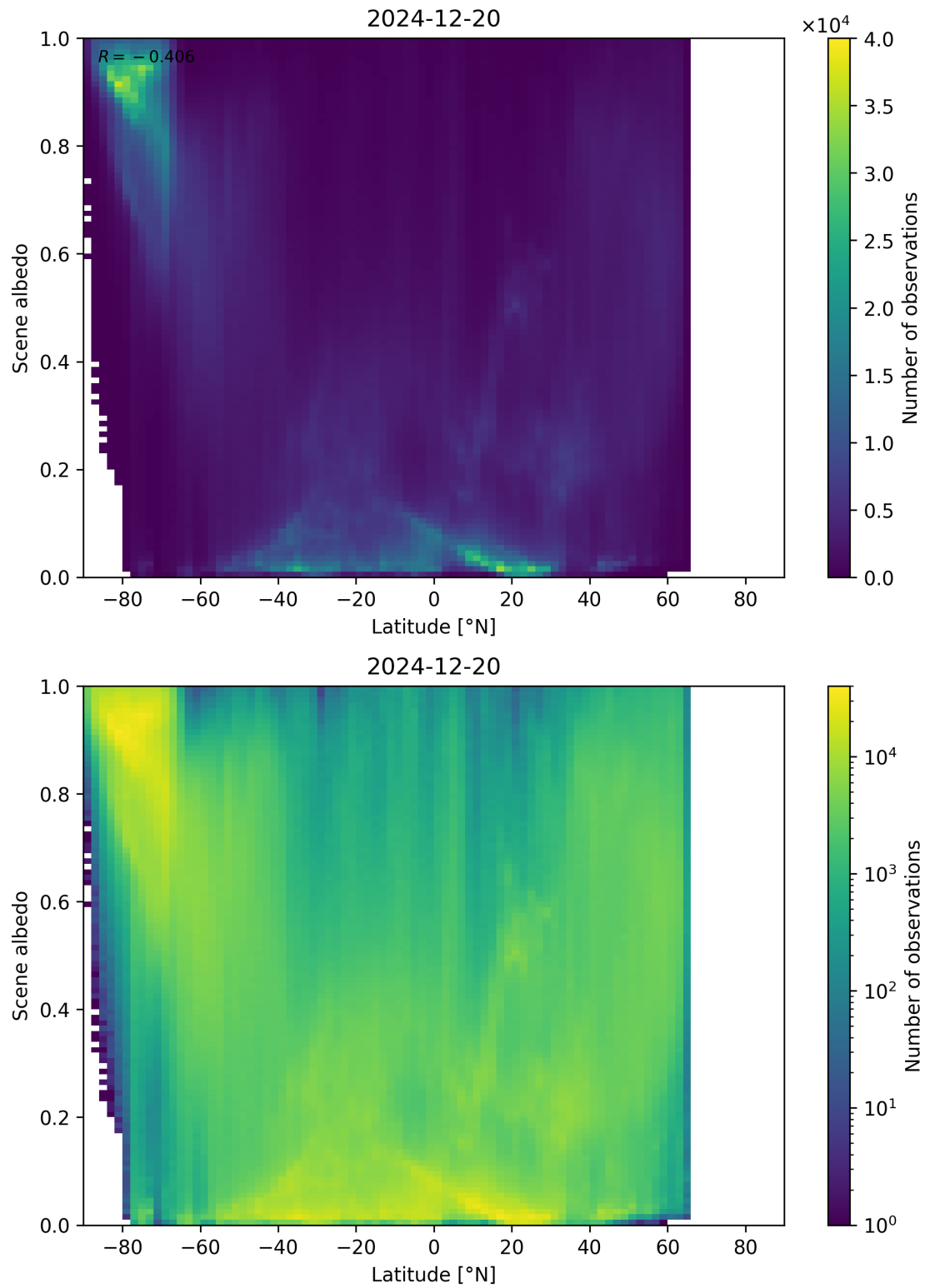
Figure 95: Scatter density plot of “Latitude” against “Scene albedo” for 2024-12-19 to 2024-12-21.
