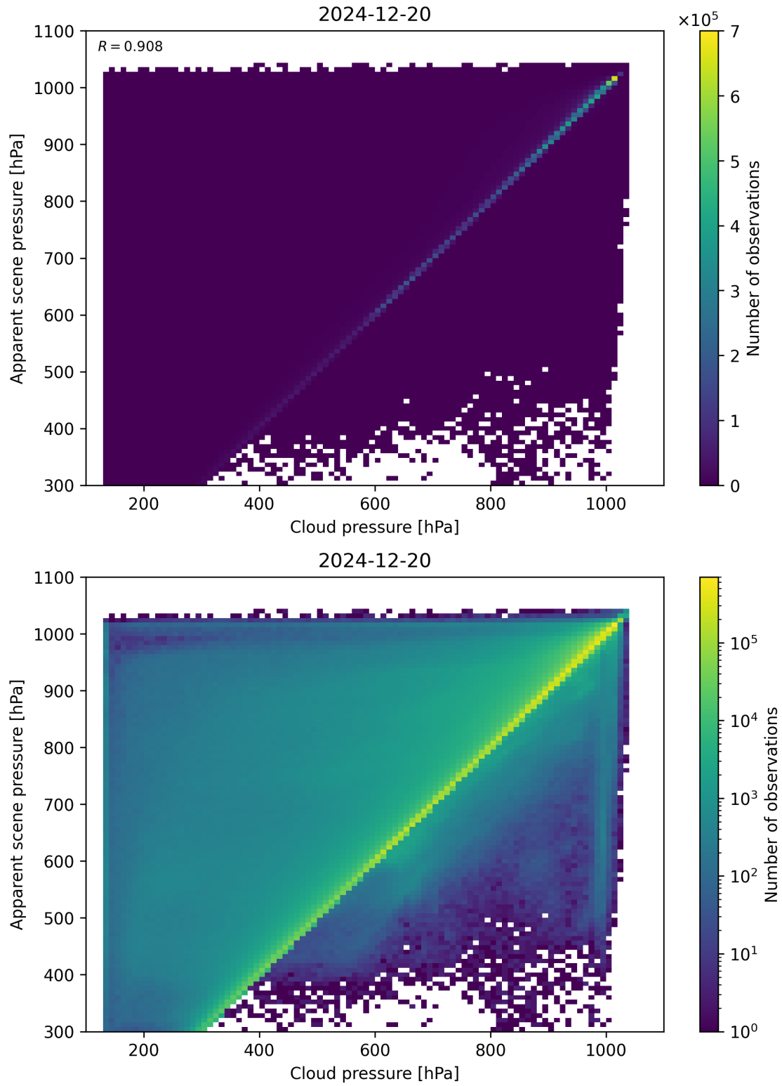
Figure 77: Scatter density plot of “Cloud pressure” against “Apparent scene pressure” for 2024-12-19 to 2024-12-21.
