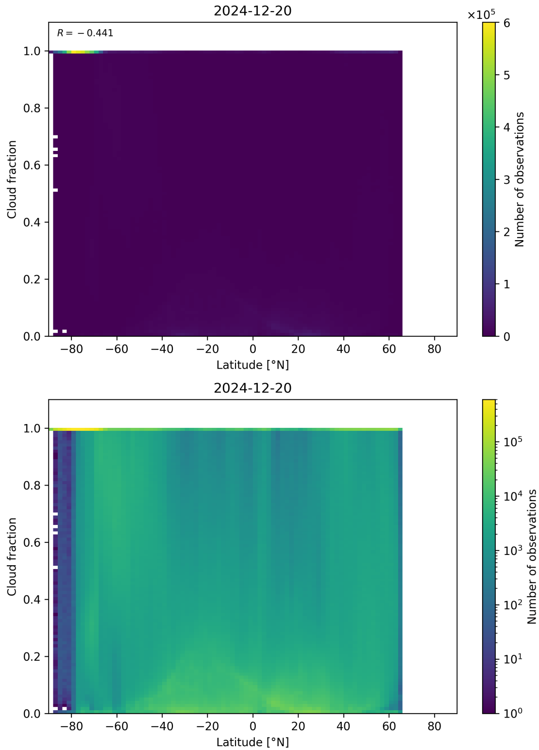
Figure 90: Scatter density plot of “Latitude” against “Cloud fraction” for 2024-12-19 to 2024-12-21.
