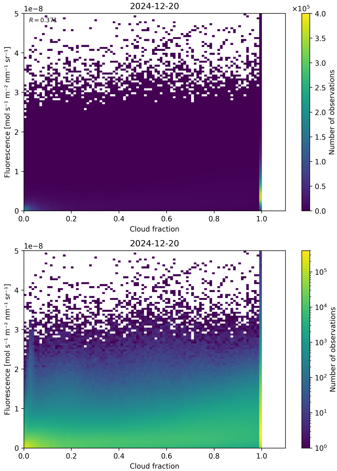
Figure 72: Scatter density plot of “Cloud fraction” against “Fluorescence” for 2024-12-19 to 2024-12-21.
