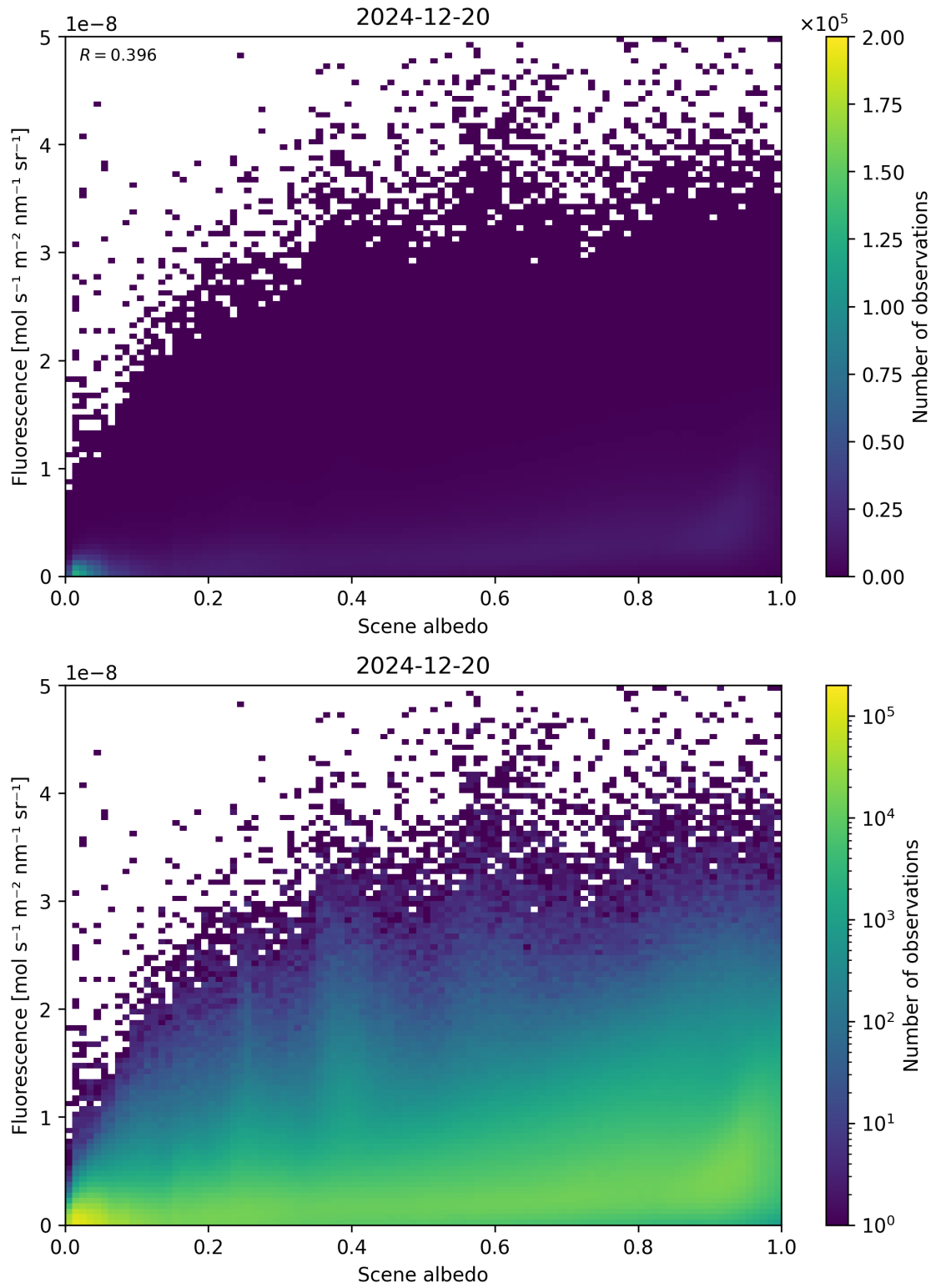
Figure 104: Scatter density plot of “Scene albedo” against “Fluorescence” for 2024-12-19 to 2024-12-21.
