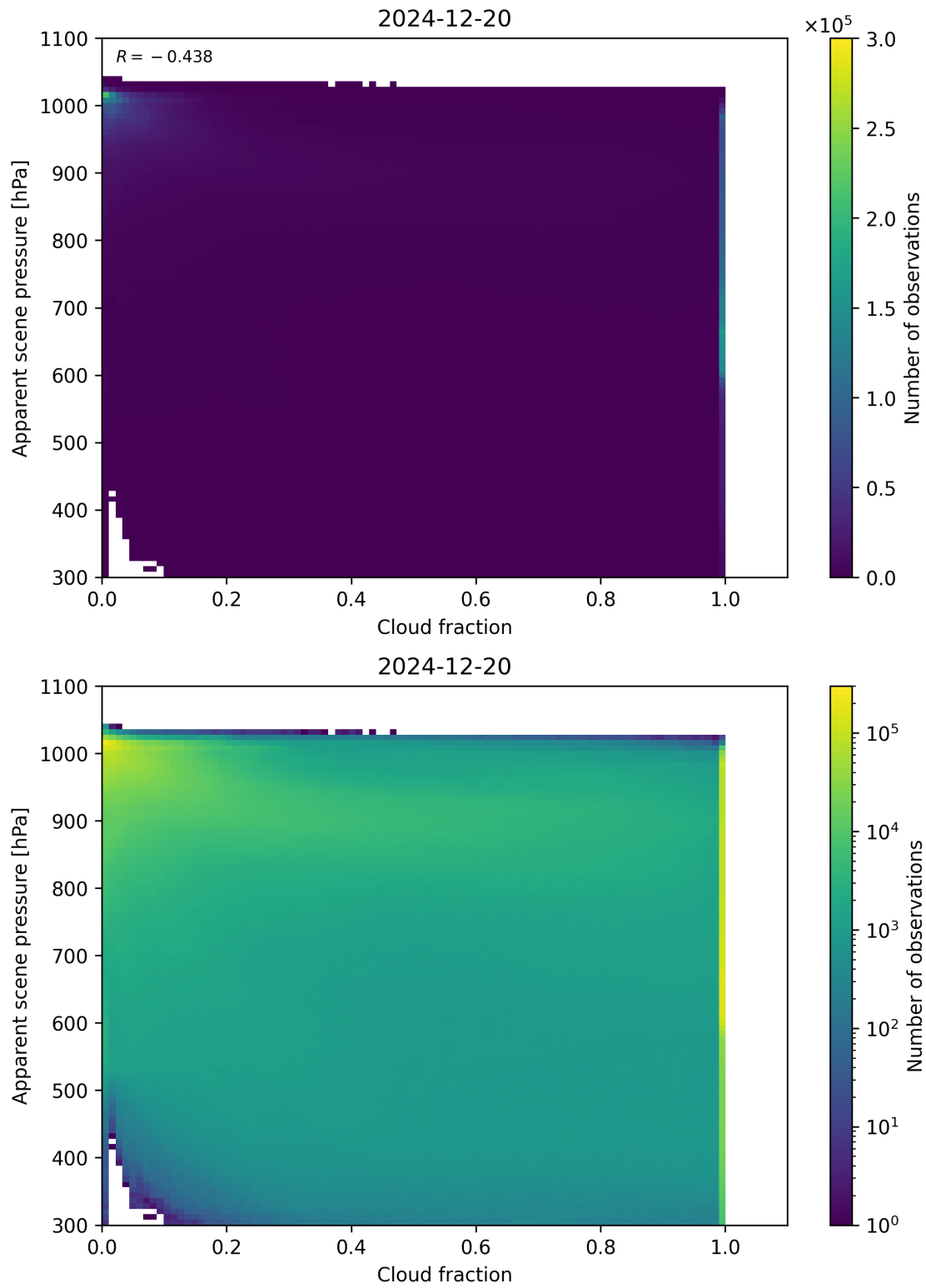
Figure 70: Scatter density plot of “Cloud fraction” against “Apparent scene pressure” for 2024-12-19 to 2024-12-21.
