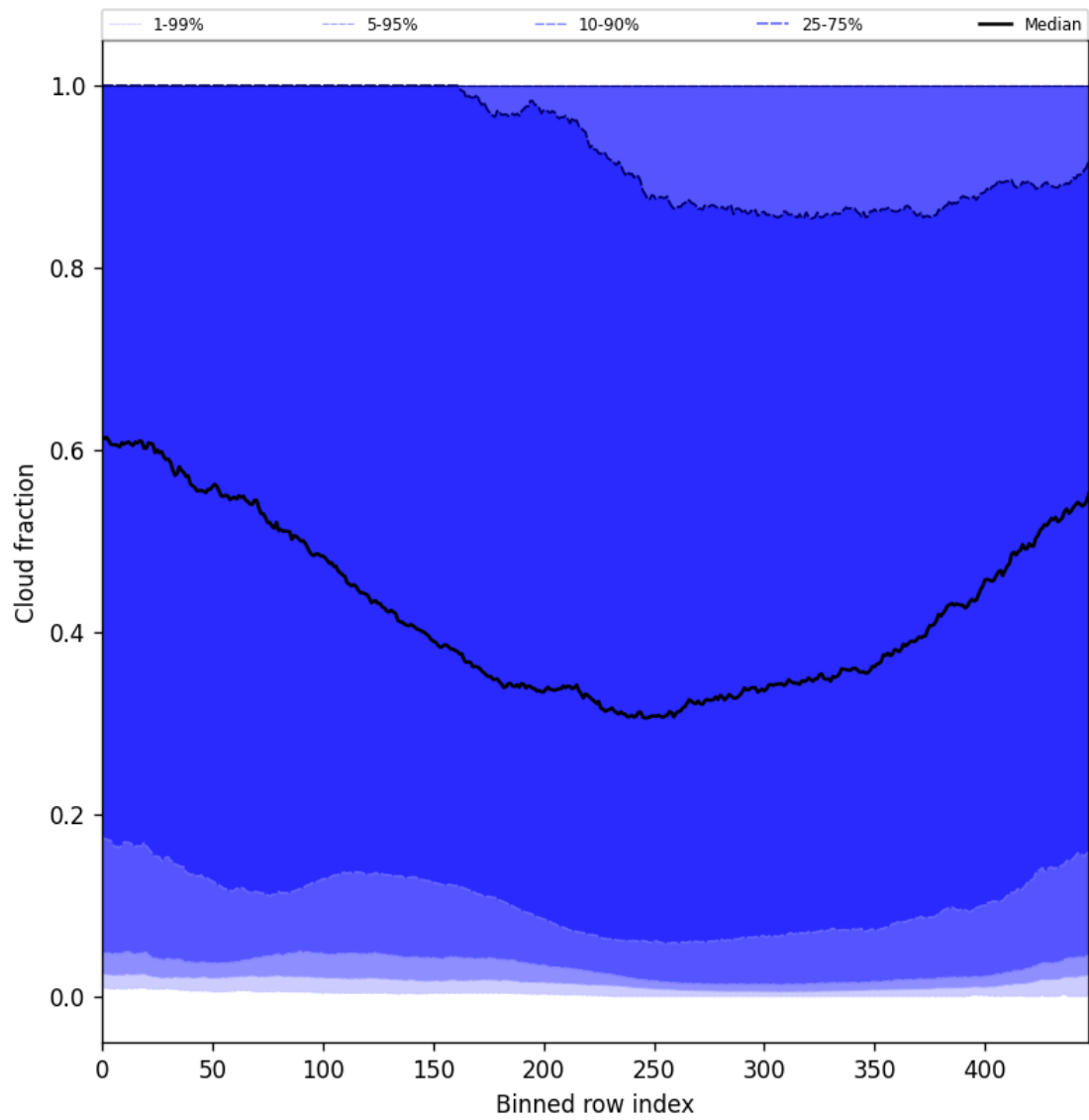
Figure 49: Along track statistics of “Cloud fraction” for 2024-12-19 to 2024-12-21
