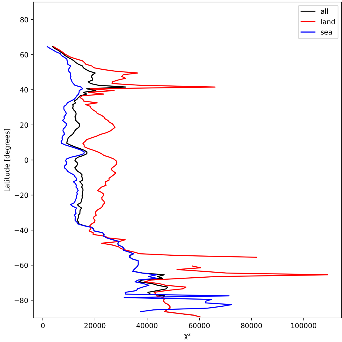
Figure 21: Zonal average of “ \chi^2 ” for 2024-12-19 to 2024-12-21.
