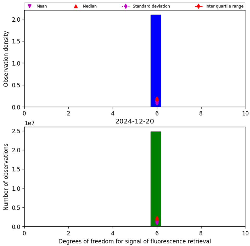
Figure 43: Histogram of "Degrees of freedom for signal of fluorescence retrieval" for 2024-12-19 to 2024-12-21
