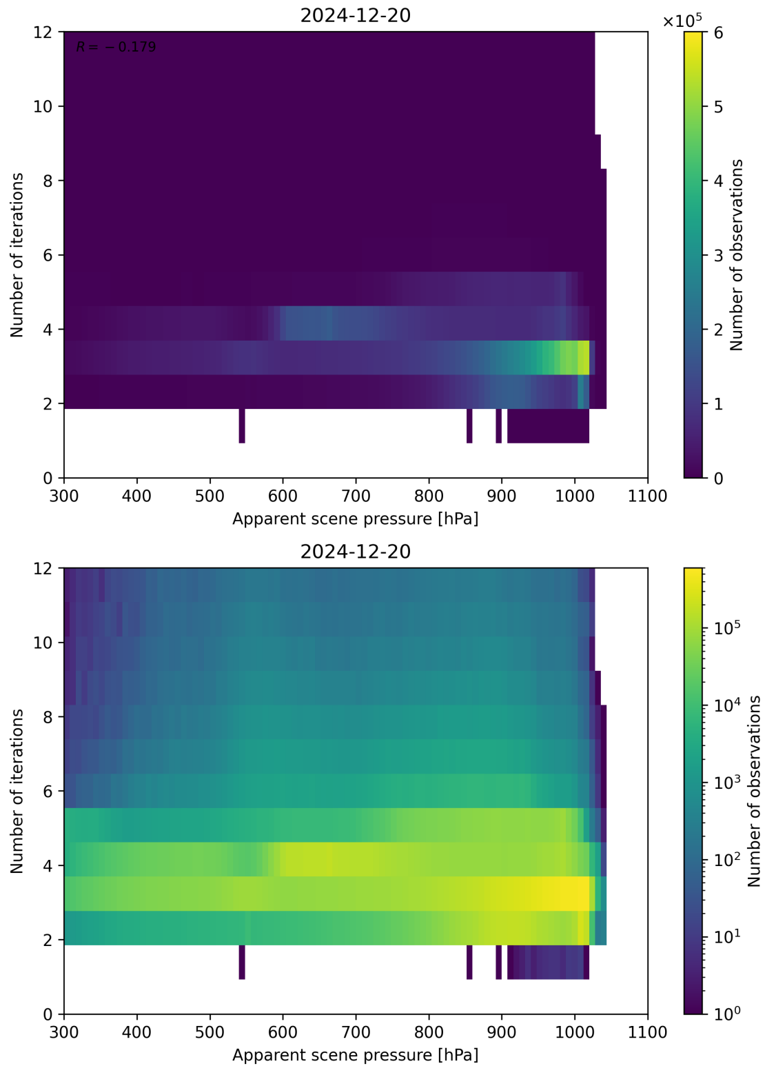
Figure 65: Scatter density plot of “Apparent scene pressure” against “Number of iterations” for 2024-12-19 to 2024-12-21.
