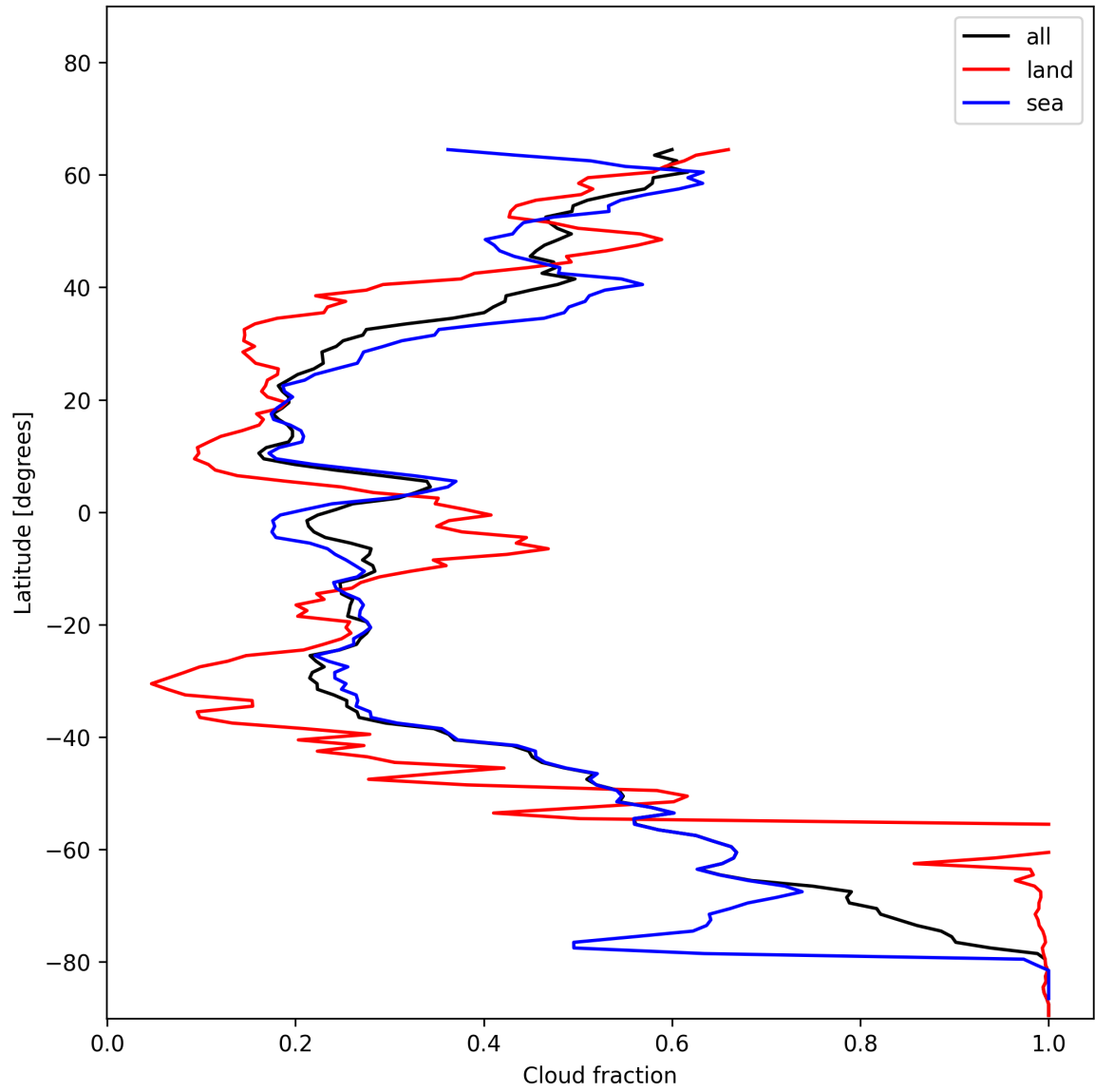
Figure 15: Zonal average of “Cloud fraction” for 2024-12-19 to 2024-12-21.
