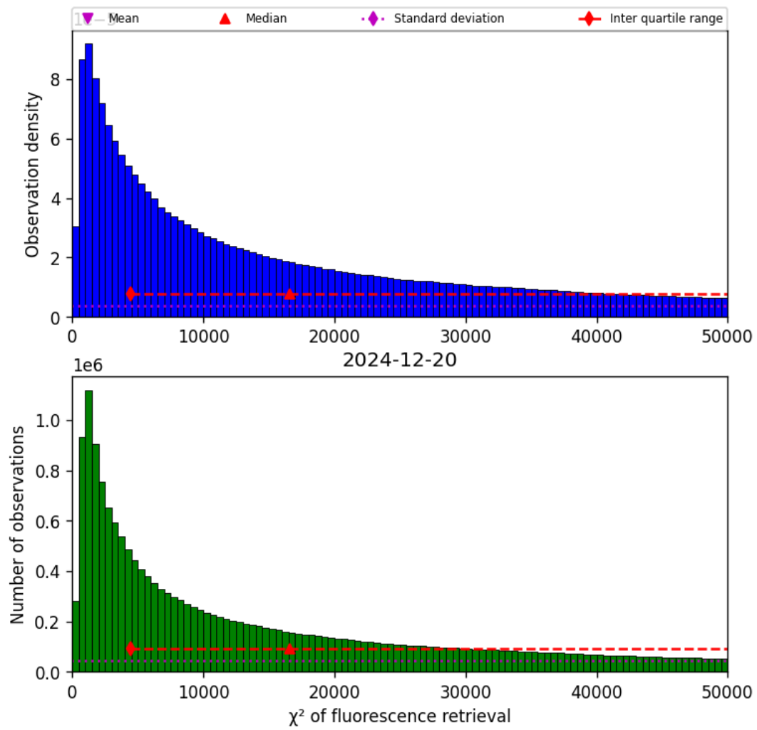
Figure 42: Histogram of “ \chi^2 of fluorescence retrieval” for 2024-12-19 to 2024-12-21
