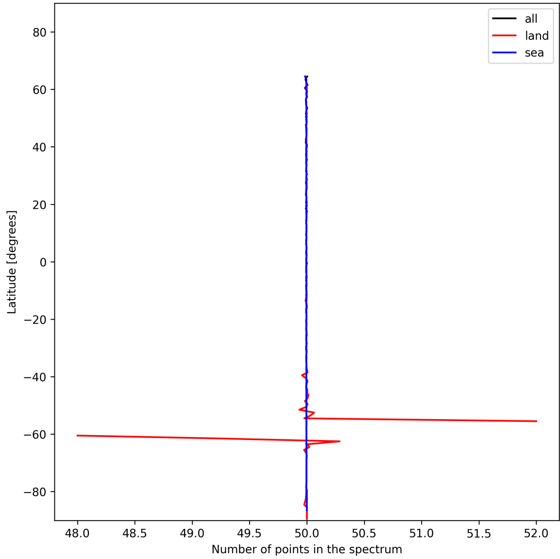
Figure 27: Zonal average of “Number of points in the spectrum” for 2024-12-19 to 2024-12-21.
