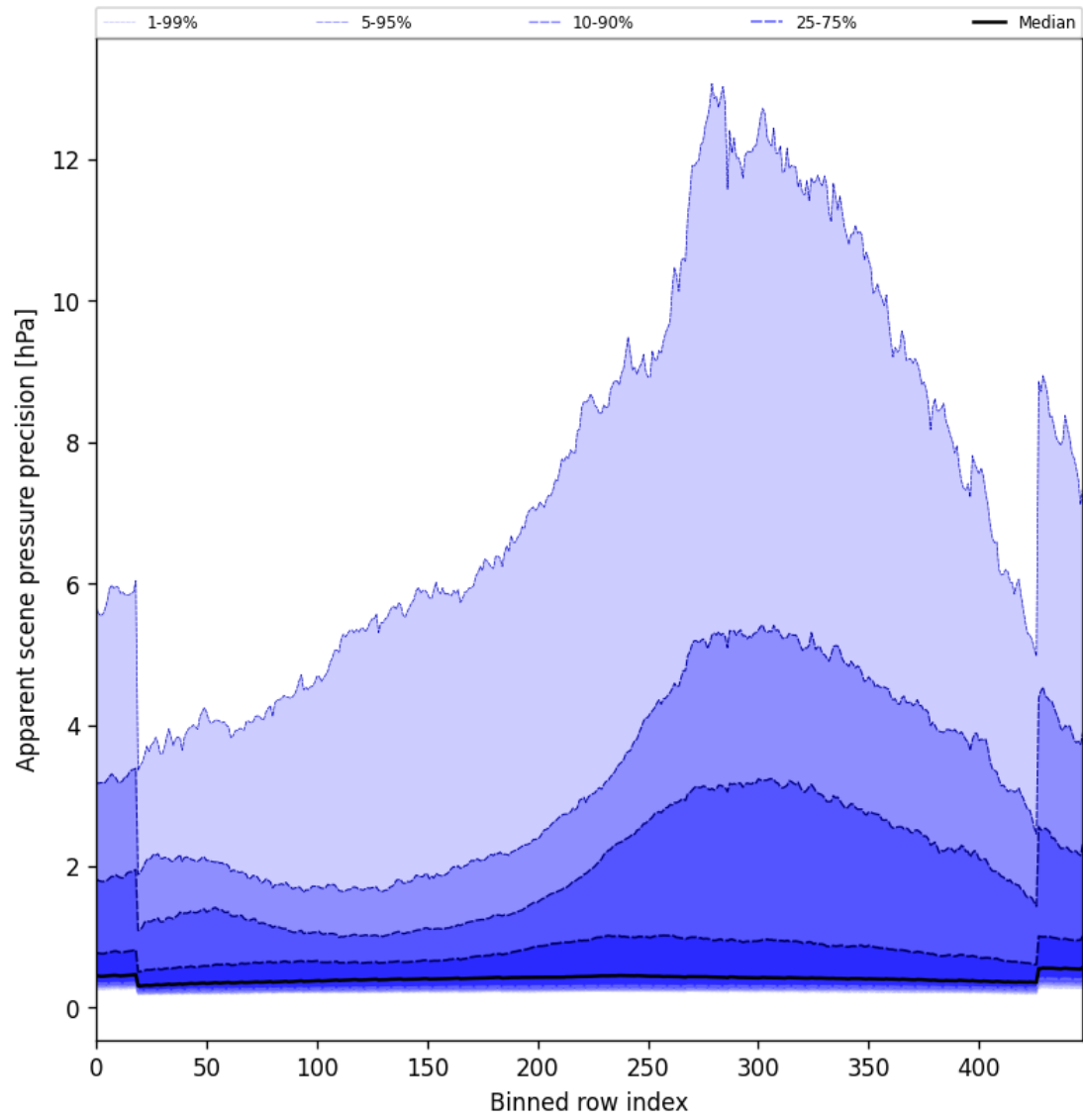
Figure 54: Along track statistics of “Apparent scene pressure precision” for 2024-12-19 to 2024-12-21
