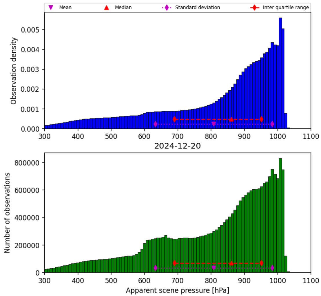
Figure 36: Histogram of “Apparent scene pressure” for 2024-12-19 to 2024-12-21
