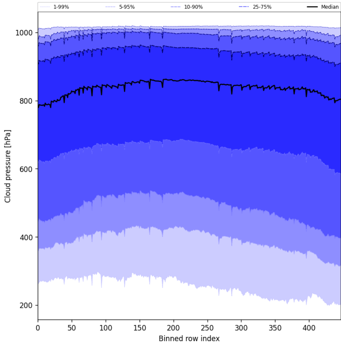
Figure 47: Along track statistics of “Cloud pressure” for 2024-12-19 to 2024-12-21
