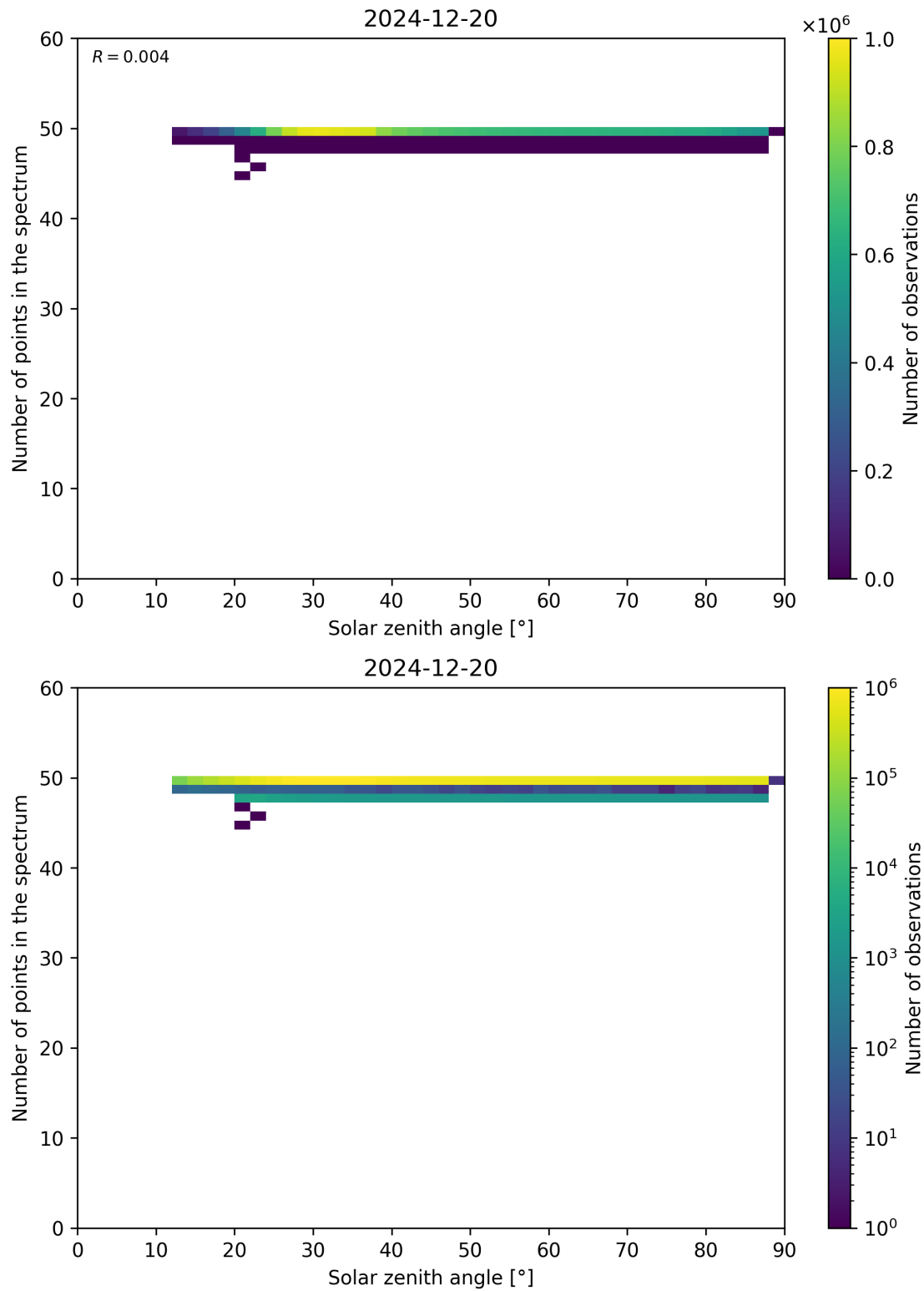
Figure 115: Scatter density plot of “Solar zenith angle” against “Number of points in the spectrum” for 2024-12-19 to 2024-12-21.
