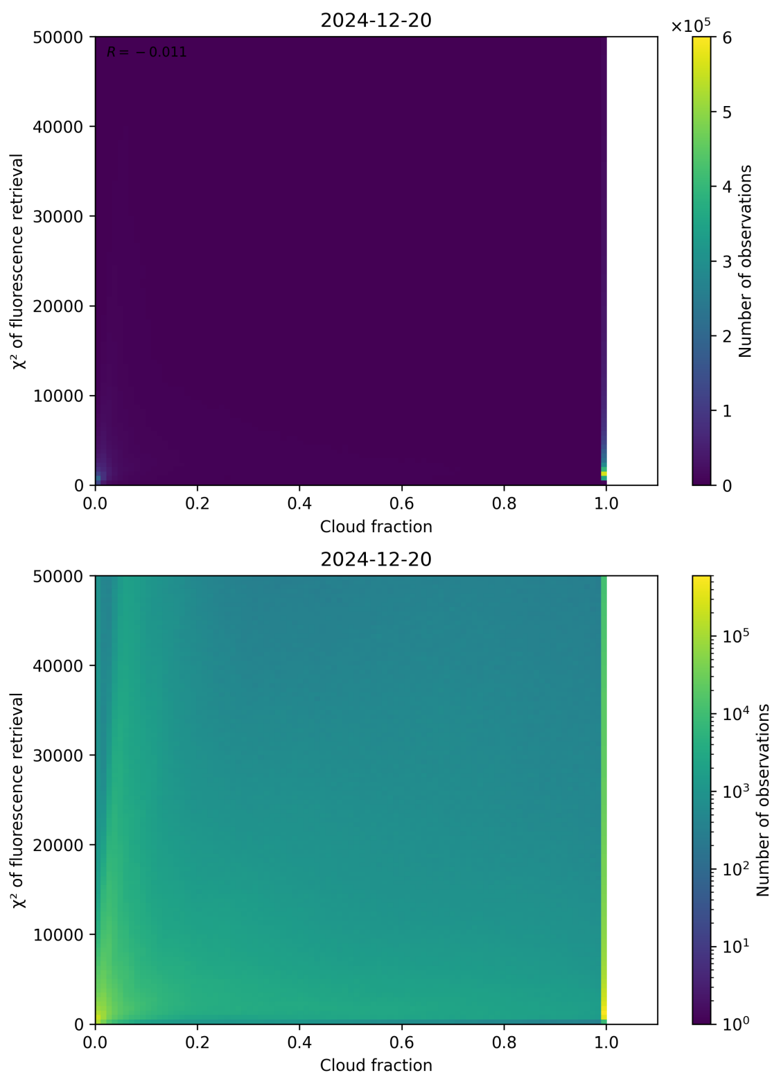
Figure 71: Scatter density plot of “Cloud fraction” against “ \chi^2 of fluorescence retrieval” for 2024-12-19 to 2024-12-21.
