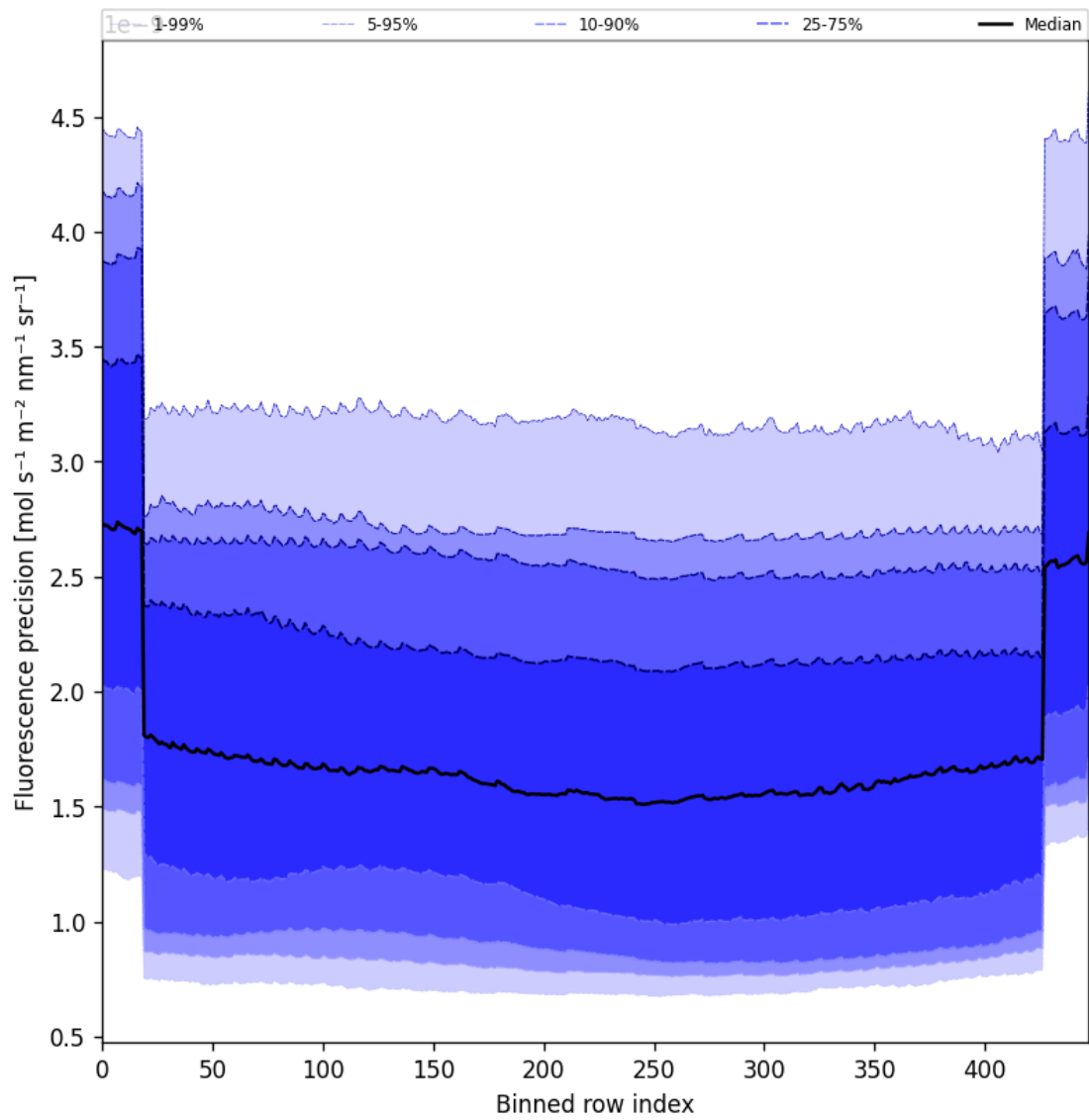
Figure 58: Along track statistics of “Fluorescence precision” for 2024-12-19 to 2024-12-21
