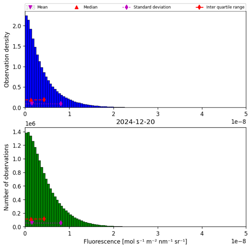
Figure 40: Histogram of “Fluorescence” for 2024-12-19 to 2024-12-21
