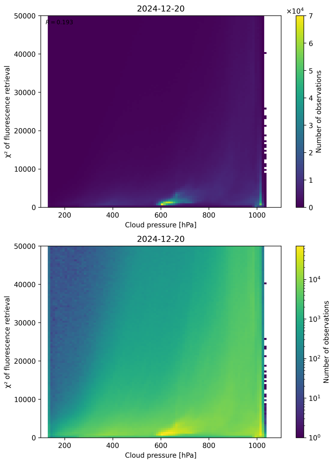
Figure 78: Scatter density plot of “Cloud pressure” against “ \chi^2 of fluorescence retrieval” for 2024-12-19 to 2024-12-21.
