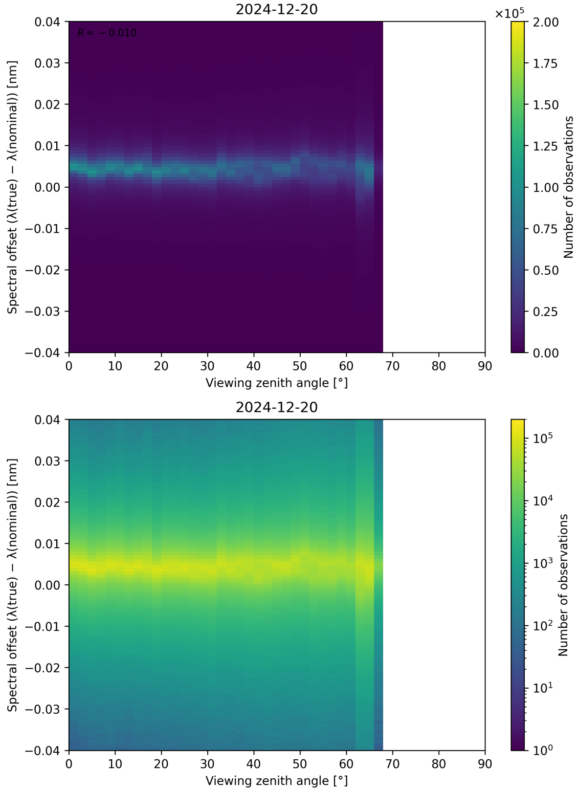
Figure 128: Scatter density plot of “Viewing zenith angle” against “Spectral offset ( \lambda_{\text{true}} - \lambda_{\text{nominal}} )” for 2024-12-19 to 2024-12-21.
