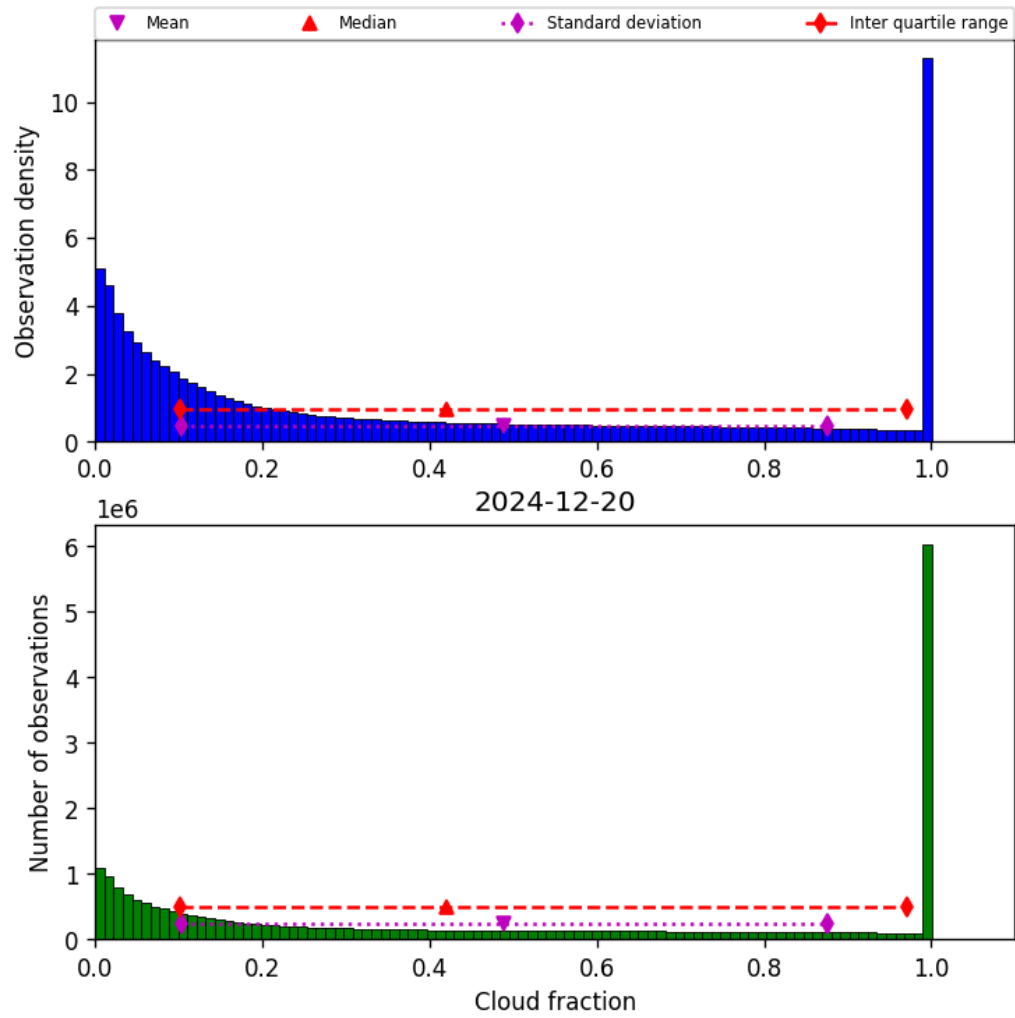
Figure 32: Histogram of “Cloud fraction” for 2024-12-19 to 2024-12-21
