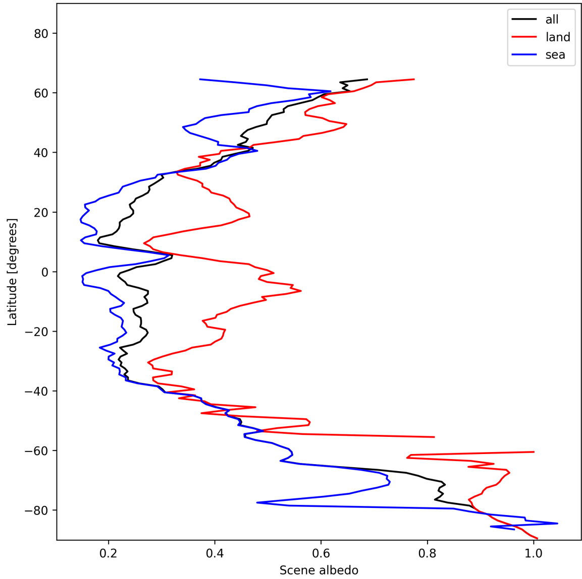
Figure 17: Zonal average of “Scene albedo” for 2024-12-19 to 2024-12-21.
