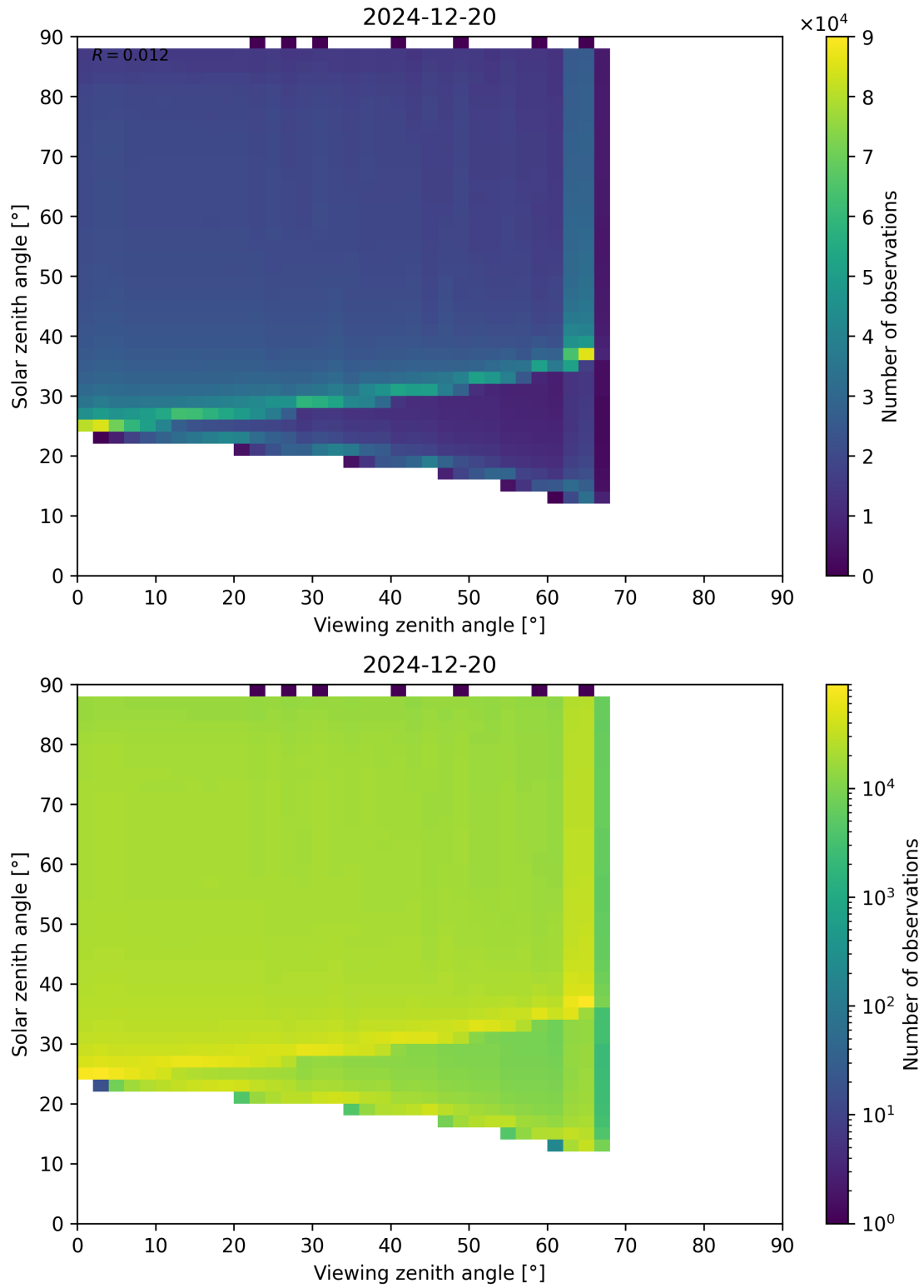
Figure 127: Scatter density plot of “Viewing zenith angle” against “Solar zenith angle” for 2024-12-19 to 2024-12-21.
