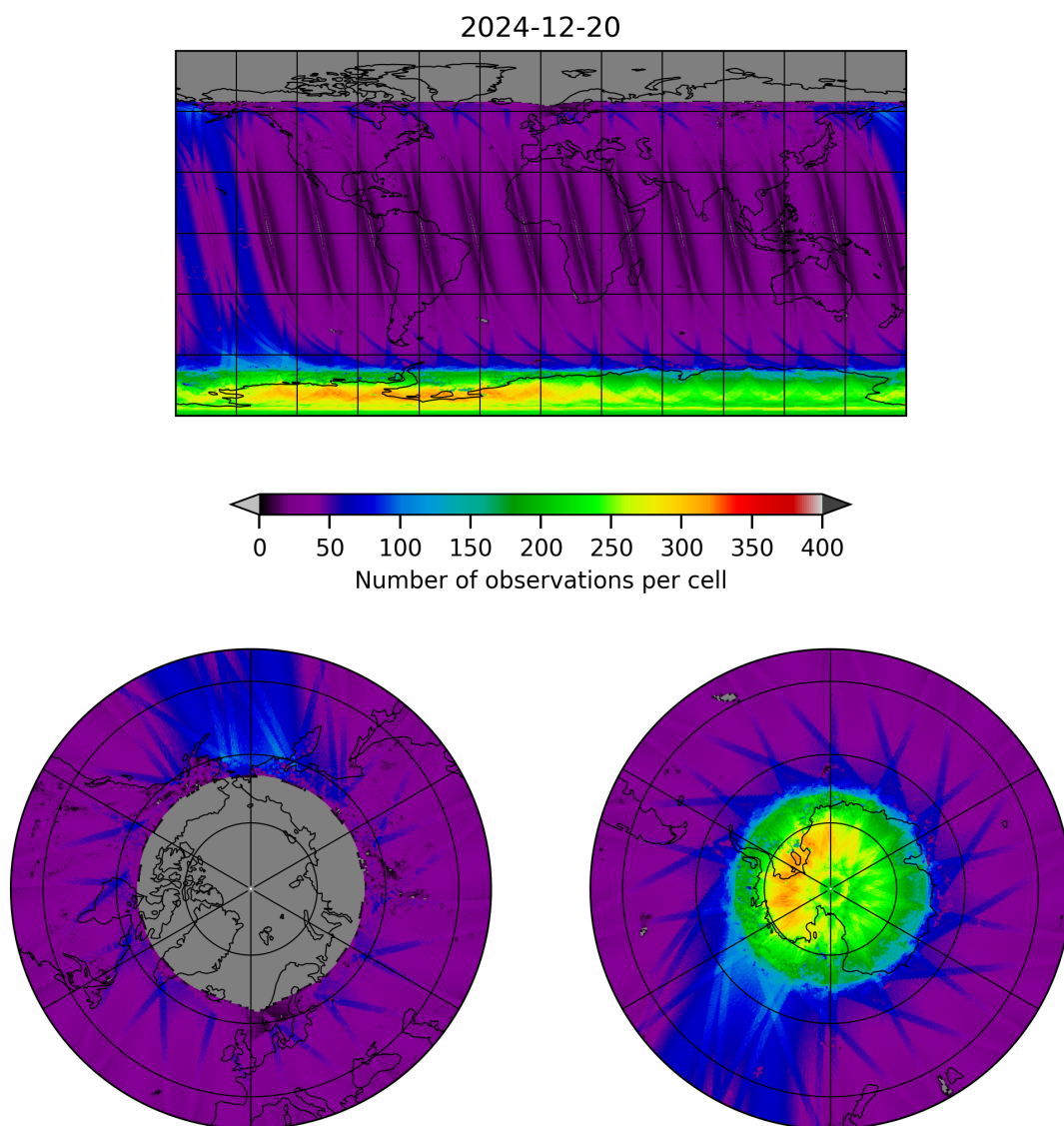
Figure 11: Map of the number of observations for 2024-12-19 to 2024-12-21
