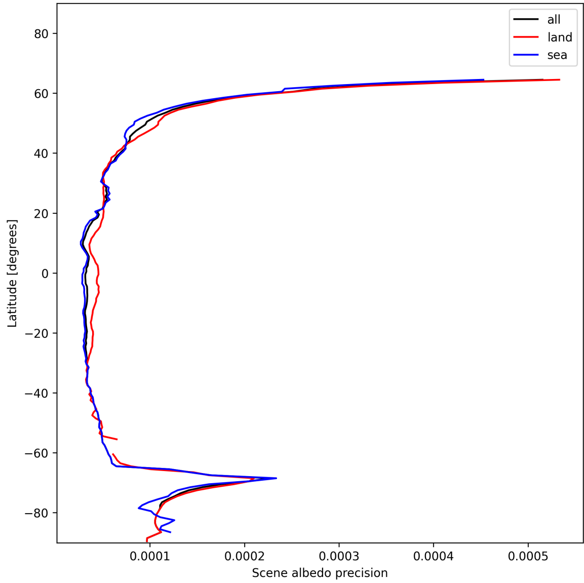
Figure 18: Zonal average of “Scene albedo precision” for 2024-12-19 to 2024-12-21.
