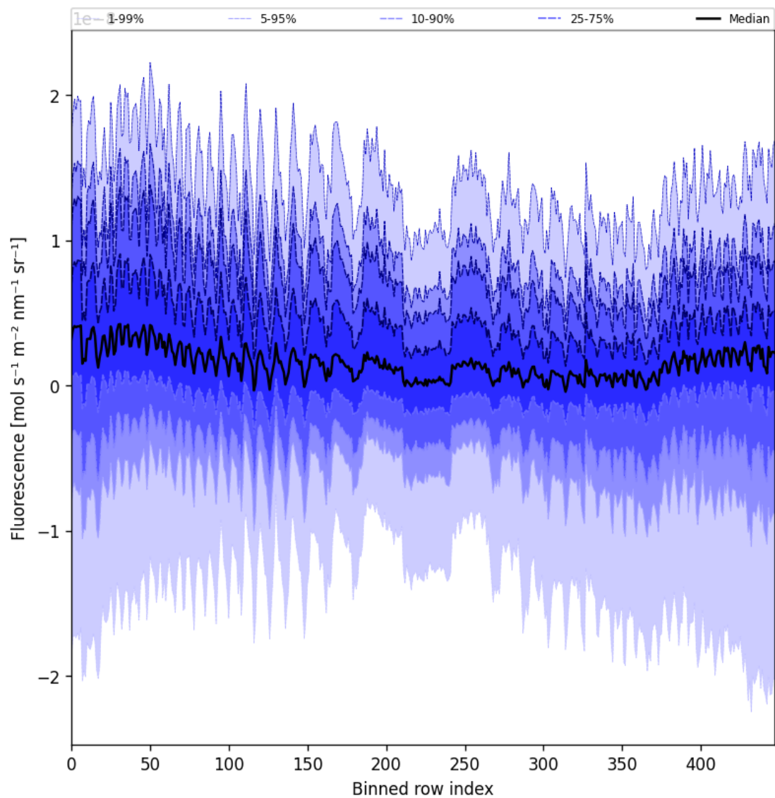
Figure 57: Along track statistics of “Fluorescence” for 2024-12-19 to 2024-12-21
