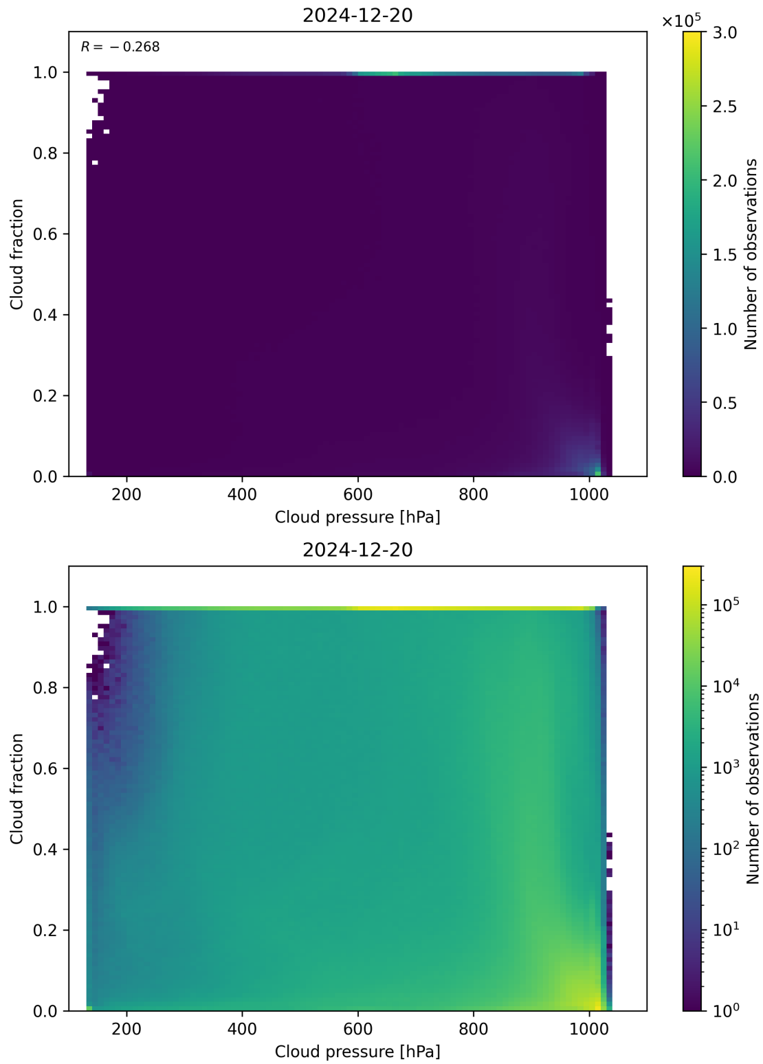
Figure 79: Scatter density plot of “Cloud pressure” against “Cloud fraction” for 2024-12-19 to 2024-12-21.
