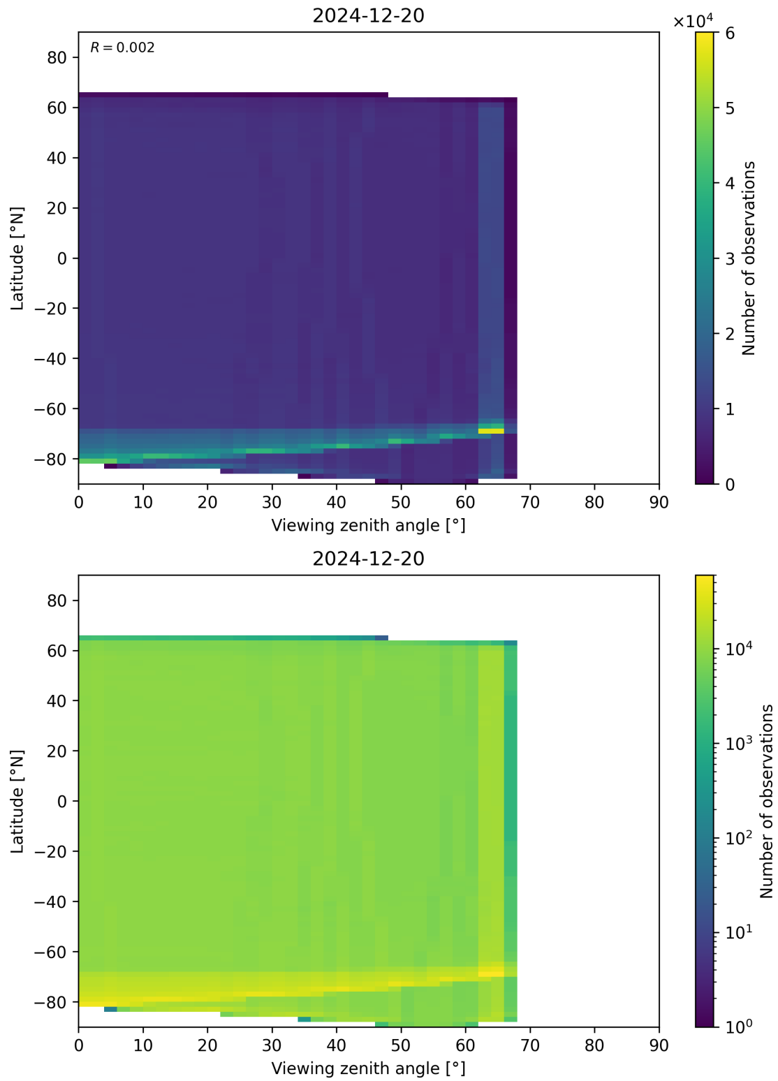
Figure 123: Scatter density plot of “Viewing zenith angle” against “Latitude” for 2024-12-19 to 2024-12-21.
