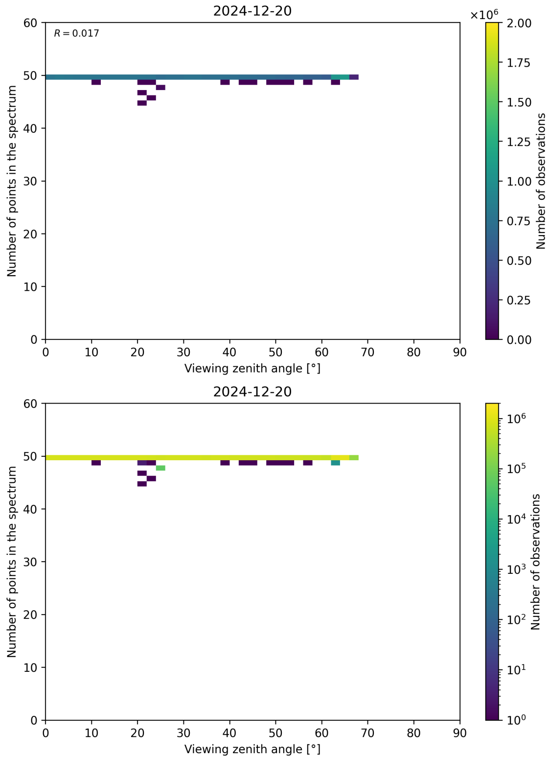
Figure 125: Scatter density plot of “Viewing zenith angle” against “Number of points in the spectrum” for 2024-12-19 to 2024-12-21.
