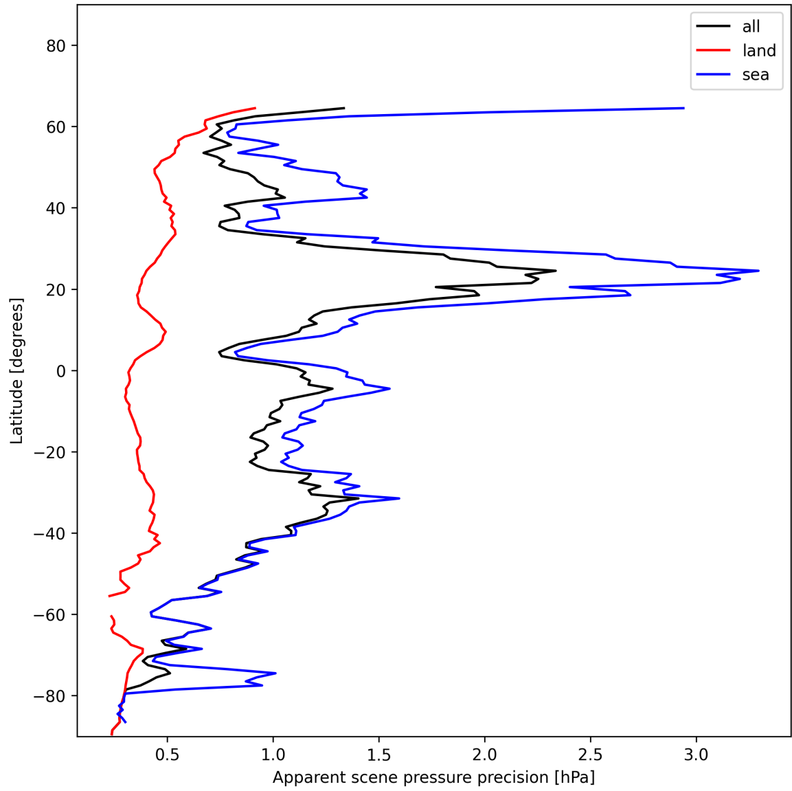
Figure 20: Zonal average of “Apparent scene pressure precision” for 2024-12-19 to 2024-12-21.
