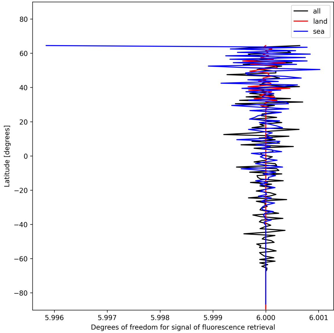
Figure 26: Zonal average of “Degrees of freedom for signal of fluorescence retrieval” for 2024-12-19 to 2024-12-21.
