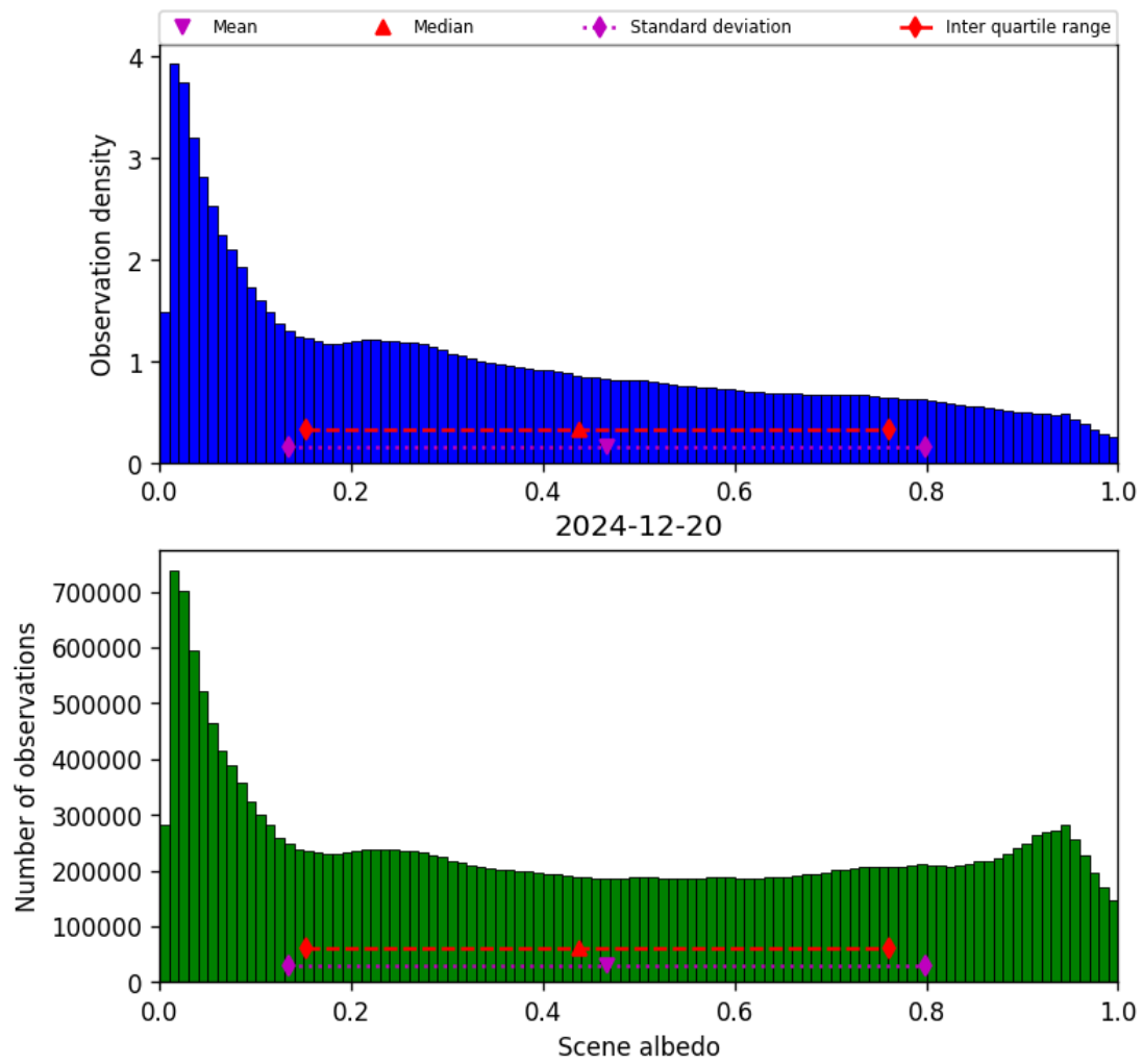
Figure 34: Histogram of “Scene albedo” for 2024-12-19 to 2024-12-21
