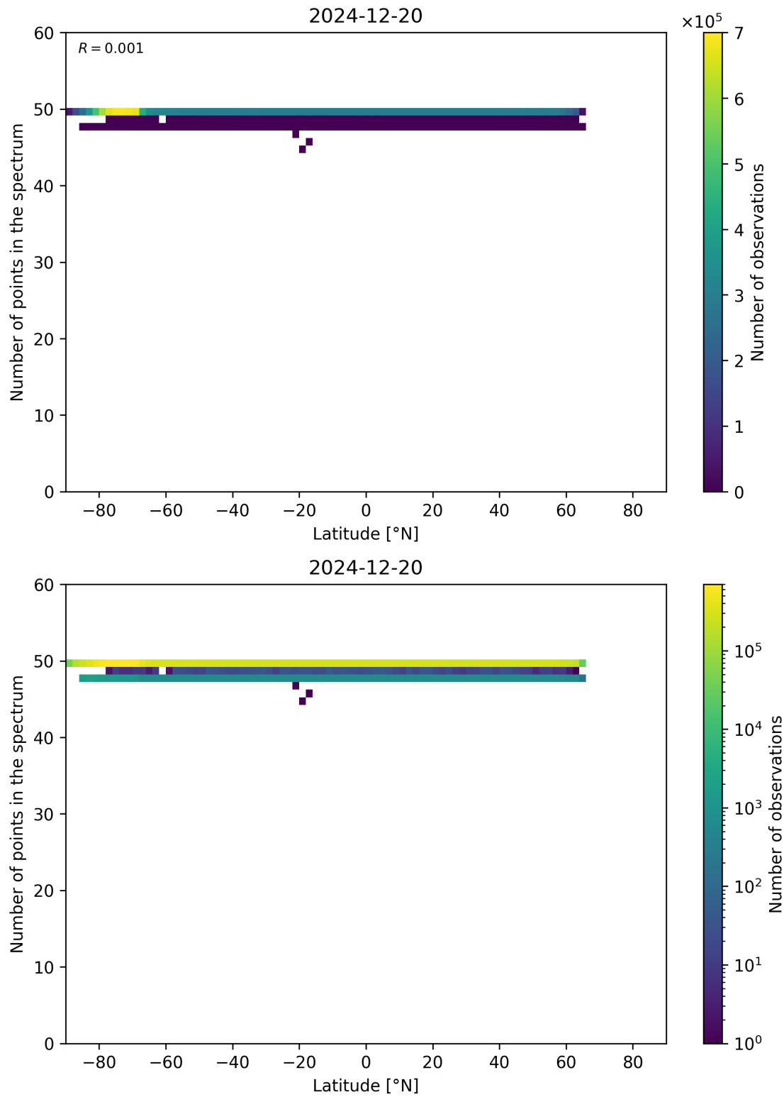
Figure 94: Scatter density plot of “Latitude” against “Number of points in the spectrum” for 2024-12-19 to 2024-12-21.
