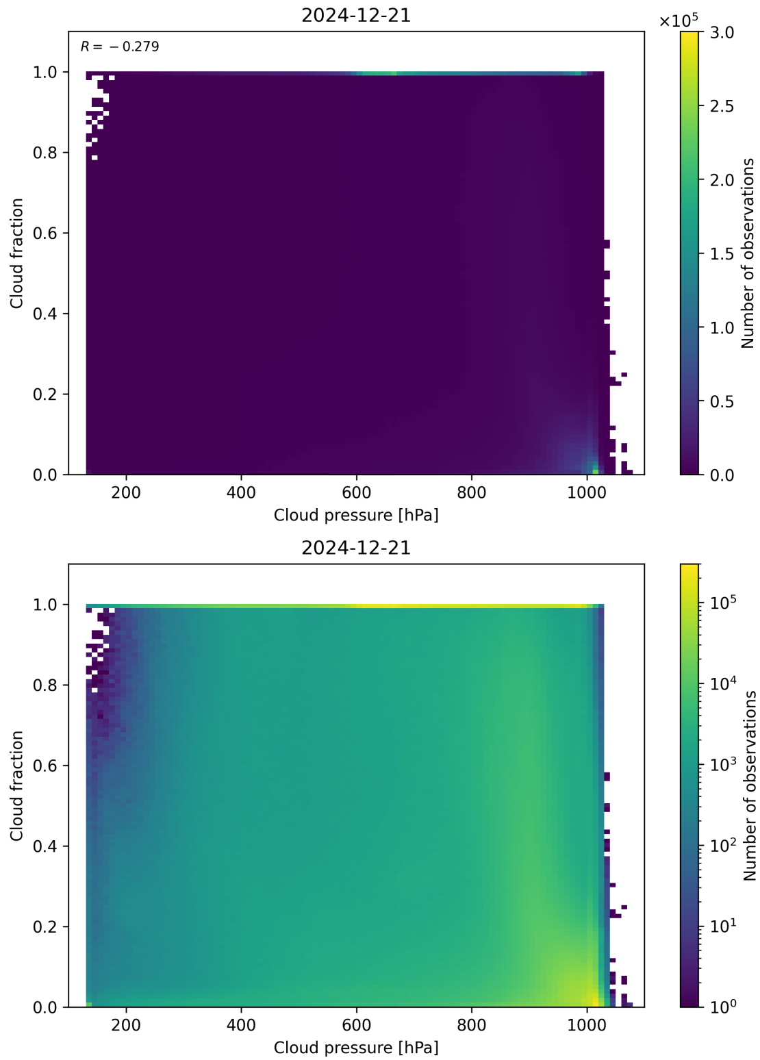
Figure 79: Scatter density plot of “Cloud pressure” against “Cloud fraction” for 2024-12-20 to 2024-12-22.
