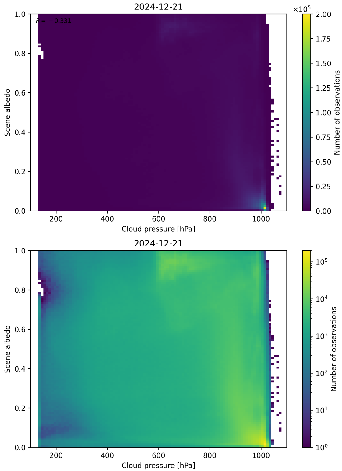
Figure 83: Scatter density plot of “Cloud pressure” against “Scene albedo” for 2024-12-20 to 2024-12-22.
