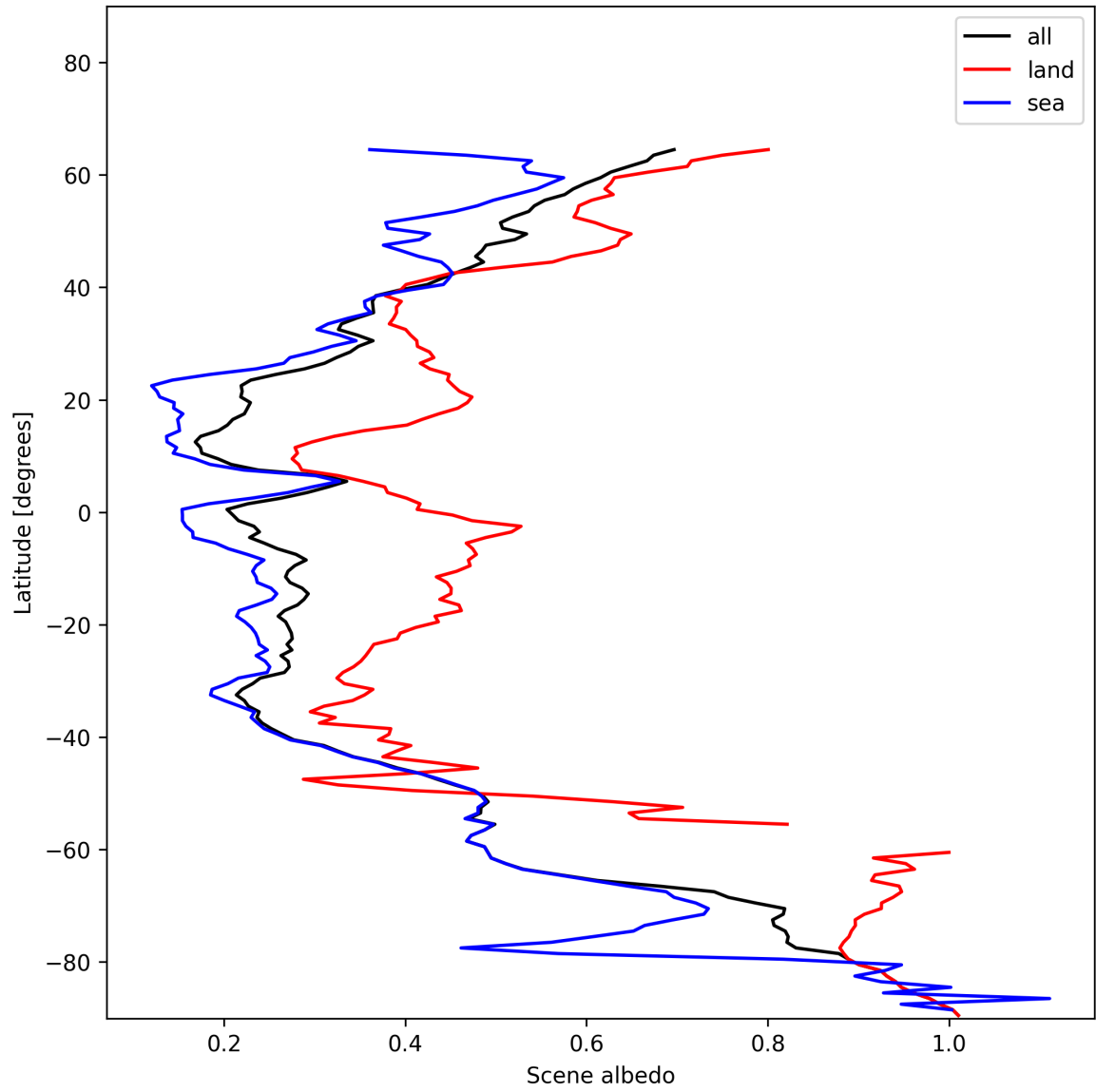
Figure 17: Zonal average of “Scene albedo” for 2024-12-20 to 2024-12-22.
