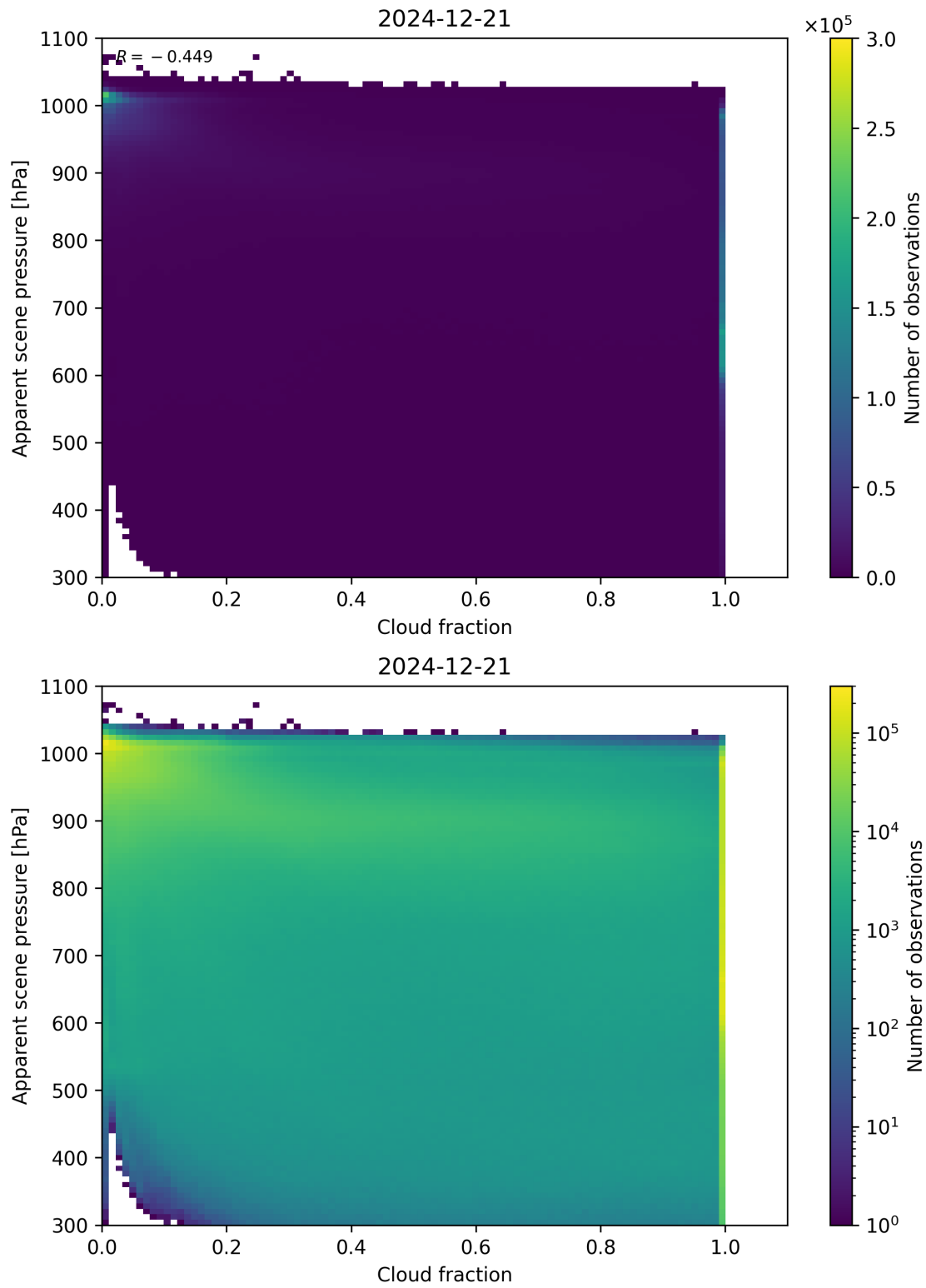
Figure 70: Scatter density plot of “Cloud fraction” against “Apparent scene pressure” for 2024-12-20 to 2024-12-22.
