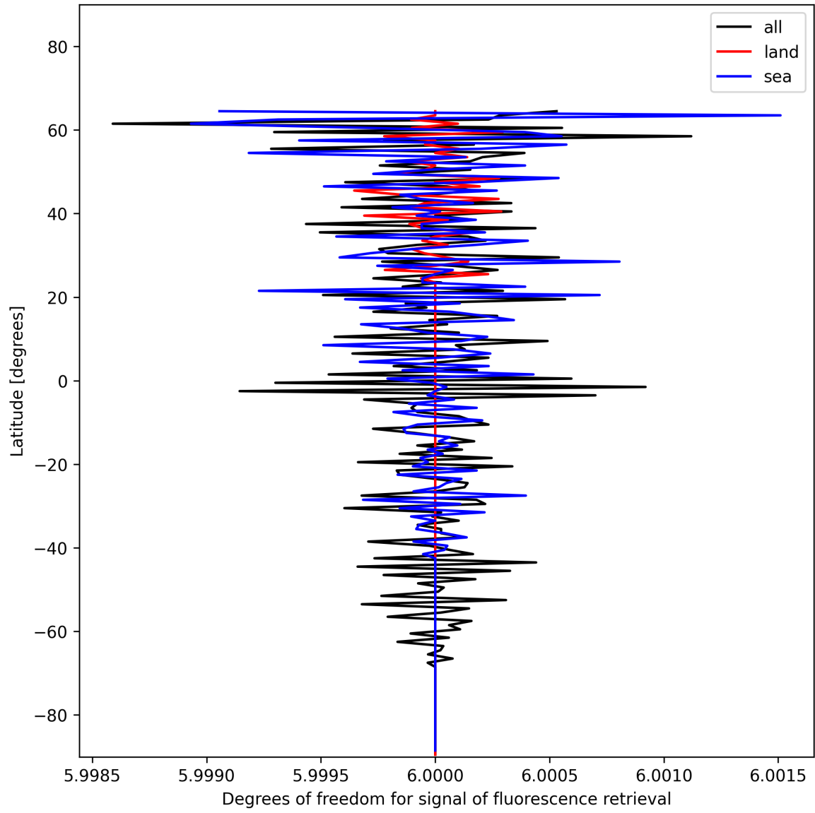
Figure 26: Zonal average of “Degrees of freedom for signal of fluorescence retrieval” for 2024-12-20 to 2024-12-22.
