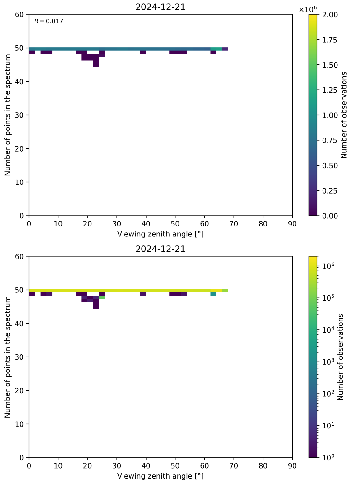
Figure 125: Scatter density plot of “Viewing zenith angle” against “Number of points in the spectrum” for 2024-12-20 to 2024-12-22.
