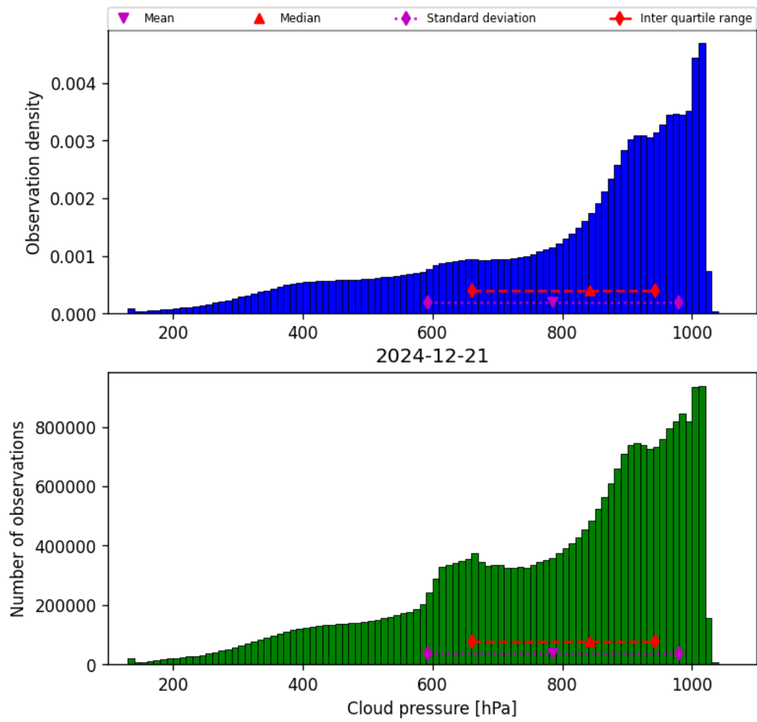
Figure 30: Histogram of “Cloud pressure” for 2024-12-20 to 2024-12-22
