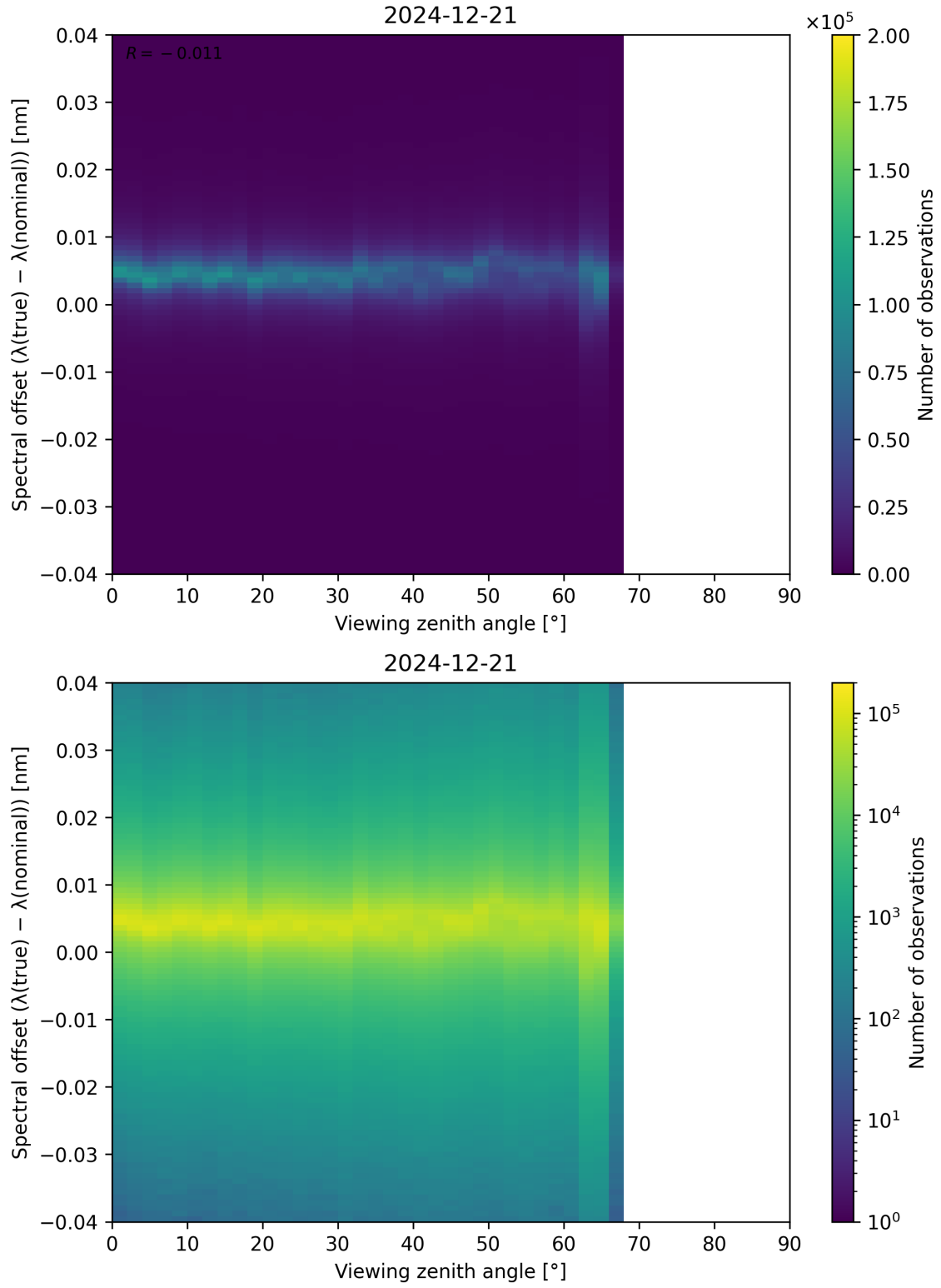
Figure 128: Scatter density plot of “Viewing zenith angle” against “Spectral offset ( \lambda_{\text{true}} - \lambda_{\text{nominal}} )” for 2024-12-20 to 2024-12-22.
