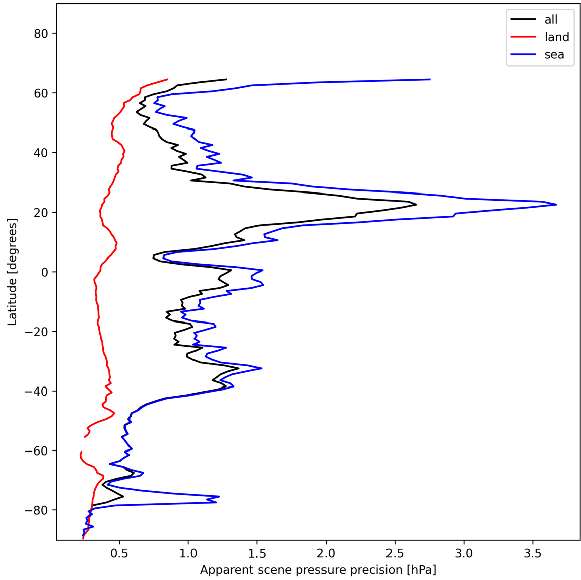
Figure 20: Zonal average of “Apparent scene pressure precision” for 2024-12-20 to 2024-12-22.
