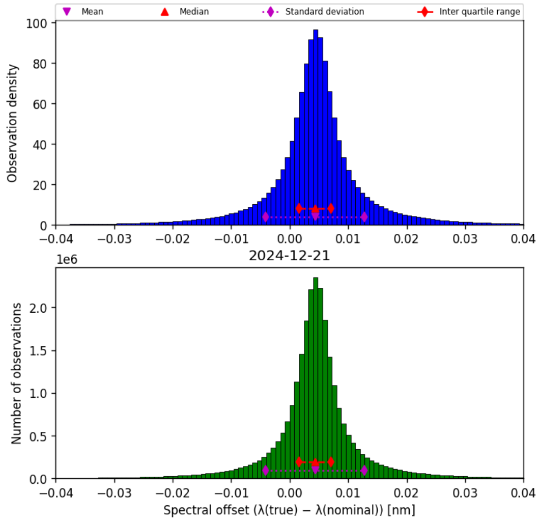
Figure 45: Histogram of “Spectral offset ( \lambda_{\text{true}} - \lambda_{\text{nominal}} )” for 2024-12-20 to 2024-12-22
