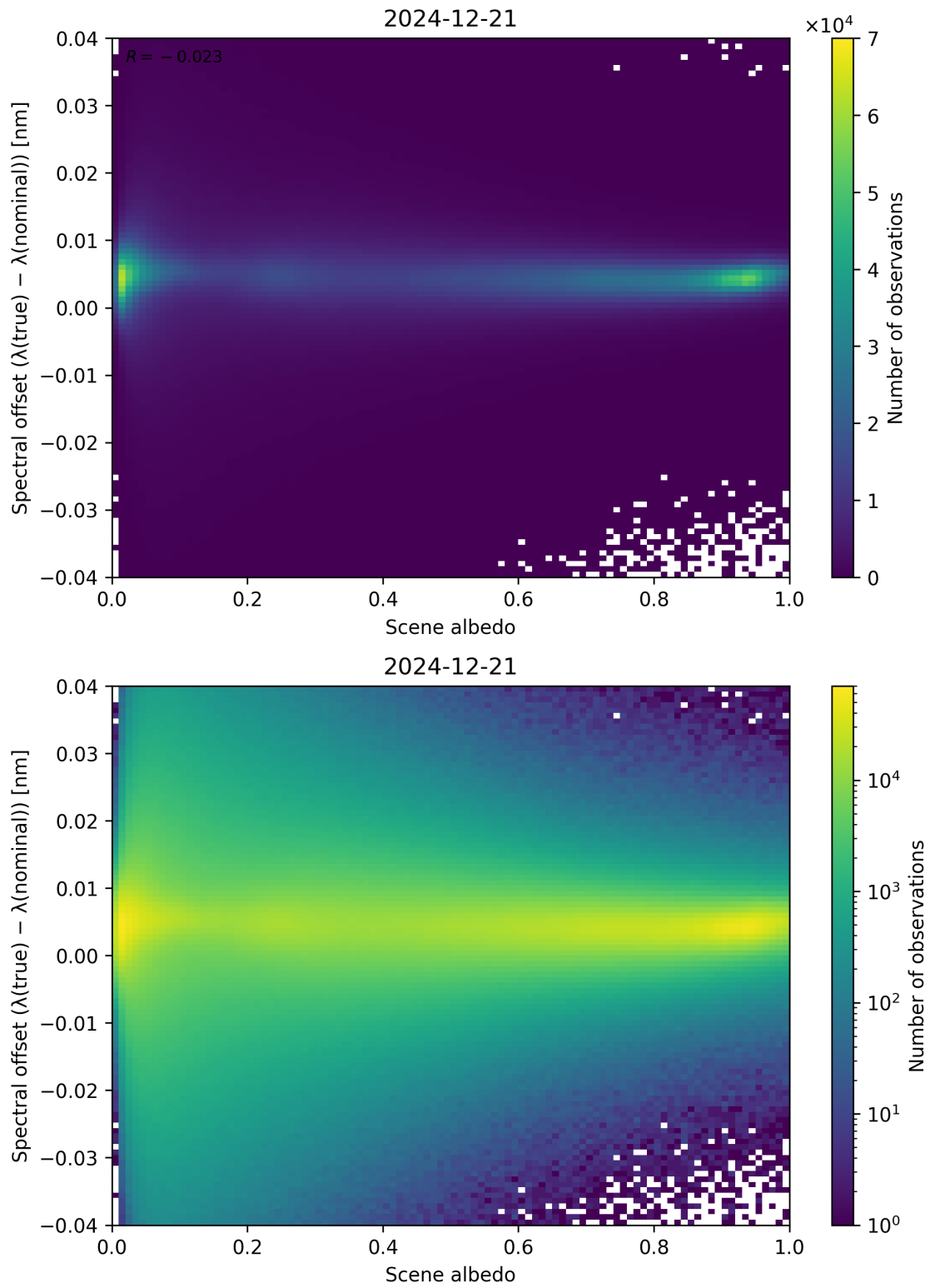
Figure 107: Scatter density plot of “Scene albedo” against “Spectral offset ( \lambda_{\text{true}} - \lambda_{\text{nominal}} )” for 2024-12-20 to 2024-12-22.
