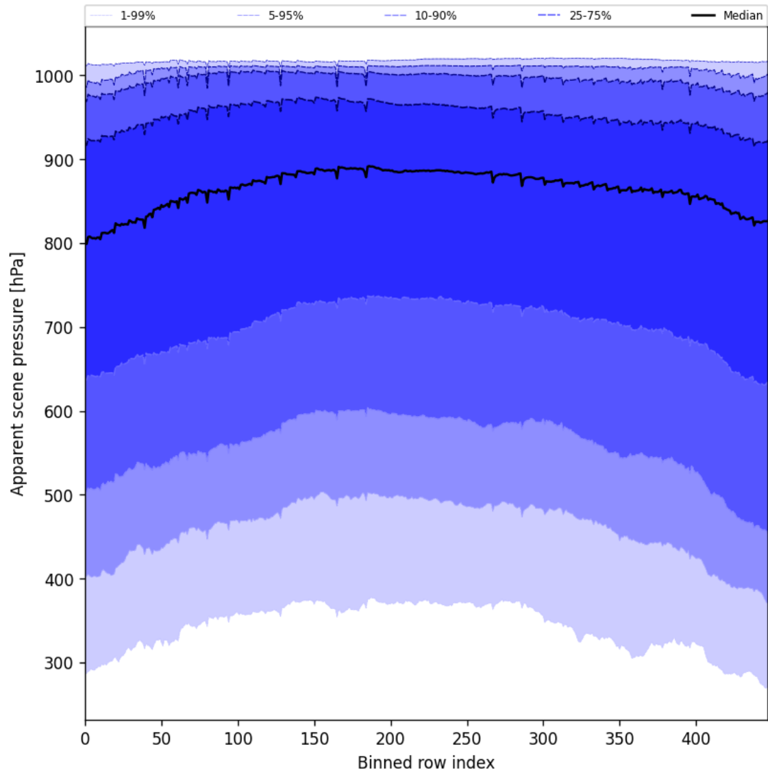
Figure 53: Along track statistics of “Apparent scene pressure” for 2024-12-20 to 2024-12-22
