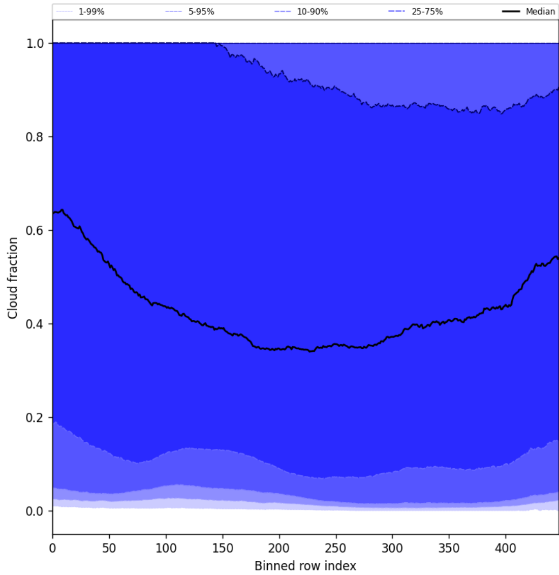
Figure 49: Along track statistics of “Cloud fraction” for 2024-12-20 to 2024-12-22
