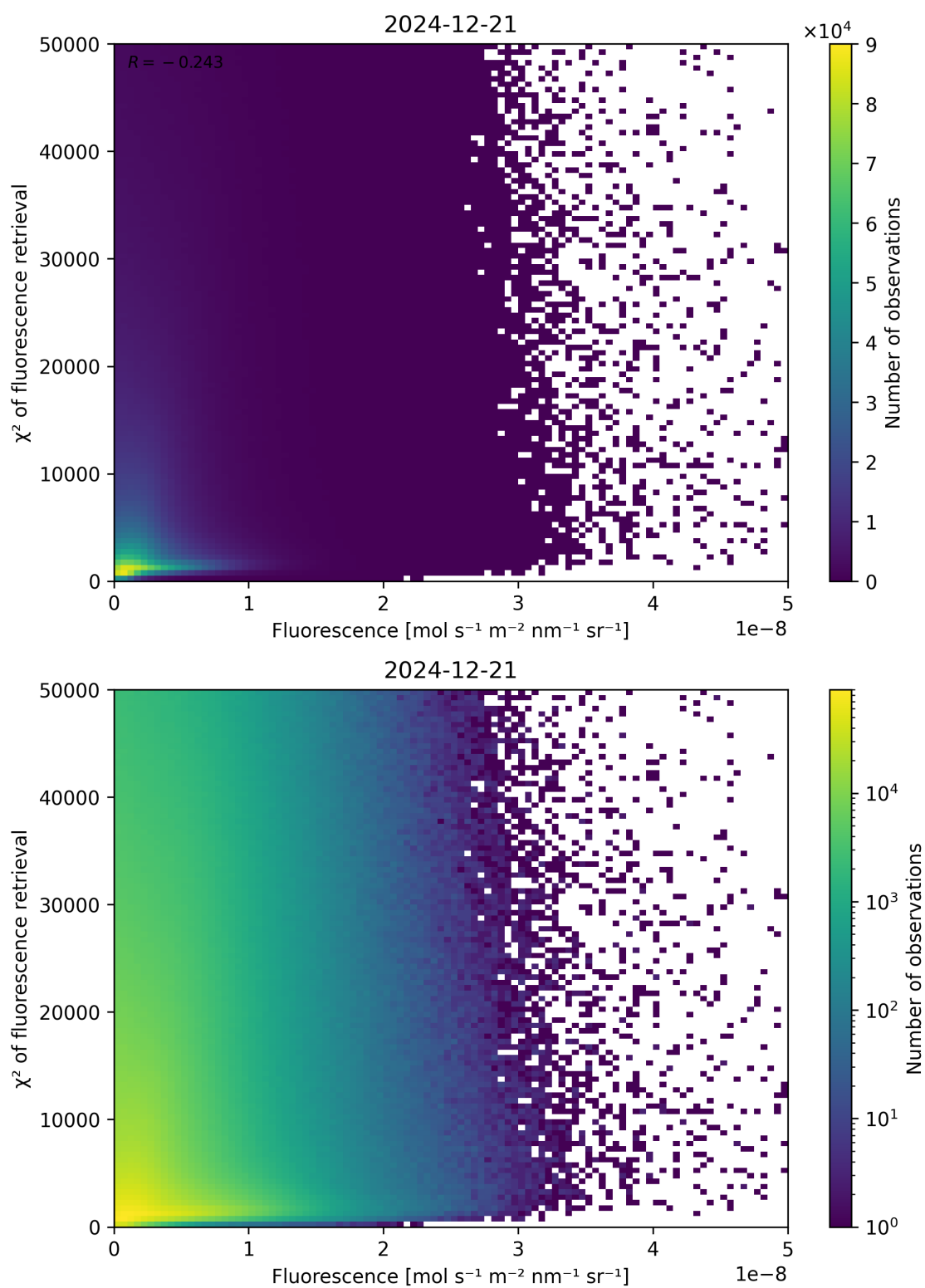
Figure 85: Scatter density plot of “Fluorescence” against “ \chi^2 of fluorescence retrieval” for 2024-12-20 to 2024-12-22.
