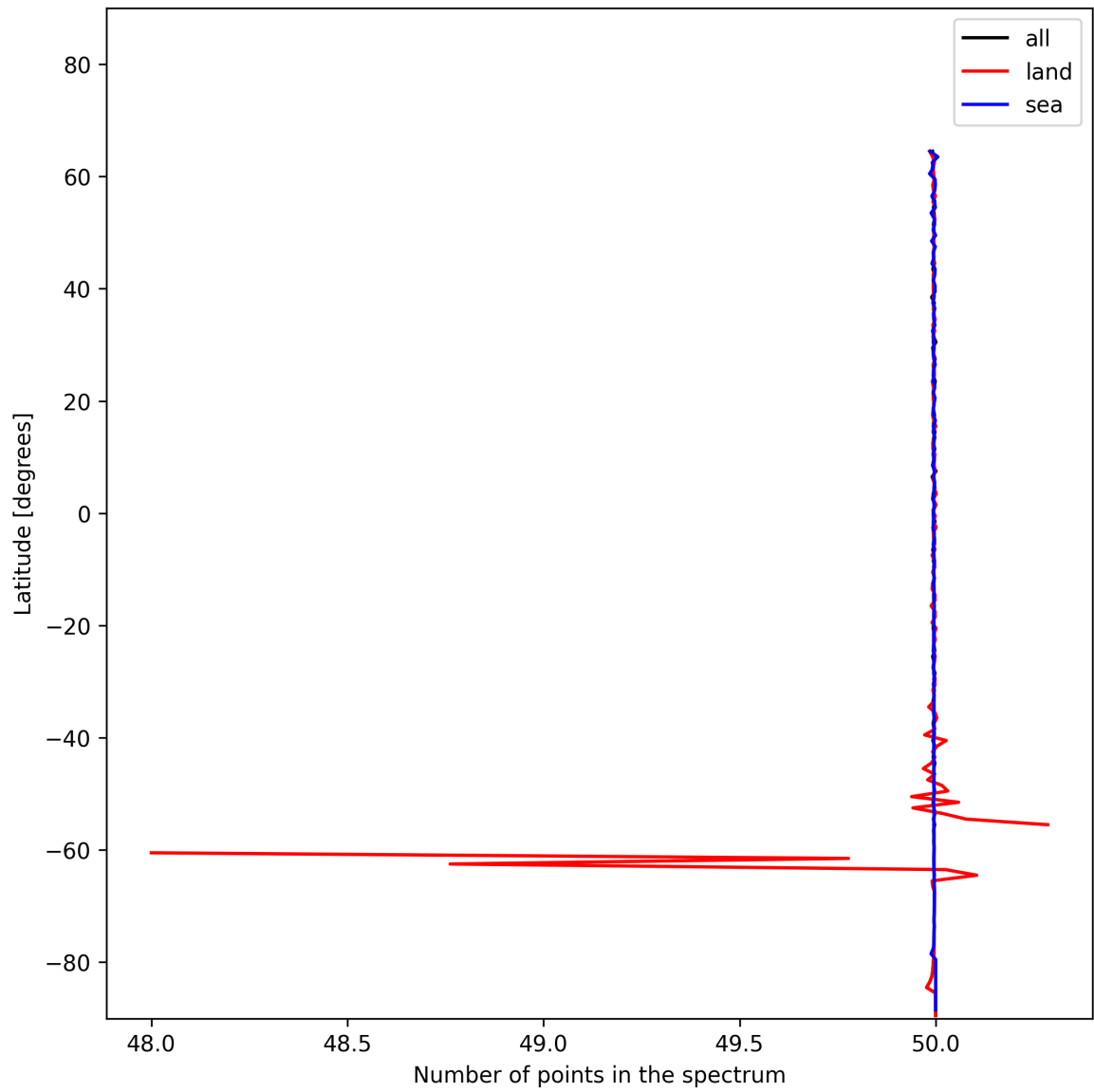
Figure 27: Zonal average of “Number of points in the spectrum” for 2024-12-20 to 2024-12-22.
