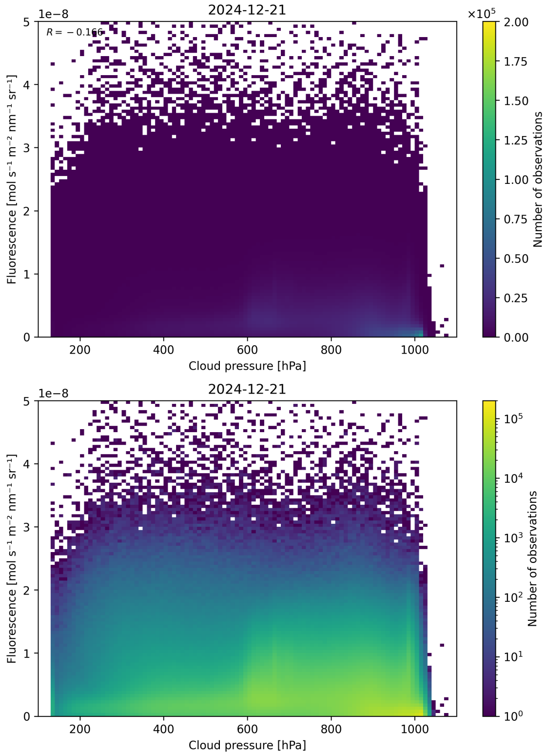
Figure 80: Scatter density plot of “Cloud pressure” against “Fluorescence” for 2024-12-20 to 2024-12-22.
