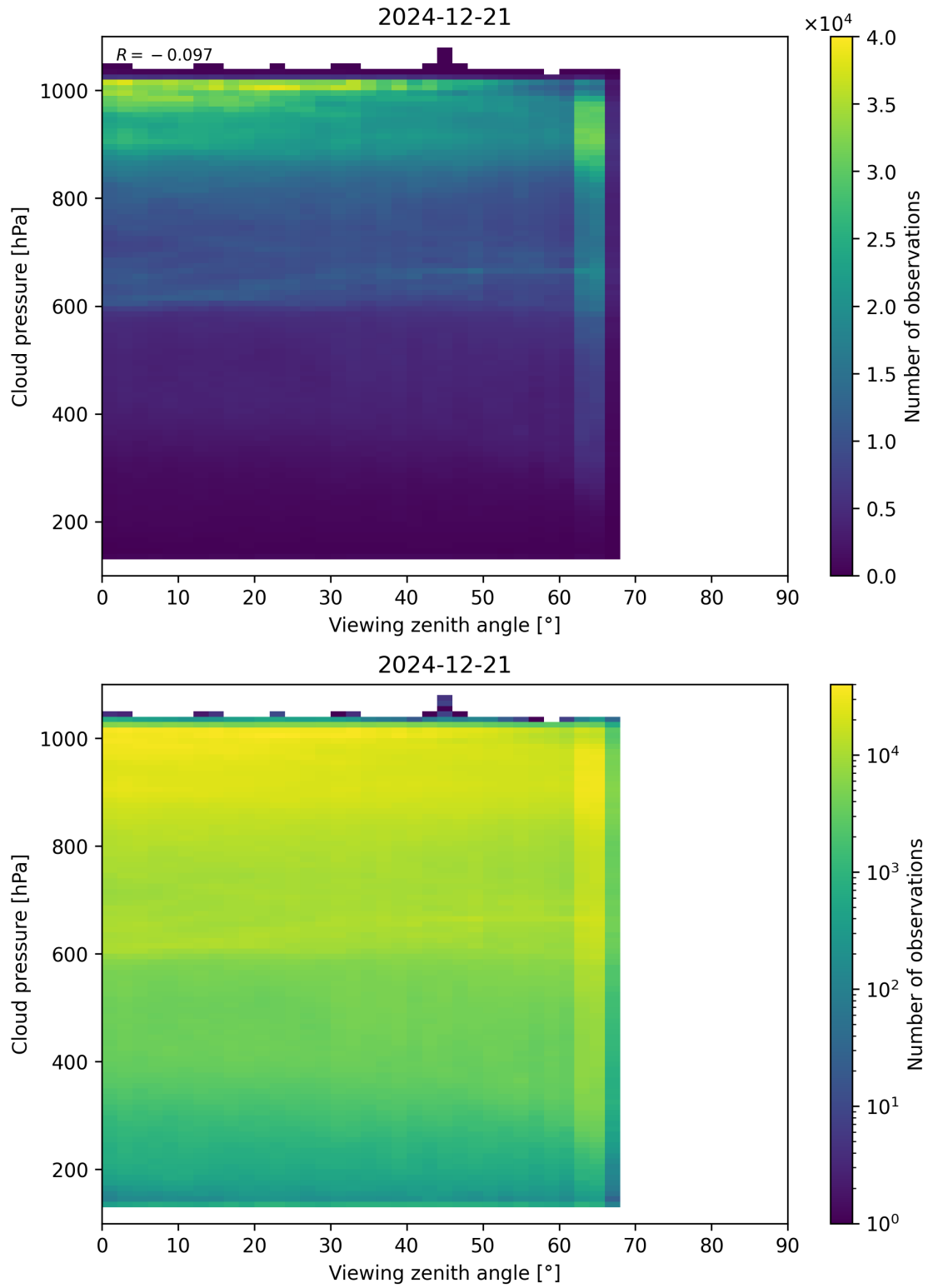
Figure 121: Scatter density plot of “Viewing zenith angle” against “Cloud pressure” for 2024-12-20 to 2024-12-22.
