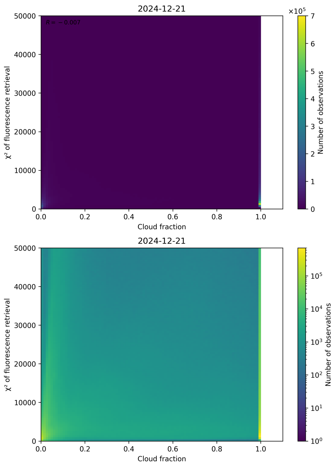
Figure 71: Scatter density plot of “Cloud fraction” against “ \chi^2 of fluorescence retrieval” for 2024-12-20 to 2024-12-22.
