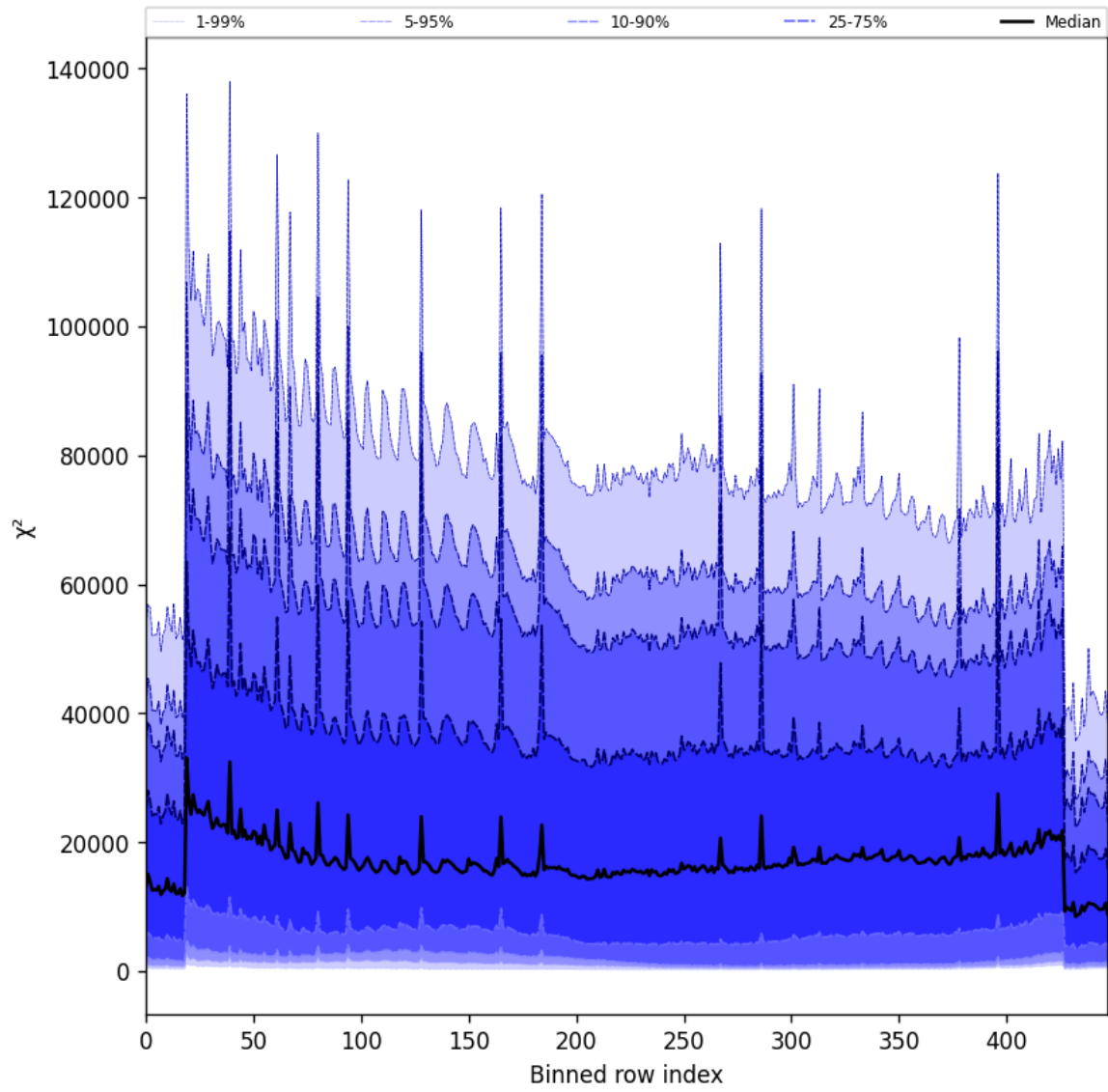
Figure 55: Along track statistics of “ \chi^2 ” for 2024-12-20 to 2024-12-22
