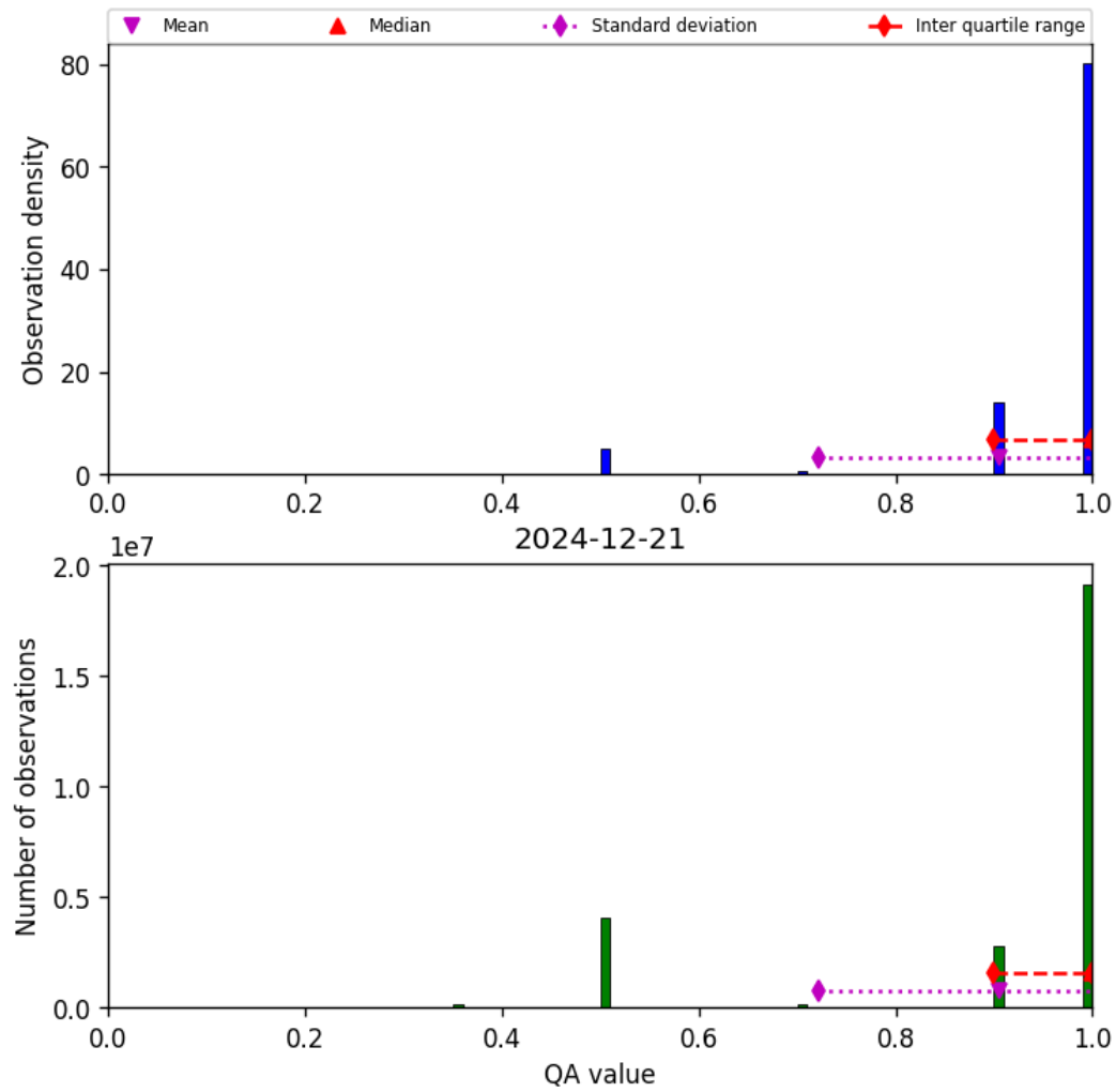
Figure 29: Histogram of “QA value” for 2024-12-20 to 2024-12-22
