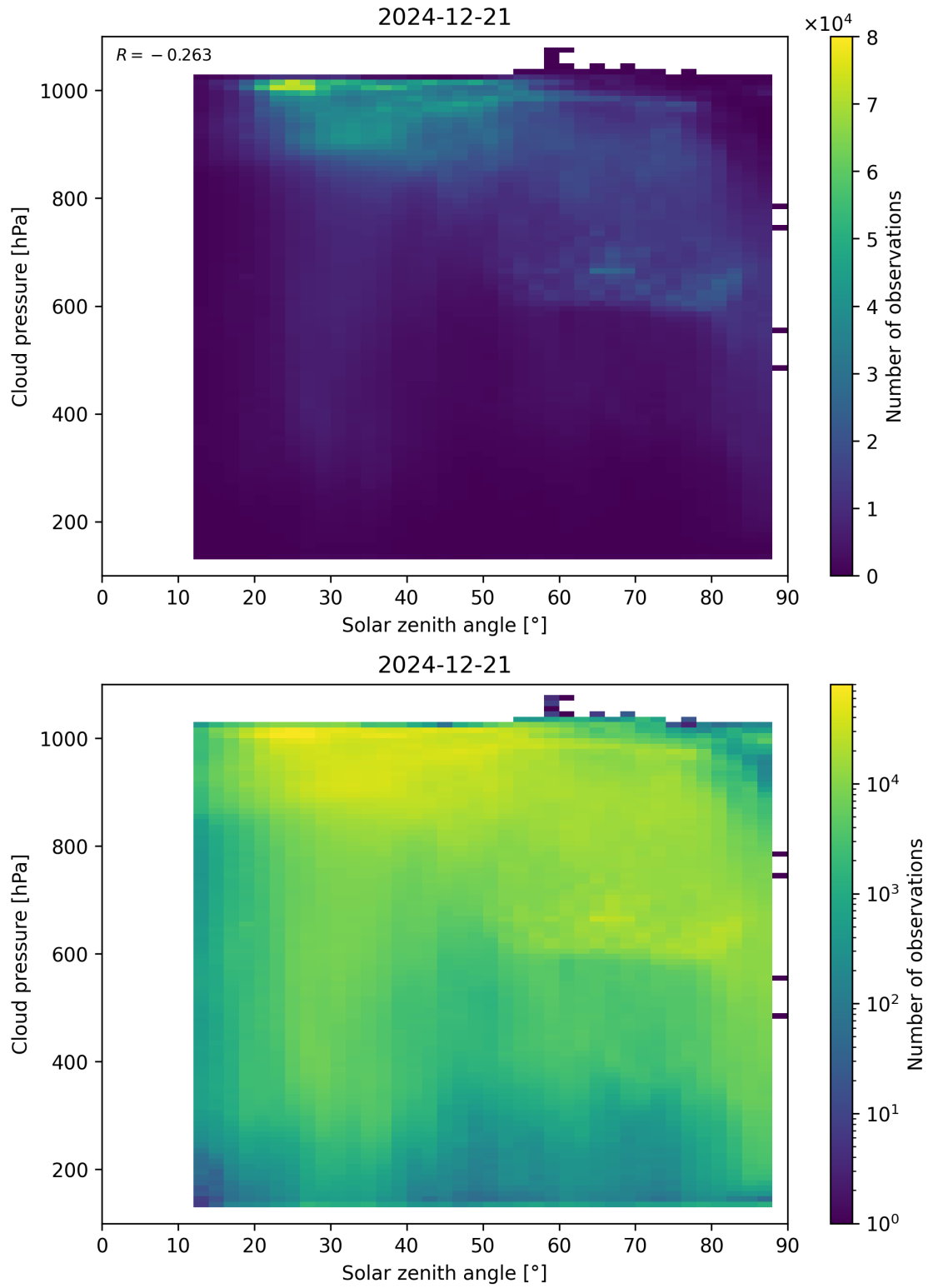
Figure 111: Scatter density plot of “Solar zenith angle” against “Cloud pressure” for 2024-12-20 to 2024-12-22.
