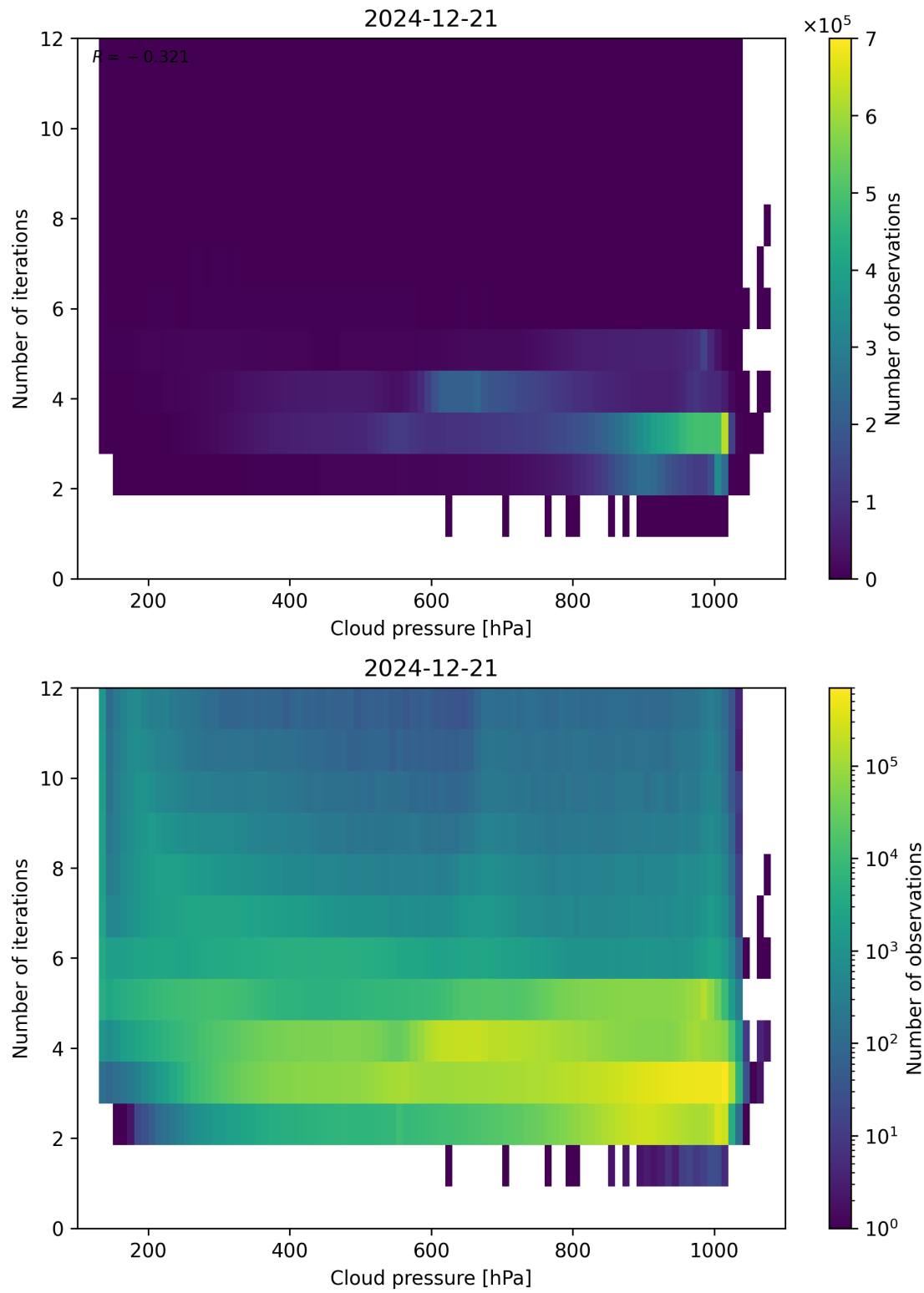
Figure 81: Scatter density plot of “Cloud pressure” against “Number of iterations” for 2024-12-20 to 2024-12-22.
