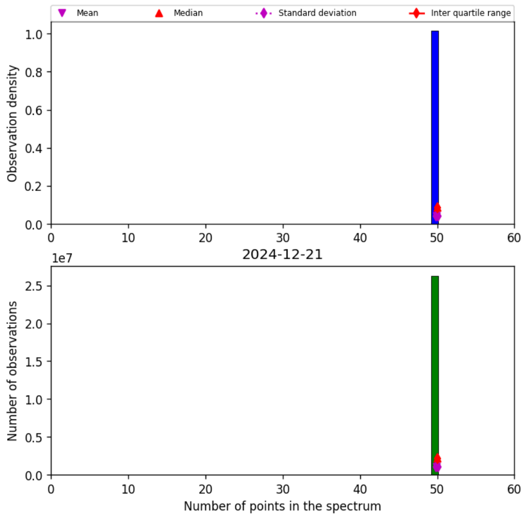
Figure 44: Histogram of "Number of points in the spectrum" for 2024-12-20 to 2024-12-22
