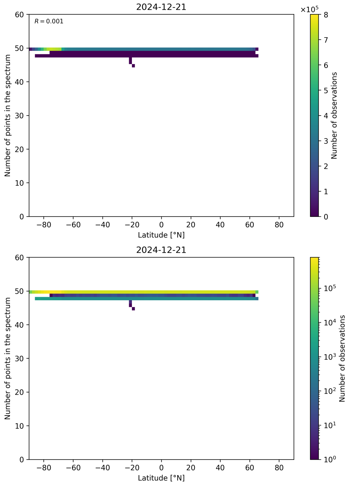
Figure 94: Scatter density plot of “Latitude” against “Number of points in the spectrum” for 2024-12-20 to 2024-12-22.
