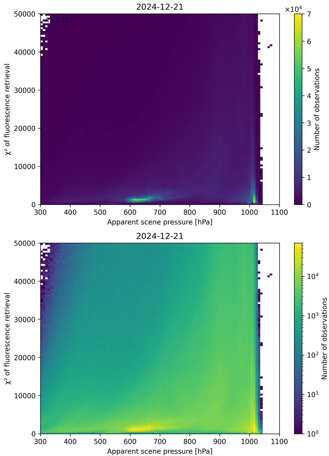
Figure 63: Scatter density plot of “Apparent scene pressure” against “ \chi^2 of fluorescence retrieval” for 2024-12-20 to 2024-12-22.
