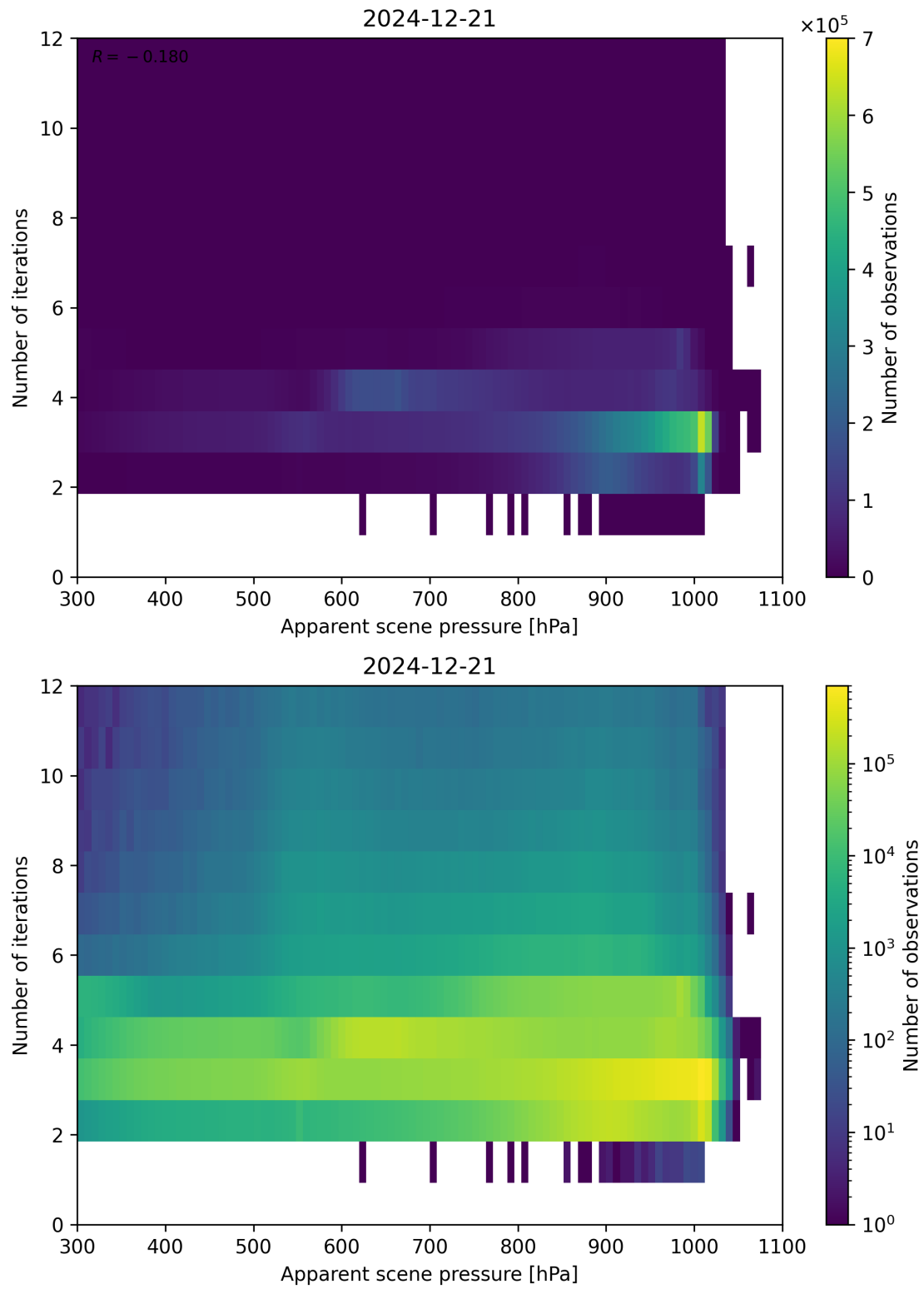
Figure 65: Scatter density plot of “Apparent scene pressure” against “Number of iterations” for 2024-12-20 to 2024-12-22.
