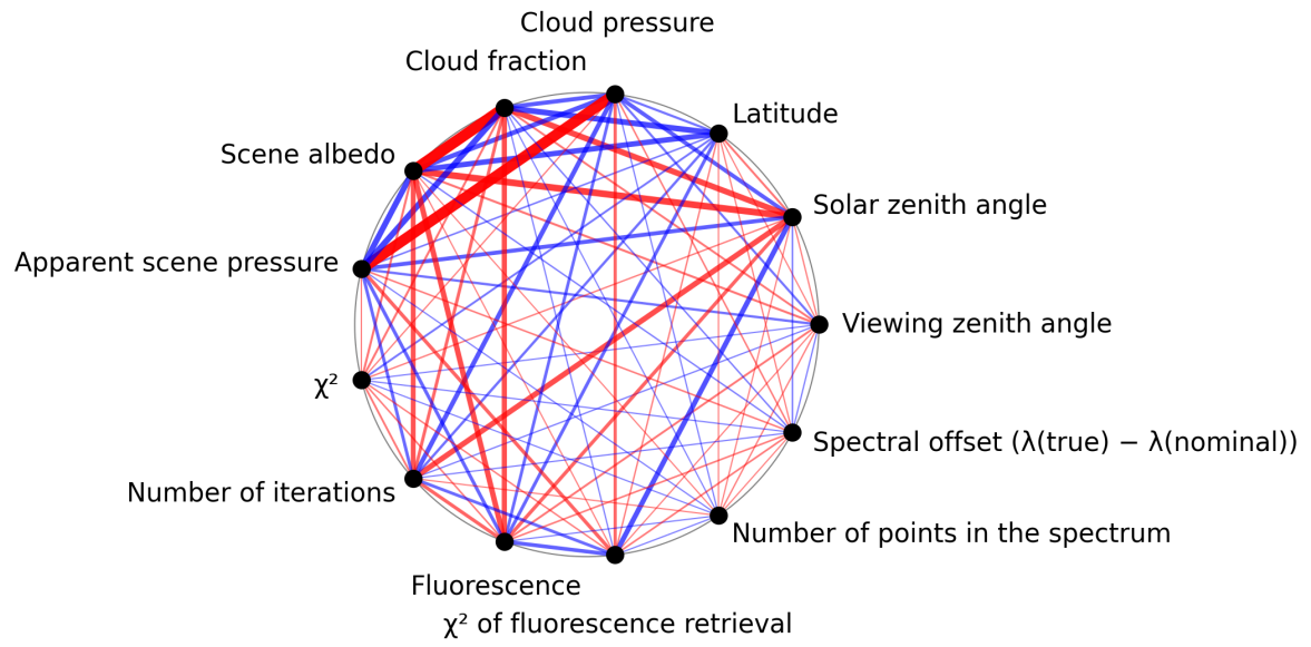
Figure 1: Map of correlation graph for 2024-12-20 to 2024-12-22.
