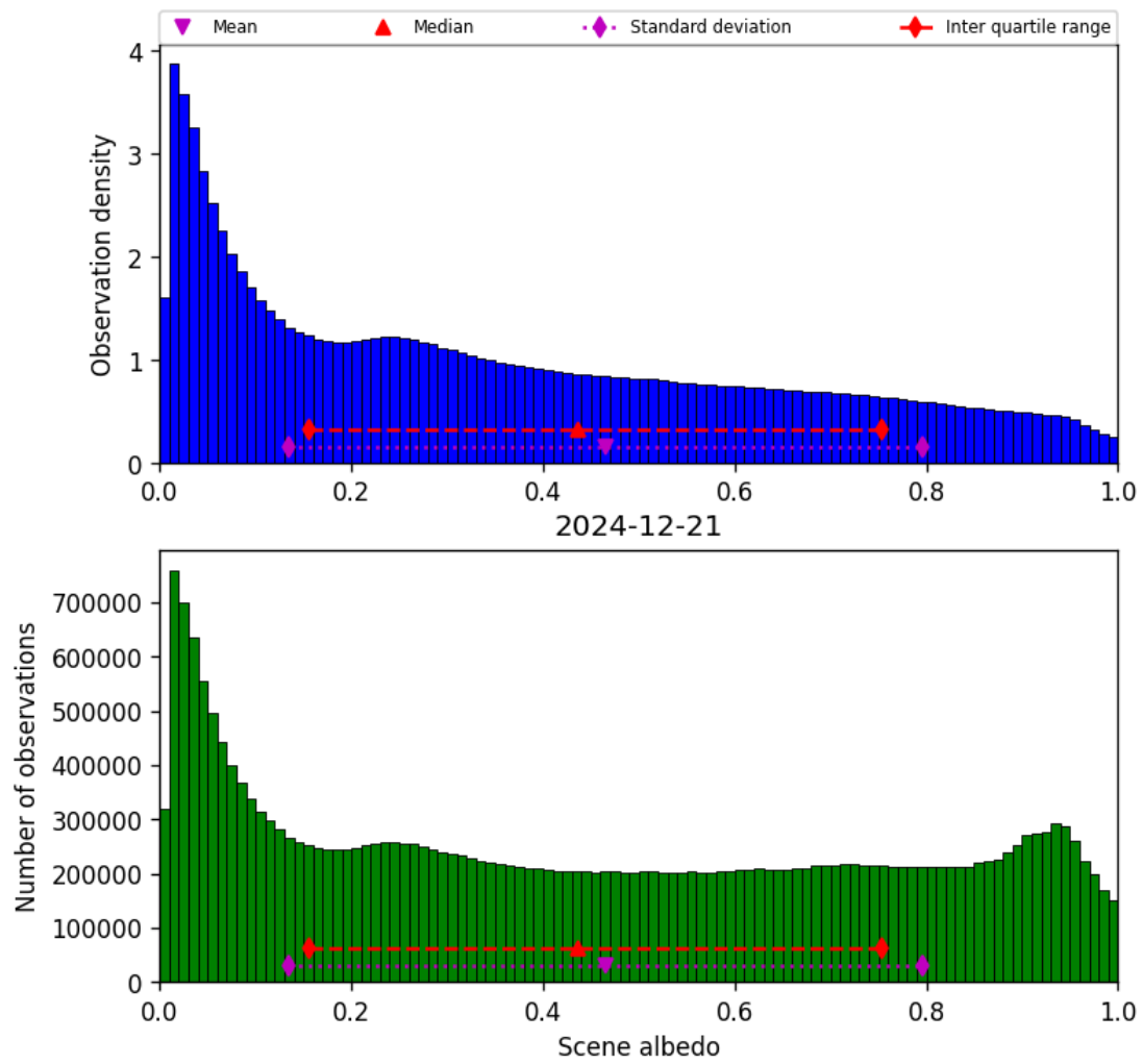
Figure 34: Histogram of “Scene albedo” for 2024-12-20 to 2024-12-22
