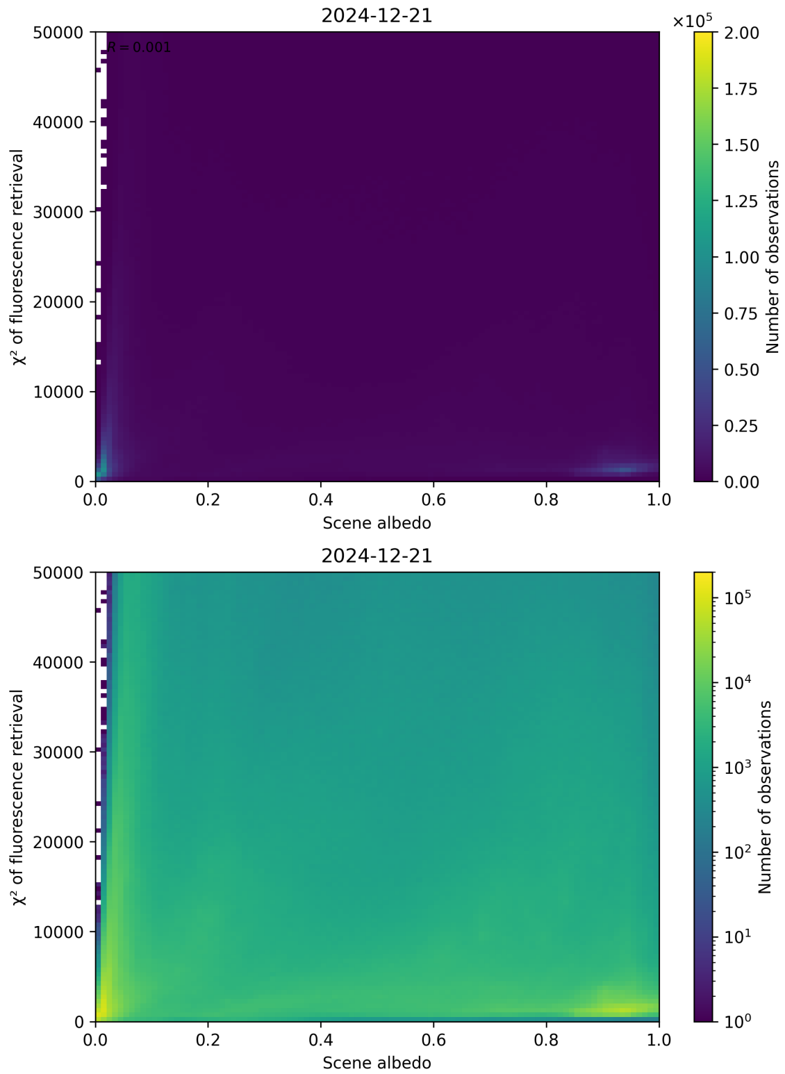
Figure 103: Scatter density plot of “Scene albedo” against “ \chi^2 of fluorescence retrieval” for 2024-12-20 to 2024-12-22.
