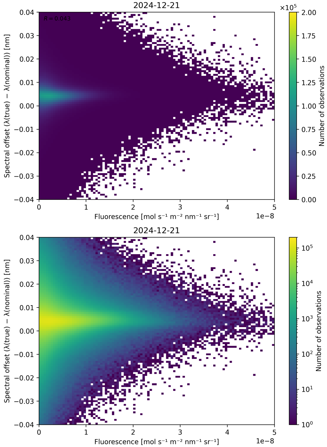
Figure 87: Scatter density plot of “Fluorescence” against “Spectral offset ( \lambda_{\text{true}} - \lambda_{\text{nominal}} )” for 2024-12-20 to 2024-12-22.
