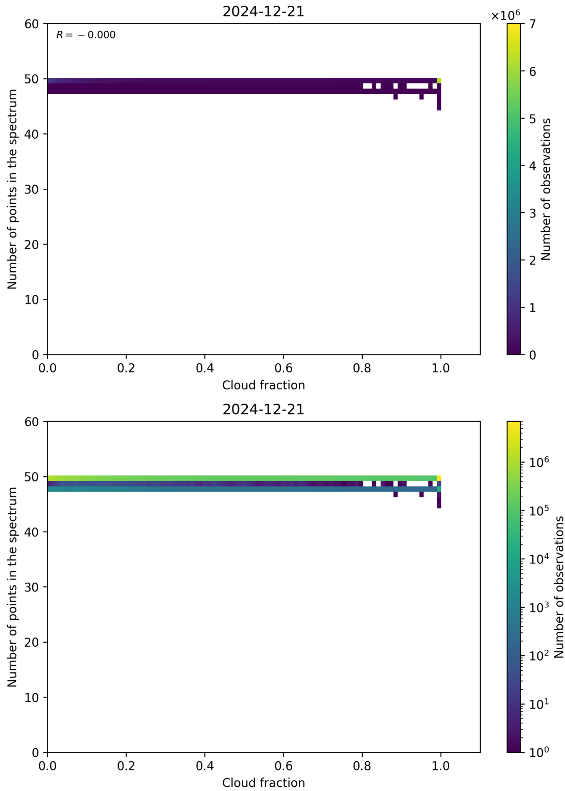
Figure 74: Scatter density plot of “Cloud fraction” against “Number of points in the spectrum” for 2024-12-20 to 2024-12-22.
