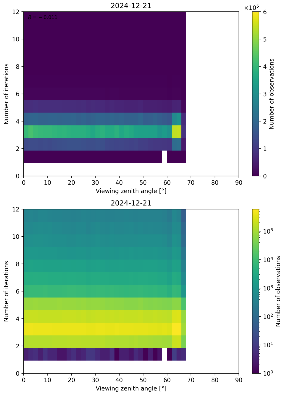
Figure 124: Scatter density plot of “Viewing zenith angle” against “Number of iterations” for 2024-12-20 to 2024-12-22.
