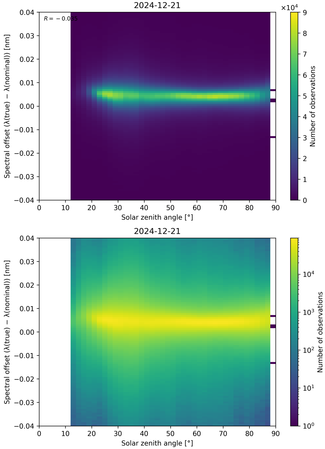
Figure 117: Scatter density plot of “Solar zenith angle” against “Spectral offset ( \lambda_{\text{true}} - \lambda_{\text{nominal}} )” for 2024-12-20 to 2024-12-22.
