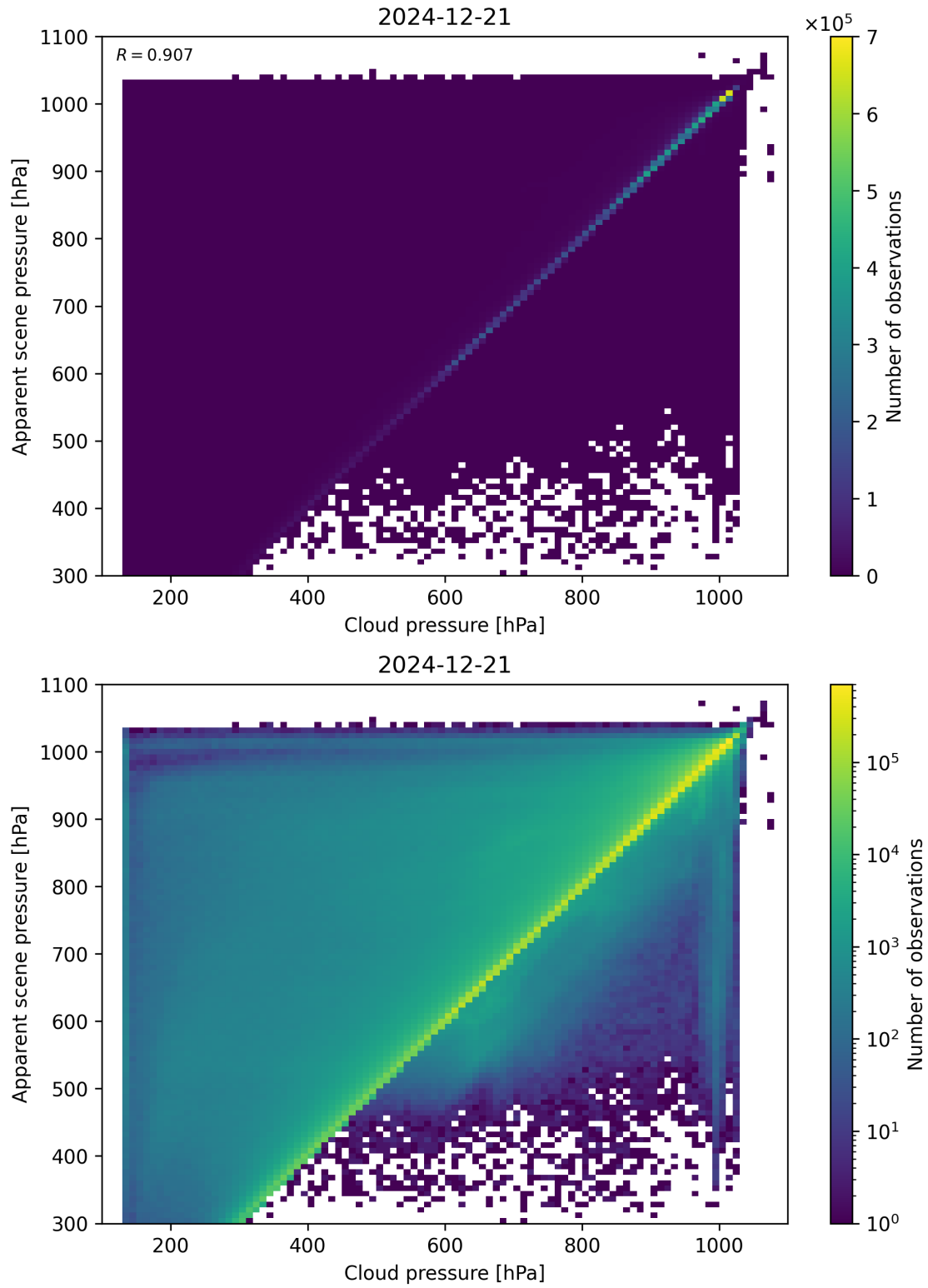
Figure 77: Scatter density plot of “Cloud pressure” against “Apparent scene pressure” for 2024-12-20 to 2024-12-22.
