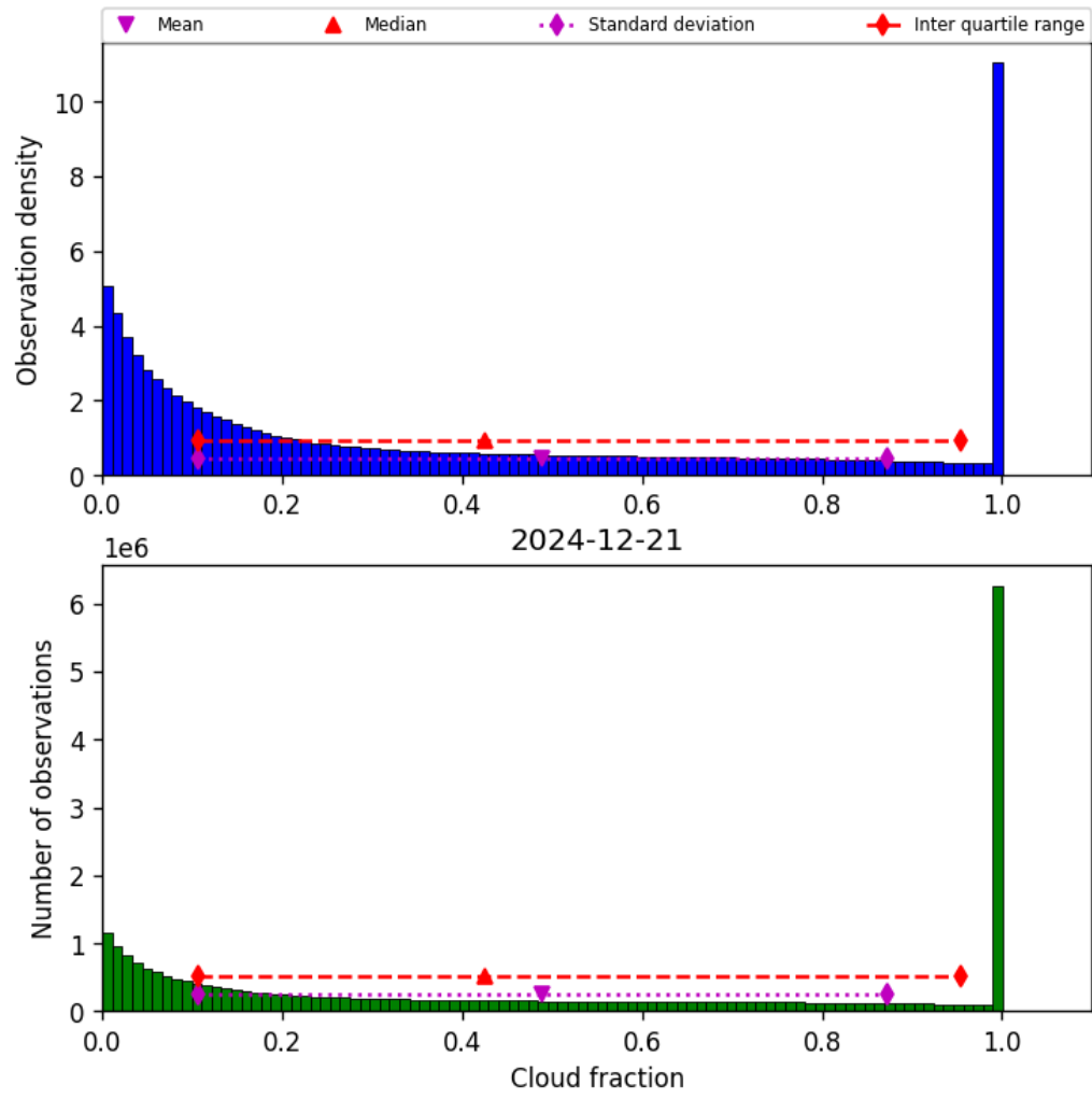
Figure 32: Histogram of “Cloud fraction” for 2024-12-20 to 2024-12-22
