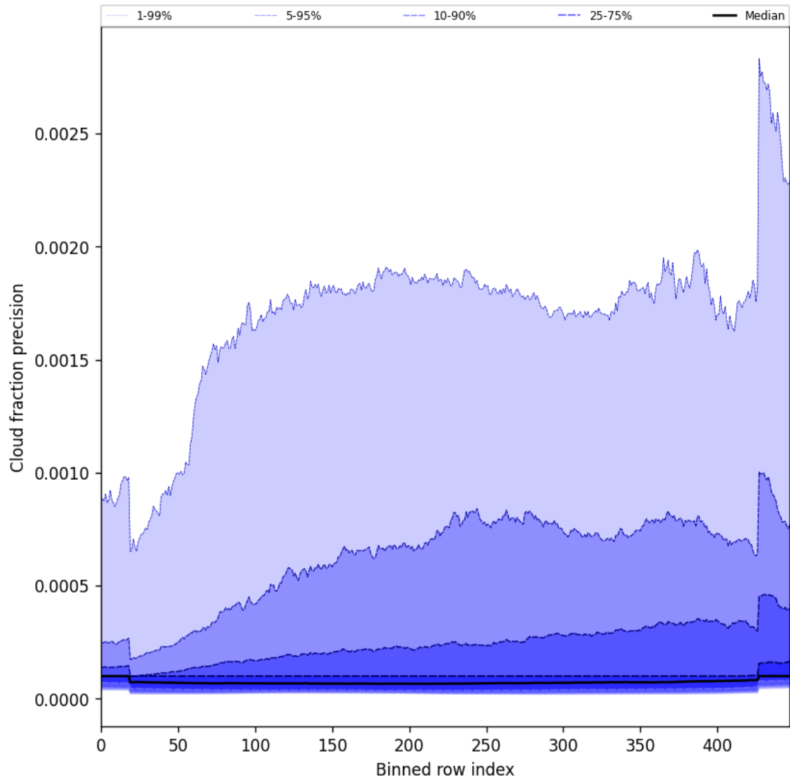
Figure 50: Along track statistics of “Cloud fraction precision” for 2024-12-20 to 2024-12-22
