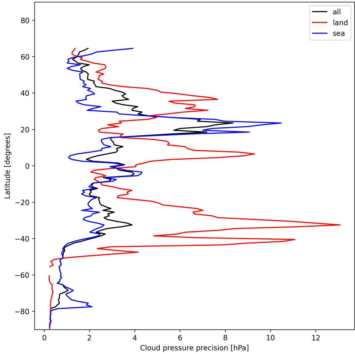
Figure 14: Zonal average of “Cloud pressure precision” for 2024-12-20 to 2024-12-22.
