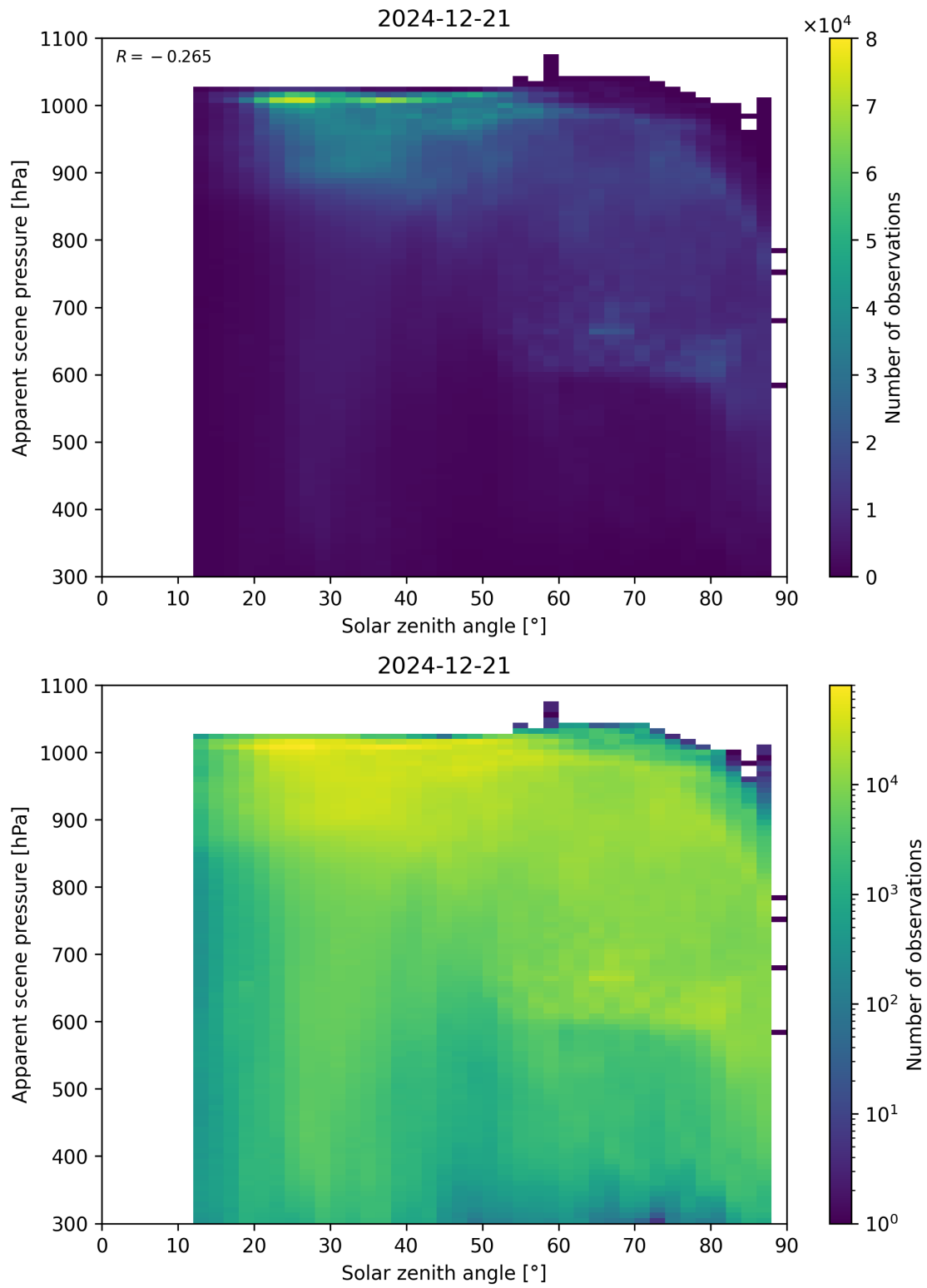
Figure 108: Scatter density plot of “Solar zenith angle” against “Apparent scene pressure” for 2024-12-20 to 2024-12-22.
