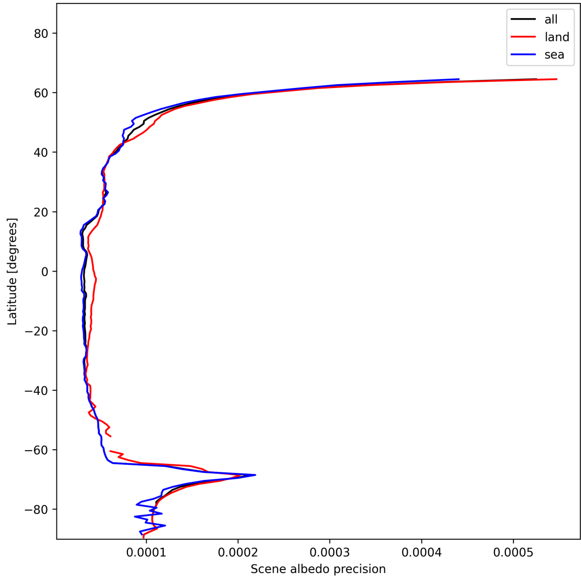
Figure 18: Zonal average of “Scene albedo precision” for 2024-12-20 to 2024-12-22.
