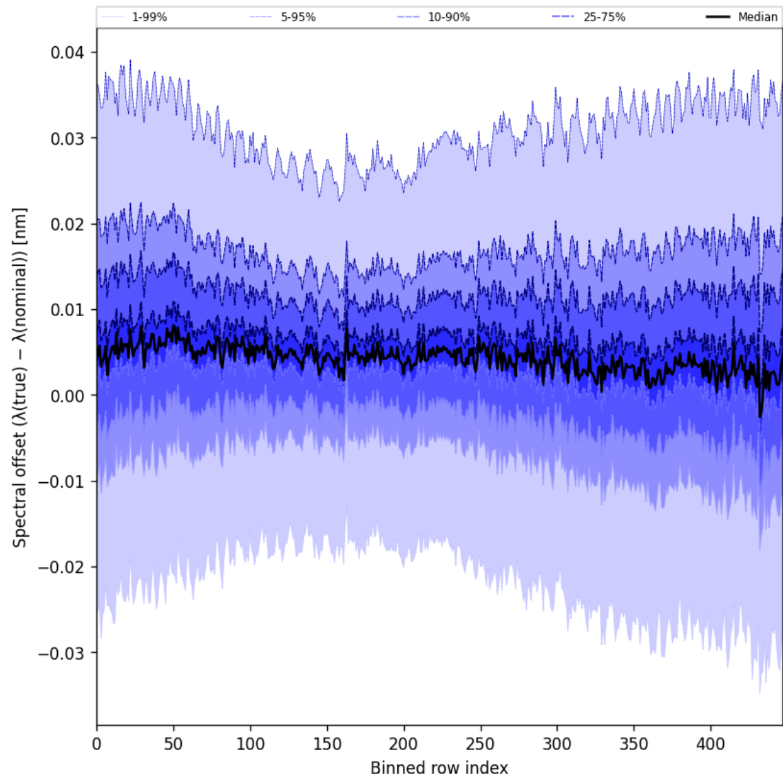
Figure 62: Along track statistics of “Spectral offset ( \lambda_{\text{true}} - \lambda_{\text{nominal}} )” for 2024-12-20 to 2024-12-22
