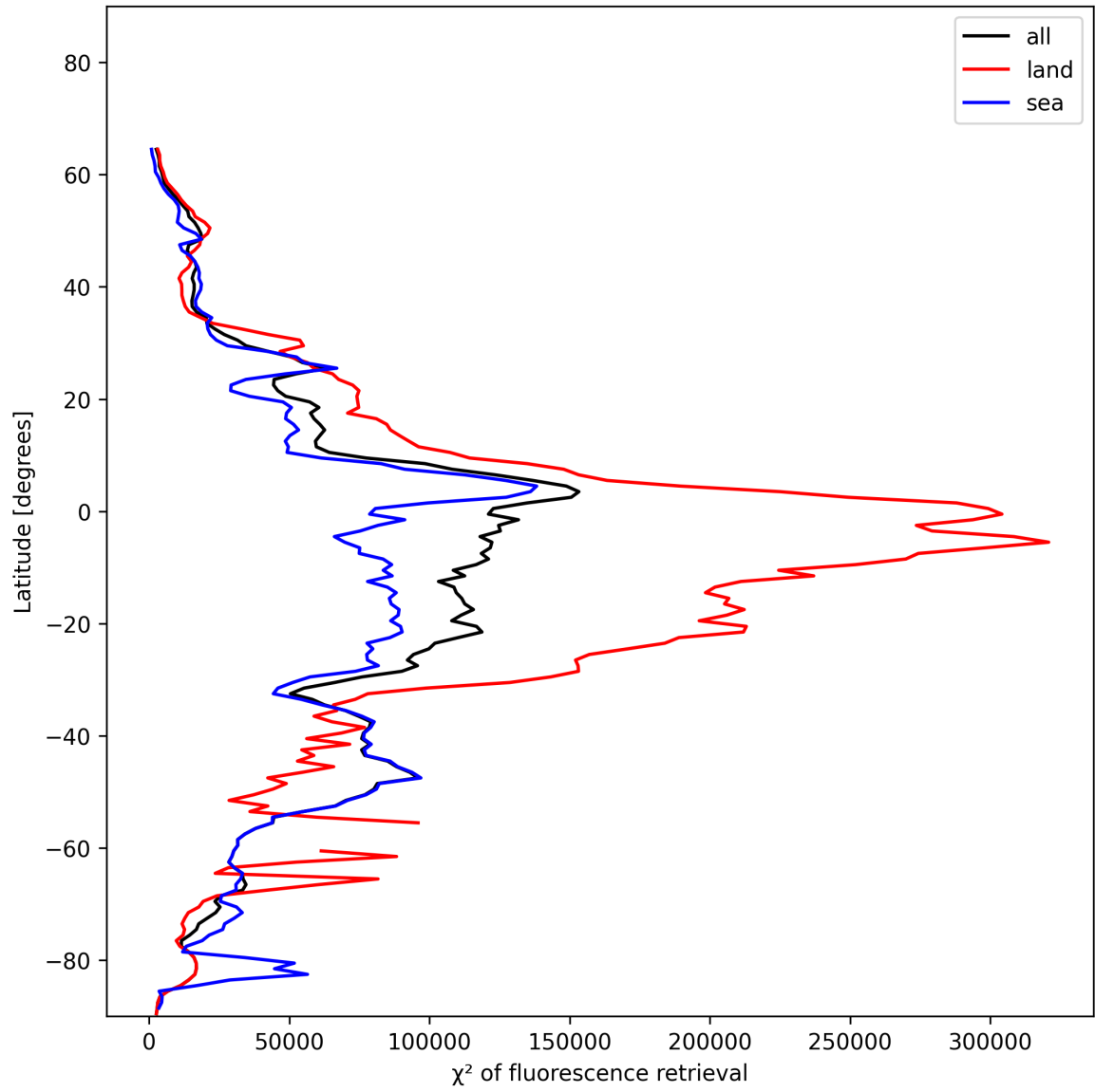
Figure 25: Zonal average of “ \chi^2 of fluorescence retrieval” for 2024-12-20 to 2024-12-22.
