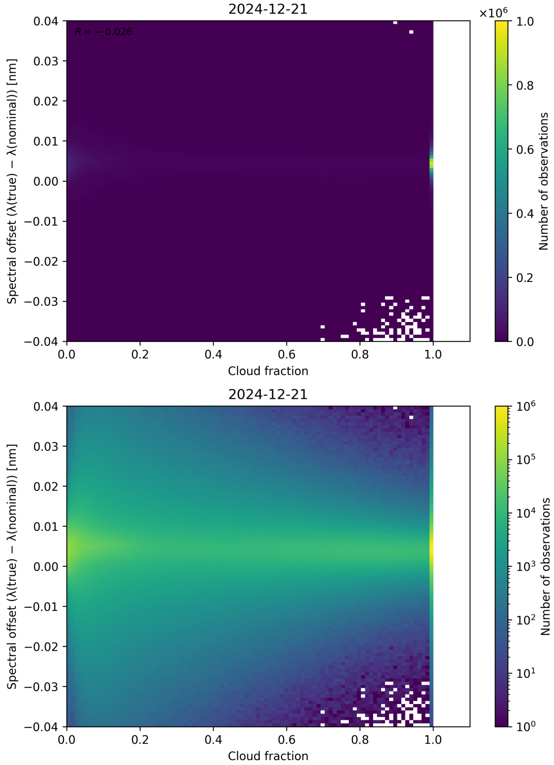
Figure 76: Scatter density plot of “Cloud fraction” against “Spectral offset ( \lambda_{\text{true}} - \lambda_{\text{nominal}} )” for 2024-12-20 to 2024-12-22.
