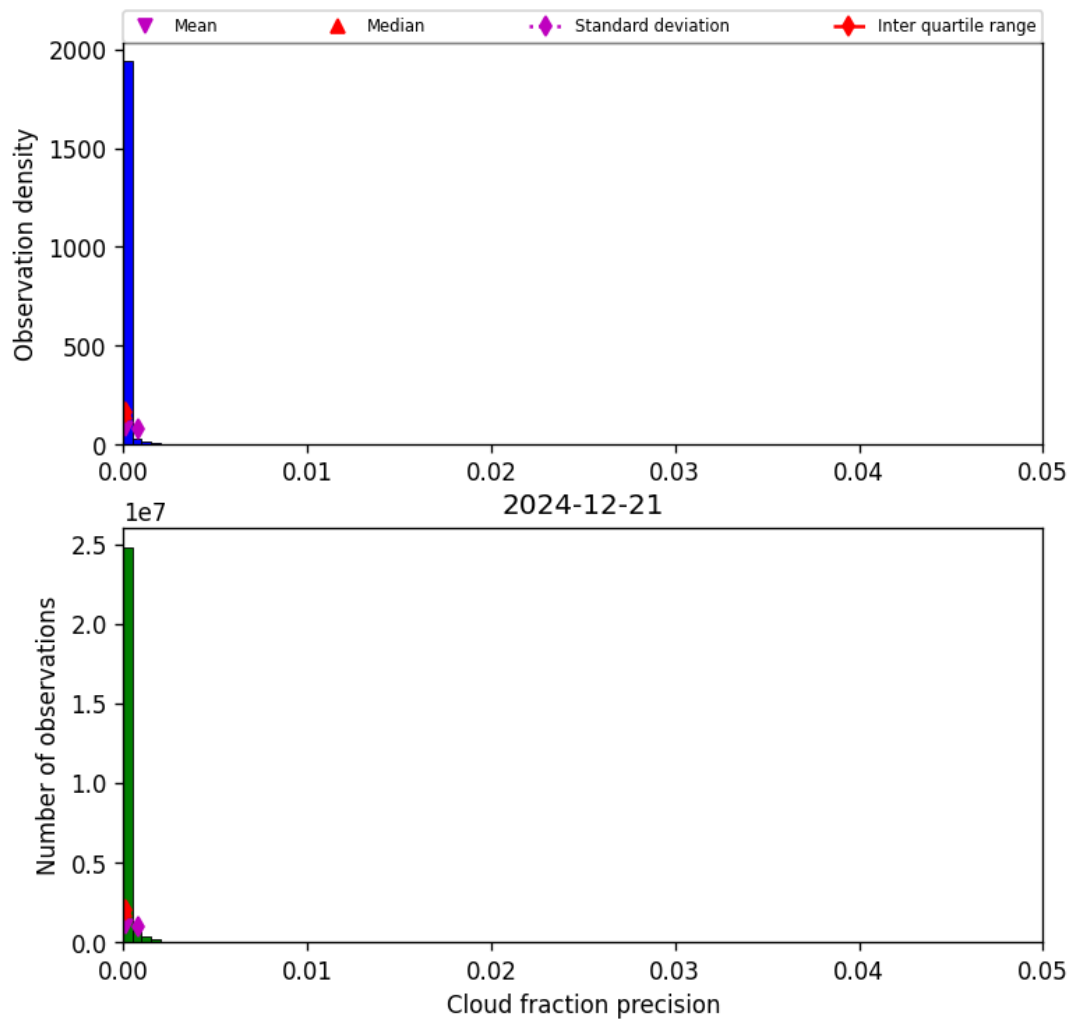
Figure 33: Histogram of “Cloud fraction precision” for 2024-12-20 to 2024-12-22
