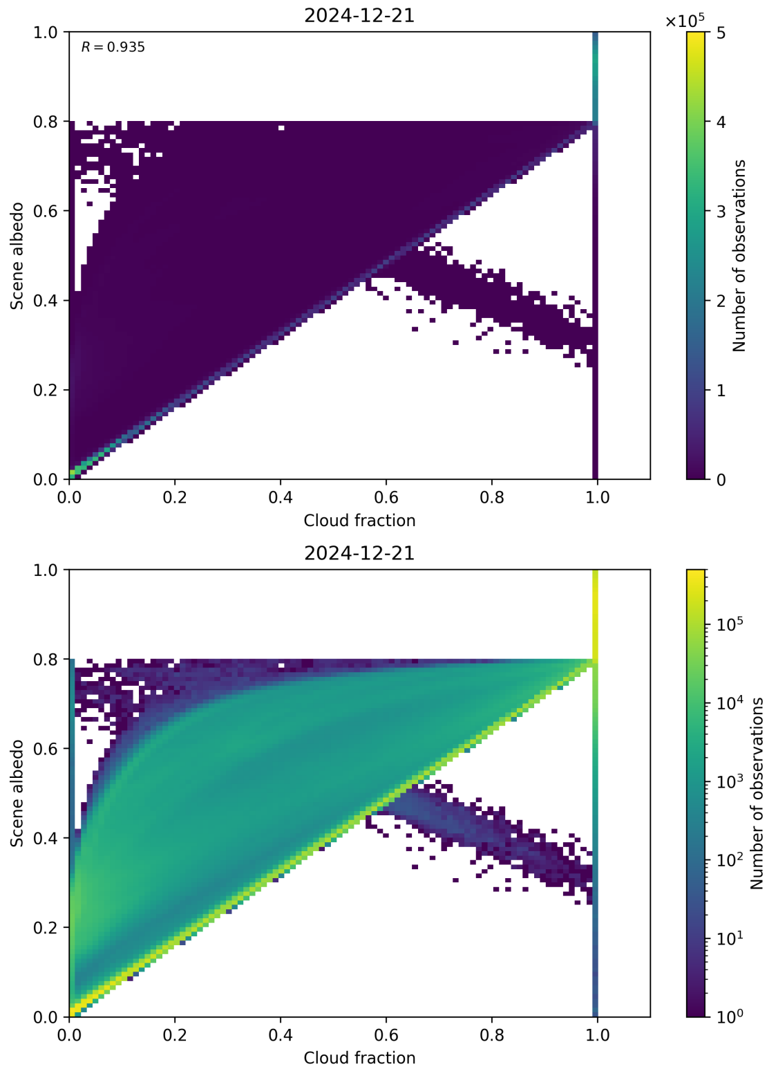
Figure 75: Scatter density plot of “Cloud fraction” against “Scene albedo” for 2024-12-20 to 2024-12-22.
