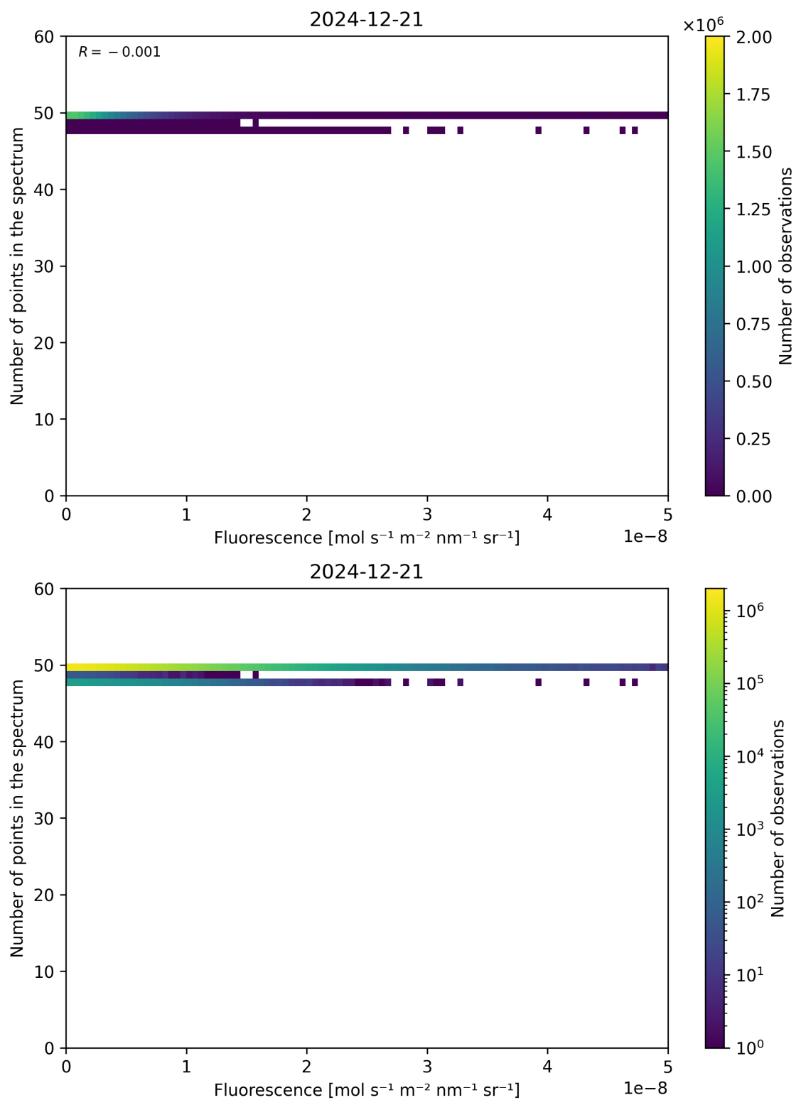
Figure 86: Scatter density plot of “Fluorescence” against “Number of points in the spectrum” for 2024-12-20 to 2024-12-22.
