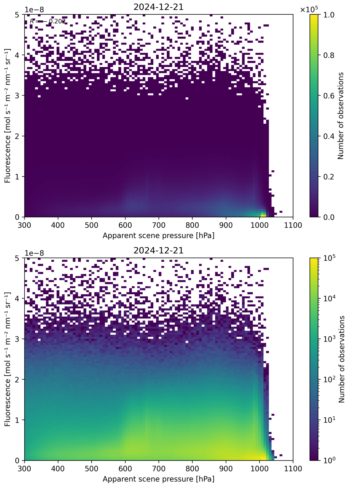
Figure 64: Scatter density plot of “Apparent scene pressure” against “Fluorescence” for 2024-12-20 to 2024-12-22.
