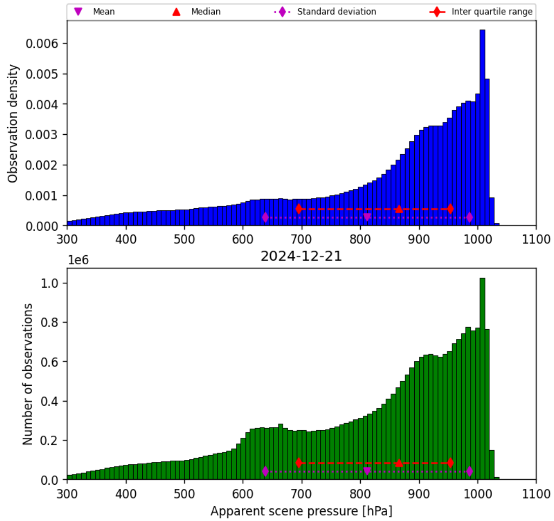
Figure 36: Histogram of “Apparent scene pressure” for 2024-12-20 to 2024-12-22
