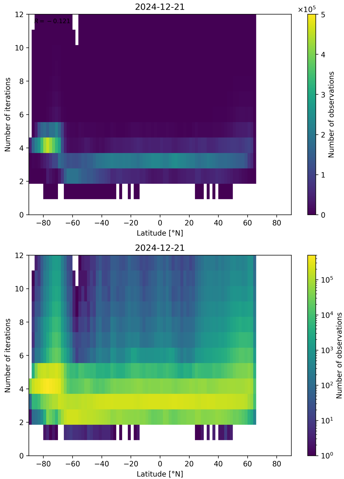
Figure 93: Scatter density plot of “Latitude” against “Number of iterations” for 2024-12-20 to 2024-12-22.
