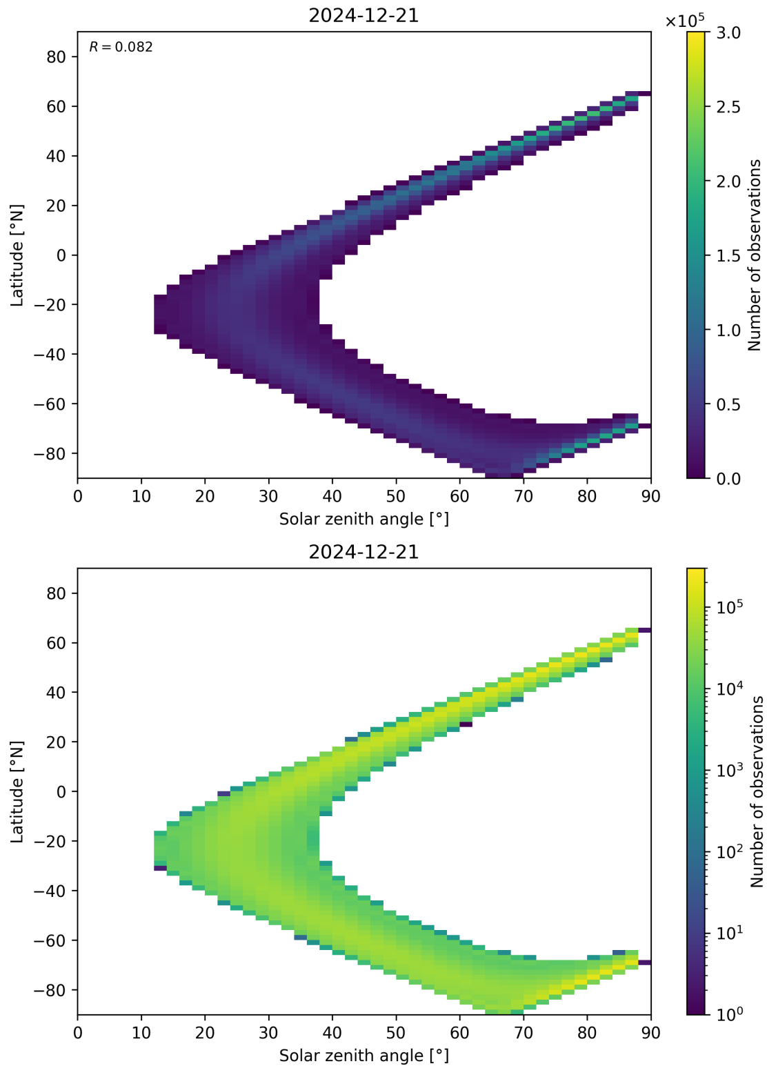
Figure 113: Scatter density plot of “Solar zenith angle” against “Latitude” for 2024-12-20 to 2024-12-22.
