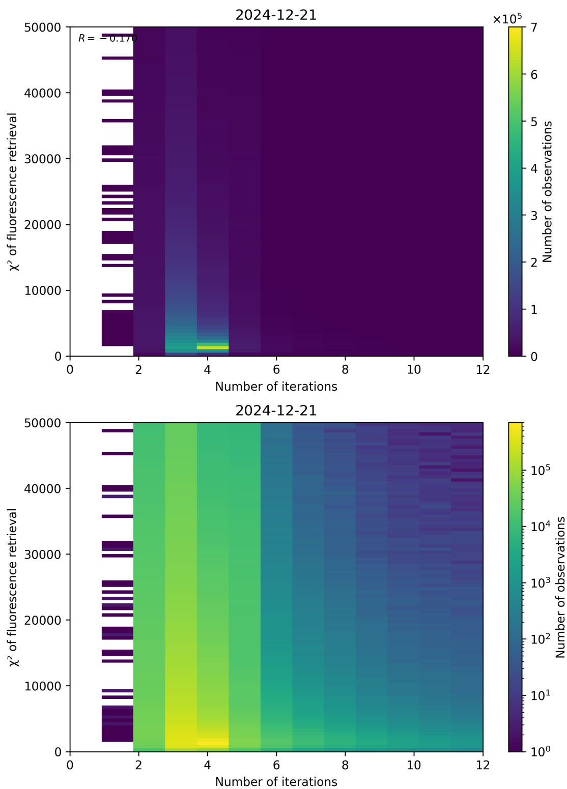
Figure 97: Scatter density plot of “Number of iterations” against “ \chi^2 of fluorescence retrieval” for 2024-12-20 to 2024-12-22.
