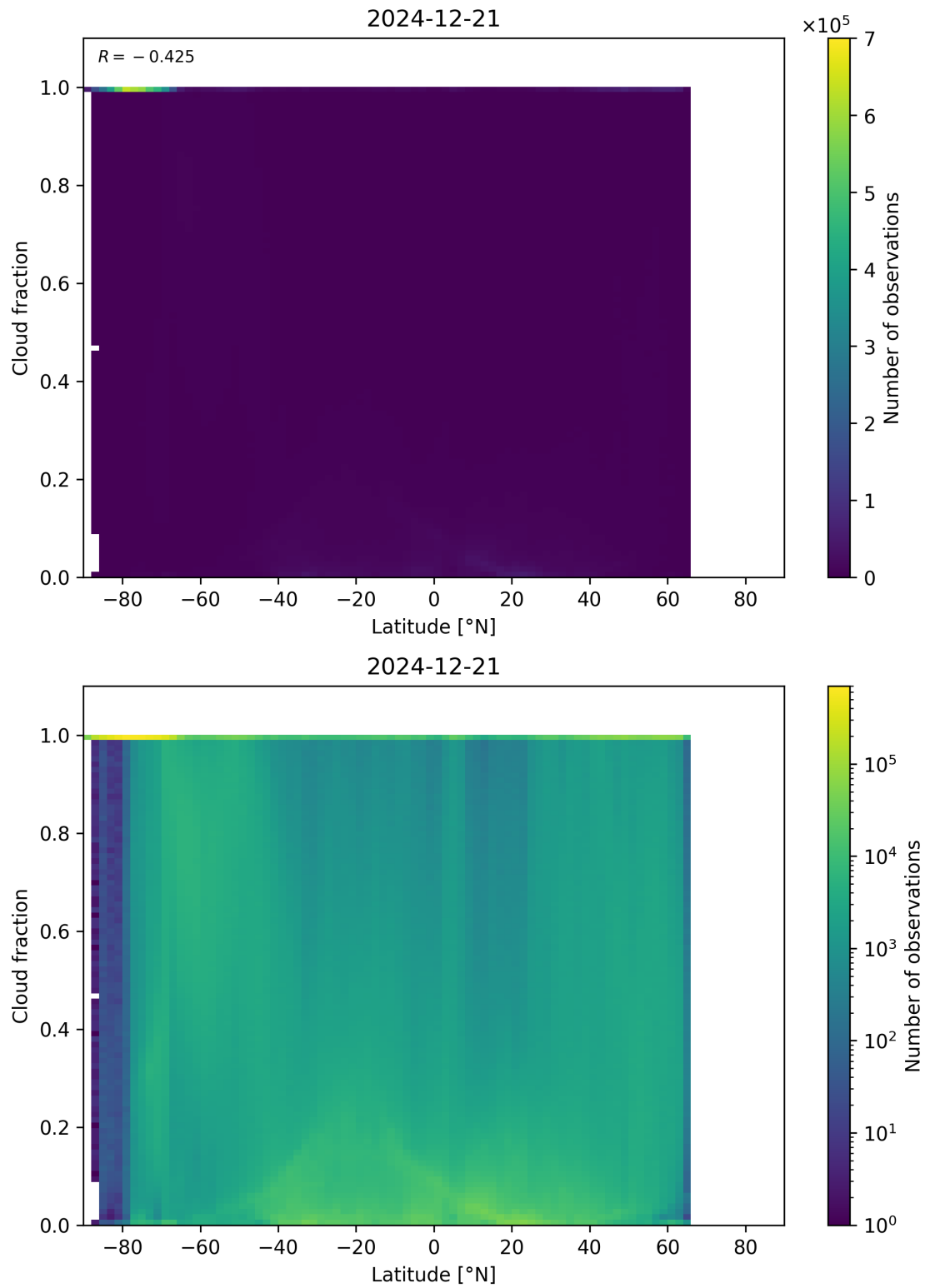
Figure 90: Scatter density plot of “Latitude” against “Cloud fraction” for 2024-12-20 to 2024-12-22.
