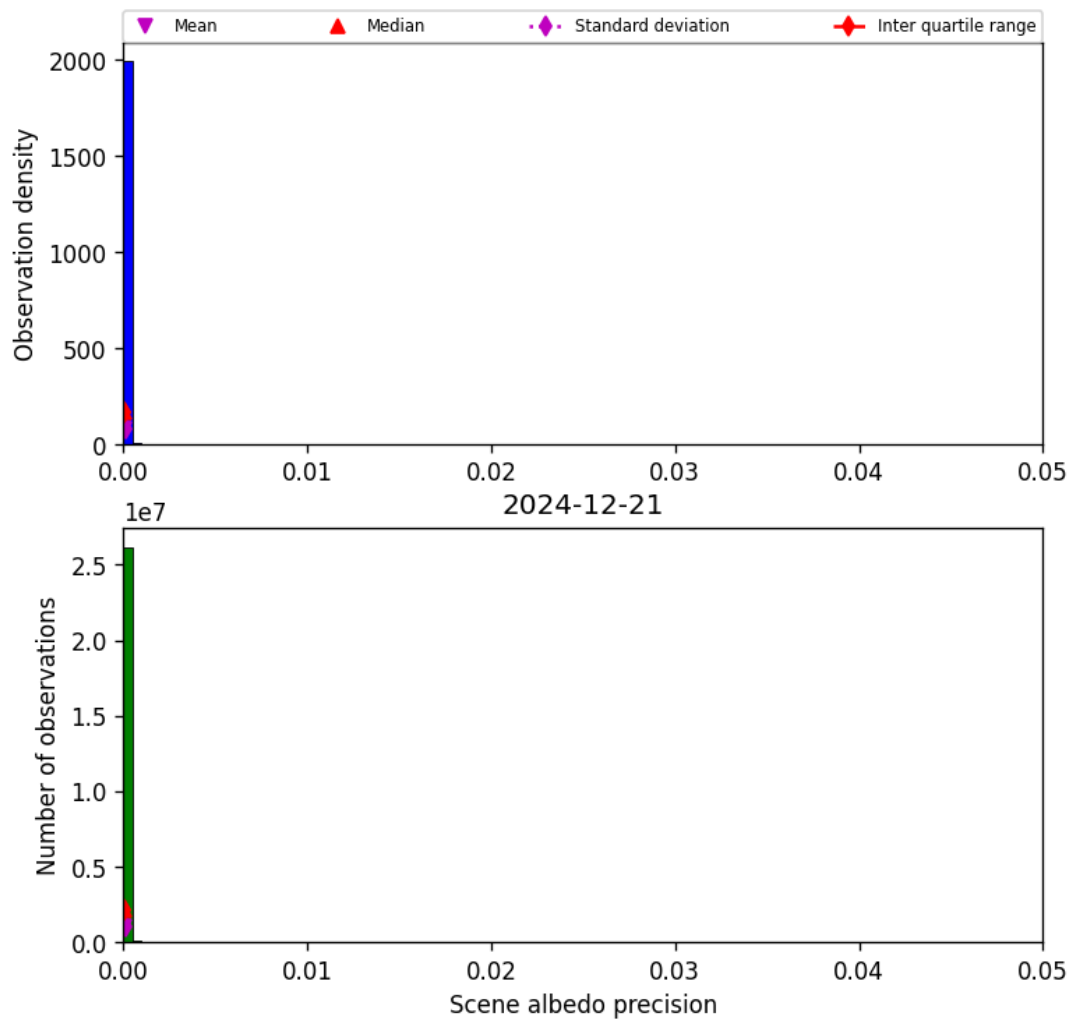
Figure 35: Histogram of “Scene albedo precision” for 2024-12-20 to 2024-12-22
