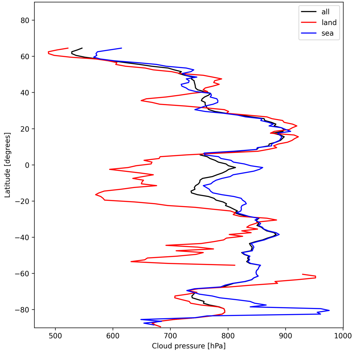
Figure 13: Zonal average of “Cloud pressure” for 2024-12-20 to 2024-12-22.
