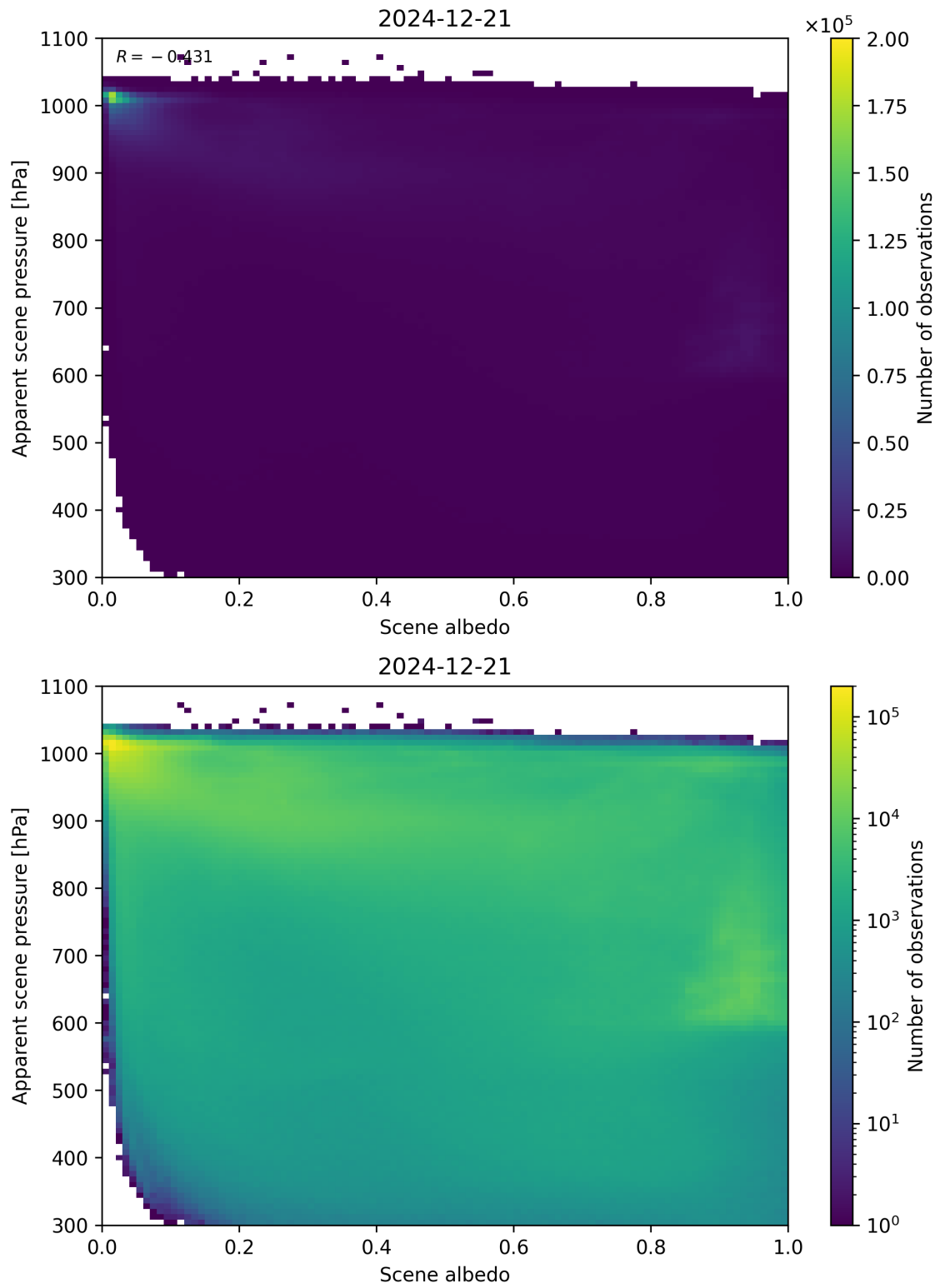
Figure 102: Scatter density plot of “Scene albedo” against “Apparent scene pressure” for 2024-12-20 to 2024-12-22.
