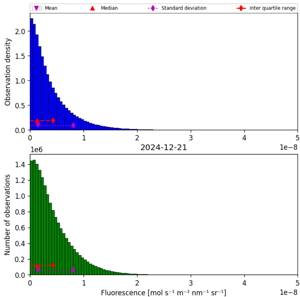
Figure 40: Histogram of “Fluorescence” for 2024-12-20 to 2024-12-22
