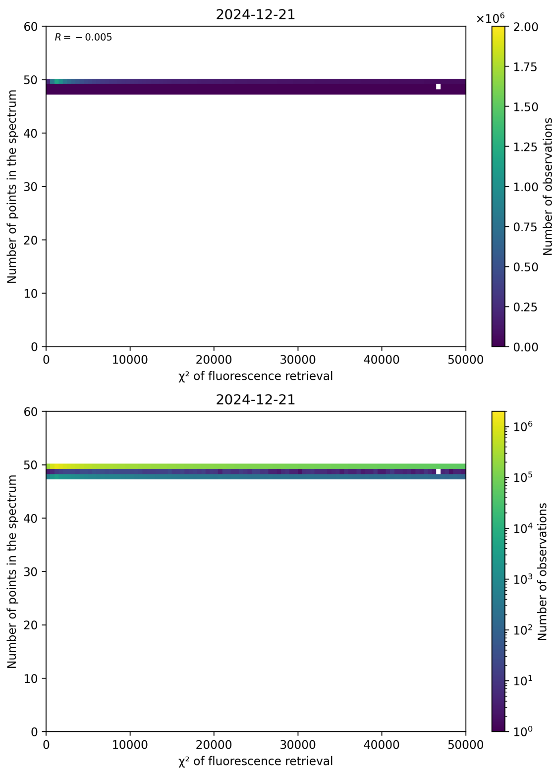
Figure 68: Scatter density plot of " \chi^2 of fluorescence retrieval" against "Number of points in the spectrum" for 2024-12-20 to 2024-12-22.
