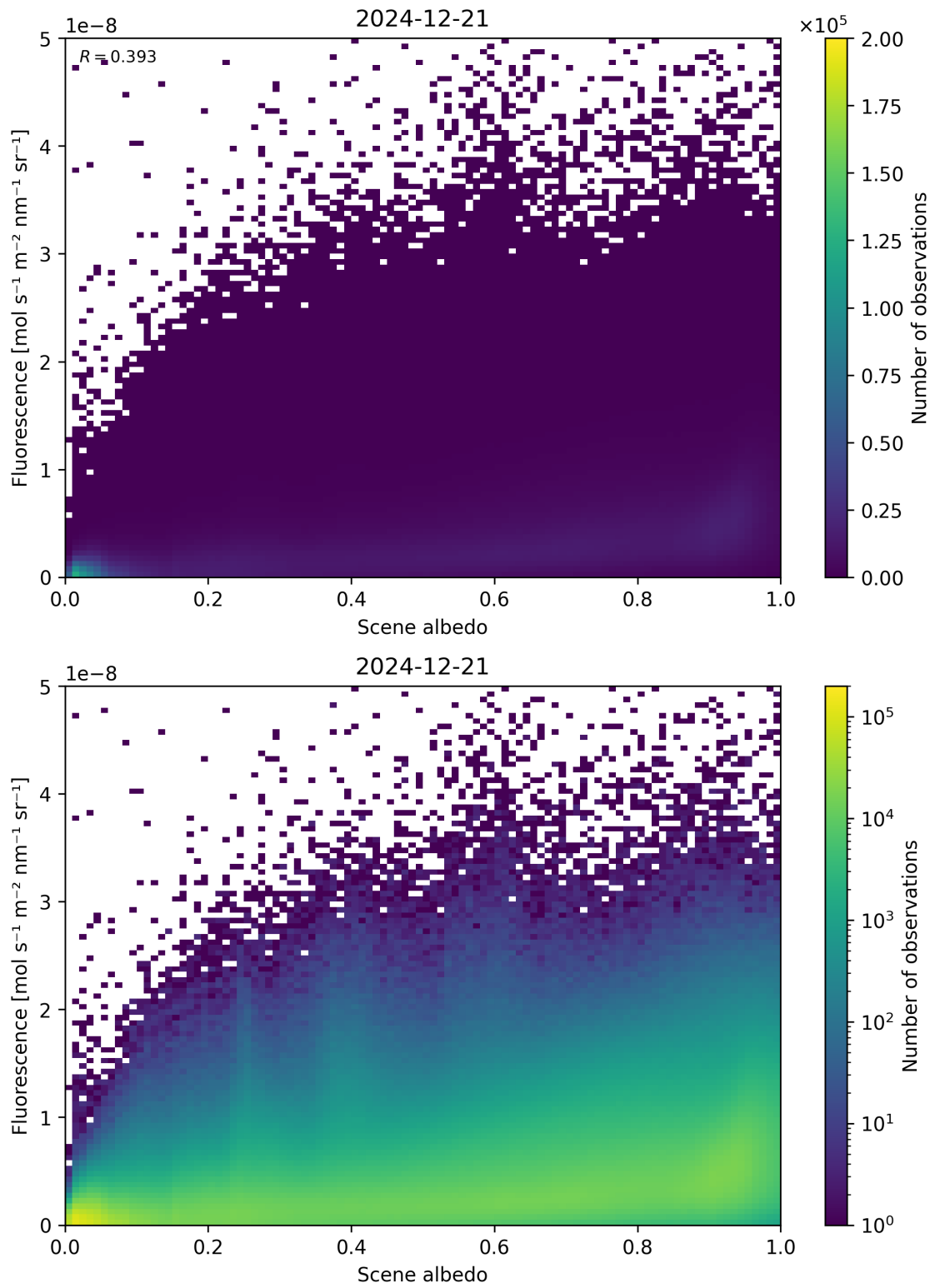
Figure 104: Scatter density plot of “Scene albedo” against “Fluorescence” for 2024-12-20 to 2024-12-22.
