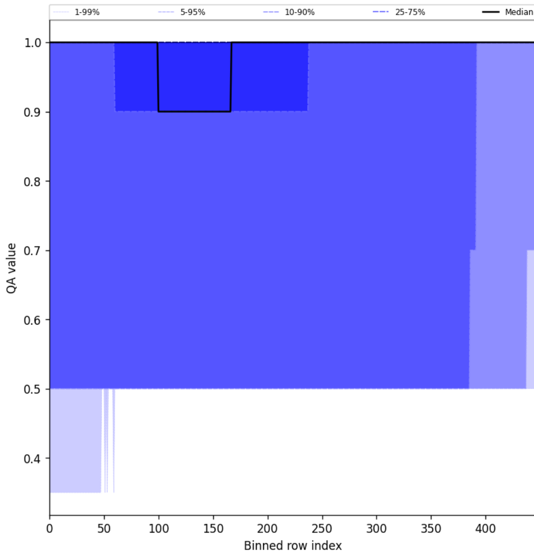
Figure 46: Along track statistics of “QA value” for 2024-12-20 to 2024-12-22
