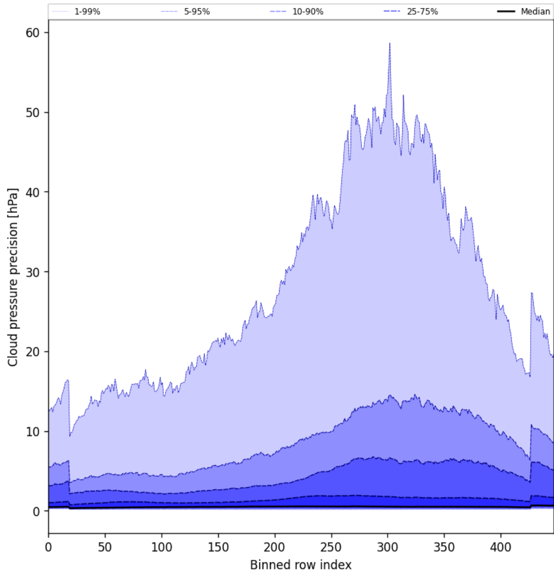
Figure 48: Along track statistics of “Cloud pressure precision” for 2024-12-20 to 2024-12-22
