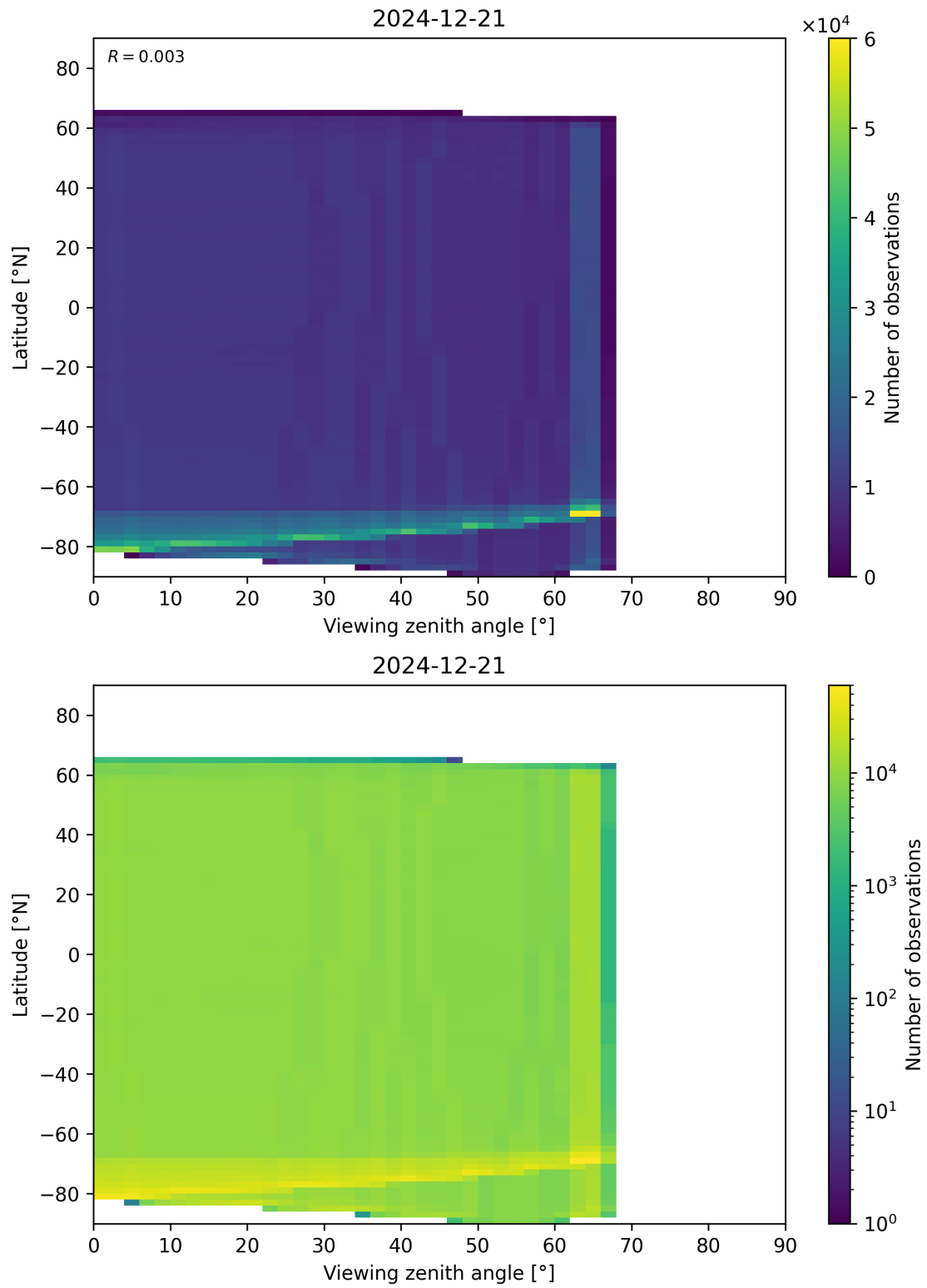
Figure 123: Scatter density plot of “Viewing zenith angle” against “Latitude” for 2024-12-20 to 2024-12-22.
