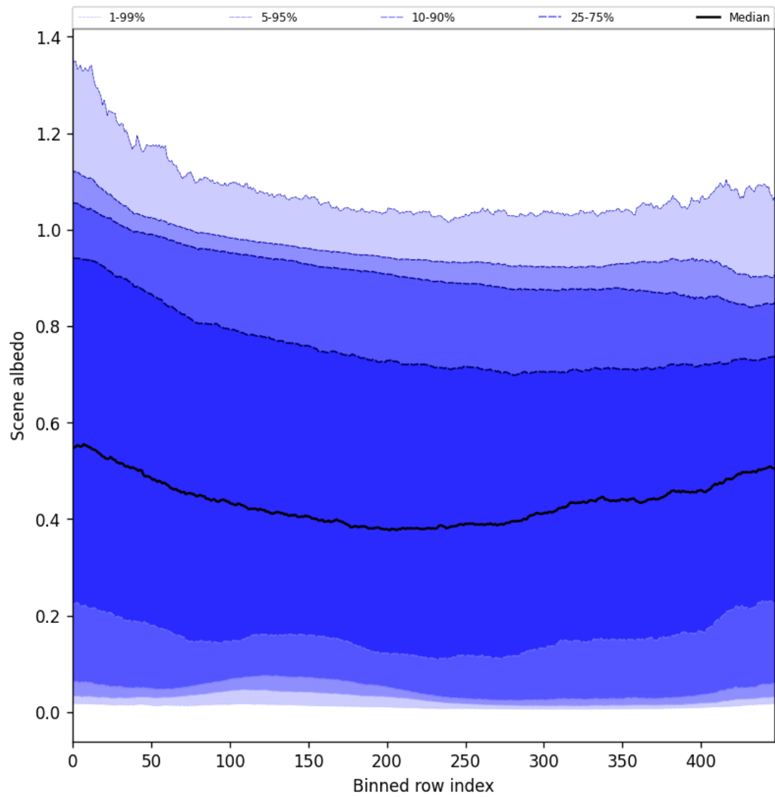
Figure 51: Along track statistics of “Scene albedo” for 2024-12-20 to 2024-12-22
