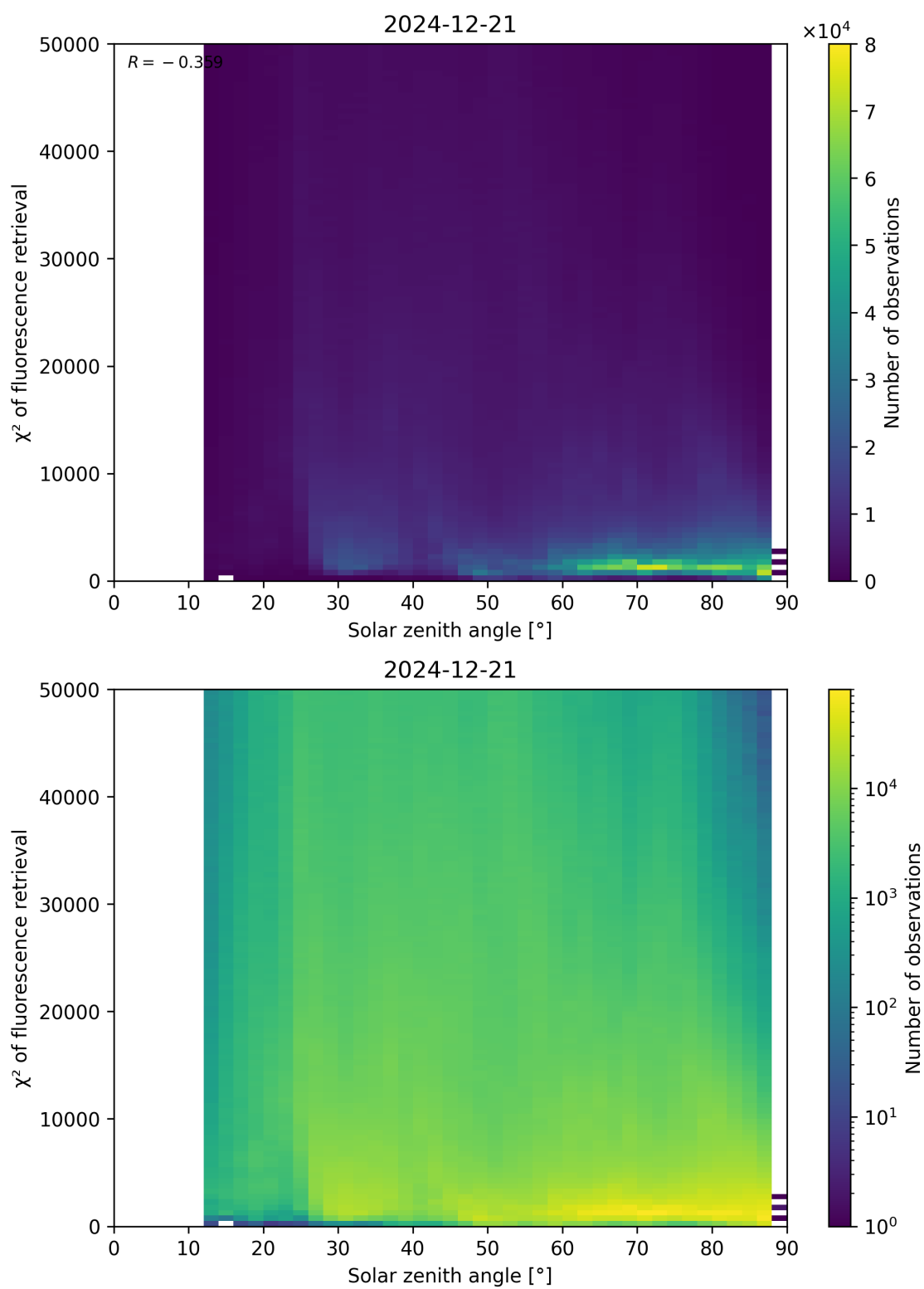
Figure 109: Scatter density plot of “Solar zenith angle” against “ \chi^2 of fluorescence retrieval” for 2024-12-20 to 2024-12-22.
