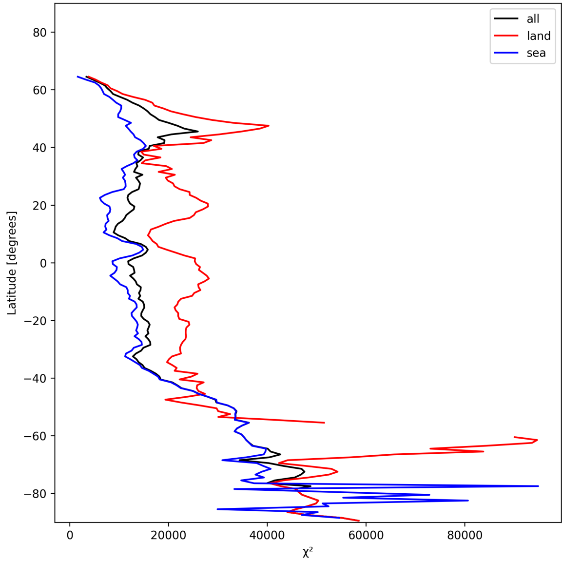
Figure 21: Zonal average of “ \chi^2 ” for 2024-12-20 to 2024-12-22.
