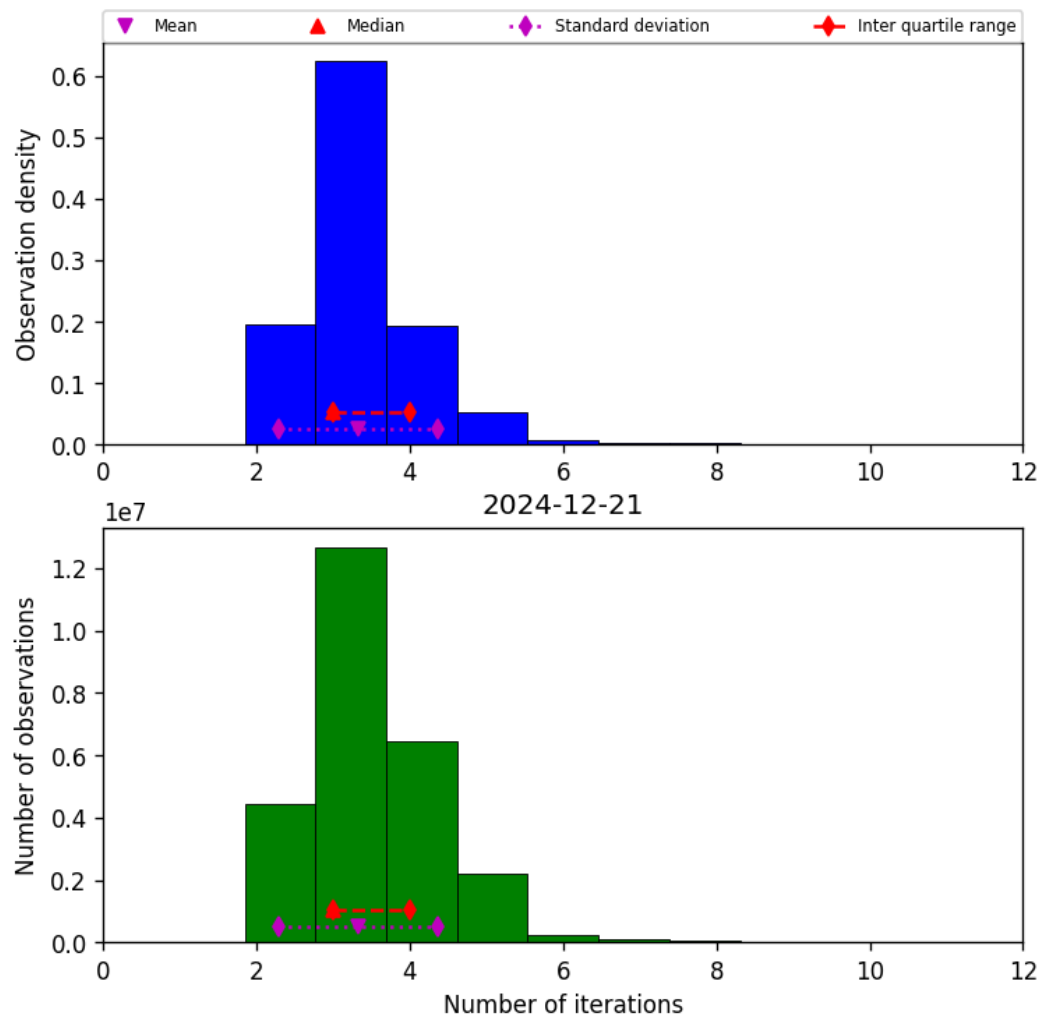
Figure 39: Histogram of “Number of iterations” for 2024-12-20 to 2024-12-22
