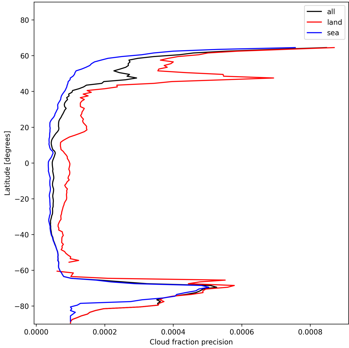
Figure 16: Zonal average of “Cloud fraction precision” for 2024-12-20 to 2024-12-22.
