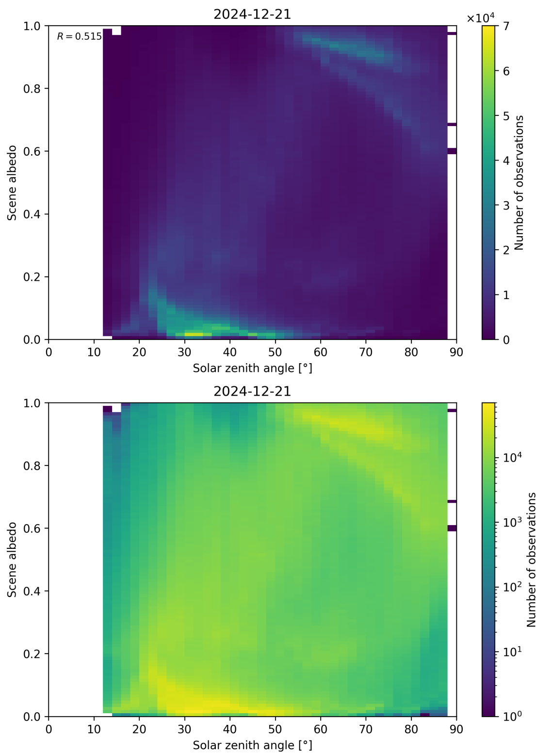
Figure 116: Scatter density plot of “Solar zenith angle” against “Scene albedo” for 2024-12-20 to 2024-12-22.
