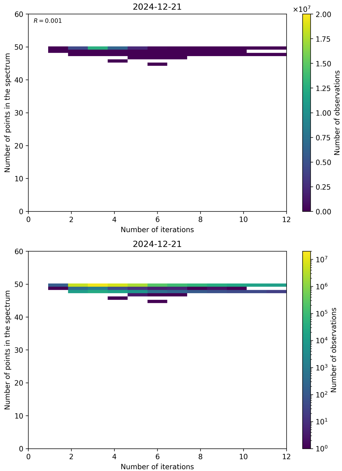
Figure 99: Scatter density plot of “Number of iterations” against “Number of points in the spectrum” for 2024-12-20 to 2024-12-22.
