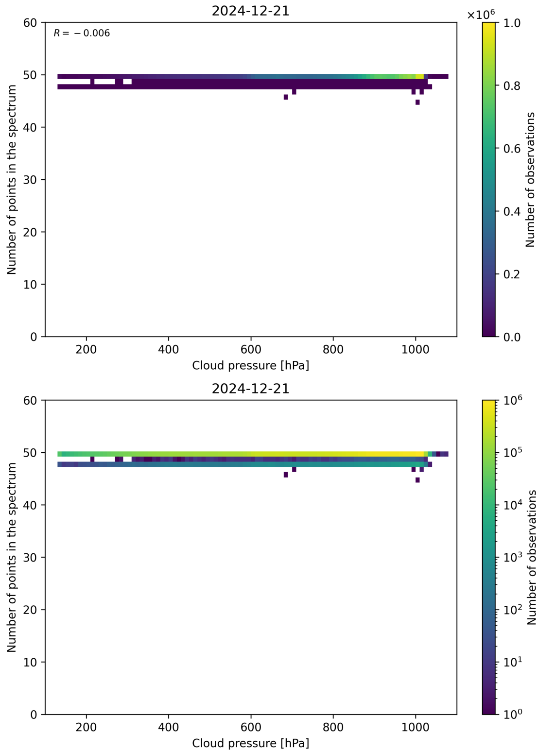
Figure 82: Scatter density plot of “Cloud pressure” against “Number of points in the spectrum” for 2024-12-20 to 2024-12-22.
