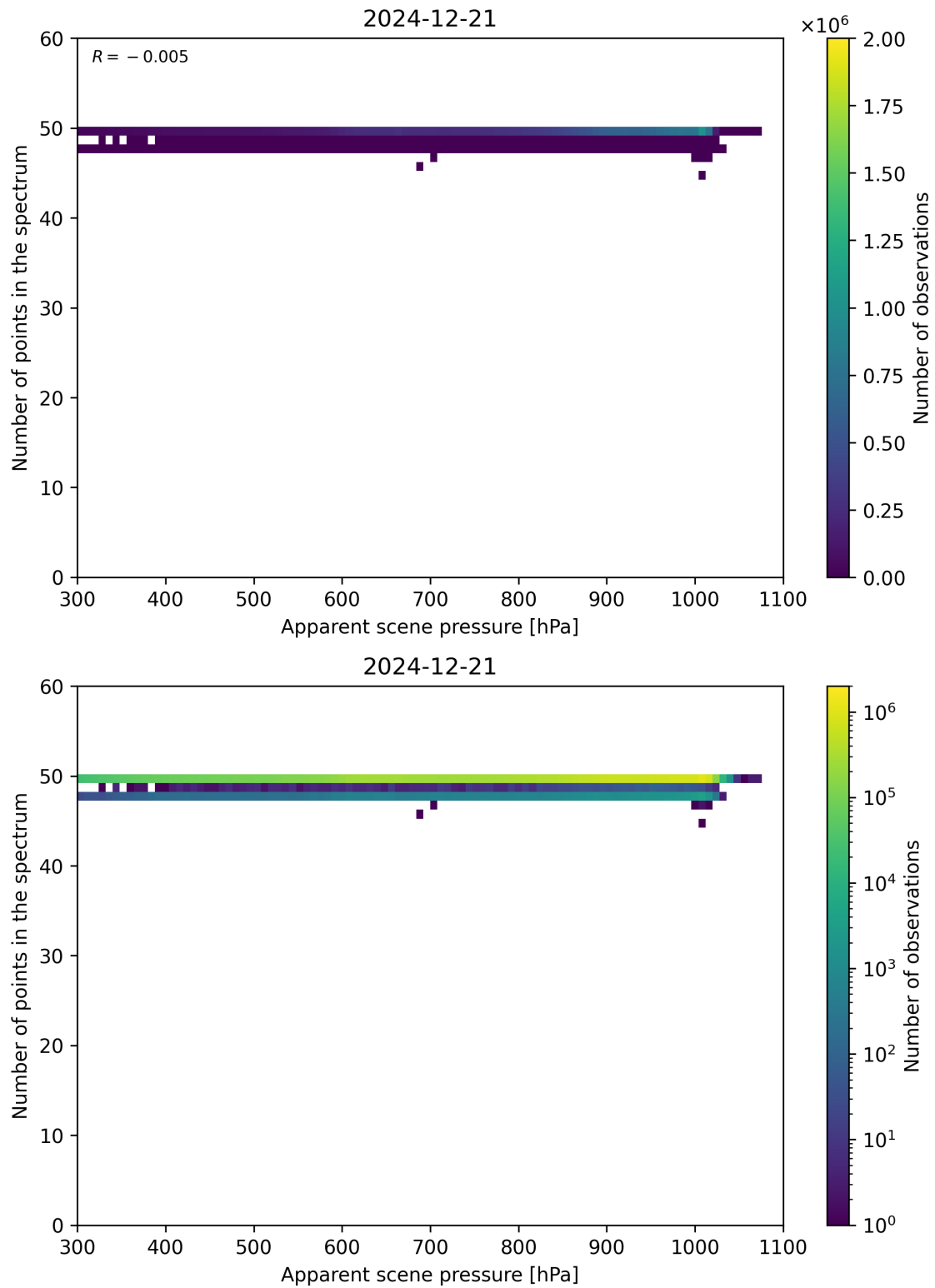
Figure 66: Scatter density plot of “Apparent scene pressure” against “Number of points in the spectrum” for 2024-12-20 to 2024-12-22.
