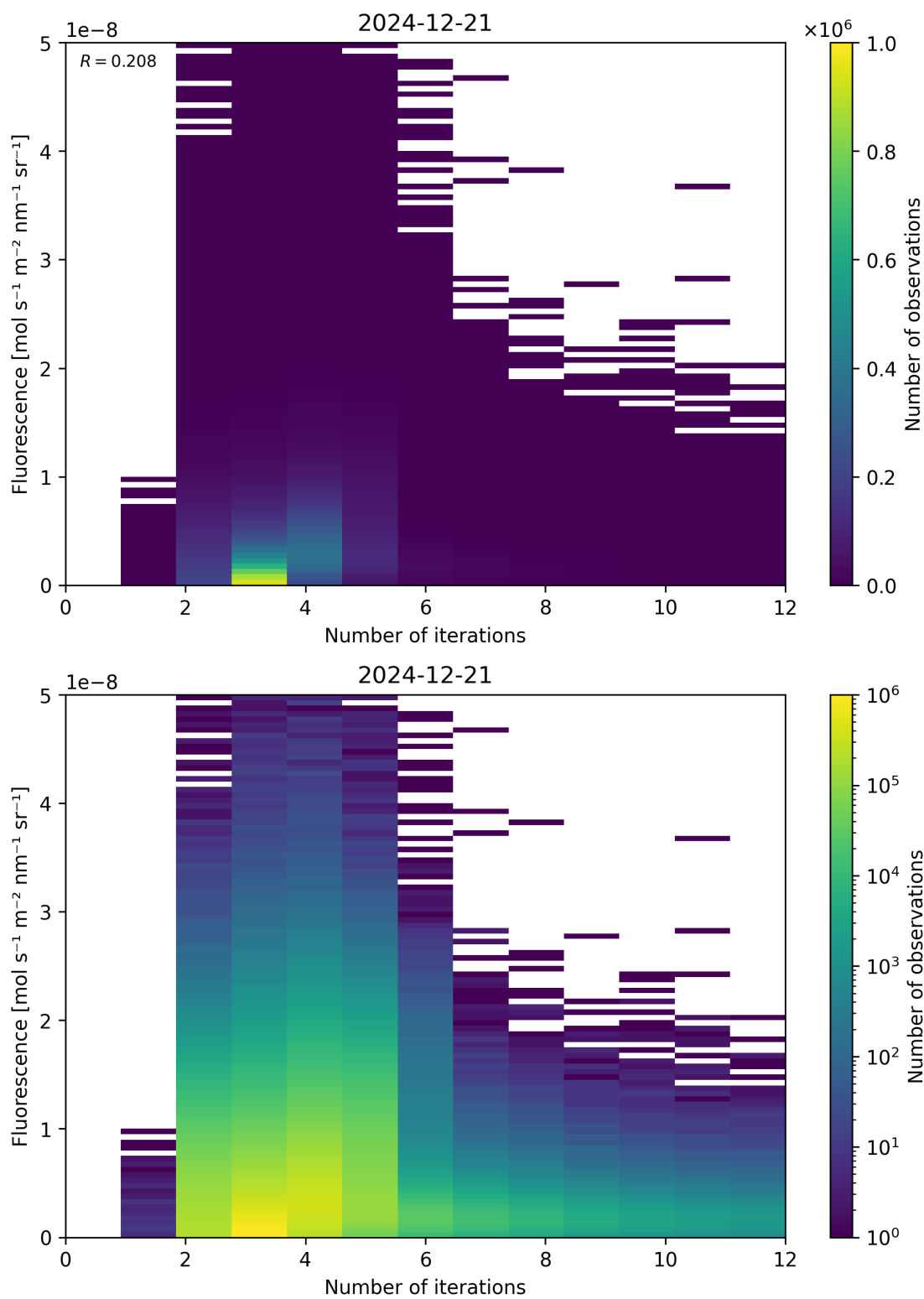
Figure 98: Scatter density plot of “Number of iterations” against “Fluorescence” for 2024-12-20 to 2024-12-22.
