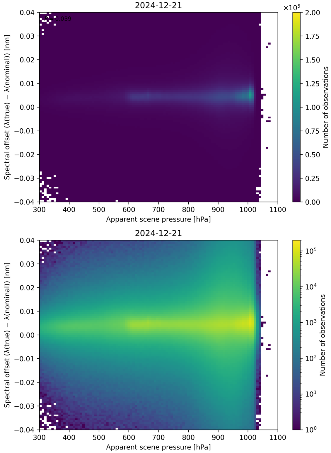
Figure 67: Scatter density plot of “Apparent scene pressure” against “Spectral offset ( \lambda_{\text{true}} - \lambda_{\text{nominal}} )” for 2024-12-20 to 2024-12-22.
