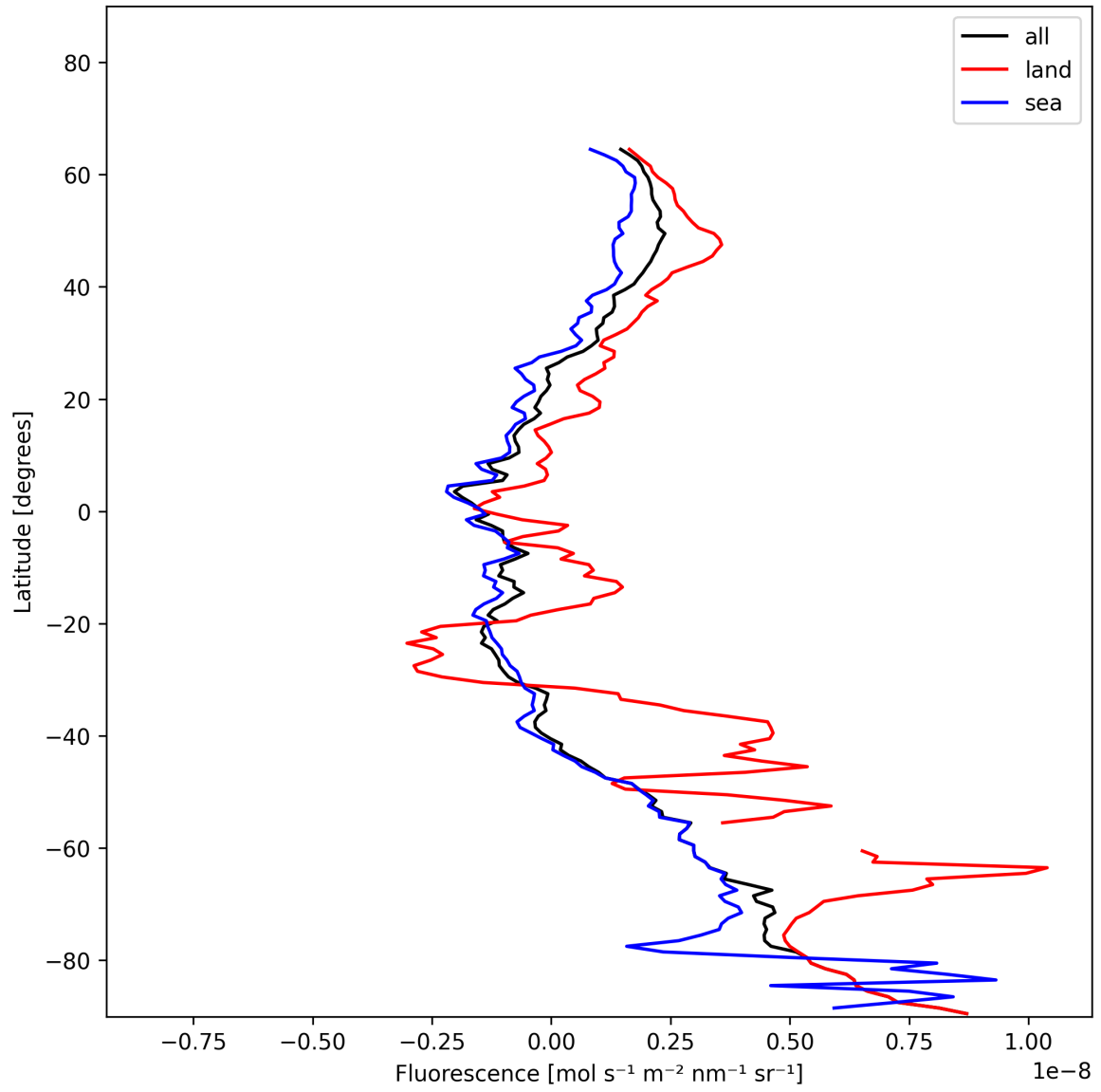
Figure 23: Zonal average of “Fluorescence” for 2024-12-20 to 2024-12-22.
