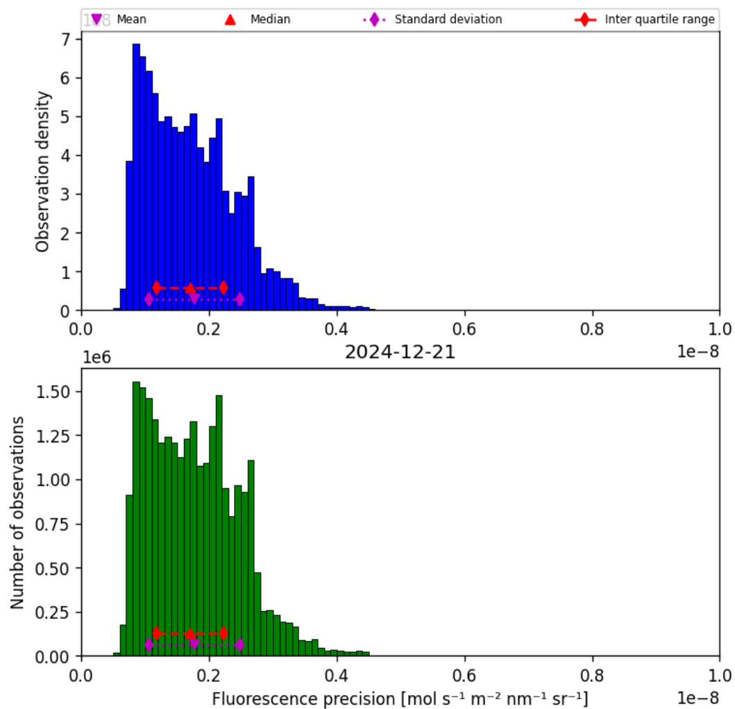
Figure 41: Histogram of “Fluorescence precision” for 2024-12-20 to 2024-12-22
