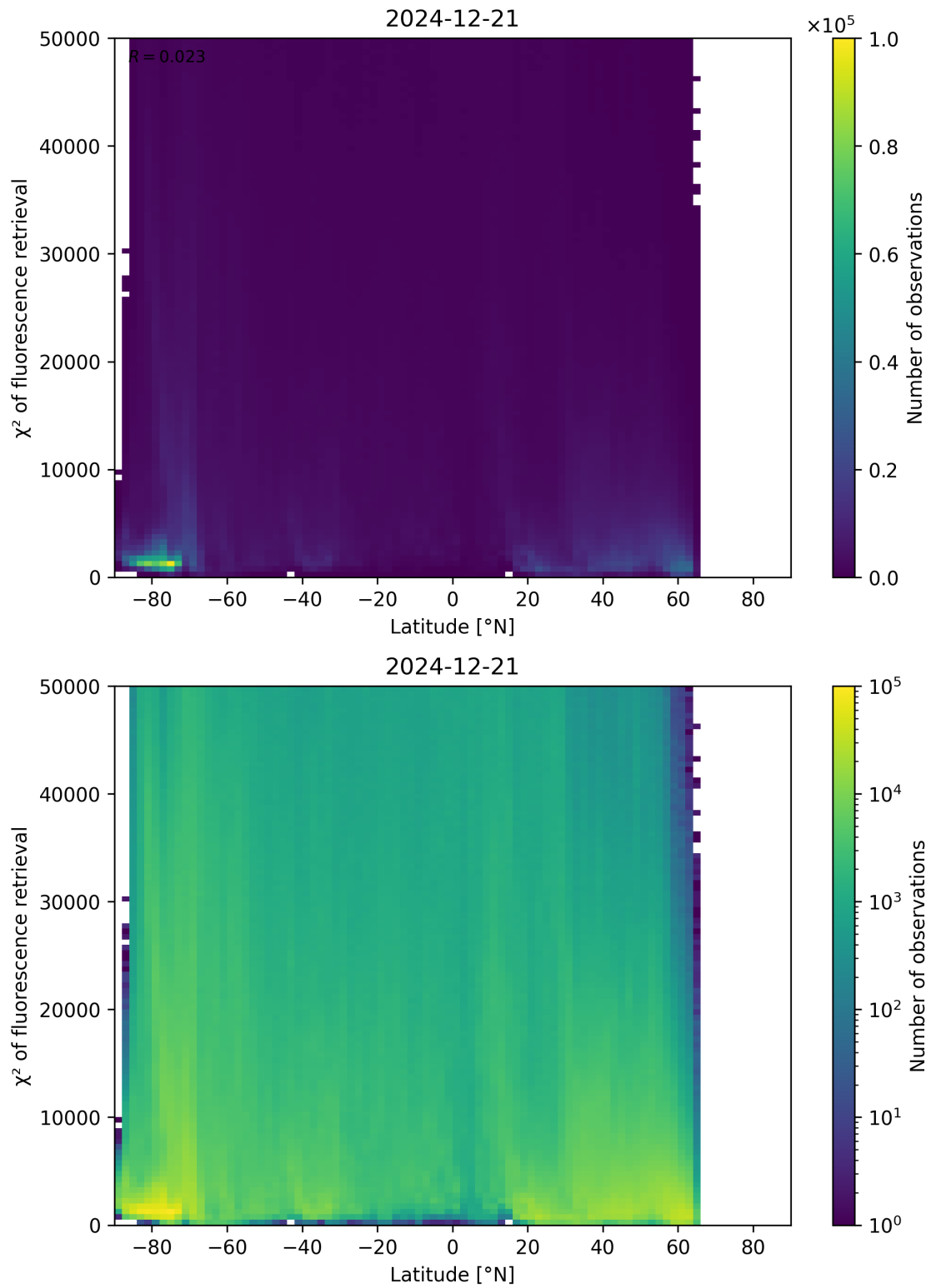
Figure 89: Scatter density plot of “Latitude” against “ \chi^2 of fluorescence retrieval” for 2024-12-20 to 2024-12-22.
