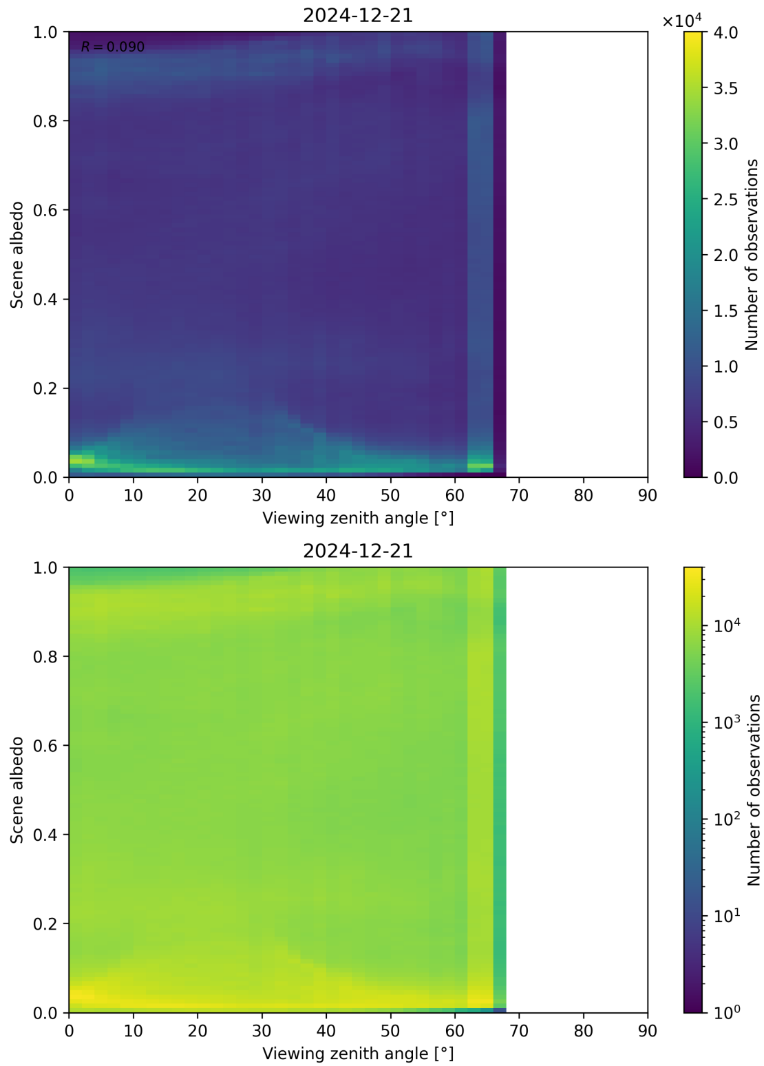
Figure 126: Scatter density plot of “Viewing zenith angle” against “Scene albedo” for 2024-12-20 to 2024-12-22.
