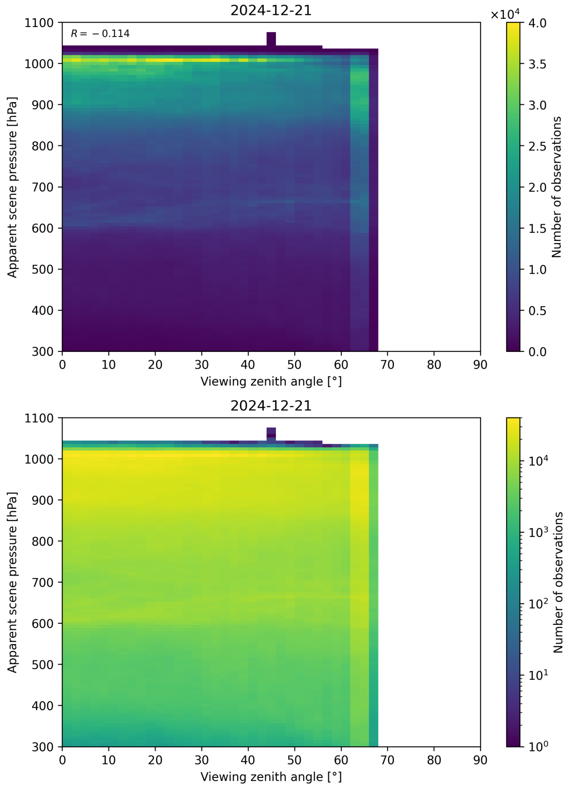
Figure 118: Scatter density plot of “Viewing zenith angle” against “Apparent scene pressure” for 2024-12-20 to 2024-12-22.
