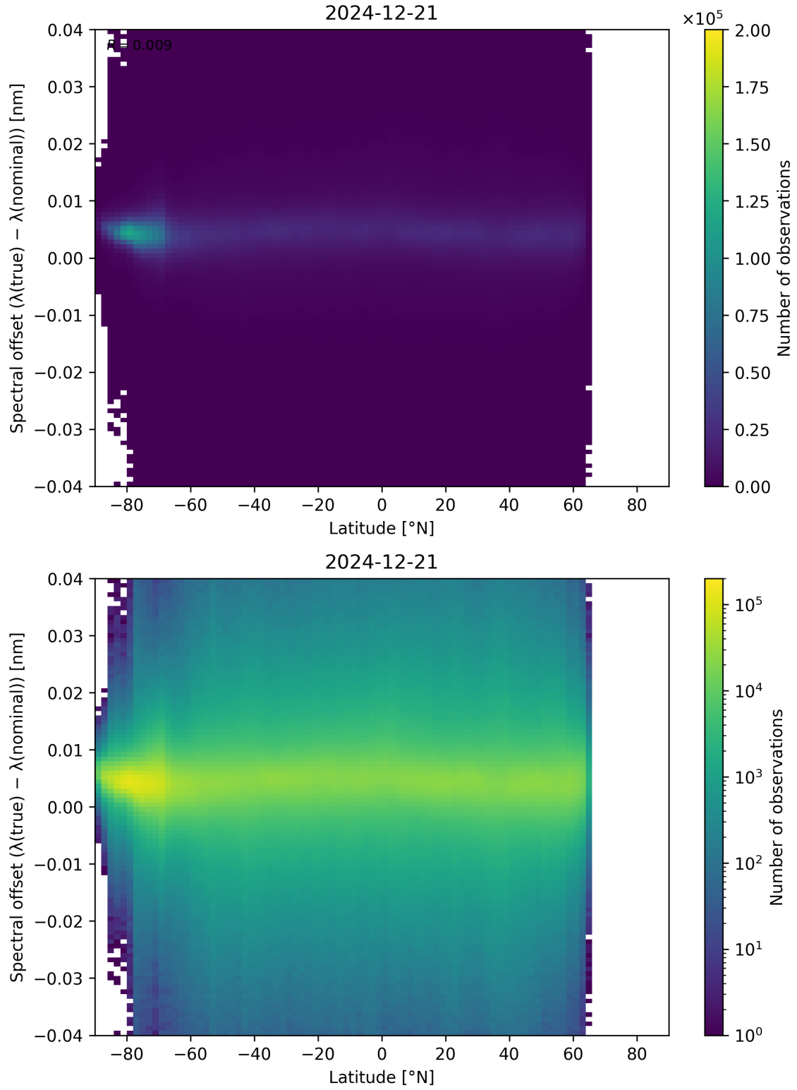
Figure 96: Scatter density plot of “Latitude” against “Spectral offset ( \lambda_{\text{true}} - \lambda_{\text{nominal}} )” for 2024-12-20 to 2024-12-22.
