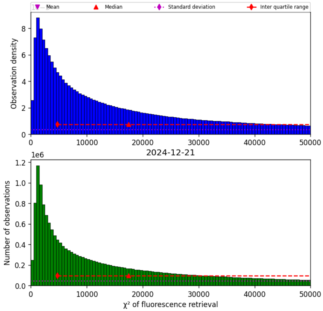
Figure 42: Histogram of “ \chi^2 of fluorescence retrieval” for 2024-12-20 to 2024-12-22
