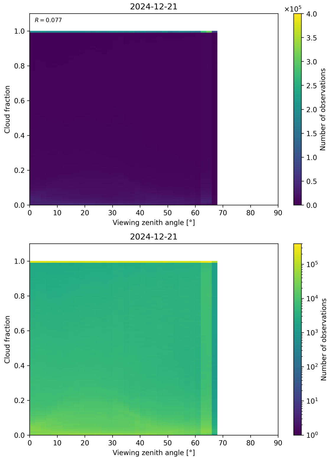
Figure 120: Scatter density plot of “Viewing zenith angle” against “Cloud fraction” for 2024-12-20 to 2024-12-22.
