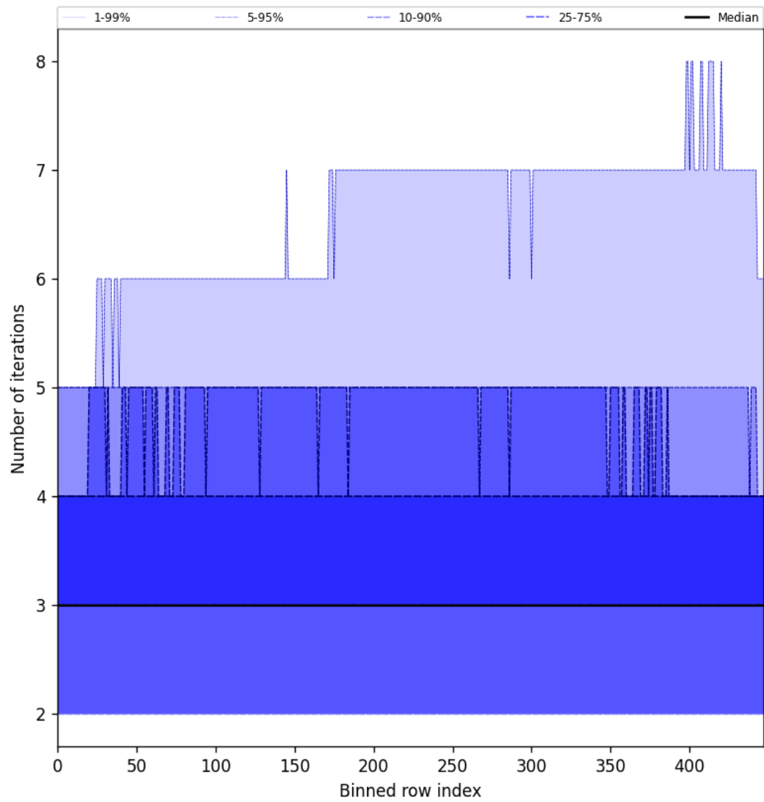
Figure 56: Along track statistics of “Number of iterations” for 2024-12-20 to 2024-12-22
