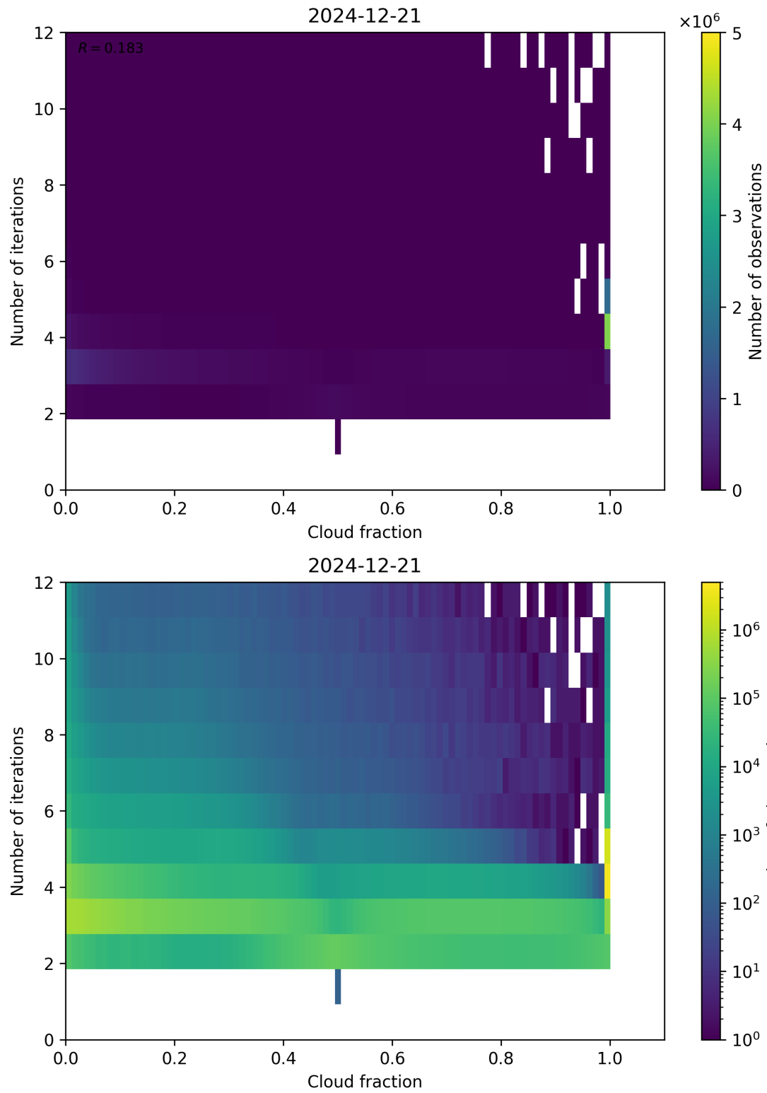
Figure 73: Scatter density plot of “Cloud fraction” against “Number of iterations” for 2024-12-20 to 2024-12-22.
