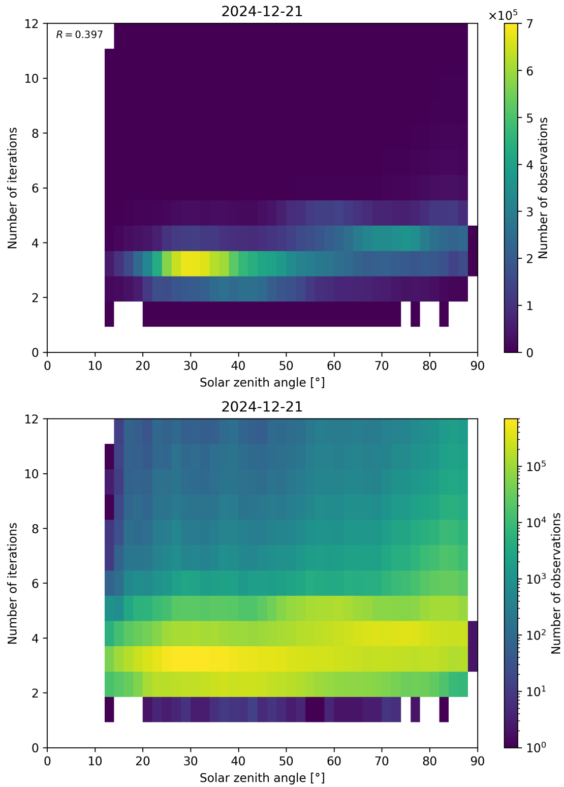
Figure 114: Scatter density plot of “Solar zenith angle” against “Number of iterations” for 2024-12-20 to 2024-12-22.
