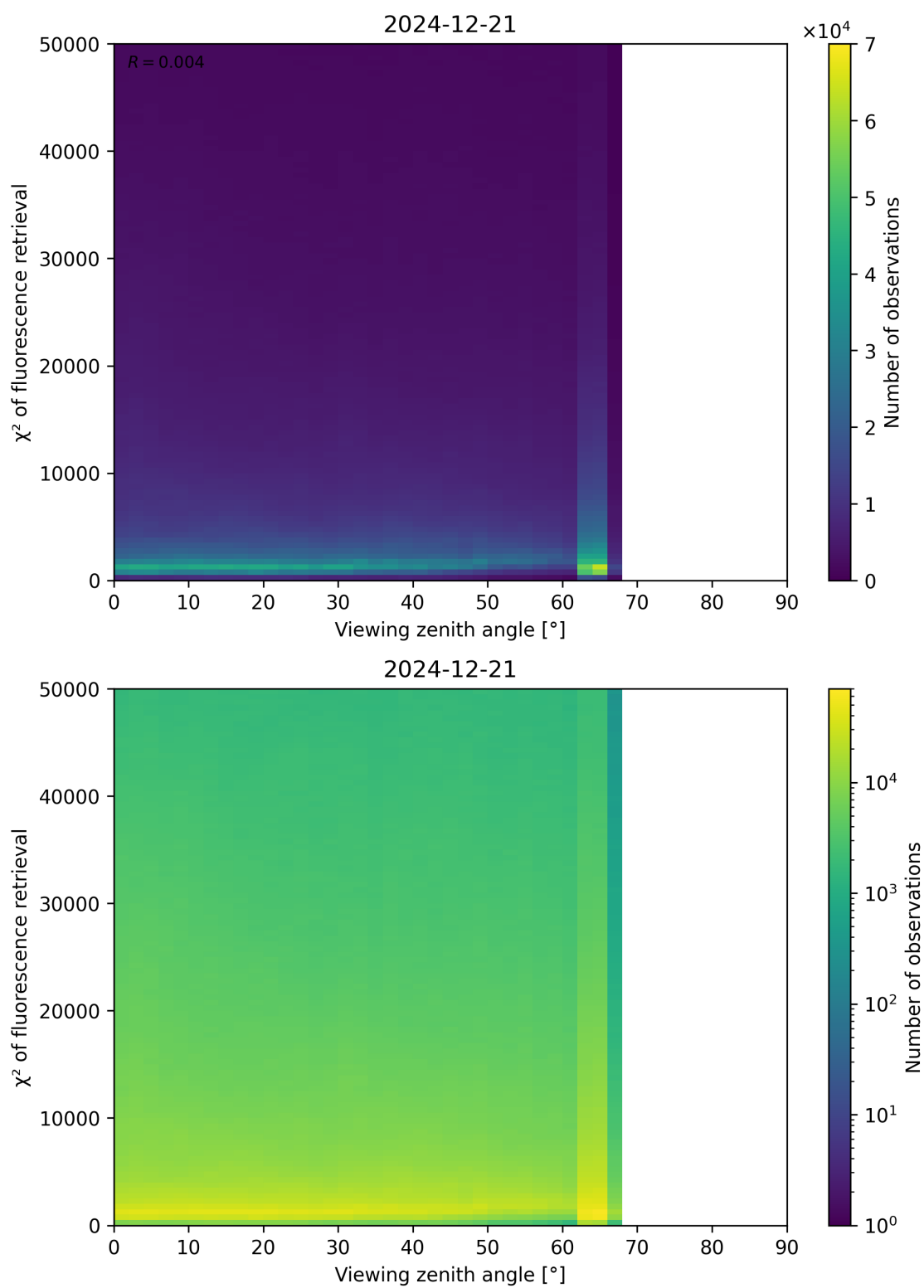
Figure 119: Scatter density plot of “Viewing zenith angle” against “ \chi^2 of fluorescence retrieval” for 2024-12-20 to 2024-12-22.
