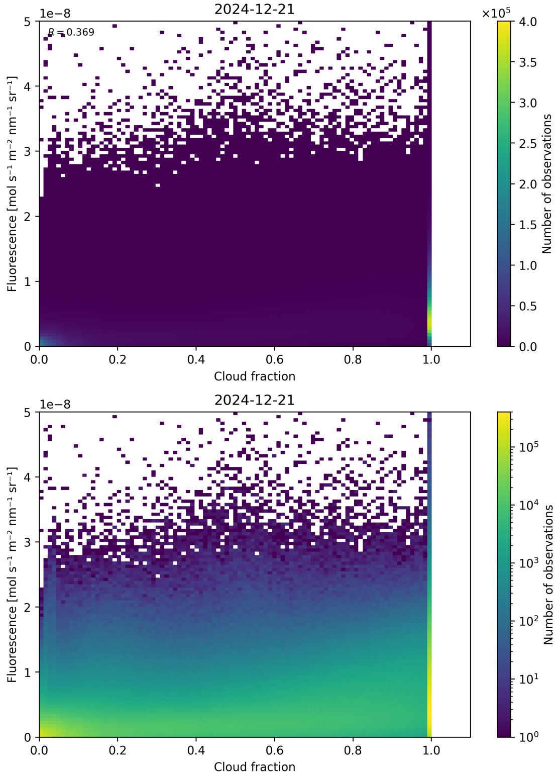
Figure 72: Scatter density plot of “Cloud fraction” against “Fluorescence” for 2024-12-20 to 2024-12-22.
