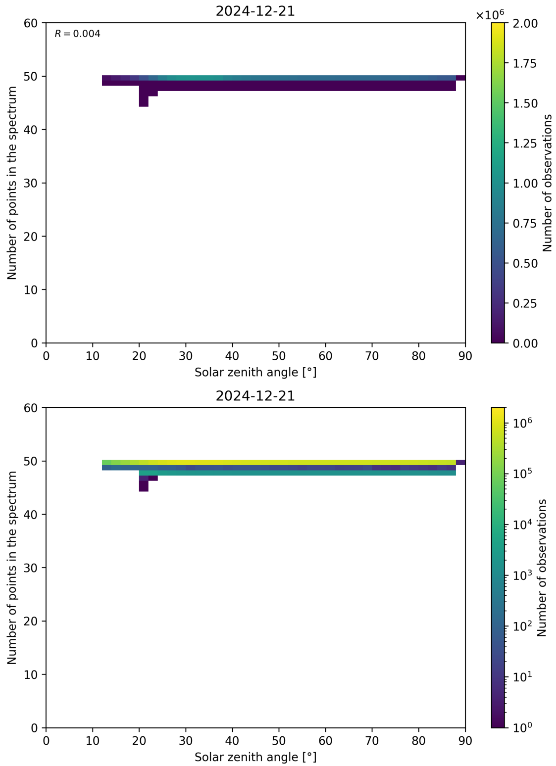
Figure 115: Scatter density plot of “Solar zenith angle” against “Number of points in the spectrum” for 2024-12-20 to 2024-12-22.
