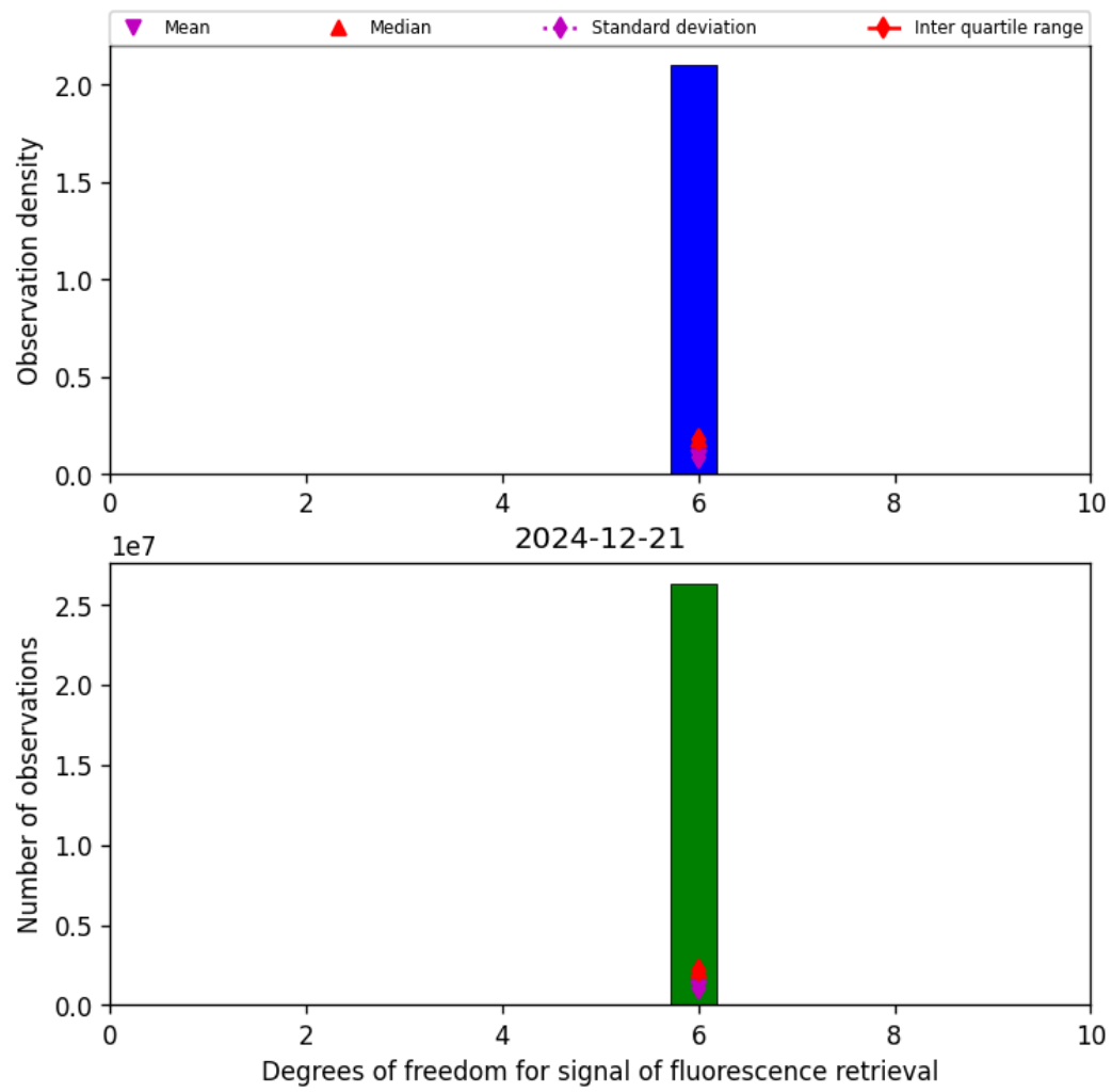
Figure 43: Histogram of "Degrees of freedom for signal of fluorescence retrieval" for 2024-12-20 to 2024-12-22
