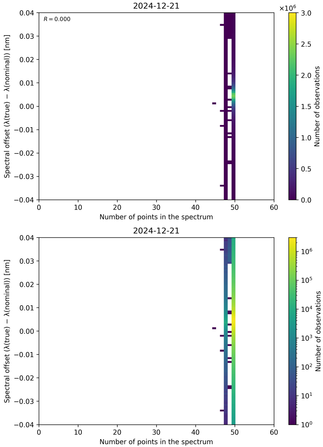
Figure 101: Scatter density plot of “Number of points in the spectrum” against “Spectral offset ( \lambda_{\text{true}} - \lambda_{\text{nominal}} )” for 2024-12-20 to 2024-12-22.
