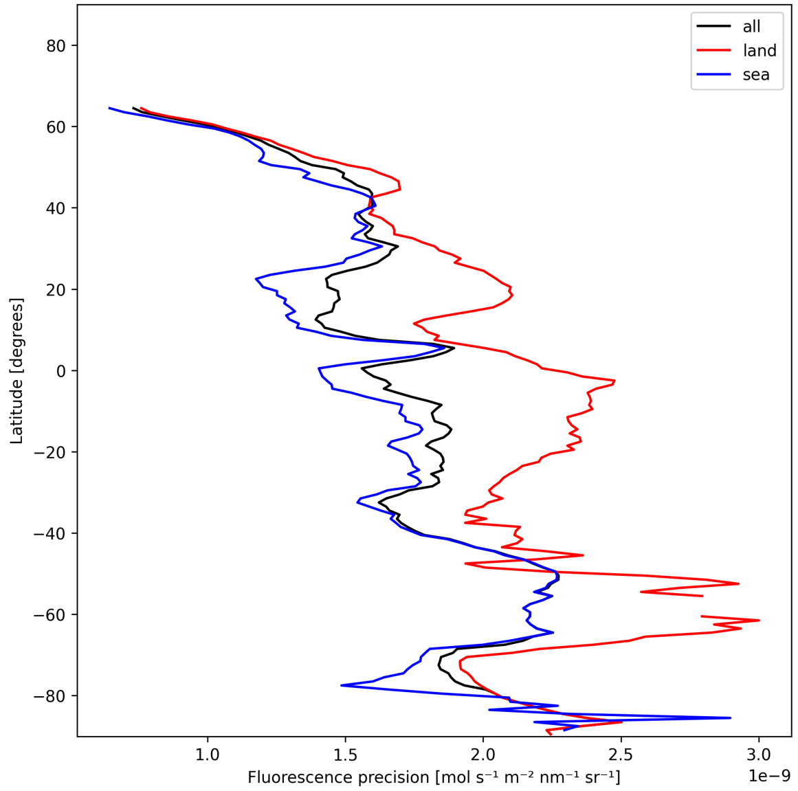
Figure 24: Zonal average of “Fluorescence precision” for 2024-12-20 to 2024-12-22.
