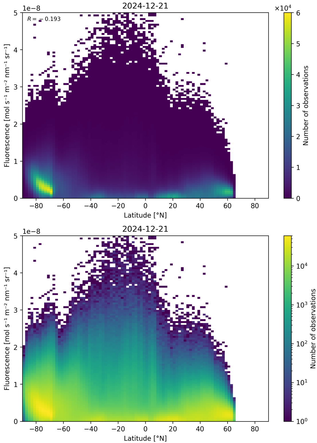
Figure 92: Scatter density plot of “Latitude” against “Fluorescence” for 2024-12-20 to 2024-12-22.
