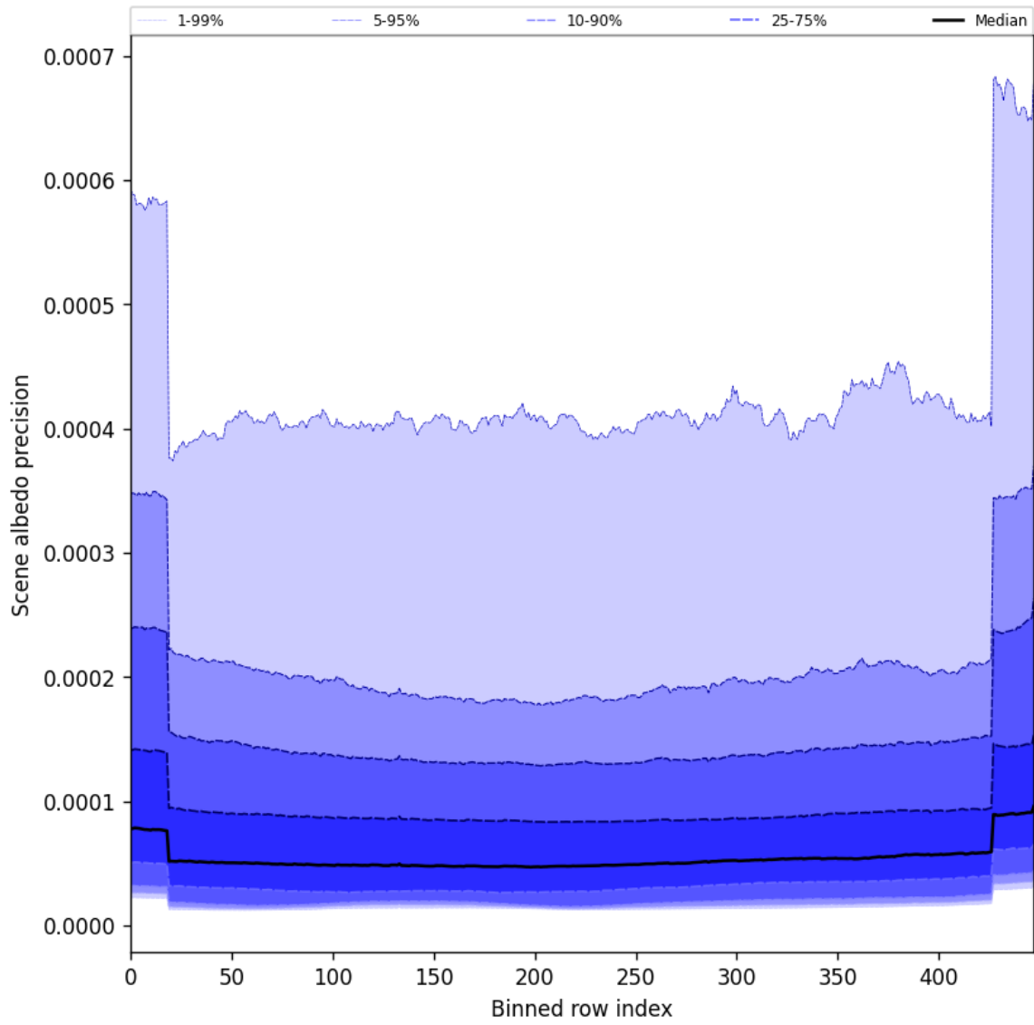
Figure 52: Along track statistics of “Scene albedo precision” for 2024-12-20 to 2024-12-22
