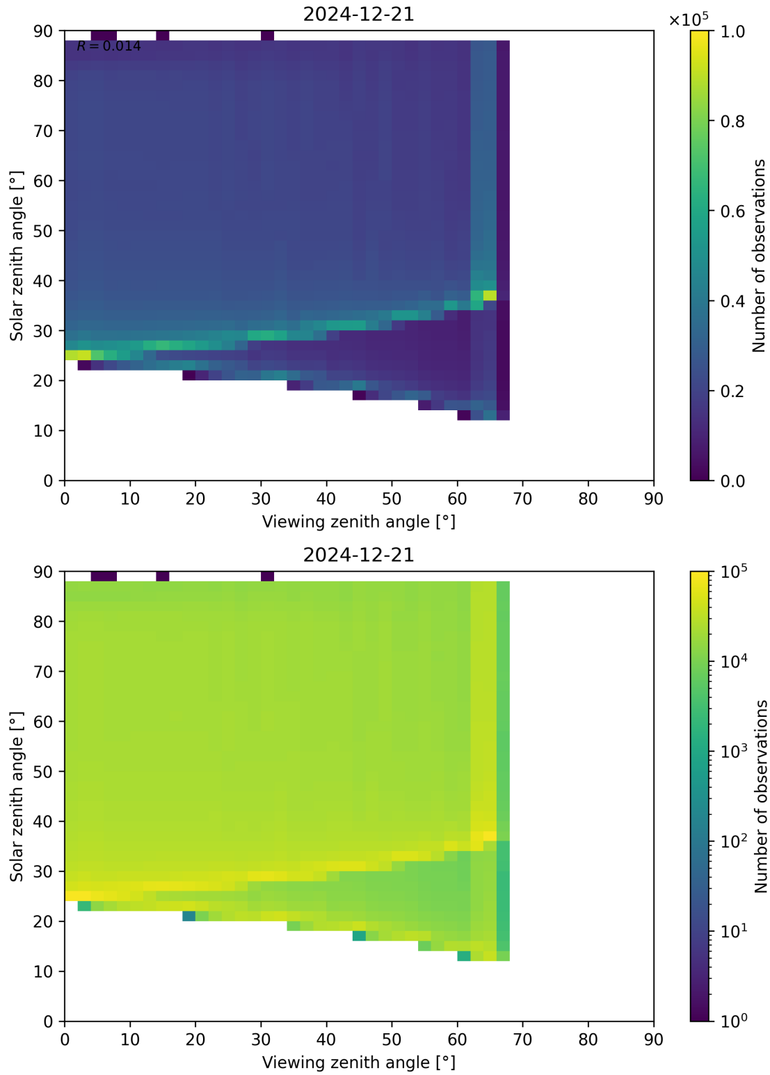
Figure 127: Scatter density plot of “Viewing zenith angle” against “Solar zenith angle” for 2024-12-20 to 2024-12-22.
