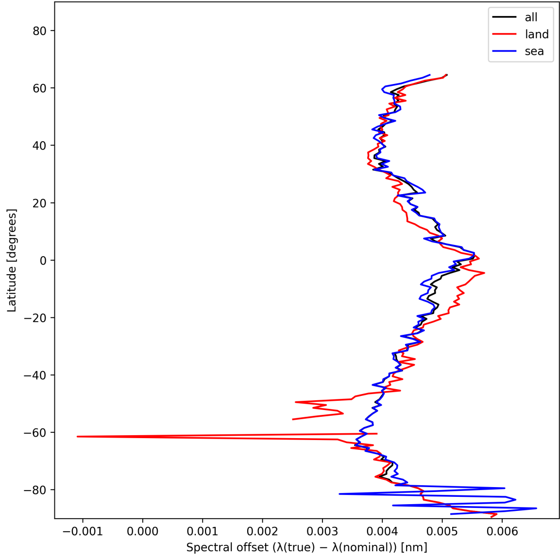
Figure 28: Zonal average of “Spectral offset ( \lambda_{\text{true}} - \lambda_{\text{nominal}} )” for 2024-12-20 to 2024-12-22.
