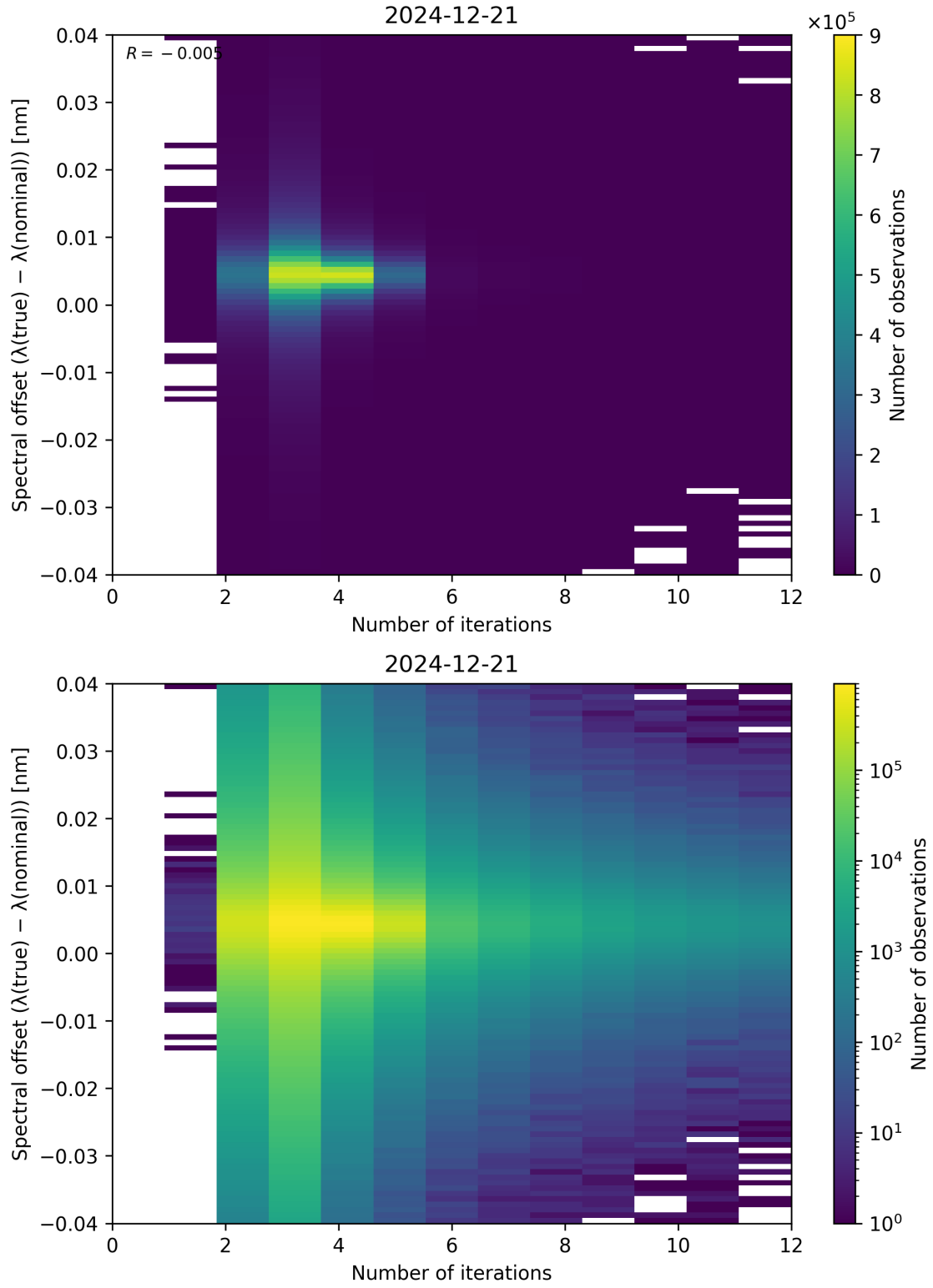
Figure 100: Scatter density plot of “Number of iterations” against “Spectral offset ( \lambda_{\text{true}} - \lambda_{\text{nominal}} )” for 2024-12-20 to 2024-12-22.
