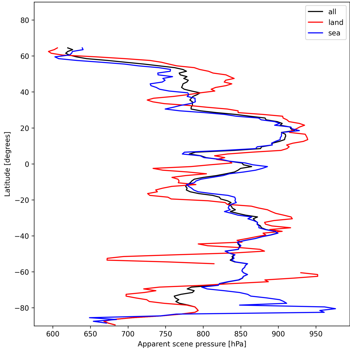
Figure 19: Zonal average of “Apparent scene pressure” for 2024-12-20 to 2024-12-22.
