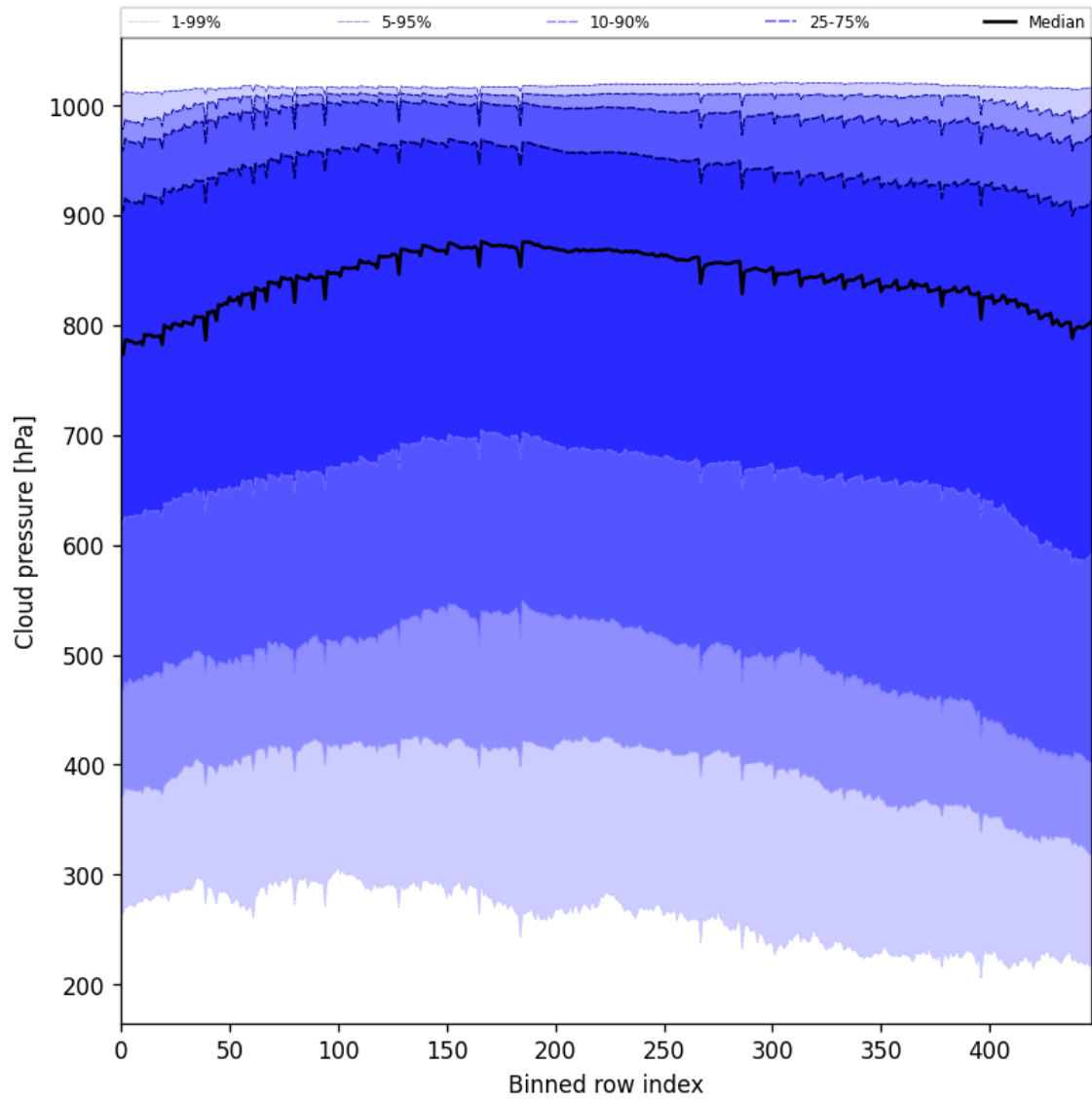
Figure 47: Along track statistics of “Cloud pressure” for 2024-12-20 to 2024-12-22
