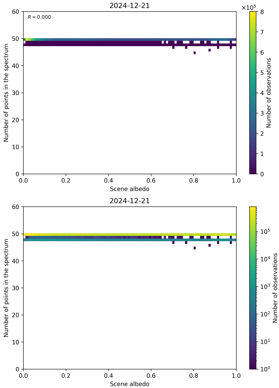
Figure 106: Scatter density plot of “Scene albedo” against “Number of points in the spectrum” for 2024-12-20 to 2024-12-22.
