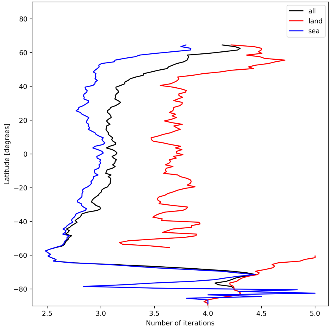
Figure 22: Zonal average of “Number of iterations” for 2024-12-20 to 2024-12-22.
