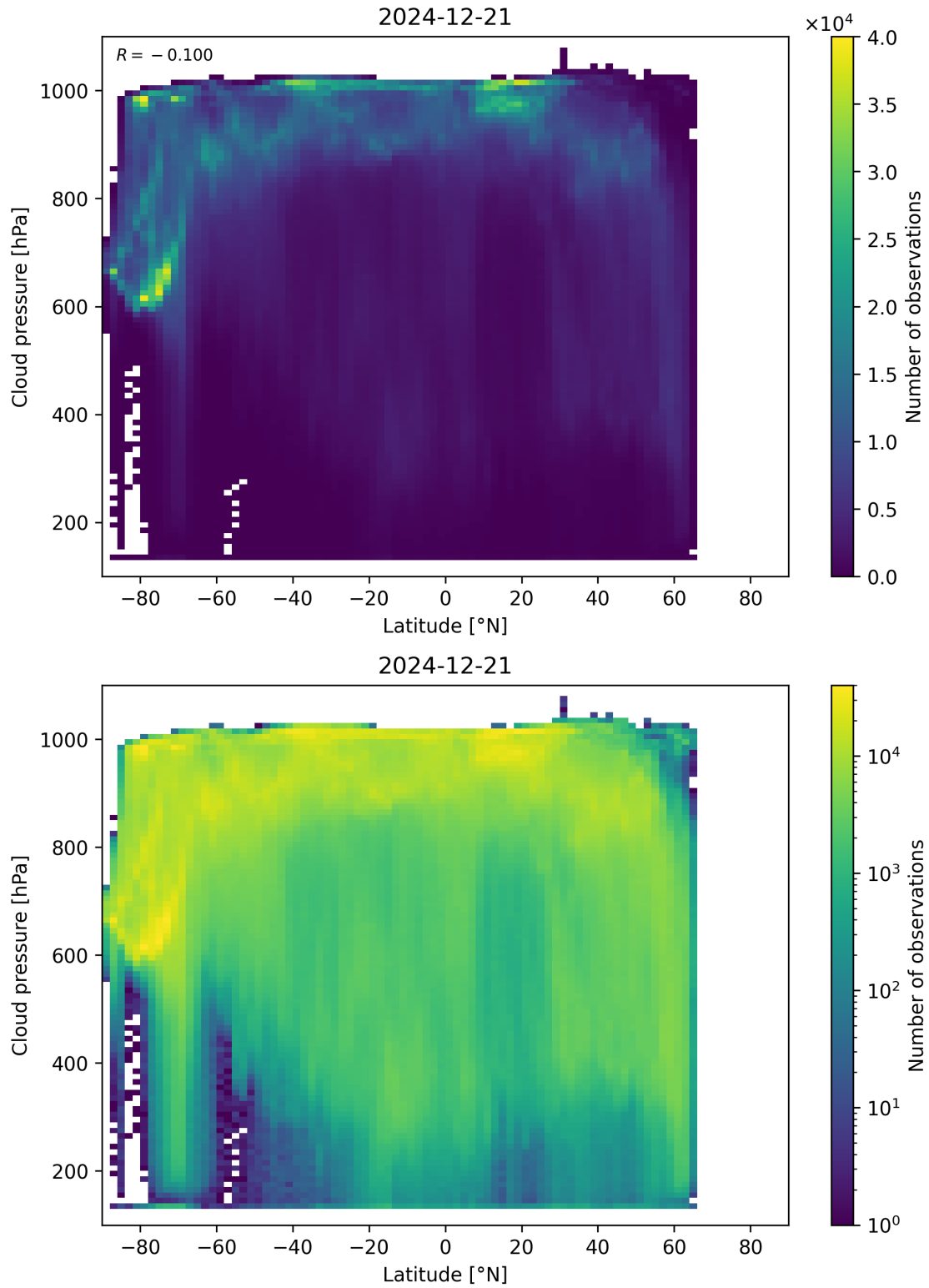
Figure 91: Scatter density plot of “Latitude” against “Cloud pressure” for 2024-12-20 to 2024-12-22.
