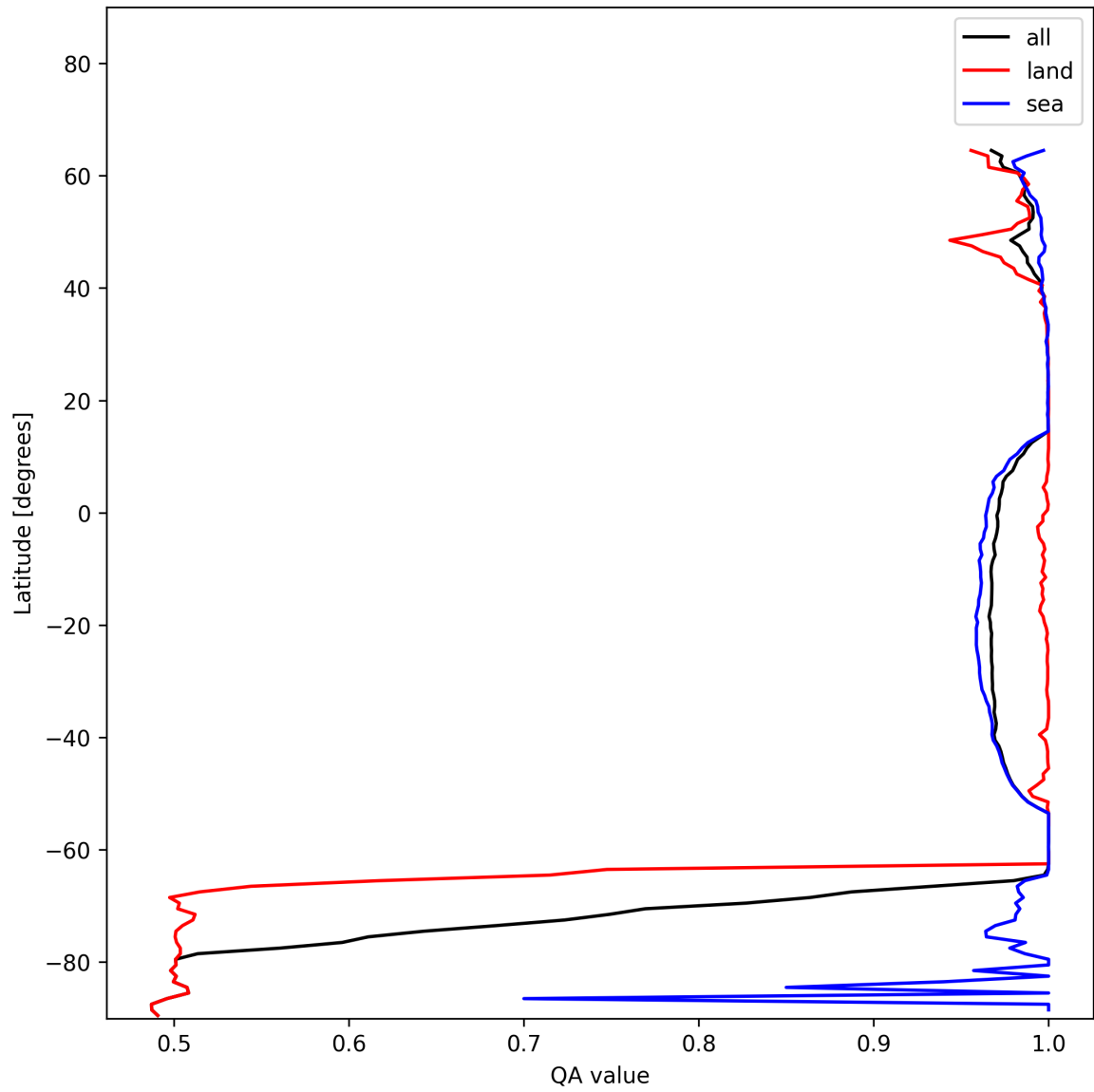
Figure 12: Zonal average of “QA value” for 2024-12-20 to 2024-12-22.
