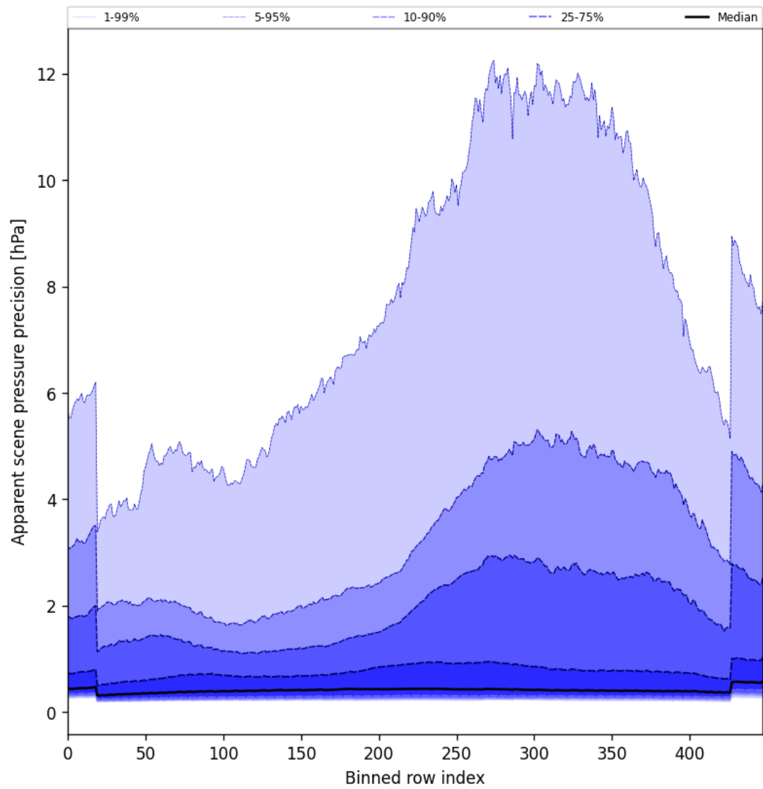
Figure 54: Along track statistics of “Apparent scene pressure precision” for 2024-12-20 to 2024-12-22
