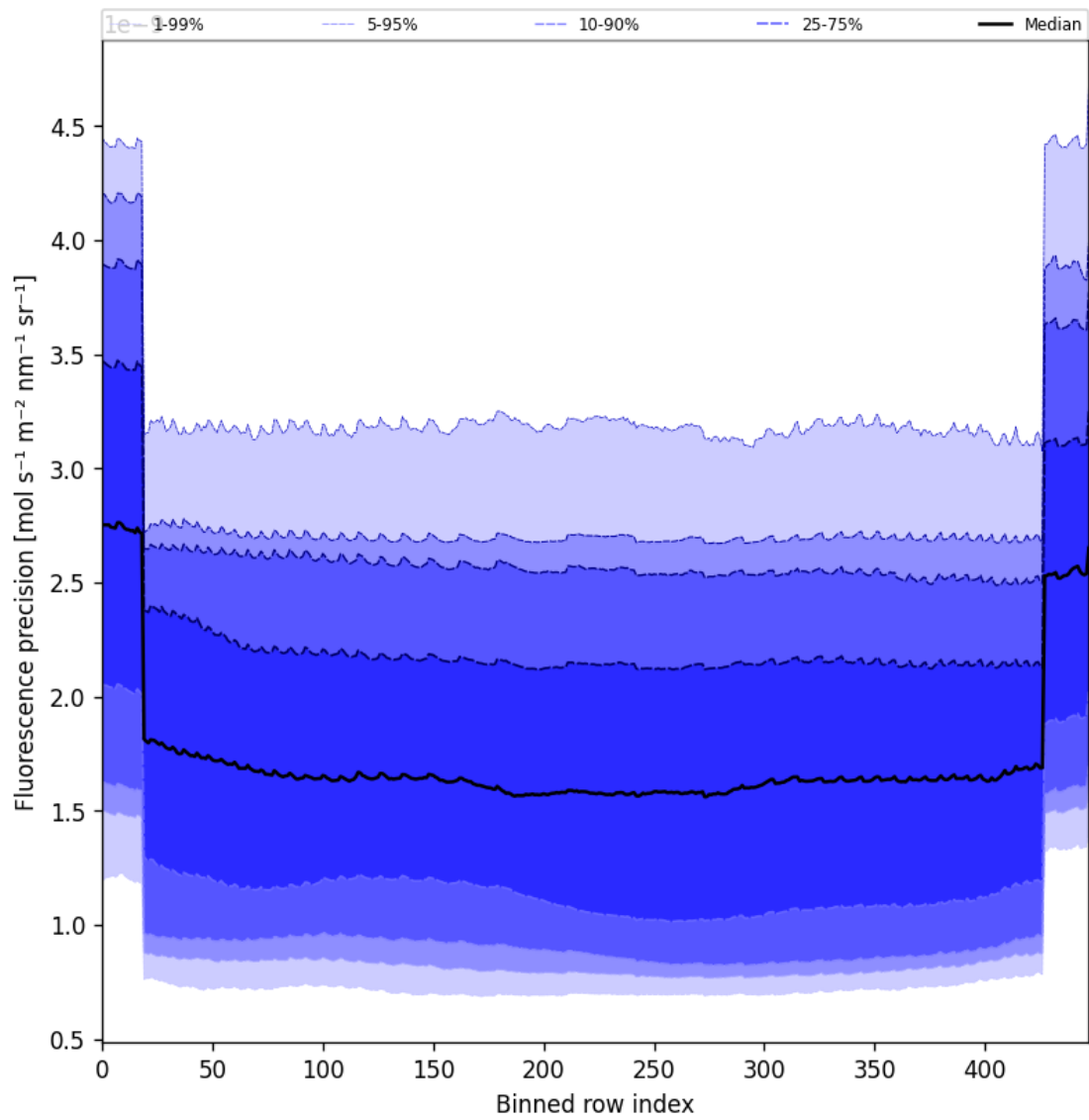
Figure 58: Along track statistics of “Fluorescence precision” for 2024-12-20 to 2024-12-22
