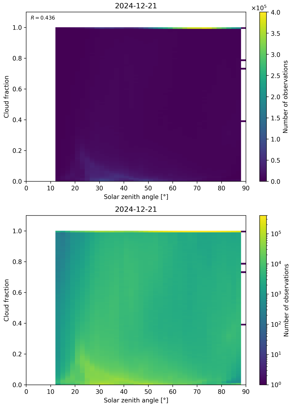
Figure 110: Scatter density plot of “Solar zenith angle” against “Cloud fraction” for 2024-12-20 to 2024-12-22.
