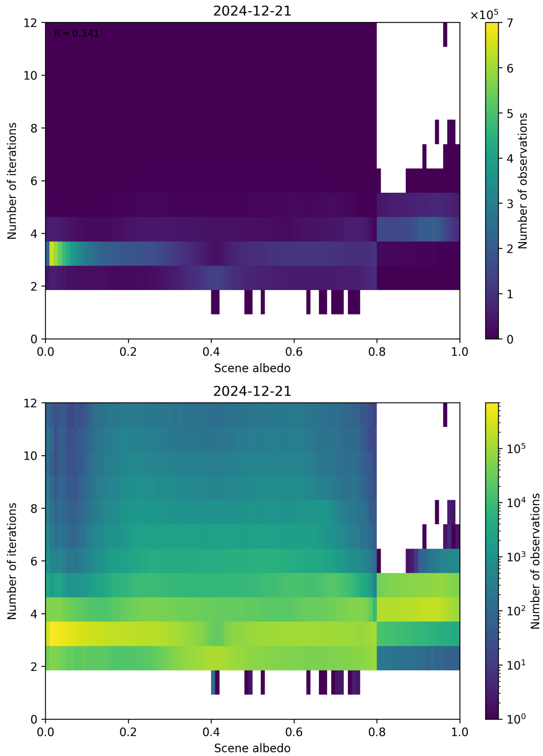
Figure 105: Scatter density plot of “Scene albedo” against “Number of iterations” for 2024-12-20 to 2024-12-22.
