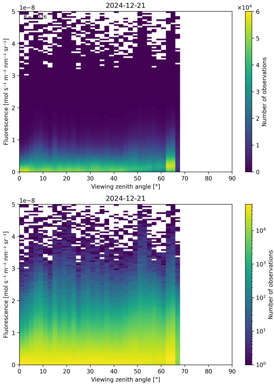
Figure 122: Scatter density plot of “Viewing zenith angle” against “Fluorescence” for 2024-12-20 to 2024-12-22.
