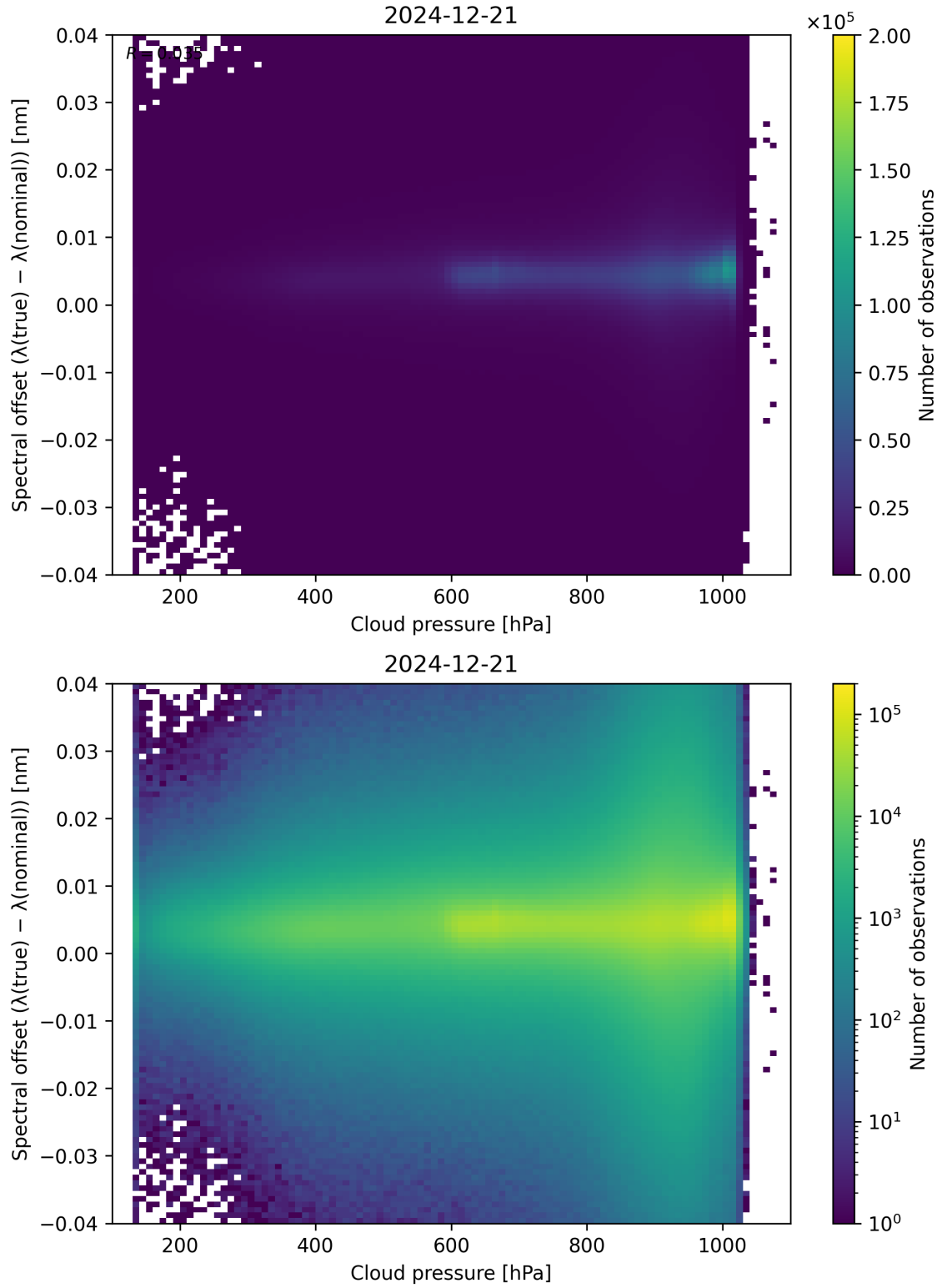
Figure 84: Scatter density plot of “Cloud pressure” against “Spectral offset ( \lambda_{\text{true}} - \lambda_{\text{nominal}} )” for 2024-12-20 to 2024-12-22.
