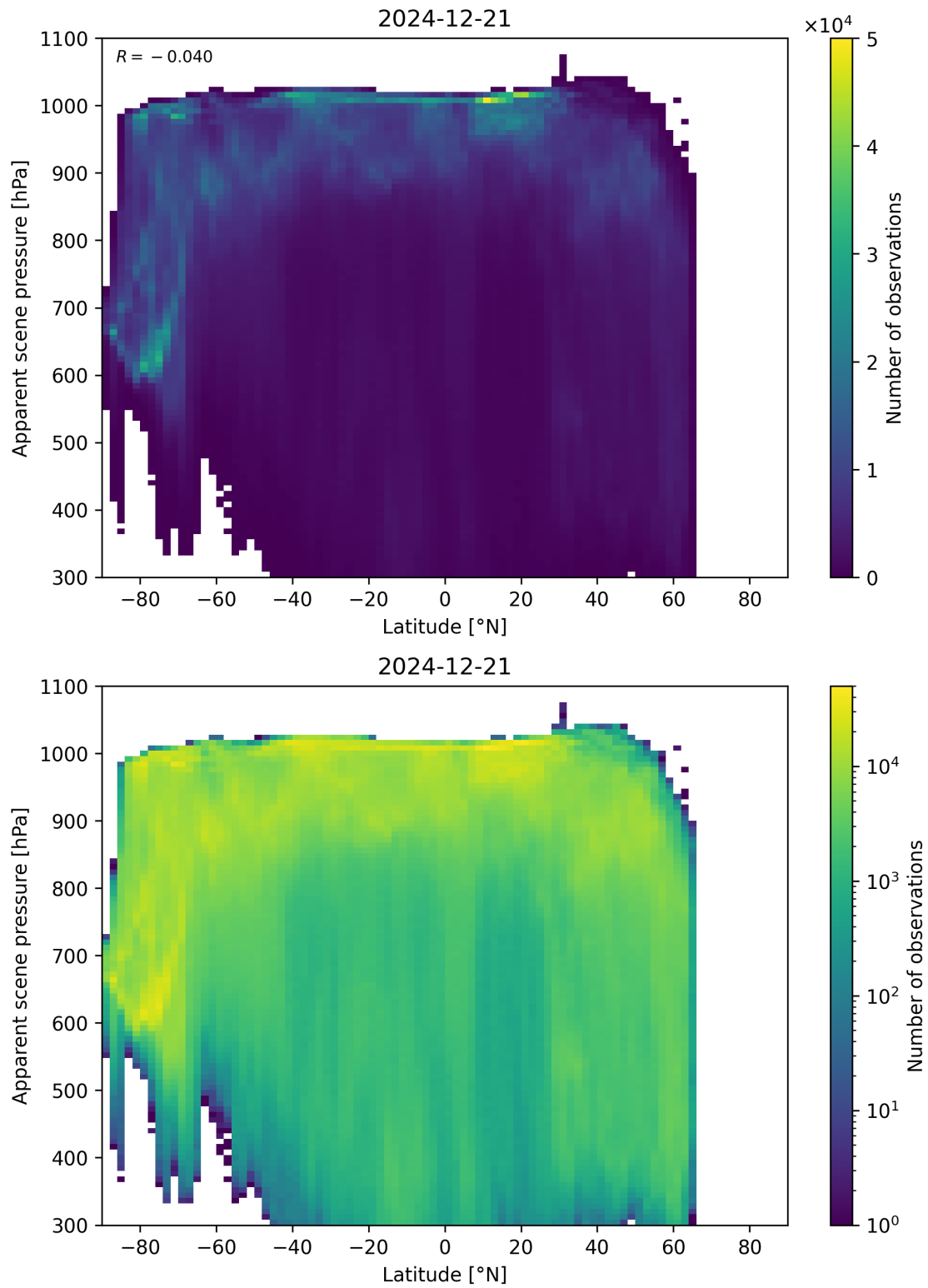
Figure 88: Scatter density plot of “Latitude” against “Apparent scene pressure” for 2024-12-20 to 2024-12-22.
