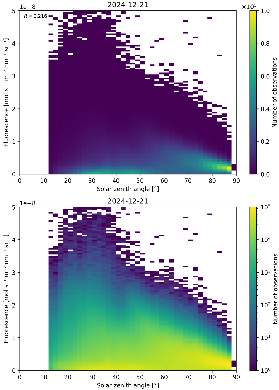
Figure 112: Scatter density plot of “Solar zenith angle” against “Fluorescence” for 2024-12-20 to 2024-12-22.
