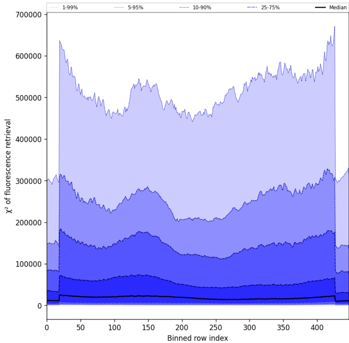
Figure 59: Along track statistics of “ \chi^2 of fluorescence retrieval” for 2024-12-20 to 2024-12-22
