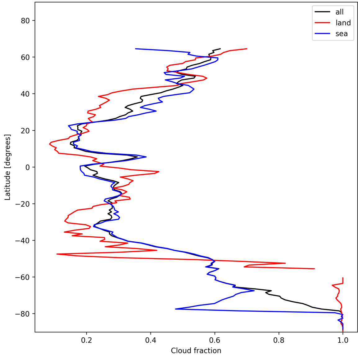
Figure 15: Zonal average of “Cloud fraction” for 2024-12-20 to 2024-12-22.
