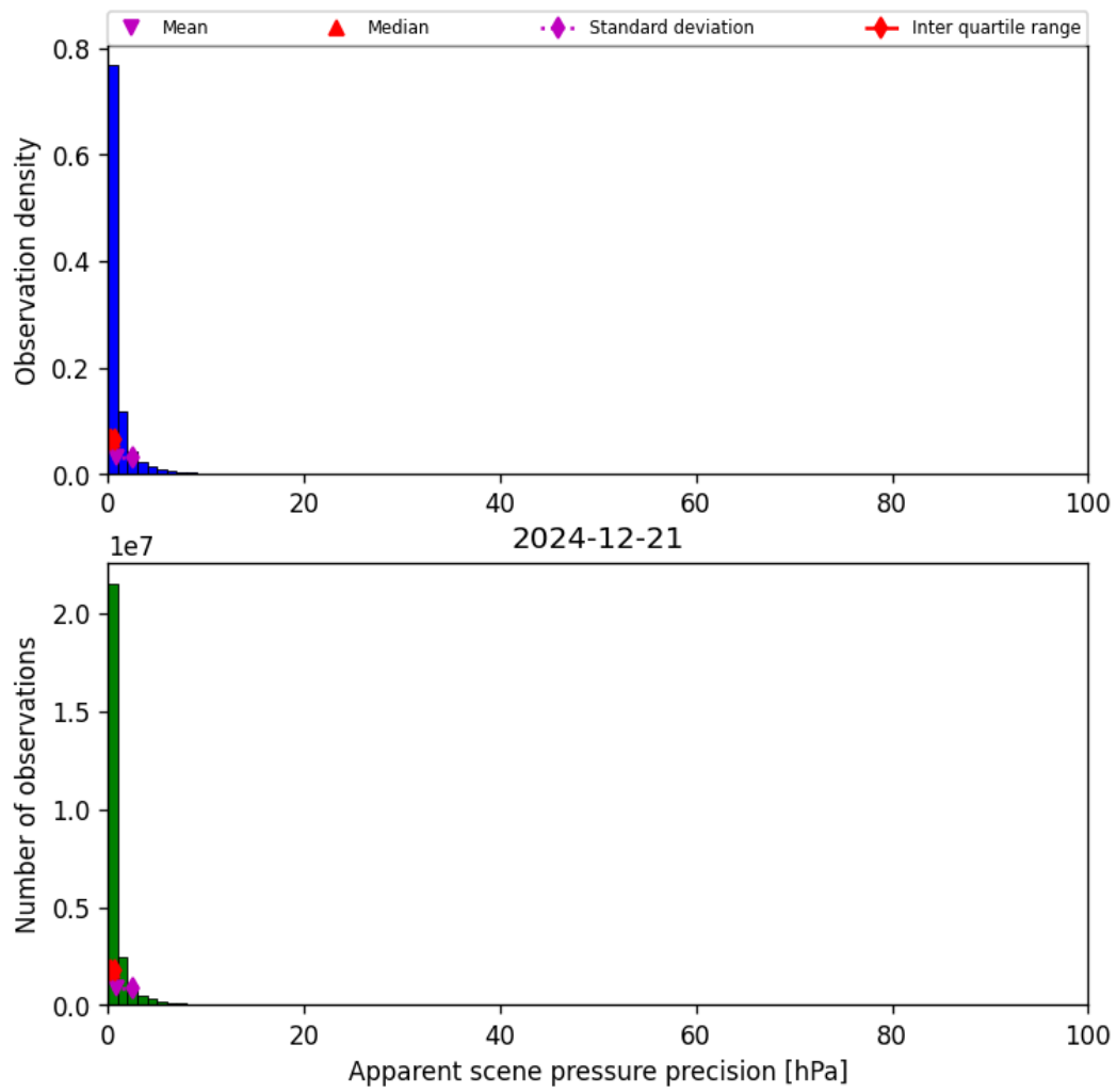
Figure 37: Histogram of “Apparent scene pressure precision” for 2024-12-20 to 2024-12-22
