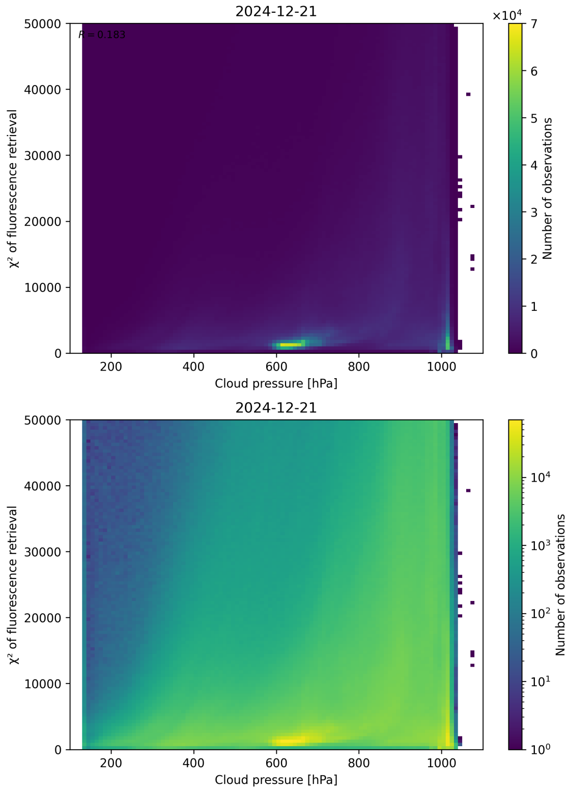
Figure 78: Scatter density plot of “Cloud pressure” against “ \chi^2 of fluorescence retrieval” for 2024-12-20 to 2024-12-22.
