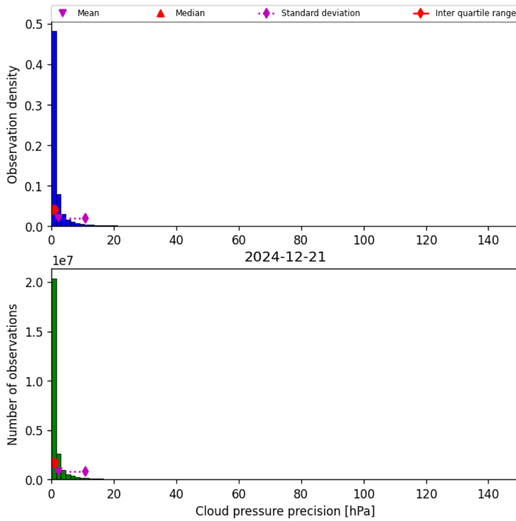
Figure 31: Histogram of “Cloud pressure precision” for 2024-12-20 to 2024-12-22
