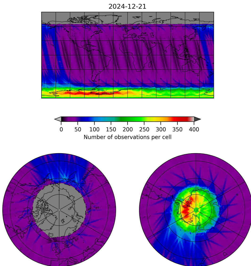
Figure 11: Map of the number of observations for 2024-12-20 to 2024-12-22
