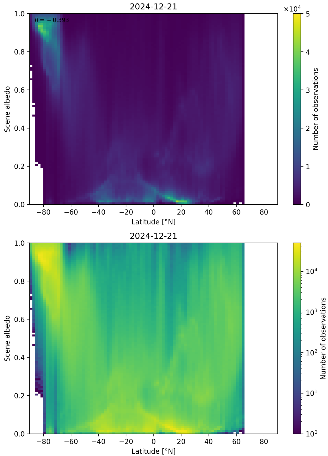
Figure 95: Scatter density plot of “Latitude” against “Scene albedo” for 2024-12-20 to 2024-12-22.
