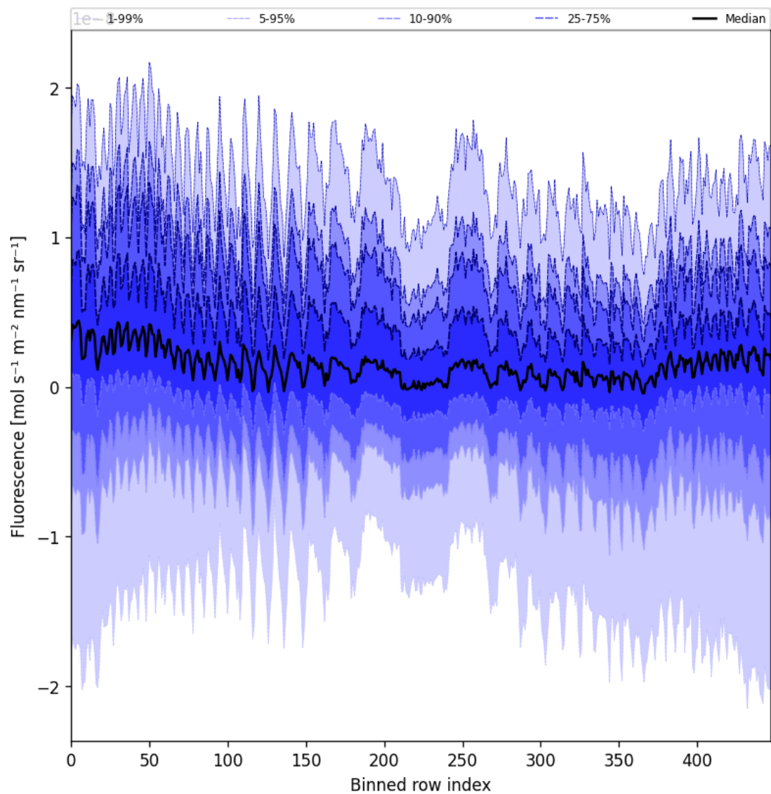
Figure 57: Along track statistics of “Fluorescence” for 2024-12-20 to 2024-12-22
