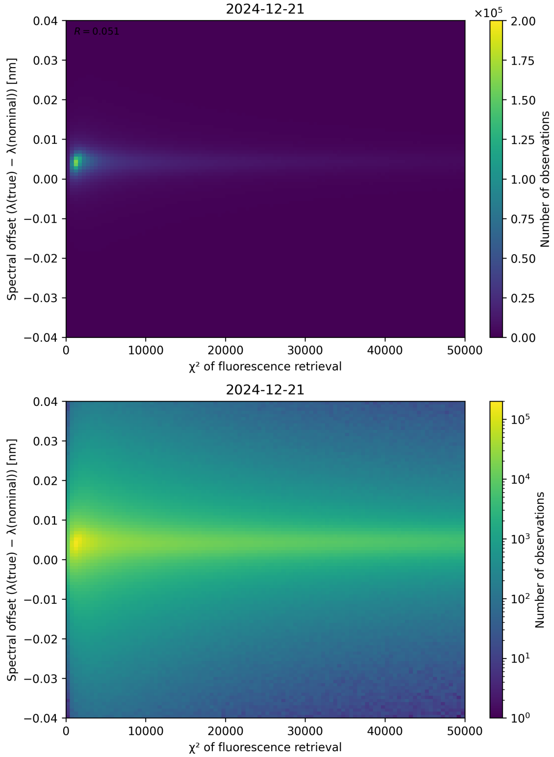
Figure 69: Scatter density plot of “ \chi^2 of fluorescence retrieval” against “Spectral offset ( \lambda_{\text{true}} - \lambda_{\text{nominal}} )” for 2024-12-20 to 2024-12-22.
