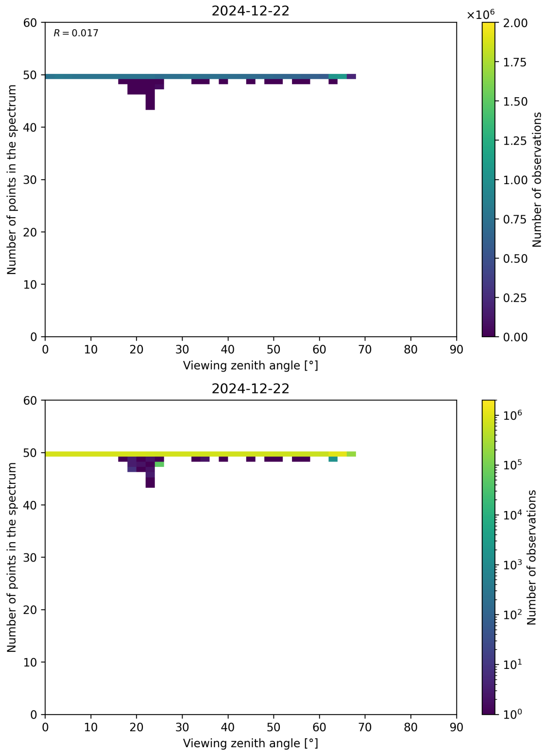
Figure 125: Scatter density plot of “Viewing zenith angle” against “Number of points in the spectrum” for 2024-12-22 to 2024-12-23.
