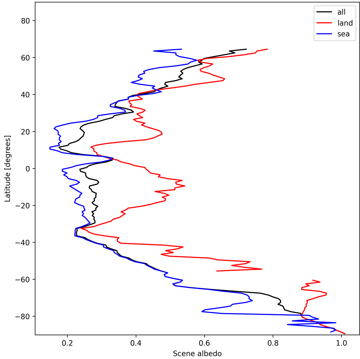
Figure 17: Zonal average of “Scene albedo” for 2024-12-22 to 2024-12-23.
