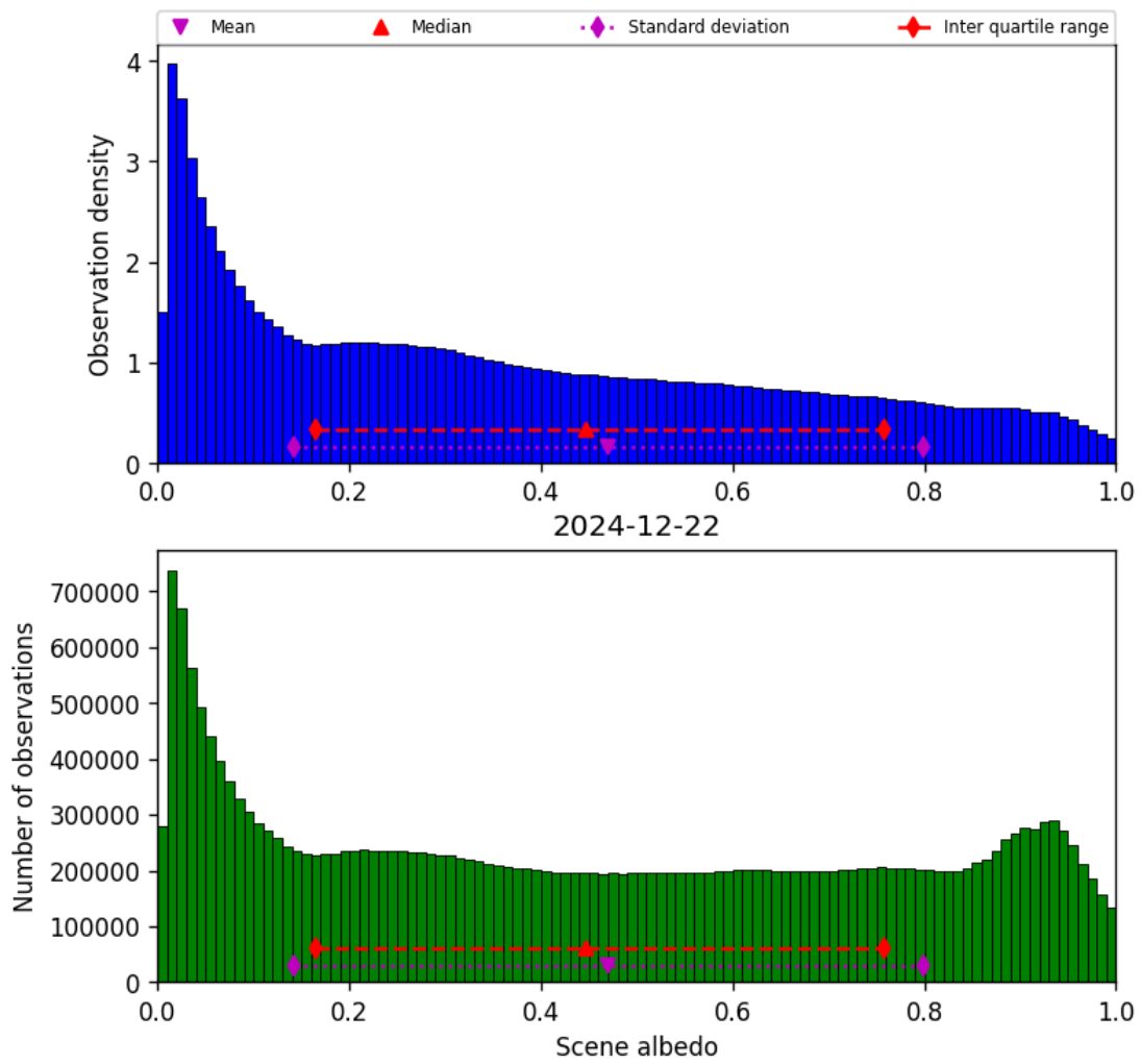
Figure 34: Histogram of “Scene albedo” for 2024-12-22 to 2024-12-23
