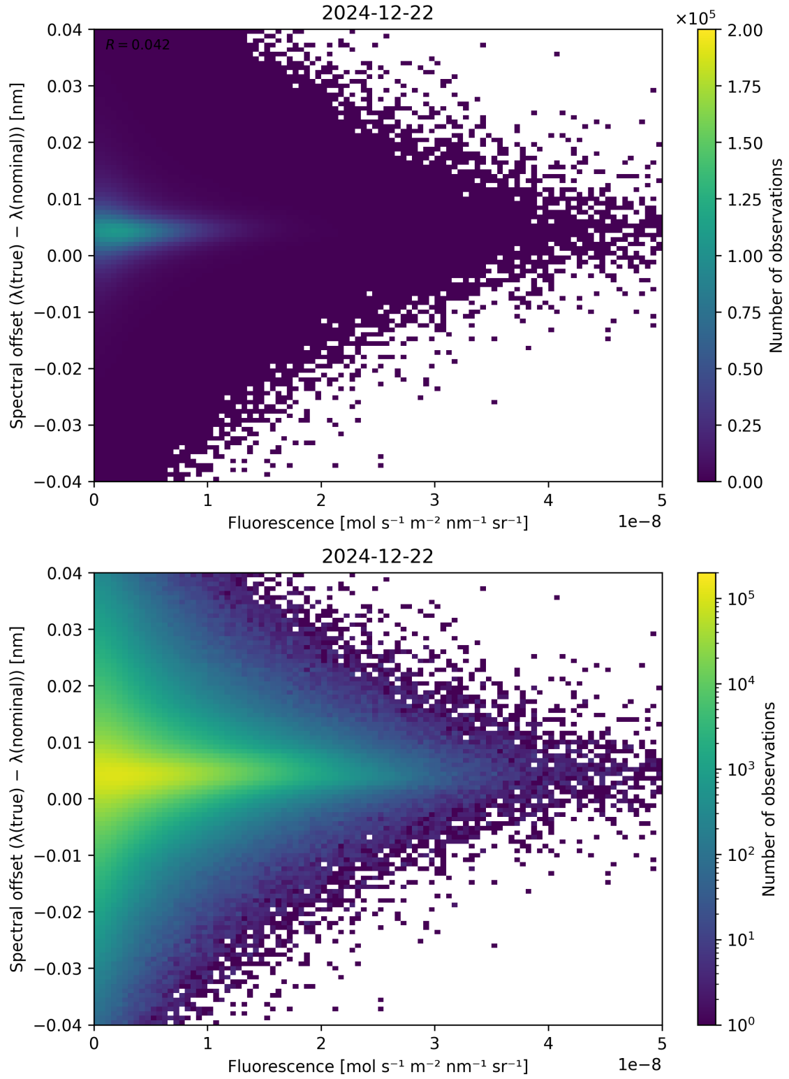
Figure 87: Scatter density plot of “Fluorescence” against “Spectral offset ( \lambda_{\text{true}} - \lambda_{\text{nominal}} )” for 2024-12-22 to 2024-12-23.
