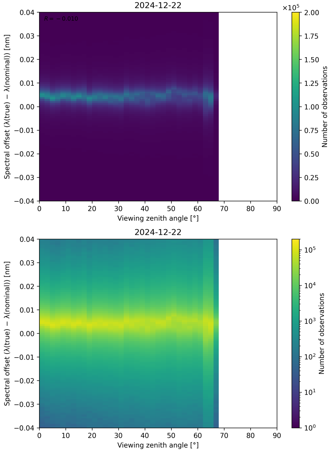
Figure 128: Scatter density plot of “Viewing zenith angle” against “Spectral offset ( \lambda_{\text{true}} - \lambda_{\text{nominal}} )” for 2024-12-22 to 2024-12-23.
