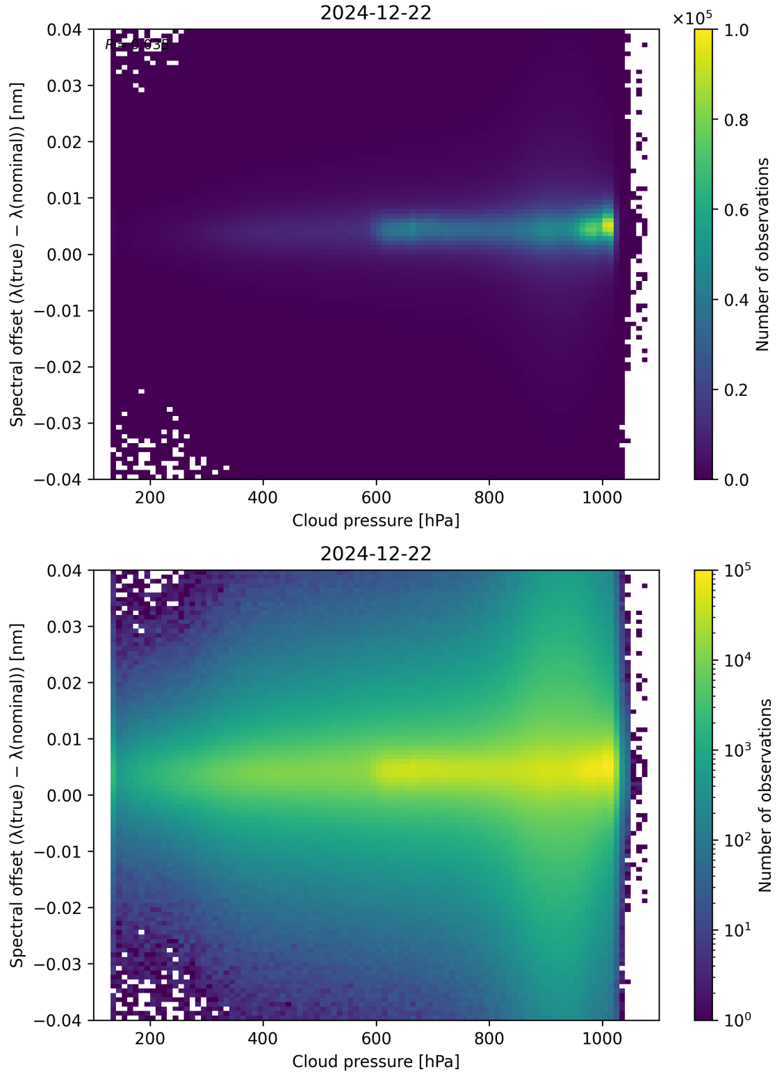
Figure 84: Scatter density plot of “Cloud pressure” against “Spectral offset ( \lambda_{\text{true}} - \lambda_{\text{nominal}} )” for 2024-12-22 to 2024-12-23.
