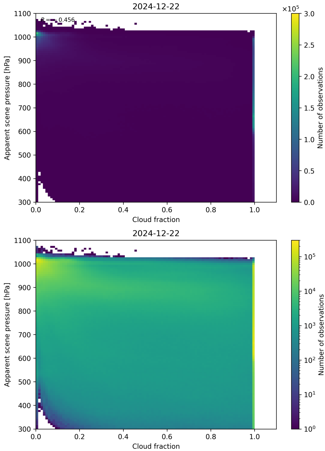
Figure 70: Scatter density plot of “Cloud fraction” against “Apparent scene pressure” for 2024-12-22 to 2024-12-23.
