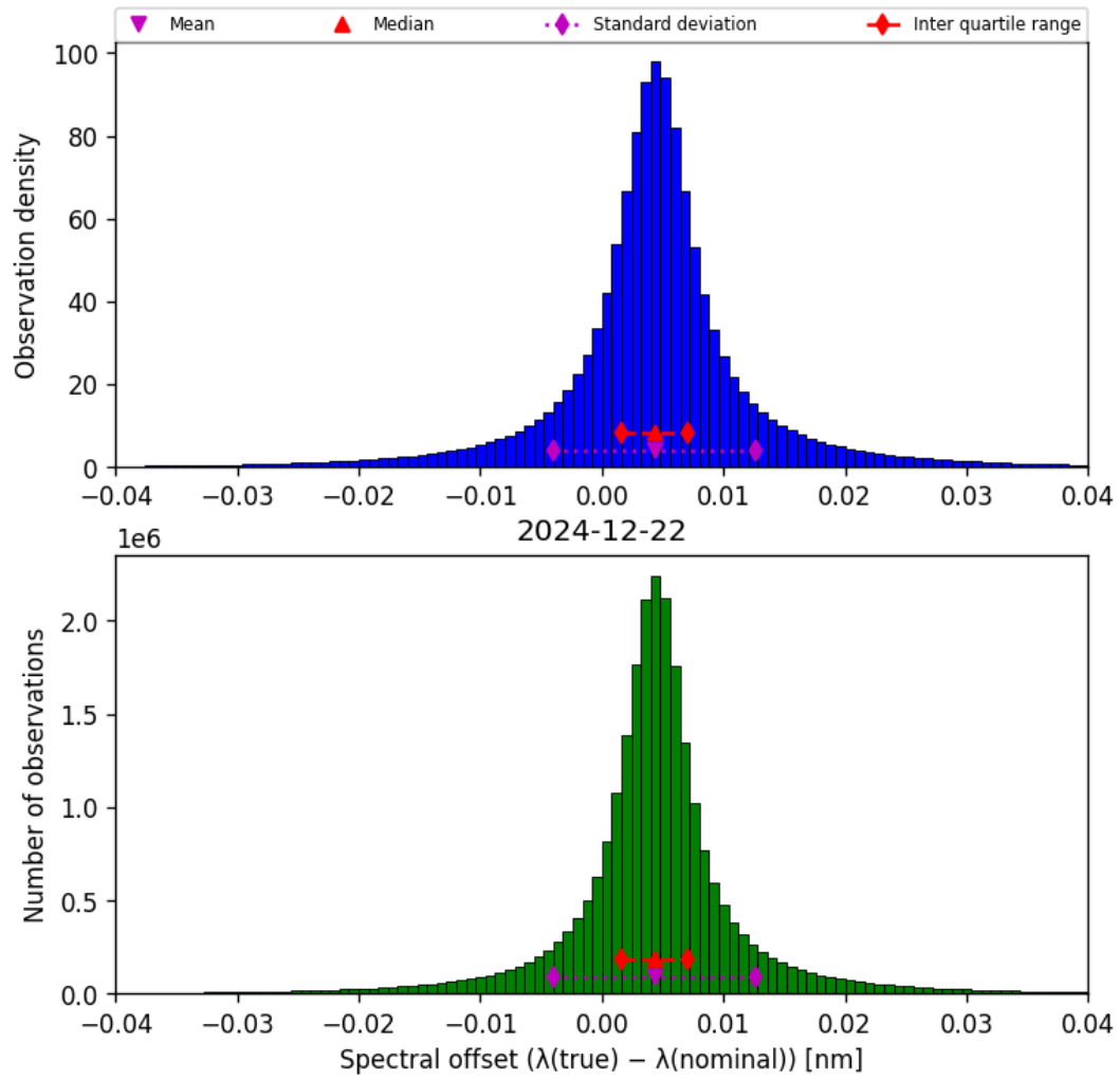
Figure 45: Histogram of “Spectral offset ( \lambda_{\text{true}} - \lambda_{\text{nominal}} )” for 2024-12-22 to 2024-12-23
