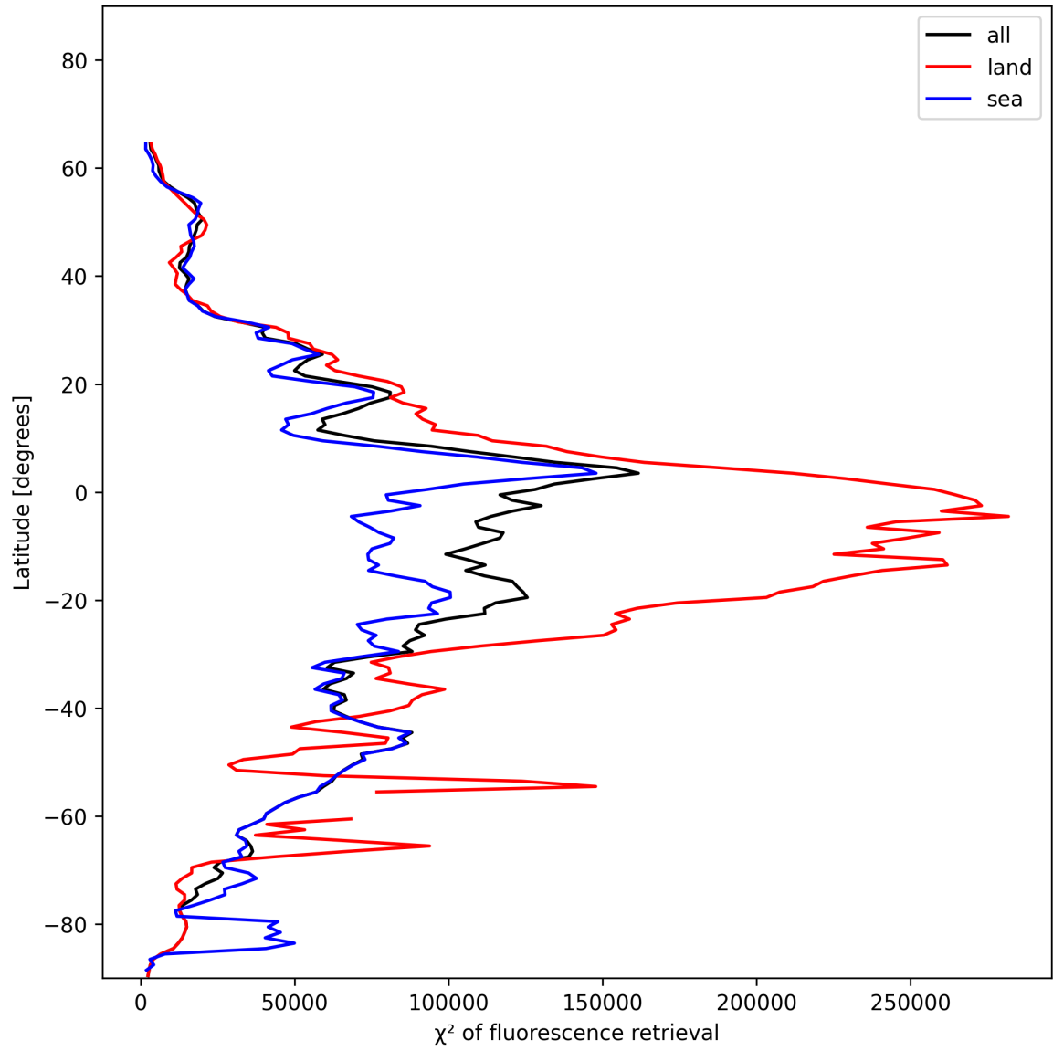
Figure 25: Zonal average of “ \chi^2 of fluorescence retrieval” for 2024-12-22 to 2024-12-23.
