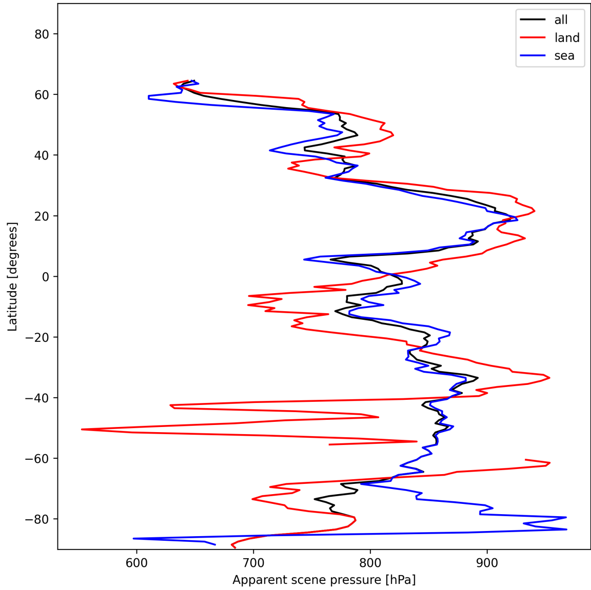
Figure 19: Zonal average of “Apparent scene pressure” for 2024-12-22 to 2024-12-23.
