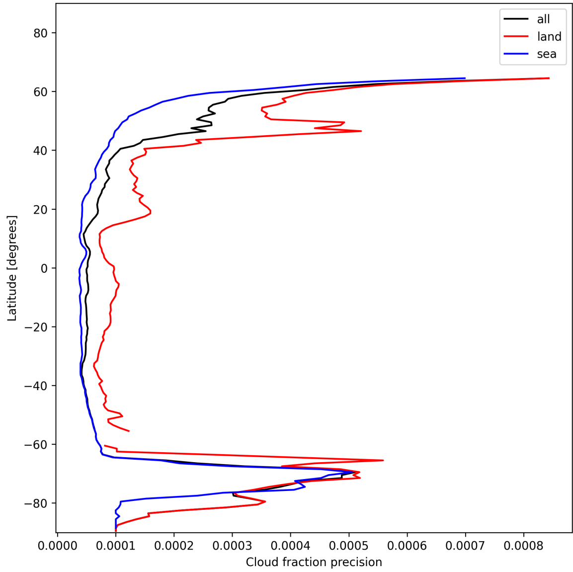
Figure 16: Zonal average of “Cloud fraction precision” for 2024-12-22 to 2024-12-23.
