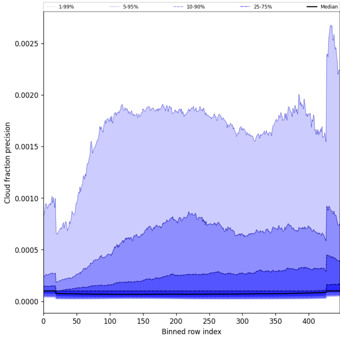
Figure 50: Along track statistics of “Cloud fraction precision” for 2024-12-22 to 2024-12-23
