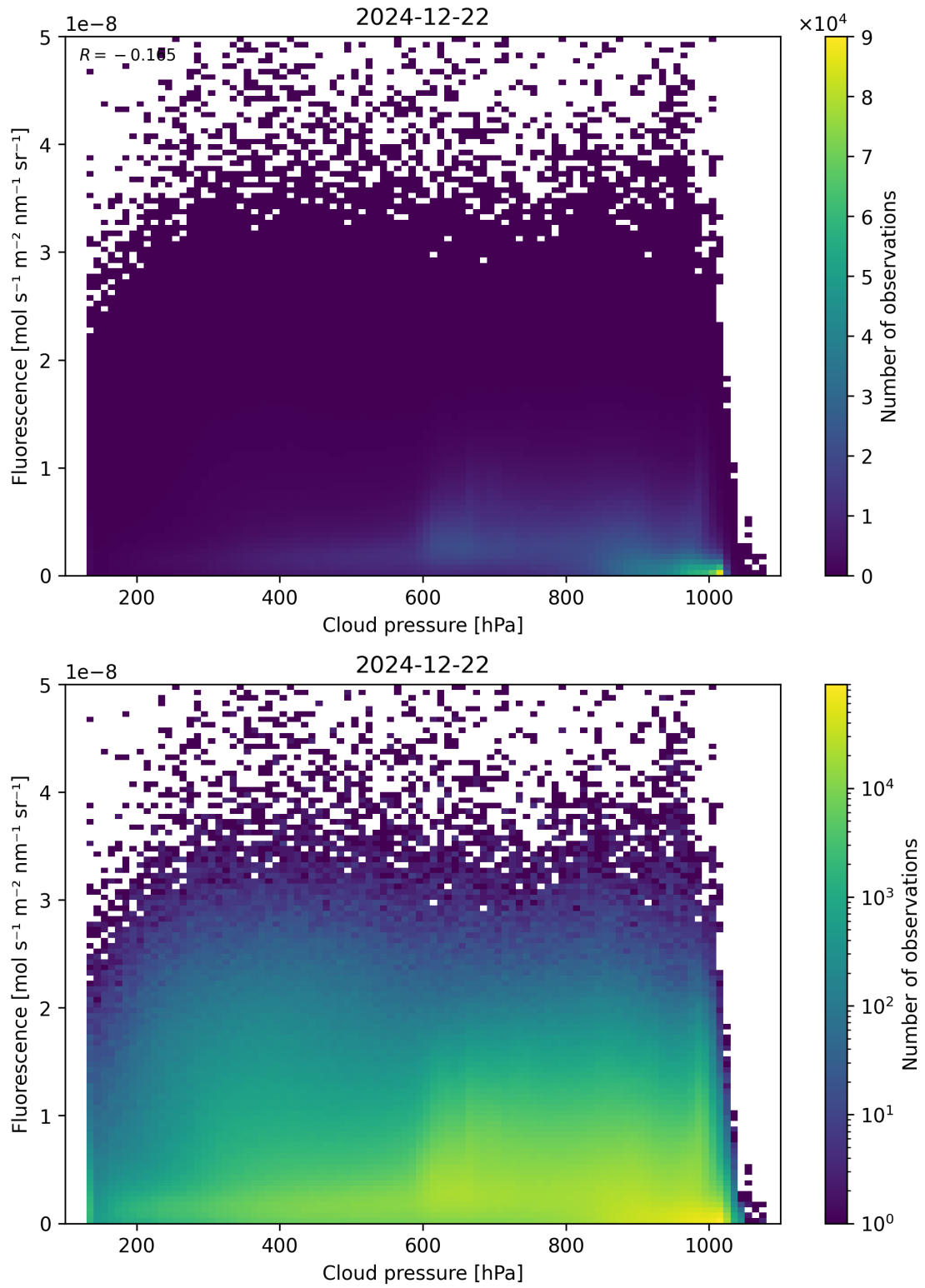
Figure 80: Scatter density plot of “Cloud pressure” against “Fluorescence” for 2024-12-22 to 2024-12-23.
