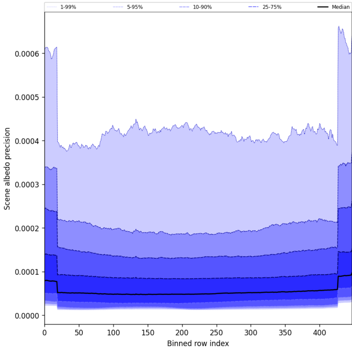
Figure 52: Along track statistics of “Scene albedo precision” for 2024-12-22 to 2024-12-23
