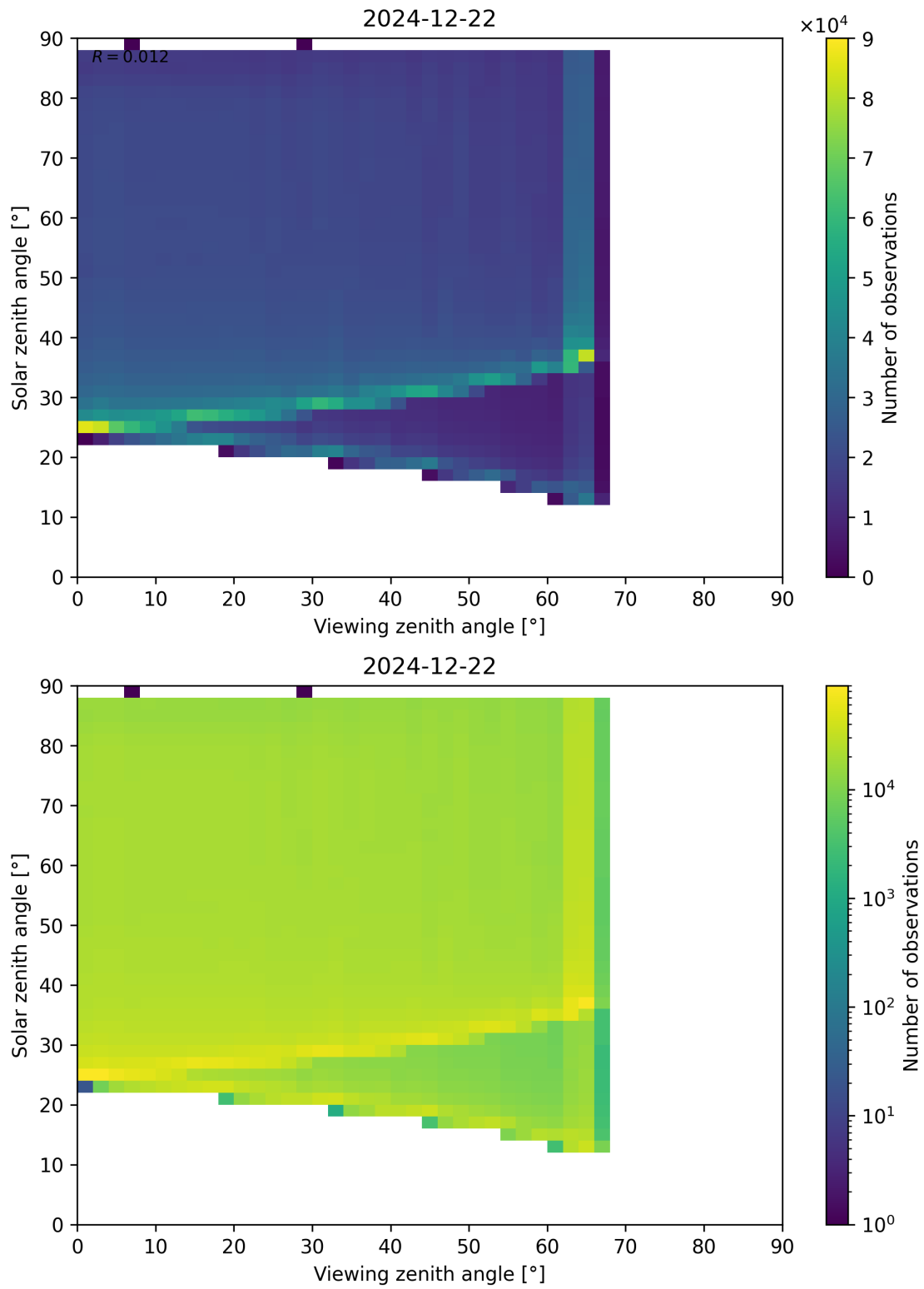
Figure 127: Scatter density plot of “Viewing zenith angle” against “Solar zenith angle” for 2024-12-22 to 2024-12-23.
