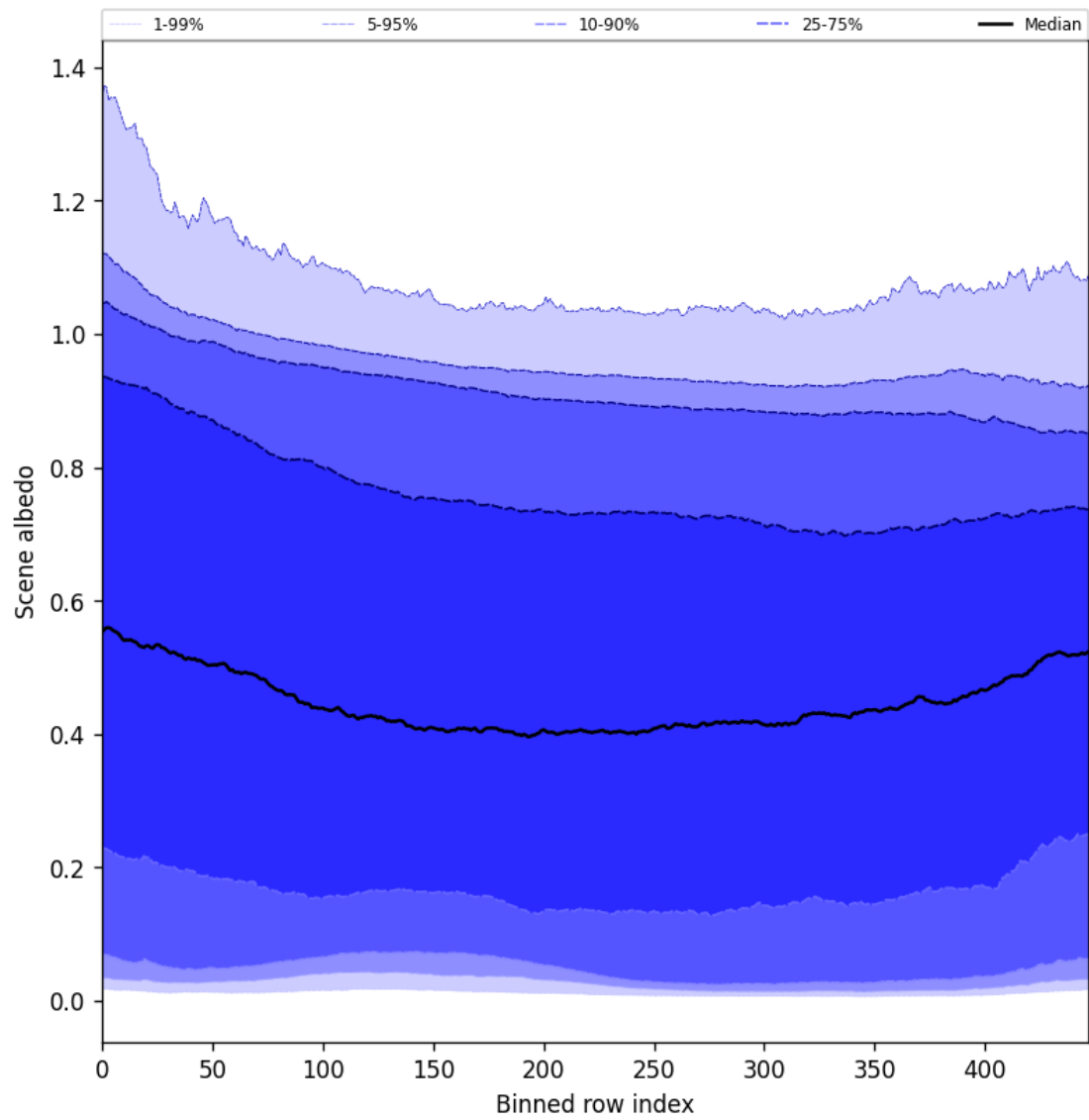
Figure 51: Along track statistics of “Scene albedo” for 2024-12-22 to 2024-12-23
