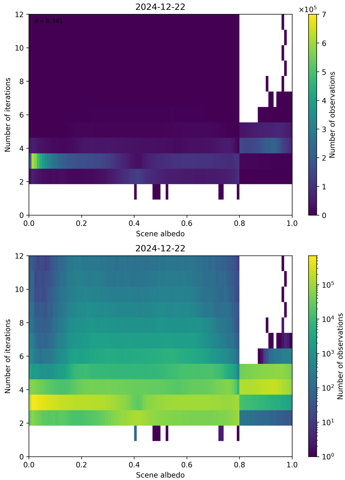
Figure 105: Scatter density plot of “Scene albedo” against “Number of iterations” for 2024-12-22 to 2024-12-23.
