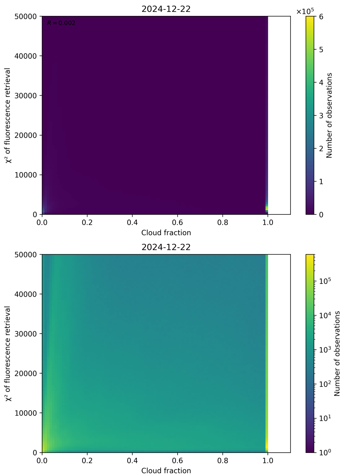
Figure 71: Scatter density plot of “Cloud fraction” against “ \chi^2 of fluorescence retrieval” for 2024-12-22 to 2024-12-23.
