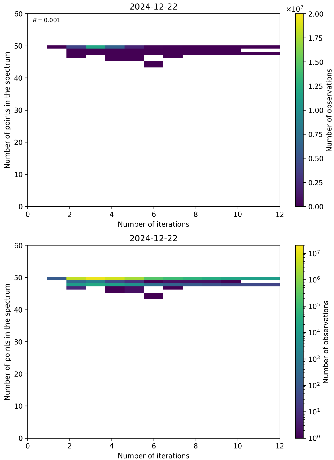
Figure 99: Scatter density plot of “Number of iterations” against “Number of points in the spectrum” for 2024-12-22 to 2024-12-23.
