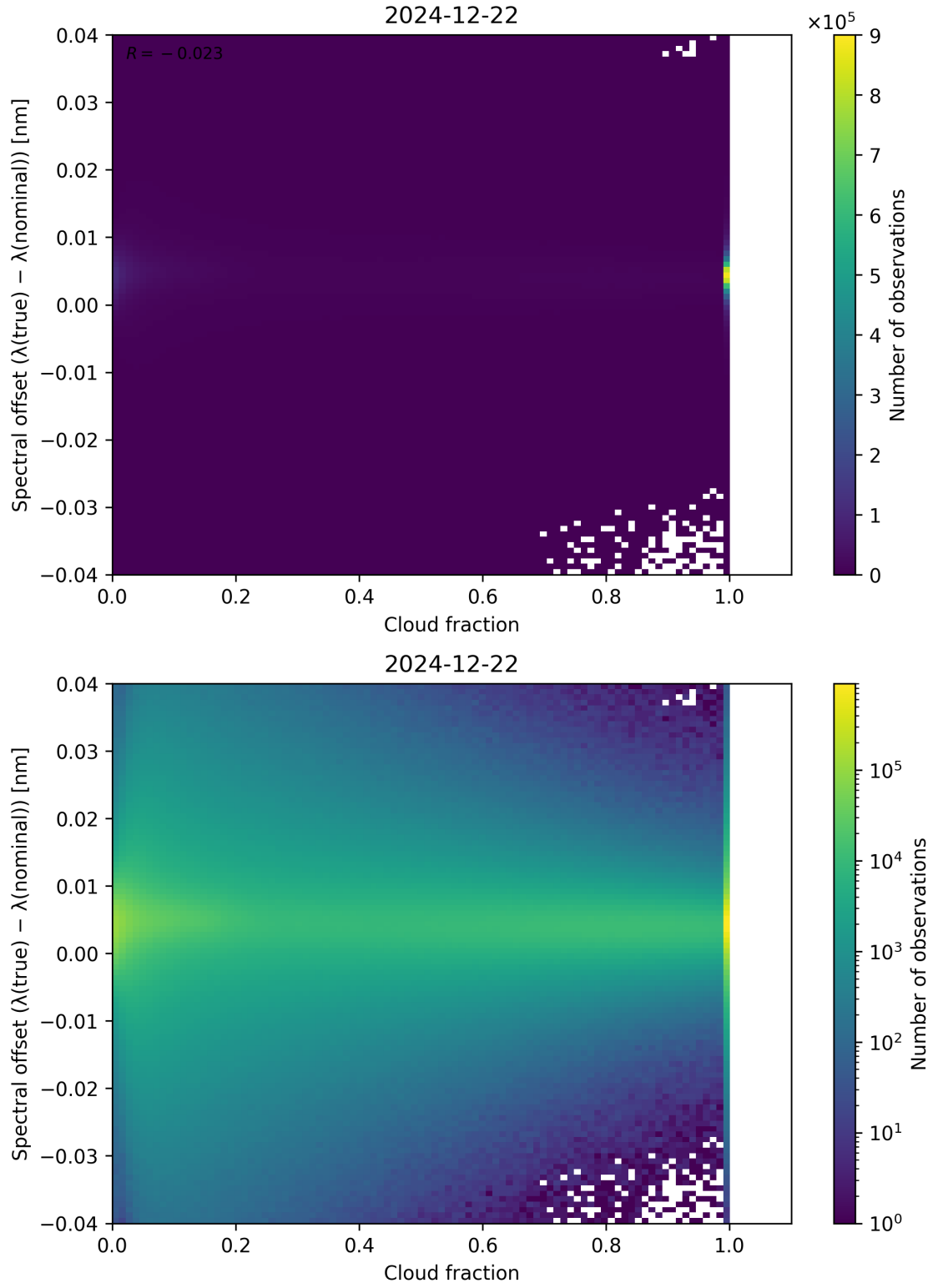
Figure 76: Scatter density plot of “Cloud fraction” against “Spectral offset ( \lambda_{\text{true}} - \lambda_{\text{nominal}} )” for 2024-12-22 to 2024-12-23.
