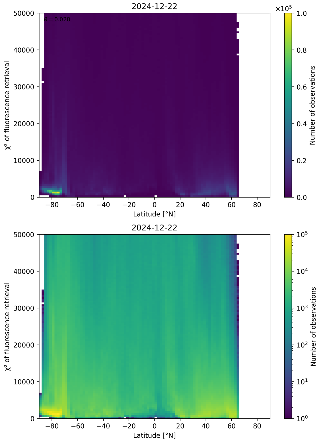
Figure 89: Scatter density plot of “Latitude” against “ \chi^2 of fluorescence retrieval” for 2024-12-22 to 2024-12-23.
