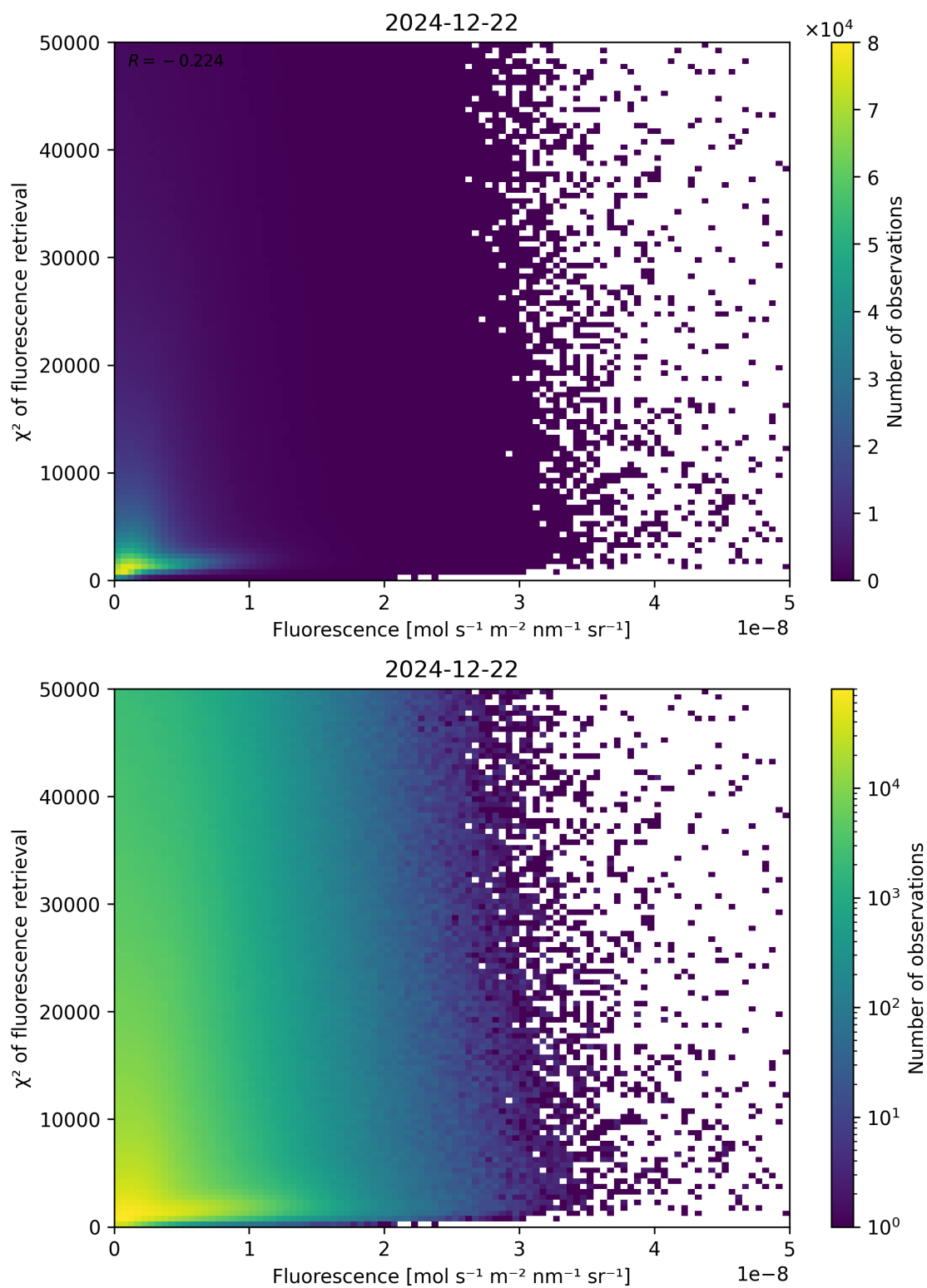
Figure 85: Scatter density plot of “Fluorescence” against “ \chi^2 of fluorescence retrieval” for 2024-12-22 to 2024-12-23.
