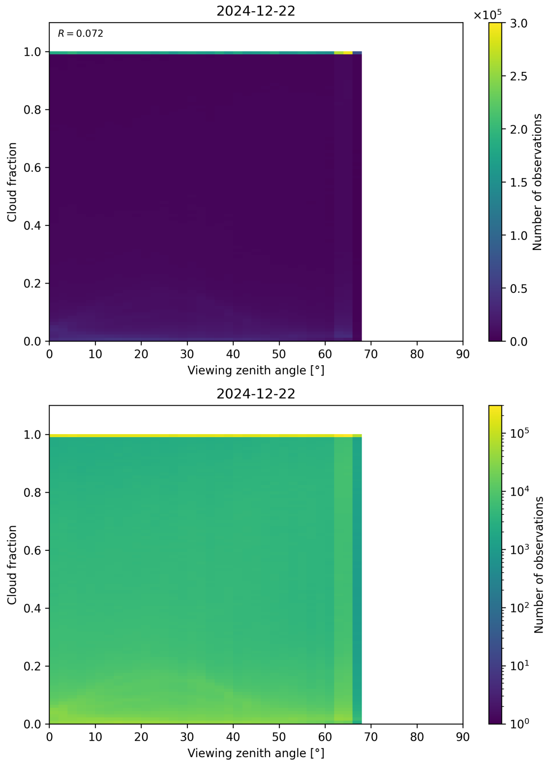
Figure 120: Scatter density plot of “Viewing zenith angle” against “Cloud fraction” for 2024-12-22 to 2024-12-23.
