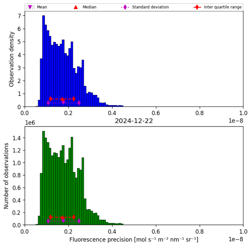
Figure 41: Histogram of “Fluorescence precision” for 2024-12-22 to 2024-12-23
