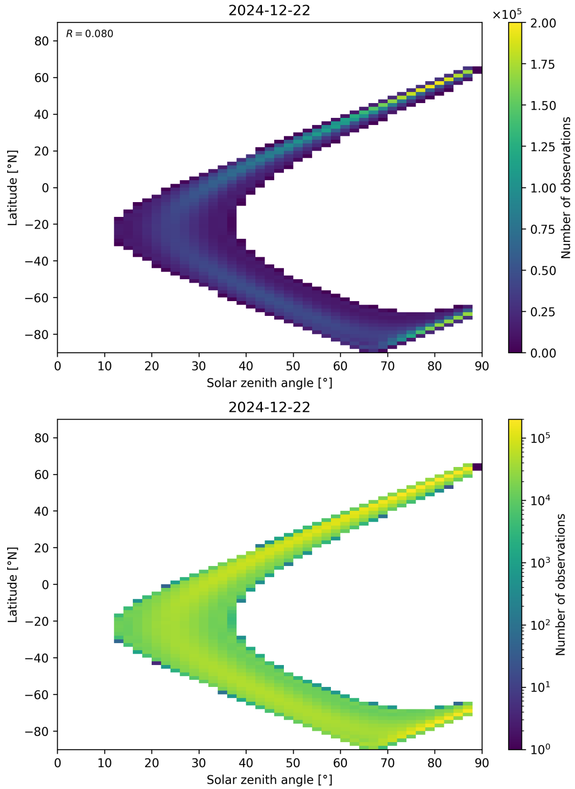
Figure 113: Scatter density plot of “Solar zenith angle” against “Latitude” for 2024-12-22 to 2024-12-23.
