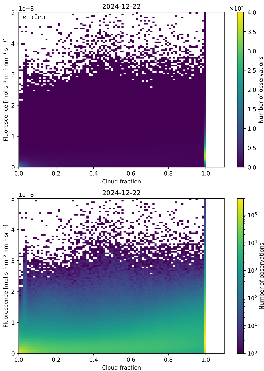
Figure 72: Scatter density plot of “Cloud fraction” against “Fluorescence” for 2024-12-22 to 2024-12-23.
