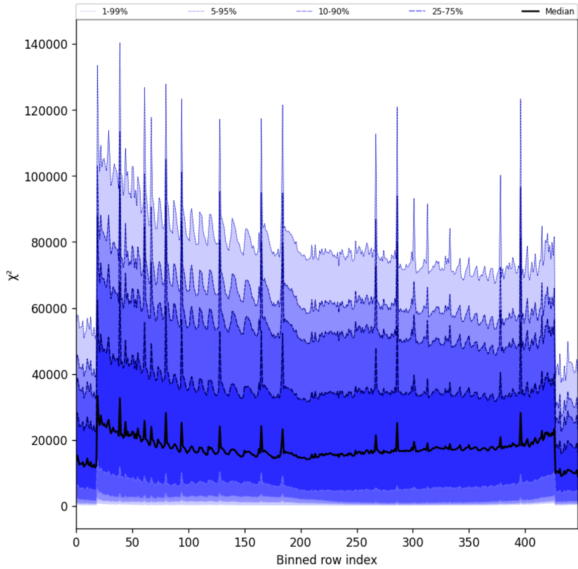
Figure 55: Along track statistics of “ \chi^2 ” for 2024-12-22 to 2024-12-23
