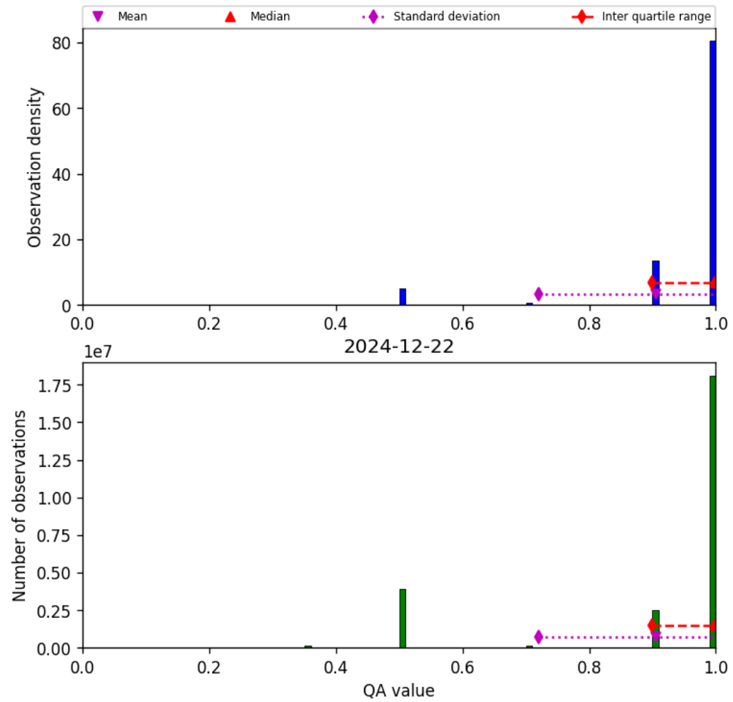
Figure 29: Histogram of “QA value” for 2024-12-22 to 2024-12-23
