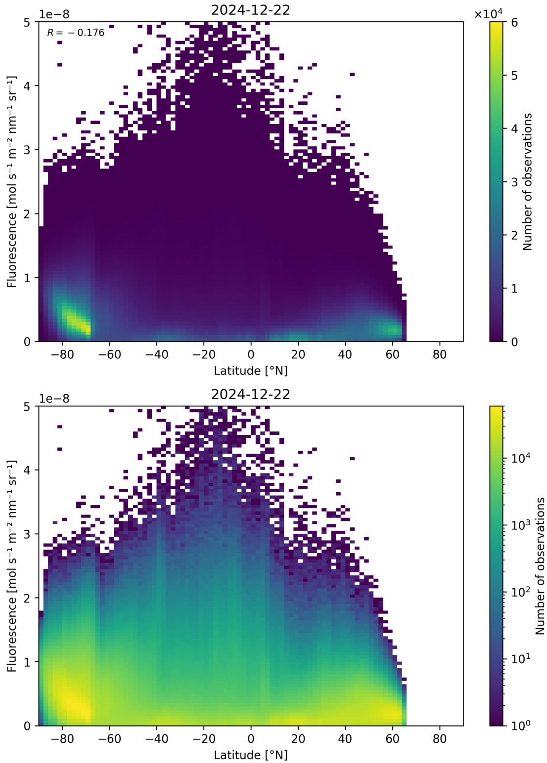
Figure 92: Scatter density plot of “Latitude” against “Fluorescence” for 2024-12-22 to 2024-12-23.
