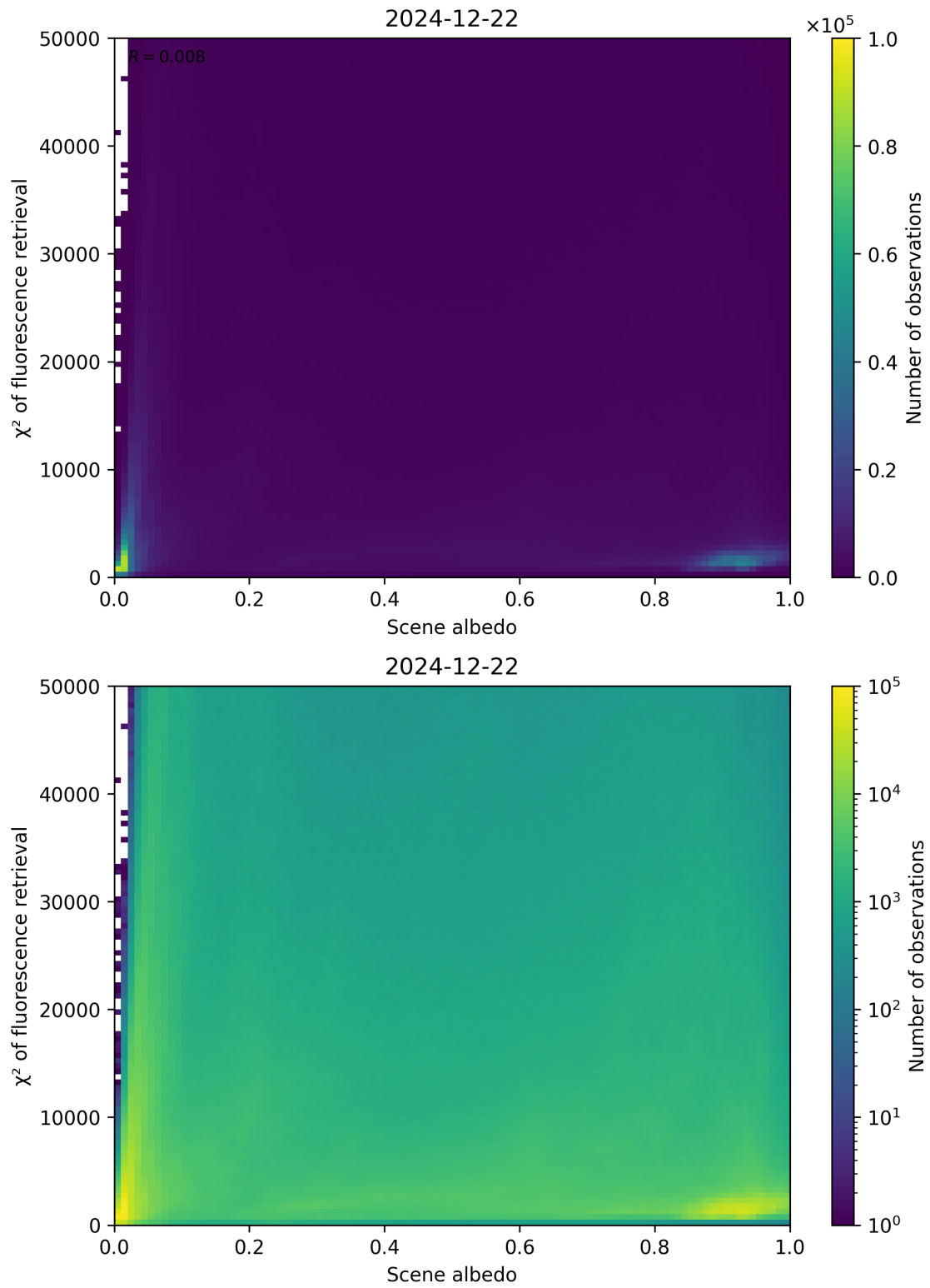
Figure 103: Scatter density plot of “Scene albedo” against “ \chi^2 of fluorescence retrieval” for 2024-12-22 to 2024-12-23.
