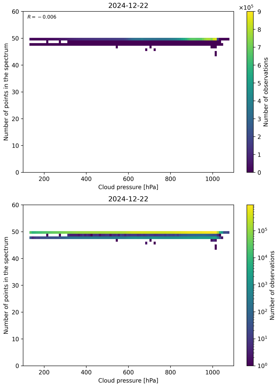
Figure 82: Scatter density plot of “Cloud pressure” against “Number of points in the spectrum” for 2024-12-22 to 2024-12-23.
