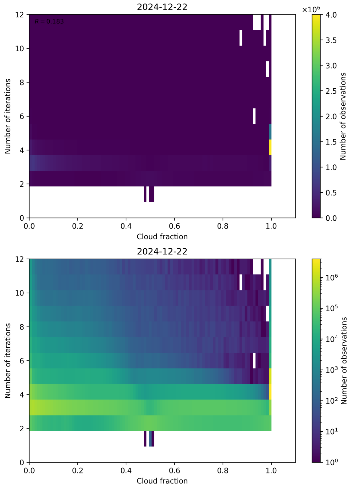
Figure 73: Scatter density plot of “Cloud fraction” against “Number of iterations” for 2024-12-22 to 2024-12-23.
