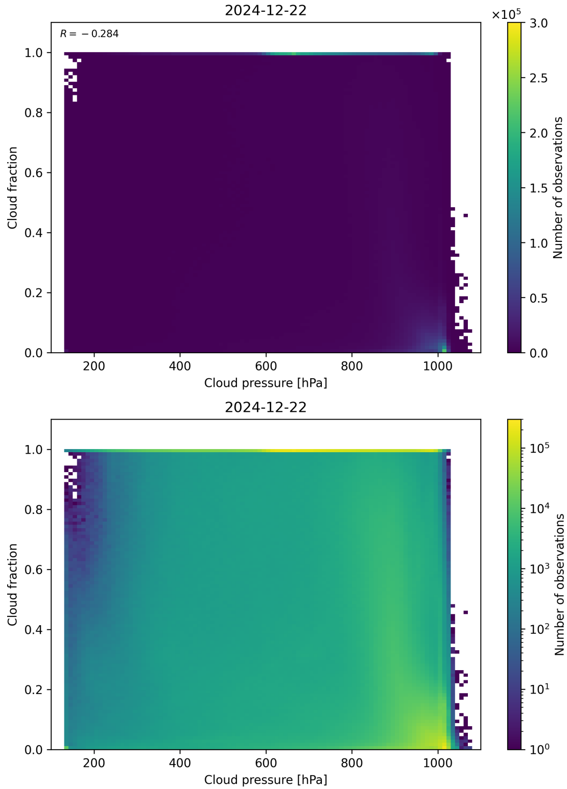
Figure 79: Scatter density plot of “Cloud pressure” against “Cloud fraction” for 2024-12-22 to 2024-12-23.
