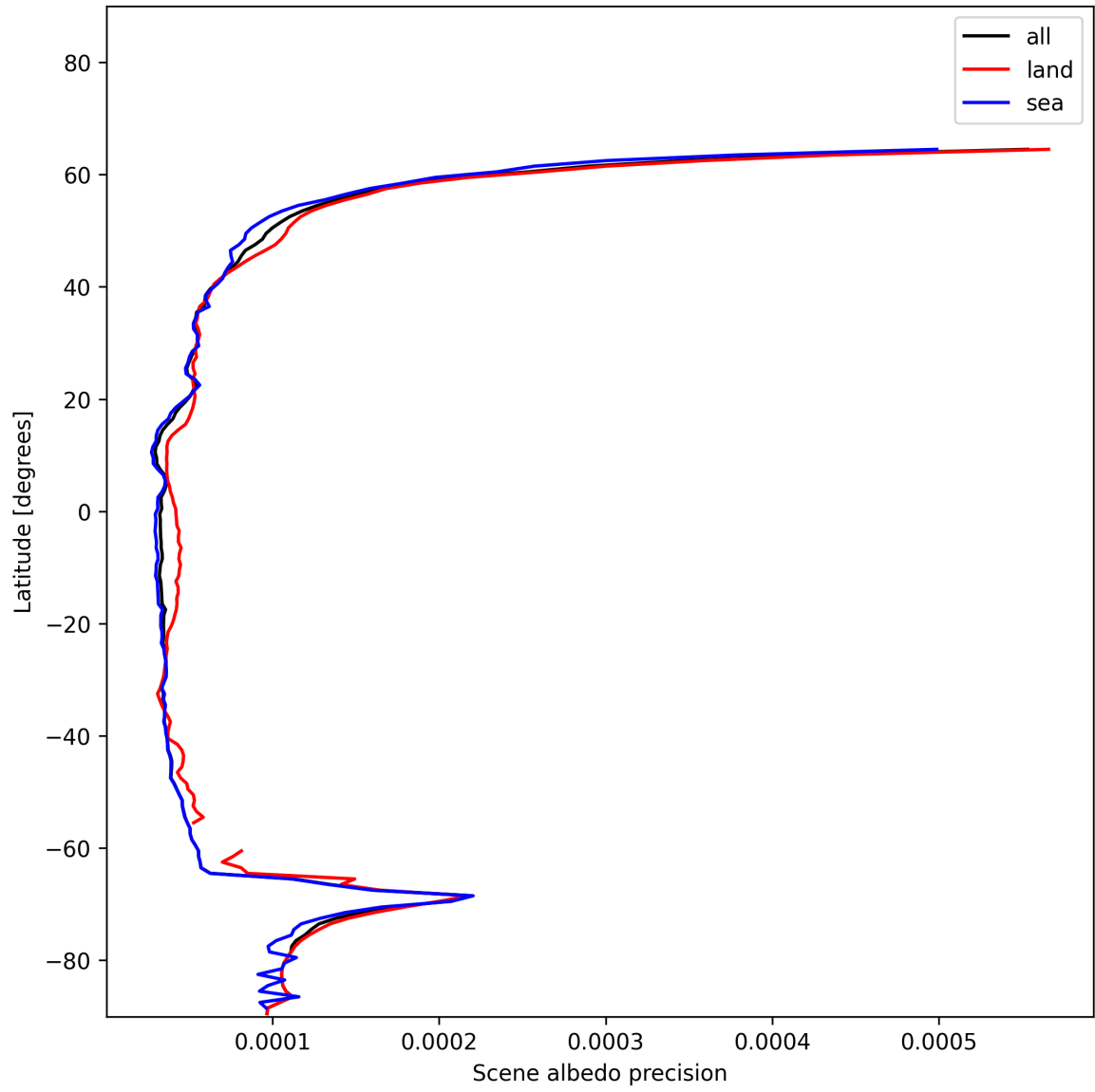
Figure 18: Zonal average of “Scene albedo precision” for 2024-12-22 to 2024-12-23.
