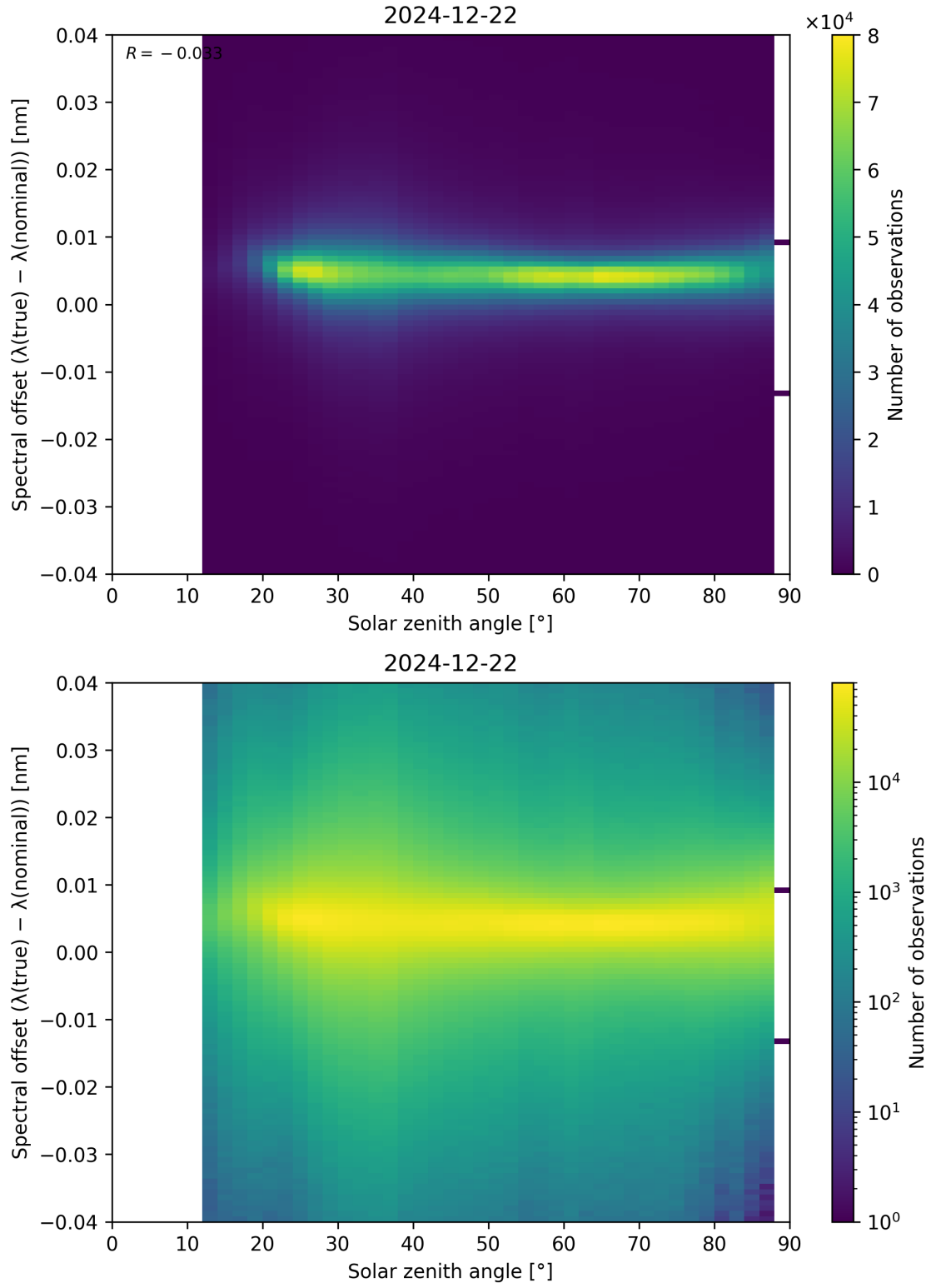
Figure 117: Scatter density plot of “Solar zenith angle” against “Spectral offset ( \lambda_{\text{true}} - \lambda_{\text{nominal}} )” for 2024-12-22 to 2024-12-23.
