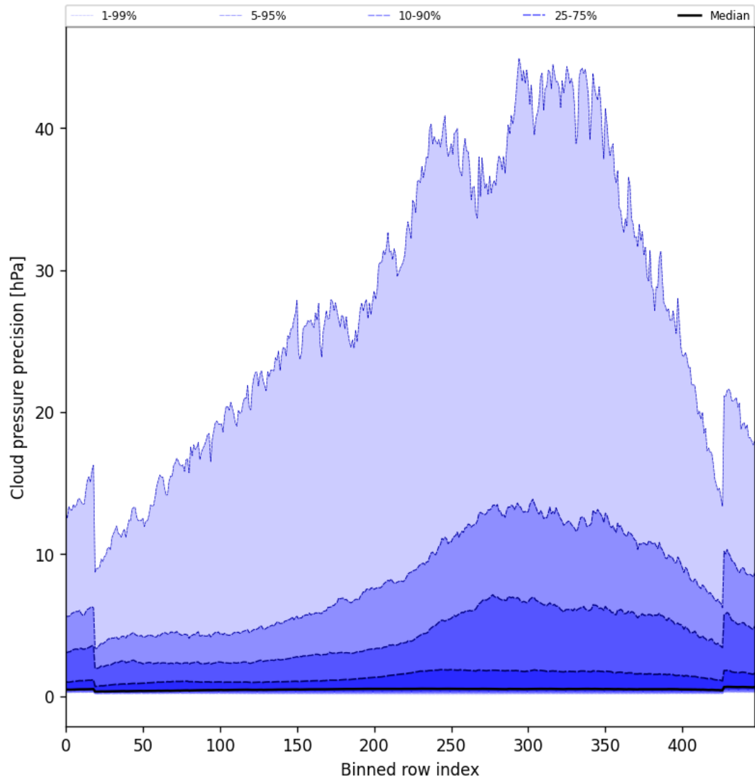
Figure 48: Along track statistics of “Cloud pressure precision” for 2024-12-22 to 2024-12-23
