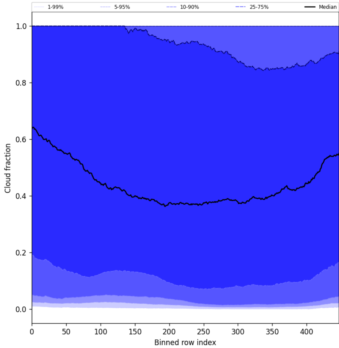
Figure 49: Along track statistics of “Cloud fraction” for 2024-12-22 to 2024-12-23
