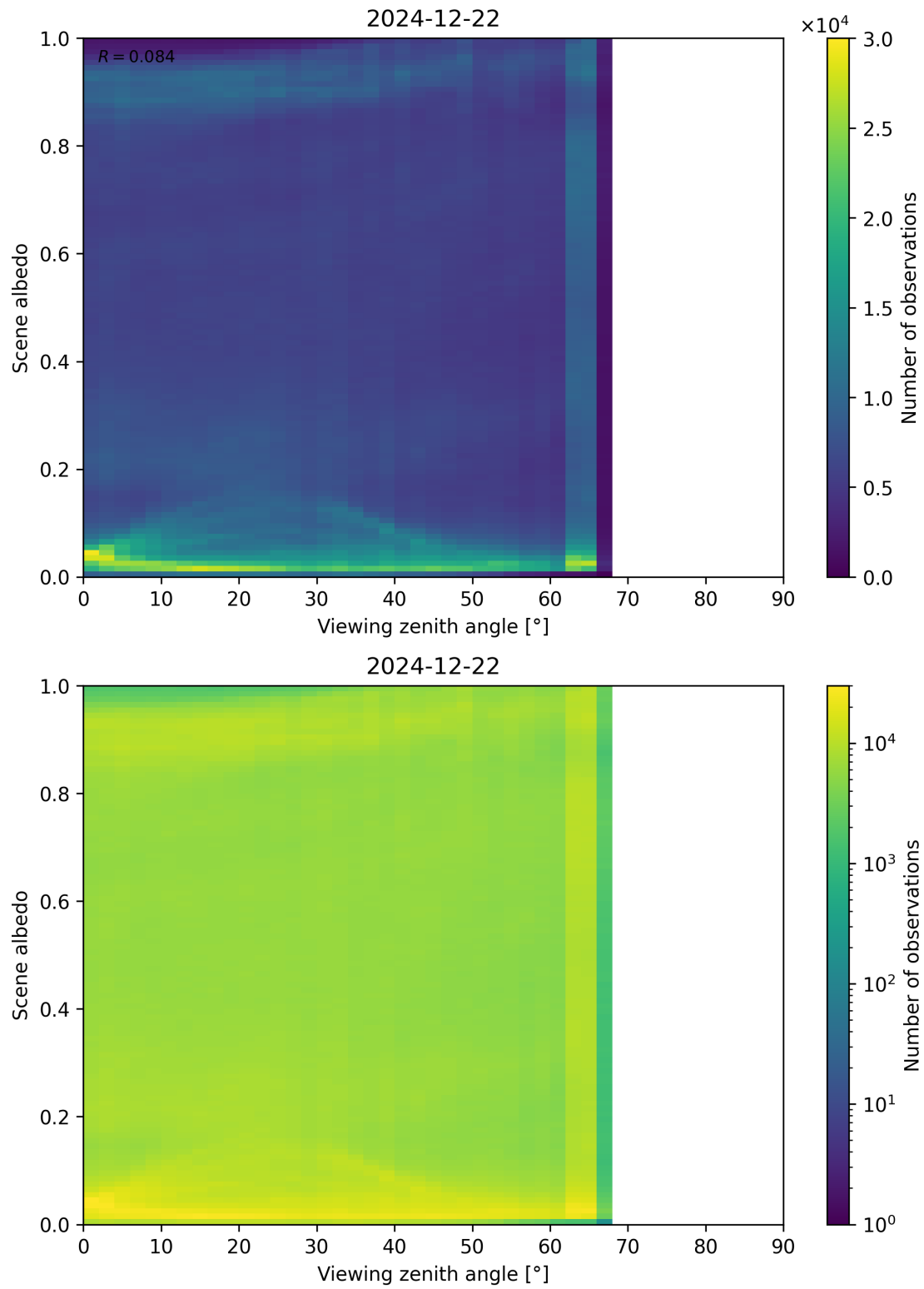
Figure 126: Scatter density plot of “Viewing zenith angle” against “Scene albedo” for 2024-12-22 to 2024-12-23.
