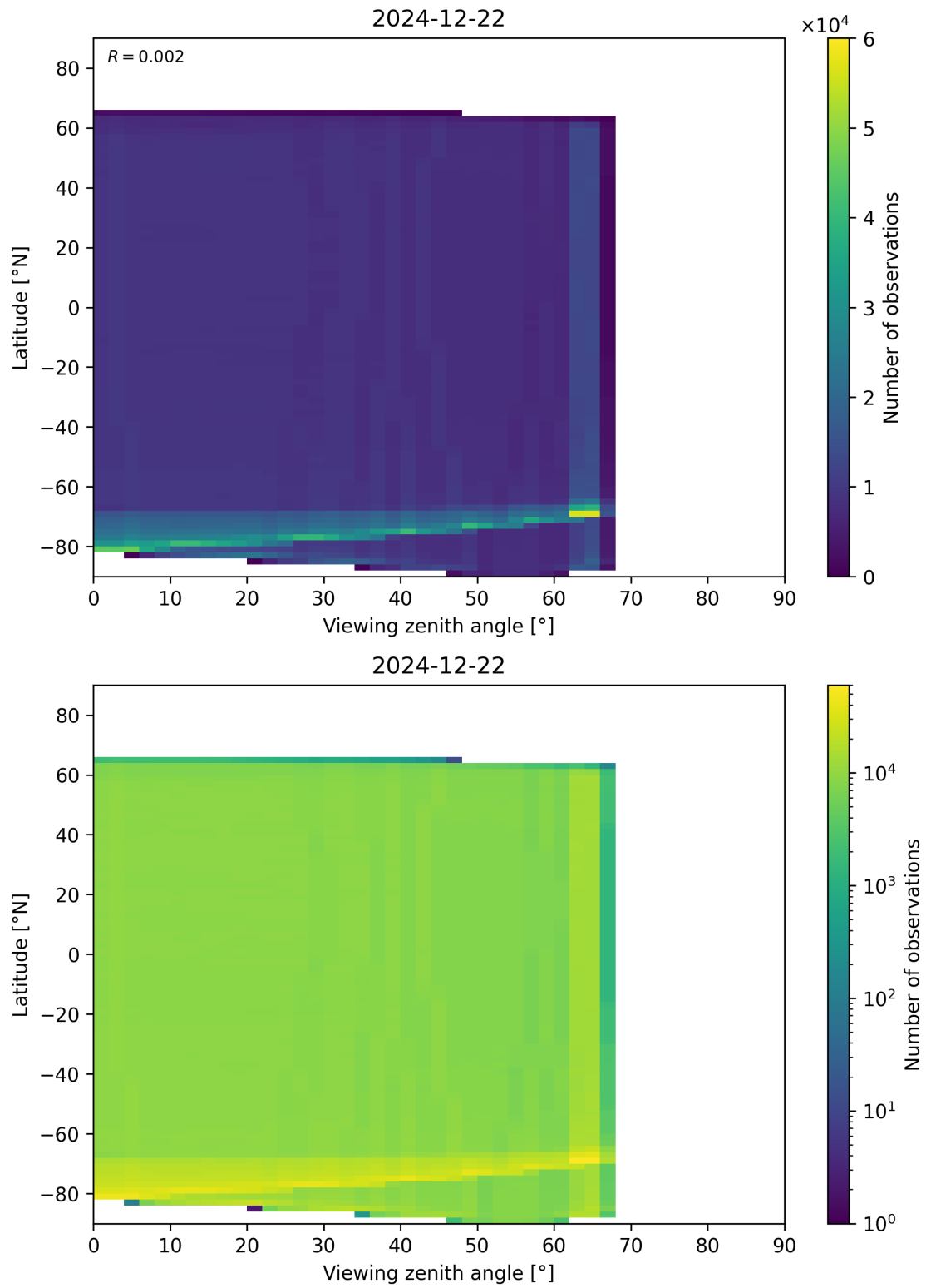
Figure 123: Scatter density plot of “Viewing zenith angle” against “Latitude” for 2024-12-22 to 2024-12-23.
