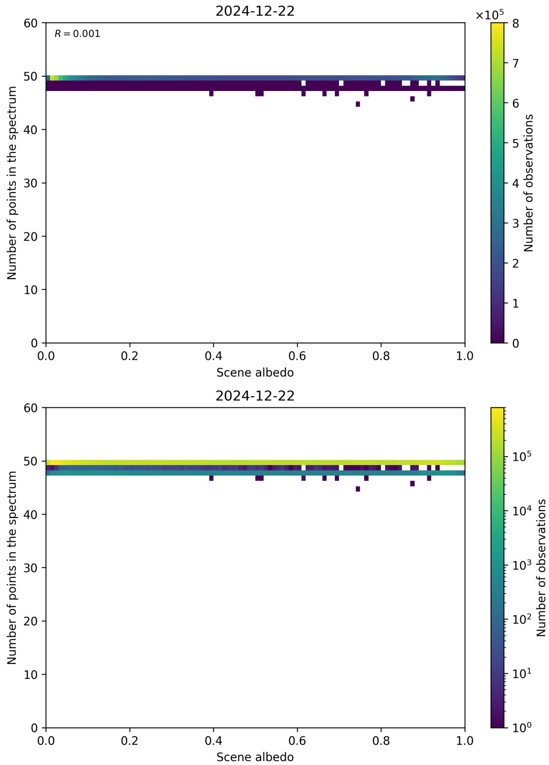
Figure 106: Scatter density plot of “Scene albedo” against “Number of points in the spectrum” for 2024-12-22 to 2024-12-23.
