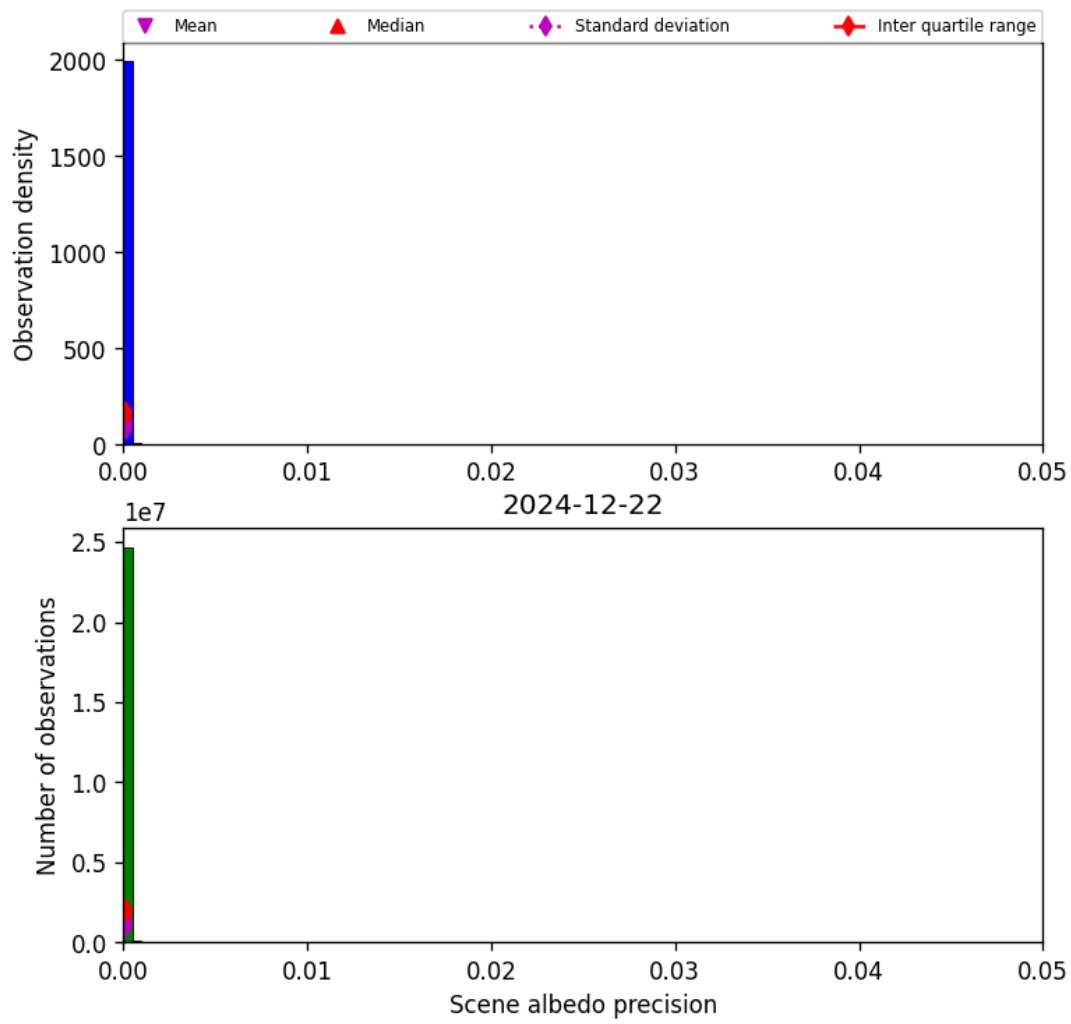
Figure 35: Histogram of “Scene albedo precision” for 2024-12-22 to 2024-12-23
