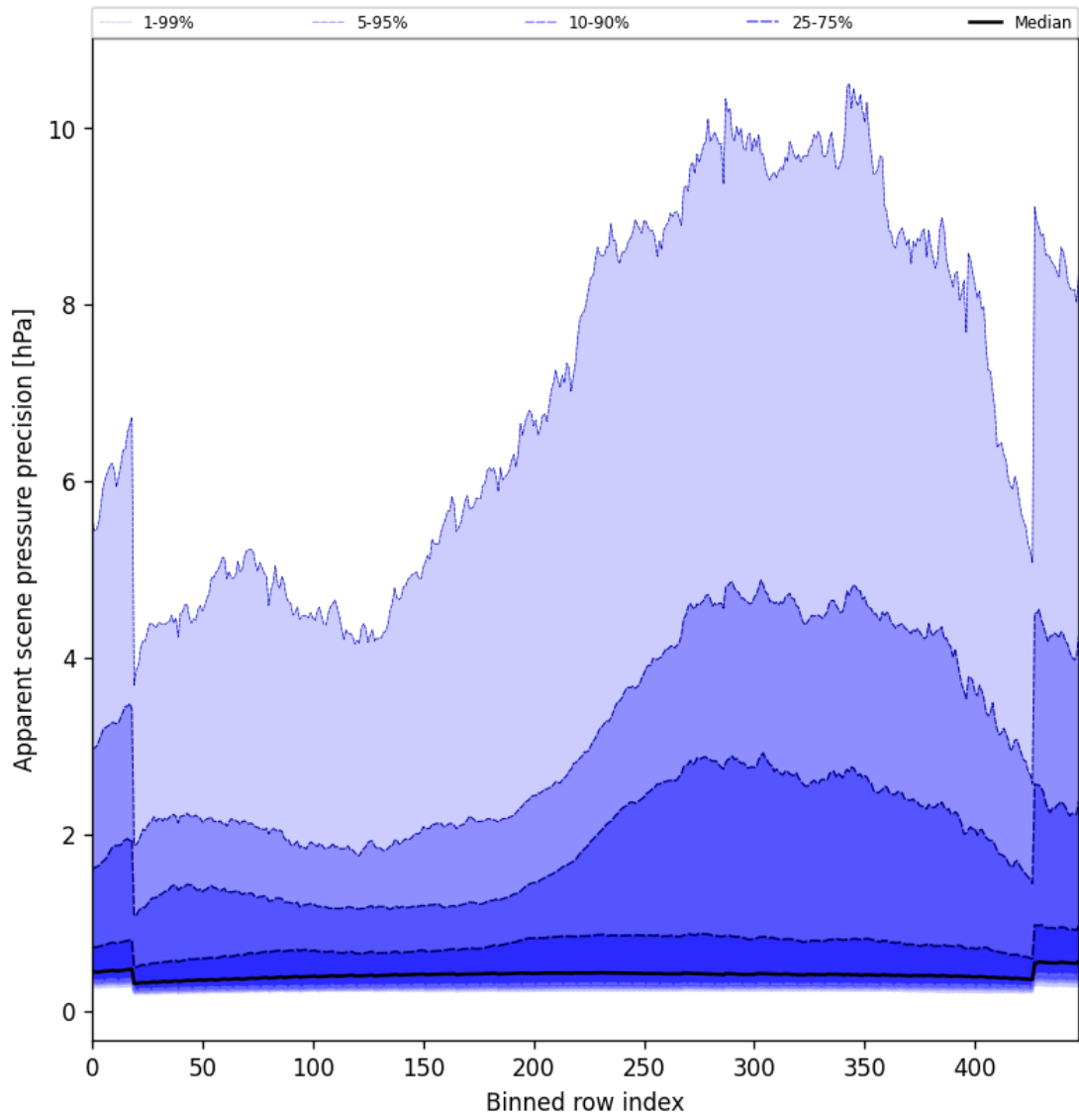
Figure 54: Along track statistics of “Apparent scene pressure precision” for 2024-12-22 to 2024-12-23
