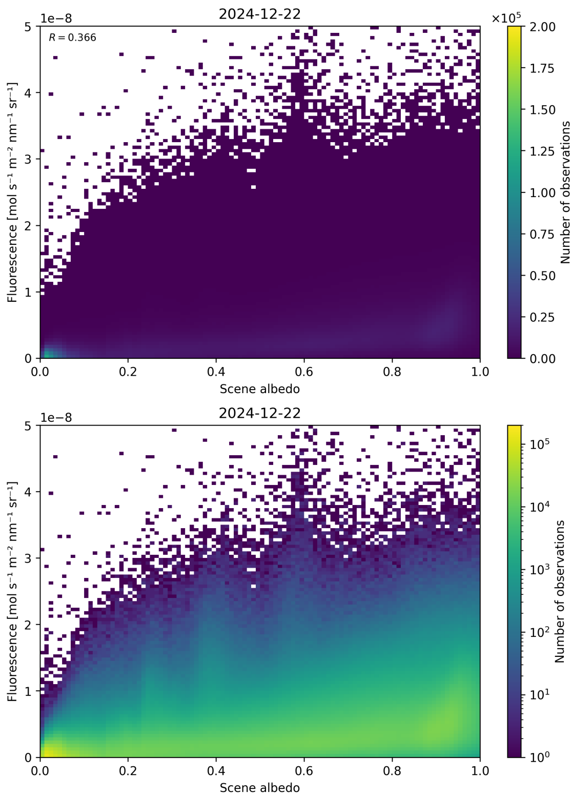
Figure 104: Scatter density plot of “Scene albedo” against “Fluorescence” for 2024-12-22 to 2024-12-23.
