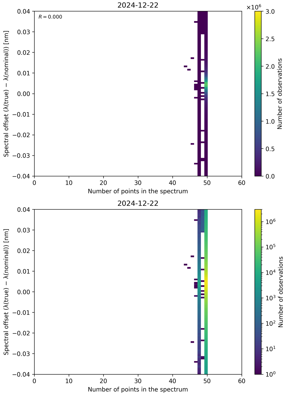
Figure 101: Scatter density plot of “Number of points in the spectrum” against “Spectral offset ( \lambda_{\text{true}} - \lambda_{\text{nominal}} )” for 2024-12-22 to 2024-12-23.
