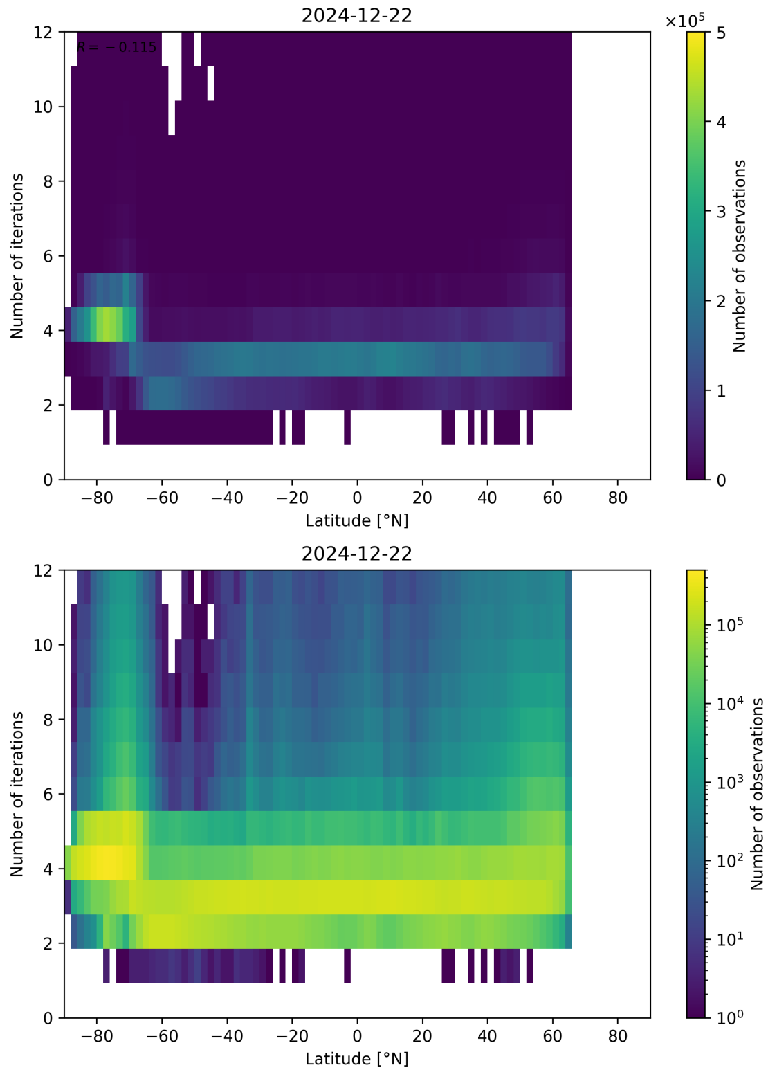
Figure 93: Scatter density plot of “Latitude” against “Number of iterations” for 2024-12-22 to 2024-12-23.
