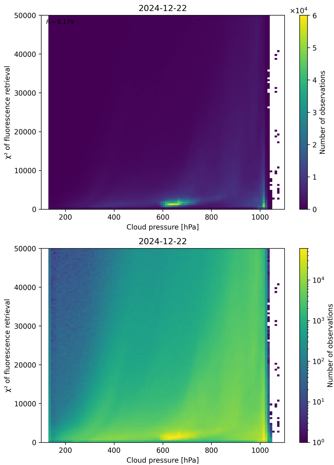
Figure 78: Scatter density plot of “Cloud pressure” against “ \chi^2 of fluorescence retrieval” for 2024-12-22 to 2024-12-23.
