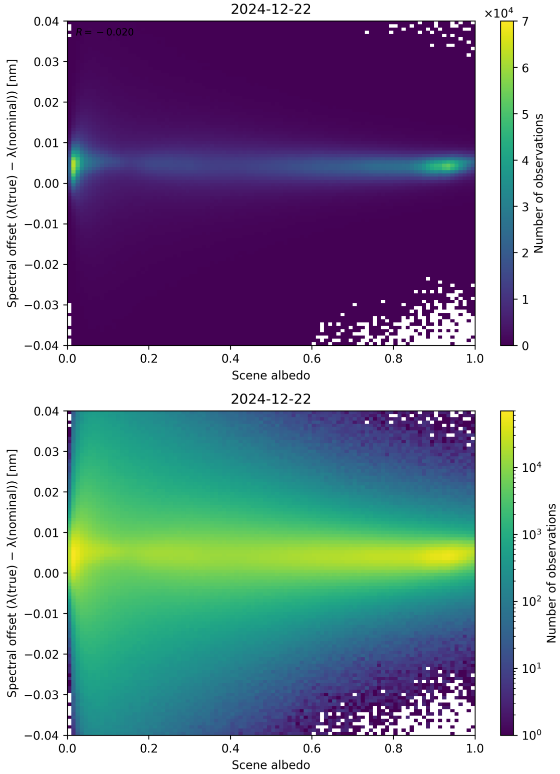
Figure 107: Scatter density plot of “Scene albedo” against “Spectral offset ( \lambda_{\text{true}} - \lambda_{\text{nominal}} )” for 2024-12-22 to 2024-12-23.
