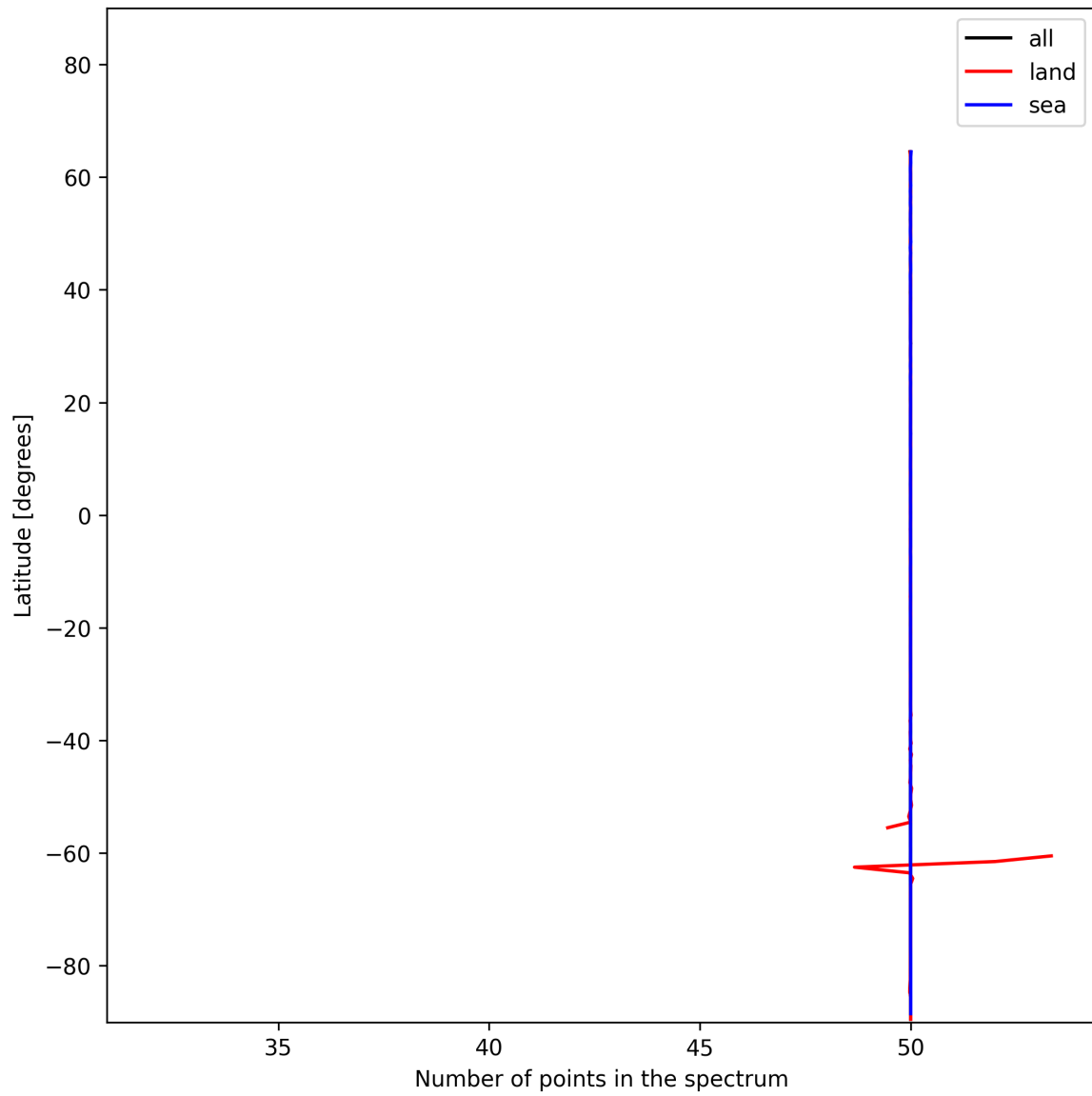
Figure 27: Zonal average of “Number of points in the spectrum” for 2024-12-22 to 2024-12-23.
