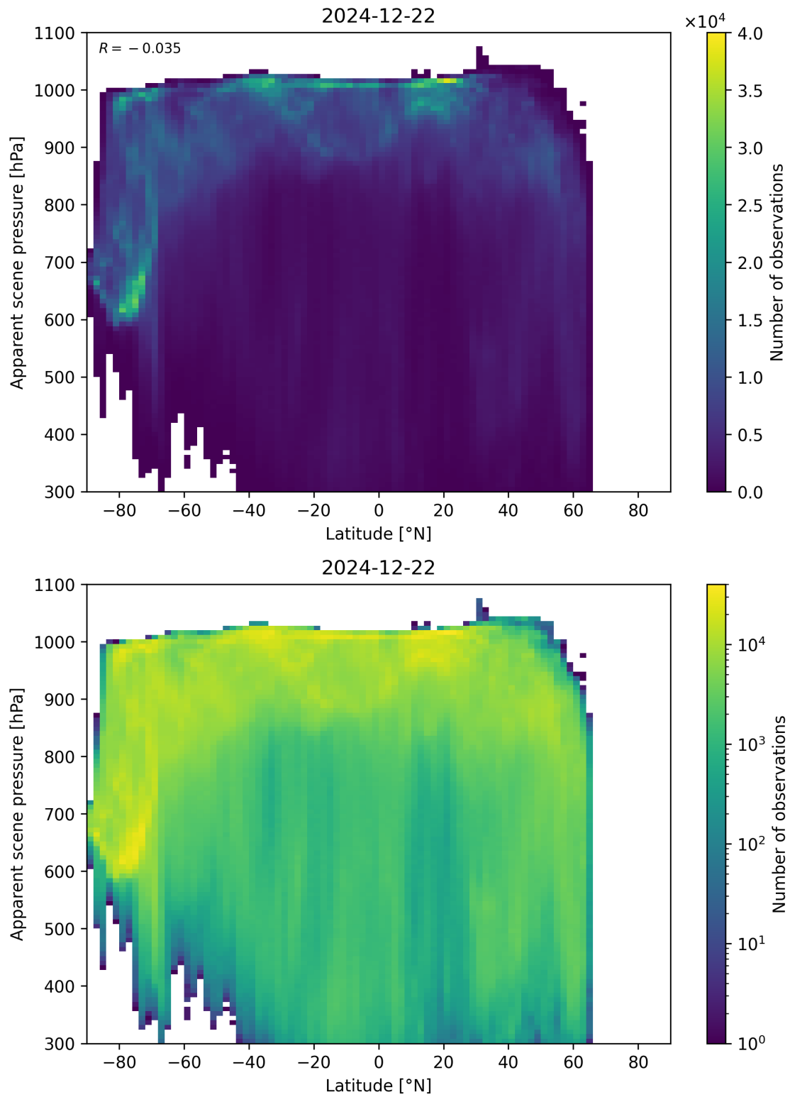
Figure 88: Scatter density plot of “Latitude” against “Apparent scene pressure” for 2024-12-22 to 2024-12-23.
