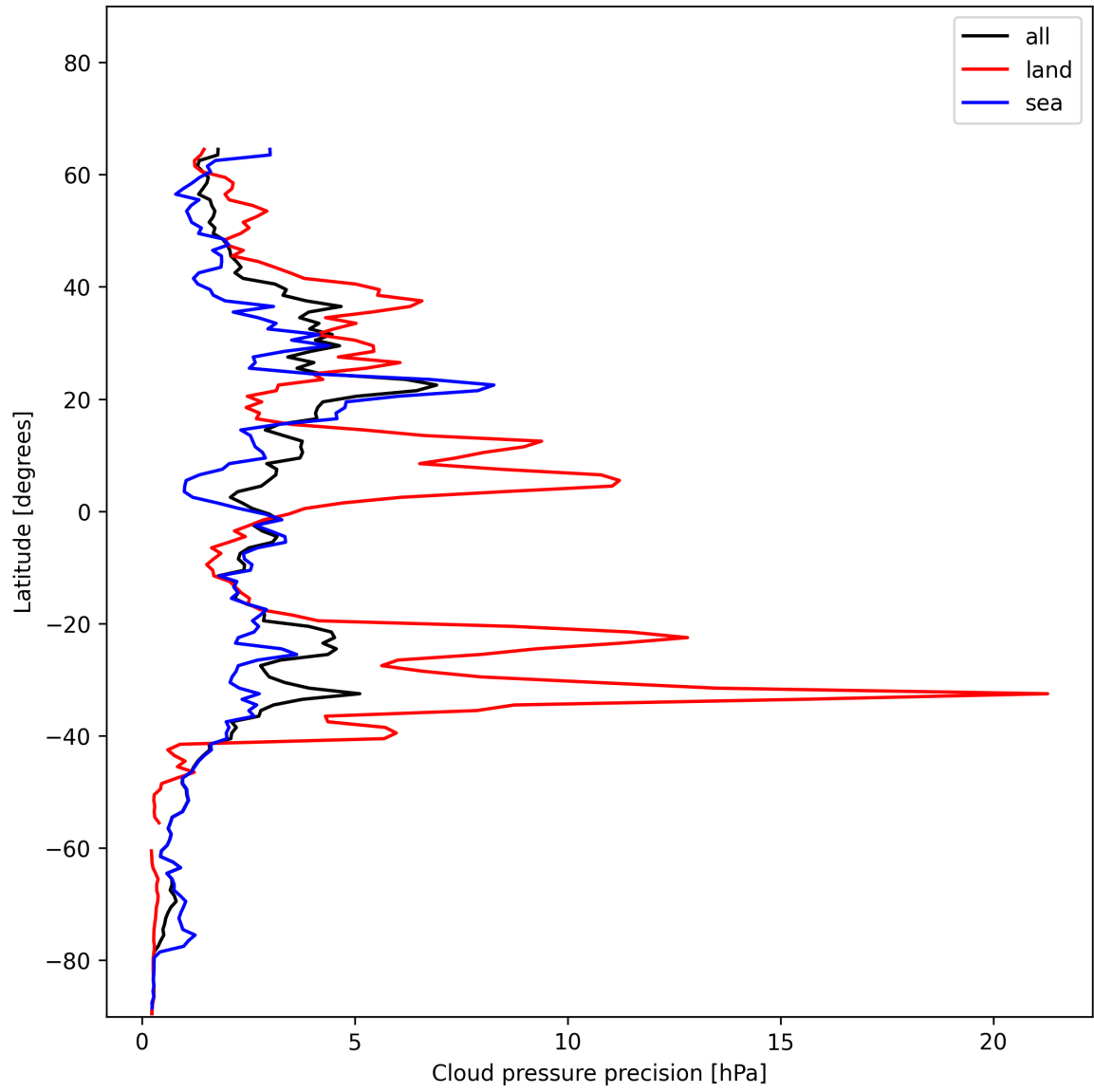
Figure 14: Zonal average of “Cloud pressure precision” for 2024-12-22 to 2024-12-23.
