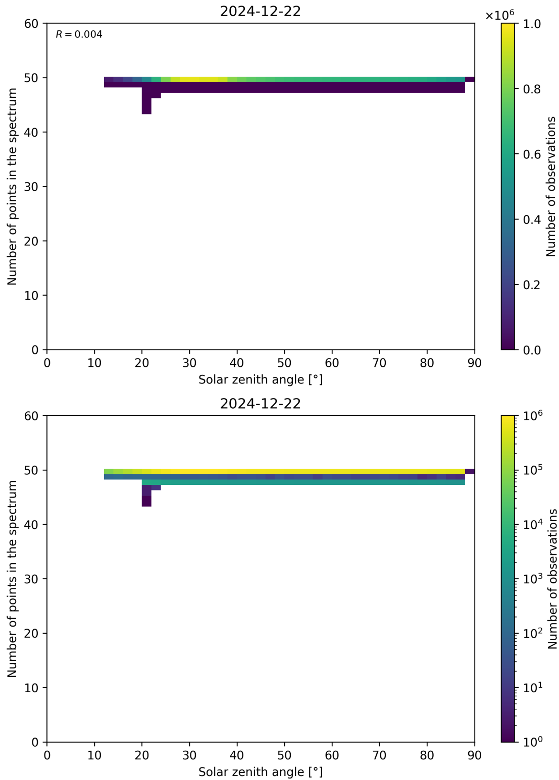
Figure 115: Scatter density plot of “Solar zenith angle” against “Number of points in the spectrum” for 2024-12-22 to 2024-12-23.
