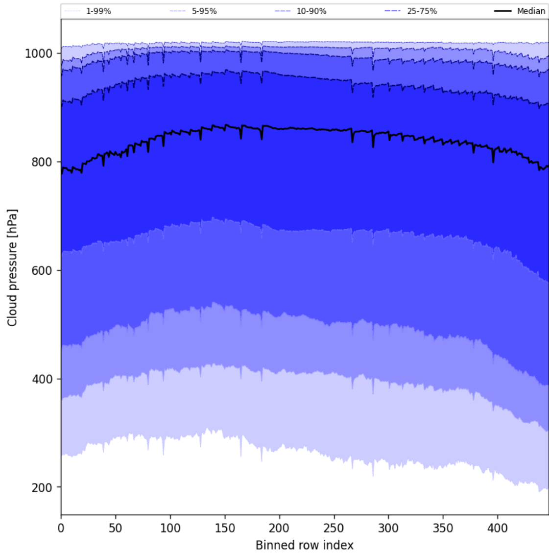
Figure 47: Along track statistics of “Cloud pressure” for 2024-12-22 to 2024-12-23
