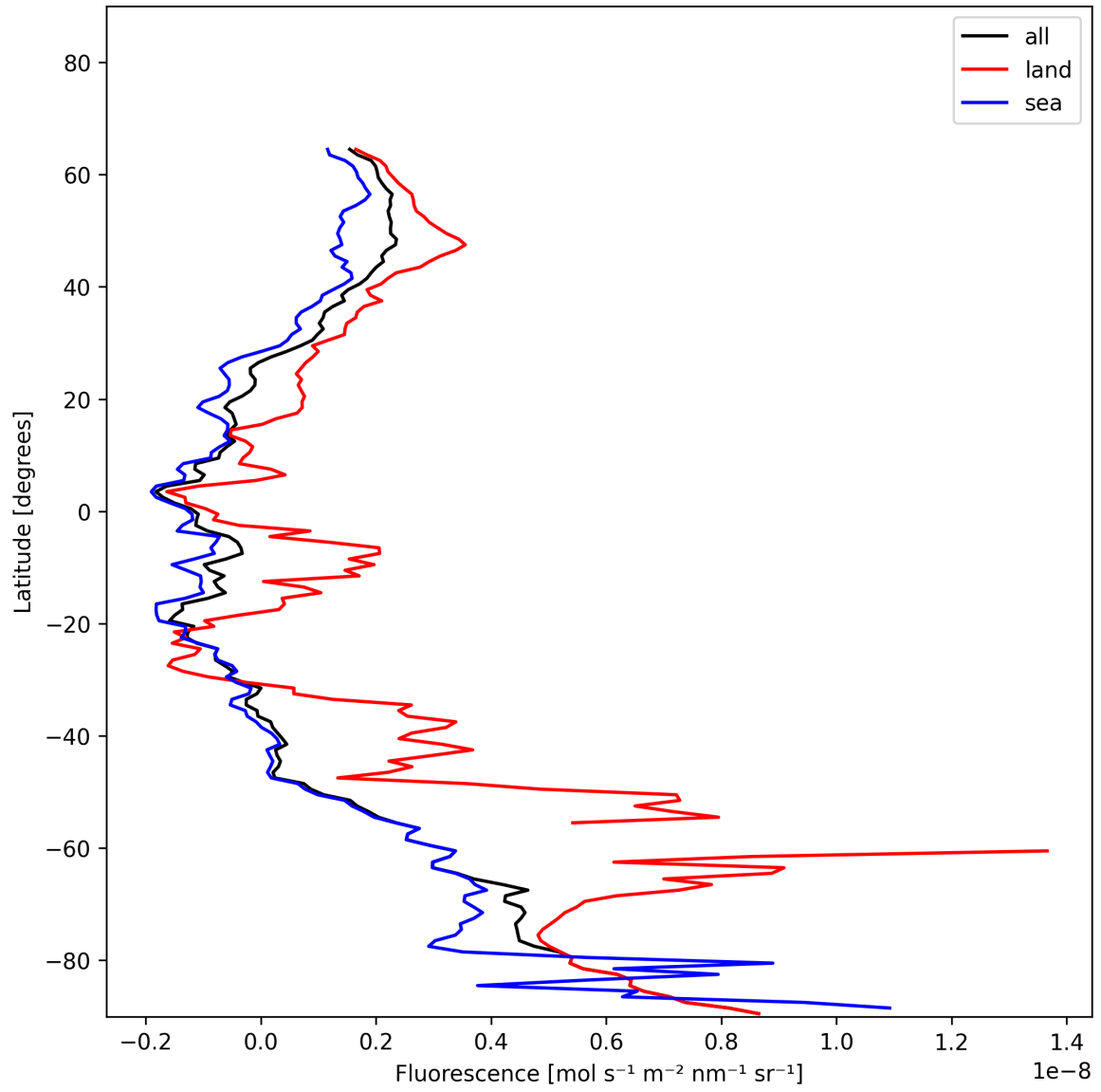
Figure 23: Zonal average of “Fluorescence” for 2024-12-22 to 2024-12-23.
