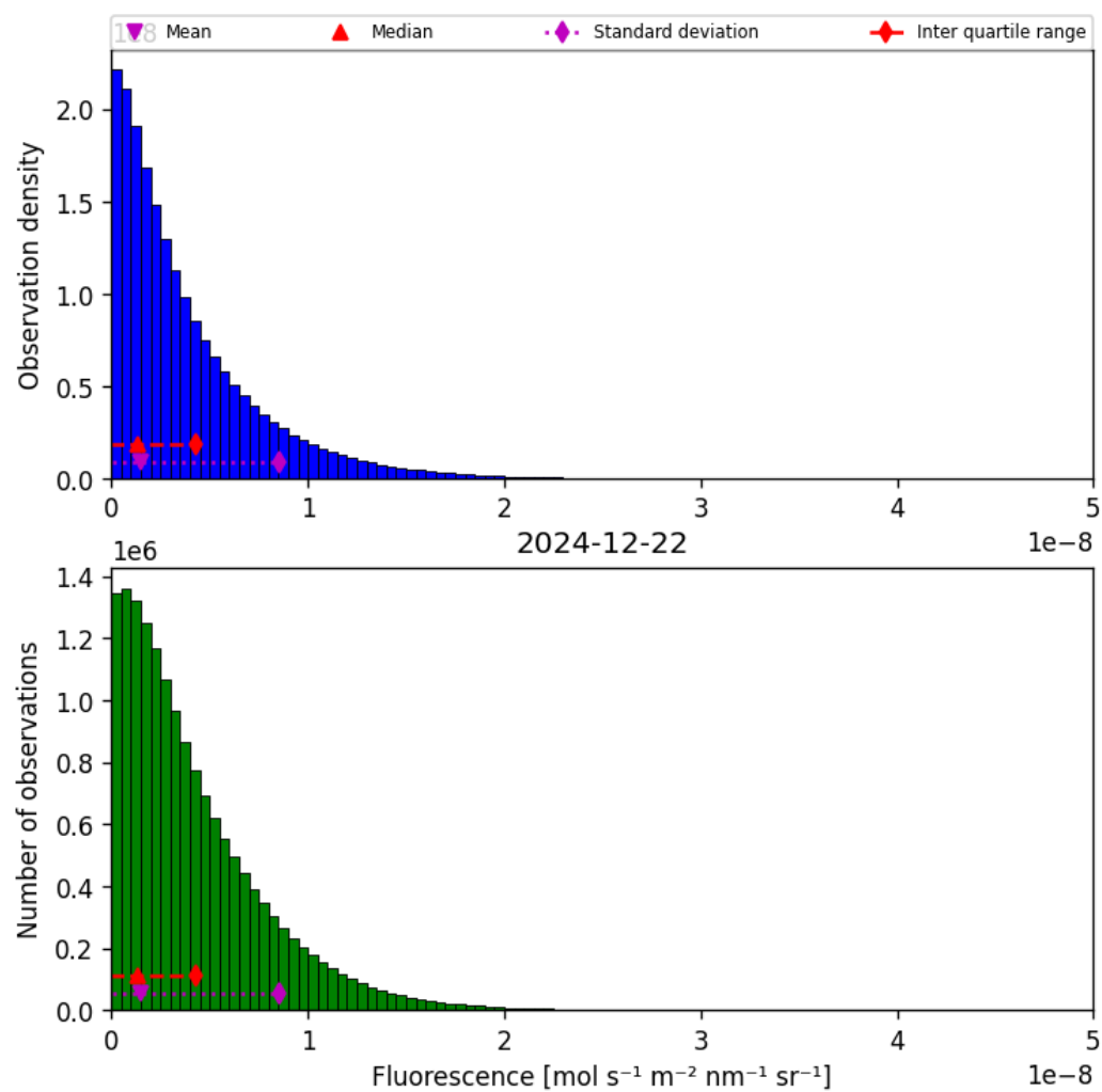
Figure 40: Histogram of “Fluorescence” for 2024-12-22 to 2024-12-23
