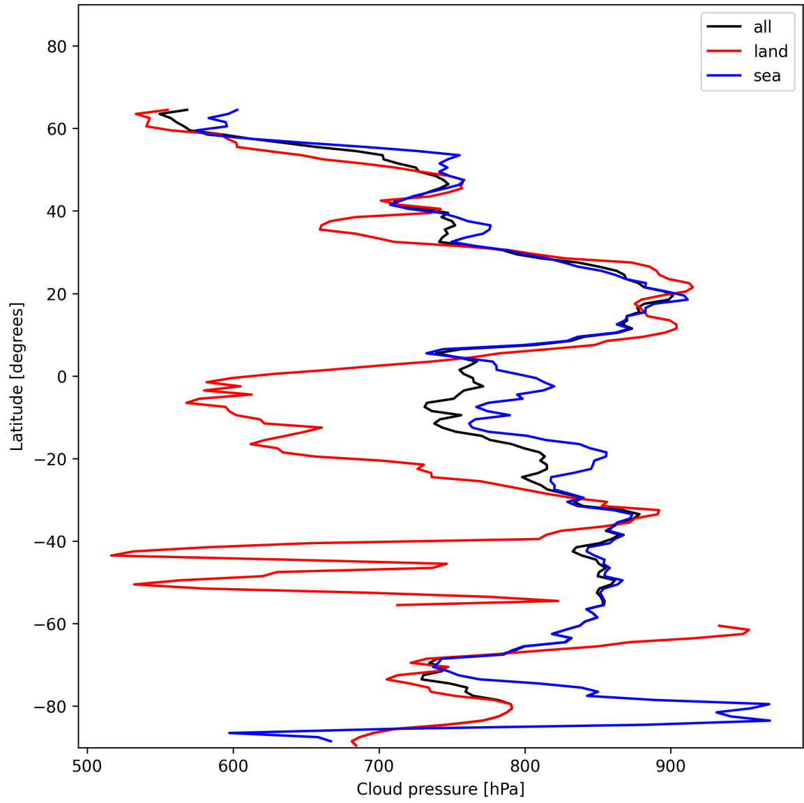
Figure 13: Zonal average of “Cloud pressure” for 2024-12-22 to 2024-12-23.
