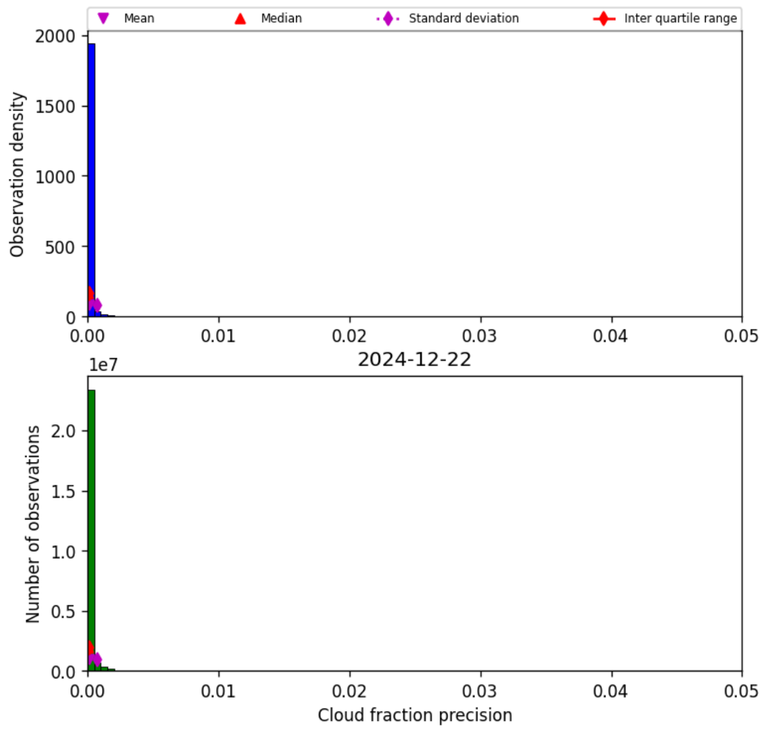
Figure 33: Histogram of “Cloud fraction precision” for 2024-12-22 to 2024-12-23
