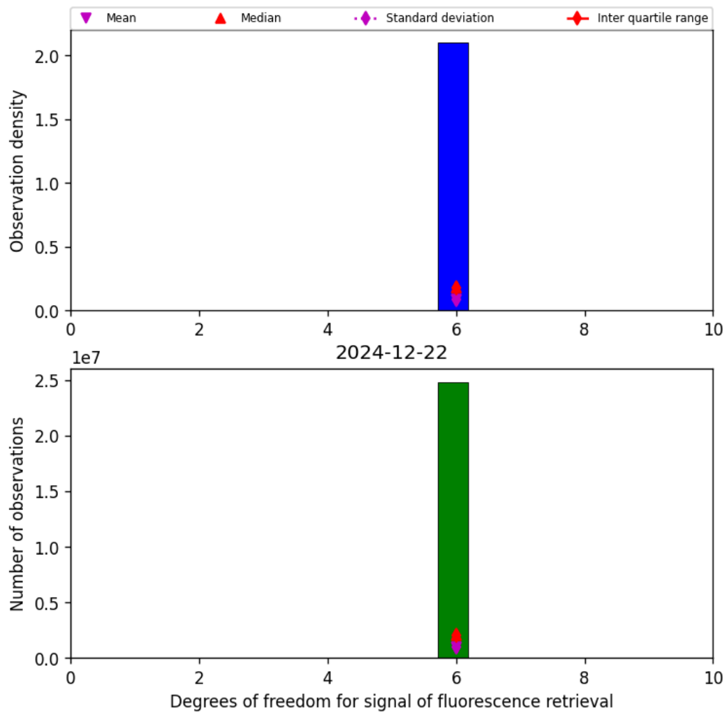
Figure 43: Histogram of “Degrees of freedom for signal of fluorescence retrieval” for 2024-12-22 to 2024-12-23
