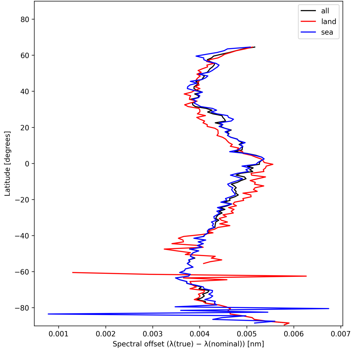
Figure 28: Zonal average of “Spectral offset ( \lambda_{\text{true}} - \lambda_{\text{nominal}} )” for 2024-12-22 to 2024-12-23.
