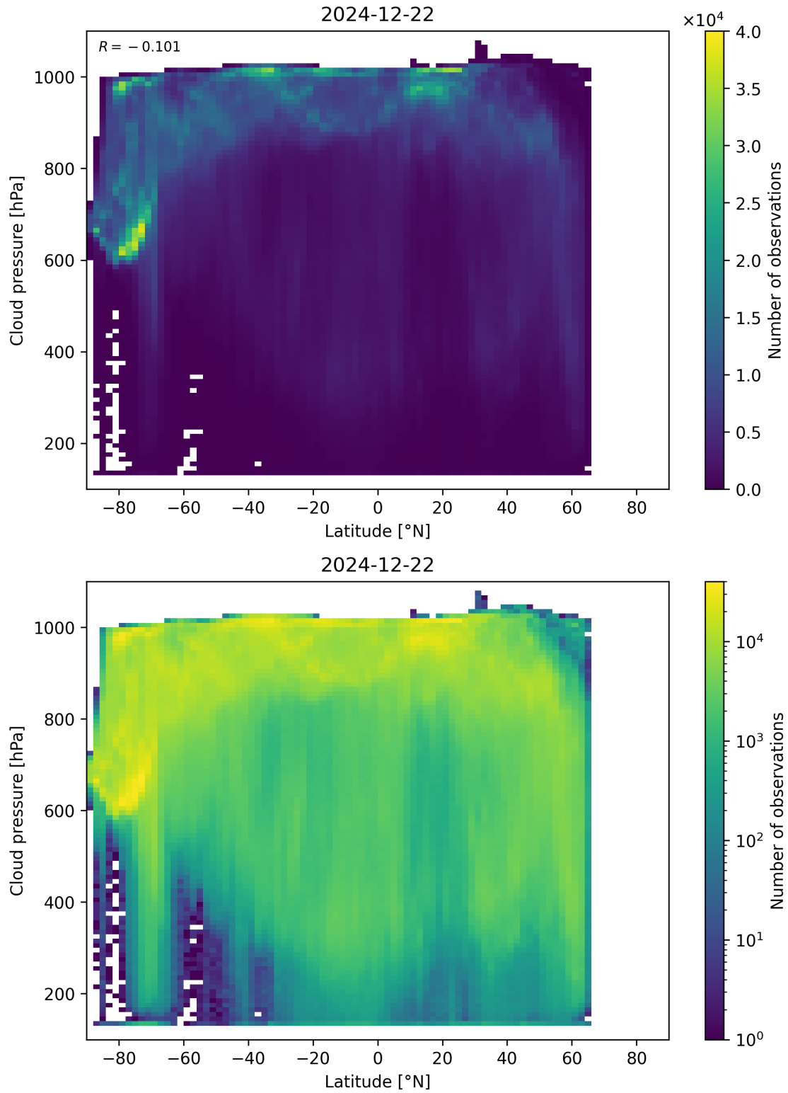
Figure 91: Scatter density plot of “Latitude” against “Cloud pressure” for 2024-12-22 to 2024-12-23.
