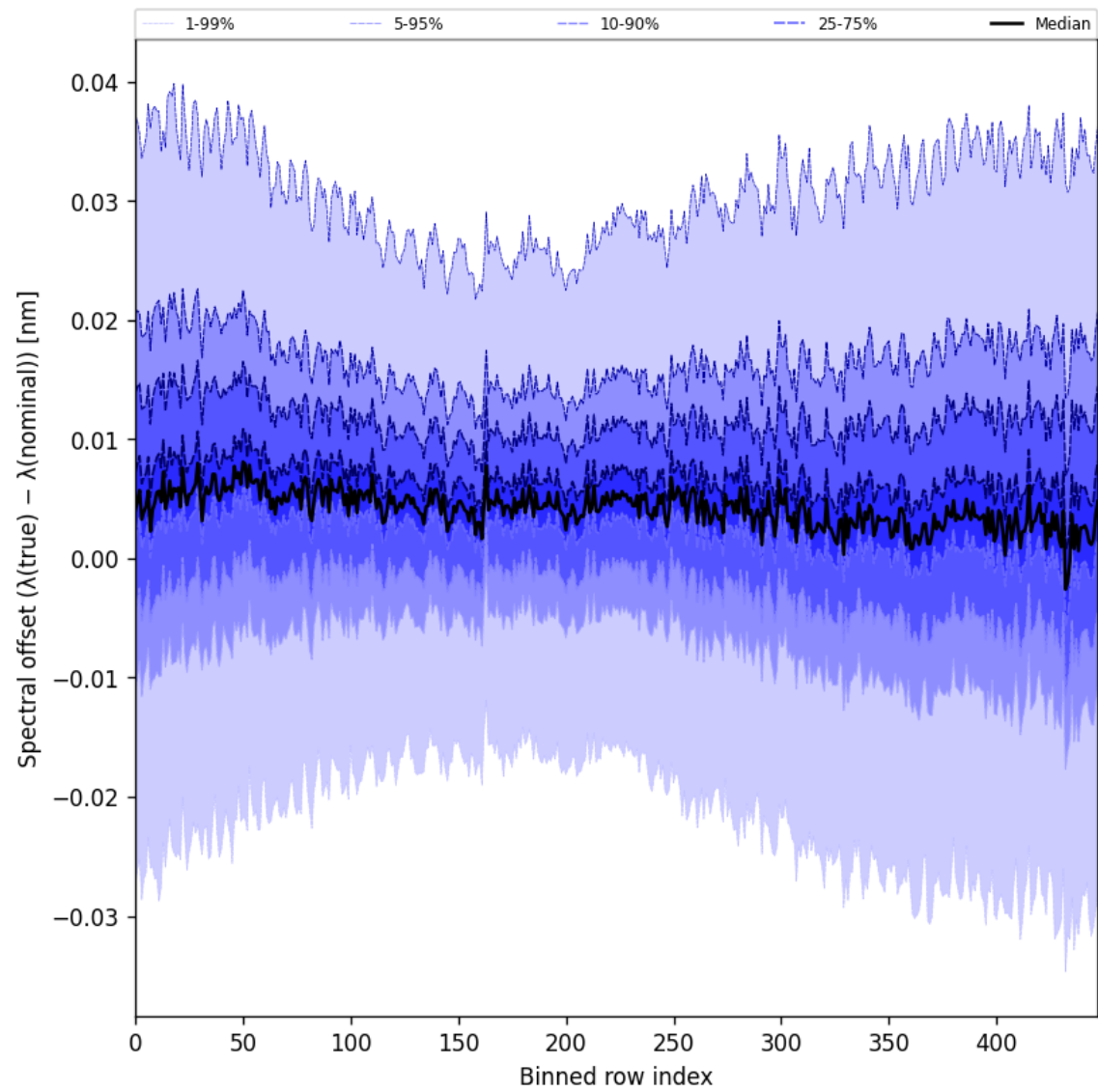
Figure 62: Along track statistics of “Spectral offset ( \lambda_{\text{true}} - \lambda_{\text{nominal}} )” for 2024-12-22 to 2024-12-23
