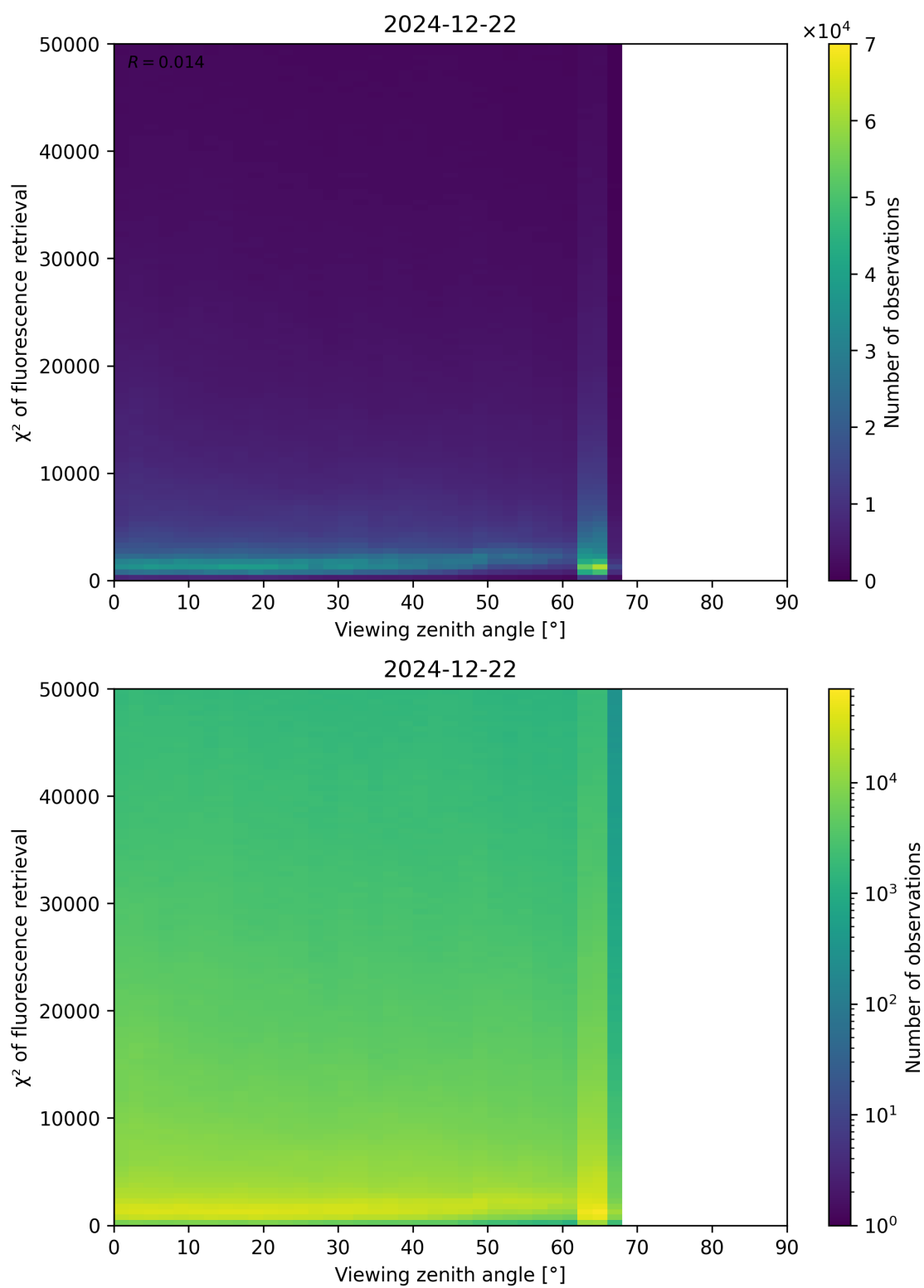
Figure 119: Scatter density plot of “Viewing zenith angle” against “ \chi^2 of fluorescence retrieval” for 2024-12-22 to 2024-12-23.
