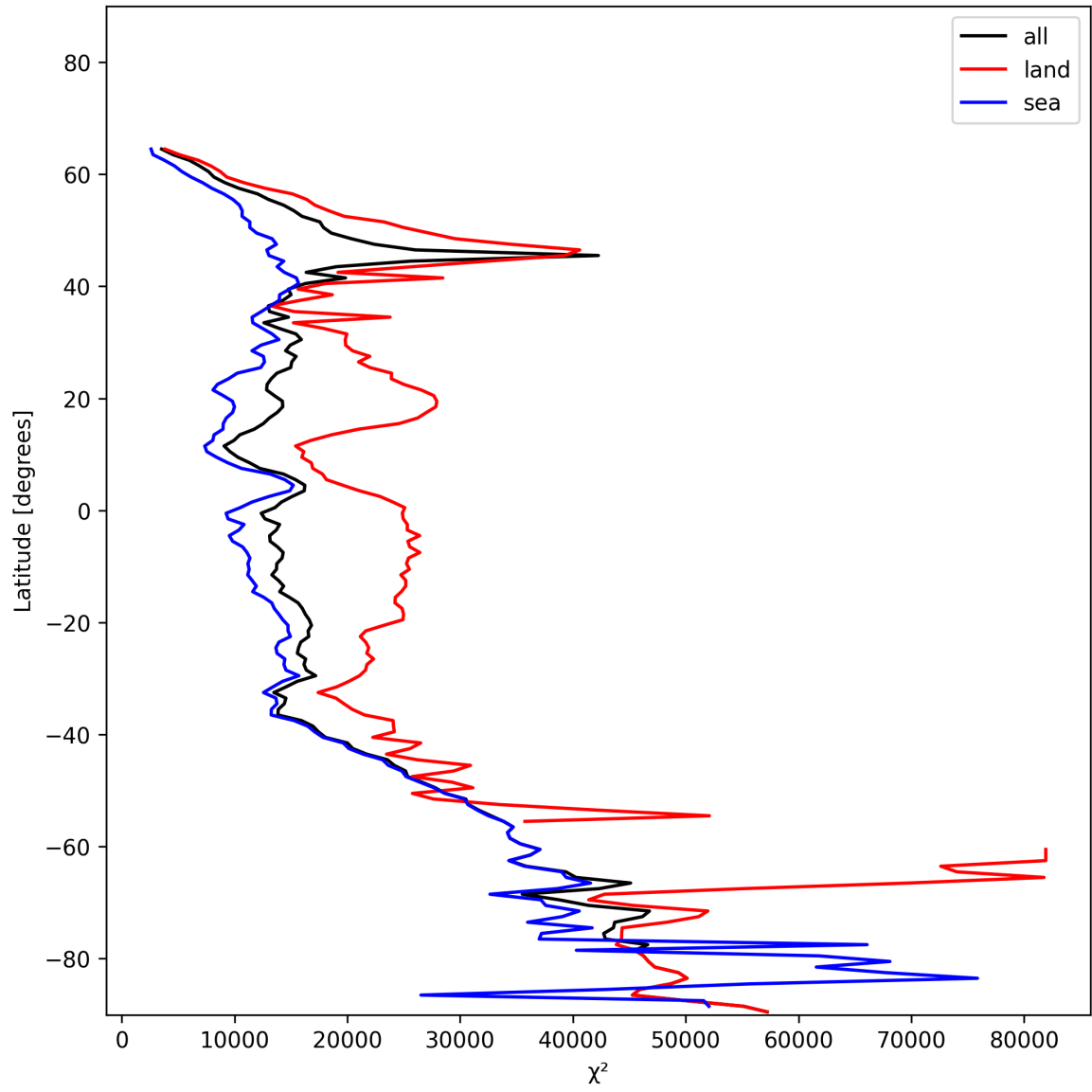
Figure 21: Zonal average of “ \chi^2 ” for 2024-12-22 to 2024-12-23.
