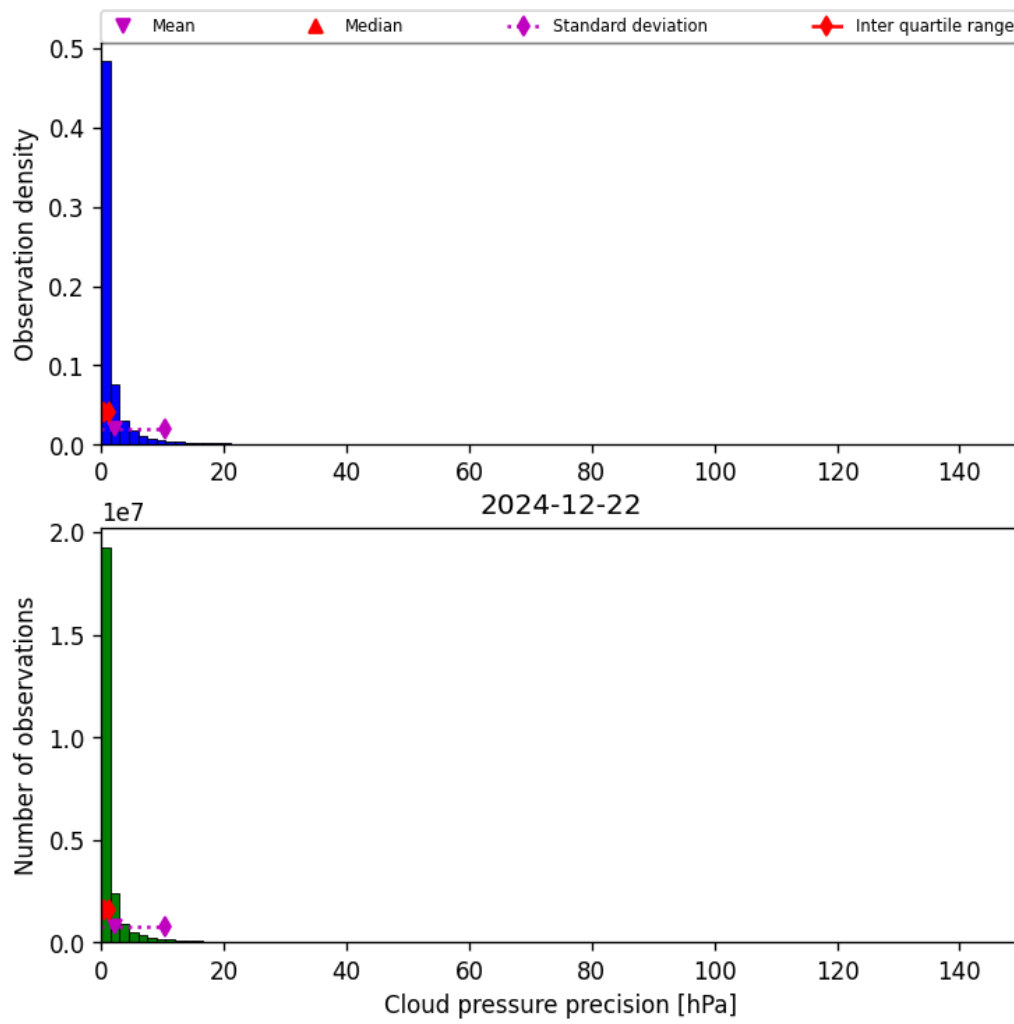
Figure 31: Histogram of “Cloud pressure precision” for 2024-12-22 to 2024-12-23
