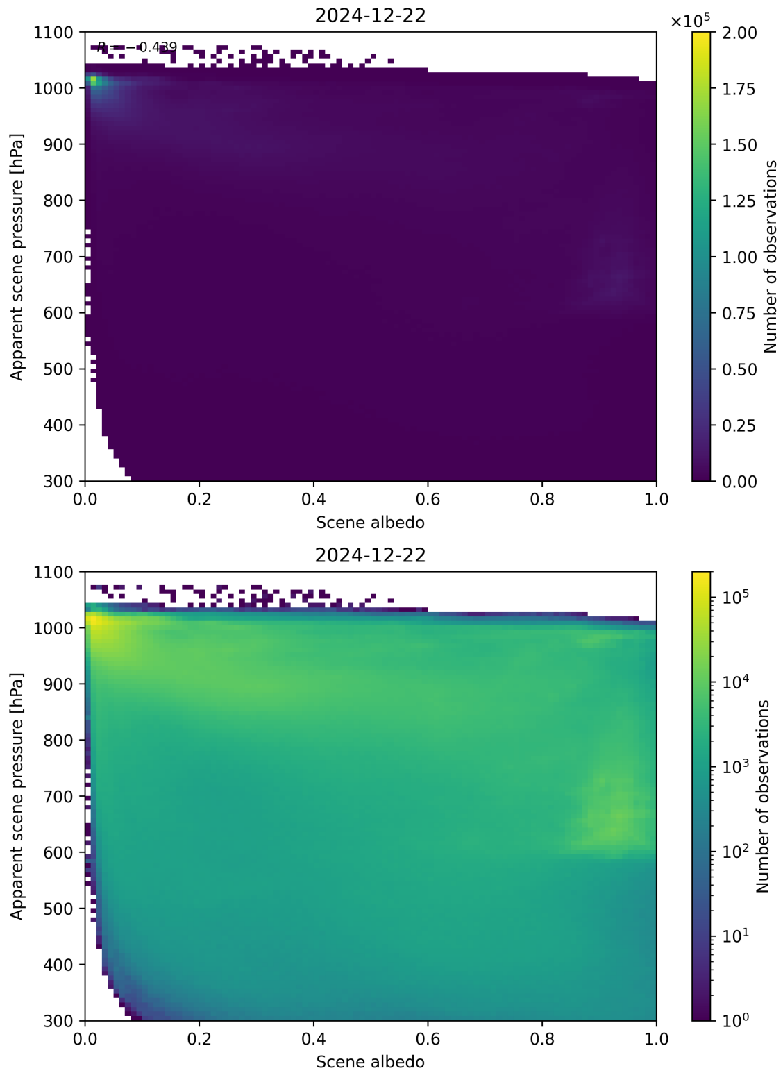
Figure 102: Scatter density plot of “Scene albedo” against “Apparent scene pressure” for 2024-12-22 to 2024-12-23.
