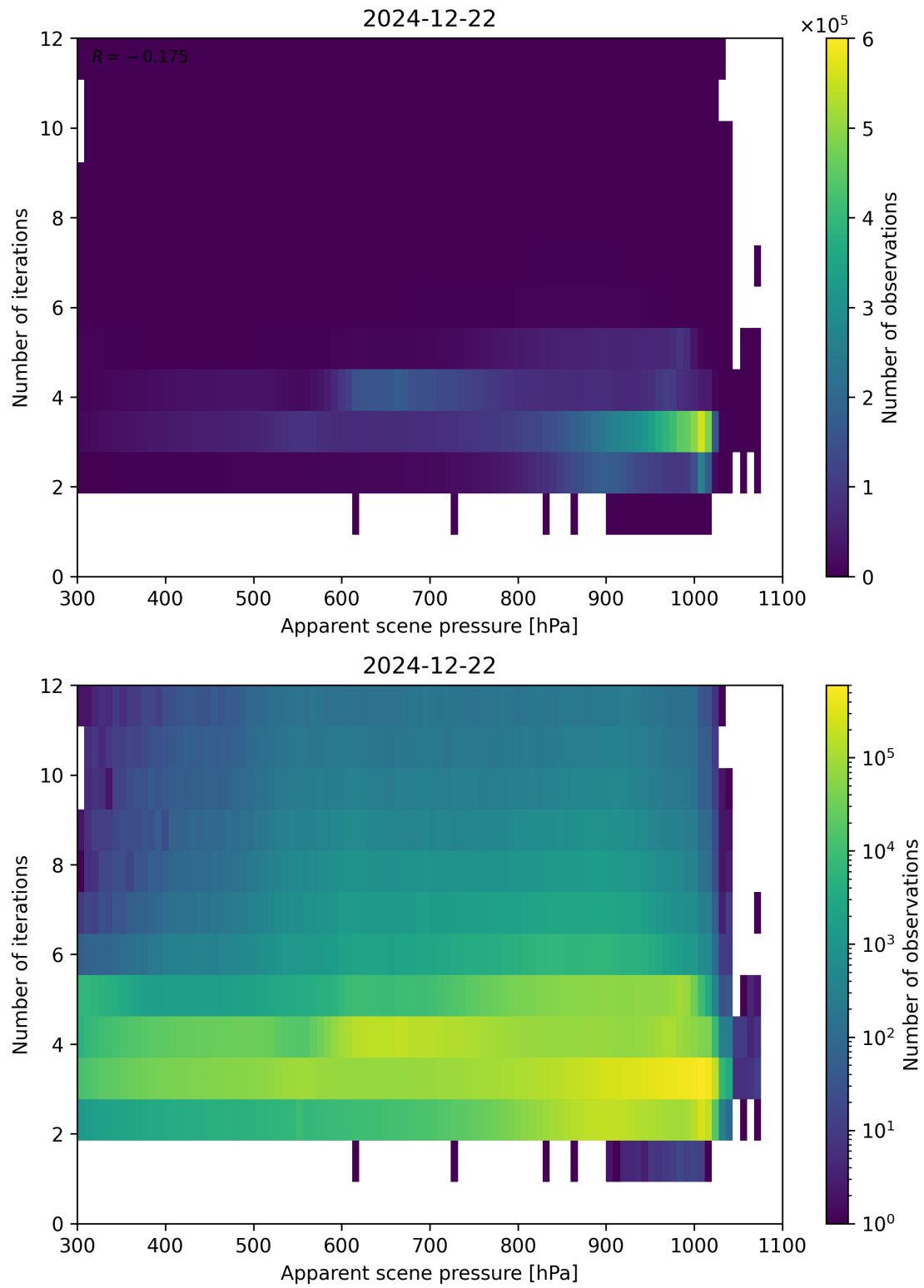
Figure 65: Scatter density plot of “Apparent scene pressure” against “Number of iterations” for 2024-12-22 to 2024-12-23.
