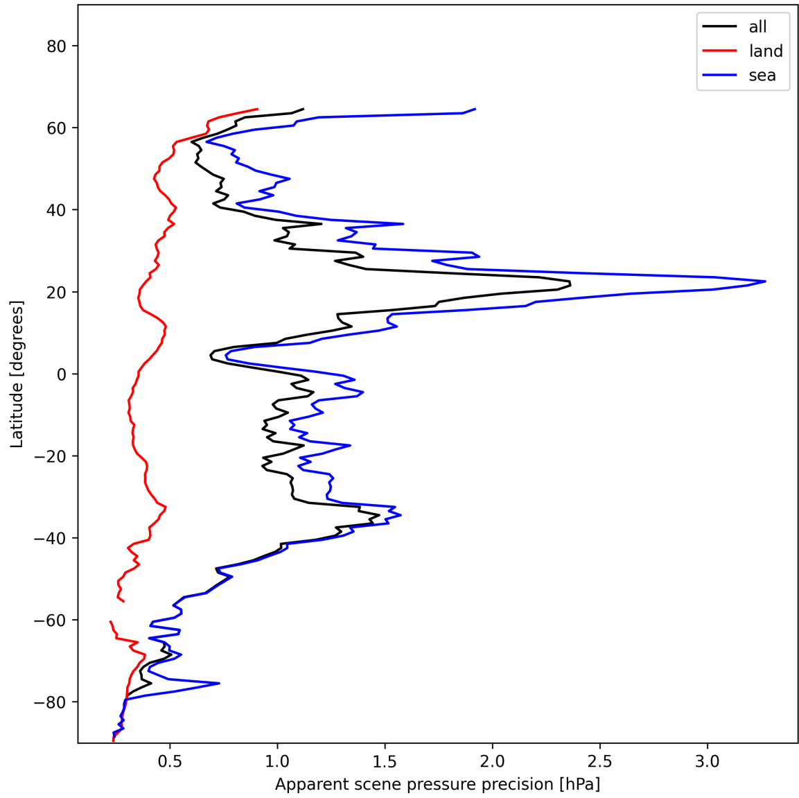
Figure 20: Zonal average of “Apparent scene pressure precision” for 2024-12-22 to 2024-12-23.
