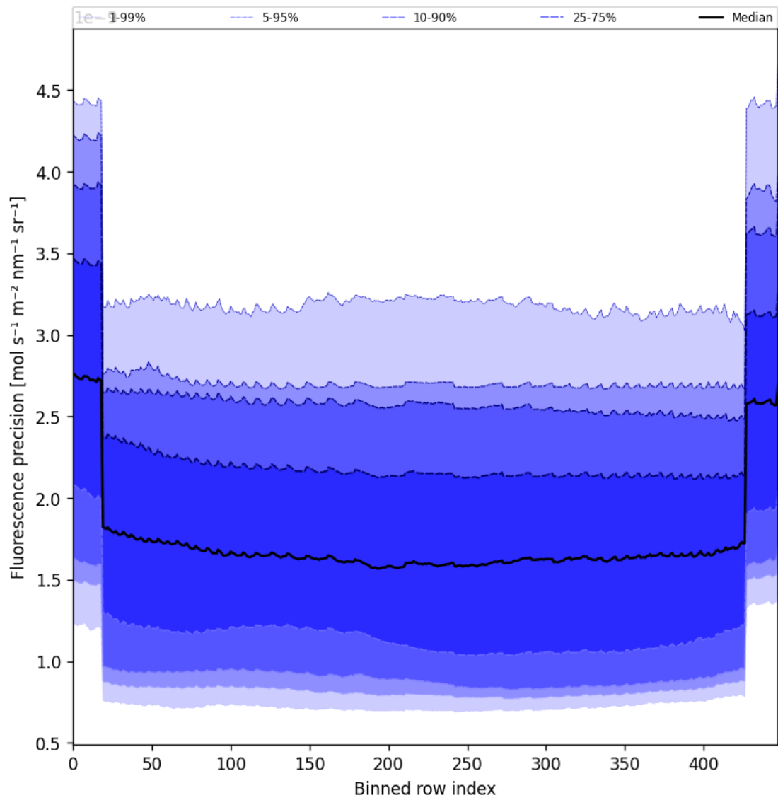
Figure 58: Along track statistics of “Fluorescence precision” for 2024-12-22 to 2024-12-23
