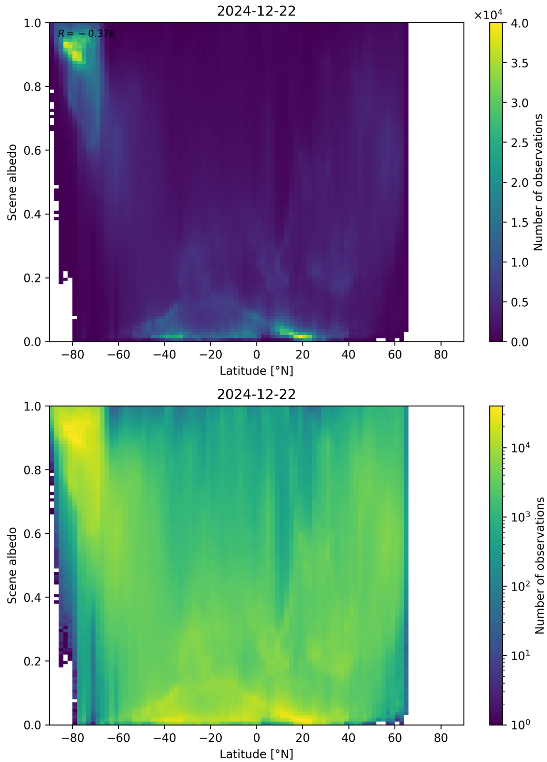
Figure 95: Scatter density plot of “Latitude” against “Scene albedo” for 2024-12-22 to 2024-12-23.
