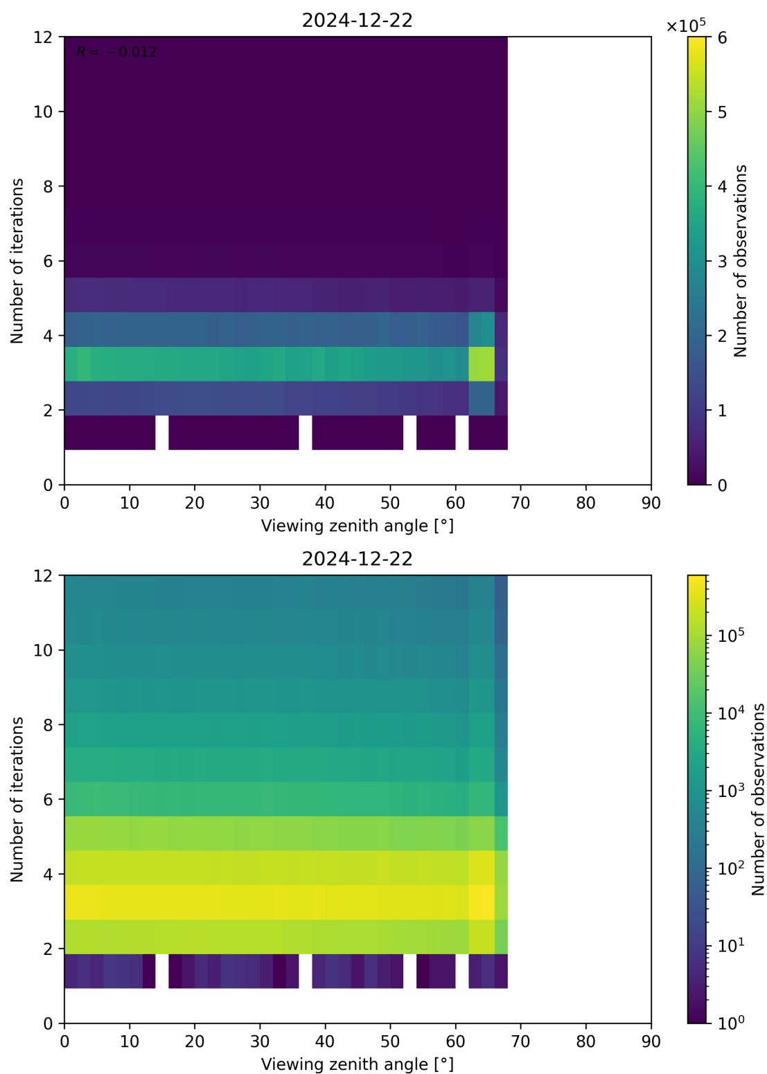
Figure 124: Scatter density plot of “Viewing zenith angle” against “Number of iterations” for 2024-12-22 to 2024-12-23.
