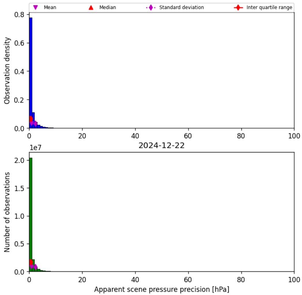
Figure 37: Histogram of “Apparent scene pressure precision” for 2024-12-22 to 2024-12-23
