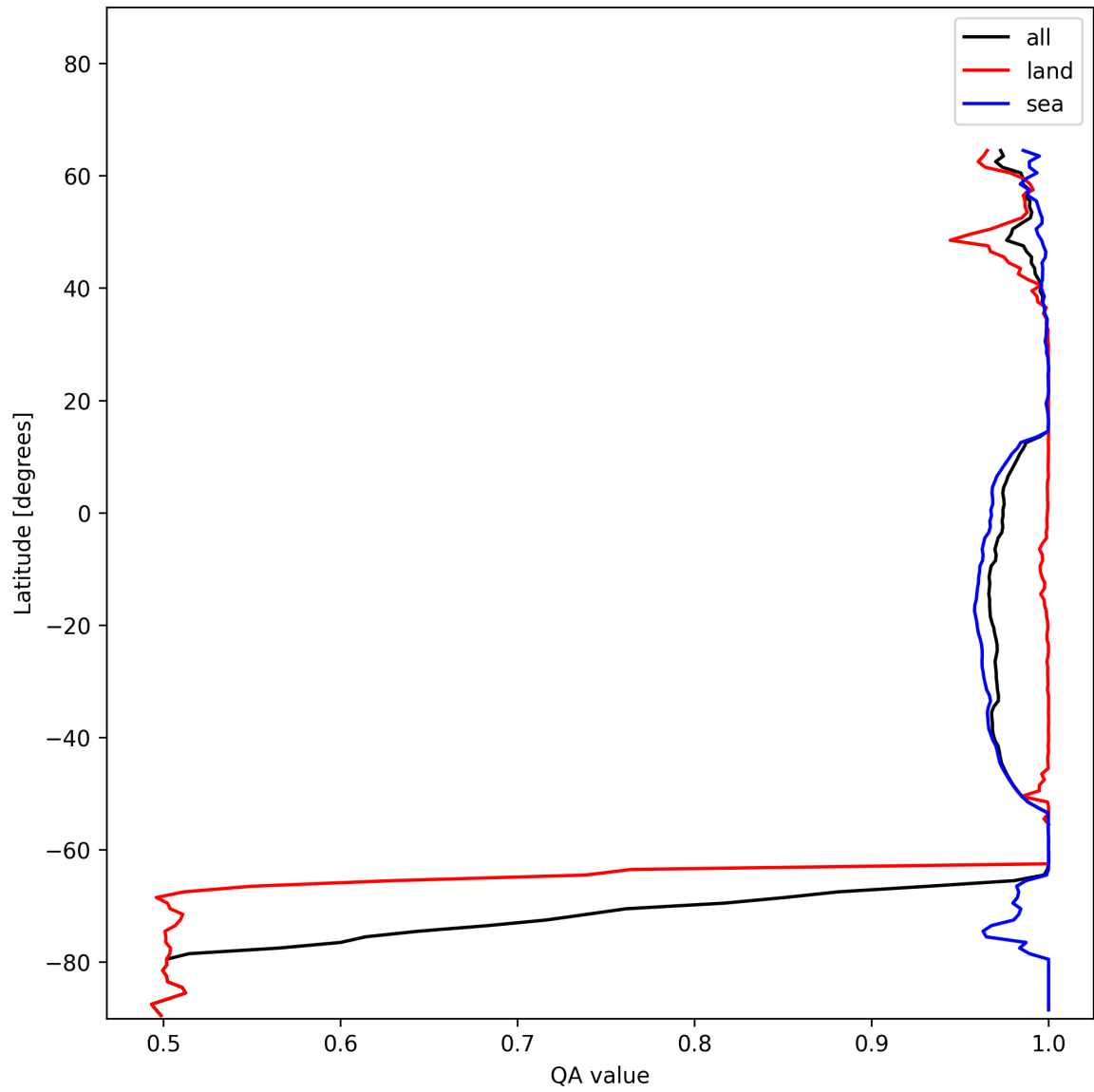
Figure 12: Zonal average of “QA value” for 2024-12-22 to 2024-12-23.
