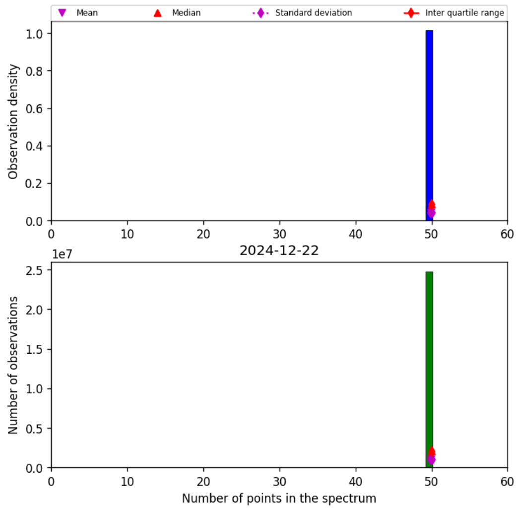
Figure 44: Histogram of “Number of points in the spectrum” for 2024-12-22 to 2024-12-23
