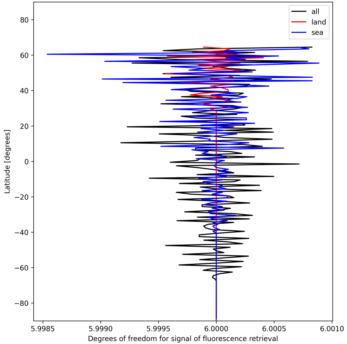
Figure 26: Zonal average of “Degrees of freedom for signal of fluorescence retrieval” for 2024-12-22 to 2024-12-23.
