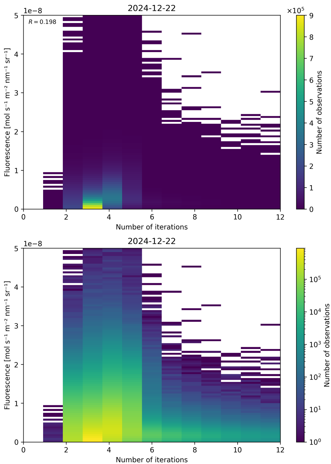
Figure 98: Scatter density plot of “Number of iterations” against “Fluorescence” for 2024-12-22 to 2024-12-23.
