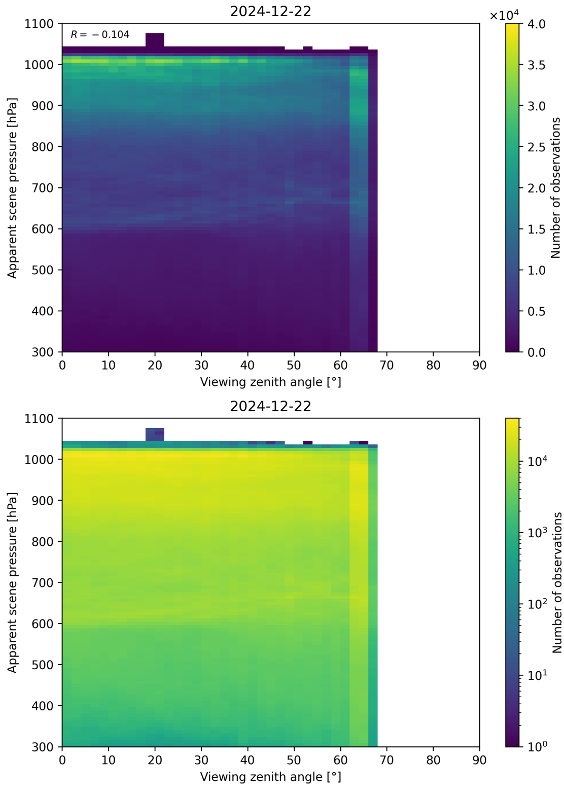
Figure 118: Scatter density plot of “Viewing zenith angle” against “Apparent scene pressure” for 2024-12-22 to 2024-12-23.
