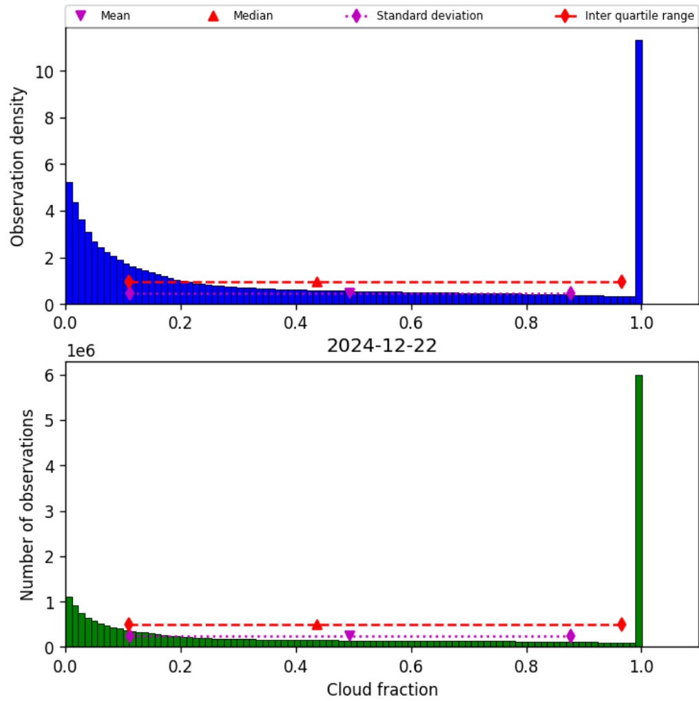
Figure 32: Histogram of “Cloud fraction” for 2024-12-22 to 2024-12-23
