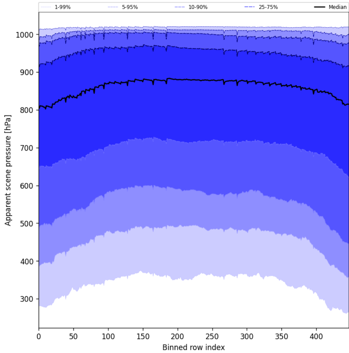
Figure 53: Along track statistics of “Apparent scene pressure” for 2024-12-22 to 2024-12-23
