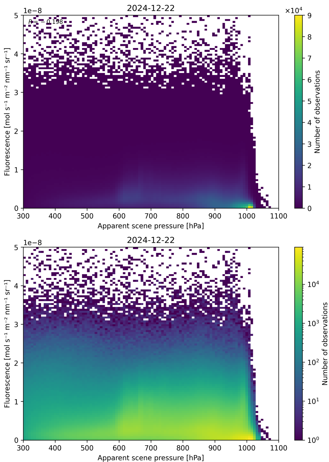
Figure 64: Scatter density plot of “Apparent scene pressure” against “Fluorescence” for 2024-12-22 to 2024-12-23.
