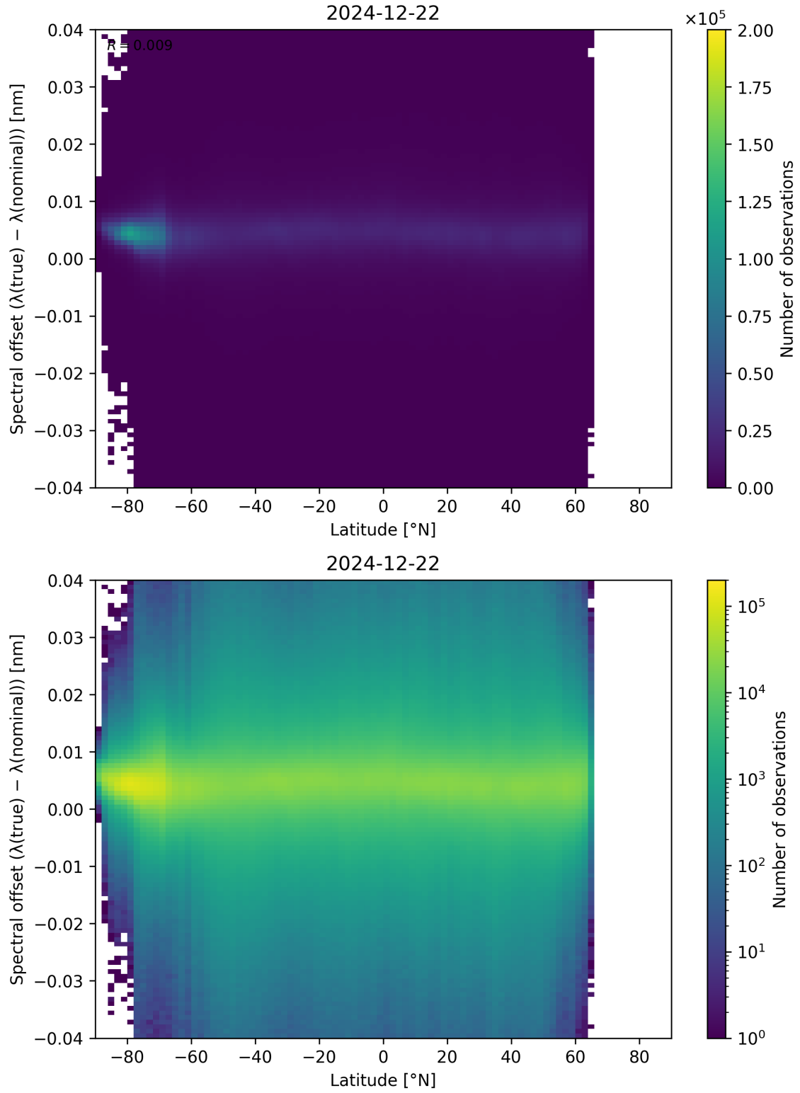
Figure 96: Scatter density plot of “Latitude” against “Spectral offset ( \lambda_{\text{true}} - \lambda_{\text{nominal}} )” for 2024-12-22 to 2024-12-23.
