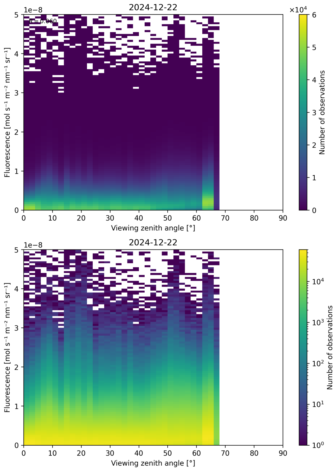
Figure 122: Scatter density plot of “Viewing zenith angle” against “Fluorescence” for 2024-12-22 to 2024-12-23.
