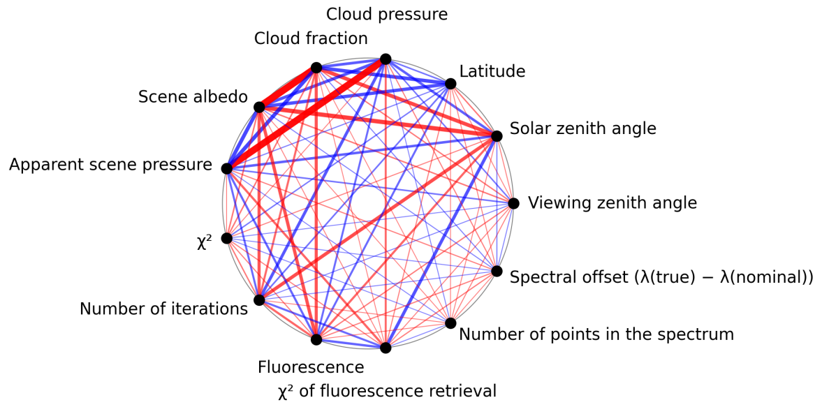
Figure 1: Map of correlation graph for 2024-12-22 to 2024-12-23.
