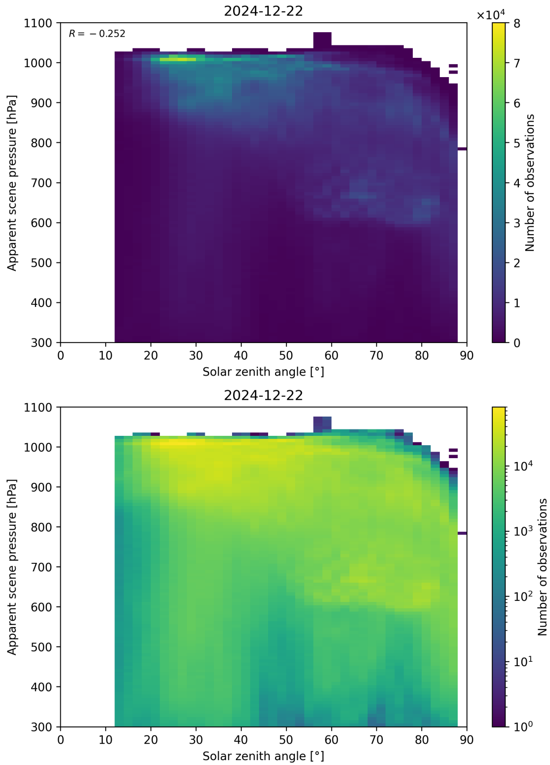
Figure 108: Scatter density plot of “Solar zenith angle” against “Apparent scene pressure” for 2024-12-22 to 2024-12-23.
