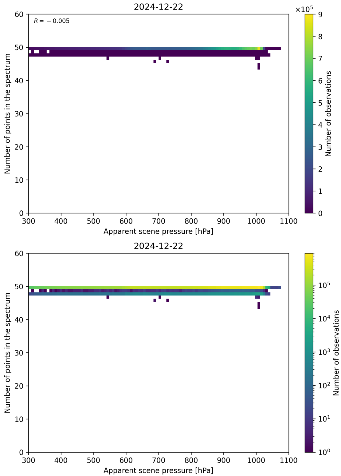
Figure 66: Scatter density plot of “Apparent scene pressure” against “Number of points in the spectrum” for 2024-12-22 to 2024-12-23.
