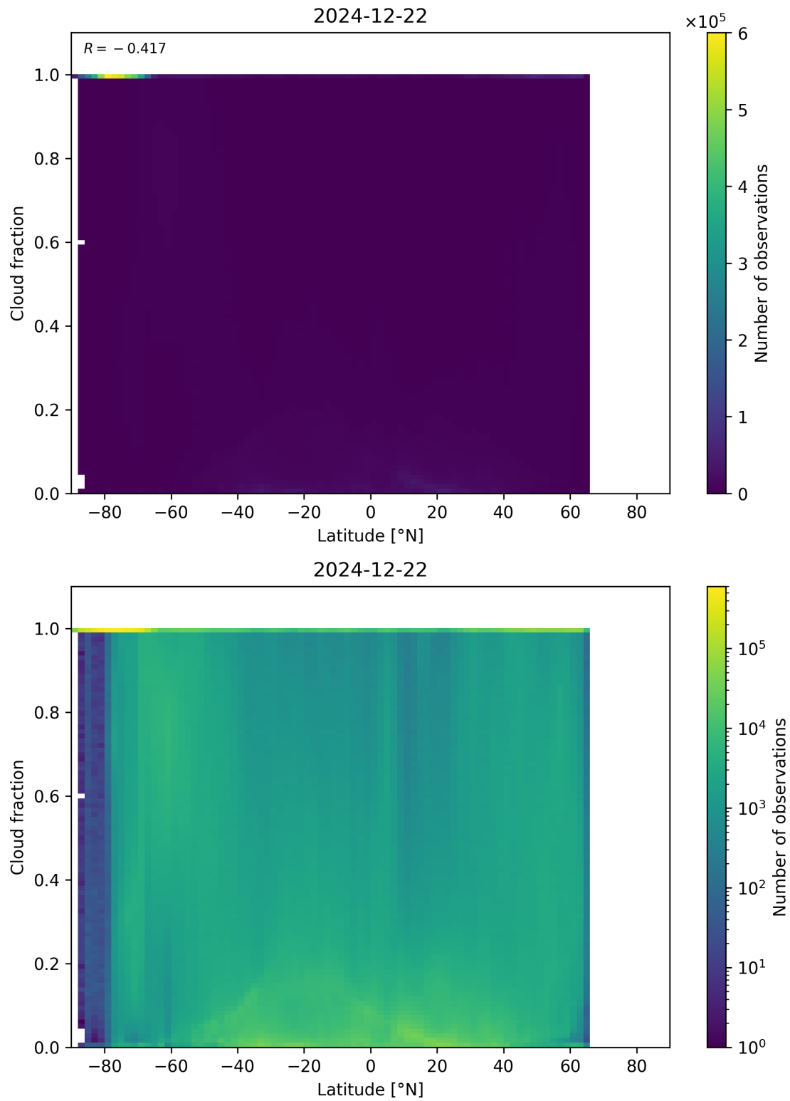
Figure 90: Scatter density plot of “Latitude” against “Cloud fraction” for 2024-12-22 to 2024-12-23.
