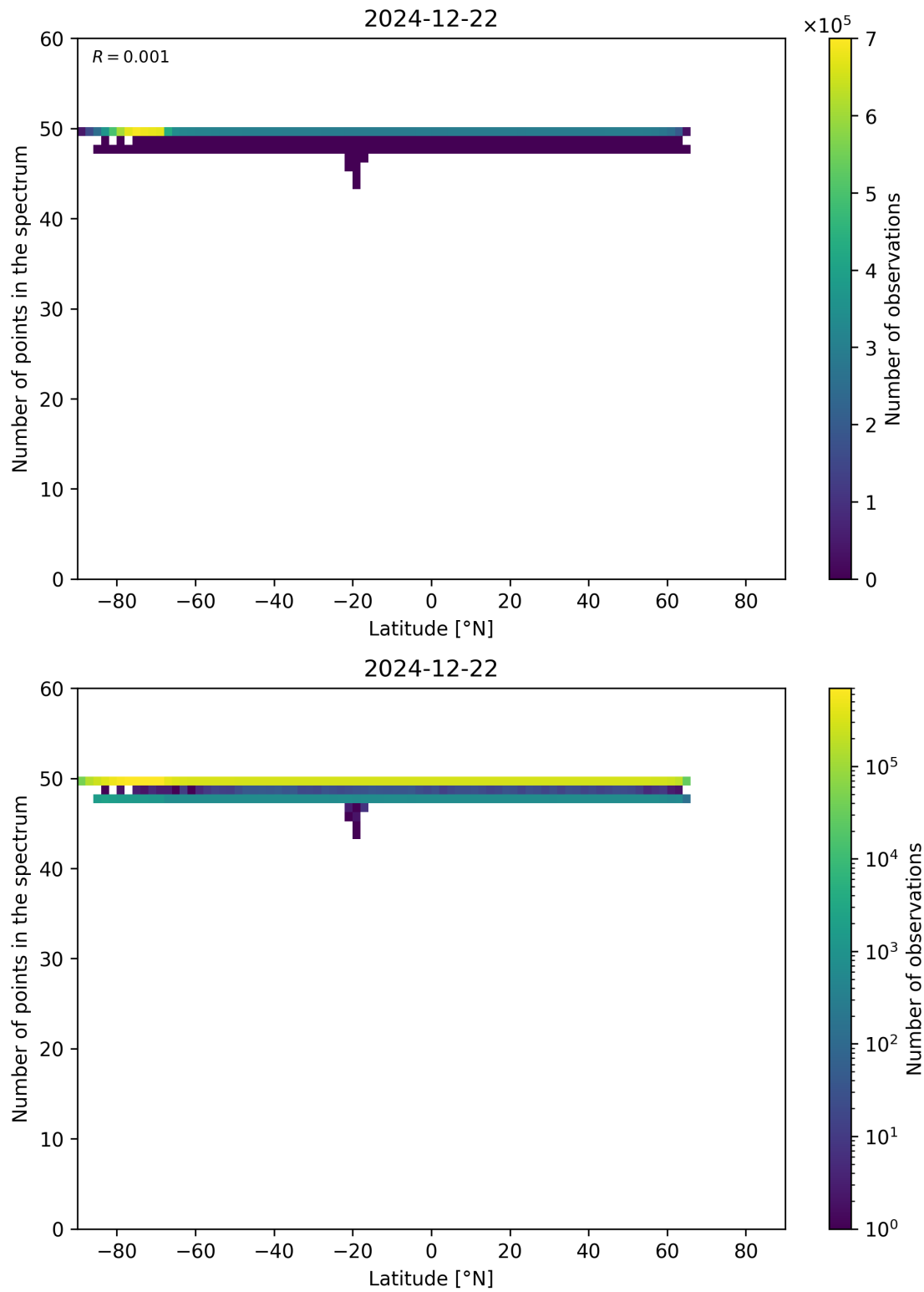
Figure 94: Scatter density plot of “Latitude” against “Number of points in the spectrum” for 2024-12-22 to 2024-12-23.
