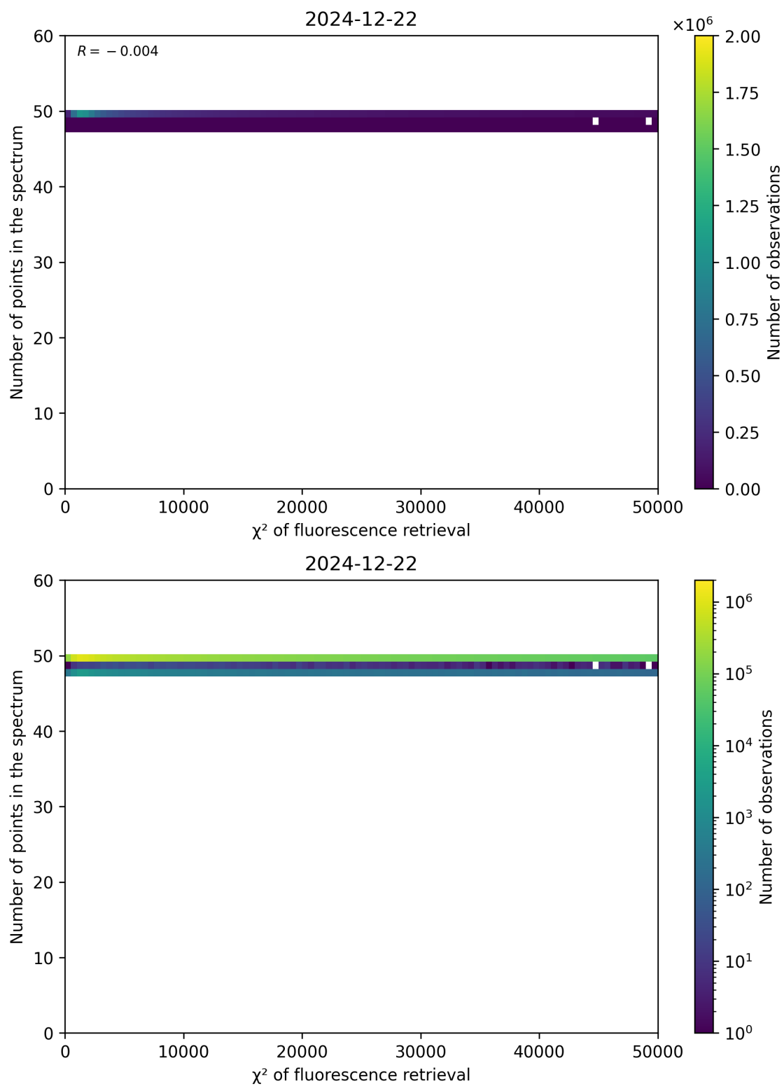
Figure 68: Scatter density plot of “ \chi^2 of fluorescence retrieval” against “Number of points in the spectrum” for 2024-12-22 to 2024-12-23.
