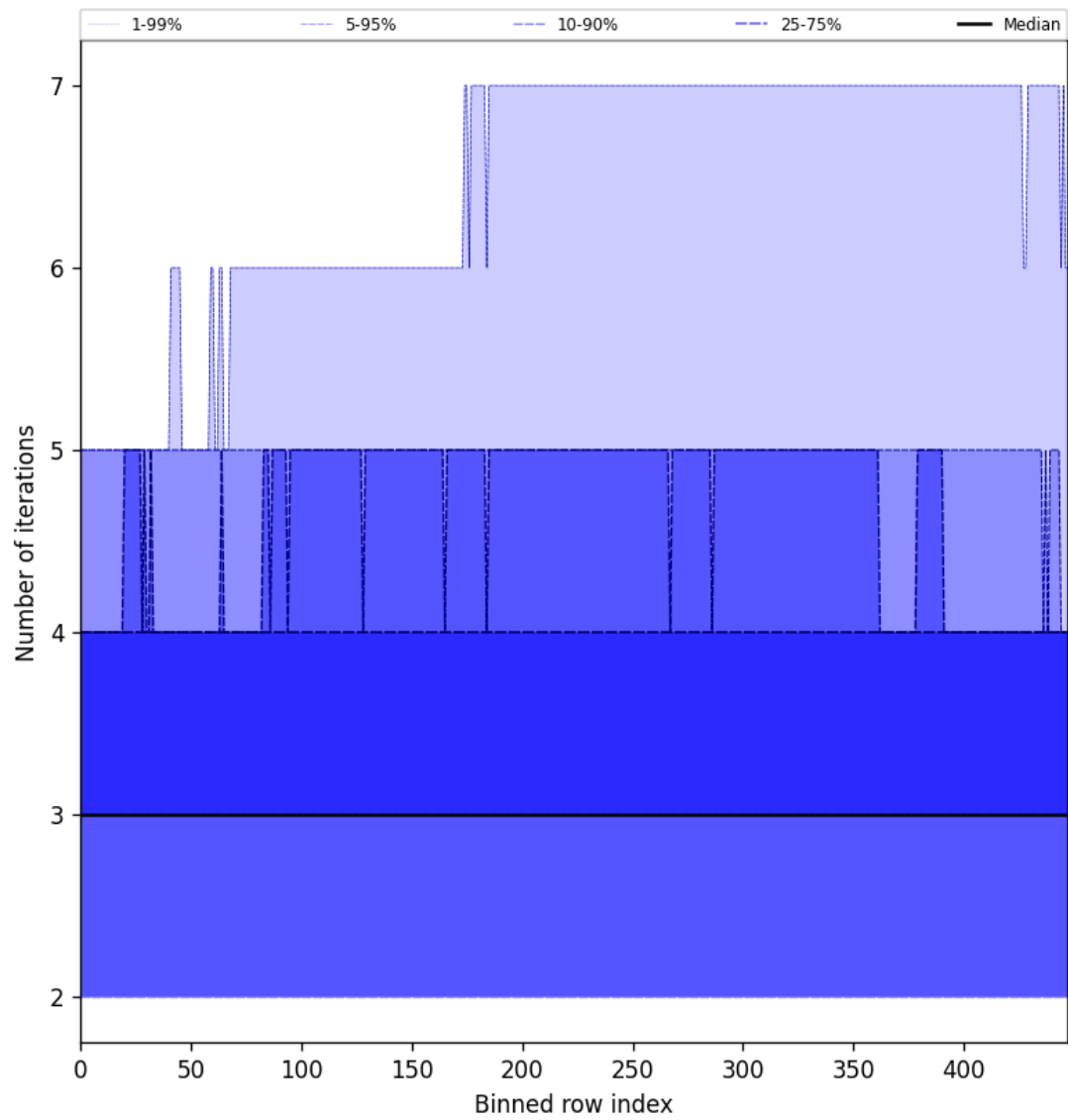
Figure 56: Along track statistics of “Number of iterations” for 2024-12-22 to 2024-12-23
