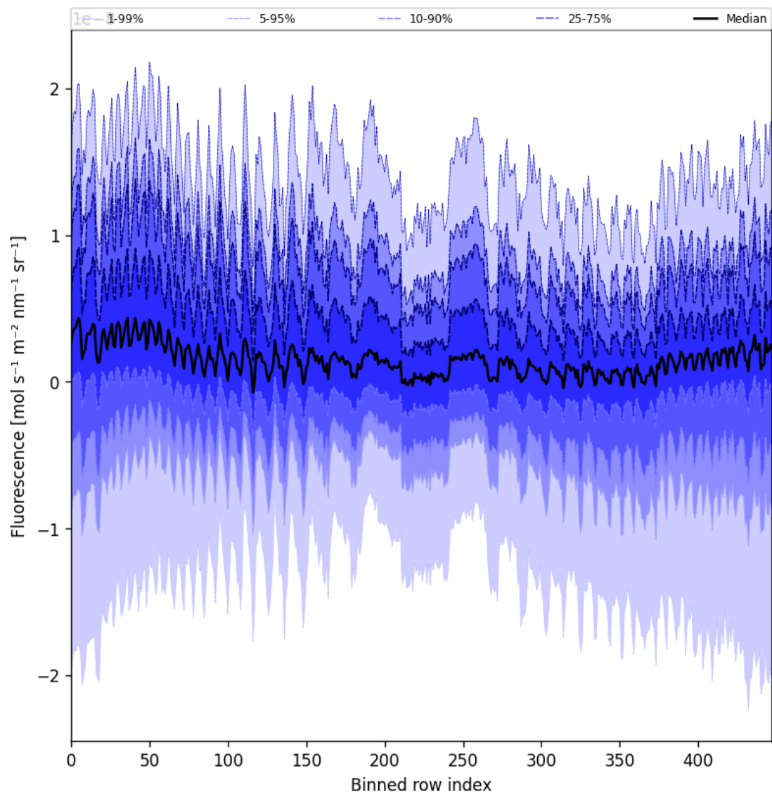
Figure 57: Along track statistics of “Fluorescence” for 2024-12-22 to 2024-12-23
