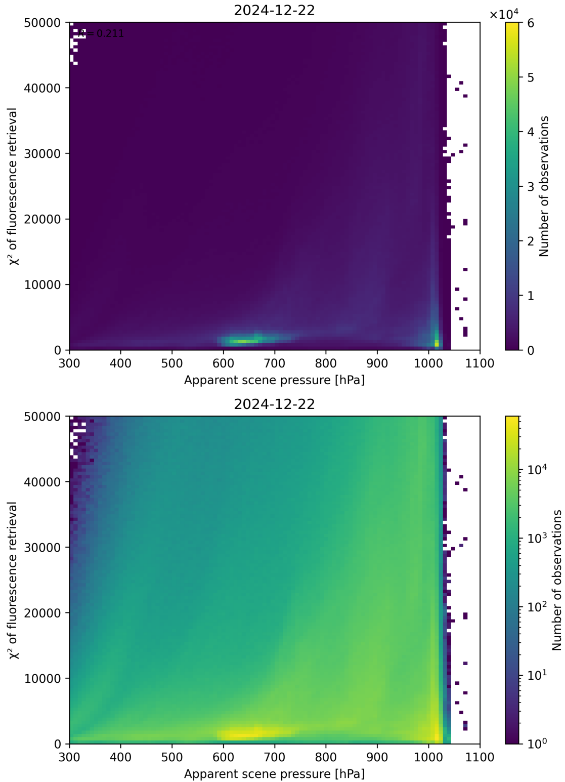
Figure 63: Scatter density plot of “Apparent scene pressure” against “ \chi^2 of fluorescence retrieval” for 2024-12-22 to 2024-12-23.
