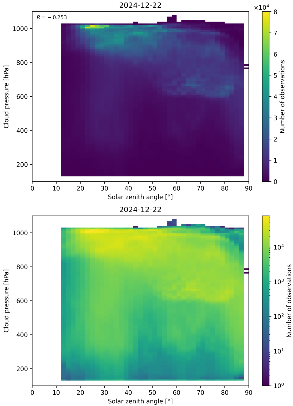
Figure 111: Scatter density plot of “Solar zenith angle” against “Cloud pressure” for 2024-12-22 to 2024-12-23.
