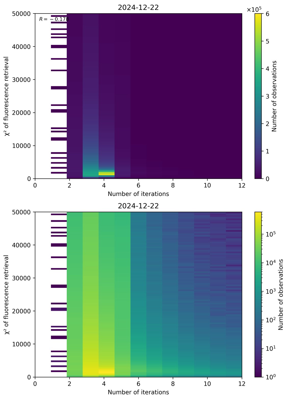
Figure 97: Scatter density plot of “Number of iterations” against “ \chi^2 of fluorescence retrieval” for 2024-12-22 to 2024-12-23.
