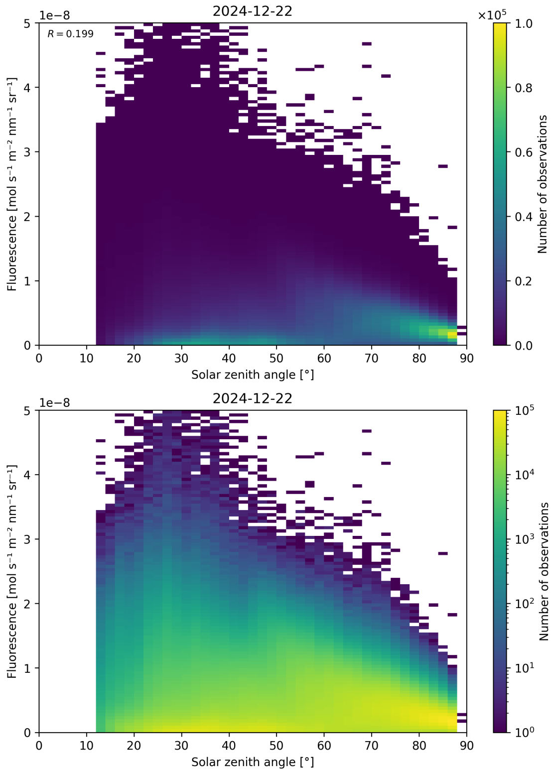
Figure 112: Scatter density plot of “Solar zenith angle” against “Fluorescence” for 2024-12-22 to 2024-12-23.
