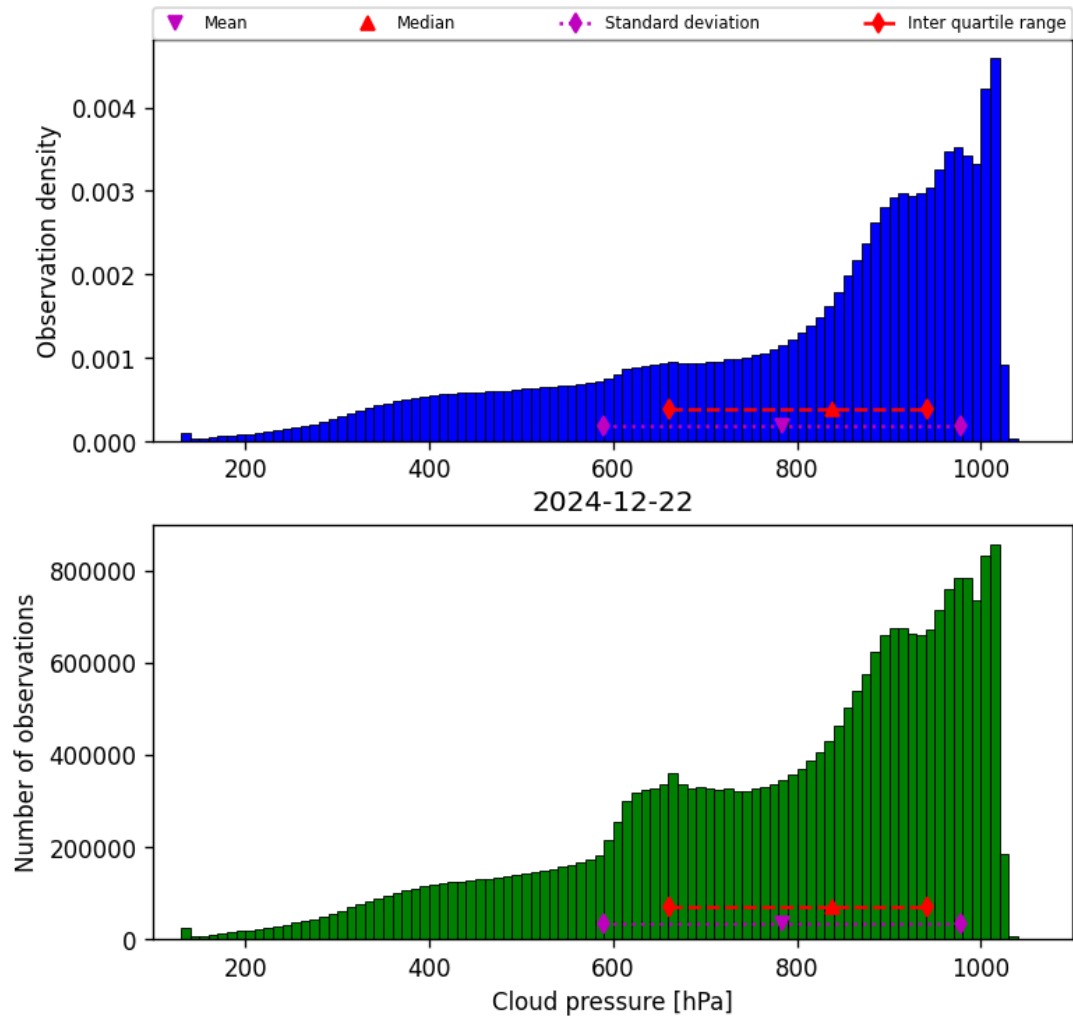
Figure 30: Histogram of “Cloud pressure” for 2024-12-22 to 2024-12-23
