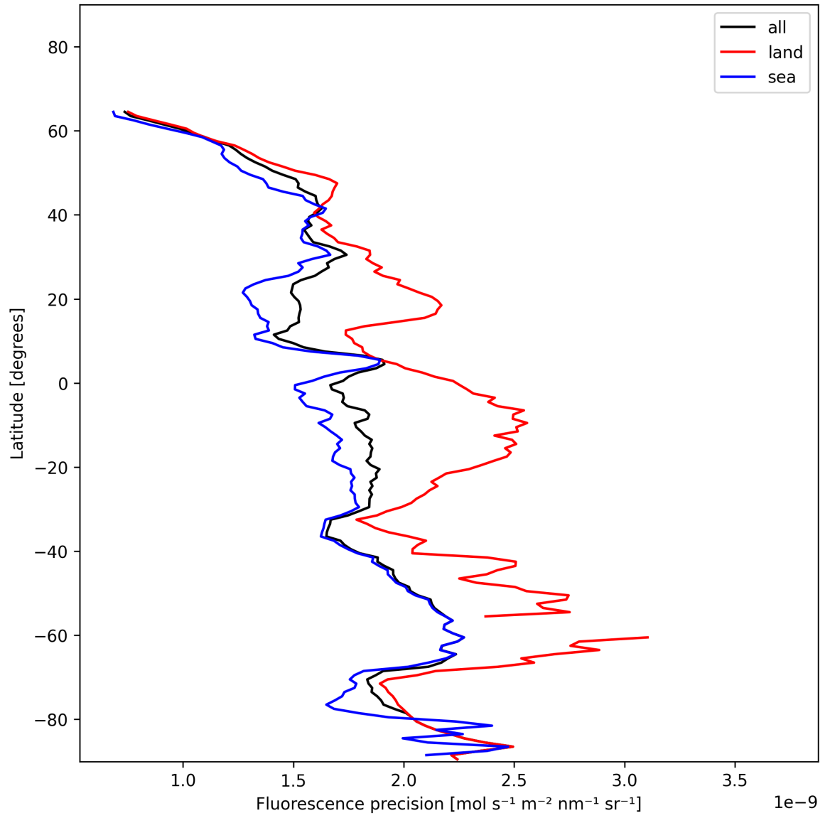
Figure 24: Zonal average of “Fluorescence precision” for 2024-12-22 to 2024-12-23.
