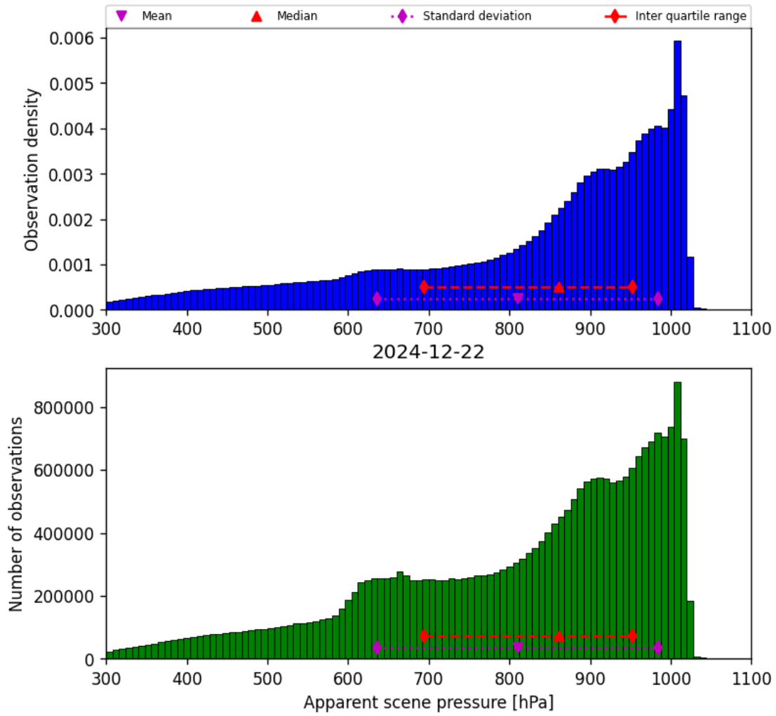
Figure 36: Histogram of “Apparent scene pressure” for 2024-12-22 to 2024-12-23
