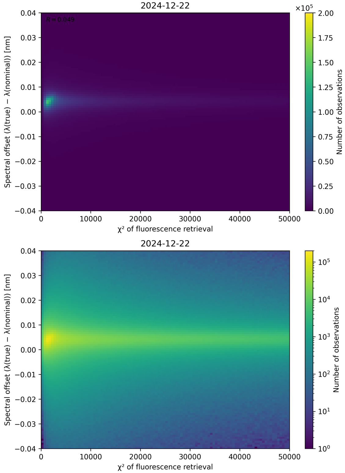
Figure 69: Scatter density plot of “ \chi^2 of fluorescence retrieval” against “Spectral offset ( \lambda_{\text{true}} - \lambda_{\text{nominal}} )” for 2024-12-22 to 2024-12-23.
