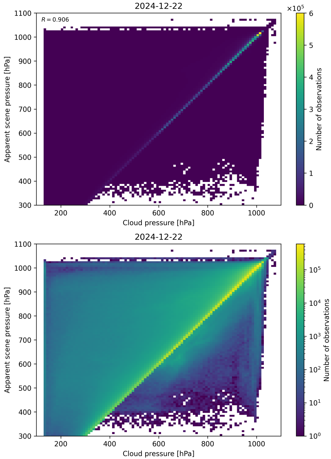
Figure 77: Scatter density plot of “Cloud pressure” against “Apparent scene pressure” for 2024-12-22 to 2024-12-23.
