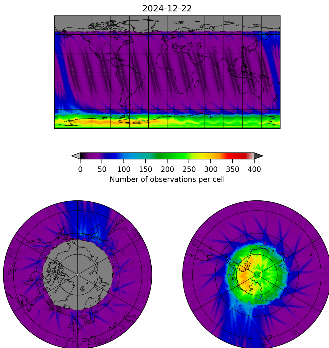
Figure 11: Map of the number of observations for 2024-12-22 to 2024-12-23
