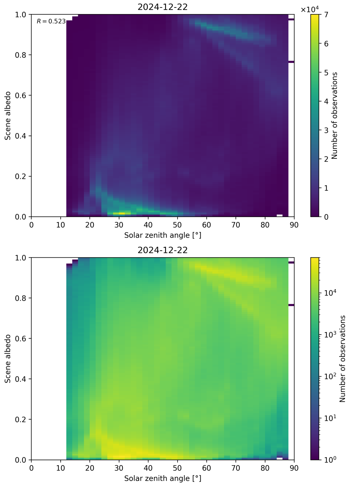
Figure 116: Scatter density plot of “Solar zenith angle” against “Scene albedo” for 2024-12-22 to 2024-12-23.
