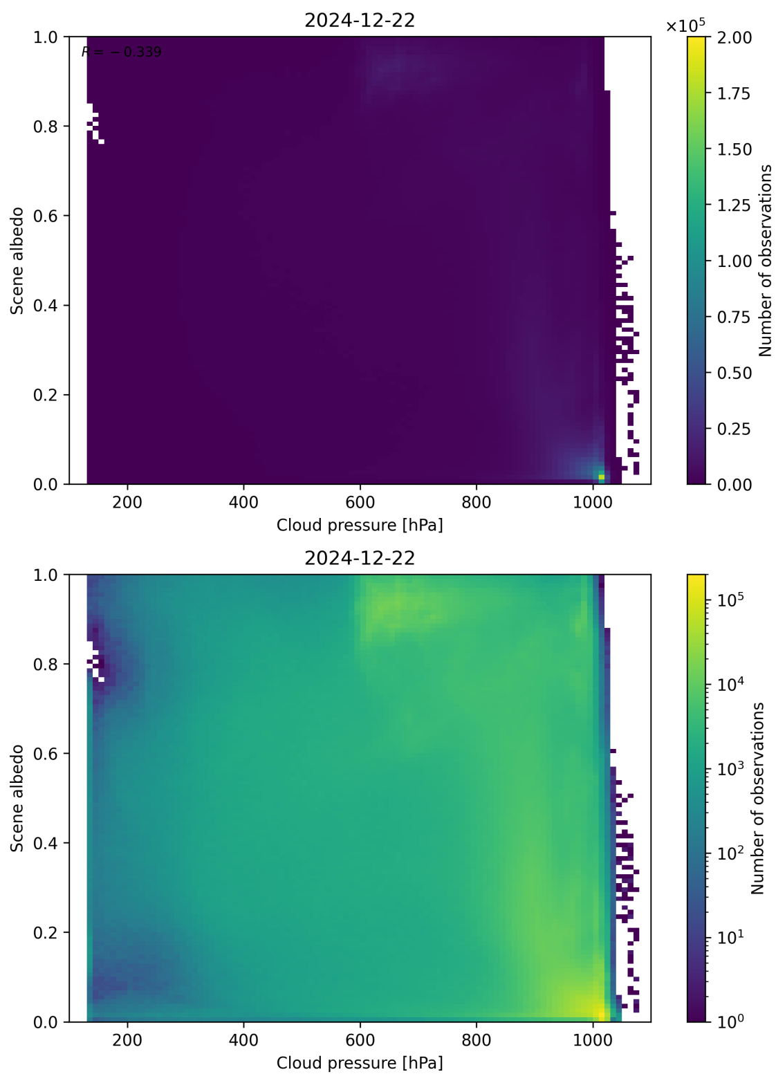
Figure 83: Scatter density plot of “Cloud pressure” against “Scene albedo” for 2024-12-22 to 2024-12-23.
