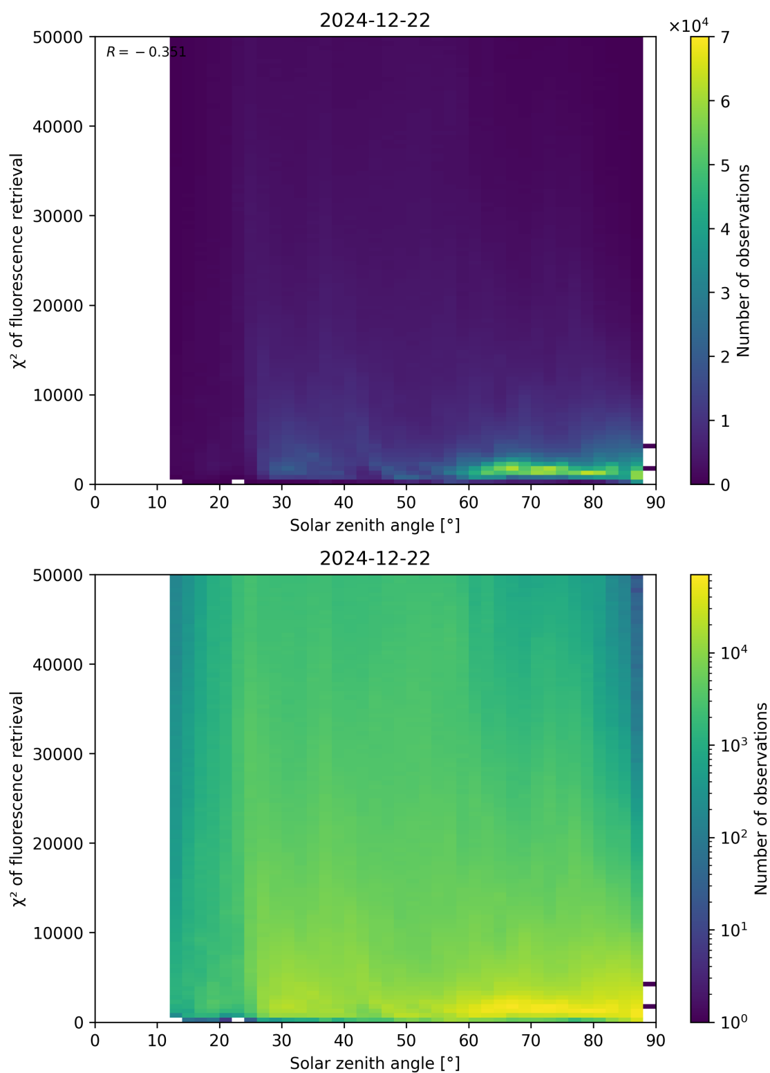
Figure 109: Scatter density plot of “Solar zenith angle” against “ \chi^2 of fluorescence retrieval” for 2024-12-22 to 2024-12-23.
