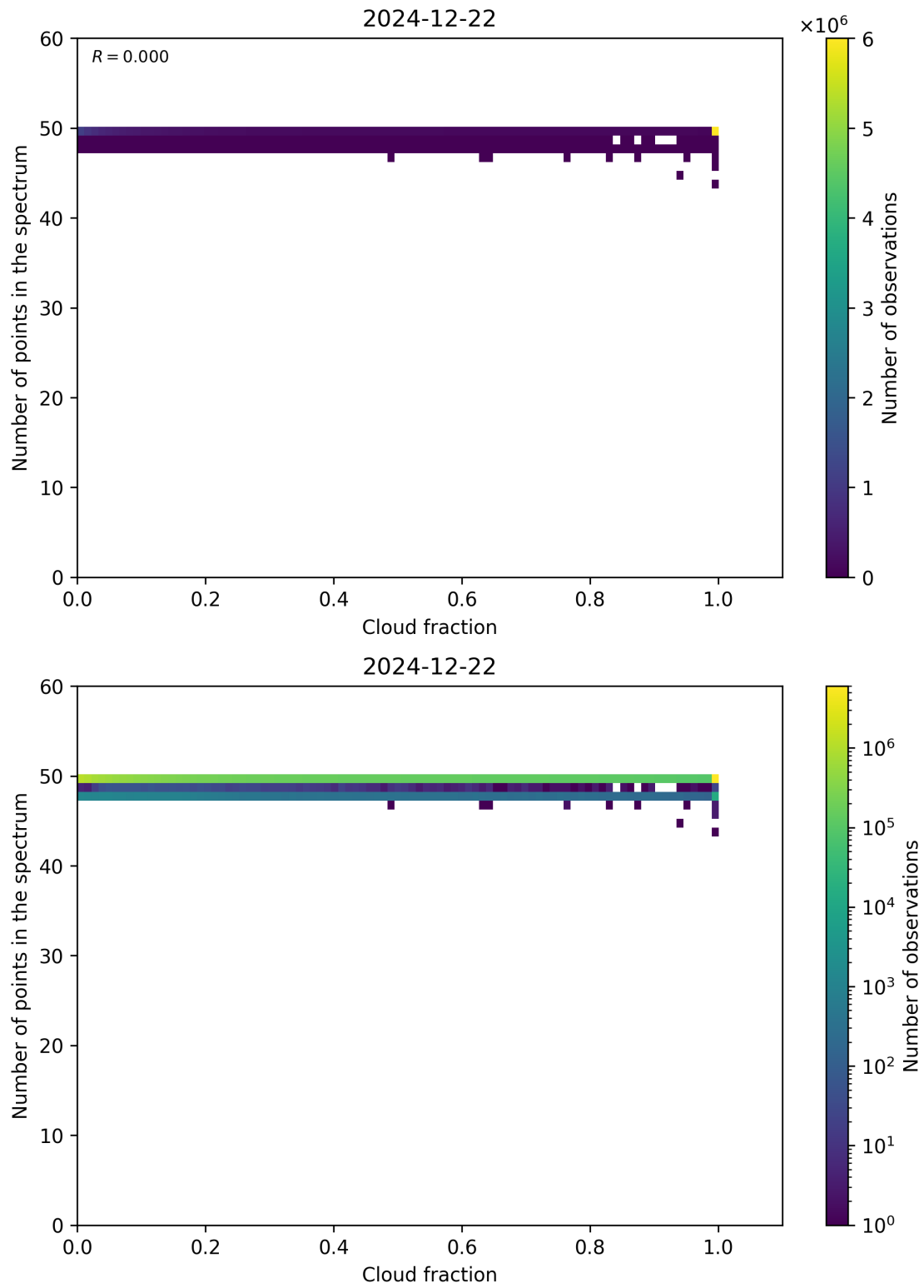
Figure 74: Scatter density plot of “Cloud fraction” against “Number of points in the spectrum” for 2024-12-22 to 2024-12-23.
