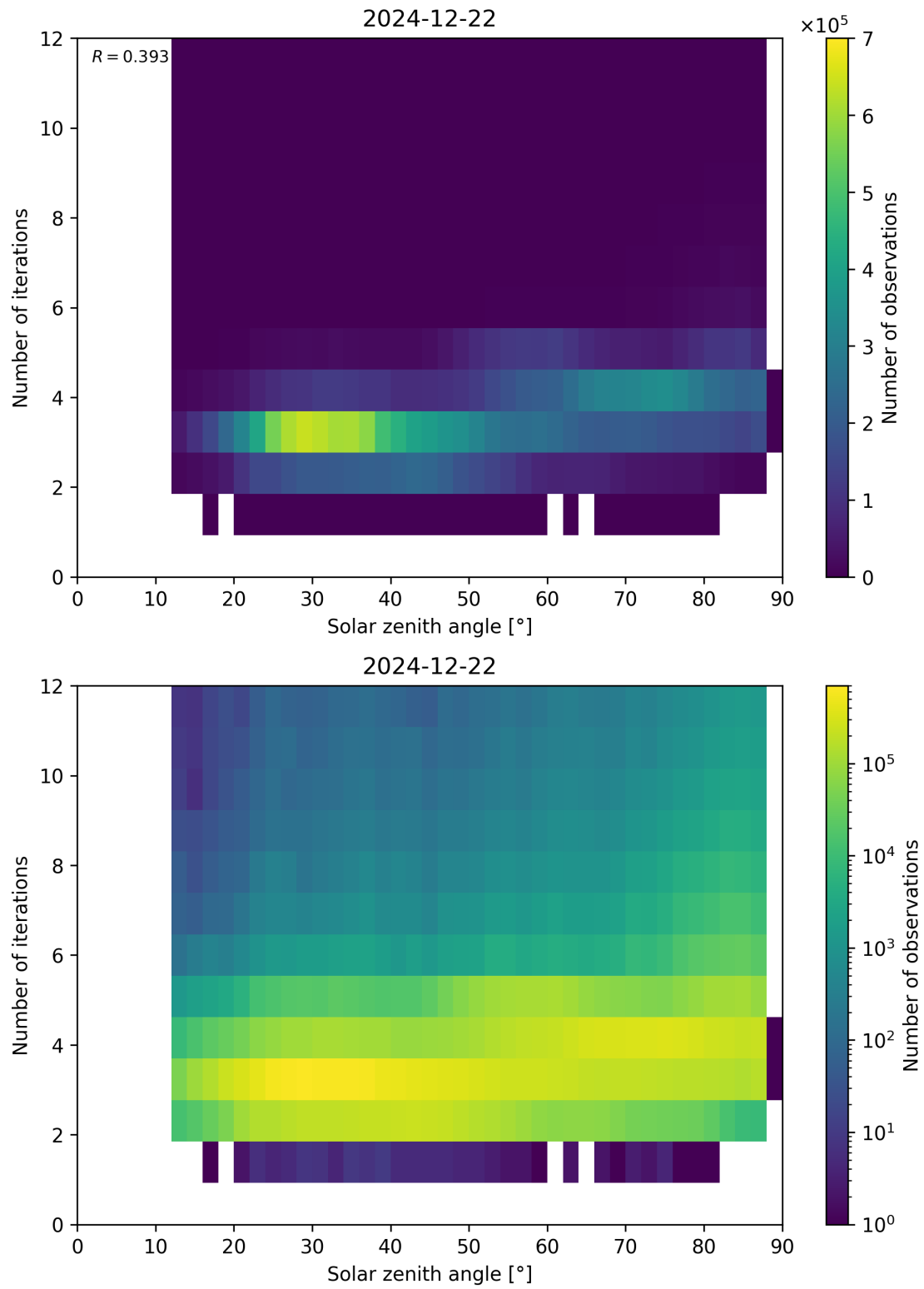
Figure 114: Scatter density plot of “Solar zenith angle” against “Number of iterations” for 2024-12-22 to 2024-12-23.
