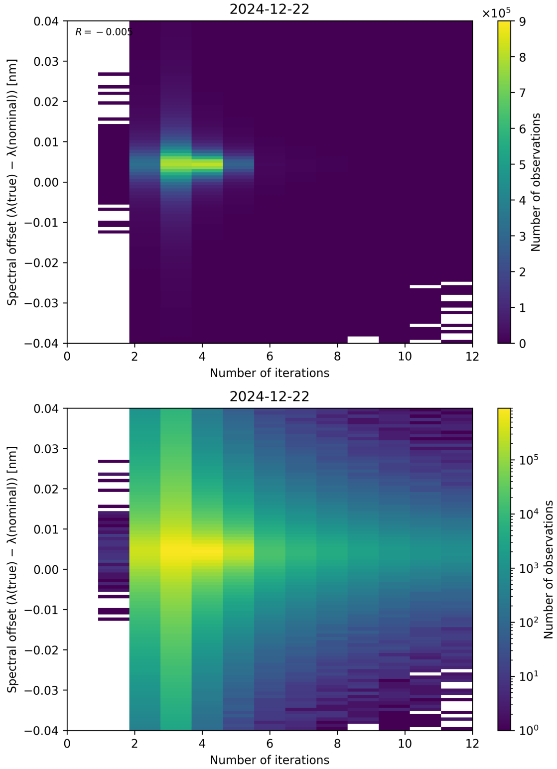
Figure 100: Scatter density plot of “Number of iterations” against “Spectral offset ( \lambda_{\text{true}} - \lambda_{\text{nominal}} )” for 2024-12-22 to 2024-12-23.
