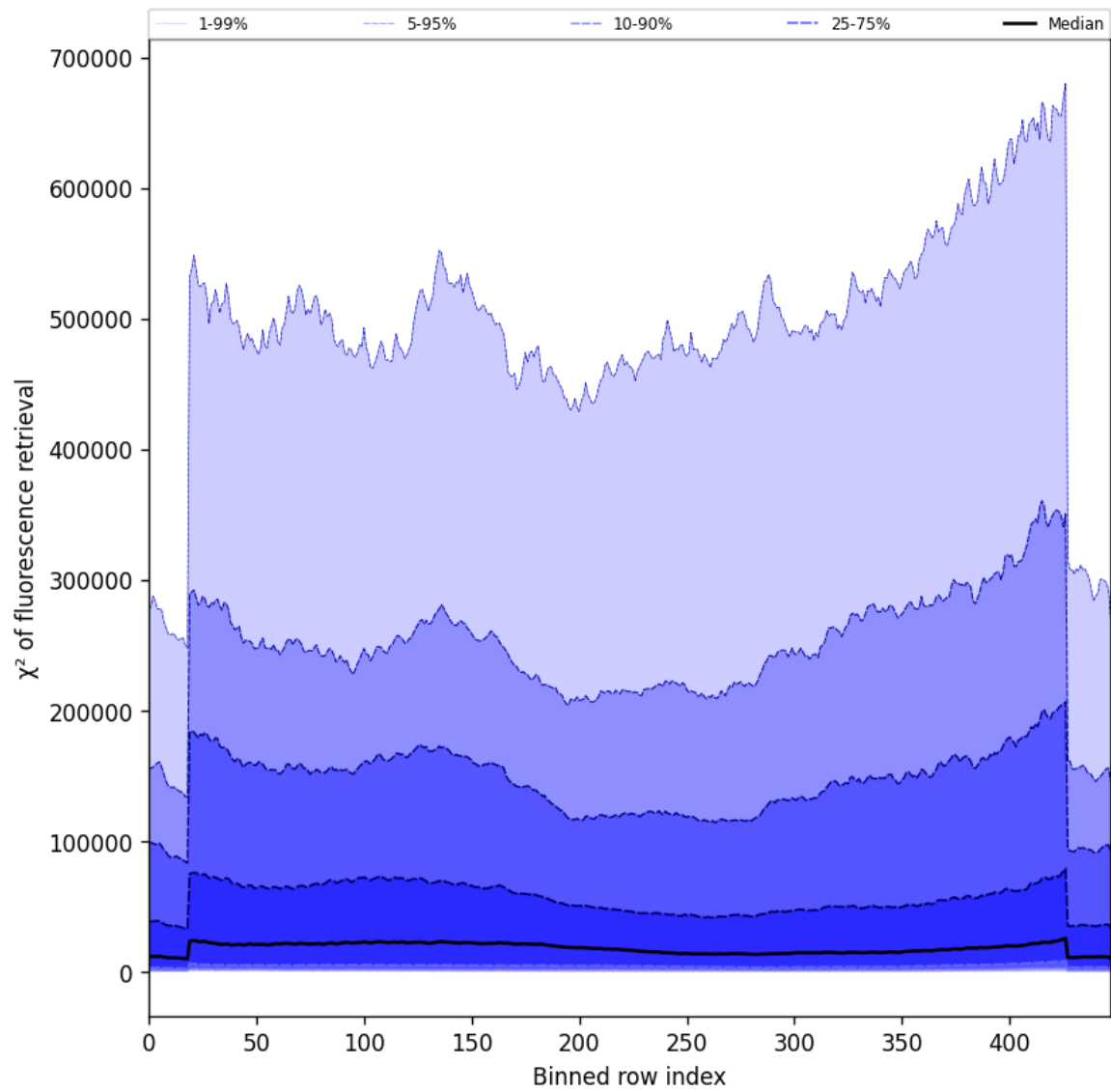
Figure 59: Along track statistics of “ \chi^2 of fluorescence retrieval” for 2024-12-22 to 2024-12-23
