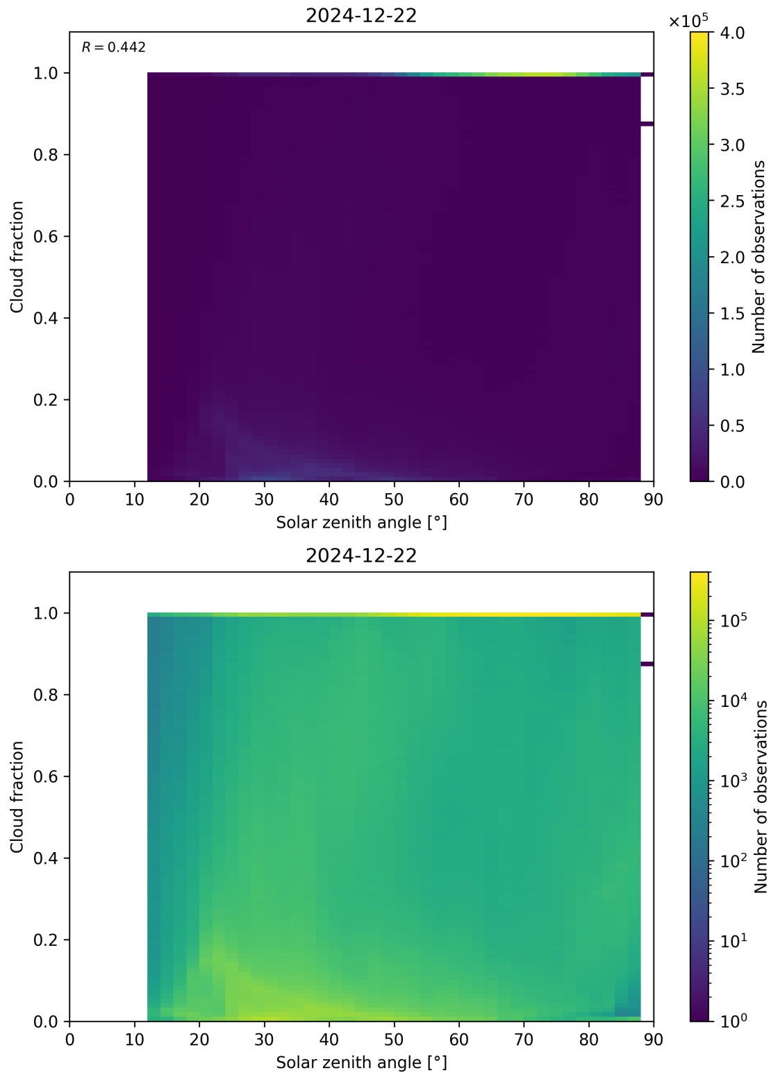
Figure 110: Scatter density plot of “Solar zenith angle” against “Cloud fraction” for 2024-12-22 to 2024-12-23.
