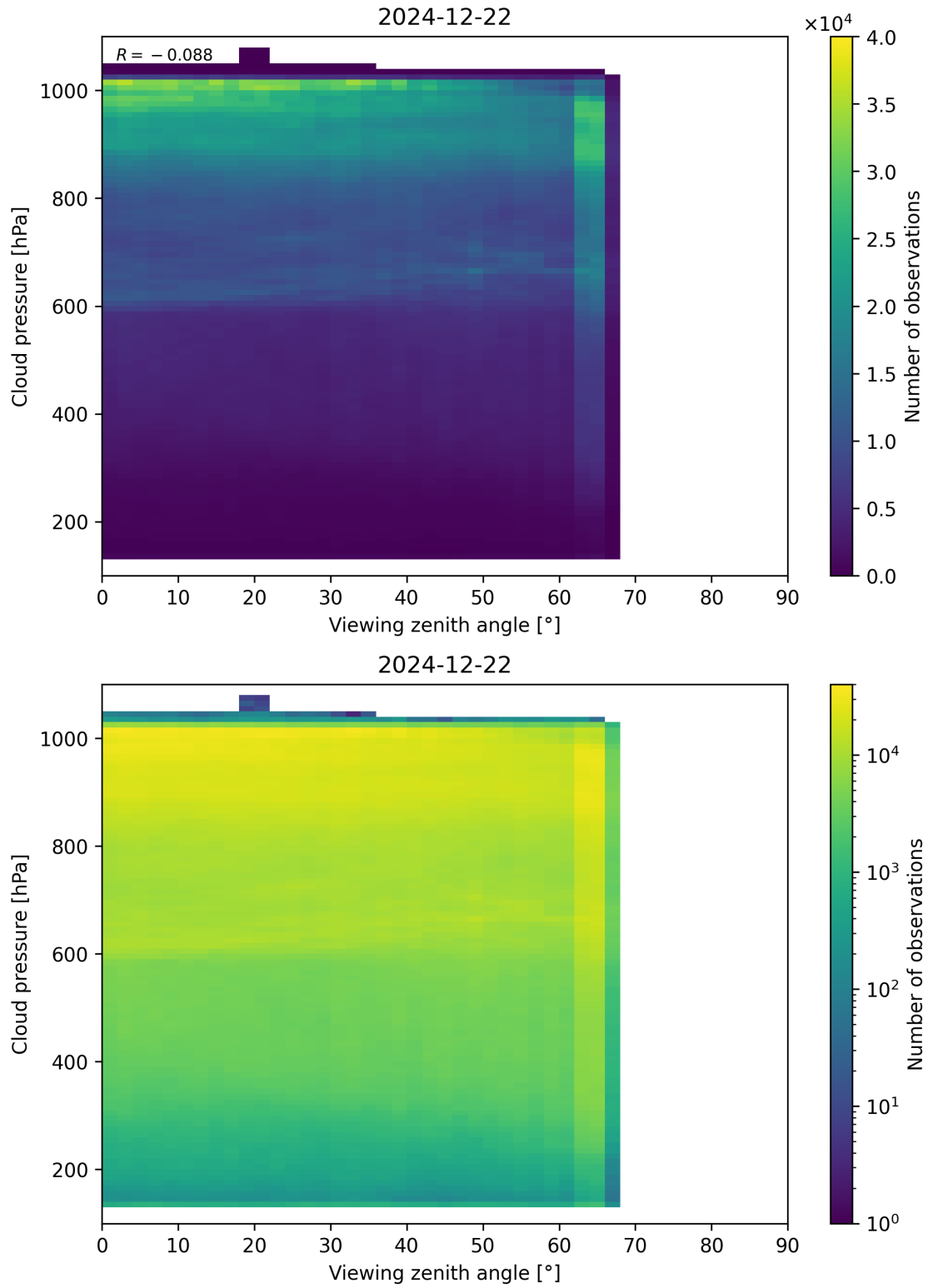
Figure 121: Scatter density plot of “Viewing zenith angle” against “Cloud pressure” for 2024-12-22 to 2024-12-23.
