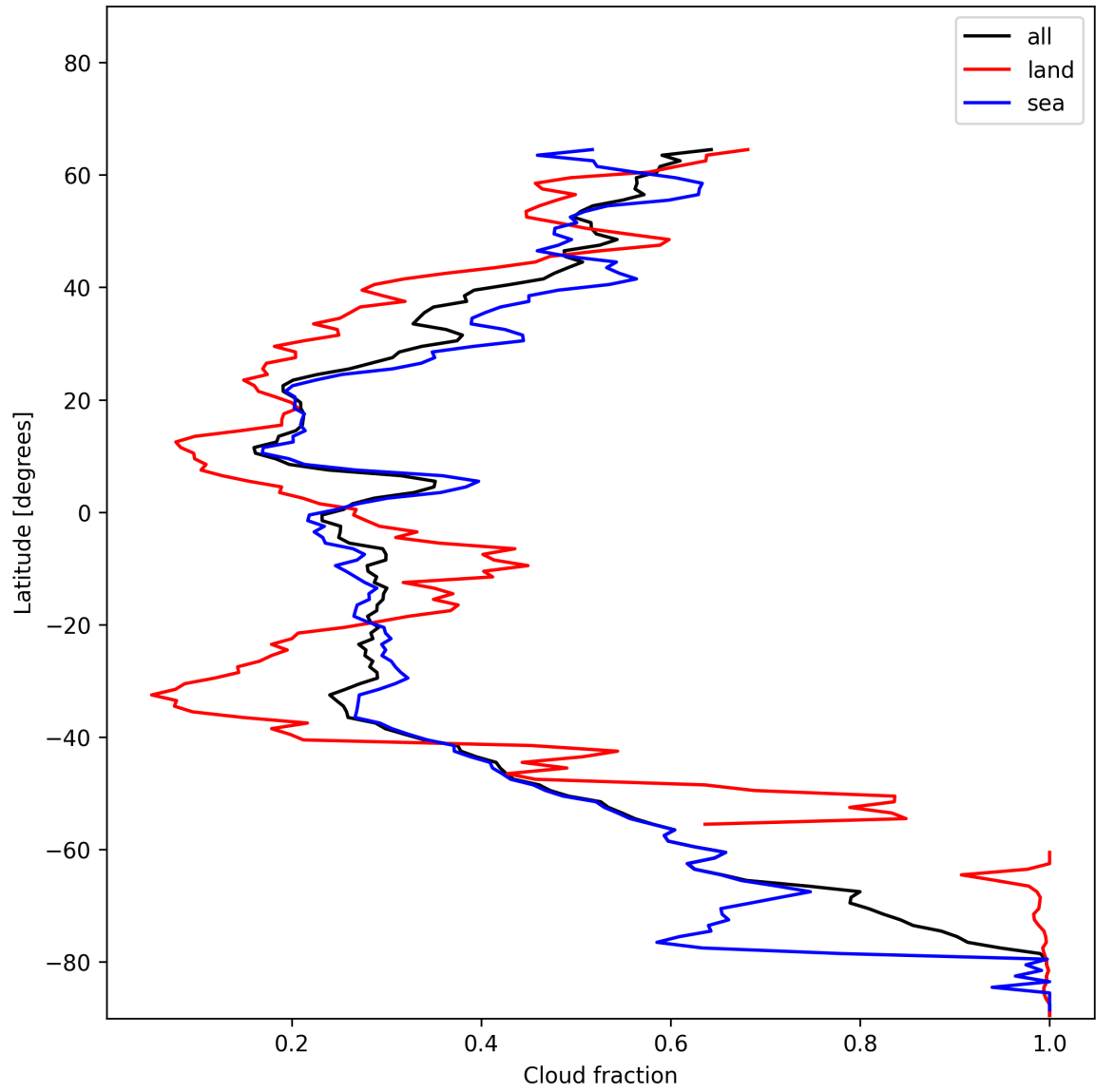
Figure 15: Zonal average of “Cloud fraction” for 2024-12-22 to 2024-12-23.
