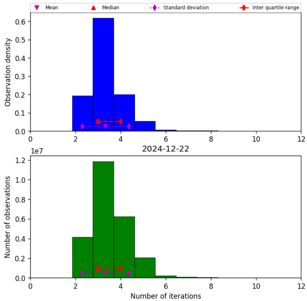
Figure 39: Histogram of “Number of iterations” for 2024-12-22 to 2024-12-23
