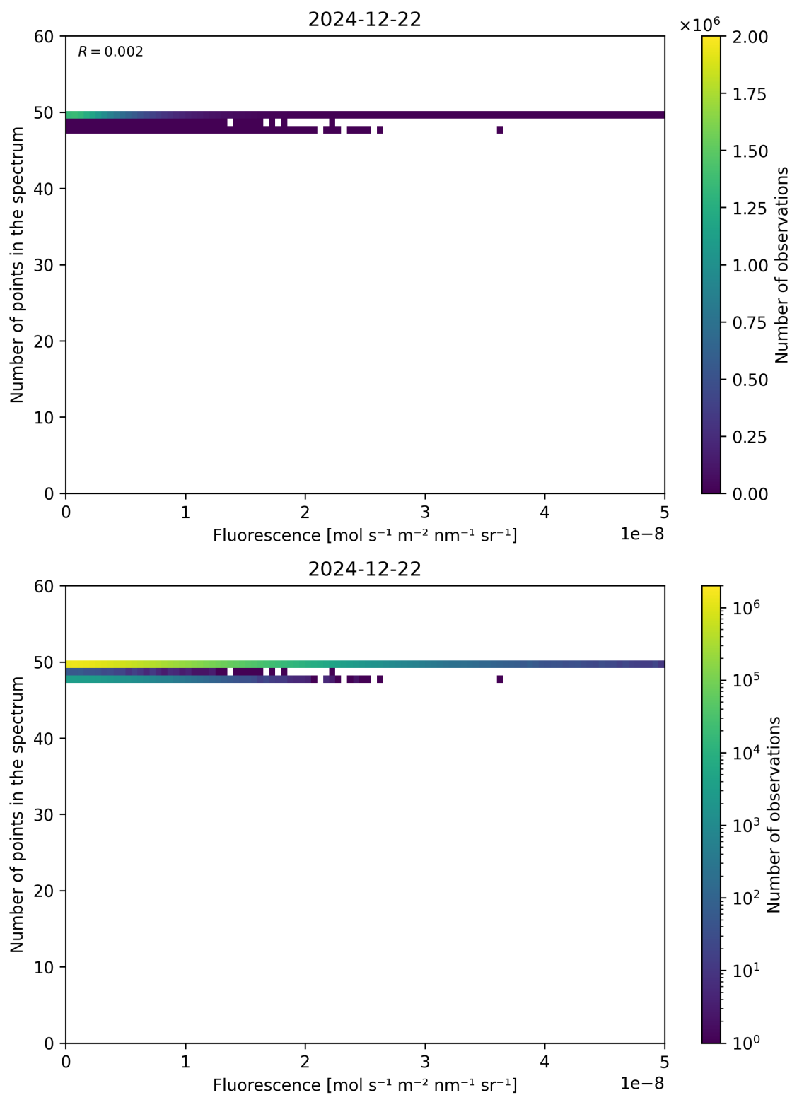
Figure 86: Scatter density plot of “Fluorescence” against “Number of points in the spectrum” for 2024-12-22 to 2024-12-23.
