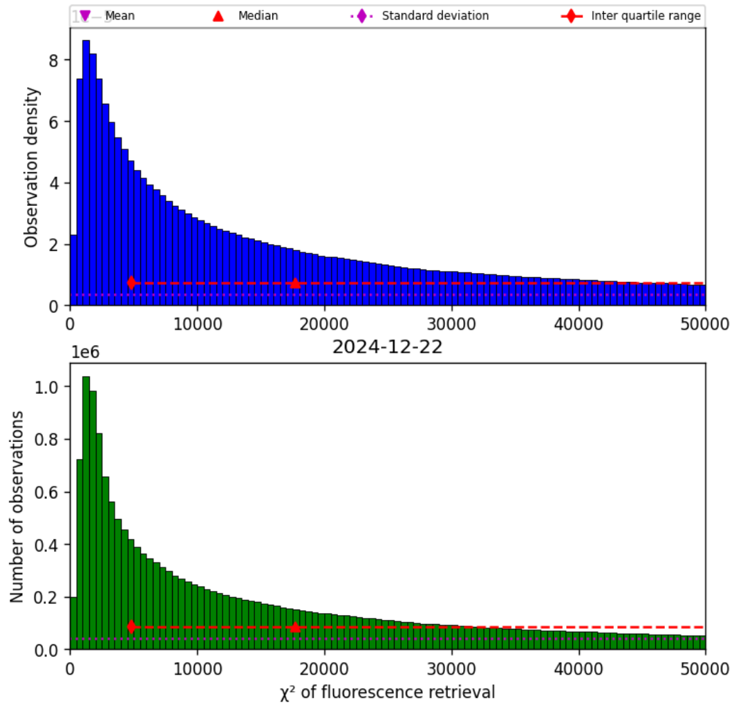
Figure 42: Histogram of “ \chi^2 of fluorescence retrieval” for 2024-12-22 to 2024-12-23
