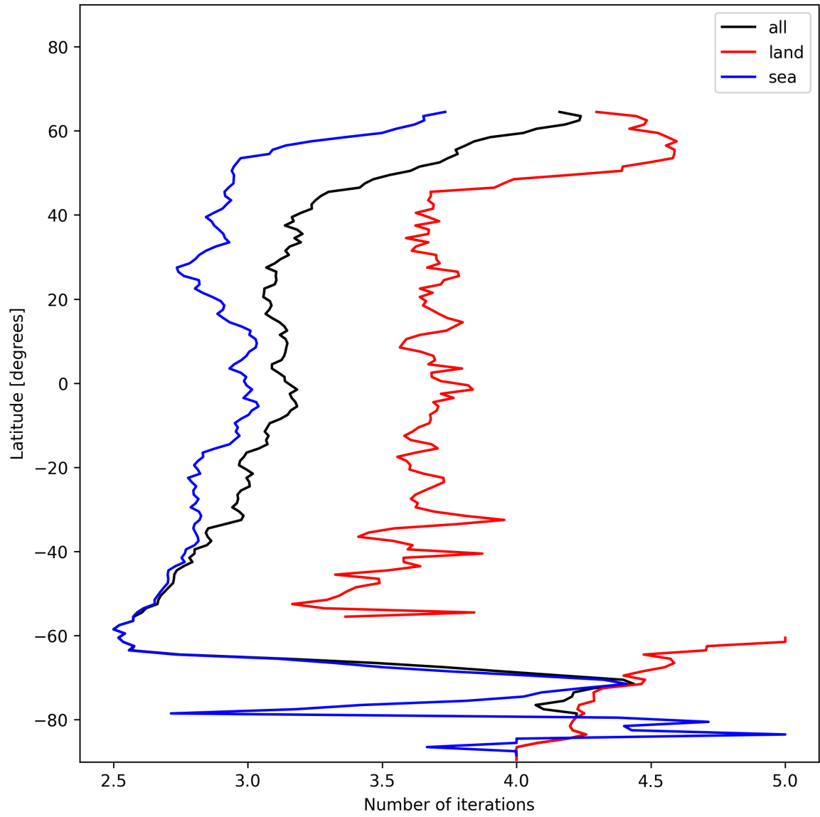
Figure 22: Zonal average of “Number of iterations” for 2024-12-22 to 2024-12-23.
