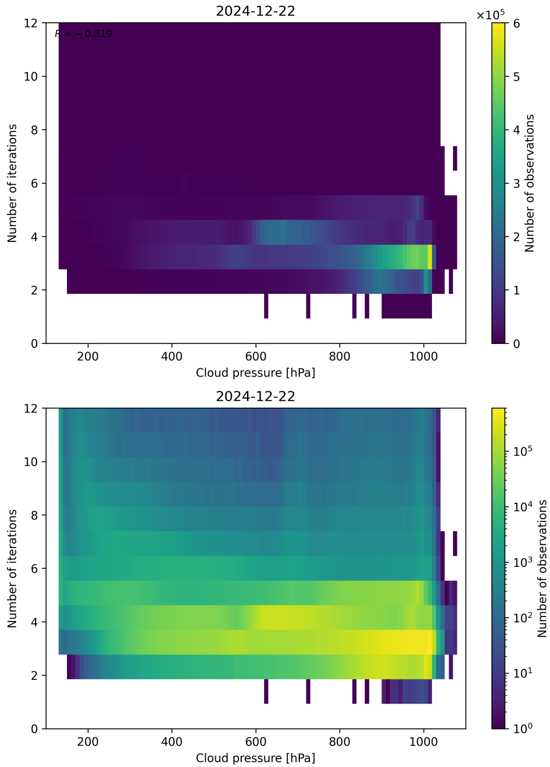
Figure 81: Scatter density plot of “Cloud pressure” against “Number of iterations” for 2024-12-22 to 2024-12-23.
