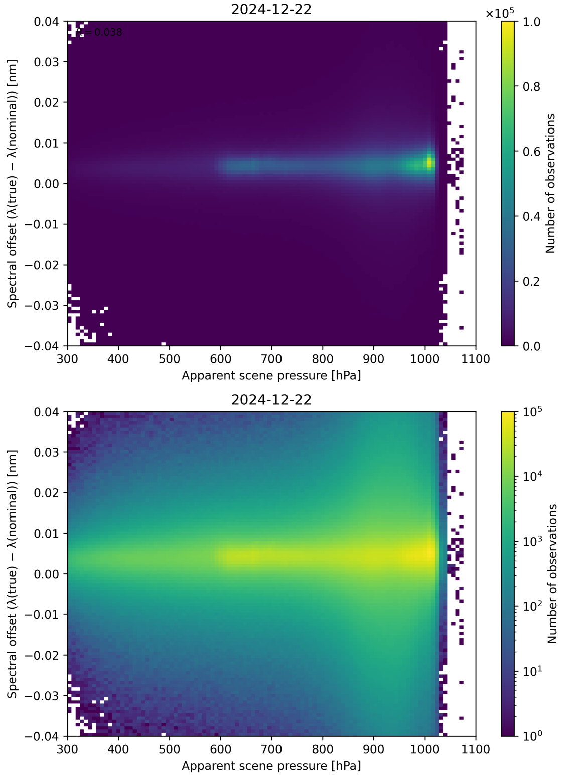
Figure 67: Scatter density plot of “Apparent scene pressure” against “Spectral offset ( \lambda_{\text{true}} - \lambda_{\text{nominal}} )” for 2024-12-22 to 2024-12-23.
