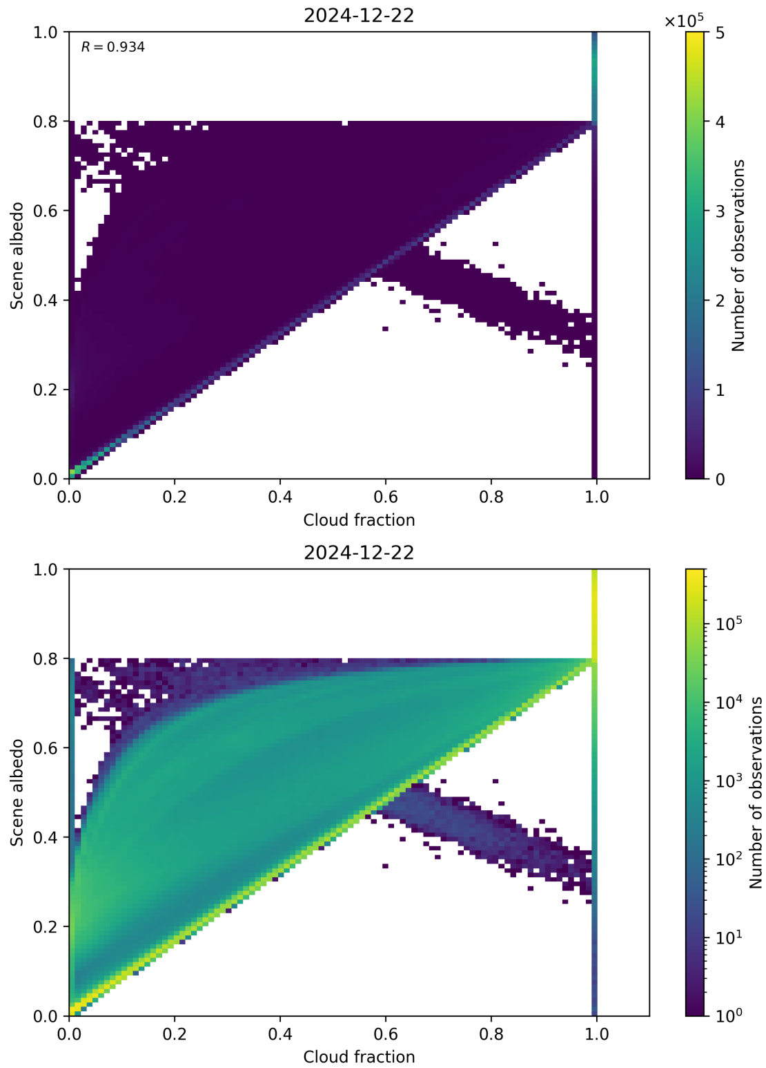
Figure 75: Scatter density plot of “Cloud fraction” against “Scene albedo” for 2024-12-22 to 2024-12-23.
