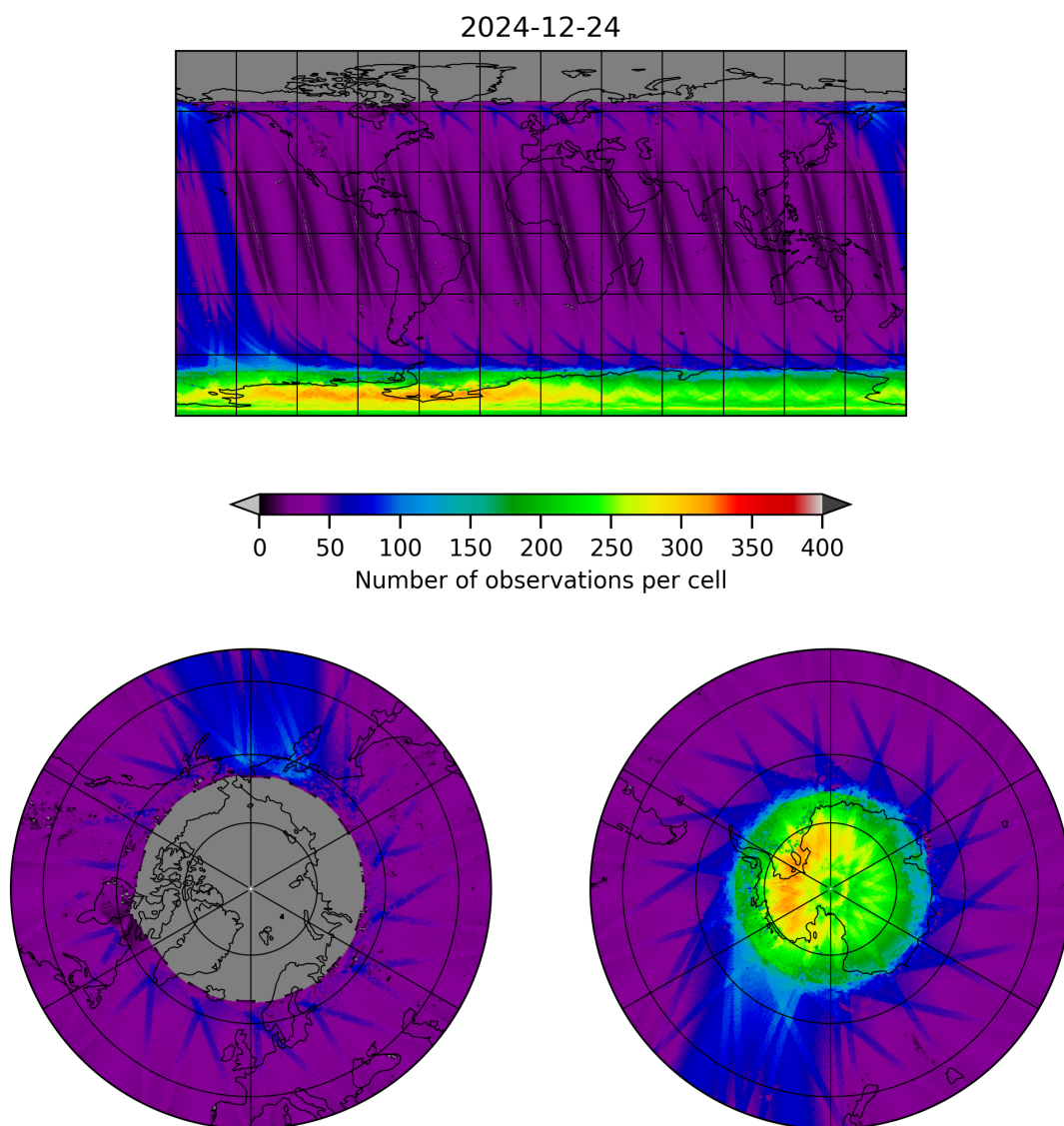
Figure 11: Map of the number of observations for 2024-12-23 to 2024-12-25
