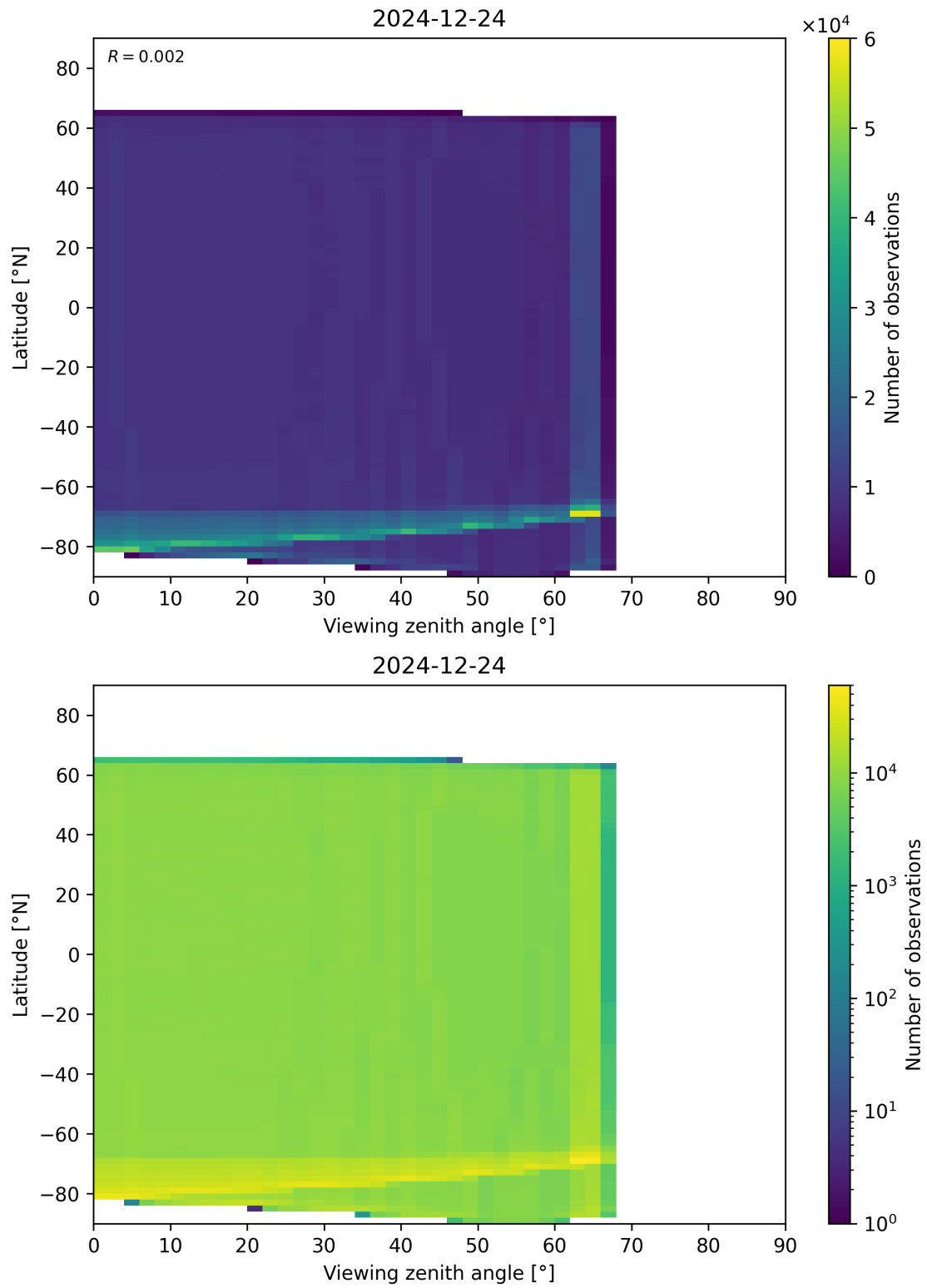
Figure 123: Scatter density plot of “Viewing zenith angle” against “Latitude” for 2024-12-23 to 2024-12-25.
