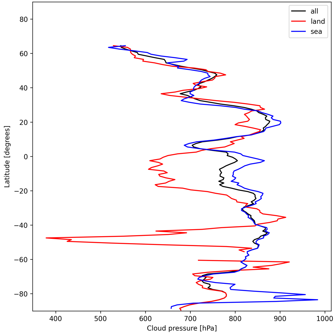
Figure 13: Zonal average of “Cloud pressure” for 2024-12-23 to 2024-12-25.
