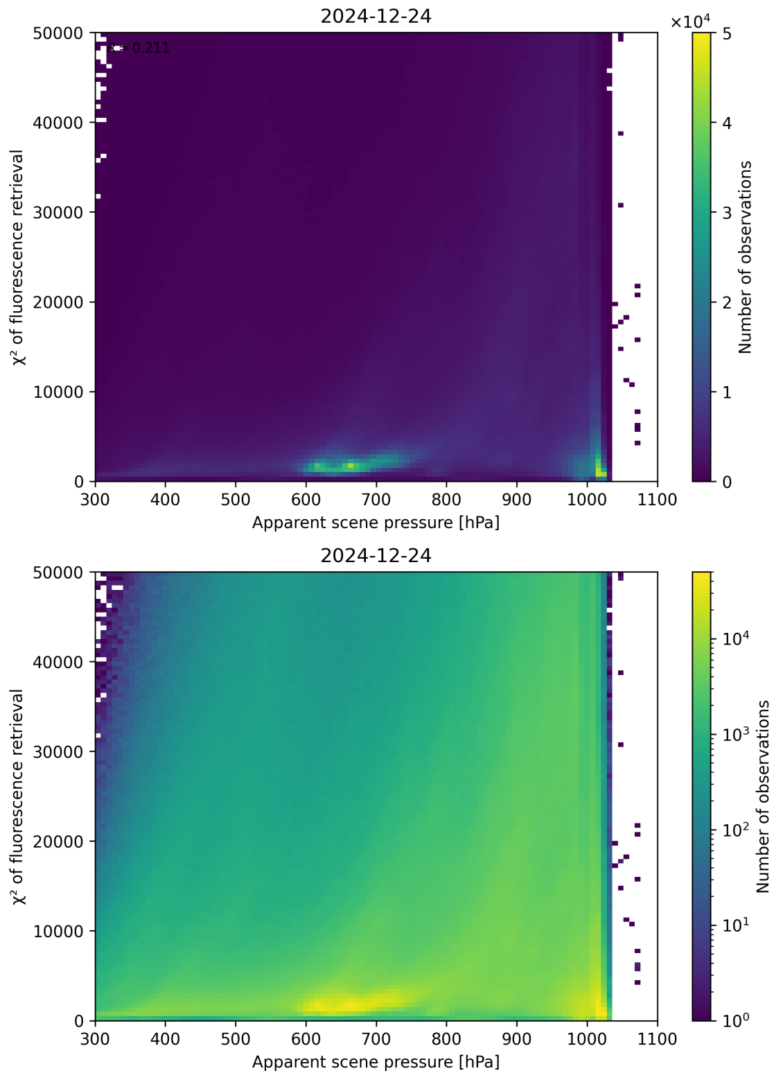
Figure 63: Scatter density plot of “Apparent scene pressure” against “ \chi^2 of fluorescence retrieval” for 2024-12-23 to 2024-12-25.
