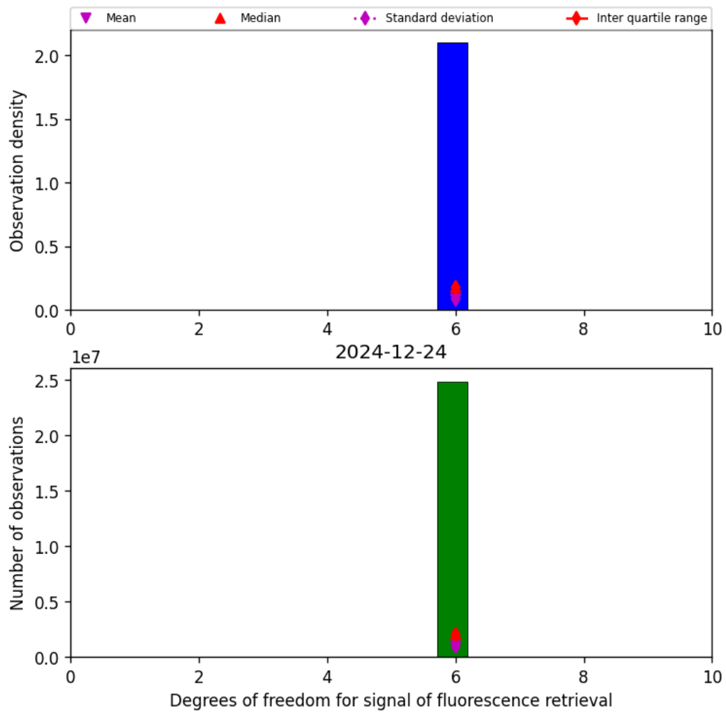
Figure 43: Histogram of "Degrees of freedom for signal of fluorescence retrieval" for 2024-12-23 to 2024-12-25
