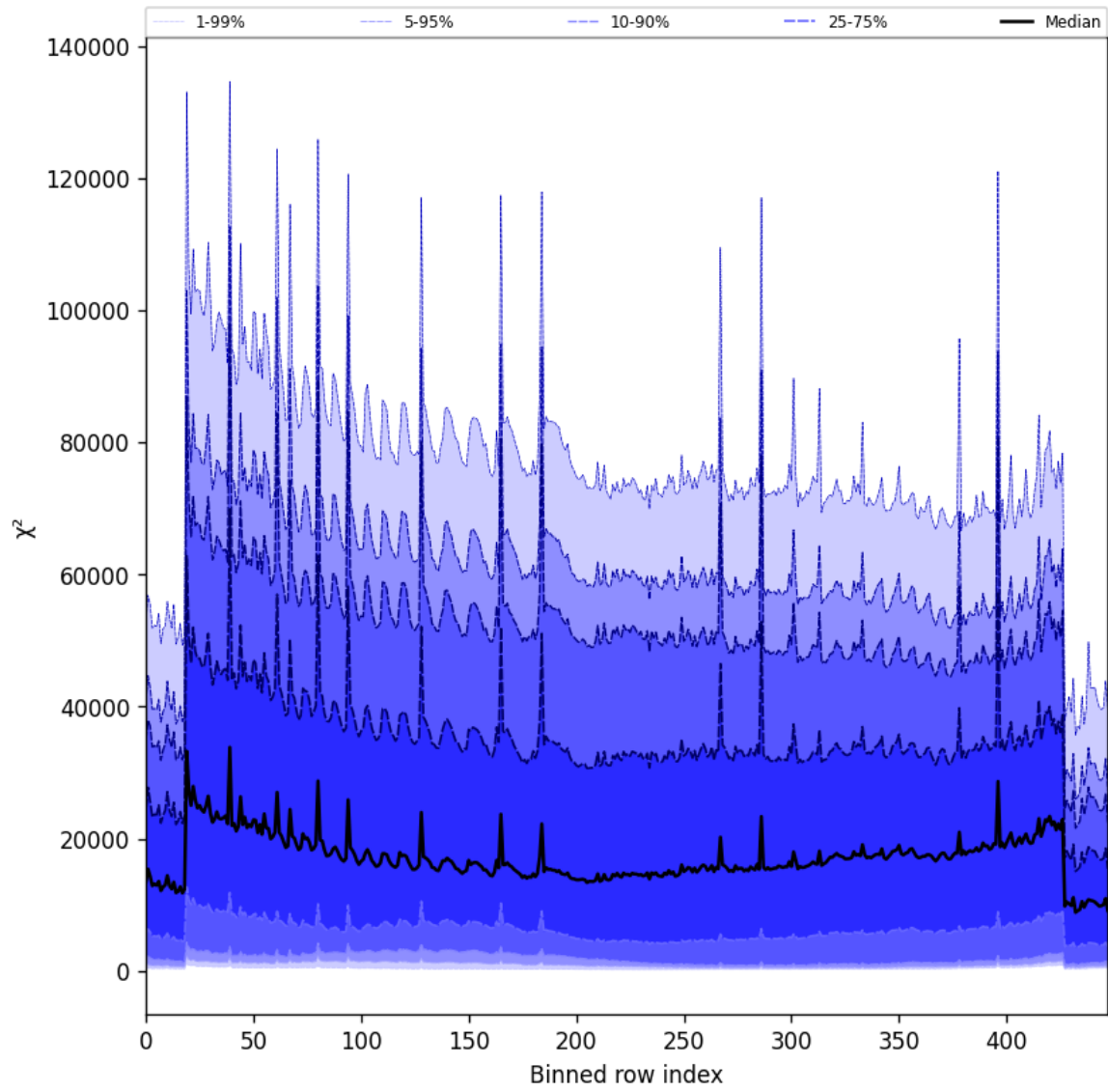
Figure 55: Along track statistics of “ \chi^2 ” for 2024-12-23 to 2024-12-25
