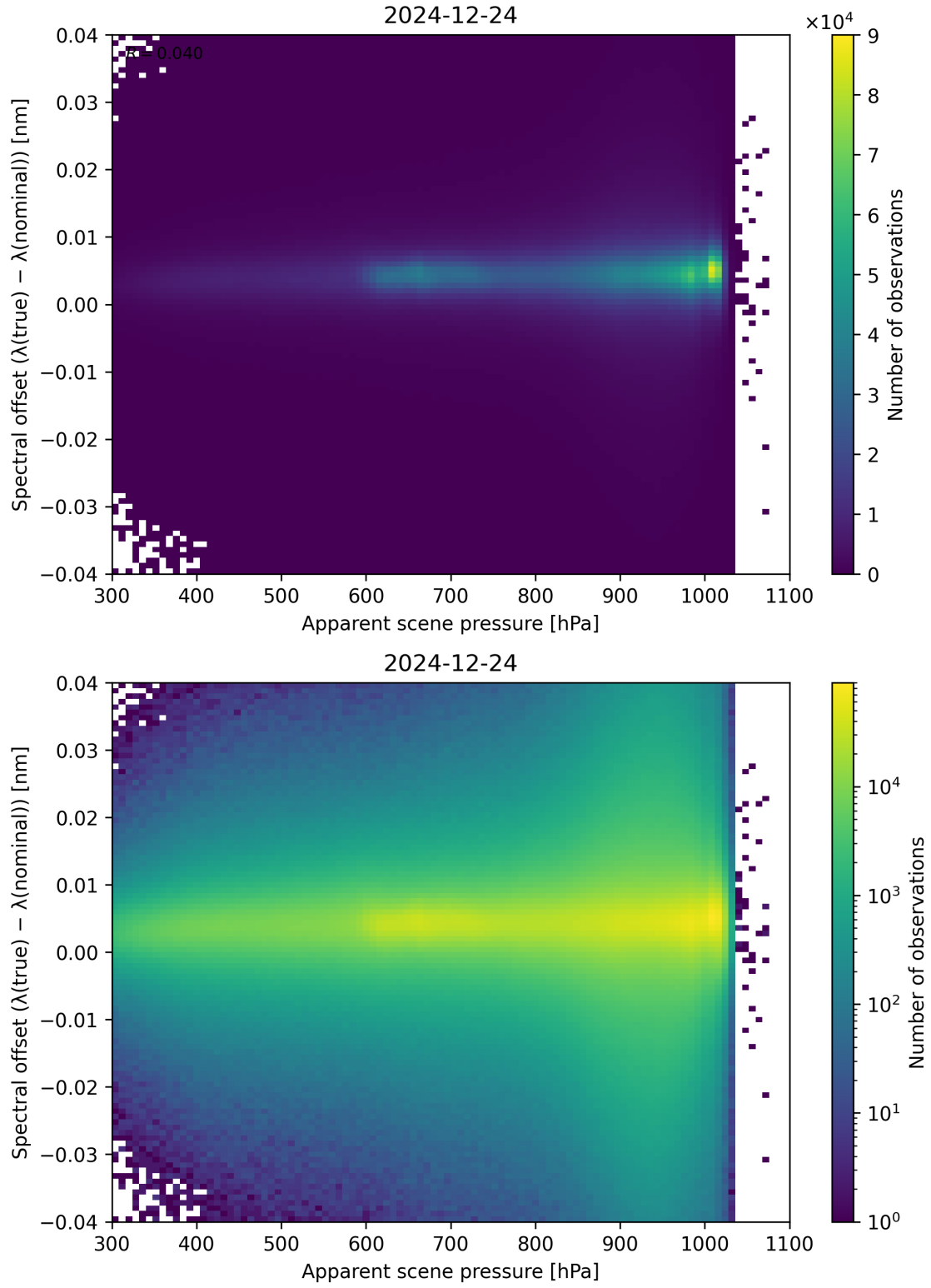
Figure 67: Scatter density plot of “Apparent scene pressure” against “Spectral offset ( \lambda_{\text{true}} - \lambda_{\text{nominal}} )” for 2024-12-23 to 2024-12-25.
