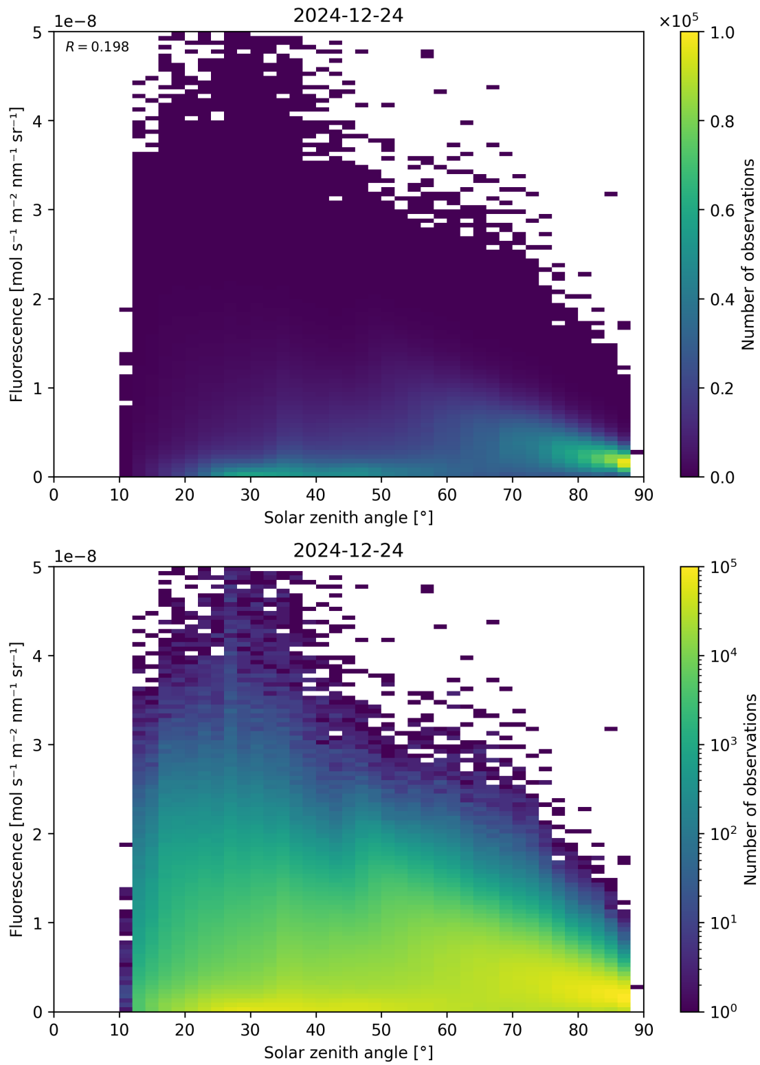
Figure 112: Scatter density plot of “Solar zenith angle” against “Fluorescence” for 2024-12-23 to 2024-12-25.
