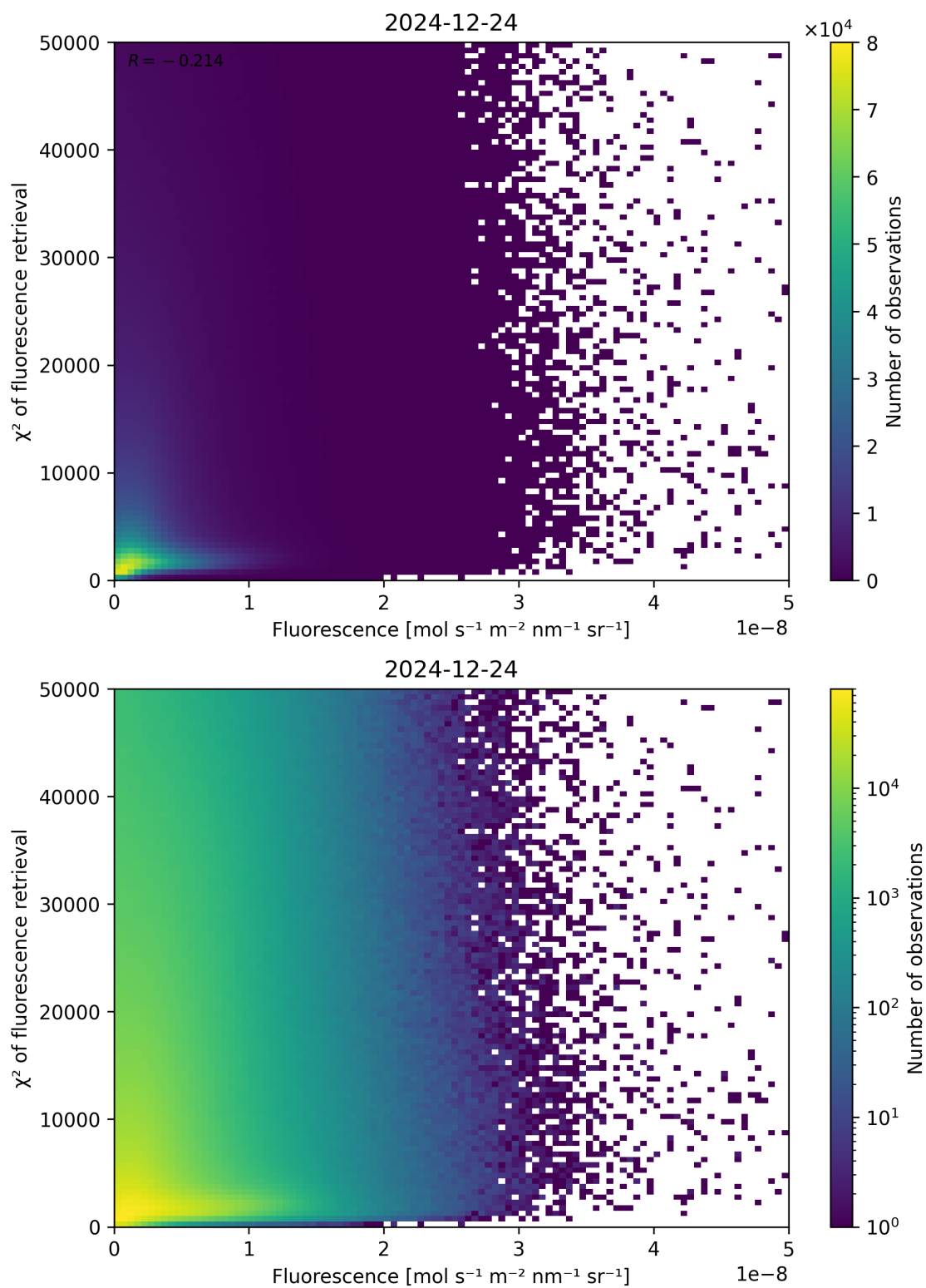
Figure 85: Scatter density plot of “Fluorescence” against “ \chi^2 of fluorescence retrieval” for 2024-12-23 to 2024-12-25.
