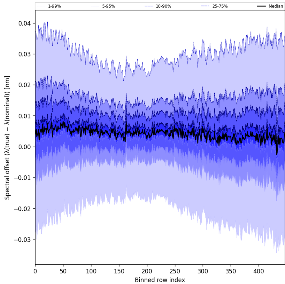
Figure 62: Along track statistics of “Spectral offset ( \lambda_{\text{true}} - \lambda_{\text{nominal}} )” for 2024-12-23 to 2024-12-25
