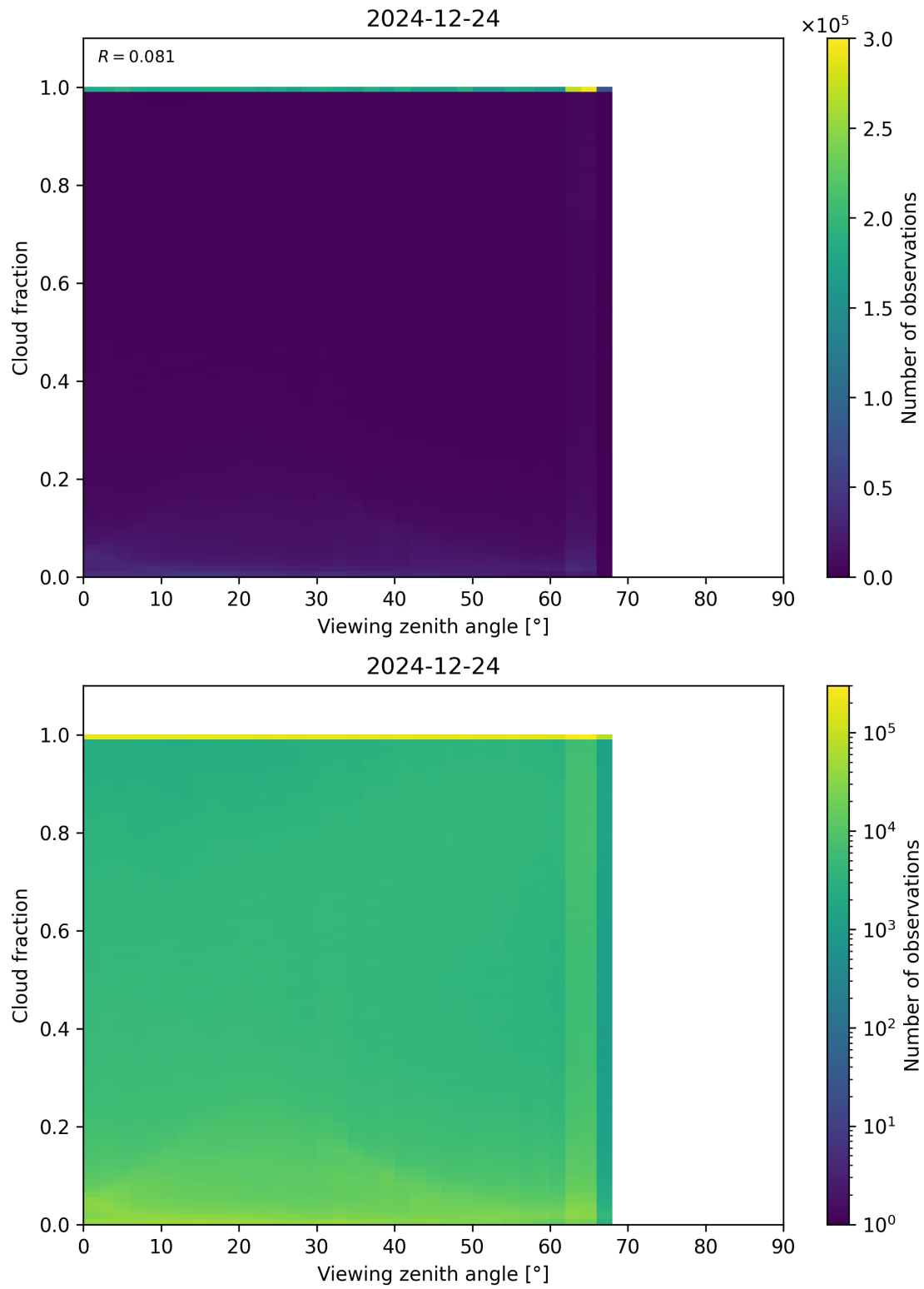
Figure 120: Scatter density plot of “Viewing zenith angle” against “Cloud fraction” for 2024-12-23 to 2024-12-25.
