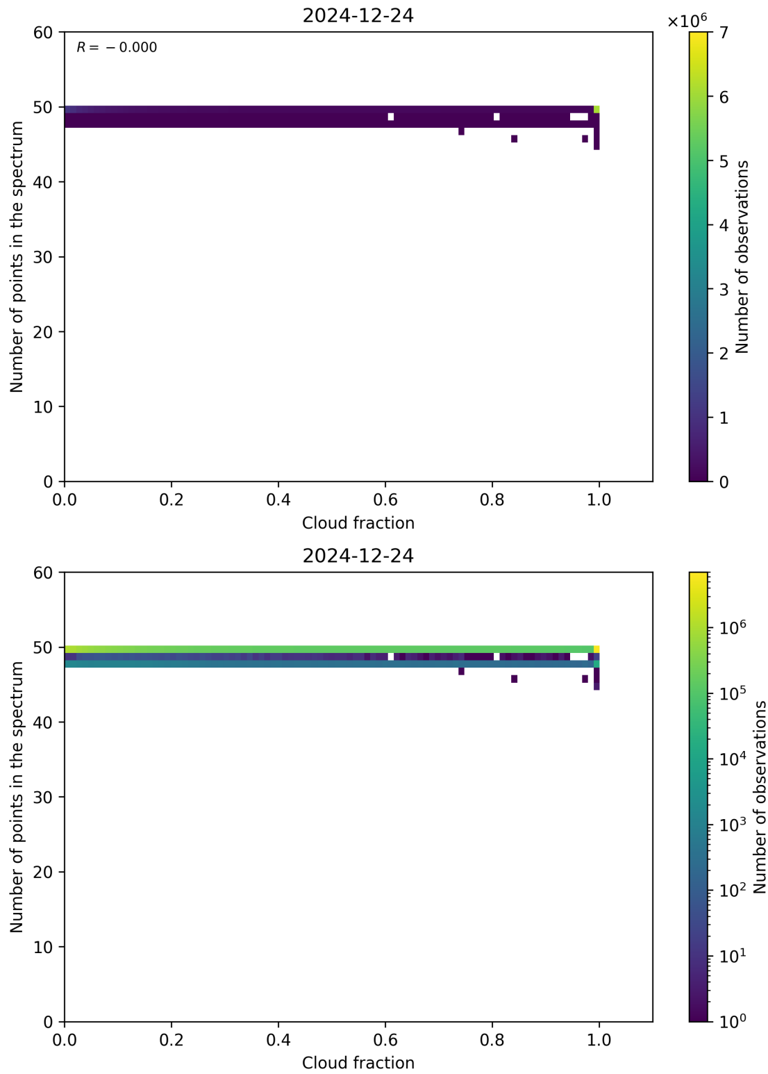
Figure 74: Scatter density plot of “Cloud fraction” against “Number of points in the spectrum” for 2024-12-23 to 2024-12-25.
