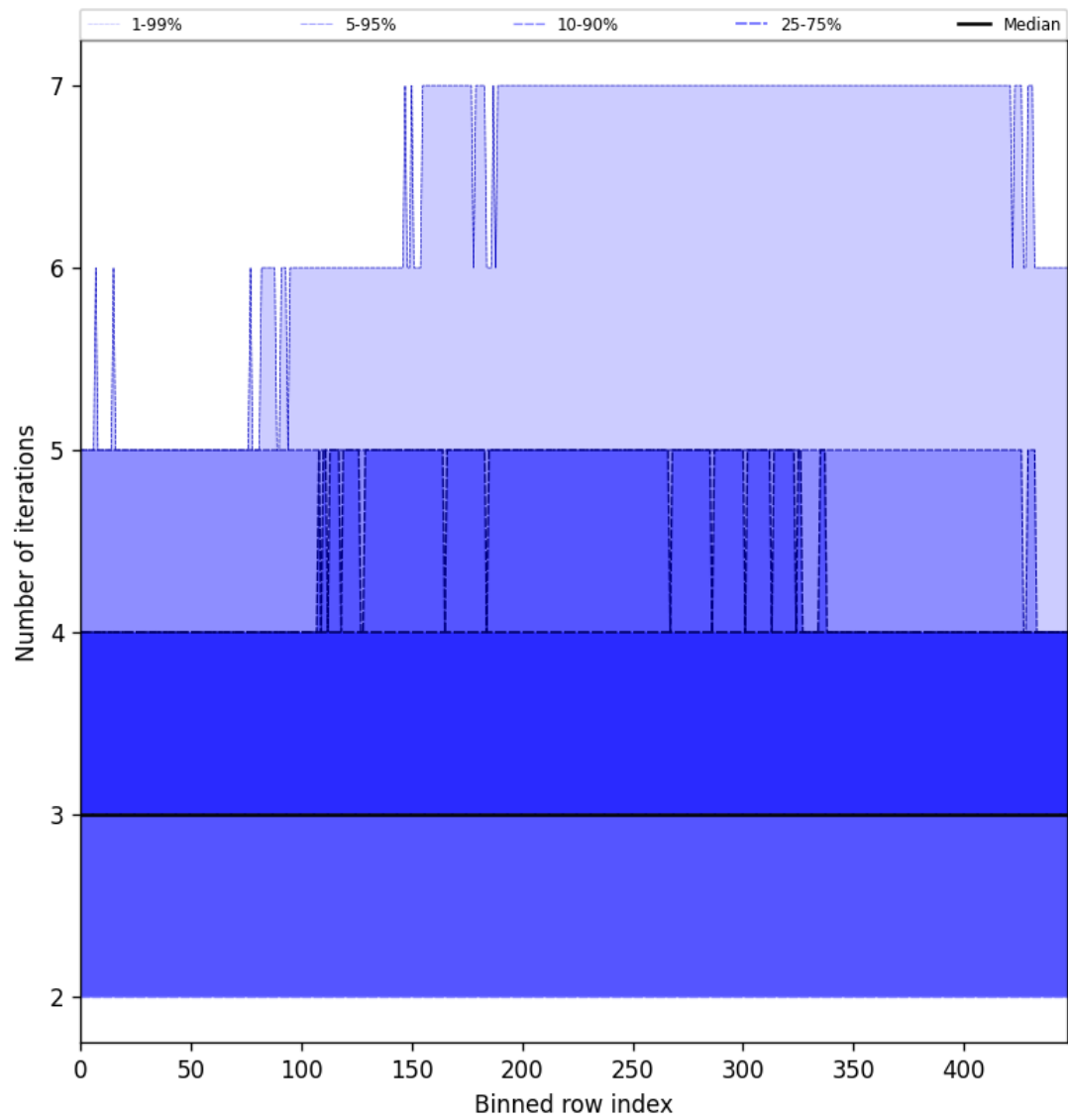
Figure 56: Along track statistics of “Number of iterations” for 2024-12-23 to 2024-12-25
