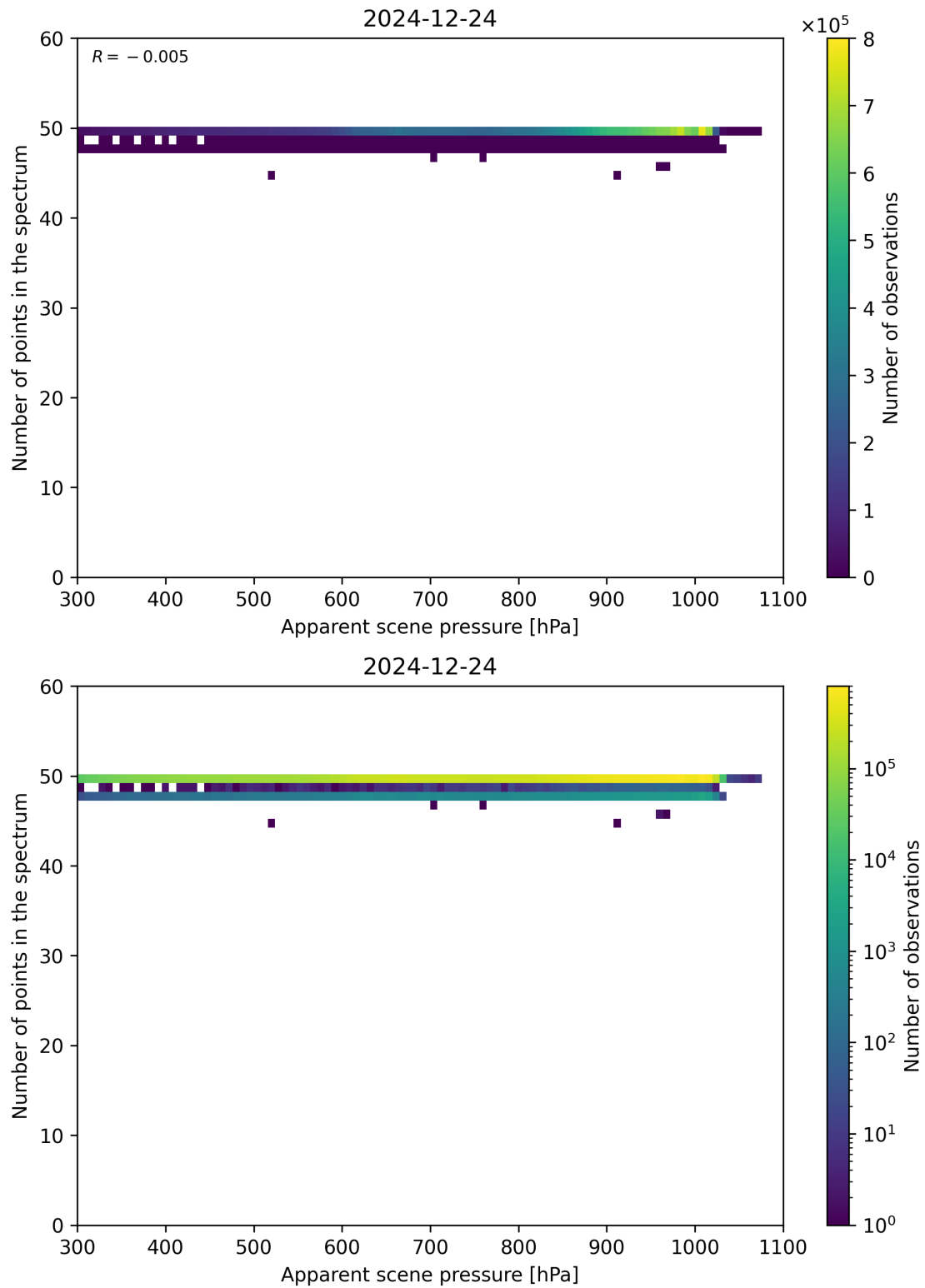
Figure 66: Scatter density plot of “Apparent scene pressure” against “Number of points in the spectrum” for 2024-12-23 to 2024-12-25.
