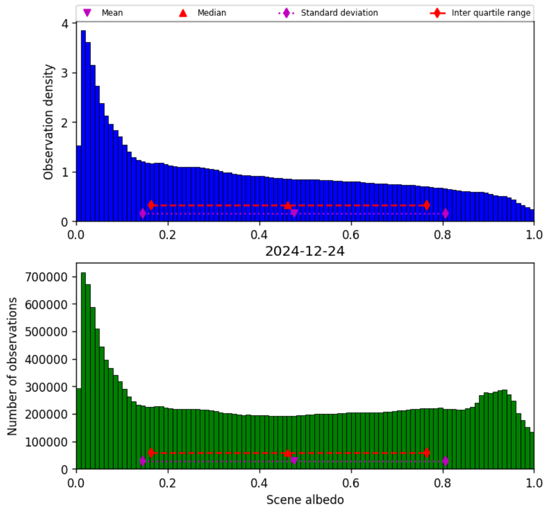
Figure 34: Histogram of “Scene albedo” for 2024-12-23 to 2024-12-25
