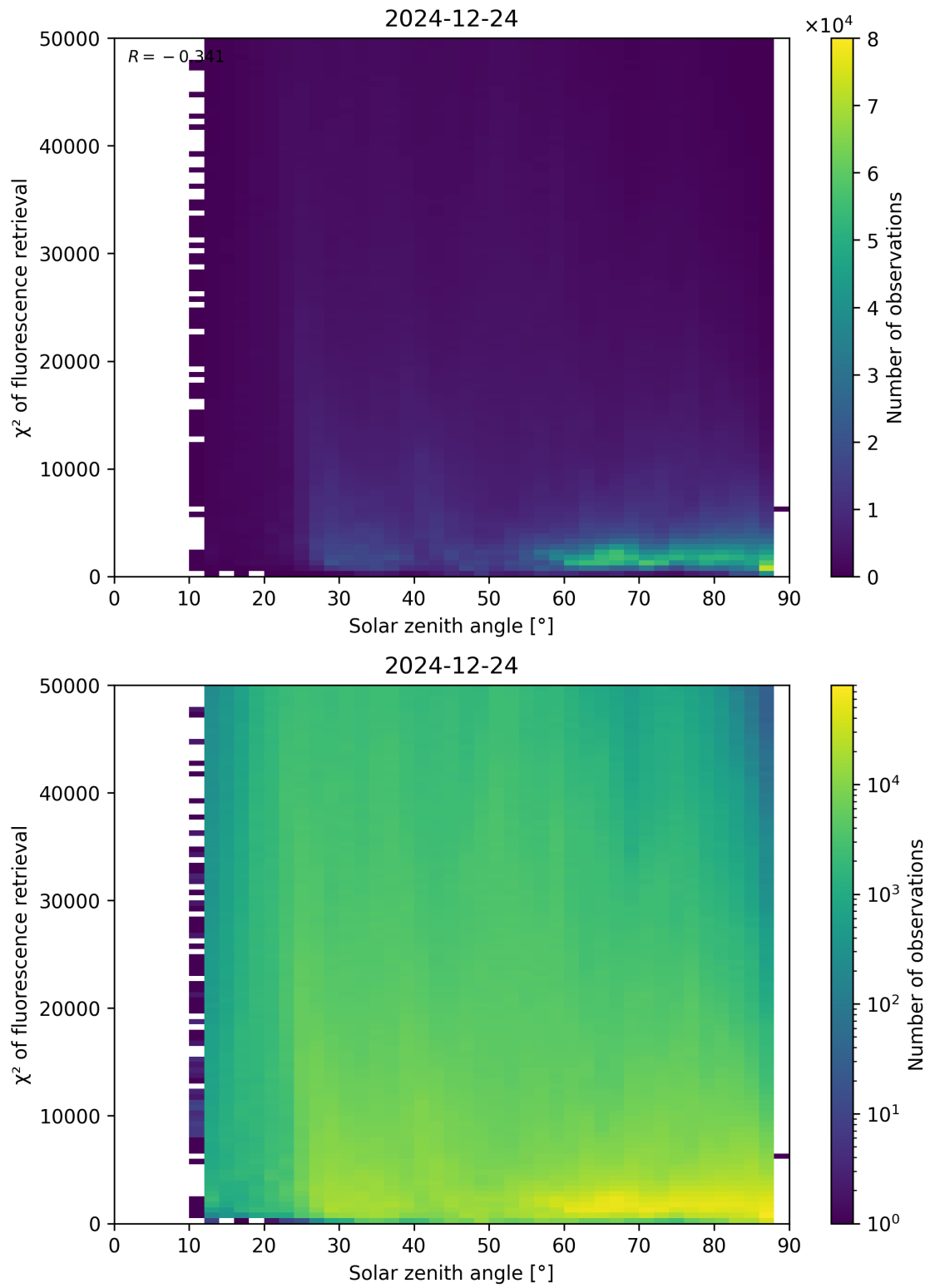
Figure 109: Scatter density plot of “Solar zenith angle” against “ \chi^2 of fluorescence retrieval” for 2024-12-23 to 2024-12-25.
