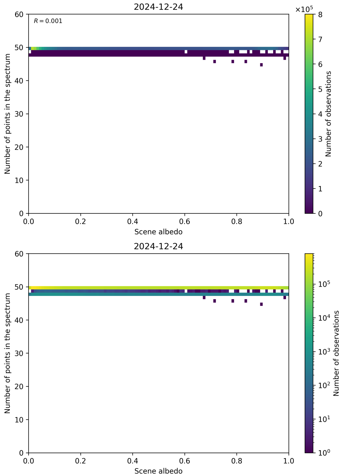
Figure 106: Scatter density plot of “Scene albedo” against “Number of points in the spectrum” for 2024-12-23 to 2024-12-25.
