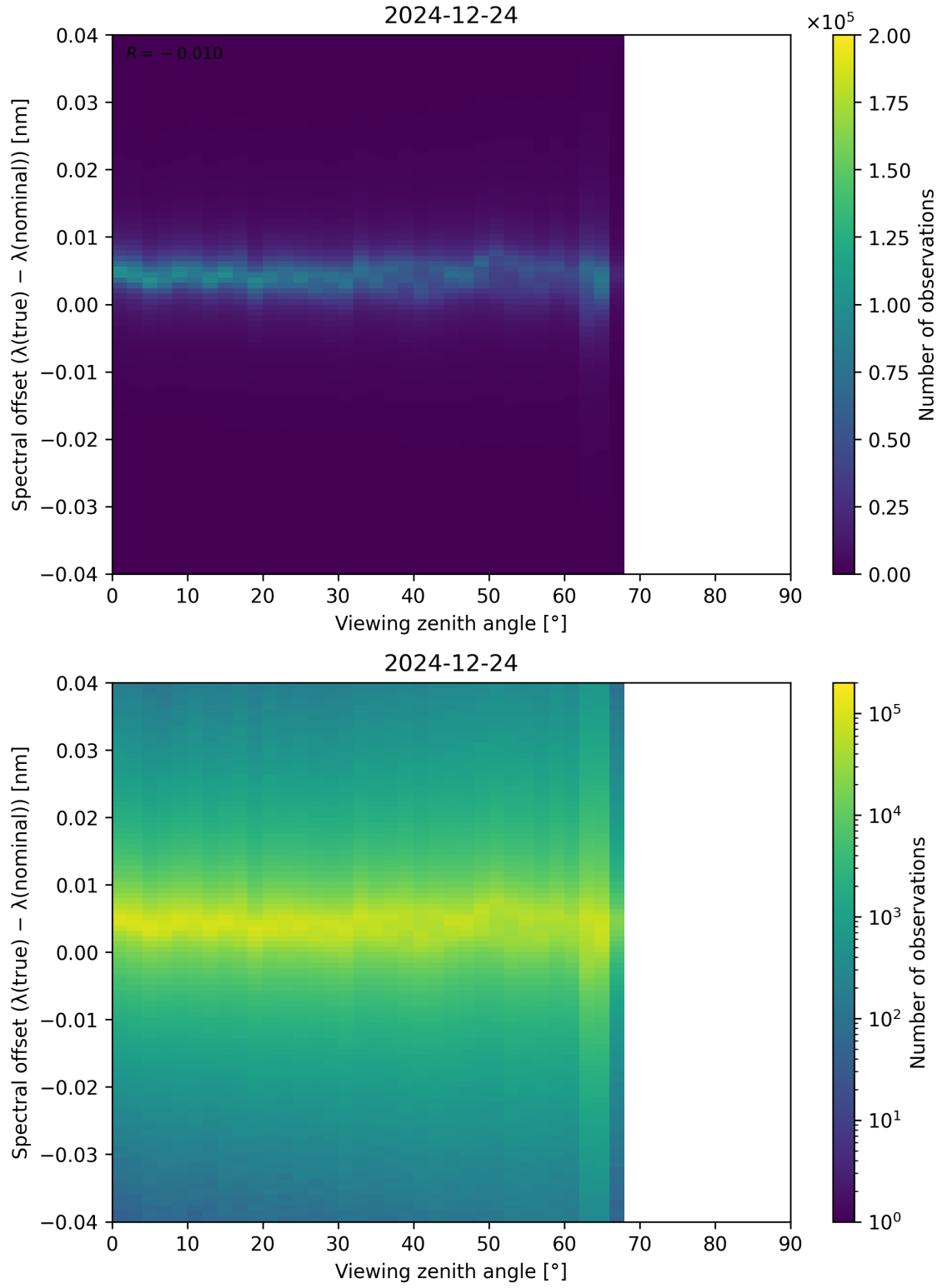
Figure 128: Scatter density plot of “Viewing zenith angle” against “Spectral offset ( \lambda_{\text{true}} - \lambda_{\text{nominal}} )” for 2024-12-23 to 2024-12-25.
