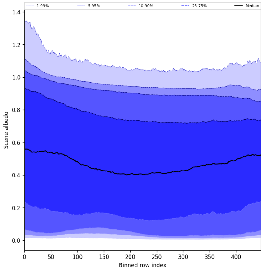
Figure 51: Along track statistics of “Scene albedo” for 2024-12-23 to 2024-12-25
