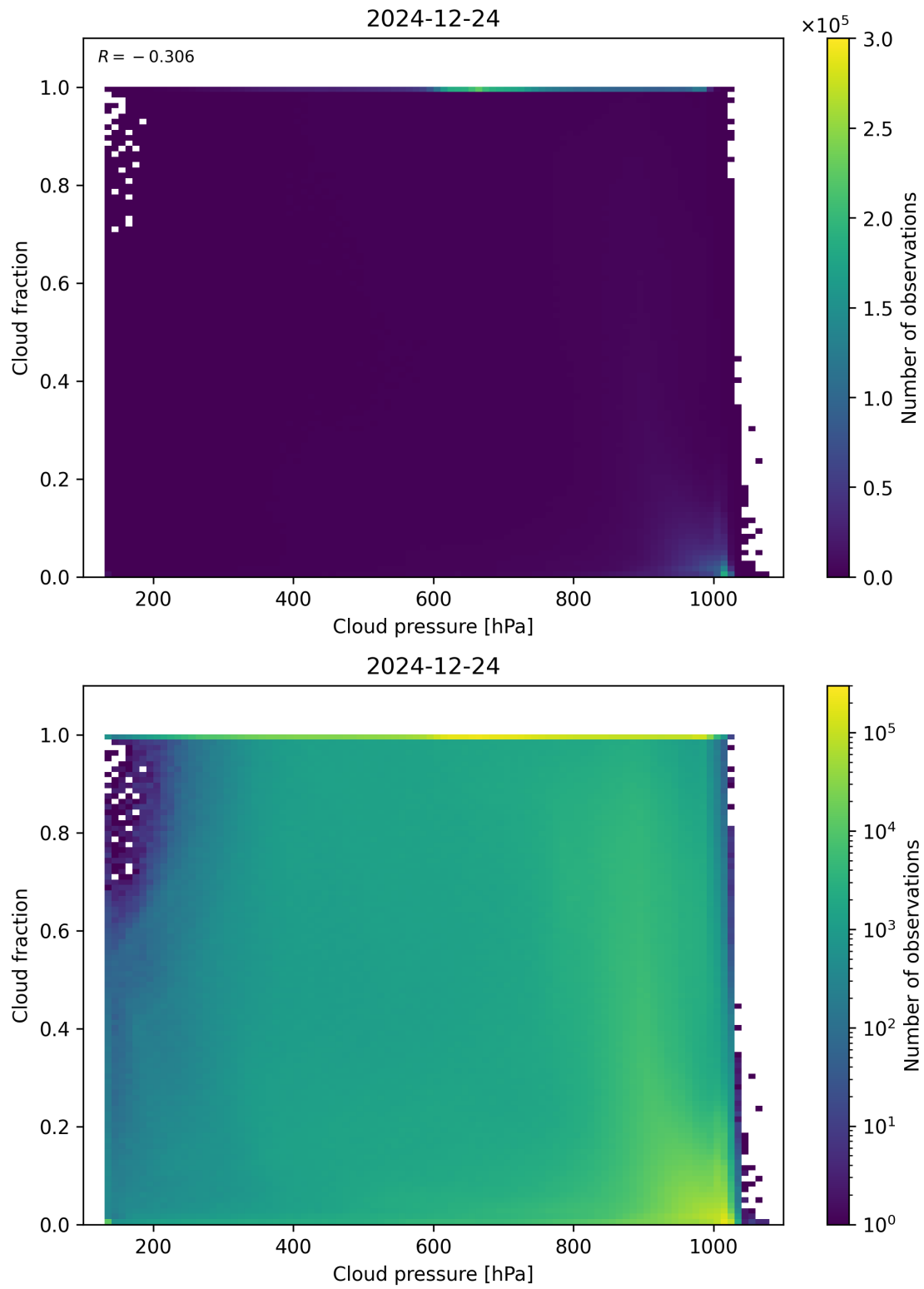
Figure 79: Scatter density plot of “Cloud pressure” against “Cloud fraction” for 2024-12-23 to 2024-12-25.
