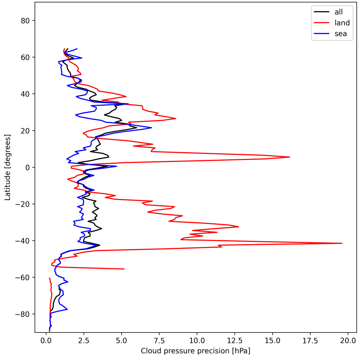
Figure 14: Zonal average of “Cloud pressure precision” for 2024-12-23 to 2024-12-25.
