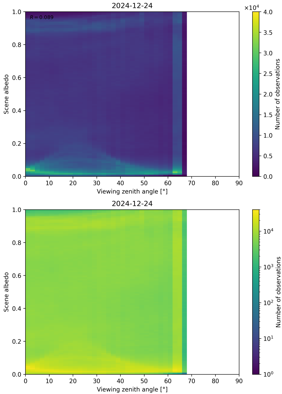
Figure 126: Scatter density plot of “Viewing zenith angle” against “Scene albedo” for 2024-12-23 to 2024-12-25.
