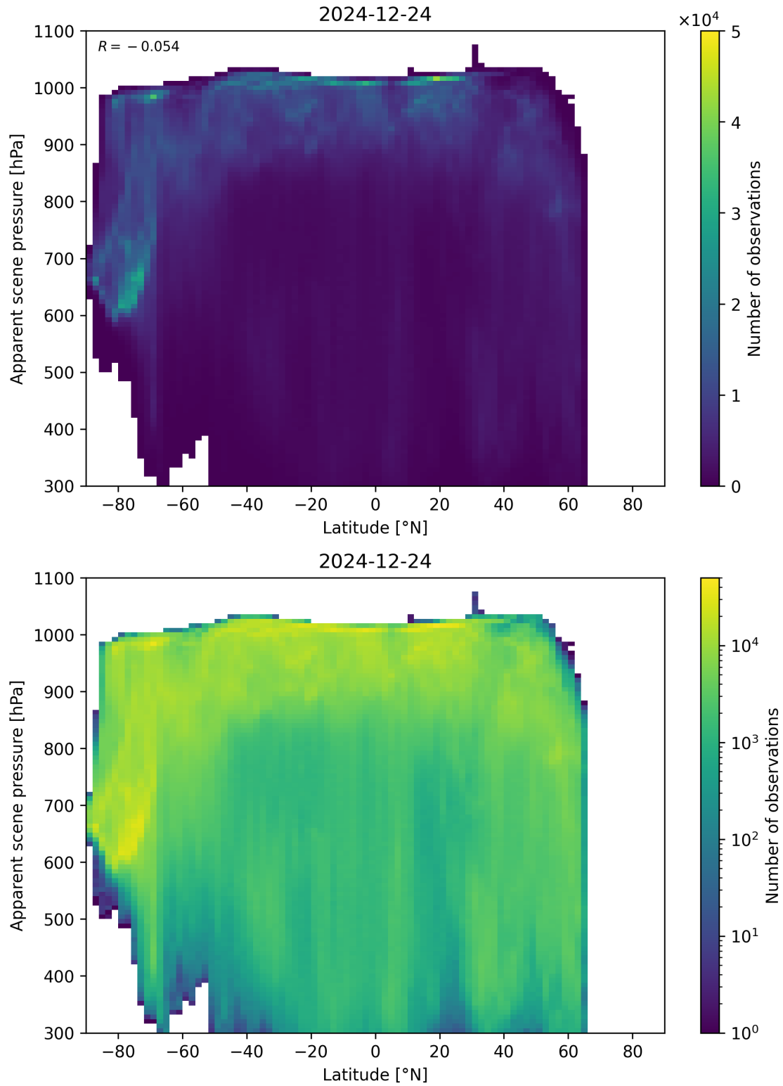
Figure 88: Scatter density plot of “Latitude” against “Apparent scene pressure” for 2024-12-23 to 2024-12-25.
