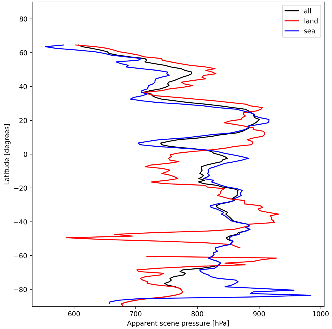
Figure 19: Zonal average of “Apparent scene pressure” for 2024-12-23 to 2024-12-25.
