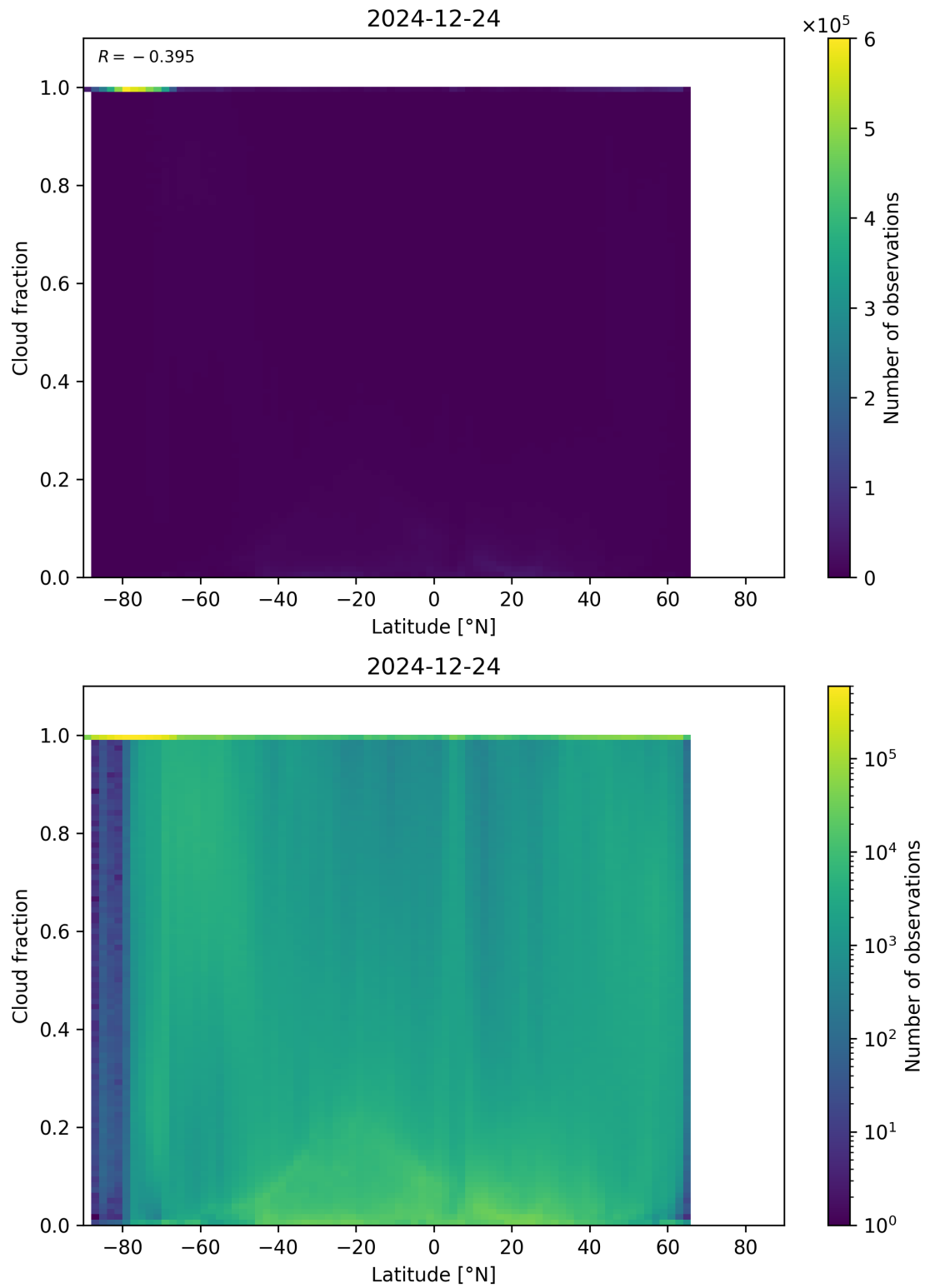
Figure 90: Scatter density plot of “Latitude” against “Cloud fraction” for 2024-12-23 to 2024-12-25.
