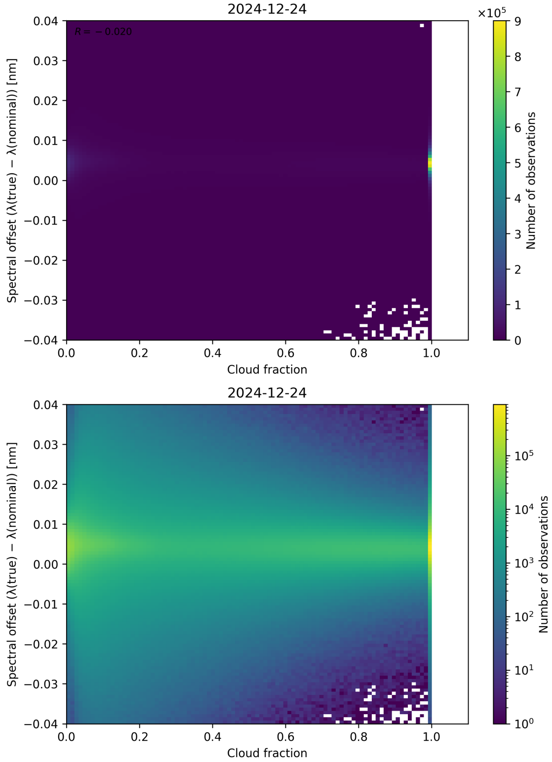
Figure 76: Scatter density plot of “Cloud fraction” against “Spectral offset ( \lambda_{\text{true}} - \lambda_{\text{nominal}} )” for 2024-12-23 to 2024-12-25.
