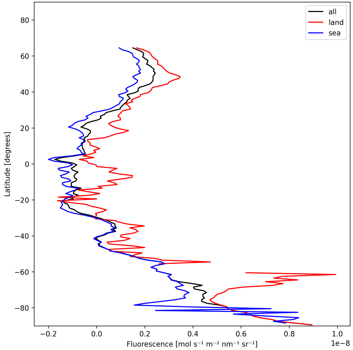
Figure 23: Zonal average of “Fluorescence” for 2024-12-23 to 2024-12-25.
