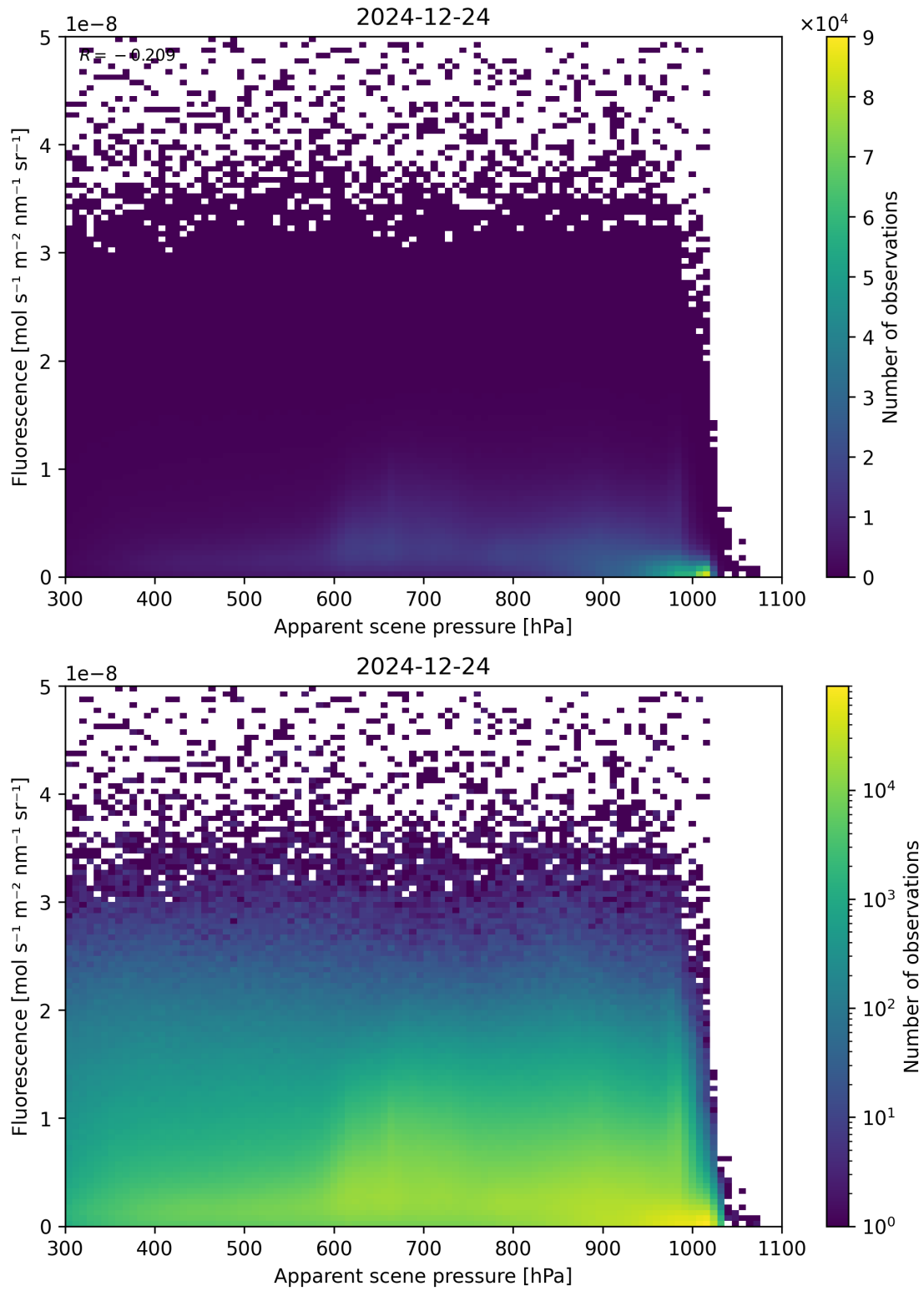
Figure 64: Scatter density plot of “Apparent scene pressure” against “Fluorescence” for 2024-12-23 to 2024-12-25.
