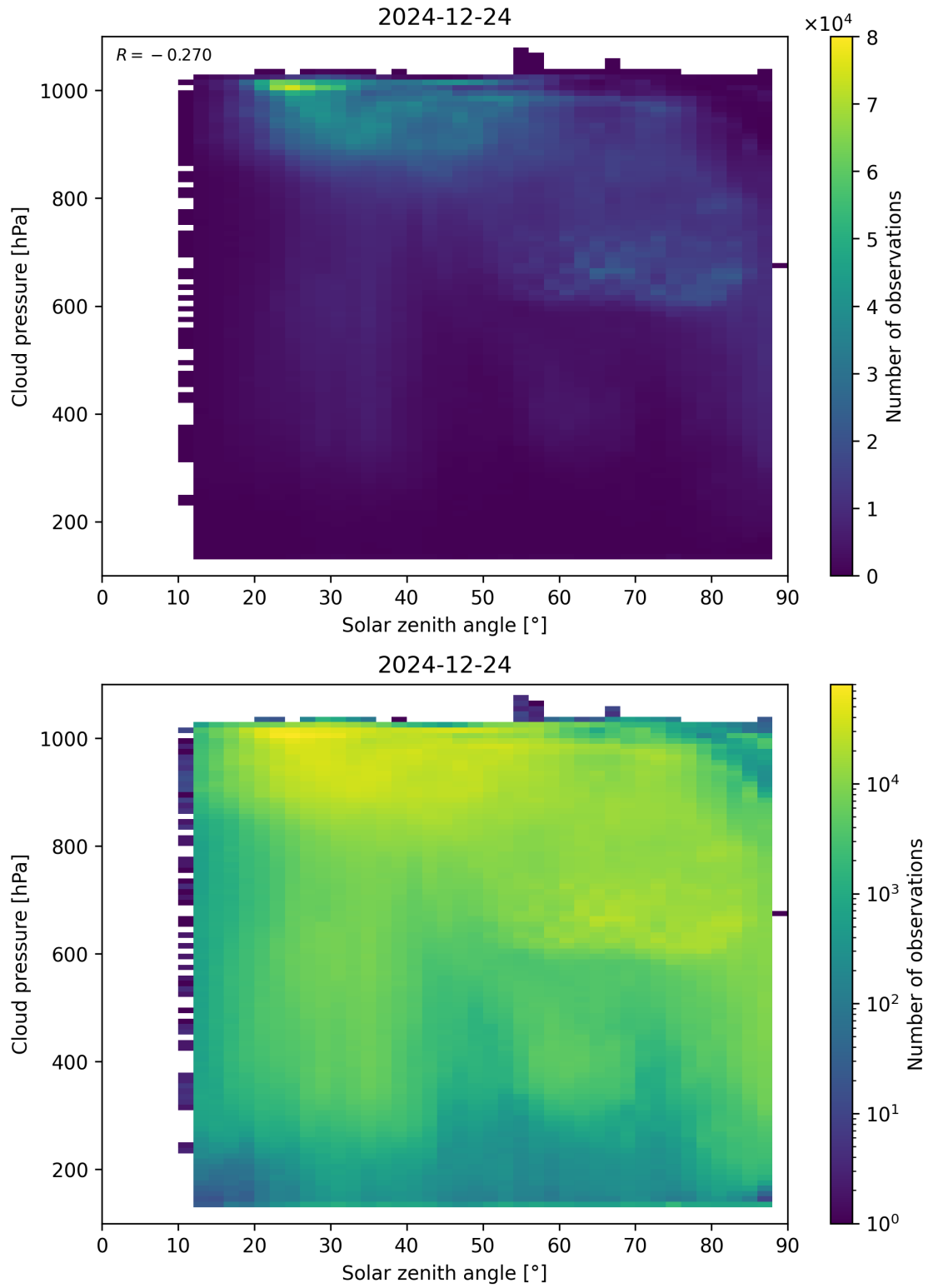
Figure 111: Scatter density plot of “Solar zenith angle” against “Cloud pressure” for 2024-12-23 to 2024-12-25.
