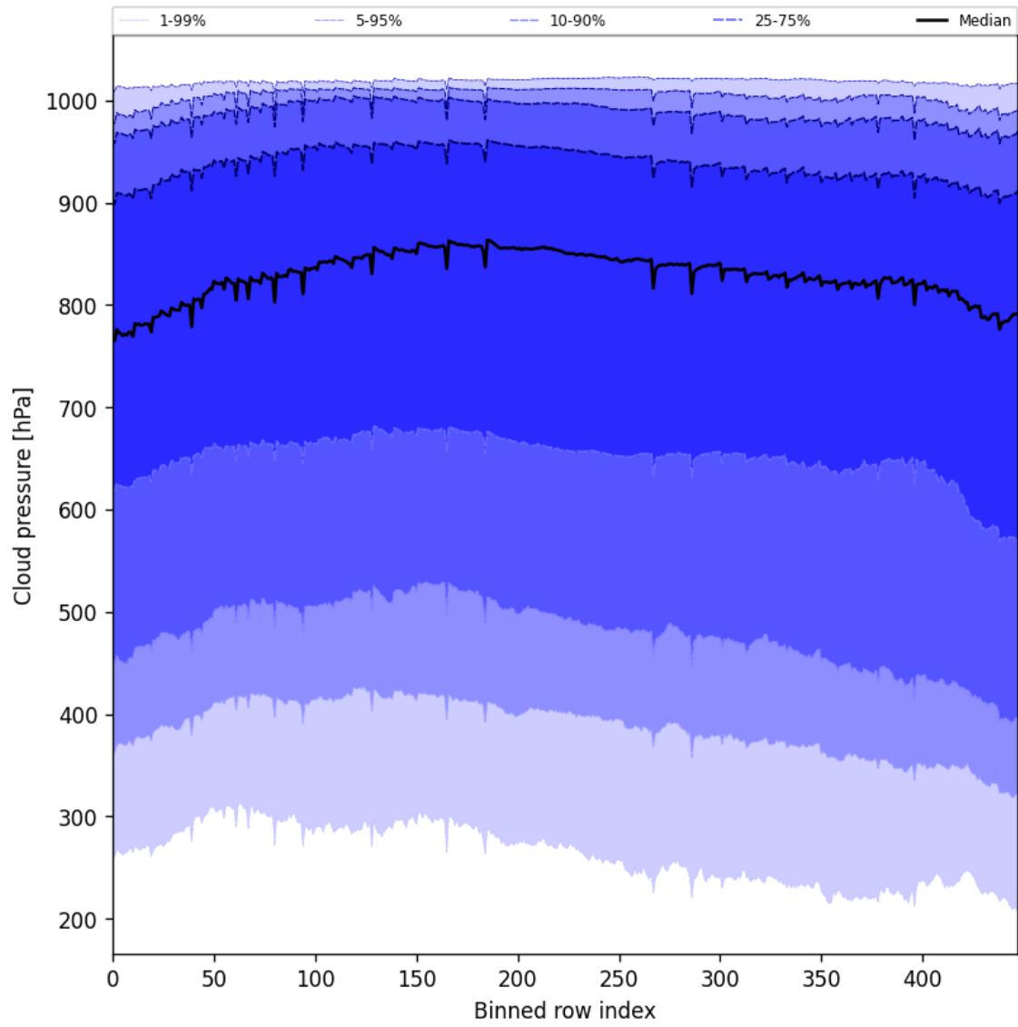
Figure 47: Along track statistics of “Cloud pressure” for 2024-12-23 to 2024-12-25
