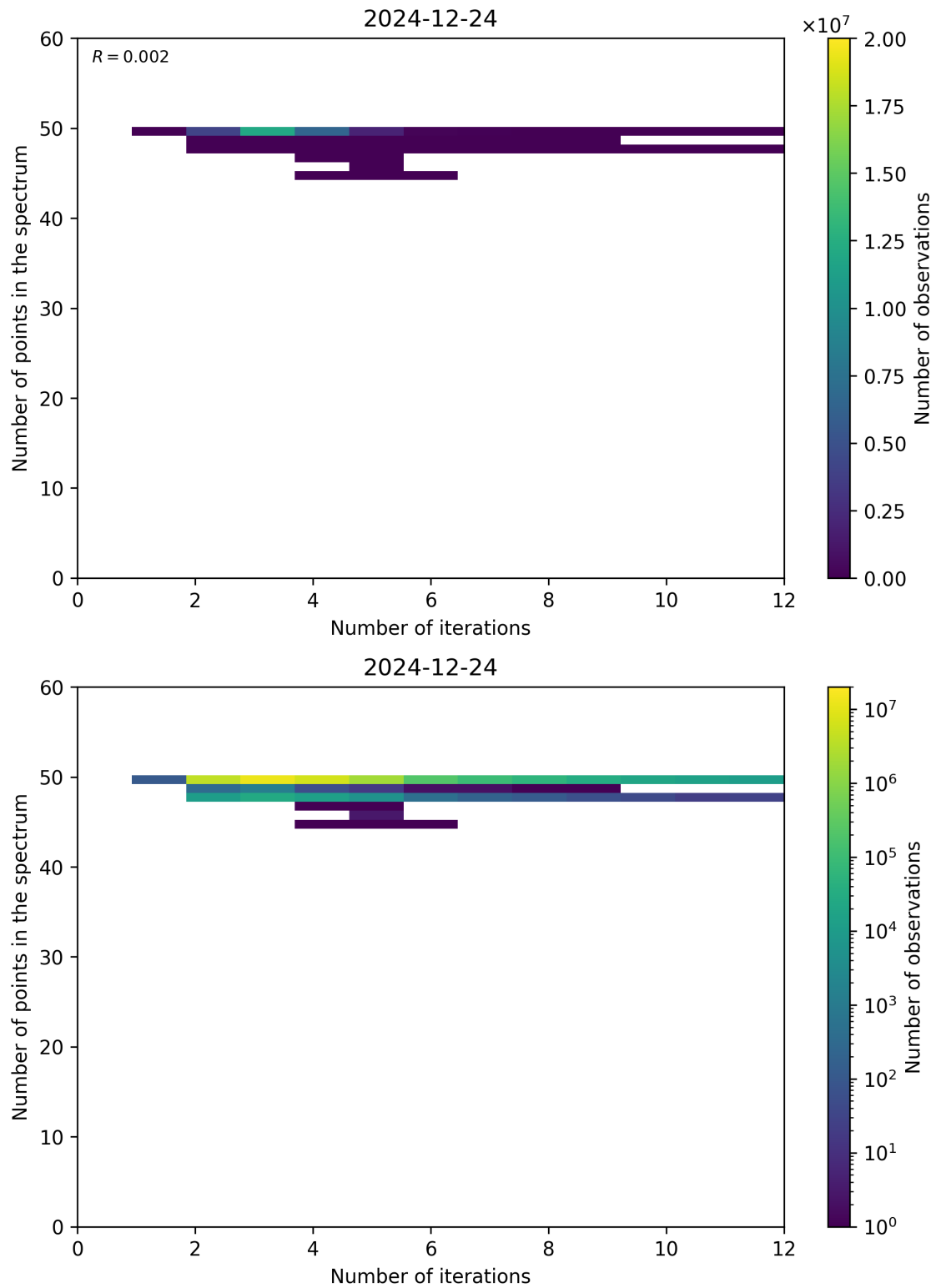
Figure 99: Scatter density plot of “Number of iterations” against “Number of points in the spectrum” for 2024-12-23 to 2024-12-25.
