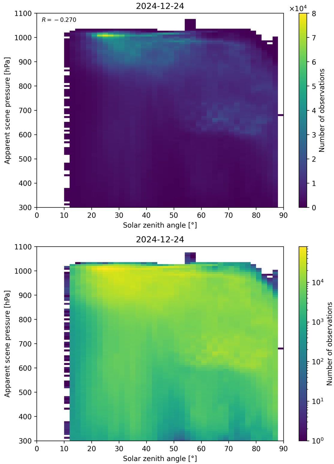
Figure 108: Scatter density plot of “Solar zenith angle” against “Apparent scene pressure” for 2024-12-23 to 2024-12-25.
