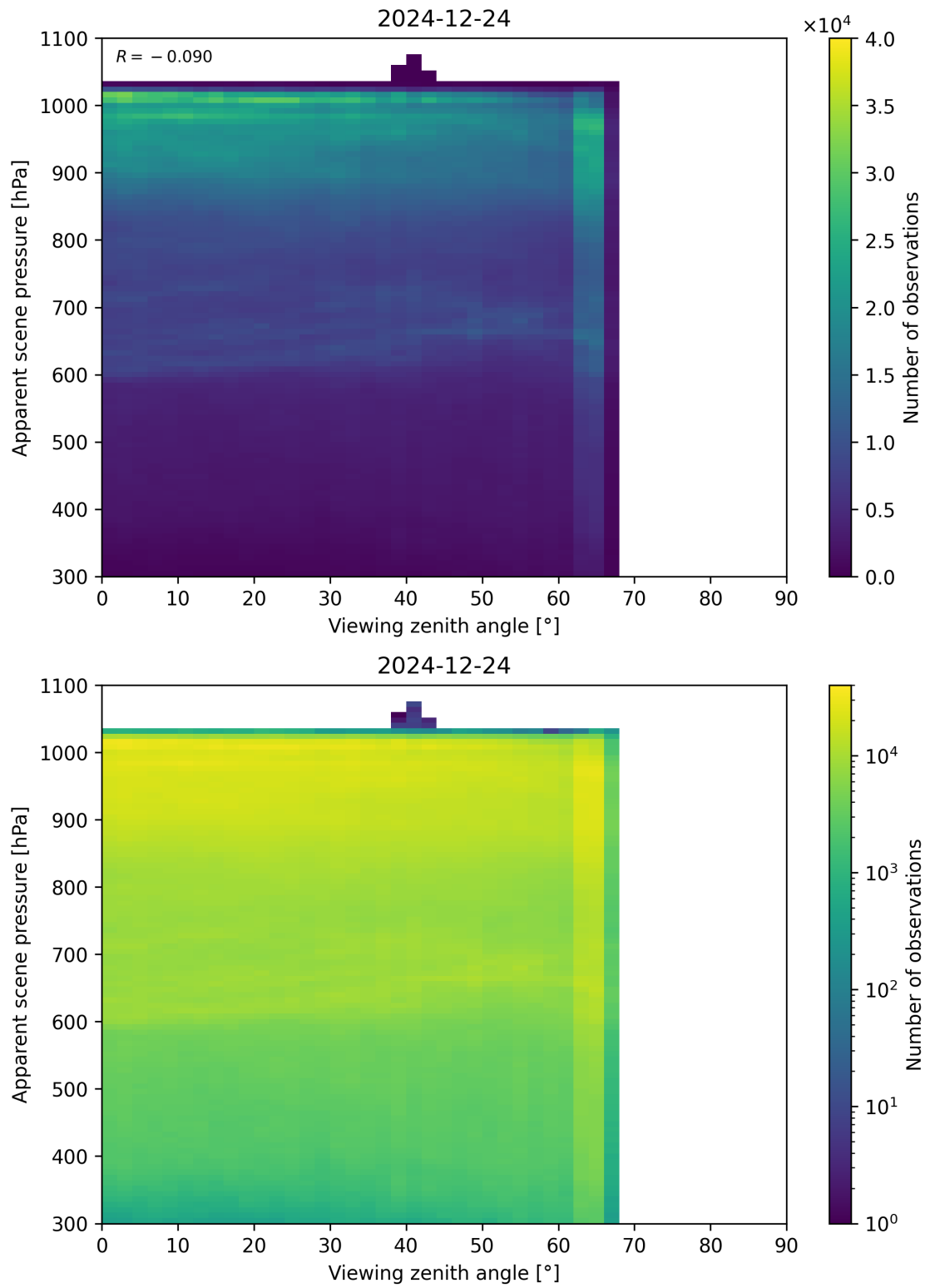
Figure 118: Scatter density plot of “Viewing zenith angle” against “Apparent scene pressure” for 2024-12-23 to 2024-12-25.
