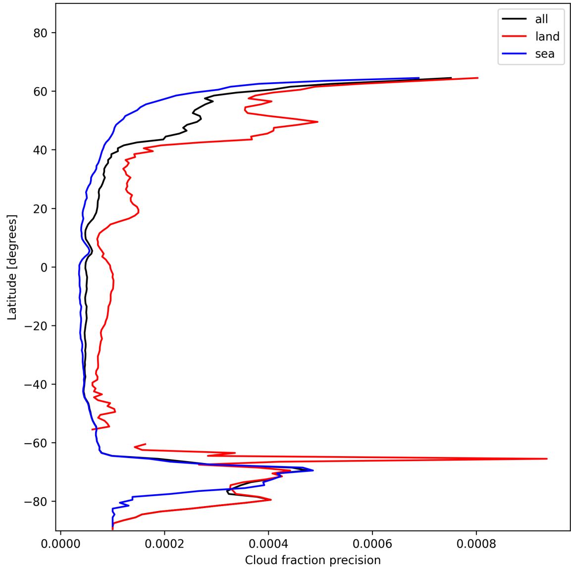
Figure 16: Zonal average of “Cloud fraction precision” for 2024-12-23 to 2024-12-25.
