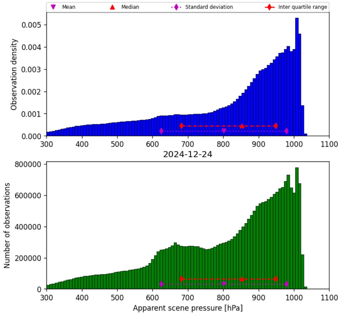
Figure 36: Histogram of “Apparent scene pressure” for 2024-12-23 to 2024-12-25
