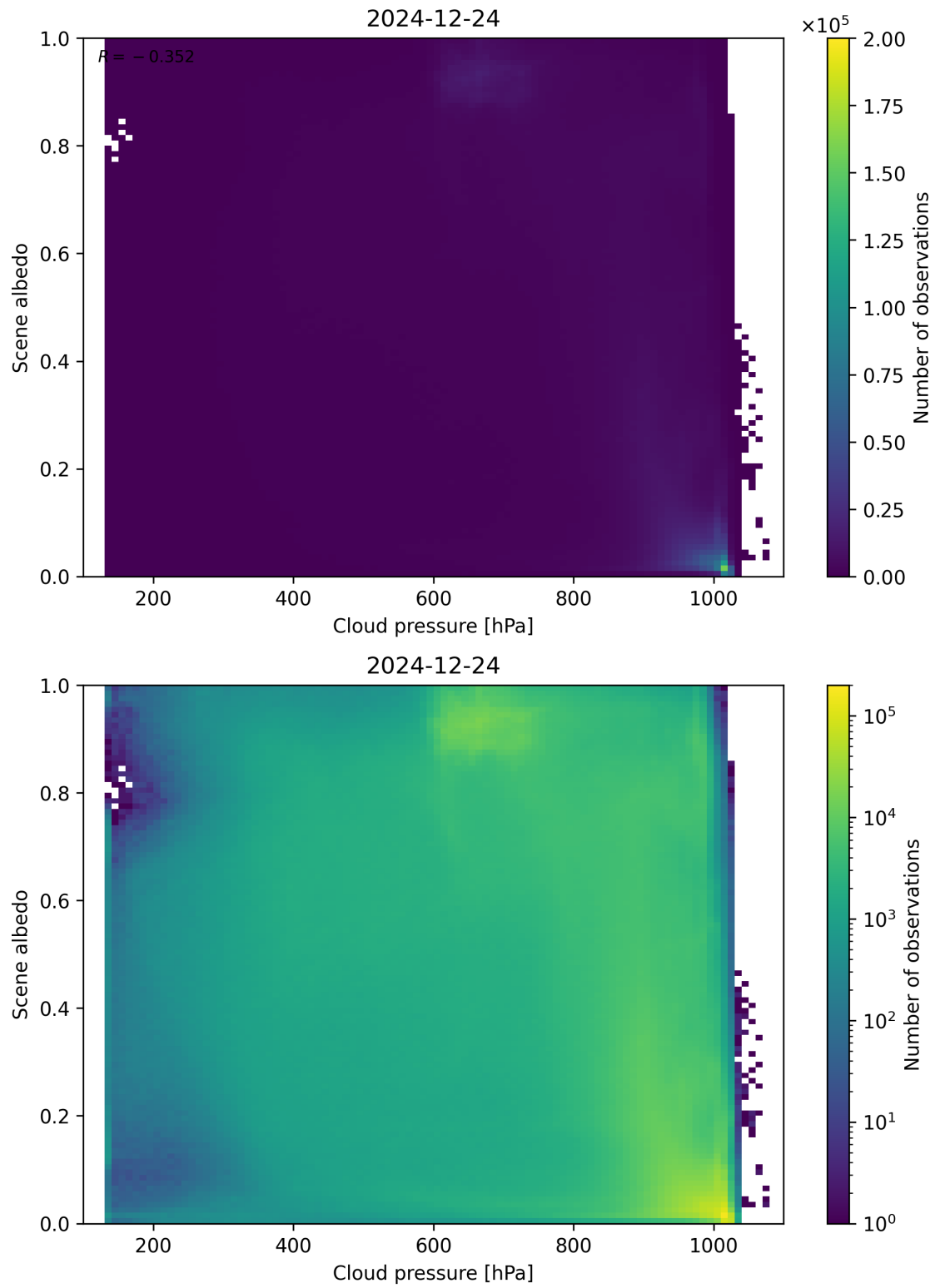
Figure 83: Scatter density plot of “Cloud pressure” against “Scene albedo” for 2024-12-23 to 2024-12-25.
