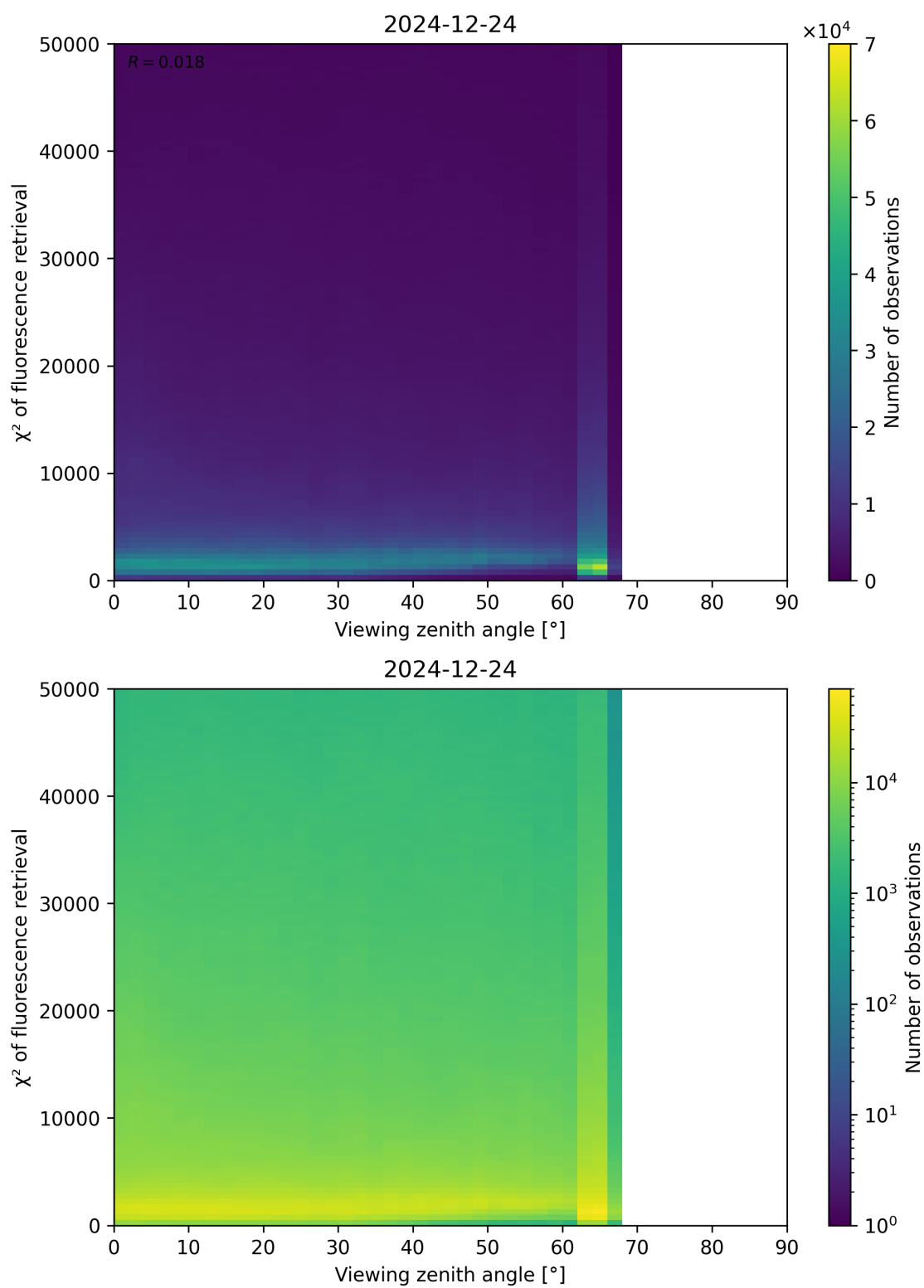
Figure 119: Scatter density plot of “Viewing zenith angle” against “ \chi^2 of fluorescence retrieval” for 2024-12-23 to 2024-12-25.
