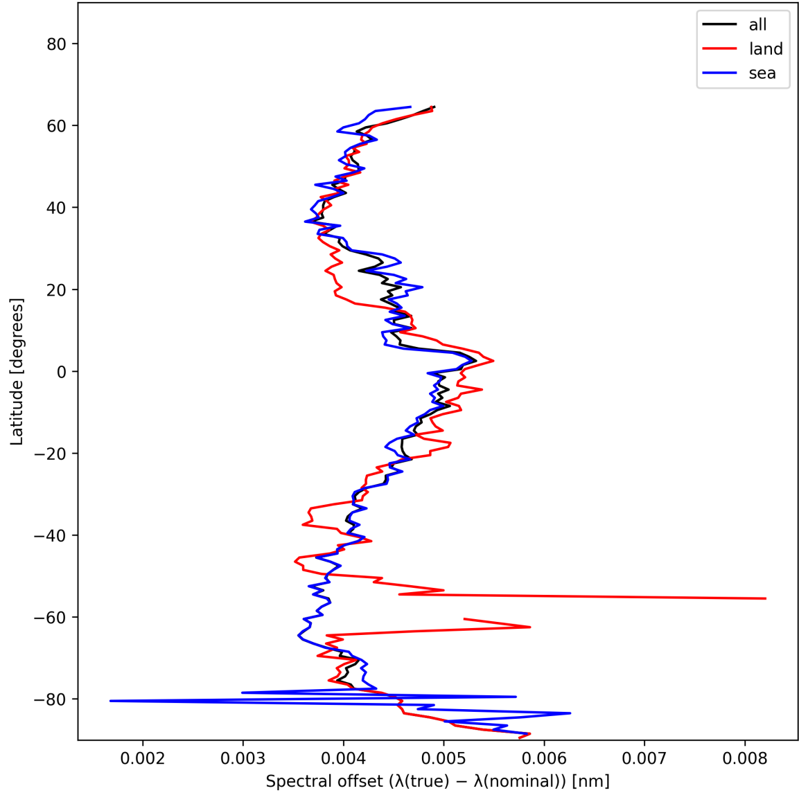
Figure 28: Zonal average of “Spectral offset ( \lambda_{\text{true}} - \lambda_{\text{nominal}} )” for 2024-12-23 to 2024-12-25.
