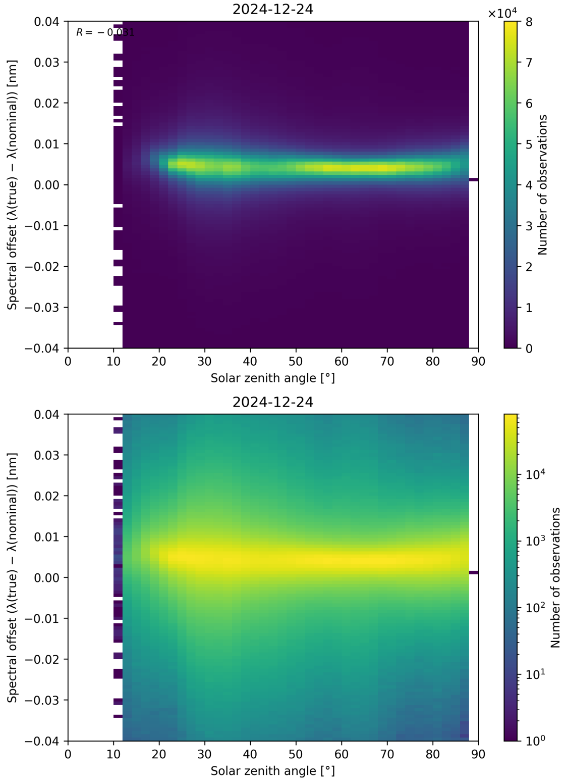
Figure 117: Scatter density plot of “Solar zenith angle” against “Spectral offset ( \lambda_{\text{true}} - \lambda_{\text{nominal}} )” for 2024-12-23 to 2024-12-25.
