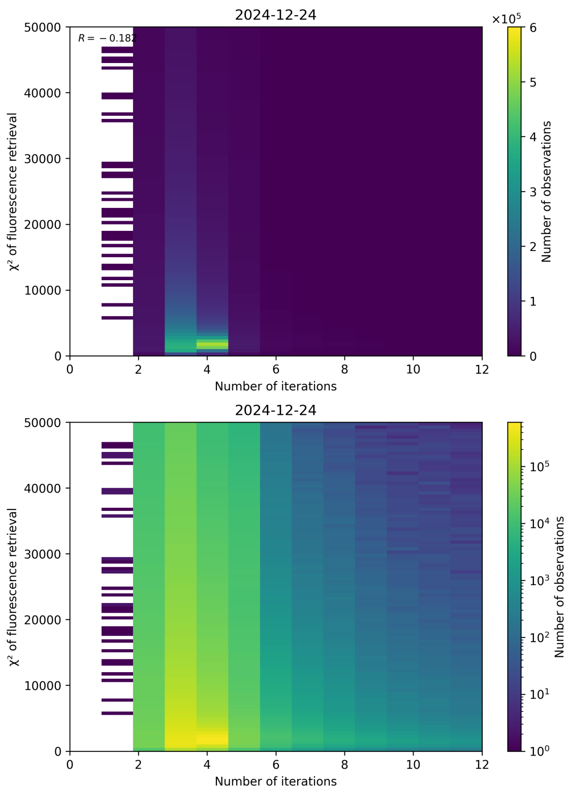
Figure 97: Scatter density plot of “Number of iterations” against “ \chi^2 of fluorescence retrieval” for 2024-12-23 to 2024-12-25.
