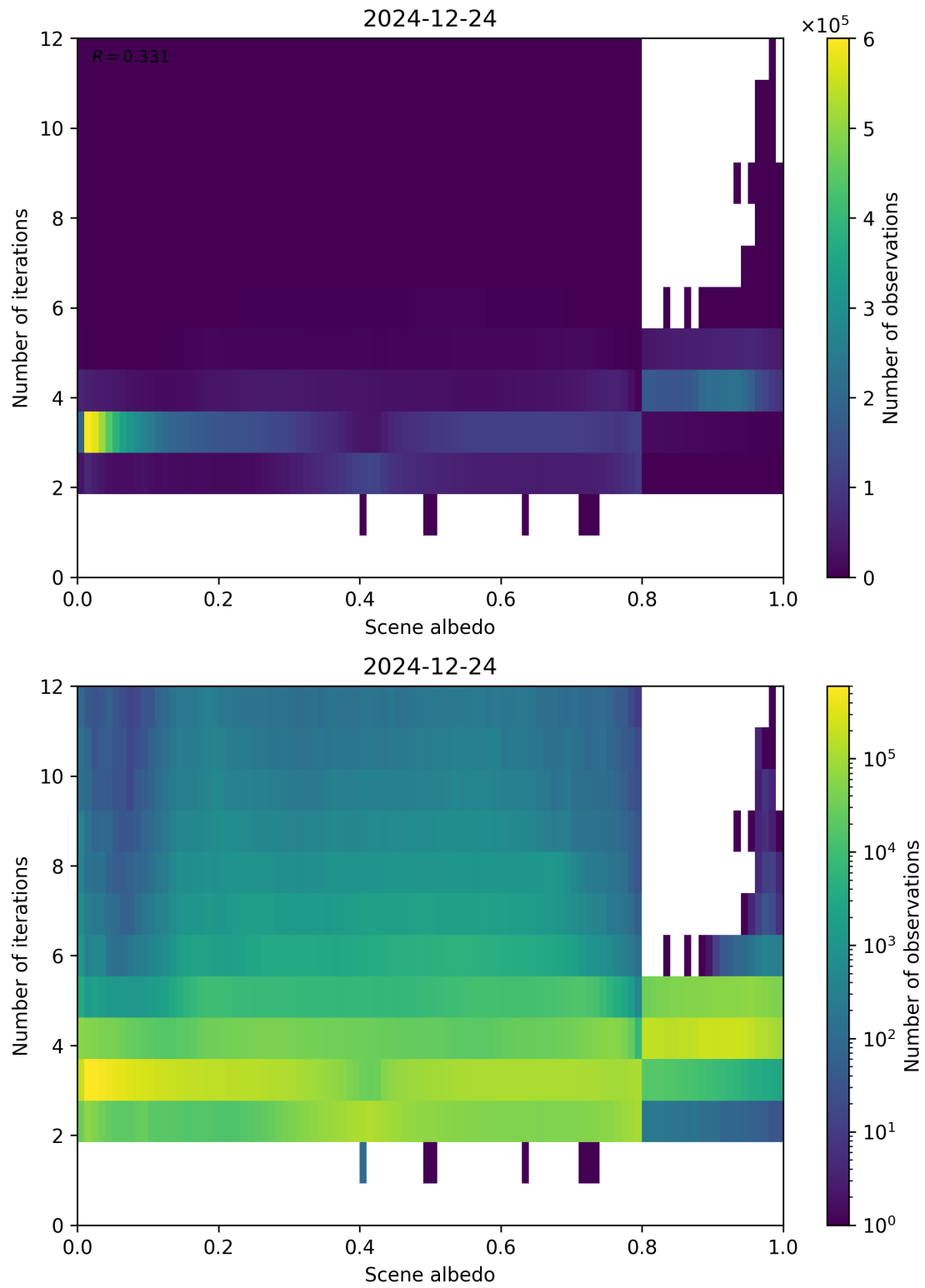
Figure 105: Scatter density plot of “Scene albedo” against “Number of iterations” for 2024-12-23 to 2024-12-25.
