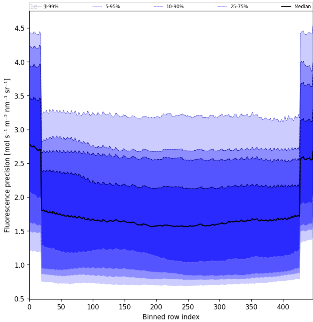
Figure 58: Along track statistics of “Fluorescence precision” for 2024-12-23 to 2024-12-25
