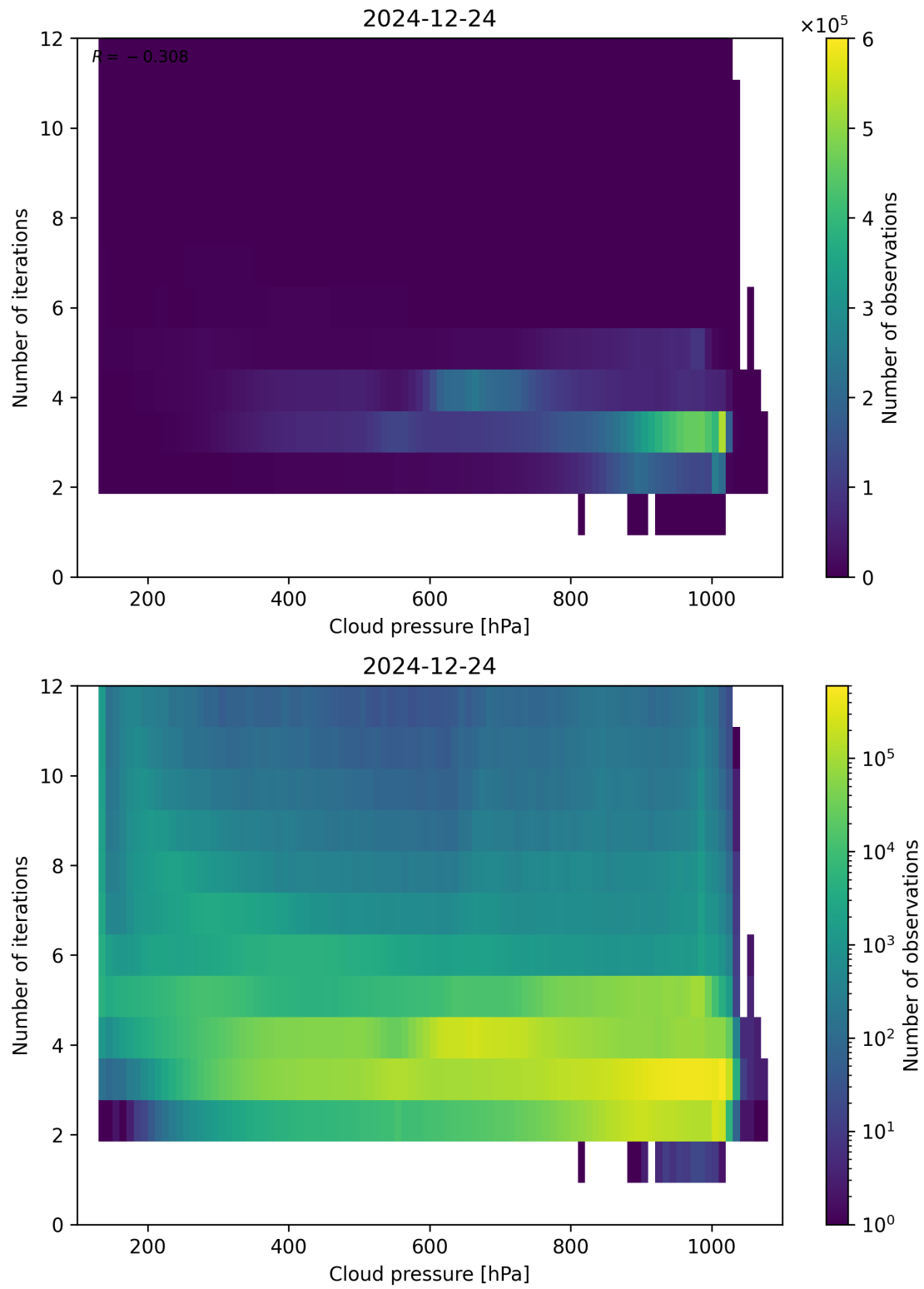
Figure 81: Scatter density plot of “Cloud pressure” against “Number of iterations” for 2024-12-23 to 2024-12-25.
