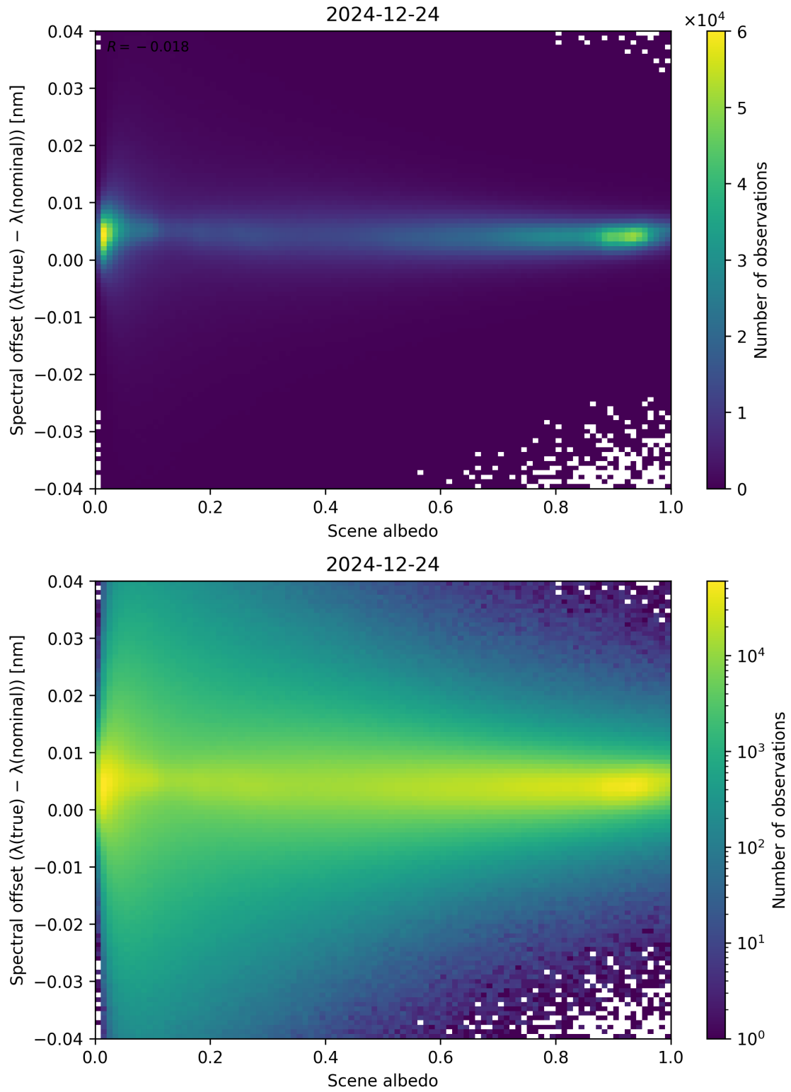
Figure 107: Scatter density plot of “Scene albedo” against “Spectral offset ( \lambda_{\text{true}} - \lambda_{\text{nominal}} )” for 2024-12-23 to 2024-12-25.
