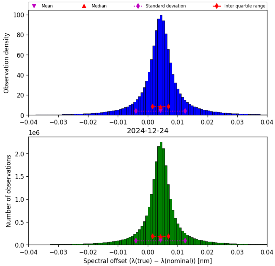
Figure 45: Histogram of “Spectral offset ( \lambda_{\text{true}} - \lambda_{\text{nominal}} )” for 2024-12-23 to 2024-12-25
