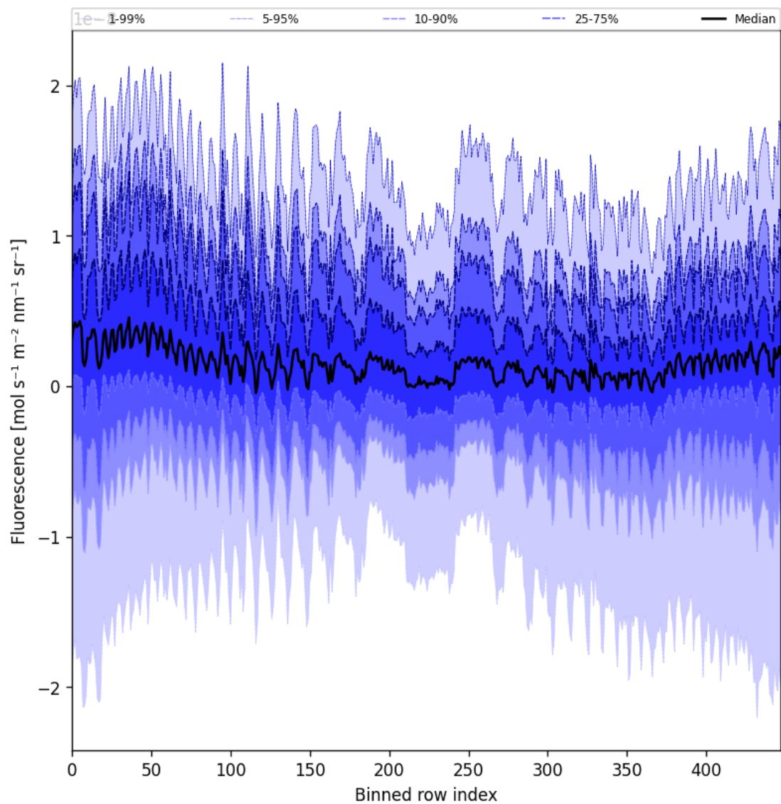
Figure 57: Along track statistics of “Fluorescence” for 2024-12-23 to 2024-12-25
