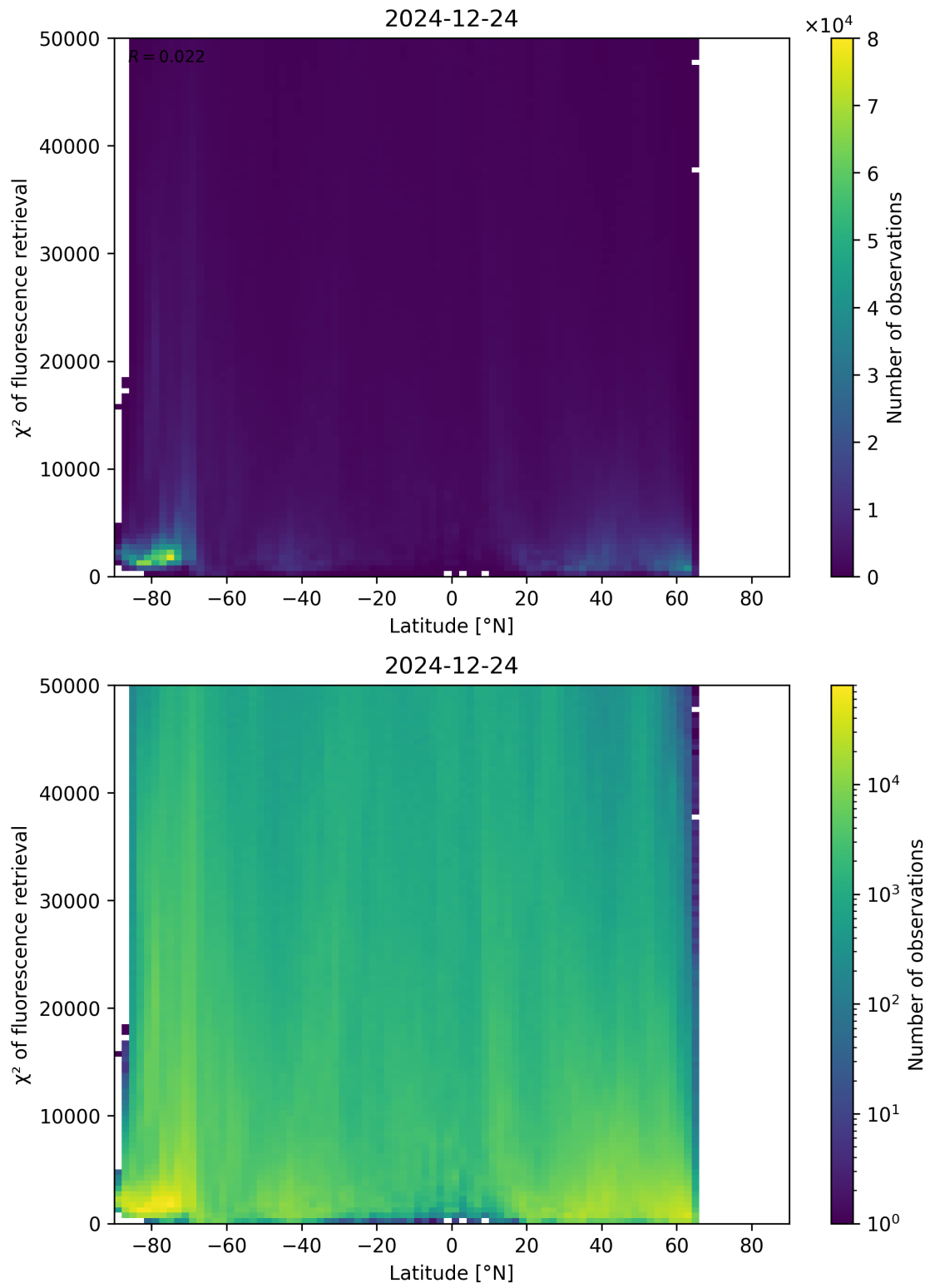
Figure 89: Scatter density plot of “Latitude” against “ \chi^2 of fluorescence retrieval” for 2024-12-23 to 2024-12-25.
