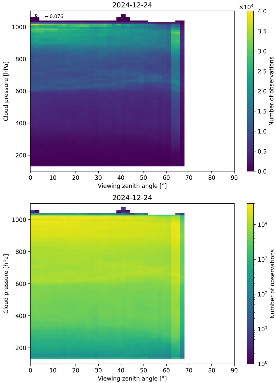
Figure 121: Scatter density plot of “Viewing zenith angle” against “Cloud pressure” for 2024-12-23 to 2024-12-25.
