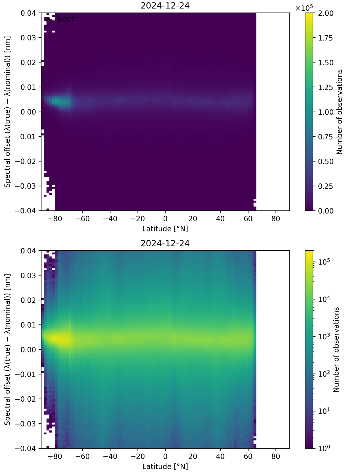
Figure 96: Scatter density plot of “Latitude” against “Spectral offset ( \lambda_{\text{true}} - \lambda_{\text{nominal}} )” for 2024-12-23 to 2024-12-25.
