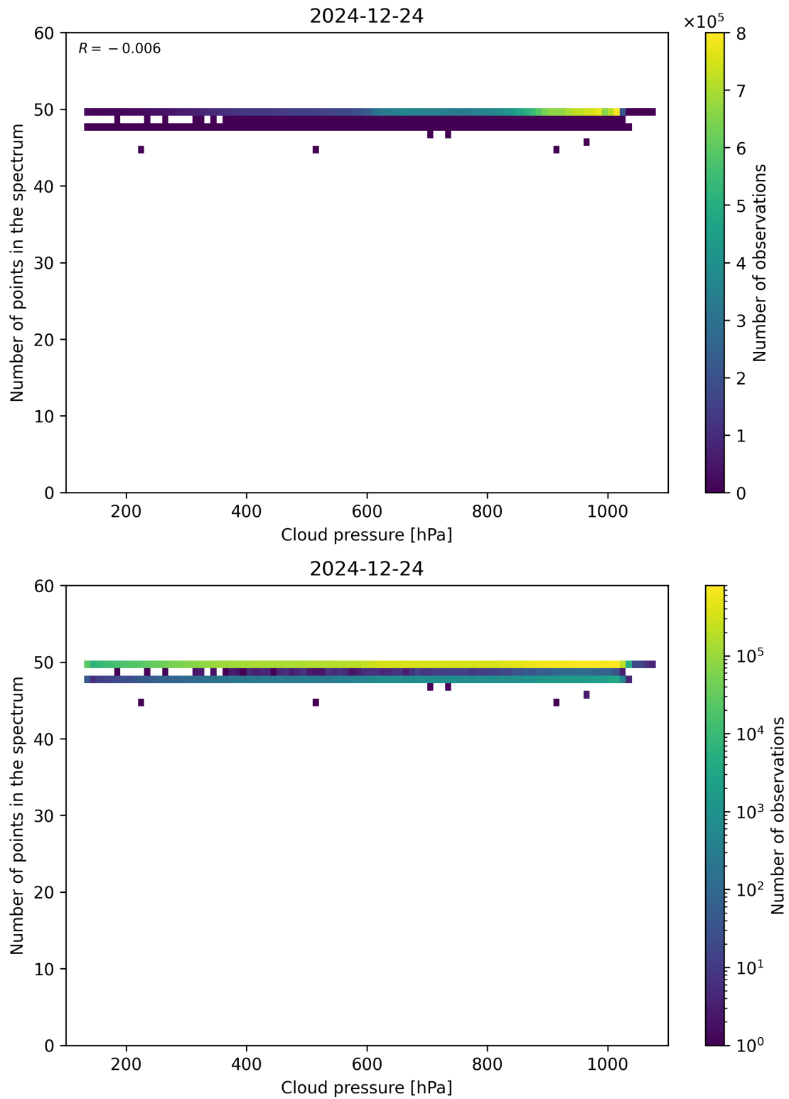
Figure 82: Scatter density plot of “Cloud pressure” against “Number of points in the spectrum” for 2024-12-23 to 2024-12-25.
