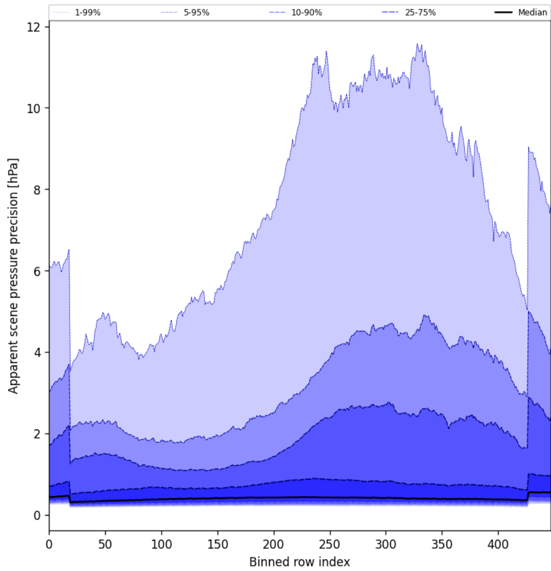
Figure 54: Along track statistics of “Apparent scene pressure precision” for 2024-12-23 to 2024-12-25
