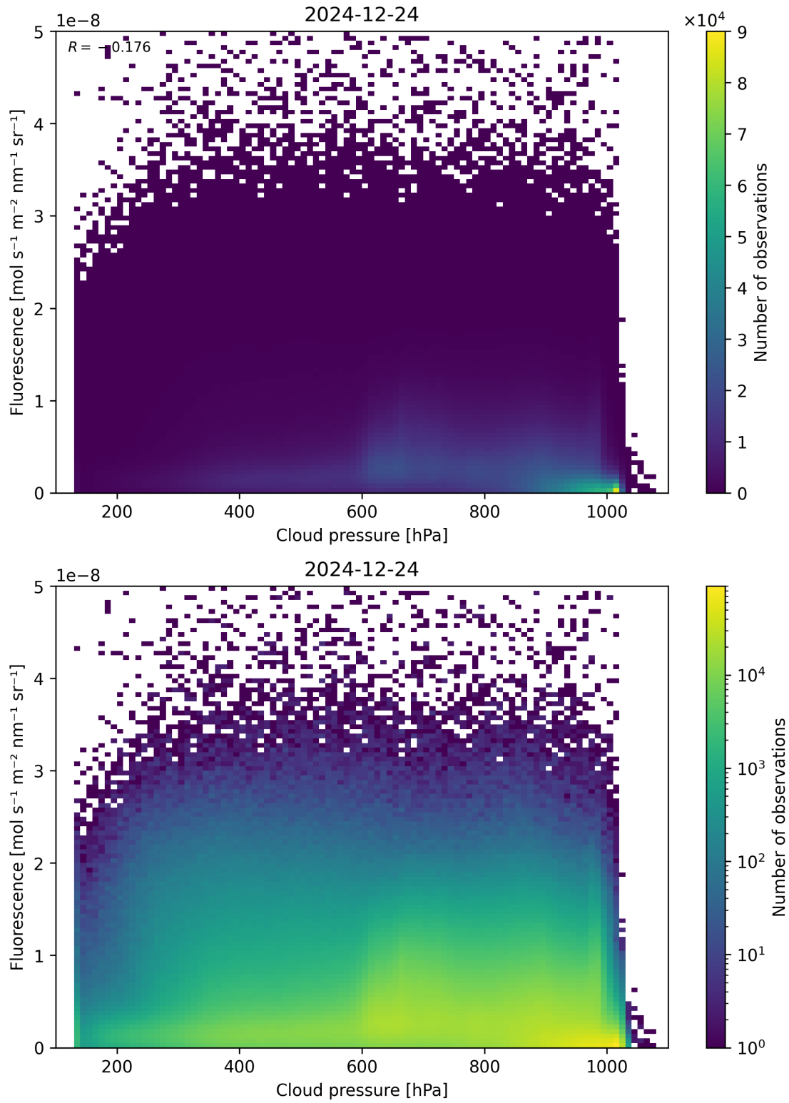
Figure 80: Scatter density plot of “Cloud pressure” against “Fluorescence” for 2024-12-23 to 2024-12-25.
