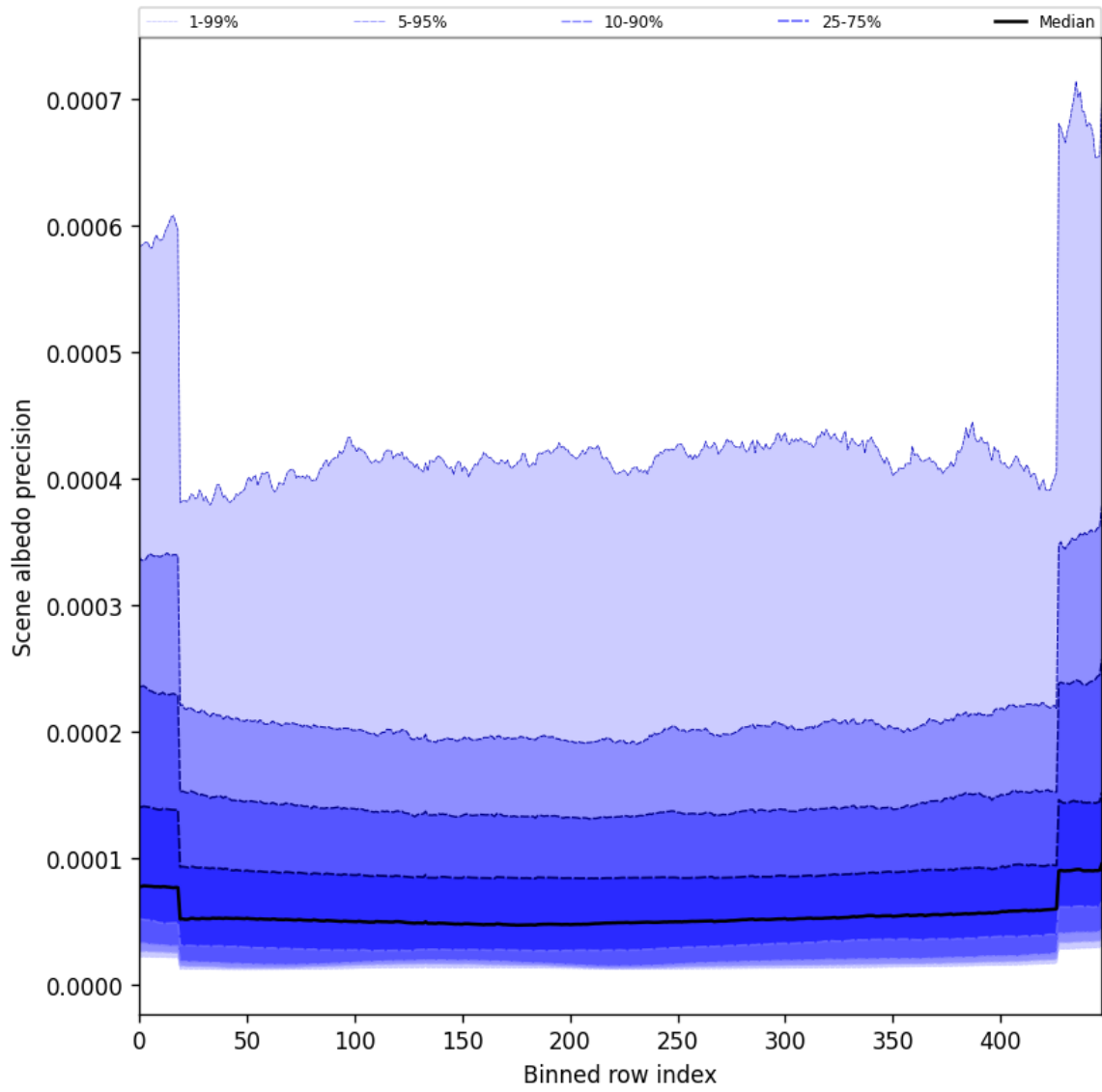
Figure 52: Along track statistics of “Scene albedo precision” for 2024-12-23 to 2024-12-25
