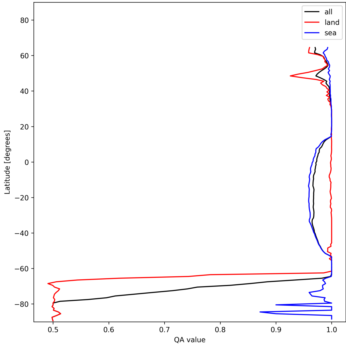
Figure 12: Zonal average of “QA value” for 2024-12-23 to 2024-12-25.
