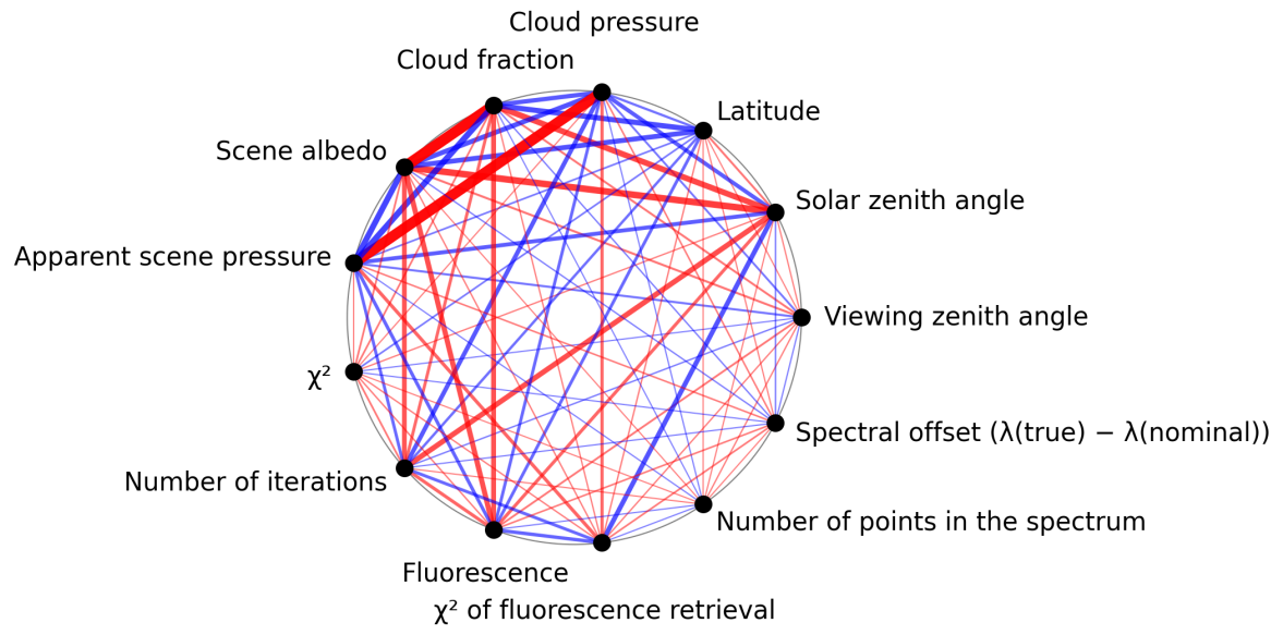
Figure 1: Map of correlation graph for 2024-12-23 to 2024-12-25.
