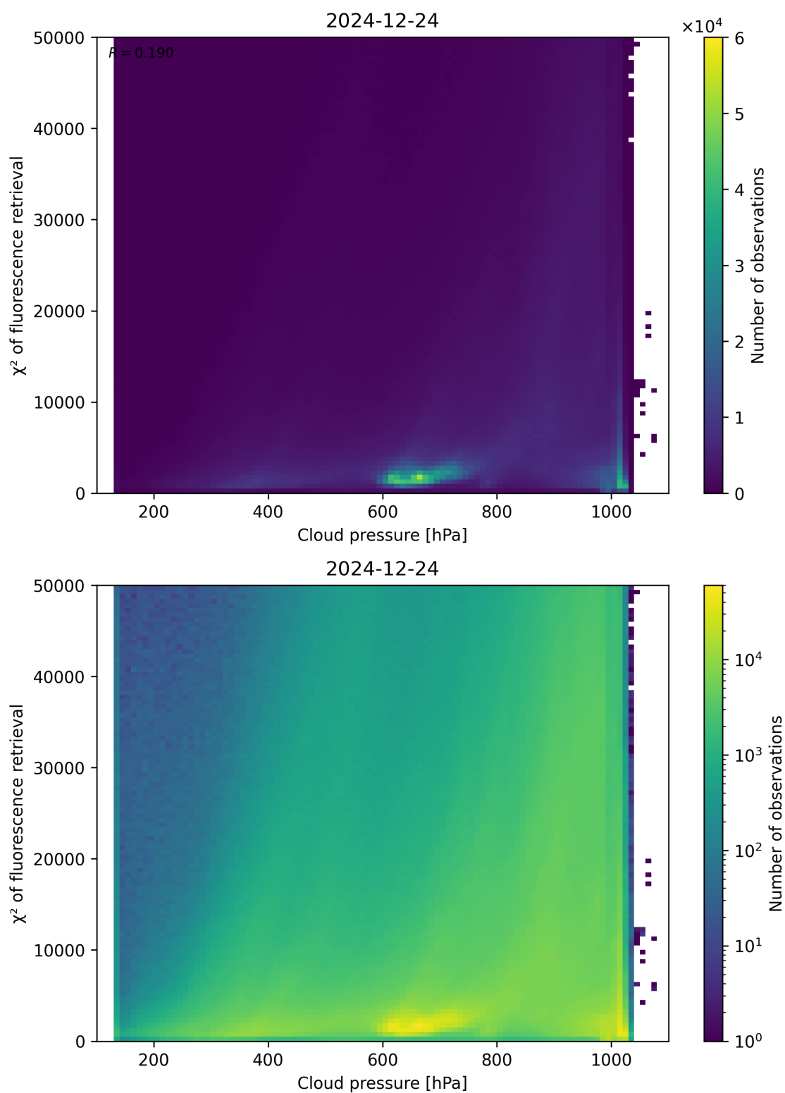
Figure 78: Scatter density plot of “Cloud pressure” against “ \chi^2 of fluorescence retrieval” for 2024-12-23 to 2024-12-25.
