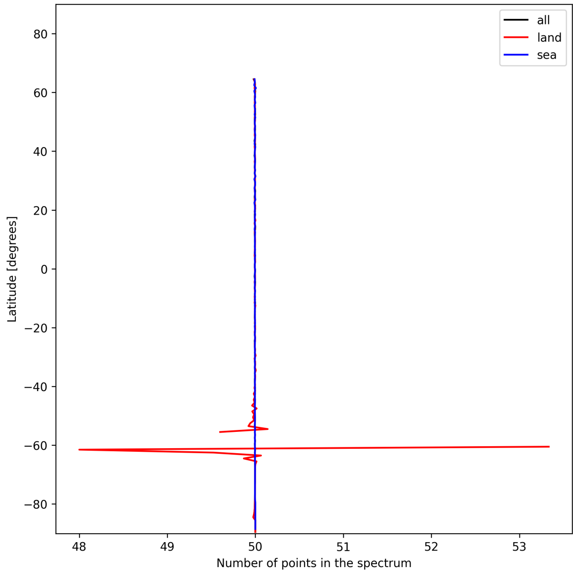
Figure 27: Zonal average of “Number of points in the spectrum” for 2024-12-23 to 2024-12-25.
