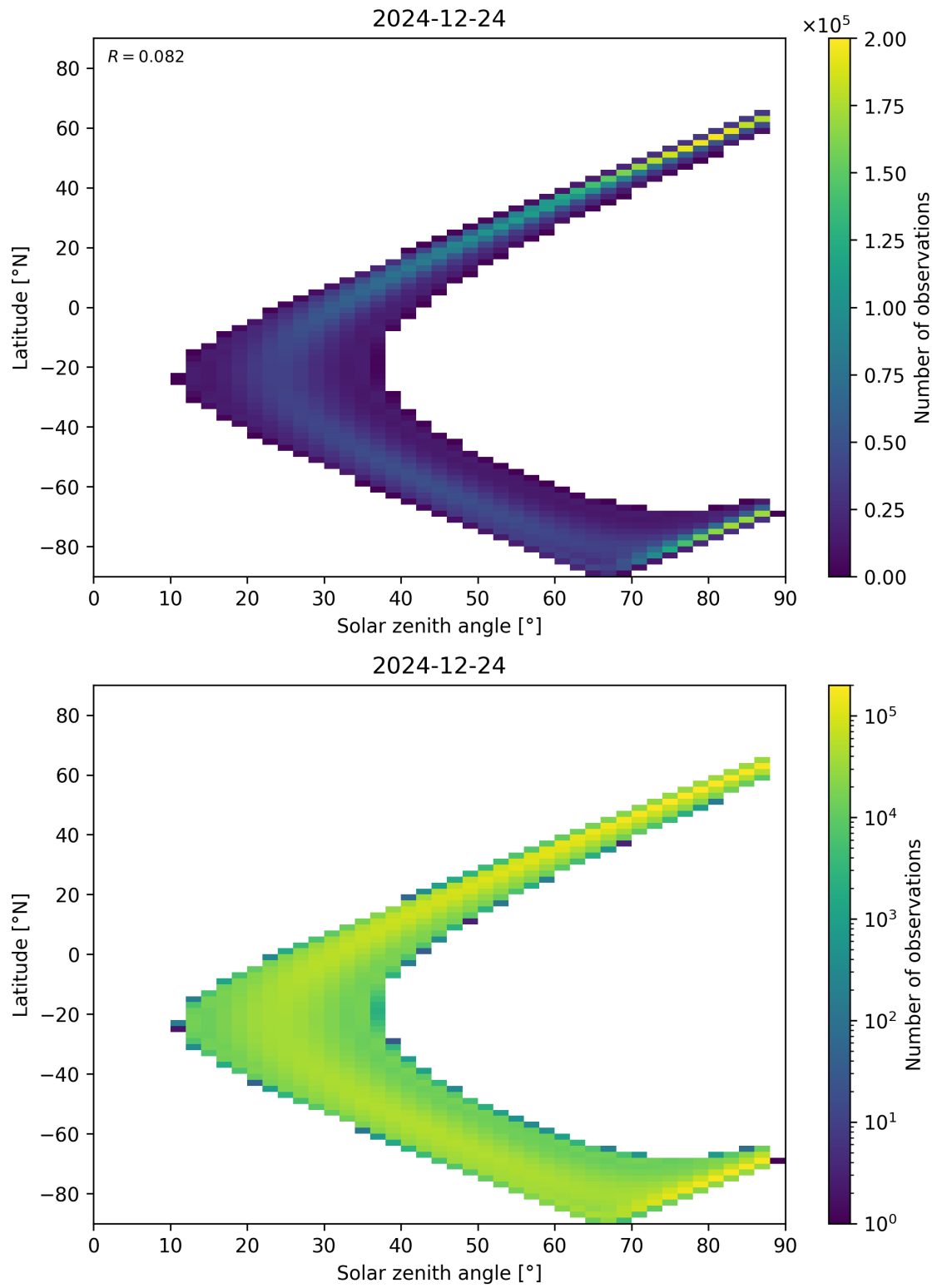
Figure 113: Scatter density plot of “Solar zenith angle” against “Latitude” for 2024-12-23 to 2024-12-25.
