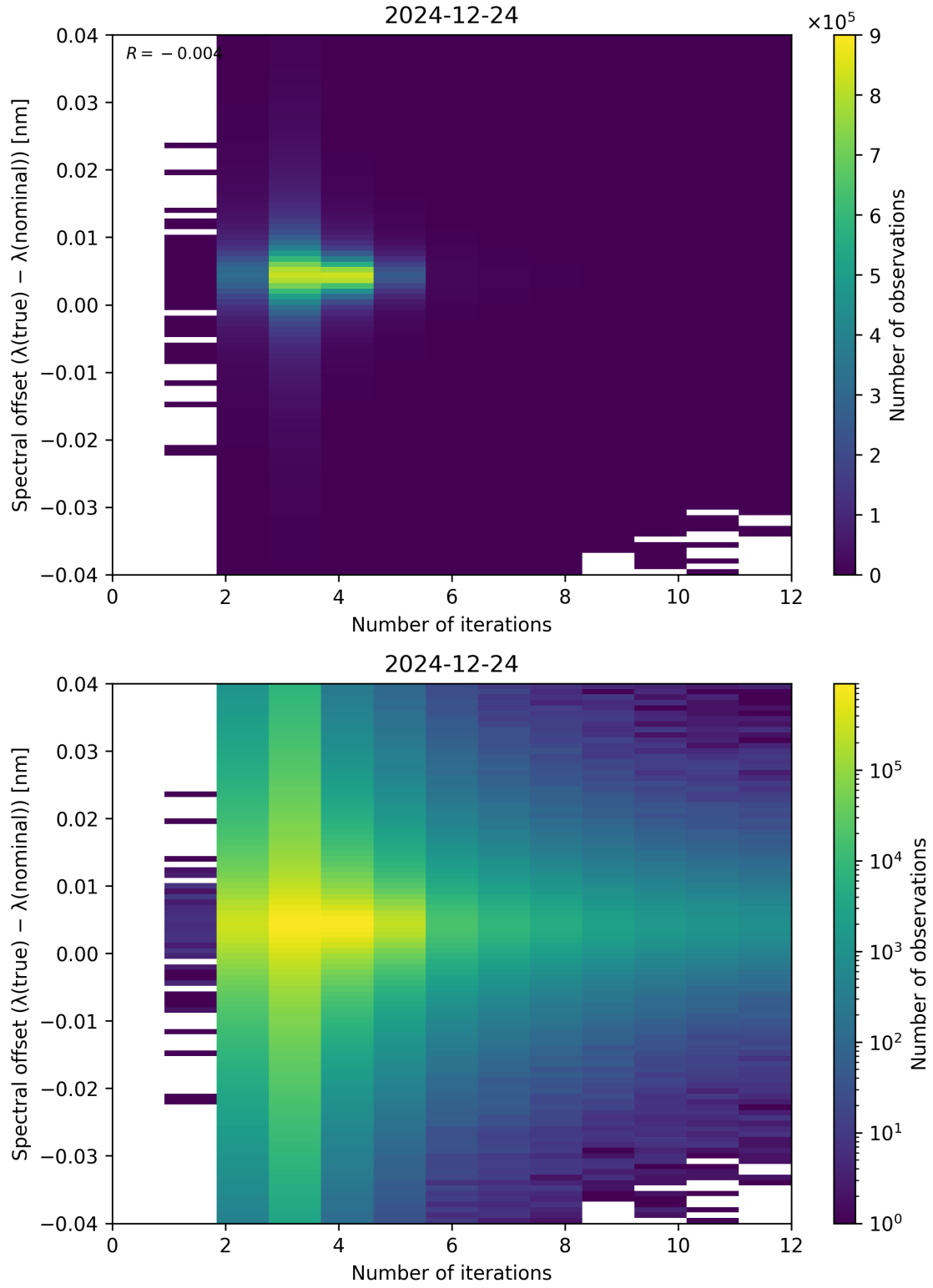
Figure 100: Scatter density plot of “Number of iterations” against “Spectral offset ( \lambda_{\text{true}} - \lambda_{\text{nominal}} )” for 2024-12-23 to 2024-12-25.
