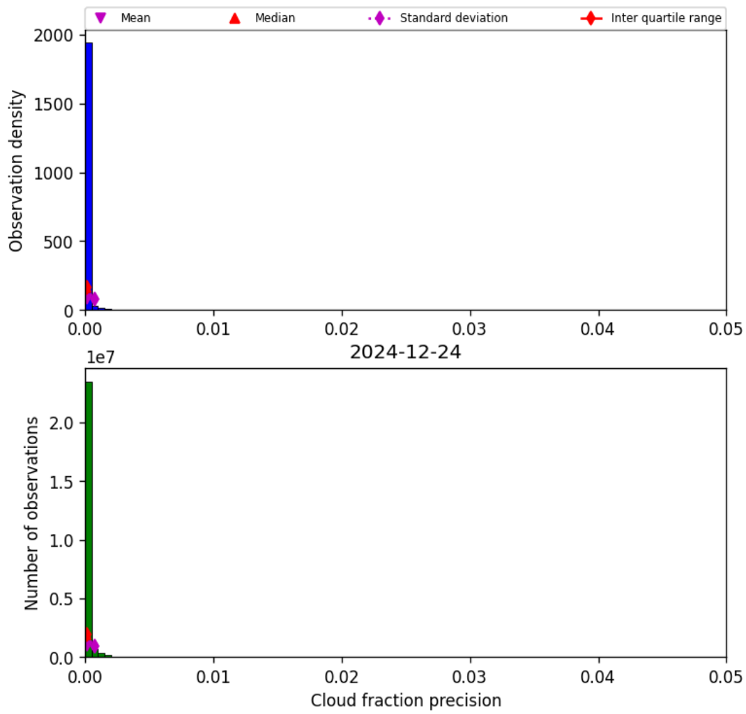
Figure 33: Histogram of “Cloud fraction precision” for 2024-12-23 to 2024-12-25
