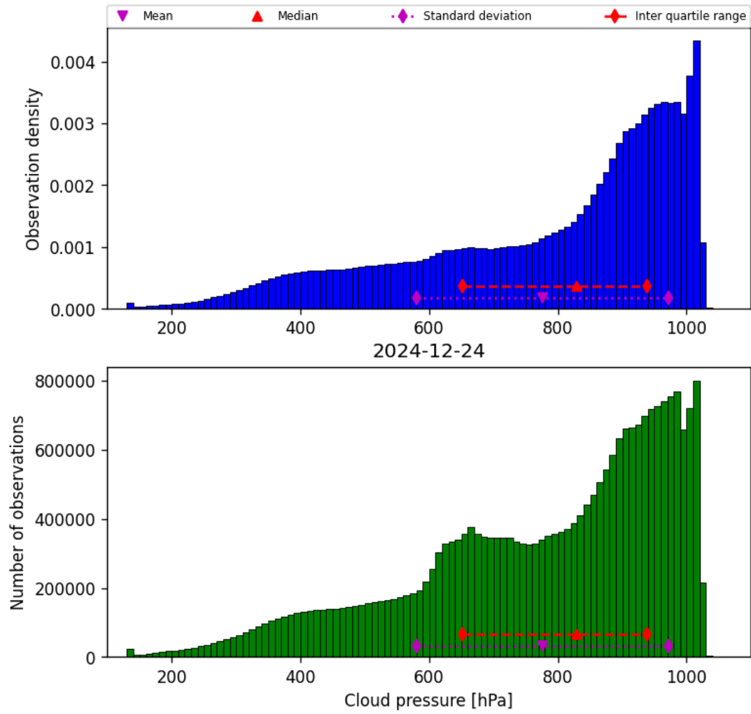
Figure 30: Histogram of “Cloud pressure” for 2024-12-23 to 2024-12-25
