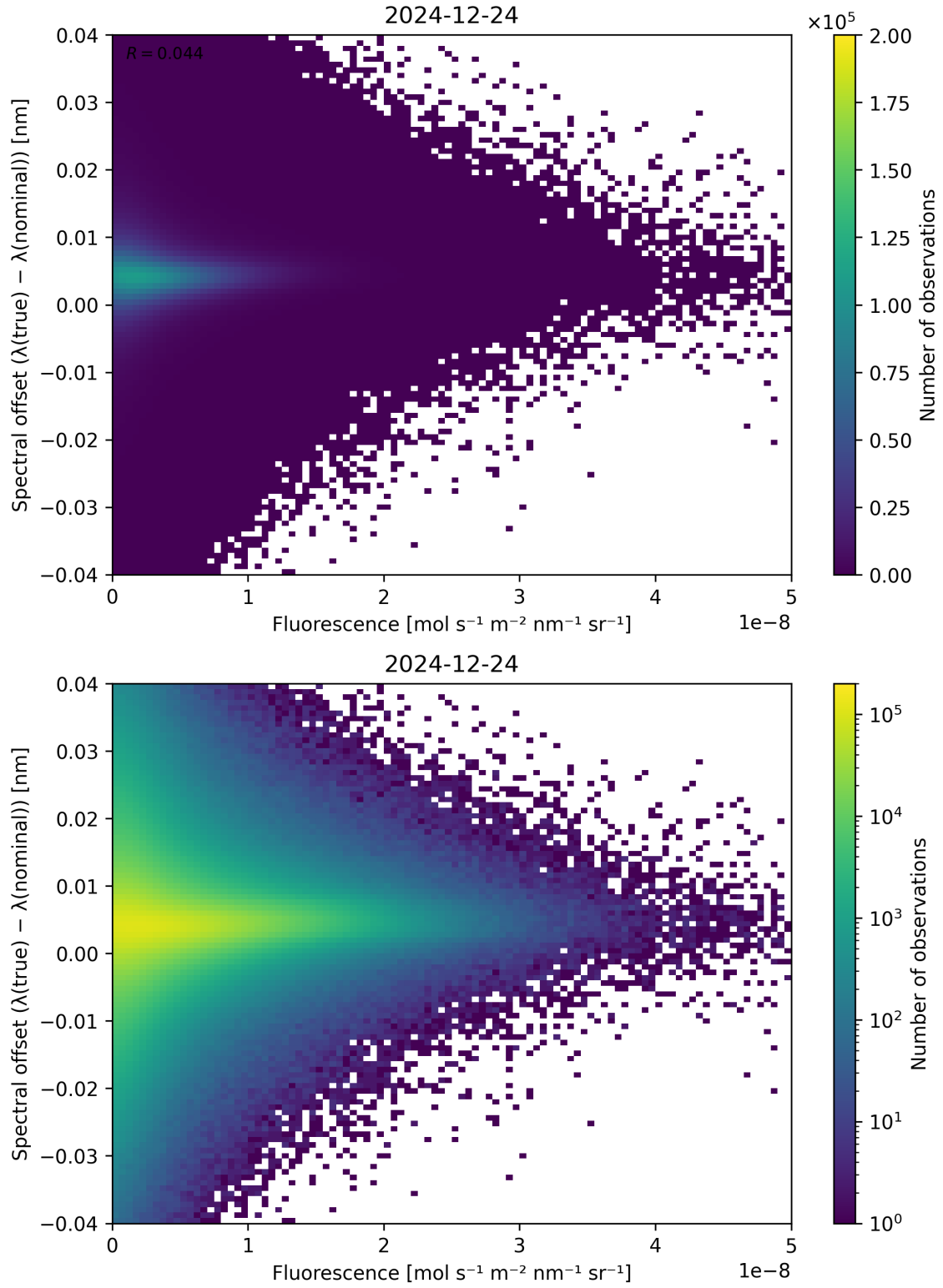
Figure 87: Scatter density plot of “Fluorescence” against “Spectral offset ( \lambda_{\text{true}} - \lambda_{\text{nominal}} )” for 2024-12-23 to 2024-12-25.
