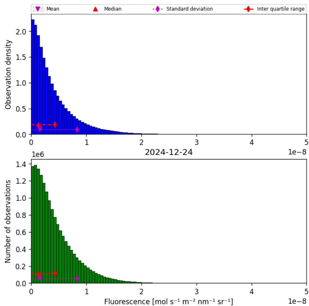
Figure 40: Histogram of “Fluorescence” for 2024-12-23 to 2024-12-25
