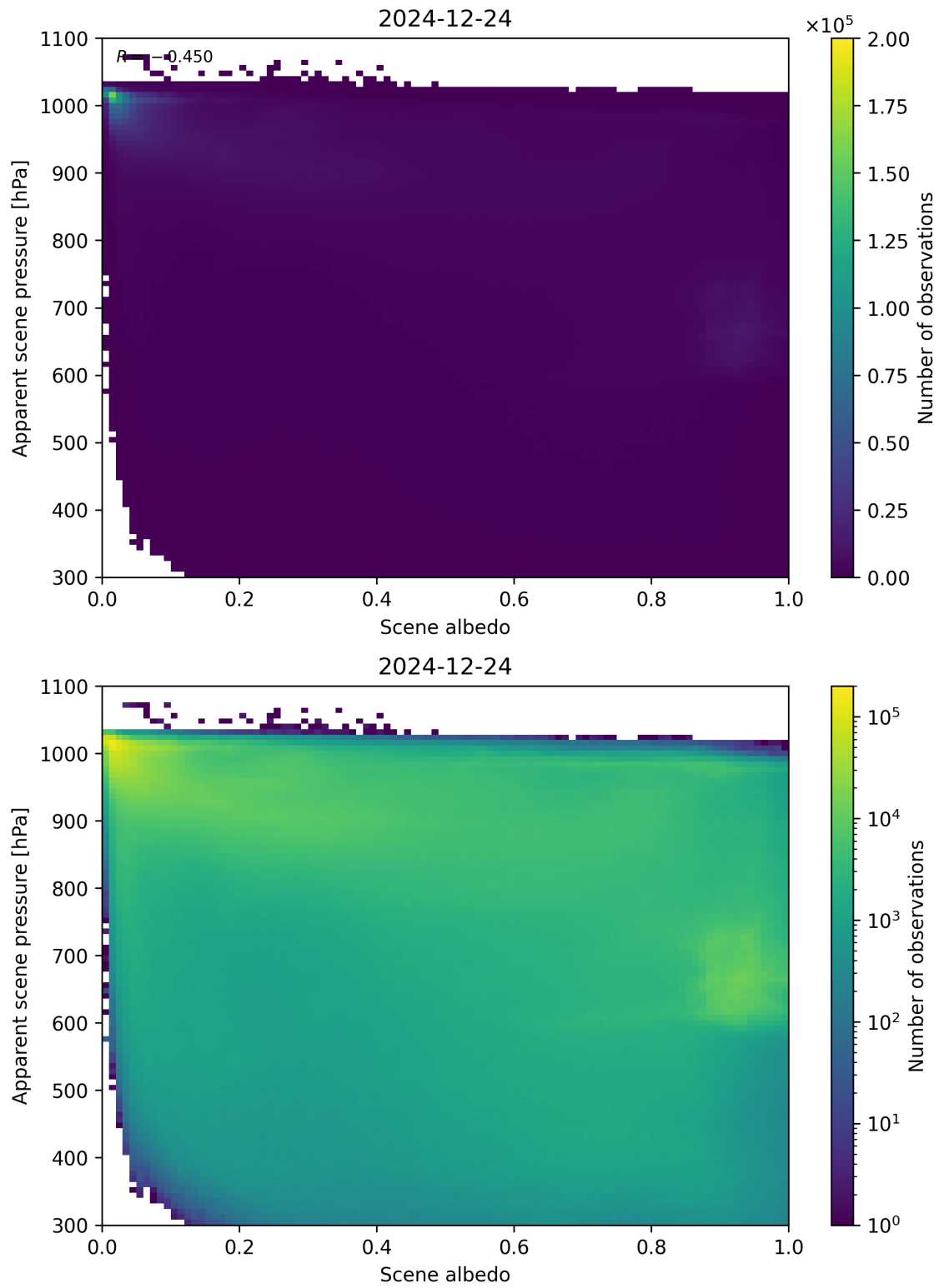
Figure 102: Scatter density plot of “Scene albedo” against “Apparent scene pressure” for 2024-12-23 to 2024-12-25.
