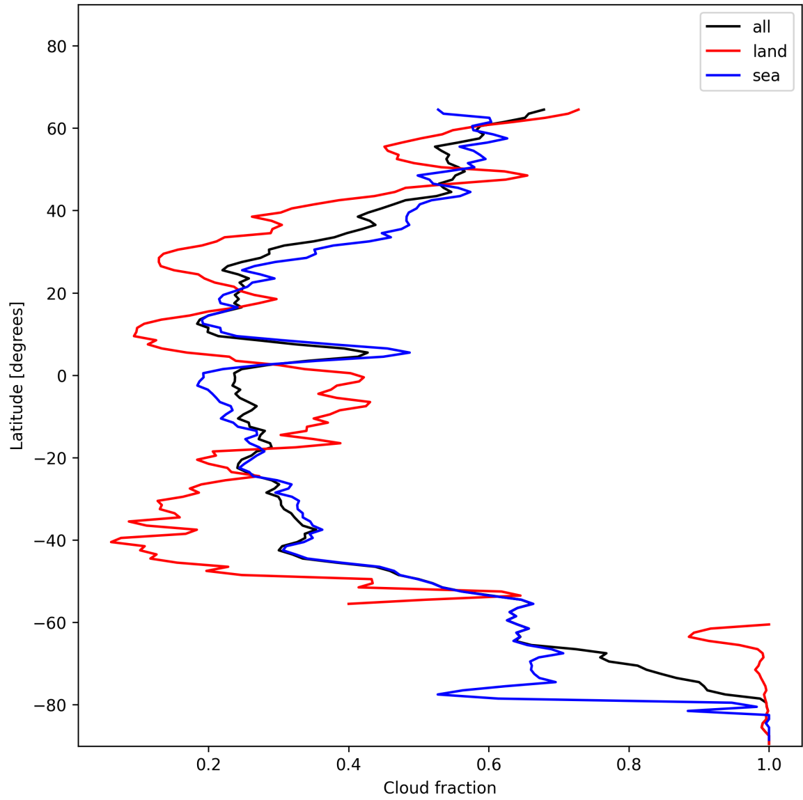
Figure 15: Zonal average of “Cloud fraction” for 2024-12-23 to 2024-12-25.
