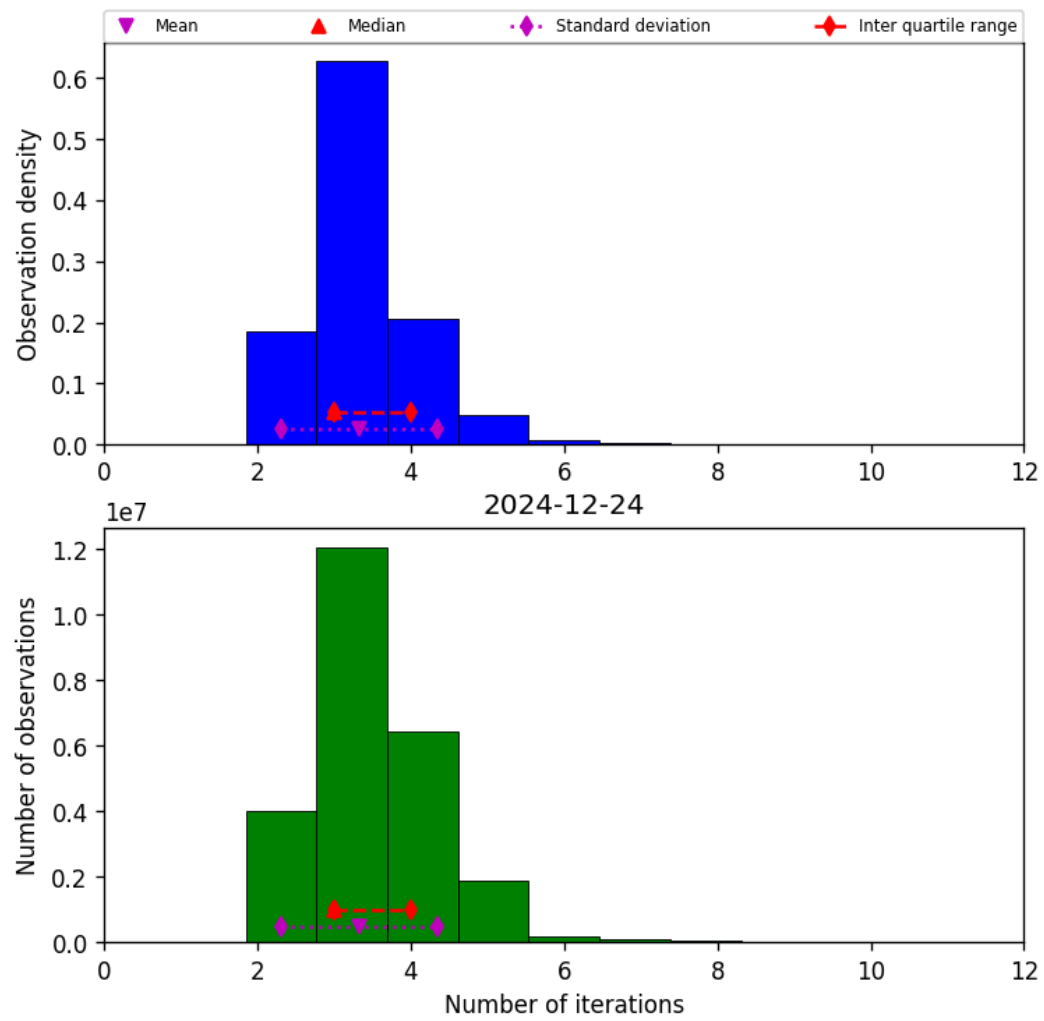
Figure 39: Histogram of “Number of iterations” for 2024-12-23 to 2024-12-25
