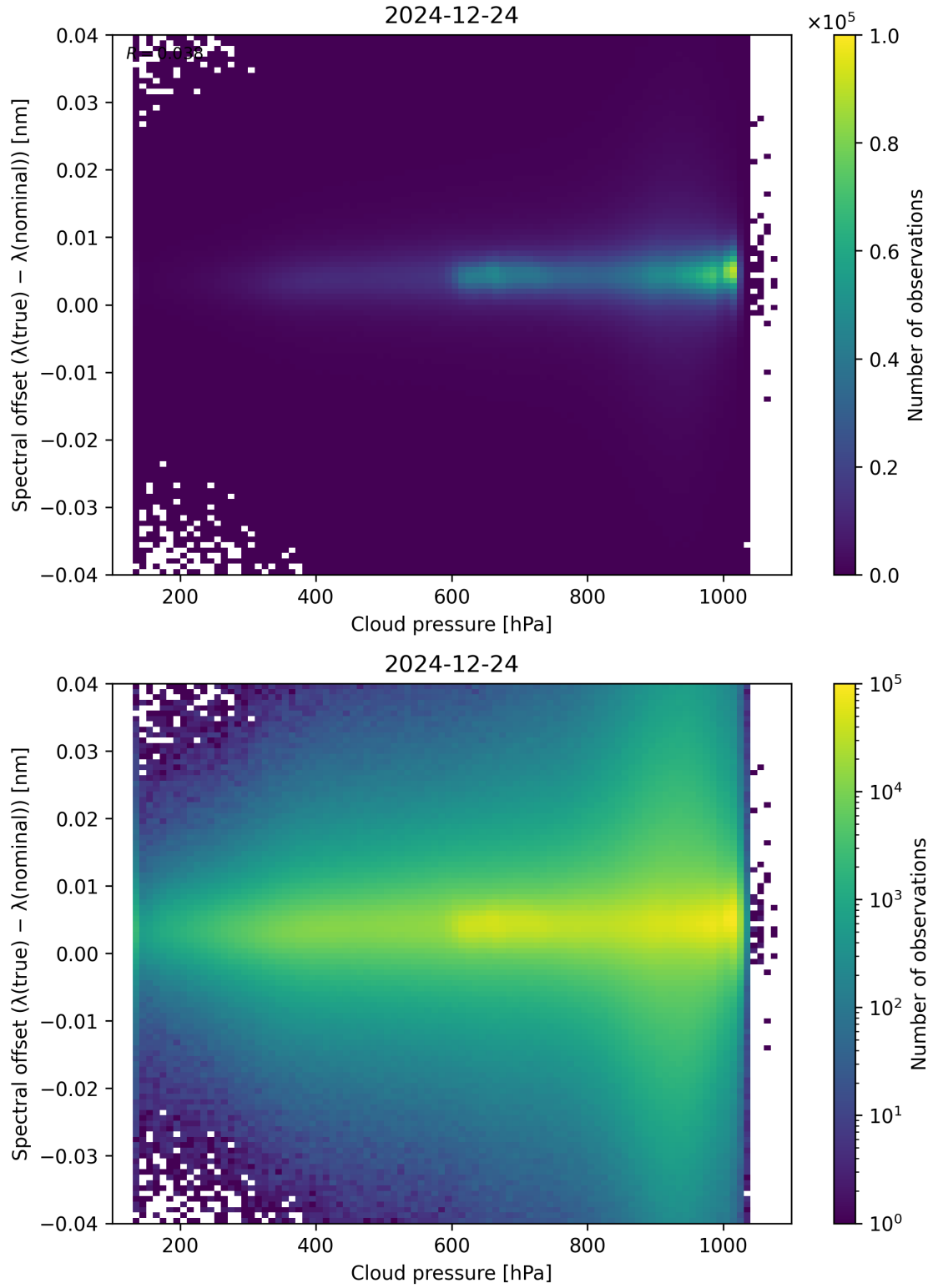
Figure 84: Scatter density plot of “Cloud pressure” against “Spectral offset ( \lambda_{\text{true}} - \lambda_{\text{nominal}} )” for 2024-12-23 to 2024-12-25.
