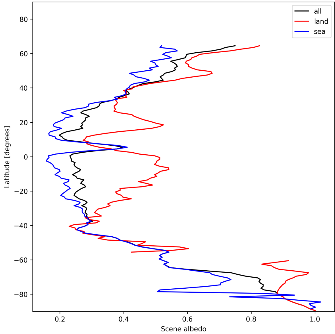
Figure 17: Zonal average of “Scene albedo” for 2024-12-23 to 2024-12-25.
