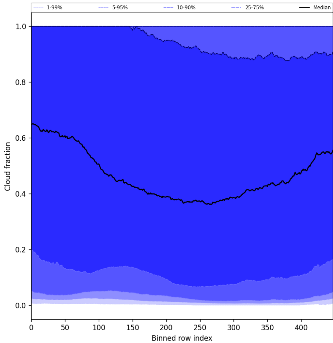
Figure 49: Along track statistics of “Cloud fraction” for 2024-12-23 to 2024-12-25
