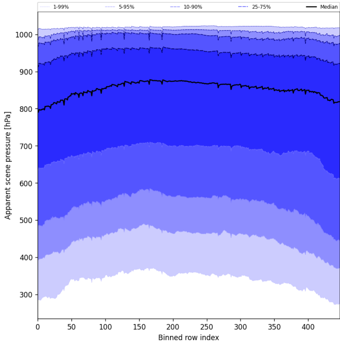
Figure 53: Along track statistics of “Apparent scene pressure” for 2024-12-23 to 2024-12-25
