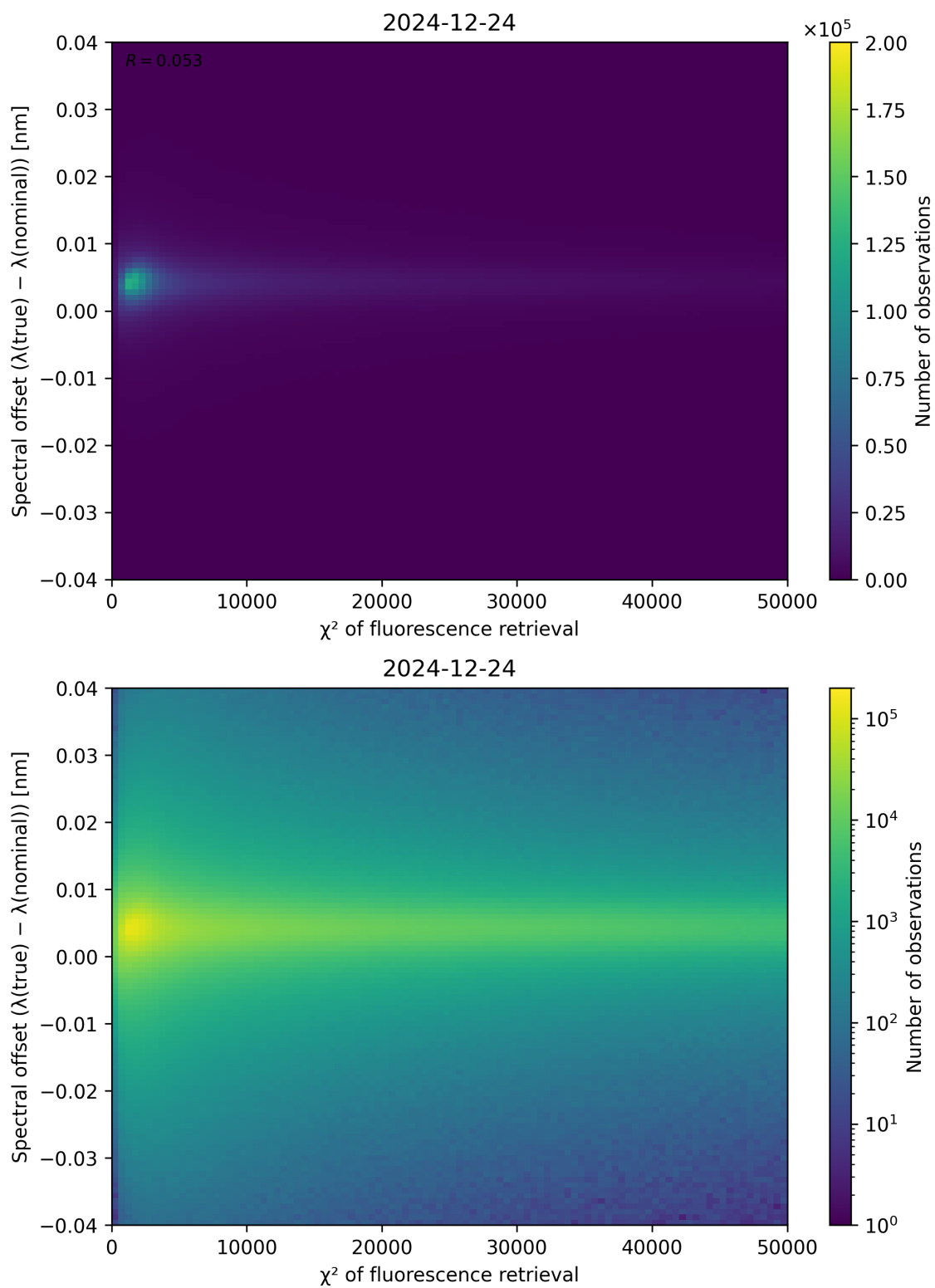
Figure 69: Scatter density plot of “ \chi^2 of fluorescence retrieval” against “Spectral offset ( \lambda_{\text{true}} - \lambda_{\text{nominal}} )” for 2024-12-23 to 2024-12-25.
