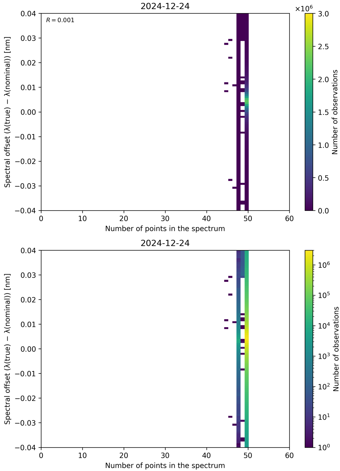
Figure 101: Scatter density plot of “Number of points in the spectrum” against “Spectral offset ( \lambda_{\text{true}} - \lambda_{\text{nominal}} )” for 2024-12-23 to 2024-12-25.
