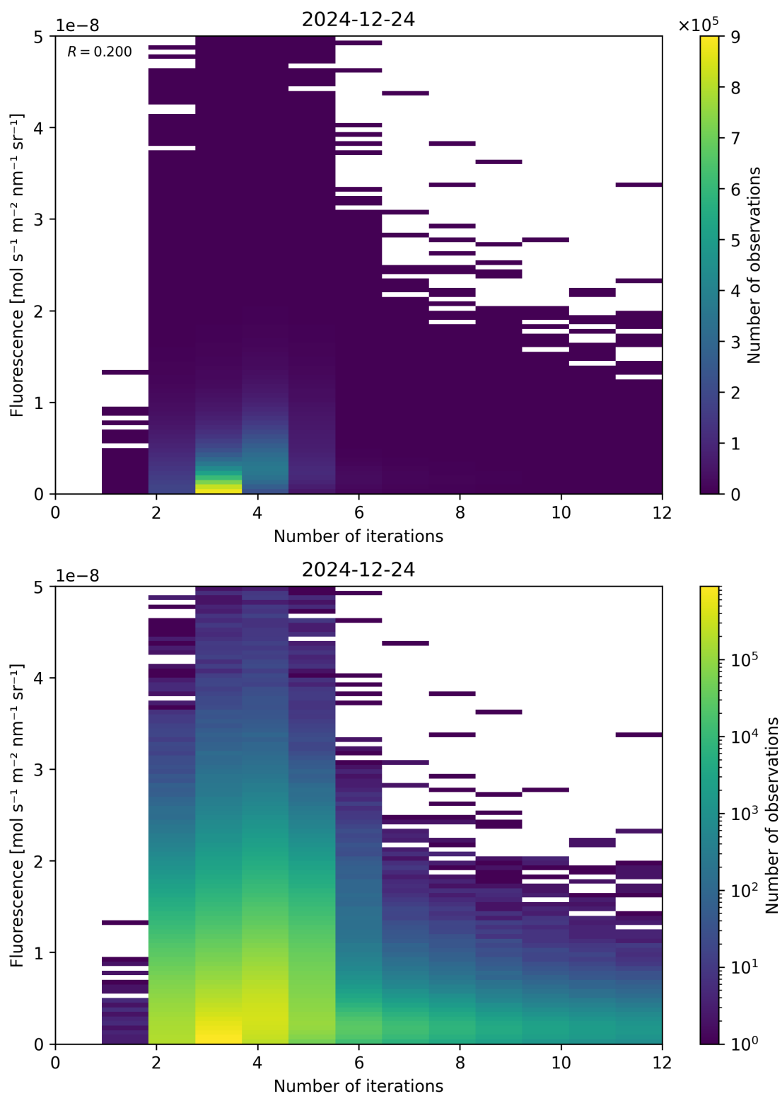
Figure 98: Scatter density plot of “Number of iterations” against “Fluorescence” for 2024-12-23 to 2024-12-25.
