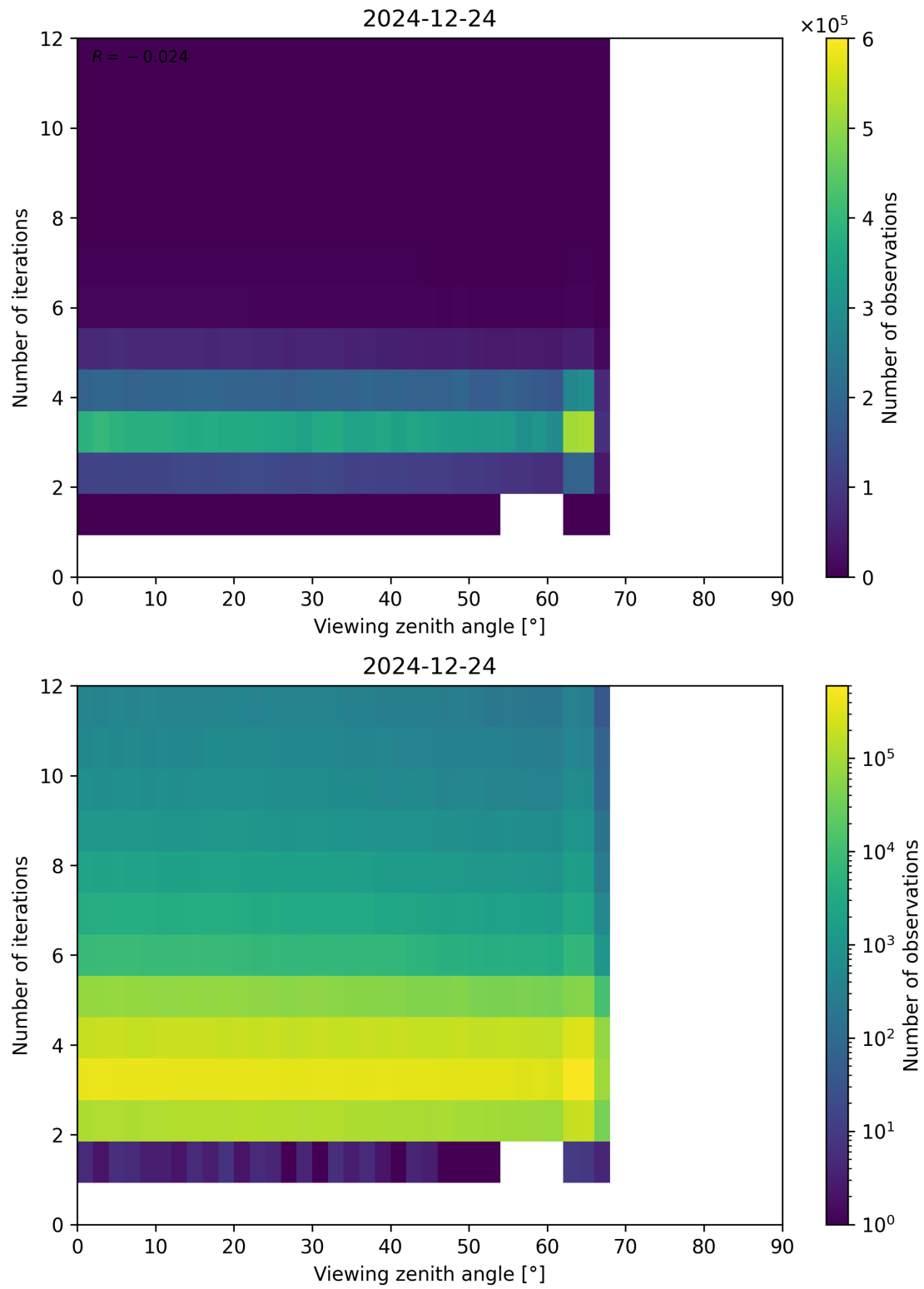
Figure 124: Scatter density plot of “Viewing zenith angle” against “Number of iterations” for 2024-12-23 to 2024-12-25.
