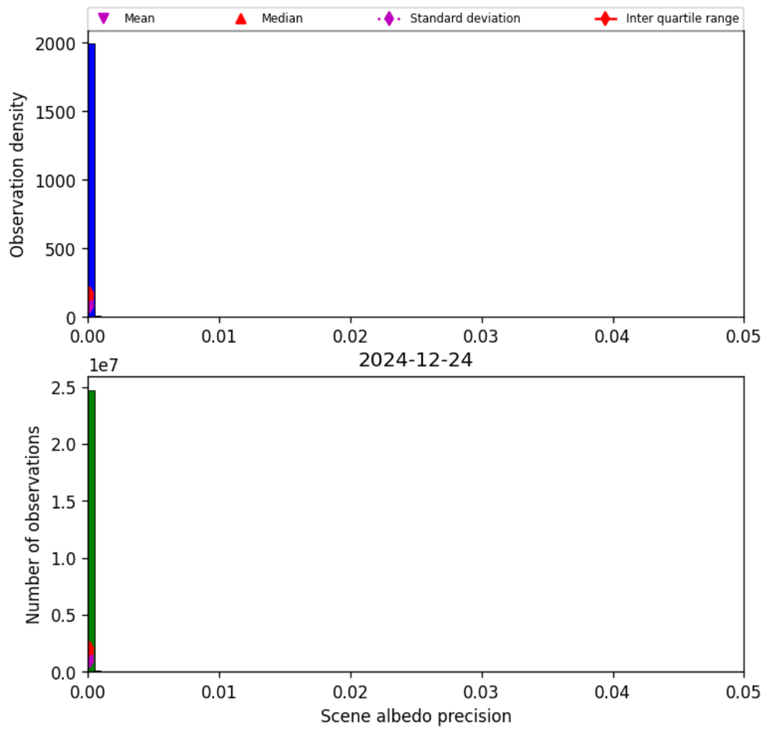
Figure 35: Histogram of “Scene albedo precision” for 2024-12-23 to 2024-12-25
