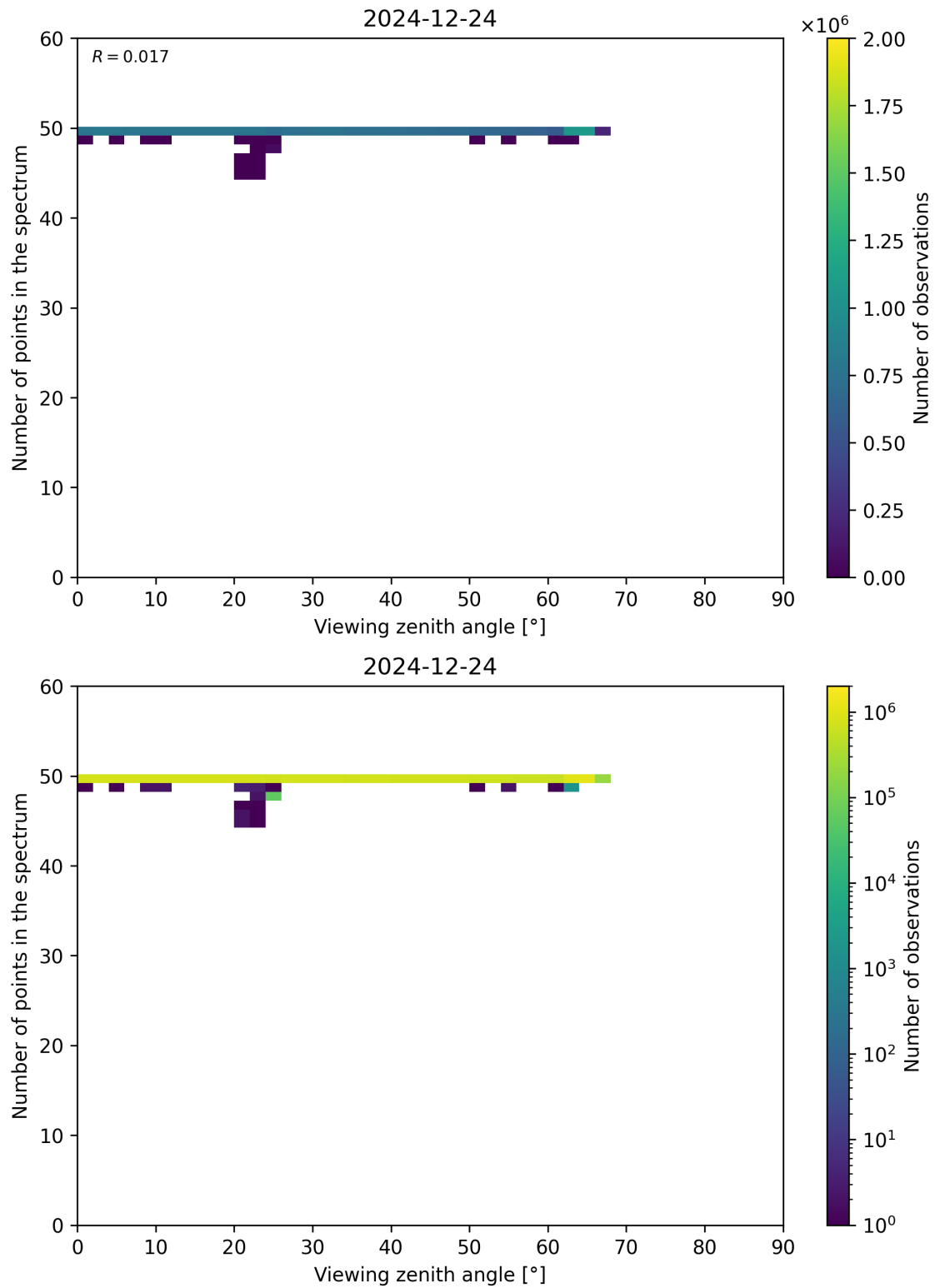
Figure 125: Scatter density plot of “Viewing zenith angle” against “Number of points in the spectrum” for 2024-12-23 to 2024-12-25.
