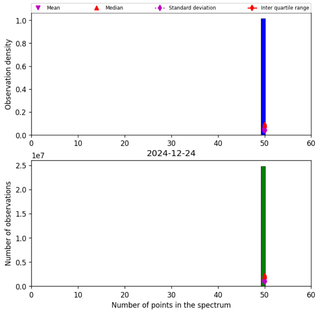
Figure 44: Histogram of “Number of points in the spectrum” for 2024-12-23 to 2024-12-25
