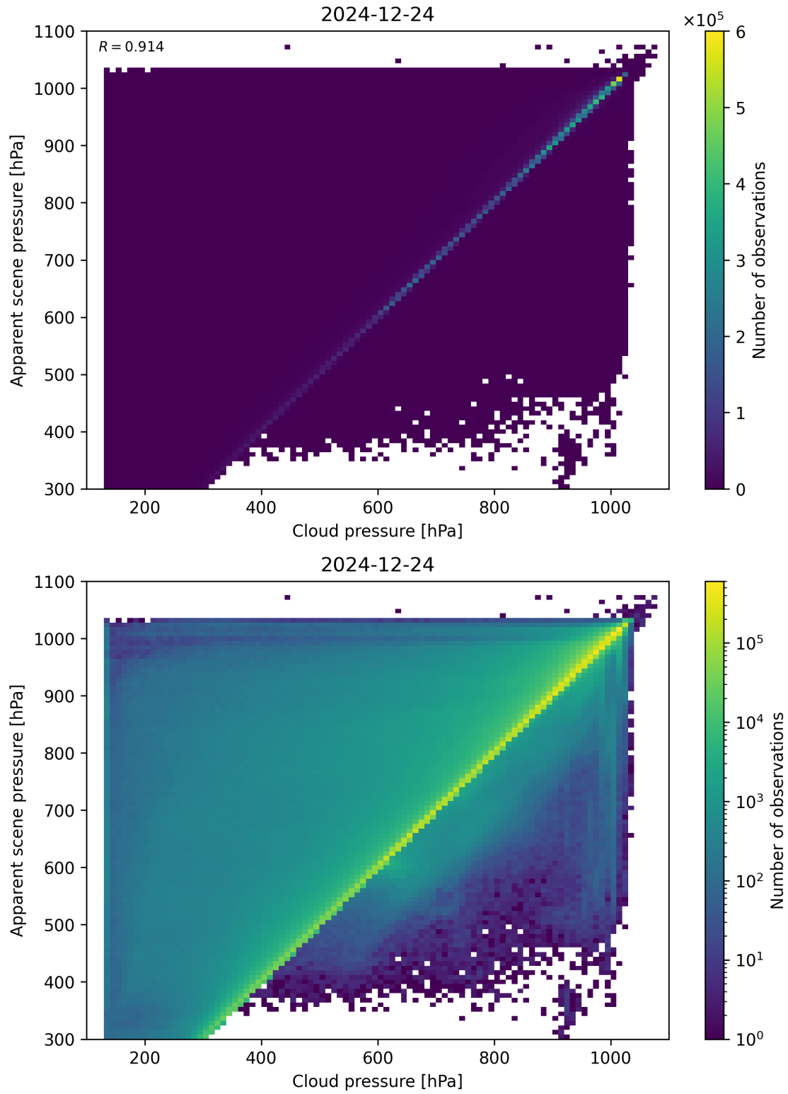
Figure 77: Scatter density plot of “Cloud pressure” against “Apparent scene pressure” for 2024-12-23 to 2024-12-25.
