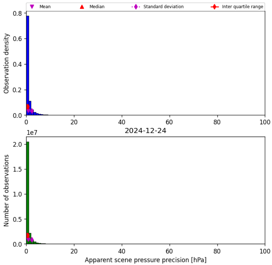
Figure 37: Histogram of “Apparent scene pressure precision” for 2024-12-23 to 2024-12-25
