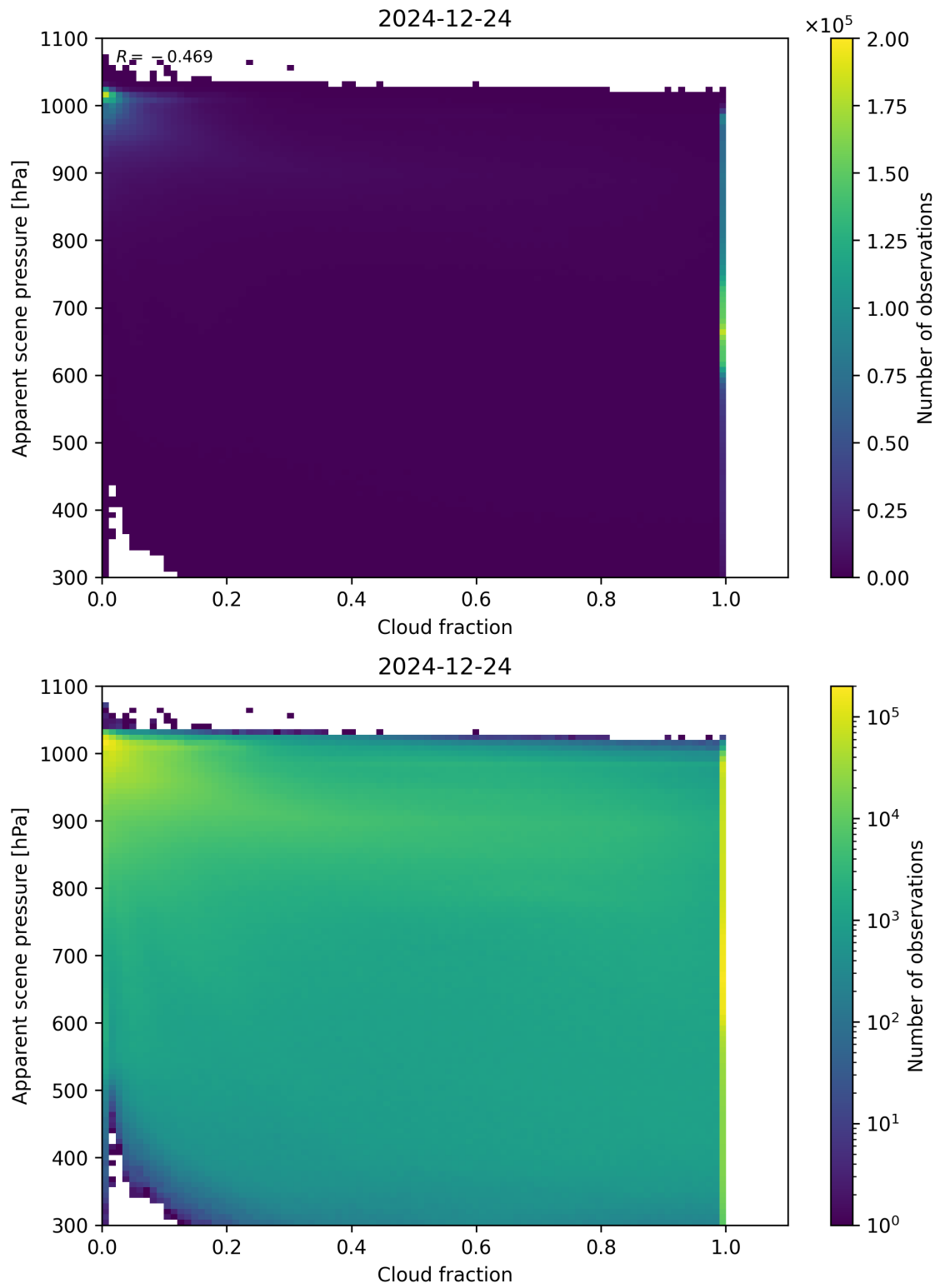
Figure 70: Scatter density plot of “Cloud fraction” against “Apparent scene pressure” for 2024-12-23 to 2024-12-25.
