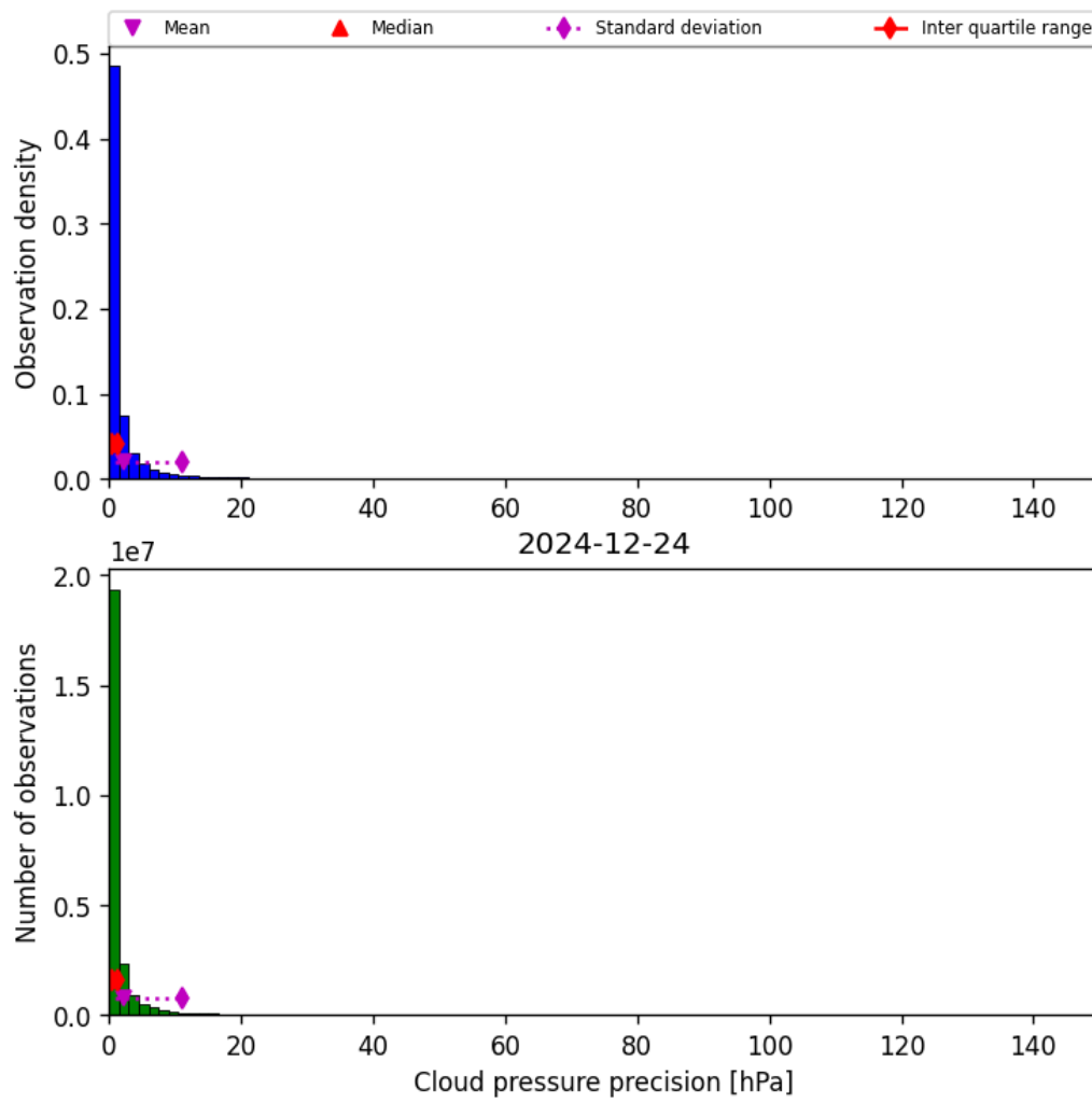
Figure 31: Histogram of “Cloud pressure precision” for 2024-12-23 to 2024-12-25
