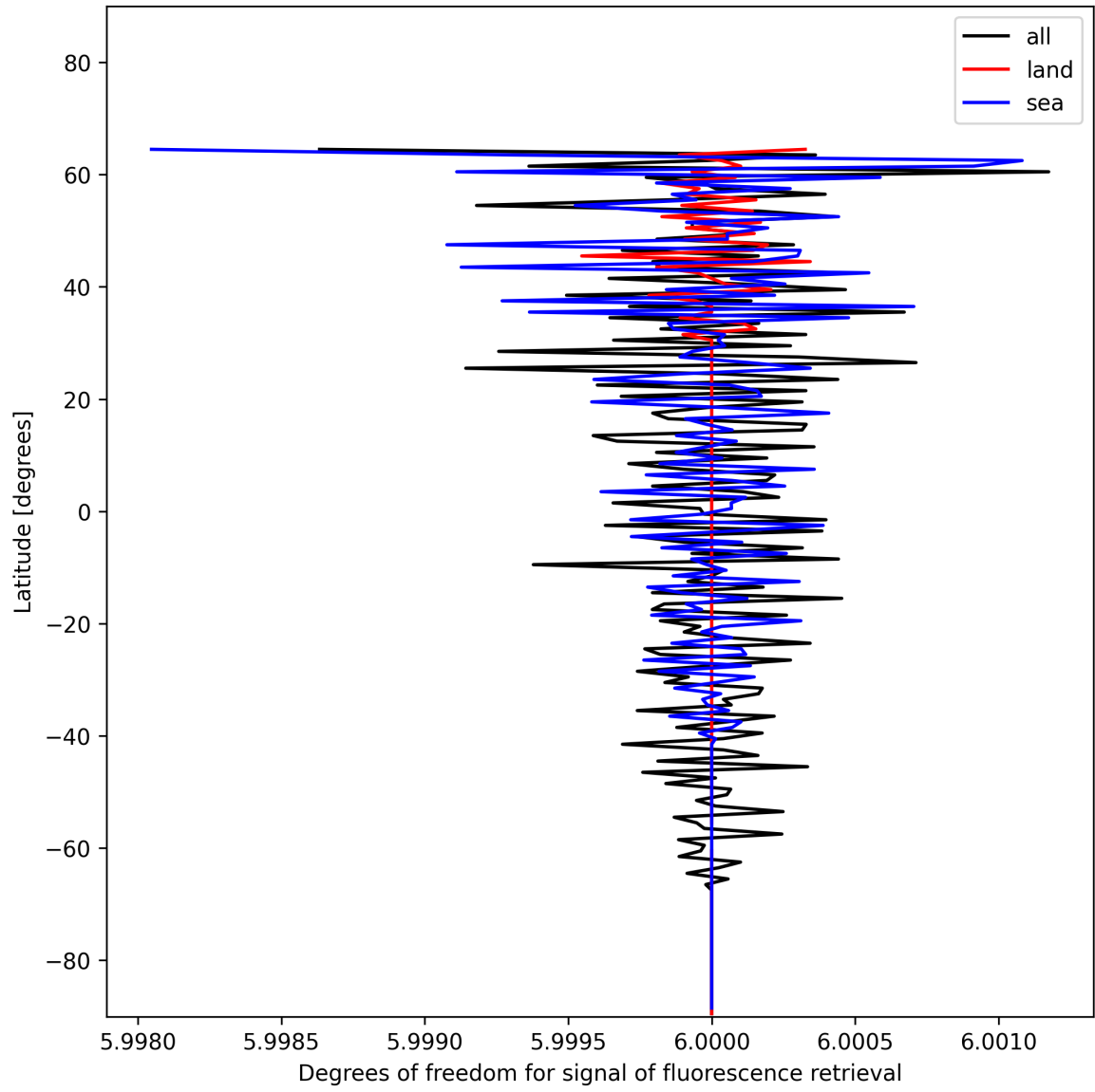
Figure 26: Zonal average of “Degrees of freedom for signal of fluorescence retrieval” for 2024-12-23 to 2024-12-25.
