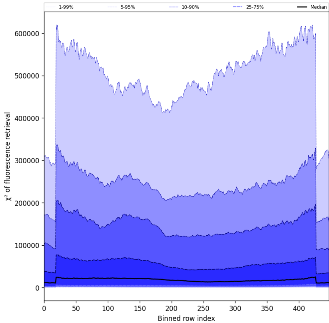
Figure 59: Along track statistics of “ \chi^2 of fluorescence retrieval” for 2024-12-23 to 2024-12-25
