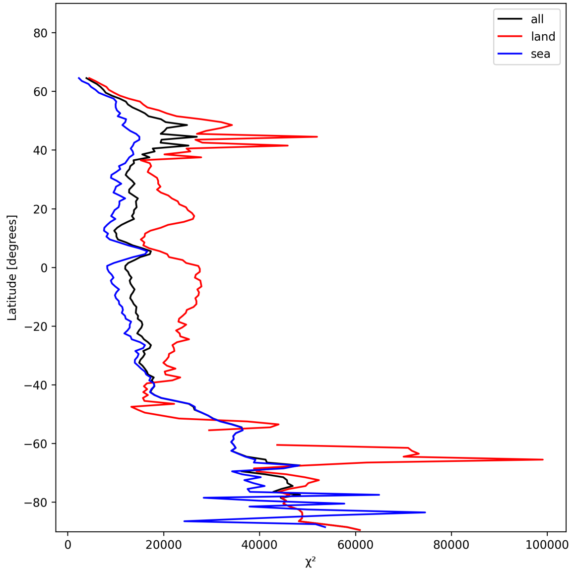
Figure 21: Zonal average of “ \chi^2 ” for 2024-12-23 to 2024-12-25.
