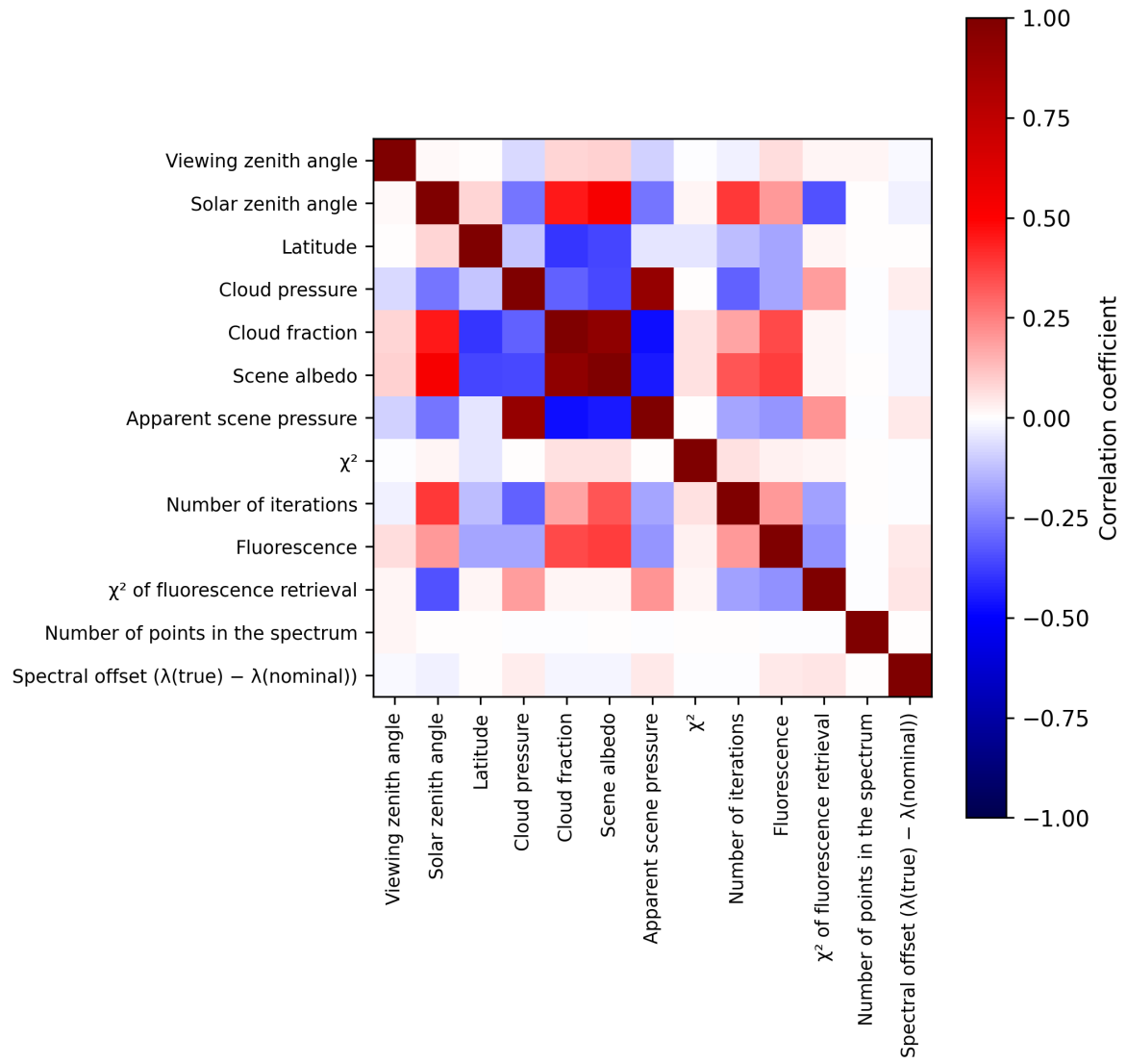
Figure 2: Map of correlation matrix for 2024-12-23 to 2024-12-25.
