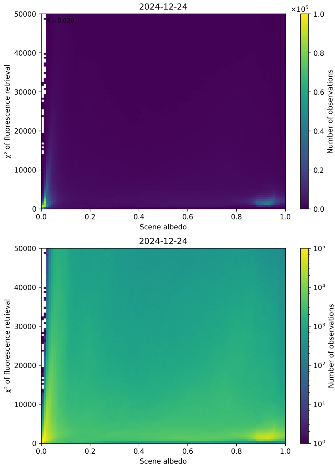
Figure 103: Scatter density plot of “Scene albedo” against “ \chi^2 of fluorescence retrieval” for 2024-12-23 to 2024-12-25.
