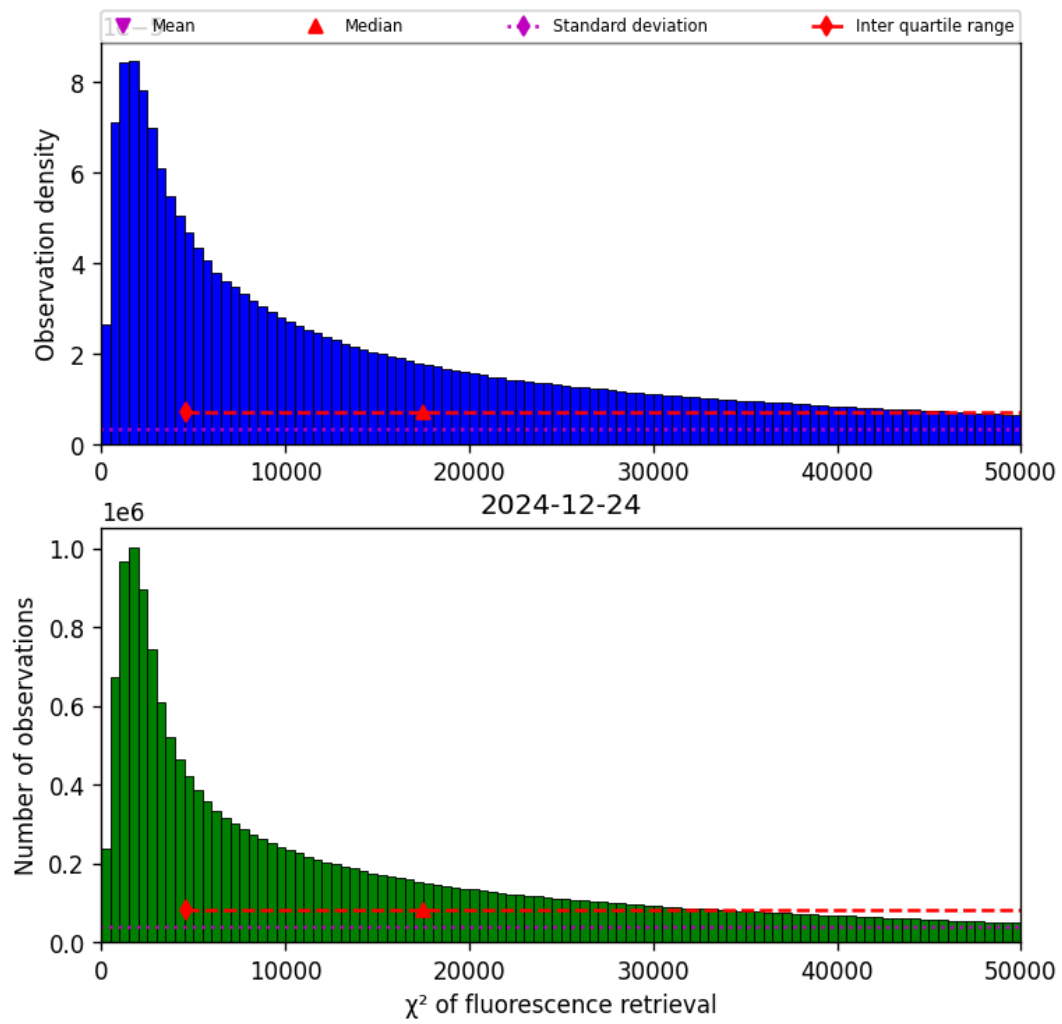
Figure 42: Histogram of “ \chi^2 of fluorescence retrieval” for 2024-12-23 to 2024-12-25
