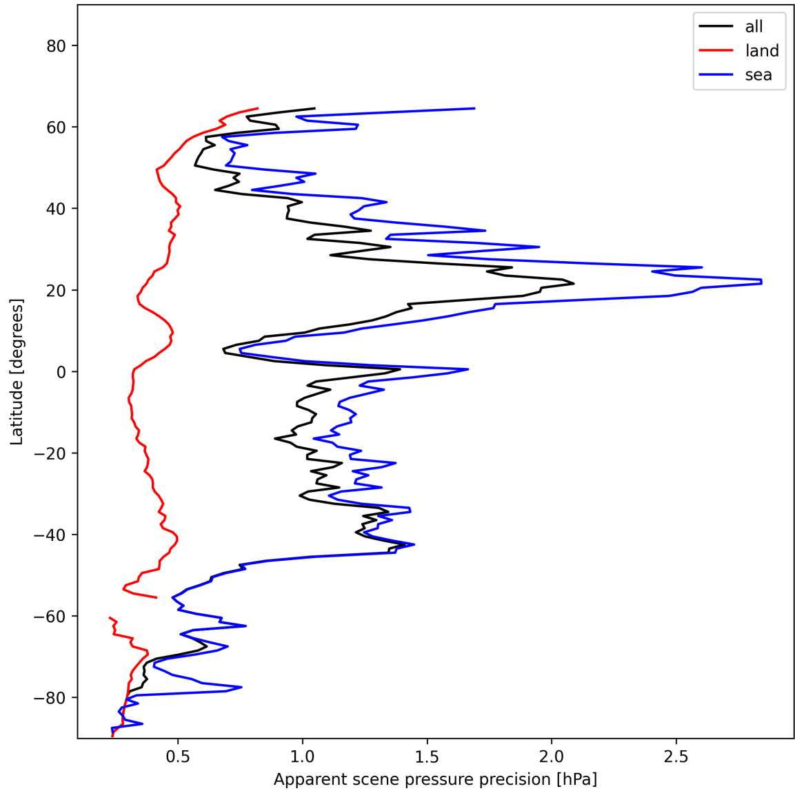
Figure 20: Zonal average of “Apparent scene pressure precision” for 2024-12-23 to 2024-12-25.
