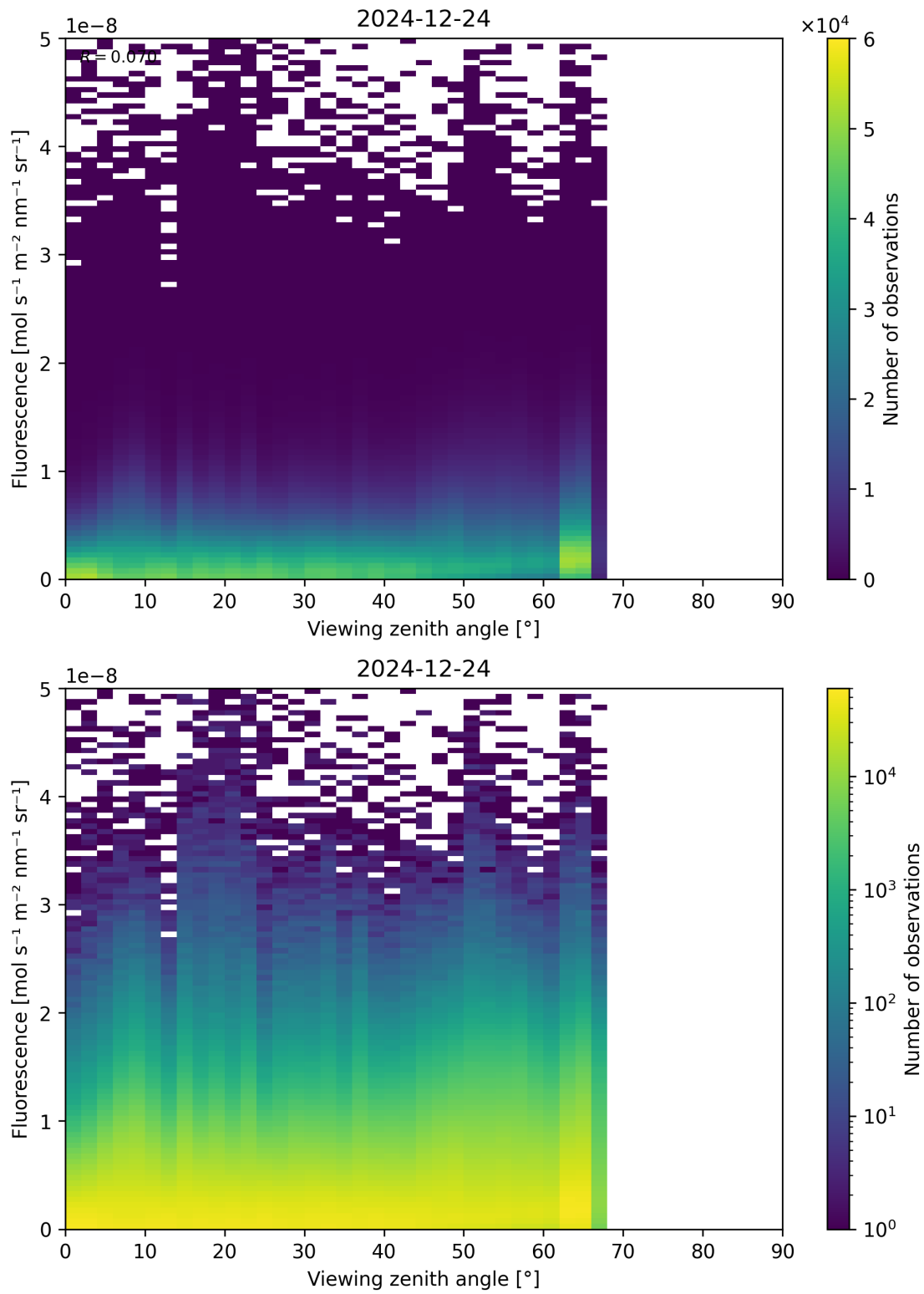
Figure 122: Scatter density plot of “Viewing zenith angle” against “Fluorescence” for 2024-12-23 to 2024-12-25.
