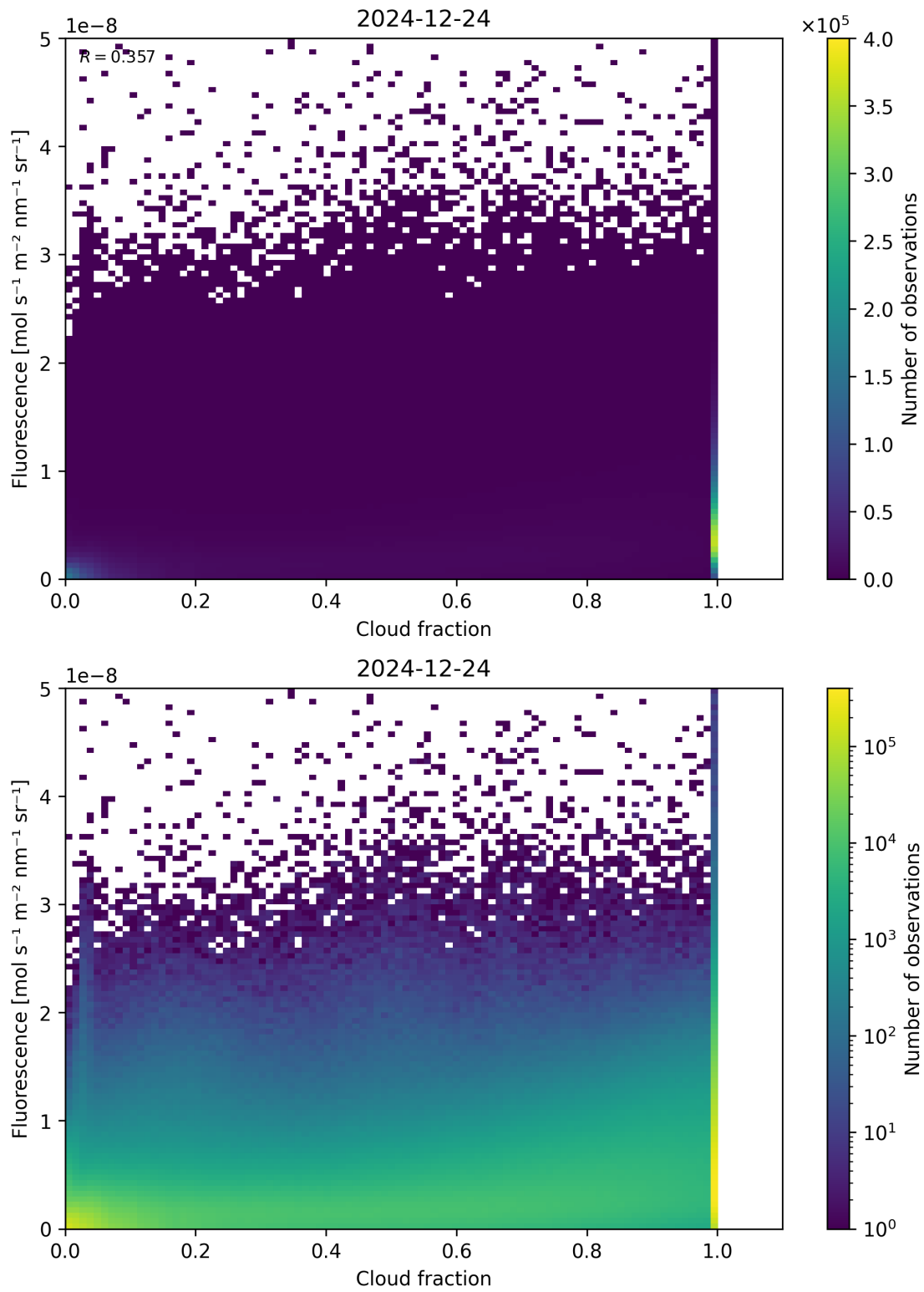
Figure 72: Scatter density plot of “Cloud fraction” against “Fluorescence” for 2024-12-23 to 2024-12-25.
