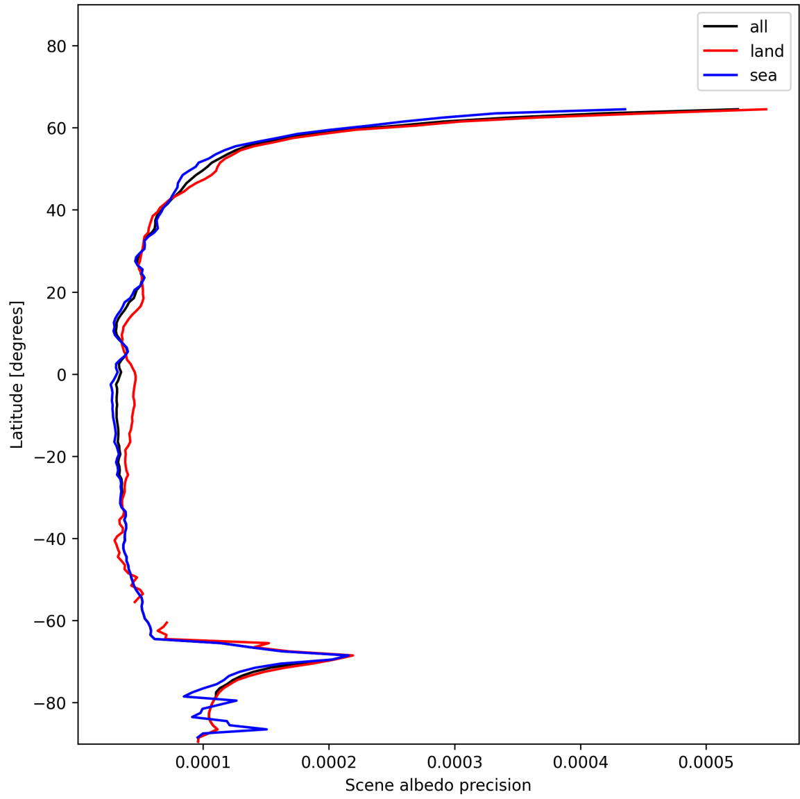
Figure 18: Zonal average of “Scene albedo precision” for 2024-12-23 to 2024-12-25.
