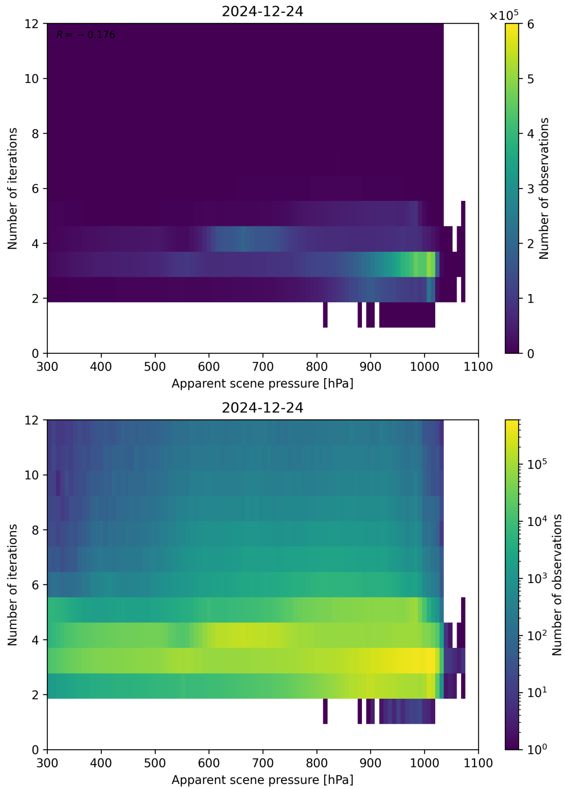
Figure 65: Scatter density plot of “Apparent scene pressure” against “Number of iterations” for 2024-12-23 to 2024-12-25.
