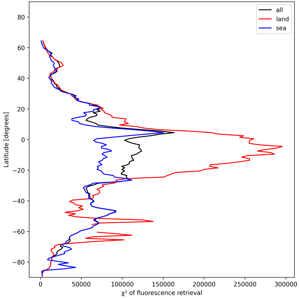
Figure 25: Zonal average of “ \chi^2 of fluorescence retrieval” for 2024-12-23 to 2024-12-25.
