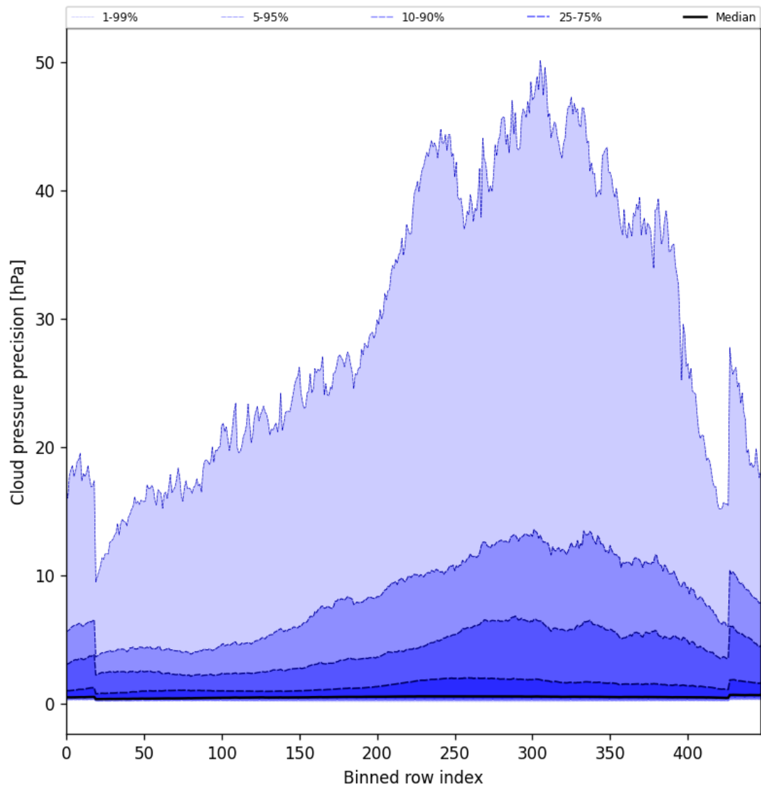
Figure 48: Along track statistics of “Cloud pressure precision” for 2024-12-23 to 2024-12-25
