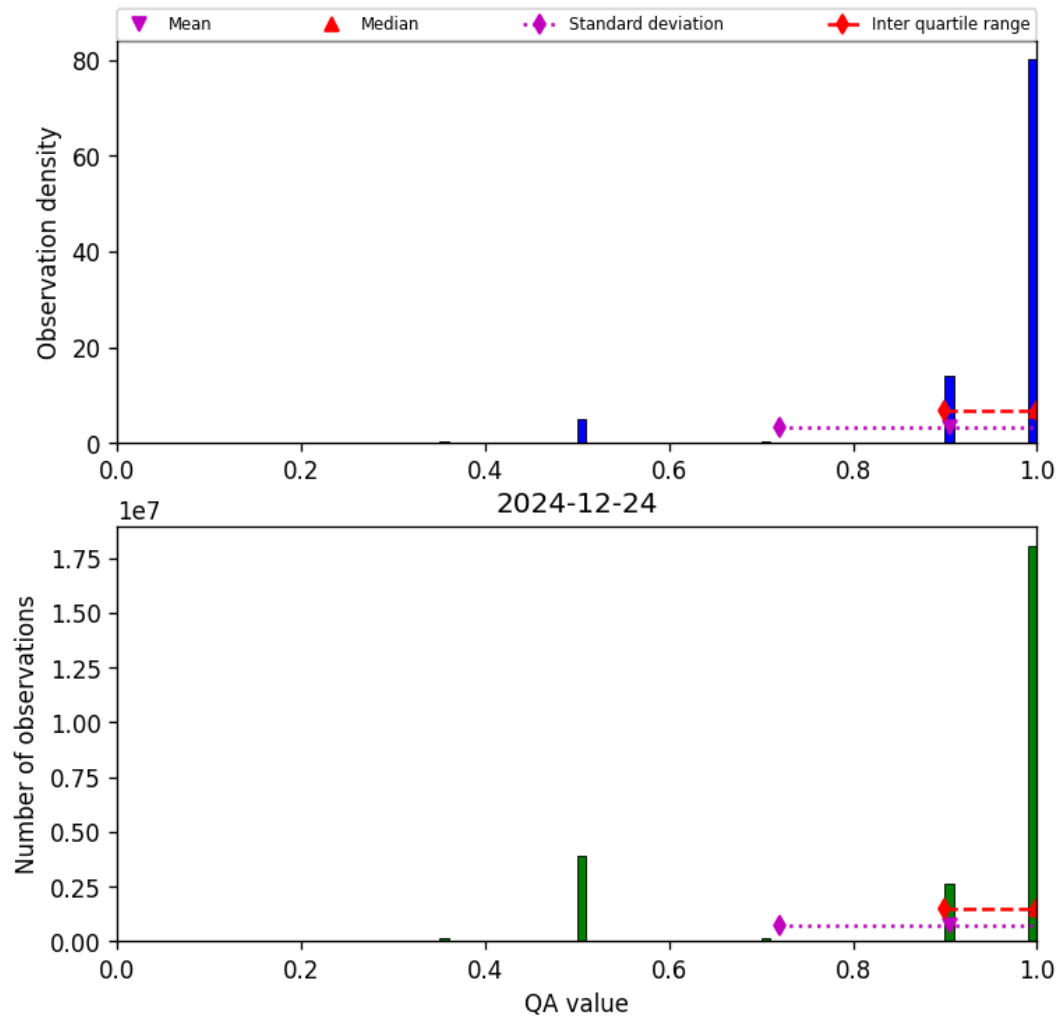
Figure 29: Histogram of “QA value” for 2024-12-23 to 2024-12-25
