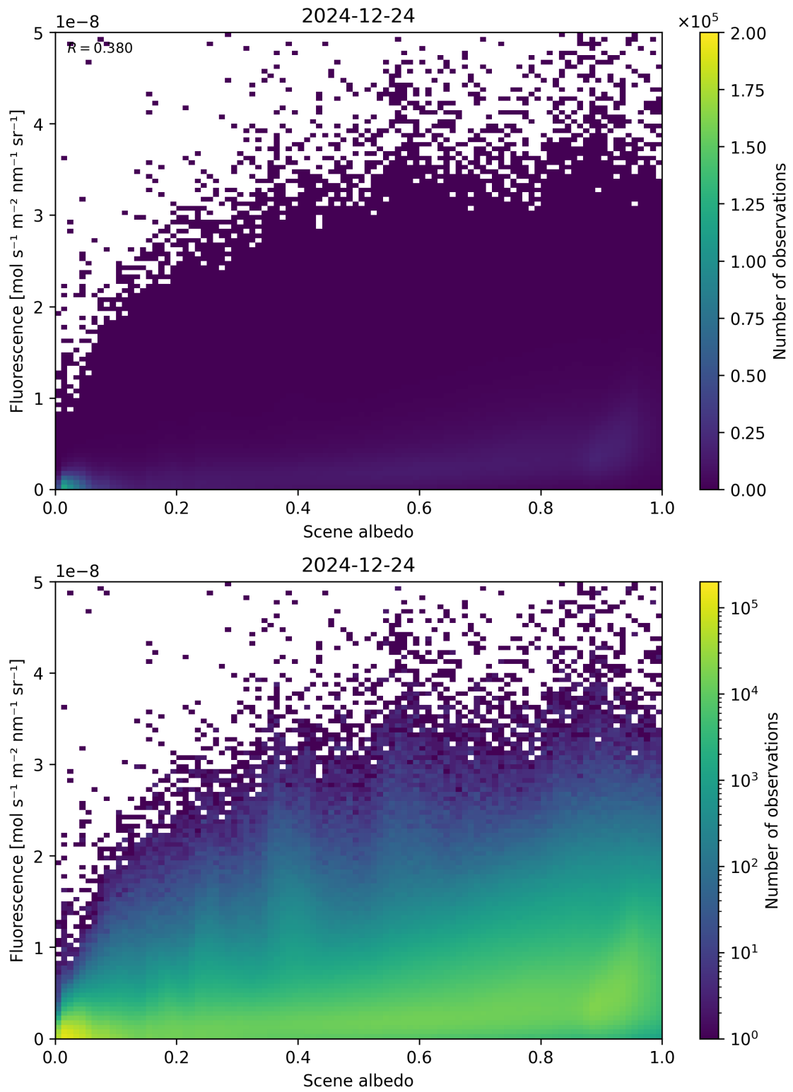
Figure 104: Scatter density plot of “Scene albedo” against “Fluorescence” for 2024-12-23 to 2024-12-25.
