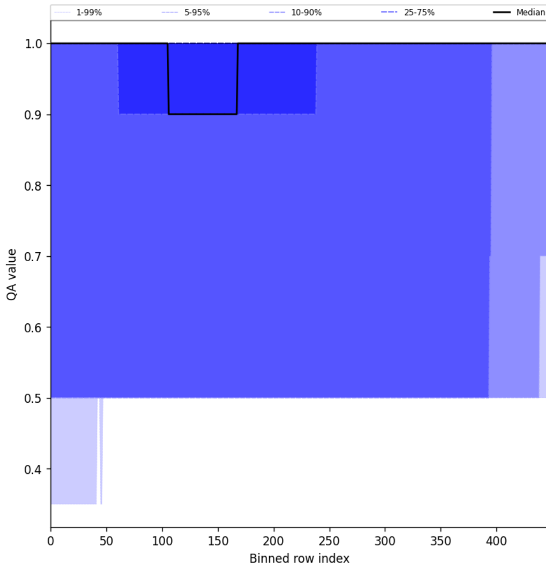
Figure 46: Along track statistics of “QA value” for 2024-12-23 to 2024-12-25
