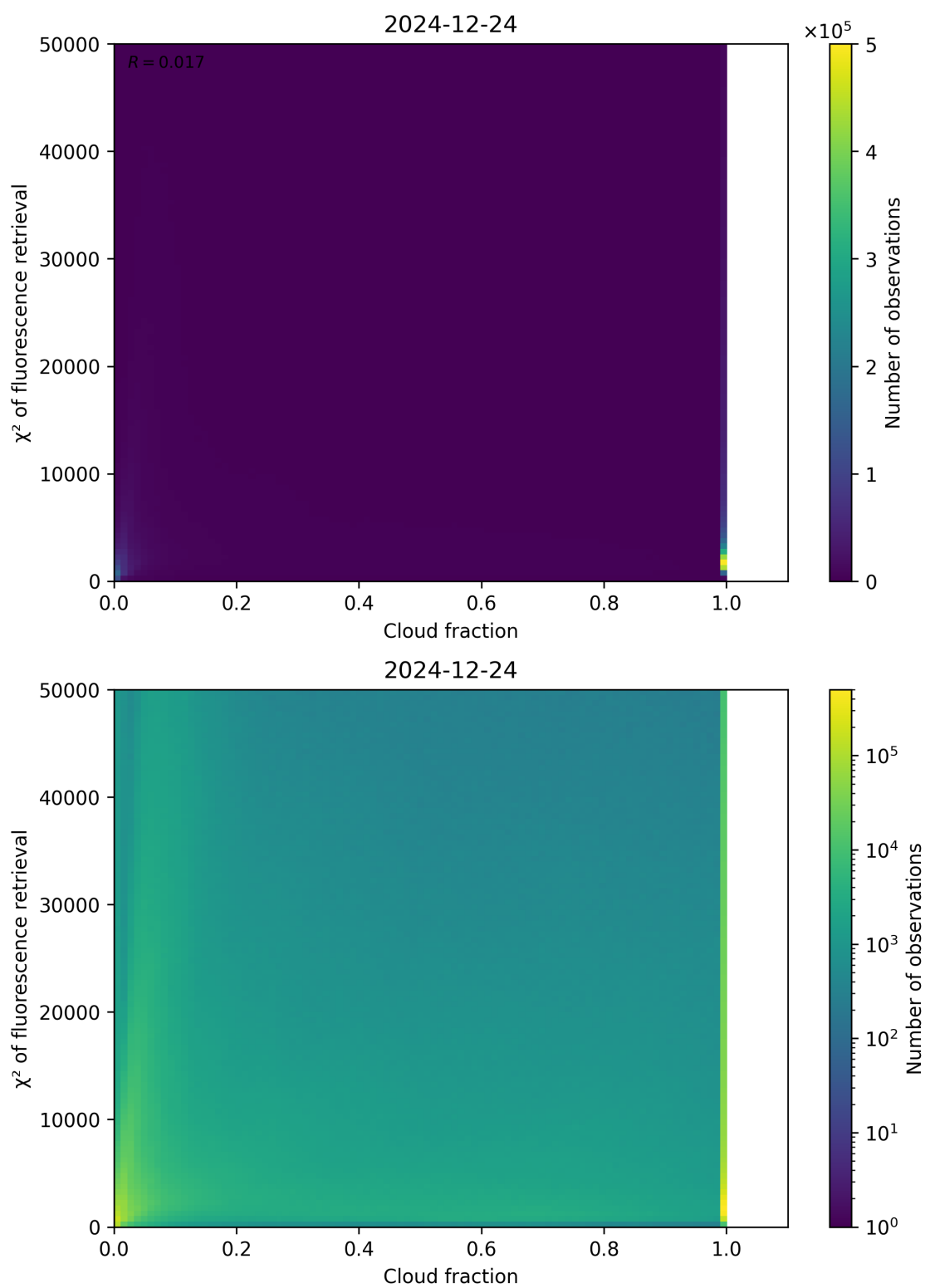
Figure 71: Scatter density plot of “Cloud fraction” against “ \chi^2 of fluorescence retrieval” for 2024-12-23 to 2024-12-25.
