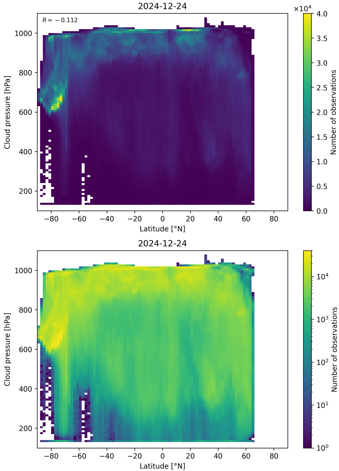
Figure 91: Scatter density plot of “Latitude” against “Cloud pressure” for 2024-12-23 to 2024-12-25.
