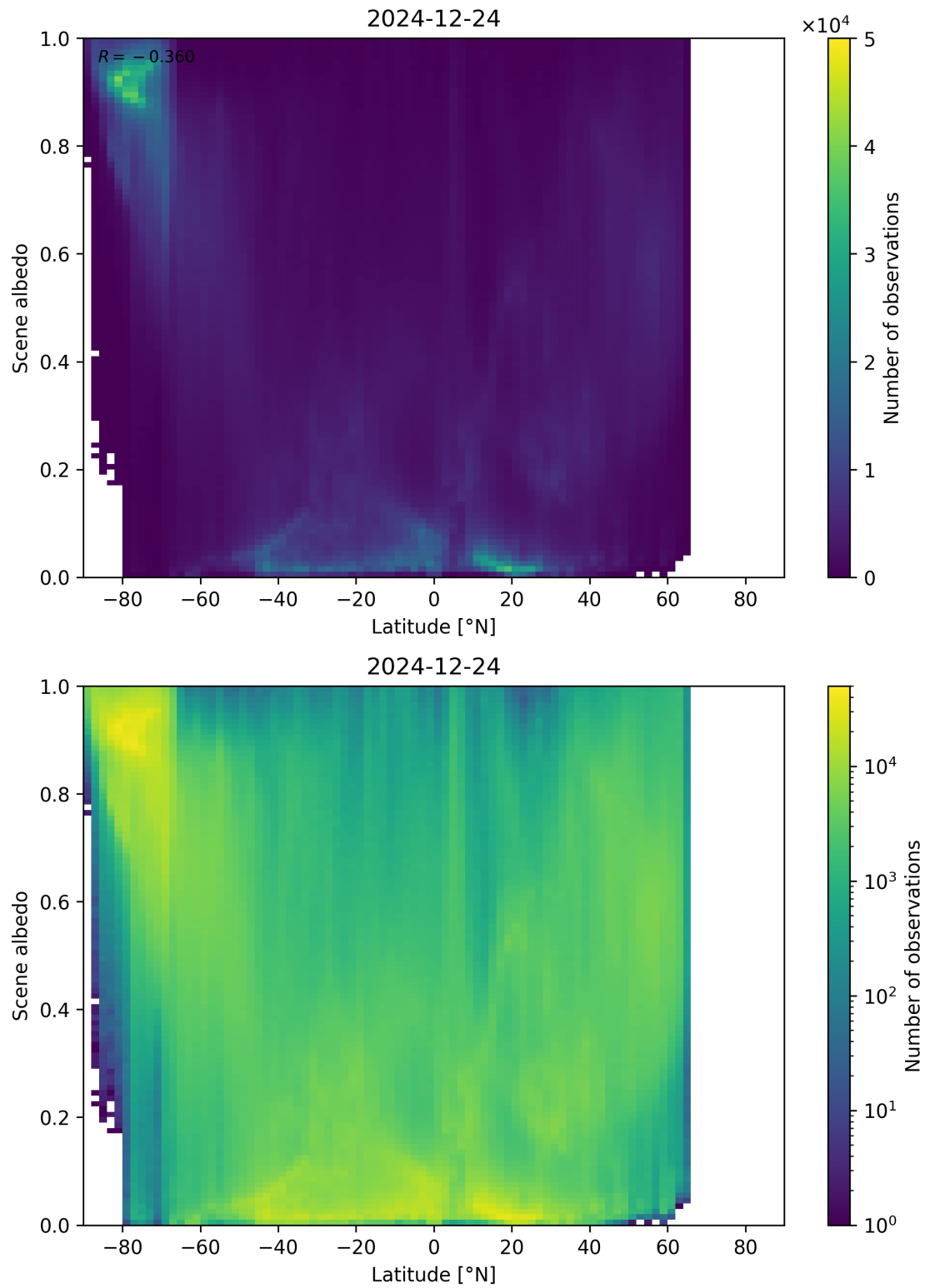
Figure 95: Scatter density plot of “Latitude” against “Scene albedo” for 2024-12-23 to 2024-12-25.
