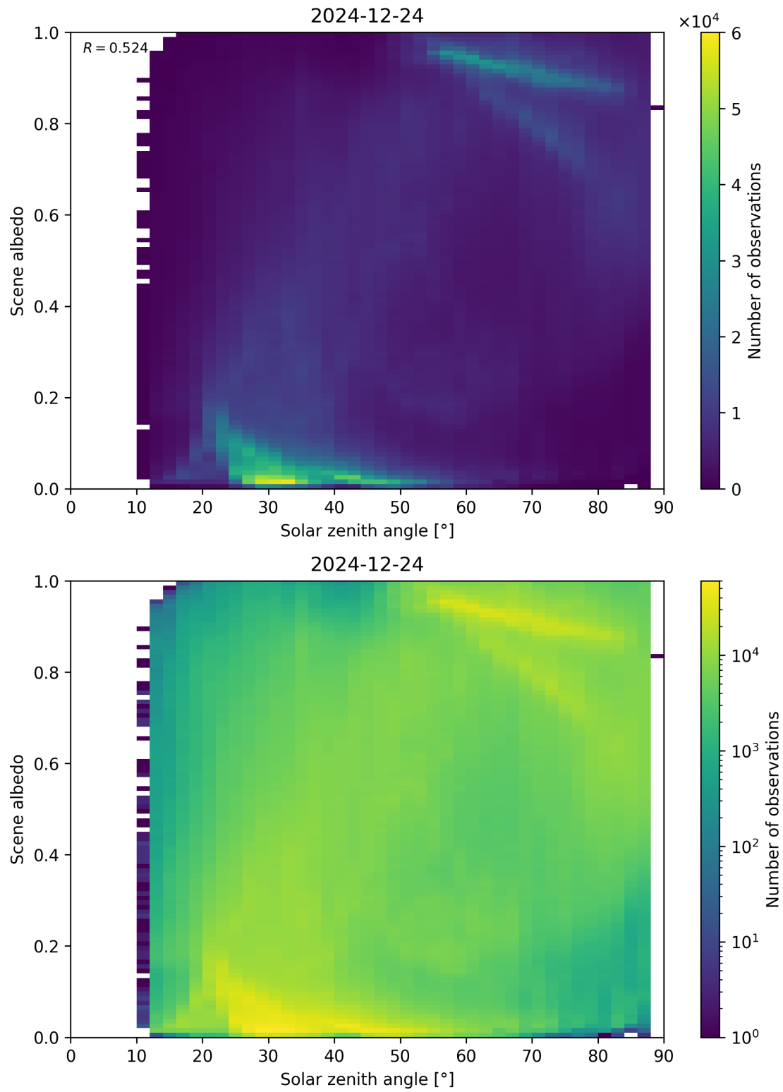
Figure 116: Scatter density plot of “Solar zenith angle” against “Scene albedo” for 2024-12-23 to 2024-12-25.
