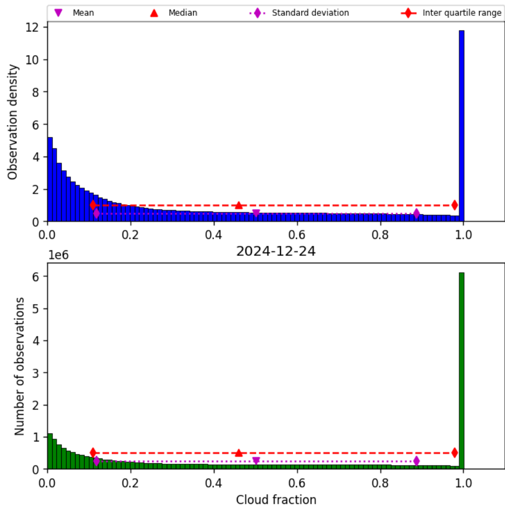
Figure 32: Histogram of “Cloud fraction” for 2024-12-23 to 2024-12-25
