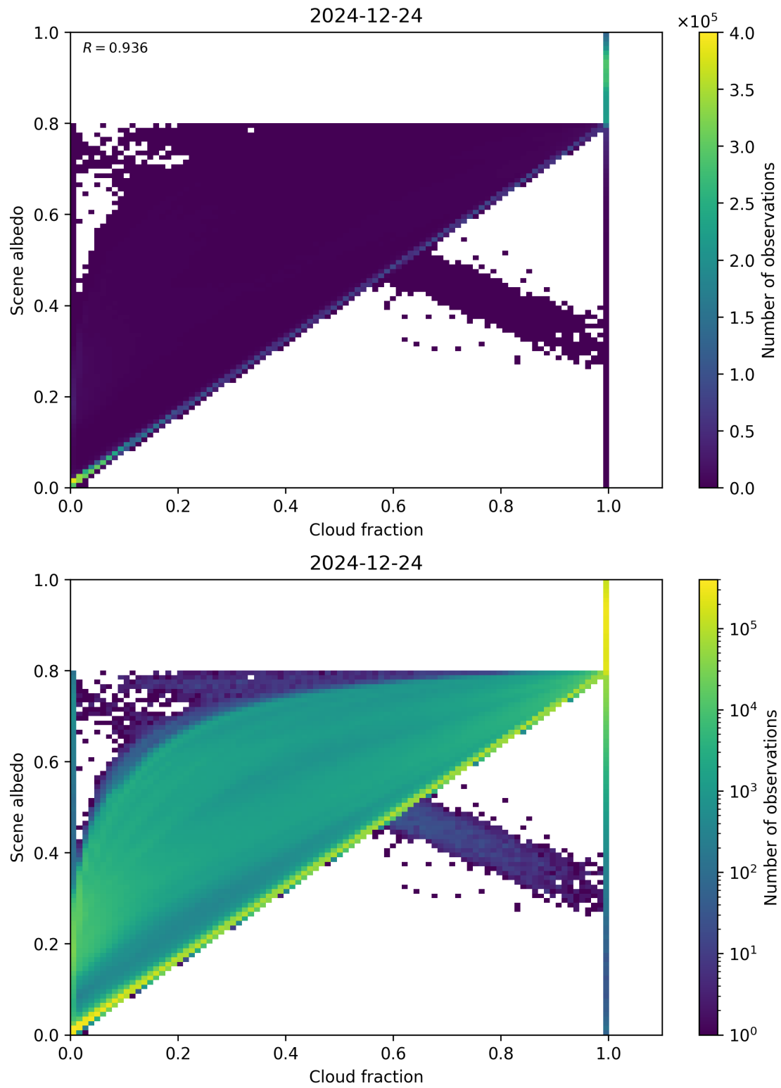
Figure 75: Scatter density plot of “Cloud fraction” against “Scene albedo” for 2024-12-23 to 2024-12-25.
