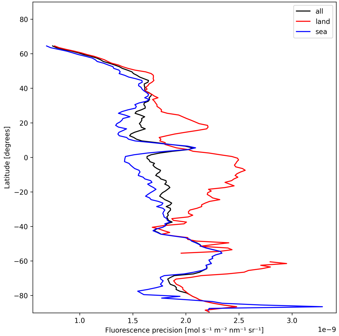
Figure 24: Zonal average of “Fluorescence precision” for 2024-12-23 to 2024-12-25.
