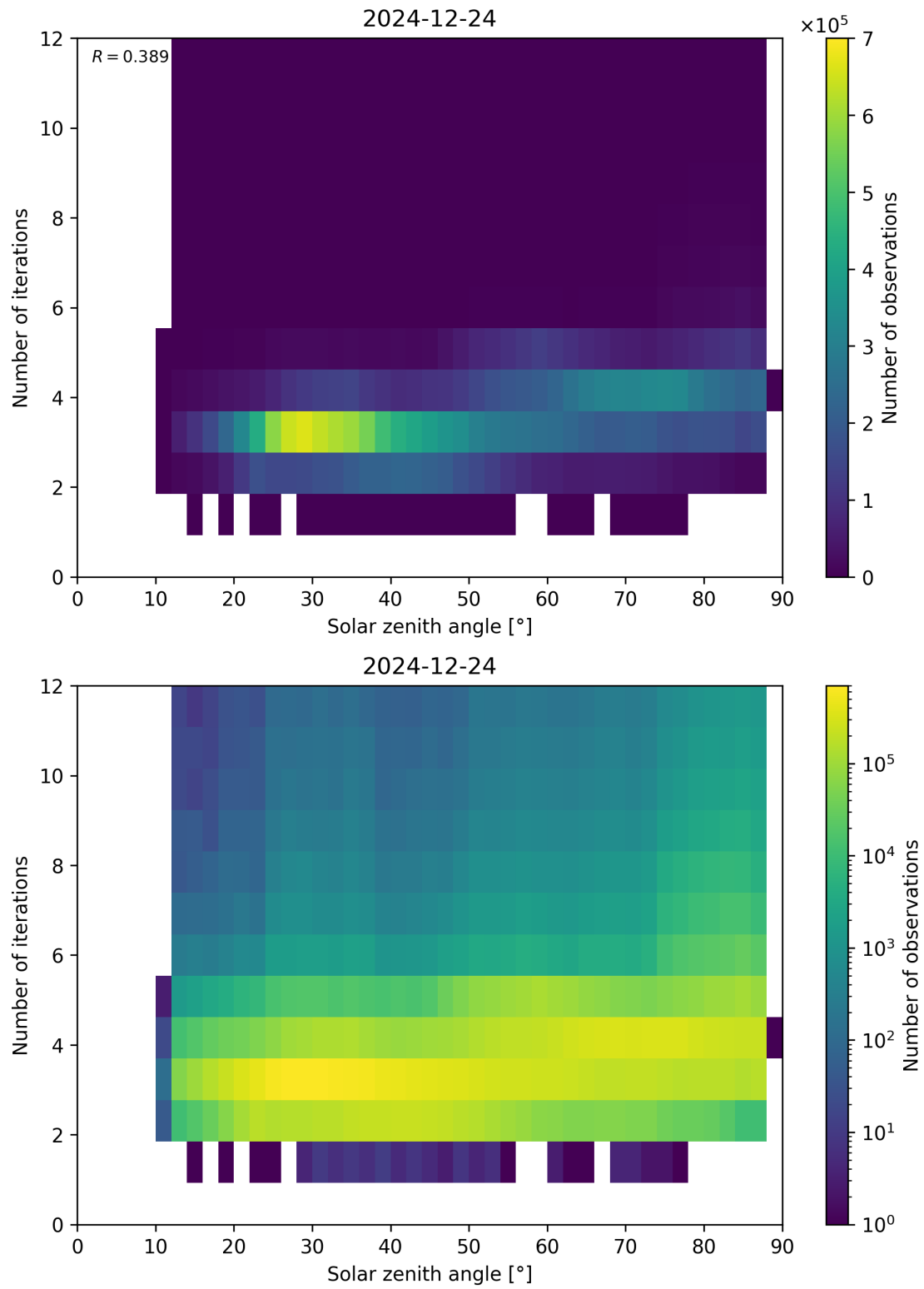
Figure 114: Scatter density plot of “Solar zenith angle” against “Number of iterations” for 2024-12-23 to 2024-12-25.
