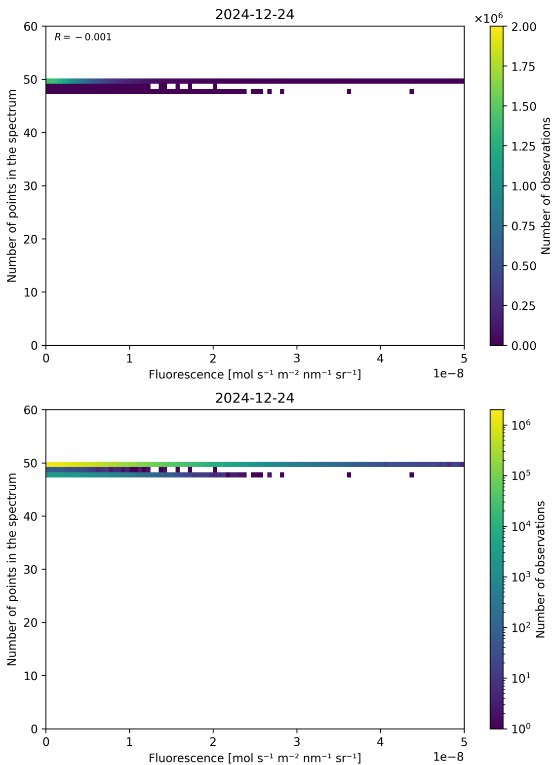
Figure 86: Scatter density plot of “Fluorescence” against “Number of points in the spectrum” for 2024-12-23 to 2024-12-25.
