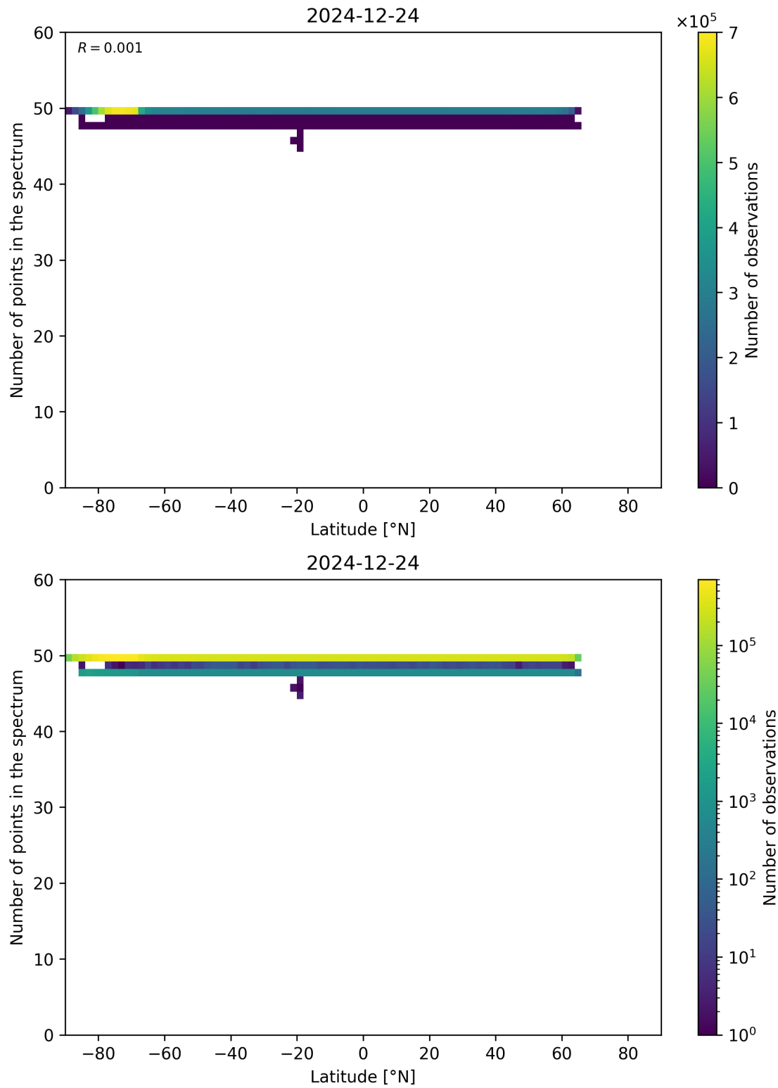
Figure 94: Scatter density plot of “Latitude” against “Number of points in the spectrum” for 2024-12-23 to 2024-12-25.
