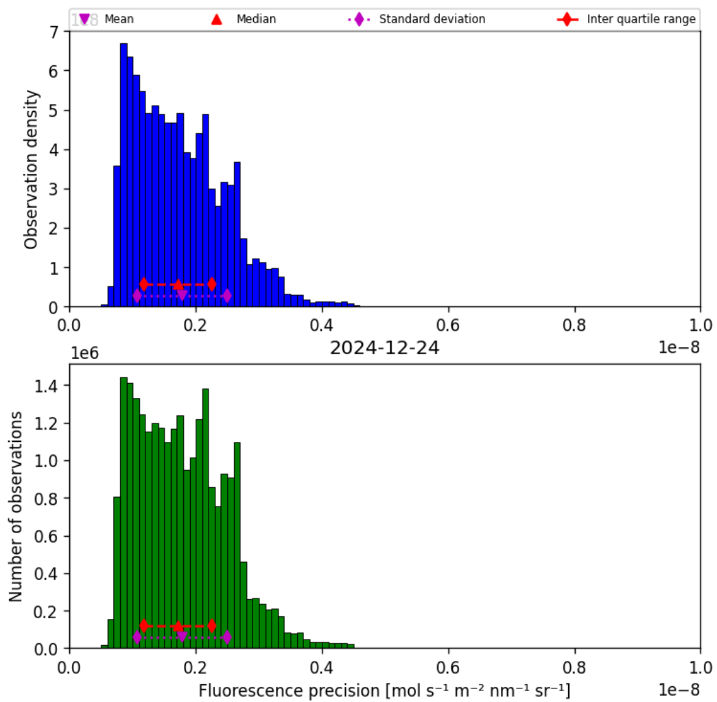
Figure 41: Histogram of “Fluorescence precision” for 2024-12-23 to 2024-12-25
