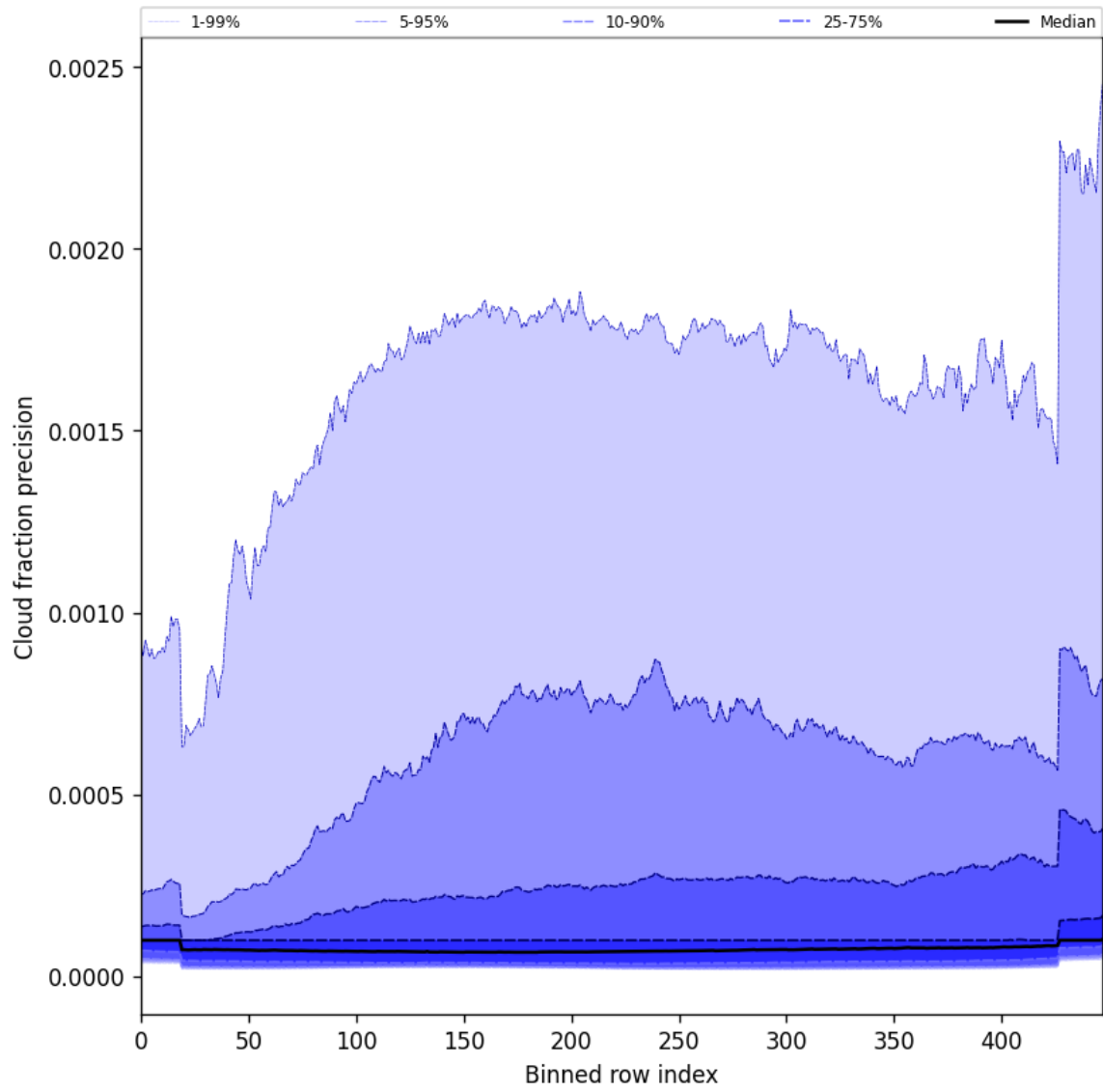
Figure 50: Along track statistics of “Cloud fraction precision” for 2024-12-23 to 2024-12-25
