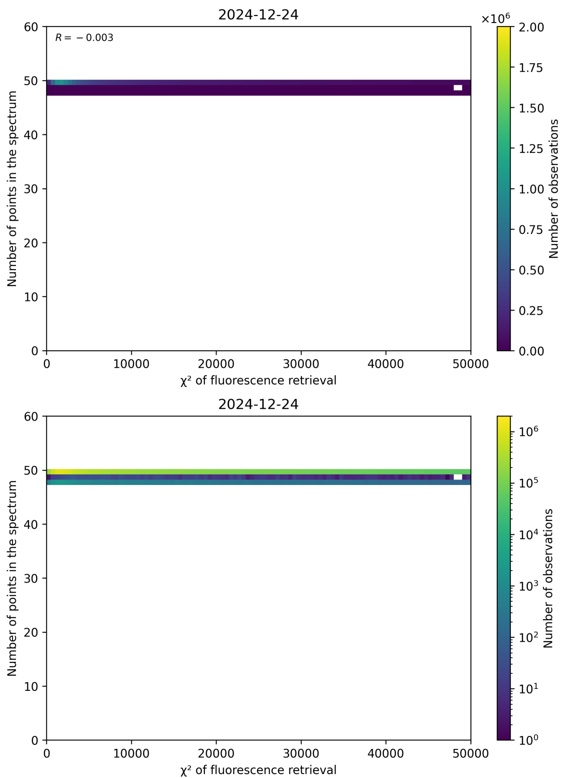
Figure 68: Scatter density plot of “ \chi^2 of fluorescence retrieval” against “Number of points in the spectrum” for 2024-12-23 to 2024-12-25.
