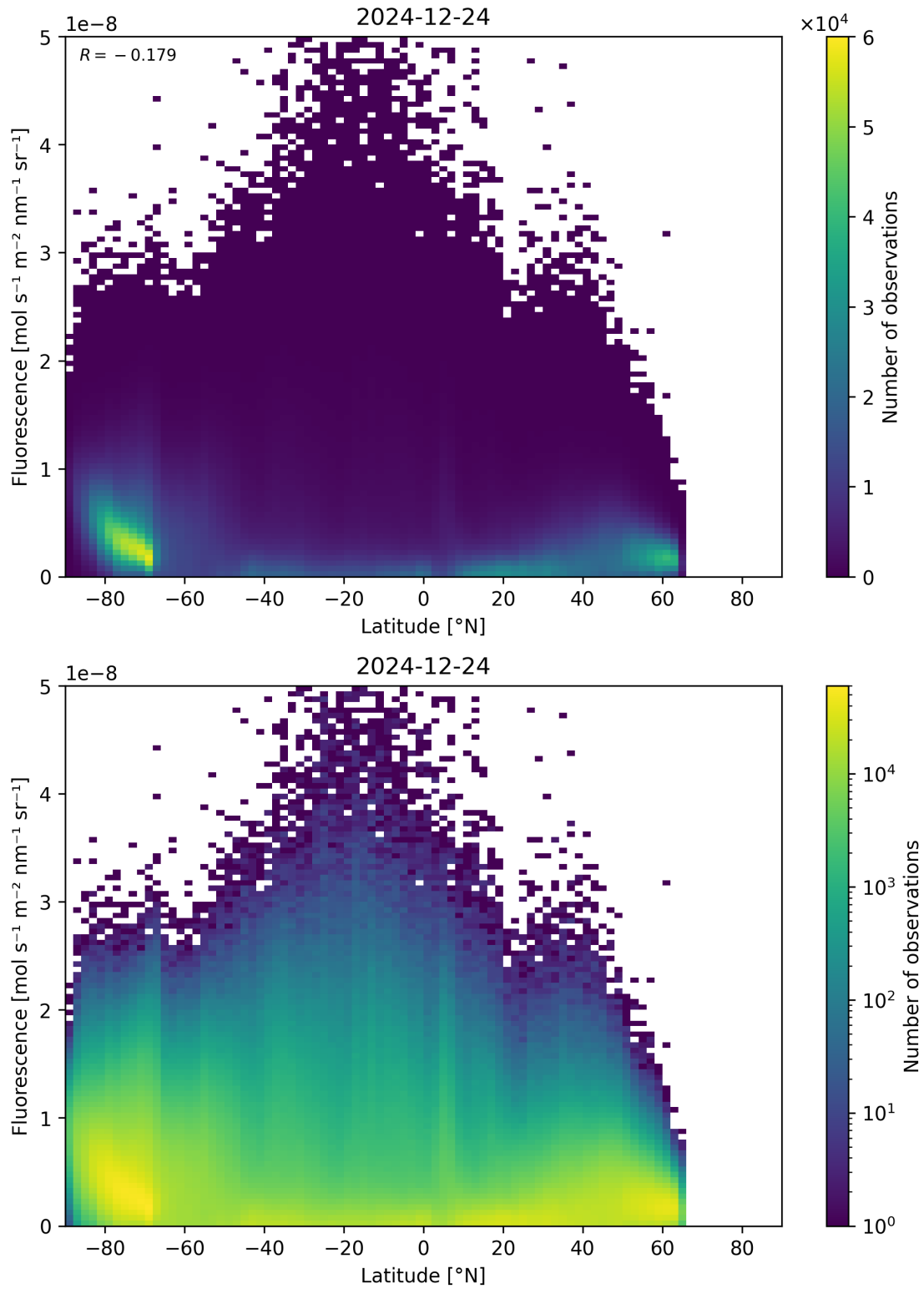
Figure 92: Scatter density plot of “Latitude” against “Fluorescence” for 2024-12-23 to 2024-12-25.
