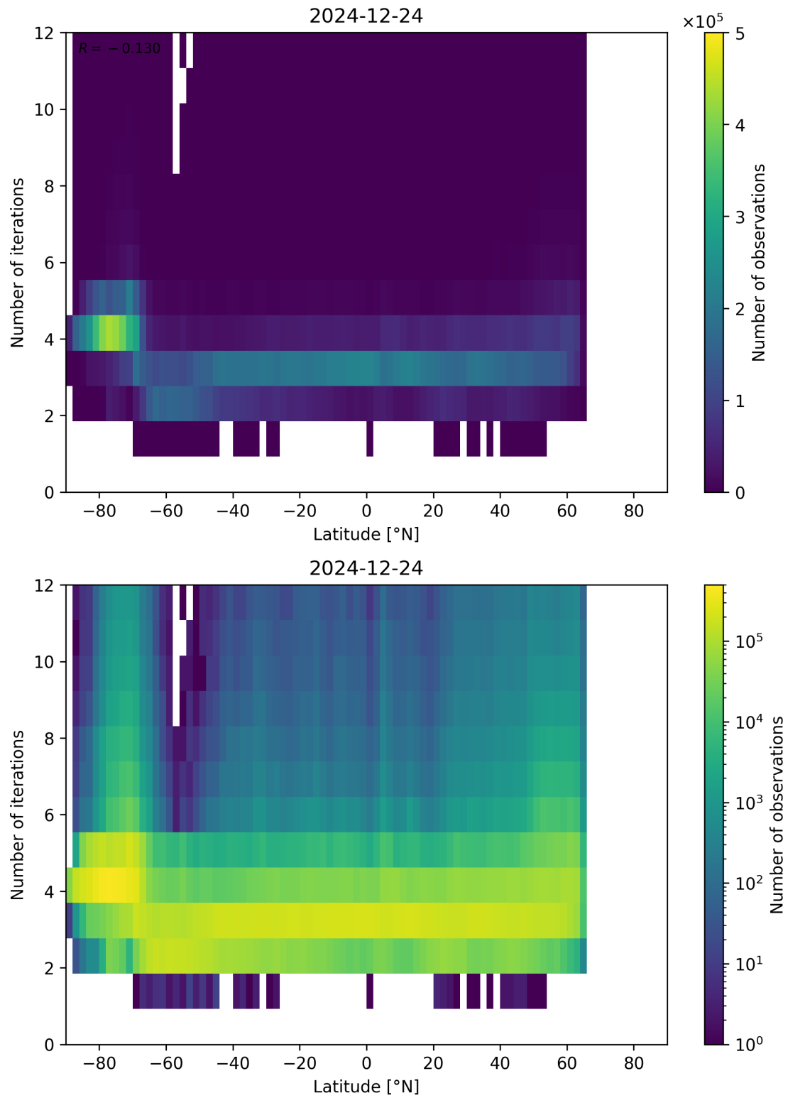
Figure 93: Scatter density plot of “Latitude” against “Number of iterations” for 2024-12-23 to 2024-12-25.
