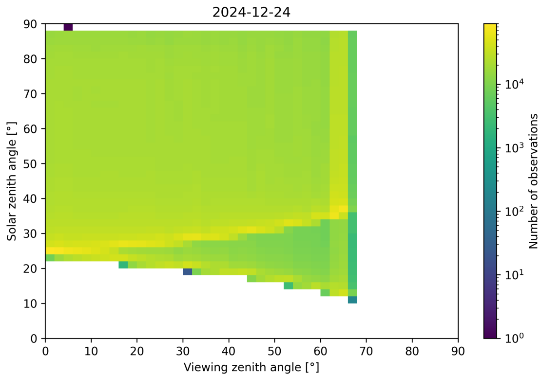
Figure 127: Scatter density plot of “Viewing zenith angle” against “Solar zenith angle” for 2024-12-23 to 2024-12-25.
