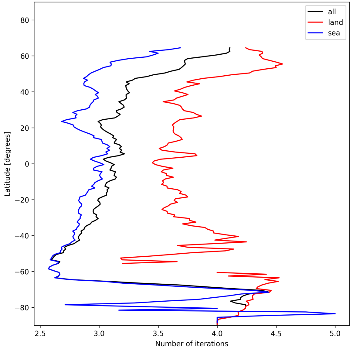
Figure 22: Zonal average of “Number of iterations” for 2024-12-23 to 2024-12-25.
