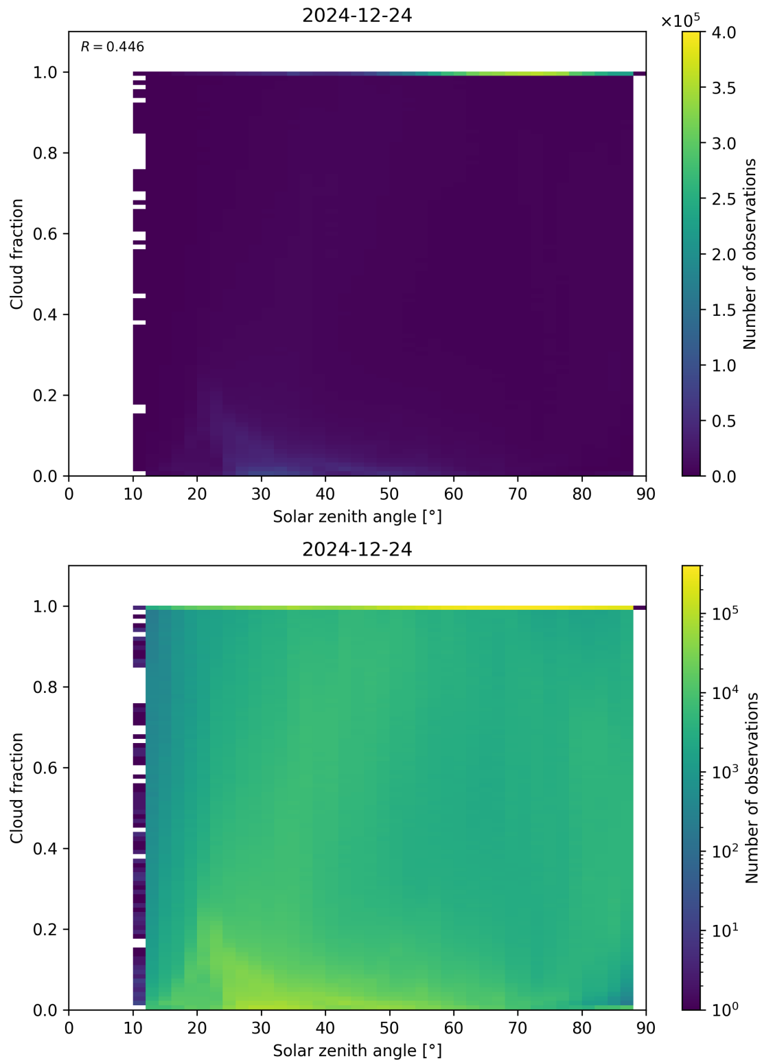
Figure 110: Scatter density plot of “Solar zenith angle” against “Cloud fraction” for 2024-12-23 to 2024-12-25.
