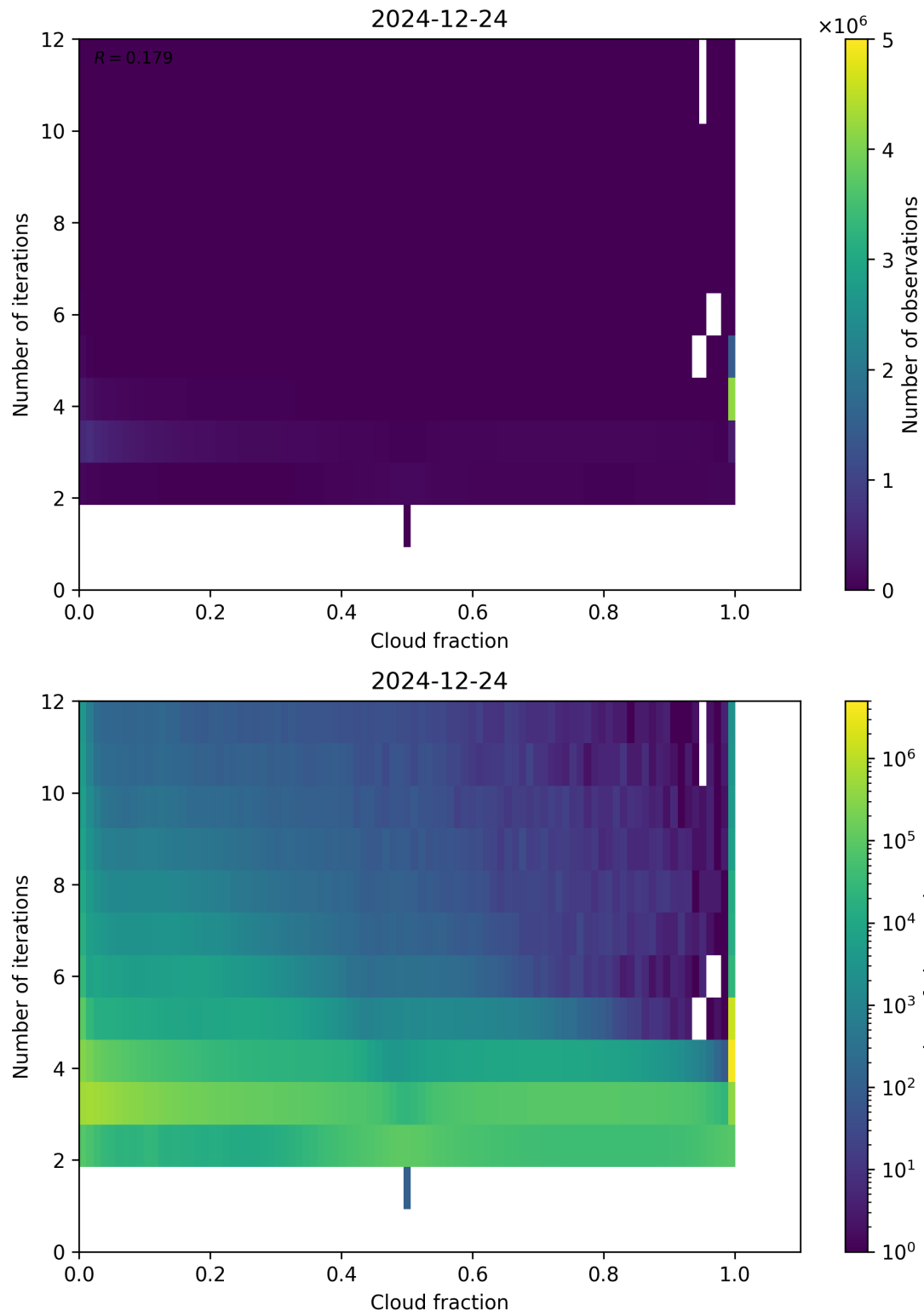
Figure 73: Scatter density plot of “Cloud fraction” against “Number of iterations” for 2024-12-23 to 2024-12-25.
