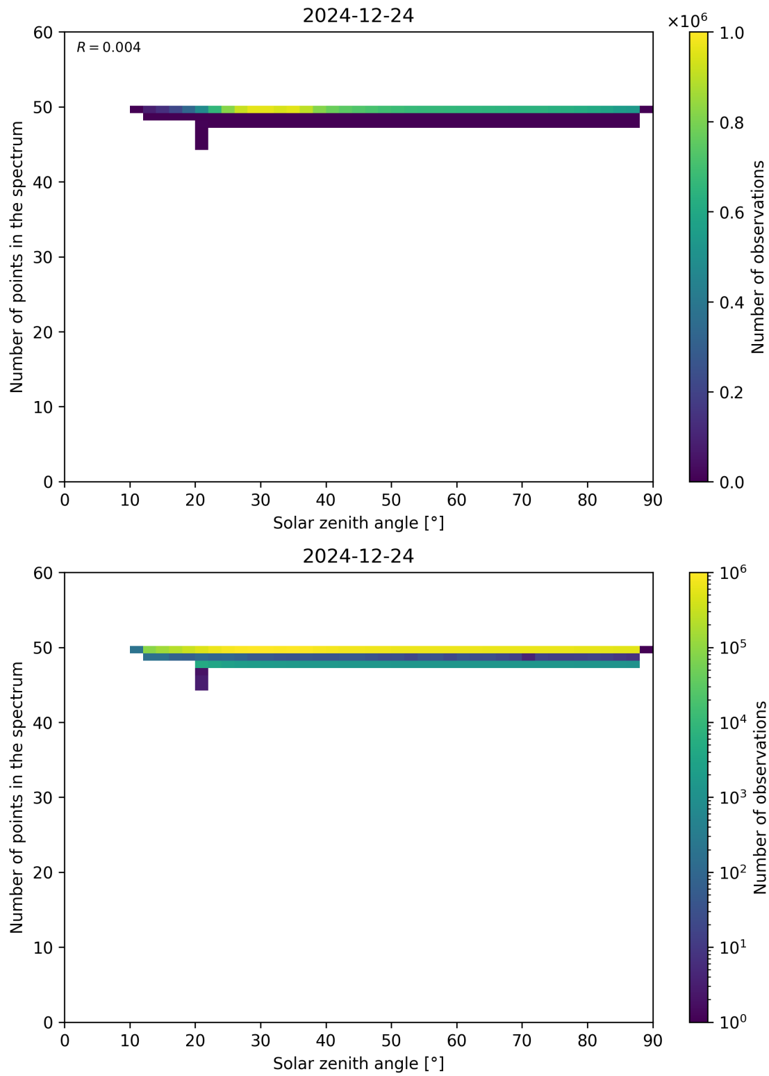
Figure 115: Scatter density plot of “Solar zenith angle” against “Number of points in the spectrum” for 2024-12-23 to 2024-12-25.
