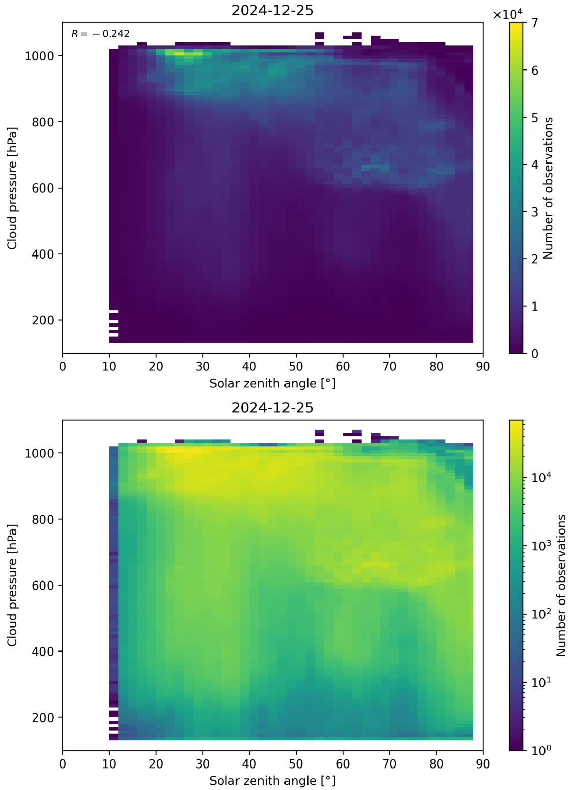
Figure 111: Scatter density plot of “Solar zenith angle” against “Cloud pressure” for 2024-12-24 to 2024-12-26.
