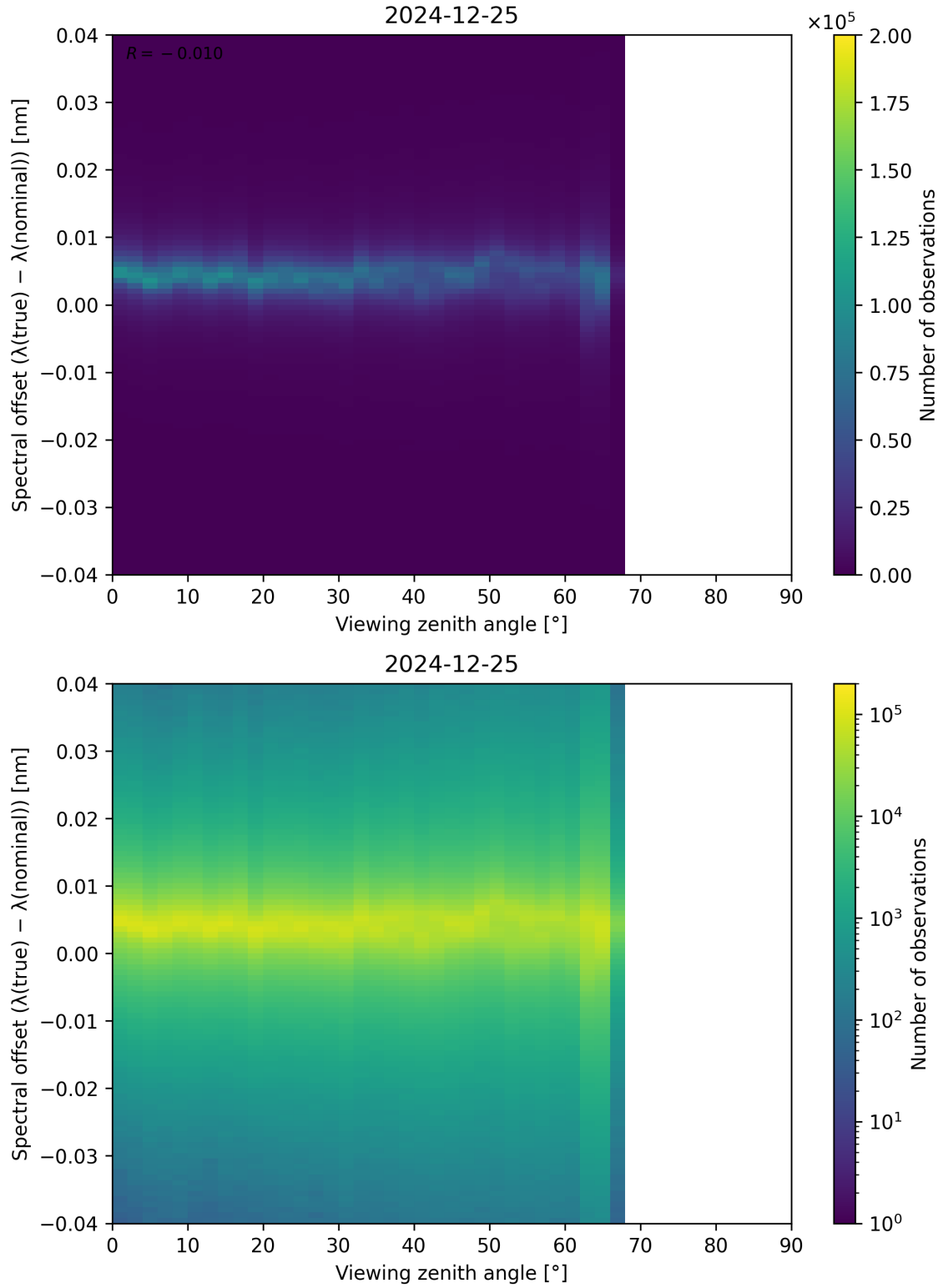
Figure 128: Scatter density plot of “Viewing zenith angle” against “Spectral offset ( \lambda_{\text{true}} - \lambda_{\text{nominal}} )” for 2024-12-24 to 2024-12-26.
