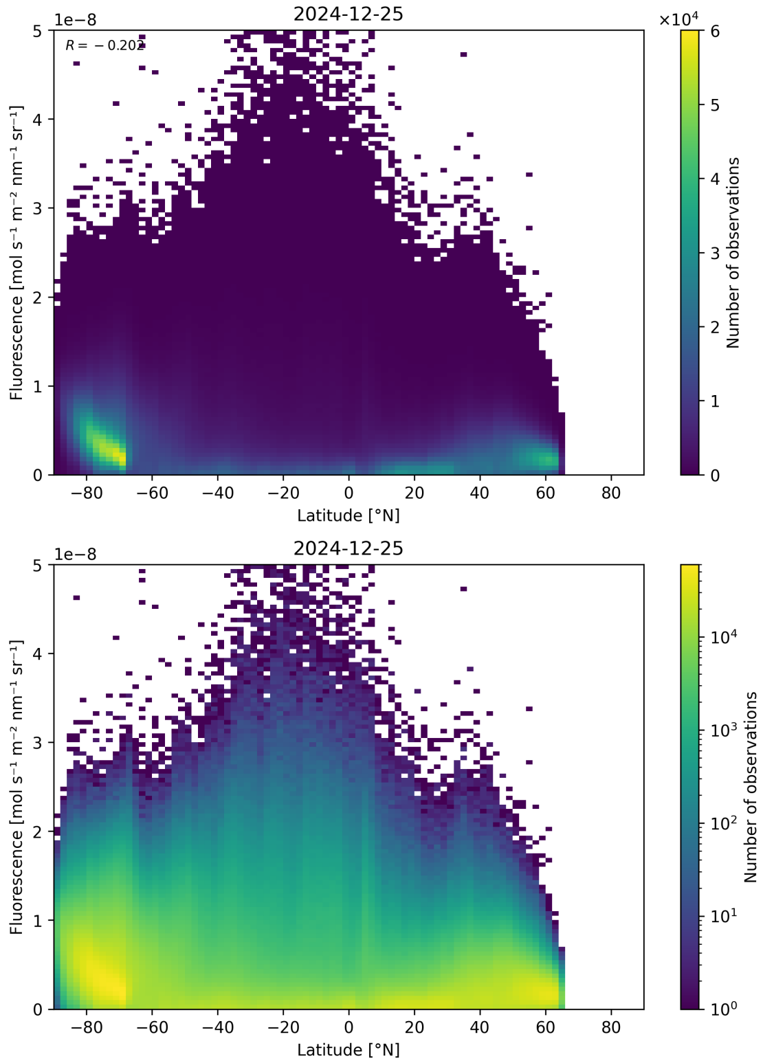
Figure 92: Scatter density plot of “Latitude” against “Fluorescence” for 2024-12-24 to 2024-12-26.
