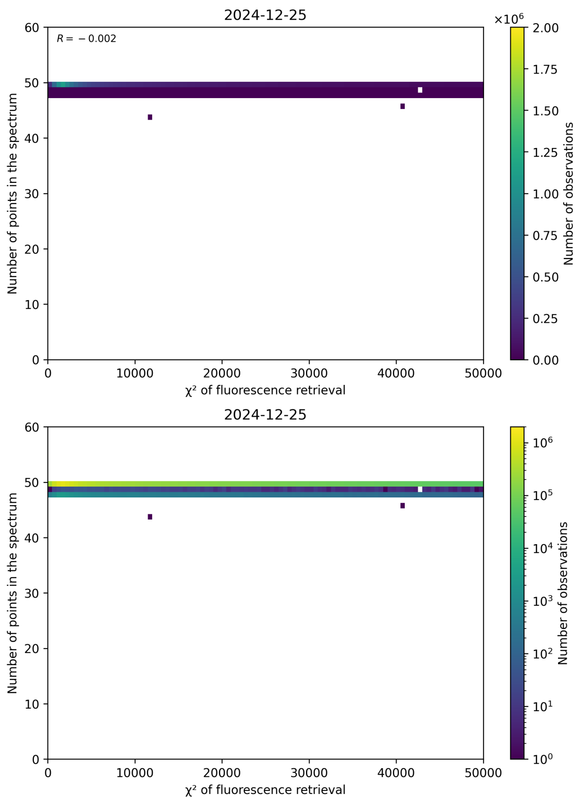
Figure 68: Scatter density plot of “ \chi^2 of fluorescence retrieval” against “Number of points in the spectrum” for 2024-12-24 to 2024-12-26.
