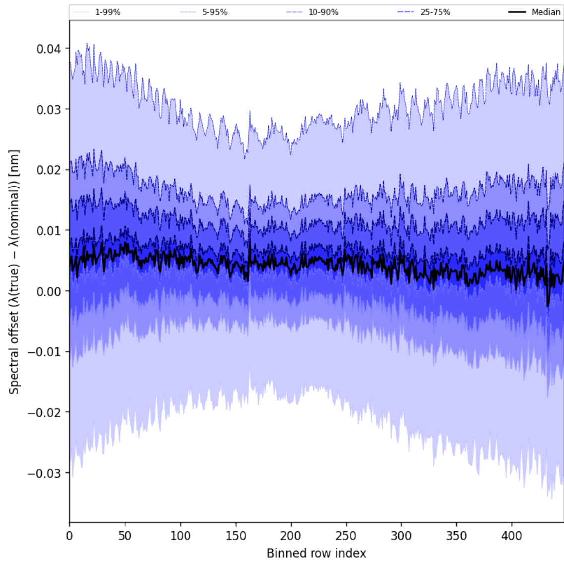
Figure 62: Along track statistics of “Spectral offset ( \lambda_{\text{true}} - \lambda_{\text{nominal}} )” for 2024-12-24 to 2024-12-26
