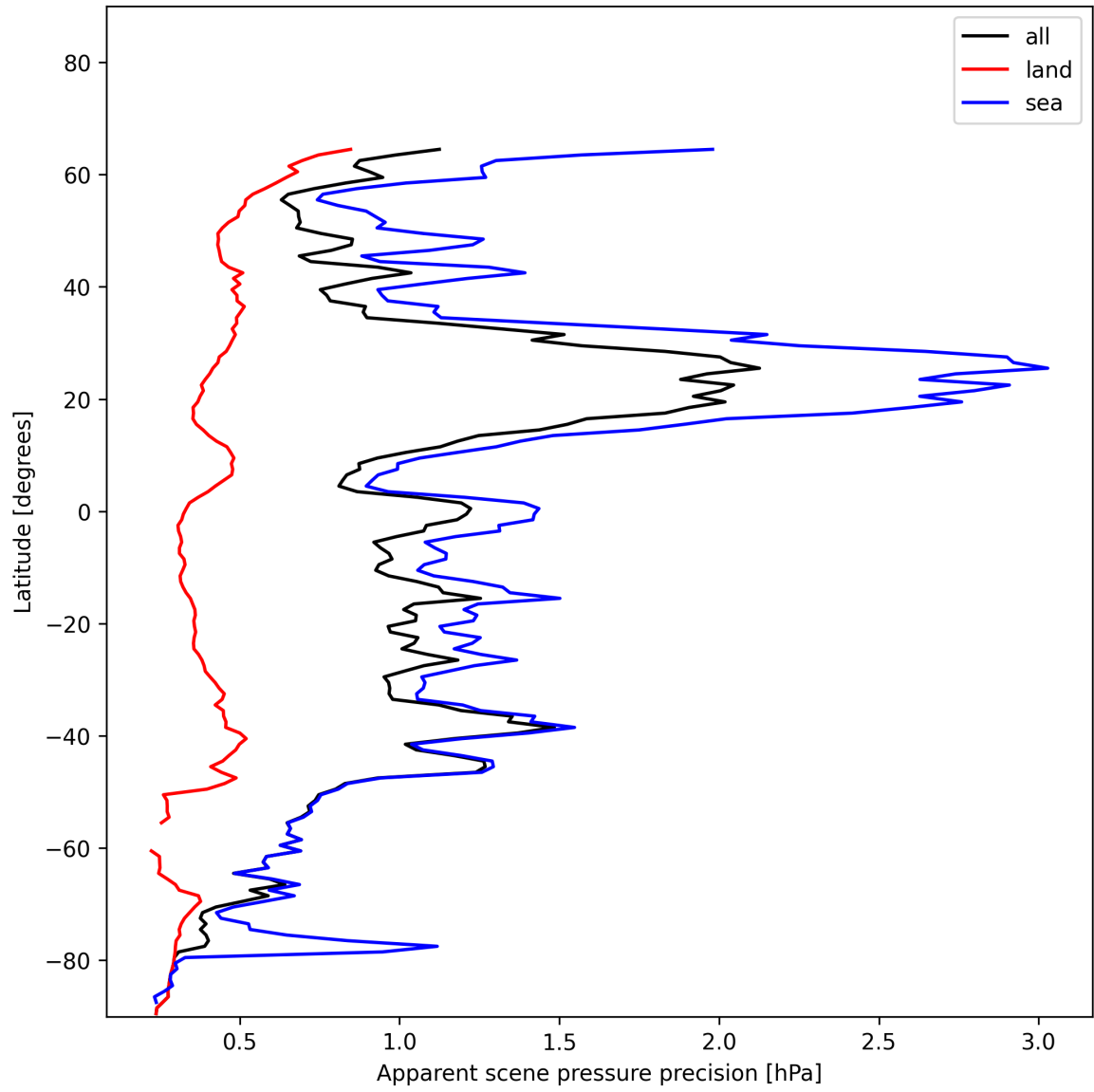
Figure 20: Zonal average of “Apparent scene pressure precision” for 2024-12-24 to 2024-12-26.
