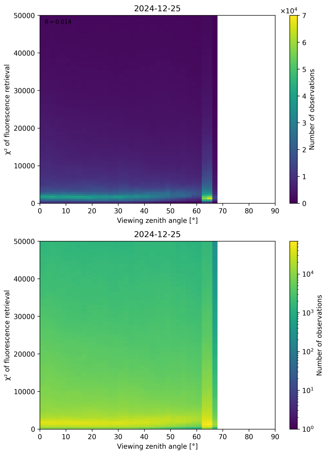
Figure 119: Scatter density plot of “Viewing zenith angle” against “ \chi^2 of fluorescence retrieval” for 2024-12-24 to 2024-12-26.
