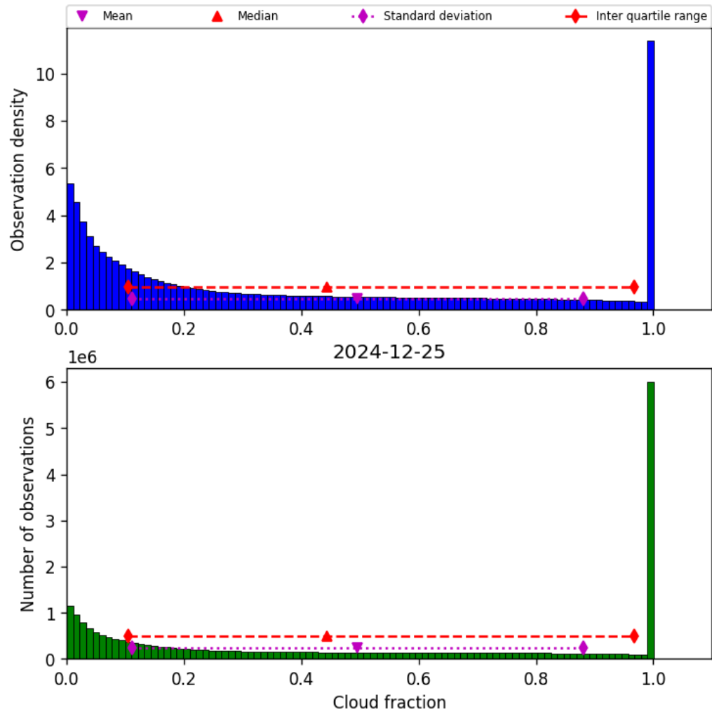
Figure 32: Histogram of “Cloud fraction” for 2024-12-24 to 2024-12-26
