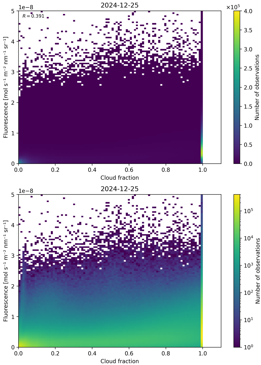
Figure 72: Scatter density plot of “Cloud fraction” against “Fluorescence” for 2024-12-24 to 2024-12-26.
