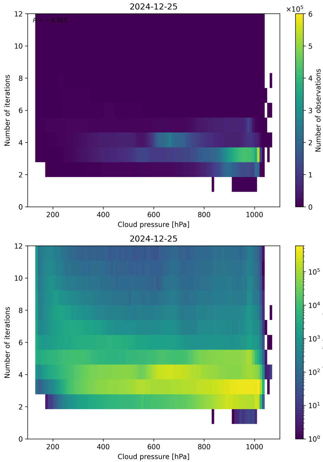
Figure 81: Scatter density plot of “Cloud pressure” against “Number of iterations” for 2024-12-24 to 2024-12-26.
