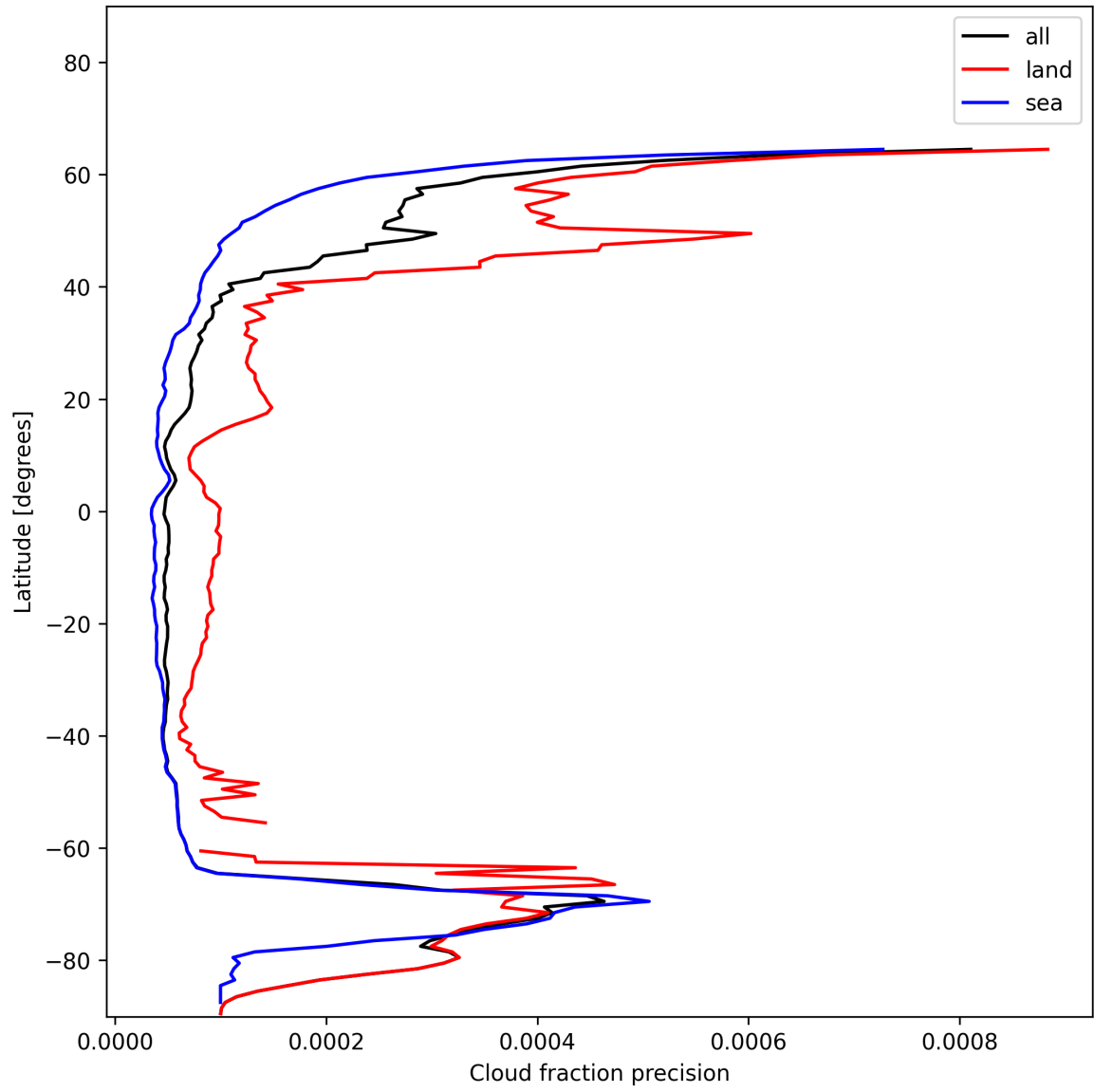
Figure 16: Zonal average of “Cloud fraction precision” for 2024-12-24 to 2024-12-26.
