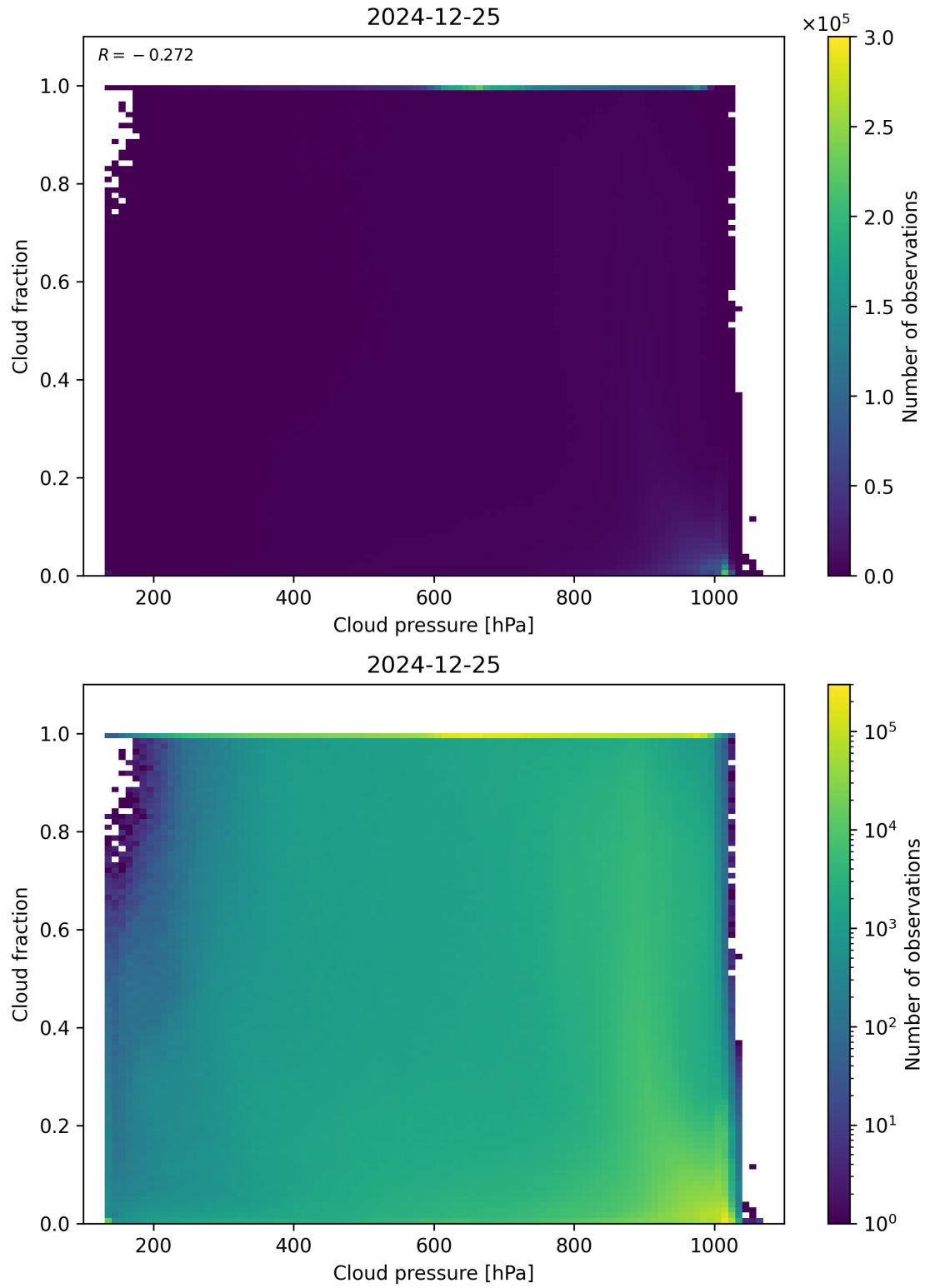
Figure 79: Scatter density plot of “Cloud pressure” against “Cloud fraction” for 2024-12-24 to 2024-12-26.
