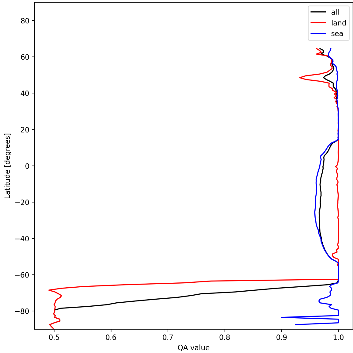
Figure 12: Zonal average of “QA value” for 2024-12-24 to 2024-12-26.
