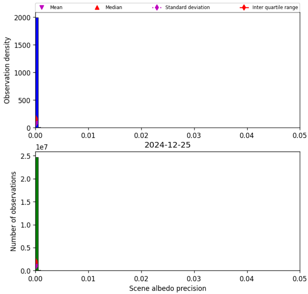
Figure 35: Histogram of “Scene albedo precision” for 2024-12-24 to 2024-12-26
