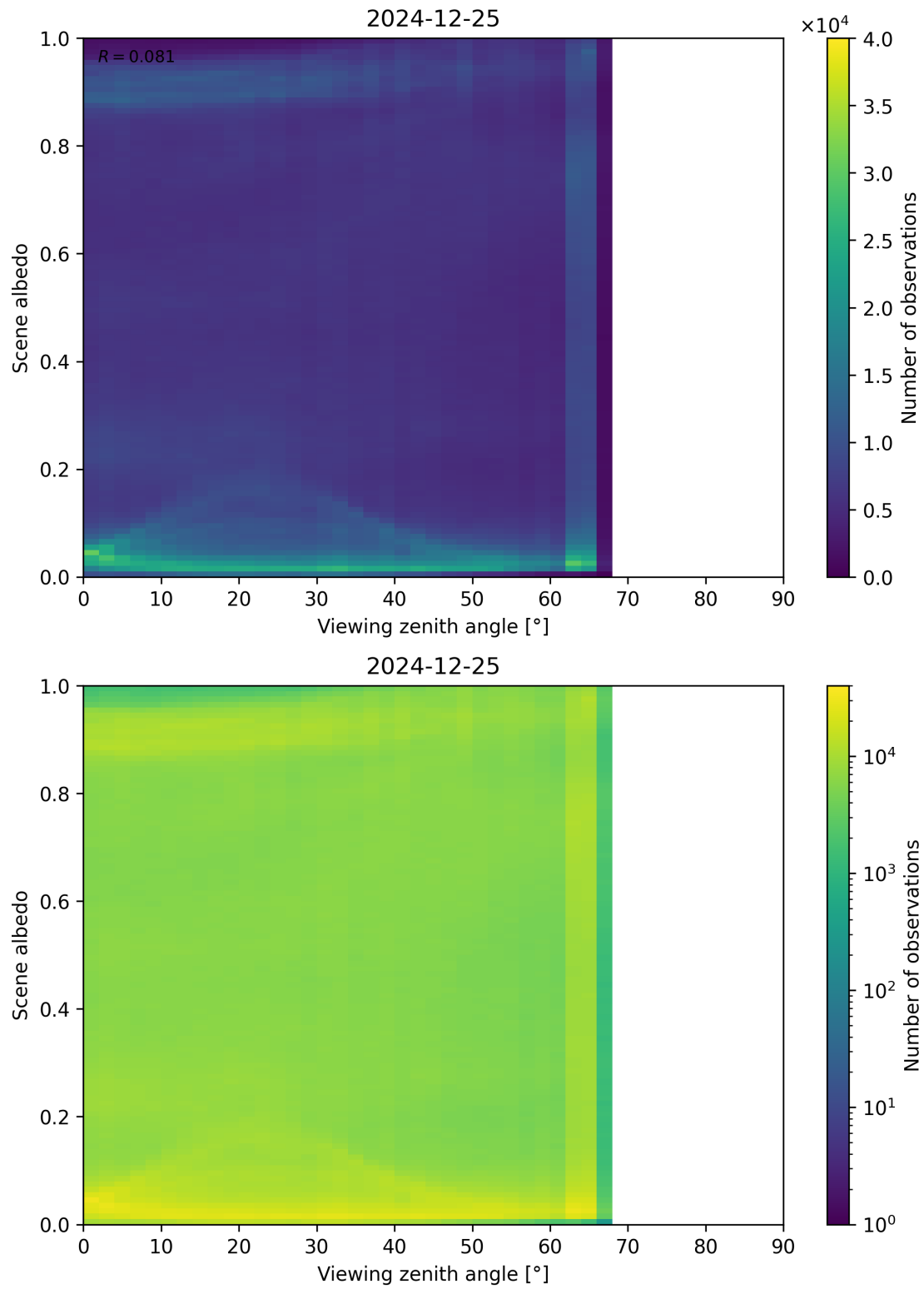
Figure 126: Scatter density plot of “Viewing zenith angle” against “Scene albedo” for 2024-12-24 to 2024-12-26.
