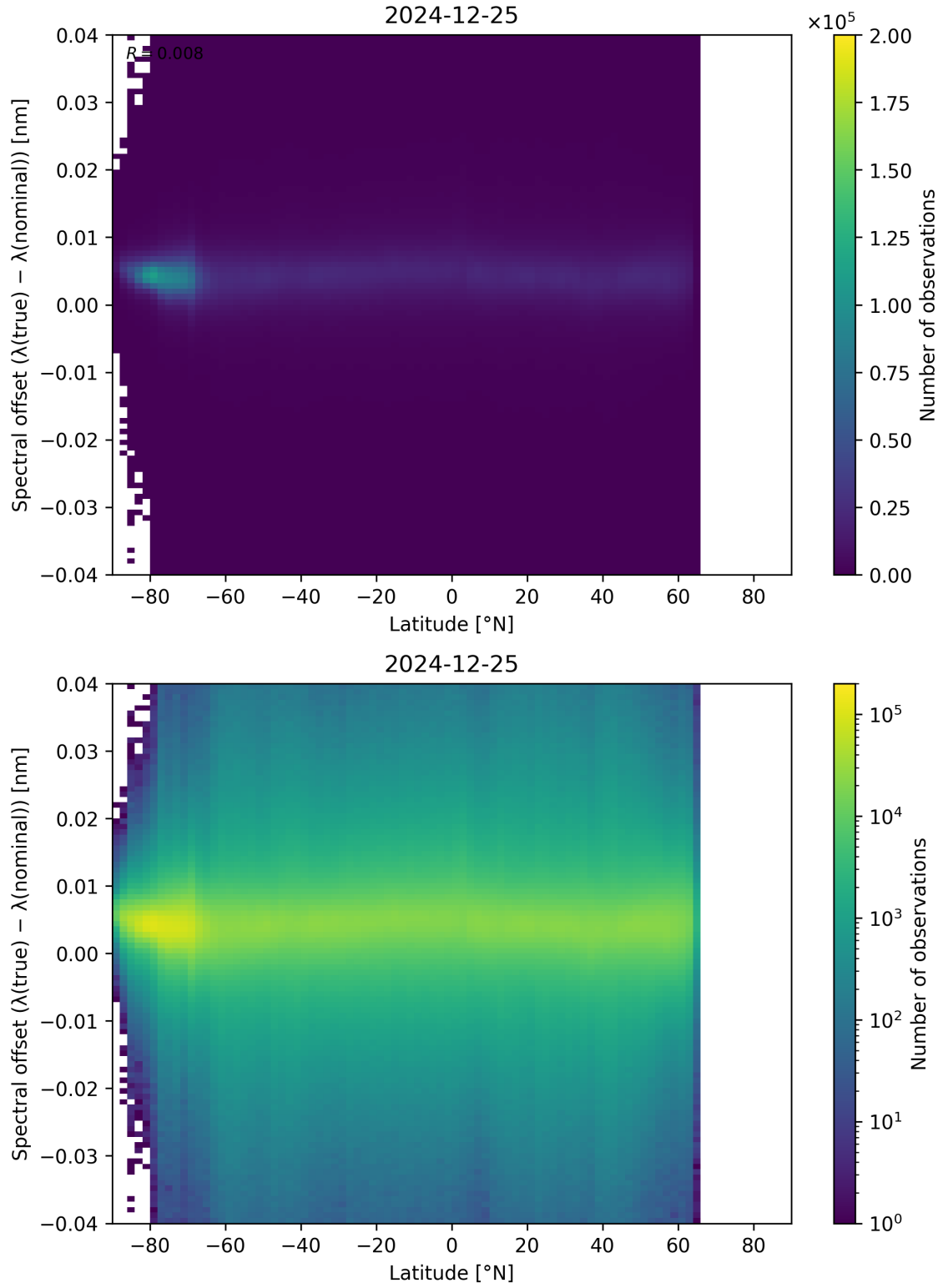
Figure 96: Scatter density plot of “Latitude” against “Spectral offset ( \lambda_{\text{true}} - \lambda_{\text{nominal}} )” for 2024-12-24 to 2024-12-26.
