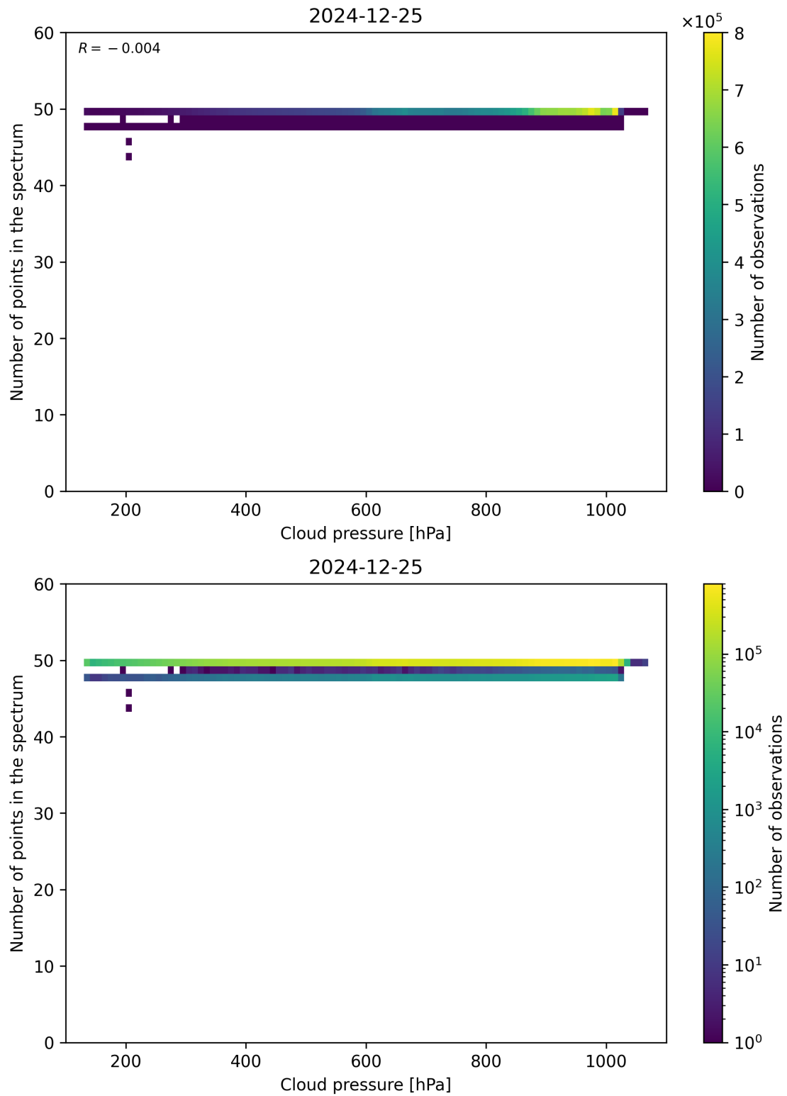
Figure 82: Scatter density plot of “Cloud pressure” against “Number of points in the spectrum” for 2024-12-24 to 2024-12-26.
