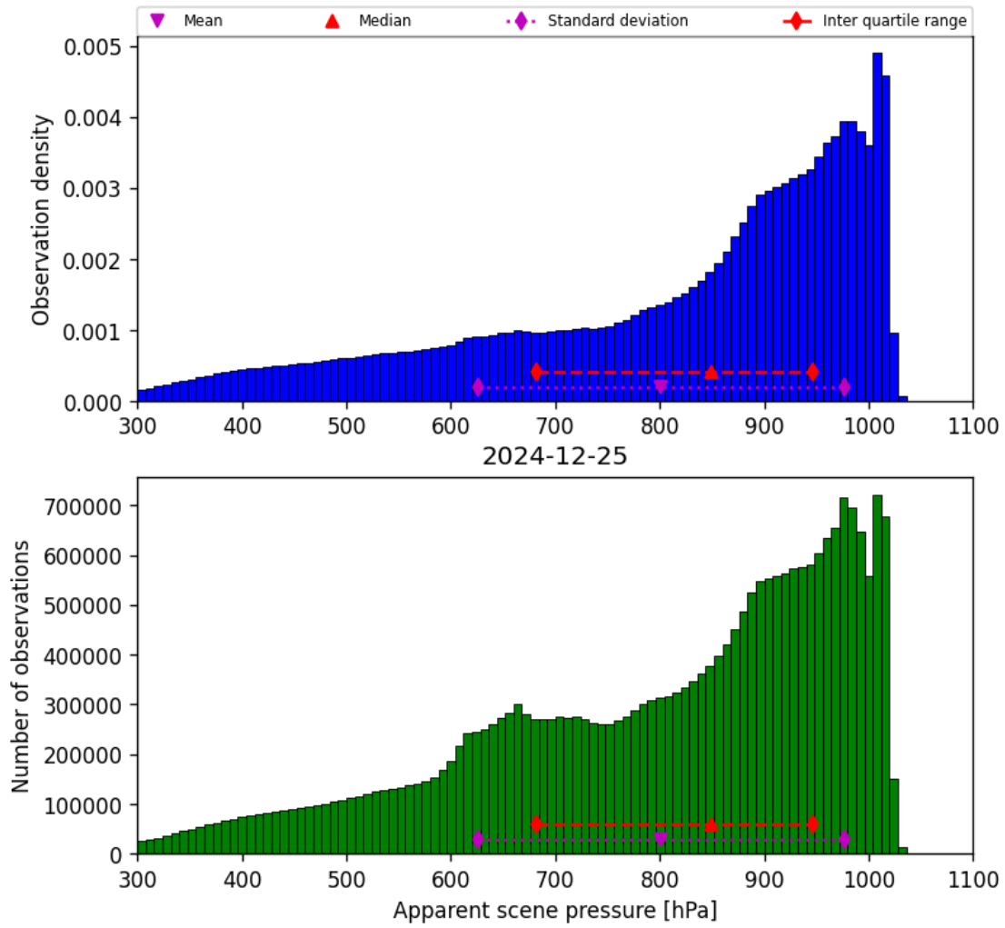
Figure 36: Histogram of “Apparent scene pressure” for 2024-12-24 to 2024-12-26
