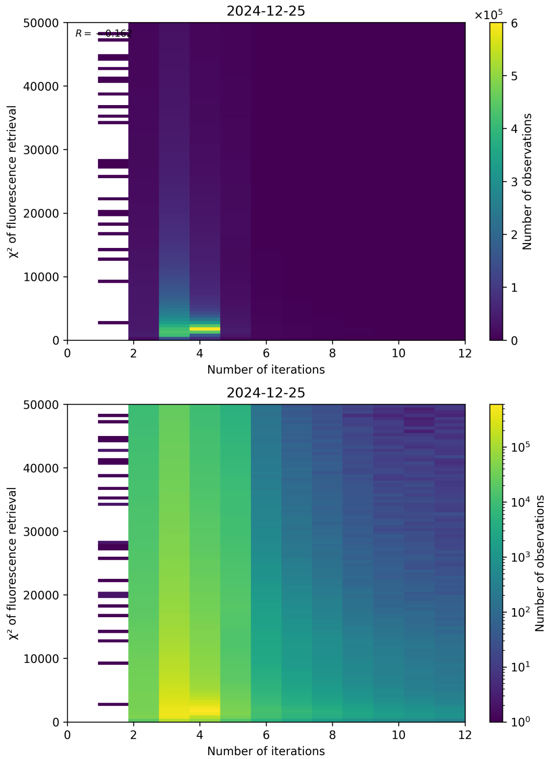
Figure 97: Scatter density plot of “Number of iterations” against “ \chi^2 of fluorescence retrieval” for 2024-12-24 to 2024-12-26.
