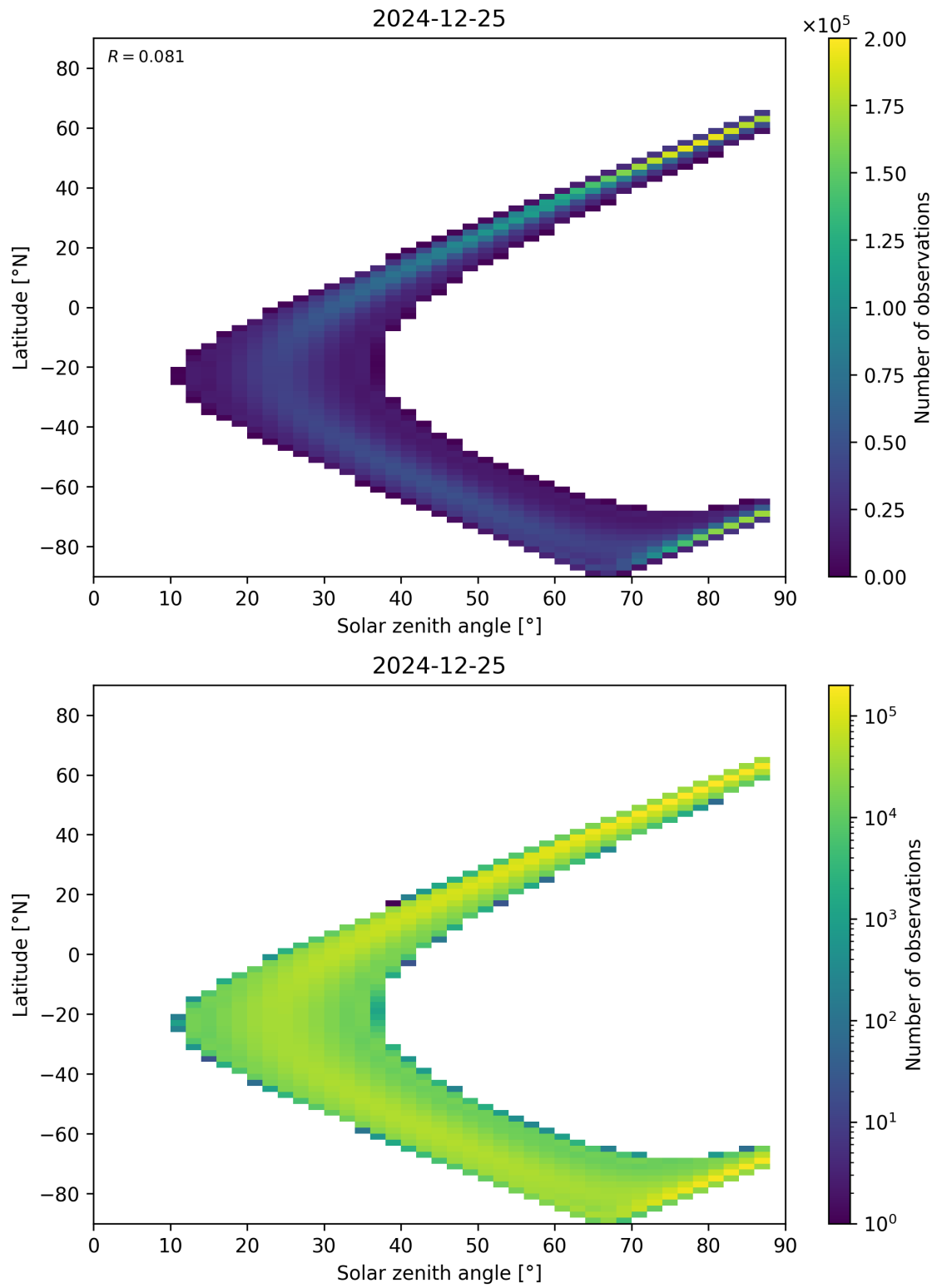
Figure 113: Scatter density plot of “Solar zenith angle” against “Latitude” for 2024-12-24 to 2024-12-26.
