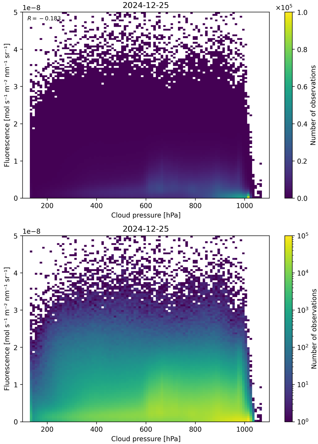
Figure 80: Scatter density plot of “Cloud pressure” against “Fluorescence” for 2024-12-24 to 2024-12-26.
