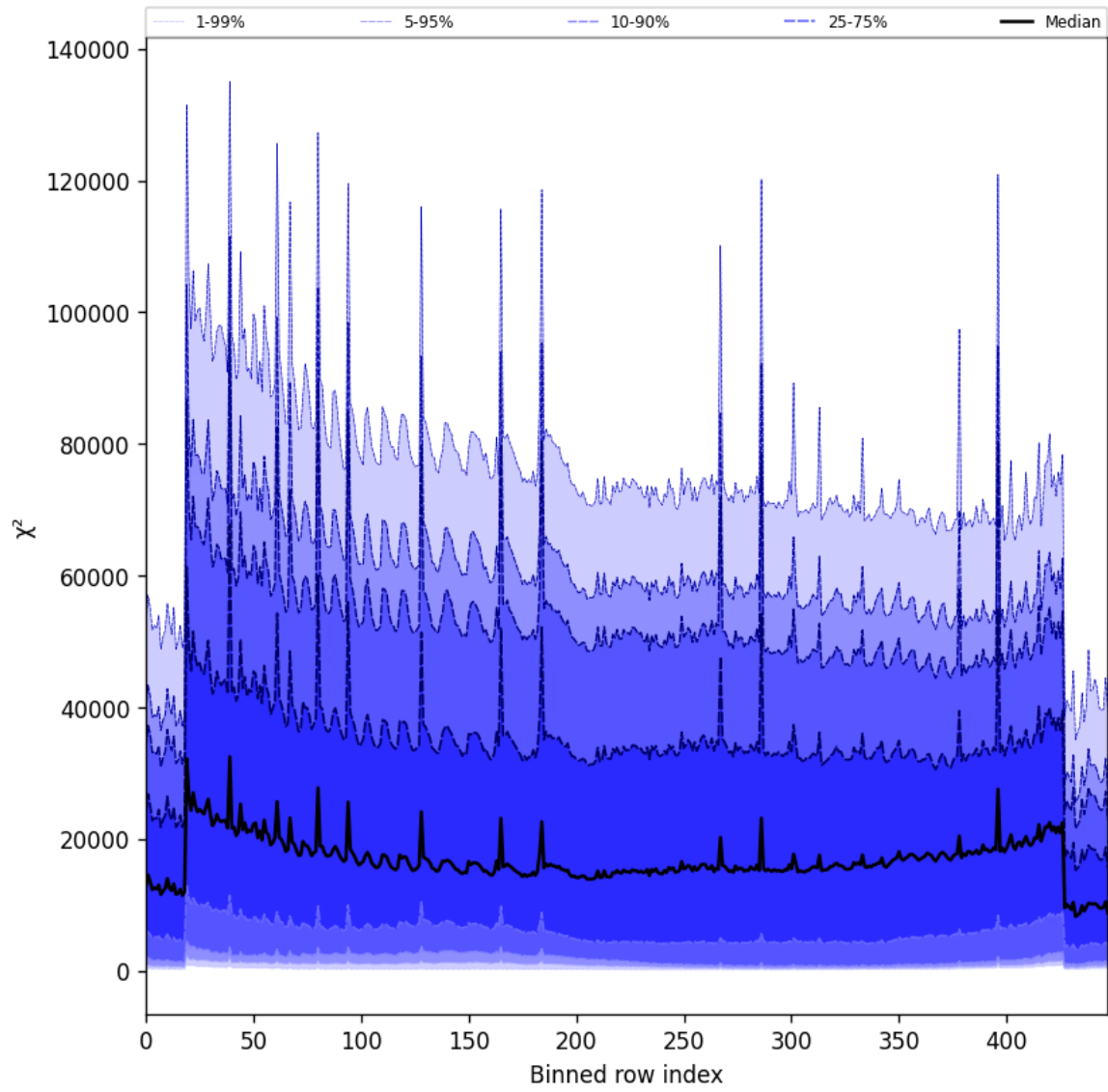
Figure 55: Along track statistics of “ \chi^2 ” for 2024-12-24 to 2024-12-26
