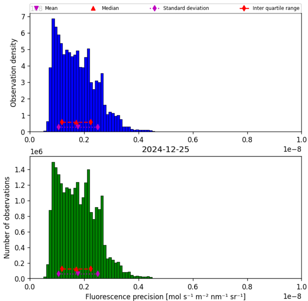
Figure 41: Histogram of “Fluorescence precision” for 2024-12-24 to 2024-12-26
