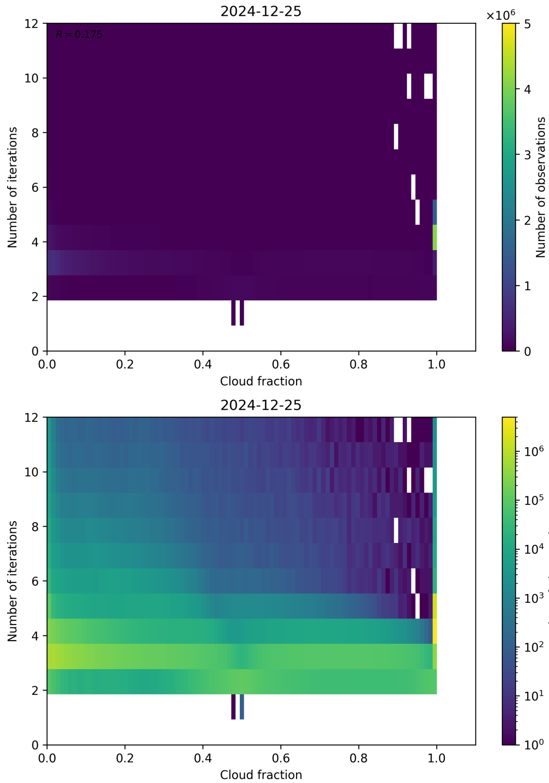
Figure 73: Scatter density plot of “Cloud fraction” against “Number of iterations” for 2024-12-24 to 2024-12-26.
