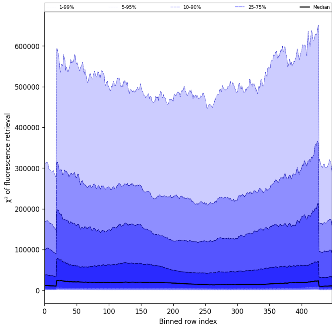
Figure 59: Along track statistics of “ \chi^2 of fluorescence retrieval” for 2024-12-24 to 2024-12-26
