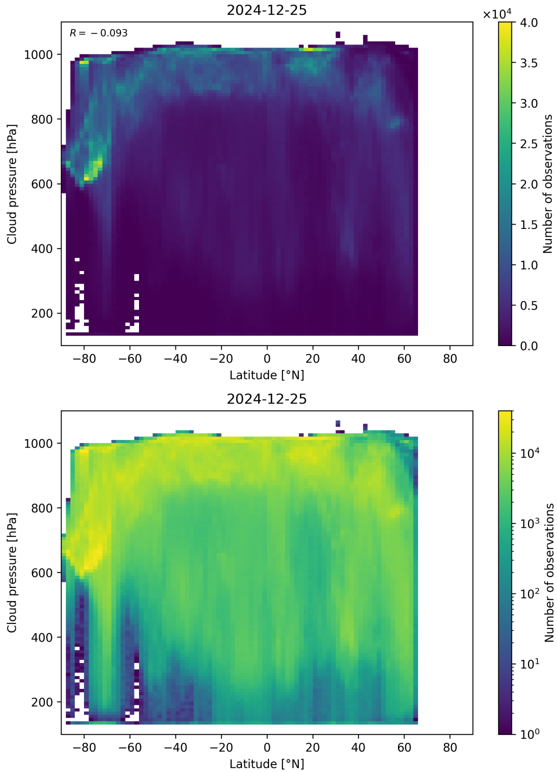
Figure 91: Scatter density plot of “Latitude” against “Cloud pressure” for 2024-12-24 to 2024-12-26.
