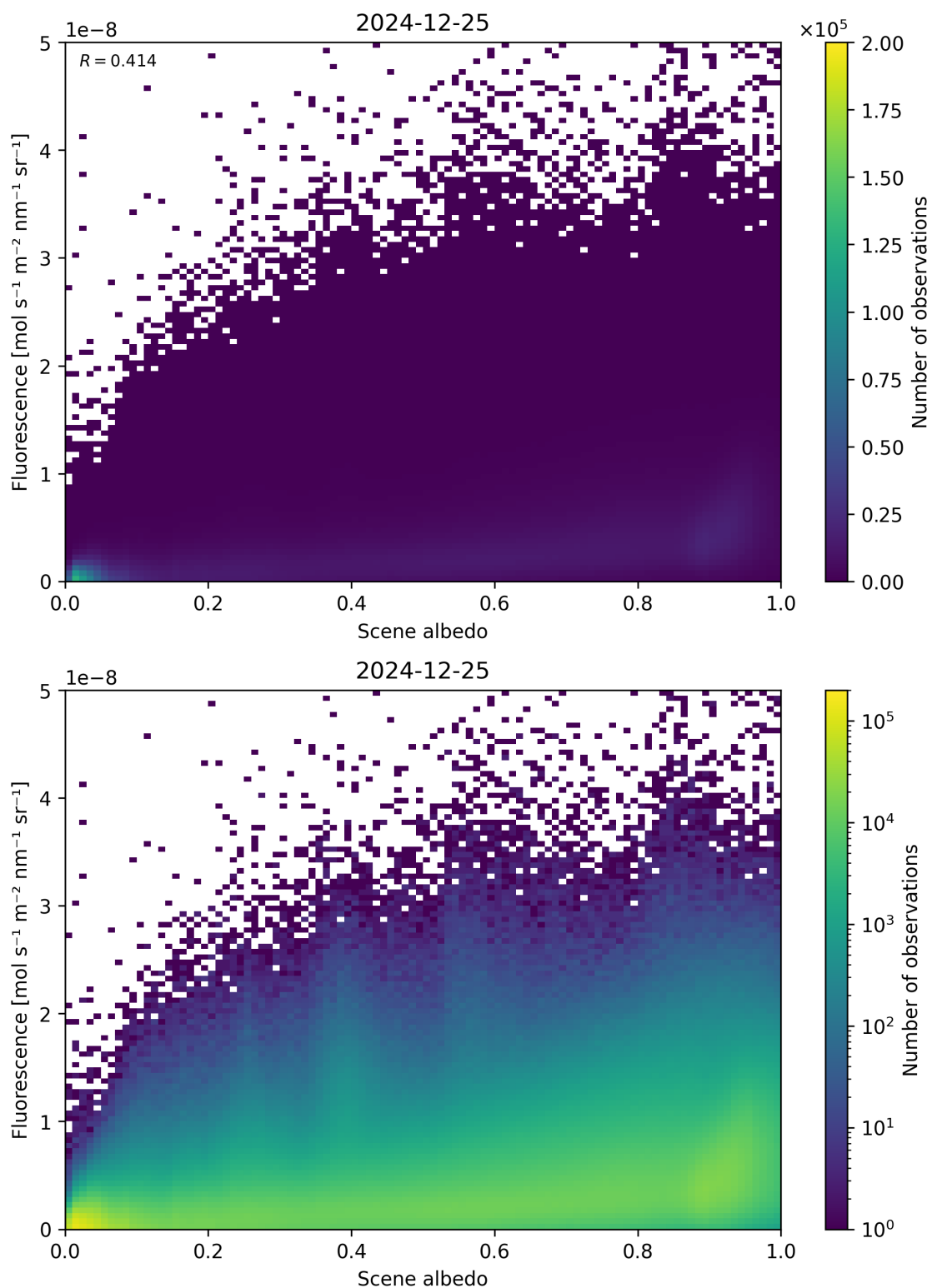
Figure 104: Scatter density plot of “Scene albedo” against “Fluorescence” for 2024-12-24 to 2024-12-26.
