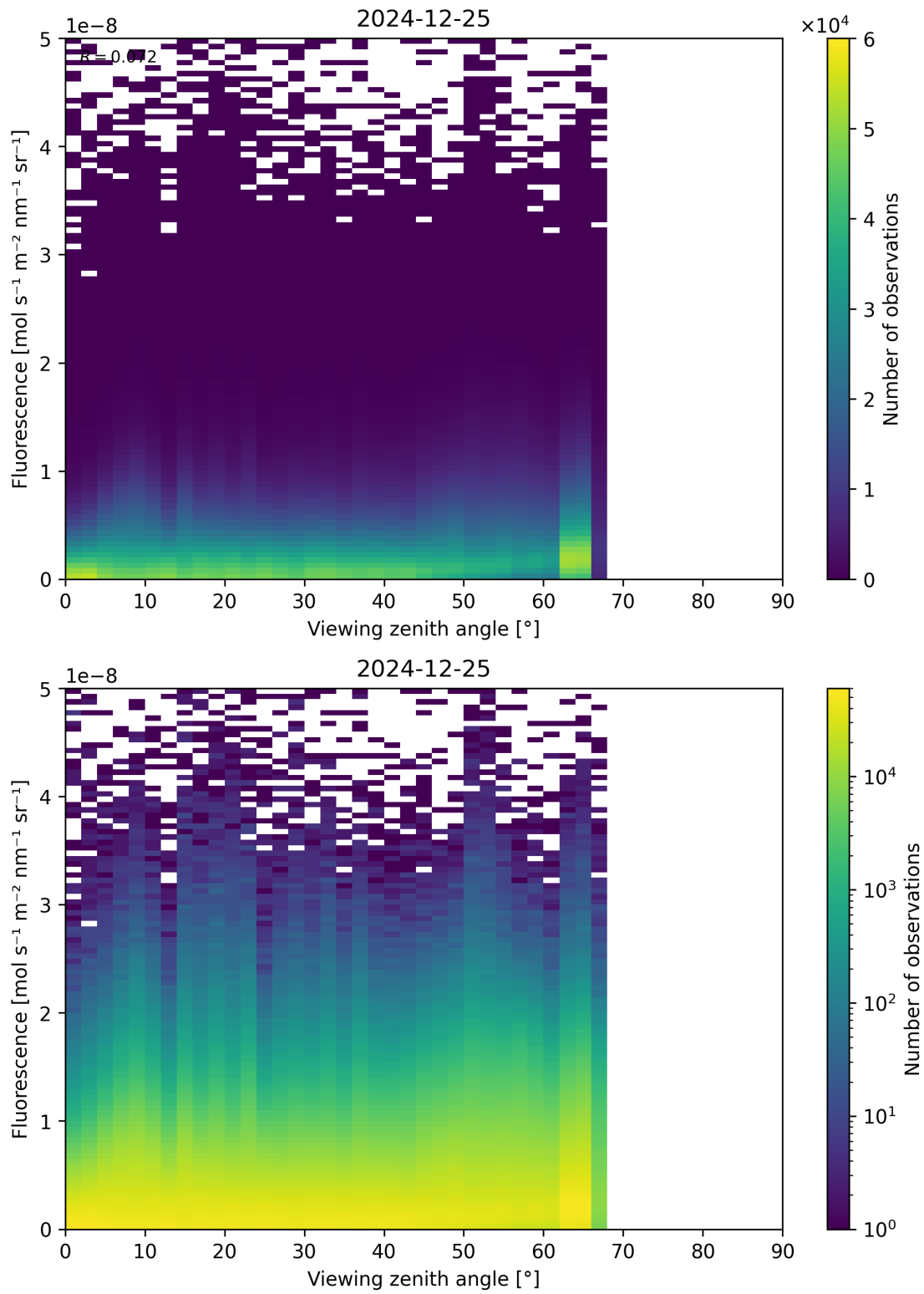
Figure 122: Scatter density plot of “Viewing zenith angle” against “Fluorescence” for 2024-12-24 to 2024-12-26.
