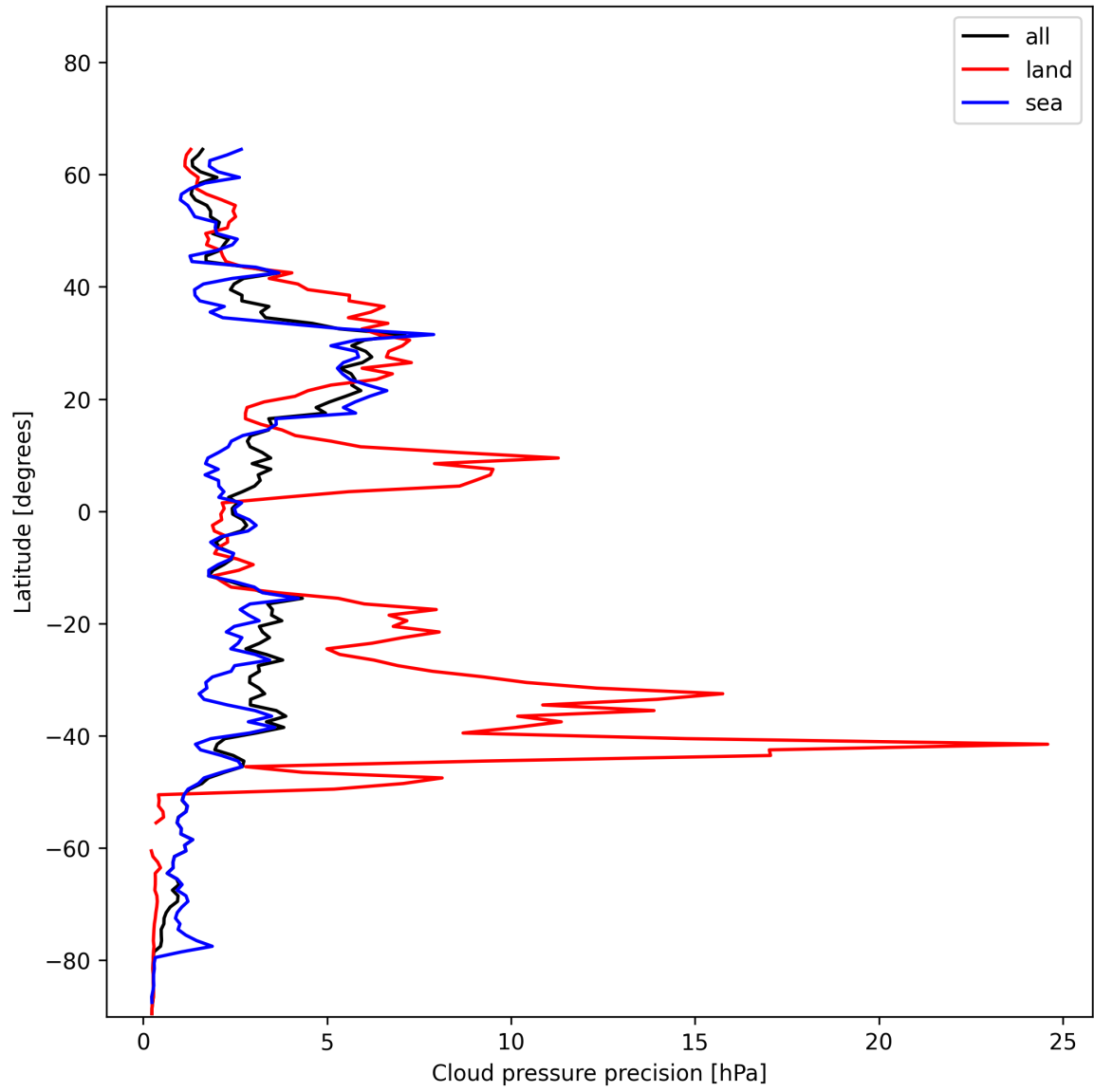
Figure 14: Zonal average of “Cloud pressure precision” for 2024-12-24 to 2024-12-26.
