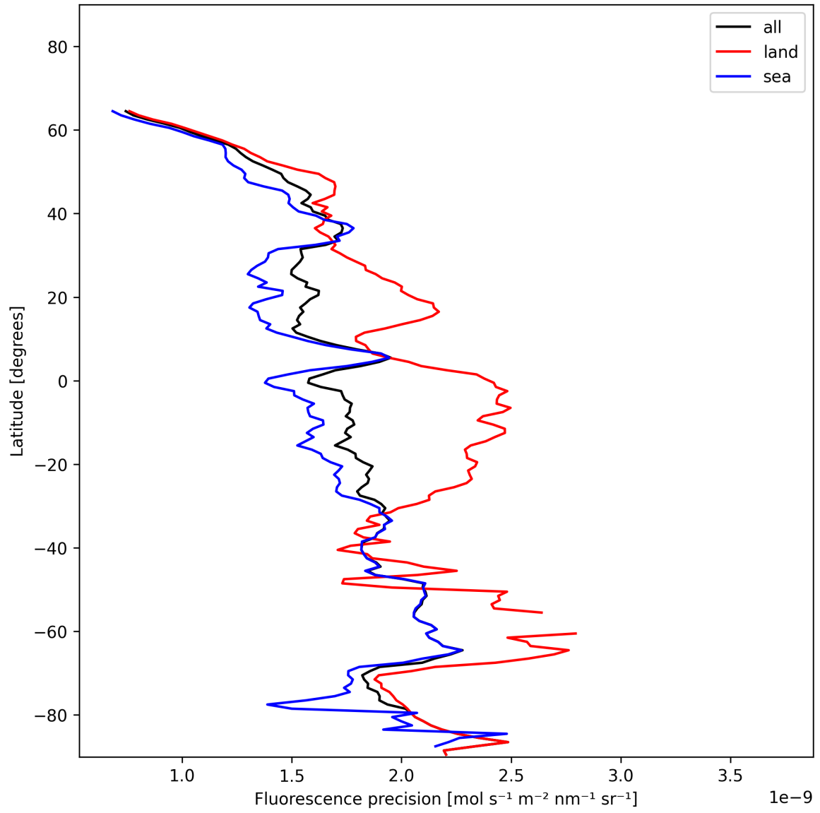
Figure 24: Zonal average of “Fluorescence precision” for 2024-12-24 to 2024-12-26.
