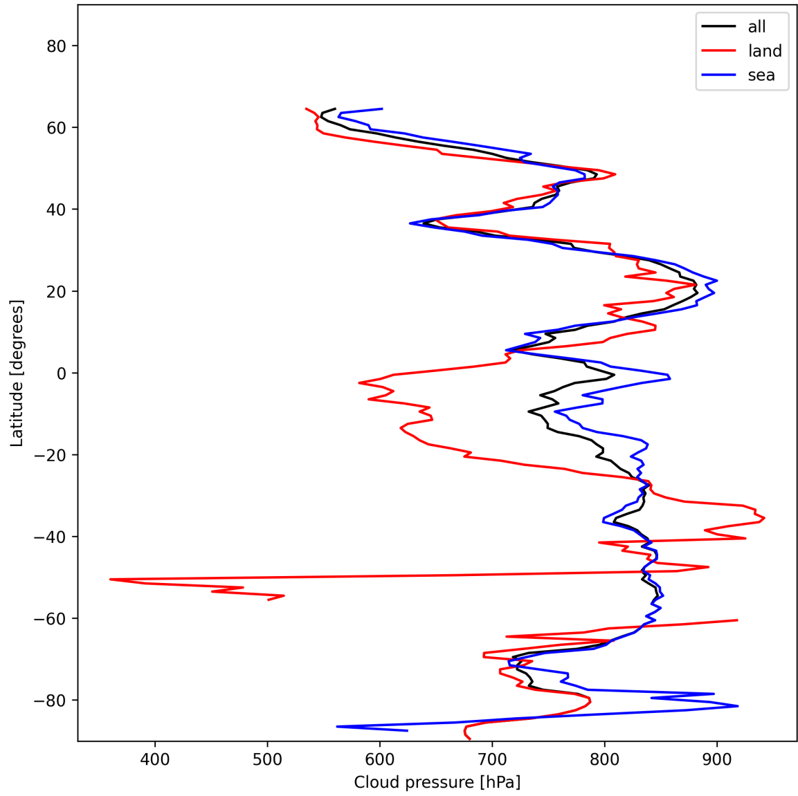
Figure 13: Zonal average of “Cloud pressure” for 2024-12-24 to 2024-12-26.
