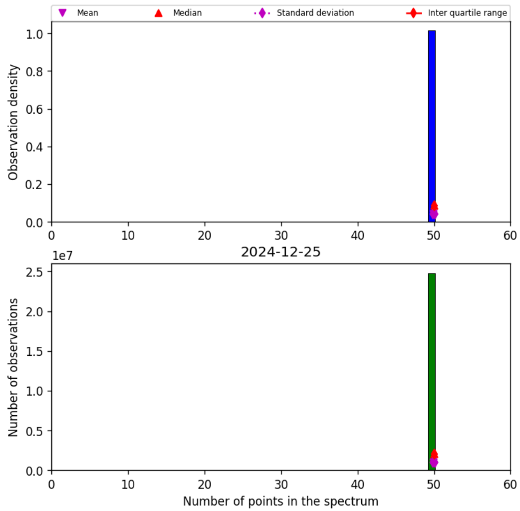
Figure 44: Histogram of “Number of points in the spectrum” for 2024-12-24 to 2024-12-26
