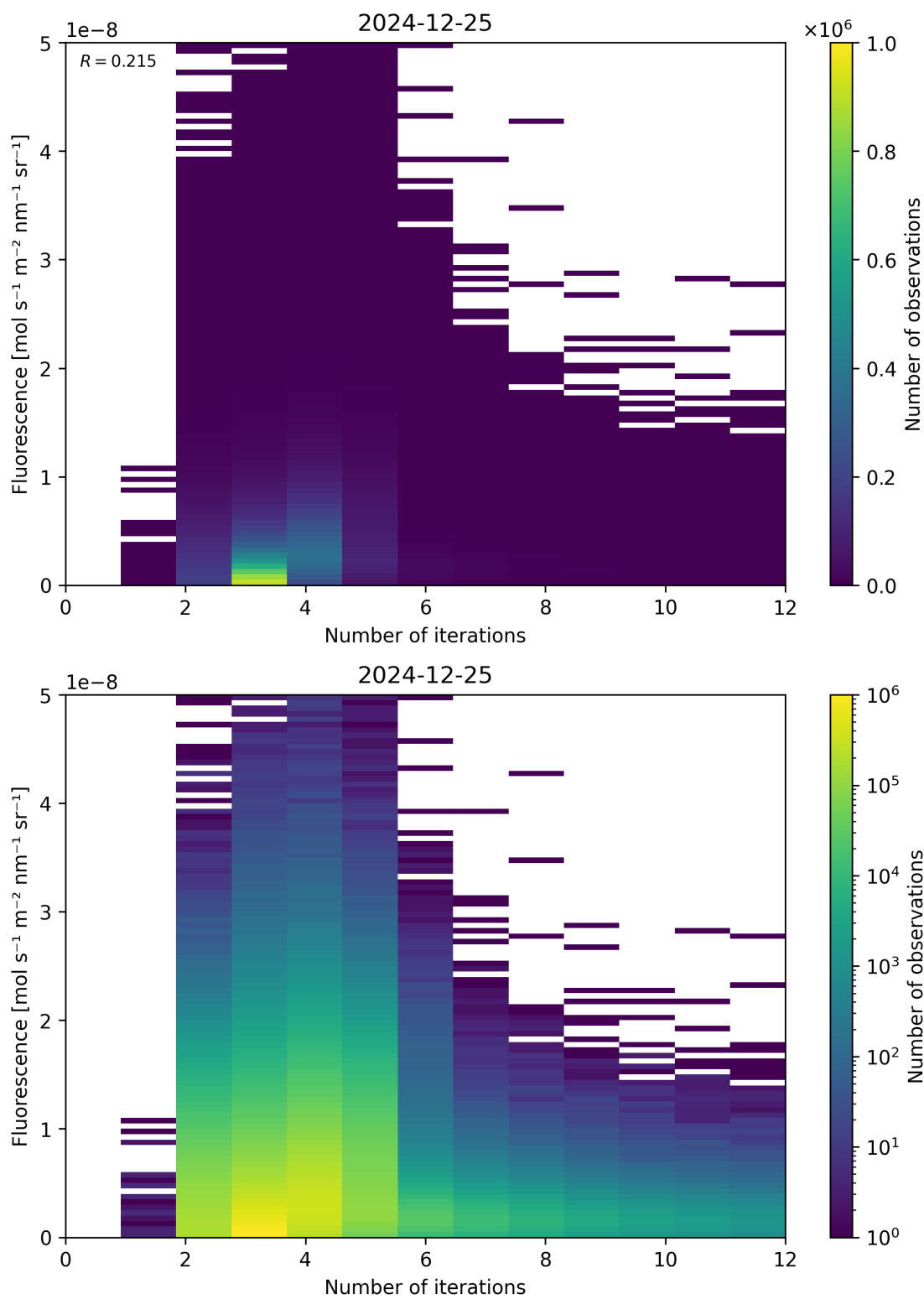
Figure 98: Scatter density plot of “Number of iterations” against “Fluorescence” for 2024-12-24 to 2024-12-26.
