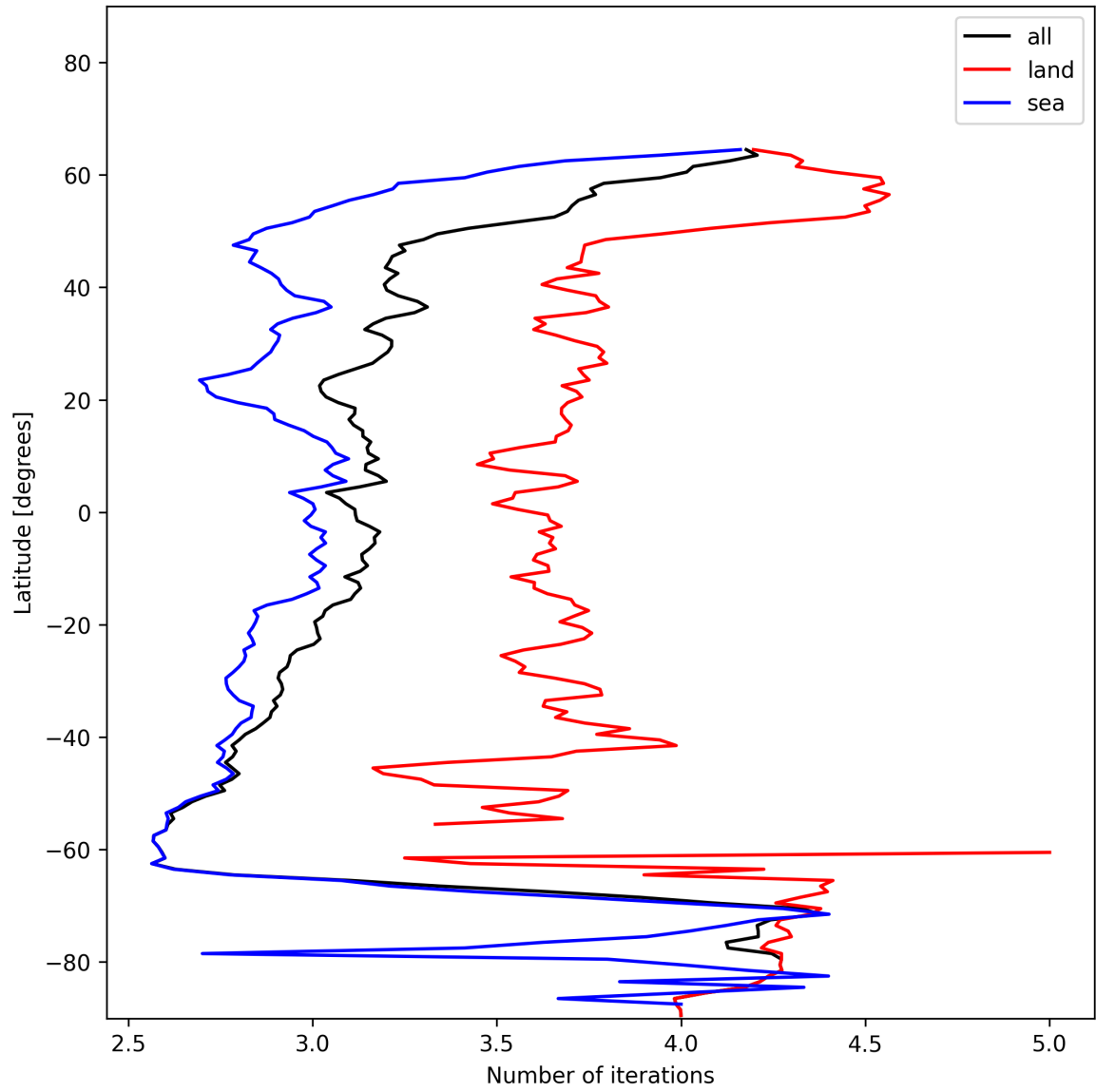
Figure 22: Zonal average of “Number of iterations” for 2024-12-24 to 2024-12-26.
