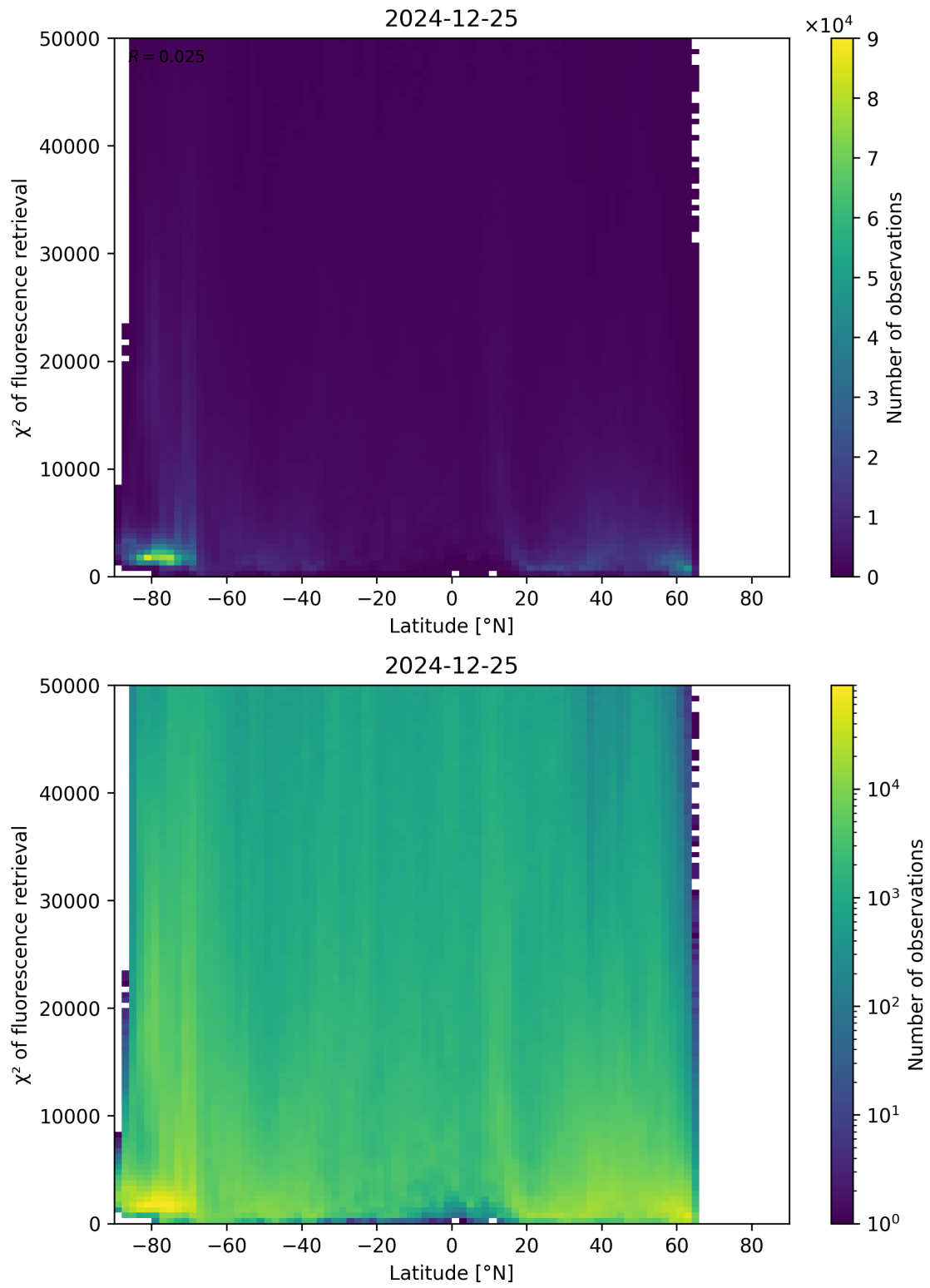
Figure 89: Scatter density plot of “Latitude” against “ \chi^2 of fluorescence retrieval” for 2024-12-24 to 2024-12-26.
