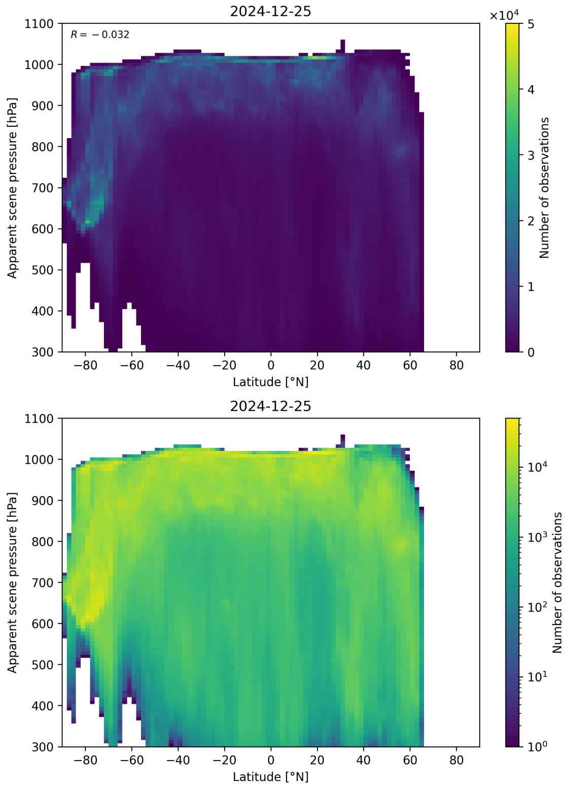
Figure 88: Scatter density plot of “Latitude” against “Apparent scene pressure” for 2024-12-24 to 2024-12-26.
