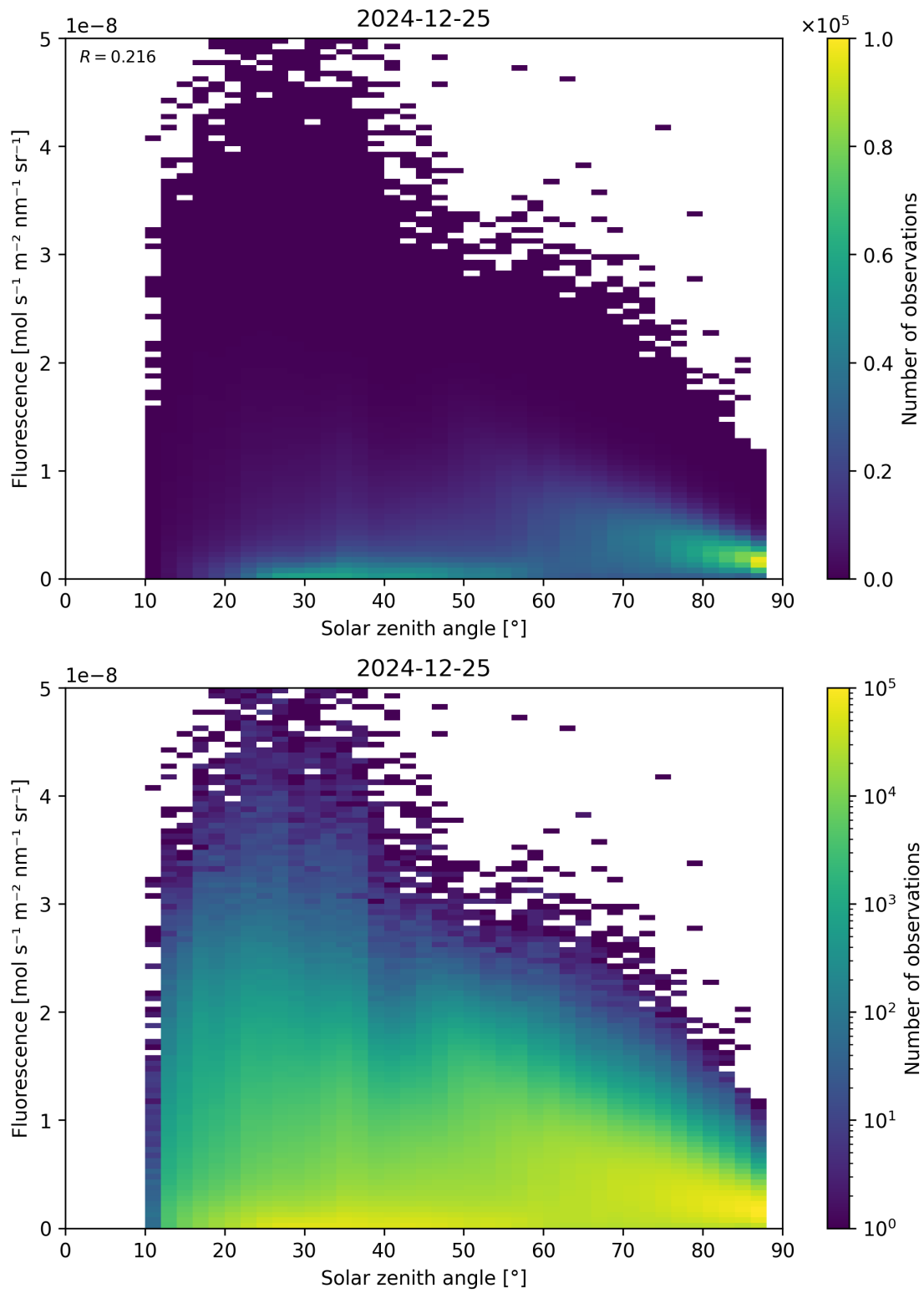
Figure 112: Scatter density plot of “Solar zenith angle” against “Fluorescence” for 2024-12-24 to 2024-12-26.
