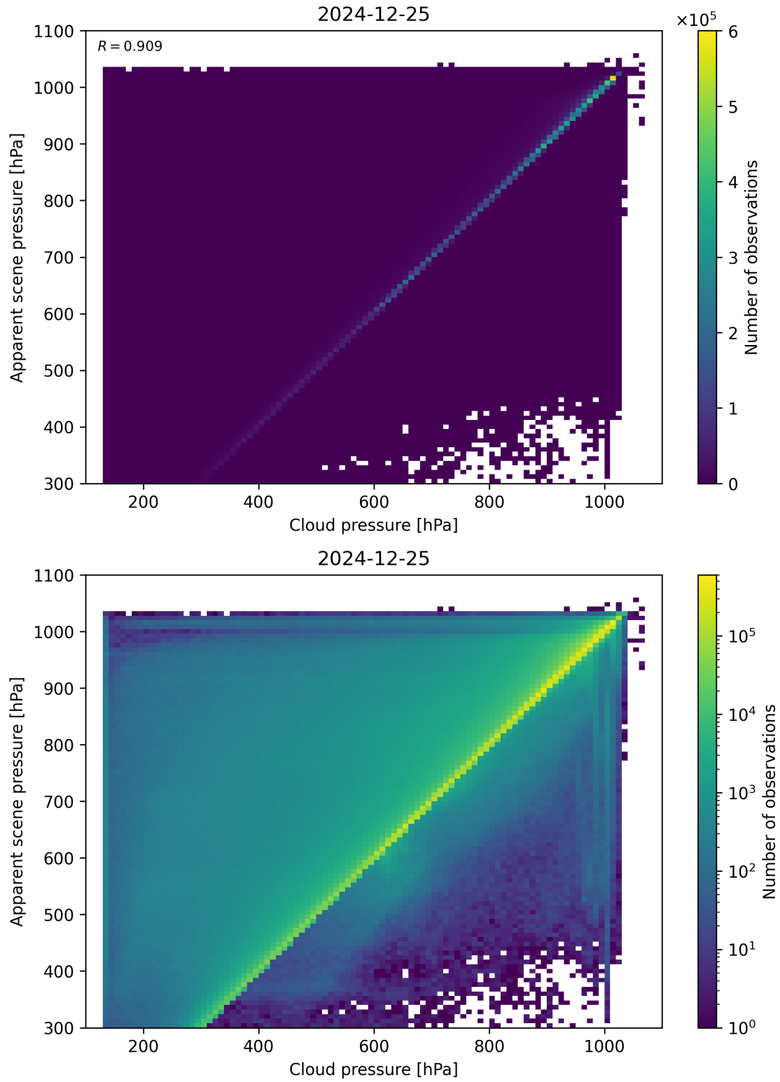
Figure 77: Scatter density plot of “Cloud pressure” against “Apparent scene pressure” for 2024-12-24 to 2024-12-26.
