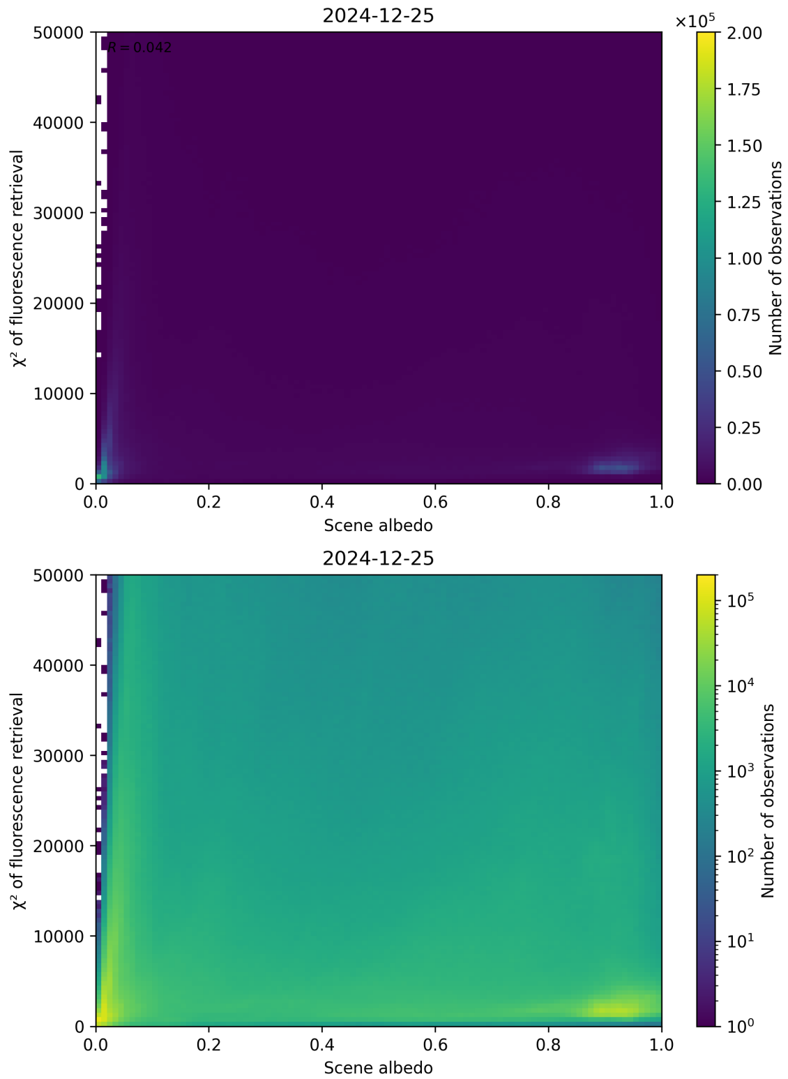
Figure 103: Scatter density plot of “Scene albedo” against “ \chi^2 of fluorescence retrieval” for 2024-12-24 to 2024-12-26.
