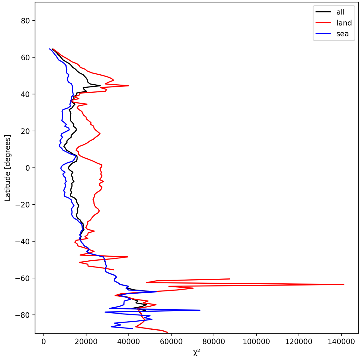
Figure 21: Zonal average of “ \chi^2 ” for 2024-12-24 to 2024-12-26.
