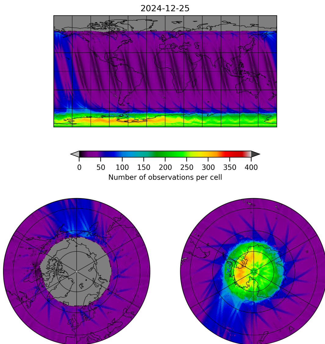
Figure 11: Map of the number of observations for 2024-12-24 to 2024-12-26
