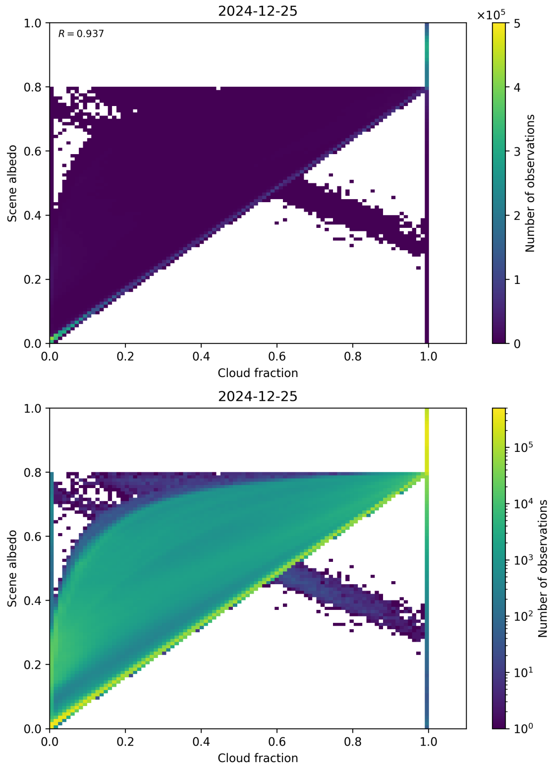
Figure 75: Scatter density plot of “Cloud fraction” against “Scene albedo” for 2024-12-24 to 2024-12-26.
