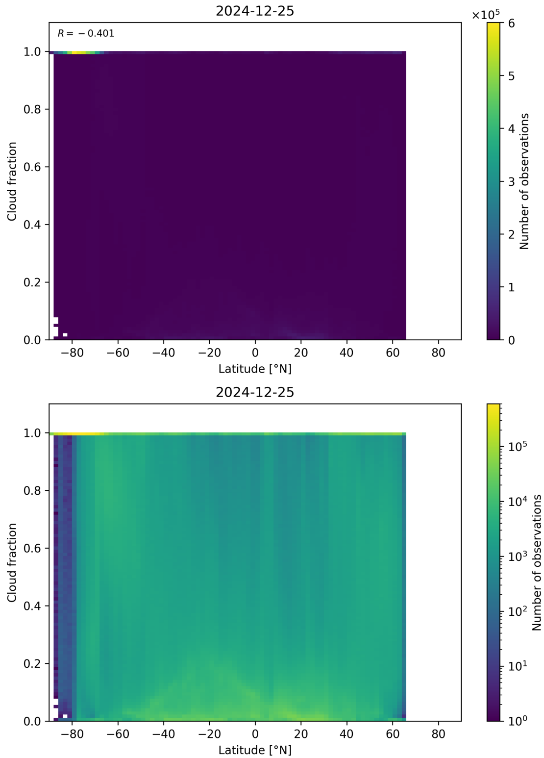
Figure 90: Scatter density plot of “Latitude” against “Cloud fraction” for 2024-12-24 to 2024-12-26.
