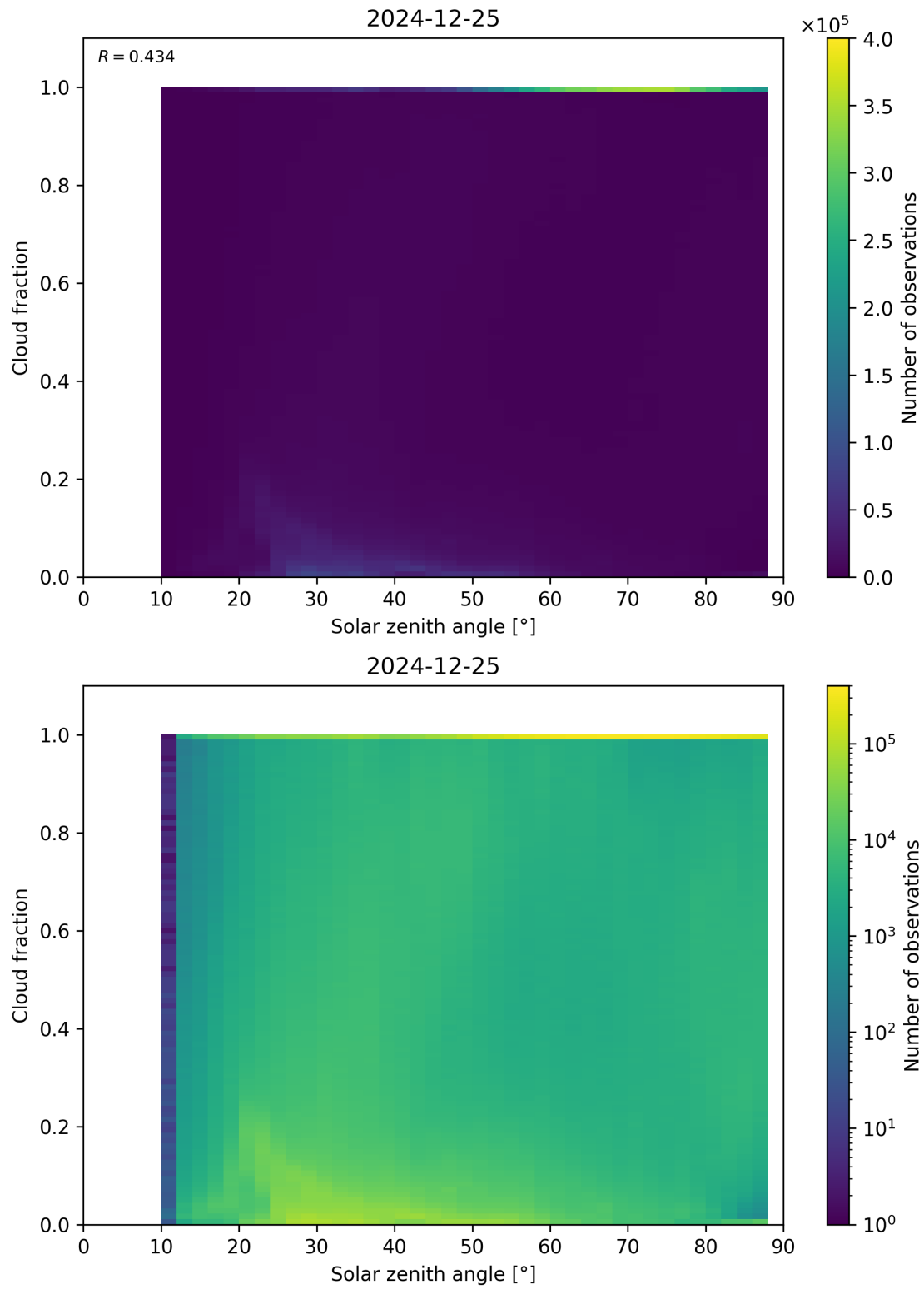
Figure 110: Scatter density plot of “Solar zenith angle” against “Cloud fraction” for 2024-12-24 to 2024-12-26.
