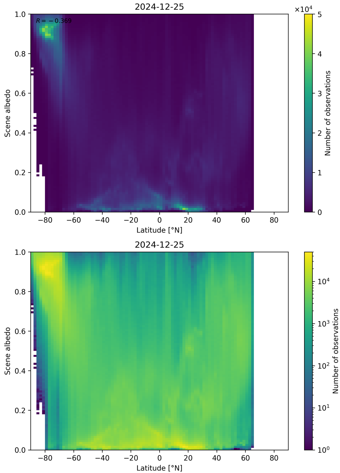
Figure 95: Scatter density plot of “Latitude” against “Scene albedo” for 2024-12-24 to 2024-12-26.
