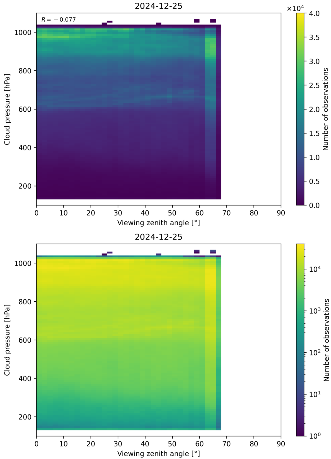
Figure 121: Scatter density plot of “Viewing zenith angle” against “Cloud pressure” for 2024-12-24 to 2024-12-26.
