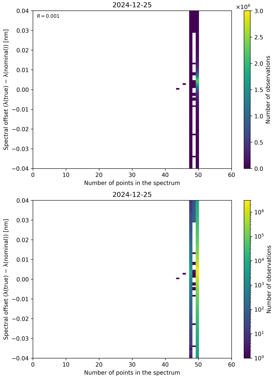
Figure 101: Scatter density plot of “Number of points in the spectrum” against “Spectral offset ( \lambda_{\text{true}} - \lambda_{\text{nominal}} )” for 2024-12-24 to 2024-12-26.
