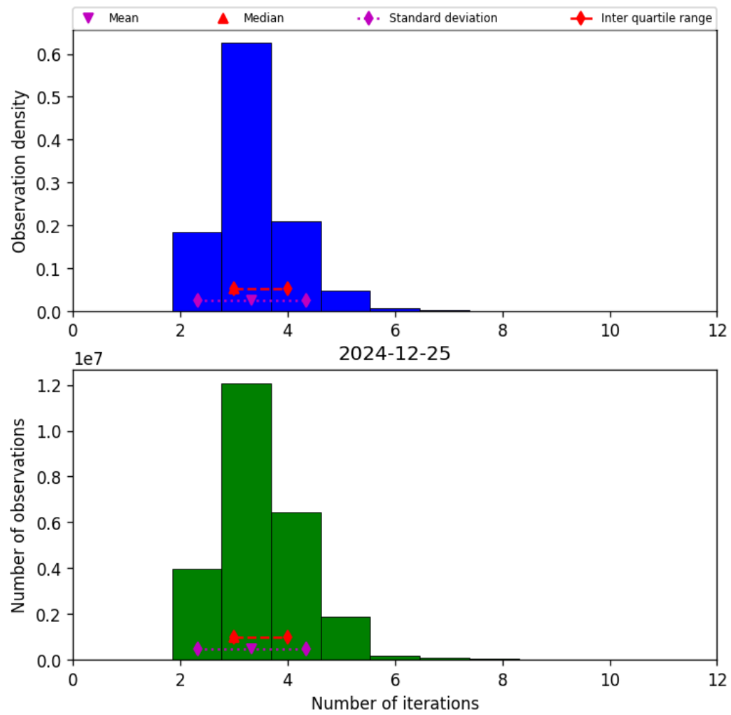
Figure 39: Histogram of “Number of iterations” for 2024-12-24 to 2024-12-26
