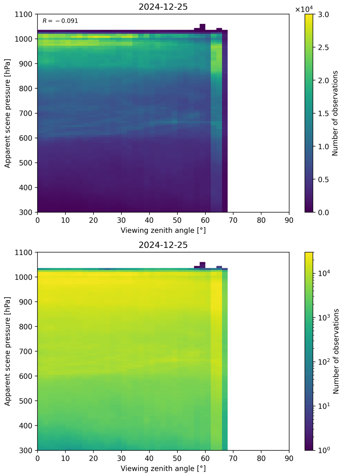
Figure 118: Scatter density plot of “Viewing zenith angle” against “Apparent scene pressure” for 2024-12-24 to 2024-12-26.
