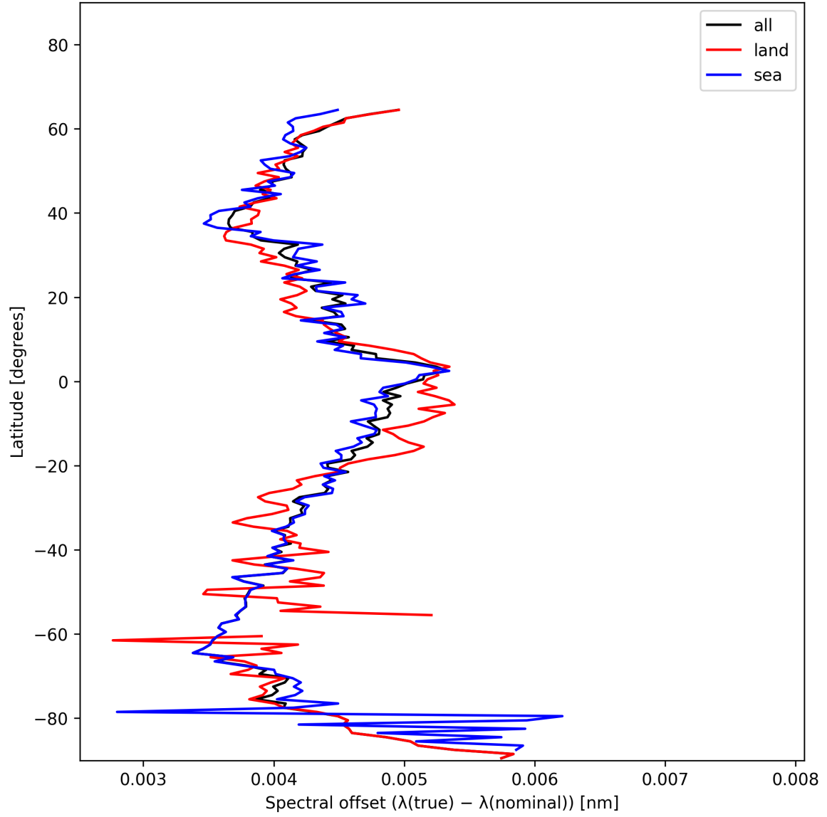
Figure 28: Zonal average of “Spectral offset ( \lambda_{\text{true}} - \lambda_{\text{nominal}} )” for 2024-12-24 to 2024-12-26.
