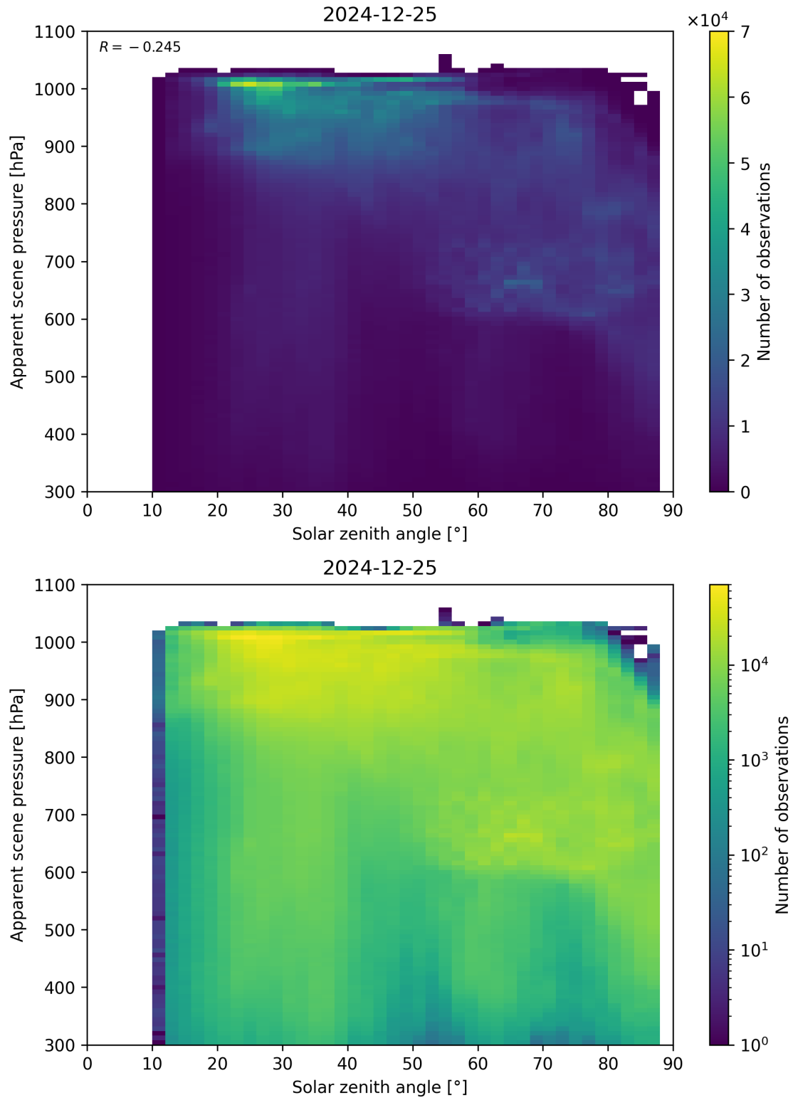
Figure 108: Scatter density plot of “Solar zenith angle” against “Apparent scene pressure” for 2024-12-24 to 2024-12-26.
