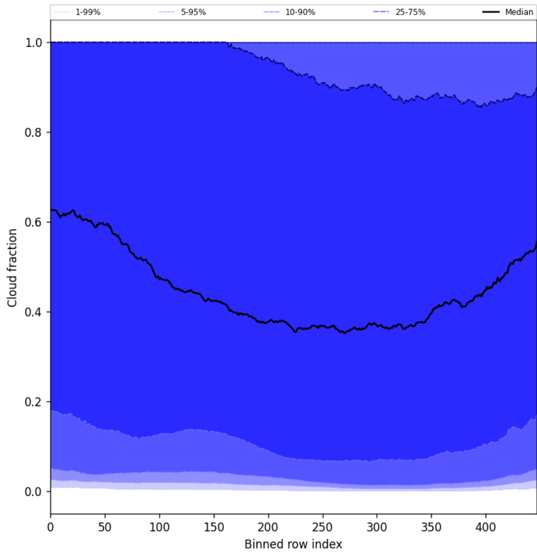
Figure 49: Along track statistics of “Cloud fraction” for 2024-12-24 to 2024-12-26
