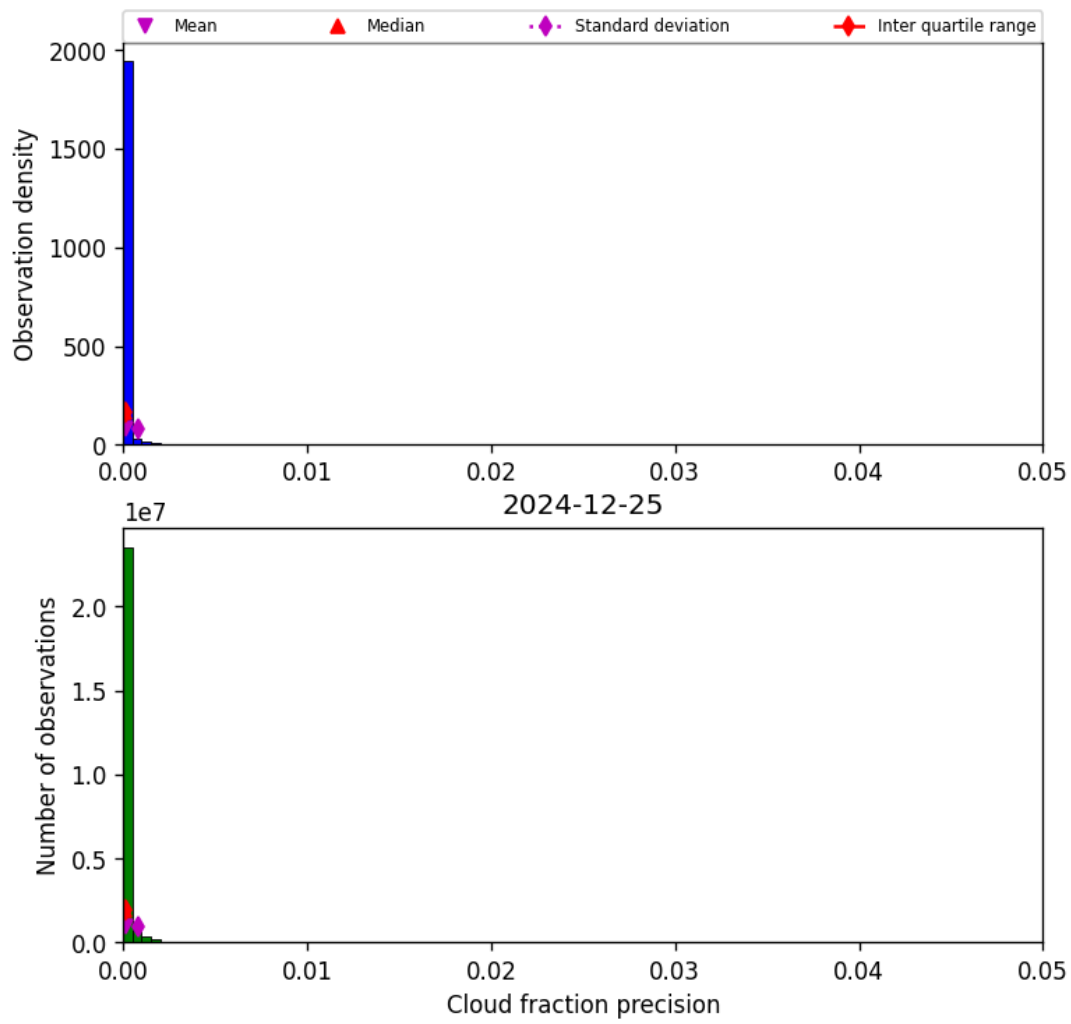
Figure 33: Histogram of “Cloud fraction precision” for 2024-12-24 to 2024-12-26
