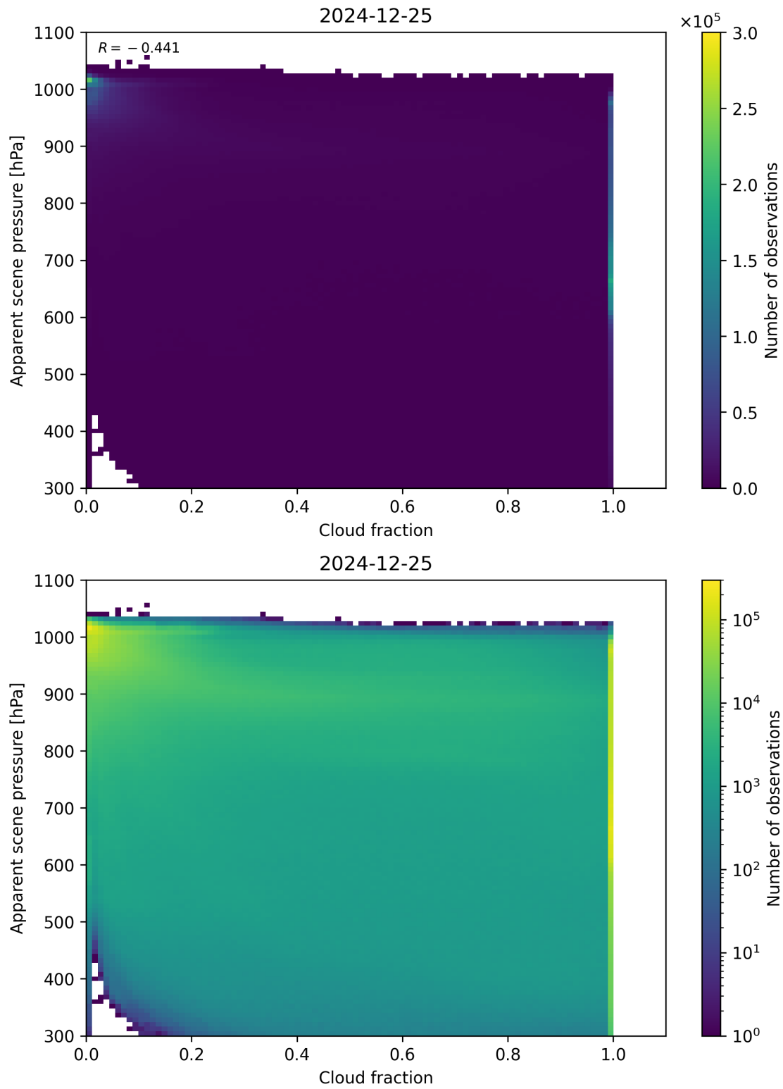
Figure 70: Scatter density plot of “Cloud fraction” against “Apparent scene pressure” for 2024-12-24 to 2024-12-26.
