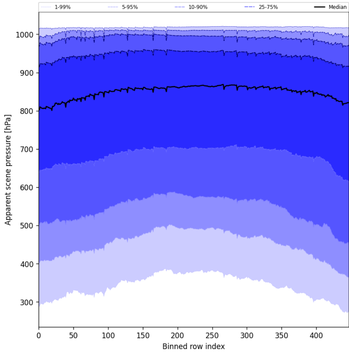
Figure 53: Along track statistics of “Apparent scene pressure” for 2024-12-24 to 2024-12-26
