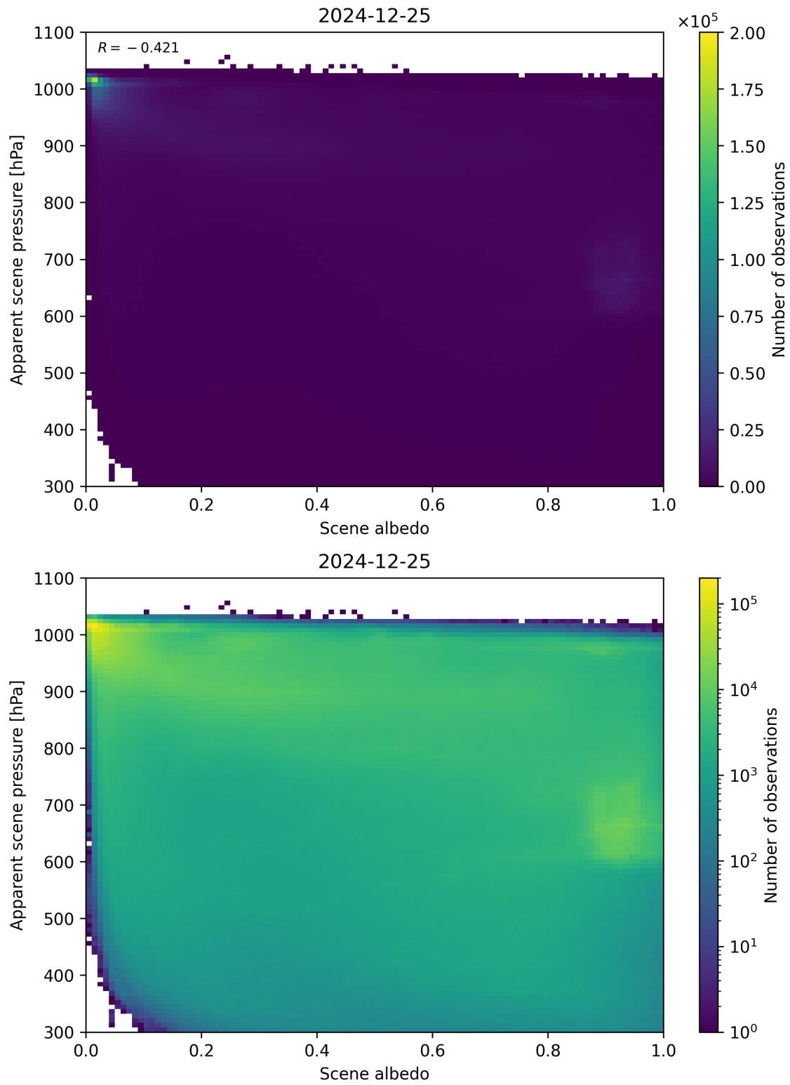
Figure 102: Scatter density plot of “Scene albedo” against “Apparent scene pressure” for 2024-12-24 to 2024-12-26.
