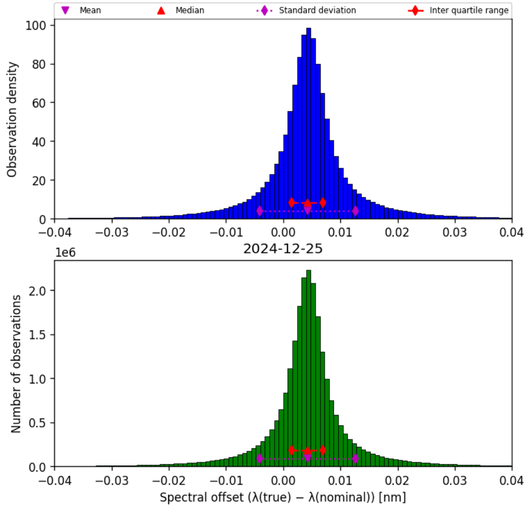
Figure 45: Histogram of “Spectral offset ( \lambda_{\text{true}} - \lambda_{\text{nominal}} )” for 2024-12-24 to 2024-12-26
