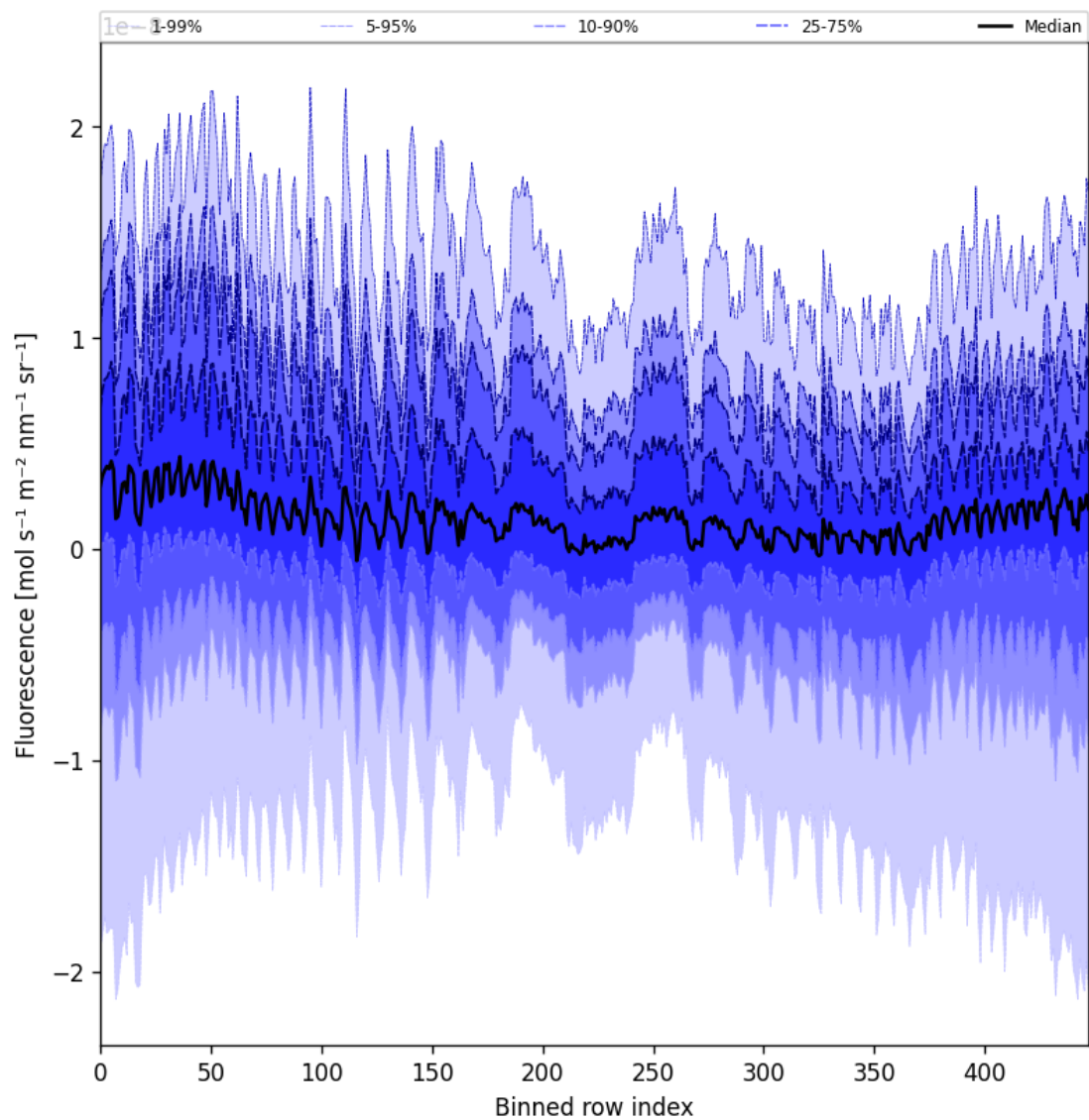
Figure 57: Along track statistics of “Fluorescence” for 2024-12-24 to 2024-12-26
