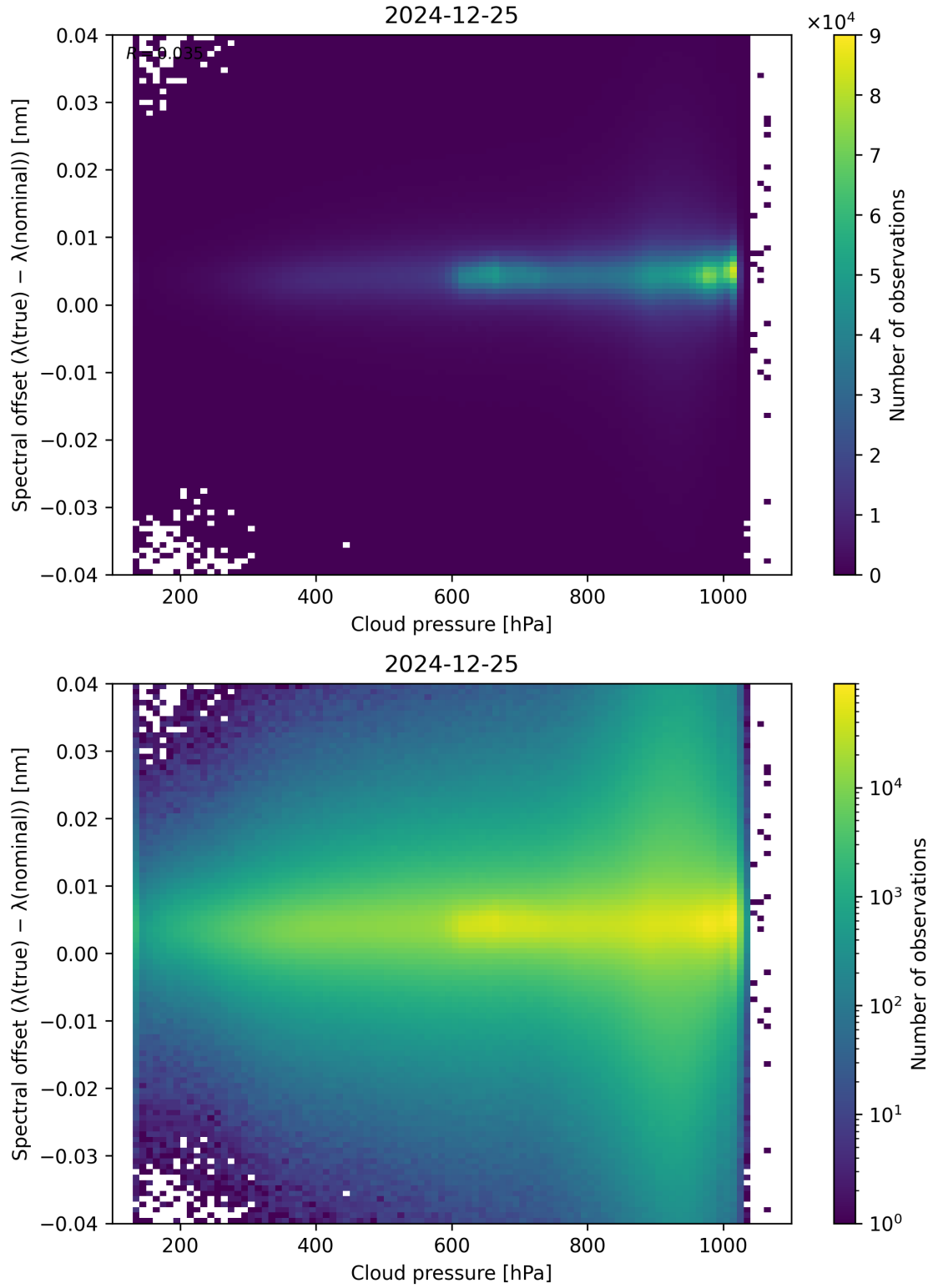
Figure 84: Scatter density plot of “Cloud pressure” against “Spectral offset ( \lambda_{\text{true}} - \lambda_{\text{nominal}} )” for 2024-12-24 to 2024-12-26.
