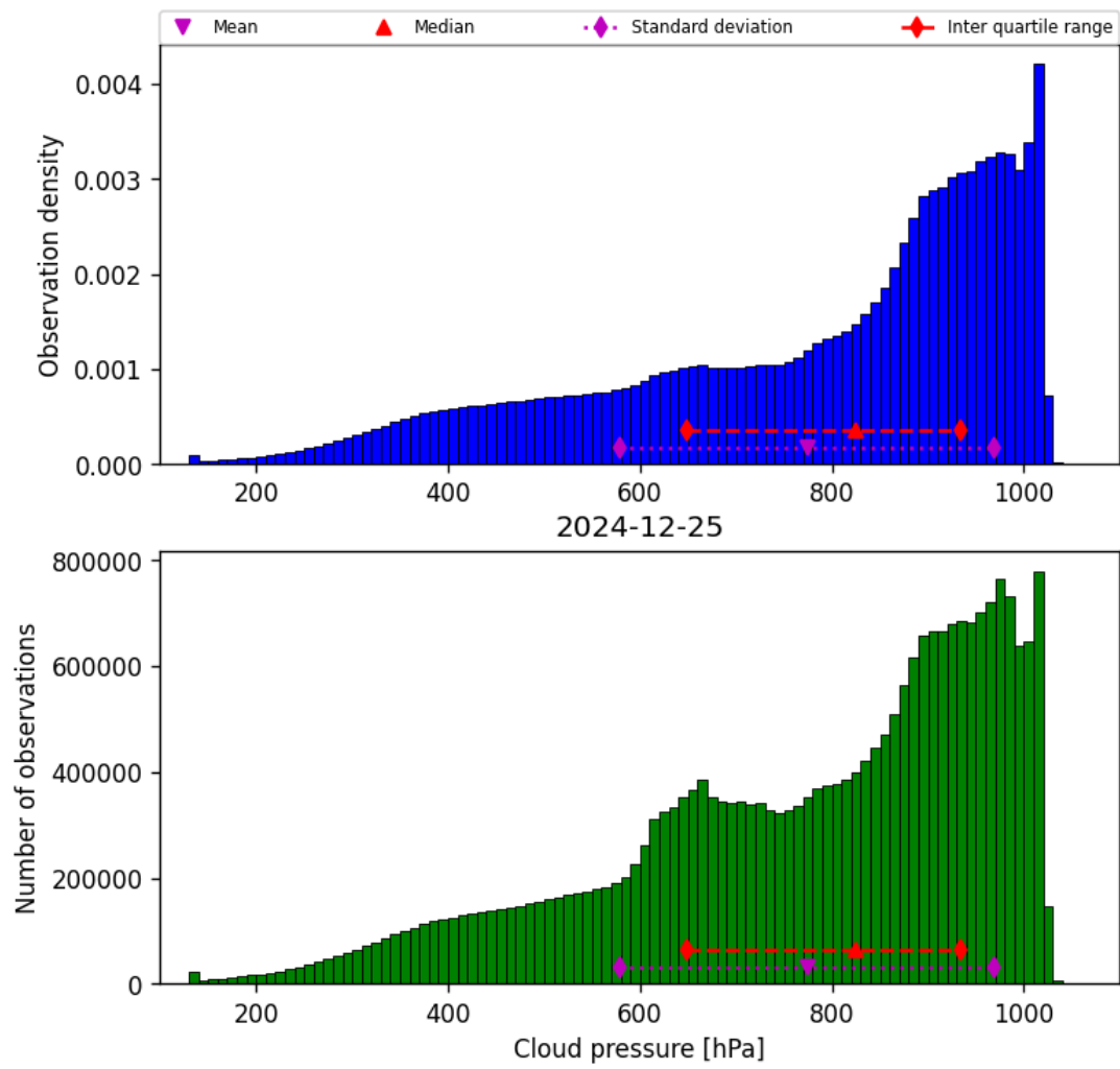
Figure 30: Histogram of “Cloud pressure” for 2024-12-24 to 2024-12-26
