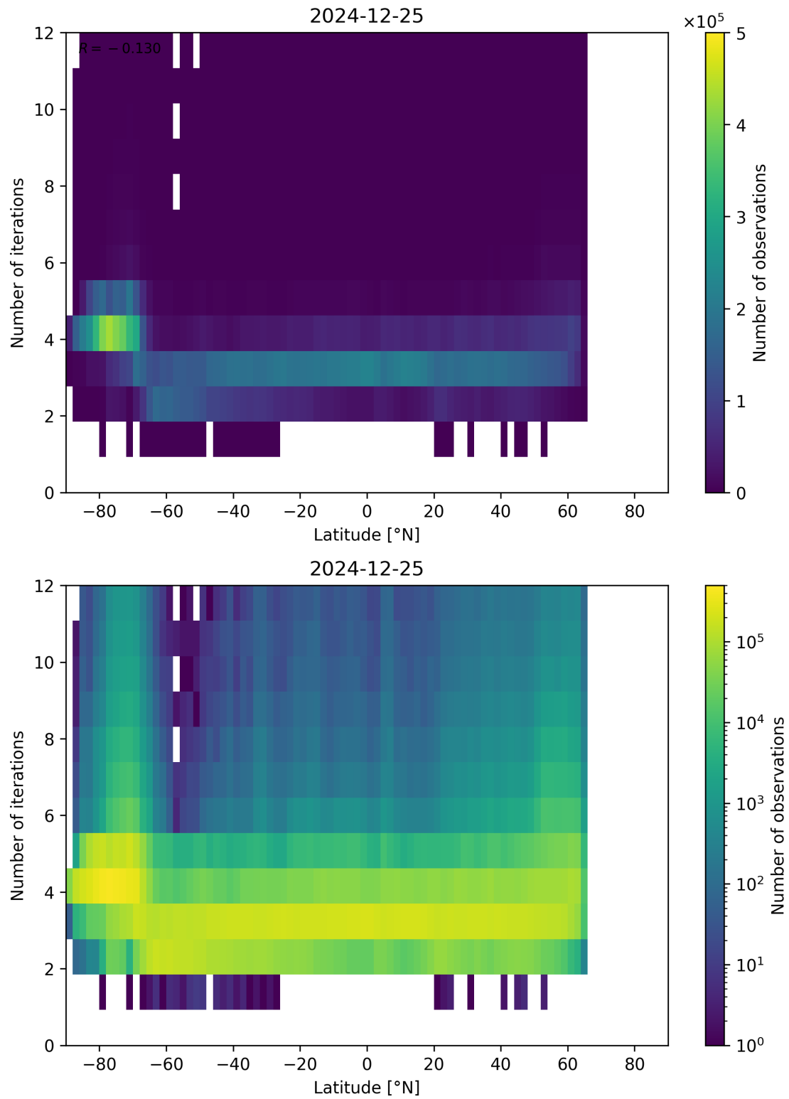
Figure 93: Scatter density plot of “Latitude” against “Number of iterations” for 2024-12-24 to 2024-12-26.
