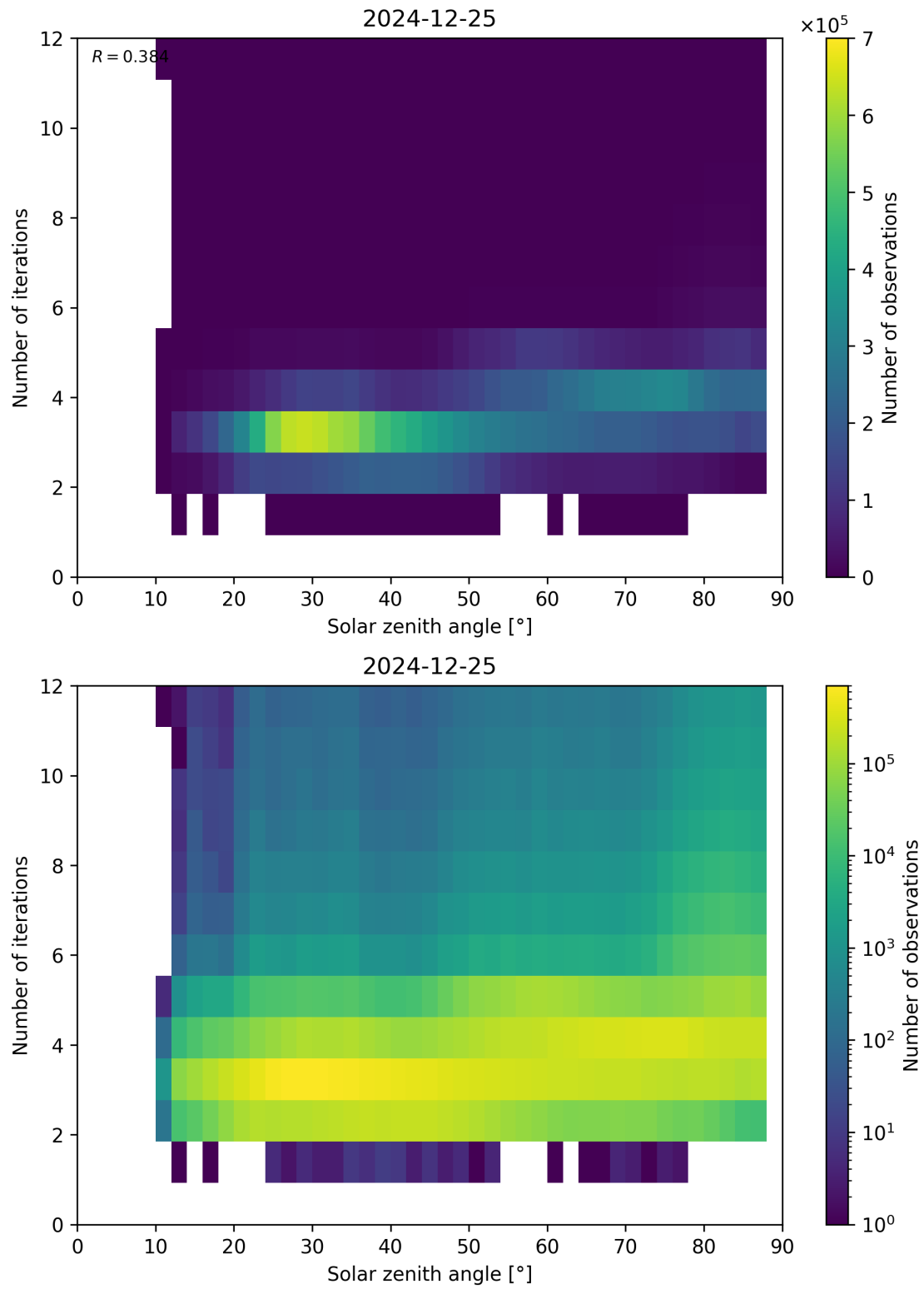
Figure 114: Scatter density plot of “Solar zenith angle” against “Number of iterations” for 2024-12-24 to 2024-12-26.
