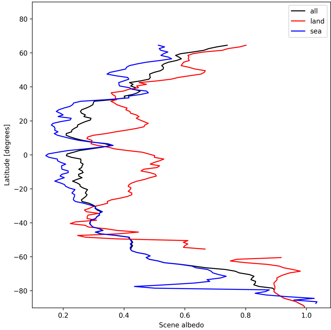
Figure 17: Zonal average of “Scene albedo” for 2024-12-24 to 2024-12-26.
