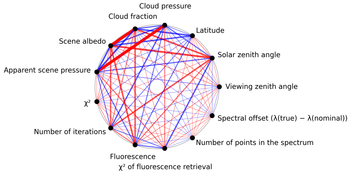
Figure 1: Map of correlation graph for 2024-12-24 to 2024-12-26.
