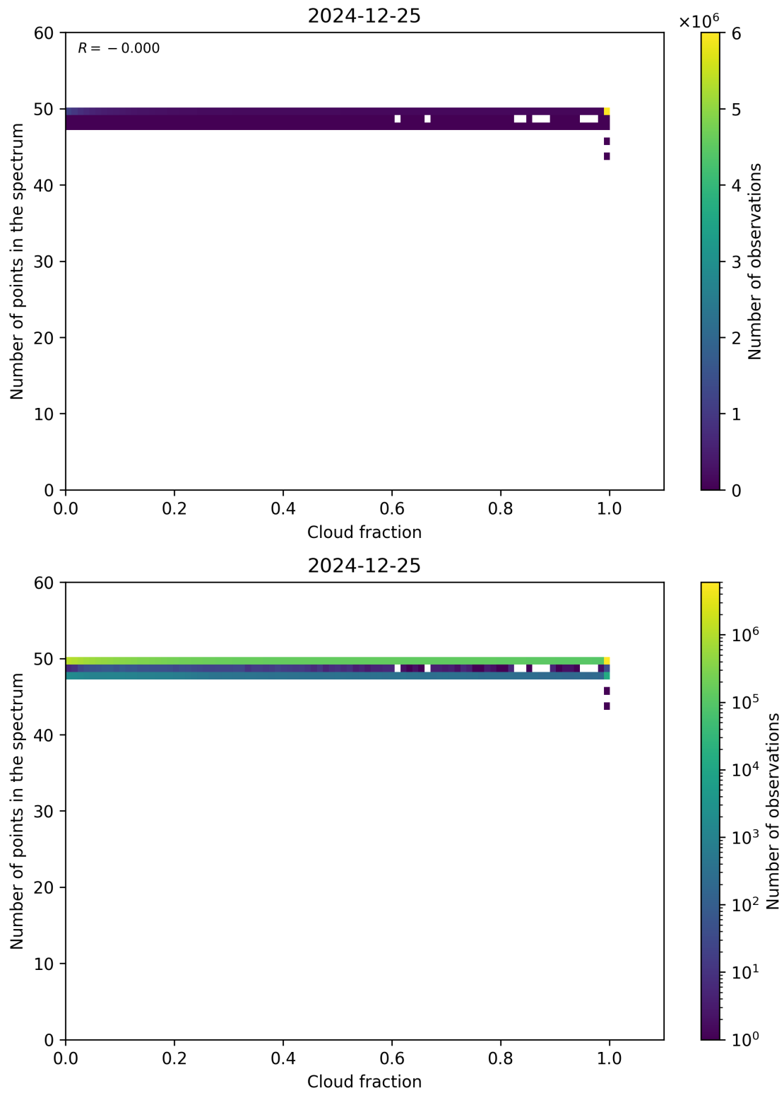
Figure 74: Scatter density plot of “Cloud fraction” against “Number of points in the spectrum” for 2024-12-24 to 2024-12-26.
