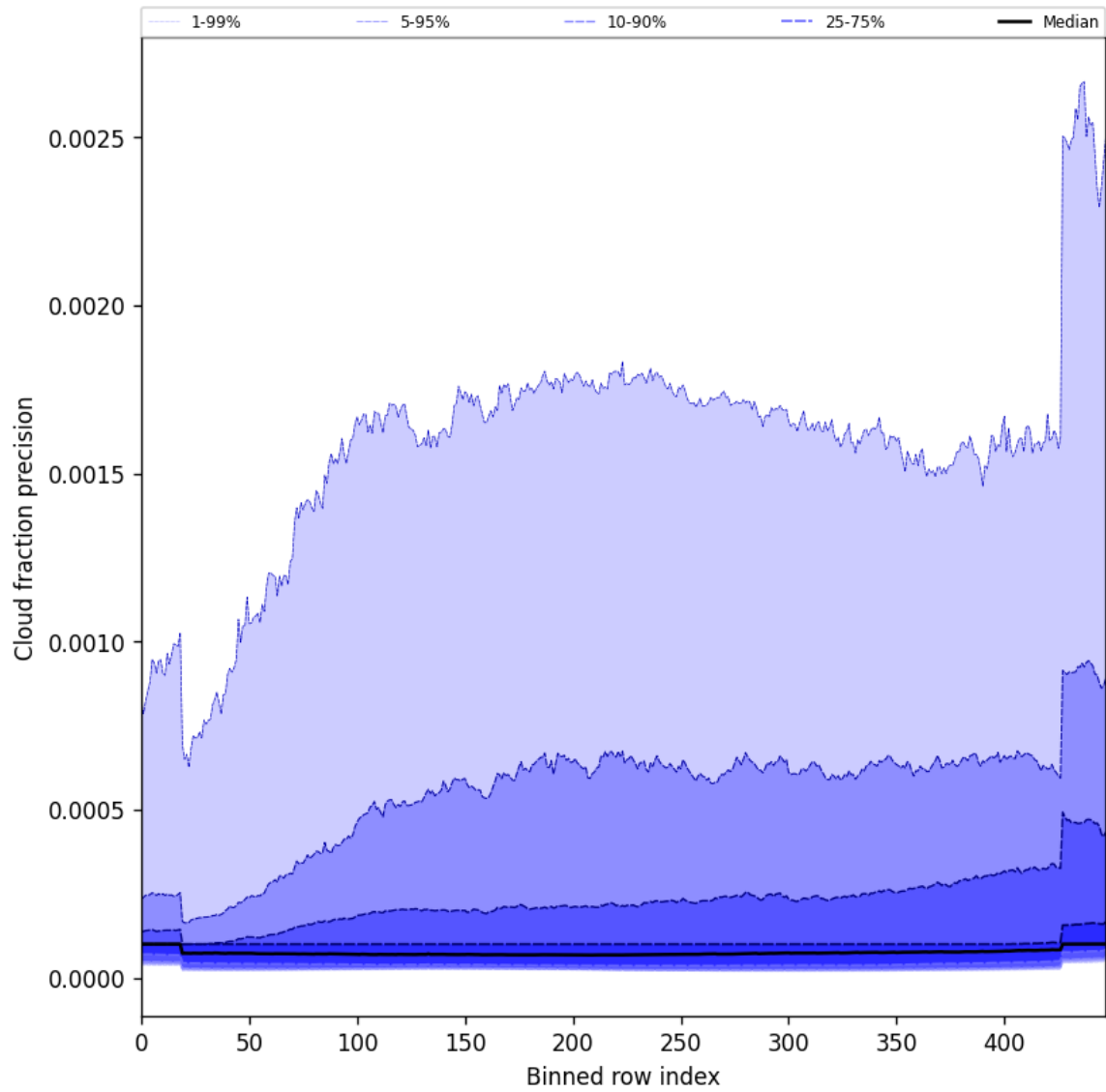
Figure 50: Along track statistics of “Cloud fraction precision” for 2024-12-24 to 2024-12-26
