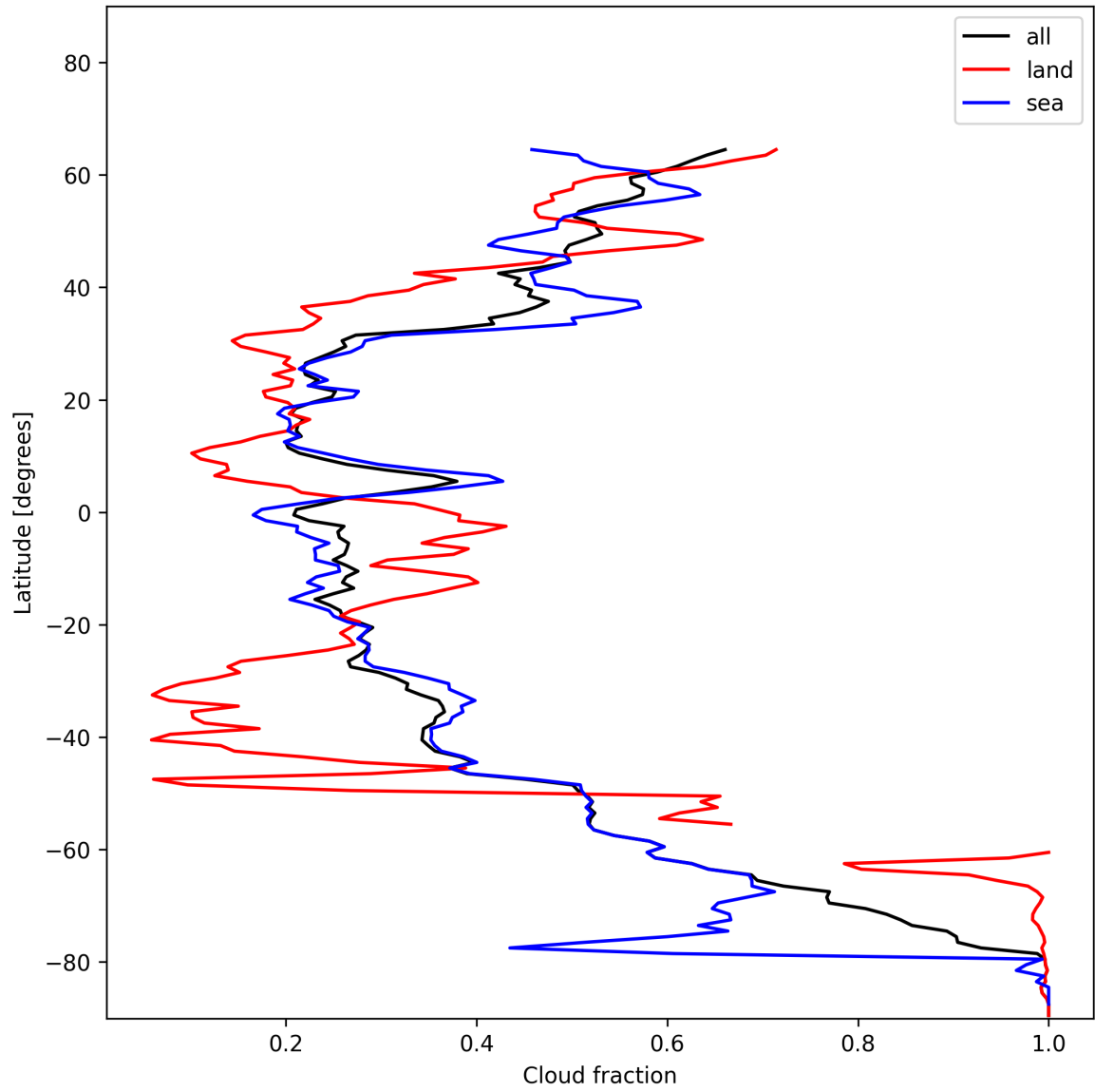
Figure 15: Zonal average of “Cloud fraction” for 2024-12-24 to 2024-12-26.
