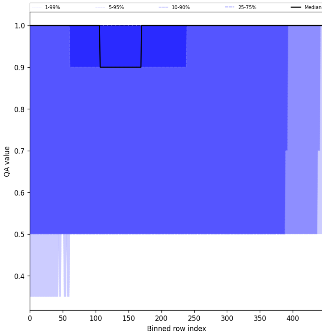
Figure 46: Along track statistics of “QA value” for 2024-12-24 to 2024-12-26
