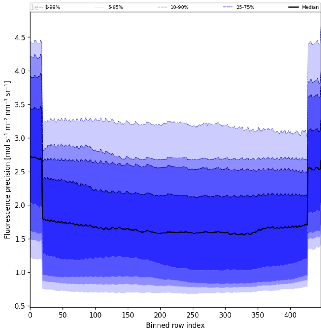
Figure 58: Along track statistics of “Fluorescence precision” for 2024-12-24 to 2024-12-26
