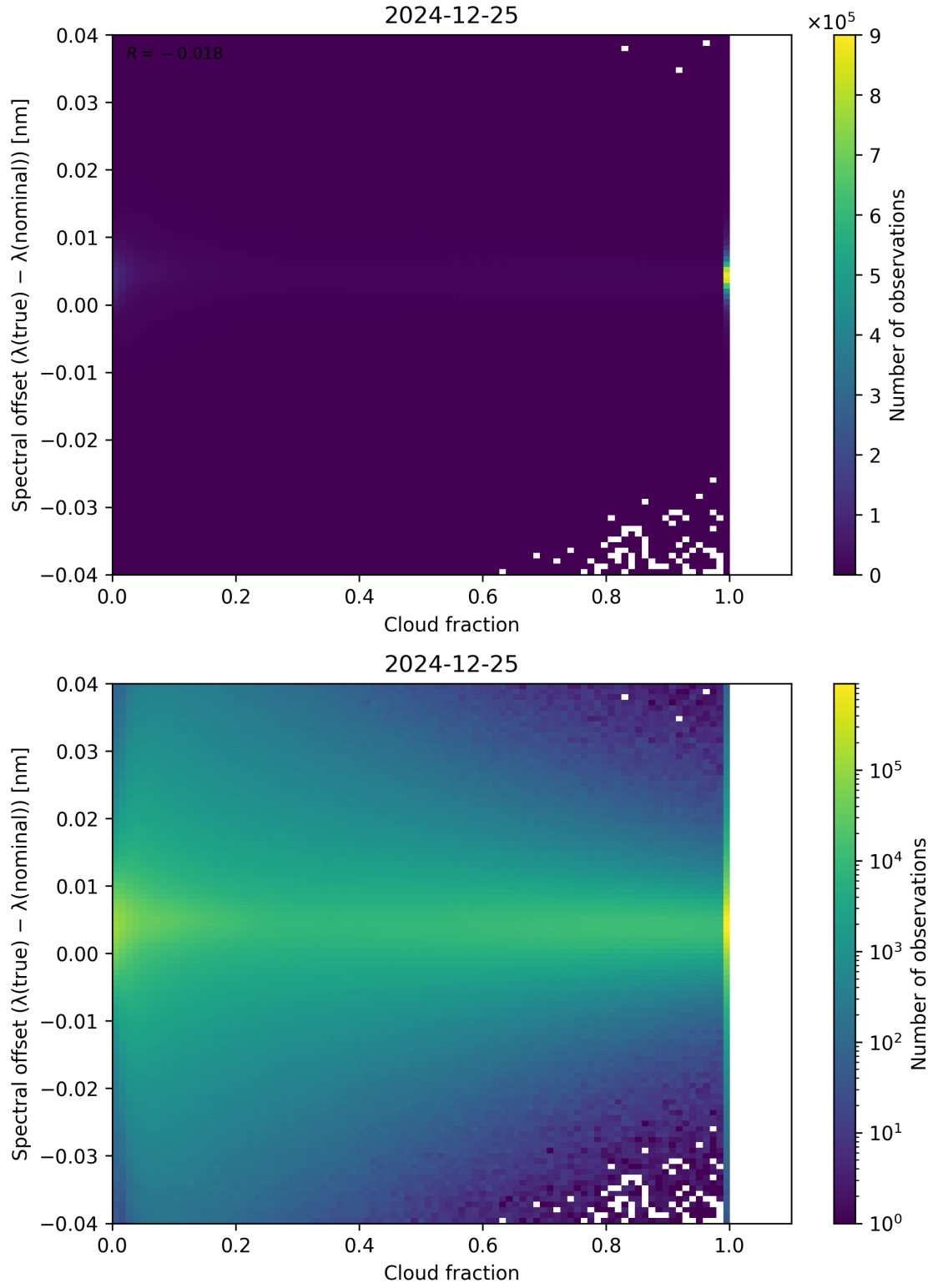
Figure 76: Scatter density plot of “Cloud fraction” against “Spectral offset ( \lambda_{\text{true}} - \lambda_{\text{nominal}} )” for 2024-12-24 to 2024-12-26.
