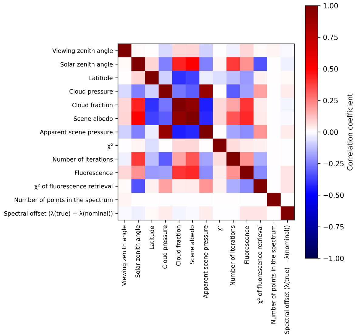
Figure 2: Map of correlation matrix for 2024-12-24 to 2024-12-26.
