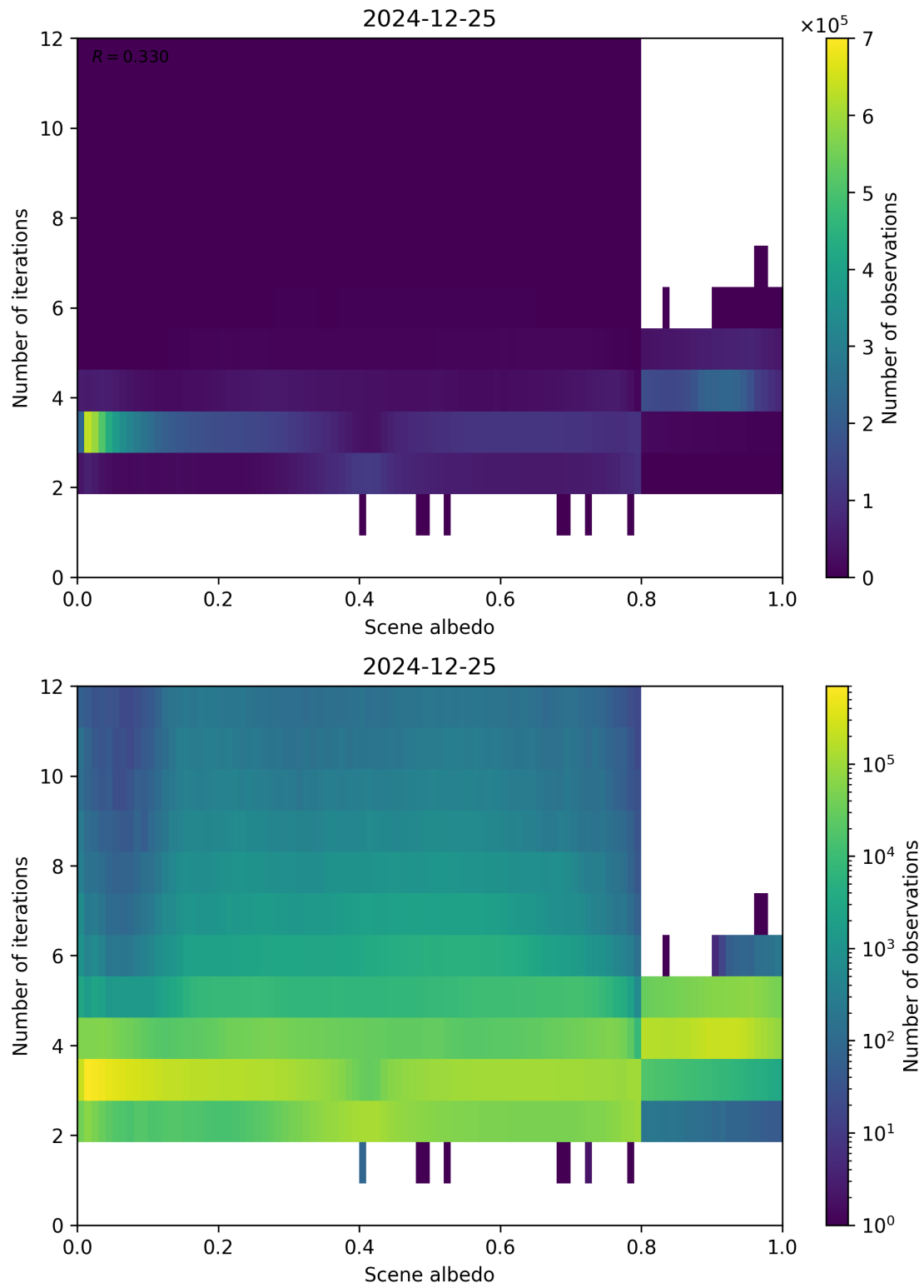
Figure 105: Scatter density plot of “Scene albedo” against “Number of iterations” for 2024-12-24 to 2024-12-26.
