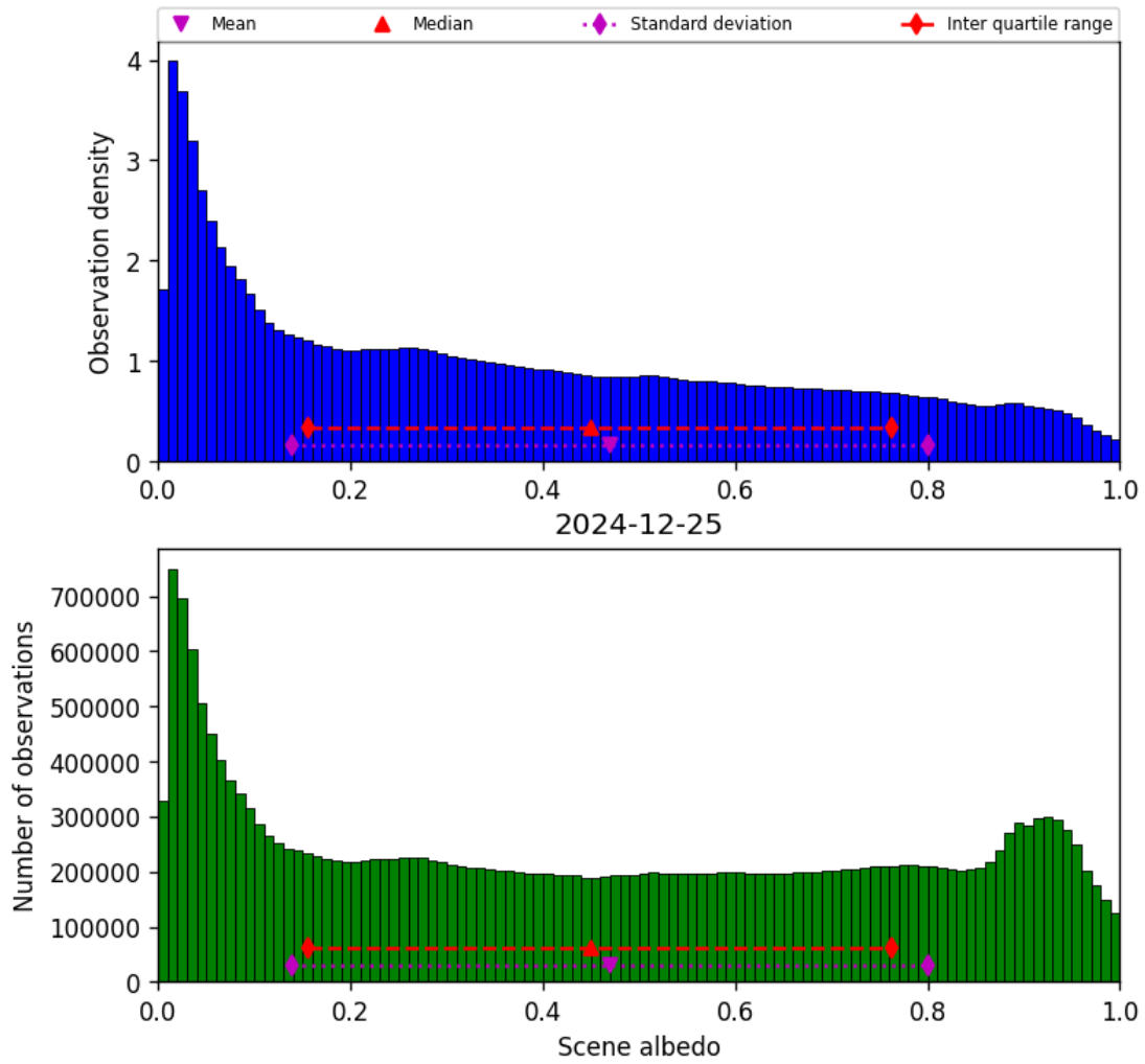
Figure 34: Histogram of “Scene albedo” for 2024-12-24 to 2024-12-26
