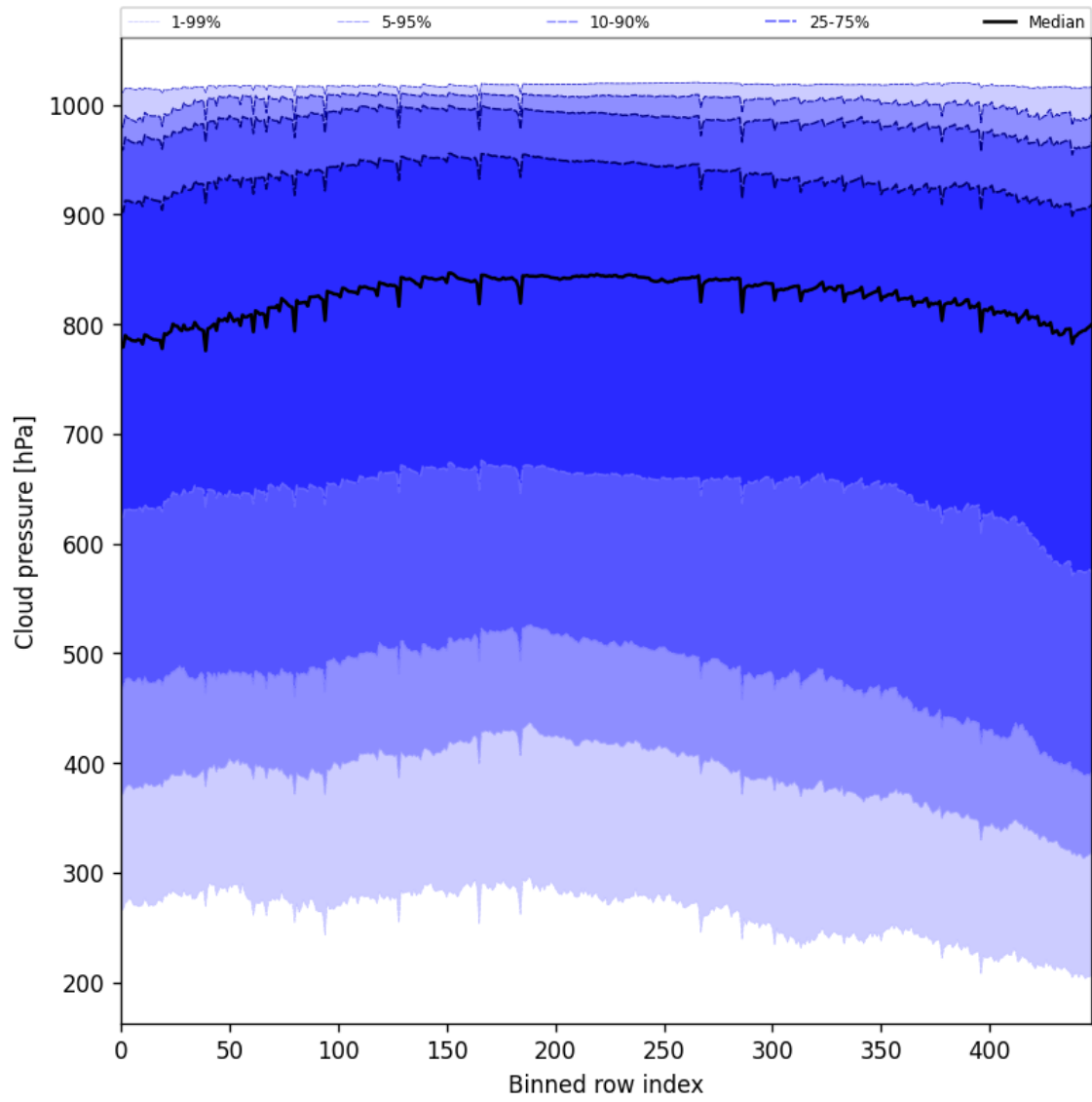
Figure 47: Along track statistics of “Cloud pressure” for 2024-12-24 to 2024-12-26
