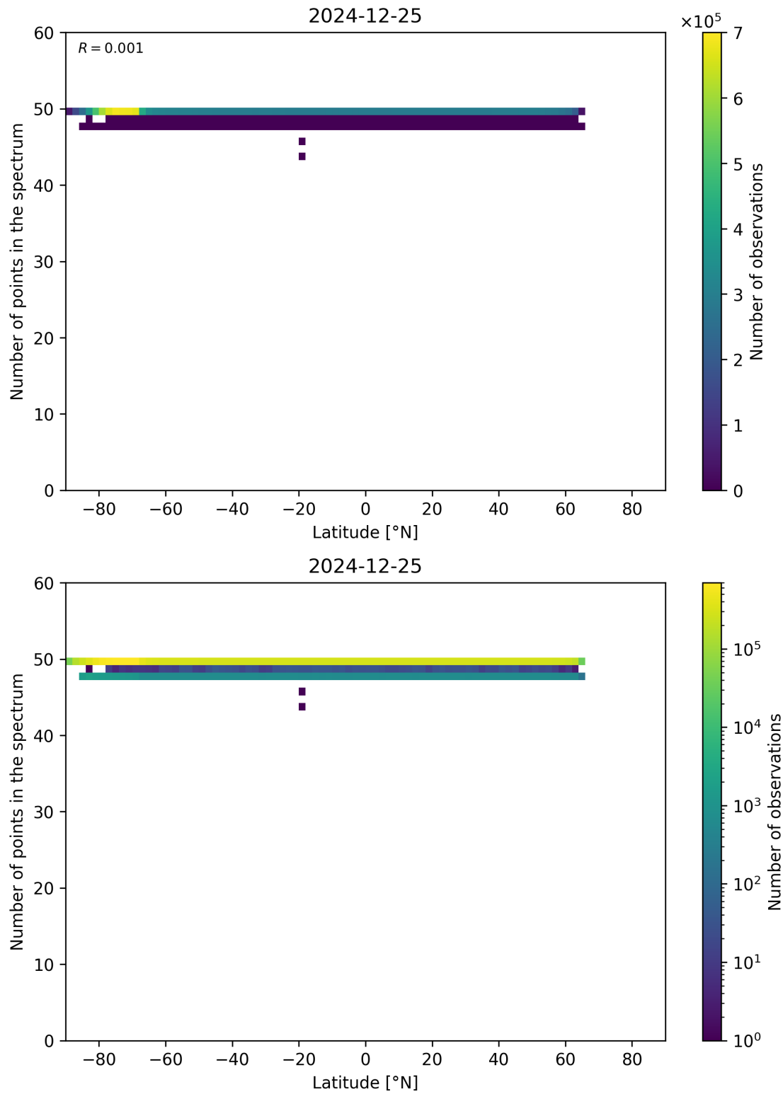
Figure 94: Scatter density plot of “Latitude” against “Number of points in the spectrum” for 2024-12-24 to 2024-12-26.
