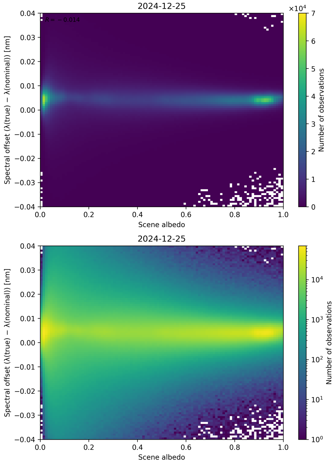
Figure 107: Scatter density plot of “Scene albedo” against “Spectral offset ( \lambda_{\text{true}} - \lambda_{\text{nominal}} )” for 2024-12-24 to 2024-12-26.
