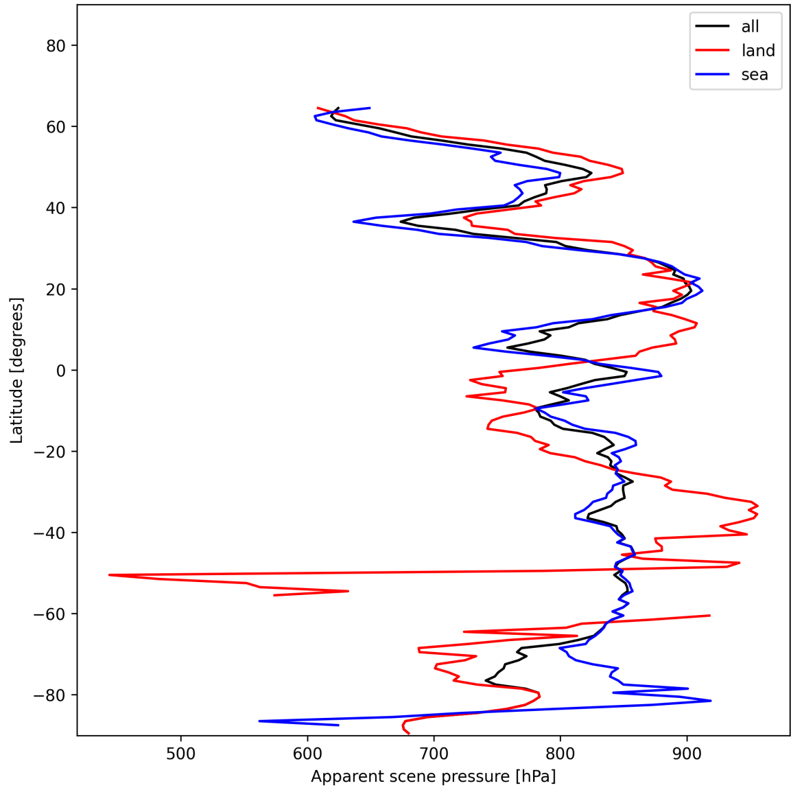
Figure 19: Zonal average of “Apparent scene pressure” for 2024-12-24 to 2024-12-26.
