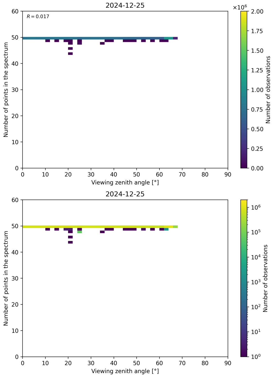
Figure 125: Scatter density plot of “Viewing zenith angle” against “Number of points in the spectrum” for 2024-12-24 to 2024-12-26.
