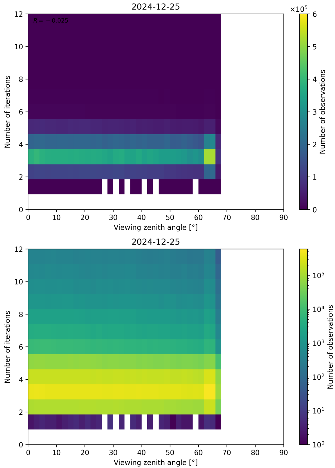
Figure 124: Scatter density plot of “Viewing zenith angle” against “Number of iterations” for 2024-12-24 to 2024-12-26.
