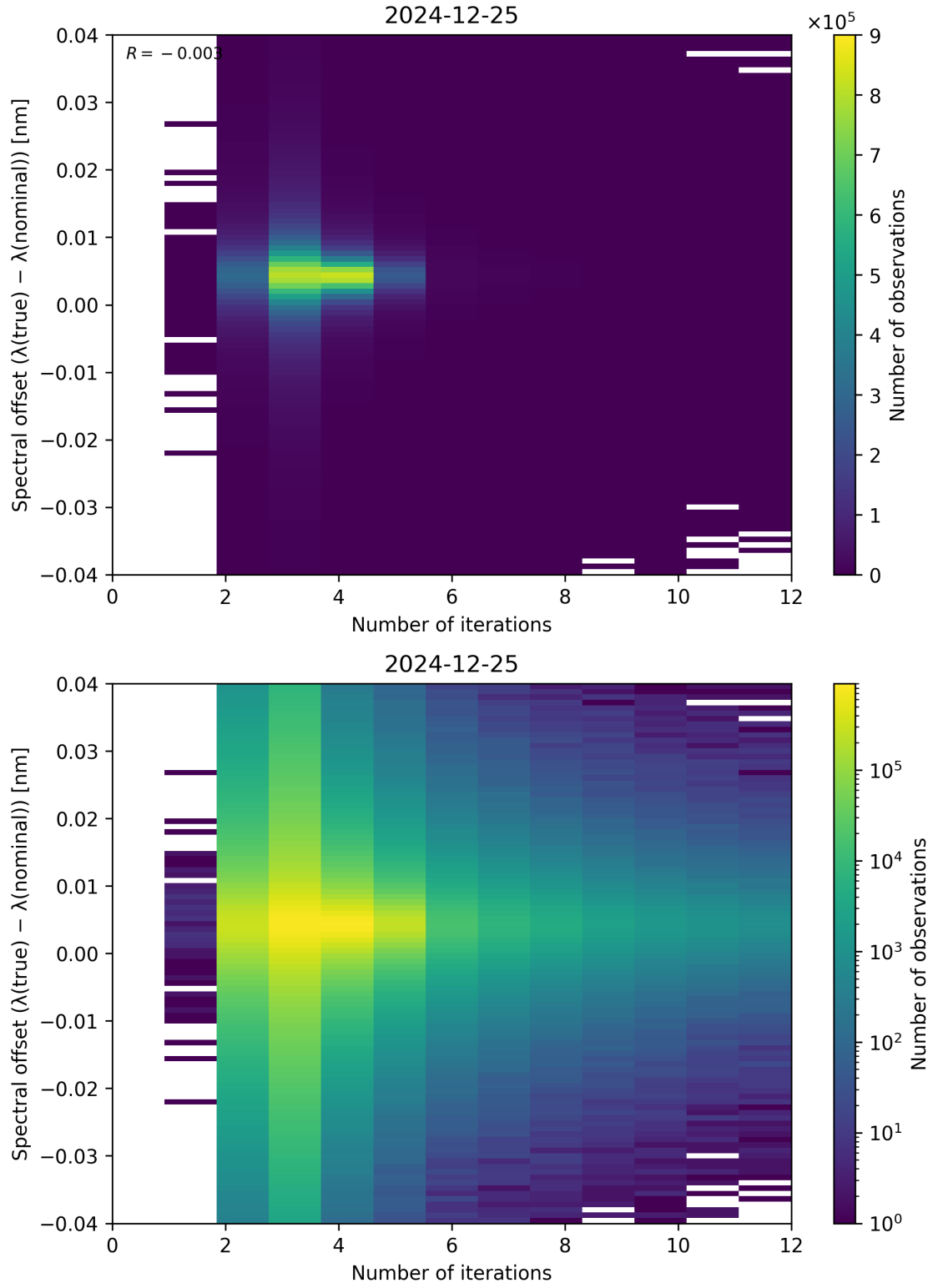
Figure 100: Scatter density plot of “Number of iterations” against “Spectral offset ( \lambda_{\text{true}} - \lambda_{\text{nominal}} )” for 2024-12-24 to 2024-12-26.
