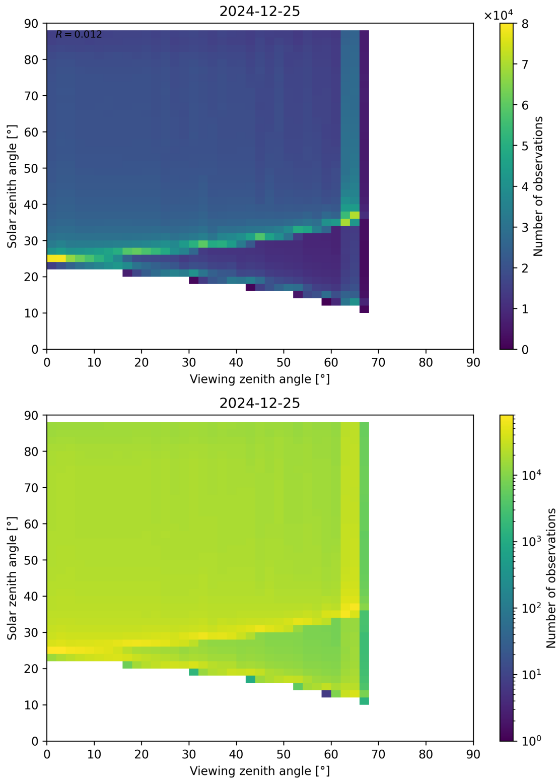
Figure 127: Scatter density plot of “Viewing zenith angle” against “Solar zenith angle” for 2024-12-24 to 2024-12-26.
