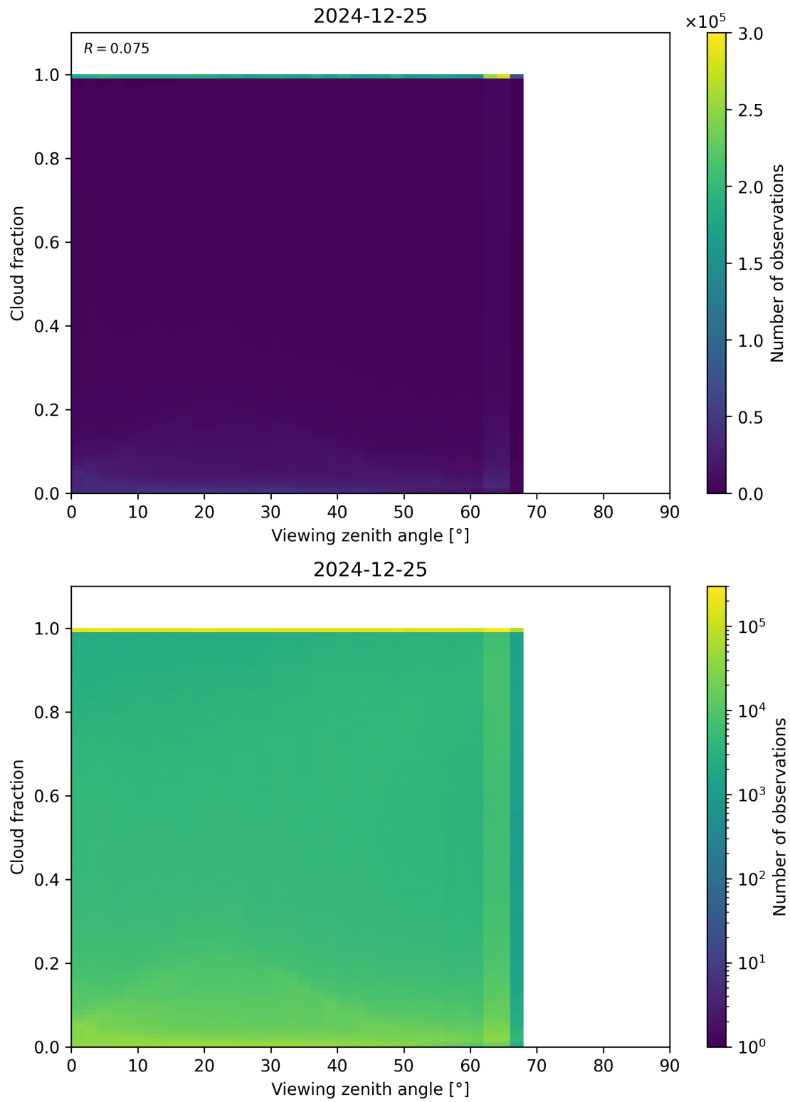
Figure 120: Scatter density plot of “Viewing zenith angle” against “Cloud fraction” for 2024-12-24 to 2024-12-26.
