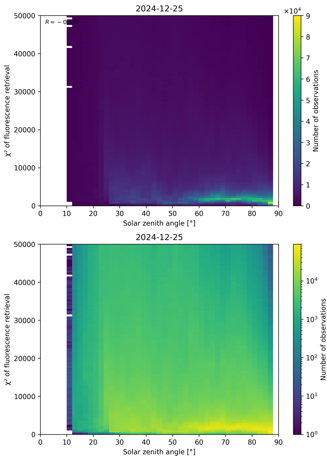
Figure 109: Scatter density plot of “Solar zenith angle” against “ \chi^2 of fluorescence retrieval” for 2024-12-24 to 2024-12-26.
