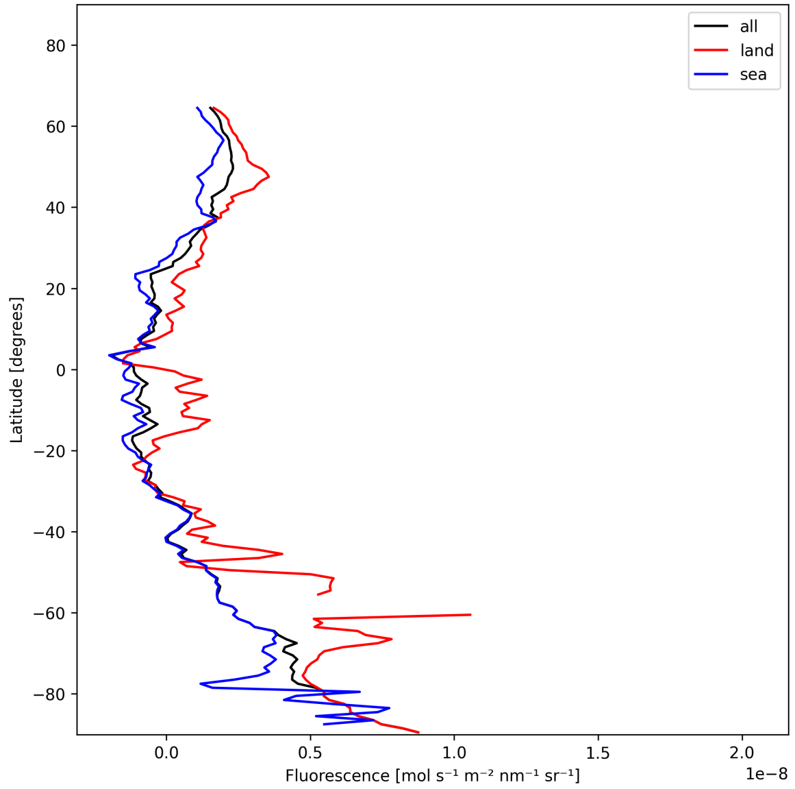
Figure 23: Zonal average of “Fluorescence” for 2024-12-24 to 2024-12-26.
