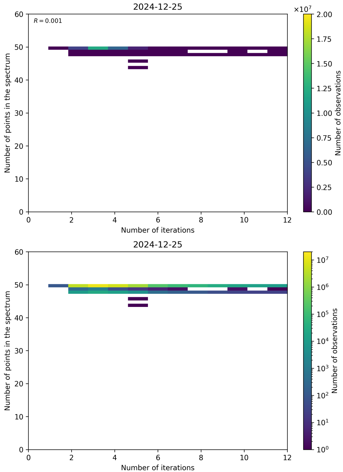
Figure 99: Scatter density plot of “Number of iterations” against “Number of points in the spectrum” for 2024-12-24 to 2024-12-26.
