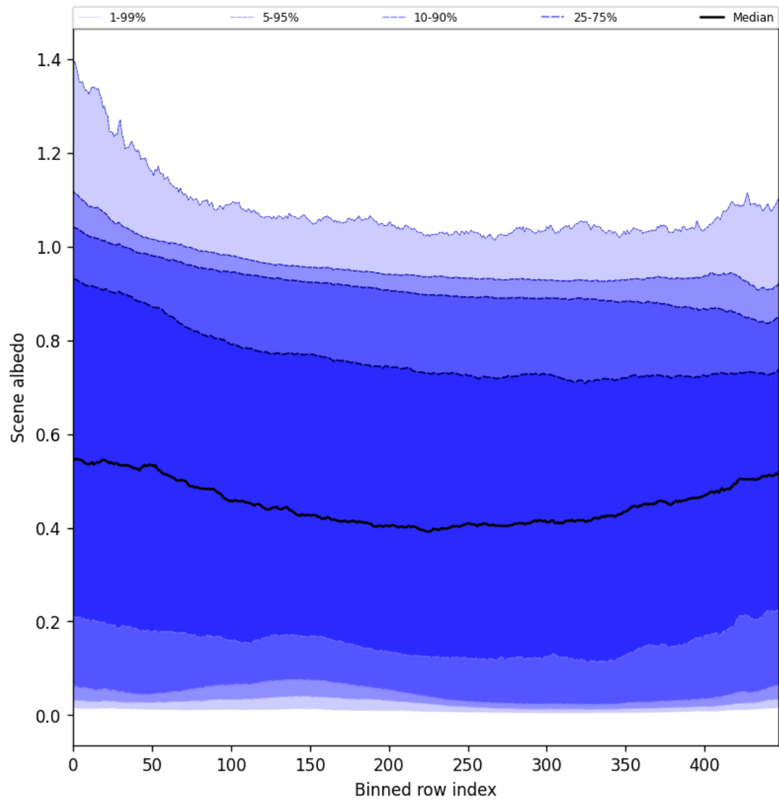
Figure 51: Along track statistics of “Scene albedo” for 2024-12-24 to 2024-12-26
