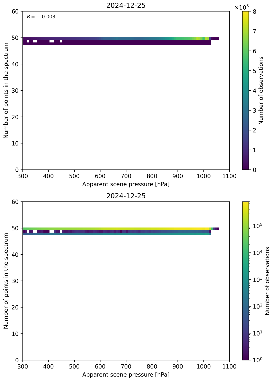
Figure 66: Scatter density plot of “Apparent scene pressure” against “Number of points in the spectrum” for 2024-12-24 to 2024-12-26.
