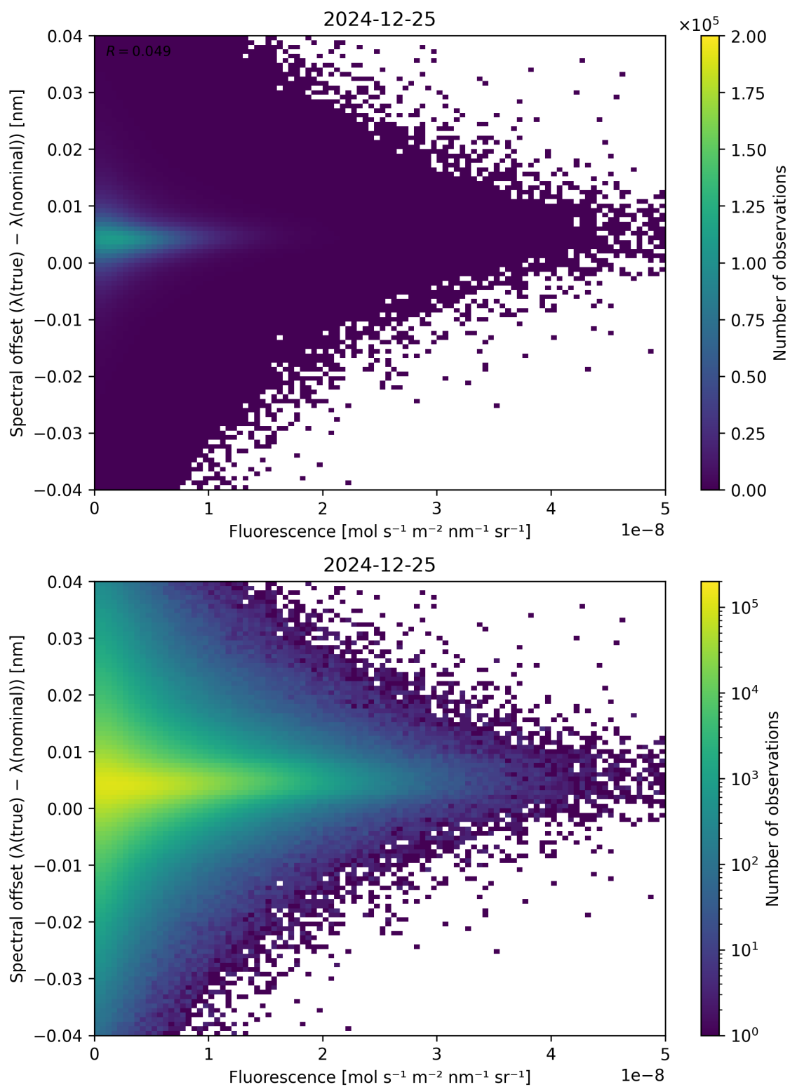
Figure 87: Scatter density plot of “Fluorescence” against “Spectral offset ( \lambda_{\text{true}} - \lambda_{\text{nominal}} )” for 2024-12-24 to 2024-12-26.
