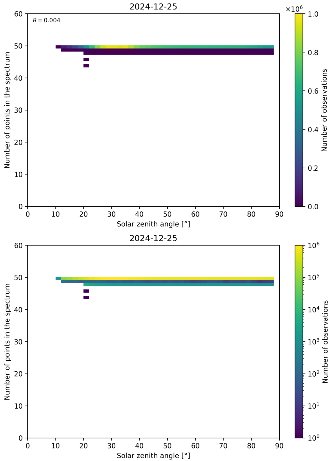
Figure 115: Scatter density plot of “Solar zenith angle” against “Number of points in the spectrum” for 2024-12-24 to 2024-12-26.
