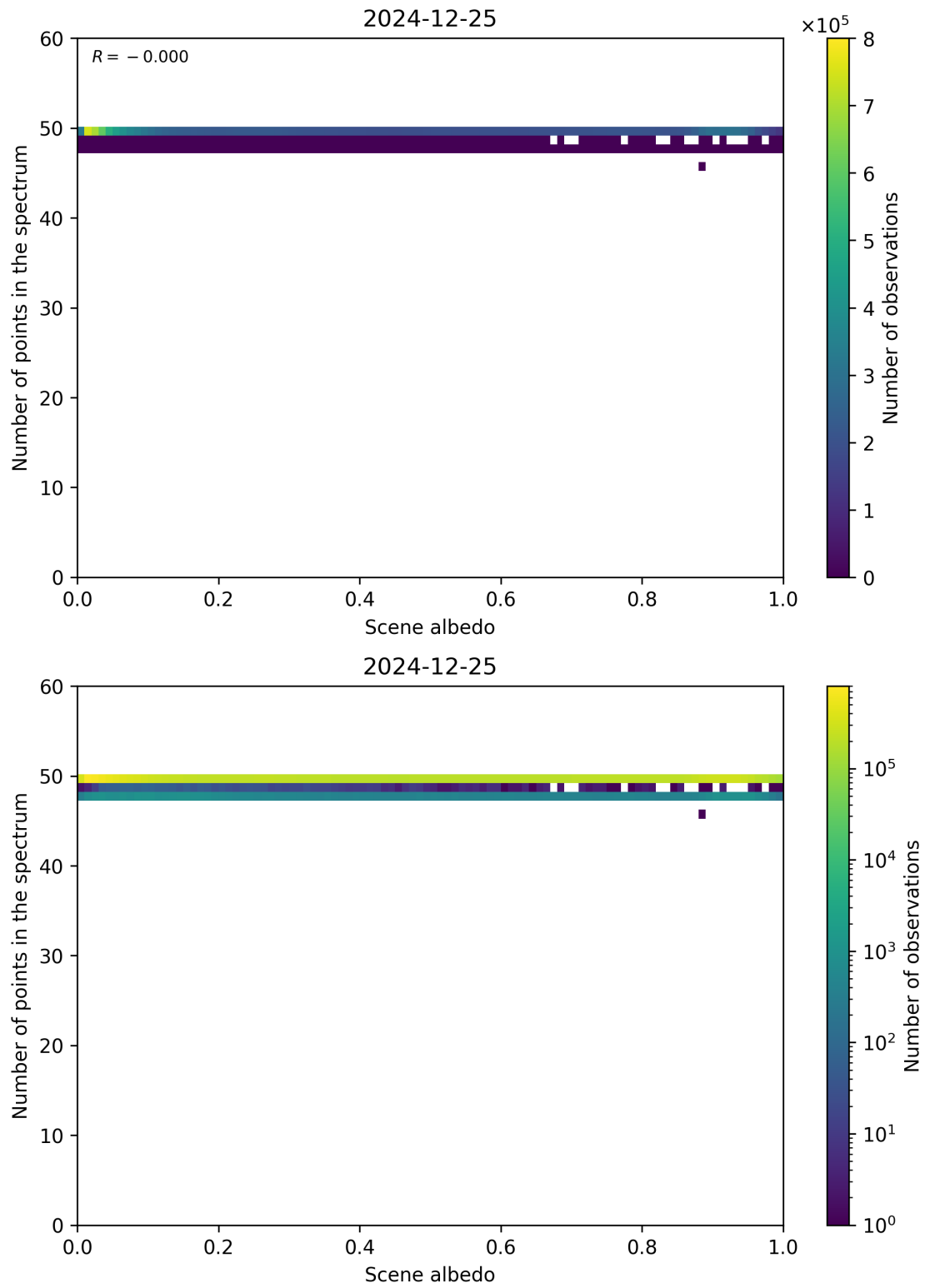
Figure 106: Scatter density plot of “Scene albedo” against “Number of points in the spectrum” for 2024-12-24 to 2024-12-26.
