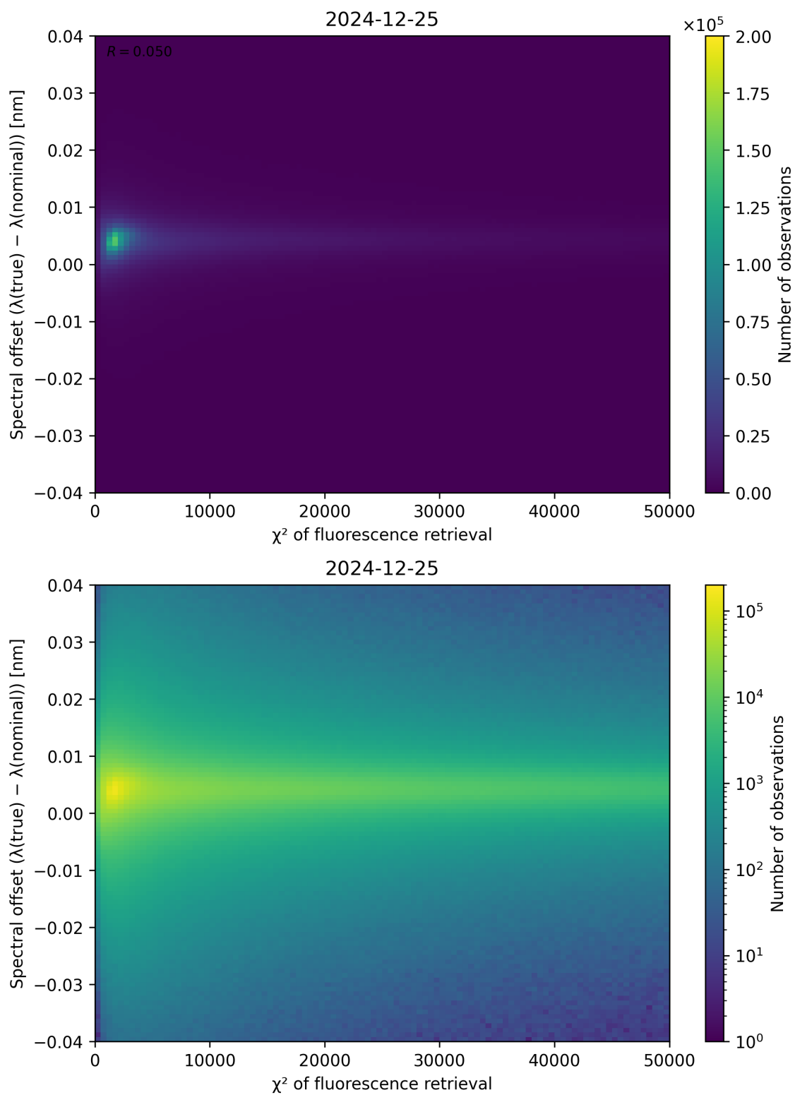
Figure 69: Scatter density plot of “ \chi^2 of fluorescence retrieval” against “Spectral offset ( \lambda_{\text{true}} - \lambda_{\text{nominal}} )” for 2024-12-24 to 2024-12-26.
