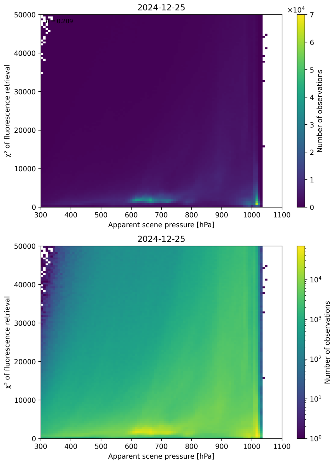
Figure 63: Scatter density plot of “Apparent scene pressure” against “ \chi^2 of fluorescence retrieval” for 2024-12-24 to 2024-12-26.
