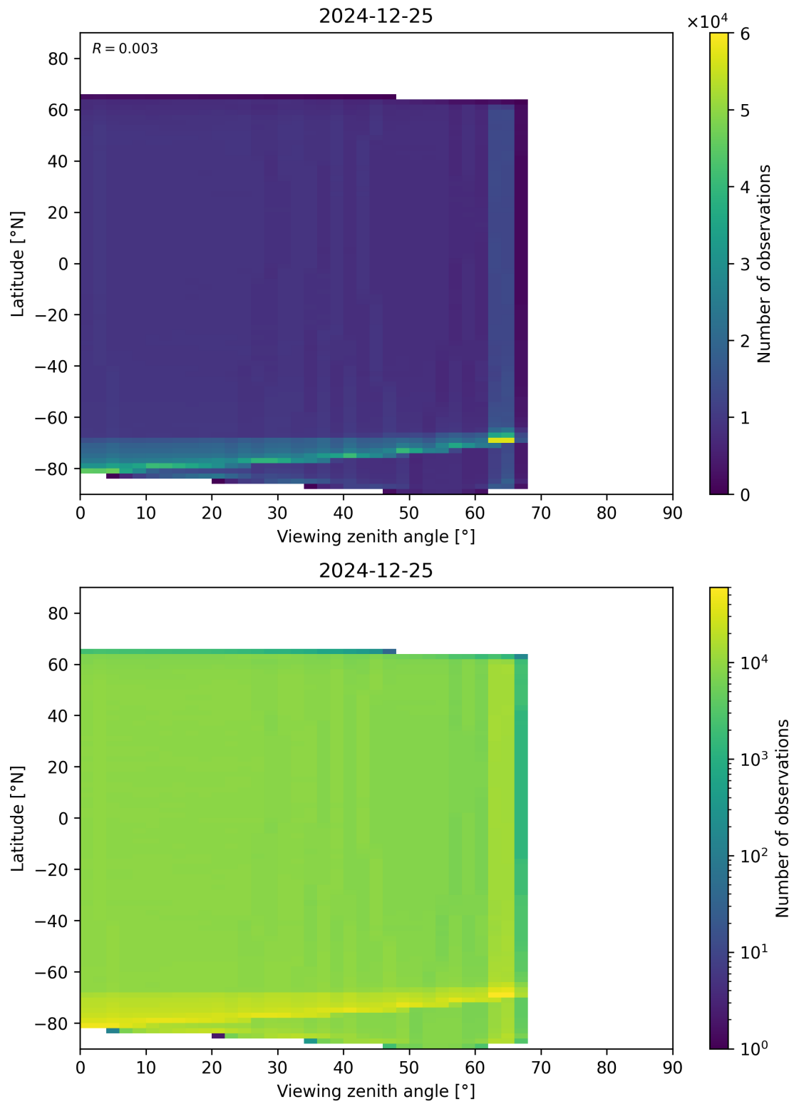
Figure 123: Scatter density plot of “Viewing zenith angle” against “Latitude” for 2024-12-24 to 2024-12-26.
