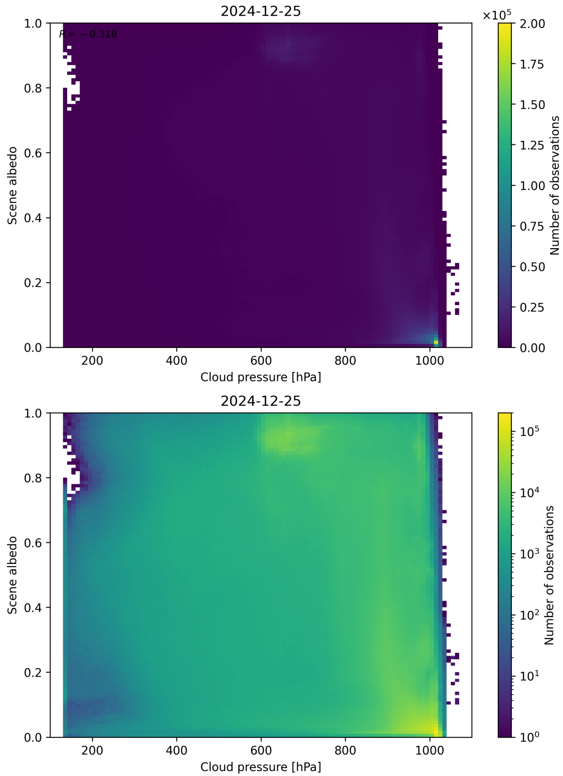
Figure 83: Scatter density plot of “Cloud pressure” against “Scene albedo” for 2024-12-24 to 2024-12-26.
