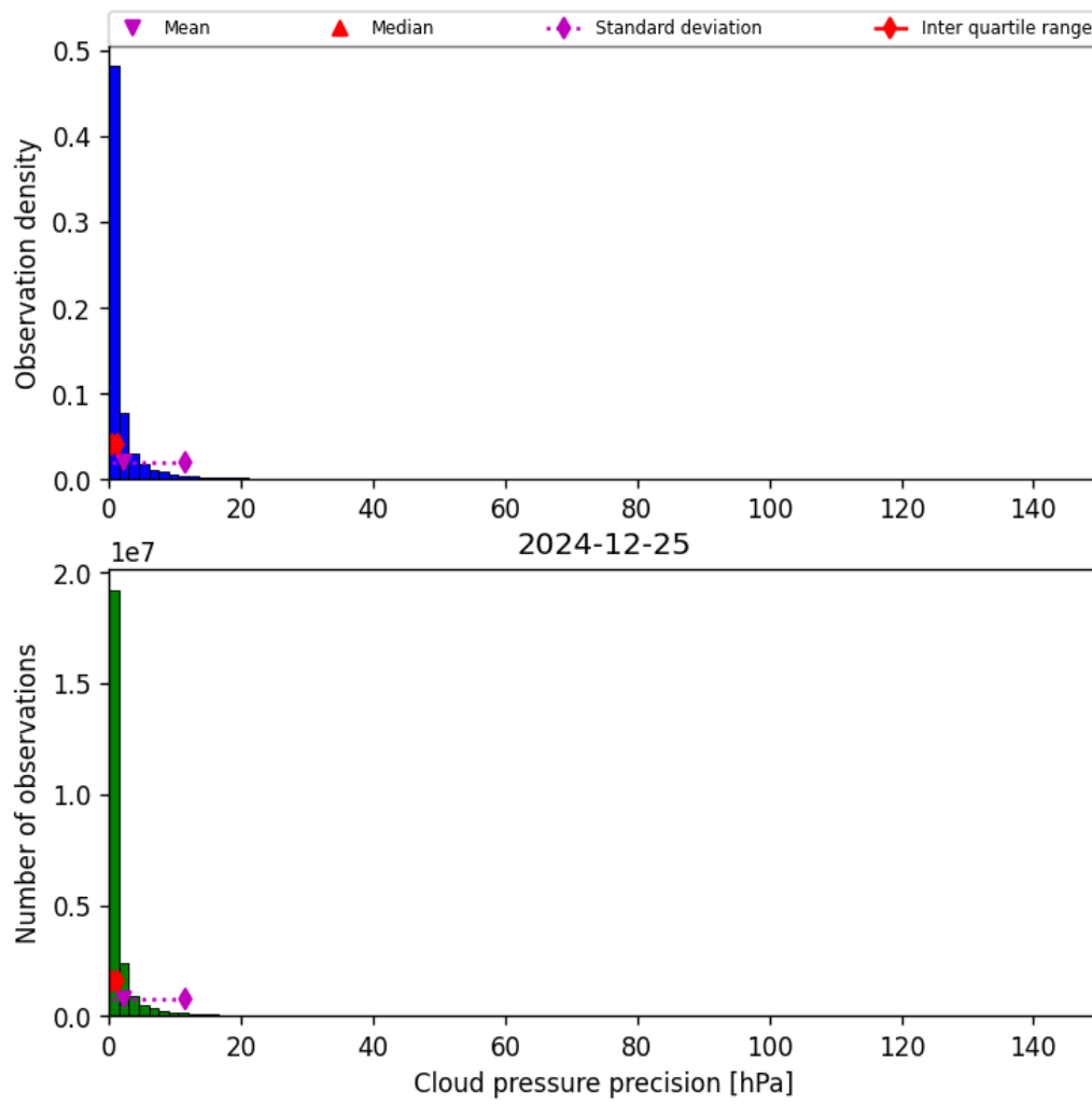
Figure 31: Histogram of “Cloud pressure precision” for 2024-12-24 to 2024-12-26
