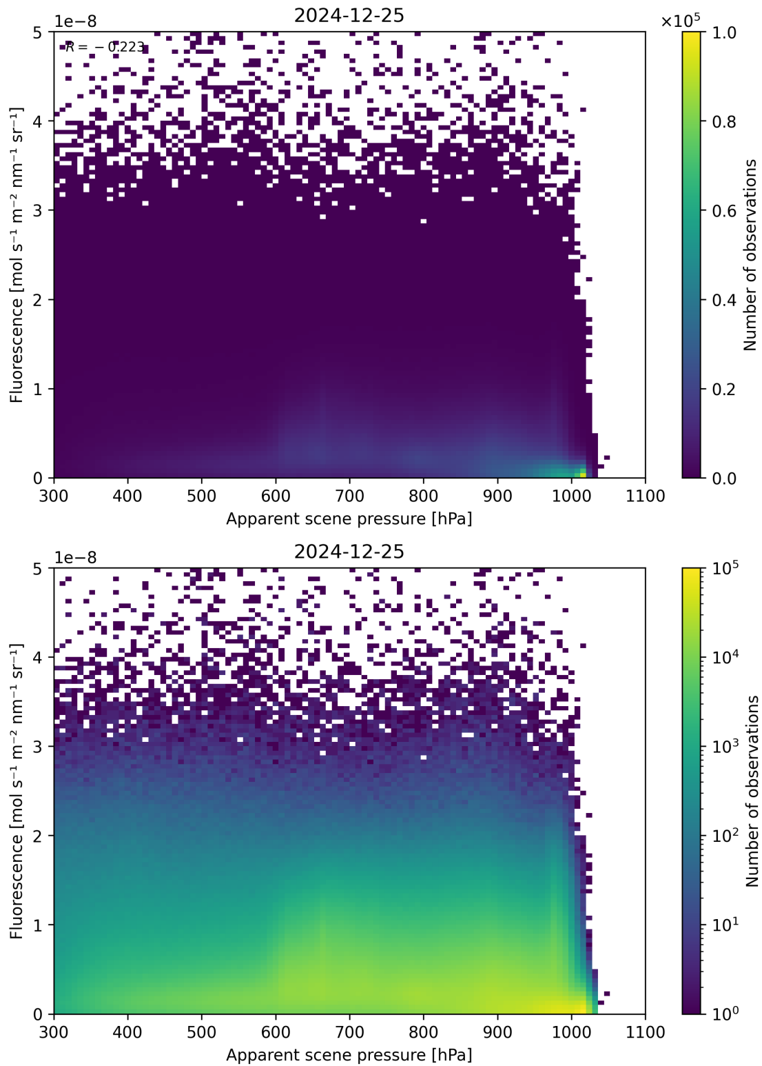
Figure 64: Scatter density plot of “Apparent scene pressure” against “Fluorescence” for 2024-12-24 to 2024-12-26.
