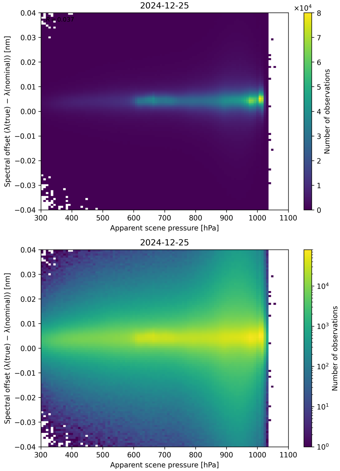
Figure 67: Scatter density plot of “Apparent scene pressure” against “Spectral offset ( \lambda_{\text{true}} - \lambda_{\text{nominal}} )” for 2024-12-24 to 2024-12-26.
