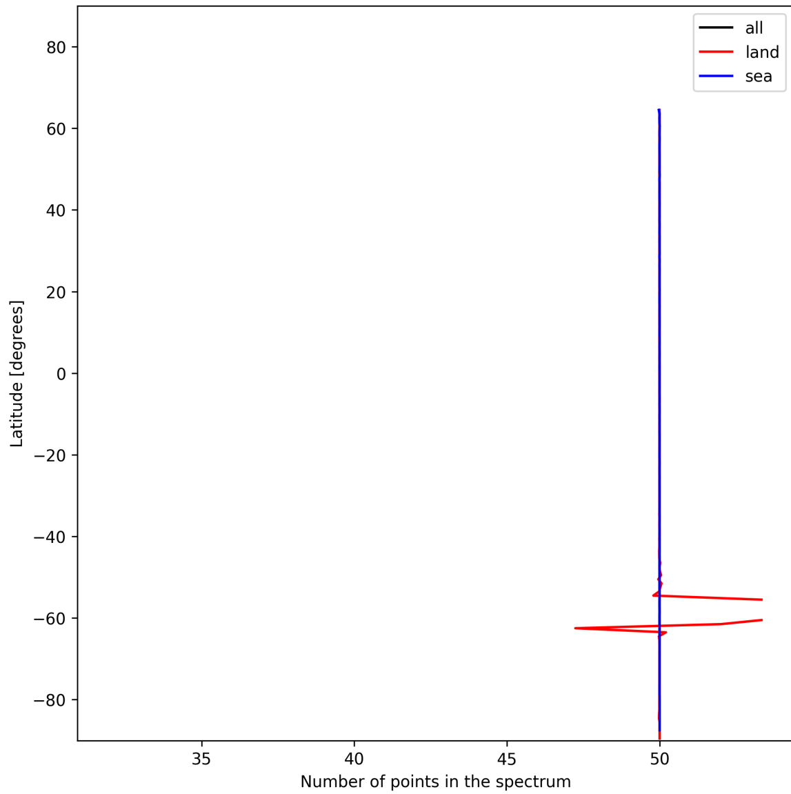
Figure 27: Zonal average of “Number of points in the spectrum” for 2024-12-24 to 2024-12-26.
