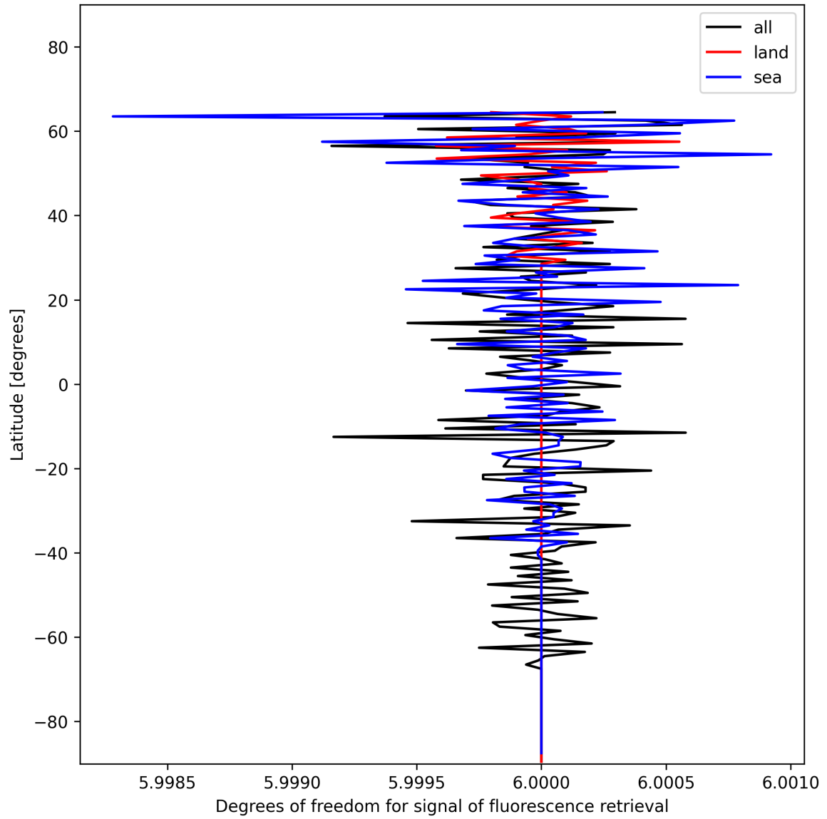
Figure 26: Zonal average of “Degrees of freedom for signal of fluorescence retrieval” for 2024-12-24 to 2024-12-26.
