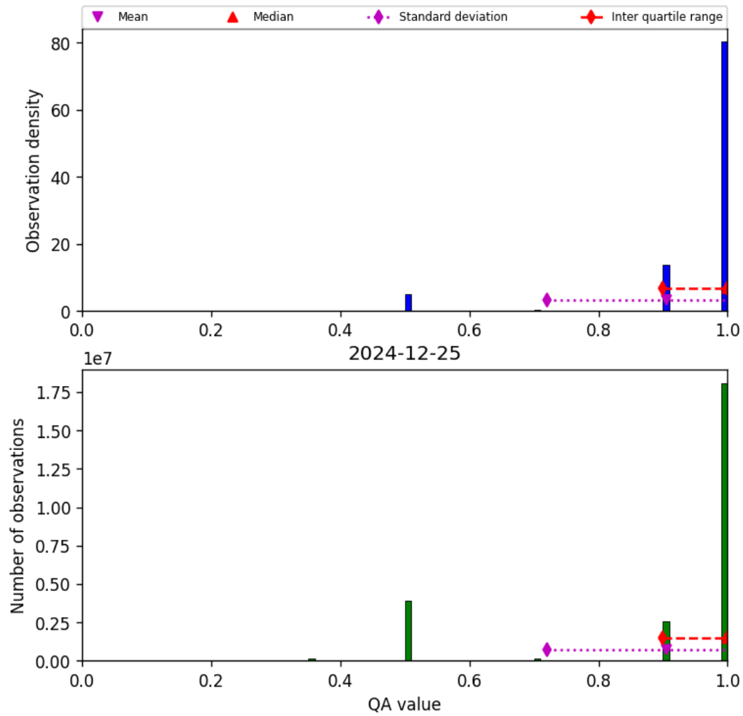
Figure 29: Histogram of “QA value” for 2024-12-24 to 2024-12-26
