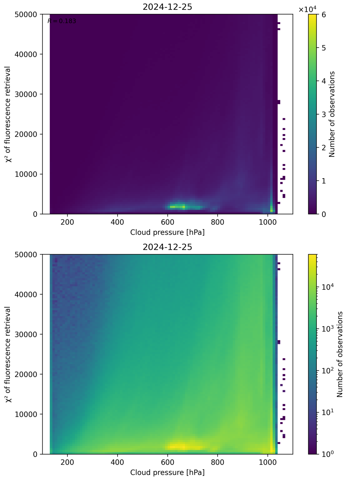
Figure 78: Scatter density plot of “Cloud pressure” against “ \chi^2 of fluorescence retrieval” for 2024-12-24 to 2024-12-26.
