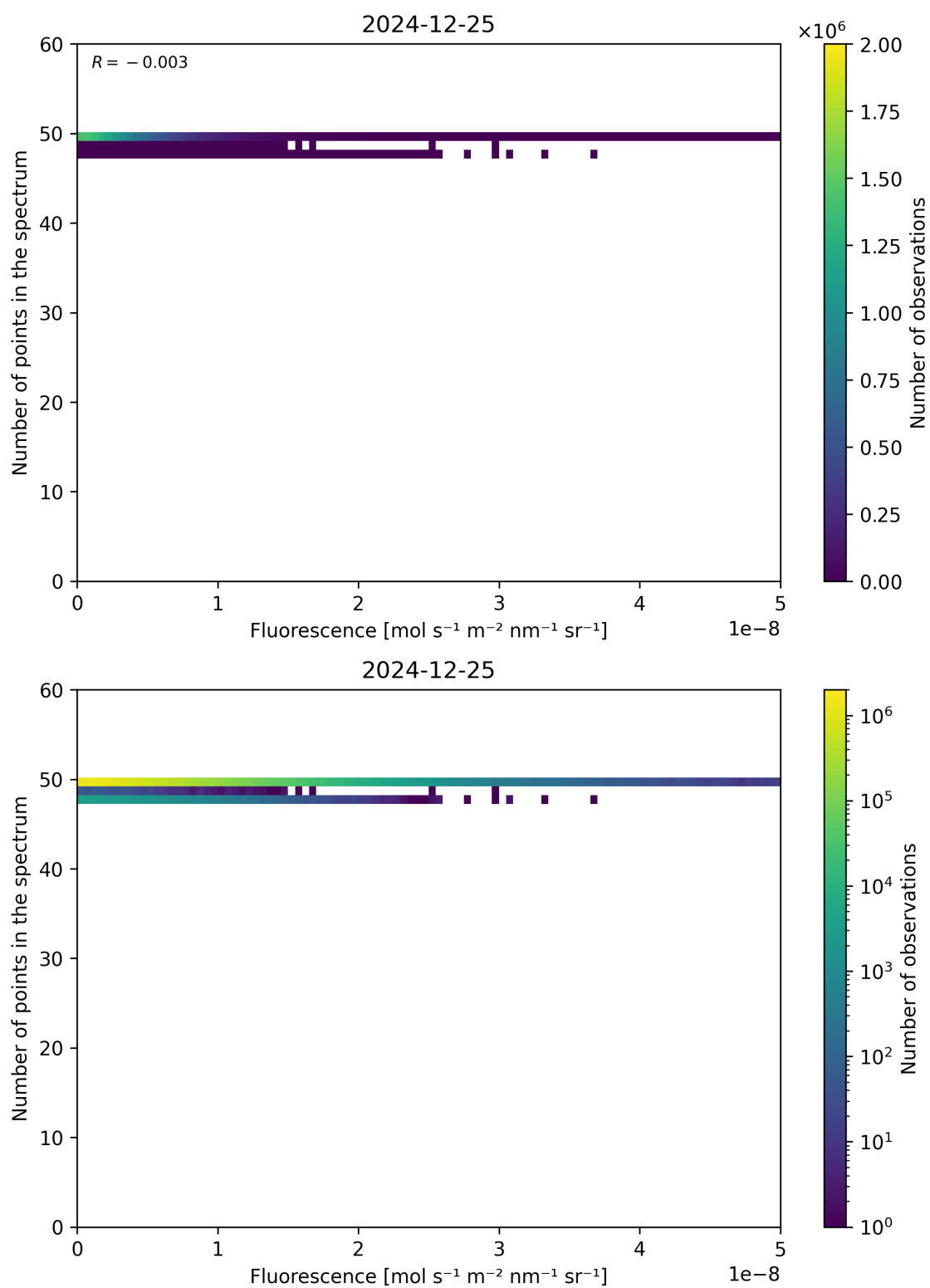
Figure 86: Scatter density plot of “Fluorescence” against “Number of points in the spectrum” for 2024-12-24 to 2024-12-26.
