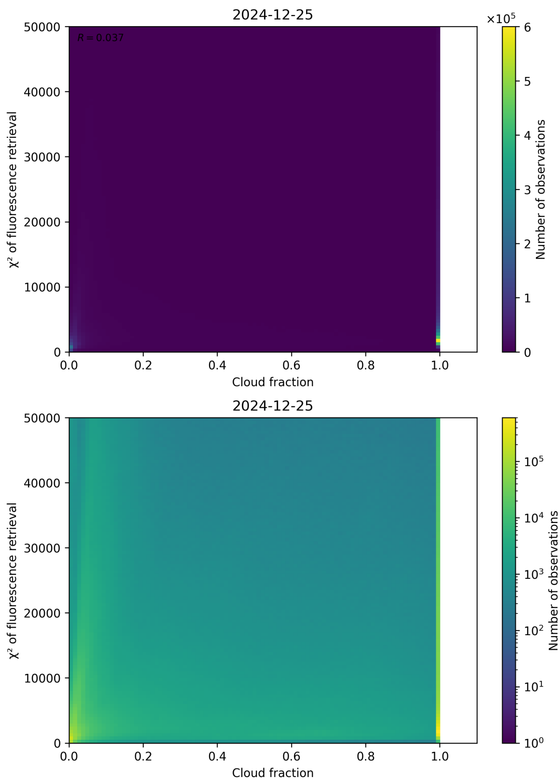
Figure 71: Scatter density plot of “Cloud fraction” against “ \chi^2 of fluorescence retrieval” for 2024-12-24 to 2024-12-26.
