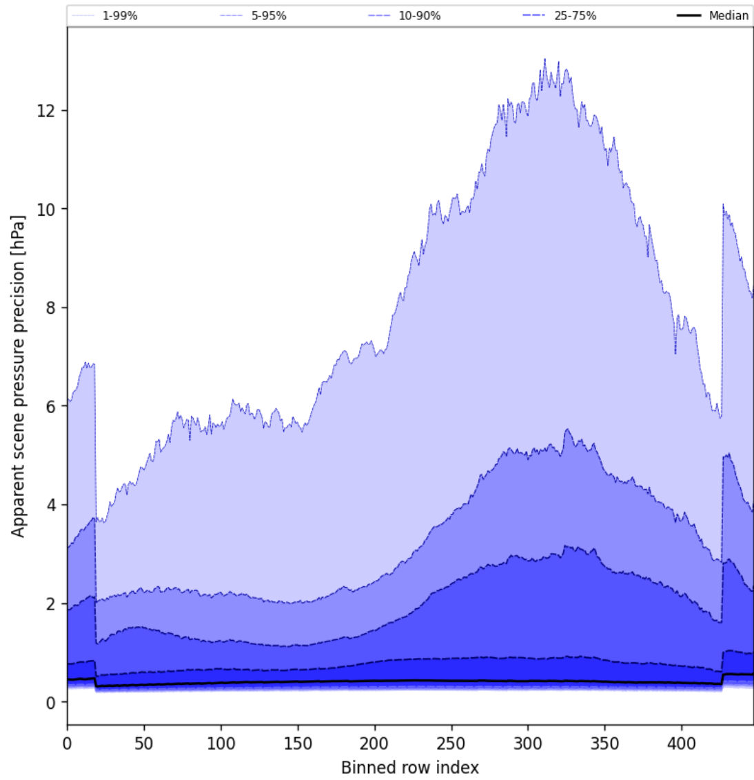
Figure 54: Along track statistics of “Apparent scene pressure precision” for 2024-12-24 to 2024-12-26
