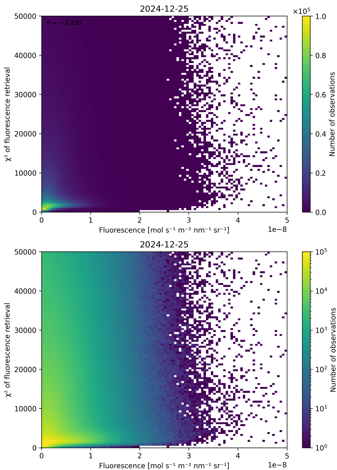
Figure 85: Scatter density plot of “Fluorescence” against “ \chi^2 of fluorescence retrieval” for 2024-12-24 to 2024-12-26.
