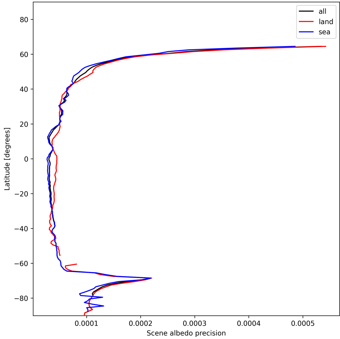
Figure 18: Zonal average of “Scene albedo precision” for 2024-12-24 to 2024-12-26.
