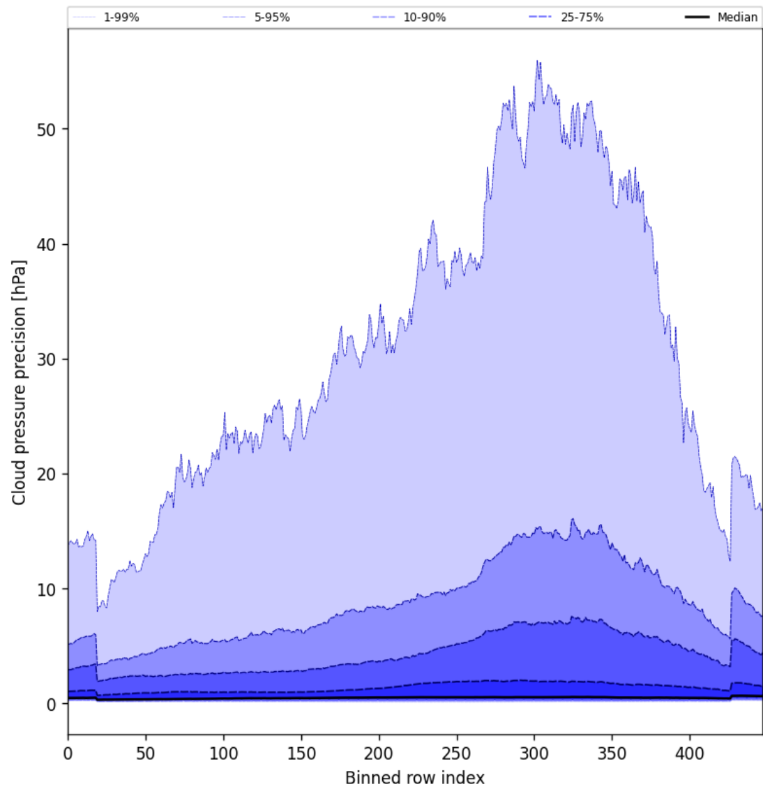
Figure 48: Along track statistics of “Cloud pressure precision” for 2024-12-24 to 2024-12-26
