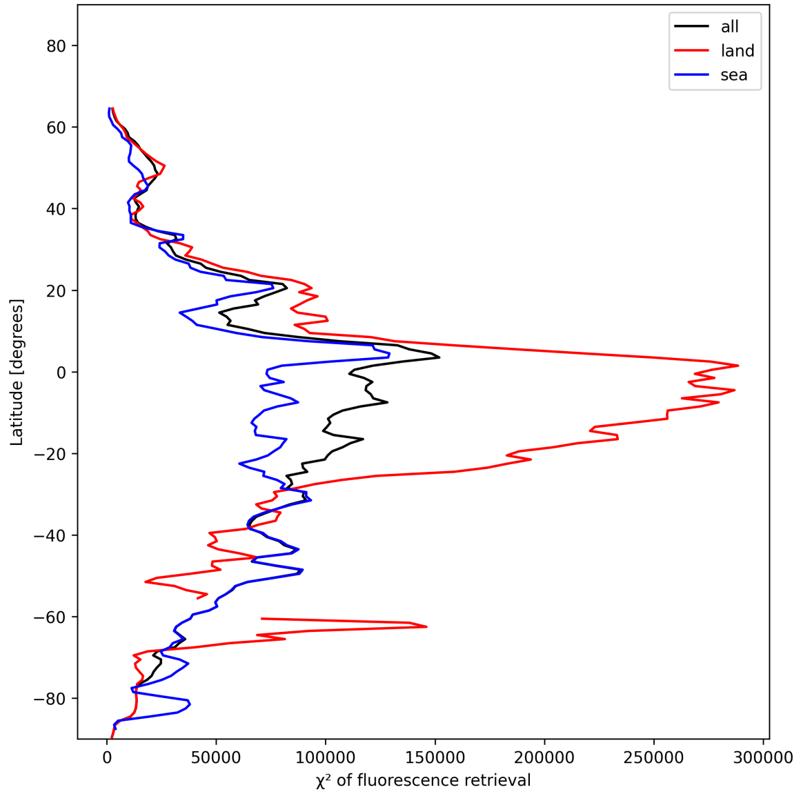
Figure 25: Zonal average of “ \chi^2 of fluorescence retrieval” for 2024-12-24 to 2024-12-26.
