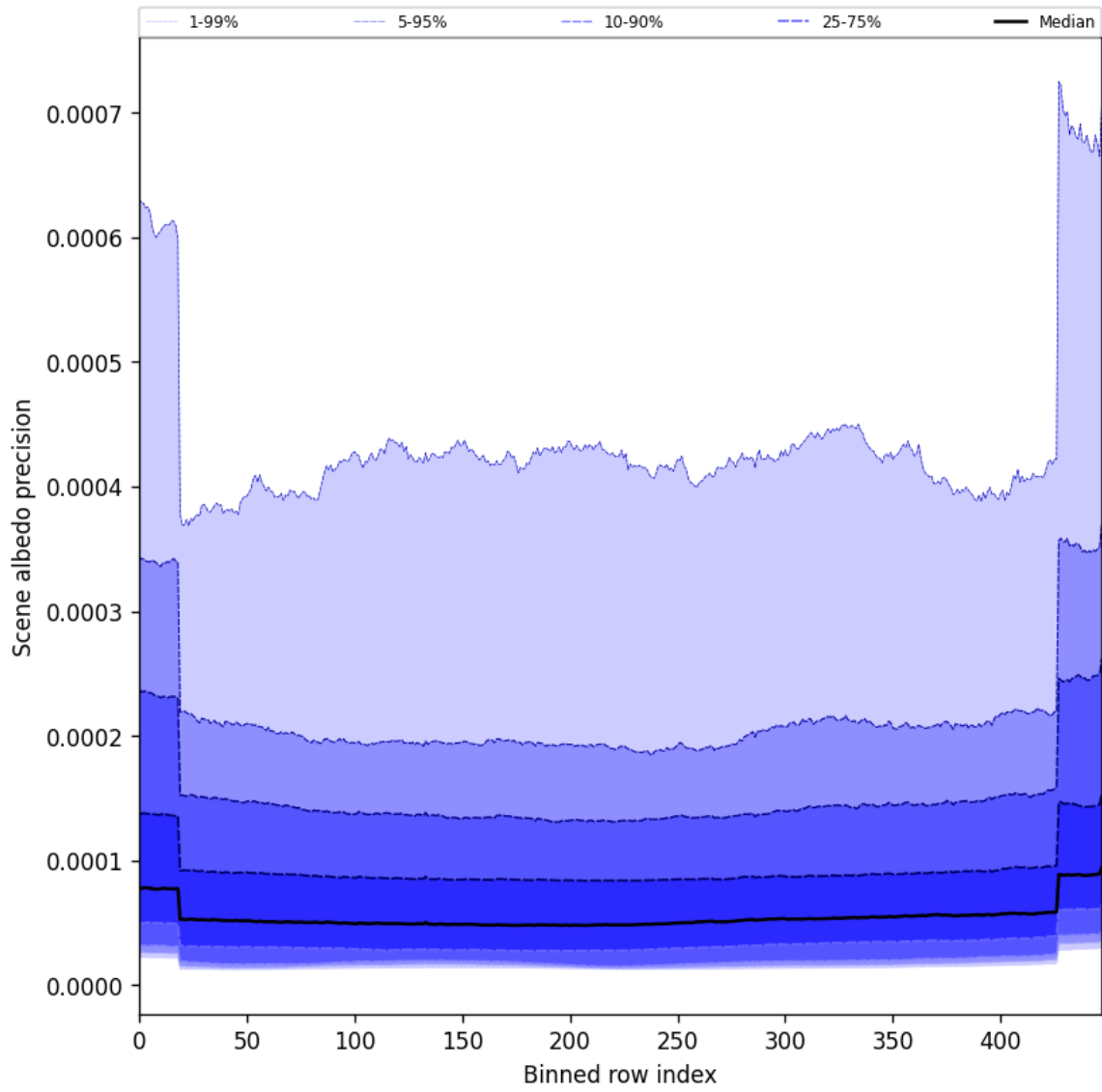
Figure 52: Along track statistics of “Scene albedo precision” for 2024-12-24 to 2024-12-26
