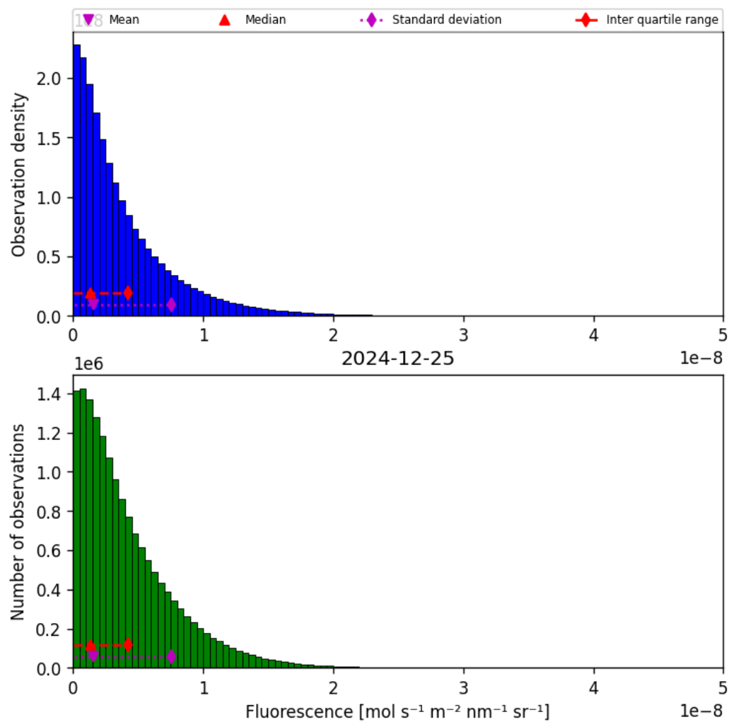
Figure 40: Histogram of “Fluorescence” for 2024-12-24 to 2024-12-26
