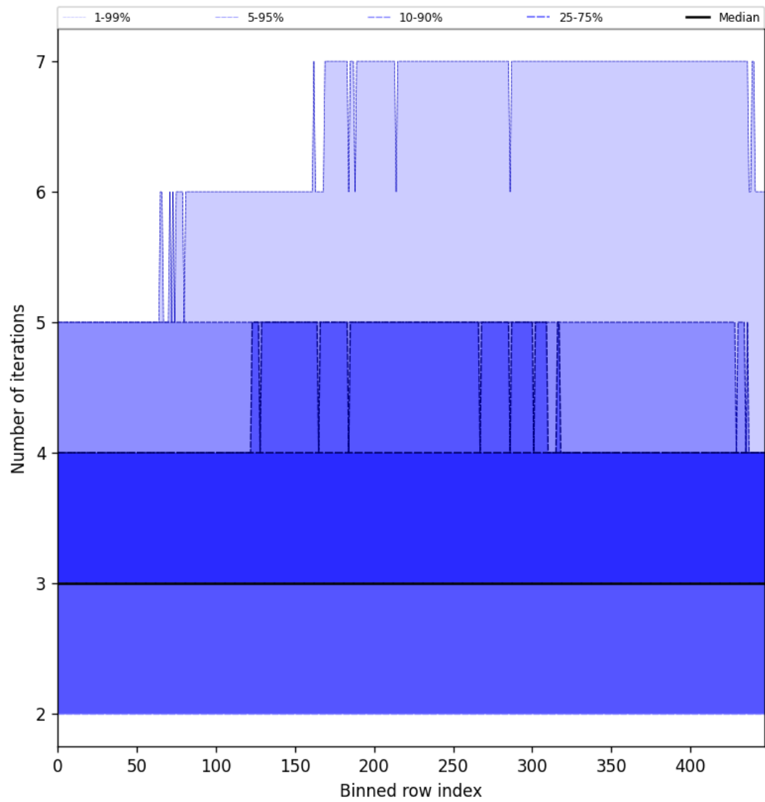
Figure 56: Along track statistics of “Number of iterations” for 2024-12-24 to 2024-12-26
