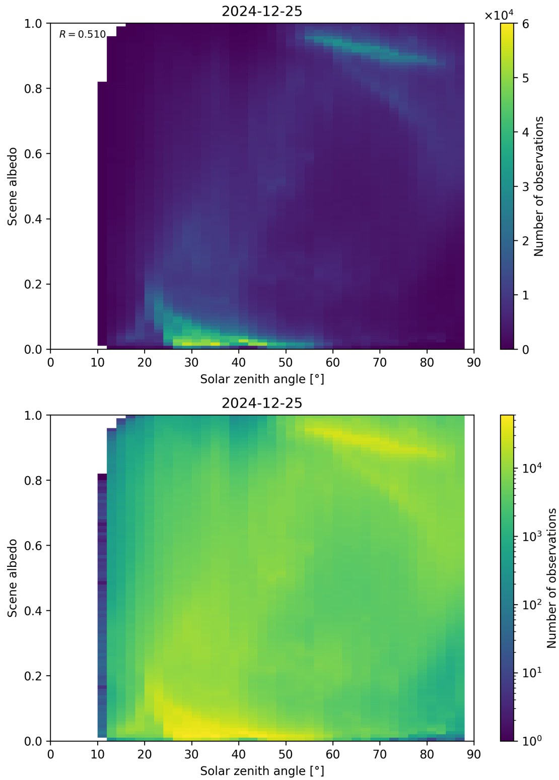
Figure 116: Scatter density plot of “Solar zenith angle” against “Scene albedo” for 2024-12-24 to 2024-12-26.
