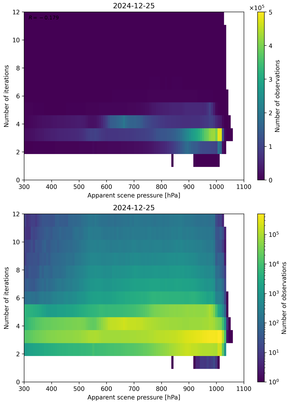
Figure 65: Scatter density plot of “Apparent scene pressure” against “Number of iterations” for 2024-12-24 to 2024-12-26.
