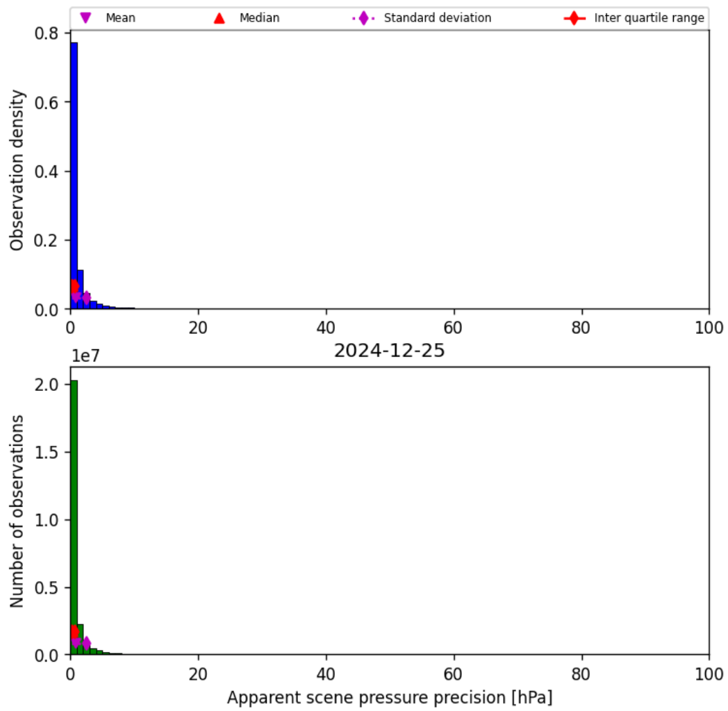
Figure 37: Histogram of “Apparent scene pressure precision” for 2024-12-24 to 2024-12-26
