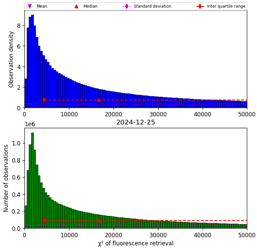
Figure 42: Histogram of “ \chi^2 of fluorescence retrieval” for 2024-12-24 to 2024-12-26
