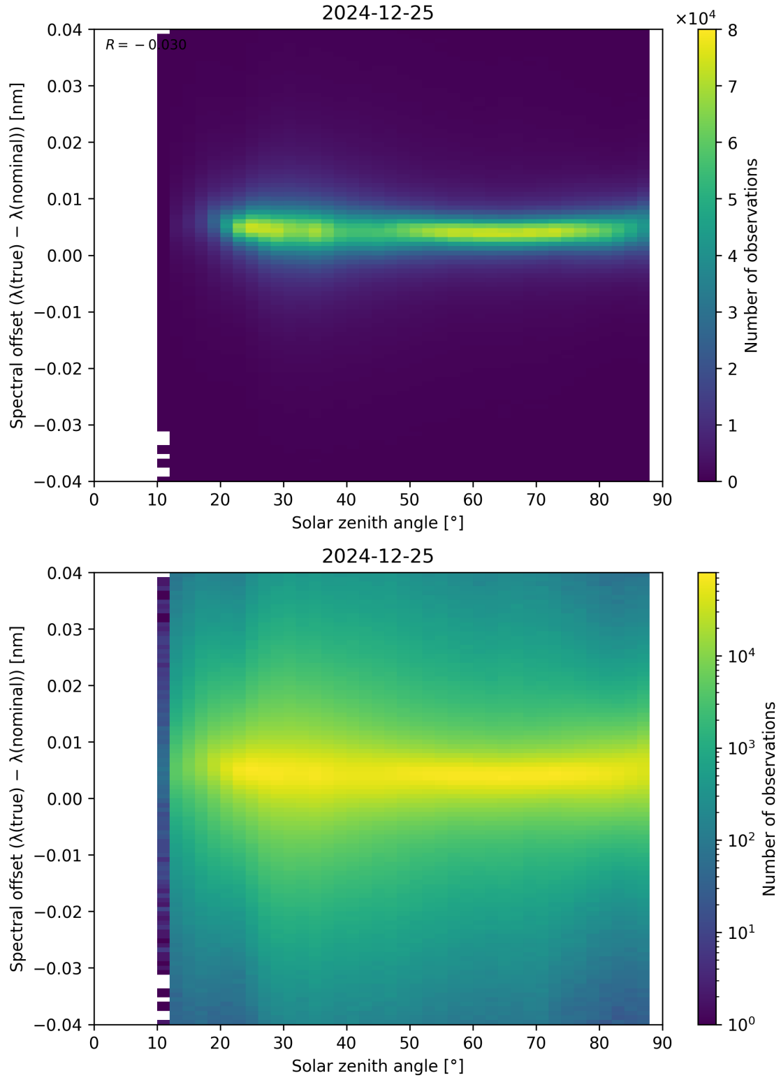
Figure 117: Scatter density plot of “Solar zenith angle” against “Spectral offset ( \lambda_{\text{true}} - \lambda_{\text{nominal}} )” for 2024-12-24 to 2024-12-26.
