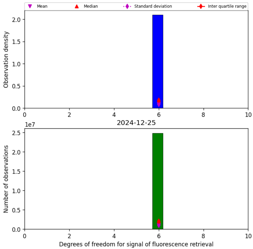
Figure 43: Histogram of "Degrees of freedom for signal of fluorescence retrieval" for 2024-12-24 to 2024-12-26
