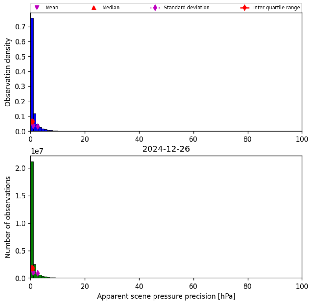
Figure 37: Histogram of “Apparent scene pressure precision” for 2024-12-25 to 2024-12-27
