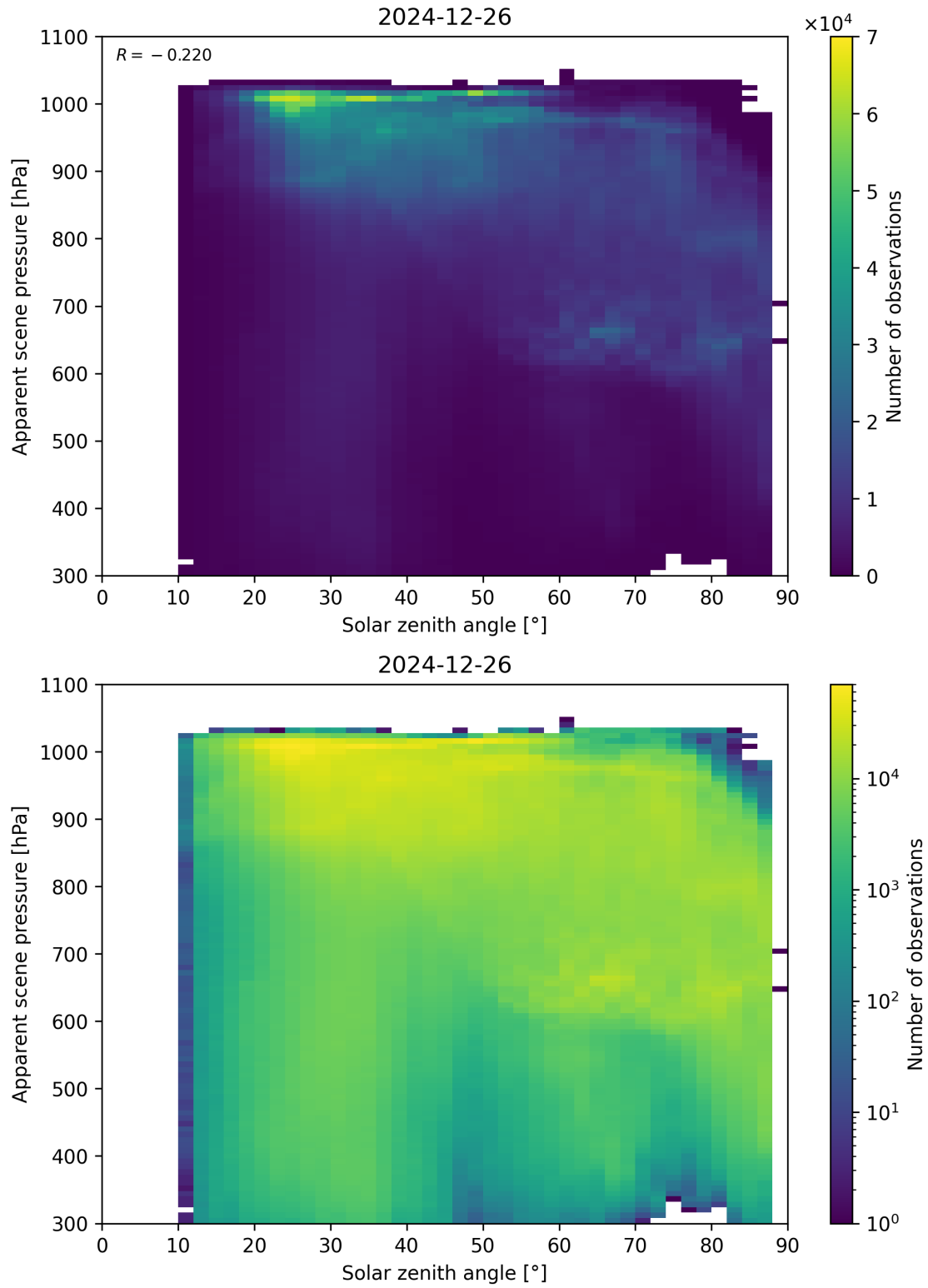
Figure 108: Scatter density plot of “Solar zenith angle” against “Apparent scene pressure” for 2024-12-25 to 2024-12-27.
