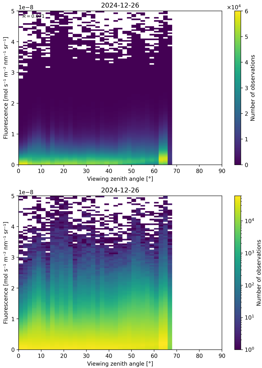
Figure 122: Scatter density plot of “Viewing zenith angle” against “Fluorescence” for 2024-12-25 to 2024-12-27.
