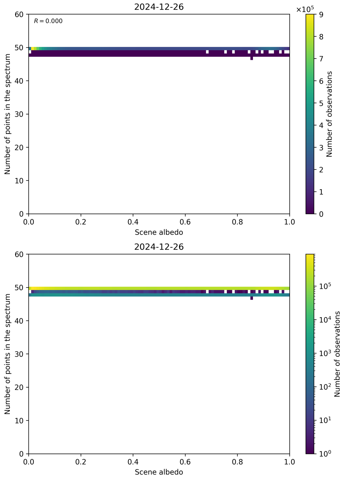
Figure 106: Scatter density plot of “Scene albedo” against “Number of points in the spectrum” for 2024-12-25 to 2024-12-27.
