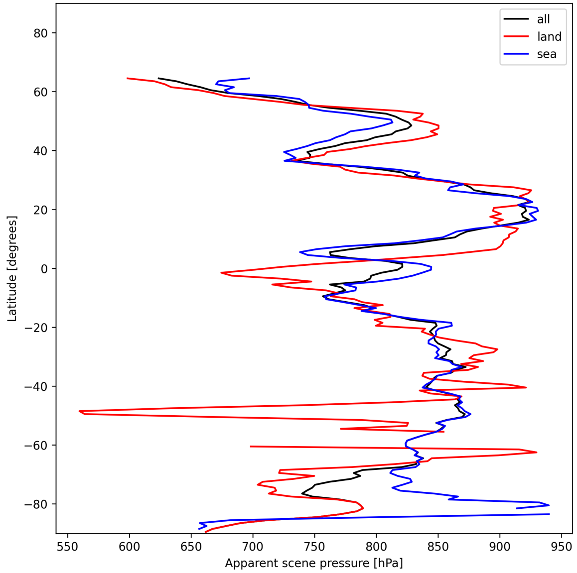
Figure 19: Zonal average of “Apparent scene pressure” for 2024-12-25 to 2024-12-27.
