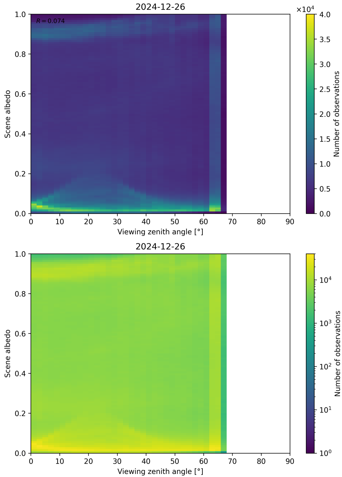
Figure 126: Scatter density plot of “Viewing zenith angle” against “Scene albedo” for 2024-12-25 to 2024-12-27.
