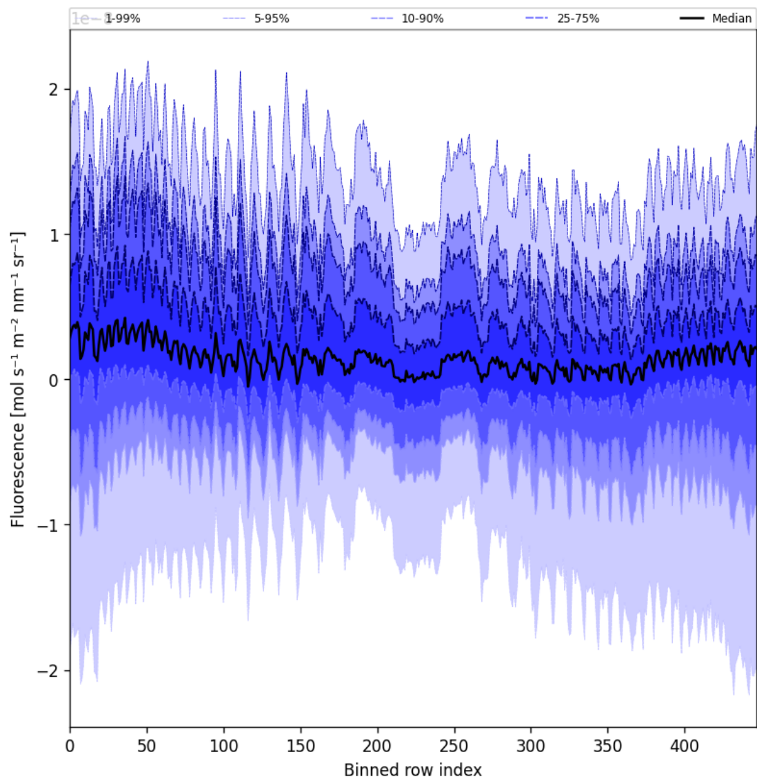
Figure 57: Along track statistics of “Fluorescence” for 2024-12-25 to 2024-12-27
