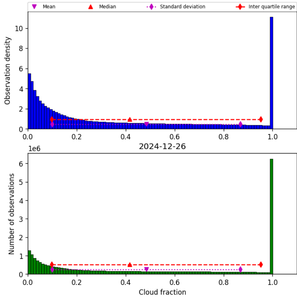
Figure 32: Histogram of “Cloud fraction” for 2024-12-25 to 2024-12-27
