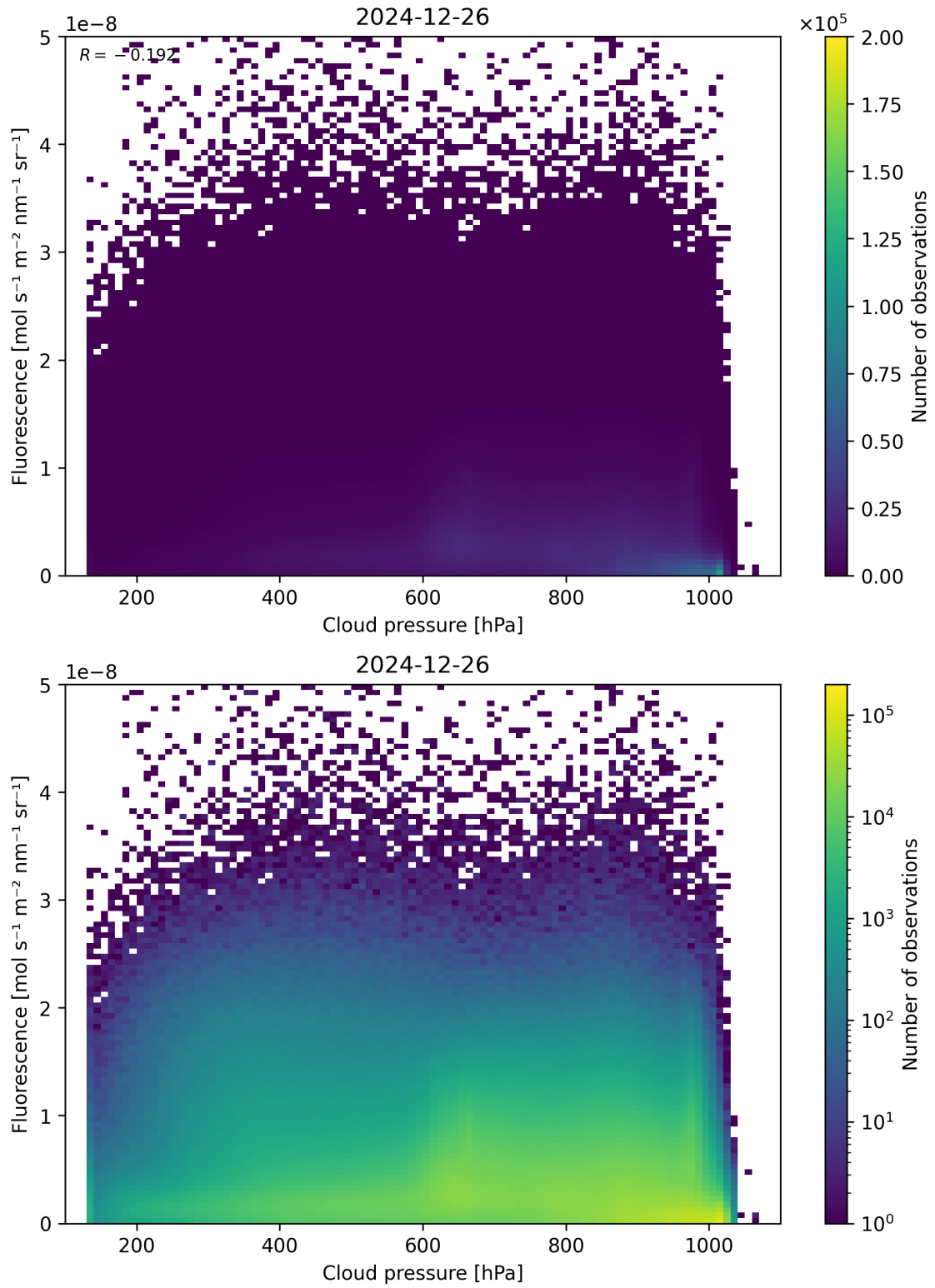
Figure 80: Scatter density plot of “Cloud pressure” against “Fluorescence” for 2024-12-25 to 2024-12-27.
