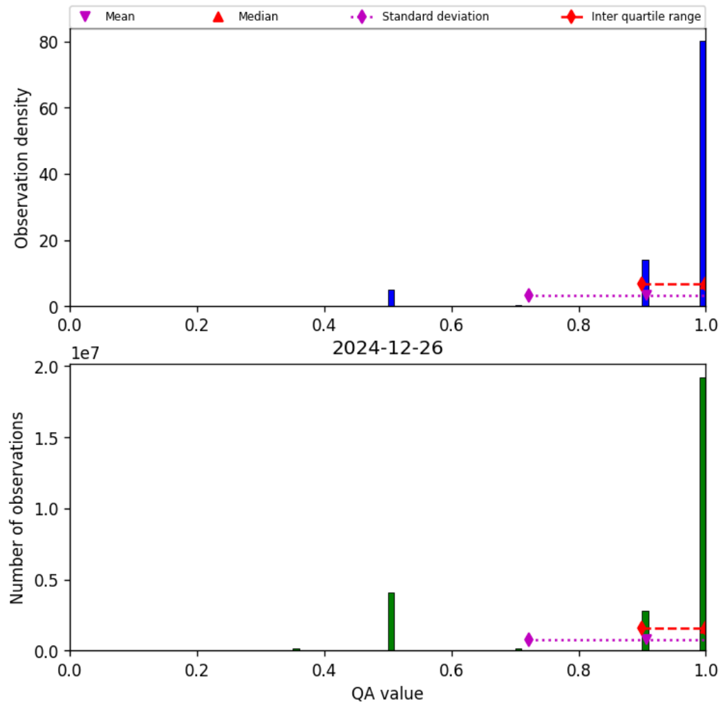
Figure 29: Histogram of “QA value” for 2024-12-25 to 2024-12-27
