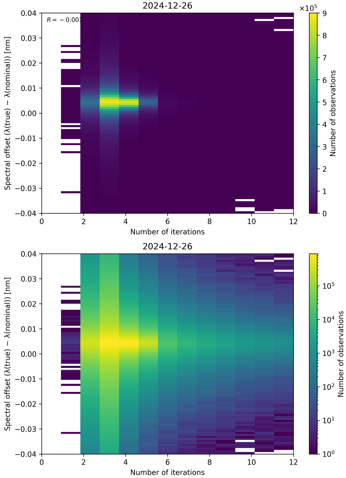
Figure 100: Scatter density plot of “Number of iterations” against “Spectral offset ( \lambda_{\text{true}} - \lambda_{\text{nominal}} )” for 2024-12-25 to 2024-12-27.
