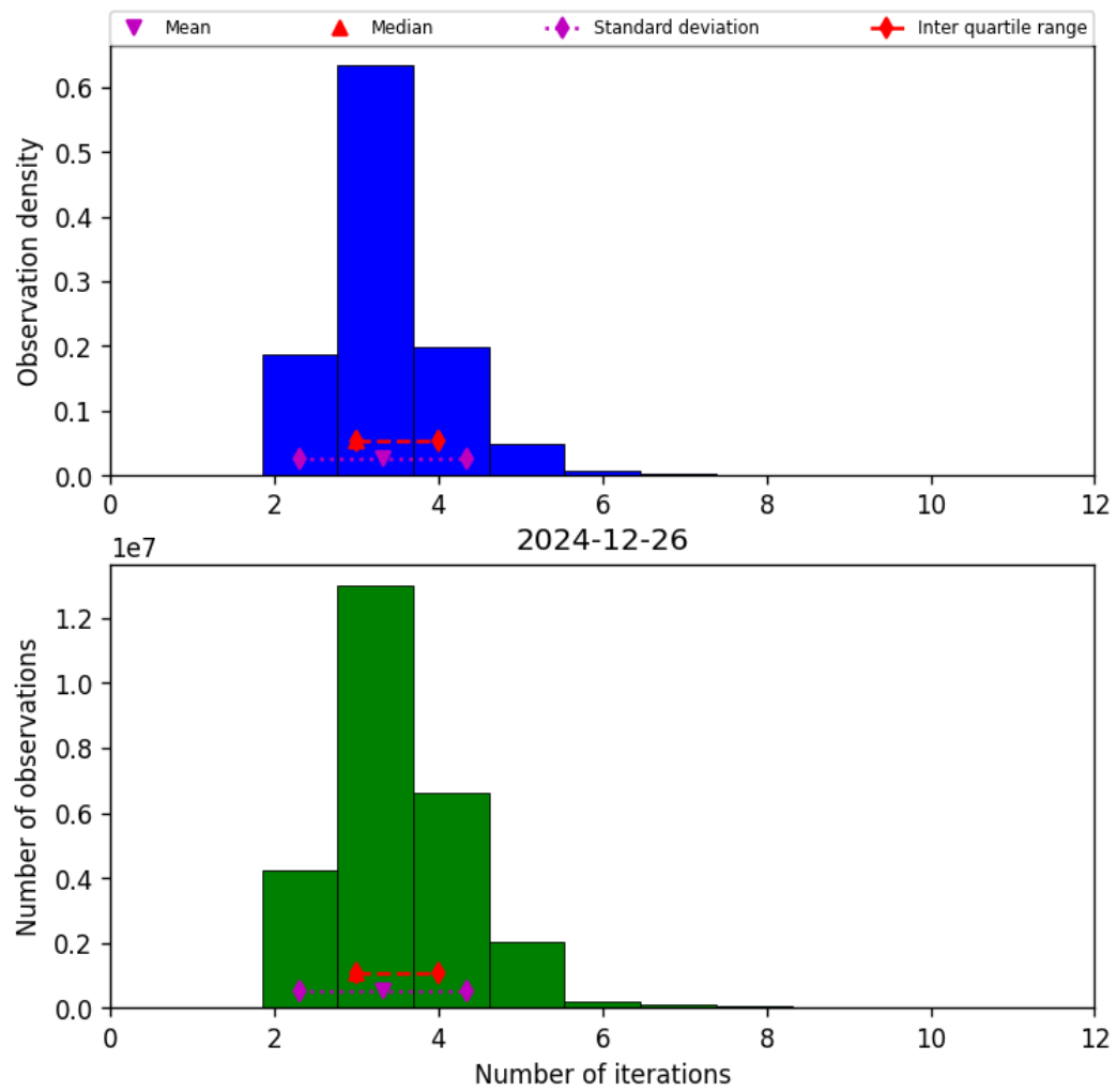
Figure 39: Histogram of “Number of iterations” for 2024-12-25 to 2024-12-27
