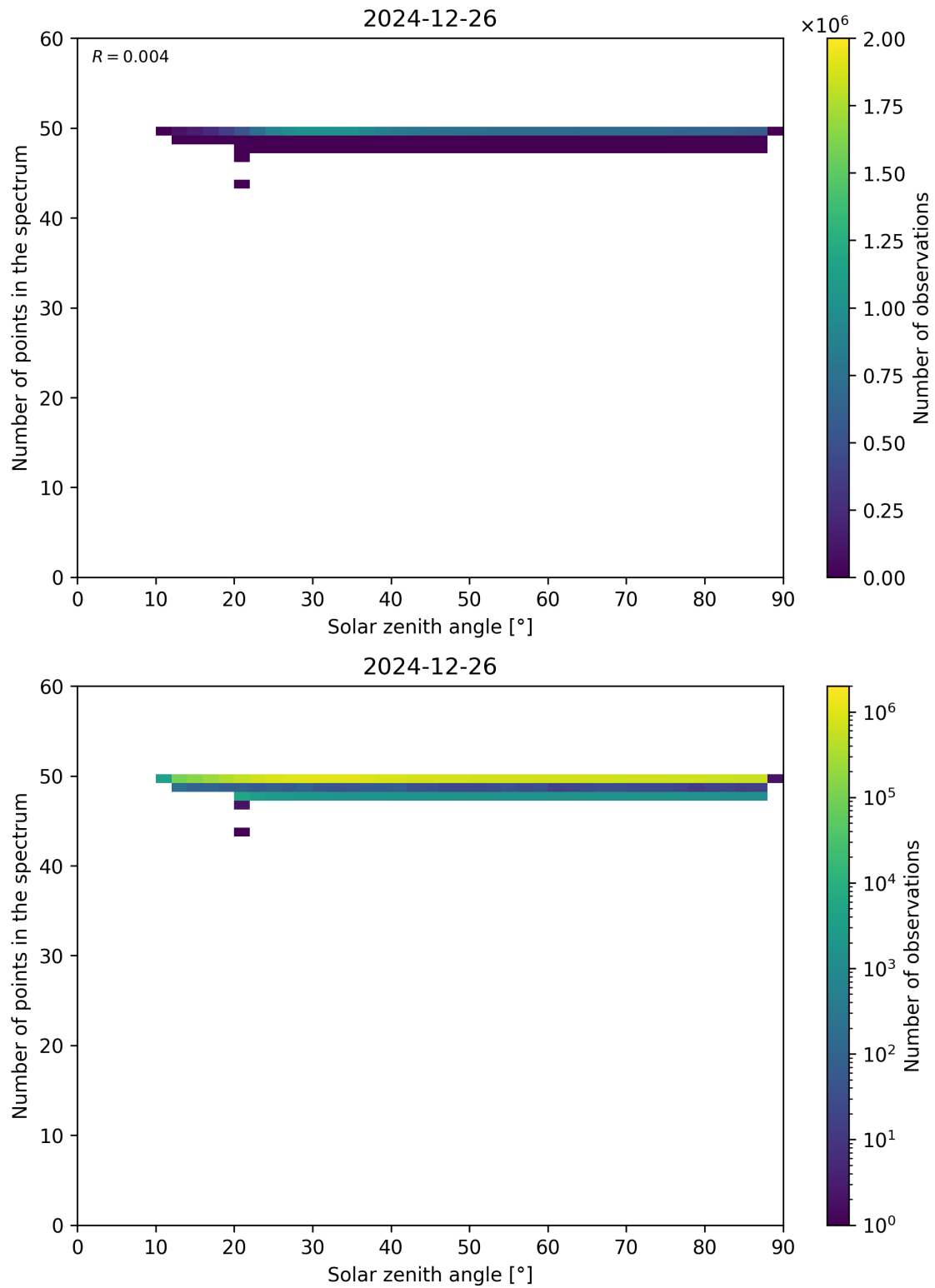
Figure 115: Scatter density plot of “Solar zenith angle” against “Number of points in the spectrum” for 2024-12-25 to 2024-12-27.
