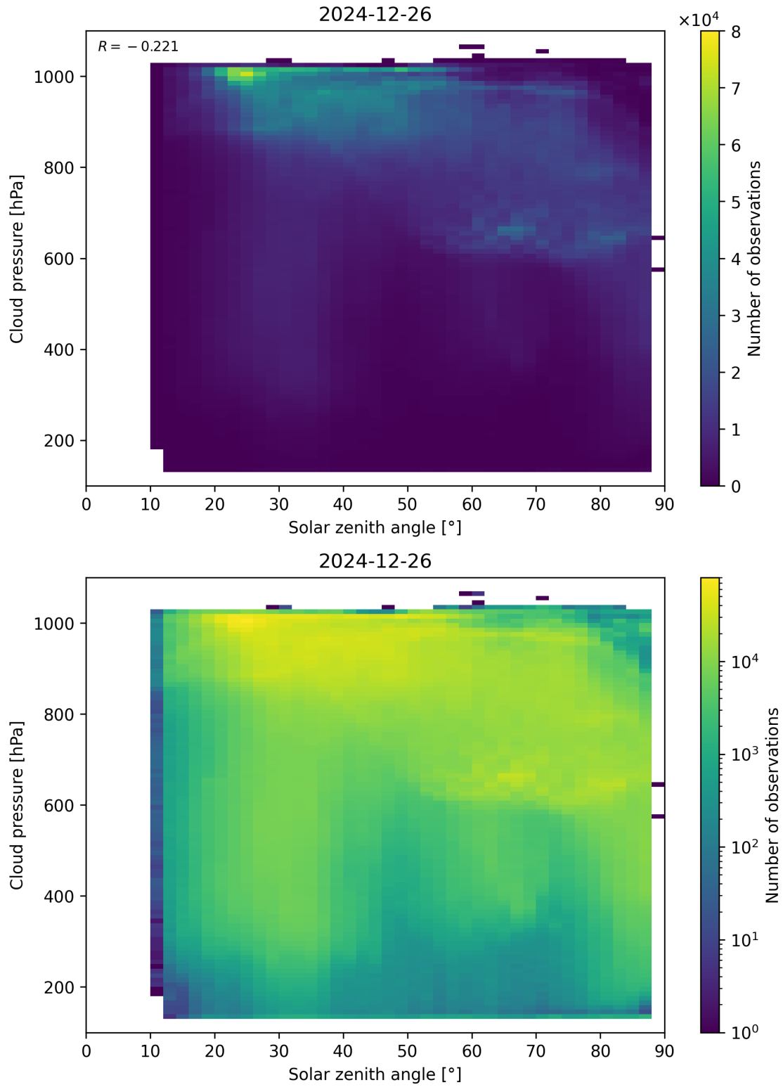
Figure 111: Scatter density plot of “Solar zenith angle” against “Cloud pressure” for 2024-12-25 to 2024-12-27.
