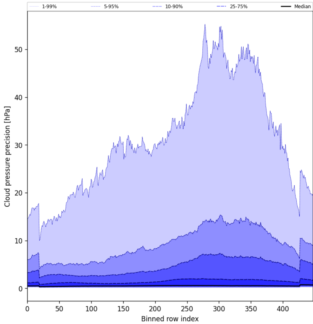
Figure 48: Along track statistics of “Cloud pressure precision” for 2024-12-27 to 2024-12-29
