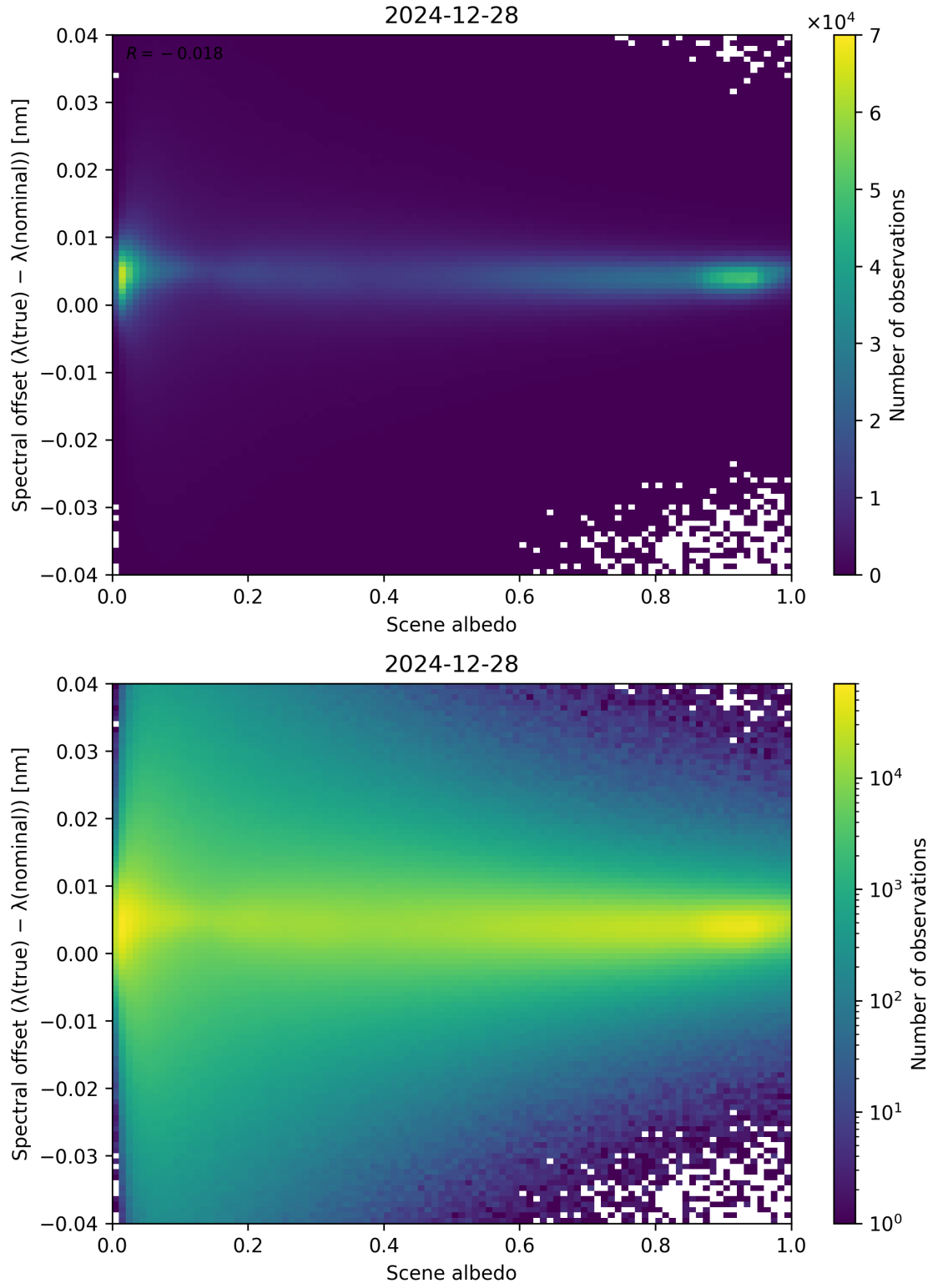
Figure 107: Scatter density plot of “Scene albedo” against “Spectral offset ( \lambda_{\text{true}} - \lambda_{\text{nominal}} )” for 2024-12-27 to 2024-12-29.
