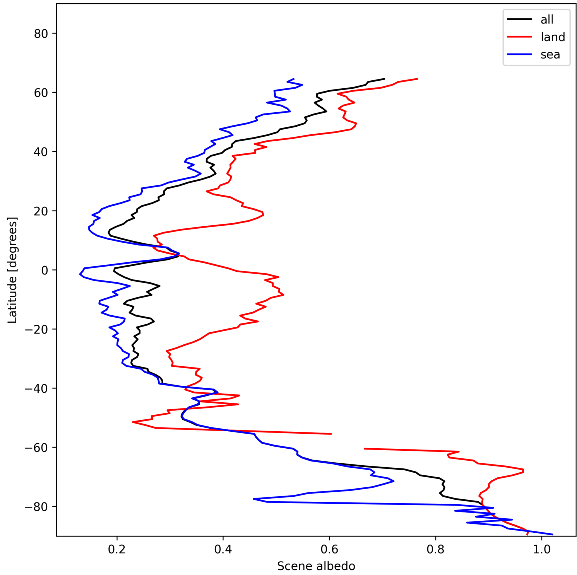
Figure 17: Zonal average of “Scene albedo” for 2024-12-27 to 2024-12-29.
