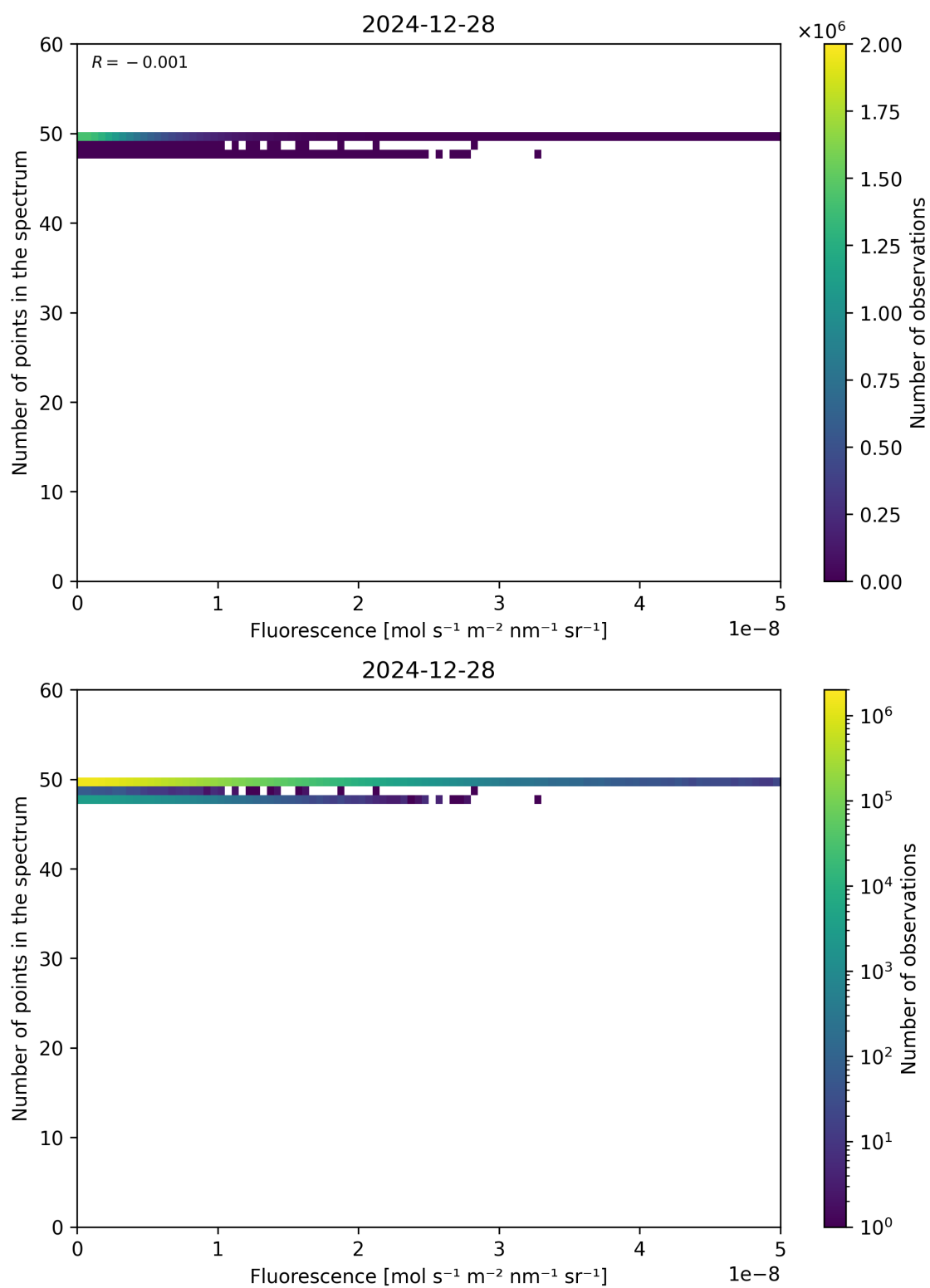
Figure 86: Scatter density plot of “Fluorescence” against “Number of points in the spectrum” for 2024-12-27 to 2024-12-29.
