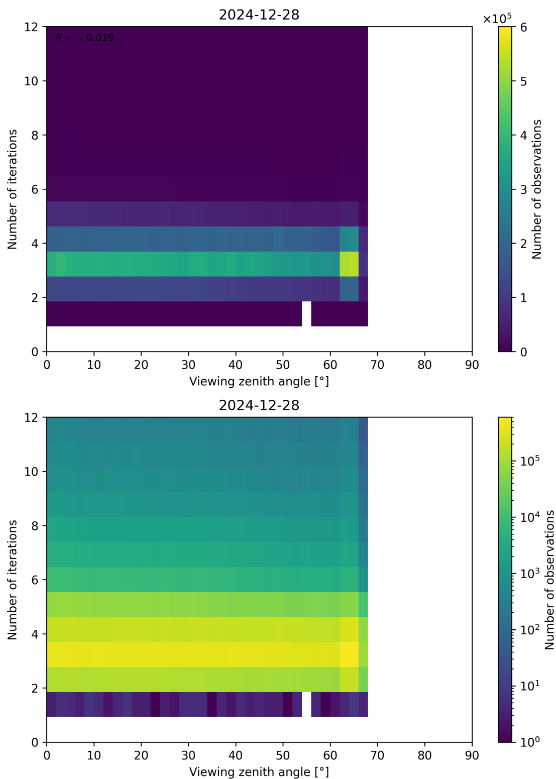
Figure 124: Scatter density plot of “Viewing zenith angle” against “Number of iterations” for 2024-12-27 to 2024-12-29.
