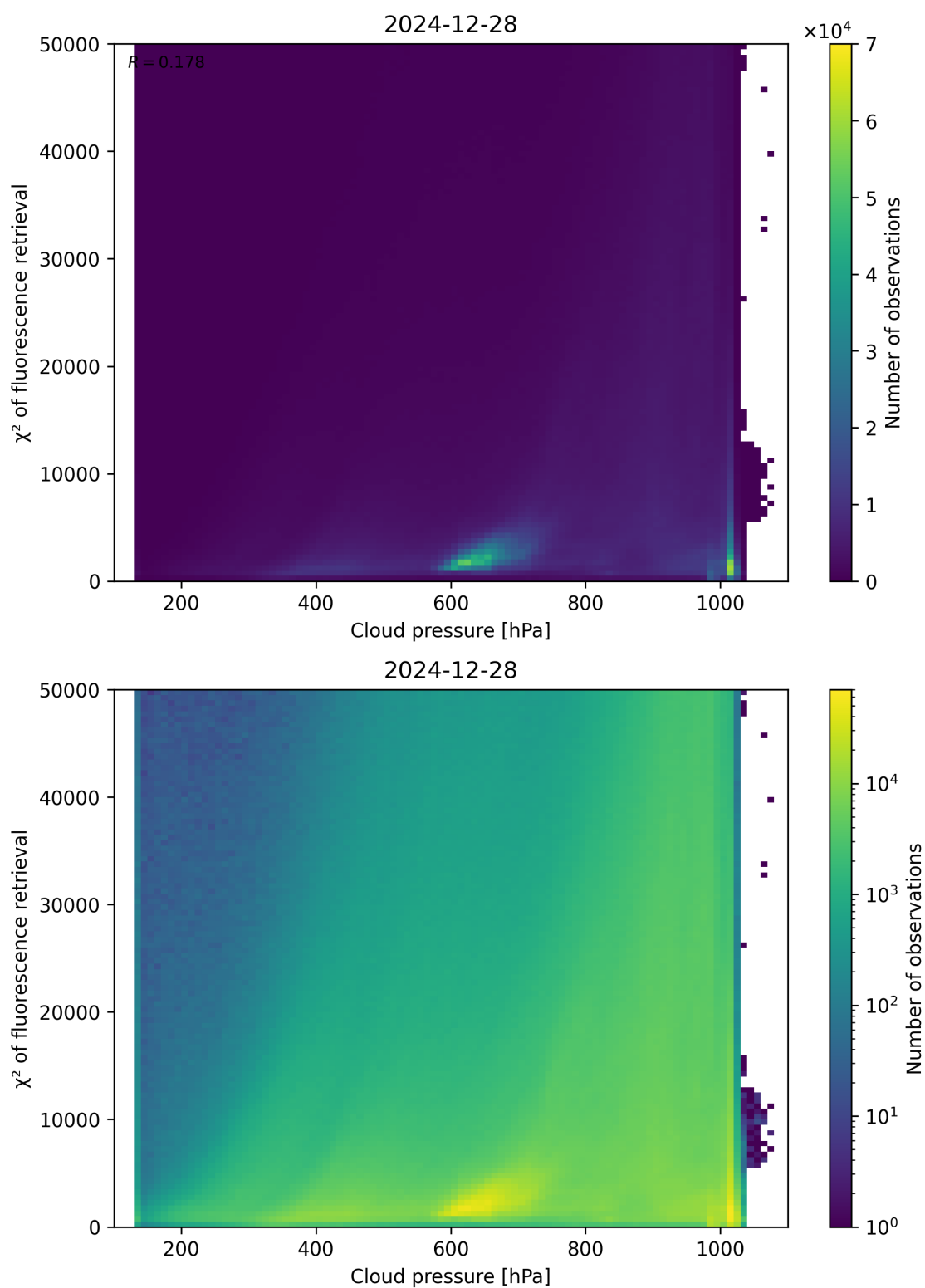
Figure 78: Scatter density plot of “Cloud pressure” against “ \chi^2 of fluorescence retrieval” for 2024-12-27 to 2024-12-29.
