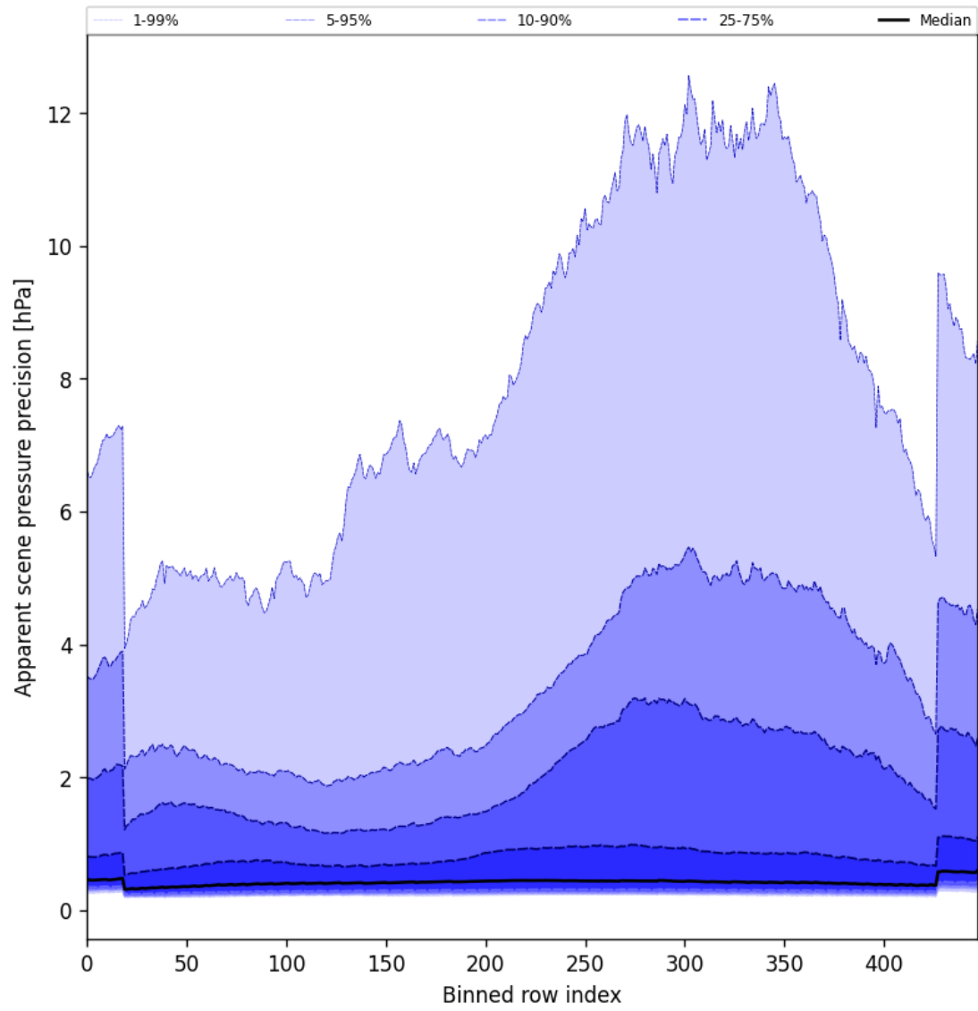
Figure 54: Along track statistics of “Apparent scene pressure precision” for 2024-12-27 to 2024-12-29
