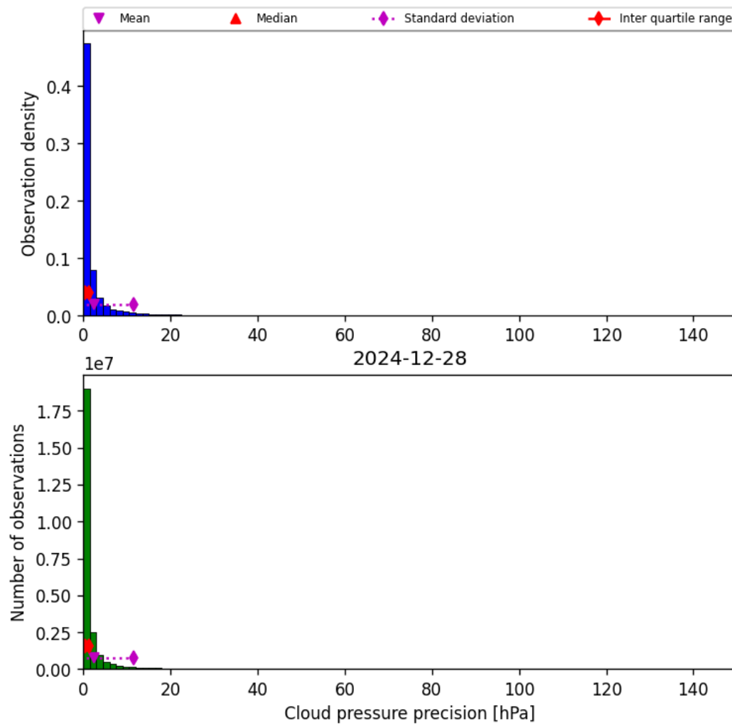
Figure 31: Histogram of “Cloud pressure precision” for 2024-12-27 to 2024-12-29
