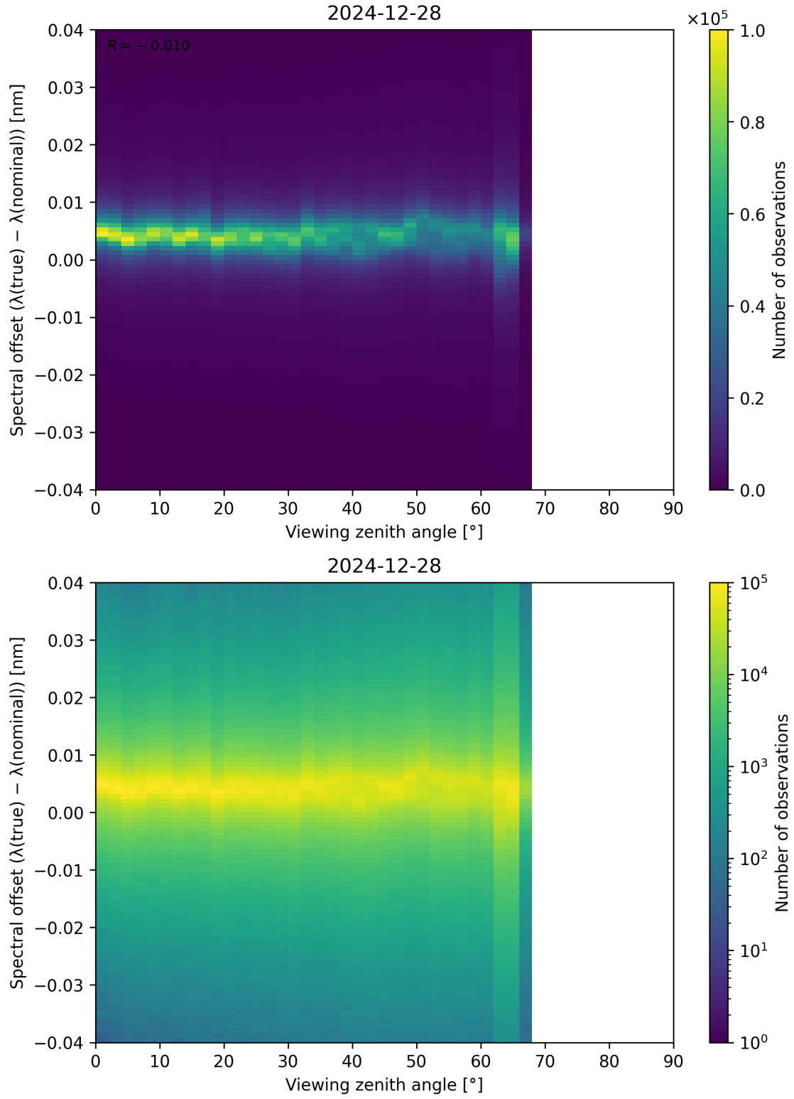
Figure 128: Scatter density plot of “Viewing zenith angle” against “Spectral offset ( \lambda_{\text{true}} - \lambda_{\text{nominal}} )” for 2024-12-27 to 2024-12-29.
