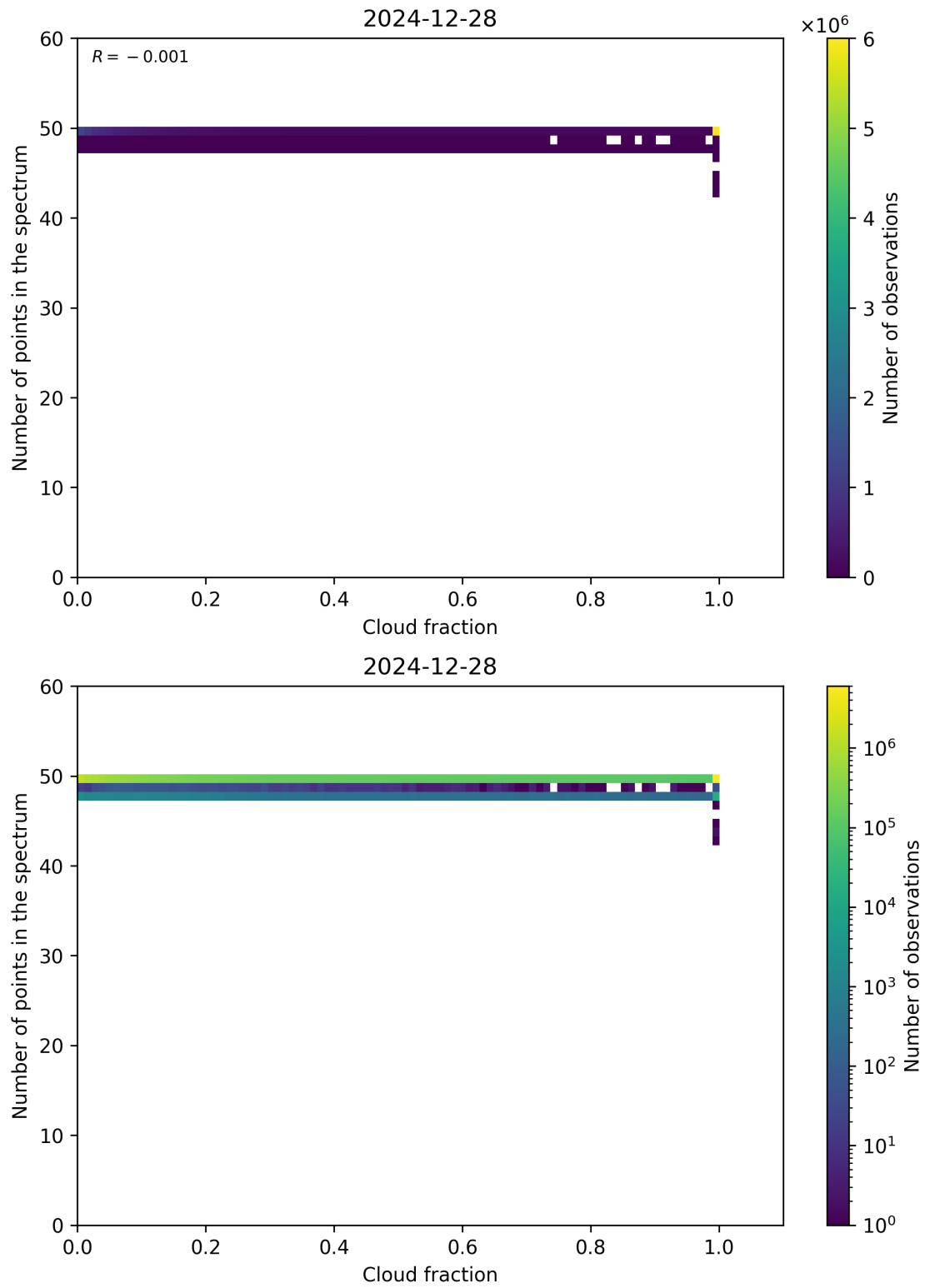
Figure 74: Scatter density plot of “Cloud fraction” against “Number of points in the spectrum” for 2024-12-27 to 2024-12-29.
