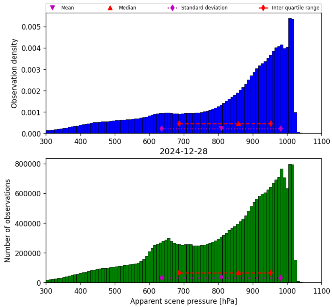
Figure 36: Histogram of “Apparent scene pressure” for 2024-12-27 to 2024-12-29
