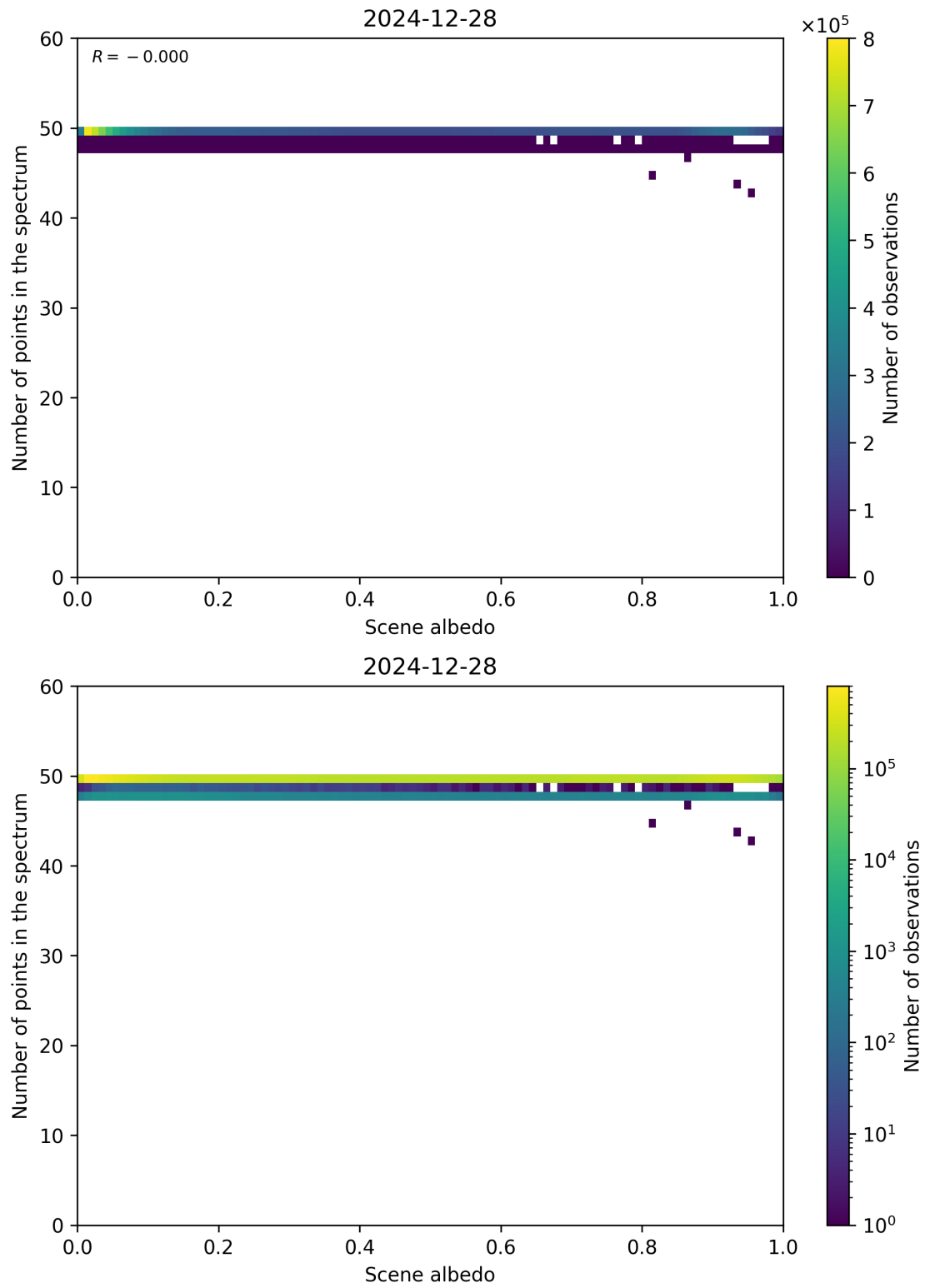
Figure 106: Scatter density plot of “Scene albedo” against “Number of points in the spectrum” for 2024-12-27 to 2024-12-29.
