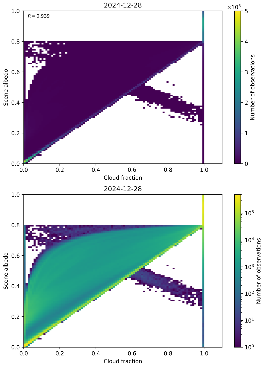
Figure 75: Scatter density plot of “Cloud fraction” against “Scene albedo” for 2024-12-27 to 2024-12-29.
