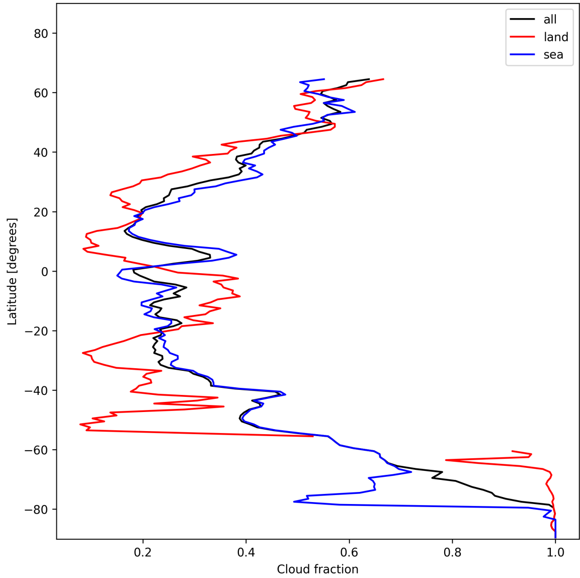
Figure 15: Zonal average of “Cloud fraction” for 2024-12-27 to 2024-12-29.
