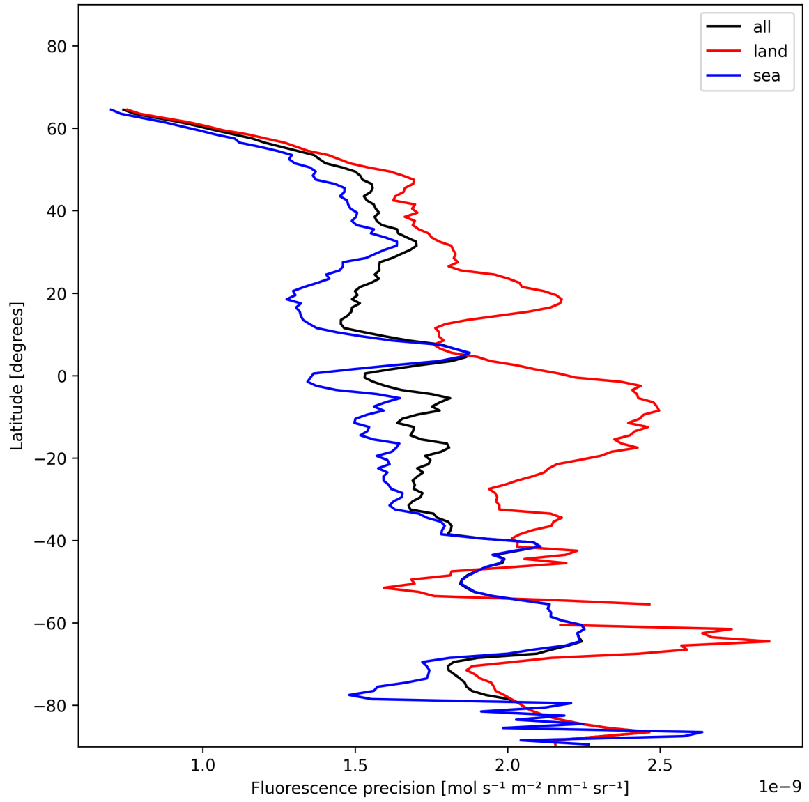
Figure 24: Zonal average of “Fluorescence precision” for 2024-12-27 to 2024-12-29.
