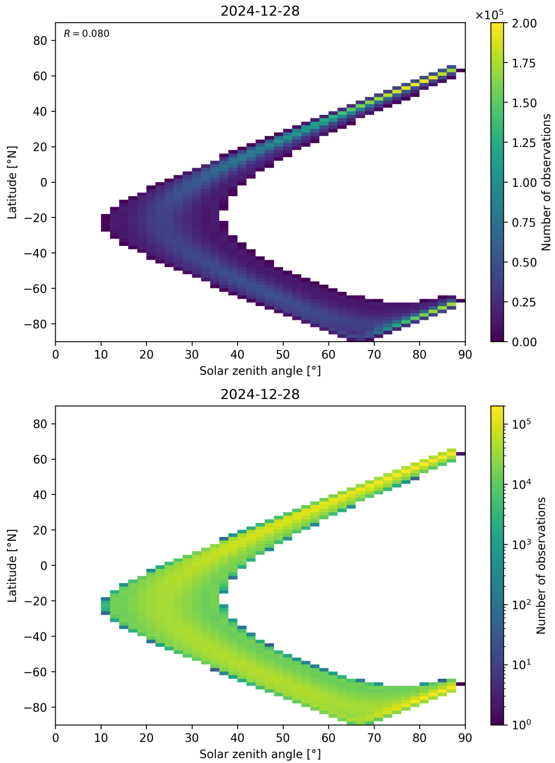
Figure 113: Scatter density plot of “Solar zenith angle” against “Latitude” for 2024-12-27 to 2024-12-29.
