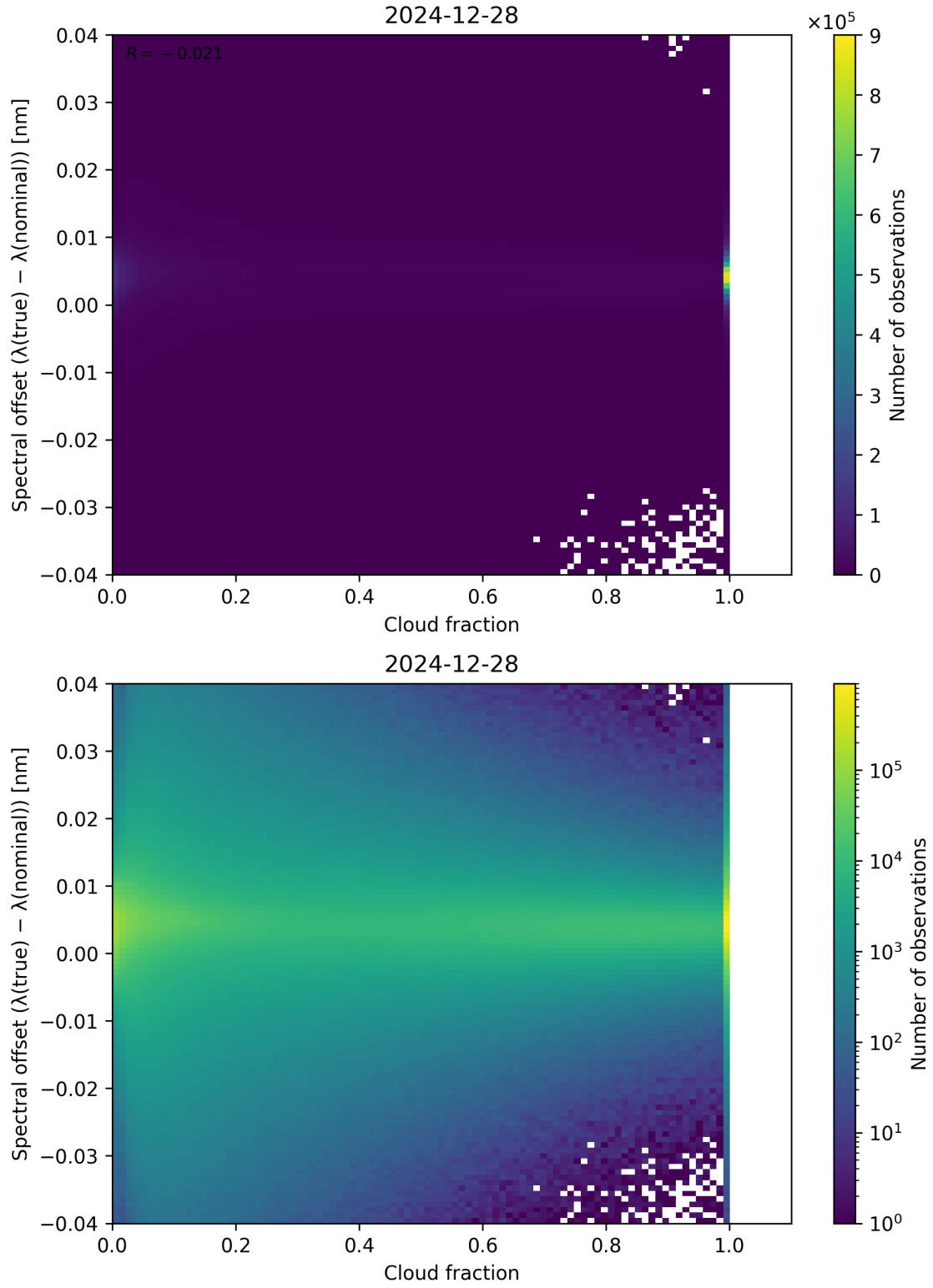
Figure 76: Scatter density plot of “Cloud fraction” against “Spectral offset ( \lambda_{\text{true}} - \lambda_{\text{nominal}} )” for 2024-12-27 to 2024-12-29.
