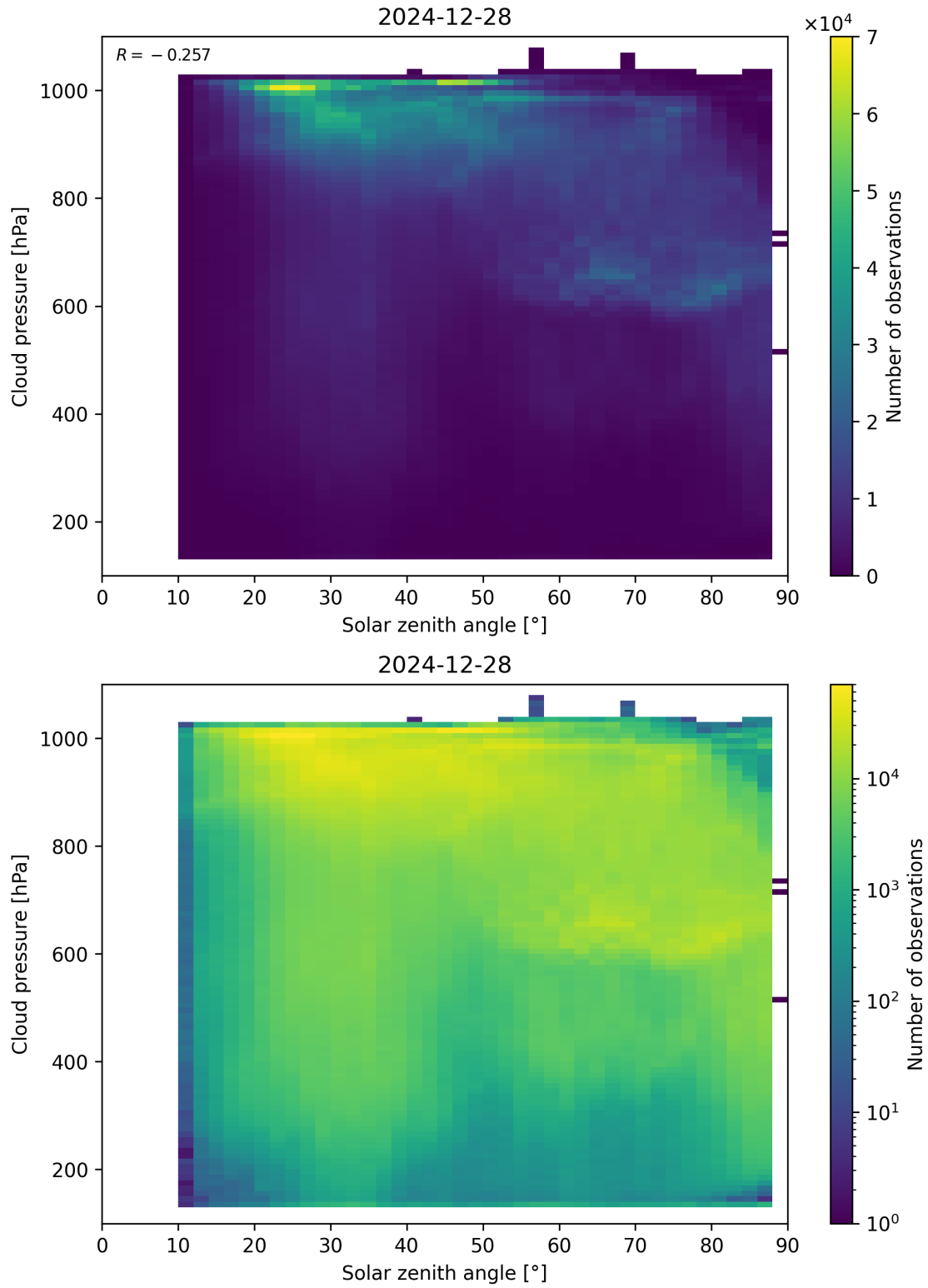
Figure 111: Scatter density plot of “Solar zenith angle” against “Cloud pressure” for 2024-12-27 to 2024-12-29.
