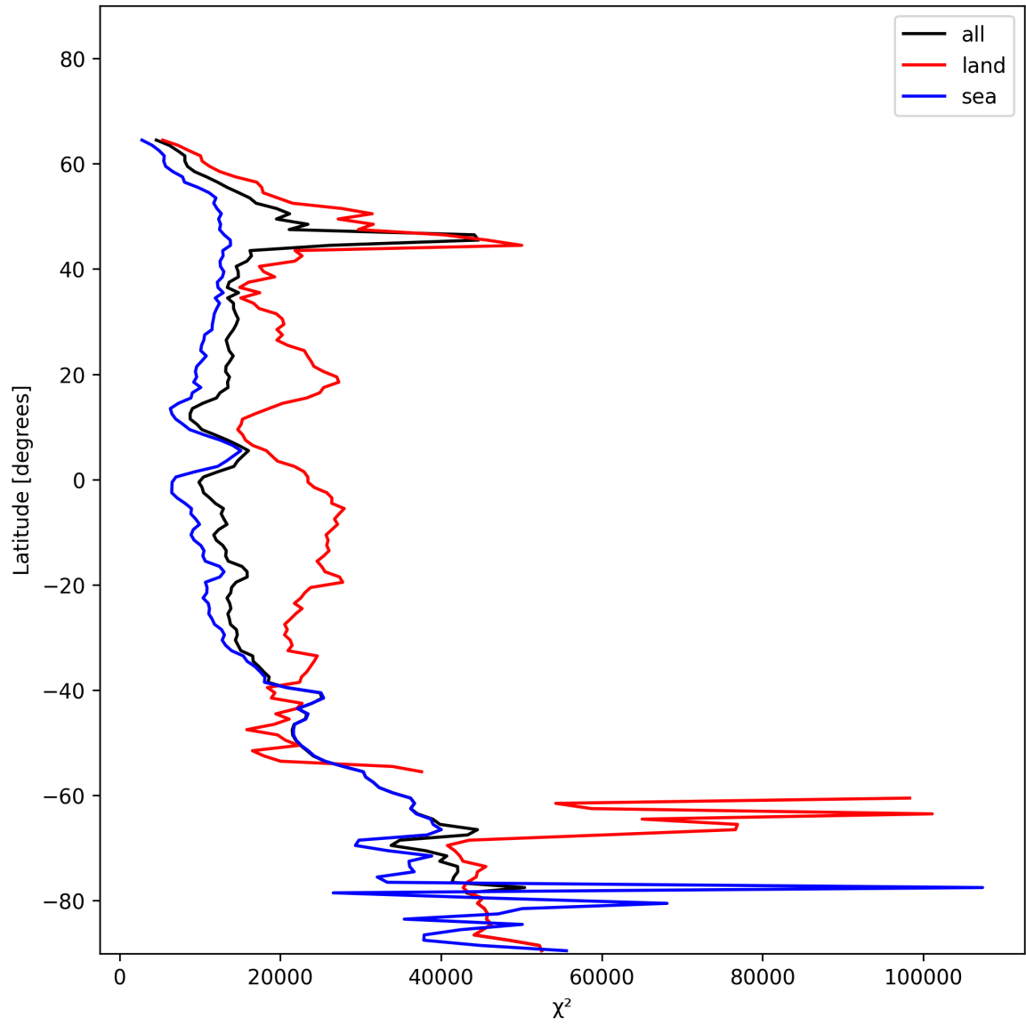
Figure 21: Zonal average of “ \chi^2 ” for 2024-12-27 to 2024-12-29.
