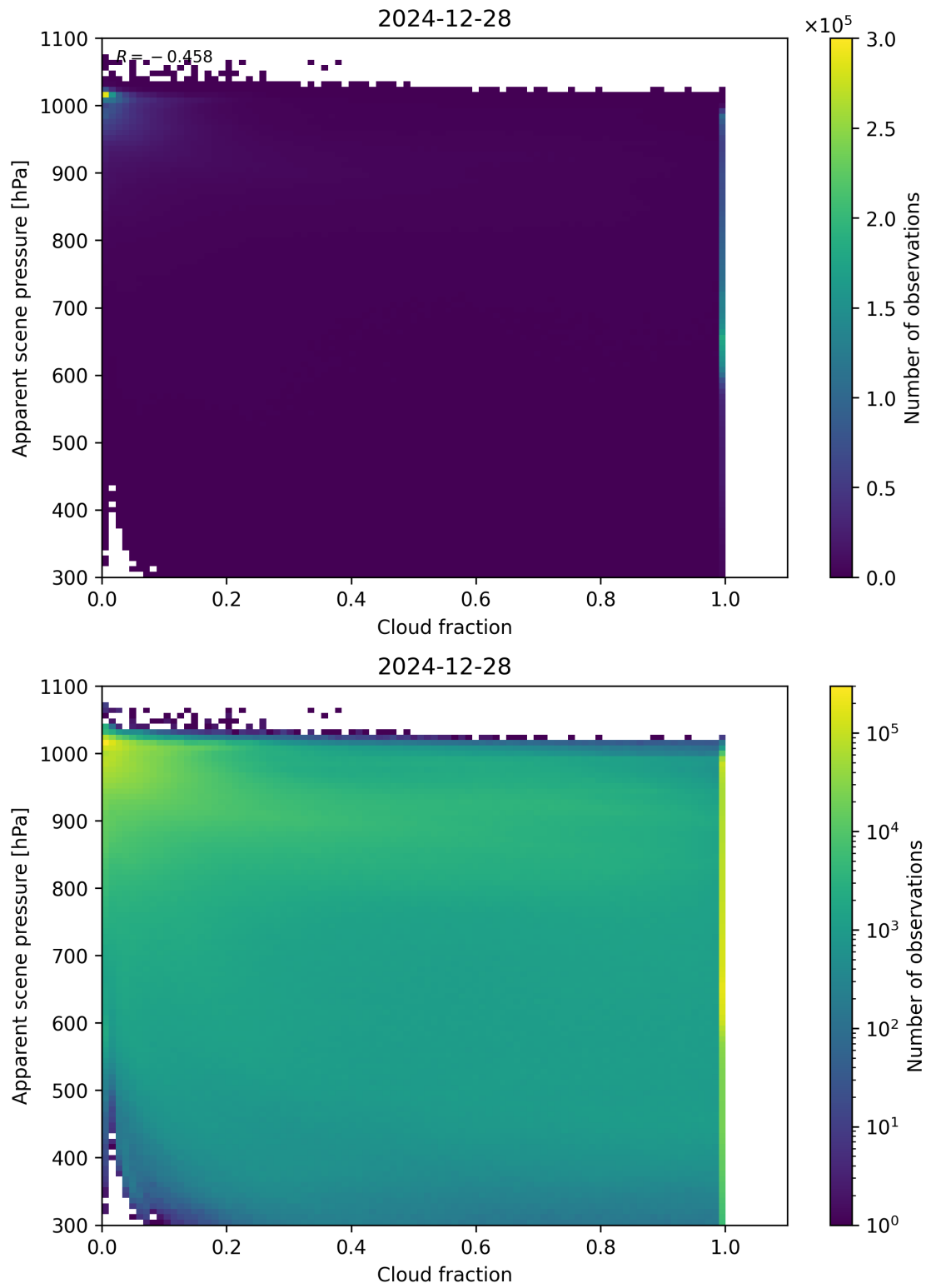
Figure 70: Scatter density plot of “Cloud fraction” against “Apparent scene pressure” for 2024-12-27 to 2024-12-29.
