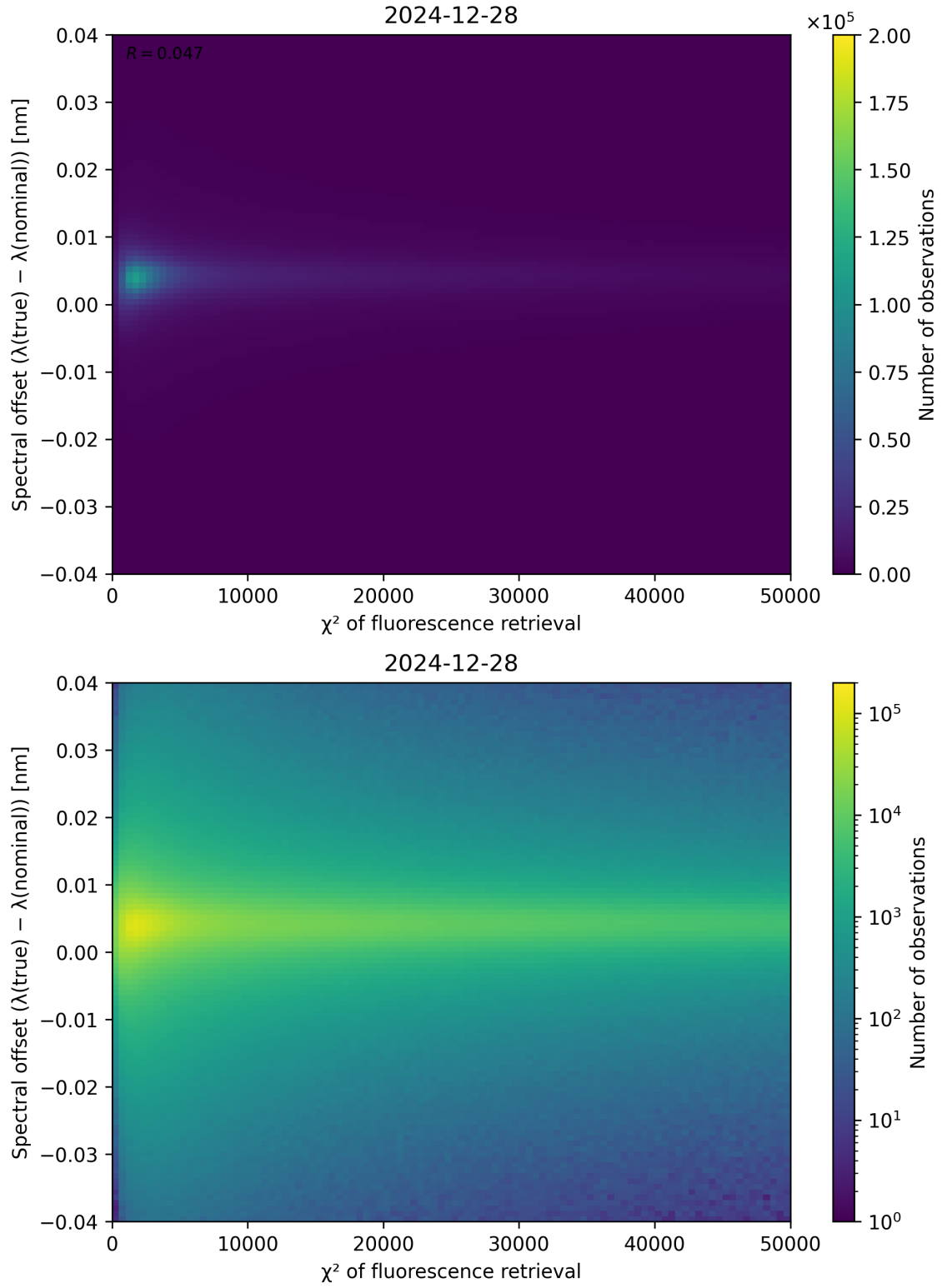
Figure 69: Scatter density plot of “ \chi^2 of fluorescence retrieval” against “Spectral offset ( \lambda_{\text{true}} - \lambda_{\text{nominal}} )” for 2024-12-27 to 2024-12-29.
