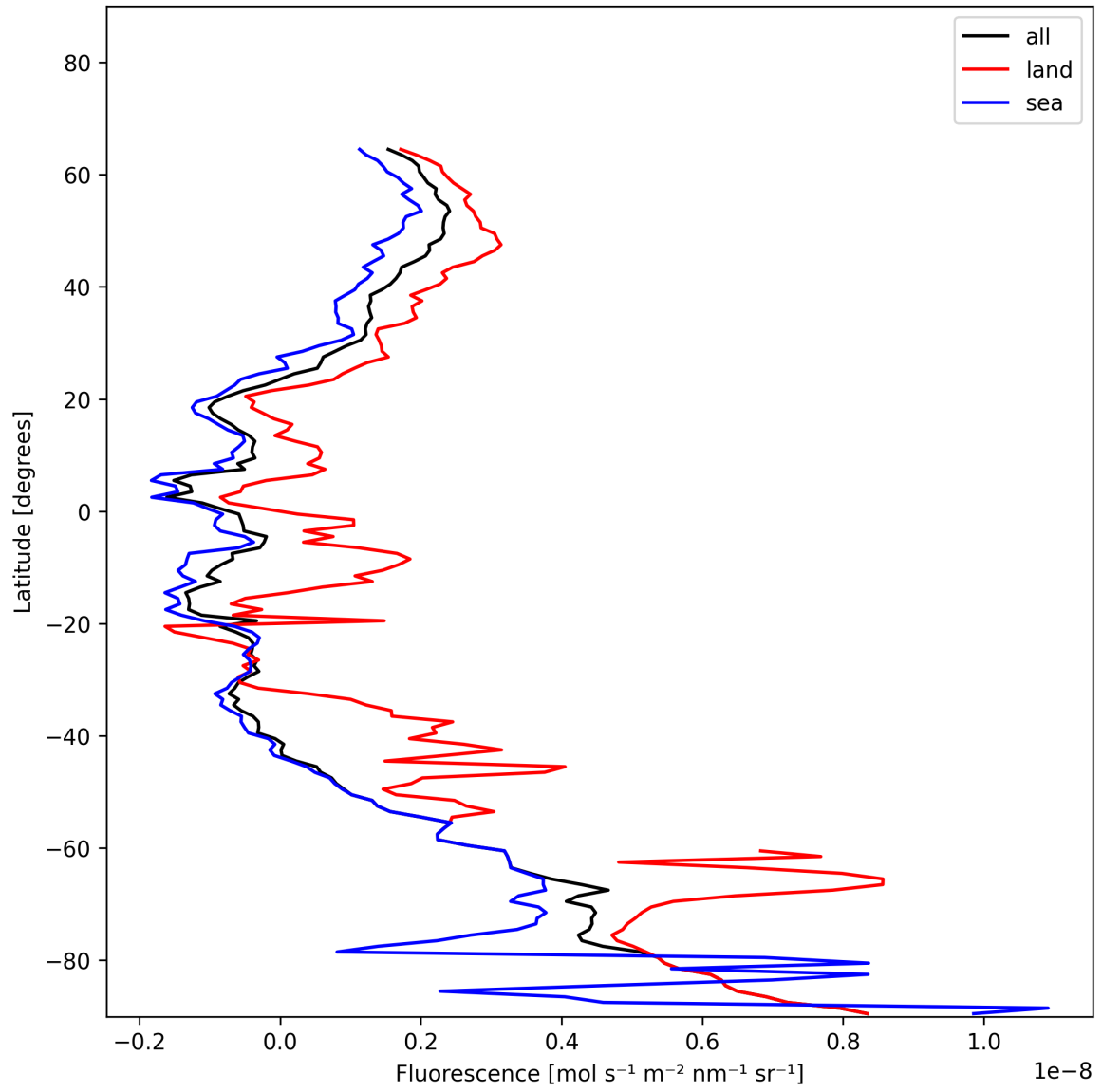
Figure 23: Zonal average of “Fluorescence” for 2024-12-27 to 2024-12-29.
