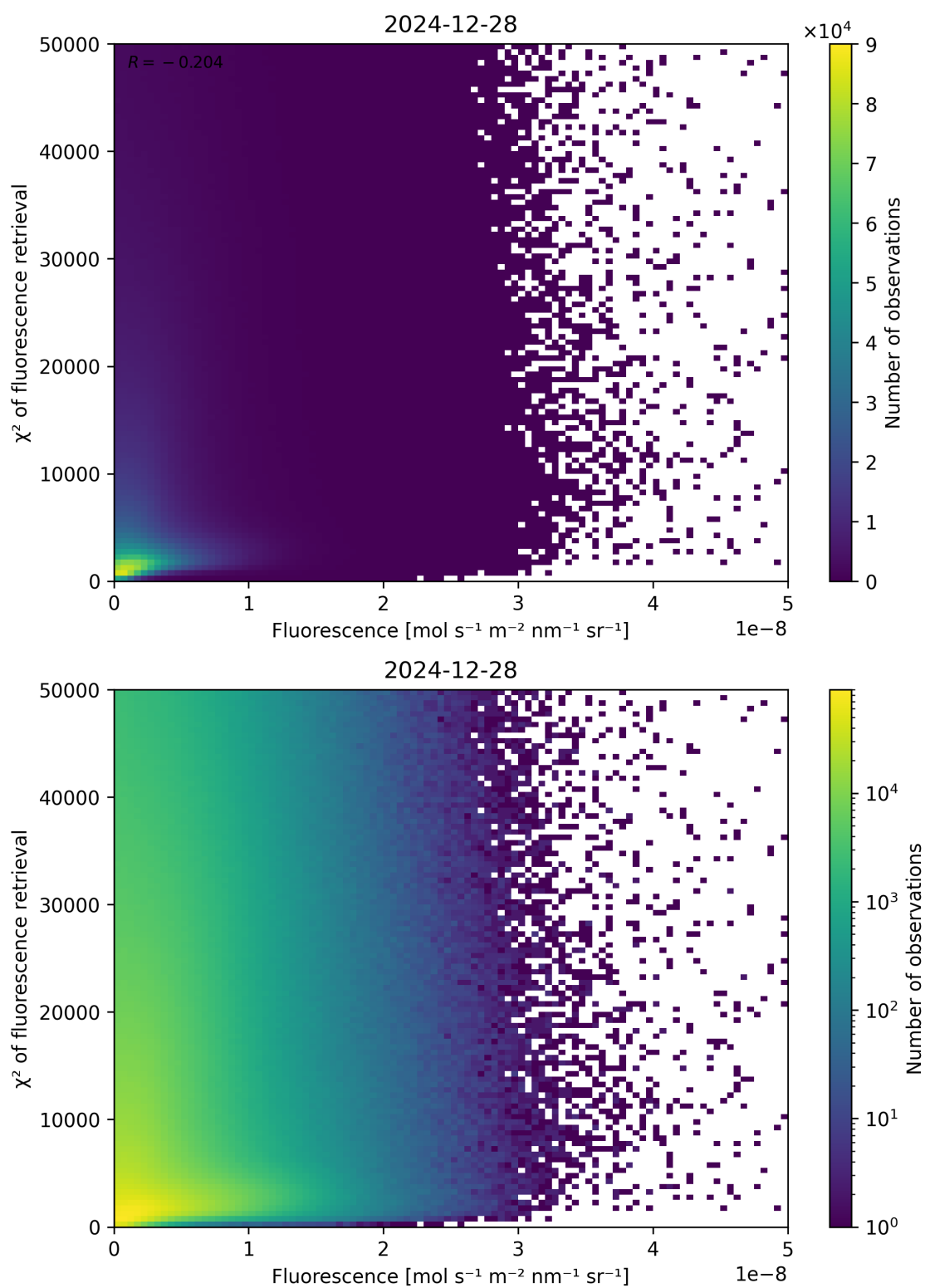
Figure 85: Scatter density plot of “Fluorescence” against “ \chi^2 of fluorescence retrieval” for 2024-12-27 to 2024-12-29.
