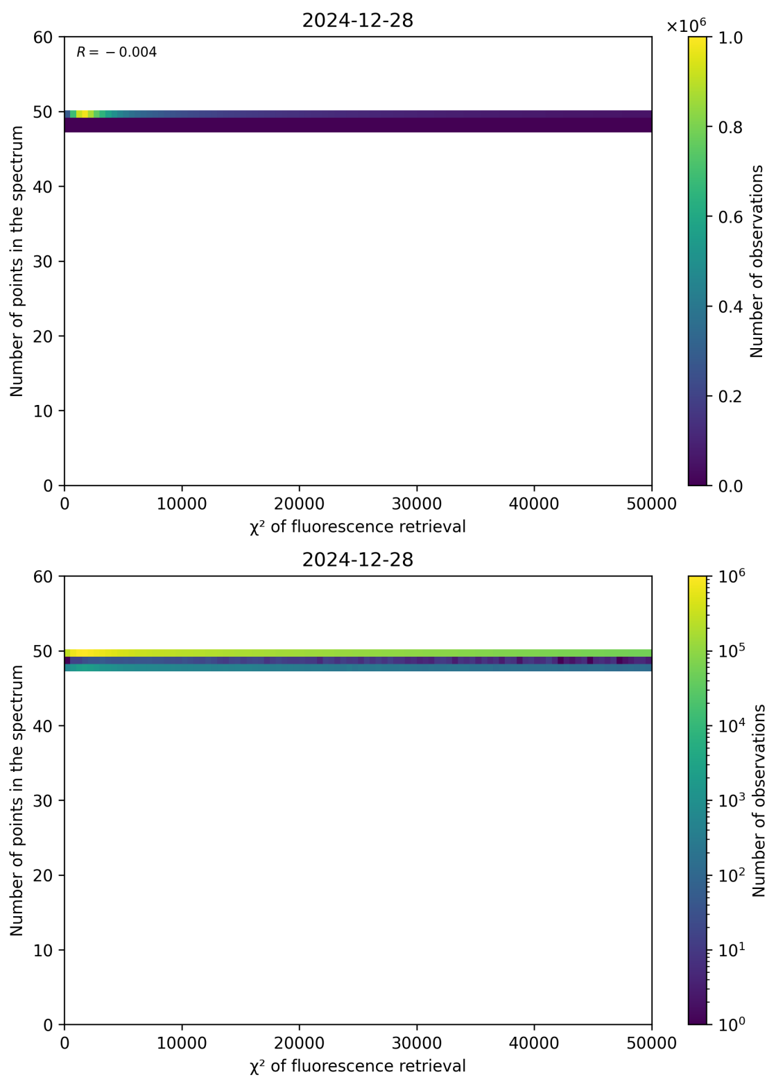
Figure 68: Scatter density plot of “ \chi^2 of fluorescence retrieval” against “Number of points in the spectrum” for 2024-12-27 to 2024-12-29.
