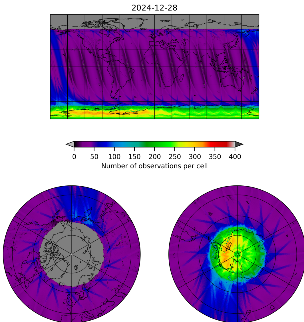
Figure 11: Map of the number of observations for 2024-12-27 to 2024-12-29
