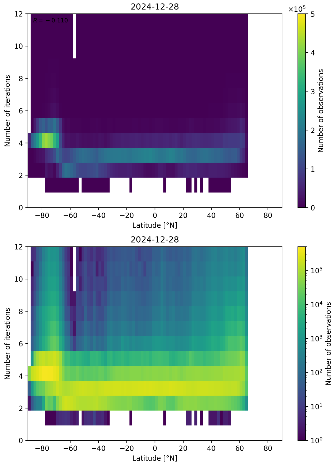
Figure 93: Scatter density plot of “Latitude” against “Number of iterations” for 2024-12-27 to 2024-12-29.
