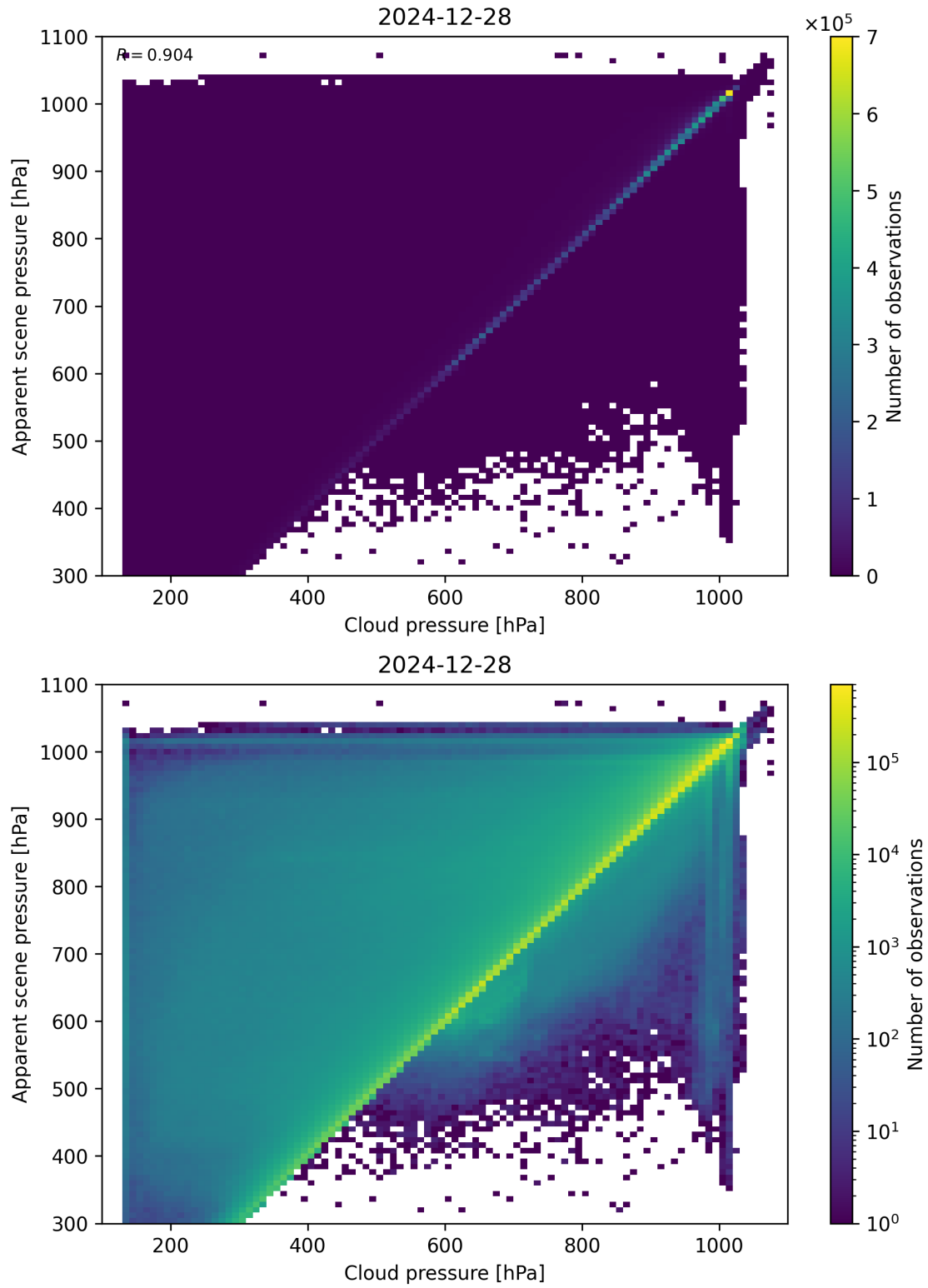
Figure 77: Scatter density plot of “Cloud pressure” against “Apparent scene pressure” for 2024-12-27 to 2024-12-29.
