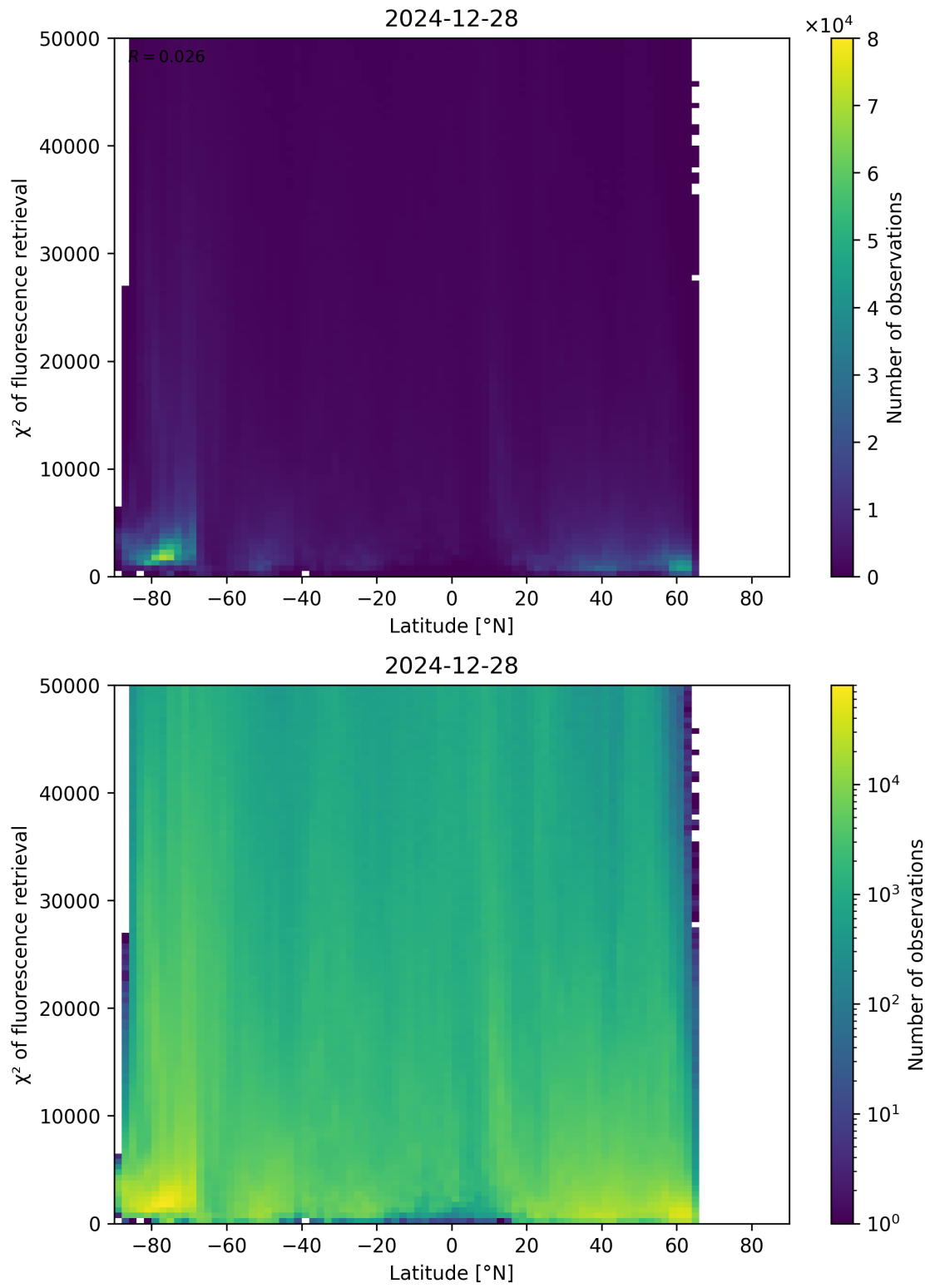
Figure 89: Scatter density plot of “Latitude” against “ \chi^2 of fluorescence retrieval” for 2024-12-27 to 2024-12-29.
