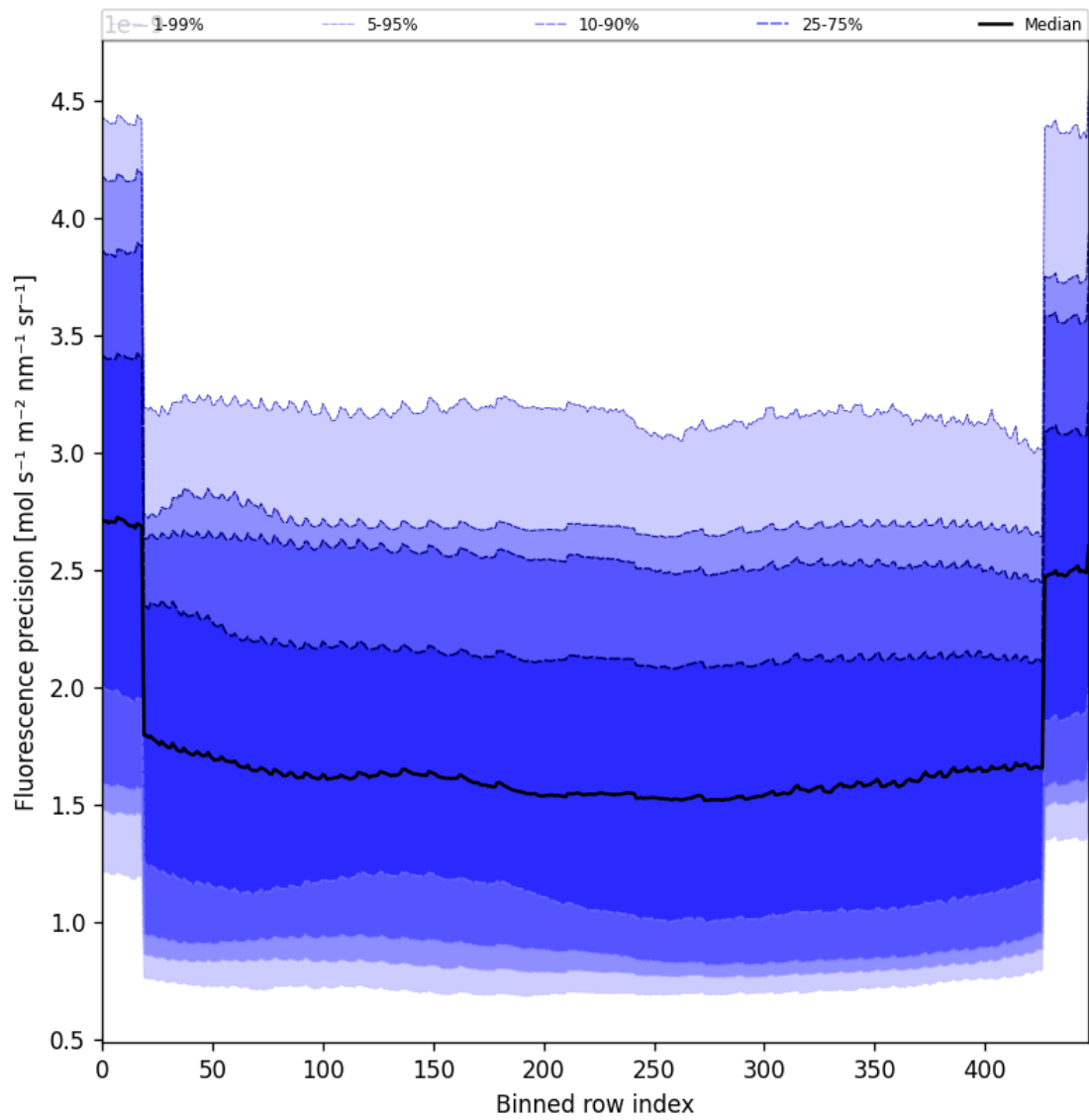
Figure 58: Along track statistics of “Fluorescence precision” for 2024-12-27 to 2024-12-29
