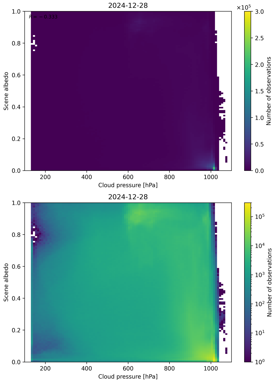
Figure 83: Scatter density plot of “Cloud pressure” against “Scene albedo” for 2024-12-27 to 2024-12-29.
