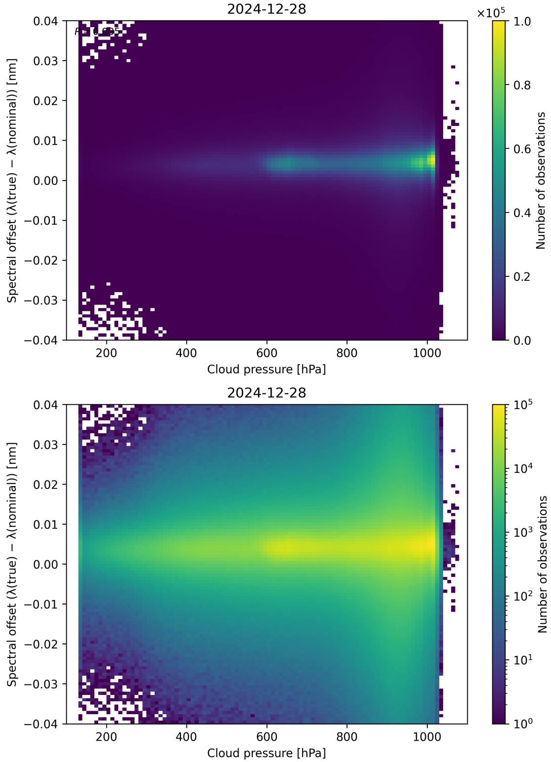
Figure 84: Scatter density plot of “Cloud pressure” against “Spectral offset ( \lambda_{\text{true}} - \lambda_{\text{nominal}} )” for 2024-12-27 to 2024-12-29.
