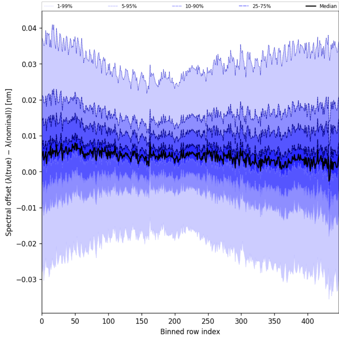
Figure 62: Along track statistics of “Spectral offset ( \lambda_{\text{true}} - \lambda_{\text{nominal}} )” for 2024-12-27 to 2024-12-29
