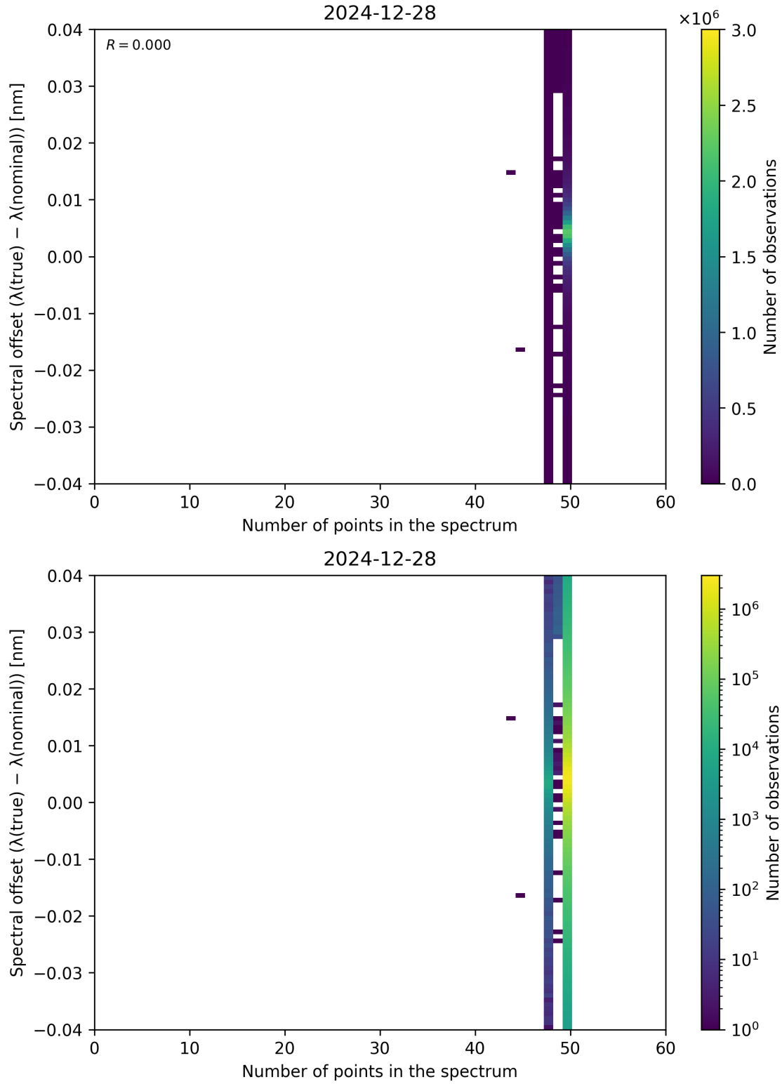
Figure 101: Scatter density plot of “Number of points in the spectrum” against “Spectral offset ( \lambda_{\text{true}} - \lambda_{\text{nominal}} )” for 2024-12-27 to 2024-12-29.
