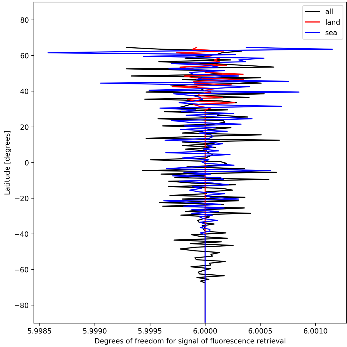
Figure 26: Zonal average of “Degrees of freedom for signal of fluorescence retrieval” for 2024-12-27 to 2024-12-29.
