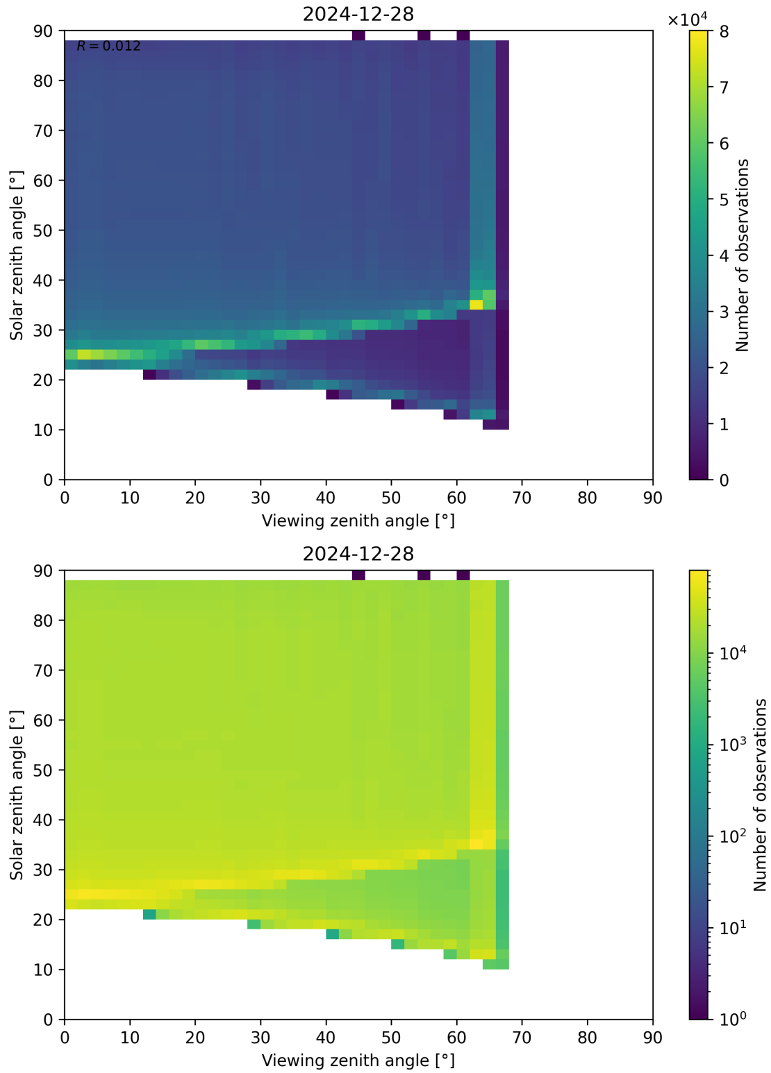
Figure 127: Scatter density plot of “Viewing zenith angle” against “Solar zenith angle” for 2024-12-27 to 2024-12-29.
