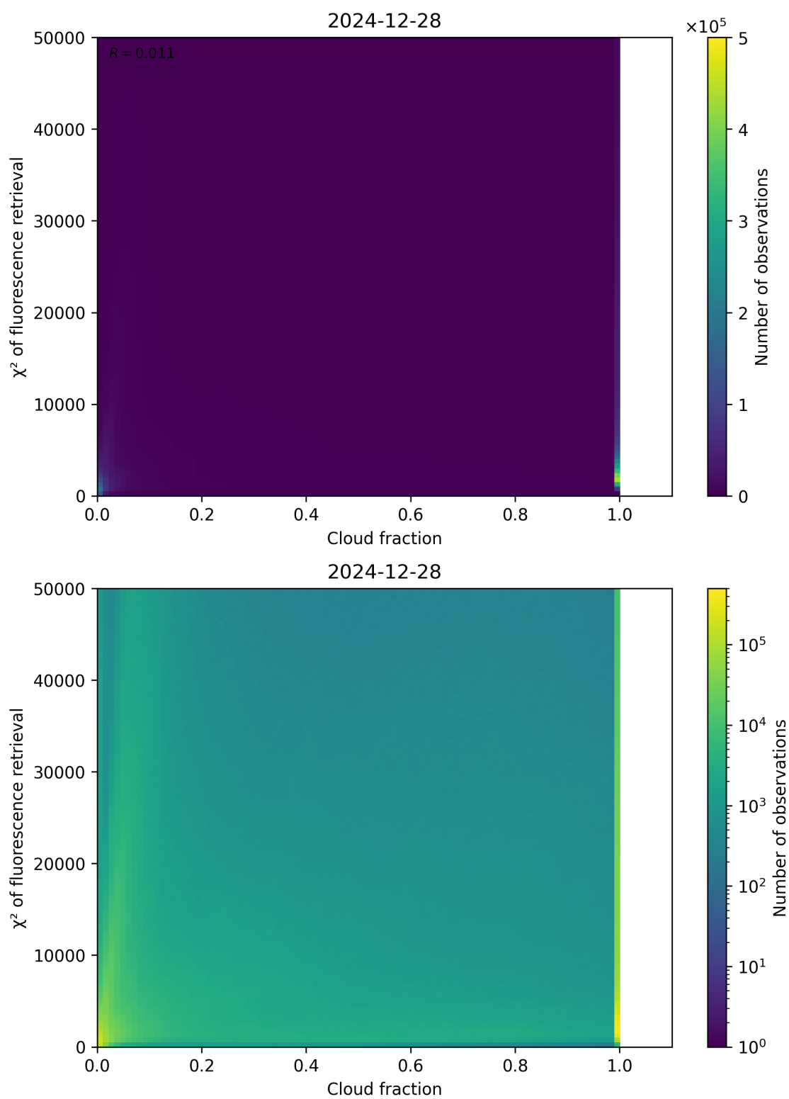
Figure 71: Scatter density plot of “Cloud fraction” against “ \chi^2 of fluorescence retrieval” for 2024-12-27 to 2024-12-29.
