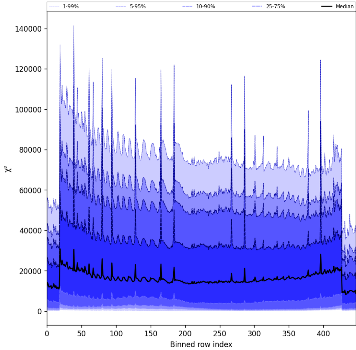
Figure 55: Along track statistics of “ \chi^2 ” for 2024-12-27 to 2024-12-29
