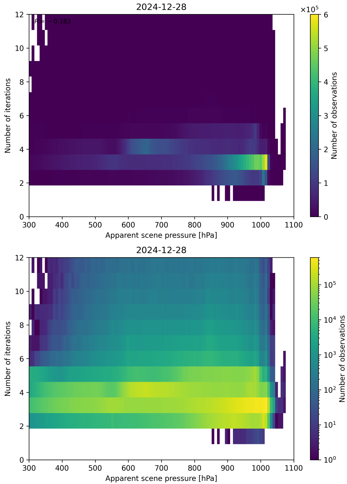
Figure 65: Scatter density plot of “Apparent scene pressure” against “Number of iterations” for 2024-12-27 to 2024-12-29.
