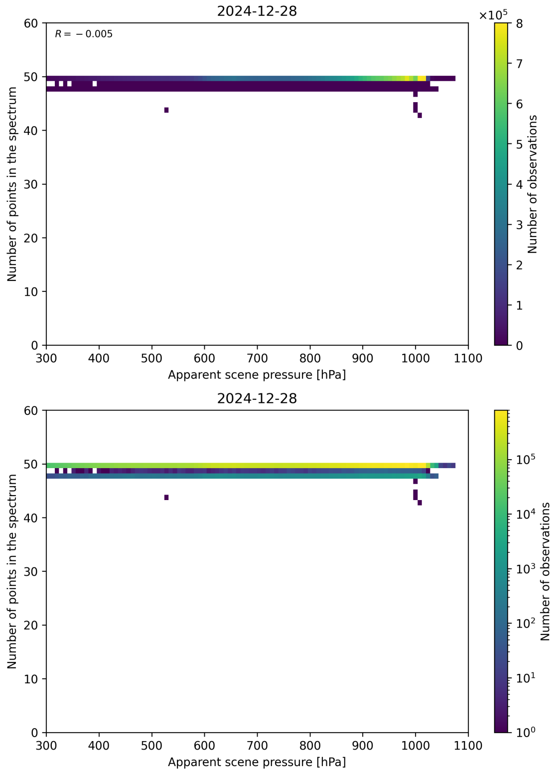
Figure 66: Scatter density plot of “Apparent scene pressure” against “Number of points in the spectrum” for 2024-12-27 to 2024-12-29.
