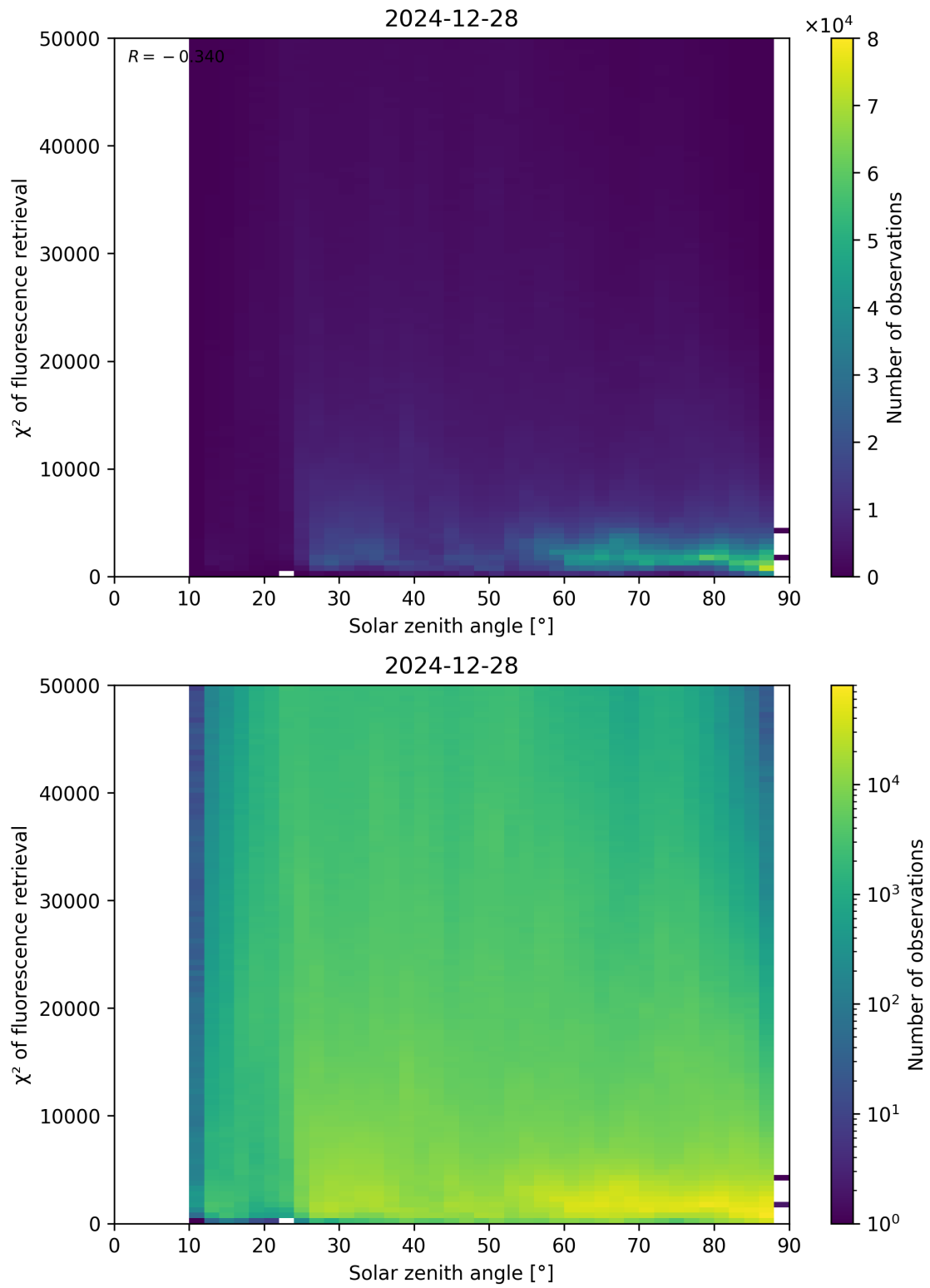
Figure 109: Scatter density plot of “Solar zenith angle” against “ \chi^2 of fluorescence retrieval” for 2024-12-27 to 2024-12-29.
