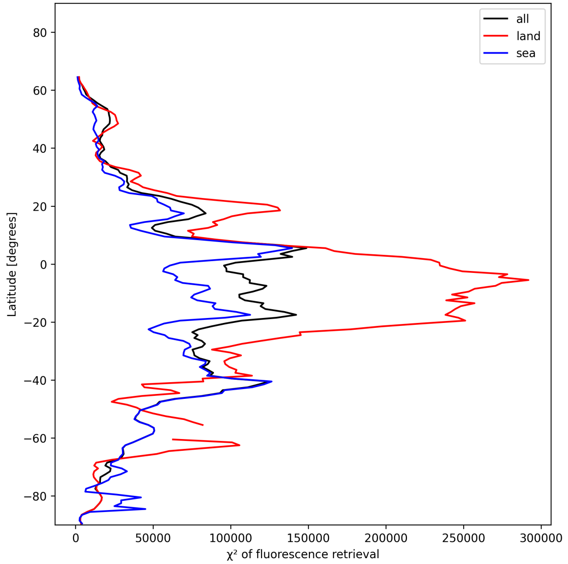
Figure 25: Zonal average of “ \chi^2 of fluorescence retrieval” for 2024-12-27 to 2024-12-29.
