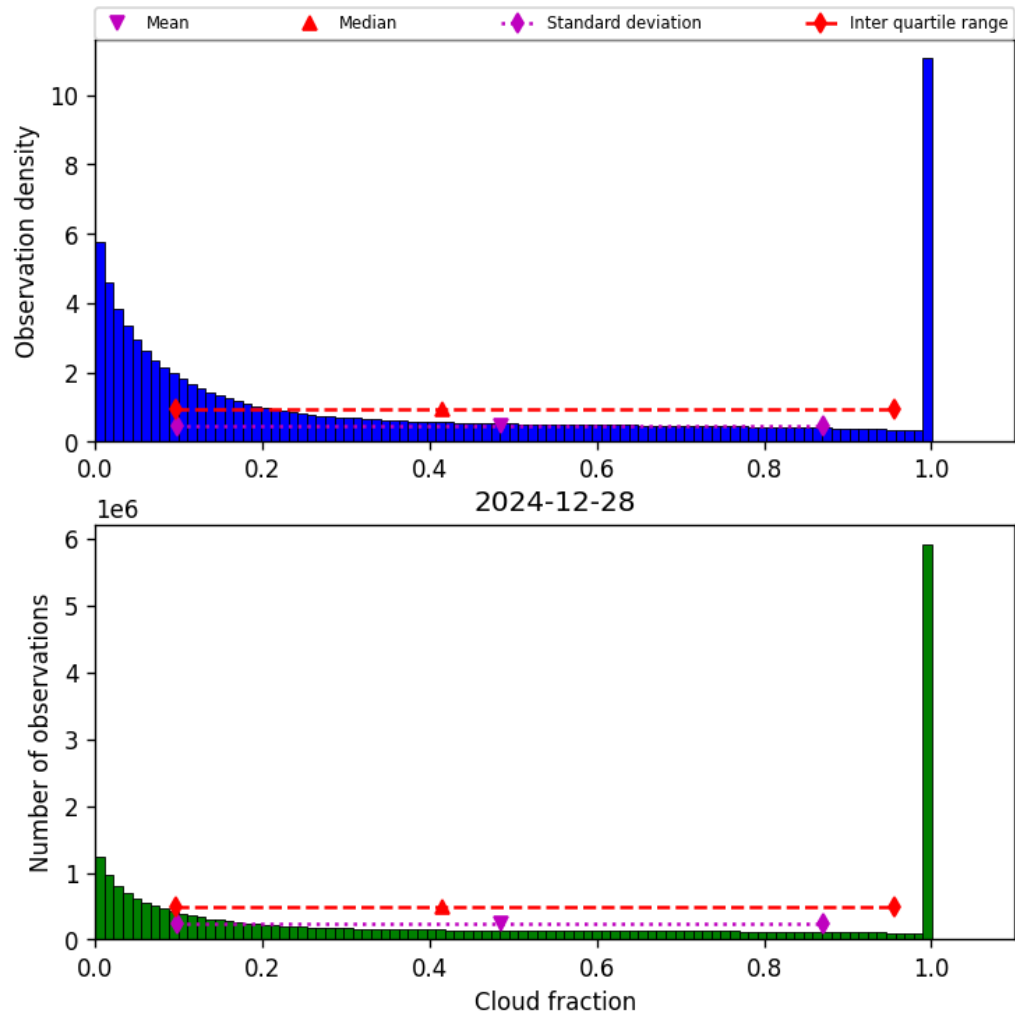
Figure 32: Histogram of “Cloud fraction” for 2024-12-27 to 2024-12-29
