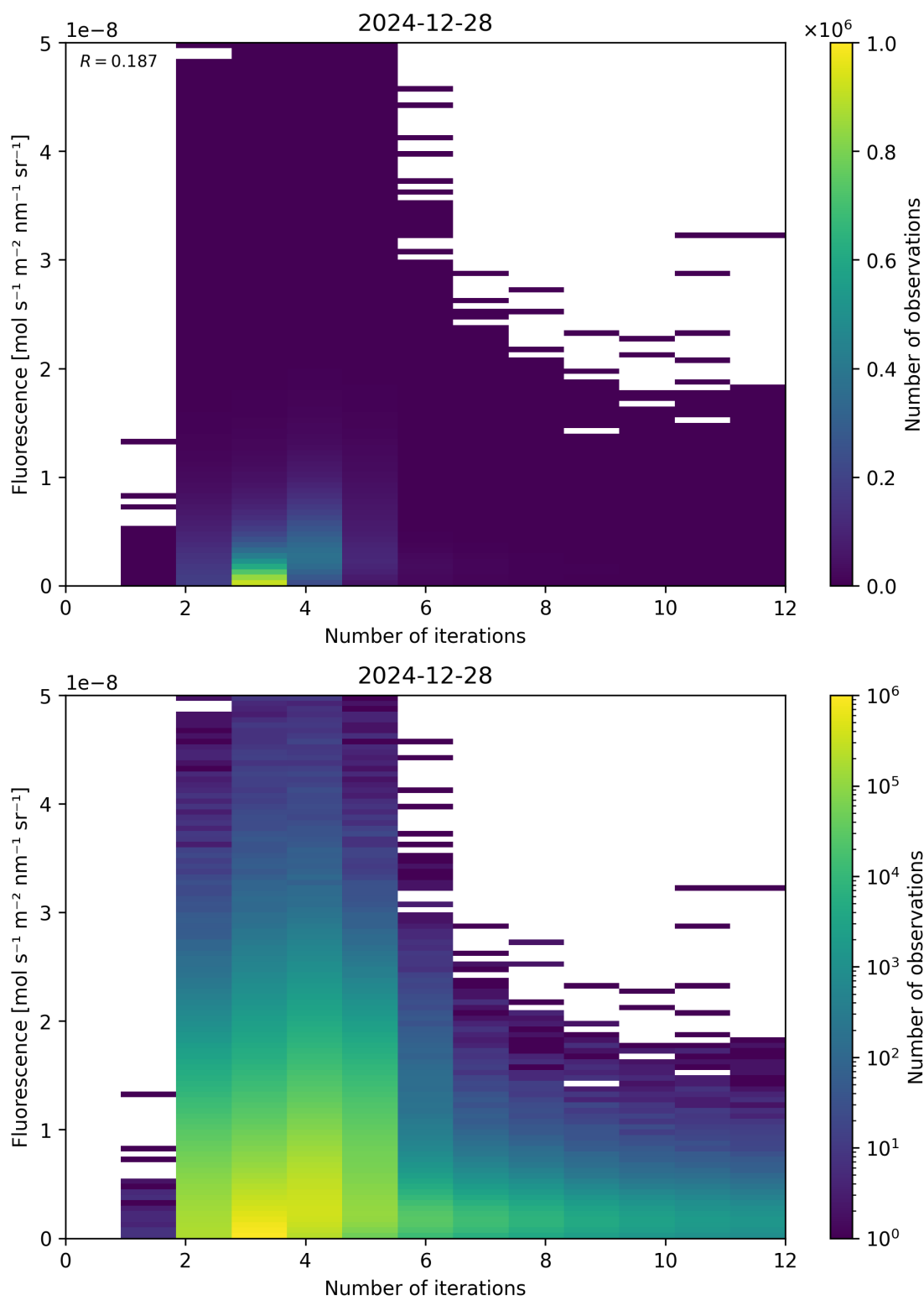
Figure 98: Scatter density plot of “Number of iterations” against “Fluorescence” for 2024-12-27 to 2024-12-29.
