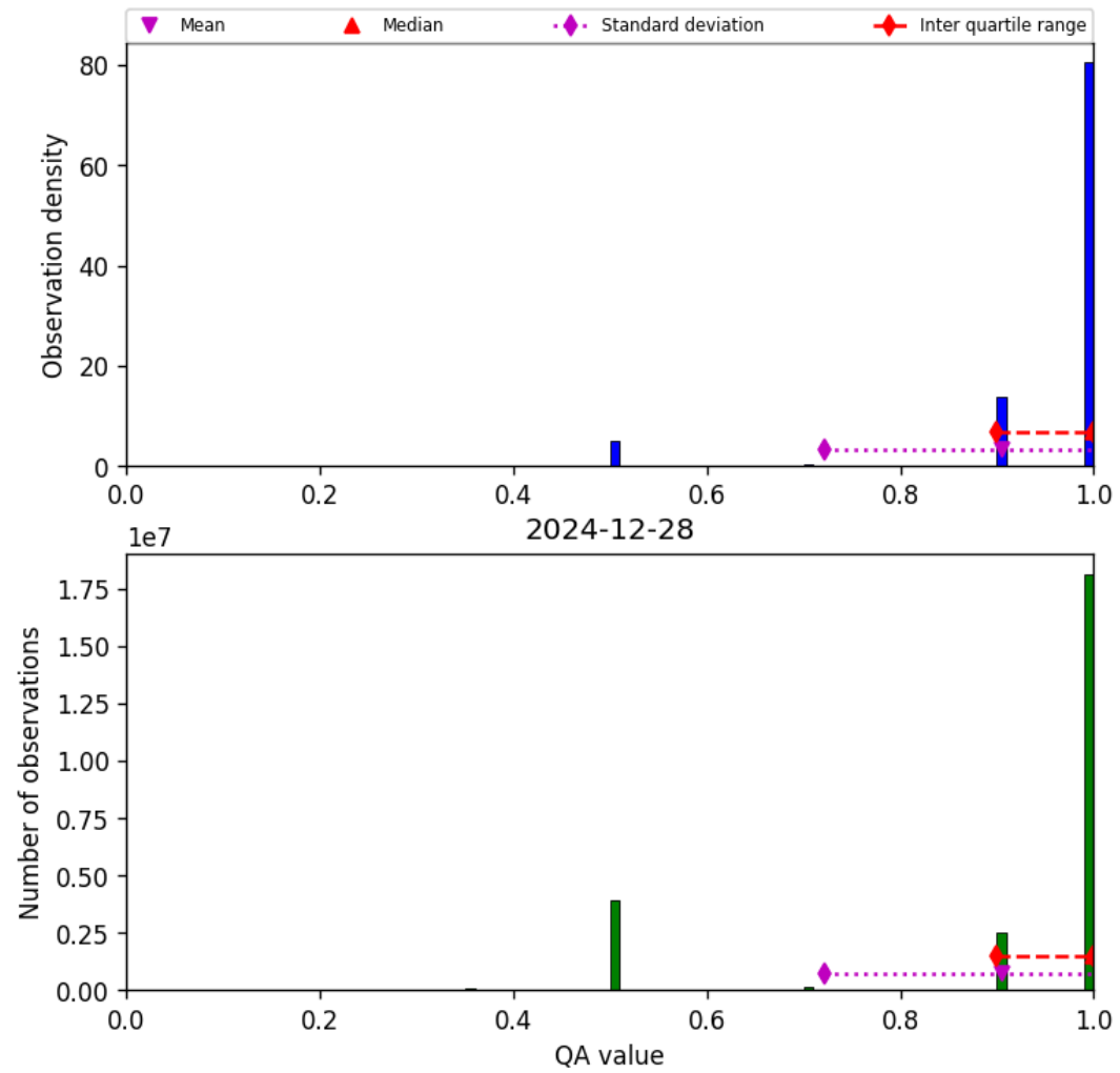
Figure 29: Histogram of “QA value” for 2024-12-27 to 2024-12-29
