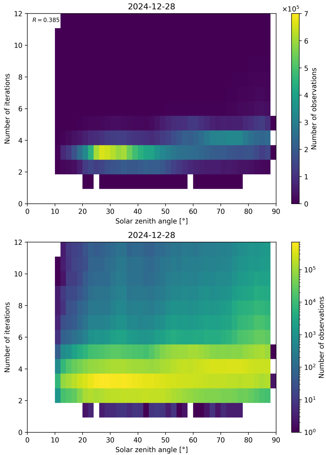
Figure 114: Scatter density plot of “Solar zenith angle” against “Number of iterations” for 2024-12-27 to 2024-12-29.
