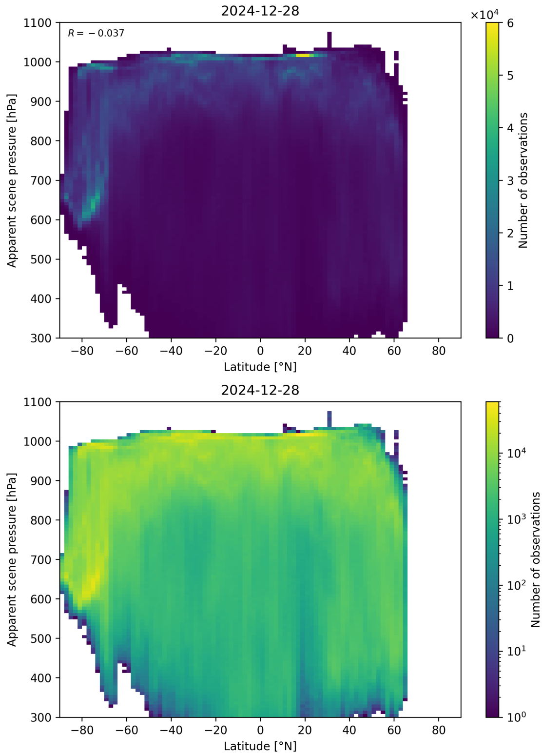
Figure 88: Scatter density plot of “Latitude” against “Apparent scene pressure” for 2024-12-27 to 2024-12-29.
