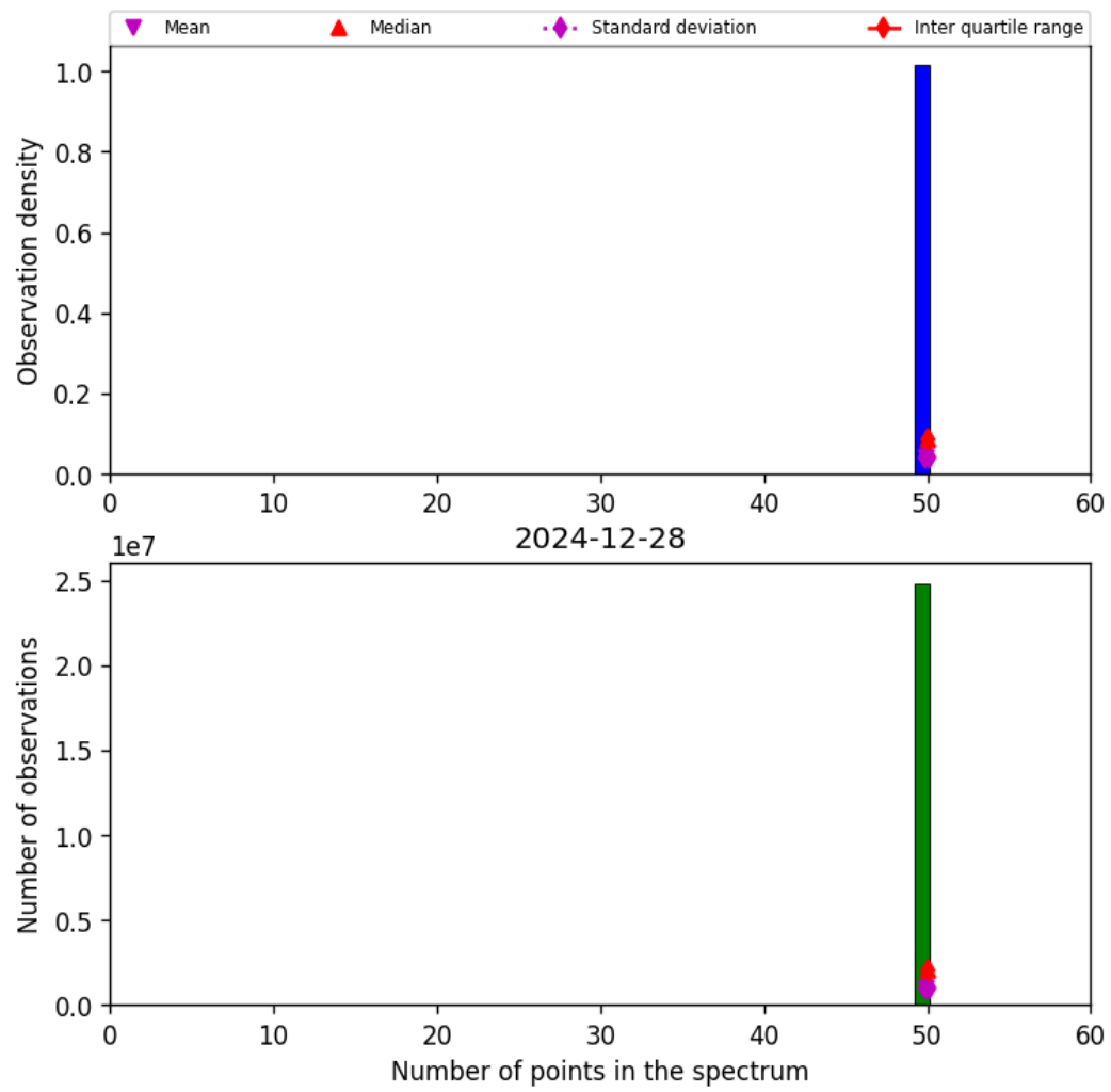
Figure 44: Histogram of “Number of points in the spectrum” for 2024-12-27 to 2024-12-29
