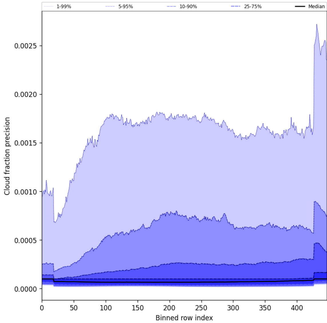
Figure 50: Along track statistics of “Cloud fraction precision” for 2024-12-27 to 2024-12-29
