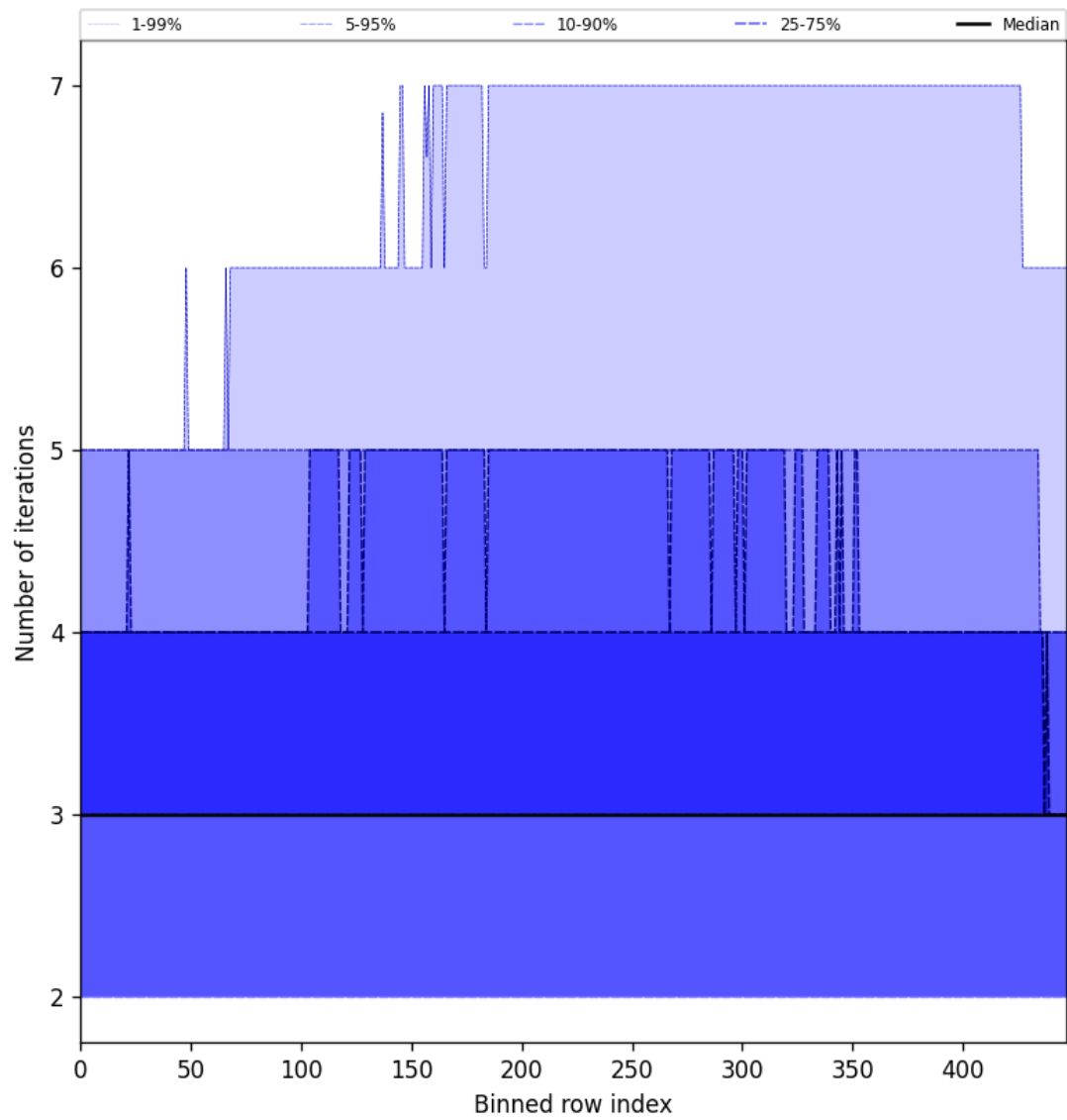
Figure 56: Along track statistics of “Number of iterations” for 2024-12-27 to 2024-12-29
