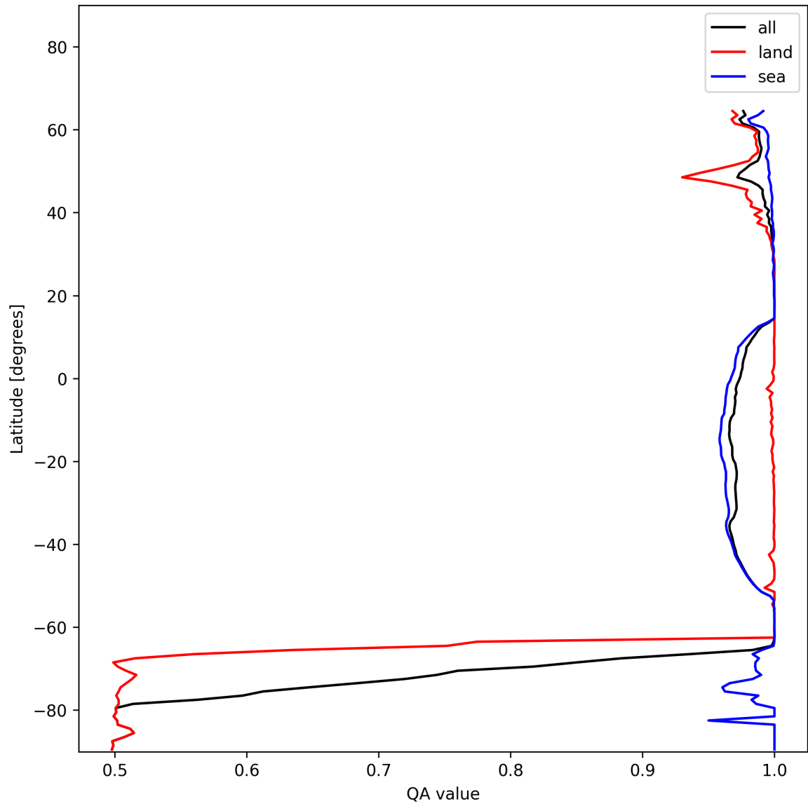
Figure 12: Zonal average of “QA value” for 2024-12-27 to 2024-12-29.
