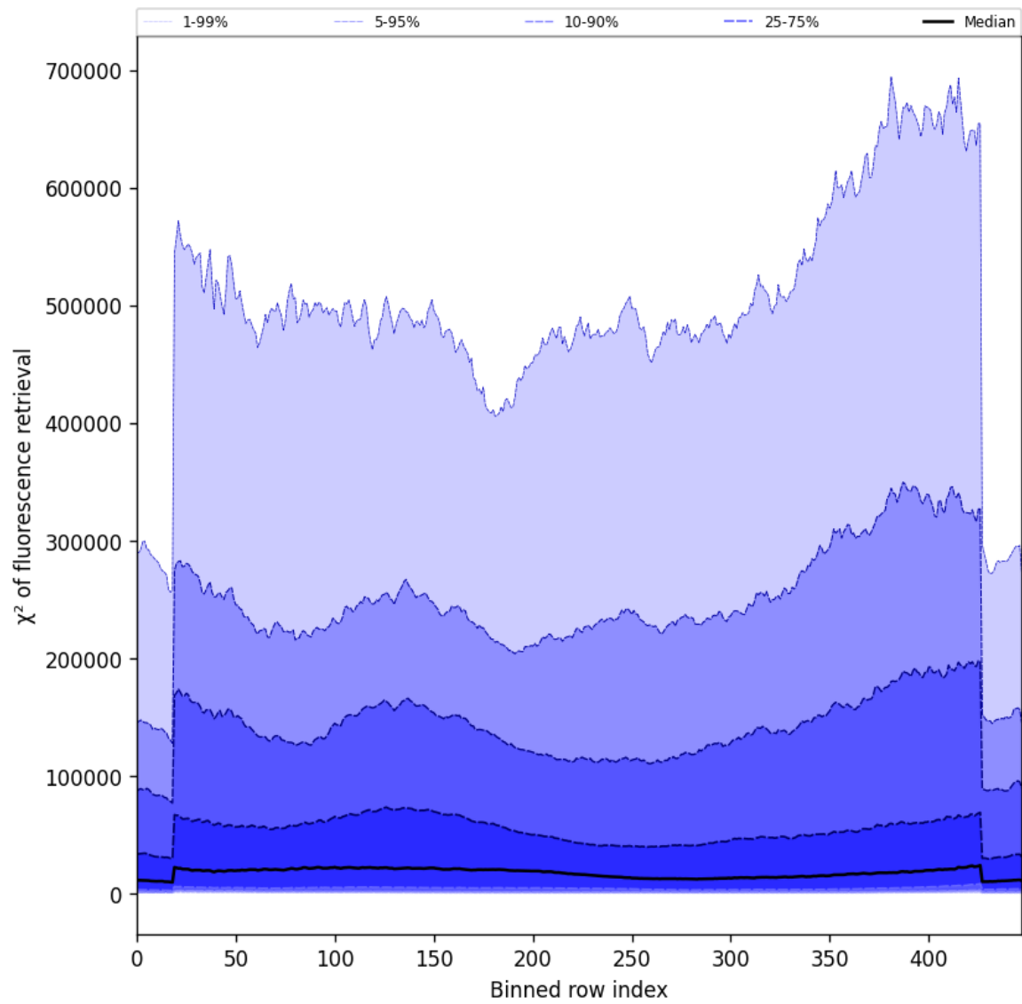
Figure 59: Along track statistics of “ \chi^2 of fluorescence retrieval” for 2024-12-27 to 2024-12-29
