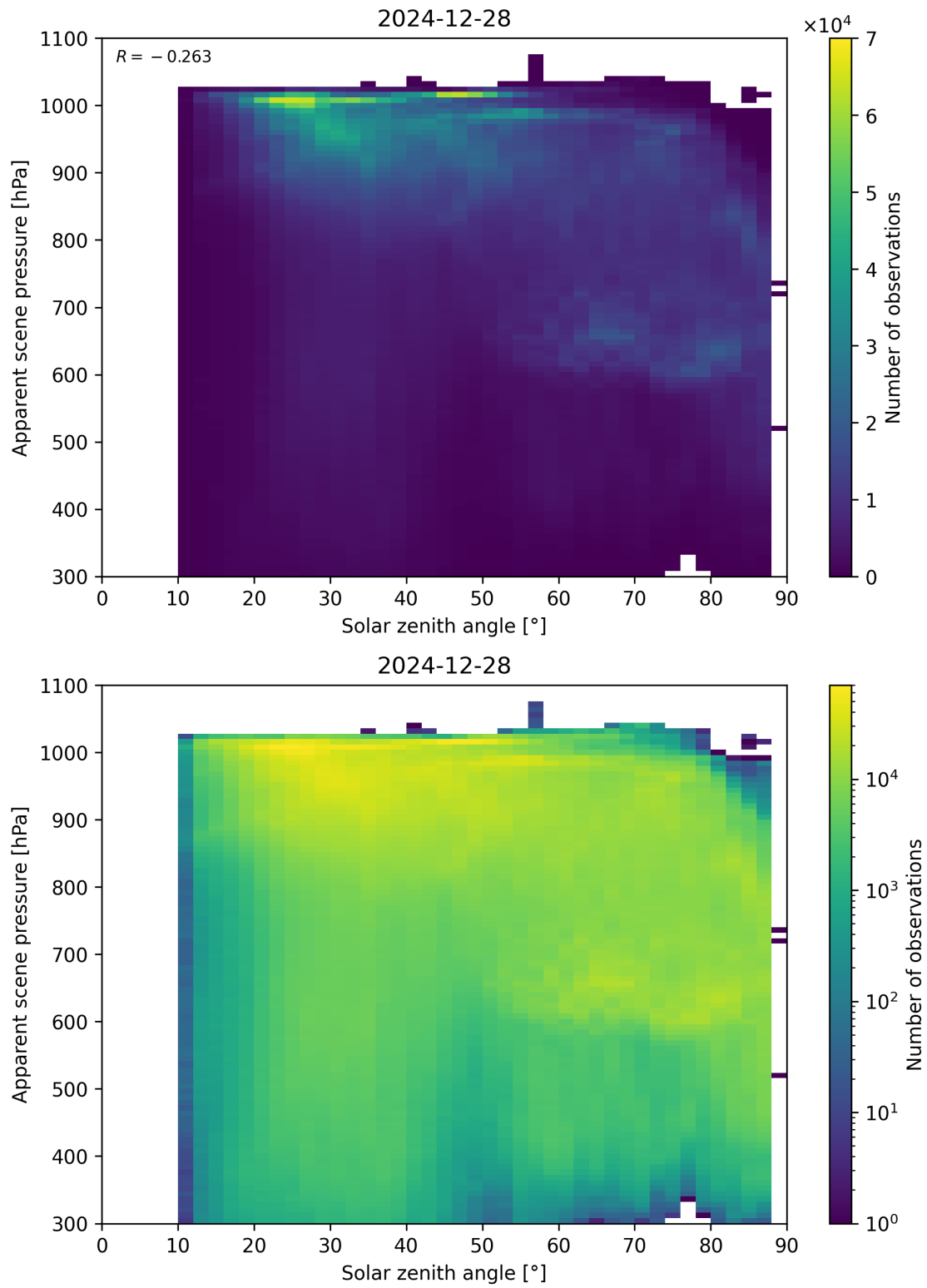
Figure 108: Scatter density plot of “Solar zenith angle” against “Apparent scene pressure” for 2024-12-27 to 2024-12-29.
