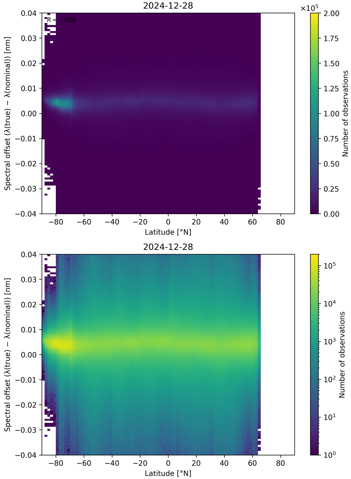
Figure 96: Scatter density plot of “Latitude” against “Spectral offset ( \lambda_{\text{true}} - \lambda_{\text{nominal}} )” for 2024-12-27 to 2024-12-29.
