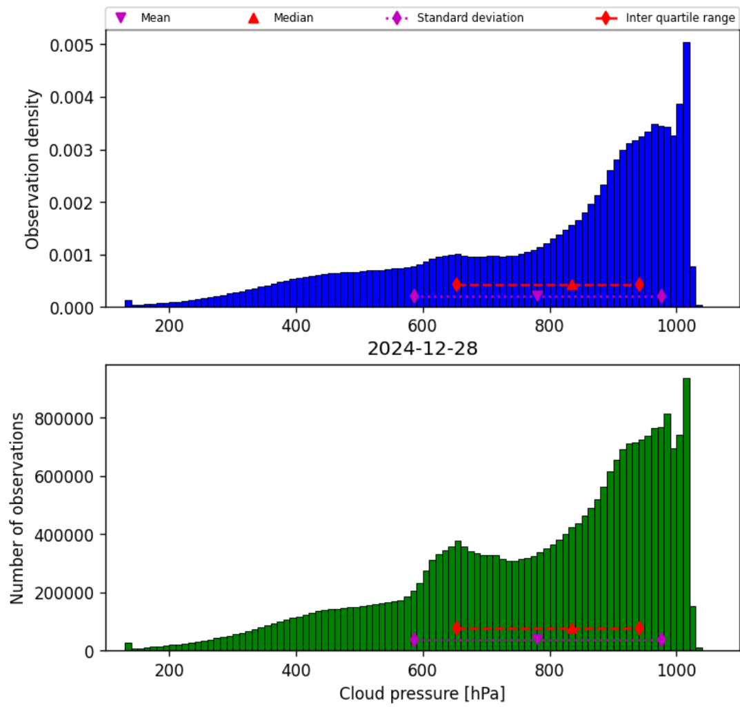
Figure 30: Histogram of “Cloud pressure” for 2024-12-27 to 2024-12-29
