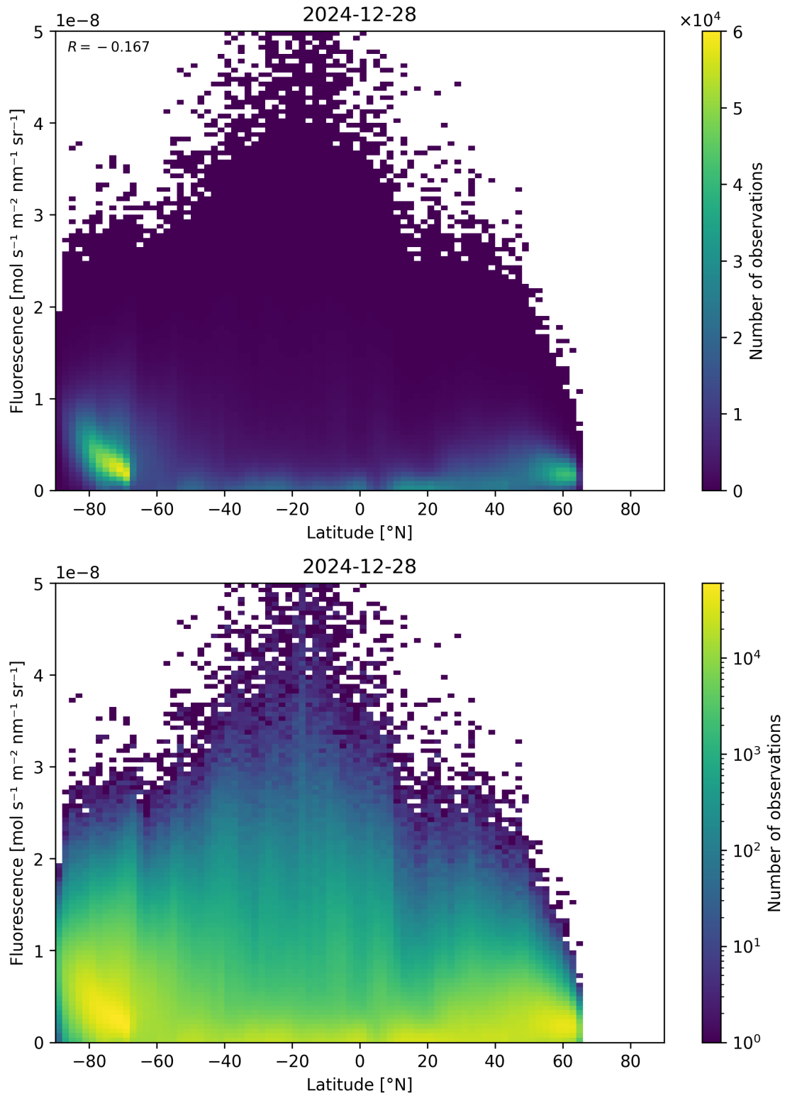
Figure 92: Scatter density plot of “Latitude” against “Fluorescence” for 2024-12-27 to 2024-12-29.
