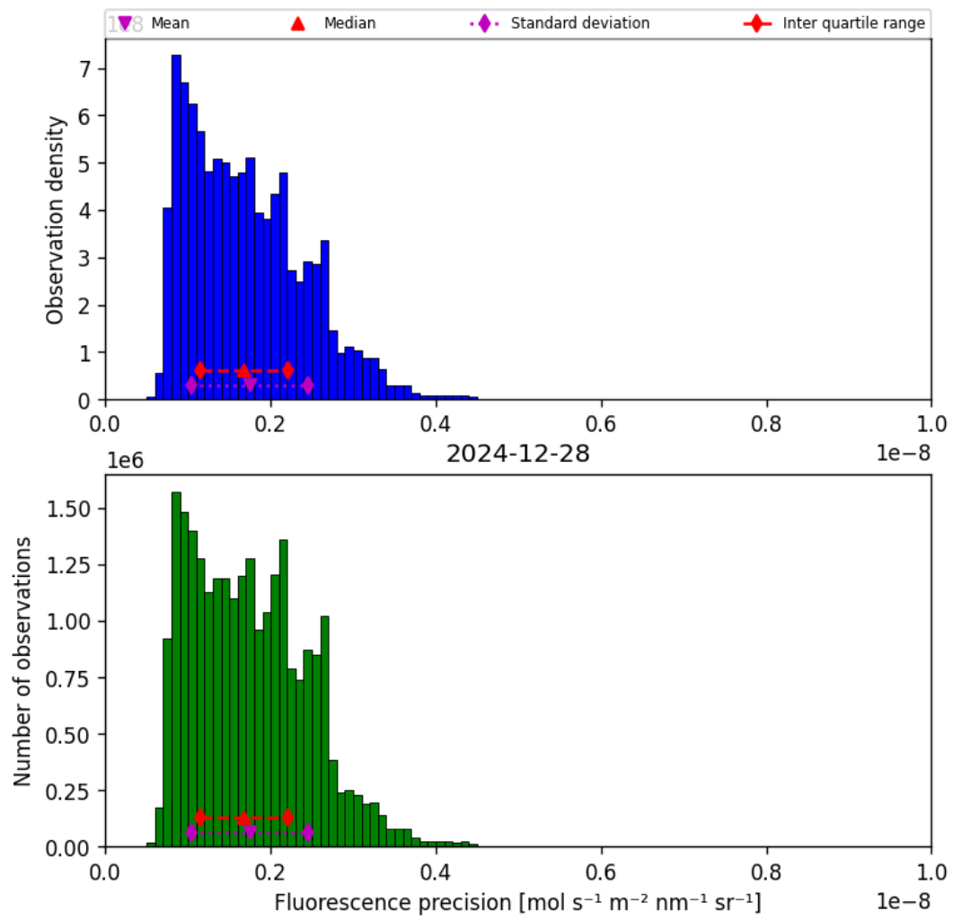
Figure 41: Histogram of “Fluorescence precision” for 2024-12-27 to 2024-12-29
