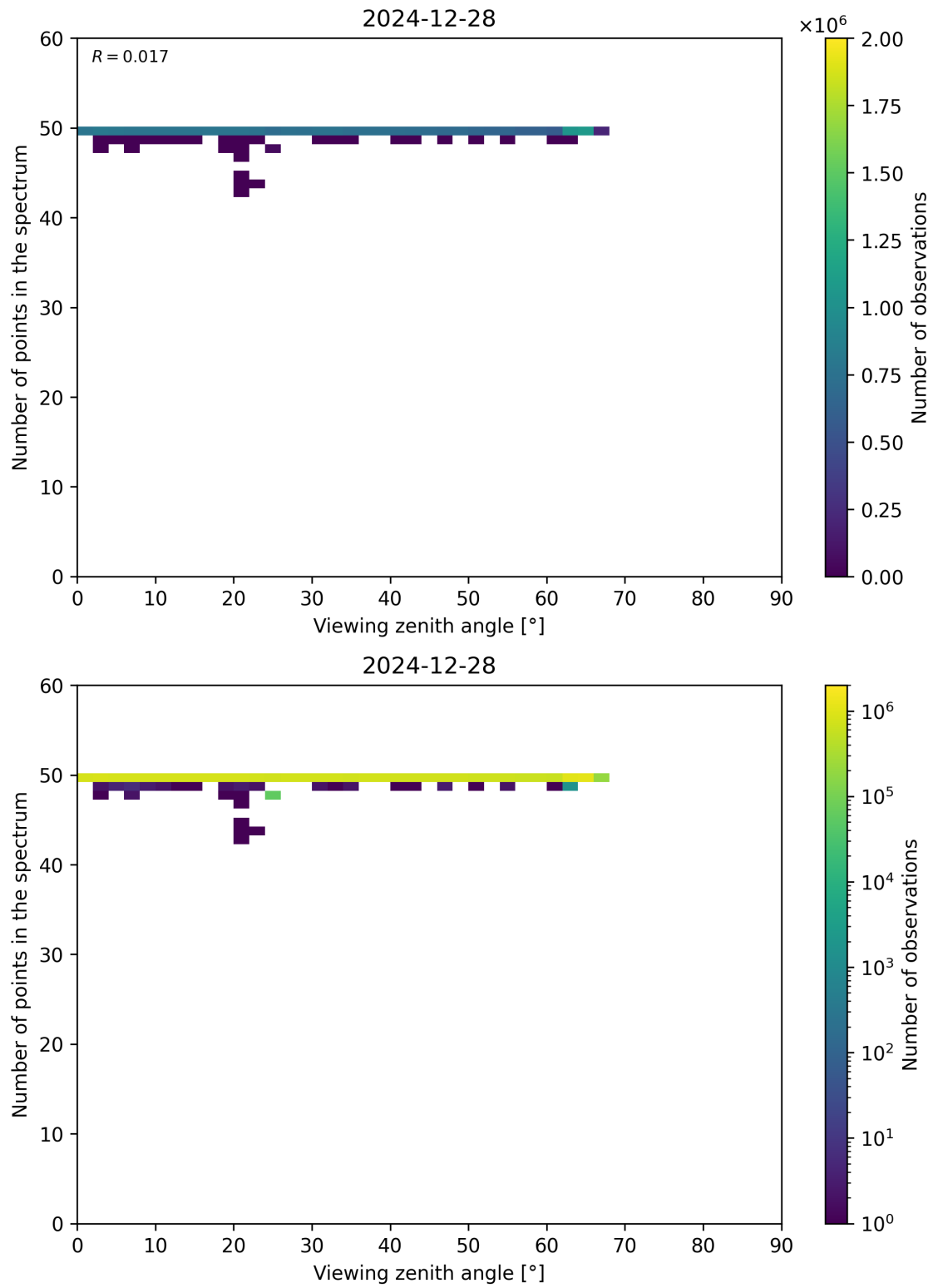
Figure 125: Scatter density plot of “Viewing zenith angle” against “Number of points in the spectrum” for 2024-12-27 to 2024-12-29.
