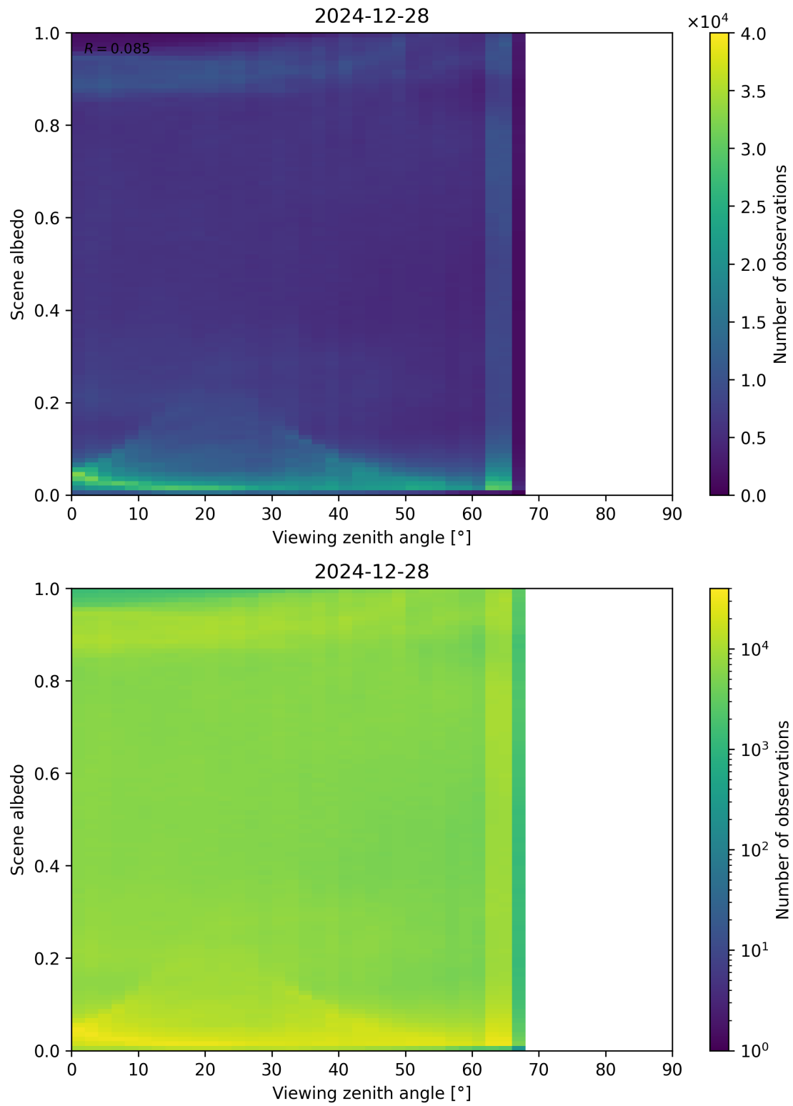
Figure 126: Scatter density plot of “Viewing zenith angle” against “Scene albedo” for 2024-12-27 to 2024-12-29.
