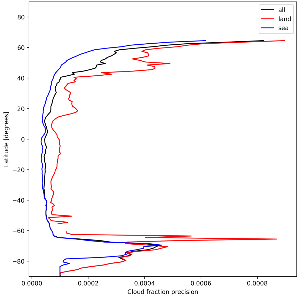
Figure 16: Zonal average of “Cloud fraction precision” for 2024-12-27 to 2024-12-29.
