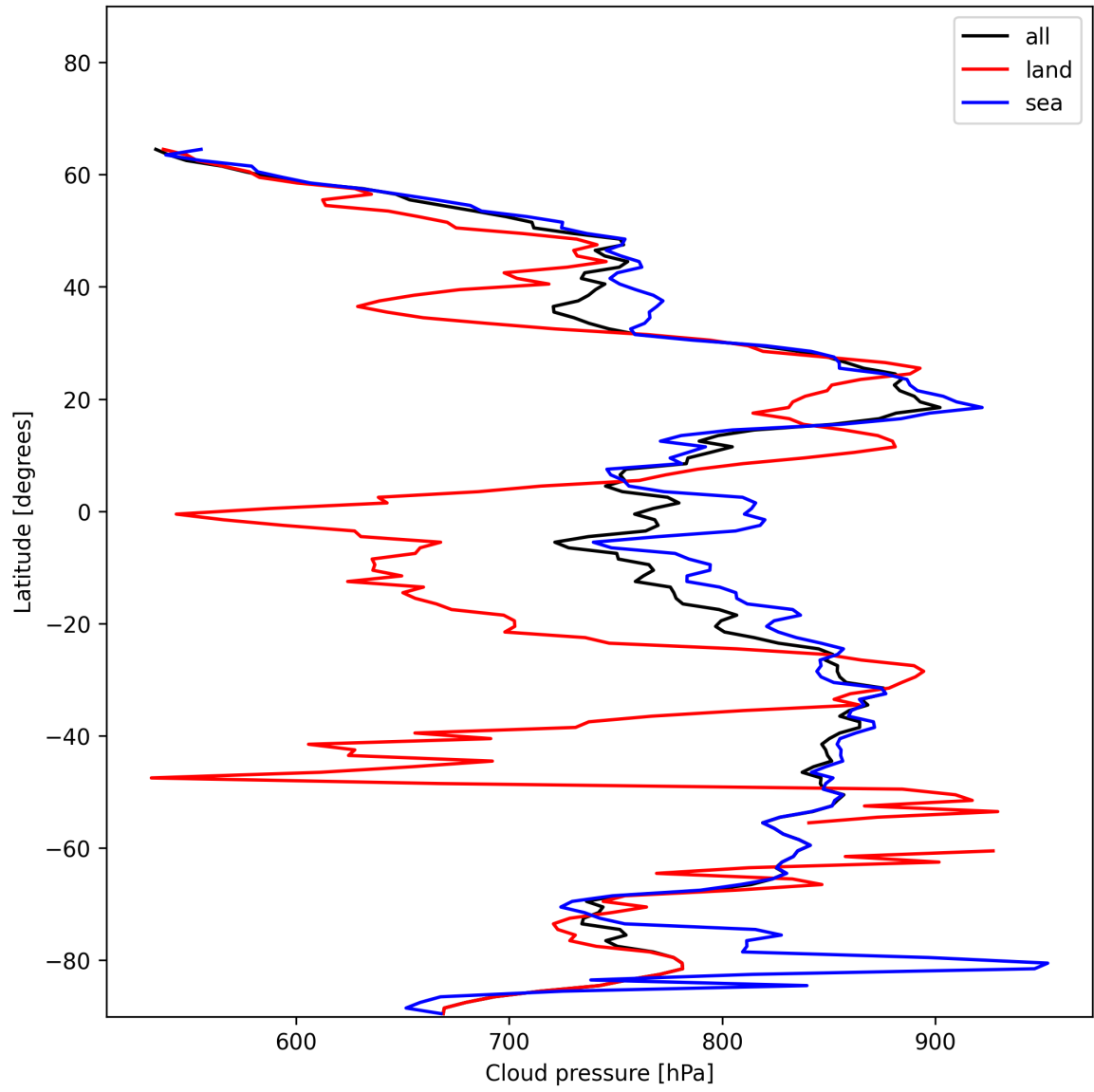
Figure 13: Zonal average of “Cloud pressure” for 2024-12-27 to 2024-12-29.
