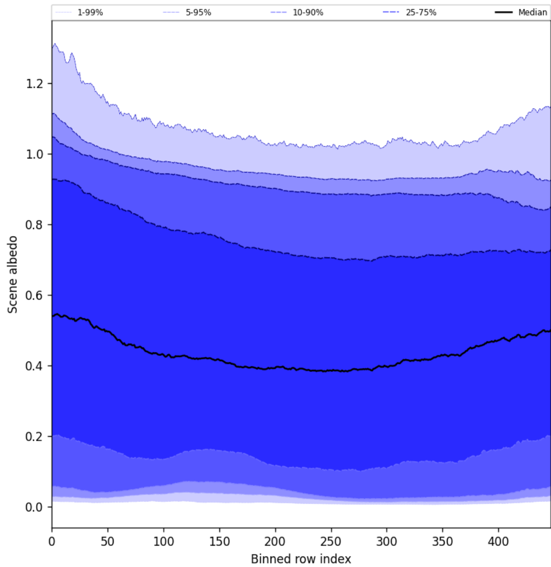
Figure 51: Along track statistics of “Scene albedo” for 2024-12-27 to 2024-12-29
