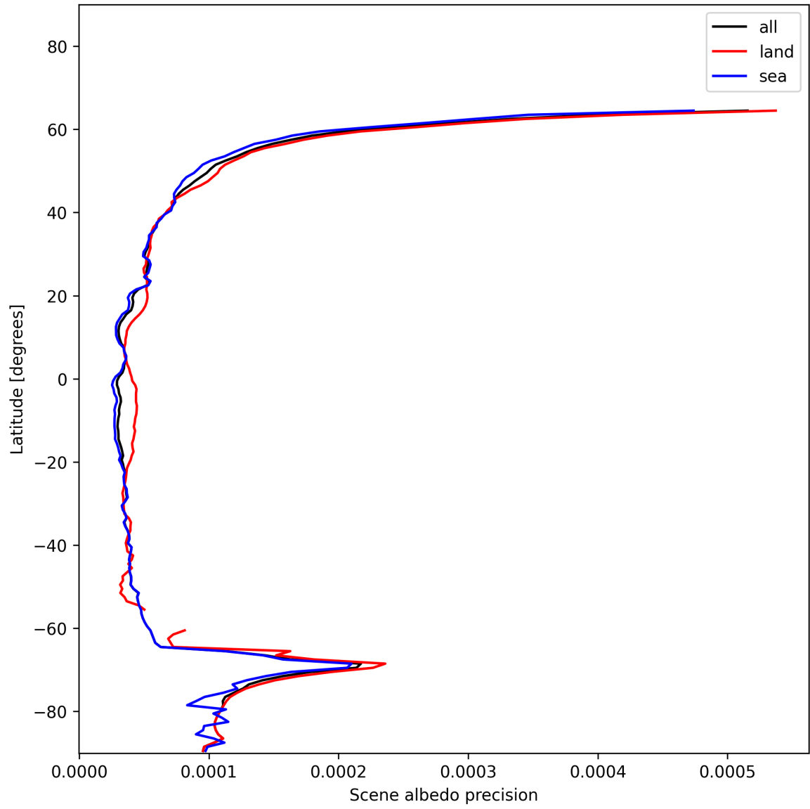
Figure 18: Zonal average of “Scene albedo precision” for 2024-12-27 to 2024-12-29.
