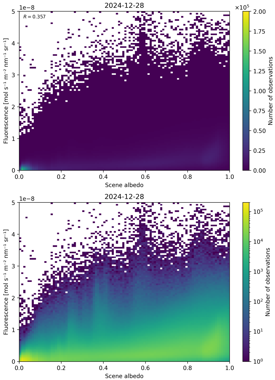
Figure 104: Scatter density plot of “Scene albedo” against “Fluorescence” for 2024-12-27 to 2024-12-29.
