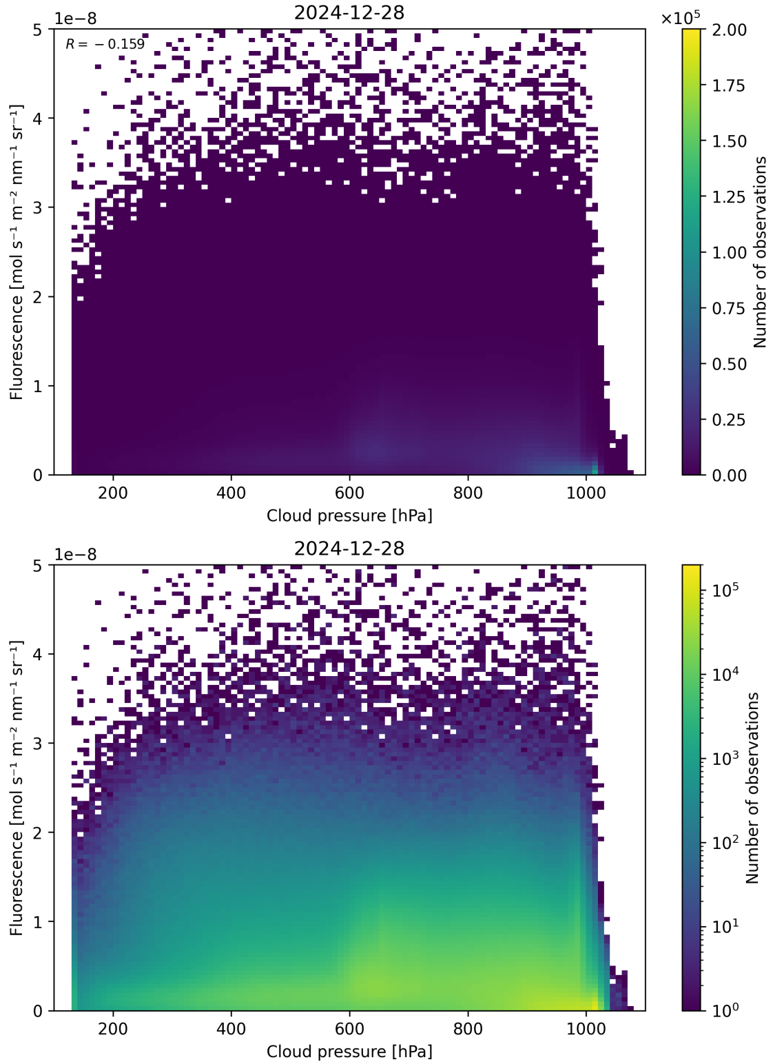
Figure 80: Scatter density plot of “Cloud pressure” against “Fluorescence” for 2024-12-27 to 2024-12-29.
