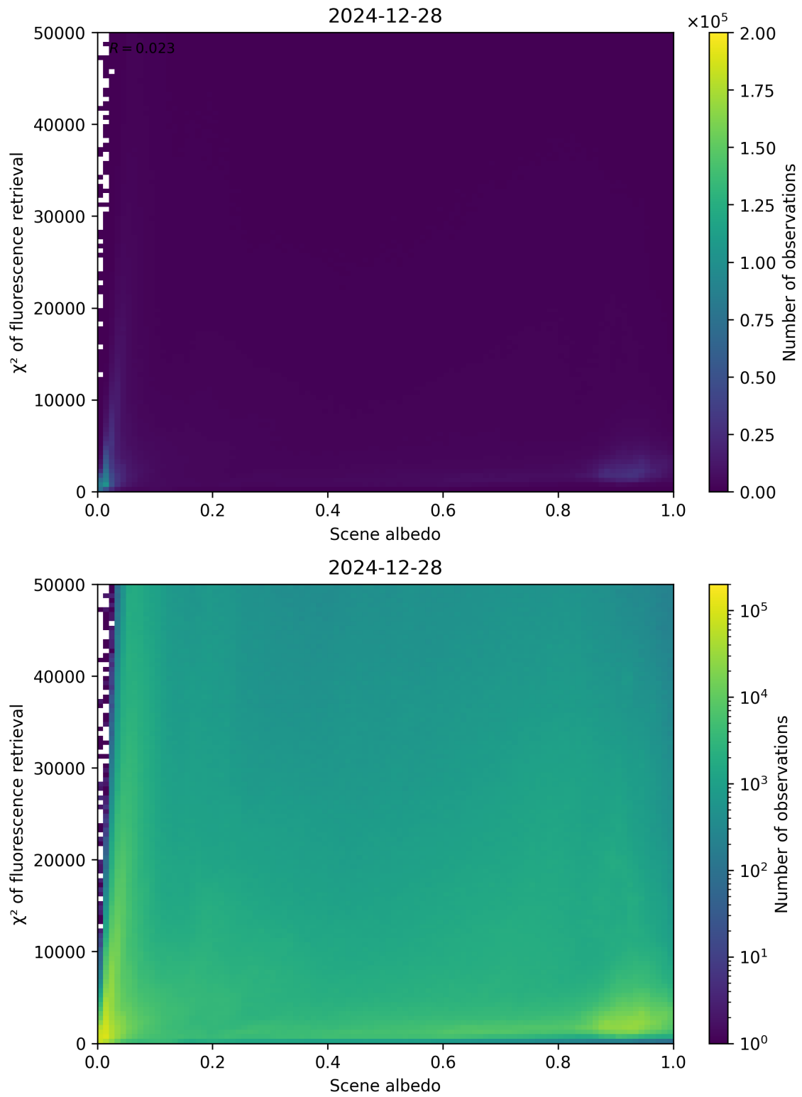
Figure 103: Scatter density plot of “Scene albedo” against “ \chi^2 of fluorescence retrieval” for 2024-12-27 to 2024-12-29.
