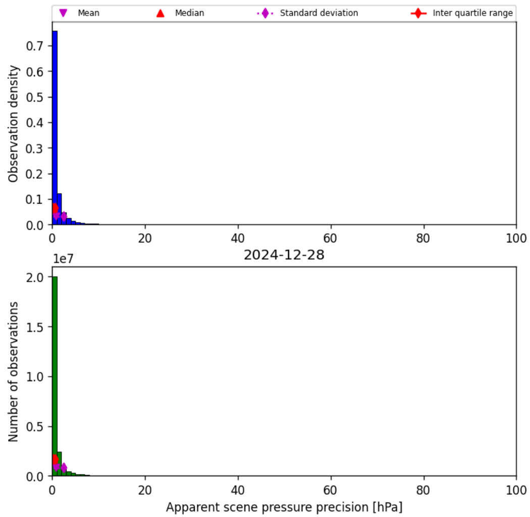
Figure 37: Histogram of “Apparent scene pressure precision” for 2024-12-27 to 2024-12-29
