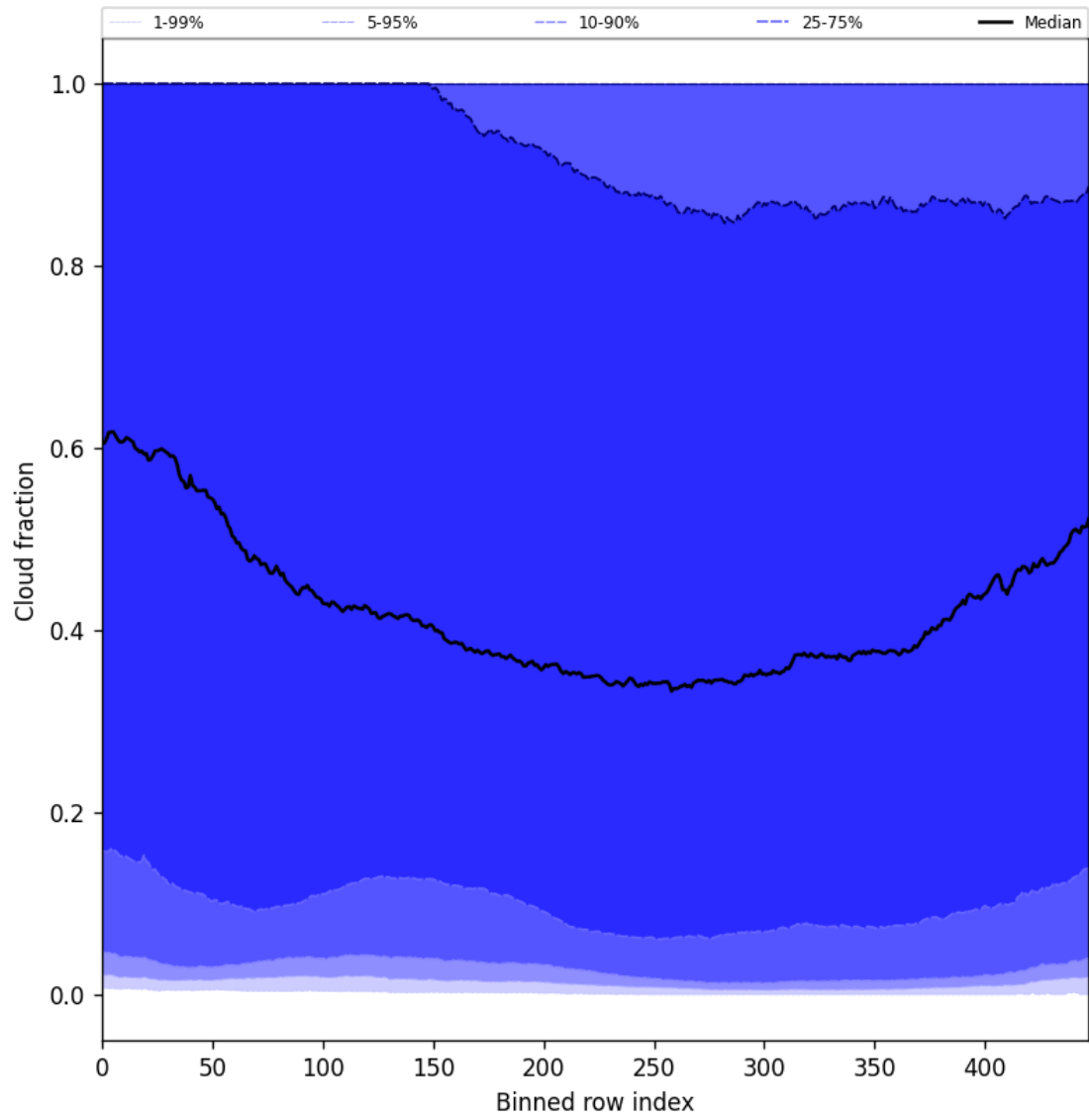
Figure 49: Along track statistics of “Cloud fraction” for 2024-12-27 to 2024-12-29
