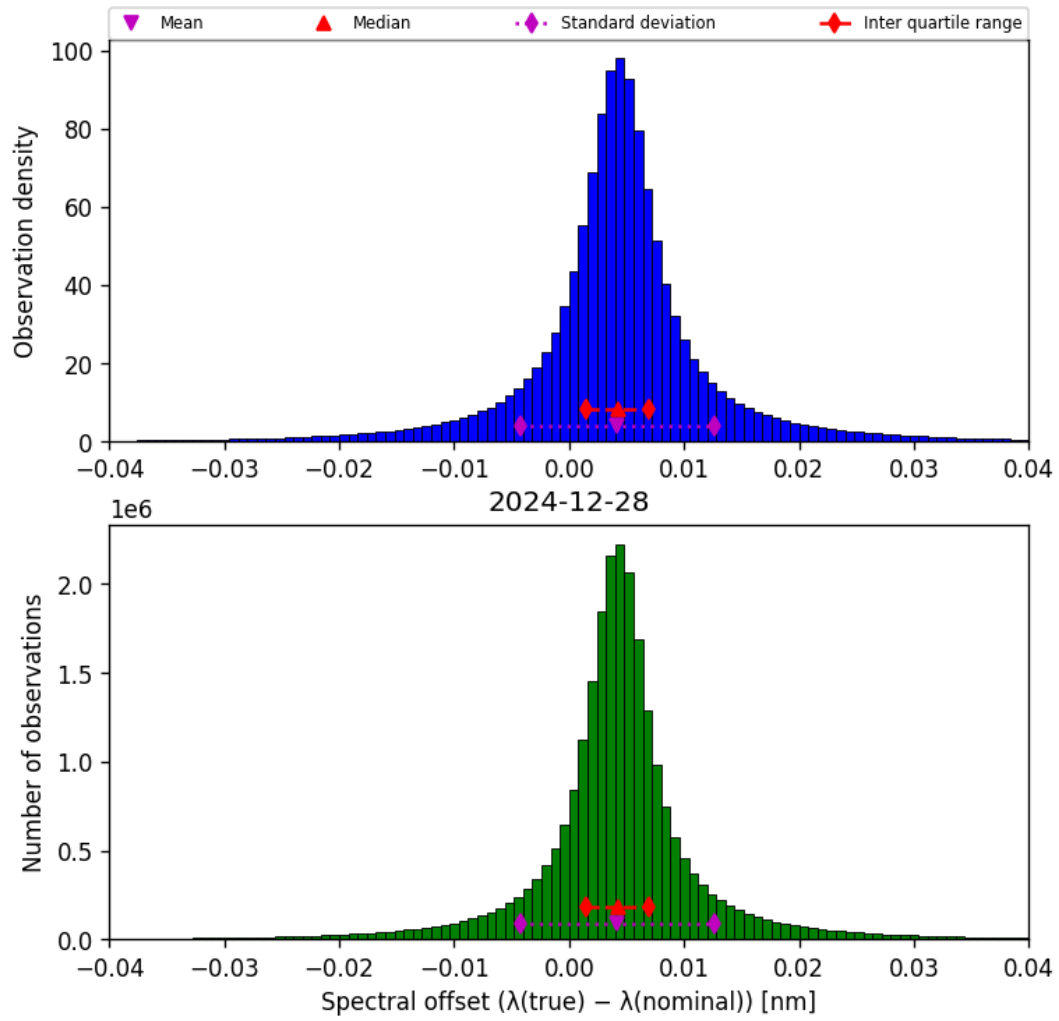
Figure 45: Histogram of “Spectral offset ( \lambda_{\text{true}} - \lambda_{\text{nominal}} )” for 2024-12-27 to 2024-12-29
