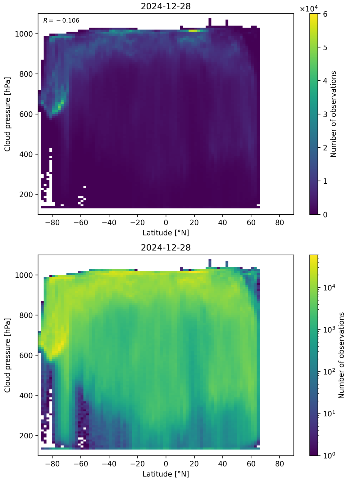
Figure 91: Scatter density plot of “Latitude” against “Cloud pressure” for 2024-12-27 to 2024-12-29.
