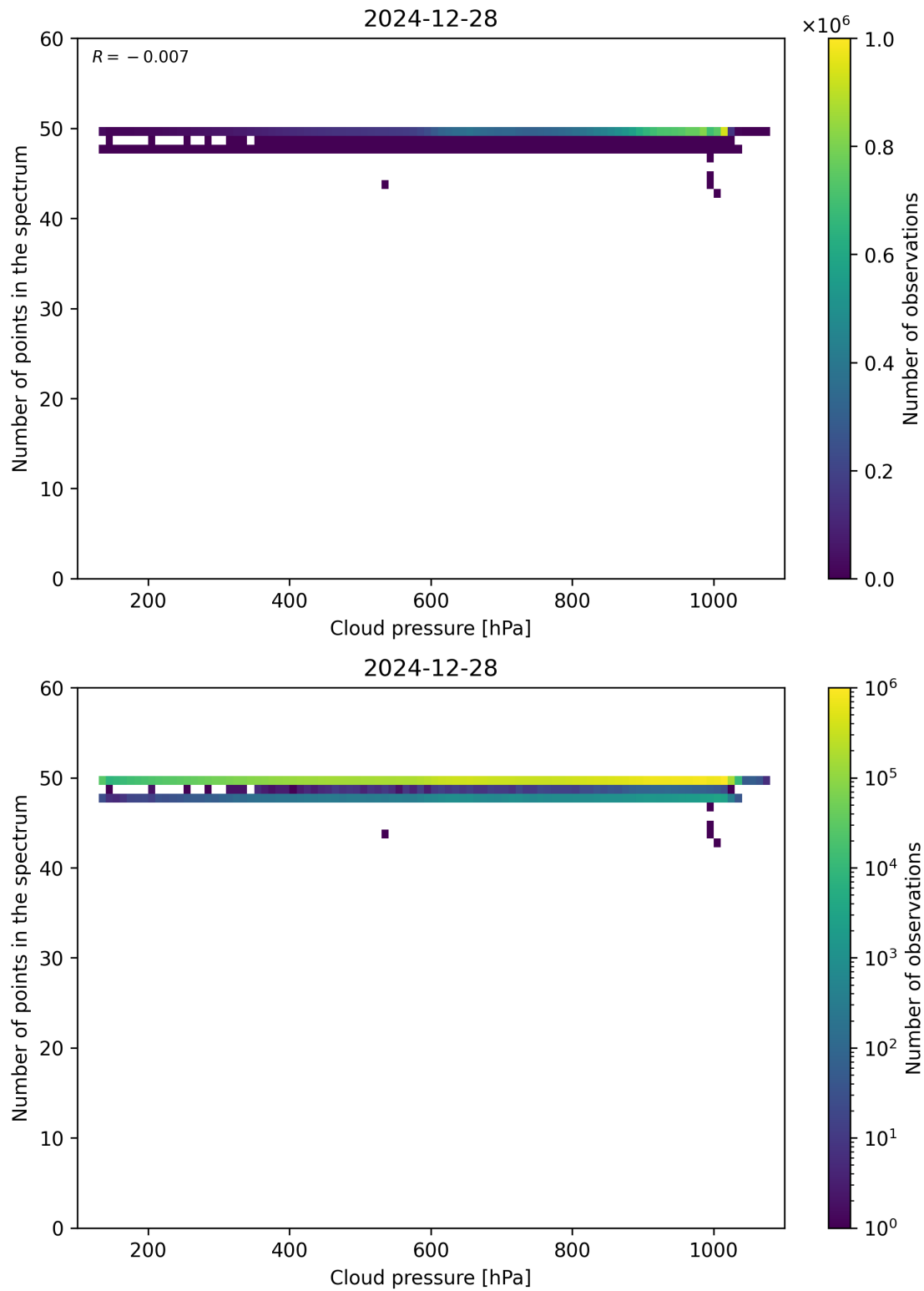
Figure 82: Scatter density plot of “Cloud pressure” against “Number of points in the spectrum” for 2024-12-27 to 2024-12-29.
