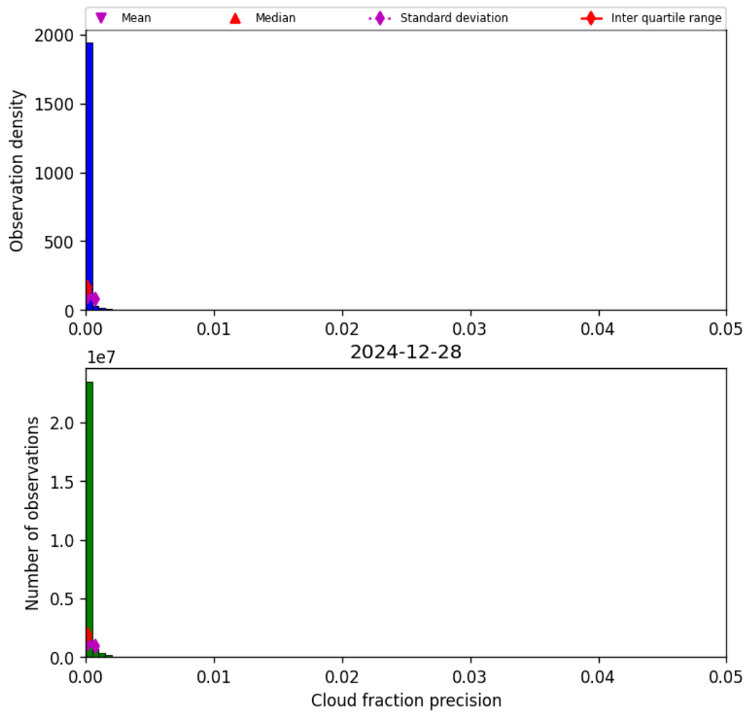
Figure 33: Histogram of “Cloud fraction precision” for 2024-12-27 to 2024-12-29
