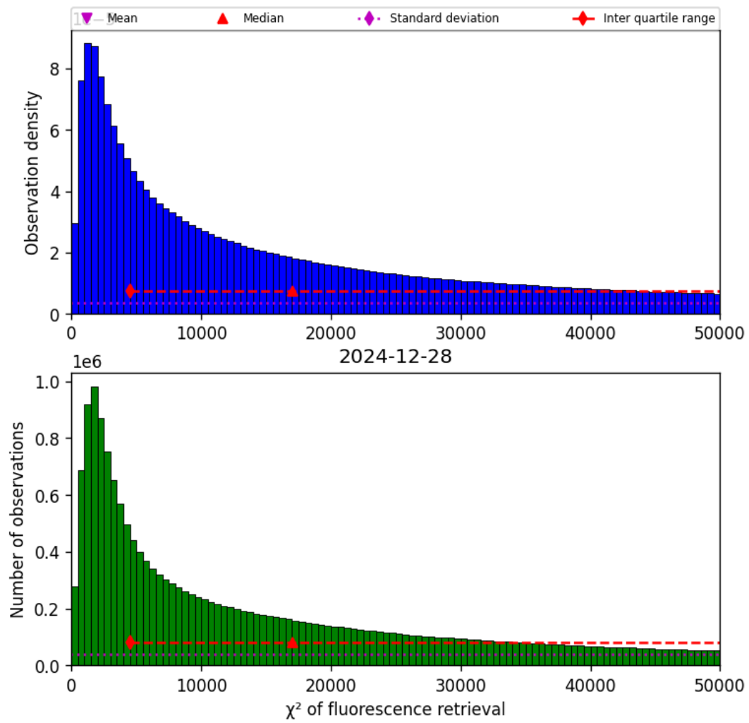
Figure 42: Histogram of “ \chi^2 of fluorescence retrieval” for 2024-12-27 to 2024-12-29
