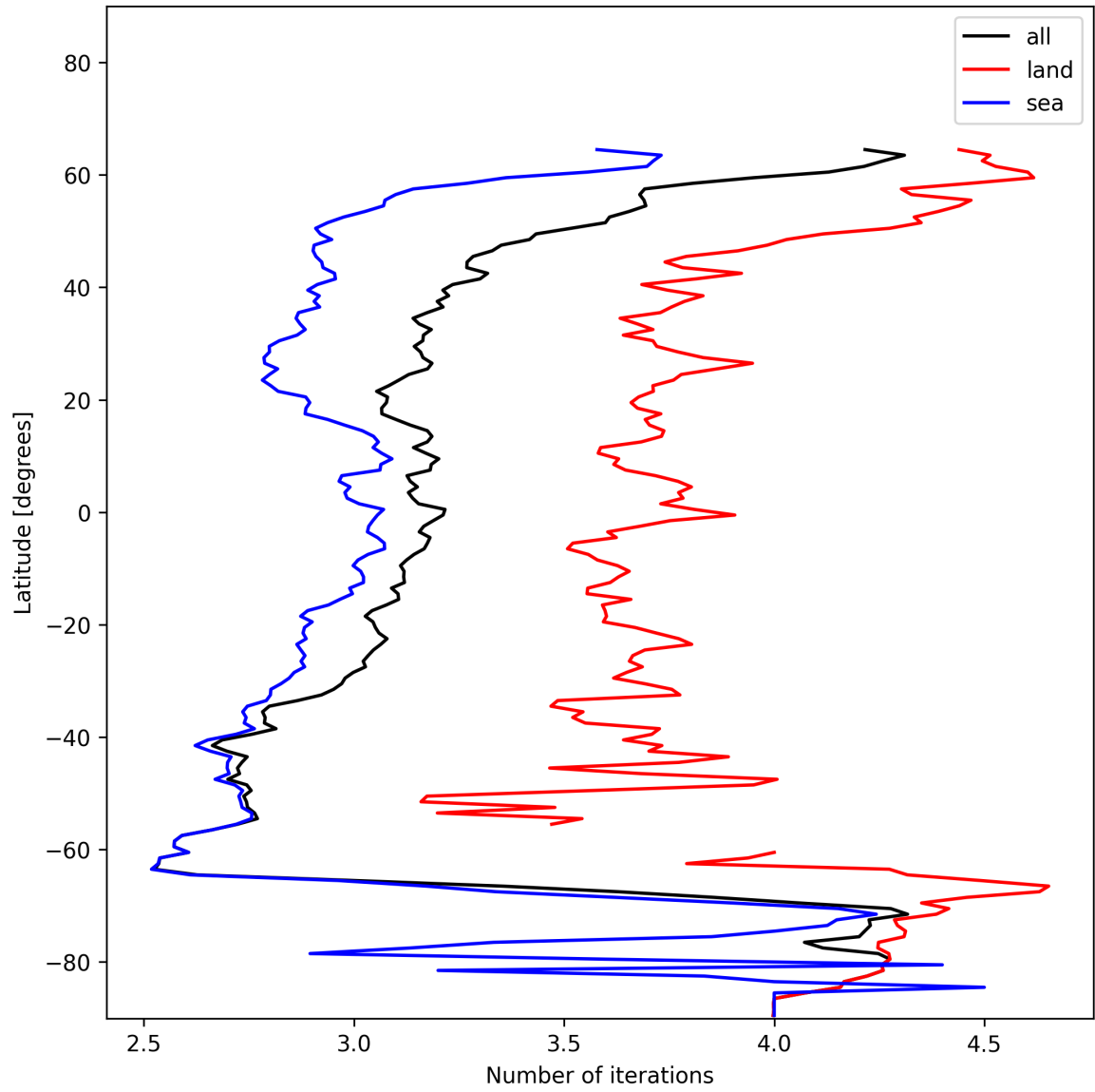
Figure 22: Zonal average of “Number of iterations” for 2024-12-27 to 2024-12-29.
