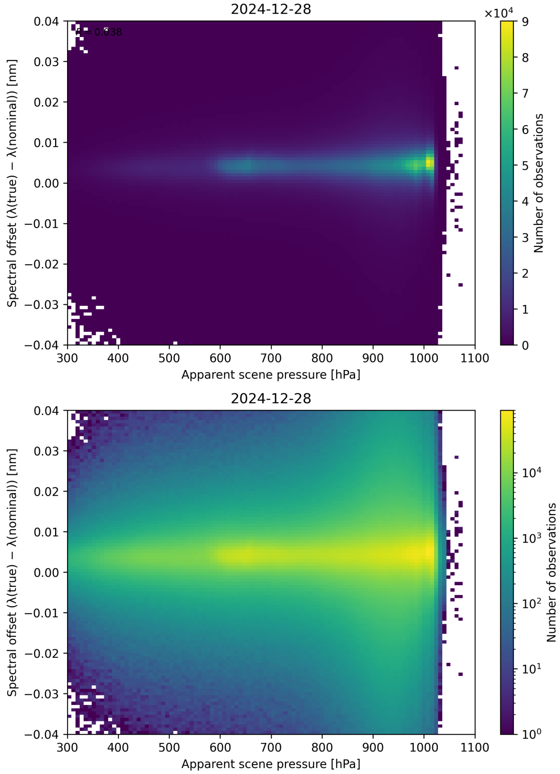
Figure 67: Scatter density plot of “Apparent scene pressure” against “Spectral offset ( \lambda_{\text{true}} - \lambda_{\text{nominal}} )” for 2024-12-27 to 2024-12-29.
