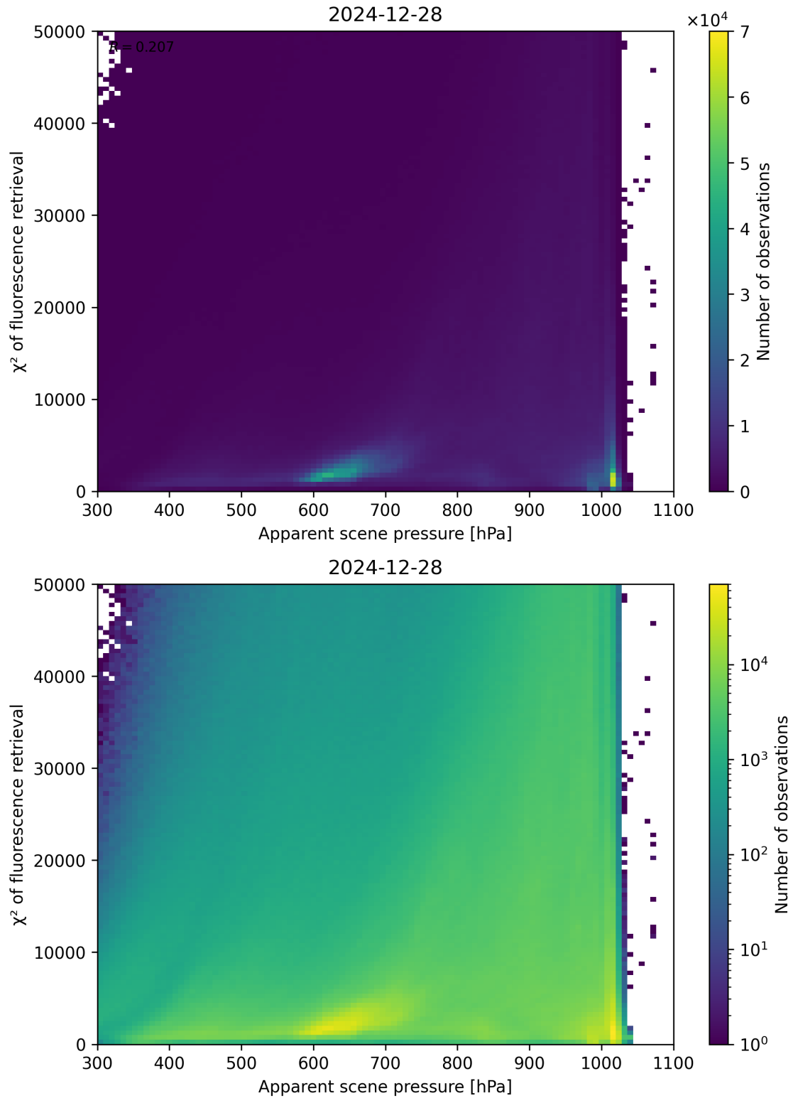
Figure 63: Scatter density plot of “Apparent scene pressure” against “ \chi^2 of fluorescence retrieval” for 2024-12-27 to 2024-12-29.
