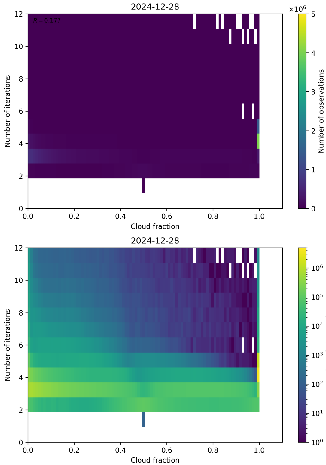
Figure 73: Scatter density plot of “Cloud fraction” against “Number of iterations” for 2024-12-27 to 2024-12-29.
