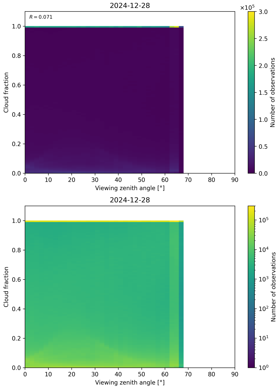
Figure 120: Scatter density plot of “Viewing zenith angle” against “Cloud fraction” for 2024-12-27 to 2024-12-29.
