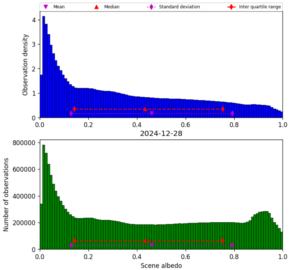
Figure 34: Histogram of “Scene albedo” for 2024-12-27 to 2024-12-29
