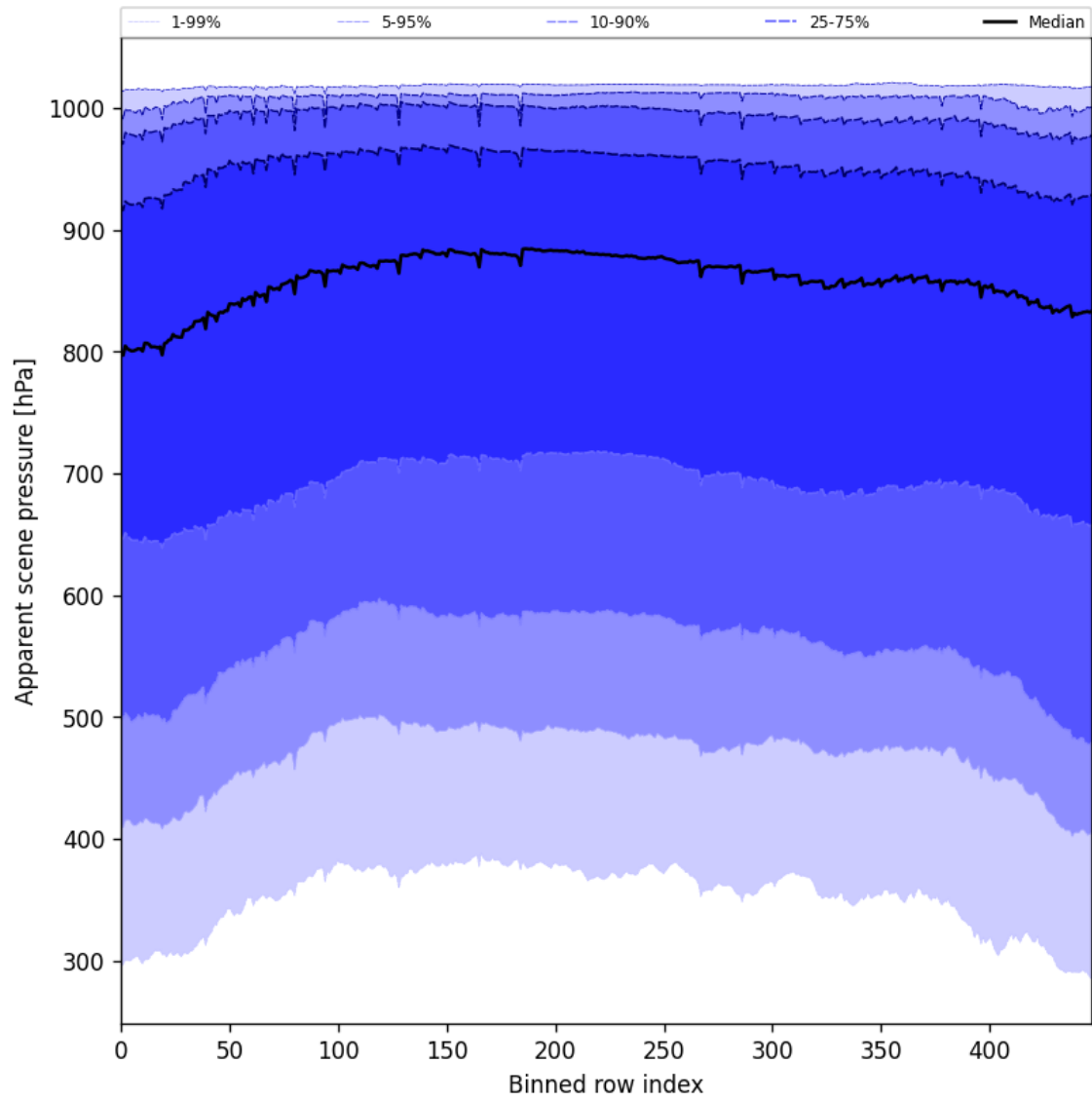
Figure 53: Along track statistics of “Apparent scene pressure” for 2024-12-27 to 2024-12-29
