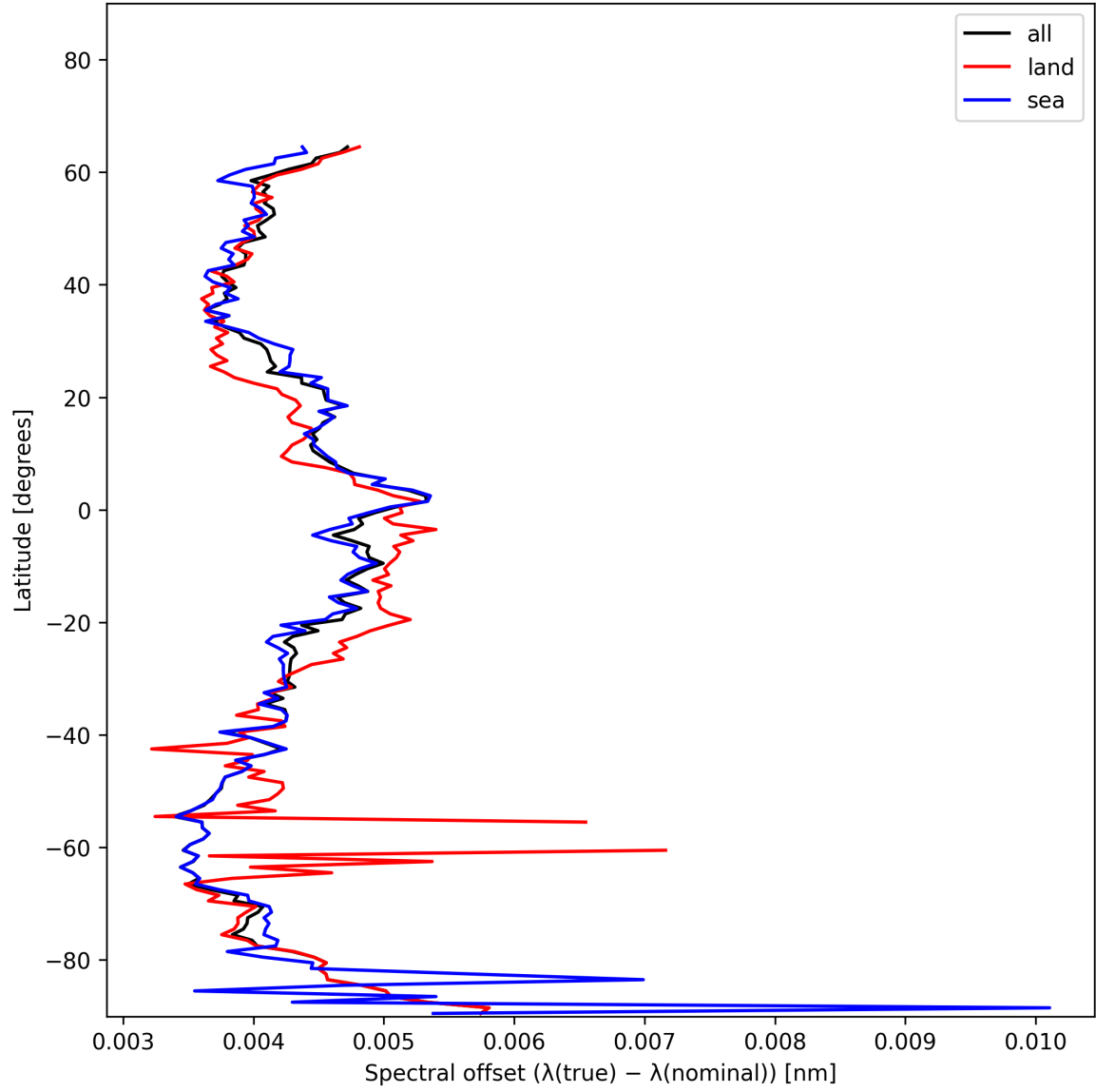
Figure 28: Zonal average of “Spectral offset ( \lambda_{\text{true}} - \lambda_{\text{nominal}} )” for 2024-12-27 to 2024-12-29.
