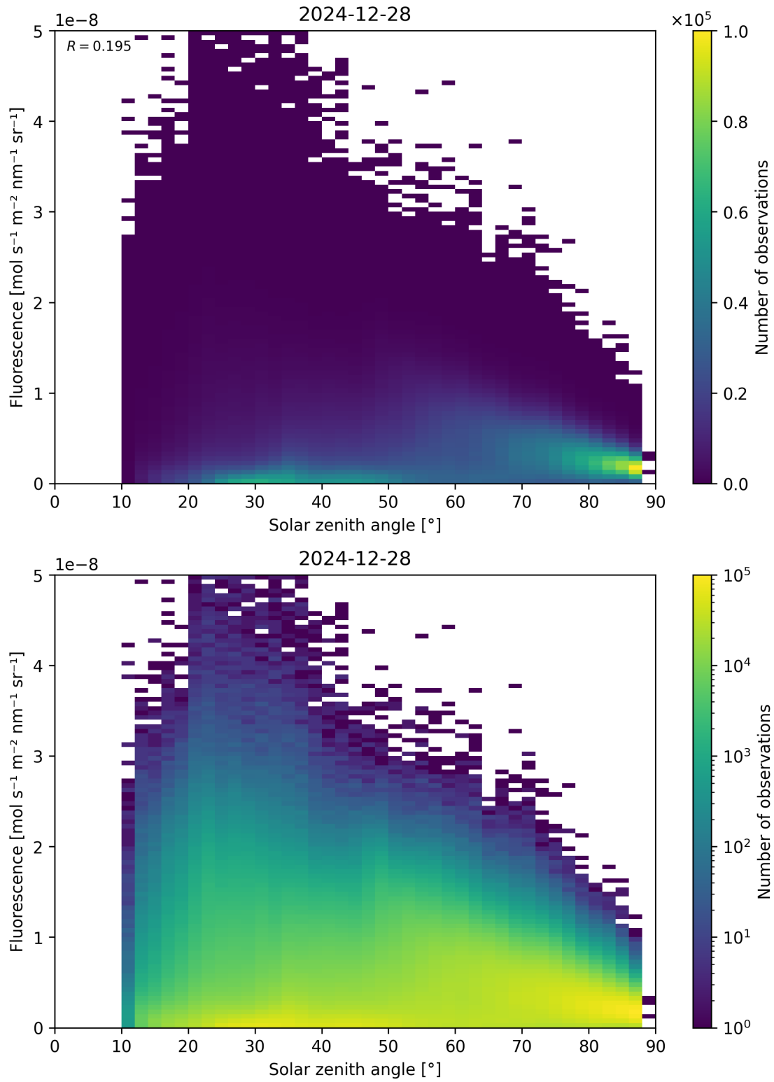
Figure 112: Scatter density plot of “Solar zenith angle” against “Fluorescence” for 2024-12-27 to 2024-12-29.
