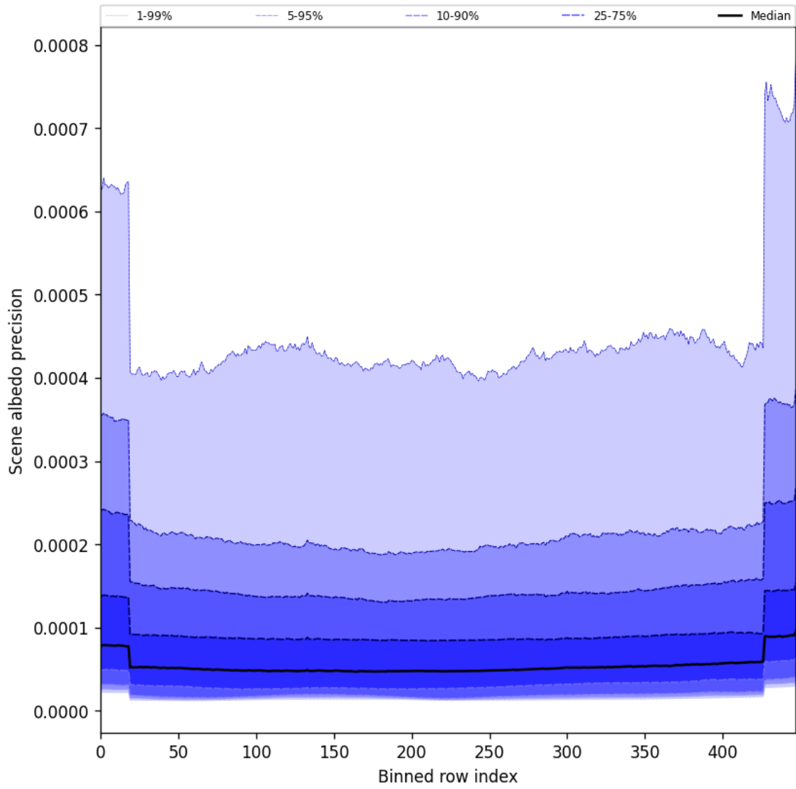
Figure 52: Along track statistics of “Scene albedo precision” for 2024-12-27 to 2024-12-29
