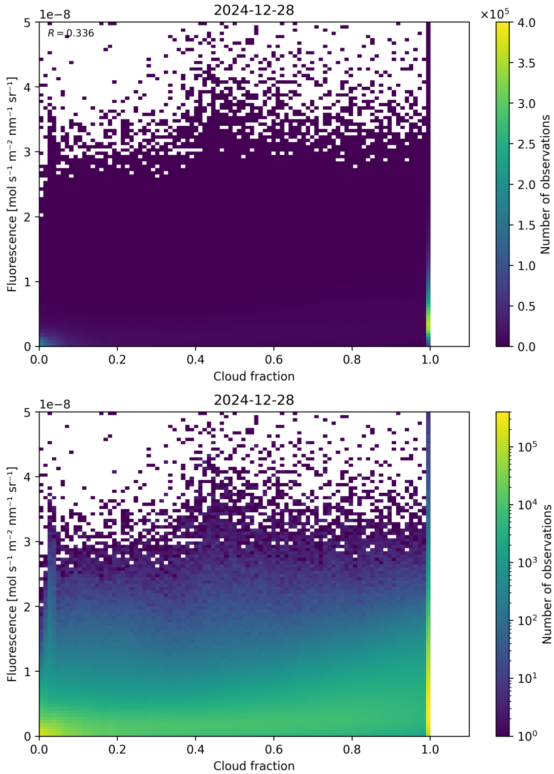
Figure 72: Scatter density plot of “Cloud fraction” against “Fluorescence” for 2024-12-27 to 2024-12-29.
