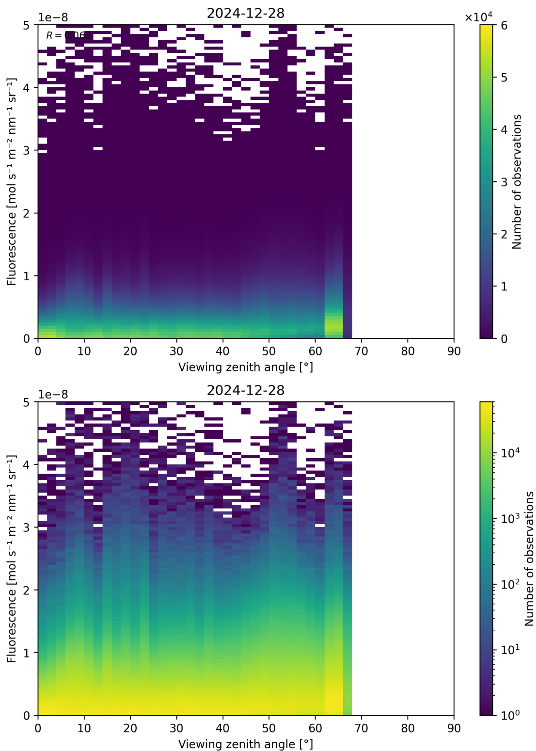
Figure 122: Scatter density plot of “Viewing zenith angle” against “Fluorescence” for 2024-12-27 to 2024-12-29.
