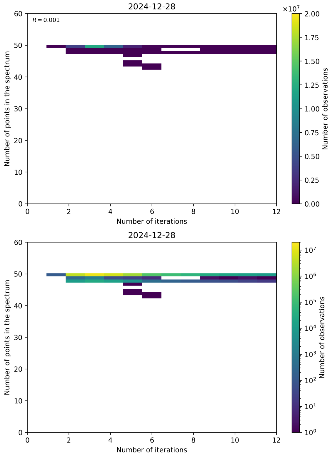
Figure 99: Scatter density plot of “Number of iterations” against “Number of points in the spectrum” for 2024-12-27 to 2024-12-29.
