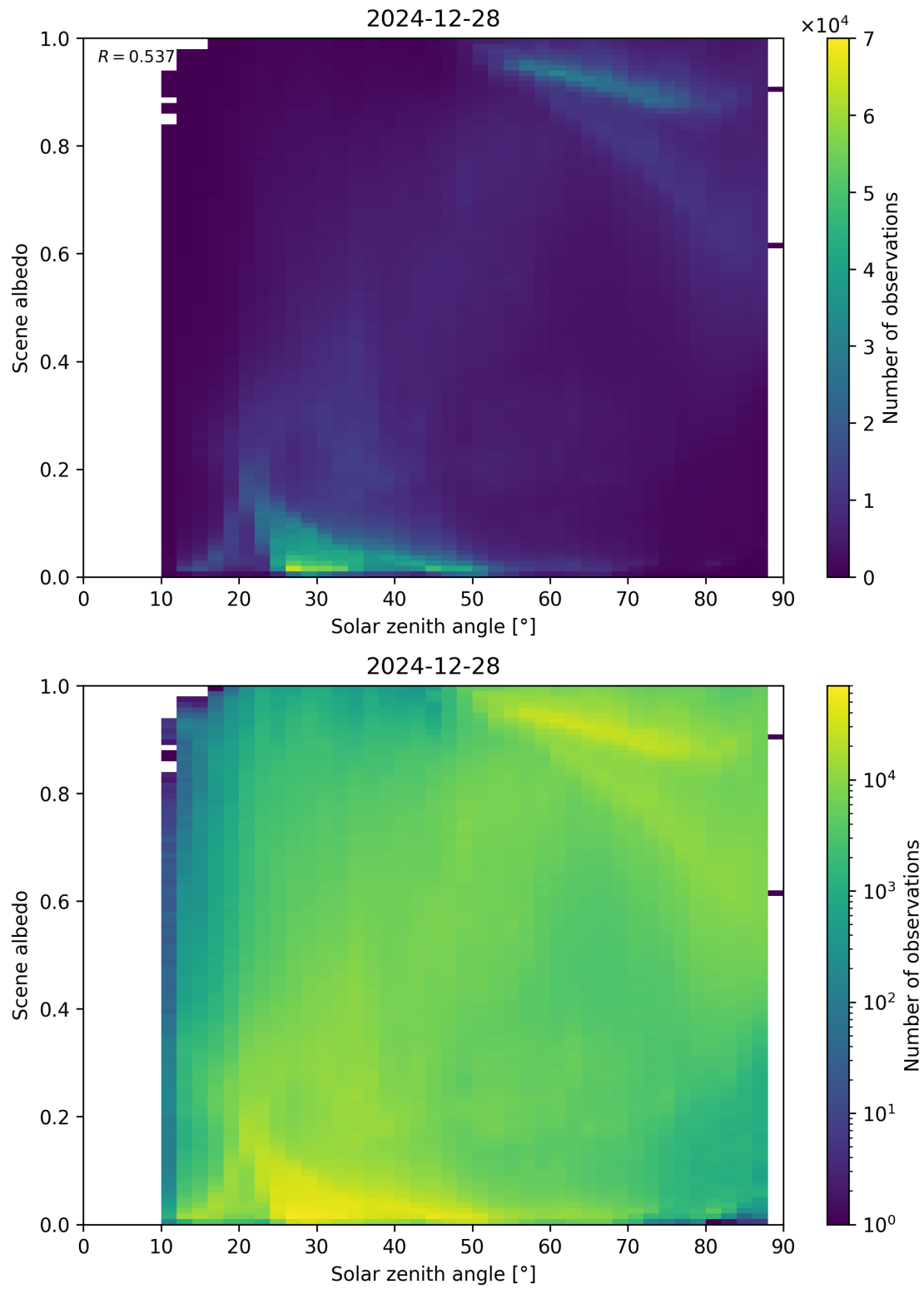
Figure 116: Scatter density plot of “Solar zenith angle” against “Scene albedo” for 2024-12-27 to 2024-12-29.
