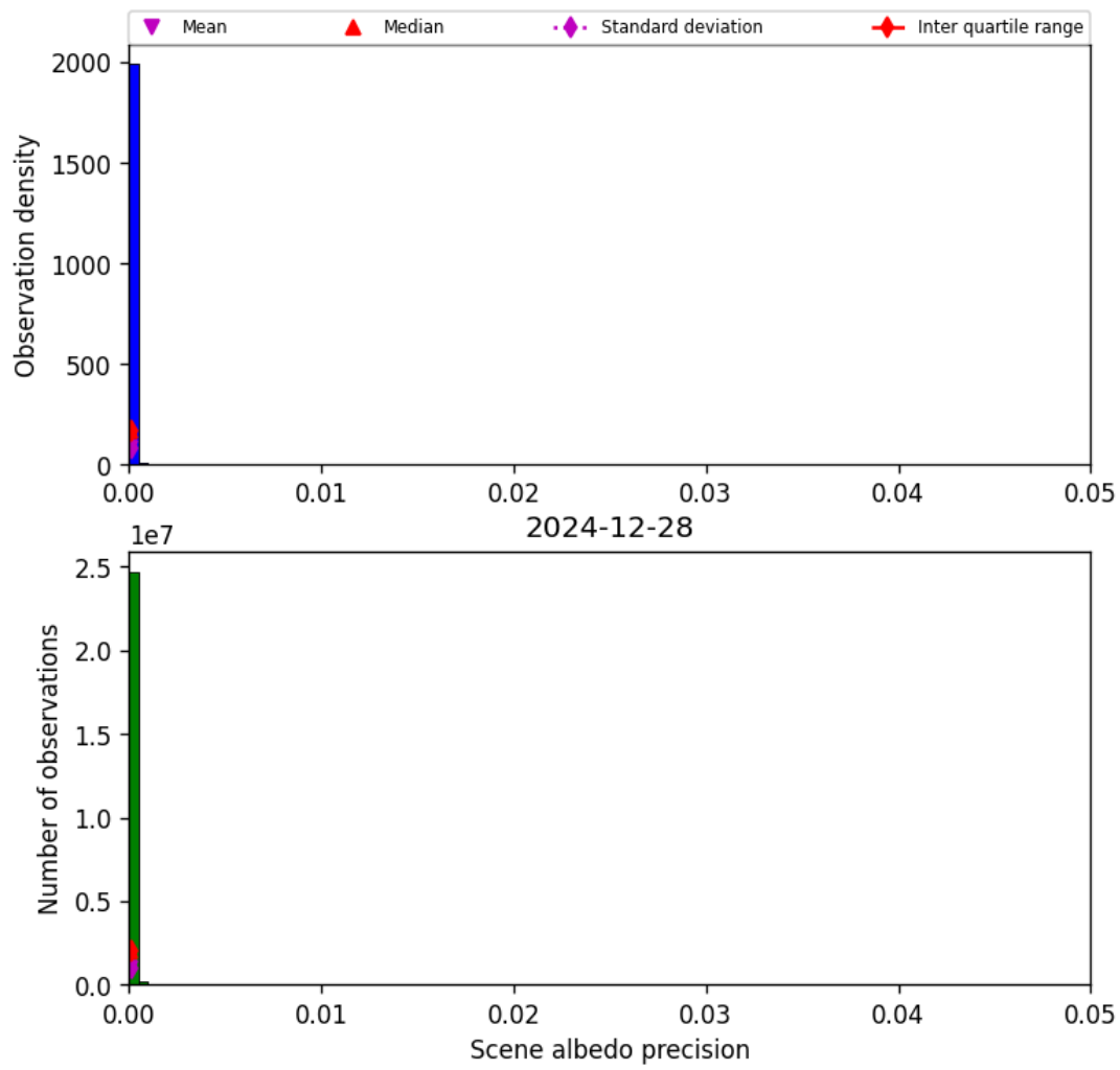
Figure 35: Histogram of “Scene albedo precision” for 2024-12-27 to 2024-12-29
