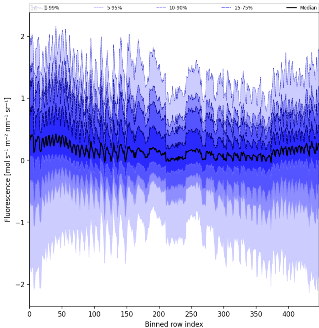
Figure 57: Along track statistics of “Fluorescence” for 2024-12-27 to 2024-12-29
