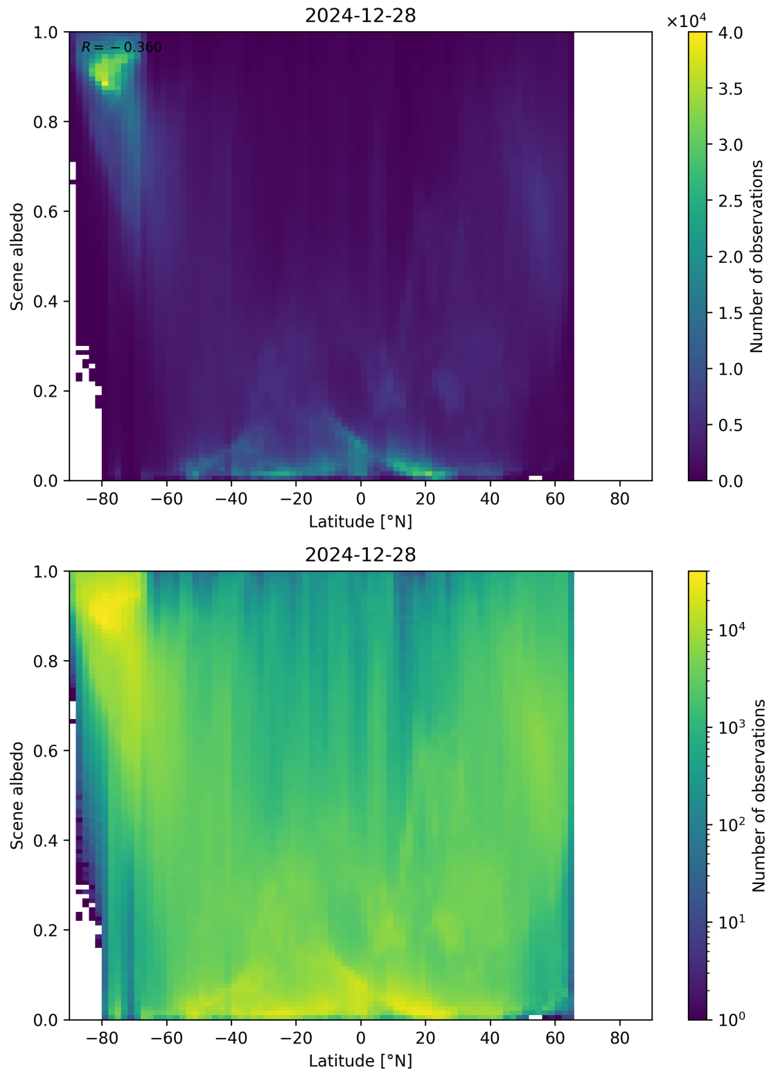
Figure 95: Scatter density plot of “Latitude” against “Scene albedo” for 2024-12-27 to 2024-12-29.
