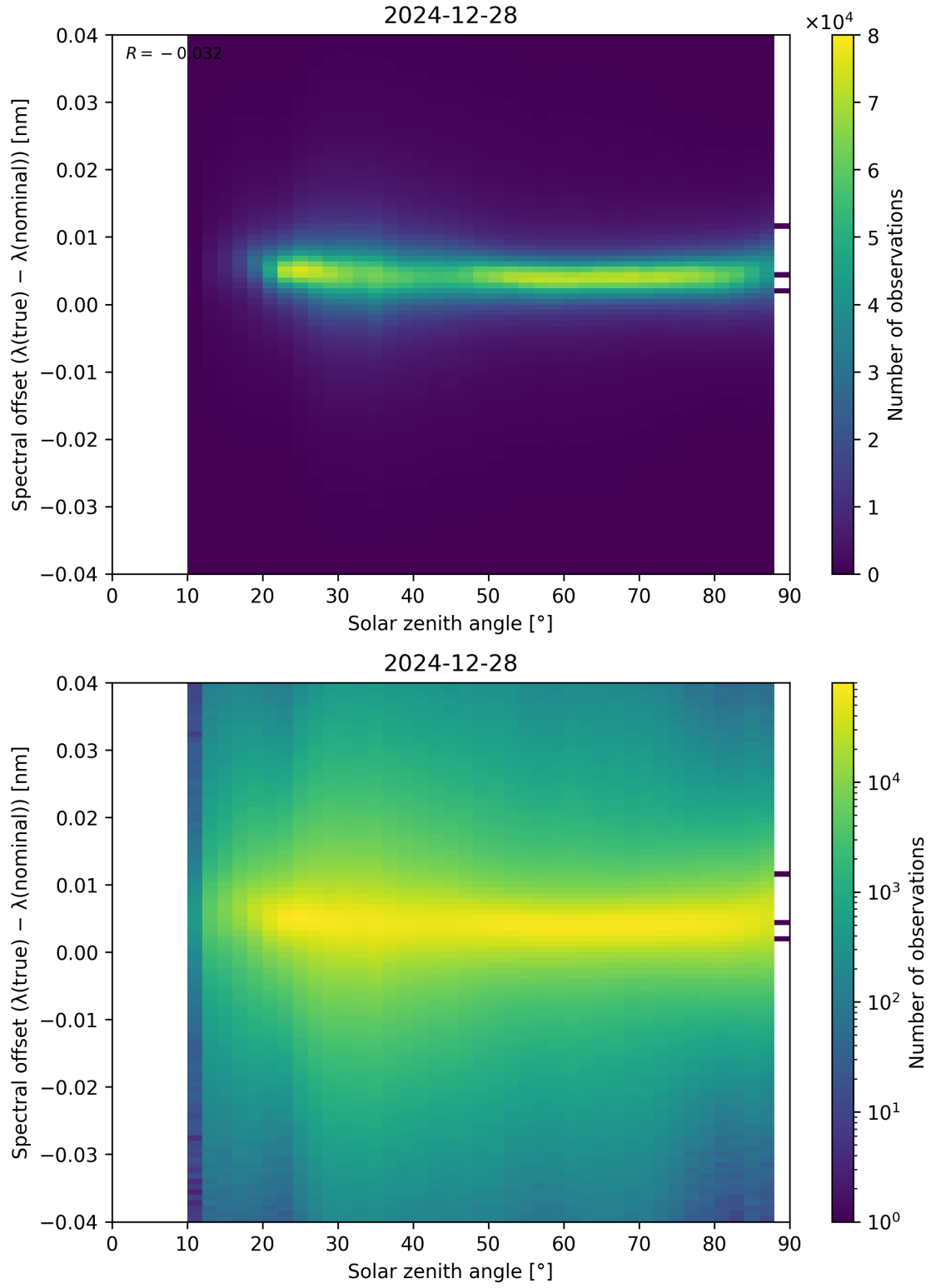
Figure 117: Scatter density plot of “Solar zenith angle” against “Spectral offset ( \lambda_{\text{true}} - \lambda_{\text{nominal}} )” for 2024-12-27 to 2024-12-29.
