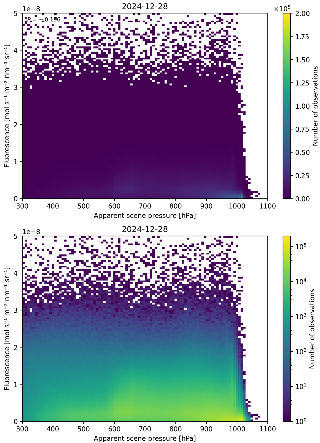
Figure 64: Scatter density plot of “Apparent scene pressure” against “Fluorescence” for 2024-12-27 to 2024-12-29.
