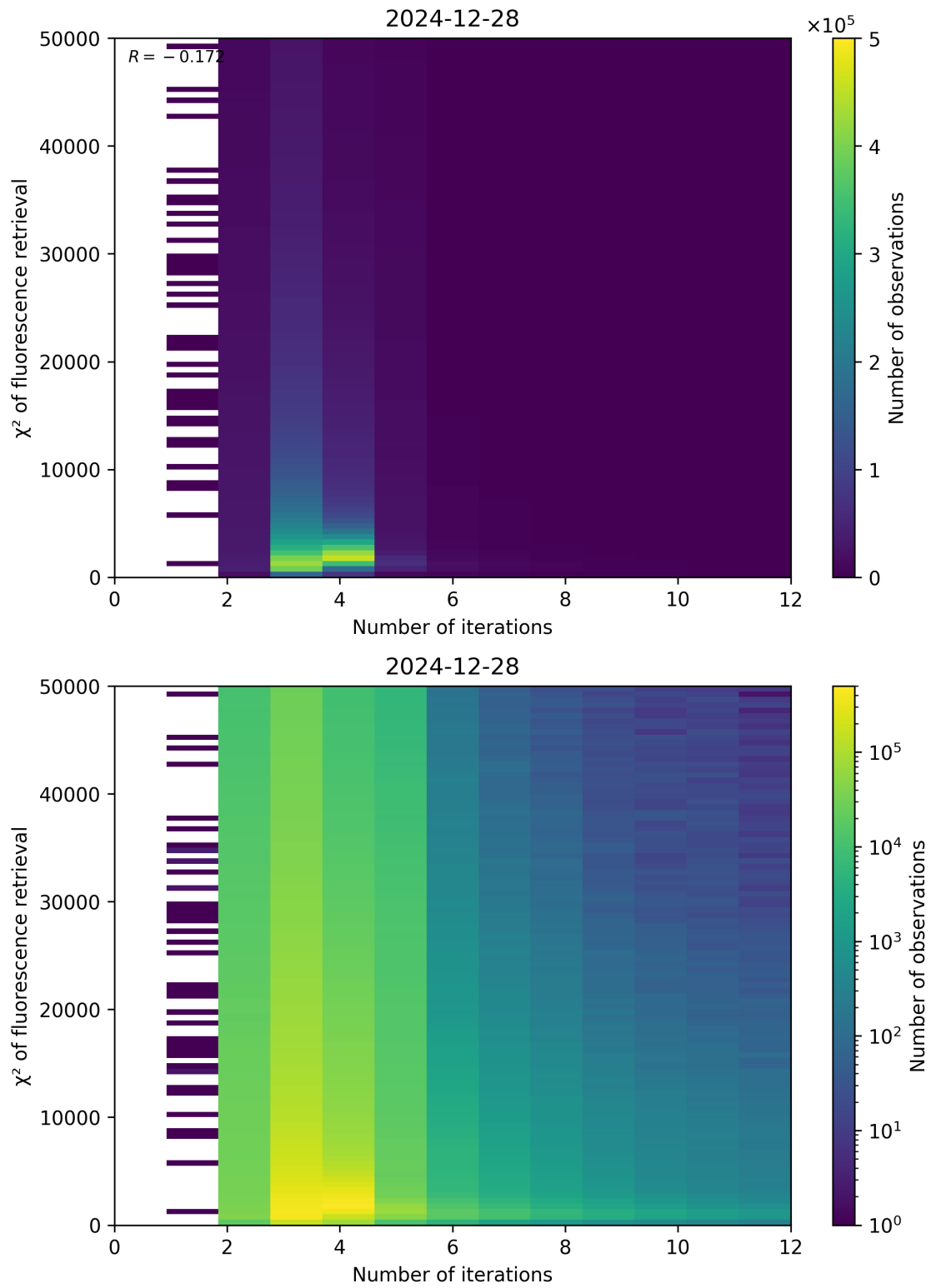
Figure 97: Scatter density plot of “Number of iterations” against “ \chi^2 of fluorescence retrieval” for 2024-12-27 to 2024-12-29.
