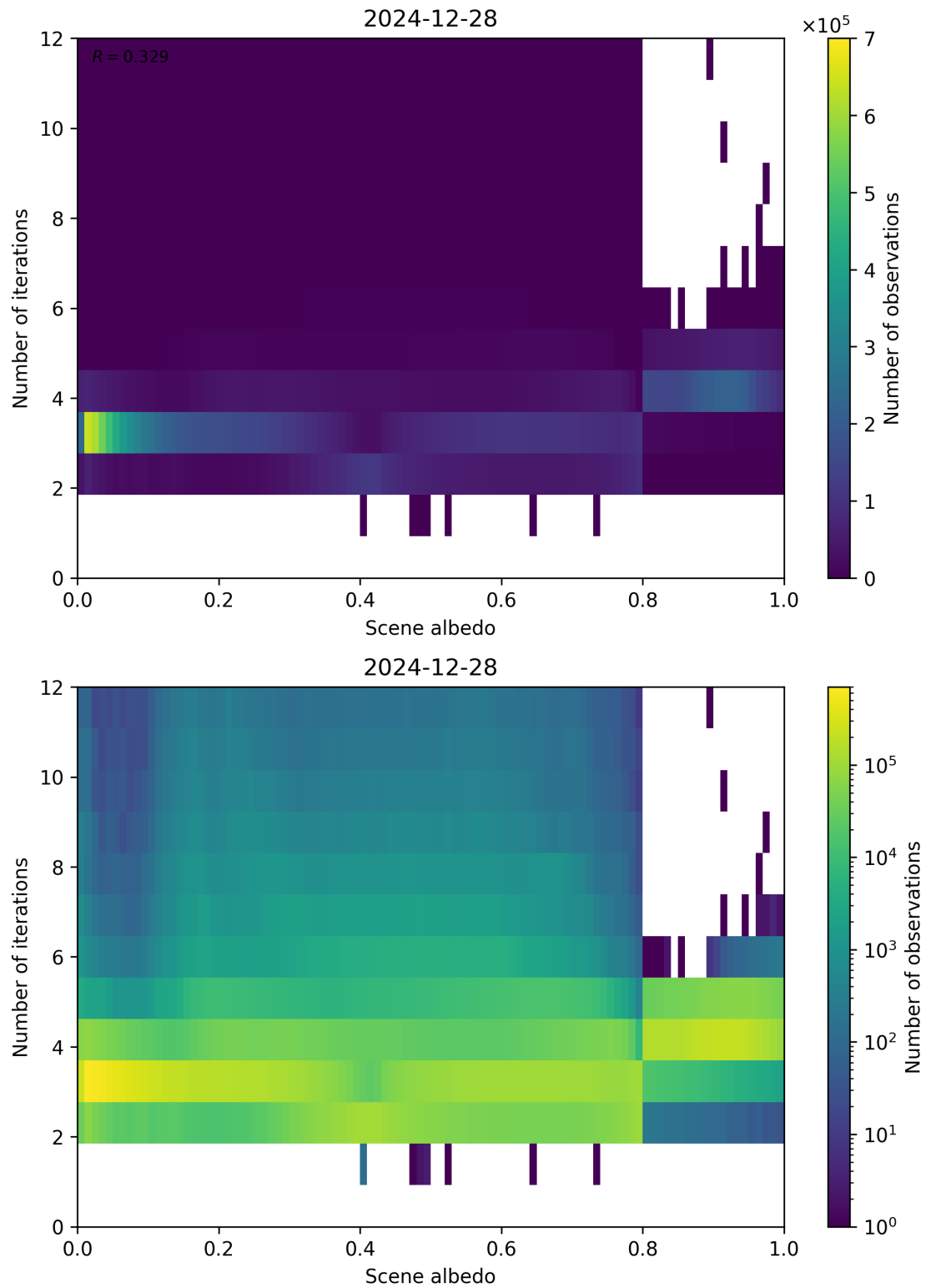
Figure 105: Scatter density plot of “Scene albedo” against “Number of iterations” for 2024-12-27 to 2024-12-29.
