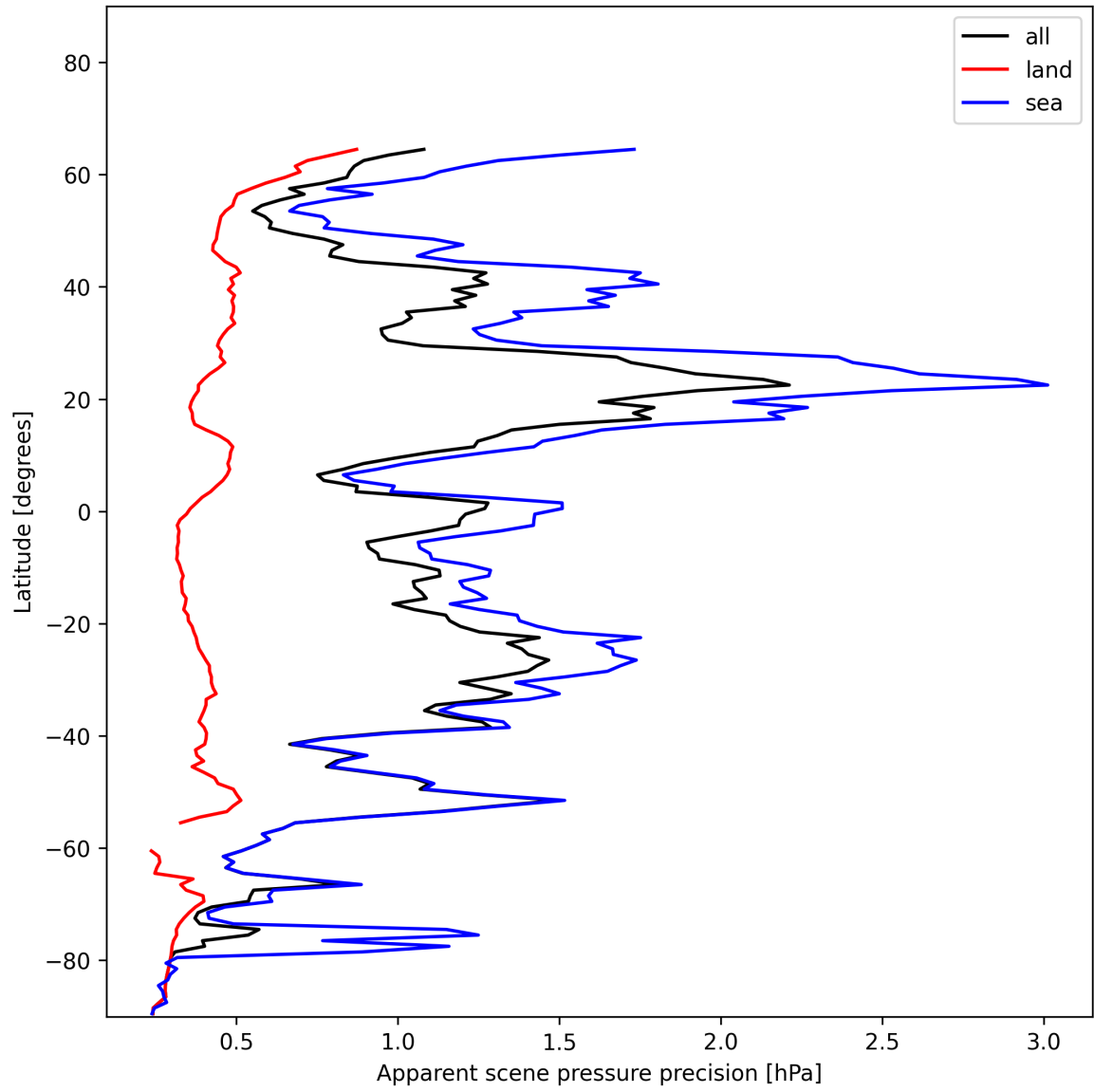
Figure 20: Zonal average of “Apparent scene pressure precision” for 2024-12-27 to 2024-12-29.
