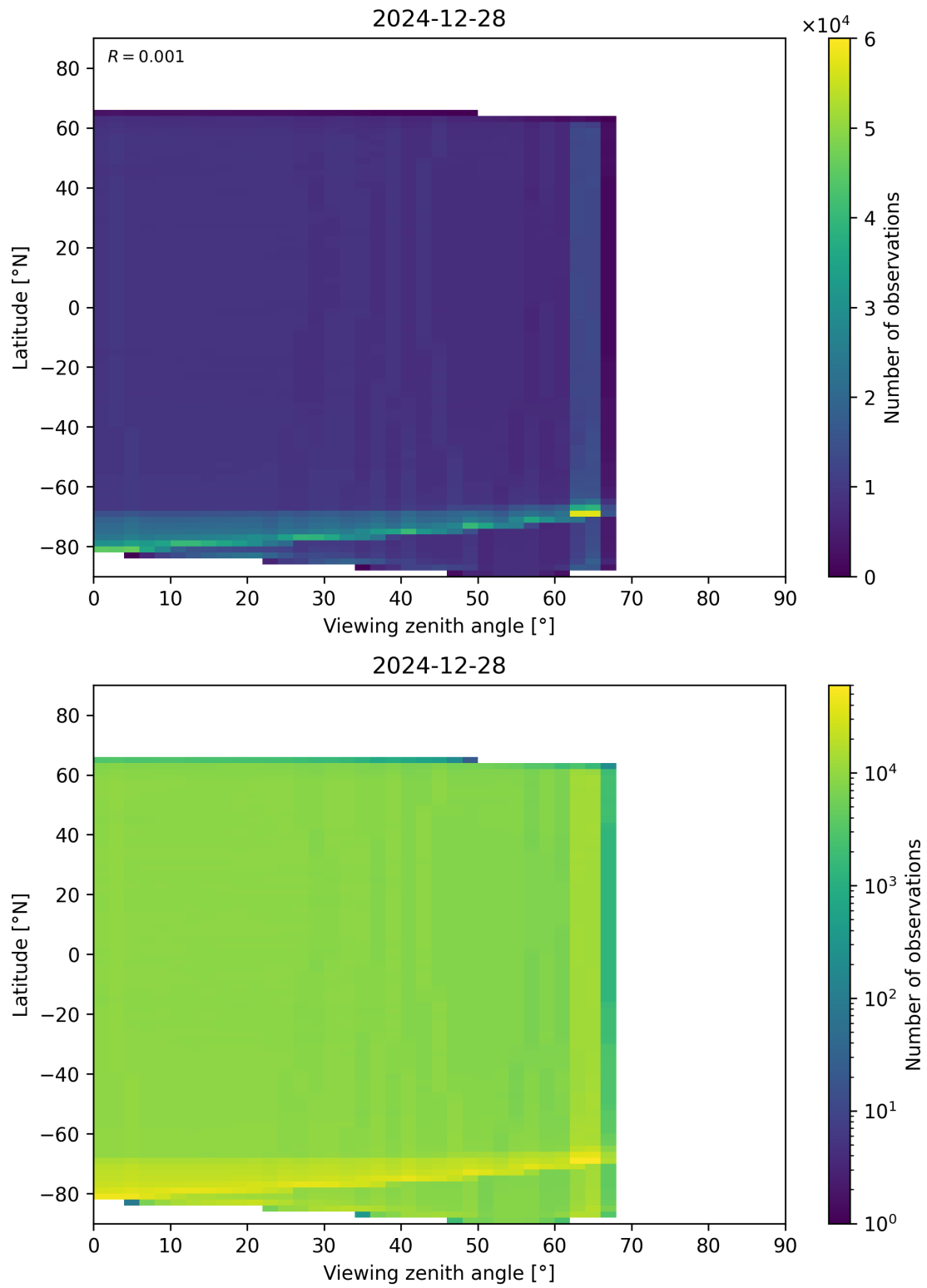
Figure 123: Scatter density plot of “Viewing zenith angle” against “Latitude” for 2024-12-27 to 2024-12-29.
