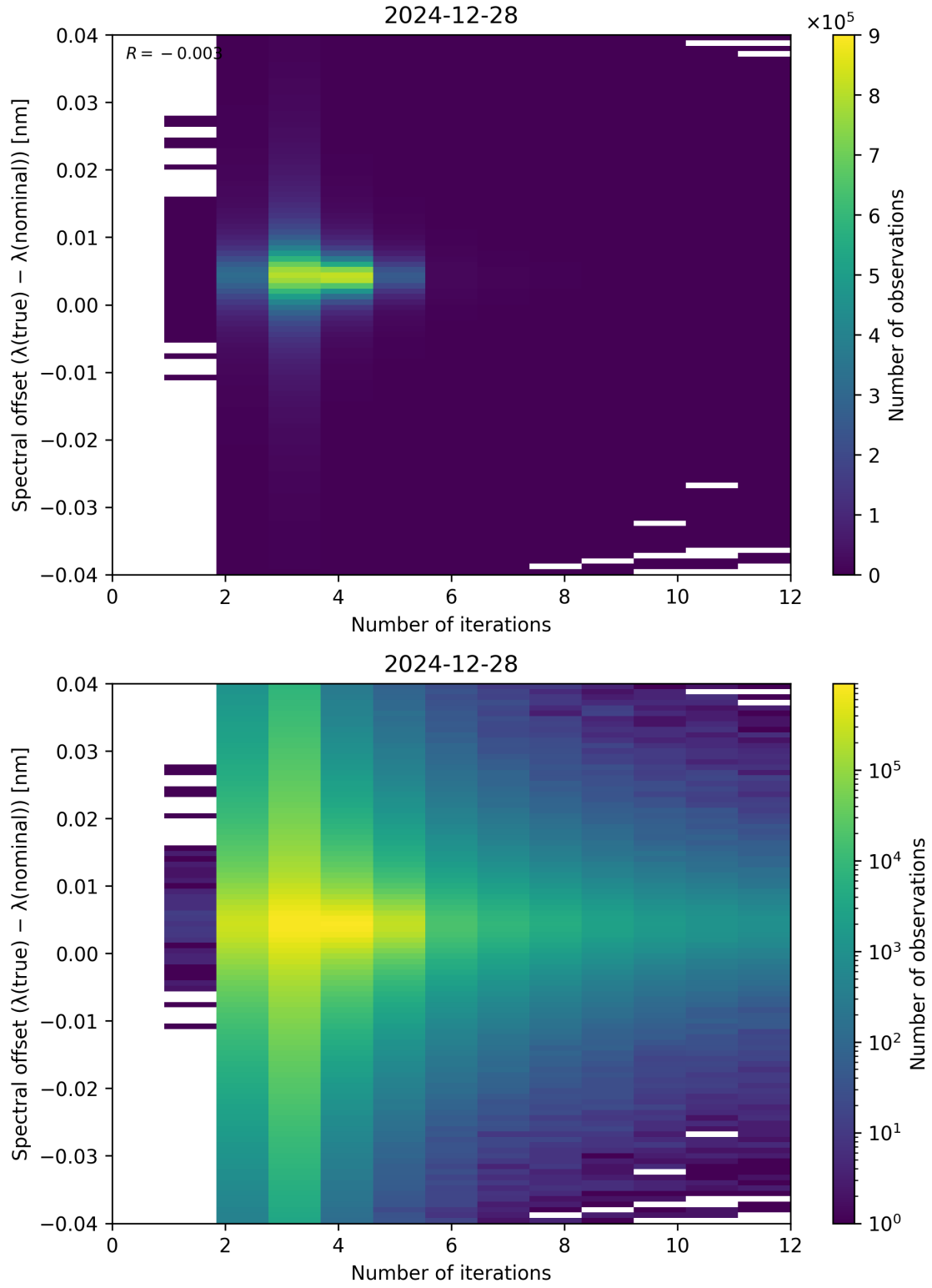
Figure 100: Scatter density plot of “Number of iterations” against “Spectral offset ( \lambda_{\text{true}} - \lambda_{\text{nominal}} )” for 2024-12-27 to 2024-12-29.
