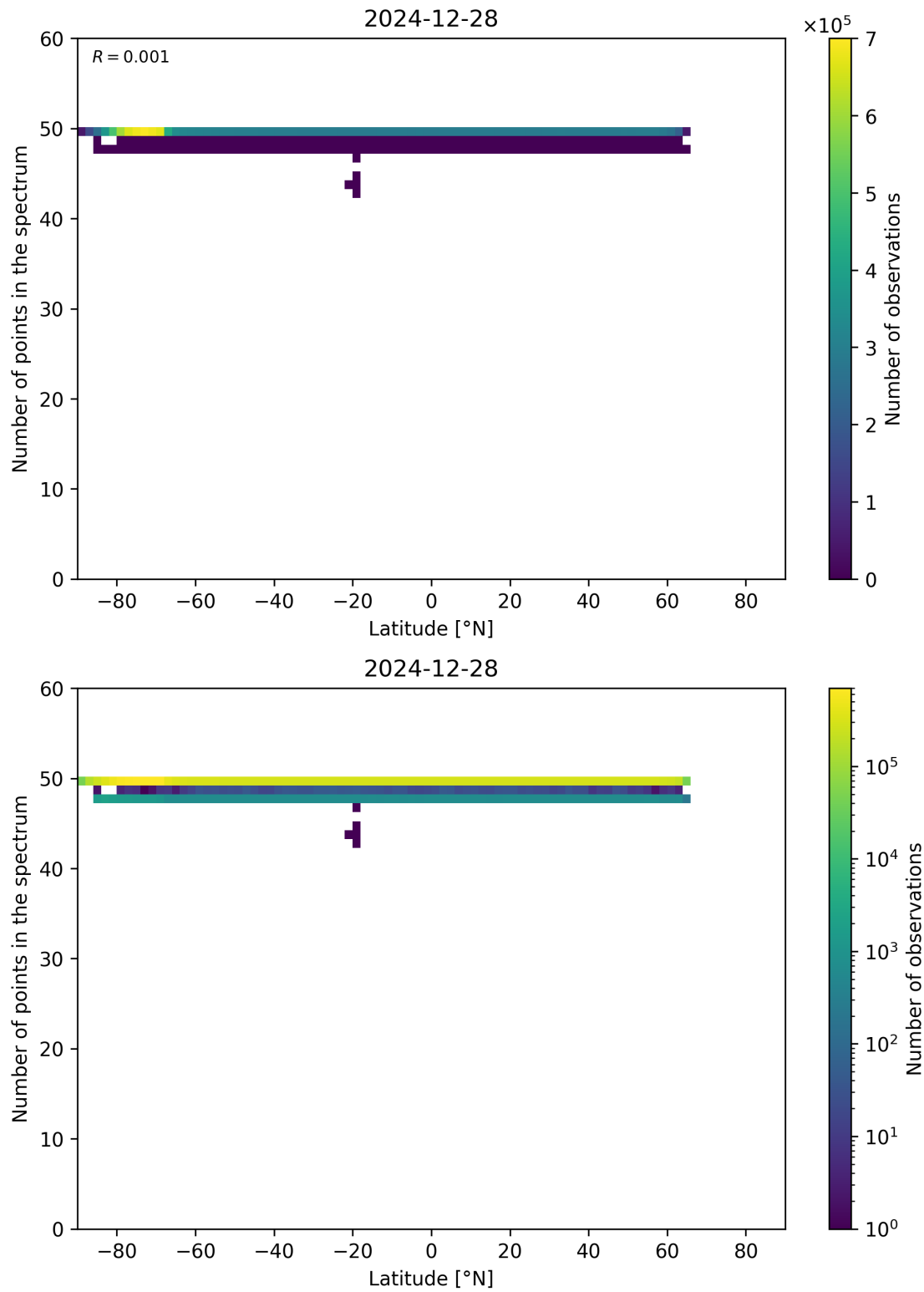
Figure 94: Scatter density plot of “Latitude” against “Number of points in the spectrum” for 2024-12-27 to 2024-12-29.
