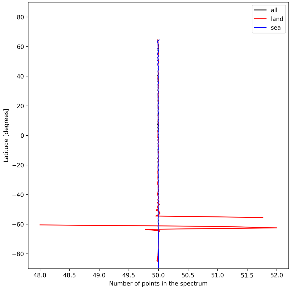
Figure 27: Zonal average of “Number of points in the spectrum” for 2024-12-27 to 2024-12-29.
