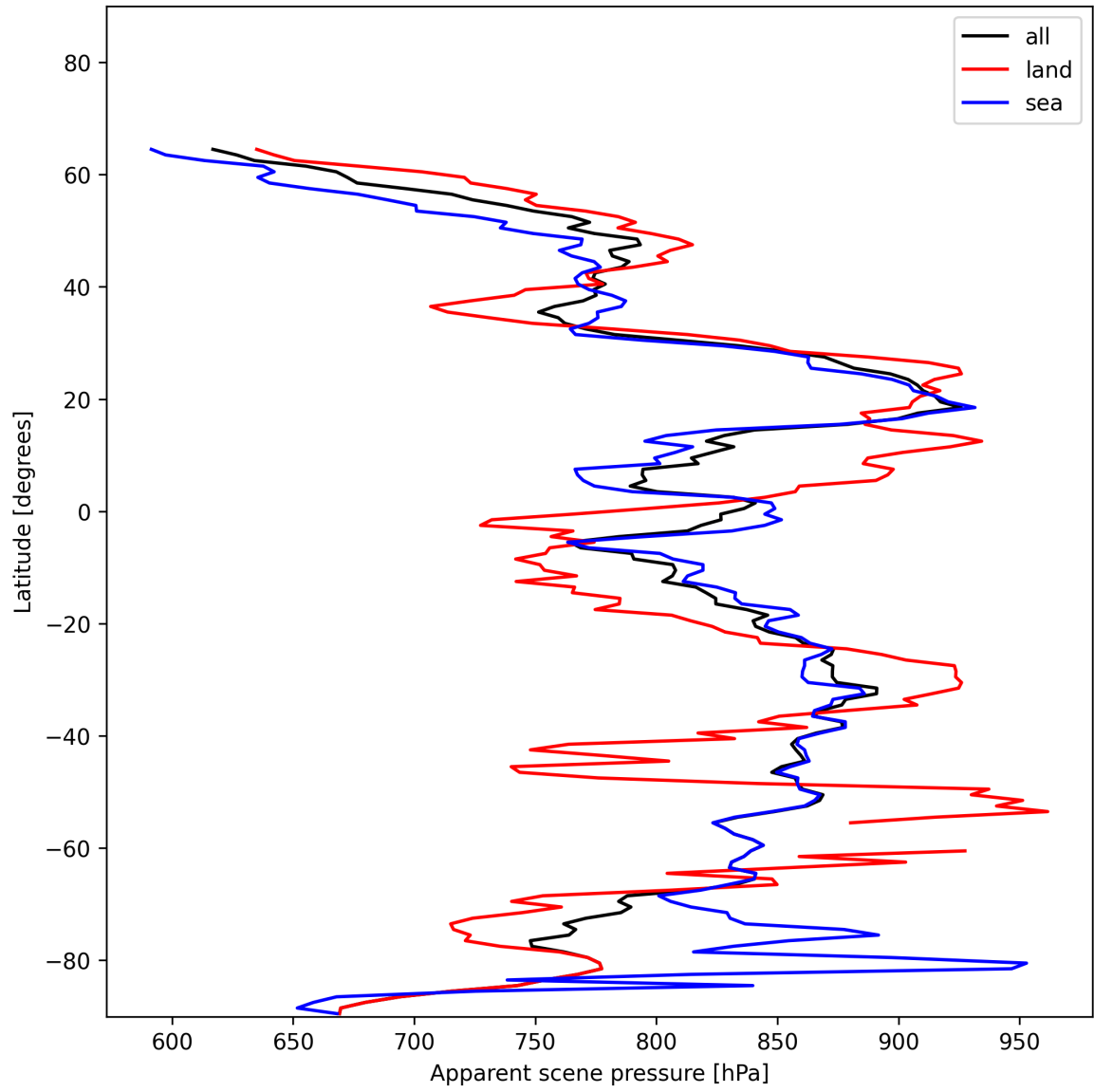
Figure 19: Zonal average of “Apparent scene pressure” for 2024-12-27 to 2024-12-29.
