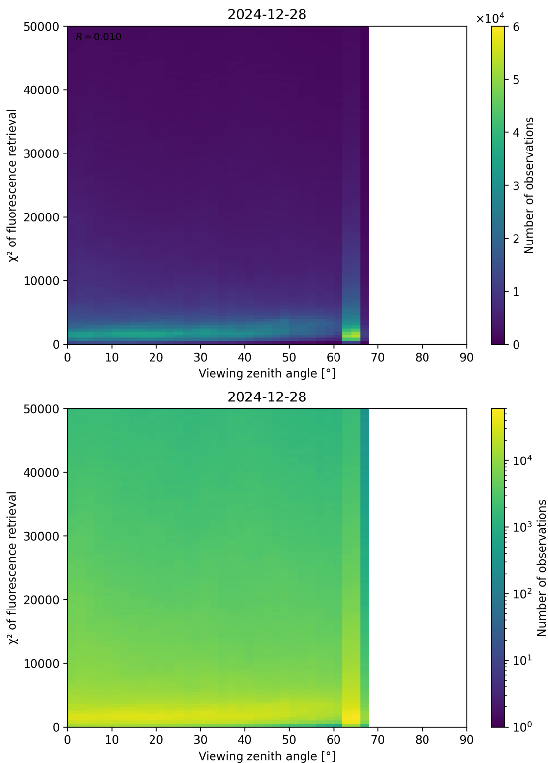
Figure 119: Scatter density plot of “Viewing zenith angle” against “ \chi^2 of fluorescence retrieval” for 2024-12-27 to 2024-12-29.
