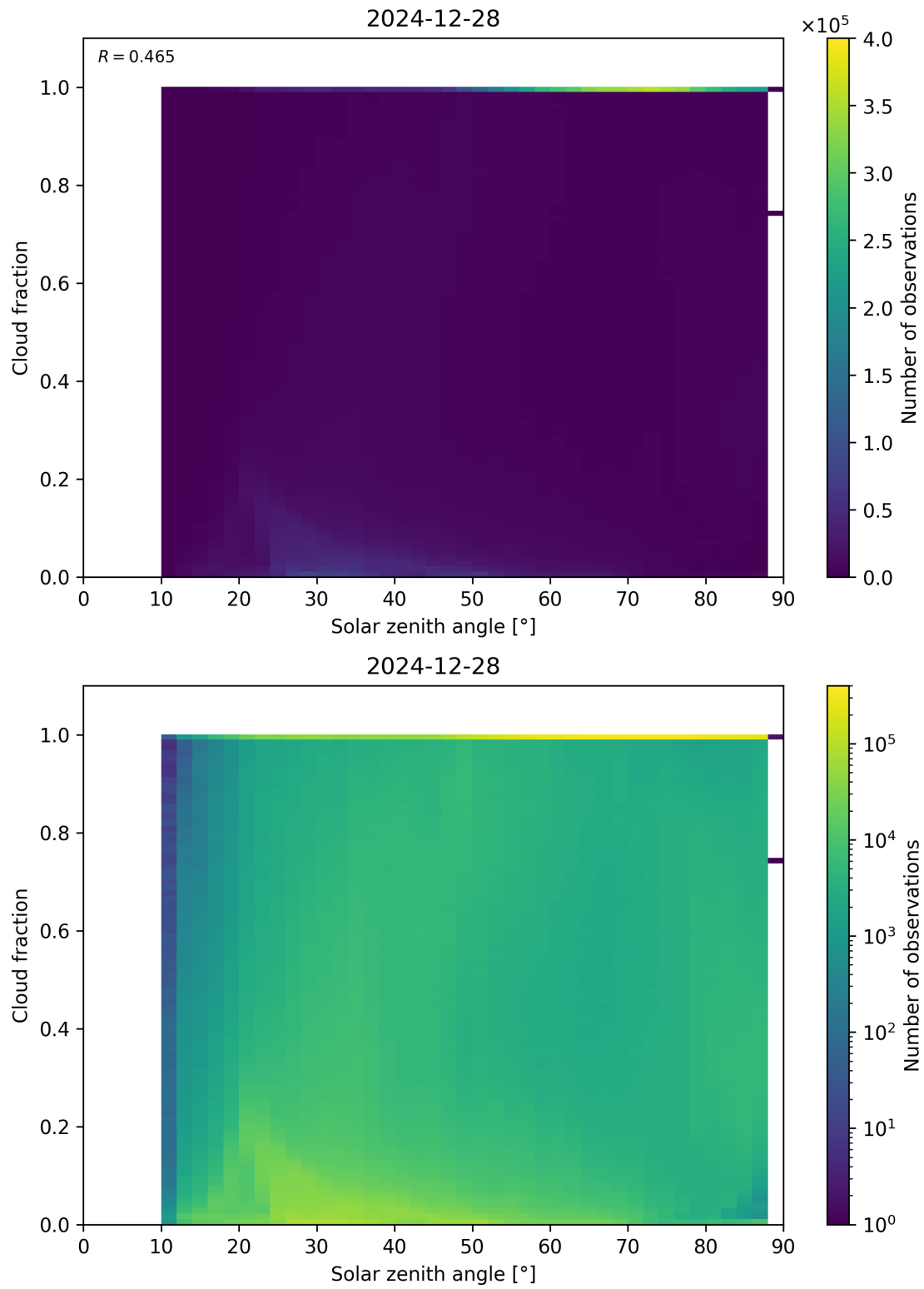
Figure 110: Scatter density plot of “Solar zenith angle” against “Cloud fraction” for 2024-12-27 to 2024-12-29.
