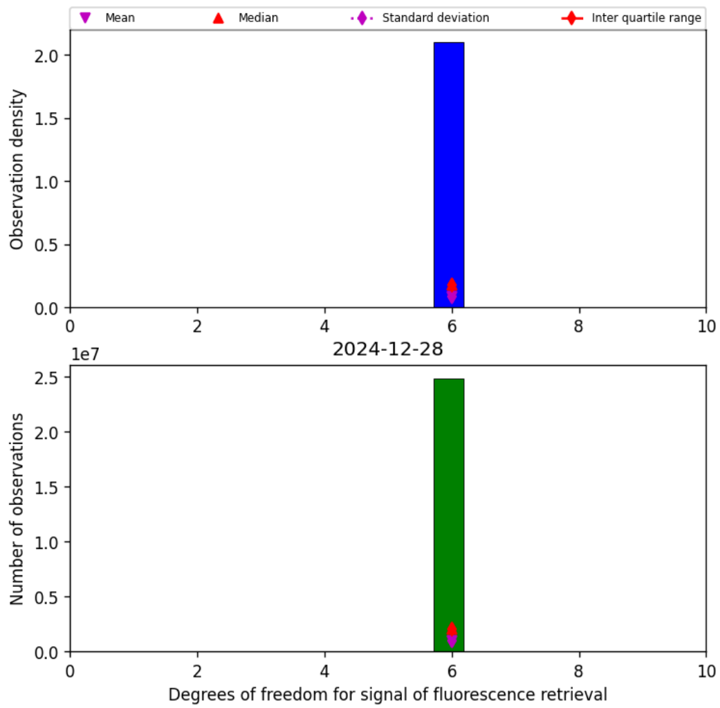
Figure 43: Histogram of “Degrees of freedom for signal of fluorescence retrieval” for 2024-12-27 to 2024-12-29
