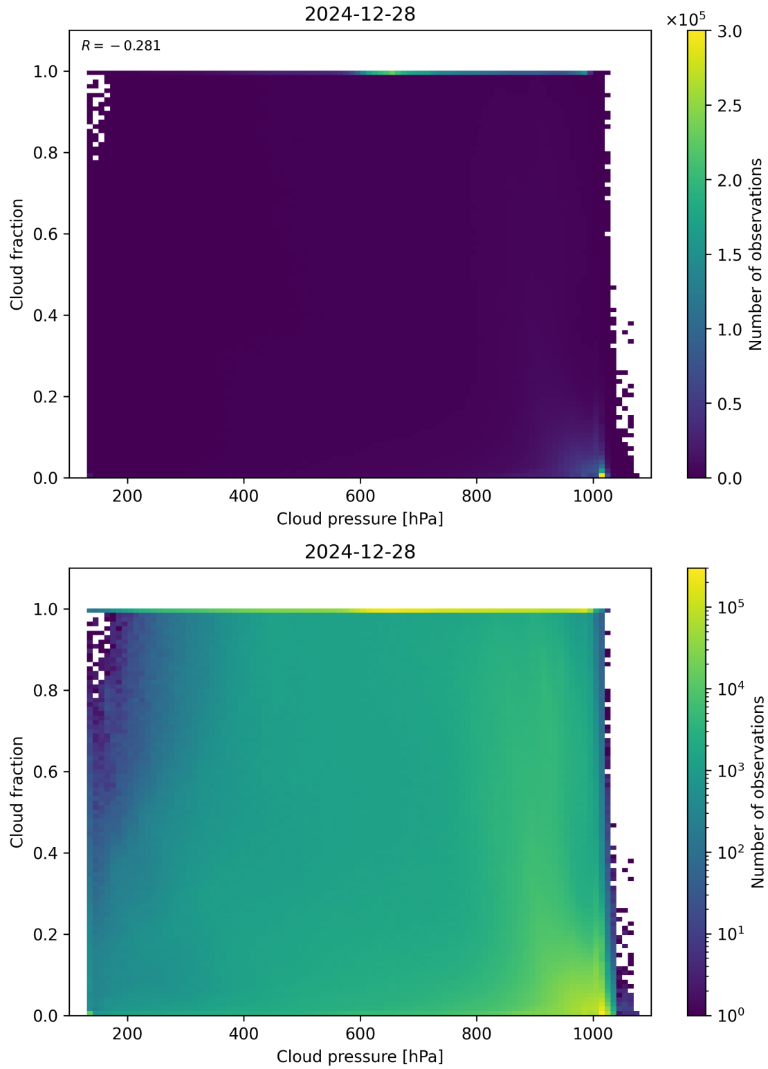
Figure 79: Scatter density plot of “Cloud pressure” against “Cloud fraction” for 2024-12-27 to 2024-12-29.
