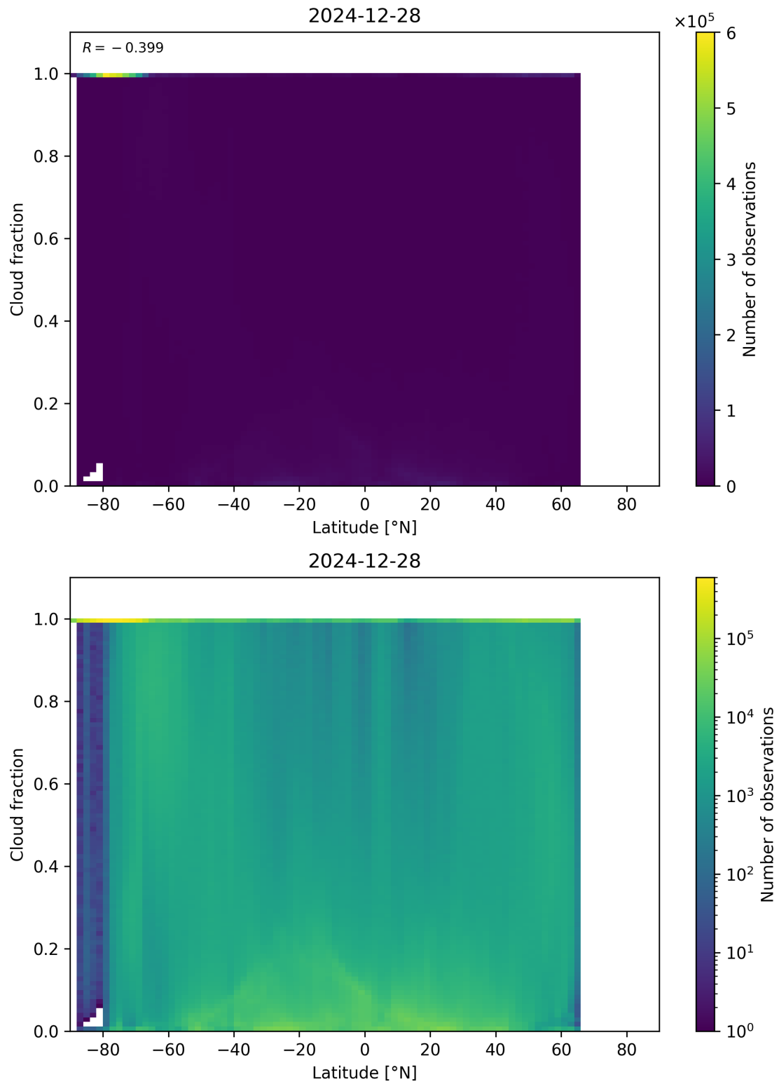
Figure 90: Scatter density plot of “Latitude” against “Cloud fraction” for 2024-12-27 to 2024-12-29.
