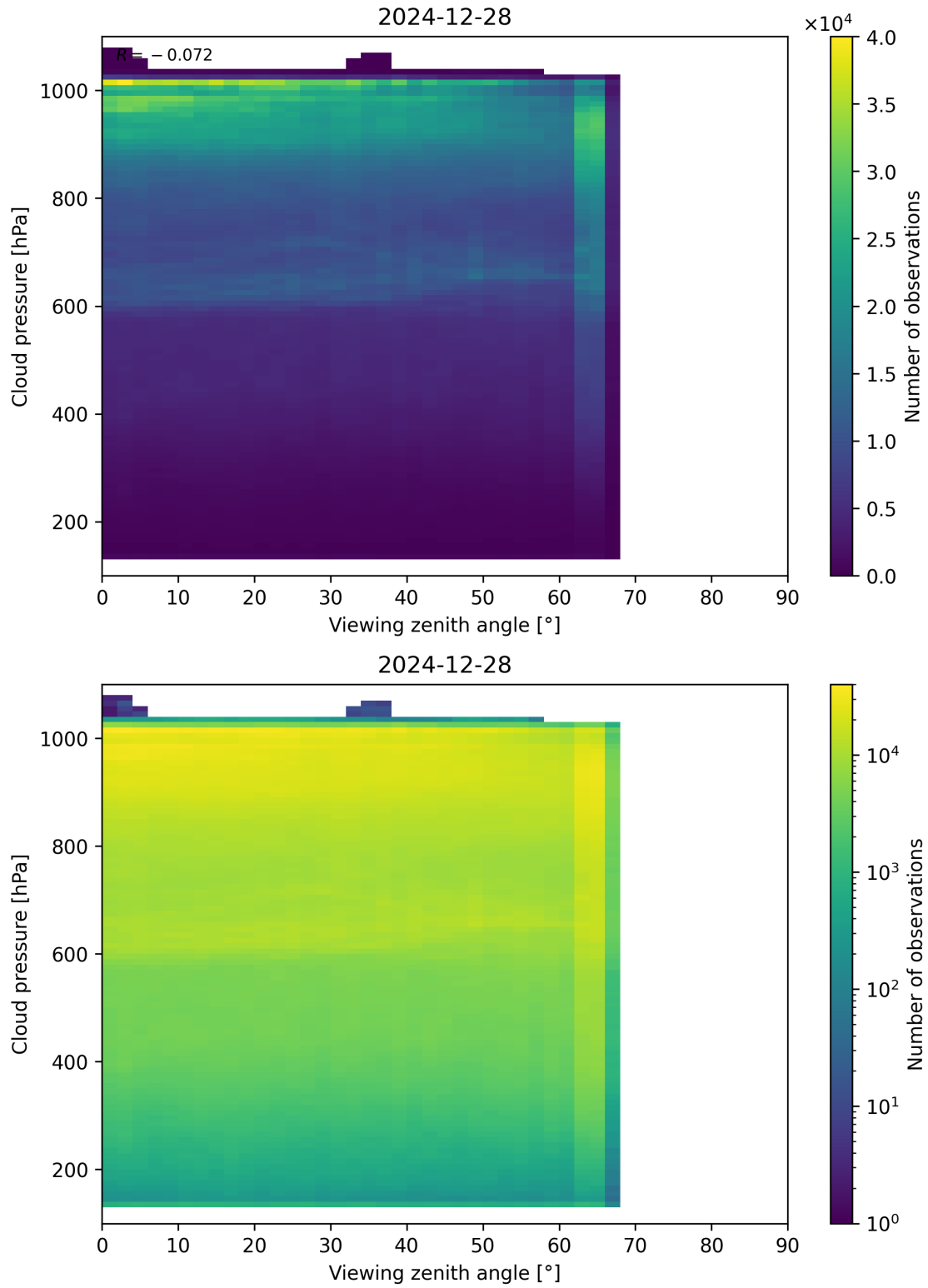
Figure 121: Scatter density plot of “Viewing zenith angle” against “Cloud pressure” for 2024-12-27 to 2024-12-29.
