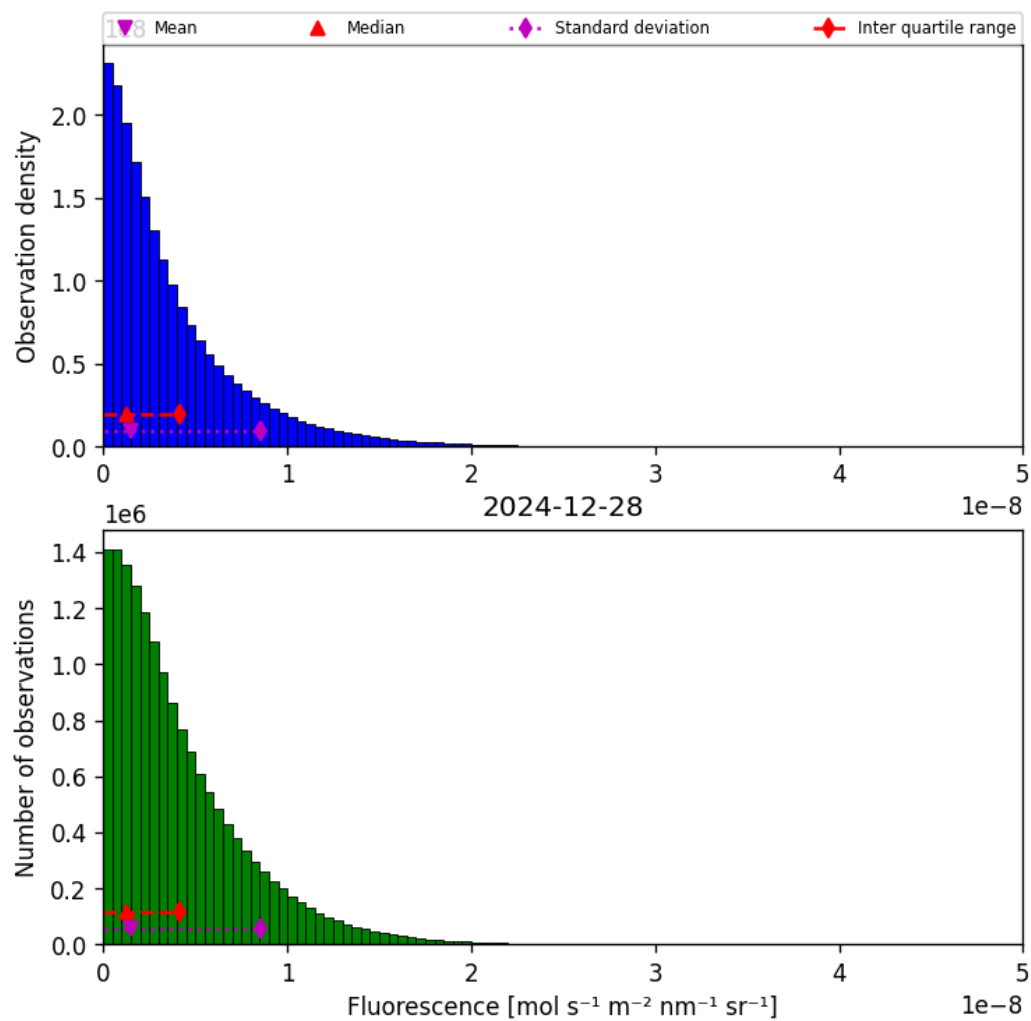
Figure 40: Histogram of “Fluorescence” for 2024-12-27 to 2024-12-29
