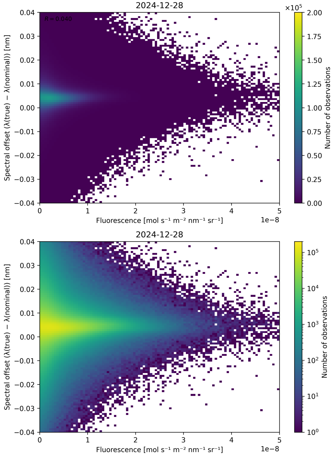
Figure 87: Scatter density plot of “Fluorescence” against “Spectral offset ( \lambda_{\text{true}} - \lambda_{\text{nominal}} )” for 2024-12-27 to 2024-12-29.
