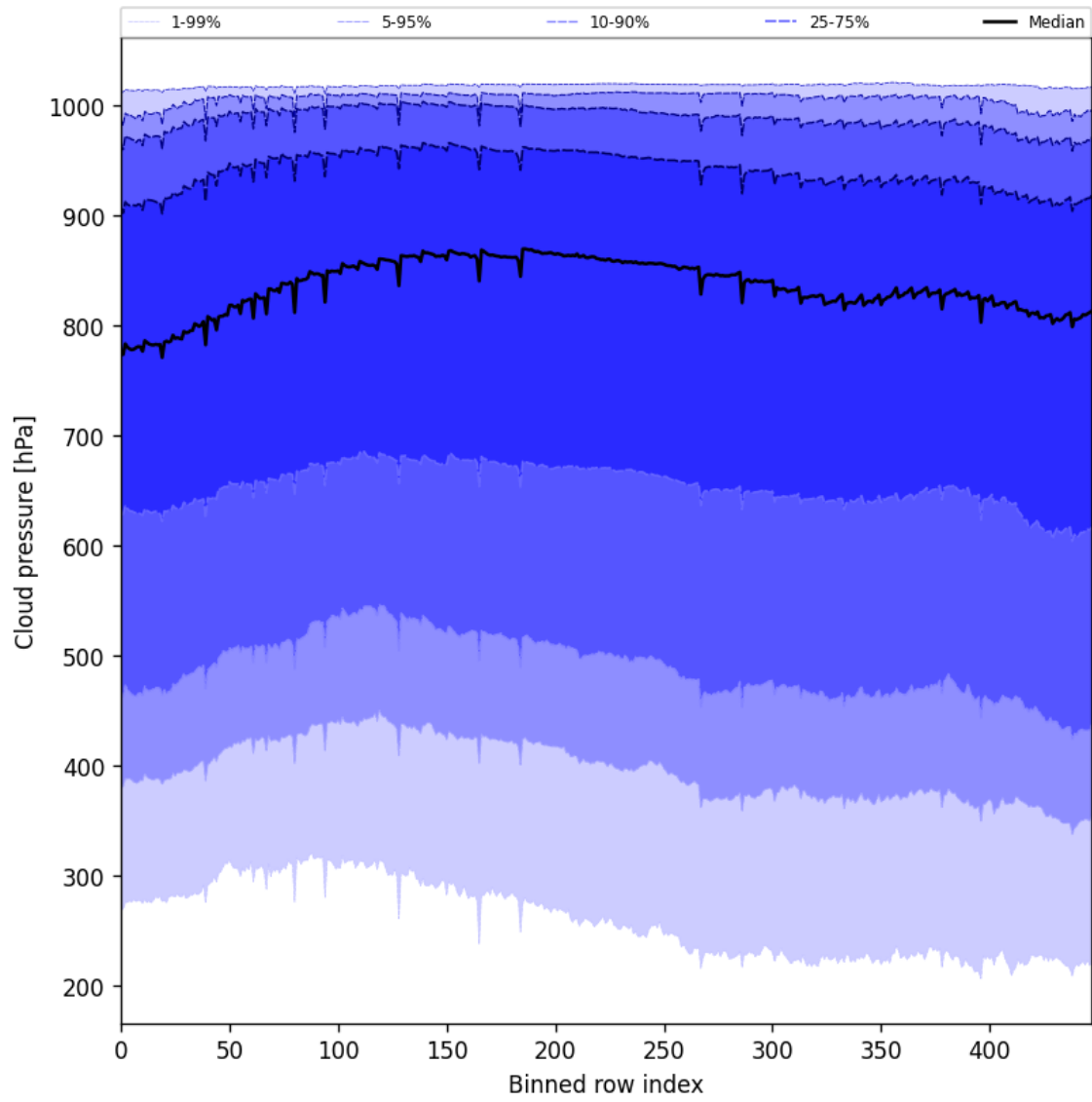
Figure 47: Along track statistics of “Cloud pressure” for 2024-12-27 to 2024-12-29
