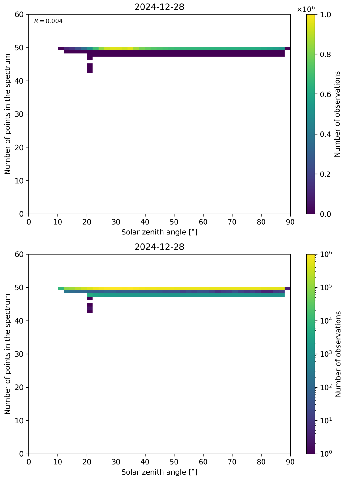
Figure 115: Scatter density plot of “Solar zenith angle” against “Number of points in the spectrum” for 2024-12-27 to 2024-12-29.
