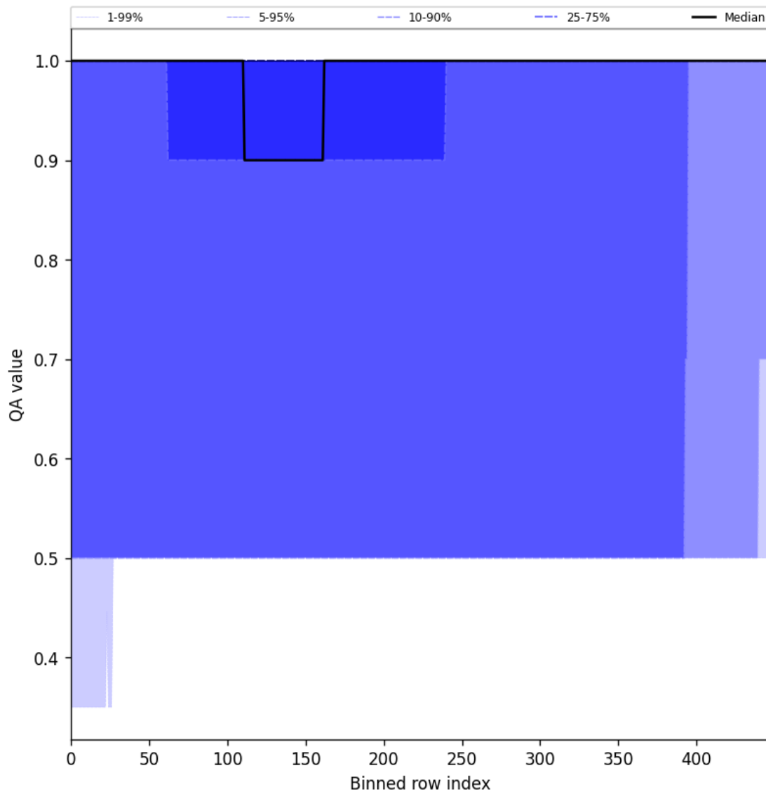
Figure 46: Along track statistics of “QA value” for 2024-12-27 to 2024-12-29
