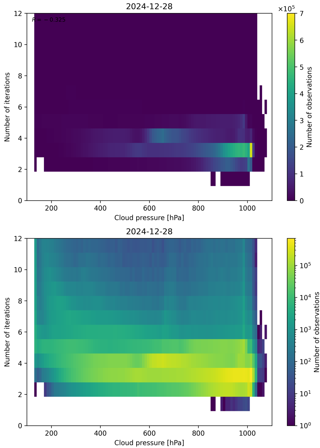
Figure 81: Scatter density plot of “Cloud pressure” against “Number of iterations” for 2024-12-27 to 2024-12-29.
