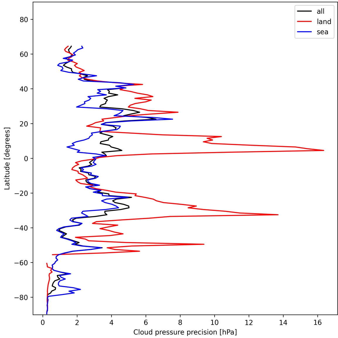
Figure 14: Zonal average of “Cloud pressure precision” for 2024-12-27 to 2024-12-29.
