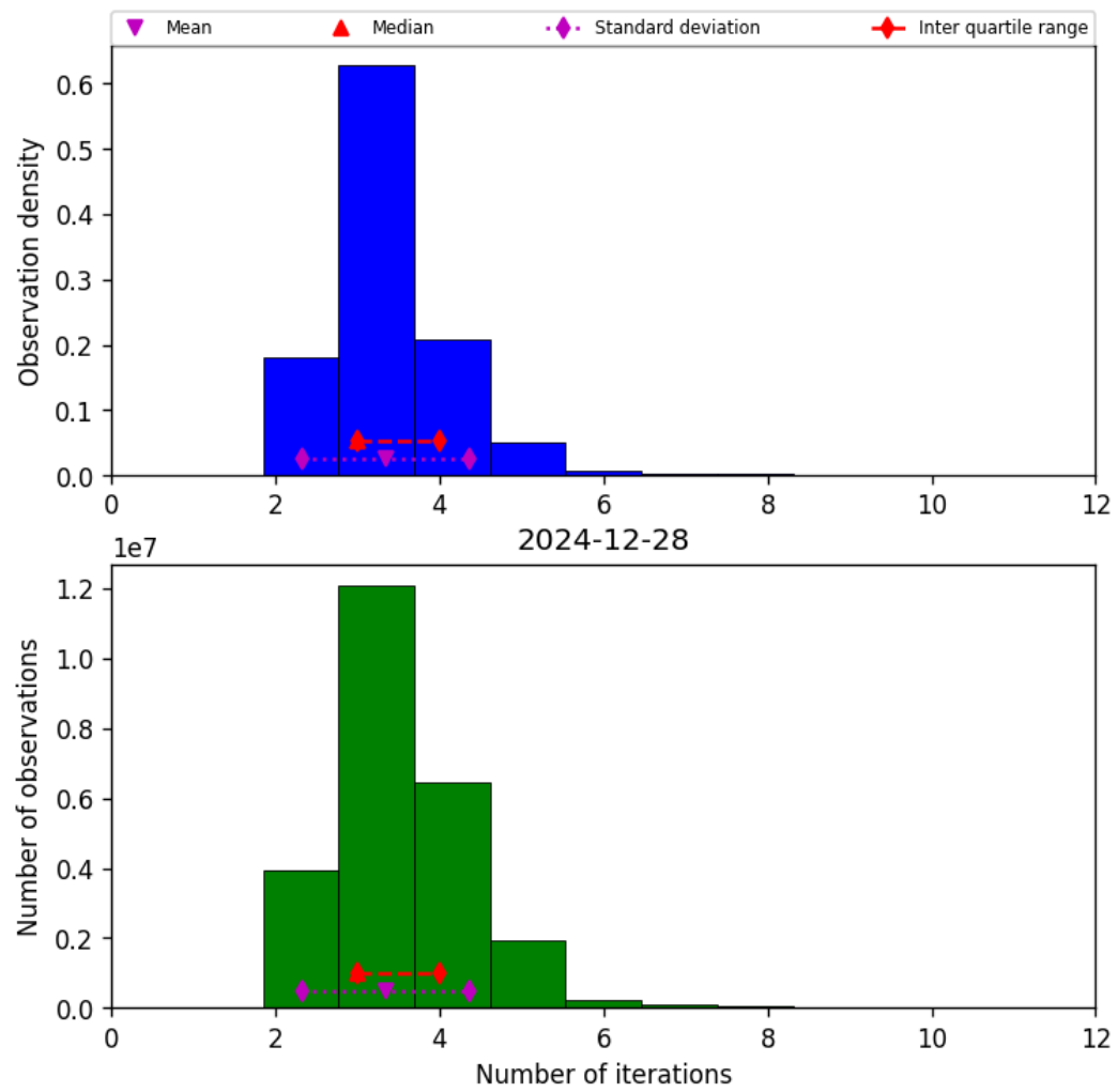
Figure 39: Histogram of “Number of iterations” for 2024-12-27 to 2024-12-29
