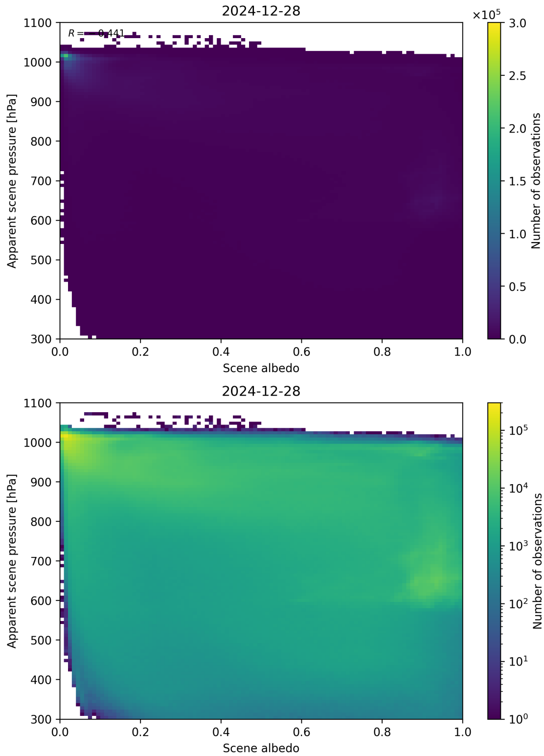
Figure 102: Scatter density plot of “Scene albedo” against “Apparent scene pressure” for 2024-12-27 to 2024-12-29.
