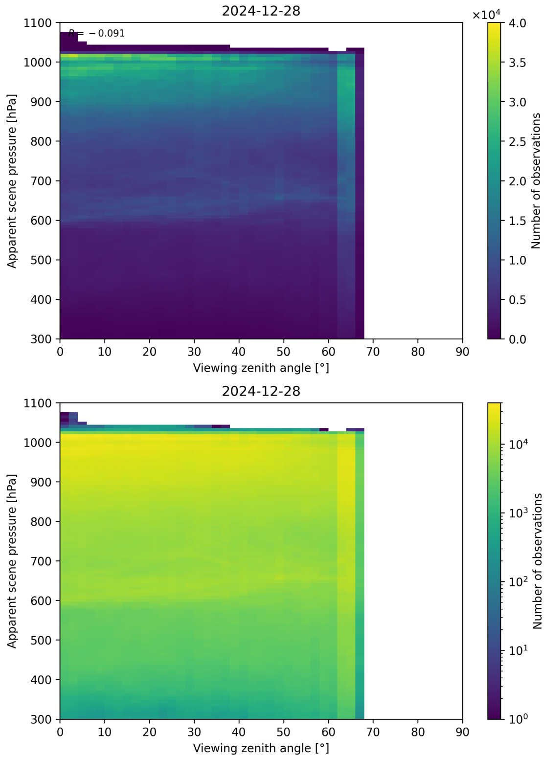
Figure 118: Scatter density plot of “Viewing zenith angle” against “Apparent scene pressure” for 2024-12-27 to 2024-12-29.
