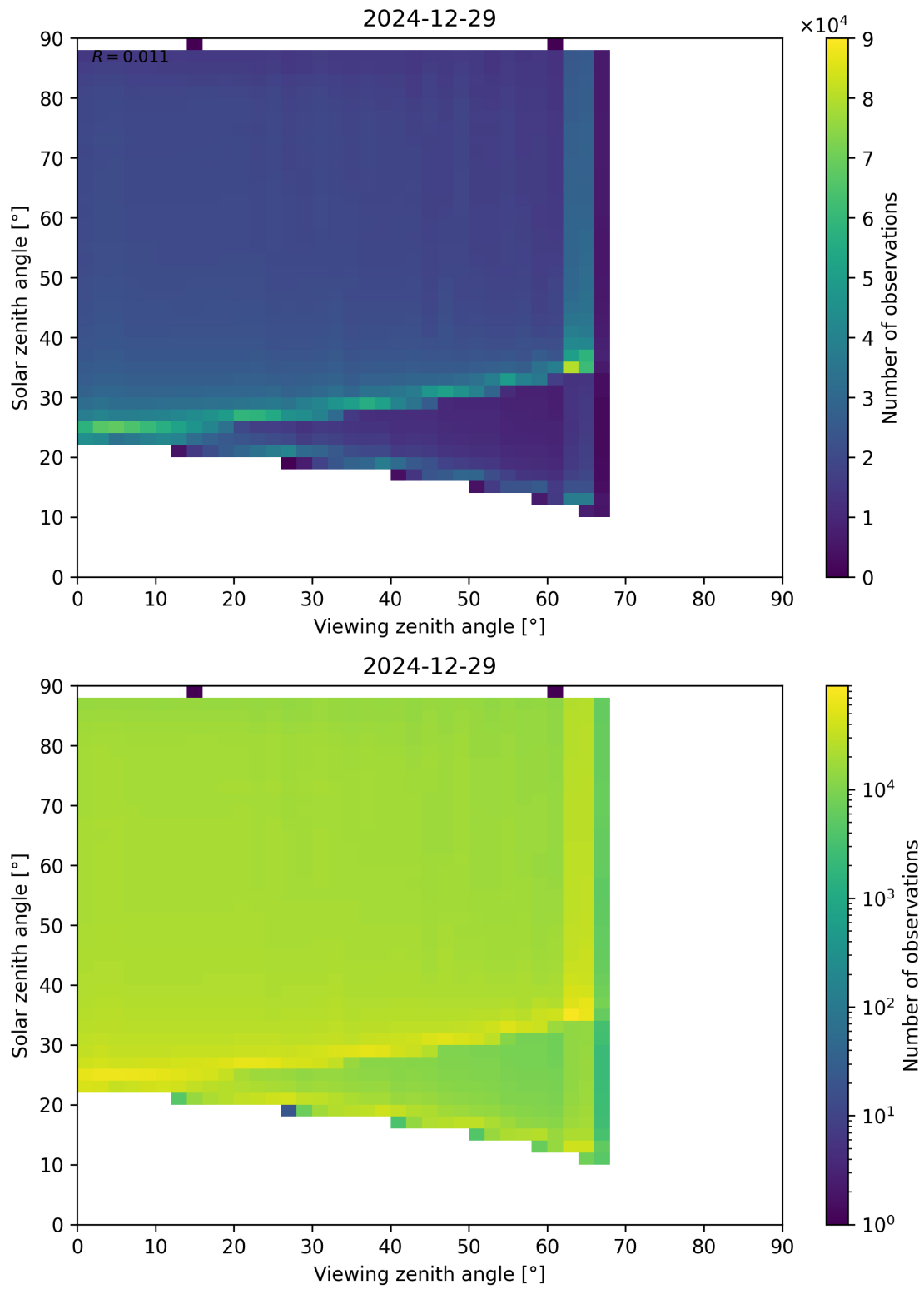
Figure 127: Scatter density plot of “Viewing zenith angle” against “Solar zenith angle” for 2024-12-28 to 2024-12-30.
