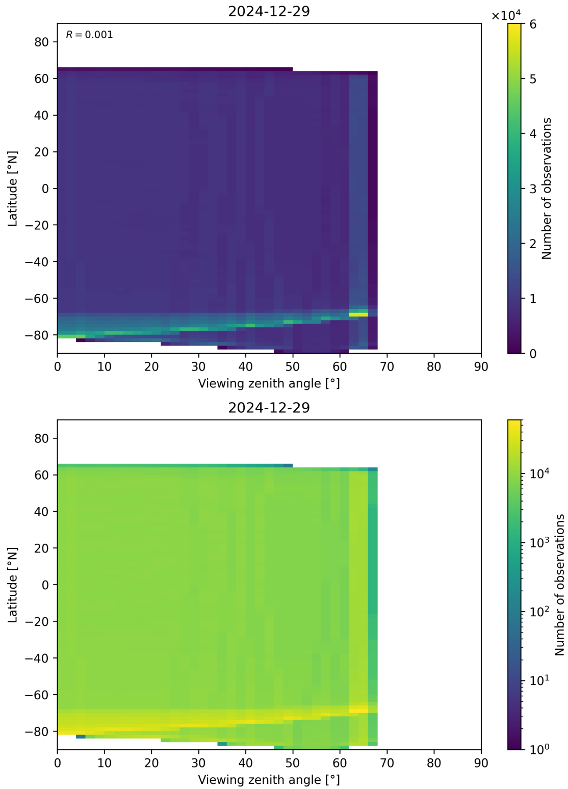
Figure 123: Scatter density plot of “Viewing zenith angle” against “Latitude” for 2024-12-28 to 2024-12-30.
