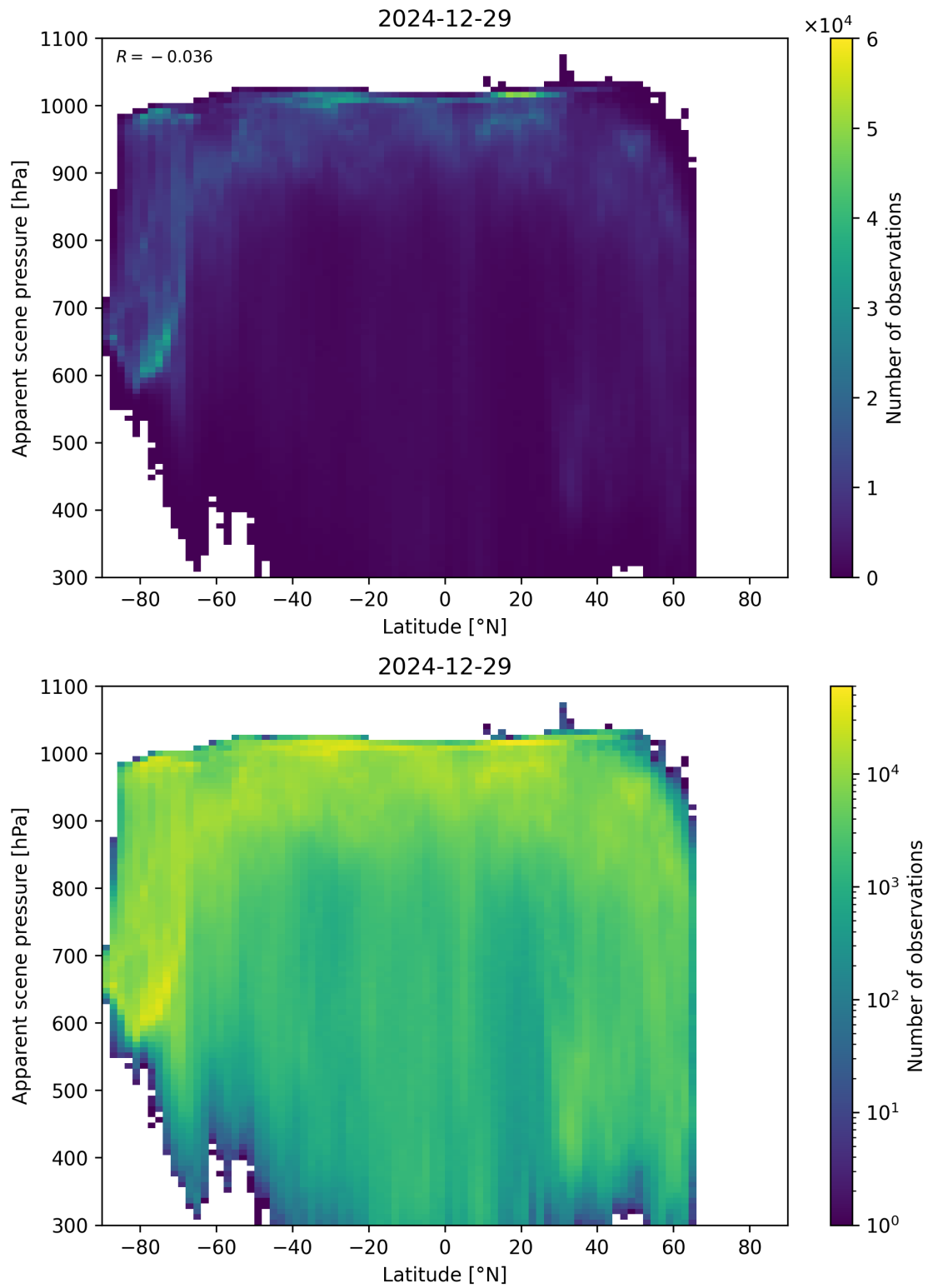
Figure 88: Scatter density plot of “Latitude” against “Apparent scene pressure” for 2024-12-28 to 2024-12-30.
