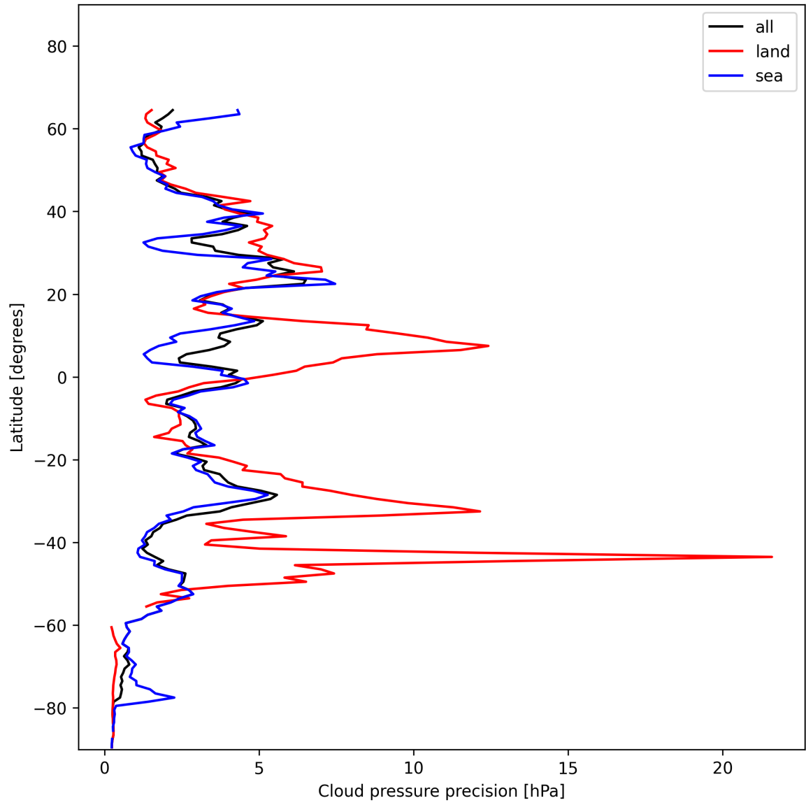
Figure 14: Zonal average of “Cloud pressure precision” for 2024-12-28 to 2024-12-30.
