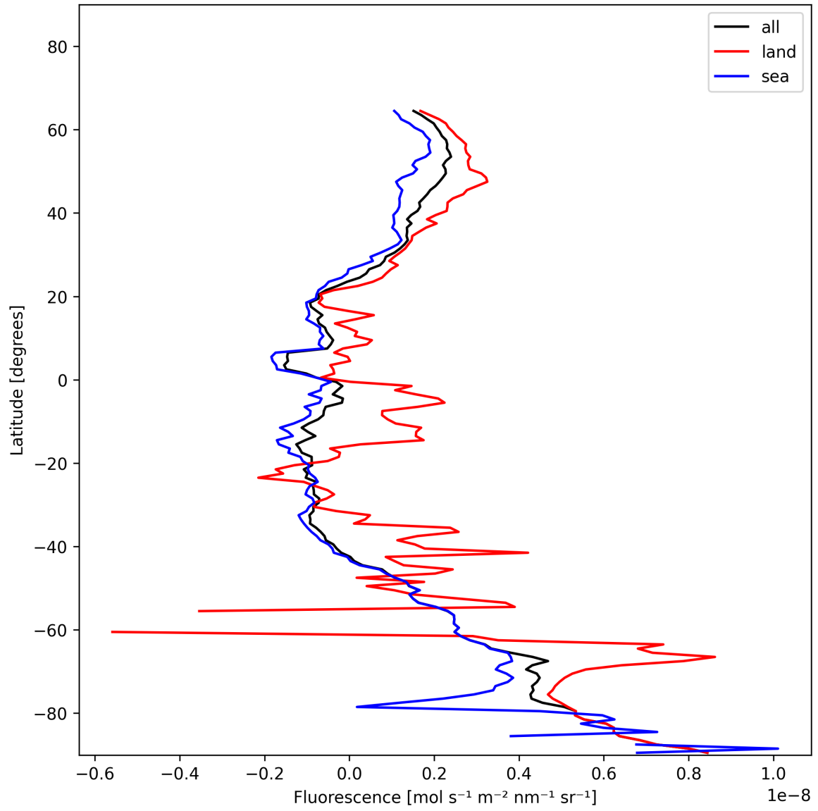
Figure 23: Zonal average of “Fluorescence” for 2024-12-28 to 2024-12-30.
