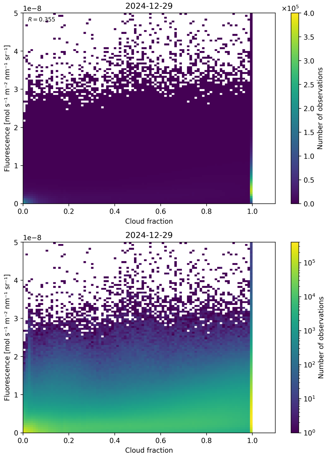
Figure 72: Scatter density plot of “Cloud fraction” against “Fluorescence” for 2024-12-28 to 2024-12-30.
