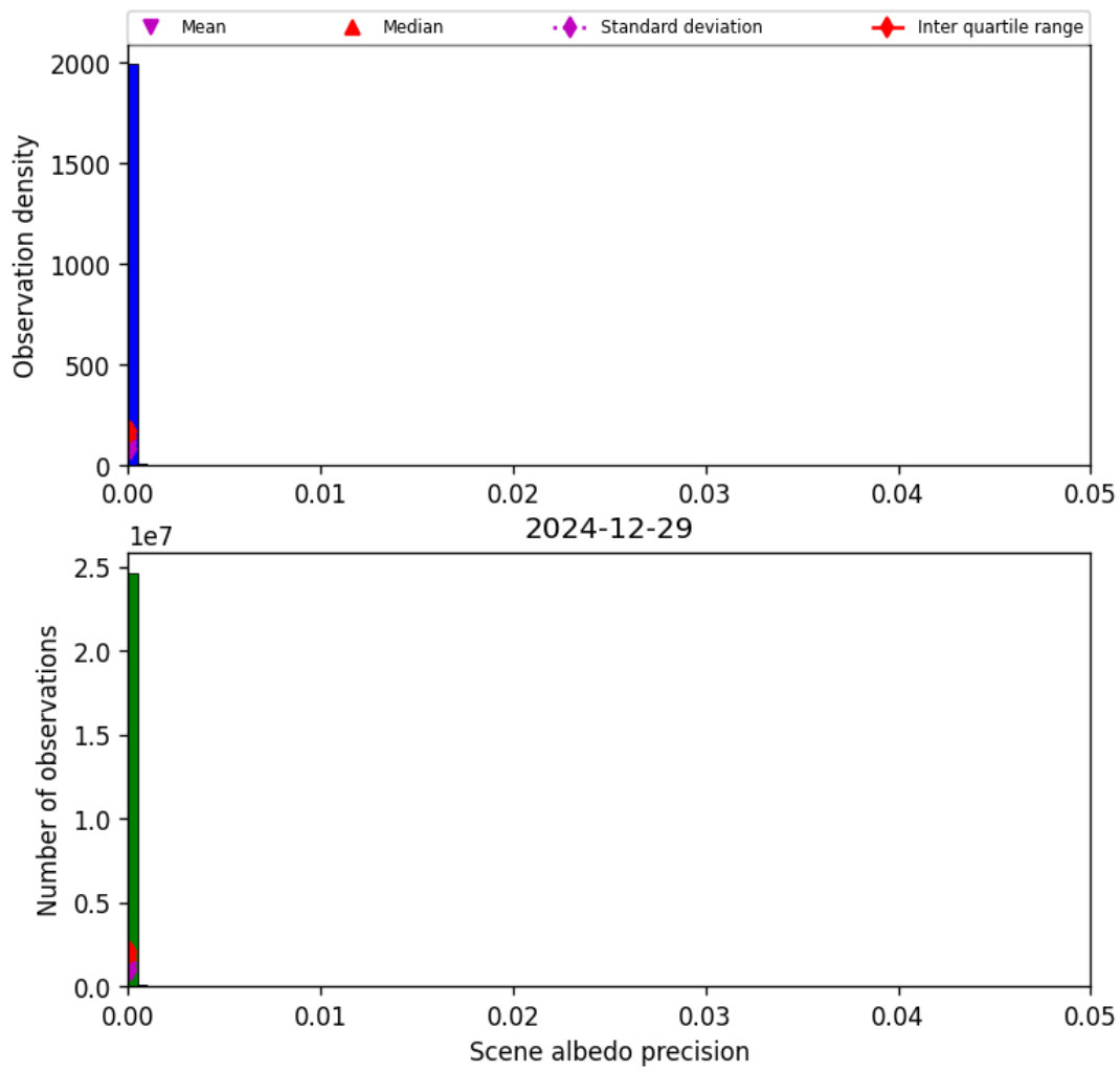
Figure 35: Histogram of “Scene albedo precision” for 2024-12-28 to 2024-12-30
