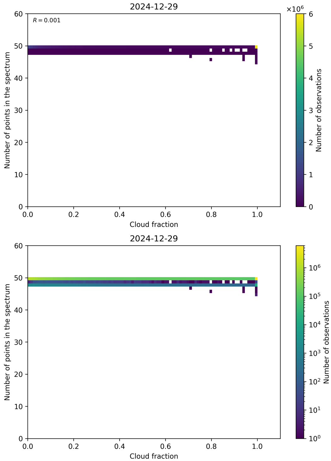
Figure 74: Scatter density plot of “Cloud fraction” against “Number of points in the spectrum” for 2024-12-28 to 2024-12-30.
