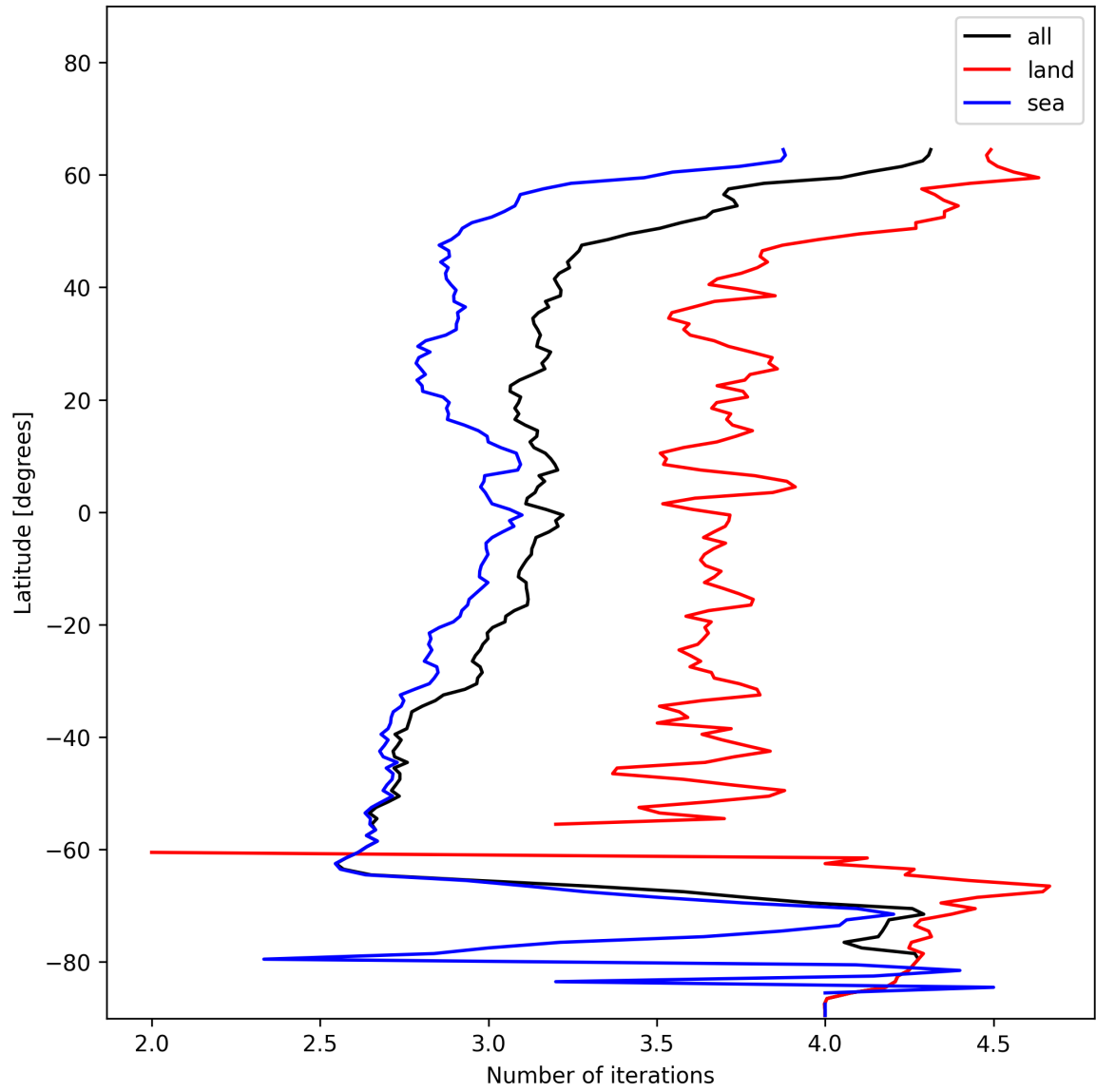
Figure 22: Zonal average of “Number of iterations” for 2024-12-28 to 2024-12-30.
