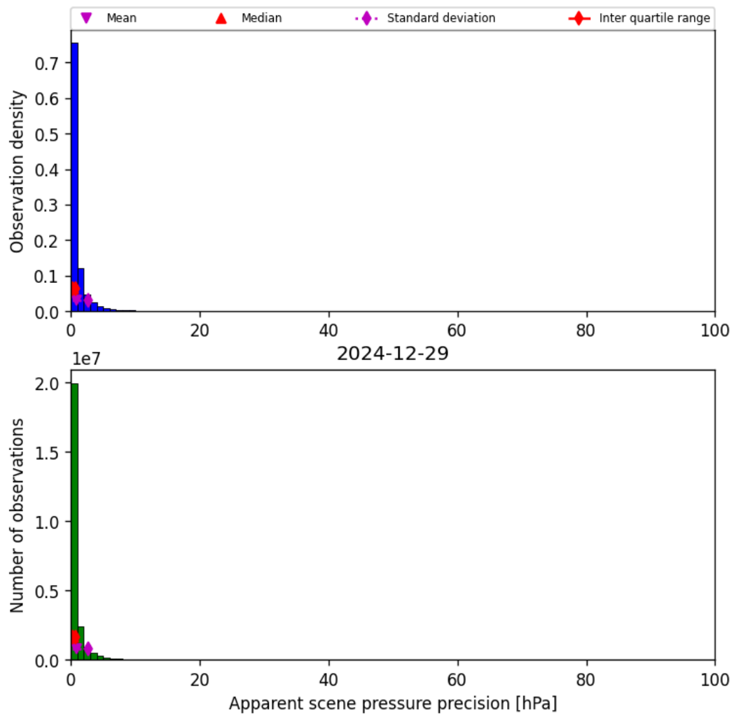
Figure 37: Histogram of “Apparent scene pressure precision” for 2024-12-28 to 2024-12-30
