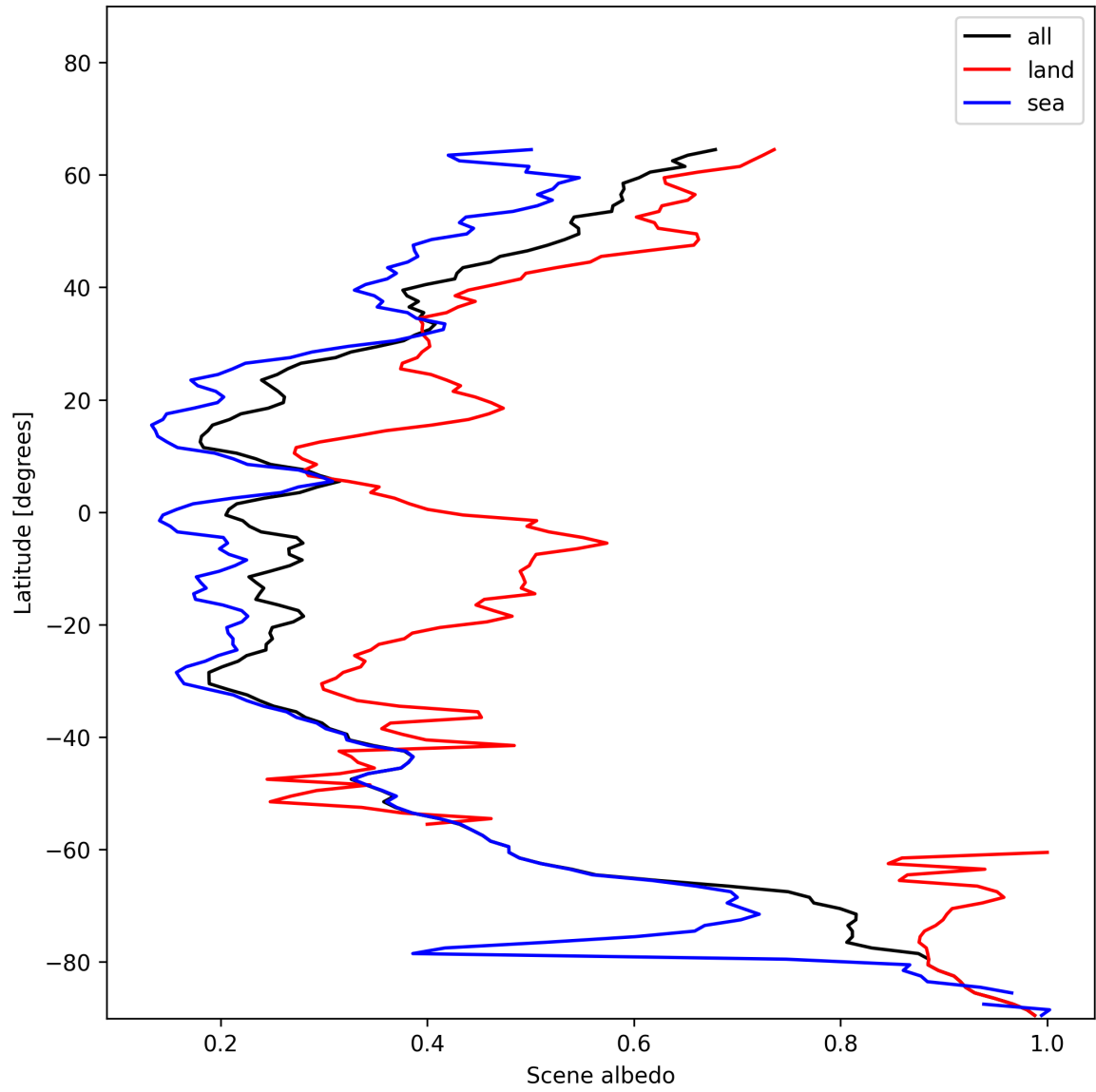
Figure 17: Zonal average of “Scene albedo” for 2024-12-28 to 2024-12-30.
