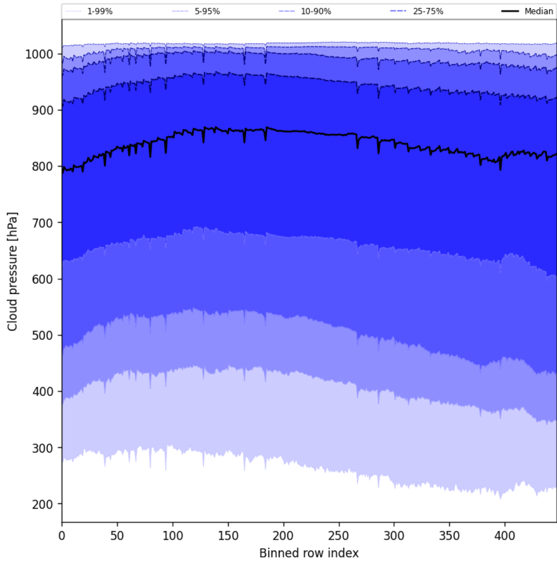
Figure 47: Along track statistics of “Cloud pressure” for 2024-12-28 to 2024-12-30
