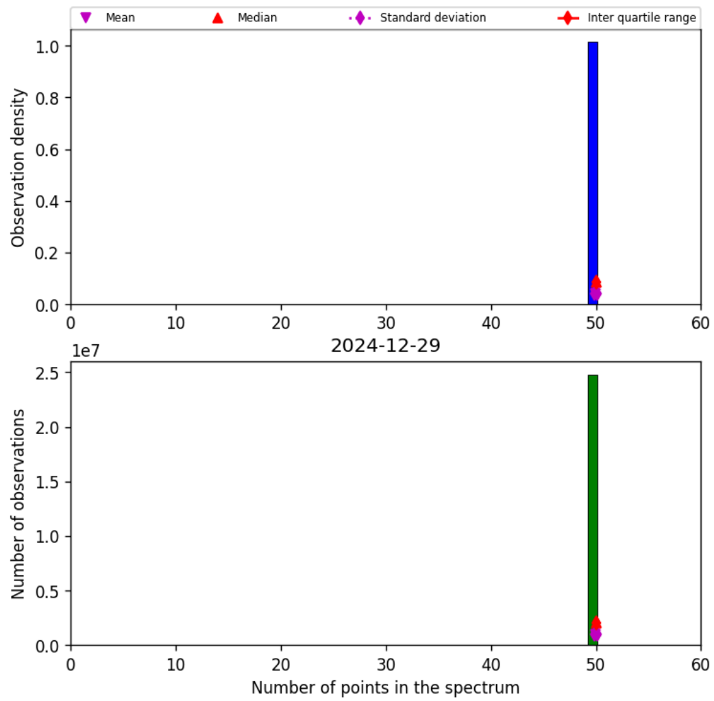
Figure 44: Histogram of “Number of points in the spectrum” for 2024-12-28 to 2024-12-30
