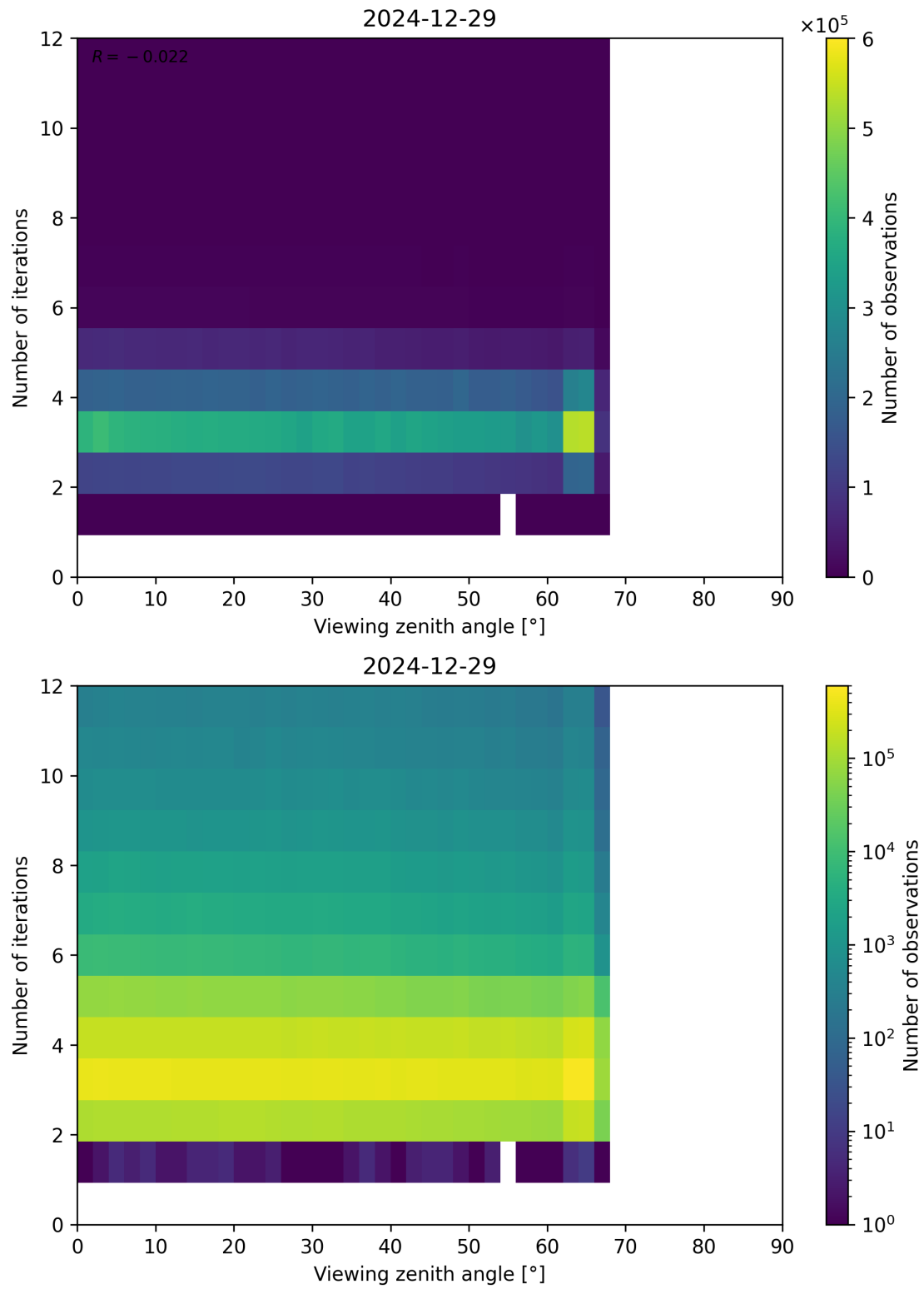
Figure 124: Scatter density plot of “Viewing zenith angle” against “Number of iterations” for 2024-12-28 to 2024-12-30.
