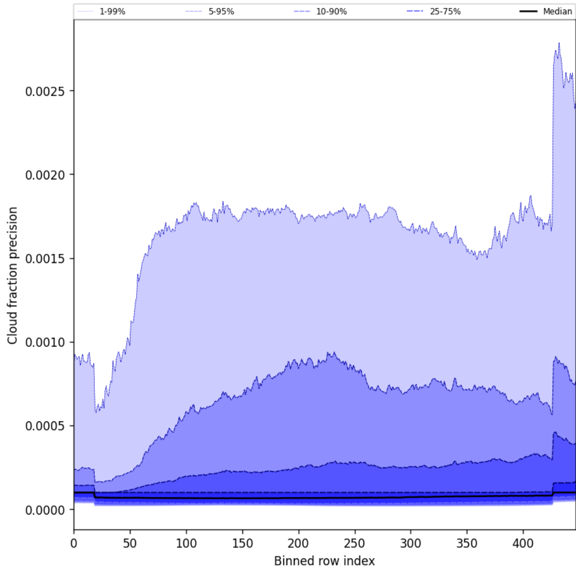
Figure 50: Along track statistics of “Cloud fraction precision” for 2024-12-28 to 2024-12-30
