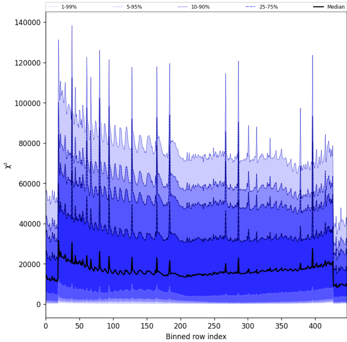
Figure 55: Along track statistics of “ \chi^2 ” for 2024-12-28 to 2024-12-30
