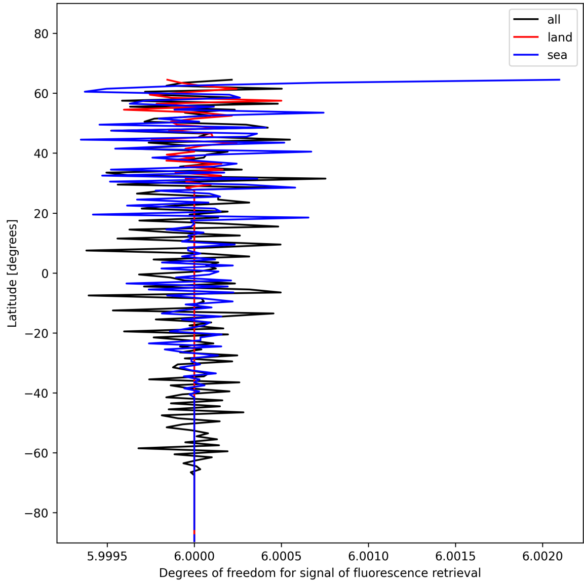
Figure 26: Zonal average of “Degrees of freedom for signal of fluorescence retrieval” for 2024-12-28 to 2024-12-30.
