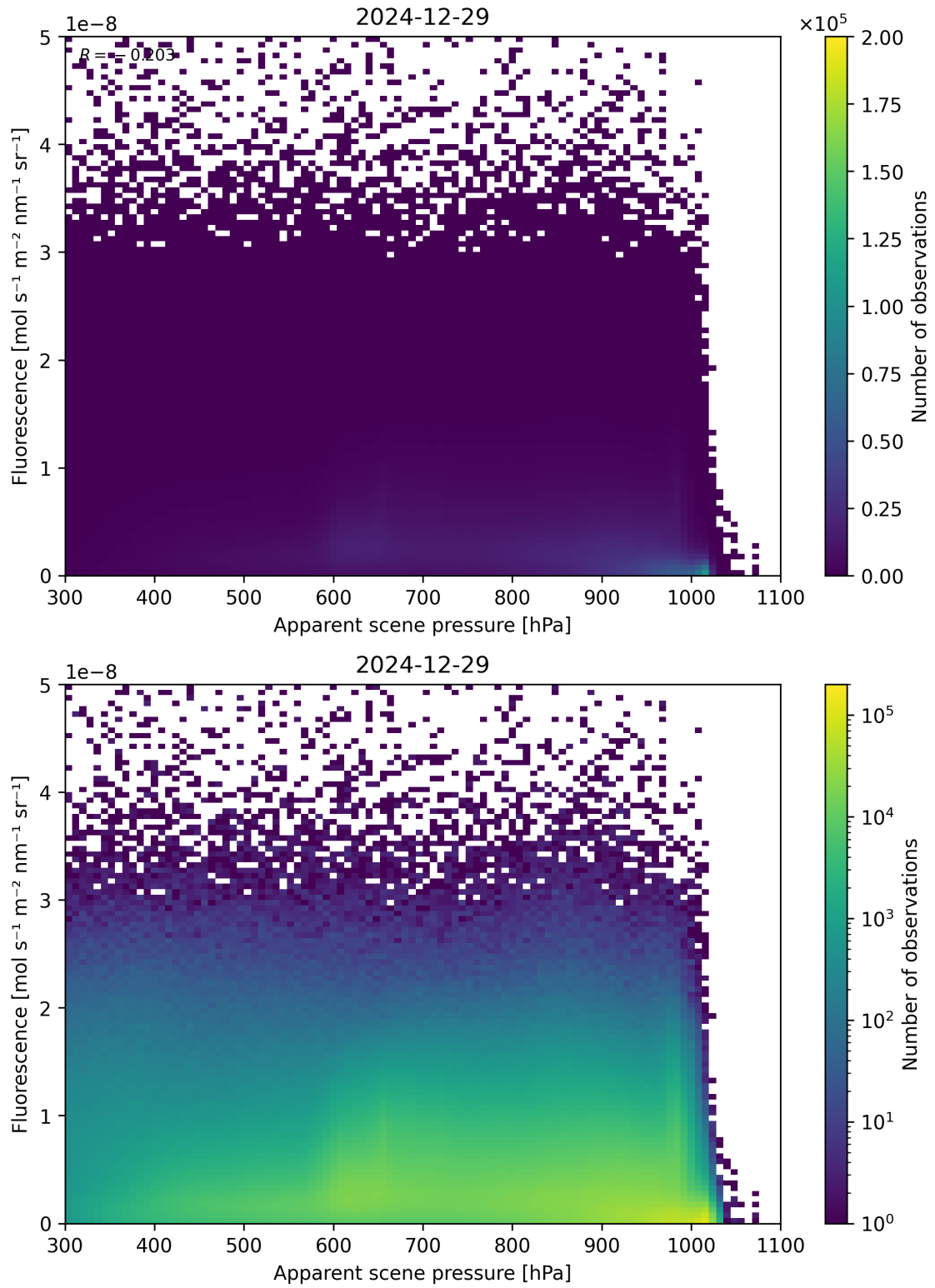
Figure 64: Scatter density plot of “Apparent scene pressure” against “Fluorescence” for 2024-12-28 to 2024-12-30.
