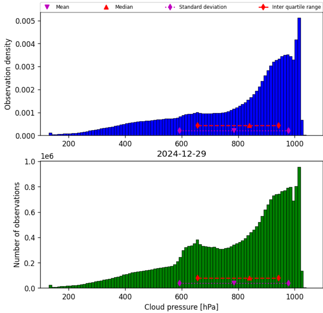
Figure 30: Histogram of “Cloud pressure” for 2024-12-28 to 2024-12-30
