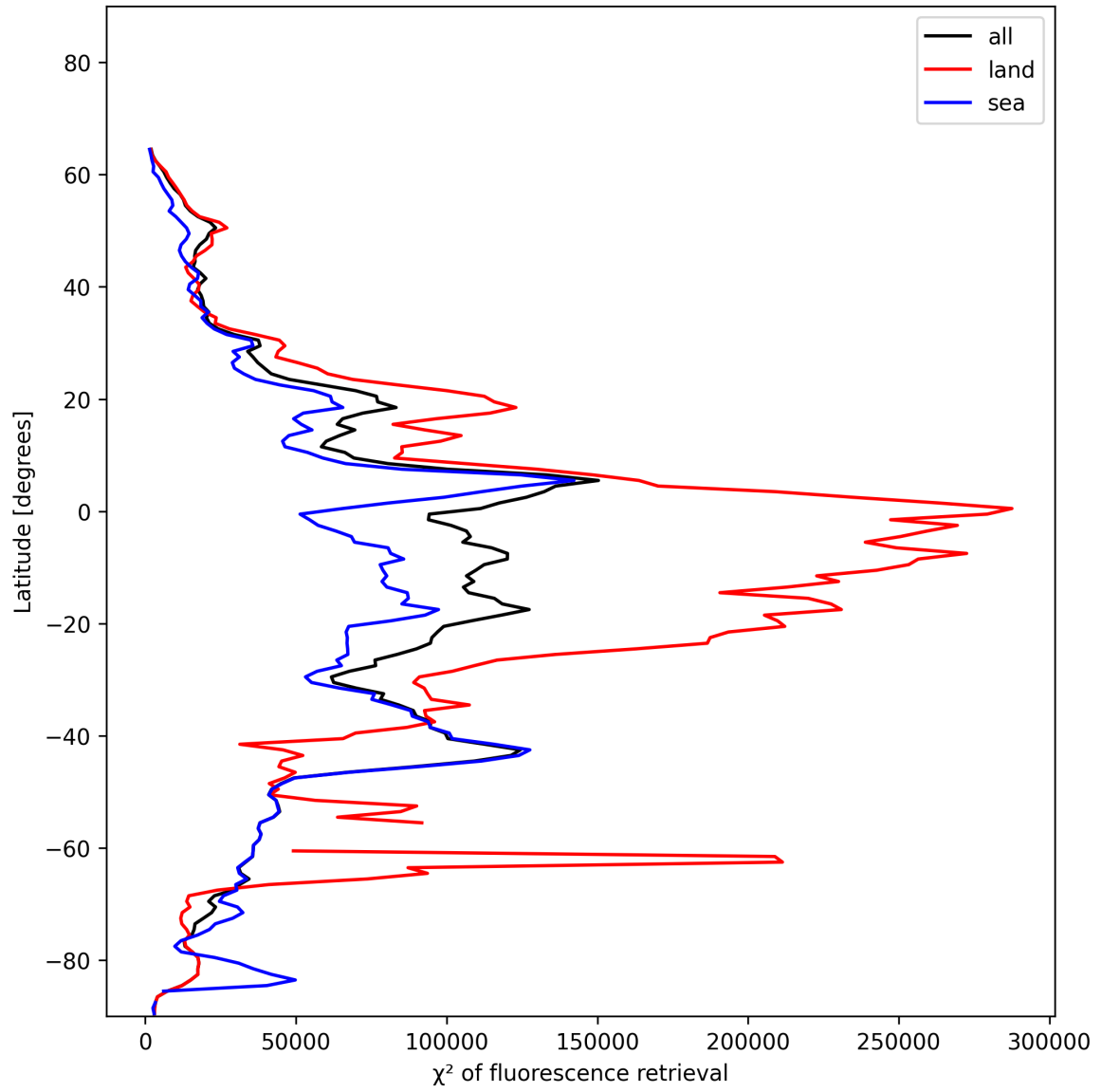
Figure 25: Zonal average of “ \chi^2 of fluorescence retrieval” for 2024-12-28 to 2024-12-30.
