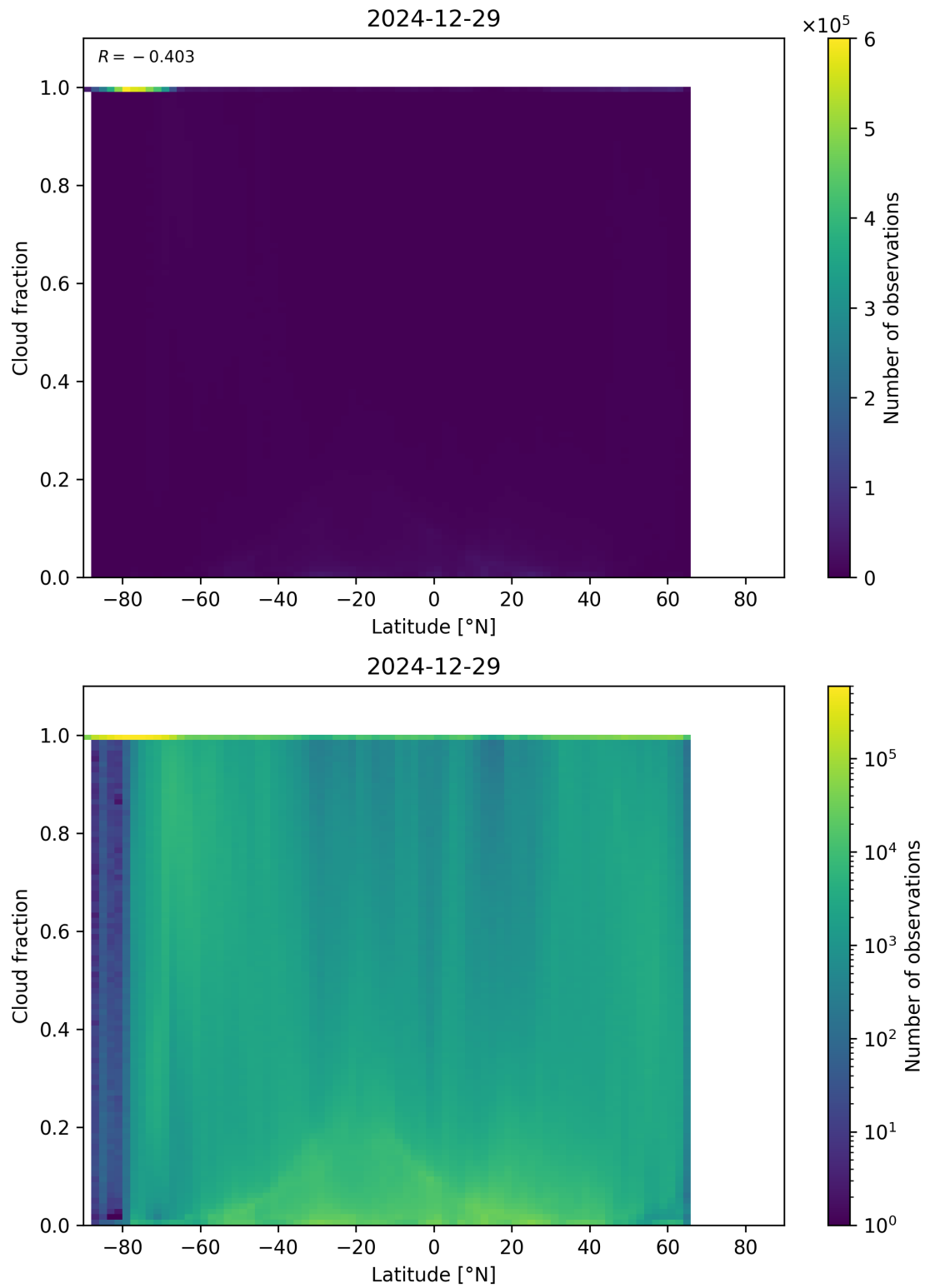
Figure 90: Scatter density plot of “Latitude” against “Cloud fraction” for 2024-12-28 to 2024-12-30.
