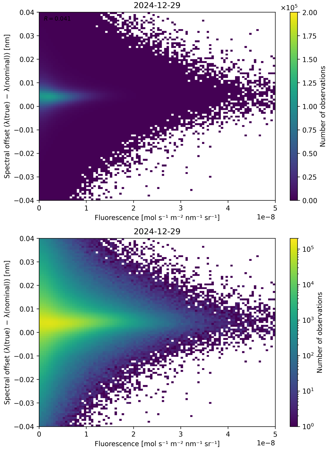
Figure 87: Scatter density plot of “Fluorescence” against “Spectral offset ( \lambda_{\text{true}} - \lambda_{\text{nominal}} )” for 2024-12-28 to 2024-12-30.
