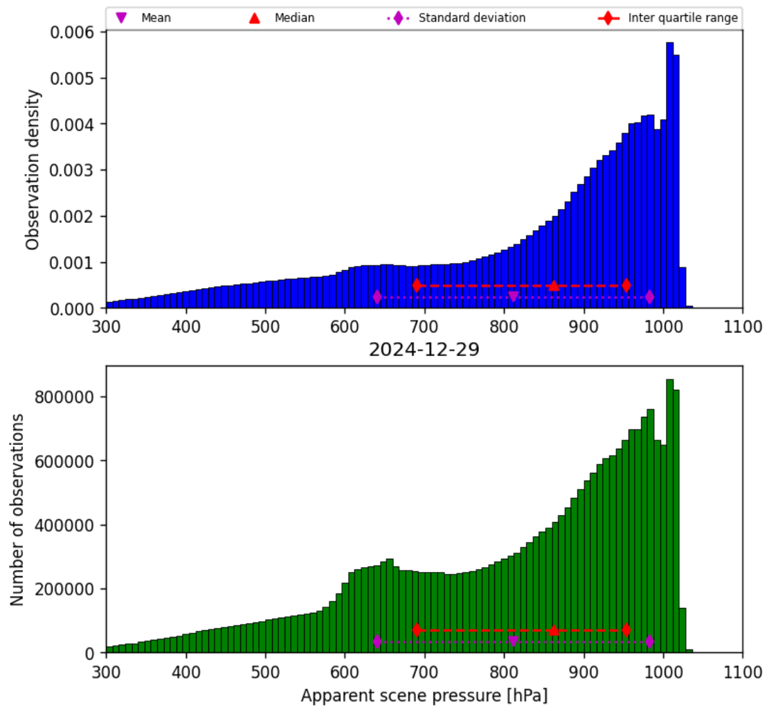
Figure 36: Histogram of “Apparent scene pressure” for 2024-12-28 to 2024-12-30
