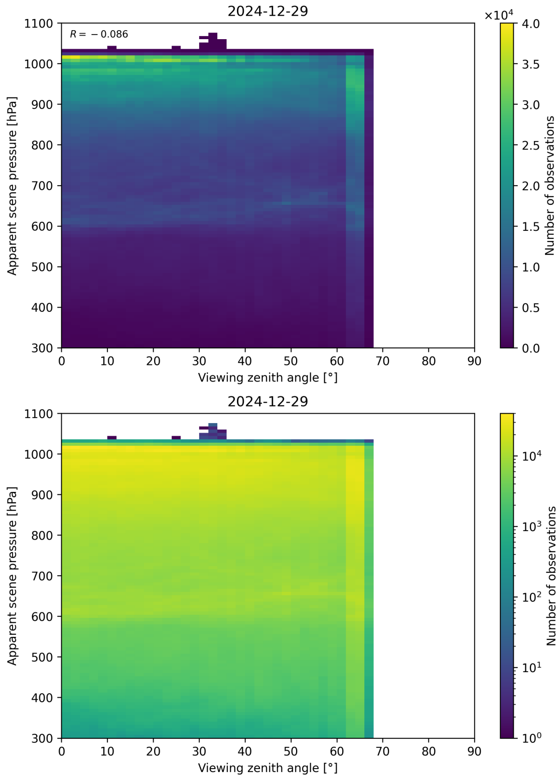
Figure 118: Scatter density plot of “Viewing zenith angle” against “Apparent scene pressure” for 2024-12-28 to 2024-12-30.
