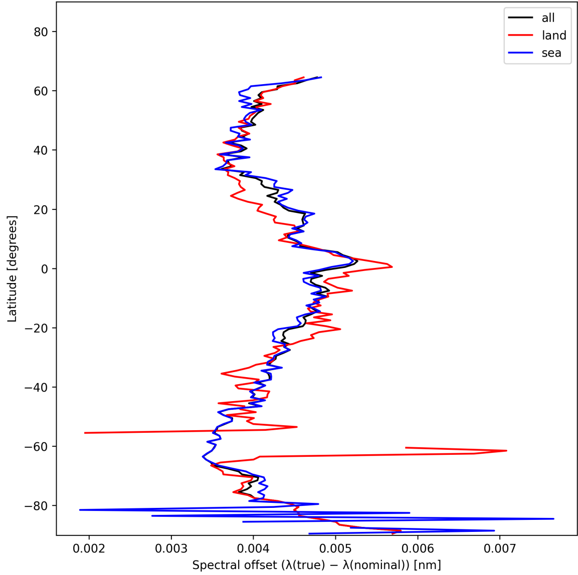
Figure 28: Zonal average of “Spectral offset ( \lambda_{\text{true}} - \lambda_{\text{nominal}} )” for 2024-12-28 to 2024-12-30.
