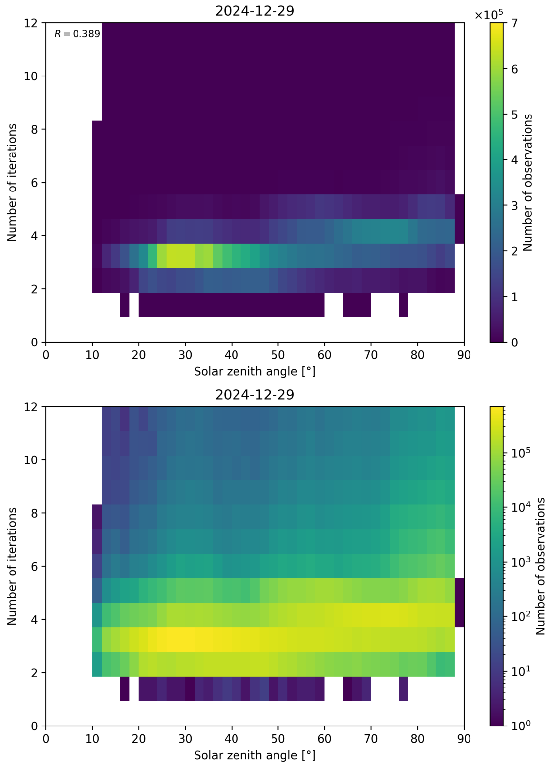
Figure 114: Scatter density plot of “Solar zenith angle” against “Number of iterations” for 2024-12-28 to 2024-12-30.
