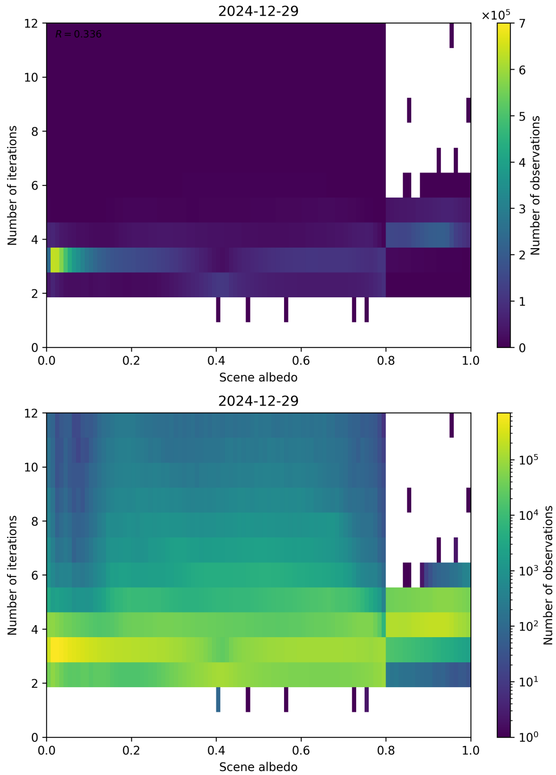
Figure 105: Scatter density plot of “Scene albedo” against “Number of iterations” for 2024-12-28 to 2024-12-30.
