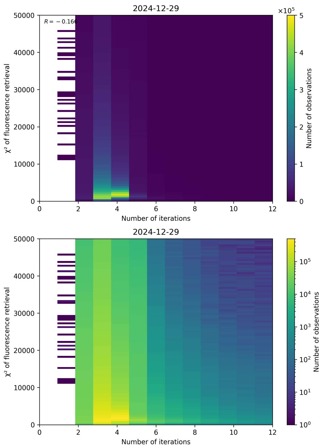
Figure 97: Scatter density plot of “Number of iterations” against “ \chi^2 of fluorescence retrieval” for 2024-12-28 to 2024-12-30.
