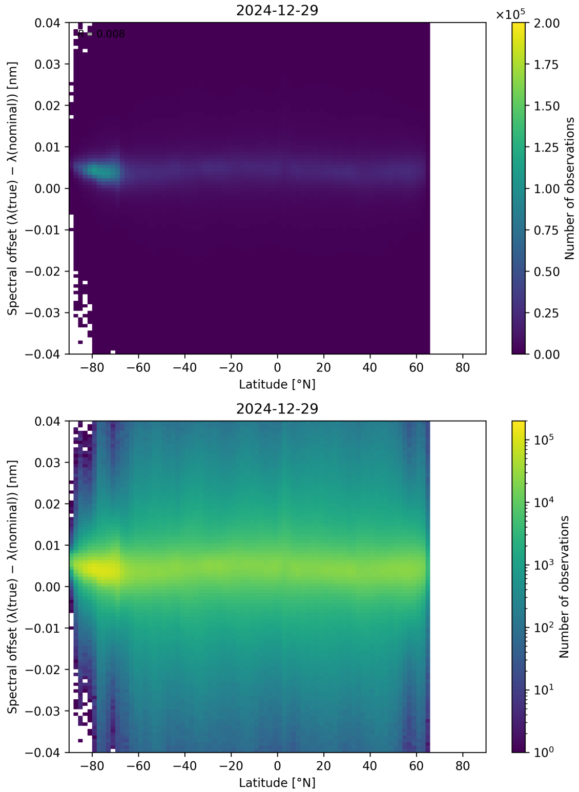
Figure 96: Scatter density plot of “Latitude” against “Spectral offset ( \lambda_{\text{true}} - \lambda_{\text{nominal}} )” for 2024-12-28 to 2024-12-30.
