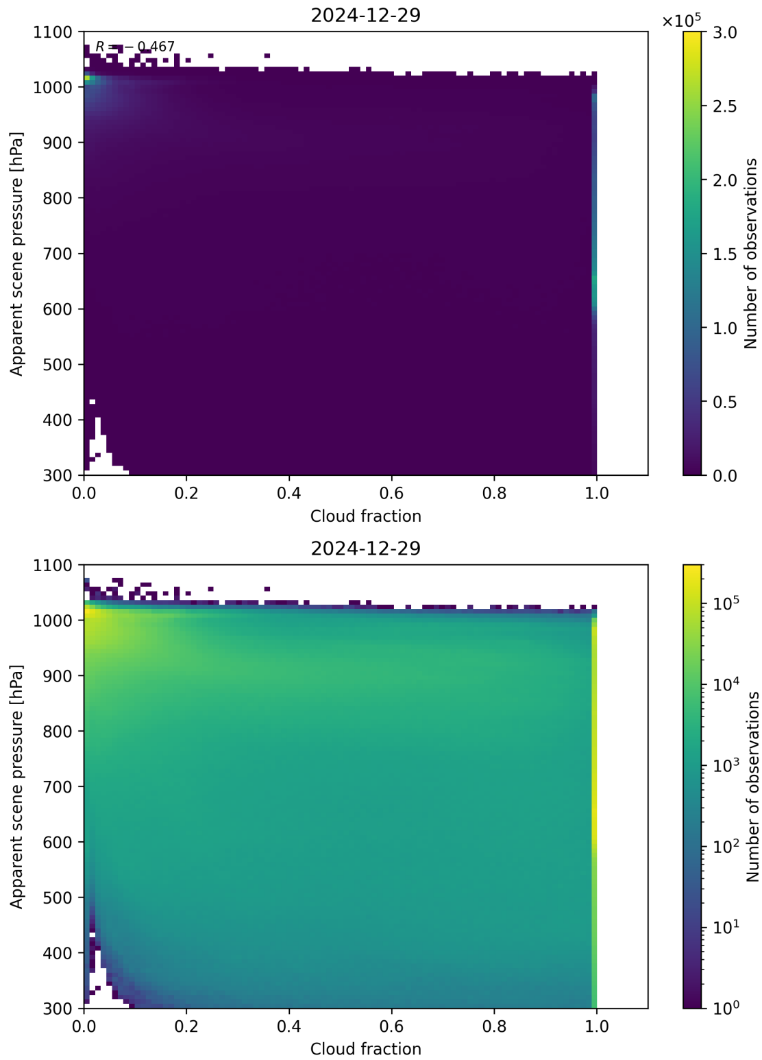
Figure 70: Scatter density plot of “Cloud fraction” against “Apparent scene pressure” for 2024-12-28 to 2024-12-30.
