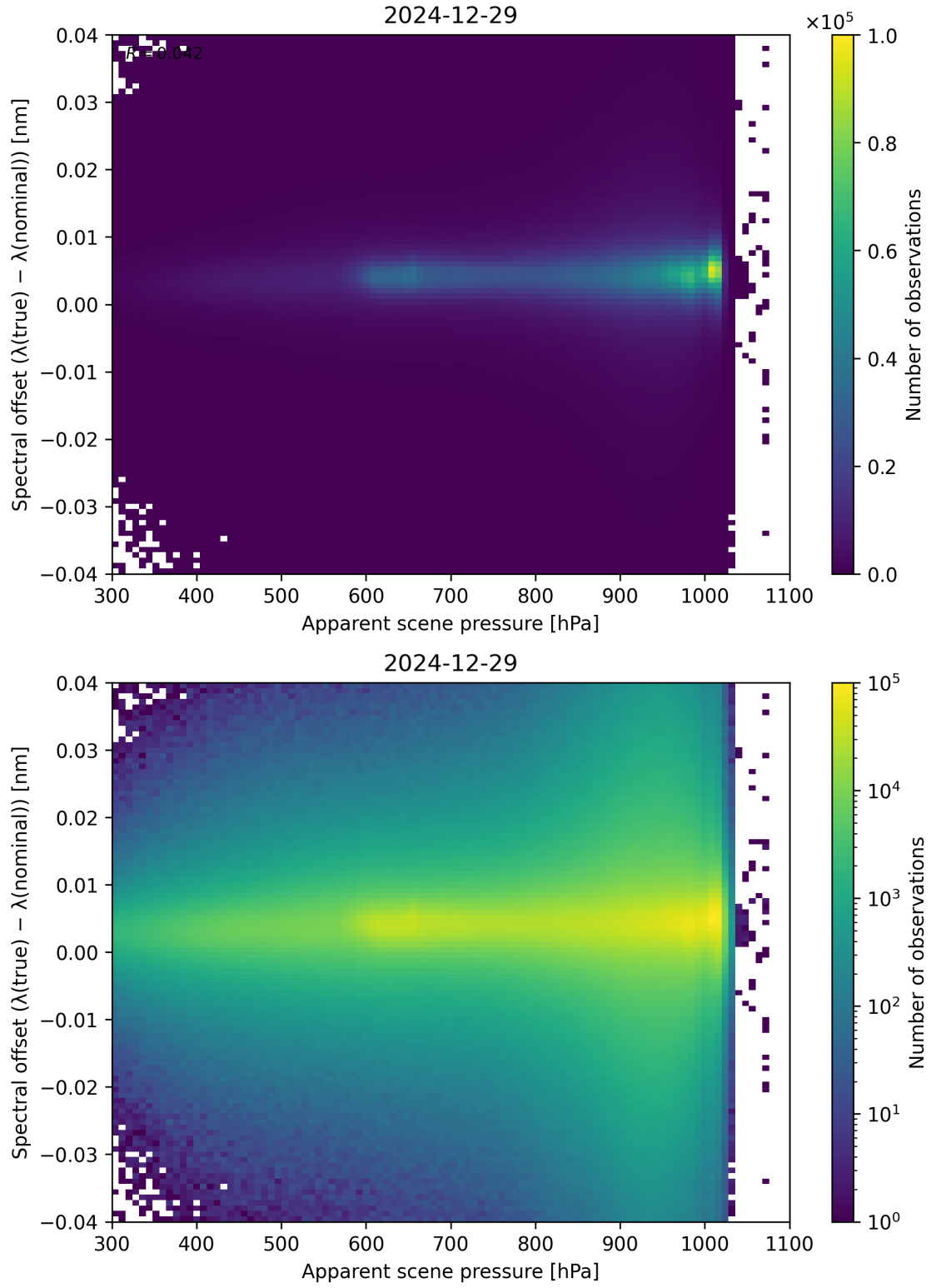
Figure 67: Scatter density plot of “Apparent scene pressure” against “Spectral offset ( \lambda_{\text{true}} - \lambda_{\text{nominal}} )” for 2024-12-28 to 2024-12-30.
