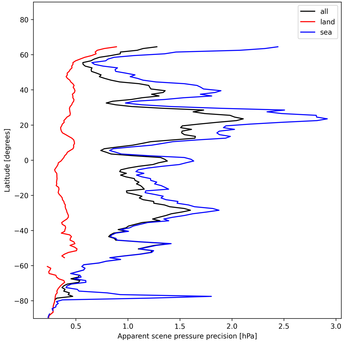
Figure 20: Zonal average of “Apparent scene pressure precision” for 2024-12-28 to 2024-12-30.
