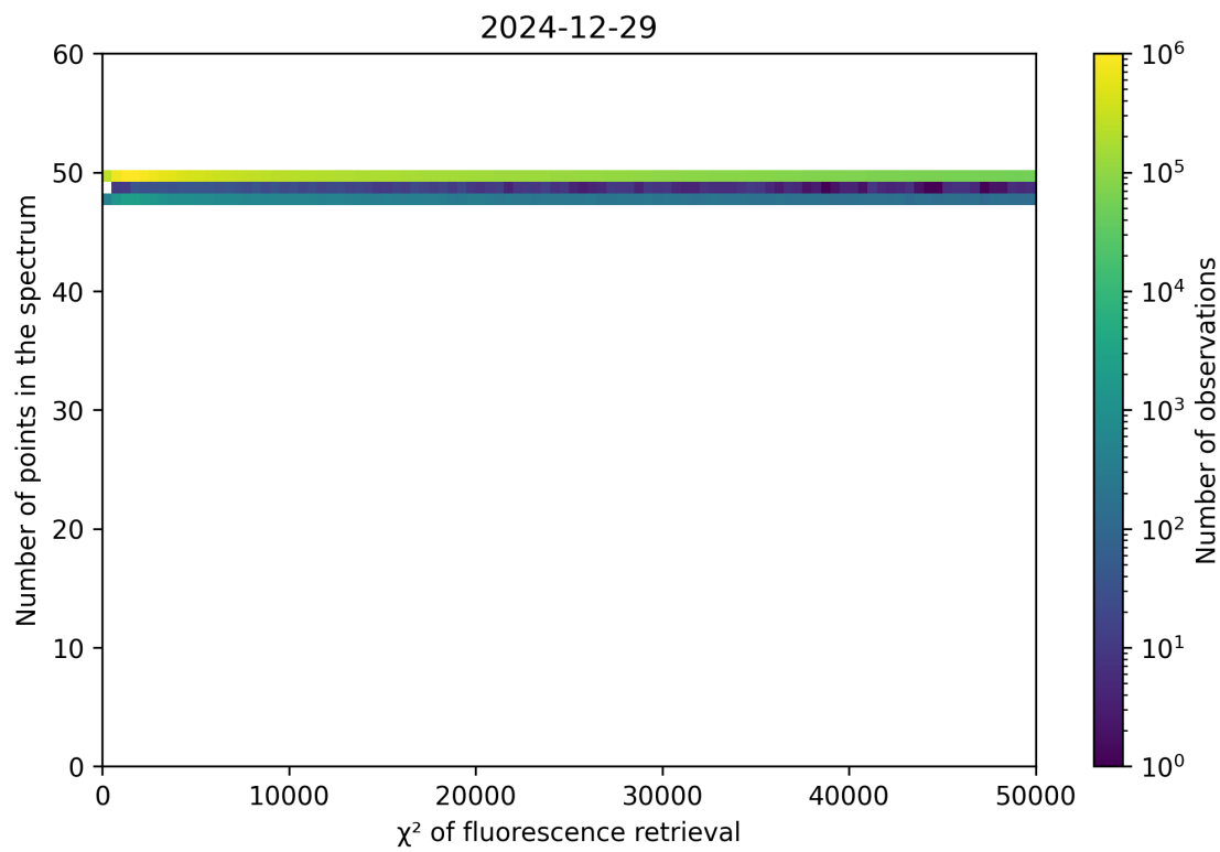
Figure 68: Scatter density plot of “ \chi^2 of fluorescence retrieval” against “Number of points in the spectrum” for 2024-12-28 to 2024-12-30.
