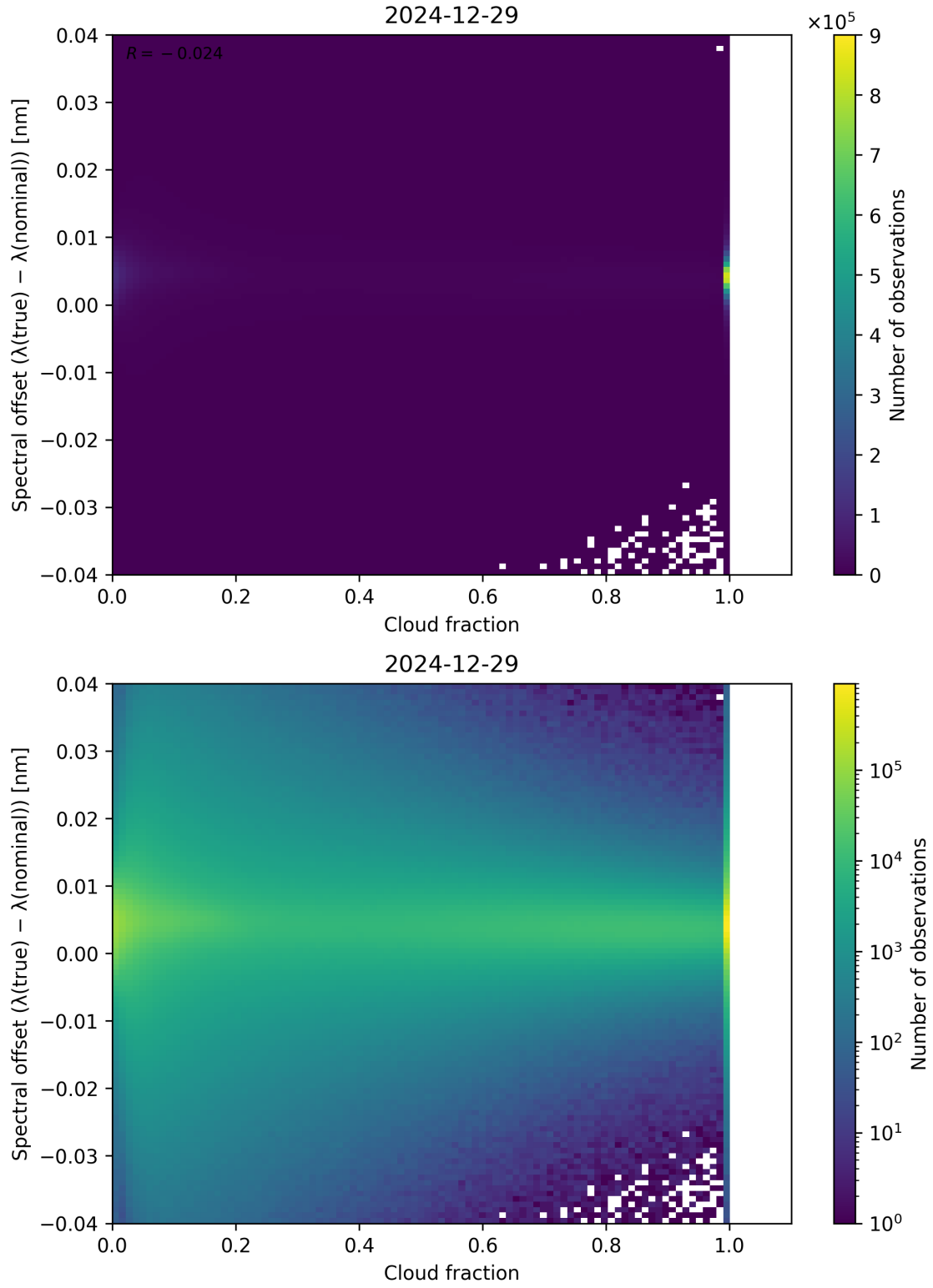
Figure 76: Scatter density plot of “Cloud fraction” against “Spectral offset ( \lambda_{\text{true}} - \lambda_{\text{nominal}} )” for 2024-12-28 to 2024-12-30.
