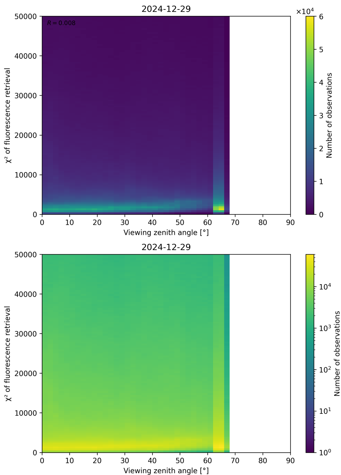
Figure 119: Scatter density plot of “Viewing zenith angle” against “ \chi^2 of fluorescence retrieval” for 2024-12-28 to 2024-12-30.
