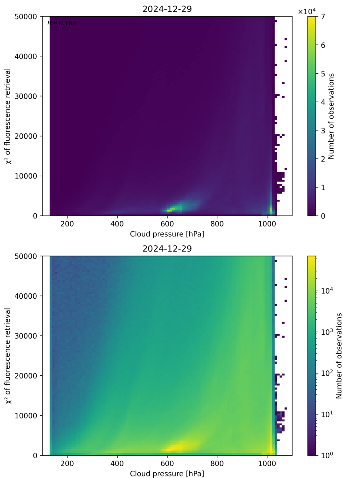
Figure 78: Scatter density plot of “Cloud pressure” against “ \chi^2 of fluorescence retrieval” for 2024-12-28 to 2024-12-30.
