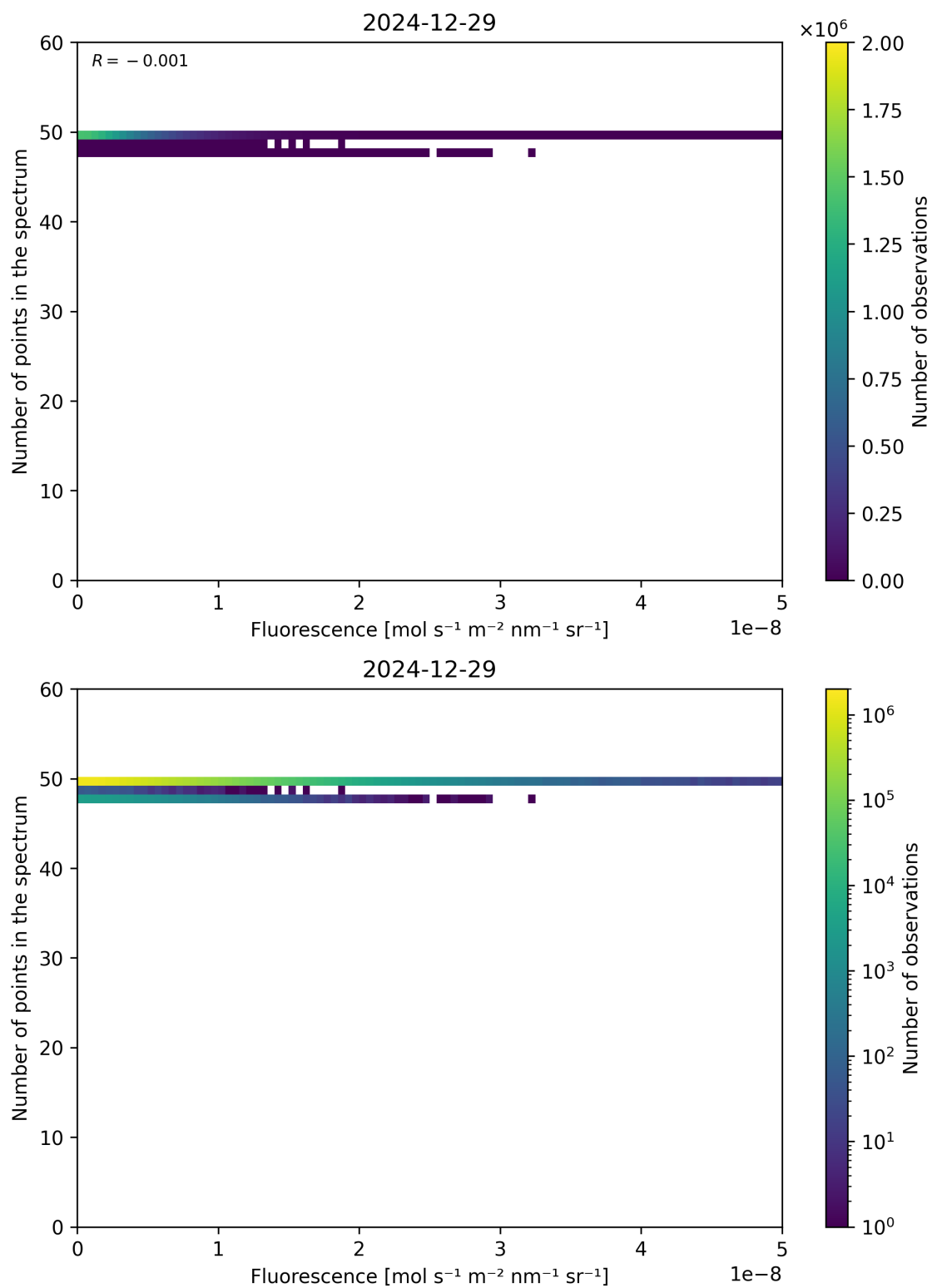
Figure 86: Scatter density plot of “Fluorescence” against “Number of points in the spectrum” for 2024-12-28 to 2024-12-30.
