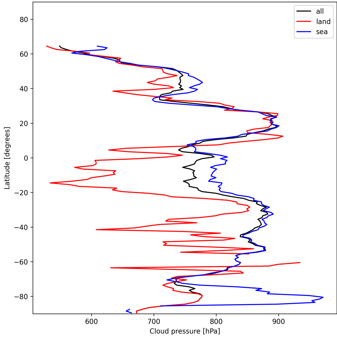
Figure 13: Zonal average of “Cloud pressure” for 2024-12-28 to 2024-12-30.
