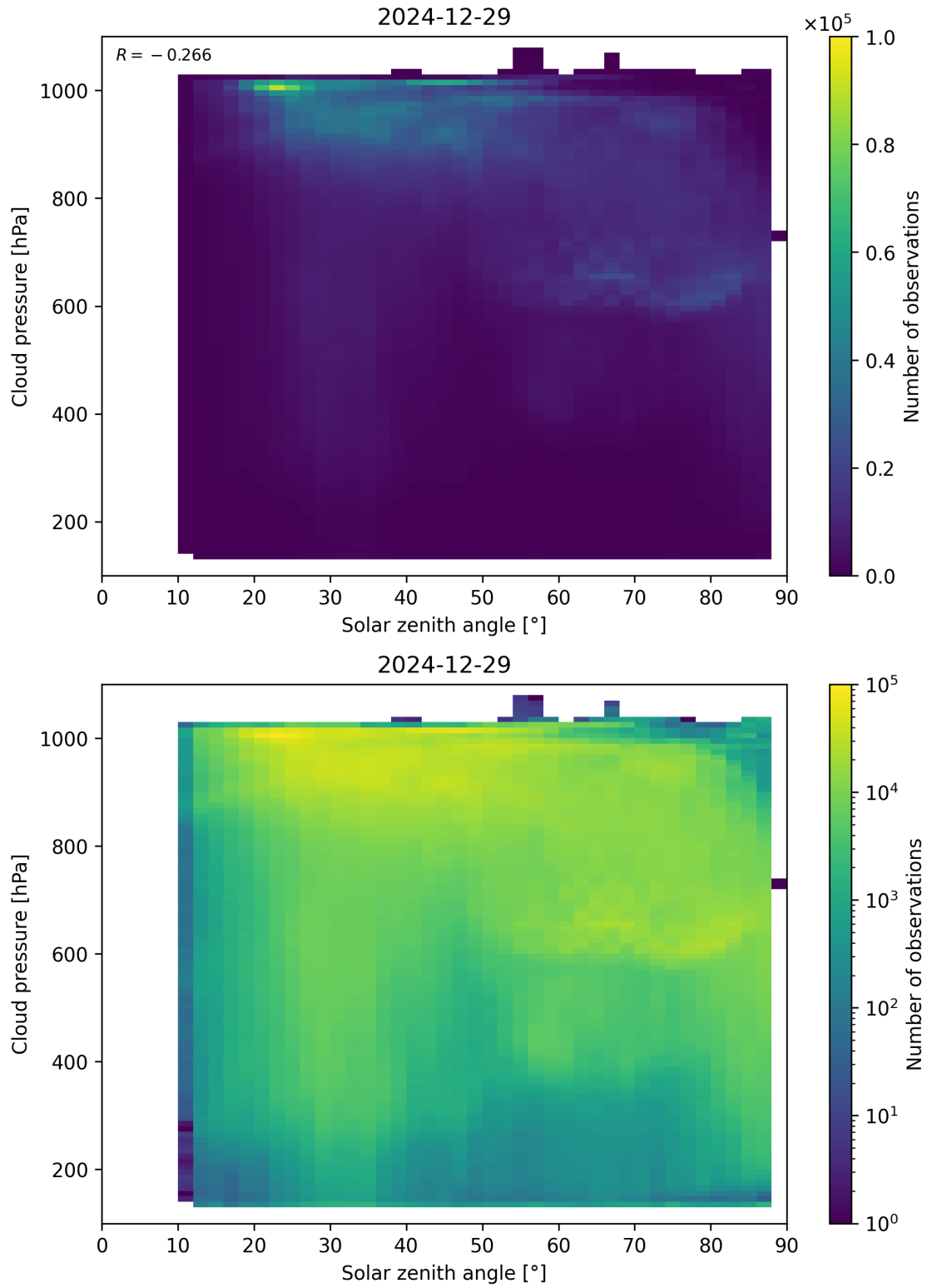
Figure 111: Scatter density plot of “Solar zenith angle” against “Cloud pressure” for 2024-12-28 to 2024-12-30.
