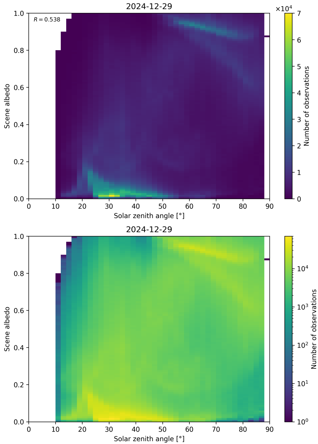
Figure 116: Scatter density plot of “Solar zenith angle” against “Scene albedo” for 2024-12-28 to 2024-12-30.
