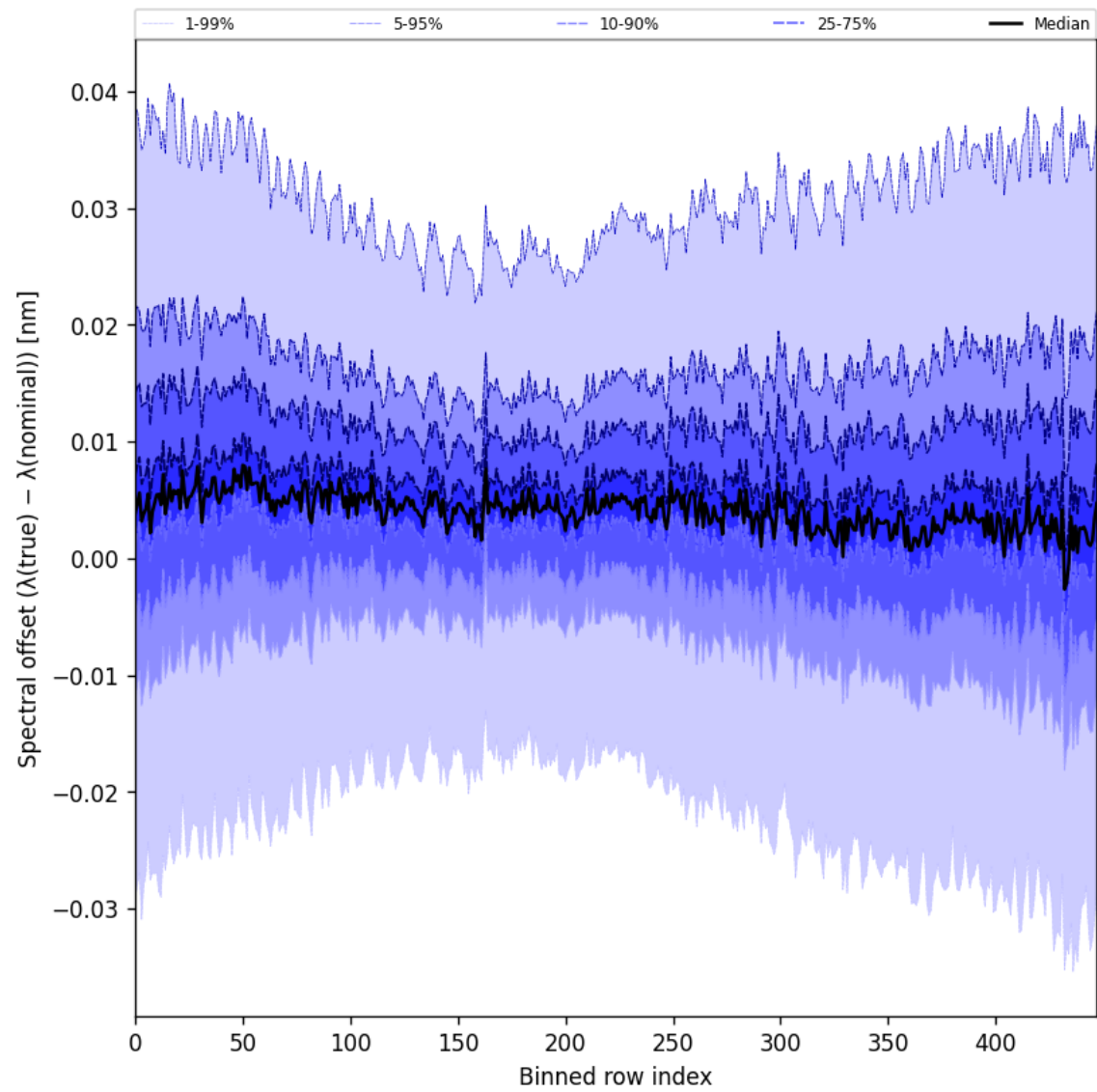
Figure 62: Along track statistics of “Spectral offset ( \lambda_{\text{true}} - \lambda_{\text{nominal}} )” for 2024-12-28 to 2024-12-30
