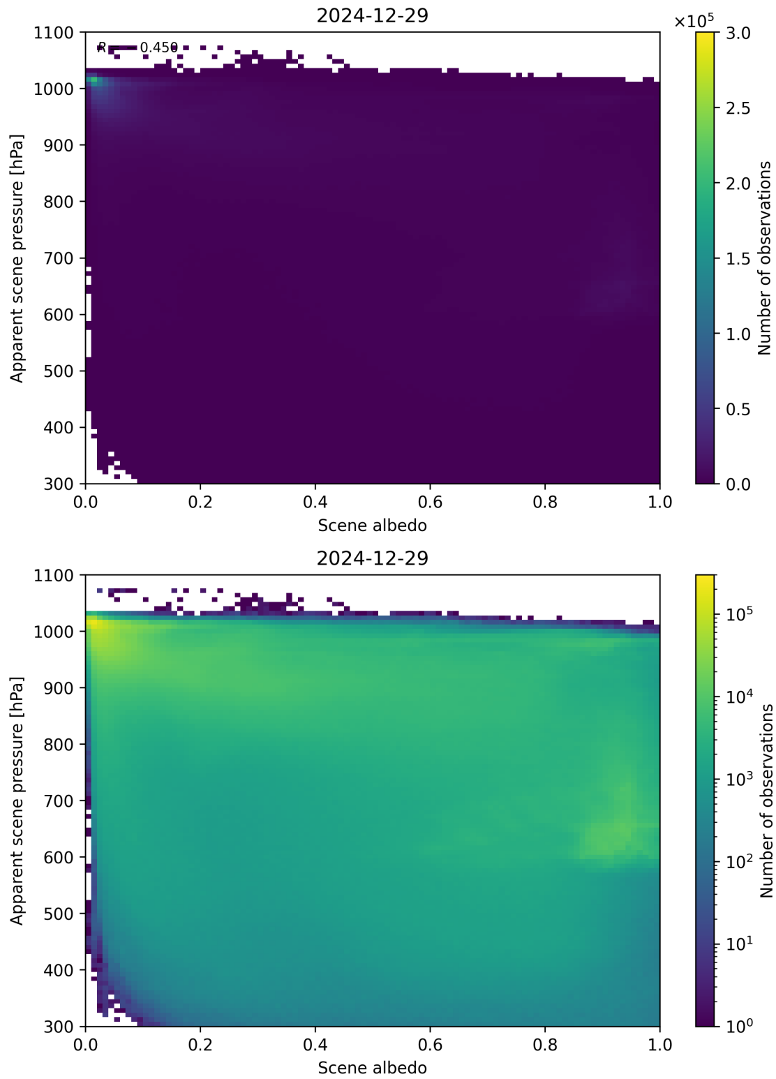
Figure 102: Scatter density plot of “Scene albedo” against “Apparent scene pressure” for 2024-12-28 to 2024-12-30.
