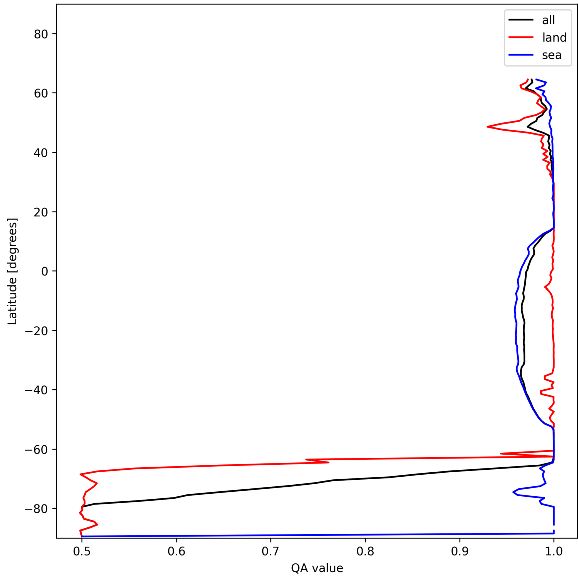
Figure 12: Zonal average of “QA value” for 2024-12-28 to 2024-12-30.
