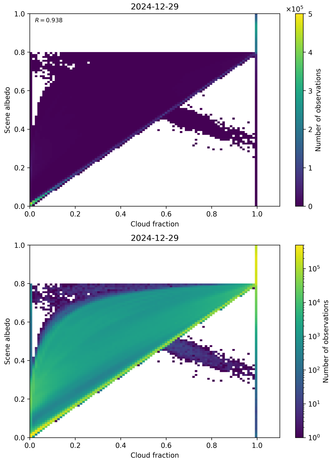
Figure 75: Scatter density plot of “Cloud fraction” against “Scene albedo” for 2024-12-28 to 2024-12-30.
