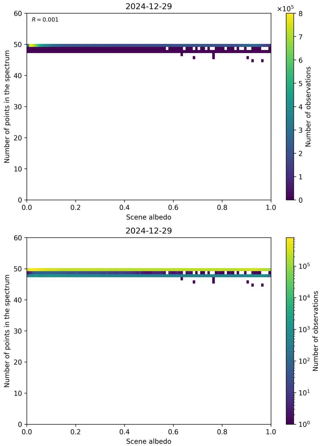
Figure 106: Scatter density plot of “Scene albedo” against “Number of points in the spectrum” for 2024-12-28 to 2024-12-30.
