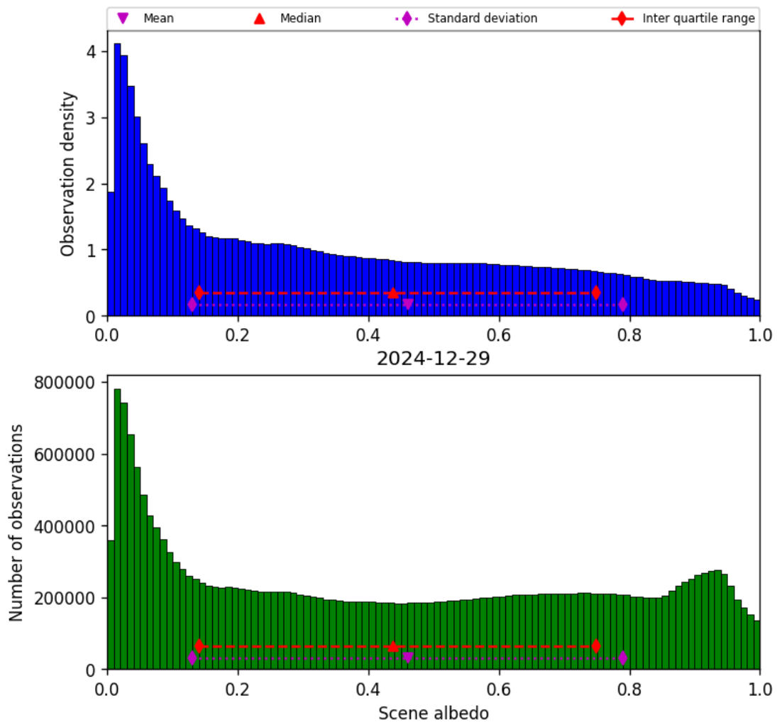
Figure 34: Histogram of “Scene albedo” for 2024-12-28 to 2024-12-30
