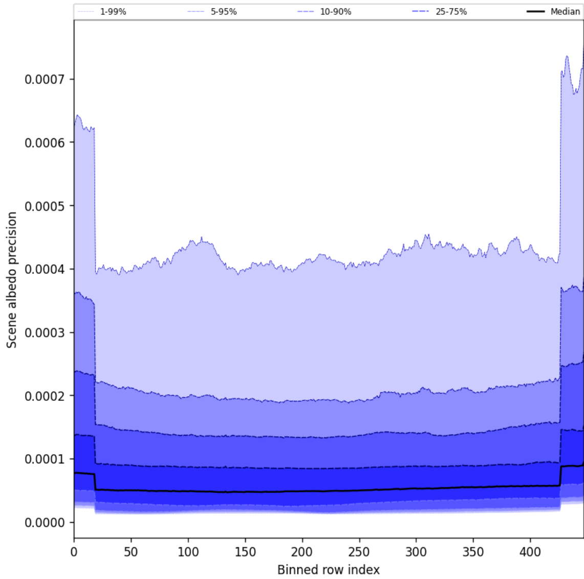
Figure 52: Along track statistics of “Scene albedo precision” for 2024-12-28 to 2024-12-30
