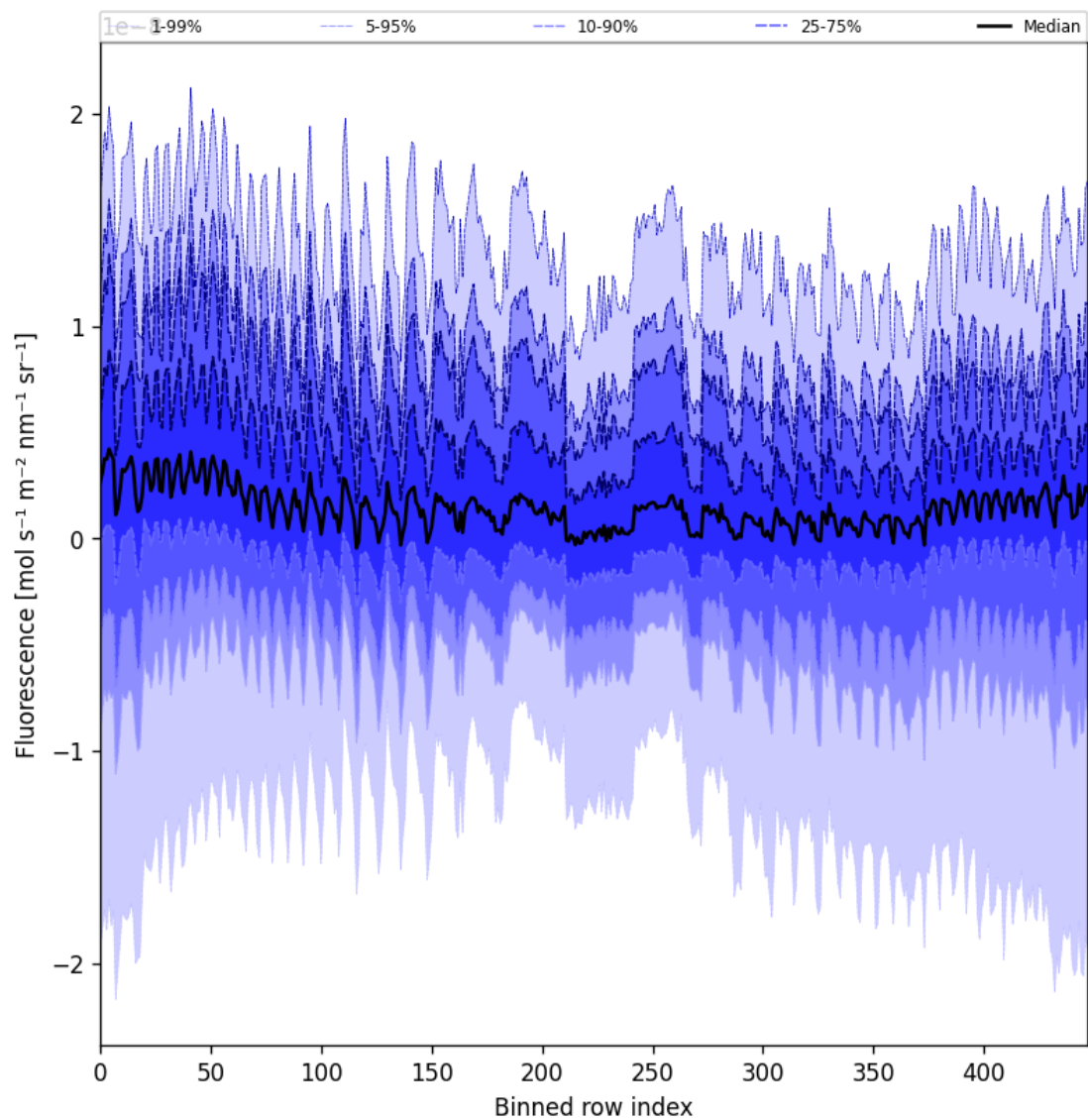
Figure 57: Along track statistics of "Fluorescence" for 2024-12-28 to 2024-12-30
