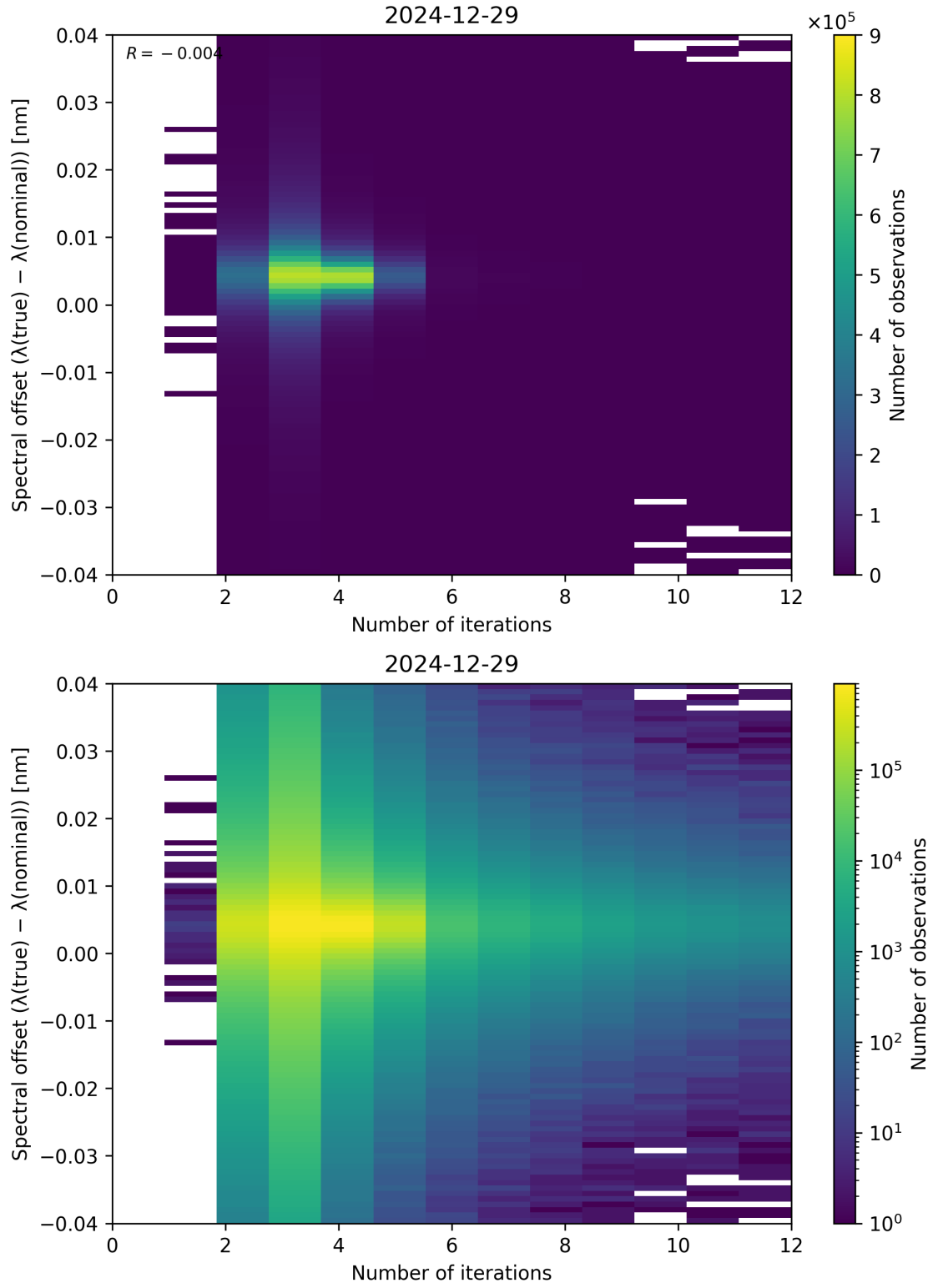
Figure 100: Scatter density plot of “Number of iterations” against “Spectral offset ( \lambda_{\text{true}} - \lambda_{\text{nominal}} )” for 2024-12-28 to 2024-12-30.
