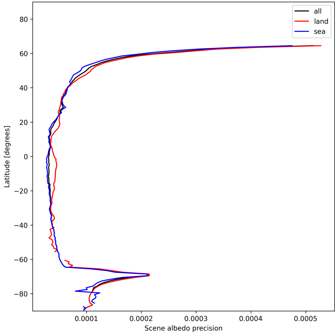
Figure 18: Zonal average of “Scene albedo precision” for 2024-12-28 to 2024-12-30.
