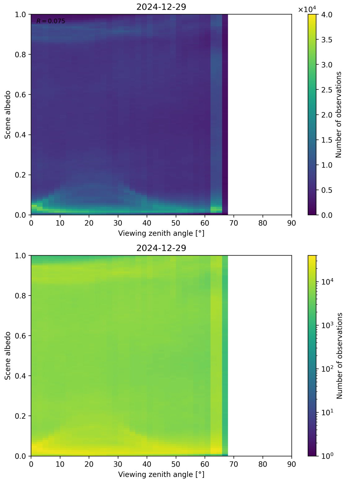
Figure 126: Scatter density plot of “Viewing zenith angle” against “Scene albedo” for 2024-12-28 to 2024-12-30.
