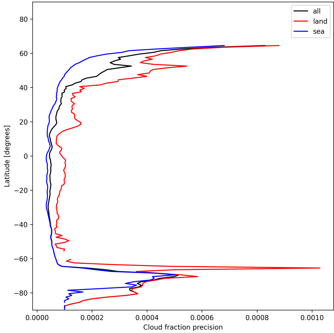
Figure 16: Zonal average of “Cloud fraction precision” for 2024-12-28 to 2024-12-30.
