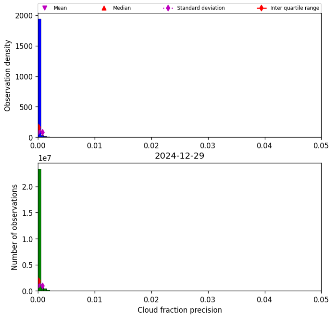
Figure 33: Histogram of “Cloud fraction precision” for 2024-12-28 to 2024-12-30
