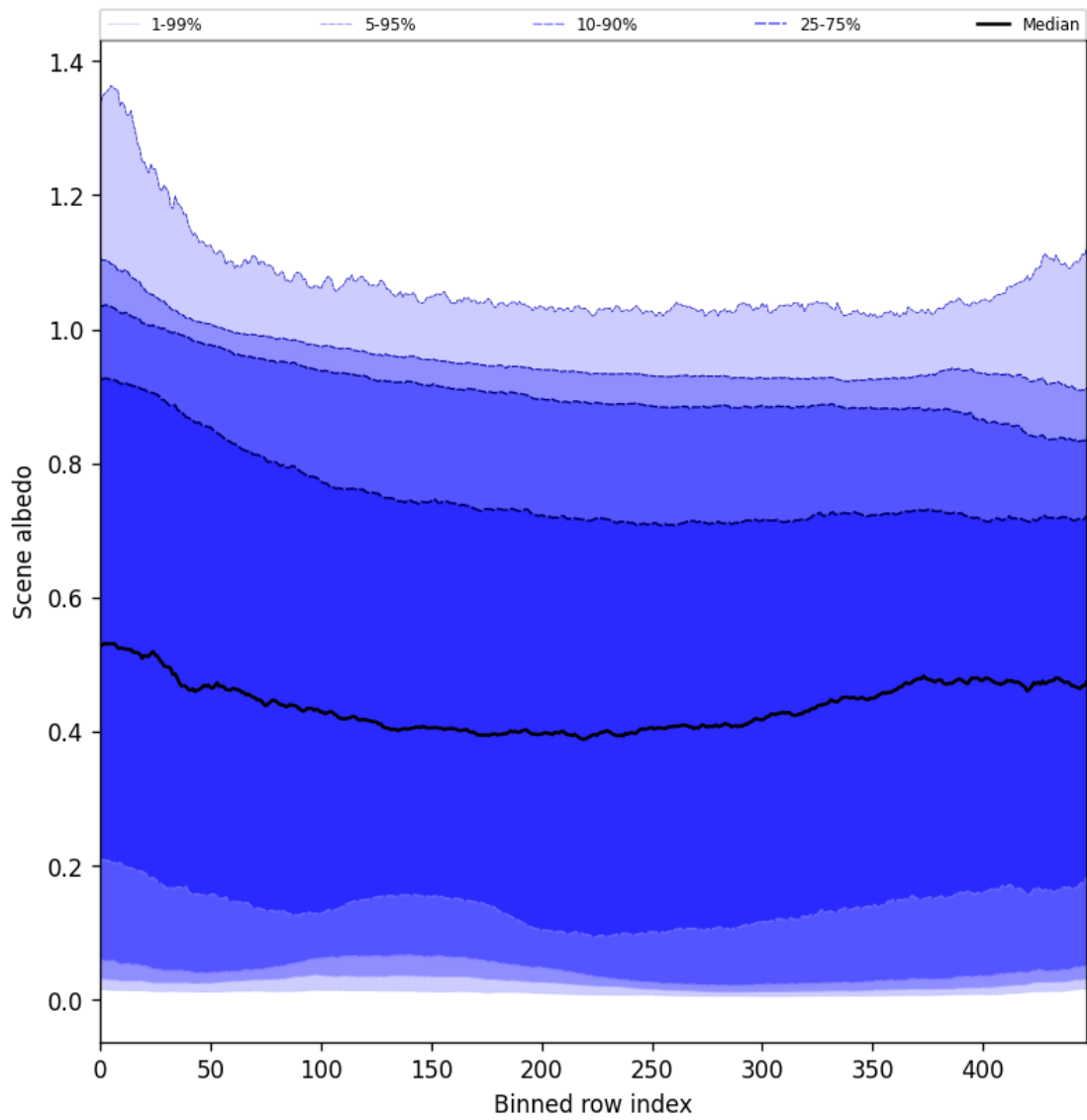
Figure 51: Along track statistics of “Scene albedo” for 2024-12-28 to 2024-12-30
