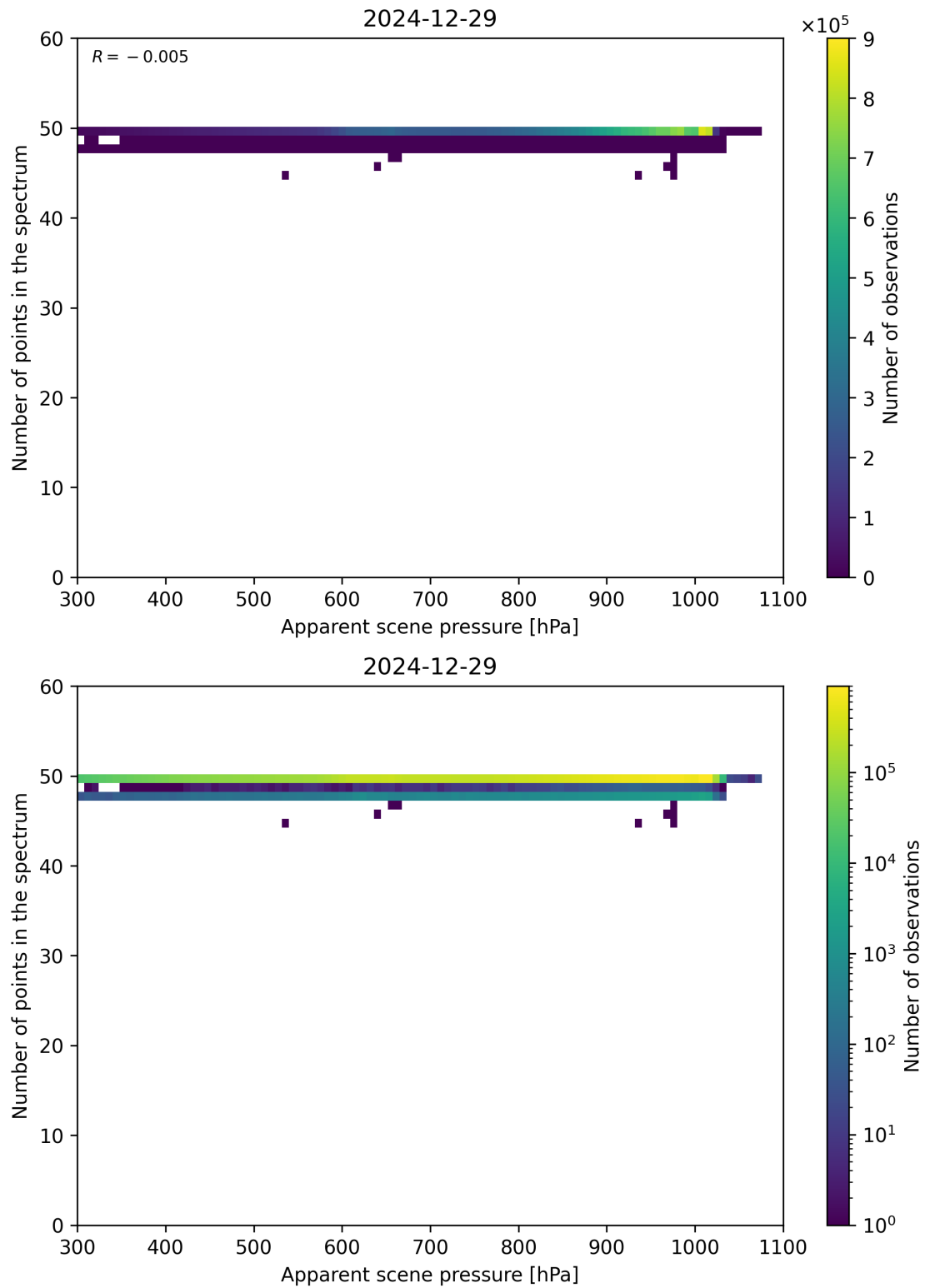
Figure 66: Scatter density plot of “Apparent scene pressure” against “Number of points in the spectrum” for 2024-12-28 to 2024-12-30.
