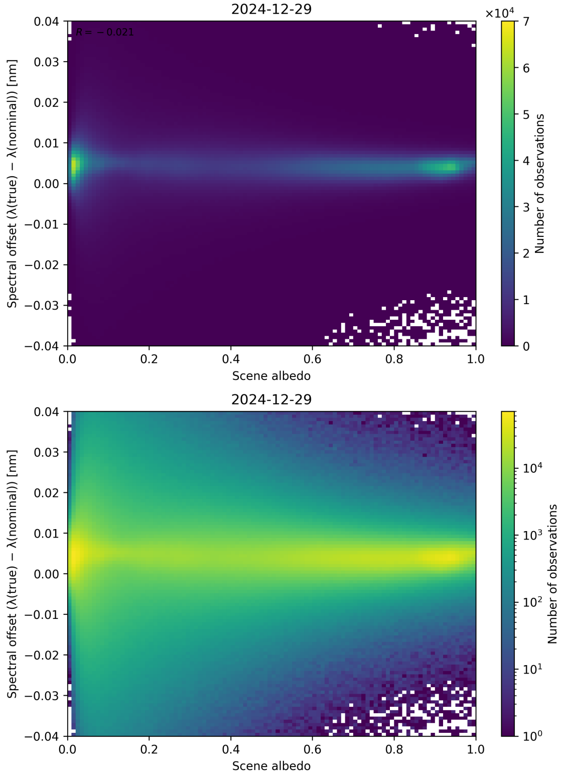
Figure 107: Scatter density plot of “Scene albedo” against “Spectral offset ( \lambda_{\text{true}} - \lambda_{\text{nominal}} )” for 2024-12-28 to 2024-12-30.
