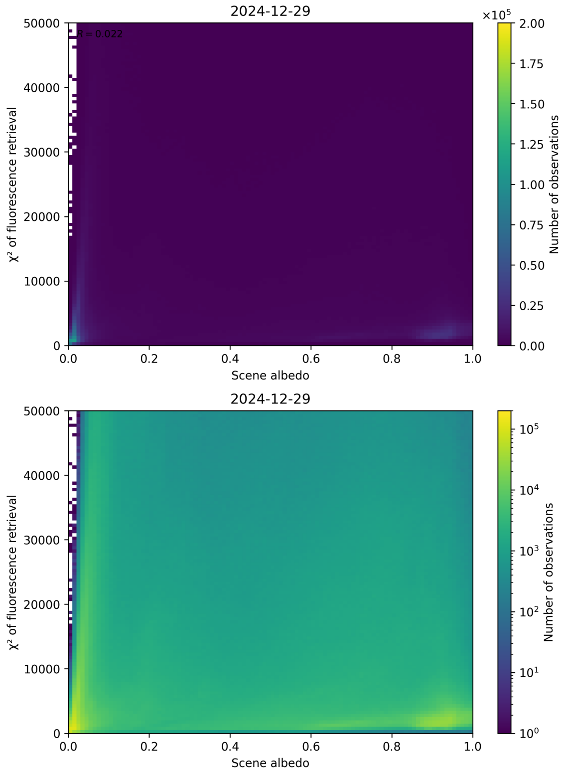
Figure 103: Scatter density plot of “Scene albedo” against “ \chi^2 of fluorescence retrieval” for 2024-12-28 to 2024-12-30.
