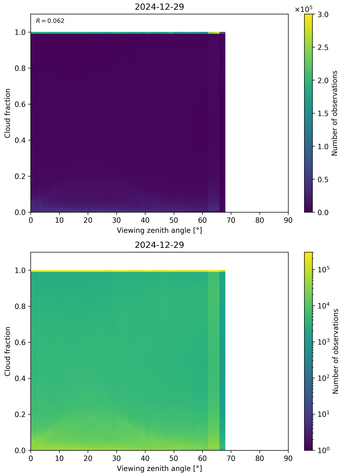
Figure 120: Scatter density plot of “Viewing zenith angle” against “Cloud fraction” for 2024-12-28 to 2024-12-30.
