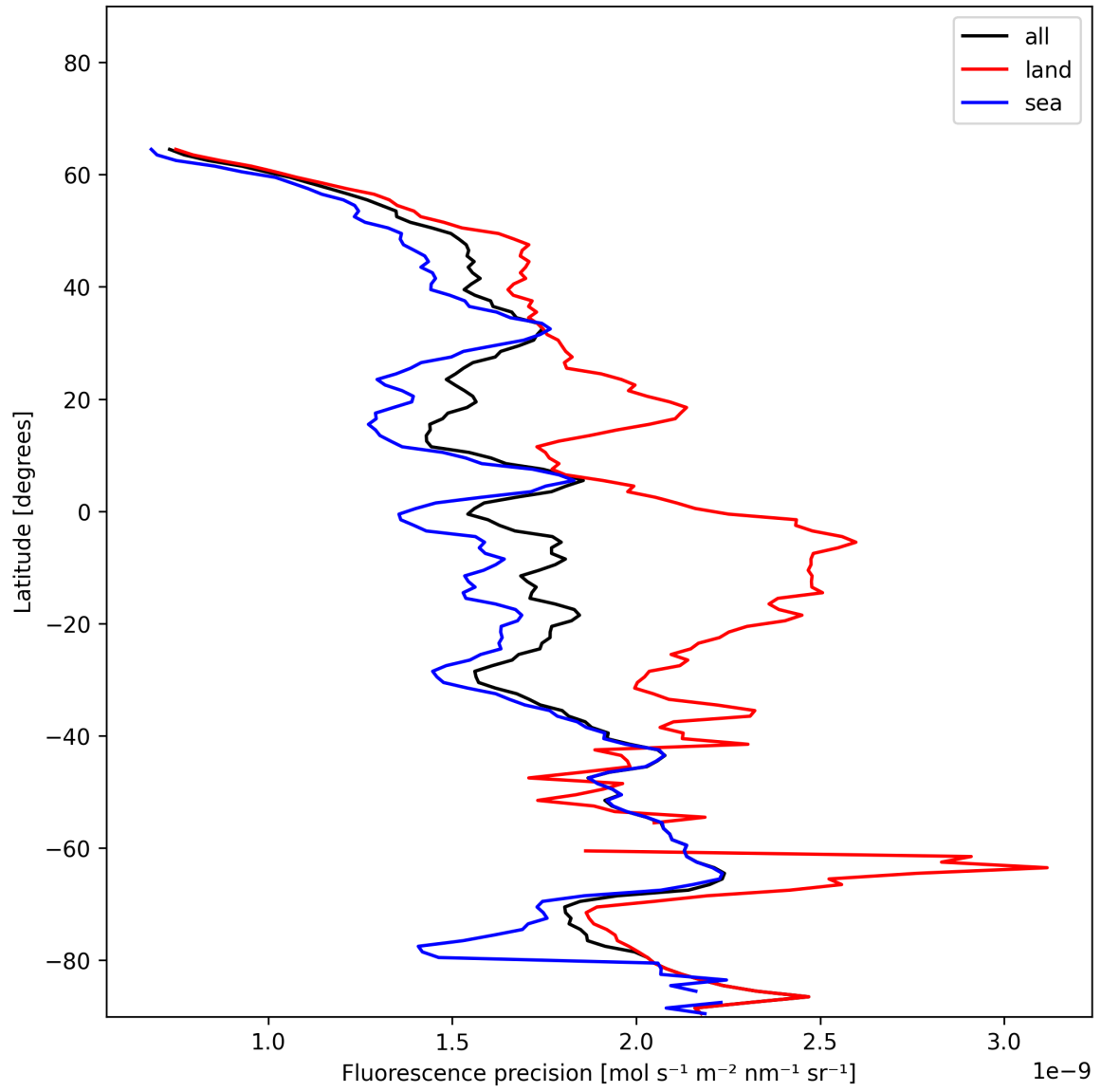
Figure 24: Zonal average of “Fluorescence precision” for 2024-12-28 to 2024-12-30.
