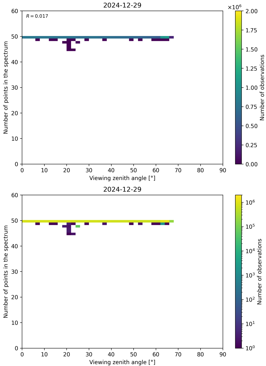
Figure 125: Scatter density plot of “Viewing zenith angle” against “Number of points in the spectrum” for 2024-12-28 to 2024-12-30.
