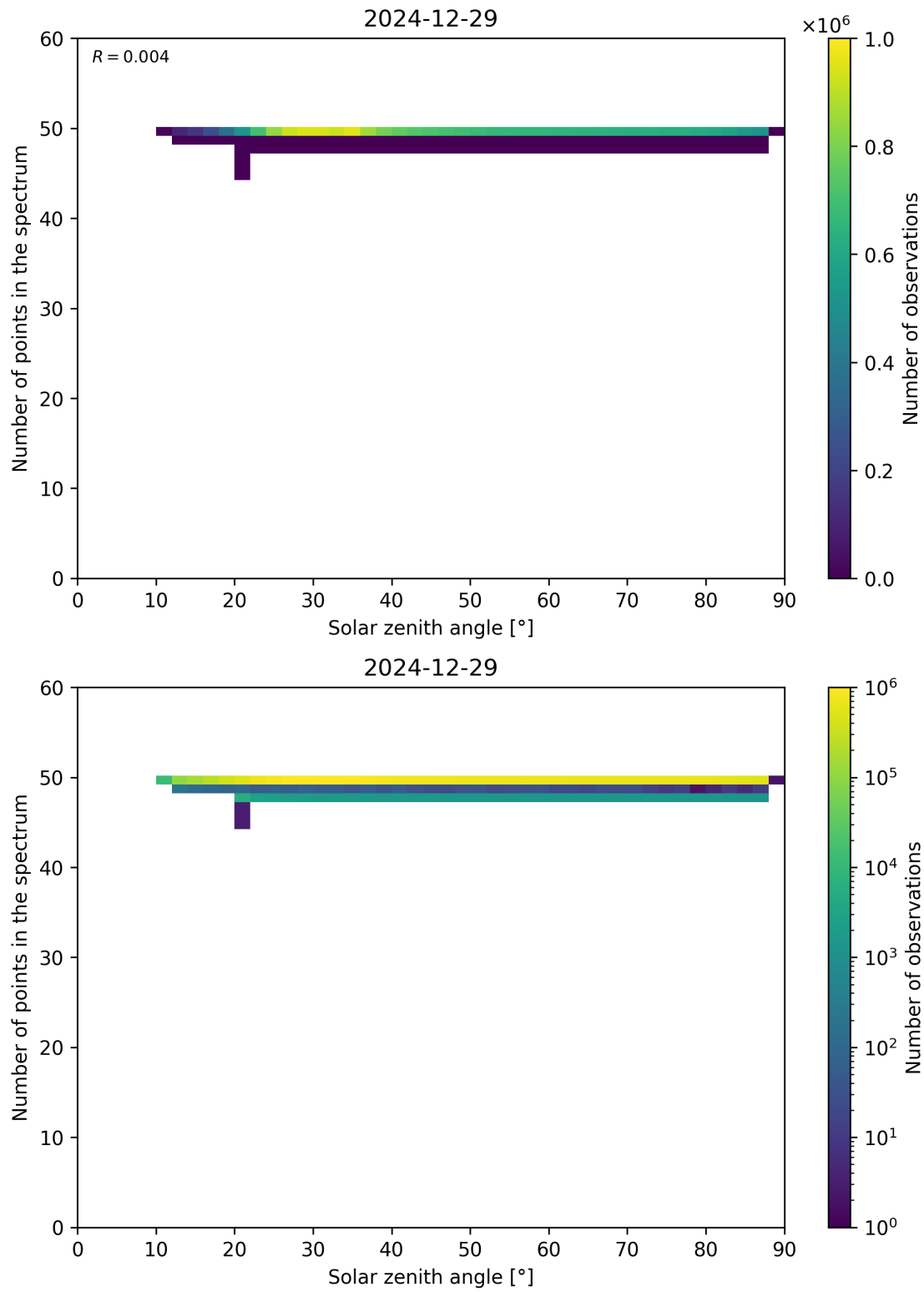
Figure 115: Scatter density plot of “Solar zenith angle” against “Number of points in the spectrum” for 2024-12-28 to 2024-12-30.
