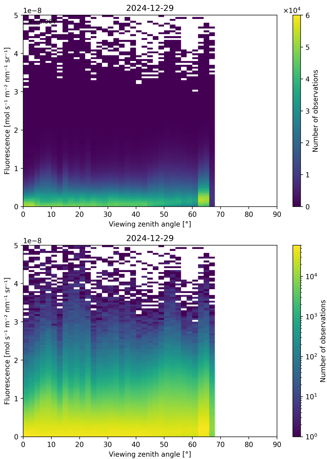
Figure 122: Scatter density plot of “Viewing zenith angle” against “Fluorescence” for 2024-12-28 to 2024-12-30.
