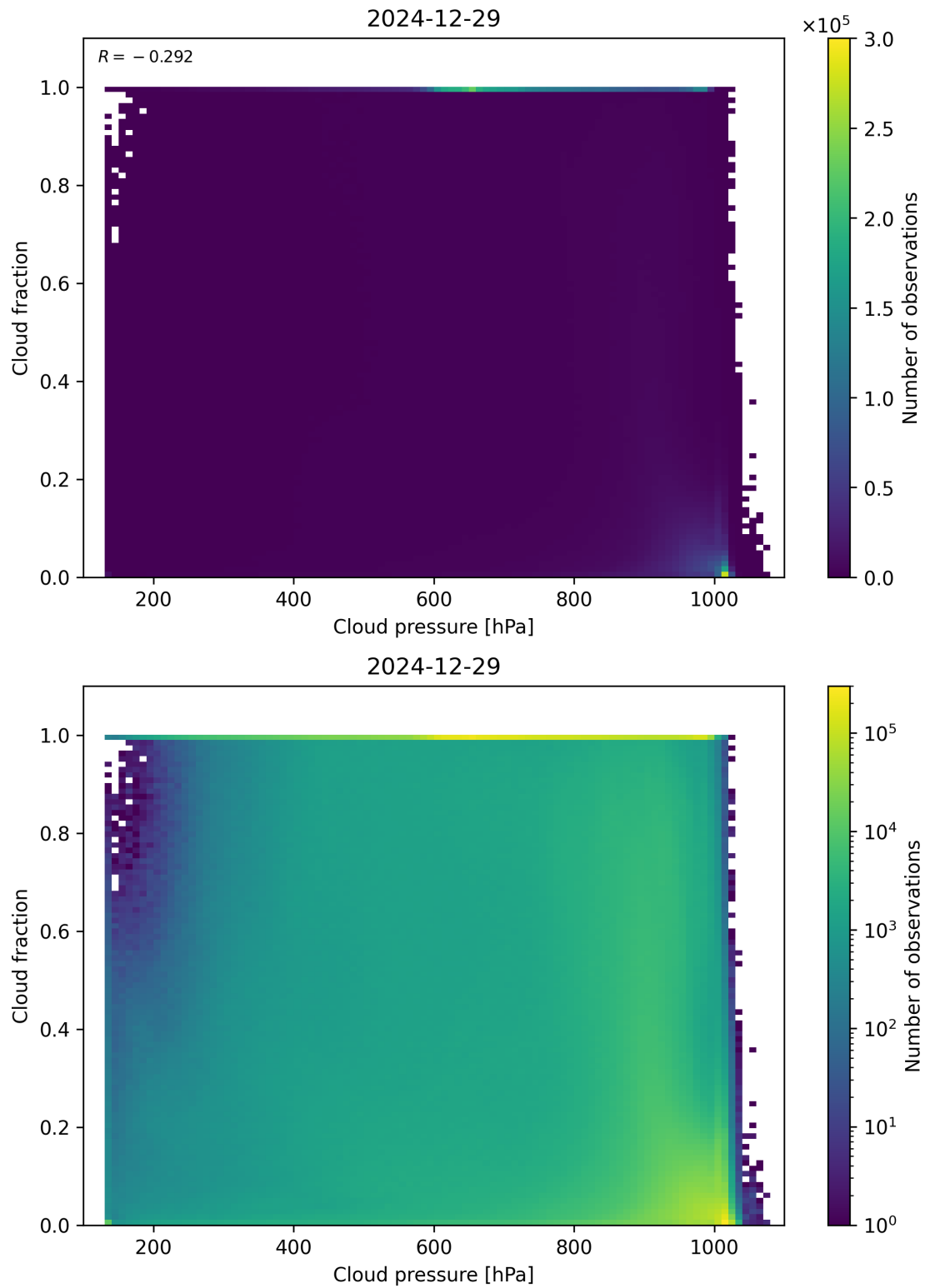
Figure 79: Scatter density plot of “Cloud pressure” against “Cloud fraction” for 2024-12-28 to 2024-12-30.
