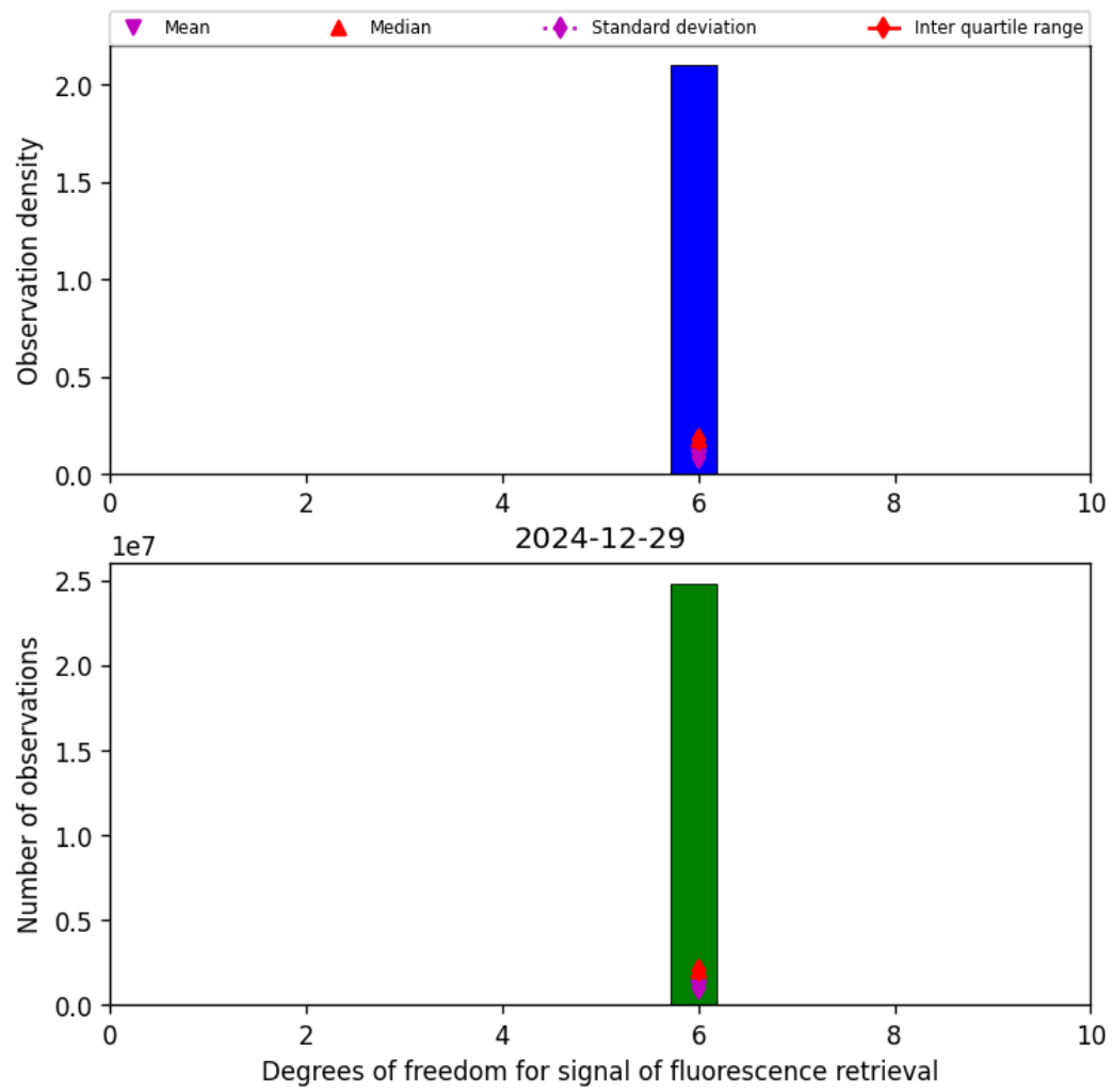
Figure 43: Histogram of “Degrees of freedom for signal of fluorescence retrieval” for 2024-12-28 to 2024-12-30
