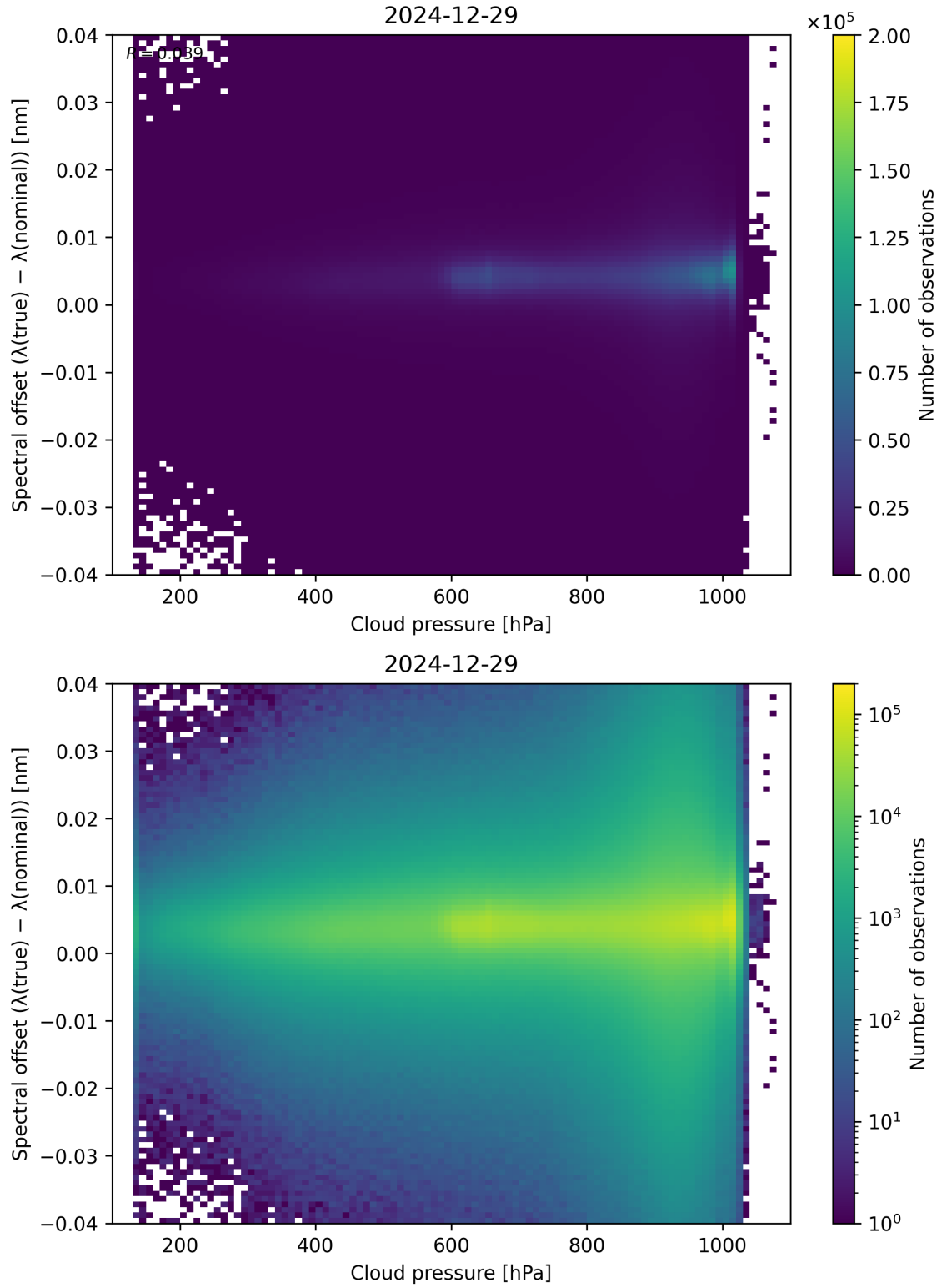
Figure 84: Scatter density plot of “Cloud pressure” against “Spectral offset ( \lambda_{\text{true}} - \lambda_{\text{nominal}} )” for 2024-12-28 to 2024-12-30.
