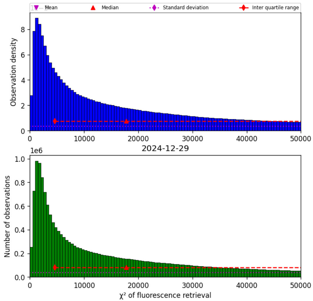
Figure 42: Histogram of “ \chi^2 of fluorescence retrieval” for 2024-12-28 to 2024-12-30
