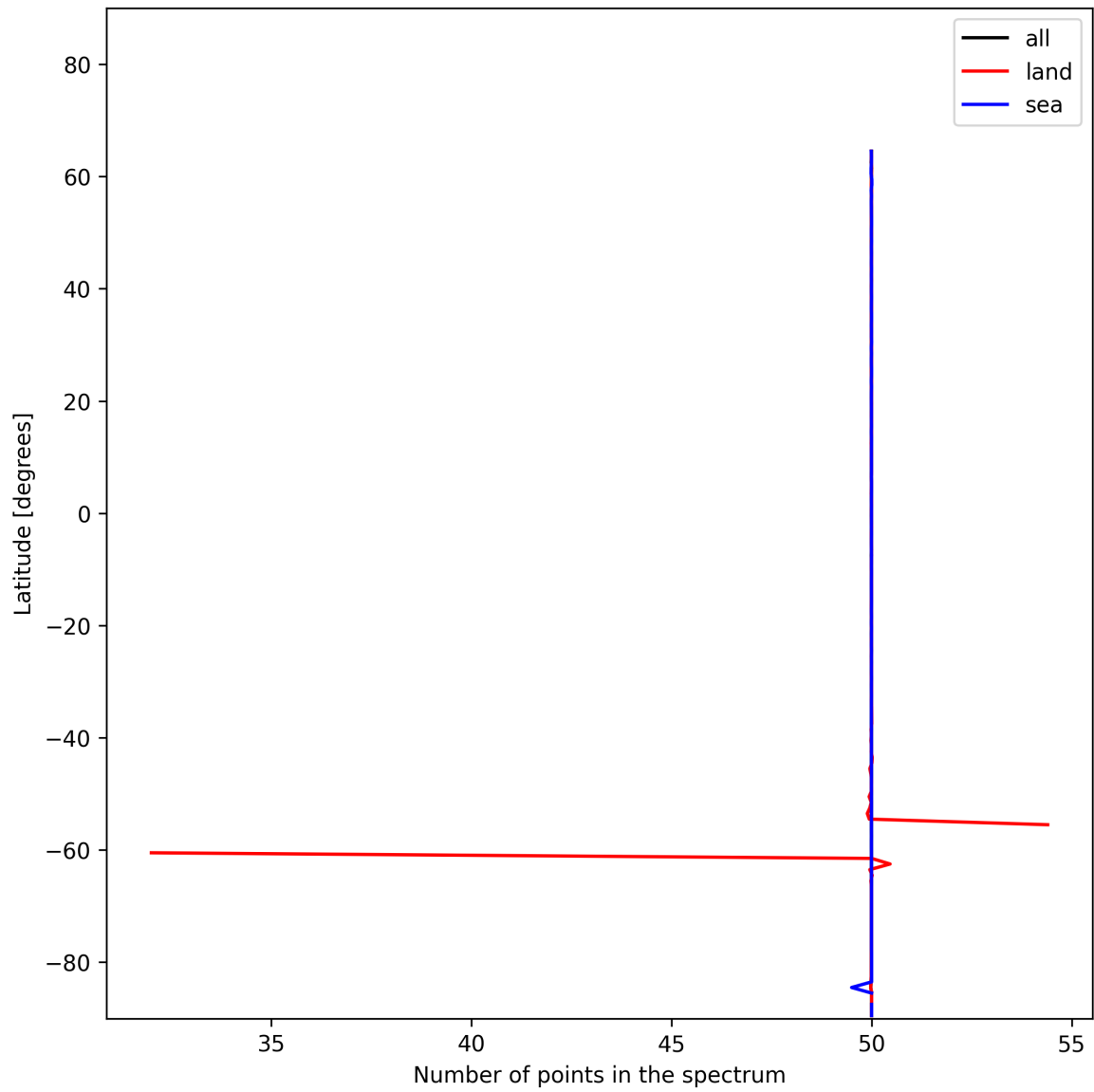
Figure 27: Zonal average of “Number of points in the spectrum” for 2024-12-28 to 2024-12-30.
