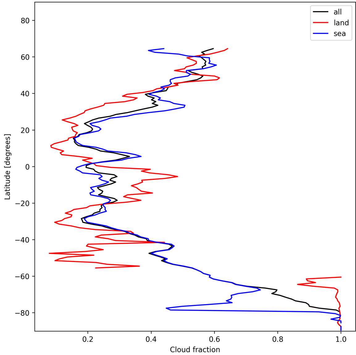
Figure 15: Zonal average of “Cloud fraction” for 2024-12-28 to 2024-12-30.
