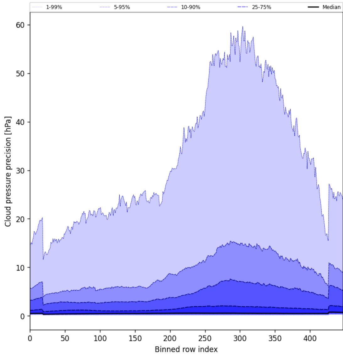
Figure 48: Along track statistics of “Cloud pressure precision” for 2024-12-28 to 2024-12-30
