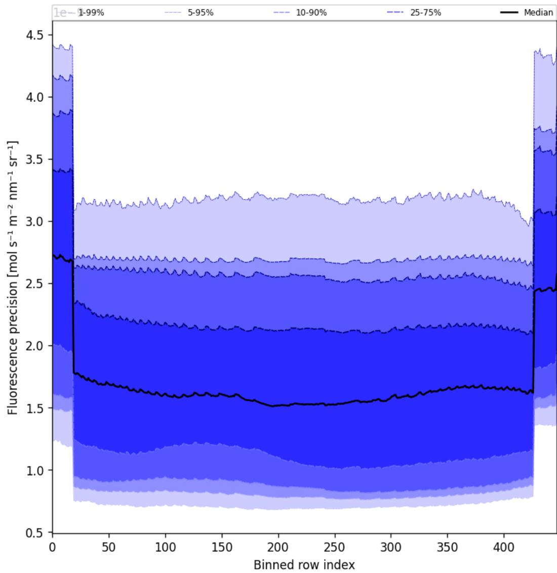
Figure 58: Along track statistics of “Fluorescence precision” for 2024-12-28 to 2024-12-30
