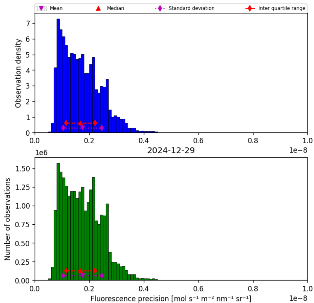
Figure 41: Histogram of “Fluorescence precision” for 2024-12-28 to 2024-12-30
