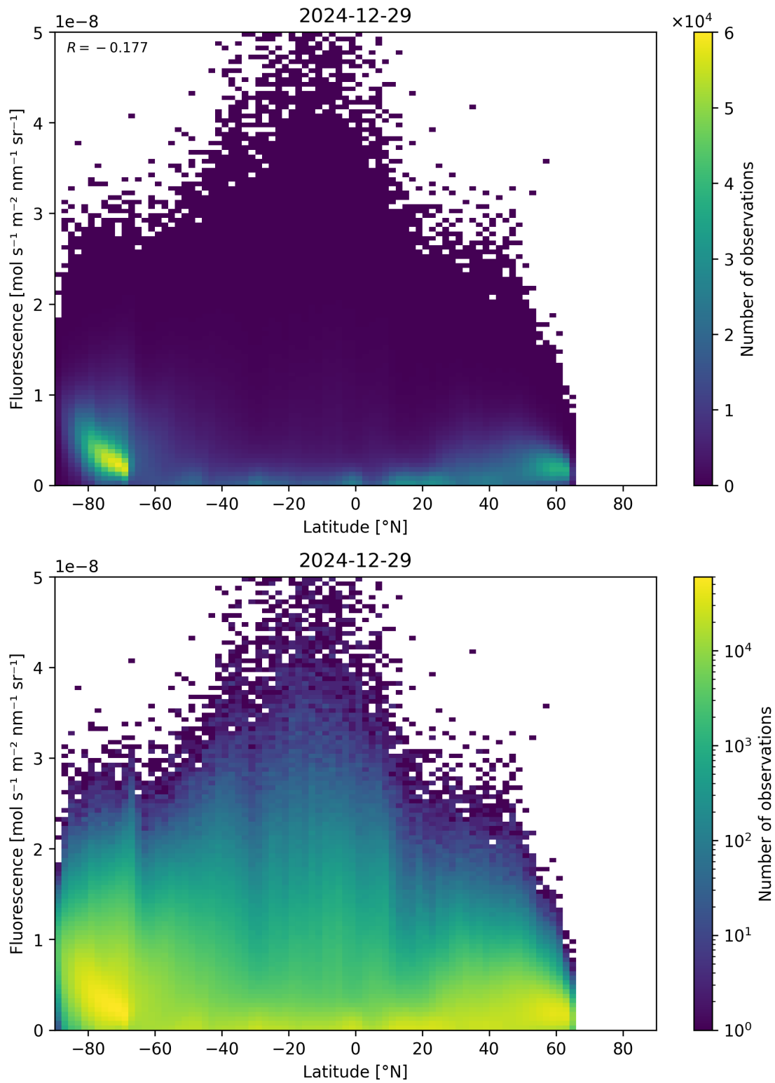
Figure 92: Scatter density plot of “Latitude” against “Fluorescence” for 2024-12-28 to 2024-12-30.
