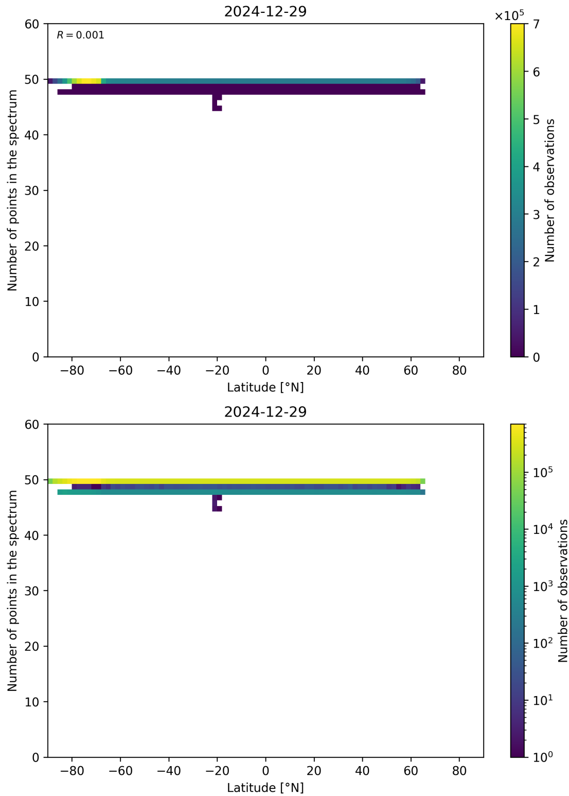
Figure 94: Scatter density plot of “Latitude” against “Number of points in the spectrum” for 2024-12-28 to 2024-12-30.
