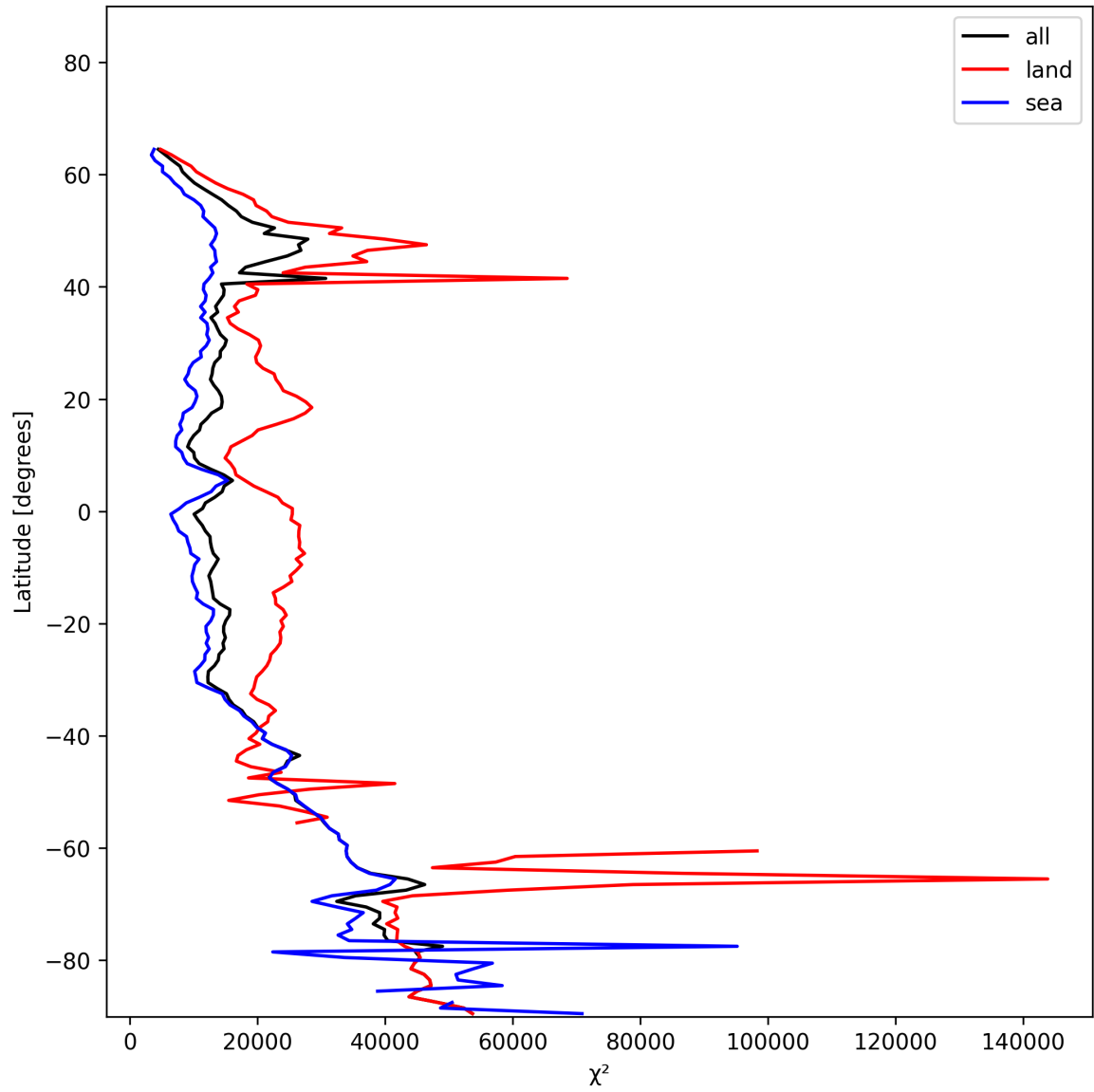
Figure 21: Zonal average of “ \chi^2 ” for 2024-12-28 to 2024-12-30.
