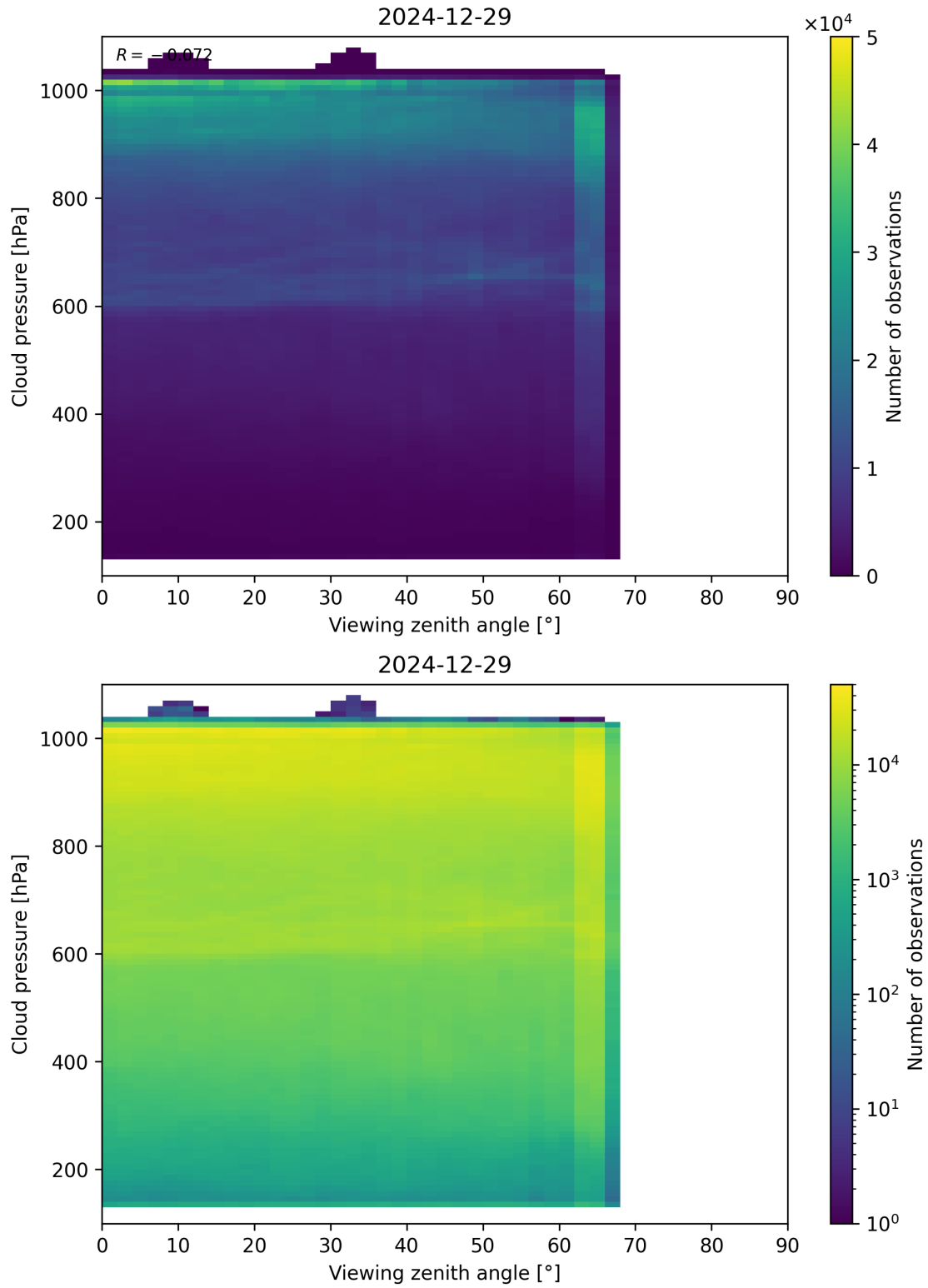
Figure 121: Scatter density plot of “Viewing zenith angle” against “Cloud pressure” for 2024-12-28 to 2024-12-30.
