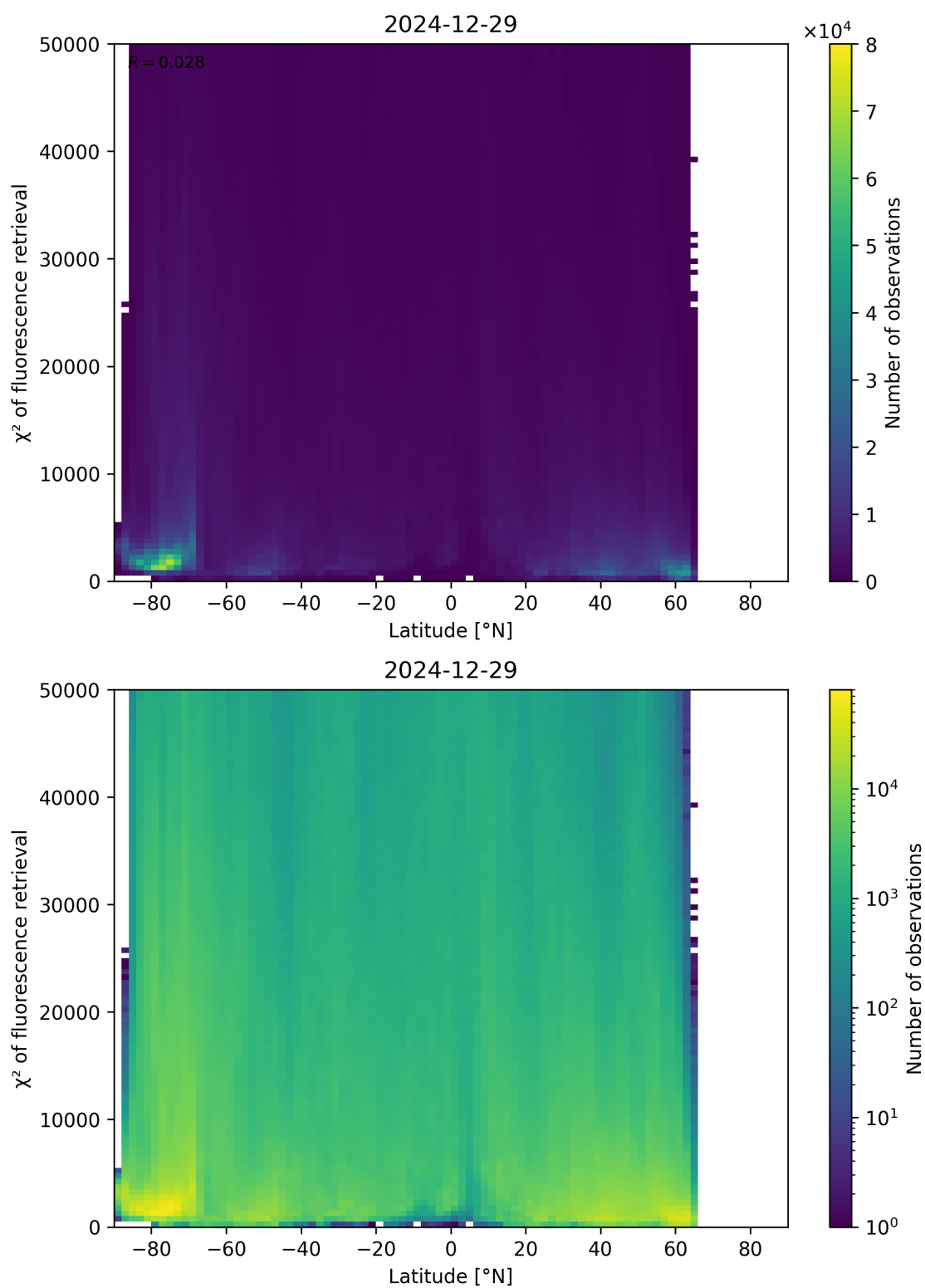
Figure 89: Scatter density plot of “Latitude” against “ \chi^2 of fluorescence retrieval” for 2024-12-28 to 2024-12-30.
