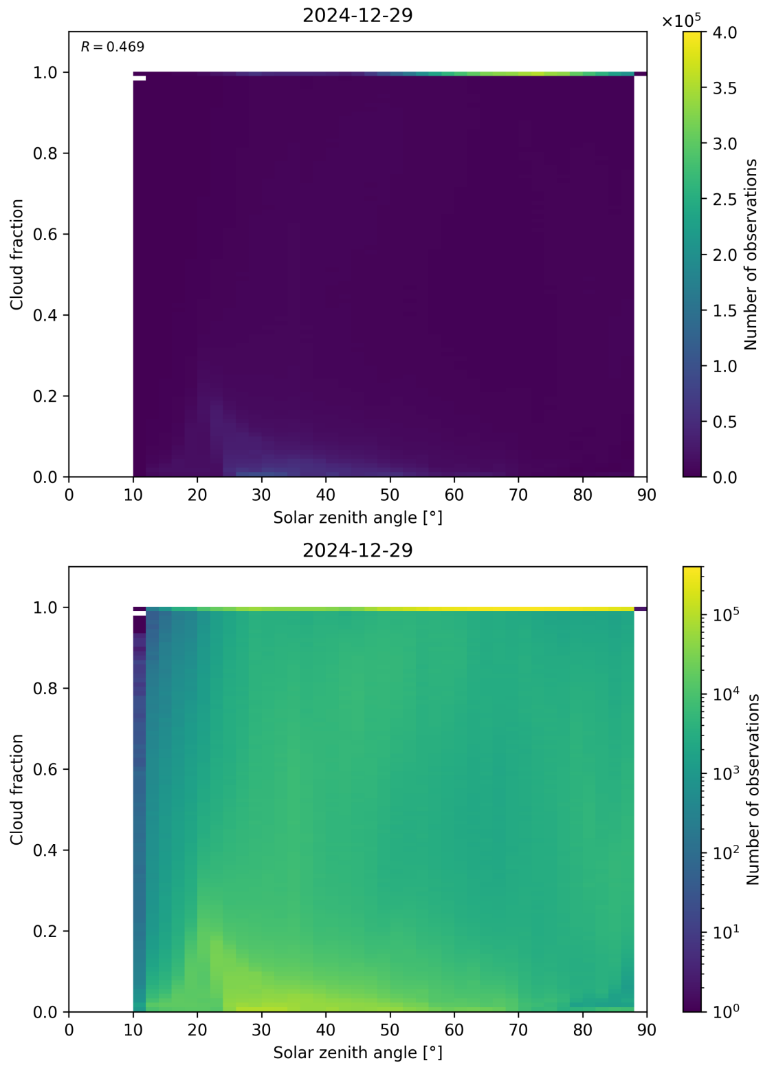
Figure 110: Scatter density plot of “Solar zenith angle” against “Cloud fraction” for 2024-12-28 to 2024-12-30.
