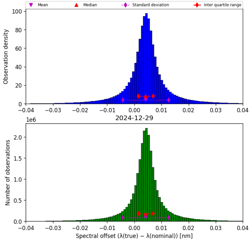
Figure 45: Histogram of “Spectral offset ( \lambda_{\text{true}} - \lambda_{\text{nominal}} )” for 2024-12-28 to 2024-12-30
