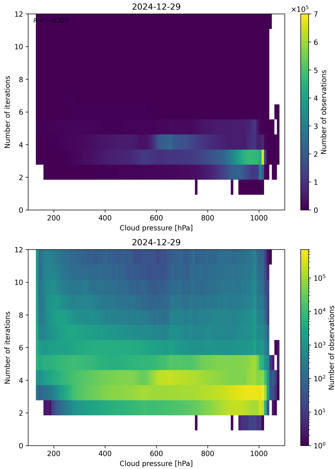
Figure 81: Scatter density plot of “Cloud pressure” against “Number of iterations” for 2024-12-28 to 2024-12-30.
