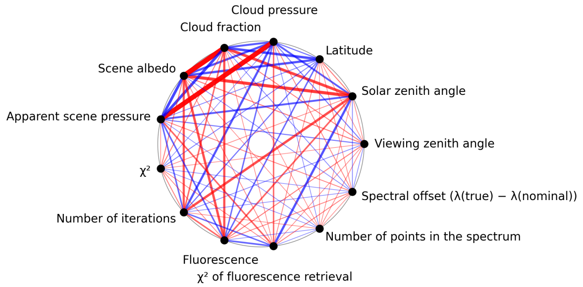
Figure 1: Map of correlation graph for 2024-12-28 to 2024-12-30.
