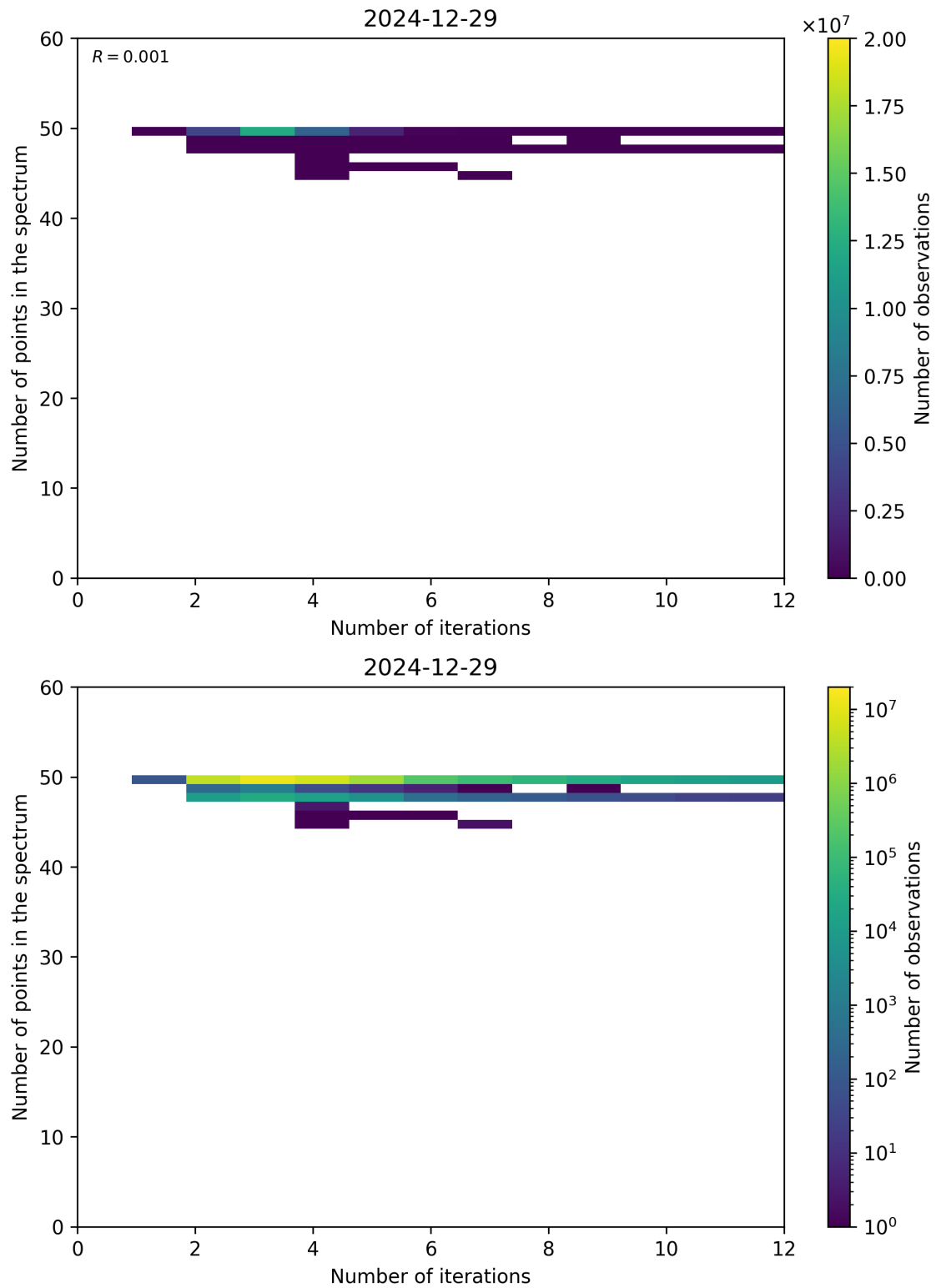
Figure 99: Scatter density plot of “Number of iterations” against “Number of points in the spectrum” for 2024-12-28 to 2024-12-30.
