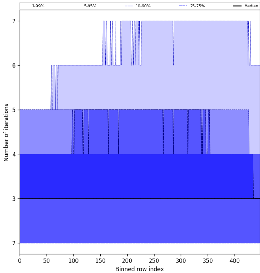
Figure 56: Along track statistics of “Number of iterations” for 2024-12-28 to 2024-12-30
