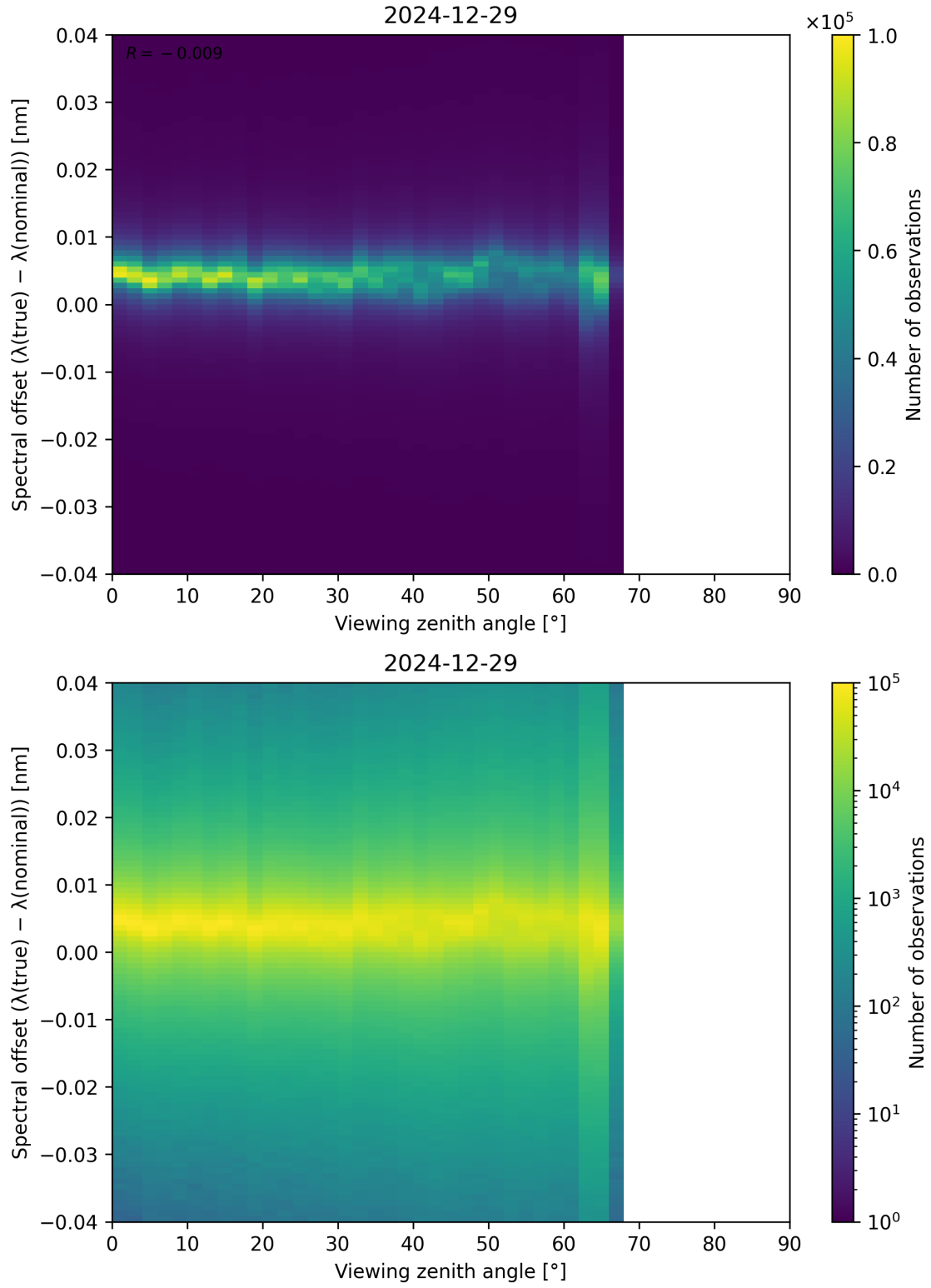
Figure 128: Scatter density plot of “Viewing zenith angle” against “Spectral offset ( \lambda_{\text{true}} - \lambda_{\text{nominal}} )” for 2024-12-28 to 2024-12-30.
