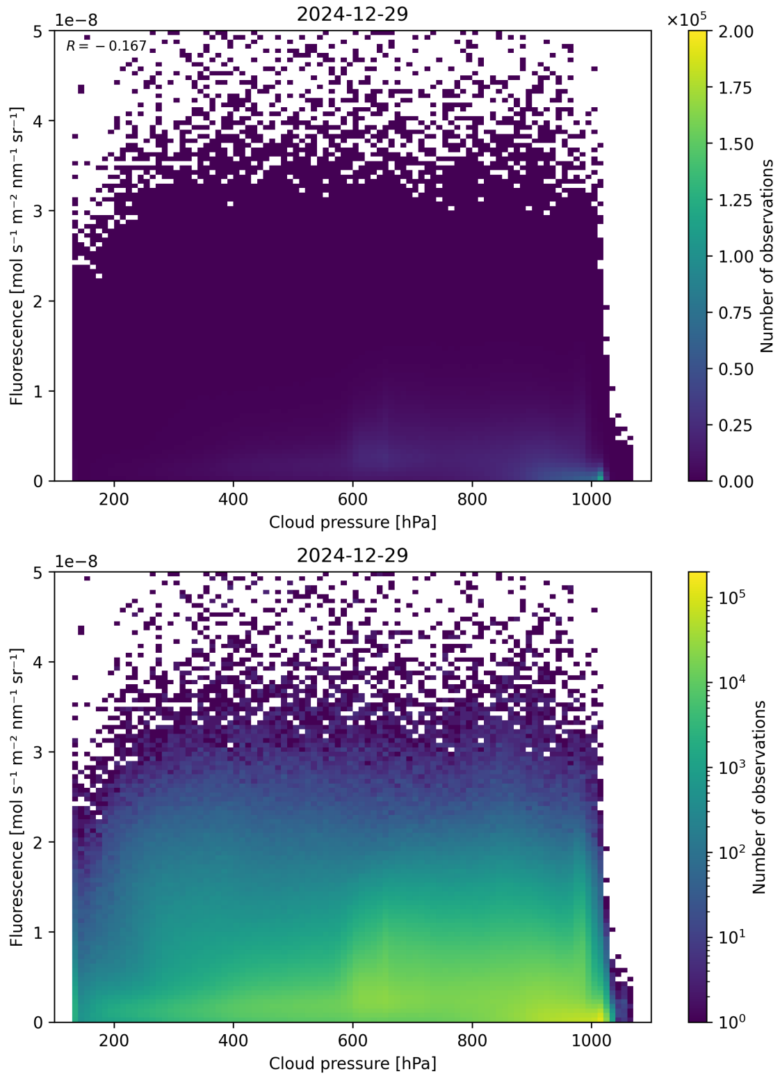
Figure 80: Scatter density plot of “Cloud pressure” against “Fluorescence” for 2024-12-28 to 2024-12-30.
