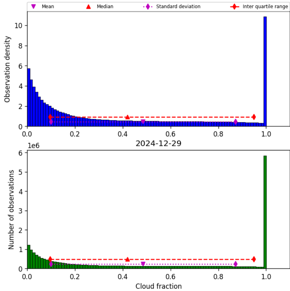
Figure 32: Histogram of “Cloud fraction” for 2024-12-28 to 2024-12-30
