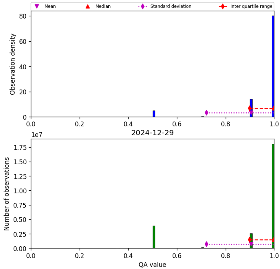
Figure 29: Histogram of “QA value” for 2024-12-28 to 2024-12-30
