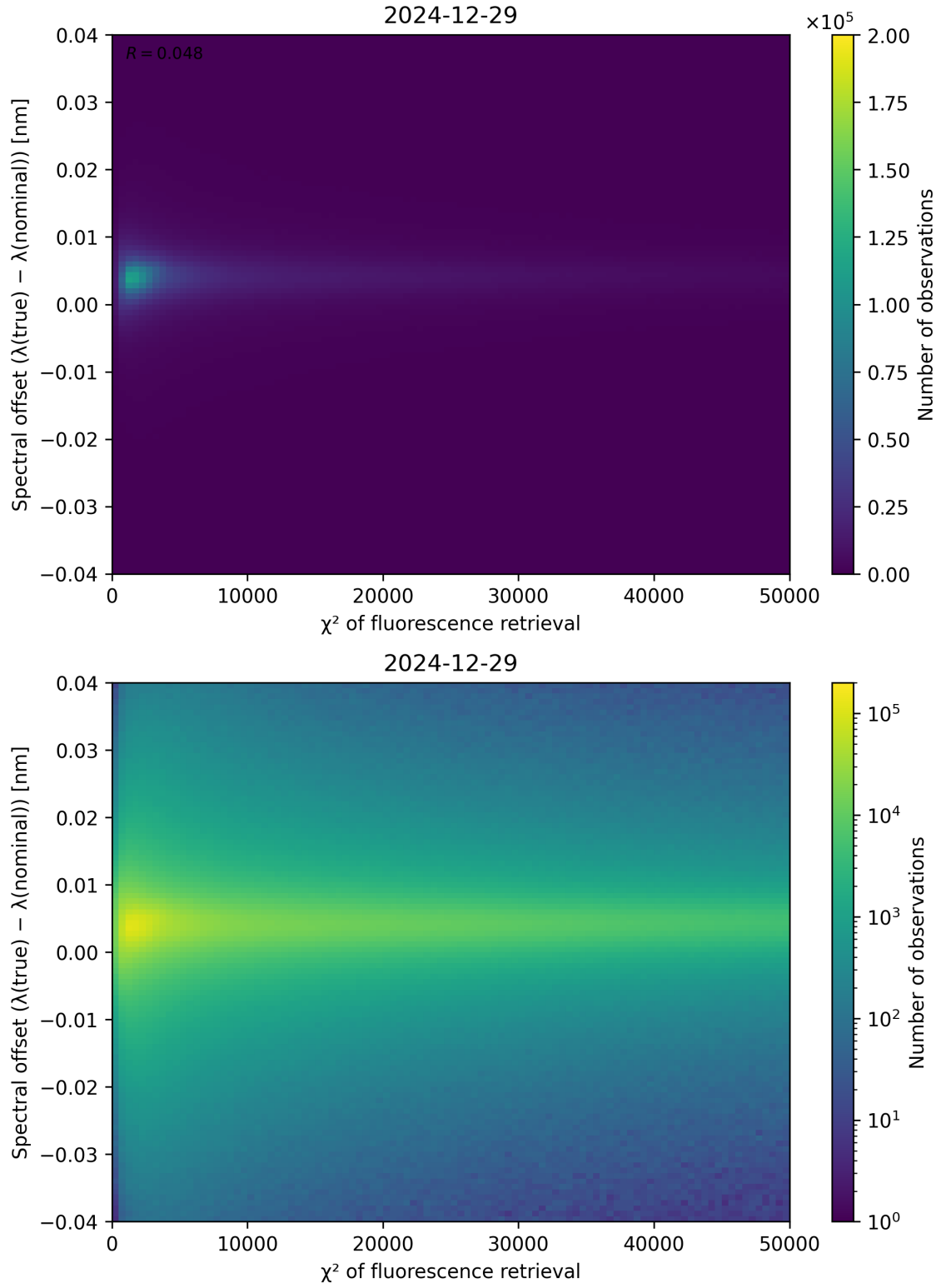
Figure 69: Scatter density plot of “ \chi^2 of fluorescence retrieval” against “Spectral offset ( \lambda_{\text{true}} - \lambda_{\text{nominal}} )” for 2024-12-28 to 2024-12-30.
