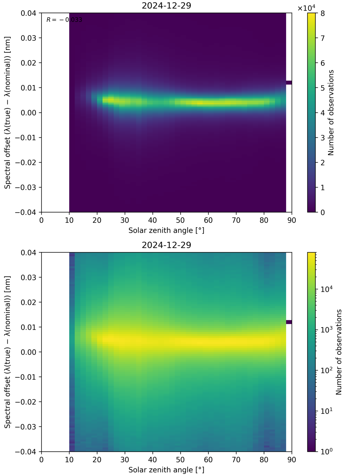
Figure 117: Scatter density plot of “Solar zenith angle” against “Spectral offset ( \lambda_{\text{true}} - \lambda_{\text{nominal}} )” for 2024-12-28 to 2024-12-30.
