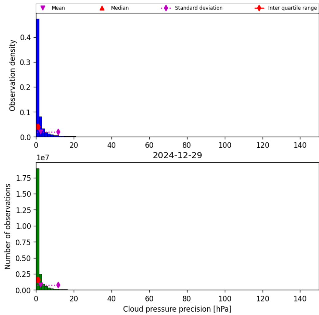
Figure 31: Histogram of “Cloud pressure precision” for 2024-12-28 to 2024-12-30
