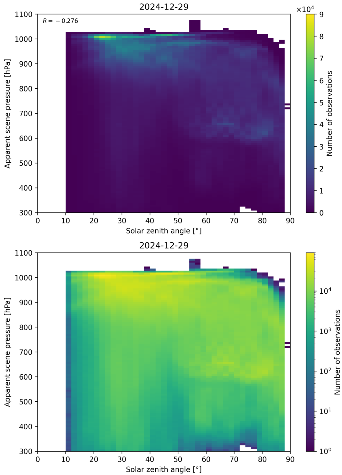
Figure 108: Scatter density plot of “Solar zenith angle” against “Apparent scene pressure” for 2024-12-28 to 2024-12-30.
