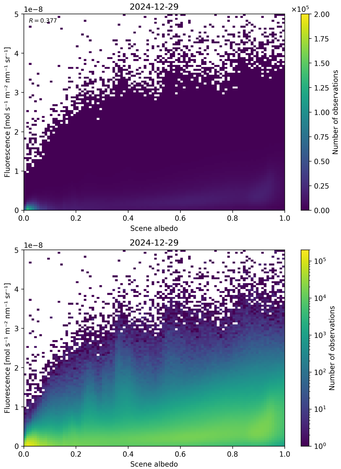
Figure 104: Scatter density plot of “Scene albedo” against “Fluorescence” for 2024-12-28 to 2024-12-30.
