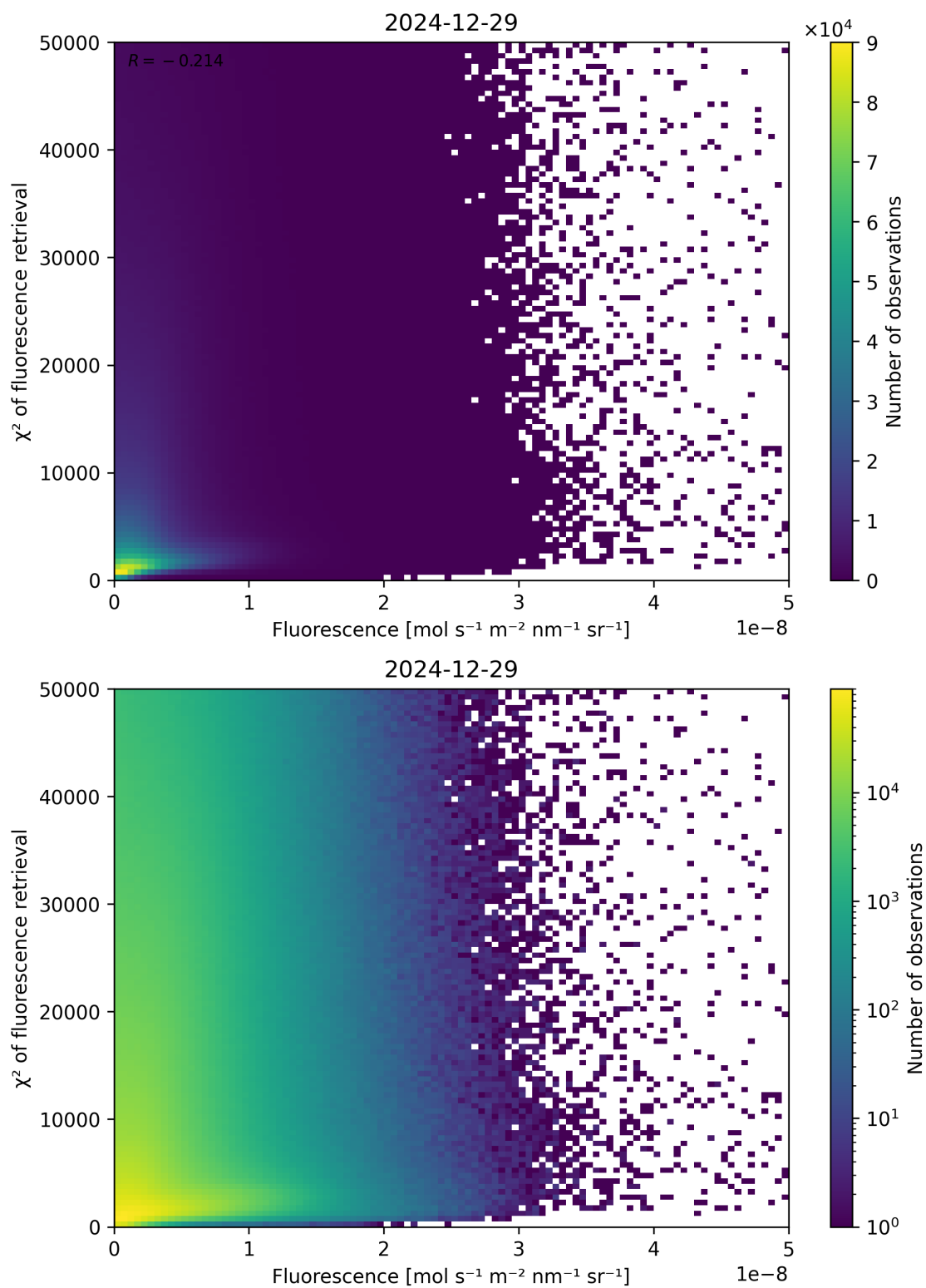
Figure 85: Scatter density plot of “Fluorescence” against “ \chi^2 of fluorescence retrieval” for 2024-12-28 to 2024-12-30.
