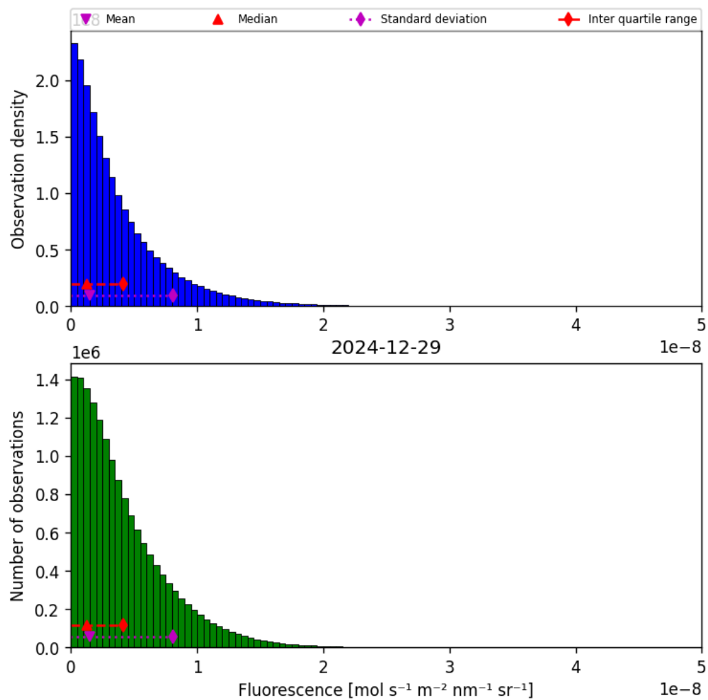
Figure 40: Histogram of “Fluorescence” for 2024-12-28 to 2024-12-30
