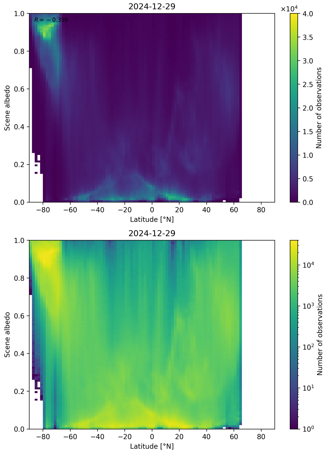
Figure 95: Scatter density plot of “Latitude” against “Scene albedo” for 2024-12-28 to 2024-12-30.
