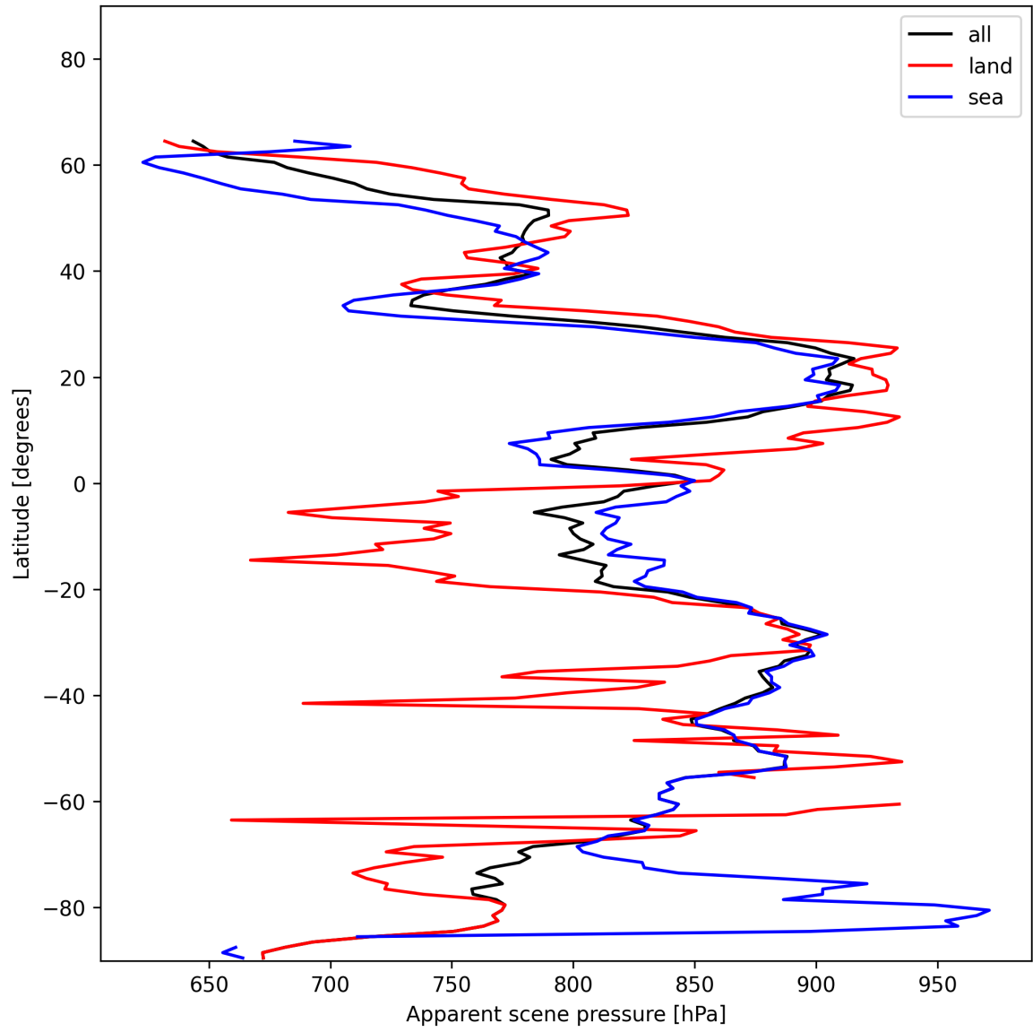
Figure 19: Zonal average of “Apparent scene pressure” for 2024-12-28 to 2024-12-30.
