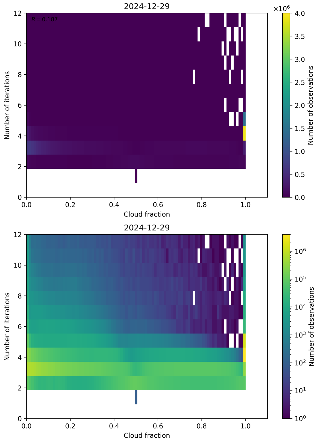
Figure 73: Scatter density plot of “Cloud fraction” against “Number of iterations” for 2024-12-28 to 2024-12-30.
