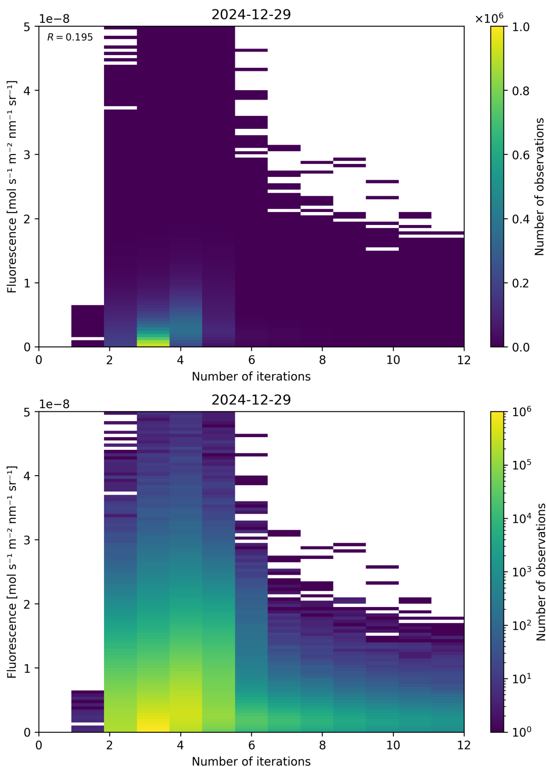
Figure 98: Scatter density plot of “Number of iterations” against “Fluorescence” for 2024-12-28 to 2024-12-30.
