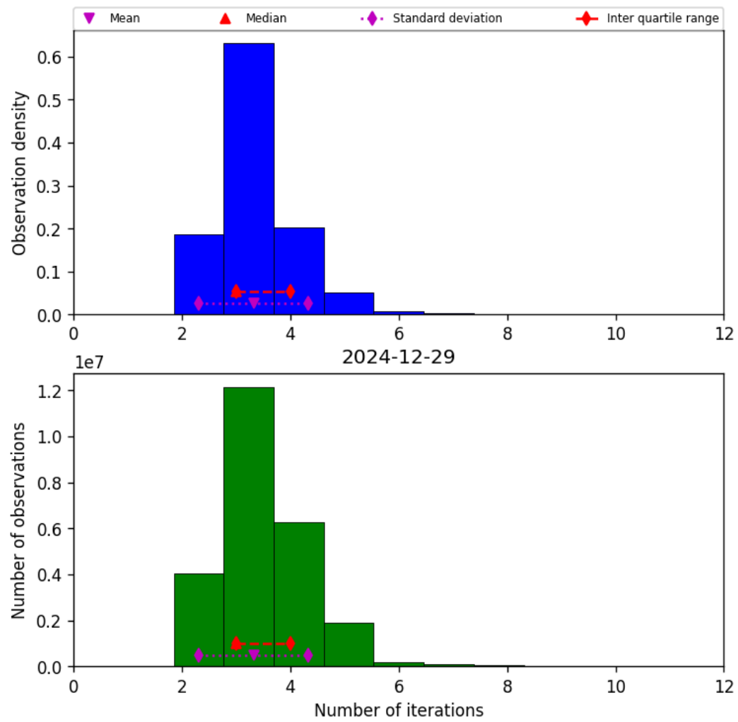
Figure 39: Histogram of “Number of iterations” for 2024-12-28 to 2024-12-30
