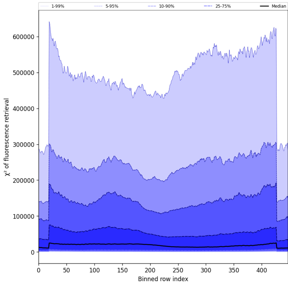
Figure 59: Along track statistics of “ \chi^2 of fluorescence retrieval” for 2024-12-28 to 2024-12-30
