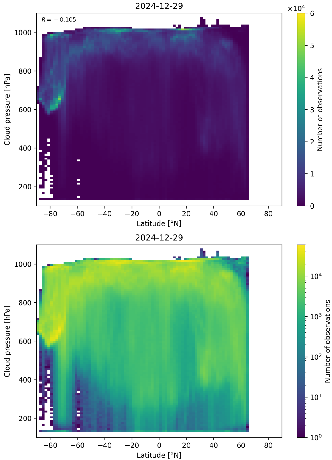
Figure 91: Scatter density plot of “Latitude” against “Cloud pressure” for 2024-12-28 to 2024-12-30.
