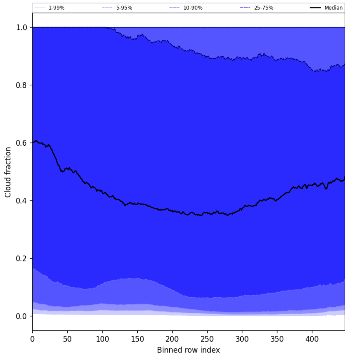
Figure 49: Along track statistics of “Cloud fraction” for 2024-12-28 to 2024-12-30
