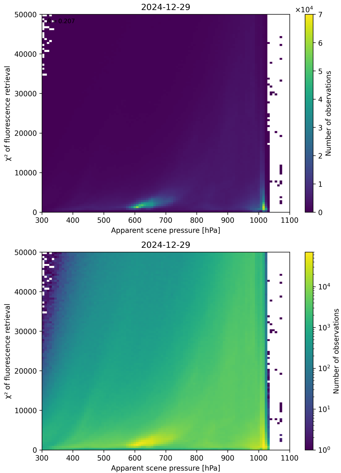
Figure 63: Scatter density plot of “Apparent scene pressure” against “ \chi^2 of fluorescence retrieval” for 2024-12-28 to 2024-12-30.
