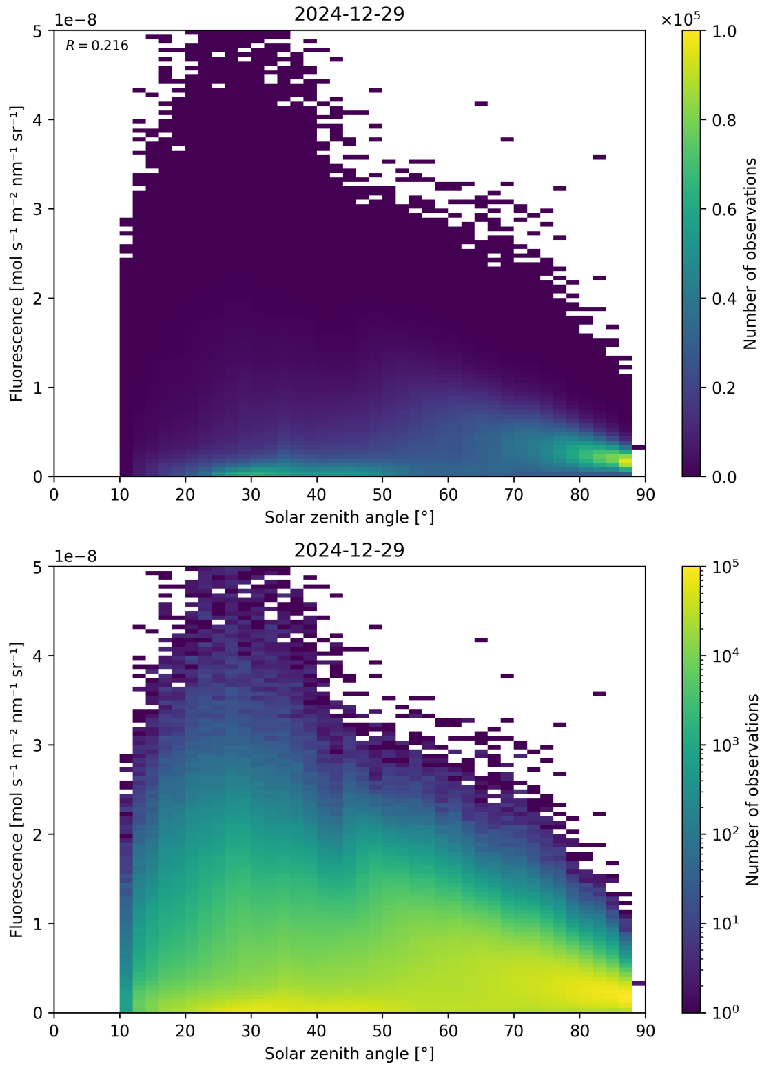
Figure 112: Scatter density plot of “Solar zenith angle” against “Fluorescence” for 2024-12-28 to 2024-12-30.
