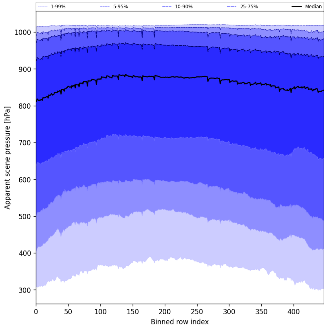
Figure 53: Along track statistics of “Apparent scene pressure” for 2024-12-28 to 2024-12-30
