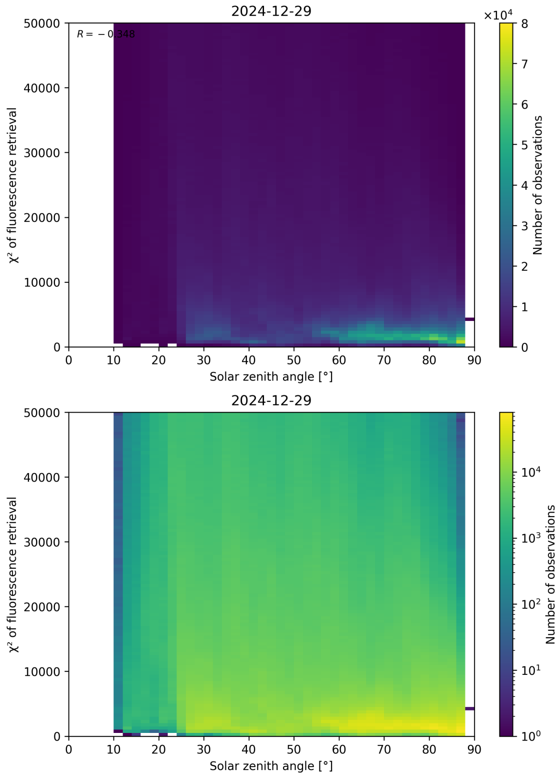
Figure 109: Scatter density plot of “Solar zenith angle” against “ \chi^2 of fluorescence retrieval” for 2024-12-28 to 2024-12-30.
