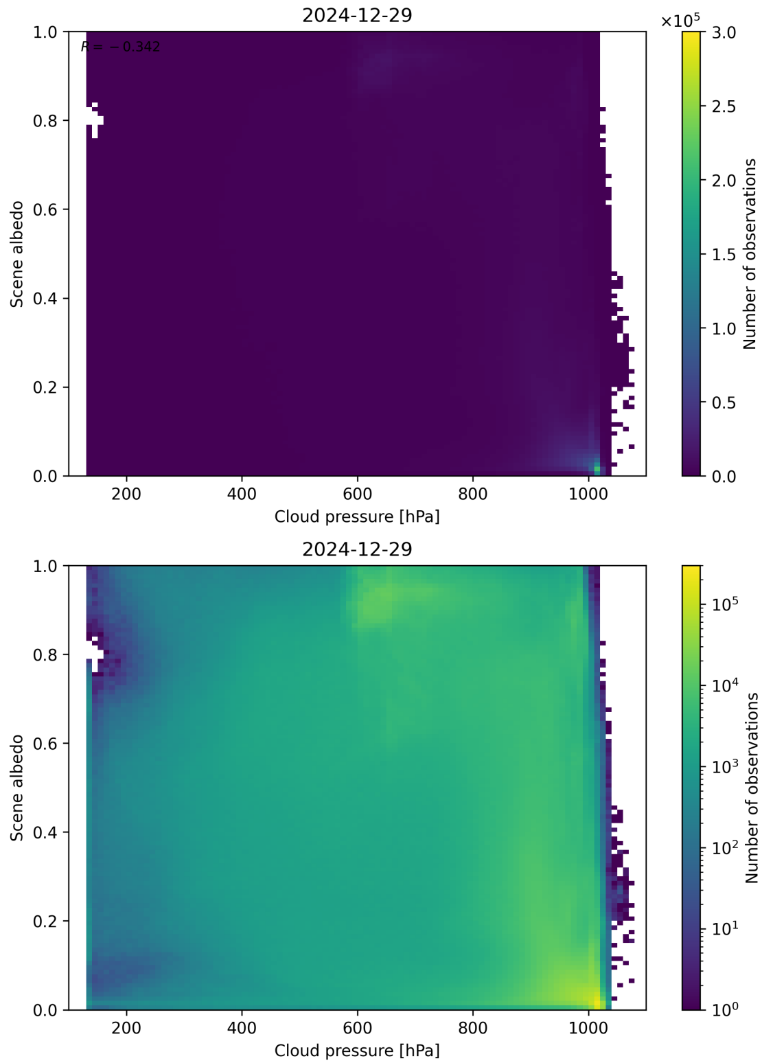
Figure 83: Scatter density plot of “Cloud pressure” against “Scene albedo” for 2024-12-28 to 2024-12-30.
