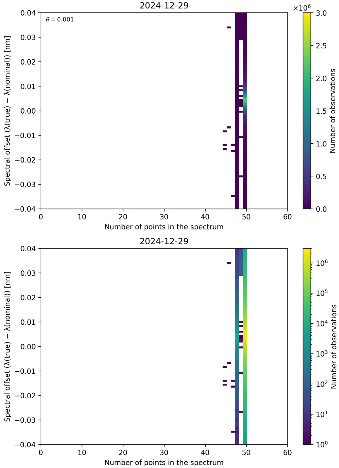
Figure 101: Scatter density plot of “Number of points in the spectrum” against “Spectral offset ( \lambda_{\text{true}} - \lambda_{\text{nominal}} )” for 2024-12-28 to 2024-12-30.
