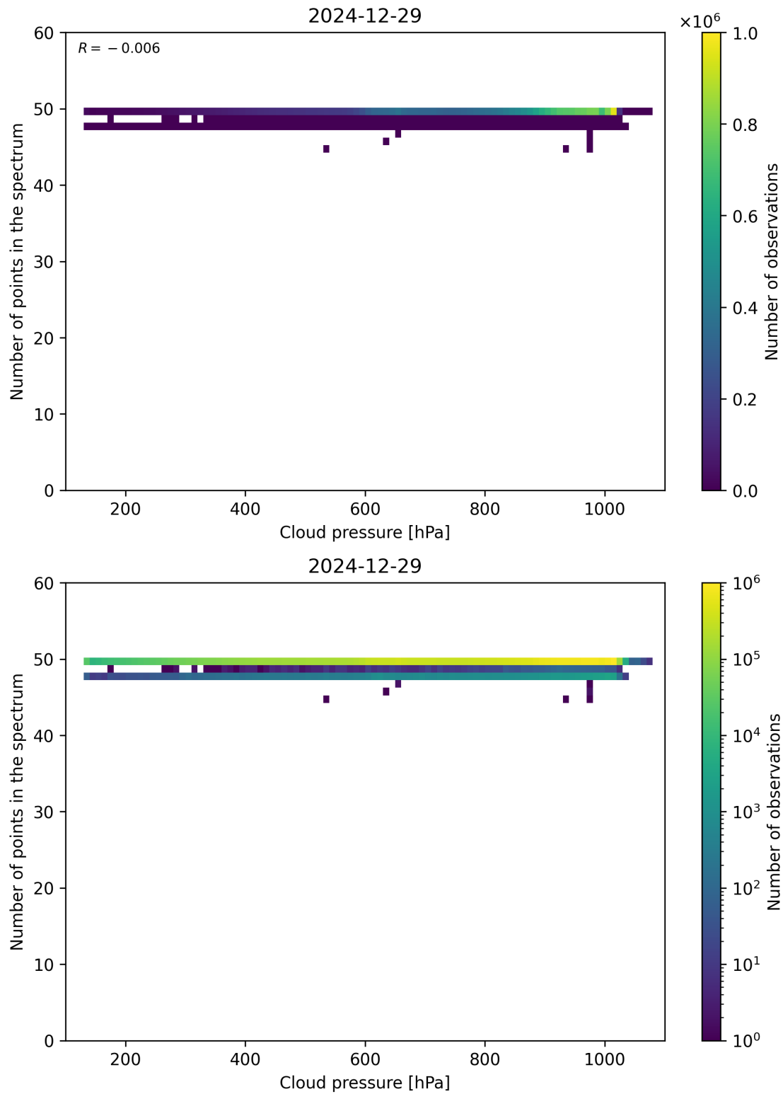
Figure 82: Scatter density plot of “Cloud pressure” against “Number of points in the spectrum” for 2024-12-28 to 2024-12-30.
