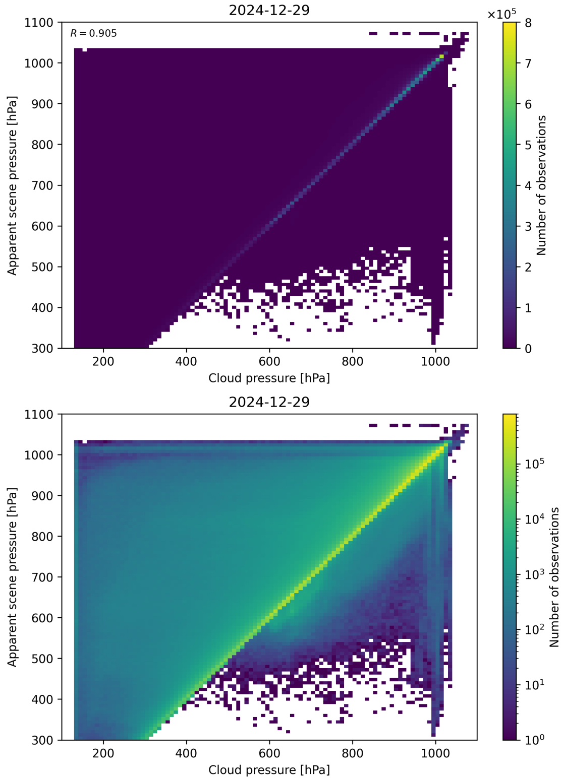
Figure 77: Scatter density plot of “Cloud pressure” against “Apparent scene pressure” for 2024-12-28 to 2024-12-30.
