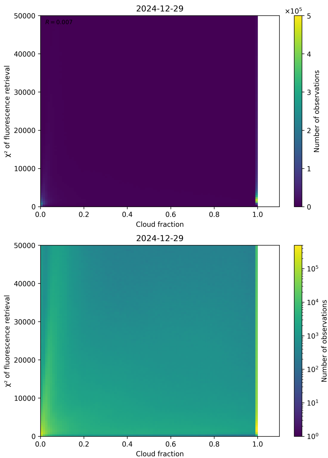
Figure 71: Scatter density plot of “Cloud fraction” against “ \chi^2 of fluorescence retrieval” for 2024-12-28 to 2024-12-30.
