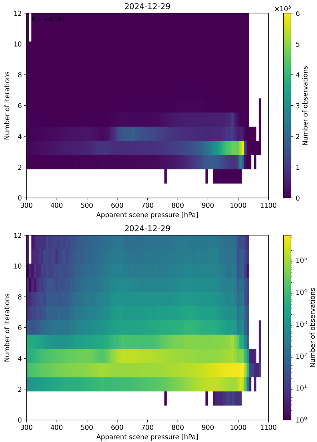
Figure 65: Scatter density plot of “Apparent scene pressure” against “Number of iterations” for 2024-12-28 to 2024-12-30.
