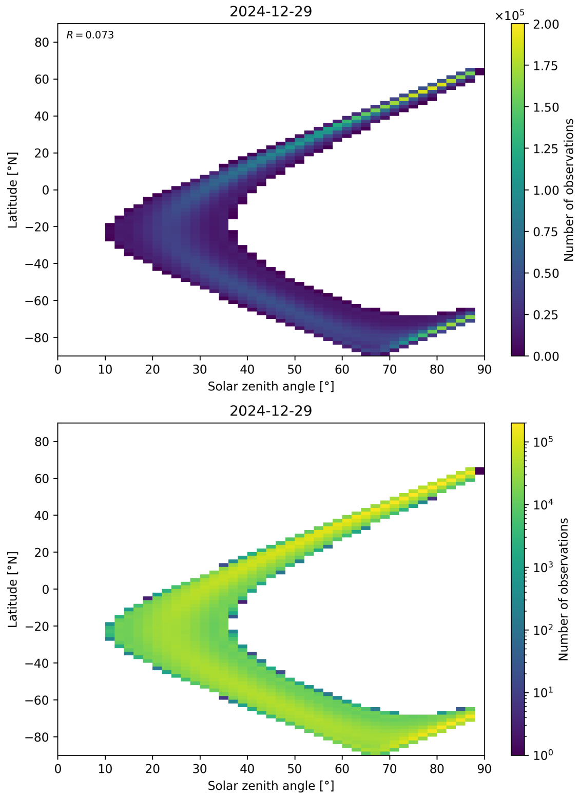
Figure 113: Scatter density plot of “Solar zenith angle” against “Latitude” for 2024-12-28 to 2024-12-30.
