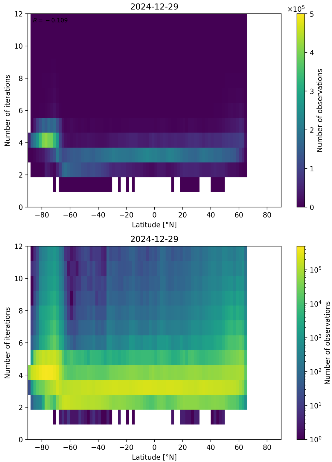
Figure 93: Scatter density plot of “Latitude” against “Number of iterations” for 2024-12-28 to 2024-12-30.
