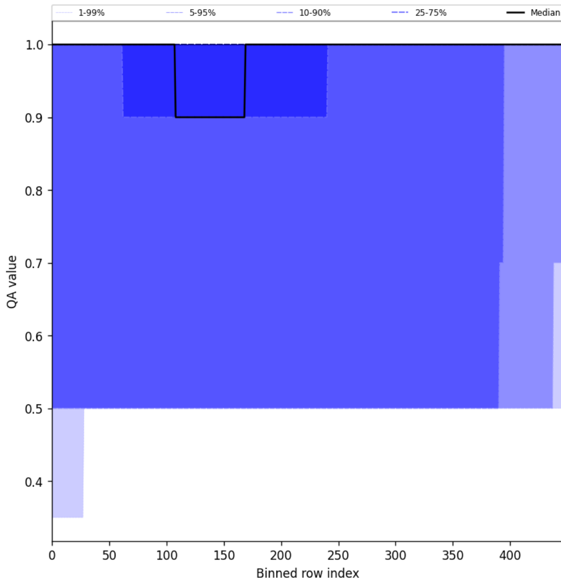
Figure 46: Along track statistics of “QA value” for 2024-12-28 to 2024-12-30
