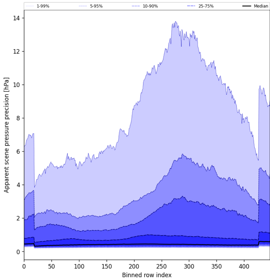
Figure 54: Along track statistics of “Apparent scene pressure precision” for 2024-12-28 to 2024-12-30
