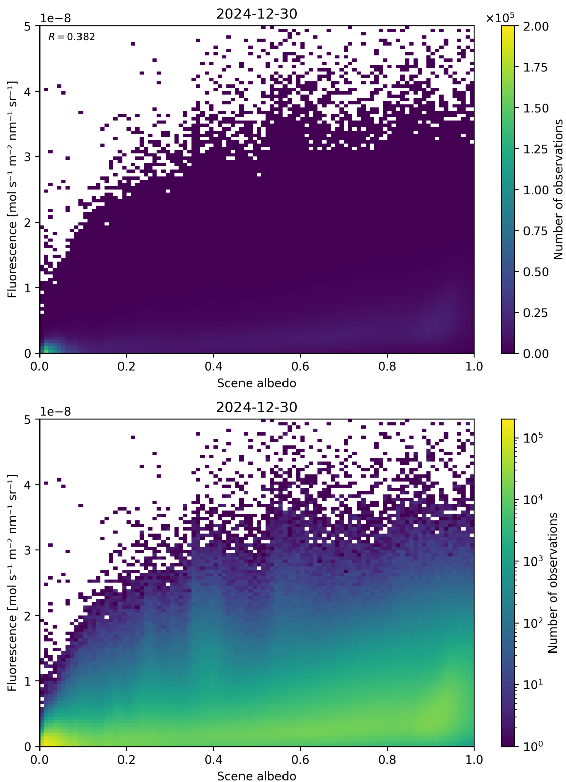
Figure 104: Scatter density plot of “Scene albedo” against “Fluorescence” for 2024-12-29 to 2024-12-31.
