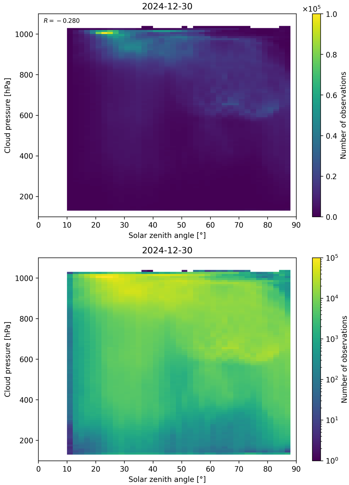
Figure 111: Scatter density plot of “Solar zenith angle” against “Cloud pressure” for 2024-12-29 to 2024-12-31.
