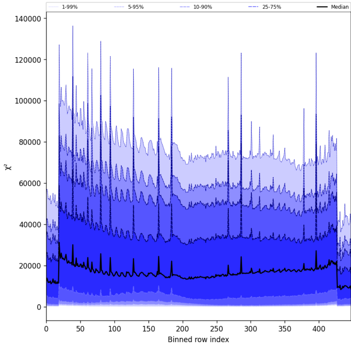
Figure 55: Along track statistics of “ \chi^2 ” for 2024-12-29 to 2024-12-31
