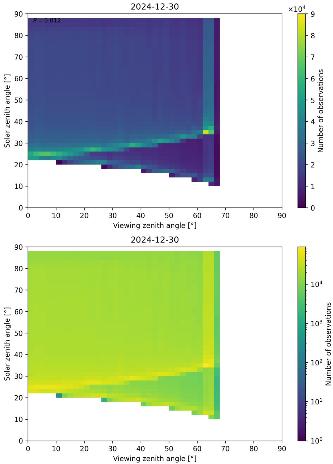
Figure 127: Scatter density plot of “Viewing zenith angle” against “Solar zenith angle” for 2024-12-29 to 2024-12-31.
