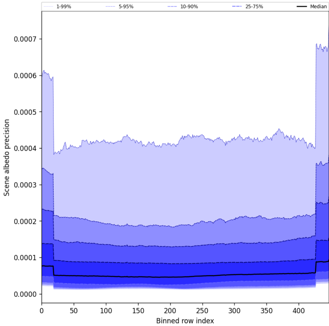
Figure 52: Along track statistics of “Scene albedo precision” for 2024-12-29 to 2024-12-31
