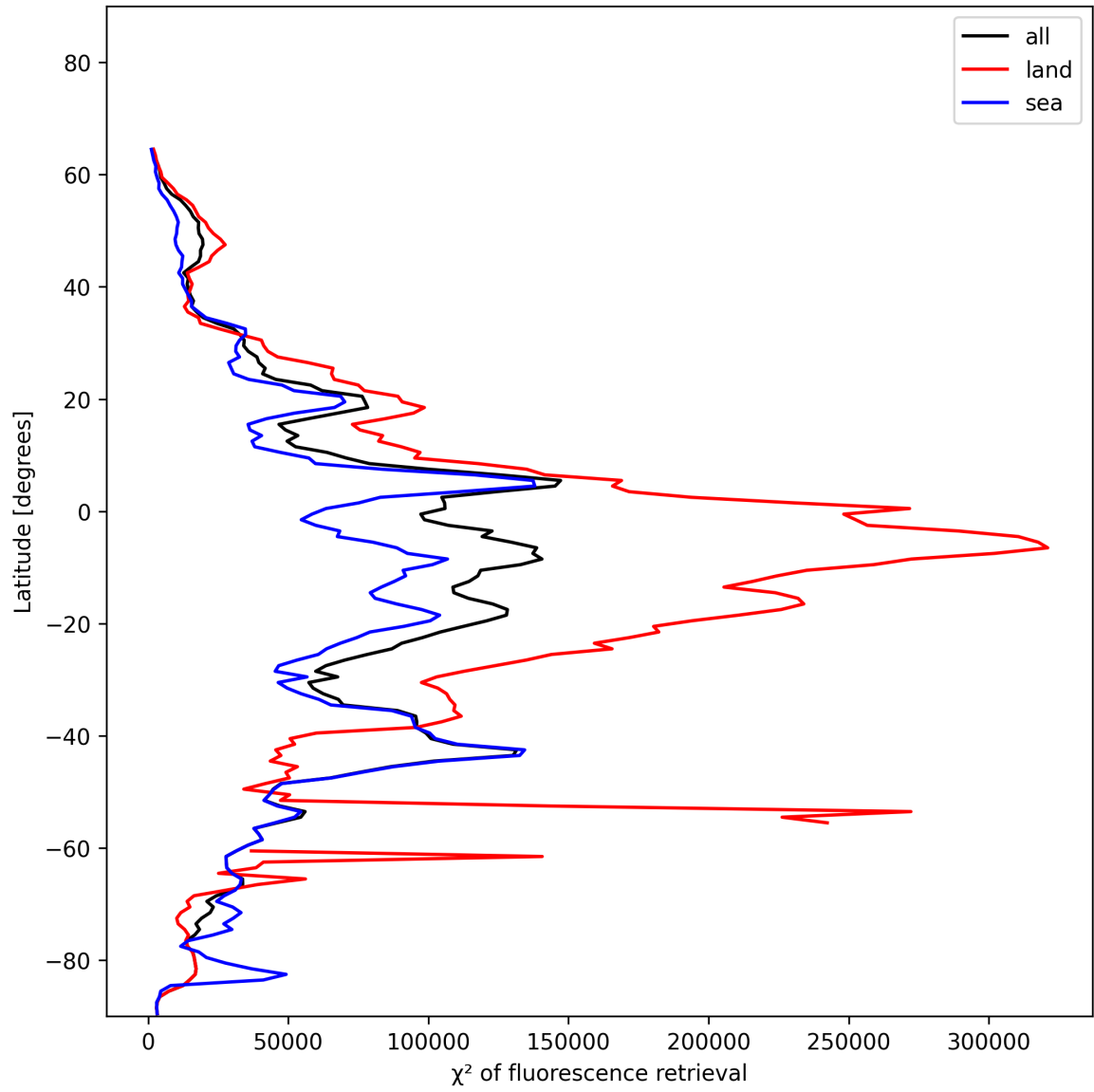
Figure 25: Zonal average of “ \chi^2 of fluorescence retrieval” for 2024-12-29 to 2024-12-31.
