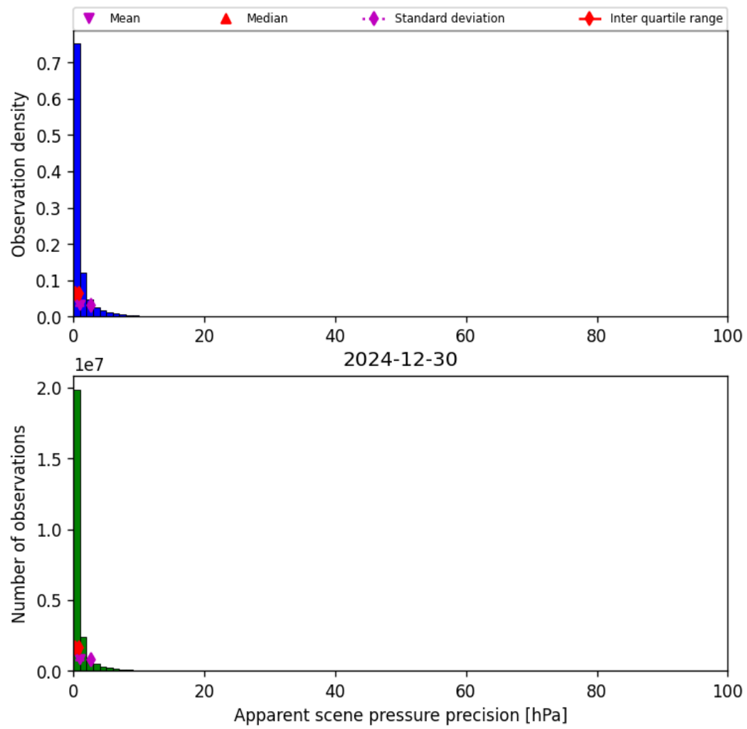
Figure 37: Histogram of “Apparent scene pressure precision” for 2024-12-29 to 2024-12-31
