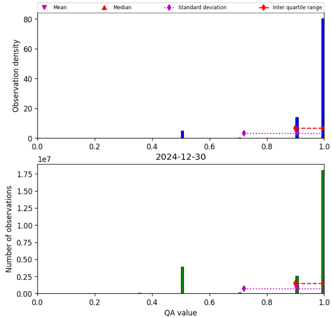
Figure 29: Histogram of “QA value” for 2024-12-29 to 2024-12-31
