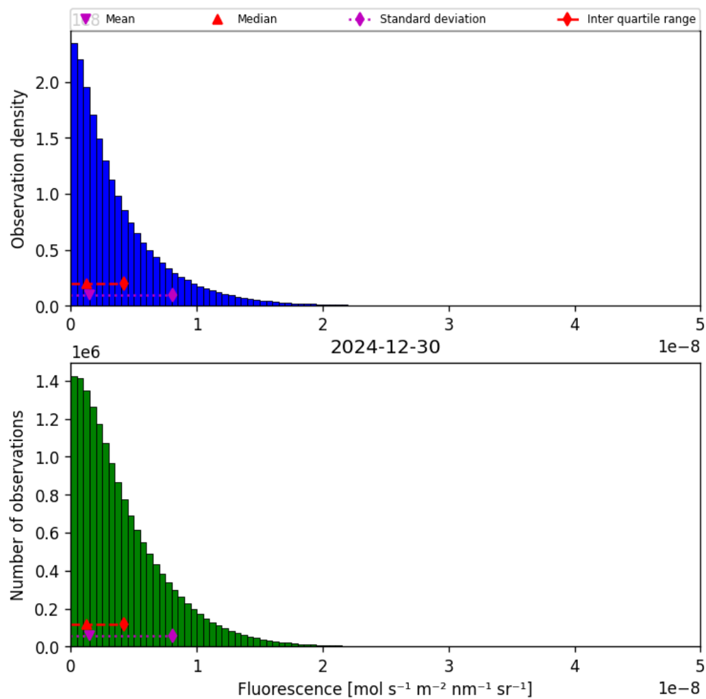
Figure 40: Histogram of “Fluorescence” for 2024-12-29 to 2024-12-31
