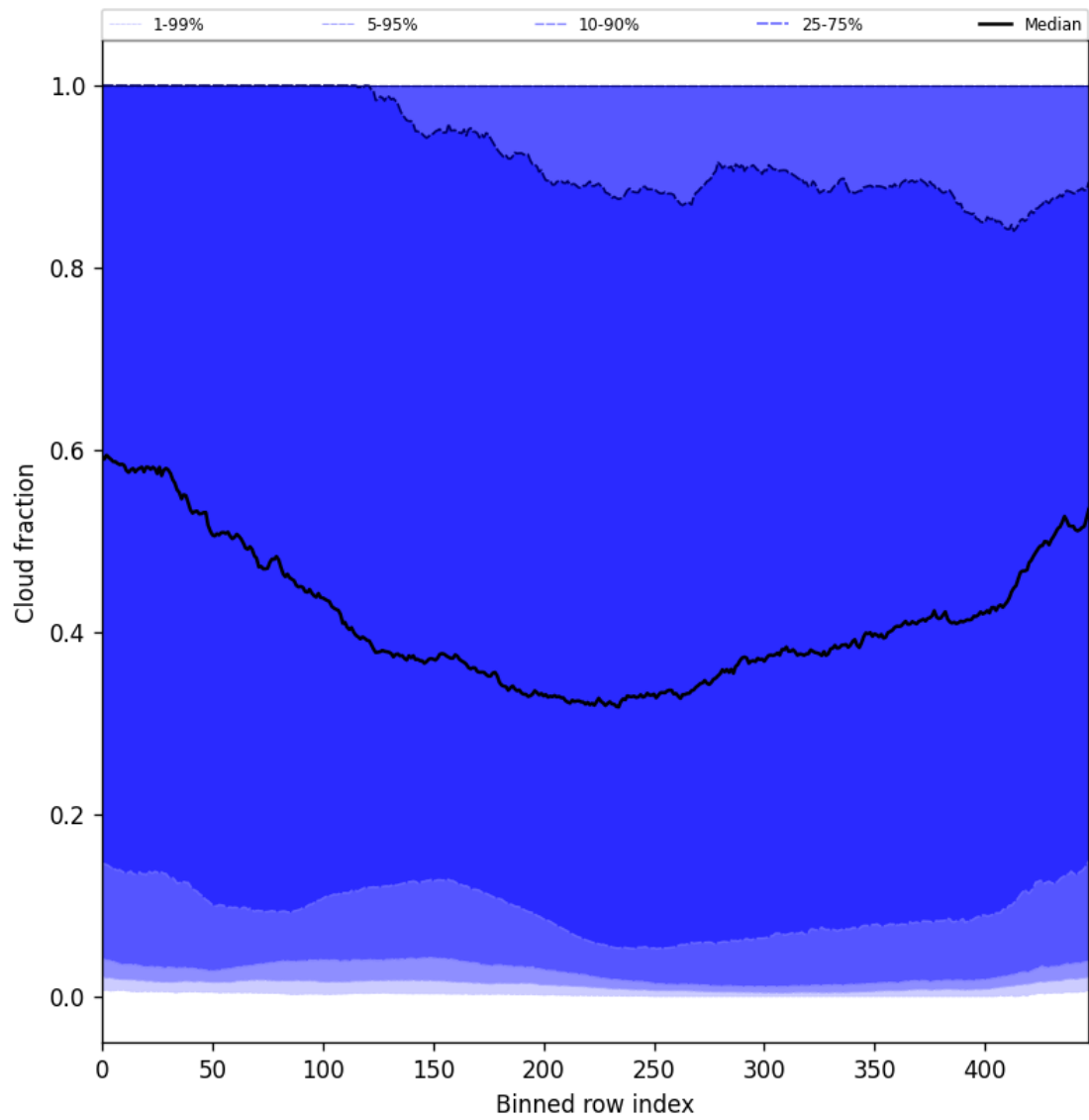
Figure 49: Along track statistics of “Cloud fraction” for 2024-12-29 to 2024-12-31
