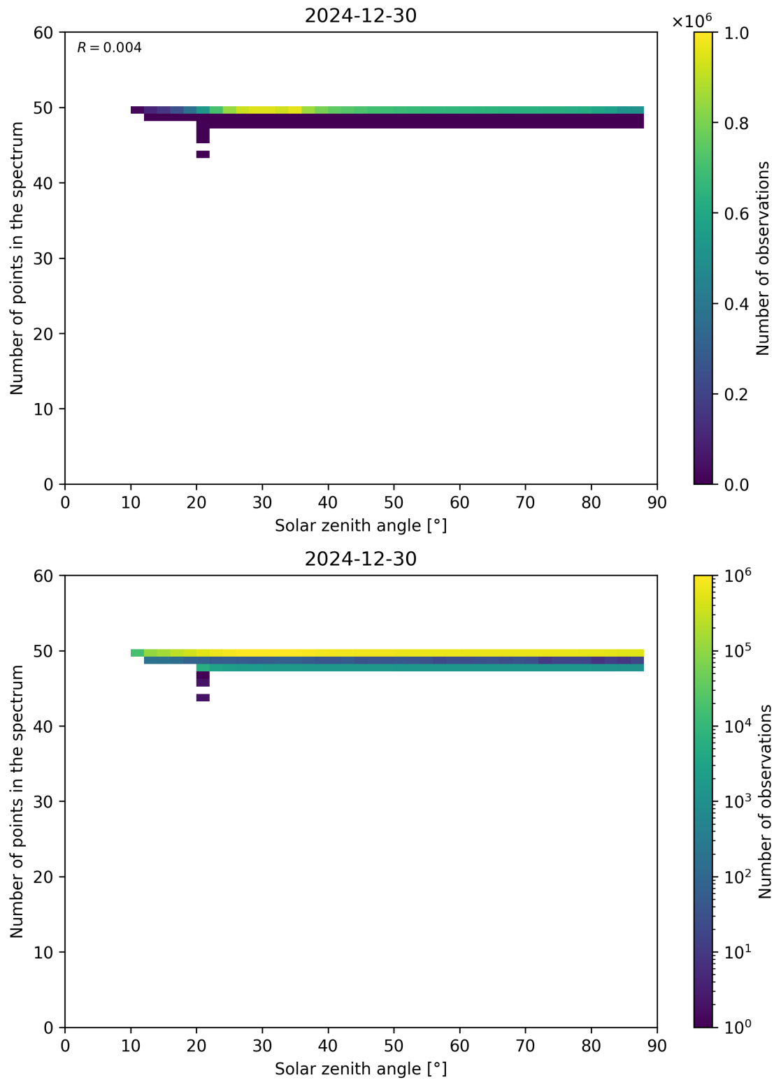
Figure 115: Scatter density plot of “Solar zenith angle” against “Number of points in the spectrum” for 2024-12-29 to 2024-12-31.
