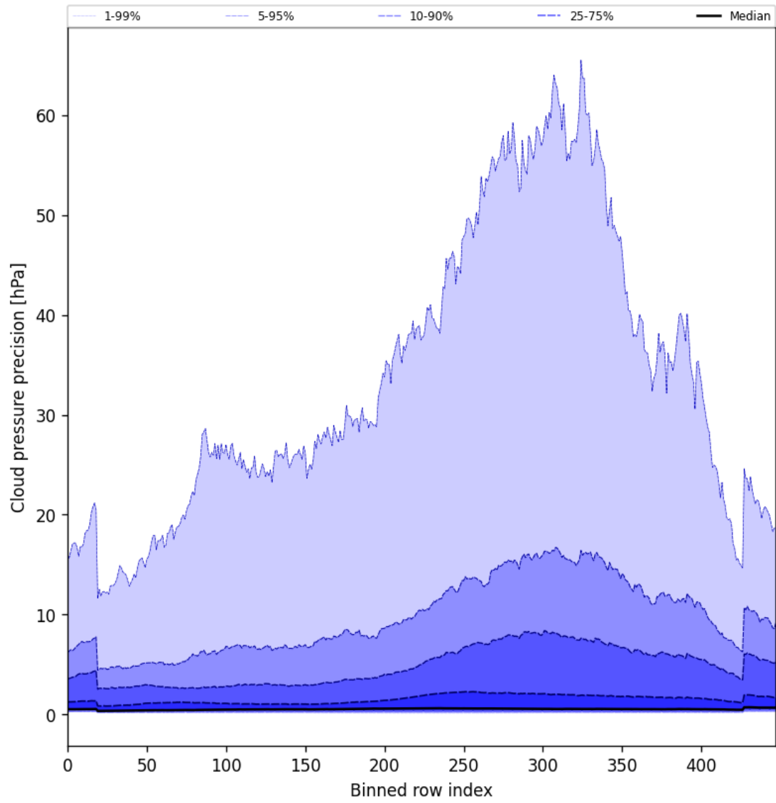
Figure 48: Along track statistics of “Cloud pressure precision” for 2024-12-29 to 2024-12-31
