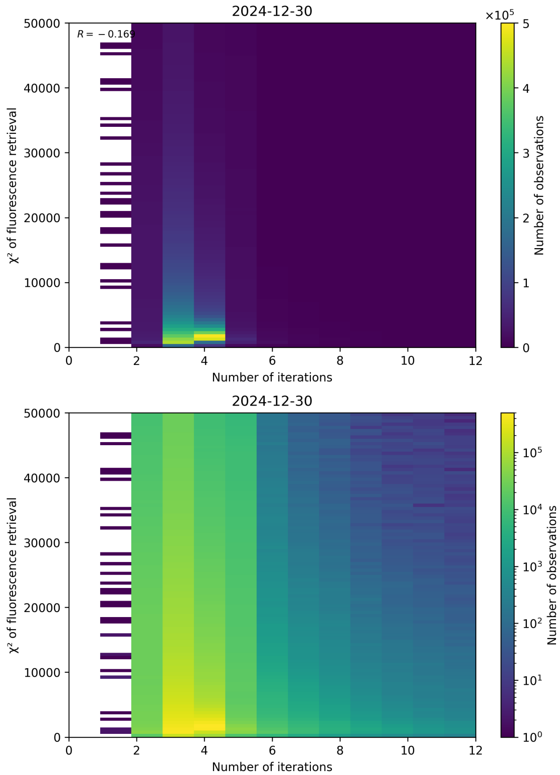
Figure 97: Scatter density plot of “Number of iterations” against “ \chi^2 of fluorescence retrieval” for 2024-12-29 to 2024-12-31.
