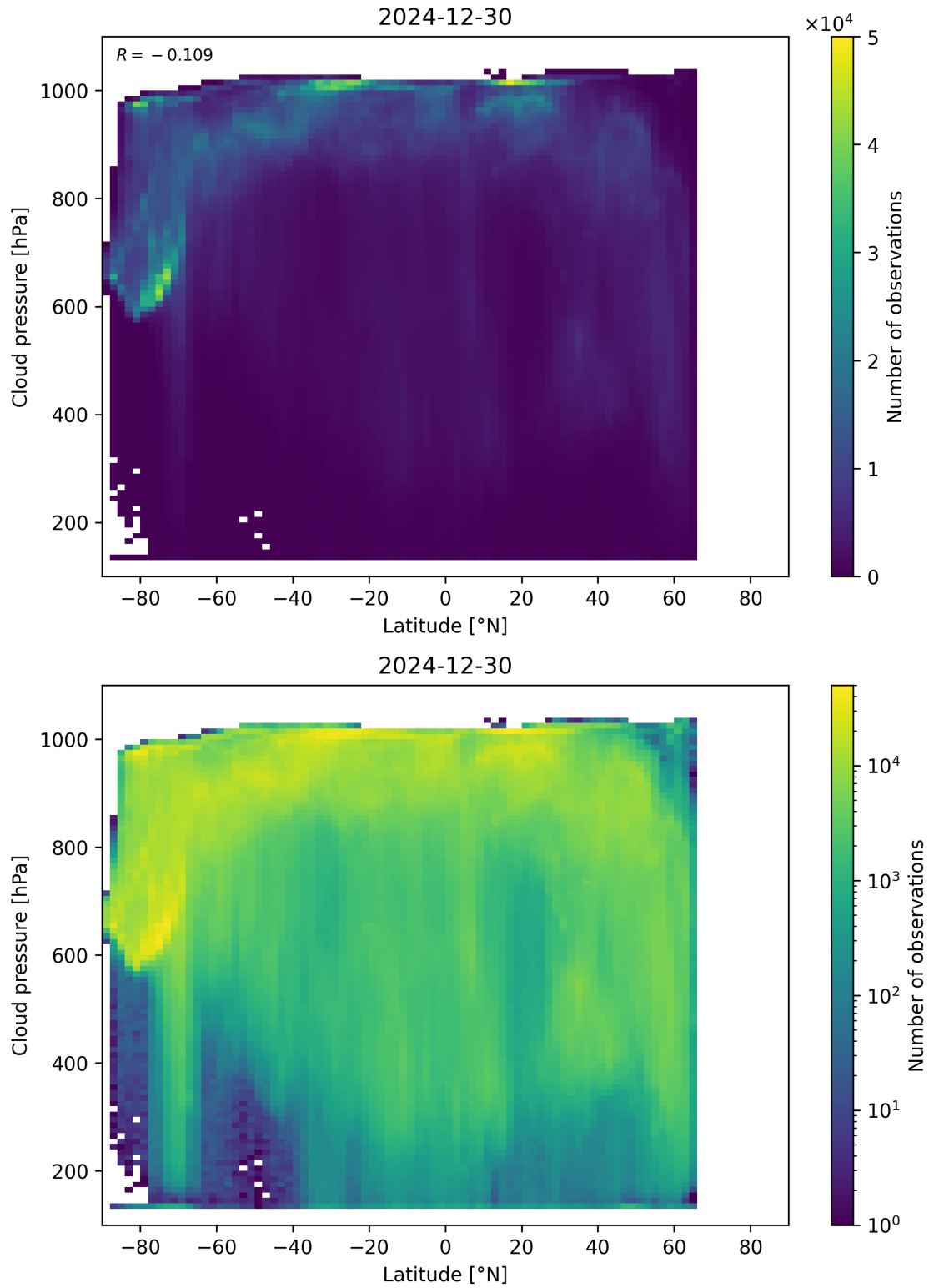
Figure 91: Scatter density plot of “Latitude” against “Cloud pressure” for 2024-12-29 to 2024-12-31.
