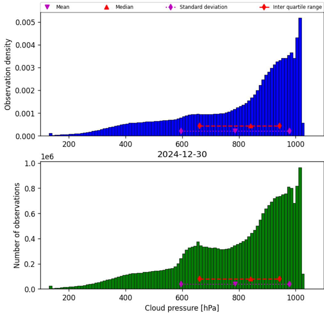
Figure 30: Histogram of “Cloud pressure” for 2024-12-29 to 2024-12-31
