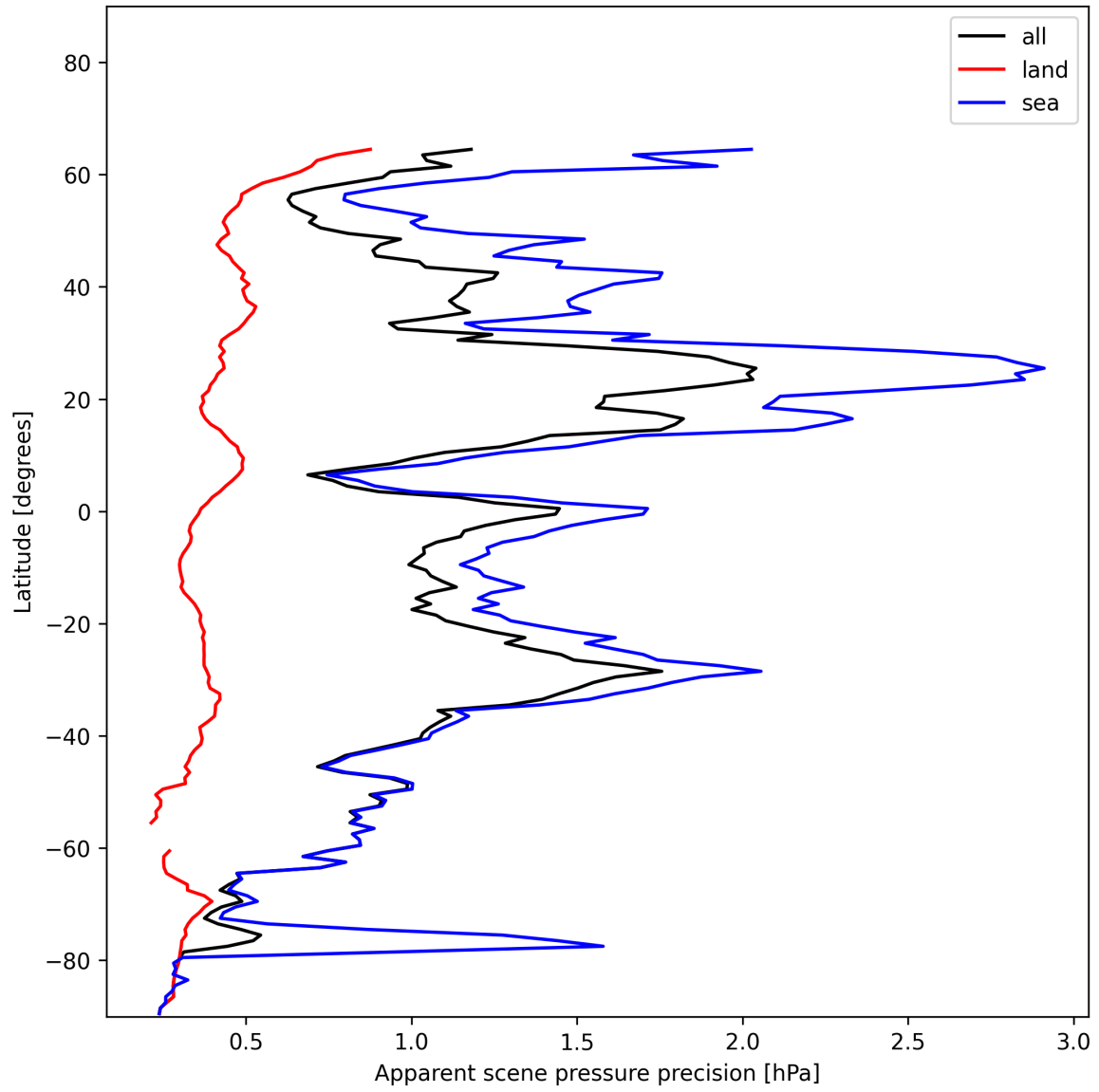
Figure 20: Zonal average of “Apparent scene pressure precision” for 2024-12-29 to 2024-12-31.
