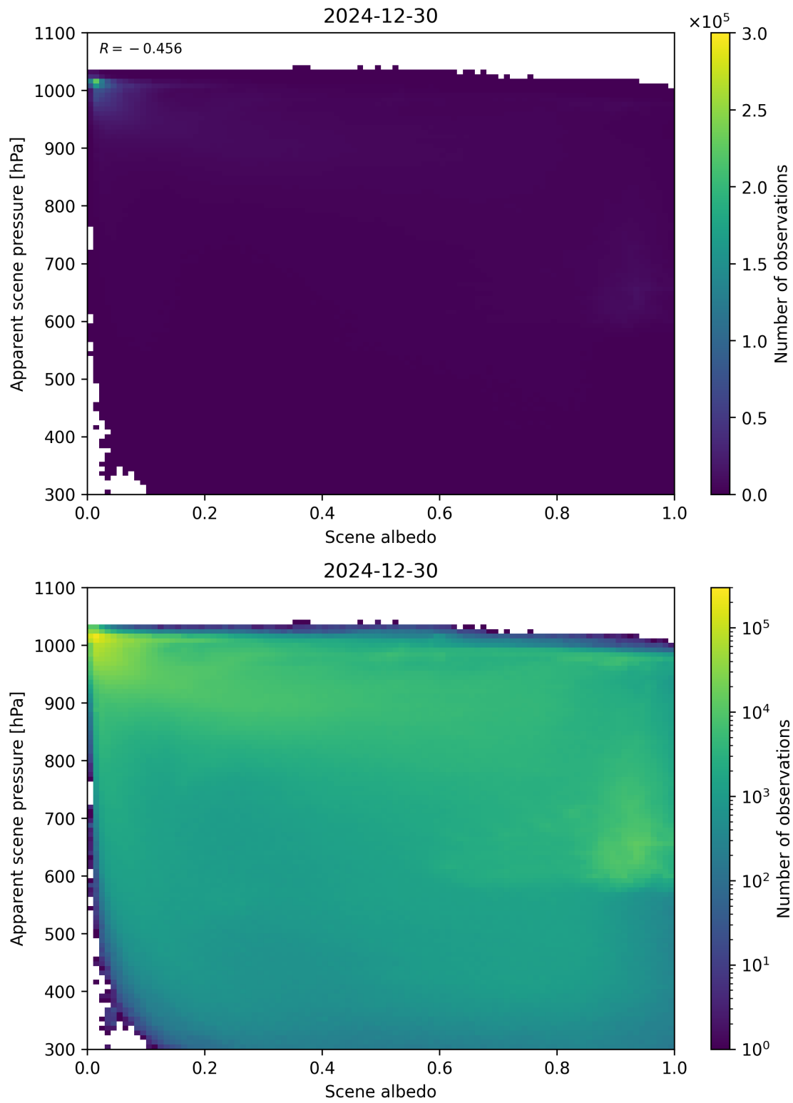
Figure 102: Scatter density plot of “Scene albedo” against “Apparent scene pressure” for 2024-12-29 to 2024-12-31.
