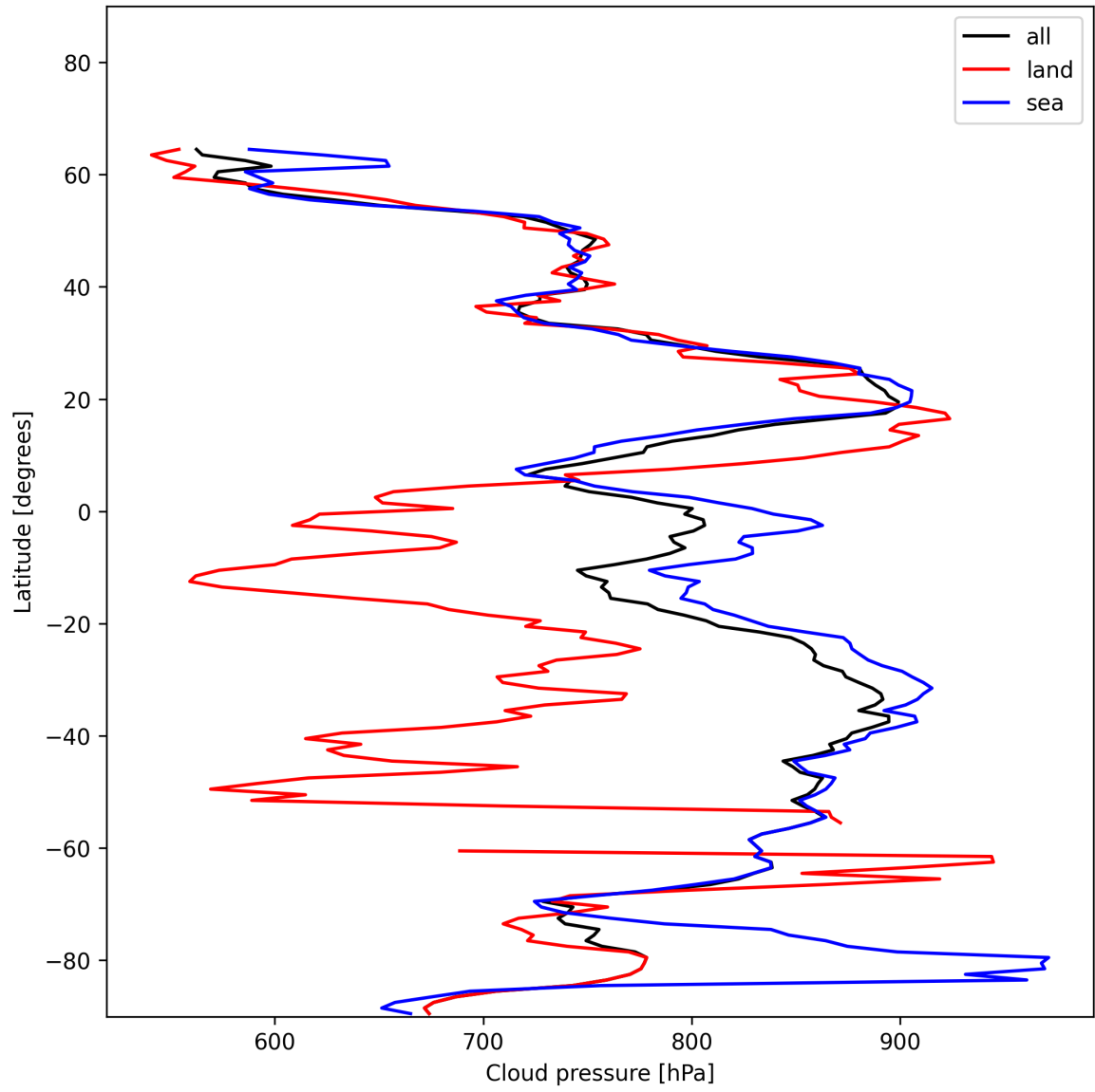
Figure 13: Zonal average of “Cloud pressure” for 2024-12-29 to 2024-12-31.
