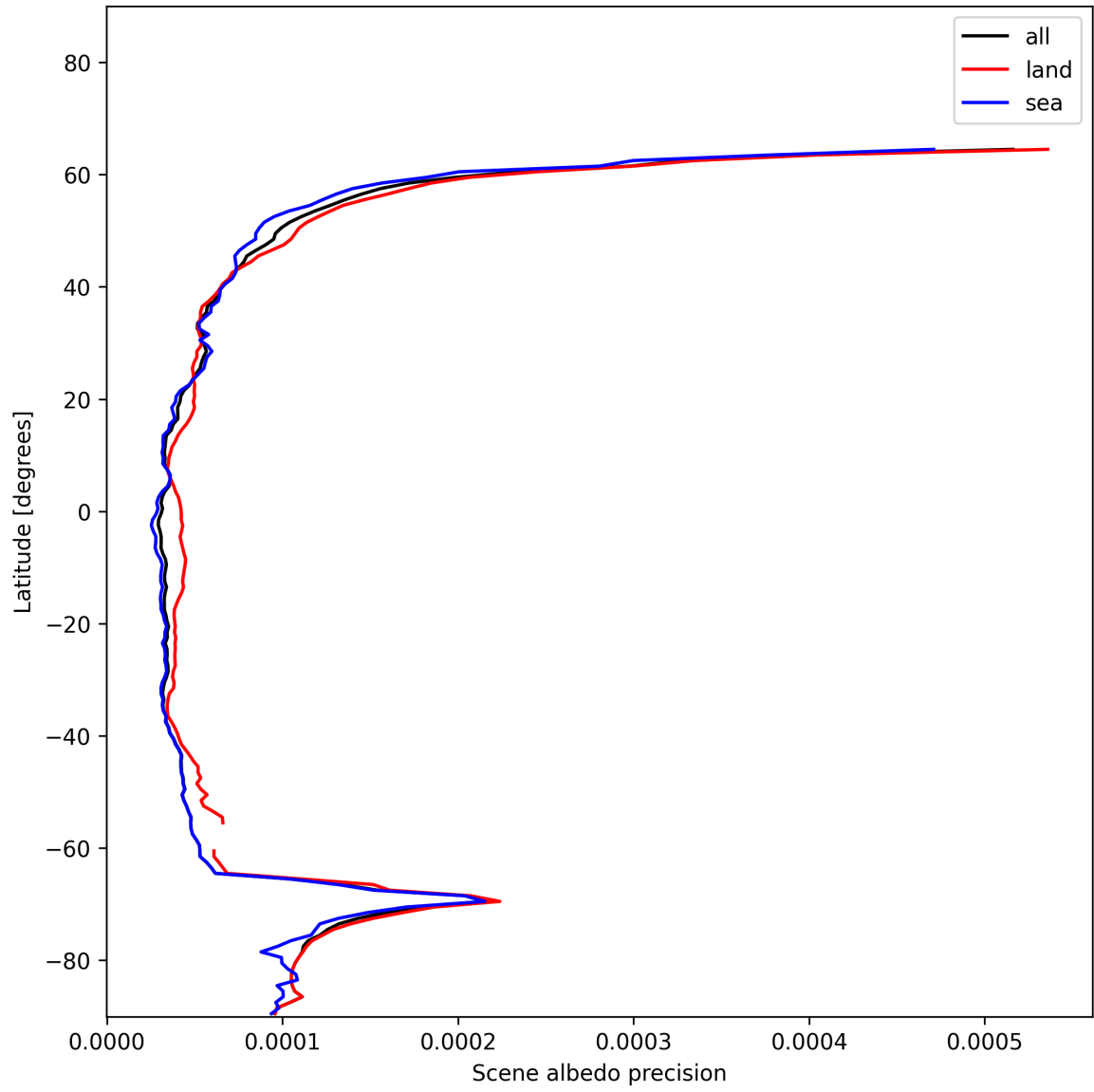
Figure 18: Zonal average of “Scene albedo precision” for 2024-12-29 to 2024-12-31.
