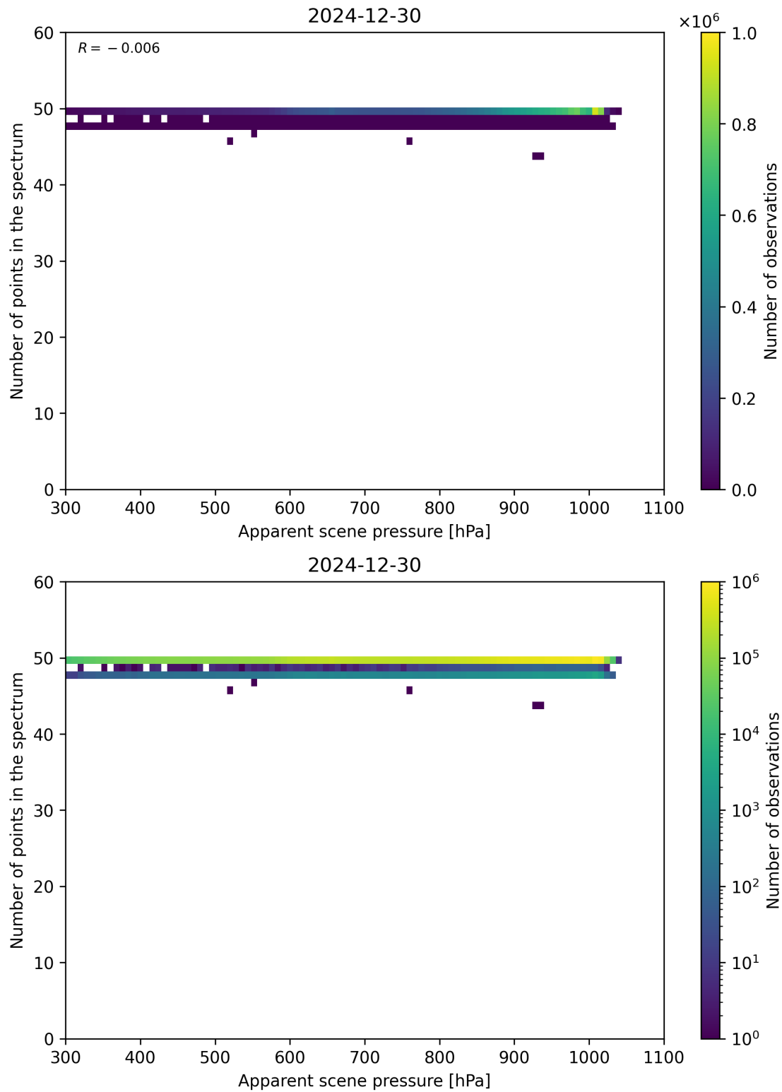
Figure 66: Scatter density plot of “Apparent scene pressure” against “Number of points in the spectrum” for 2024-12-29 to 2024-12-31.
