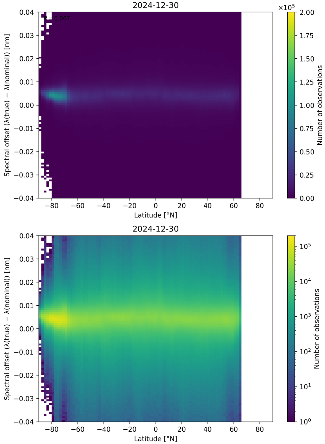
Figure 96: Scatter density plot of “Latitude” against “Spectral offset ( \lambda_{\text{true}} - \lambda_{\text{nominal}} )” for 2024-12-29 to 2024-12-31.
