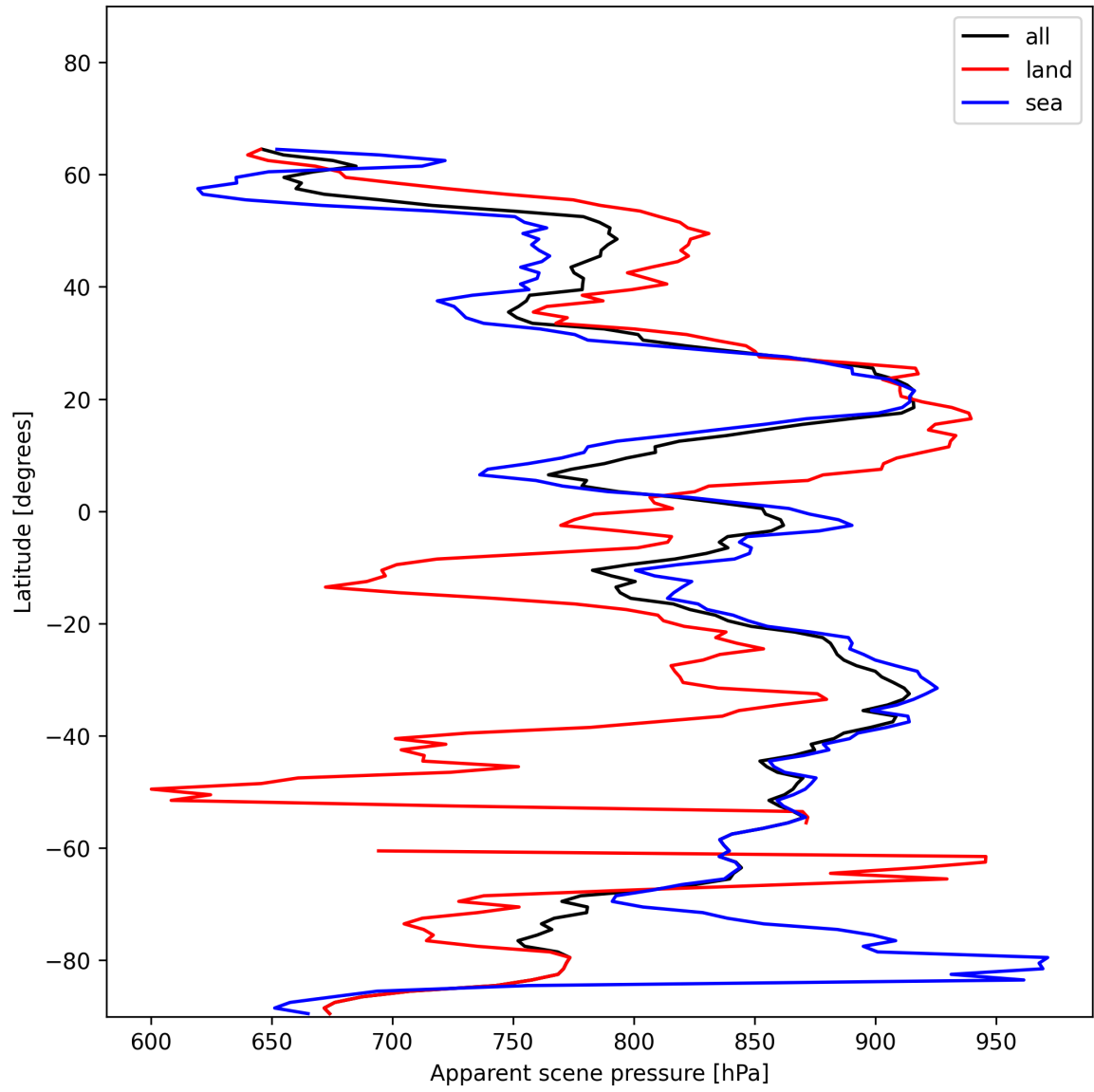
Figure 19: Zonal average of “Apparent scene pressure” for 2024-12-29 to 2024-12-31.
