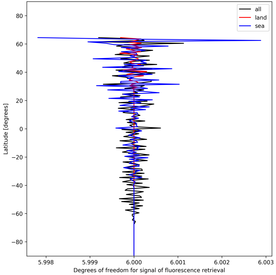
Figure 26: Zonal average of “Degrees of freedom for signal of fluorescence retrieval” for 2024-12-29 to 2024-12-31.
