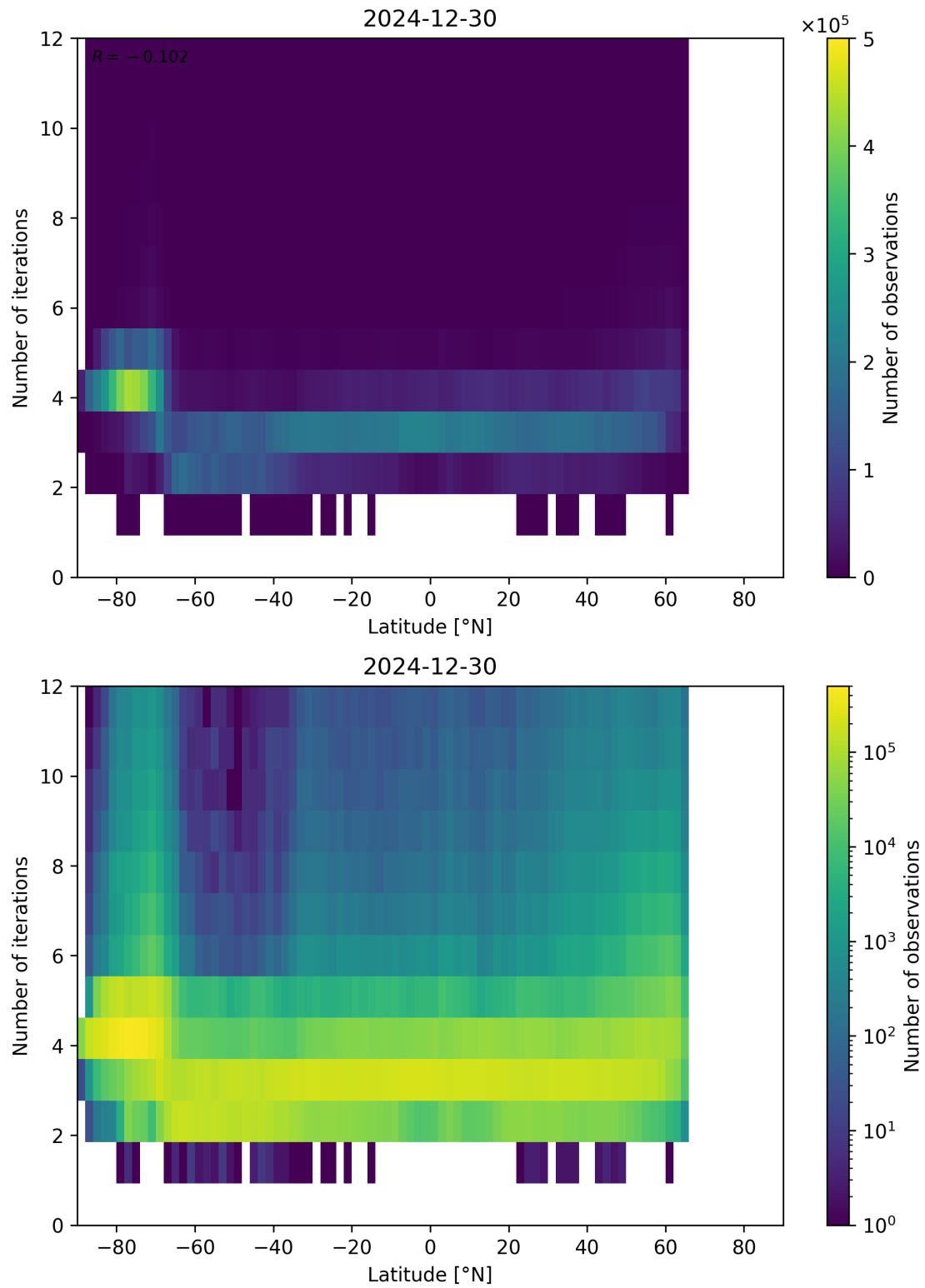
Figure 93: Scatter density plot of “Latitude” against “Number of iterations” for 2024-12-29 to 2024-12-31.
