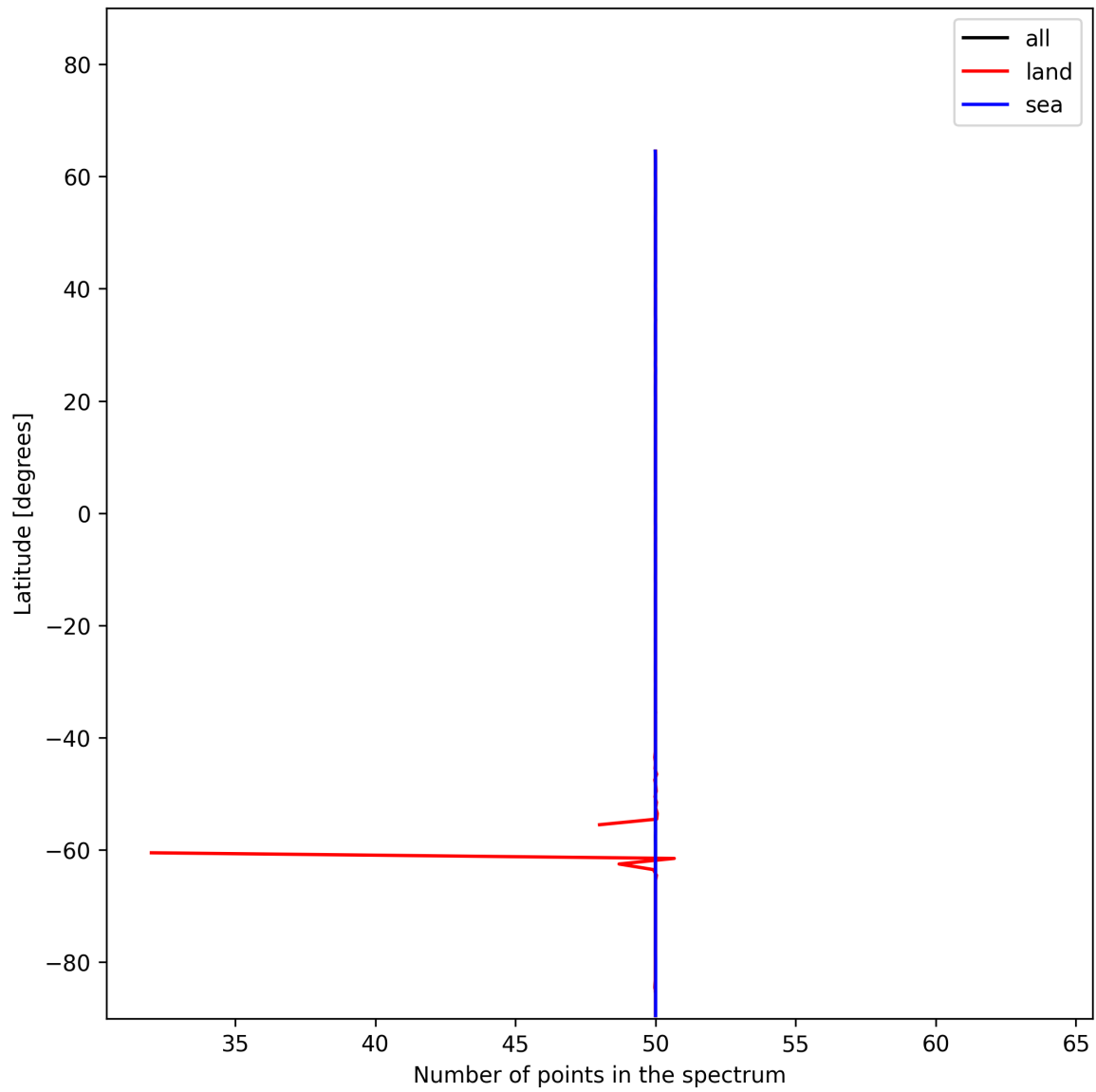
Figure 27: Zonal average of “Number of points in the spectrum” for 2024-12-29 to 2024-12-31.
