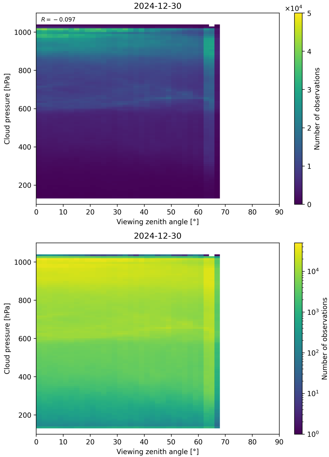
Figure 121: Scatter density plot of “Viewing zenith angle” against “Cloud pressure” for 2024-12-29 to 2024-12-31.
