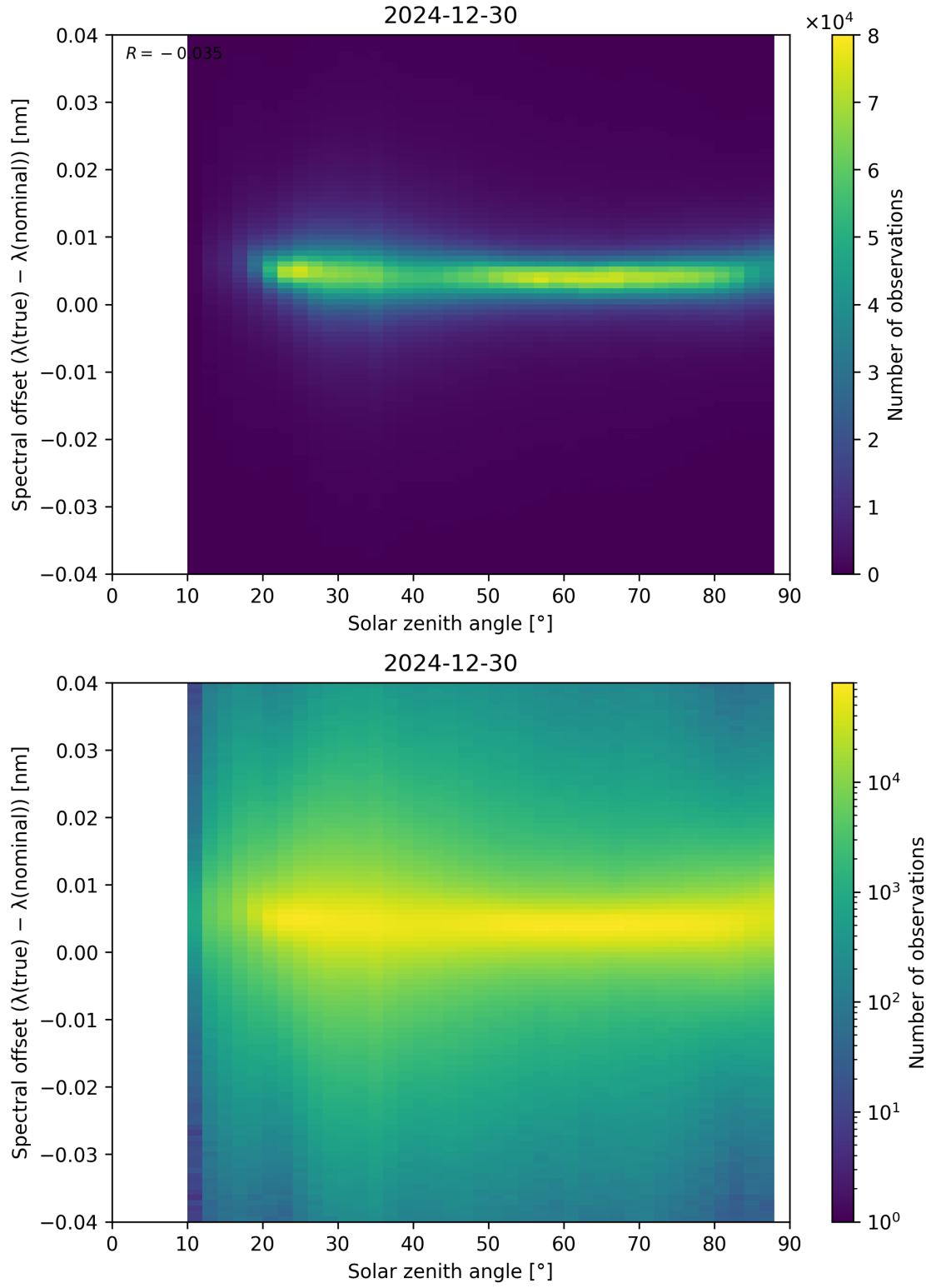
Figure 117: Scatter density plot of “Solar zenith angle” against “Spectral offset ( \lambda_{\text{true}} - \lambda_{\text{nominal}} )” for 2024-12-29 to 2024-12-31.
