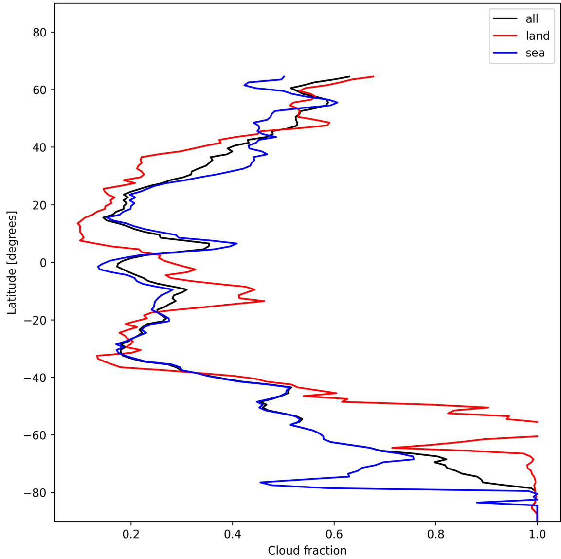
Figure 15: Zonal average of “Cloud fraction” for 2024-12-29 to 2024-12-31.
