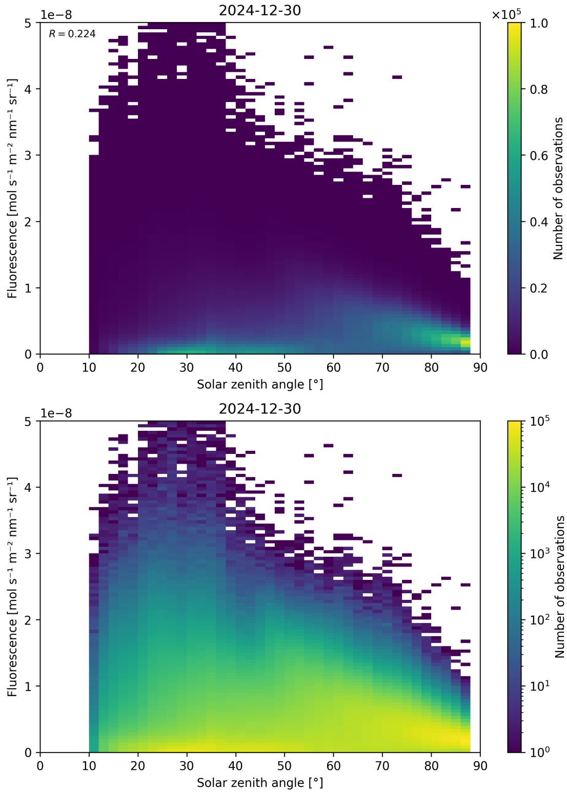
Figure 112: Scatter density plot of “Solar zenith angle” against “Fluorescence” for 2024-12-29 to 2024-12-31.
