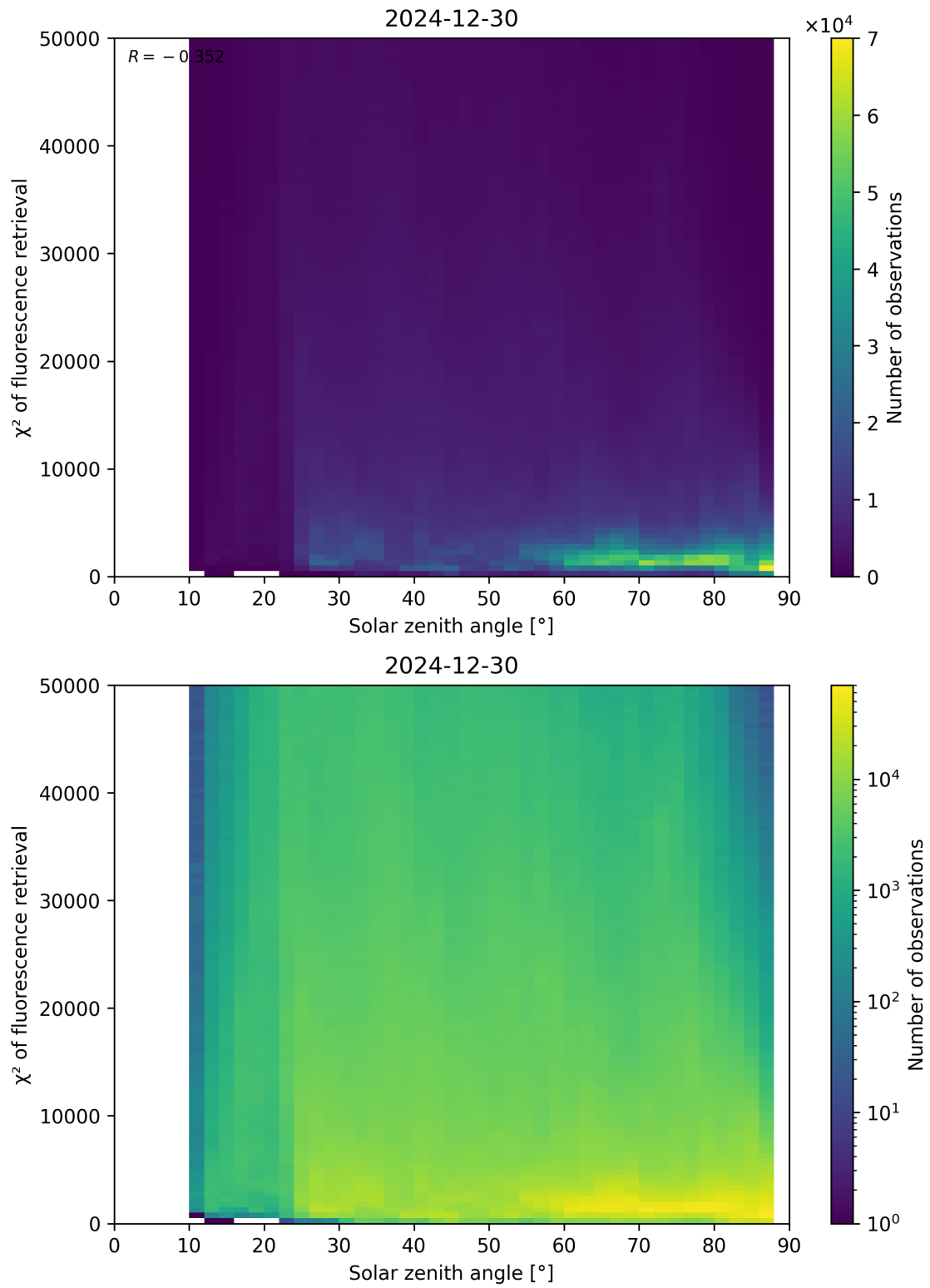
Figure 109: Scatter density plot of “Solar zenith angle” against “ \chi^2 of fluorescence retrieval” for 2024-12-29 to 2024-12-31.
