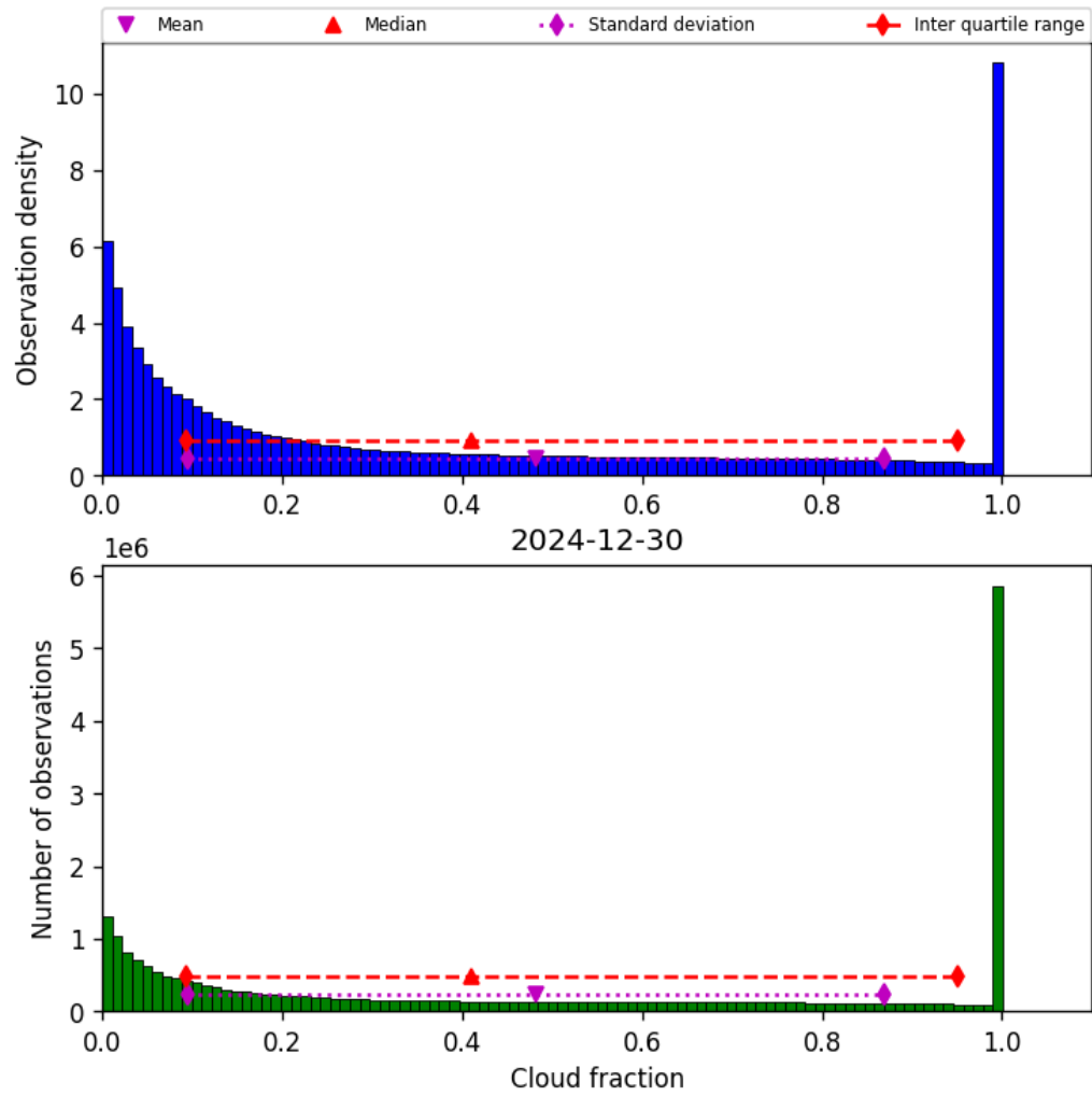
Figure 32: Histogram of “Cloud fraction” for 2024-12-29 to 2024-12-31
