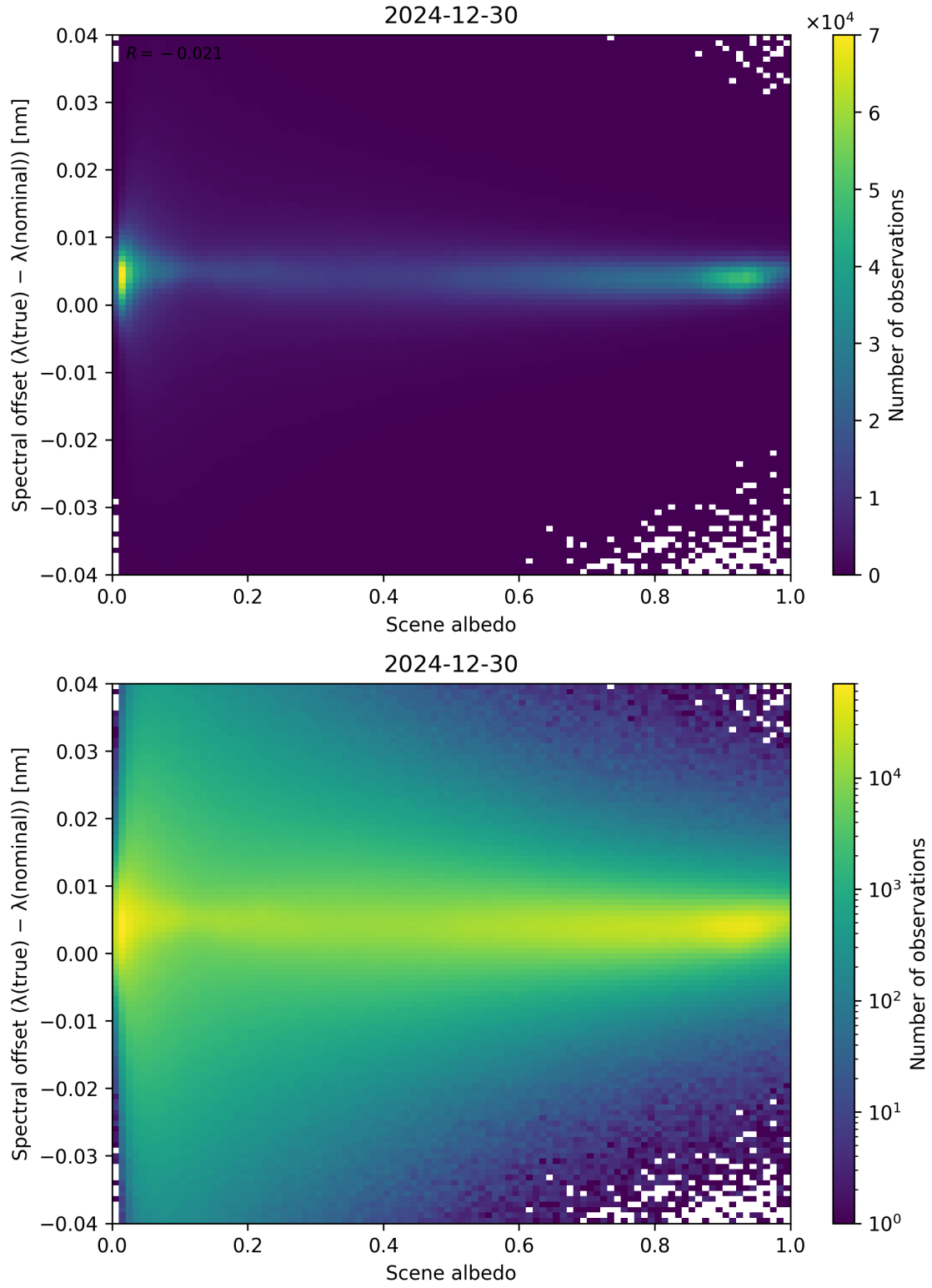
Figure 107: Scatter density plot of “Scene albedo” against “Spectral offset ( \lambda_{\text{true}} - \lambda_{\text{nominal}} )” for 2024-12-29 to 2024-12-31.
