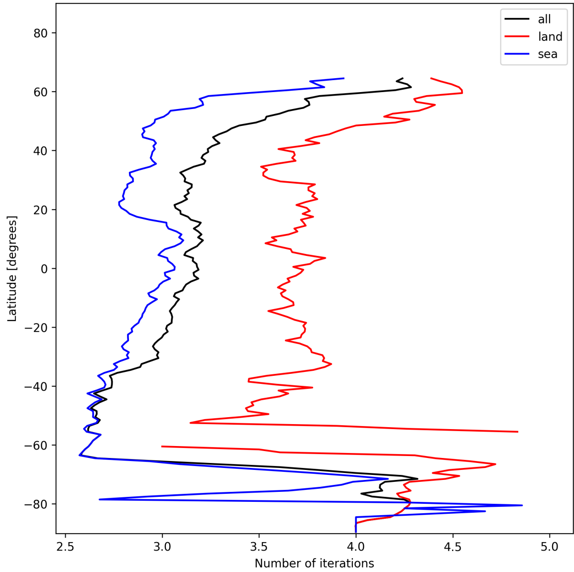
Figure 22: Zonal average of “Number of iterations” for 2024-12-29 to 2024-12-31.
