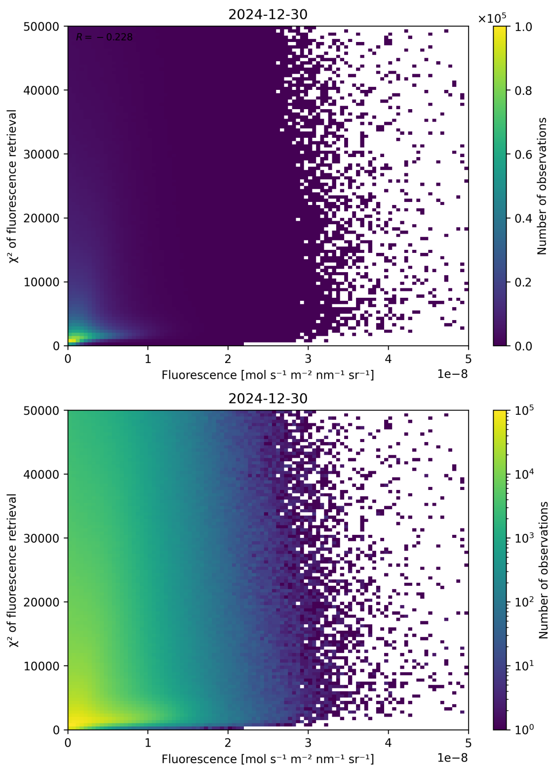
Figure 85: Scatter density plot of “Fluorescence” against “ \chi^2 of fluorescence retrieval” for 2024-12-29 to 2024-12-31.
