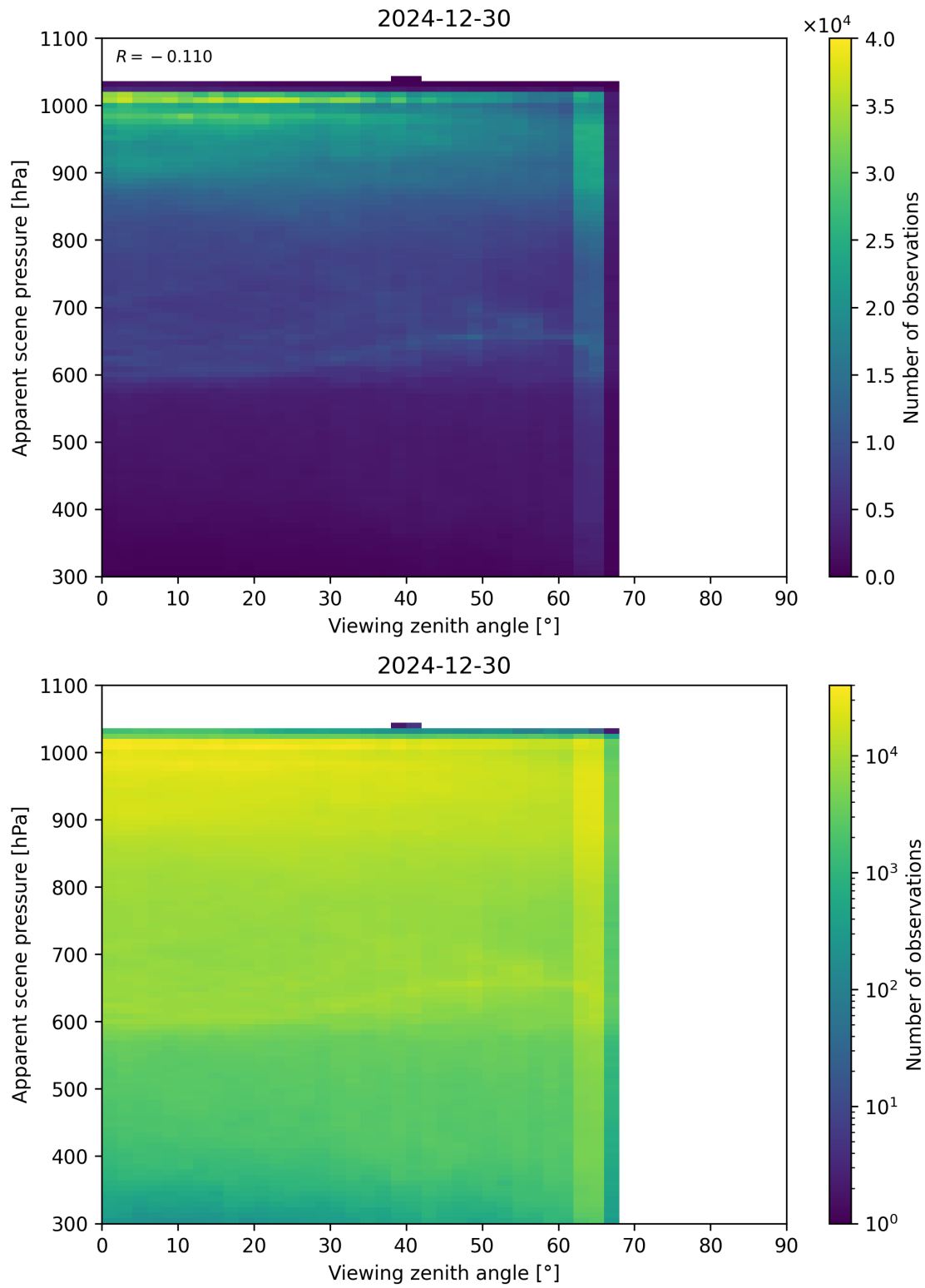
Figure 118: Scatter density plot of “Viewing zenith angle” against “Apparent scene pressure” for 2024-12-29 to 2024-12-31.
