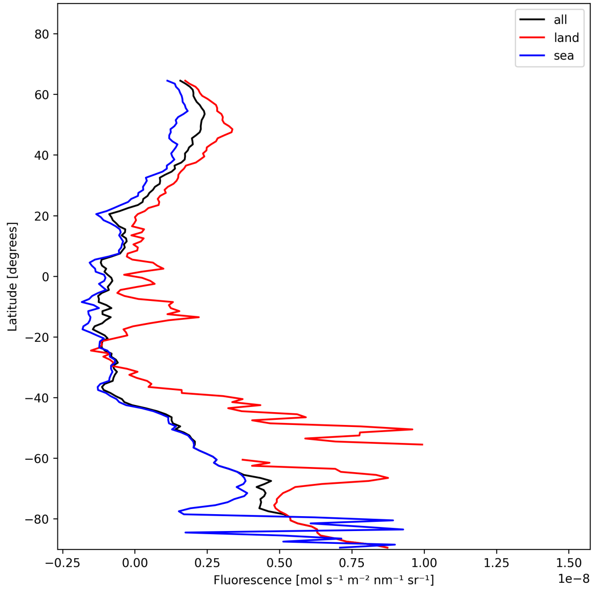
Figure 23: Zonal average of “Fluorescence” for 2024-12-29 to 2024-12-31.
