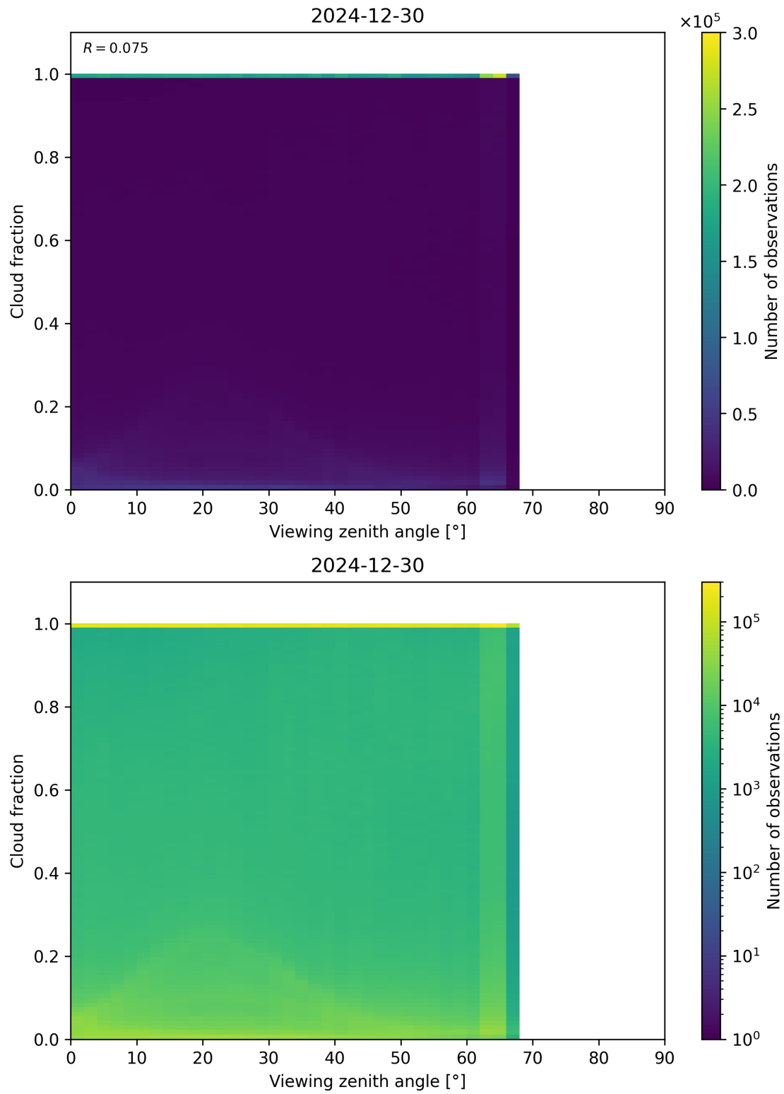
Figure 120: Scatter density plot of “Viewing zenith angle” against “Cloud fraction” for 2024-12-29 to 2024-12-31.
