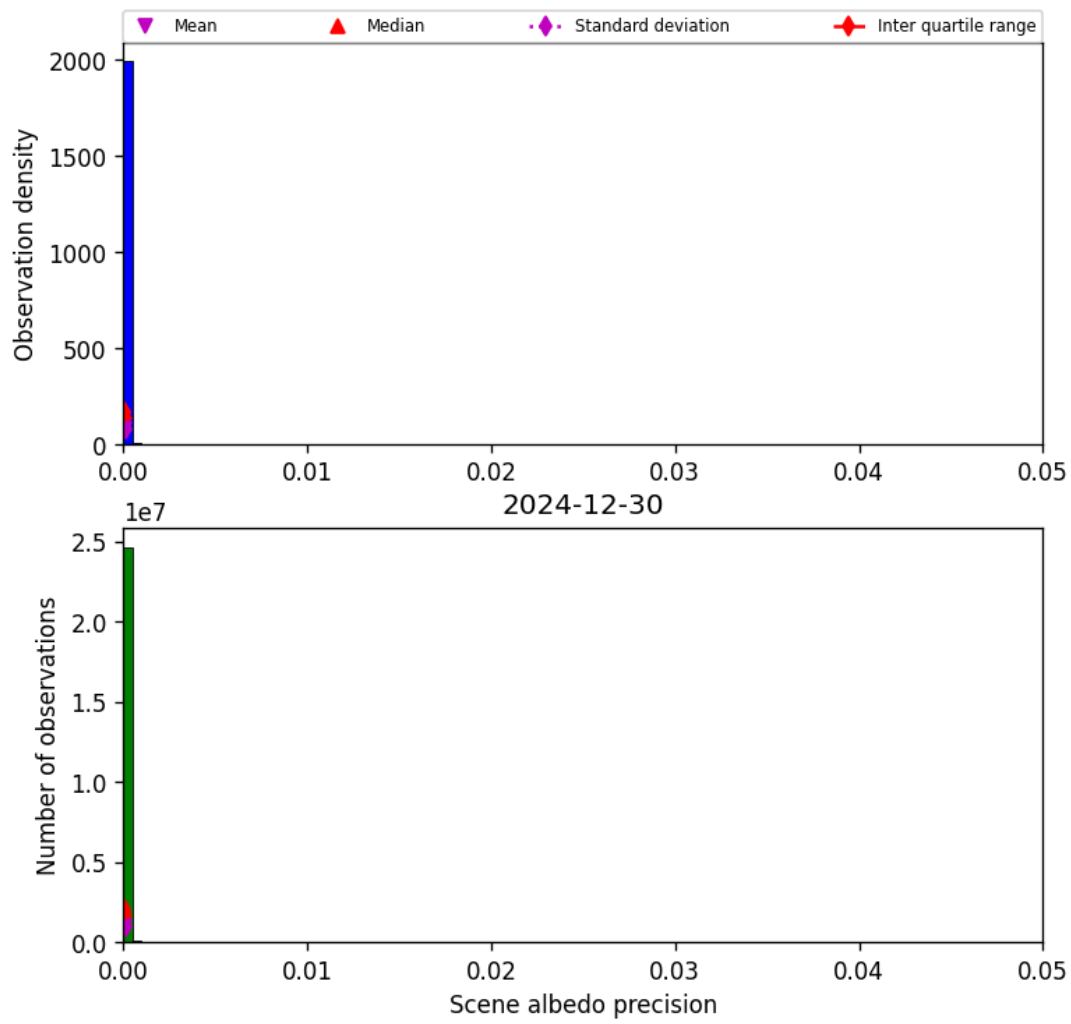
Figure 35: Histogram of “Scene albedo precision” for 2024-12-29 to 2024-12-31
