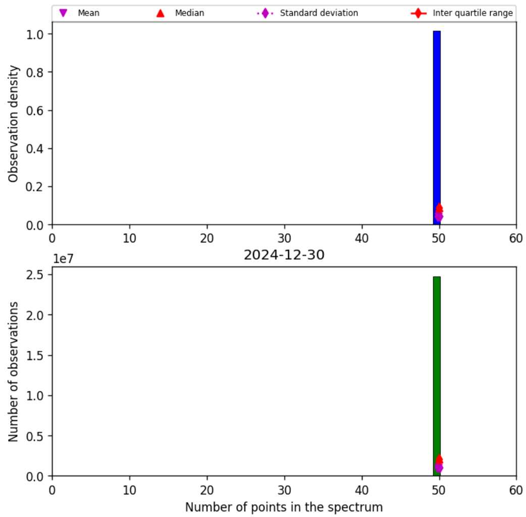
Figure 44: Histogram of "Number of points in the spectrum" for 2024-12-29 to 2024-12-31
