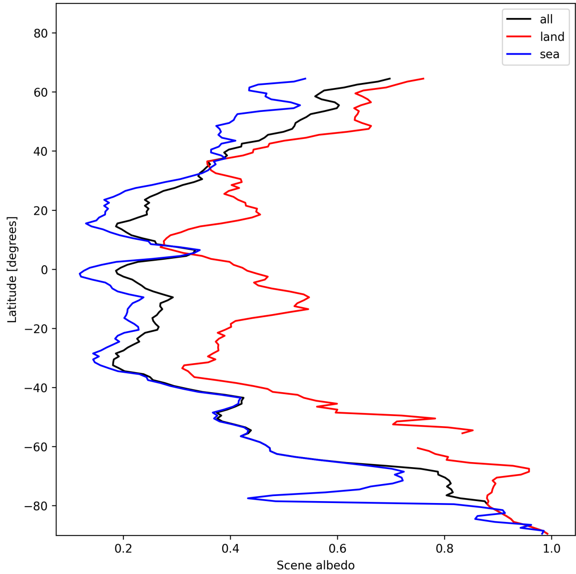
Figure 17: Zonal average of “Scene albedo” for 2024-12-29 to 2024-12-31.
