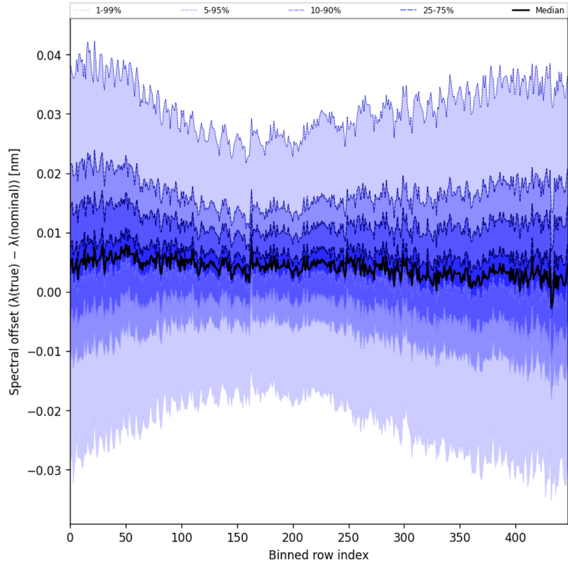
Figure 62: Along track statistics of “Spectral offset ( \lambda_{\text{true}} - \lambda_{\text{nominal}} )” for 2024-12-29 to 2024-12-31
