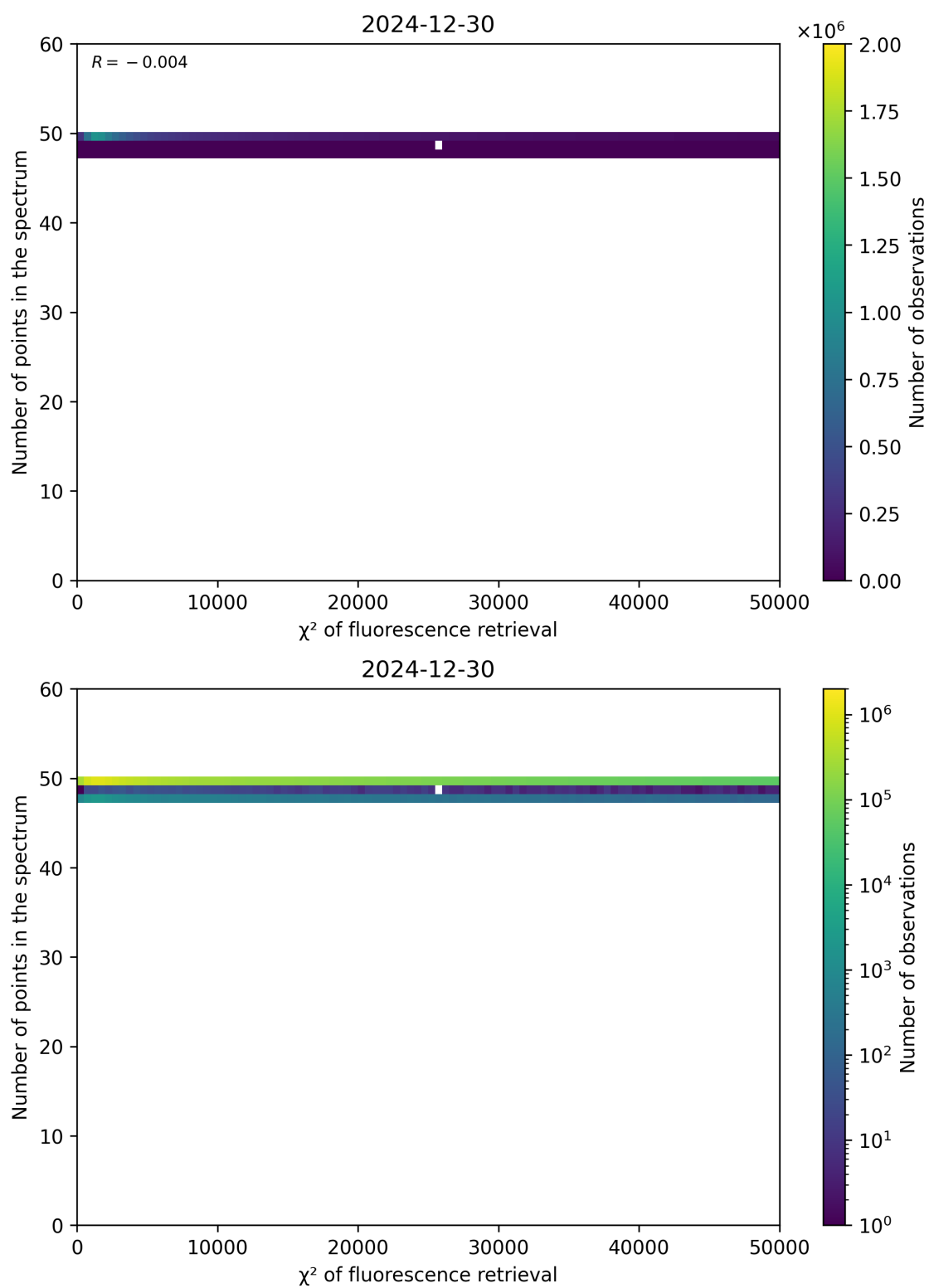
Figure 68: Scatter density plot of “ \chi^2 of fluorescence retrieval” against “Number of points in the spectrum” for 2024-12-29 to 2024-12-31.
