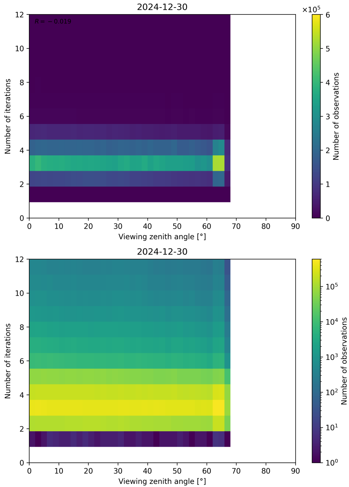
Figure 124: Scatter density plot of “Viewing zenith angle” against “Number of iterations” for 2024-12-29 to 2024-12-31.
