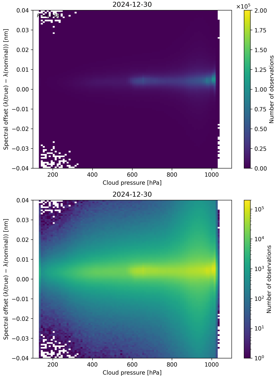
Figure 84: Scatter density plot of “Cloud pressure” against “Spectral offset ( \lambda_{\text{true}} - \lambda_{\text{nominal}} )” for 2024-12-29 to 2024-12-31.
