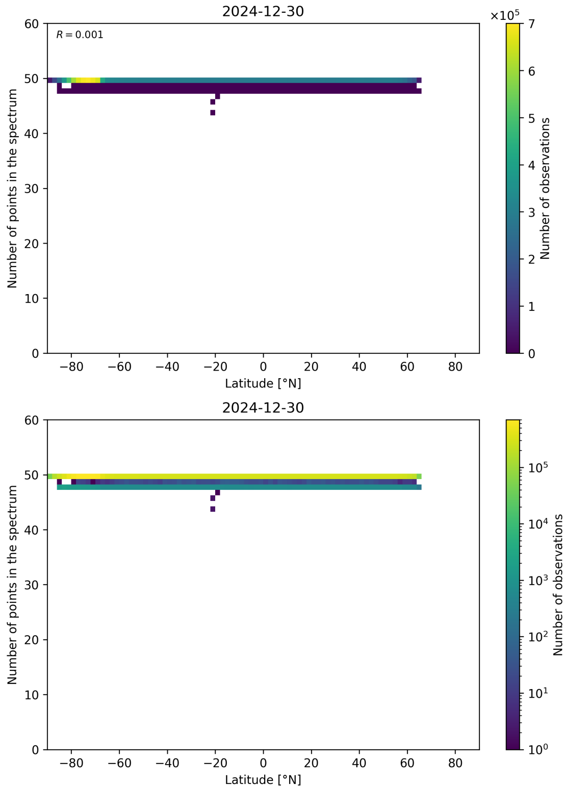
Figure 94: Scatter density plot of “Latitude” against “Number of points in the spectrum” for 2024-12-29 to 2024-12-31.
