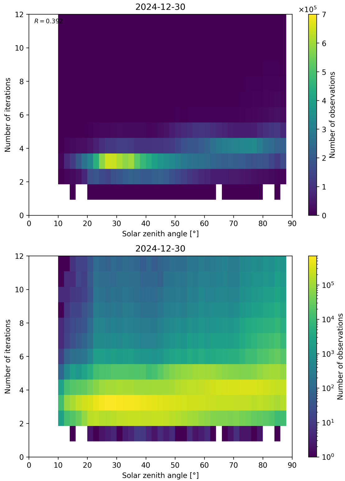
Figure 114: Scatter density plot of “Solar zenith angle” against “Number of iterations” for 2024-12-29 to 2024-12-31.
