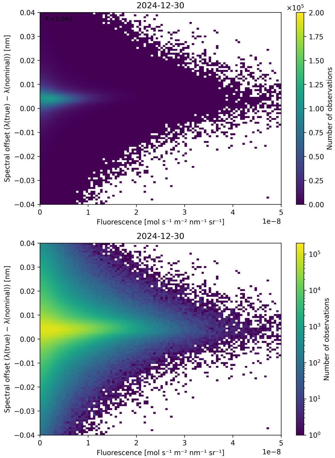
Figure 87: Scatter density plot of “Fluorescence” against “Spectral offset ( \lambda_{\text{true}} - \lambda_{\text{nominal}} )” for 2024-12-29 to 2024-12-31.
