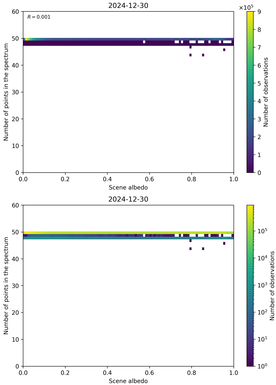
Figure 106: Scatter density plot of “Scene albedo” against “Number of points in the spectrum” for 2024-12-29 to 2024-12-31.
