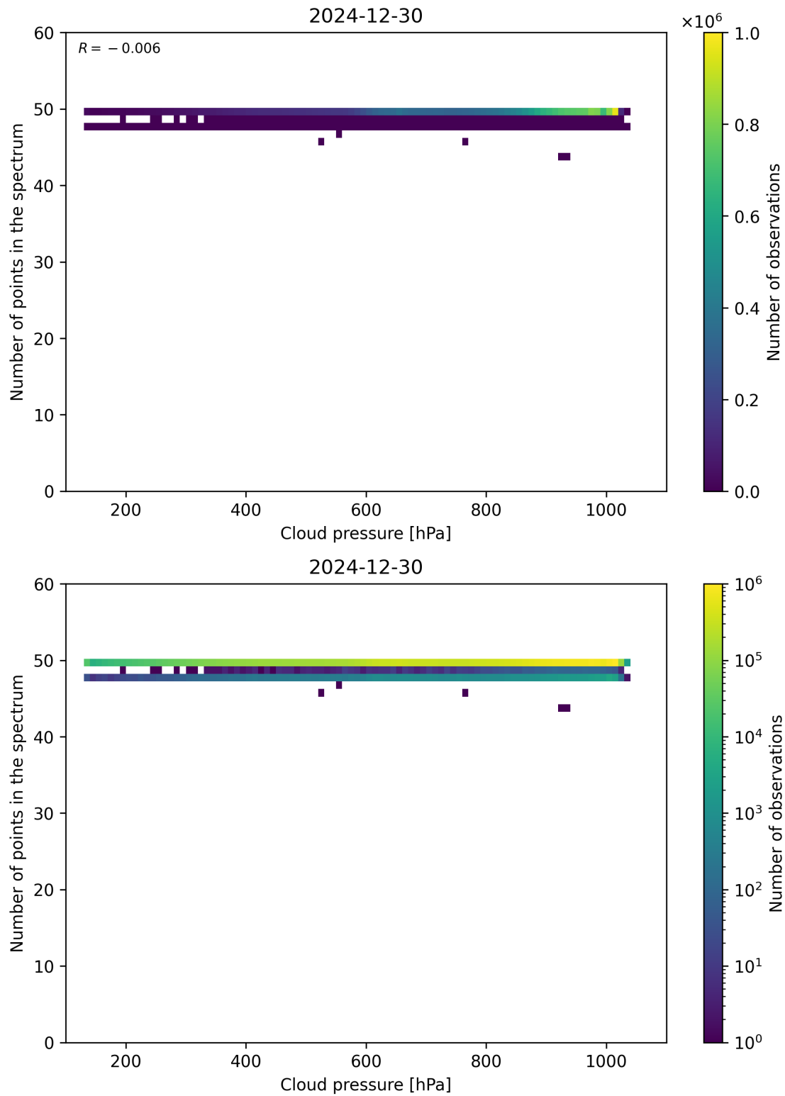
Figure 82: Scatter density plot of “Cloud pressure” against “Number of points in the spectrum” for 2024-12-29 to 2024-12-31.
