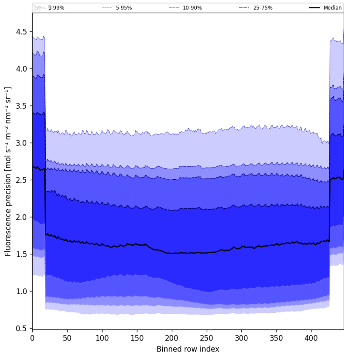
Figure 58: Along track statistics of “Fluorescence precision” for 2024-12-29 to 2024-12-31
