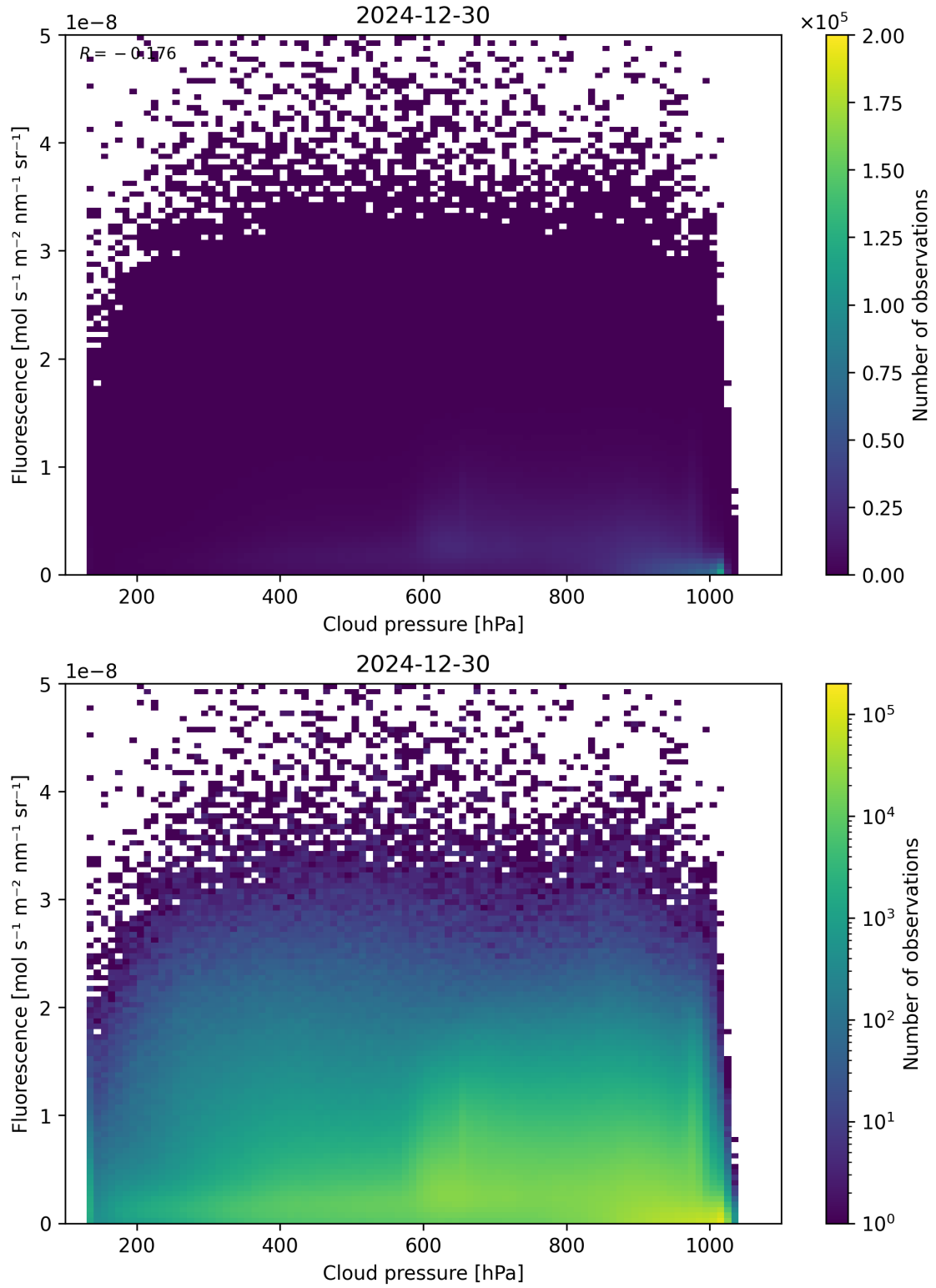
Figure 80: Scatter density plot of “Cloud pressure” against “Fluorescence” for 2024-12-29 to 2024-12-31.
