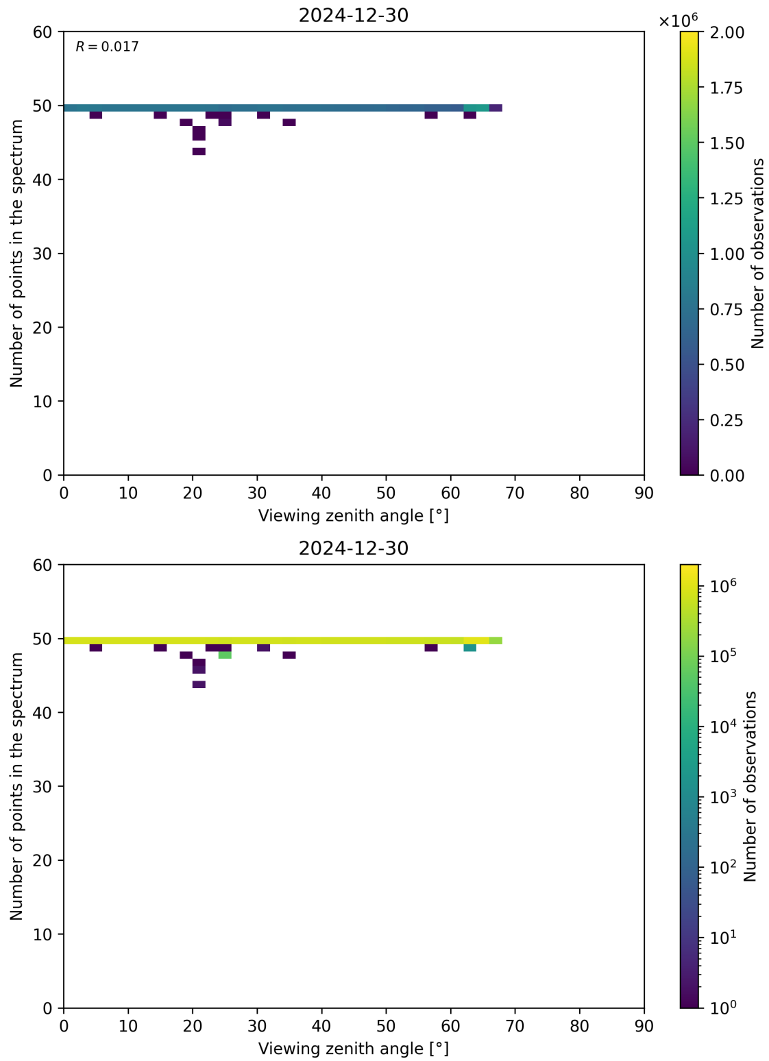
Figure 125: Scatter density plot of “Viewing zenith angle” against “Number of points in the spectrum” for 2024-12-29 to 2024-12-31.
