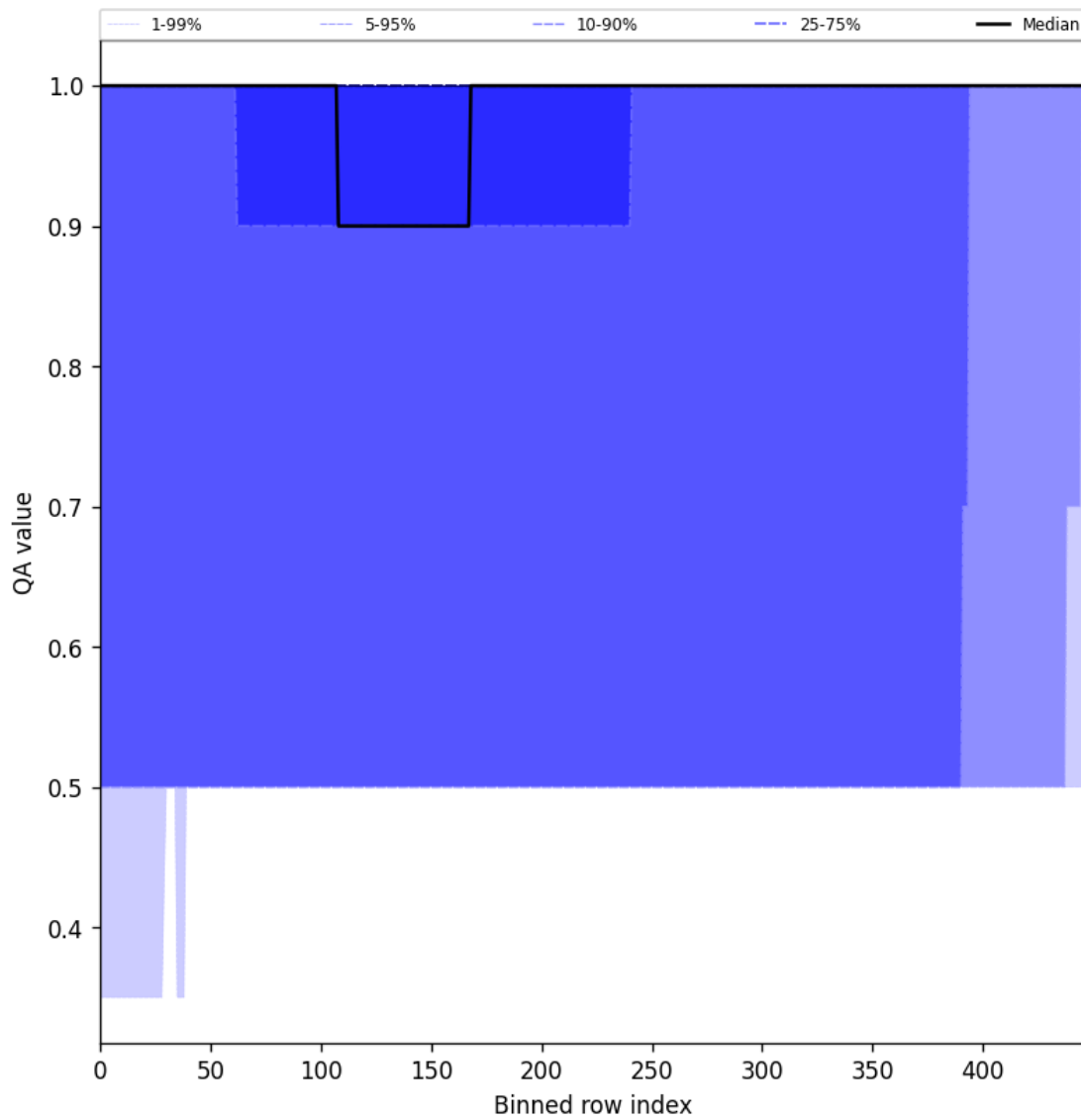
Figure 46: Along track statistics of “QA value” for 2024-12-29 to 2024-12-31
