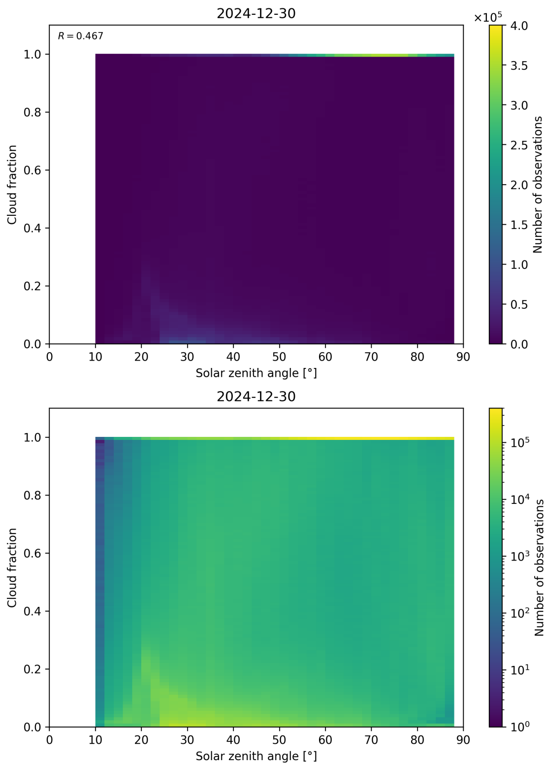
Figure 110: Scatter density plot of “Solar zenith angle” against “Cloud fraction” for 2024-12-29 to 2024-12-31.
