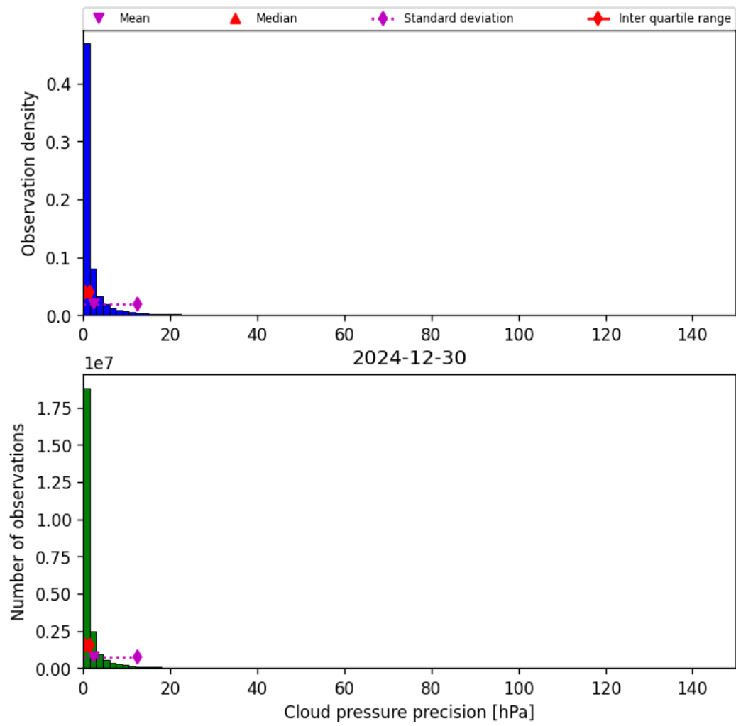
Figure 31: Histogram of “Cloud pressure precision” for 2024-12-29 to 2024-12-31
