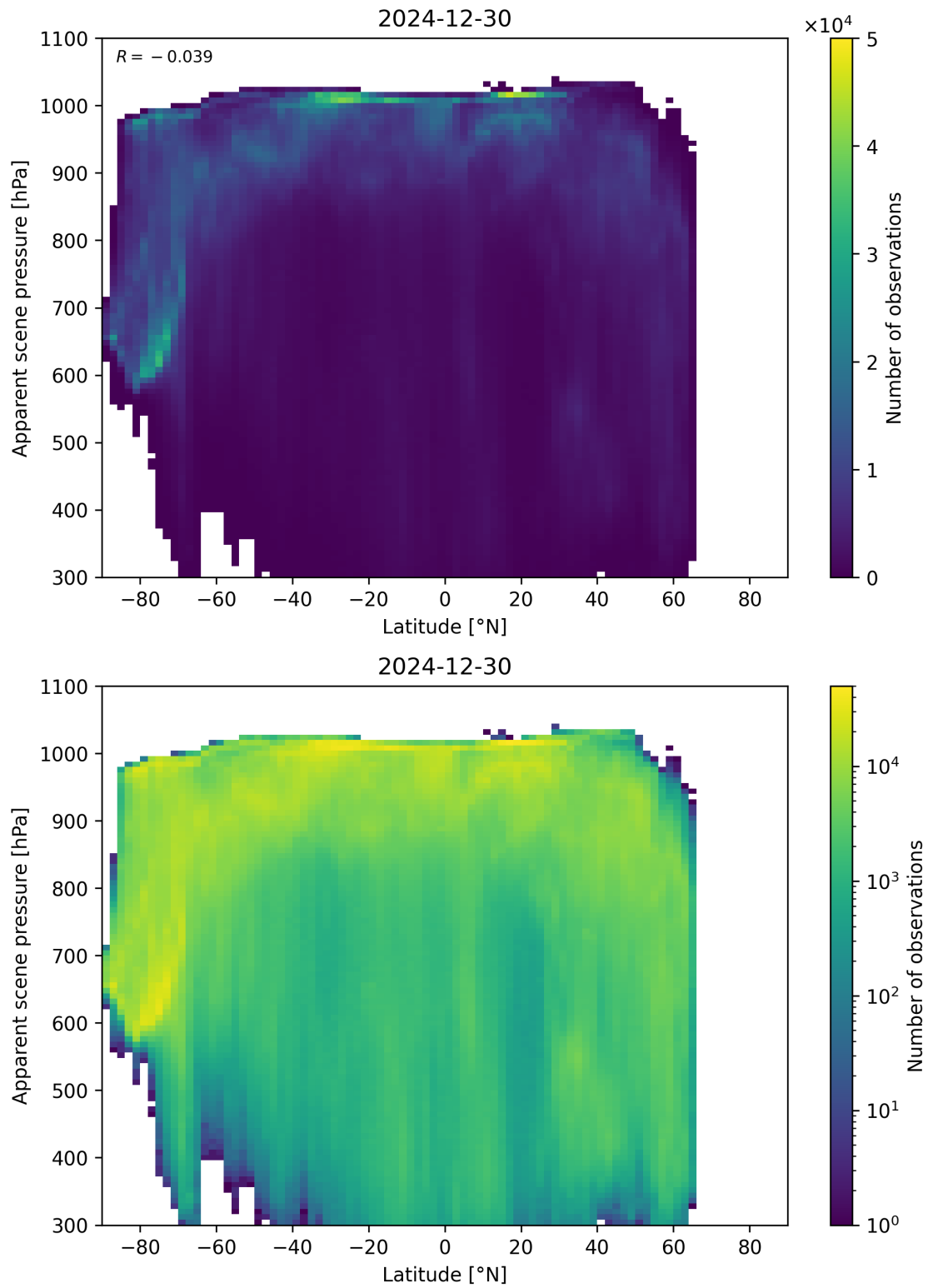
Figure 88: Scatter density plot of “Latitude” against “Apparent scene pressure” for 2024-12-29 to 2024-12-31.
