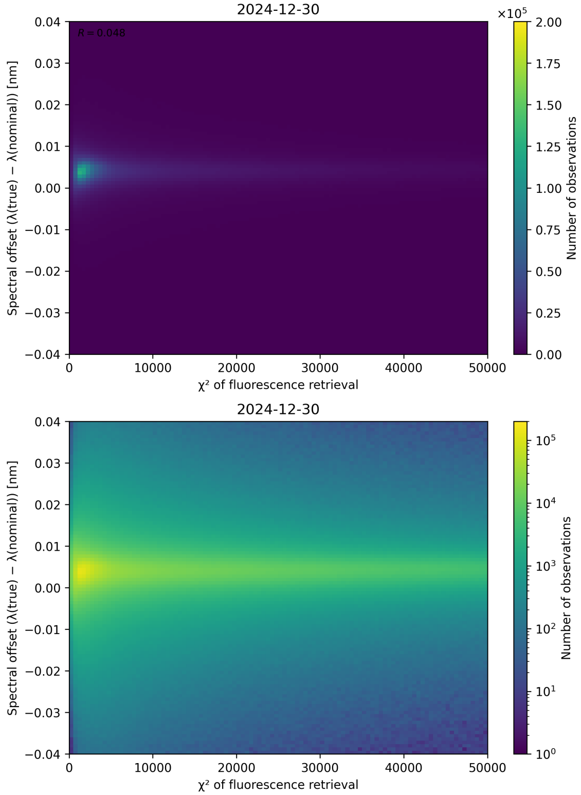
Figure 69: Scatter density plot of “ \chi^2 of fluorescence retrieval” against “Spectral offset ( \lambda_{\text{true}} - \lambda_{\text{nominal}} )” for 2024-12-29 to 2024-12-31.
