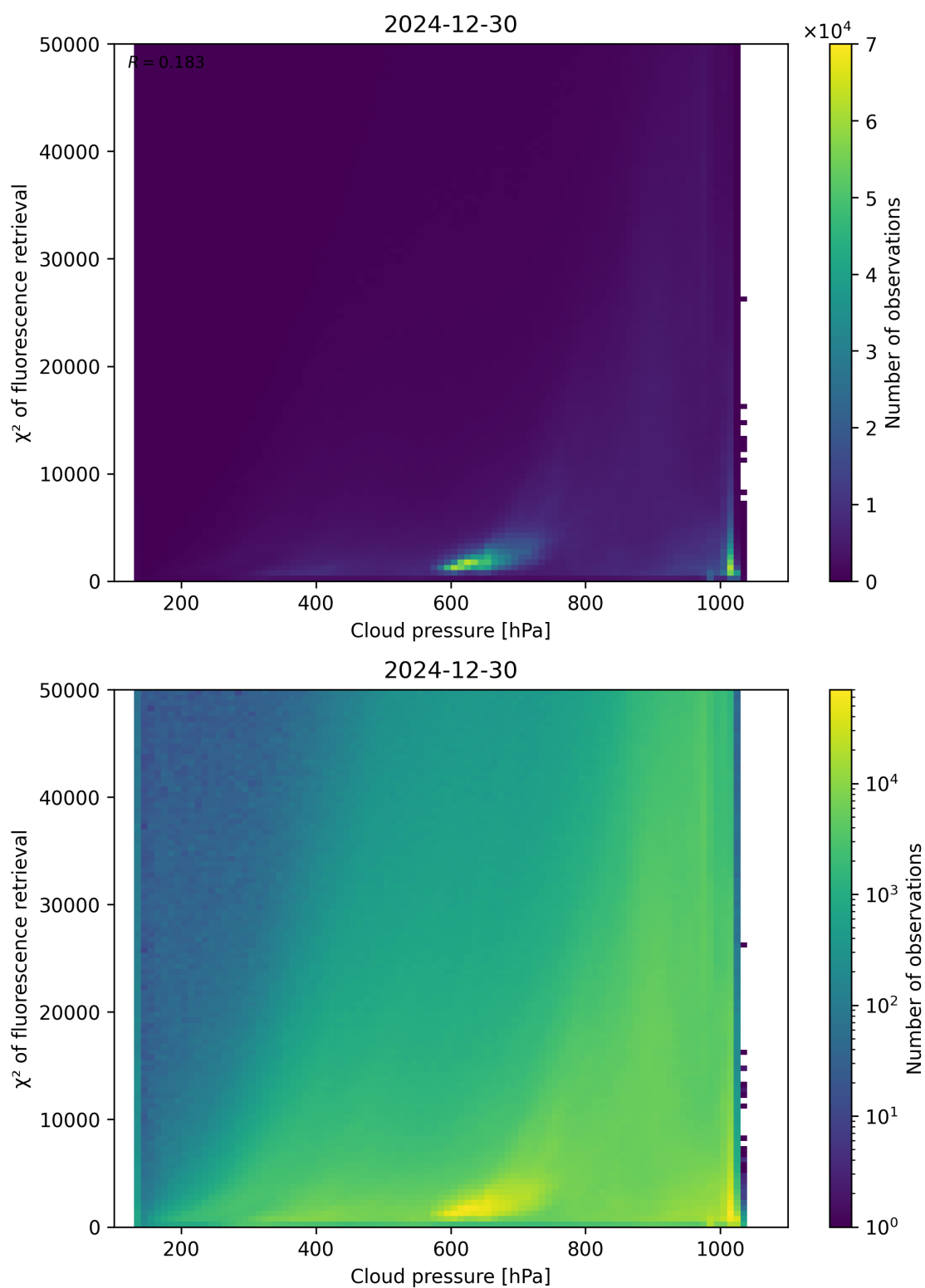
Figure 78: Scatter density plot of “Cloud pressure” against “ \chi^2 of fluorescence retrieval” for 2024-12-29 to 2024-12-31.
