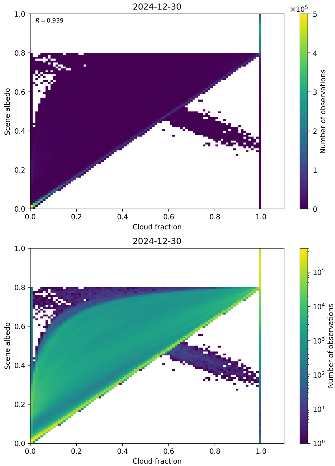
Figure 75: Scatter density plot of “Cloud fraction” against “Scene albedo” for 2024-12-29 to 2024-12-31.
