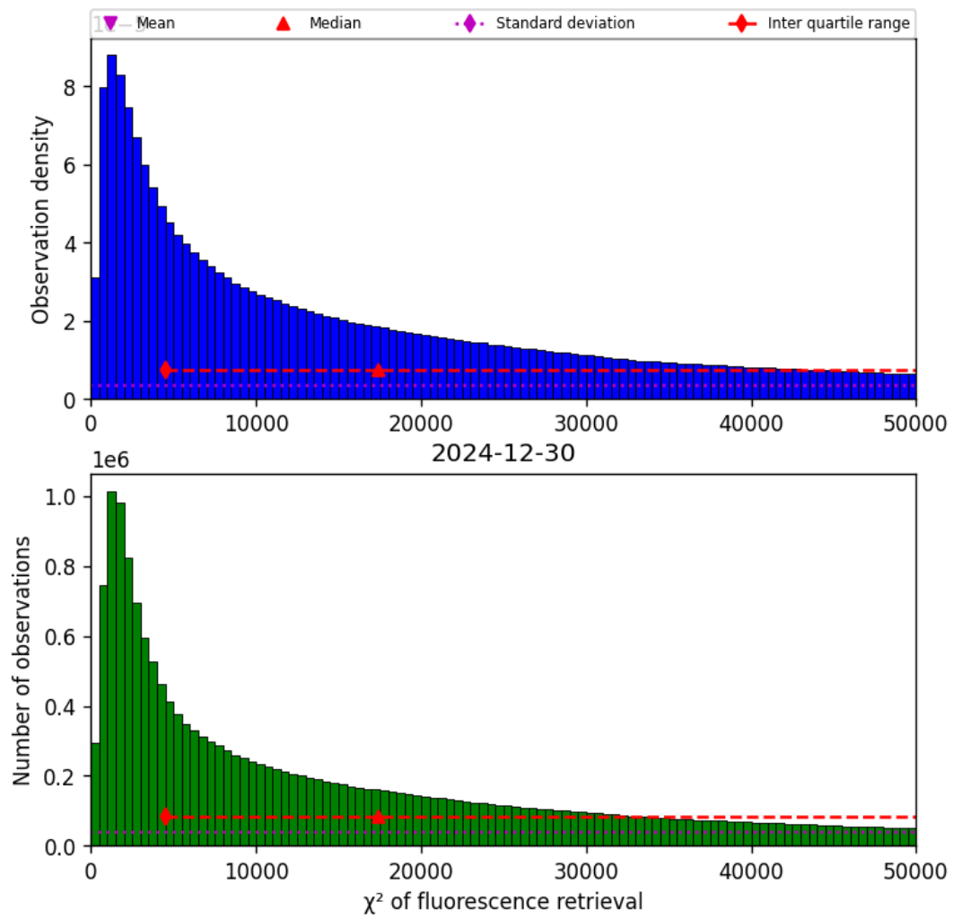
Figure 42: Histogram of “ \chi^2 of fluorescence retrieval” for 2024-12-29 to 2024-12-31
