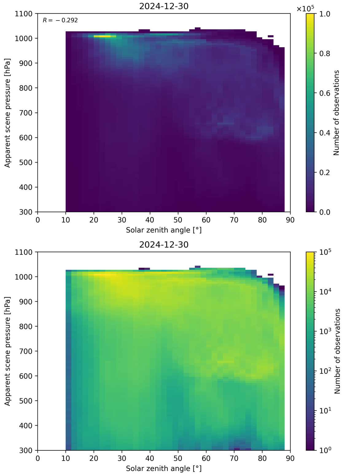
Figure 108: Scatter density plot of “Solar zenith angle” against “Apparent scene pressure” for 2024-12-29 to 2024-12-31.
