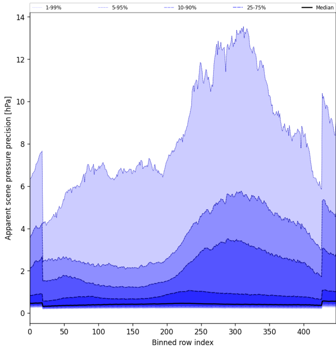
Figure 54: Along track statistics of “Apparent scene pressure precision” for 2024-12-29 to 2024-12-31
