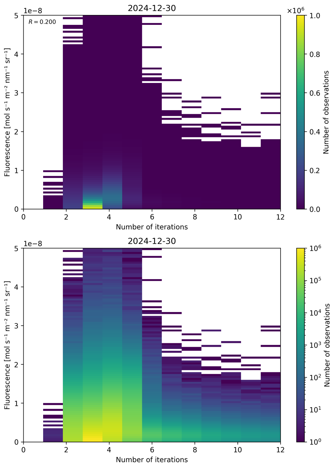
Figure 98: Scatter density plot of “Number of iterations” against “Fluorescence” for 2024-12-29 to 2024-12-31.
