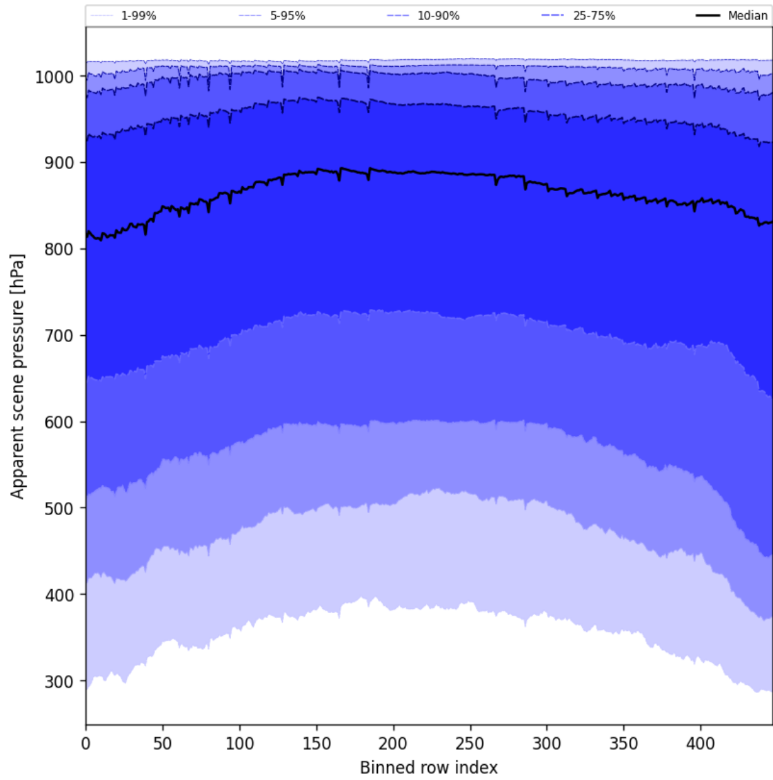
Figure 53: Along track statistics of “Apparent scene pressure” for 2024-12-29 to 2024-12-31
