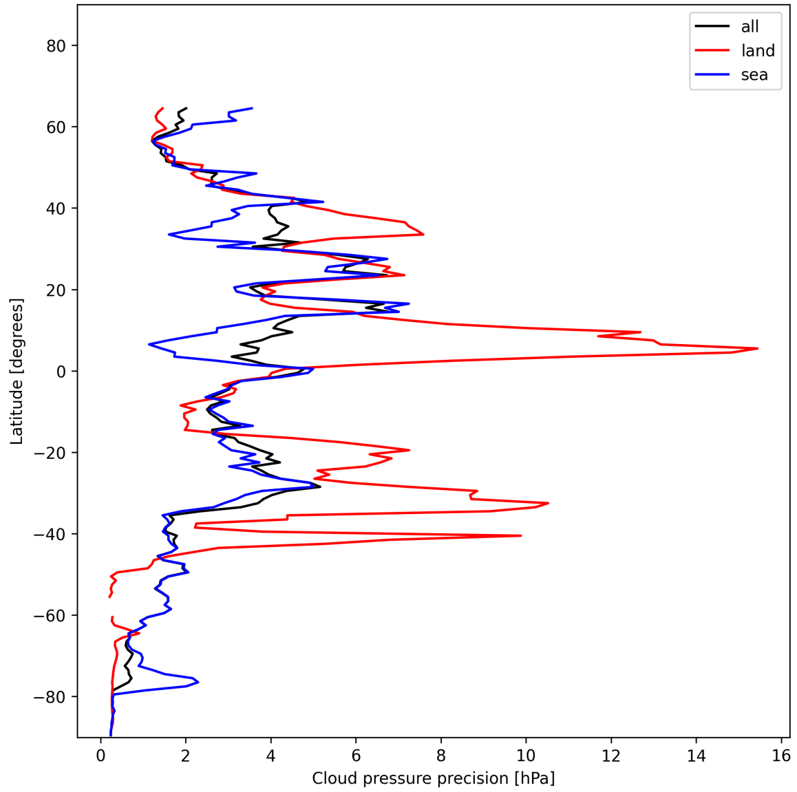
Figure 14: Zonal average of “Cloud pressure precision” for 2024-12-29 to 2024-12-31.
