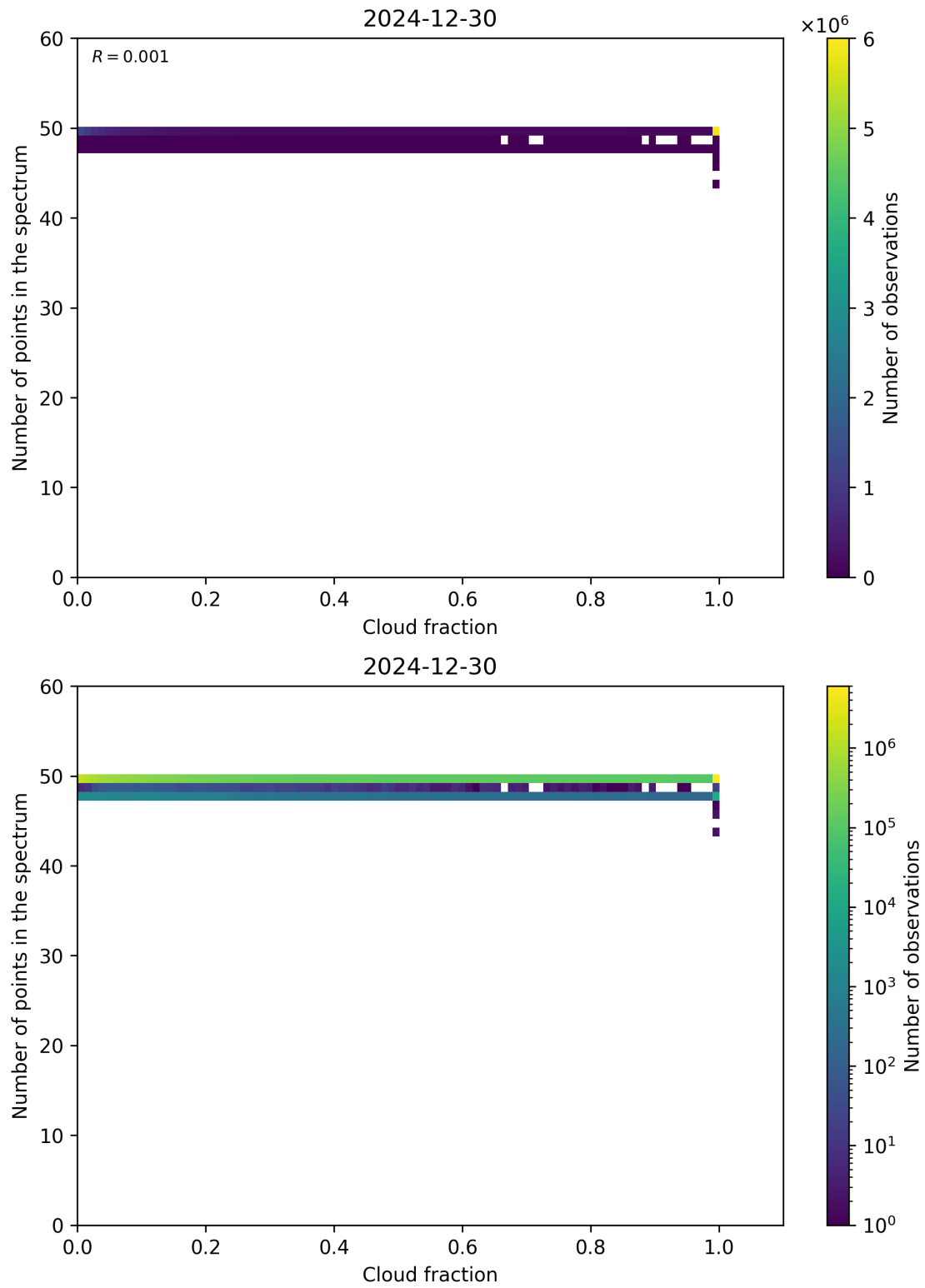
Figure 74: Scatter density plot of “Cloud fraction” against “Number of points in the spectrum” for 2024-12-29 to 2024-12-31.
