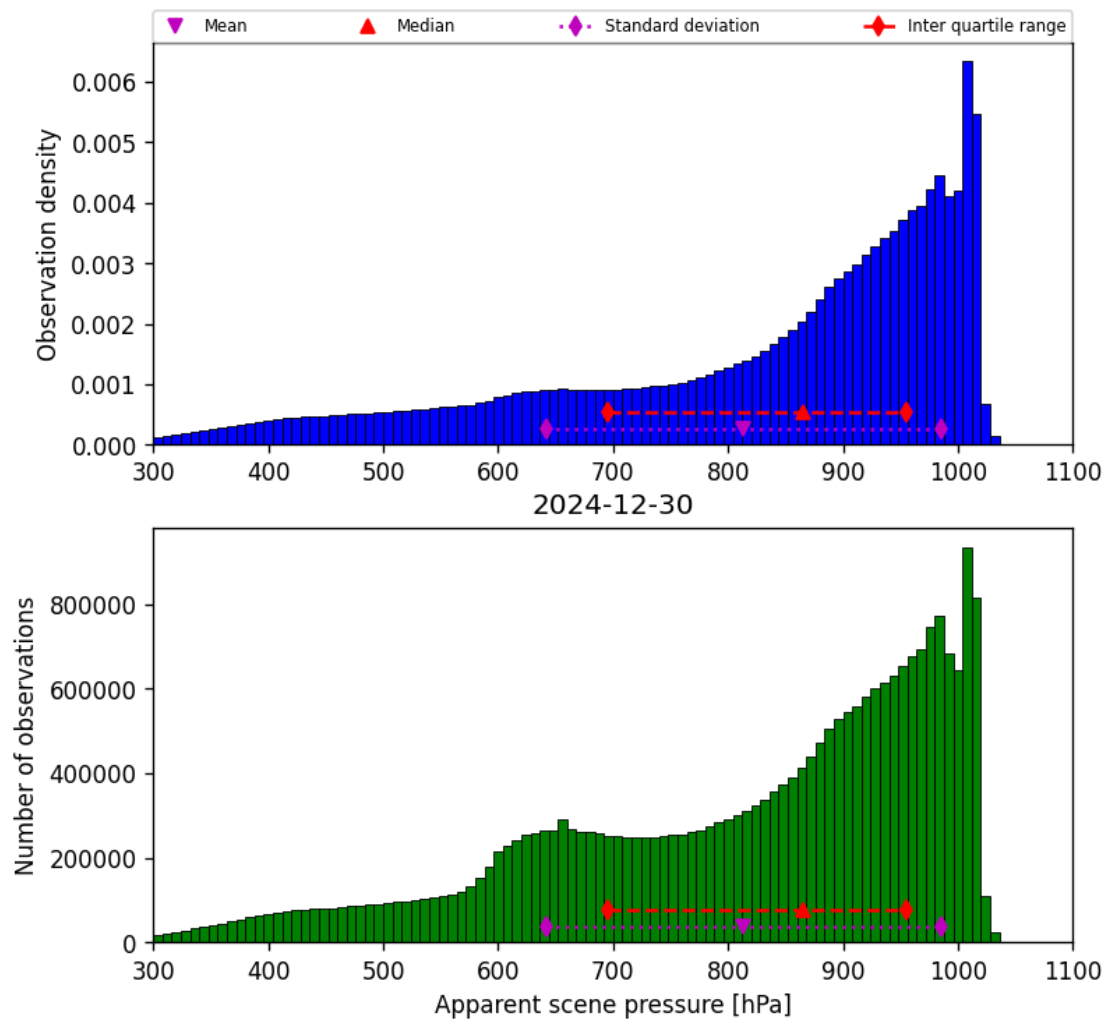
Figure 36: Histogram of “Apparent scene pressure” for 2024-12-29 to 2024-12-31
