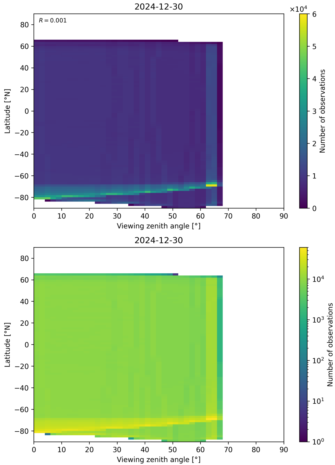
Figure 123: Scatter density plot of “Viewing zenith angle” against “Latitude” for 2024-12-29 to 2024-12-31.
