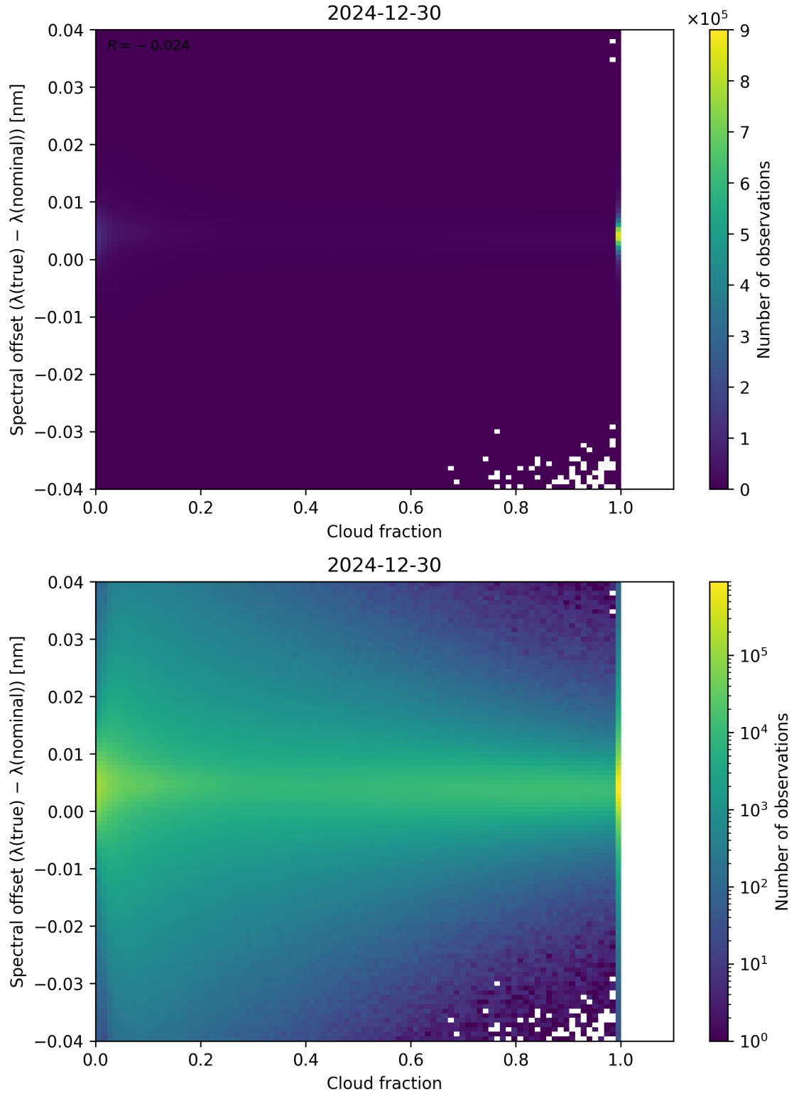
Figure 76: Scatter density plot of “Cloud fraction” against “Spectral offset ( \lambda_{\text{true}} - \lambda_{\text{nominal}} )” for 2024-12-29 to 2024-12-31.
