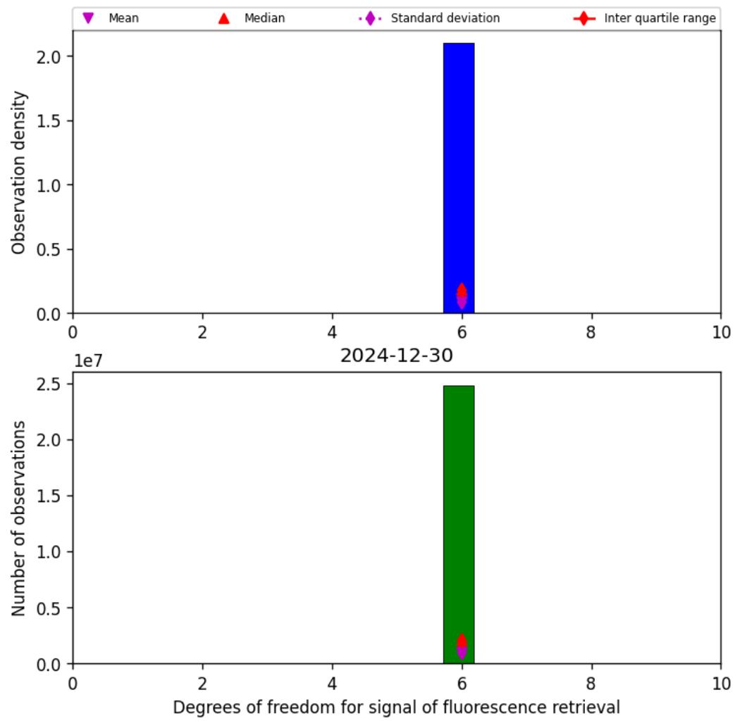
Figure 43: Histogram of “Degrees of freedom for signal of fluorescence retrieval” for 2024-12-29 to 2024-12-31
