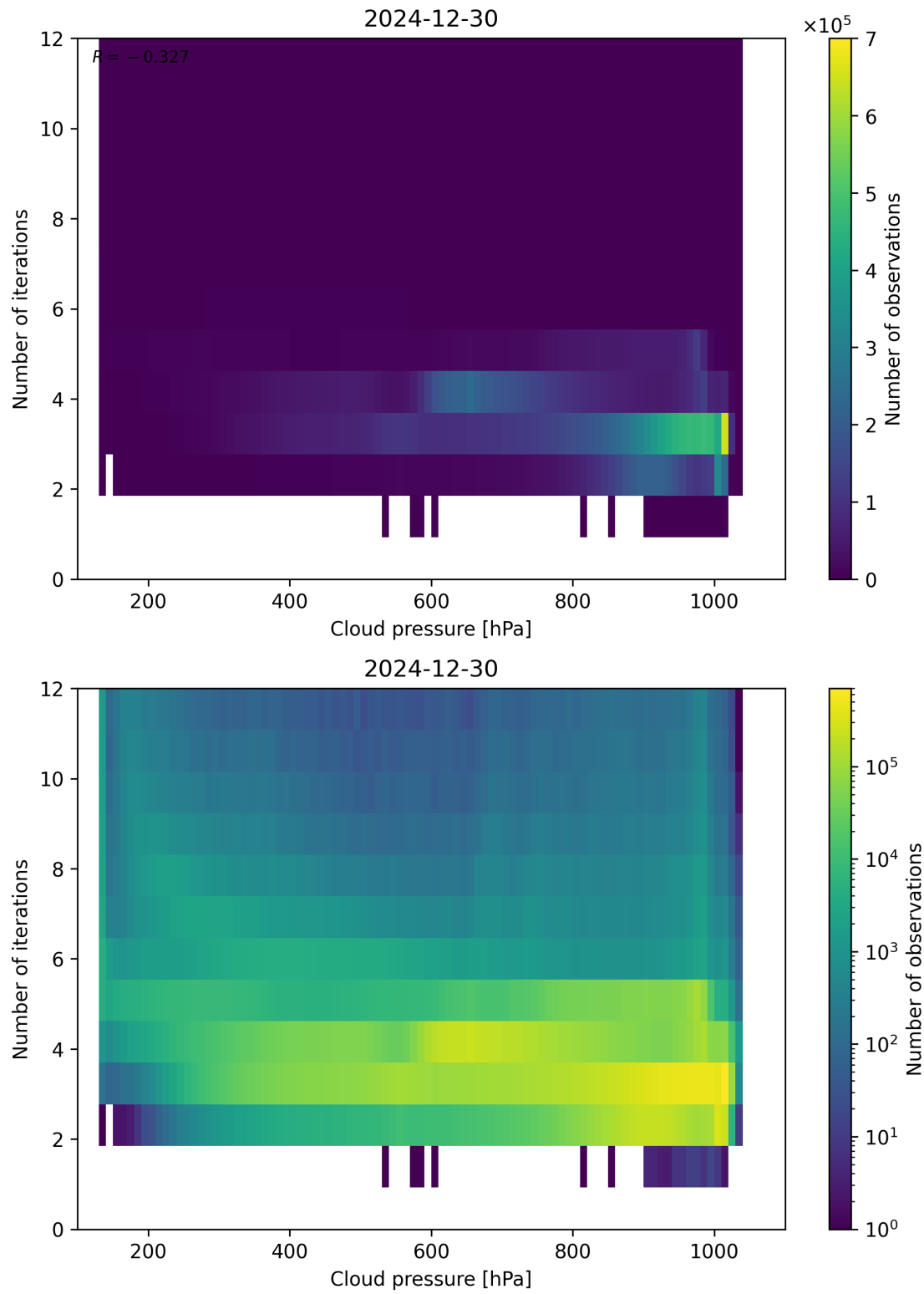
Figure 81: Scatter density plot of “Cloud pressure” against “Number of iterations” for 2024-12-29 to 2024-12-31.
