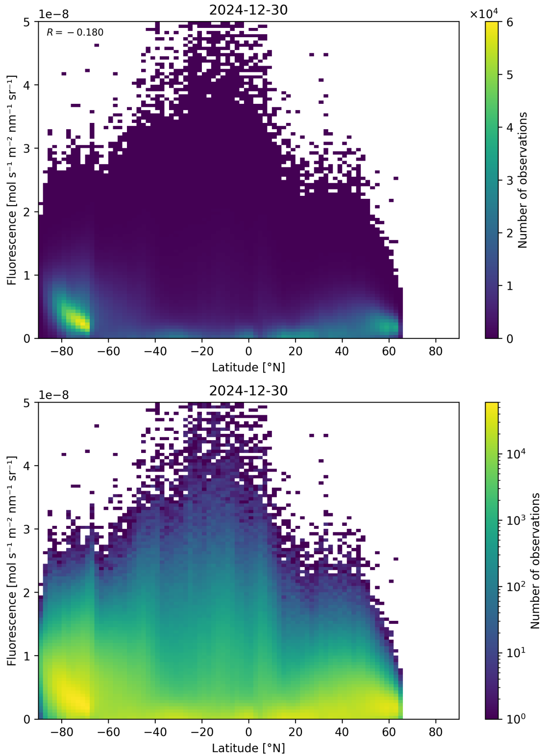
Figure 92: Scatter density plot of “Latitude” against “Fluorescence” for 2024-12-29 to 2024-12-31.
