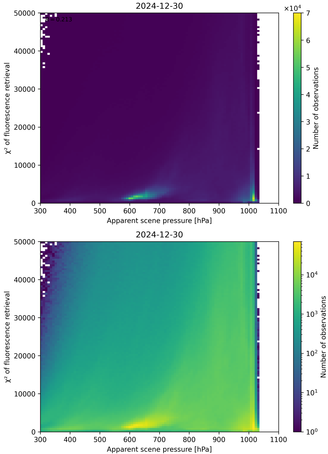
Figure 63: Scatter density plot of “Apparent scene pressure” against “ \chi^2 of fluorescence retrieval” for 2024-12-29 to 2024-12-31.
