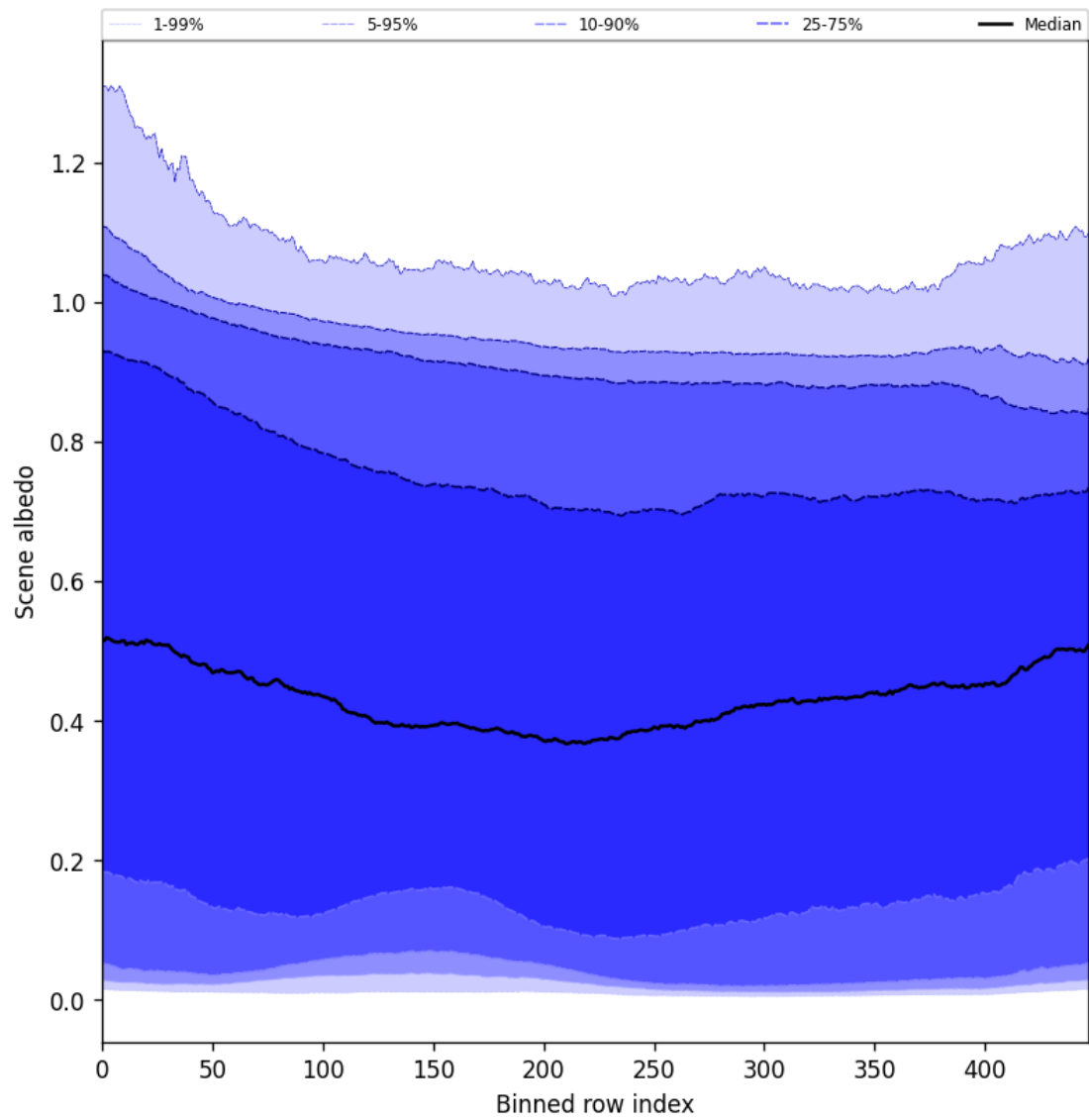
Figure 51: Along track statistics of “Scene albedo” for 2024-12-29 to 2024-12-31
