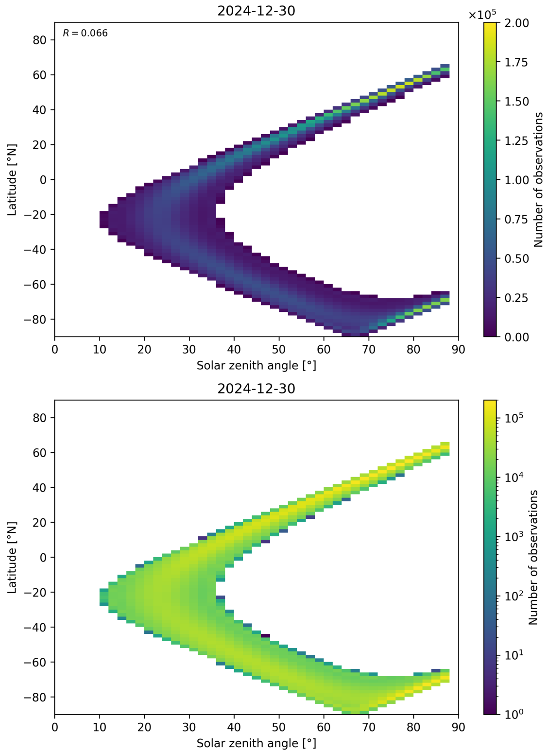
Figure 113: Scatter density plot of “Solar zenith angle” against “Latitude” for 2024-12-29 to 2024-12-31.
