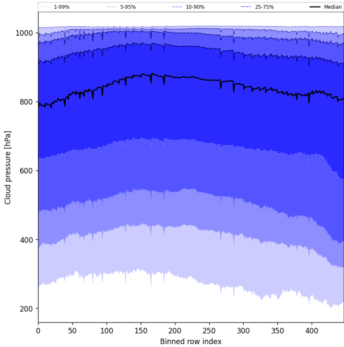
Figure 47: Along track statistics of “Cloud pressure” for 2024-12-29 to 2024-12-31
