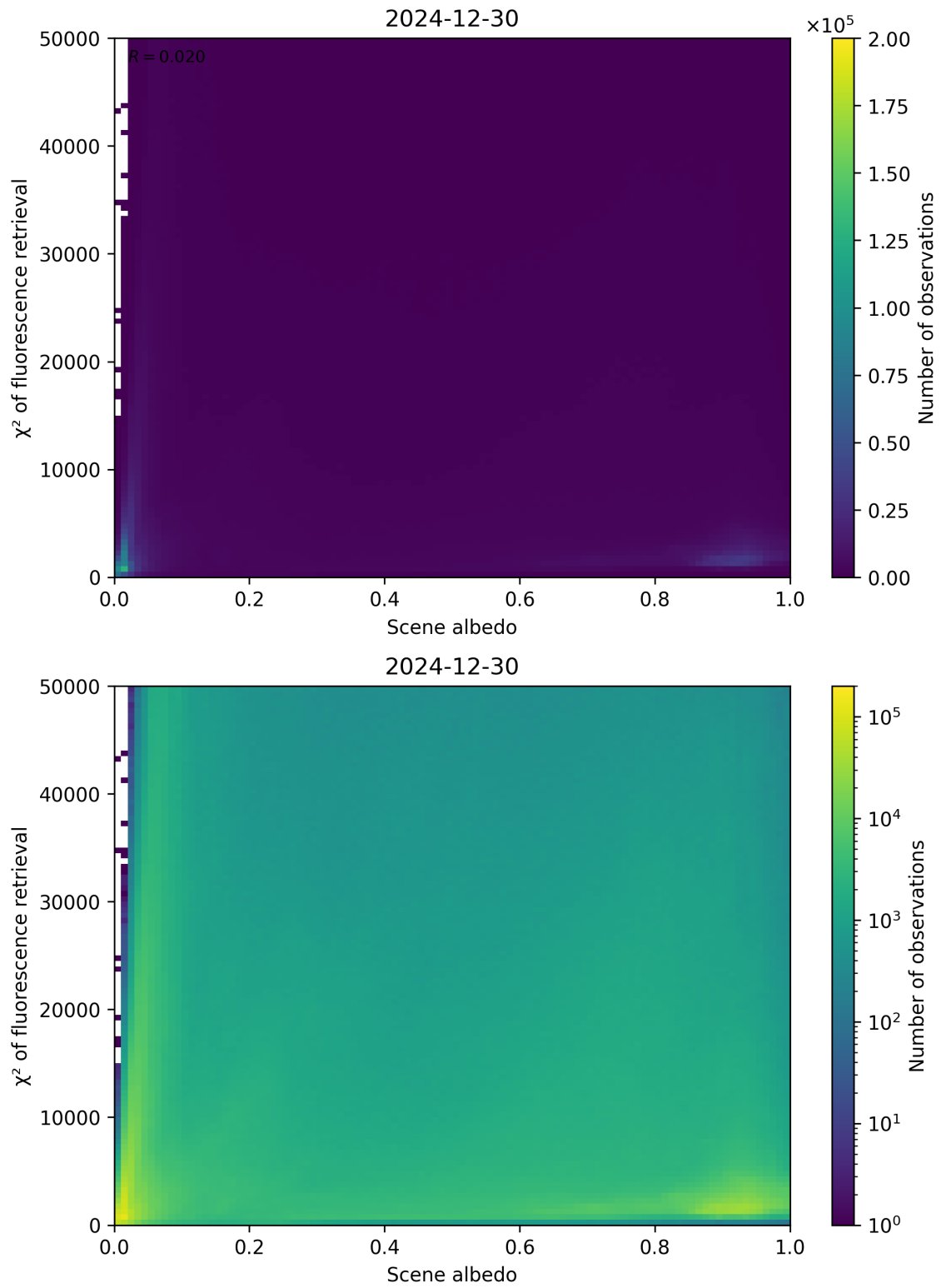
Figure 103: Scatter density plot of “Scene albedo” against “ \chi^2 of fluorescence retrieval” for 2024-12-29 to 2024-12-31.
