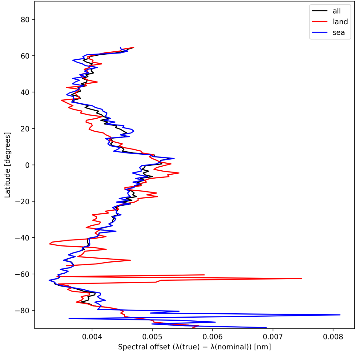
Figure 28: Zonal average of “Spectral offset ( \lambda_{\text{true}} - \lambda_{\text{nominal}} )” for 2024-12-29 to 2024-12-31.
