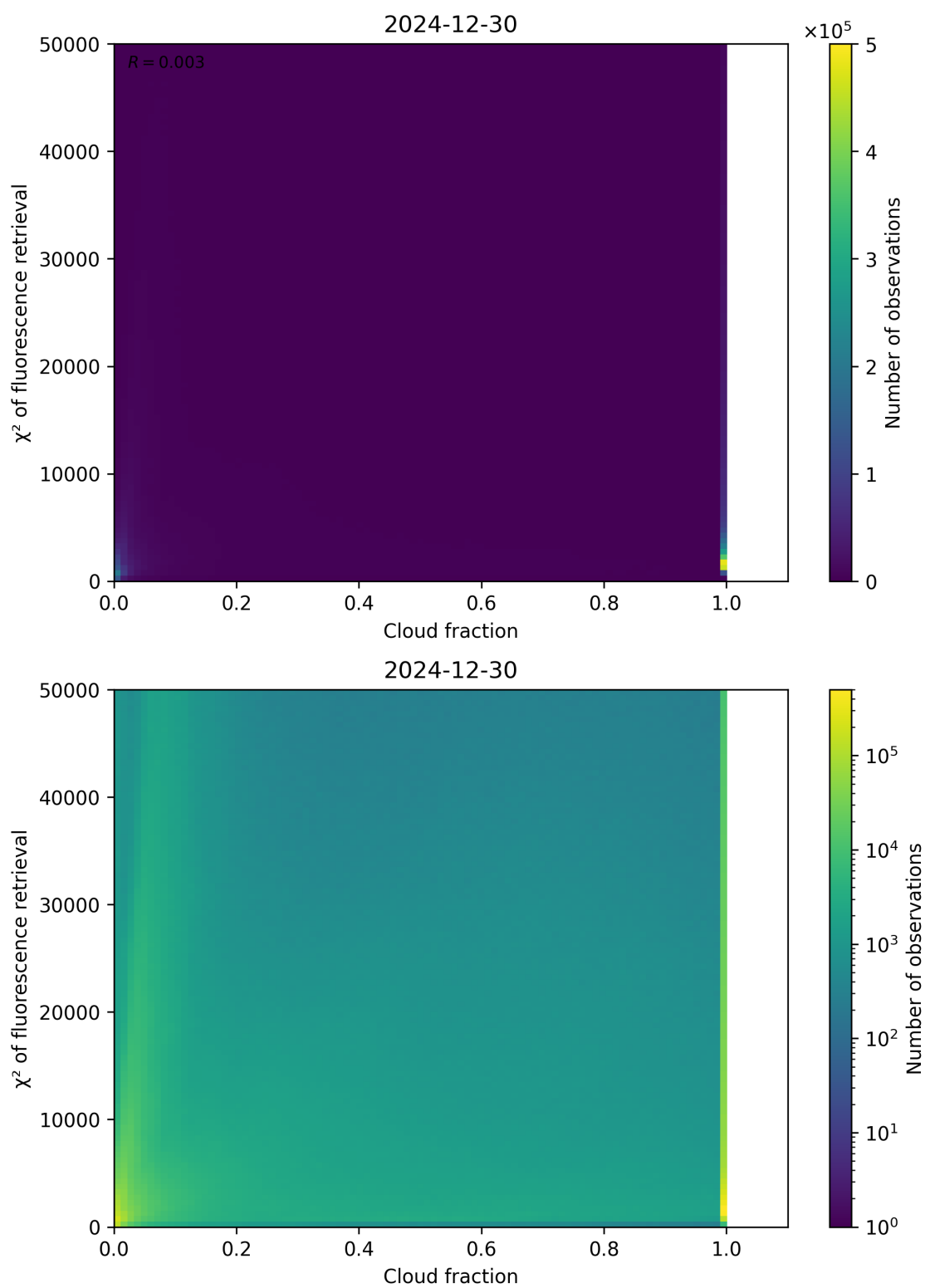
Figure 71: Scatter density plot of “Cloud fraction” against “ \chi^2 of fluorescence retrieval” for 2024-12-29 to 2024-12-31.
