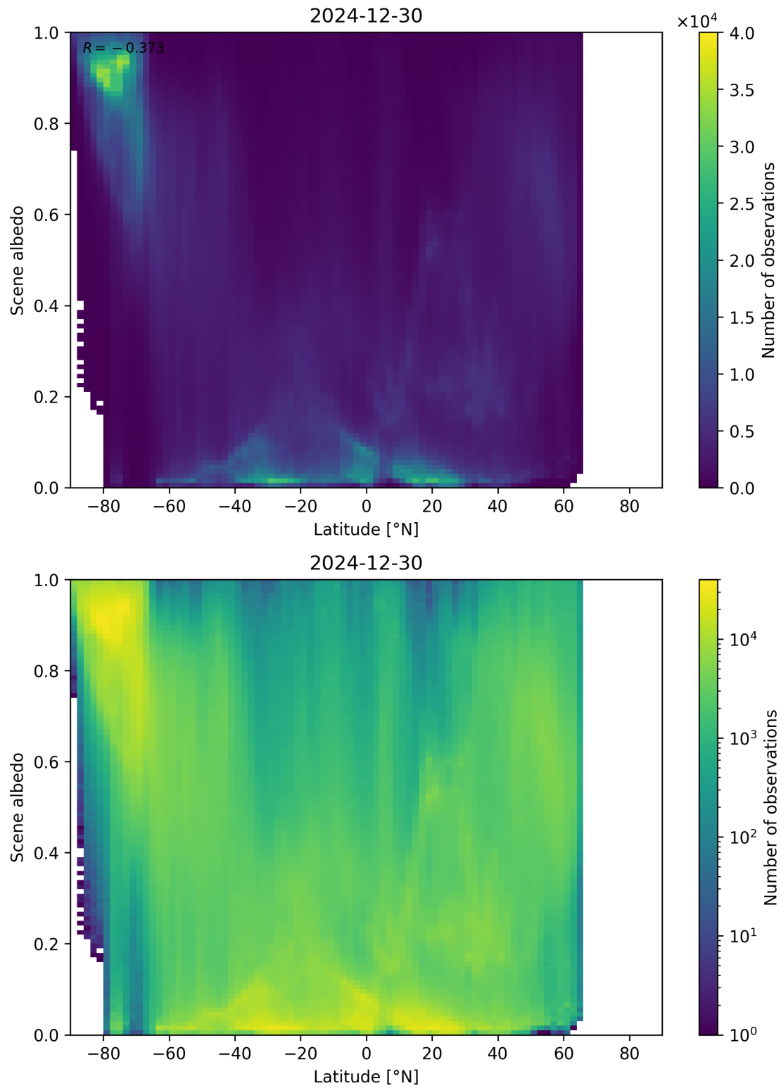
Figure 95: Scatter density plot of “Latitude” against “Scene albedo” for 2024-12-29 to 2024-12-31.
