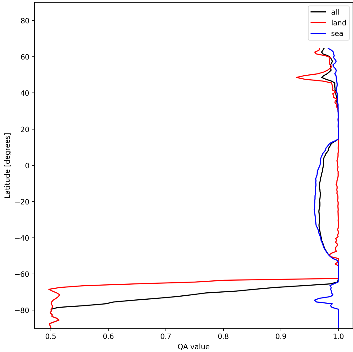
Figure 12: Zonal average of “QA value” for 2024-12-29 to 2024-12-31.
