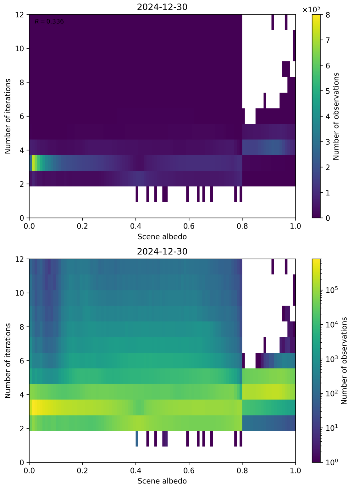
Figure 105: Scatter density plot of “Scene albedo” against “Number of iterations” for 2024-12-29 to 2024-12-31.
