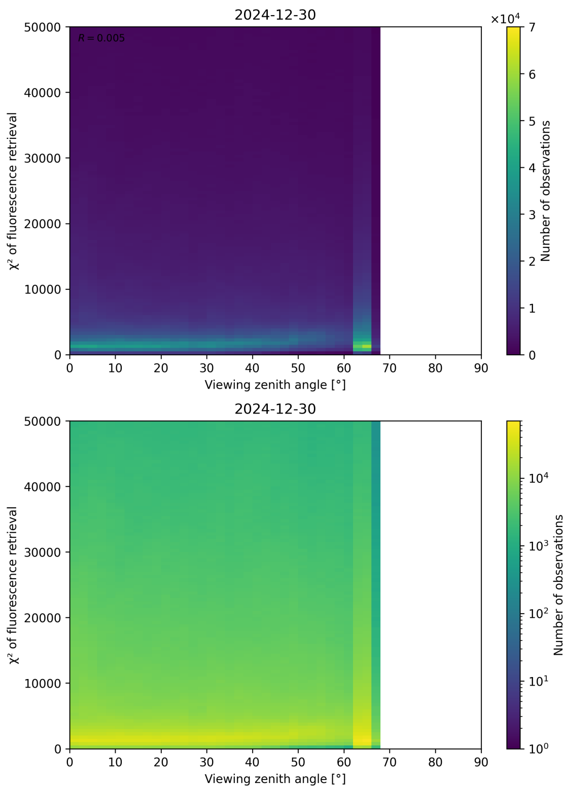
Figure 119: Scatter density plot of “Viewing zenith angle” against “ \chi^2 of fluorescence retrieval” for 2024-12-29 to 2024-12-31.
