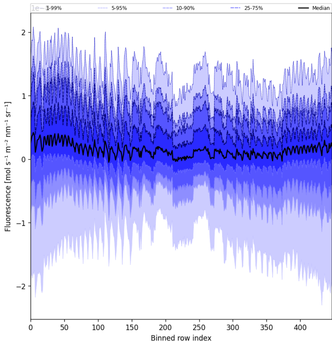
Figure 57: Along track statistics of “Fluorescence” for 2024-12-29 to 2024-12-31
