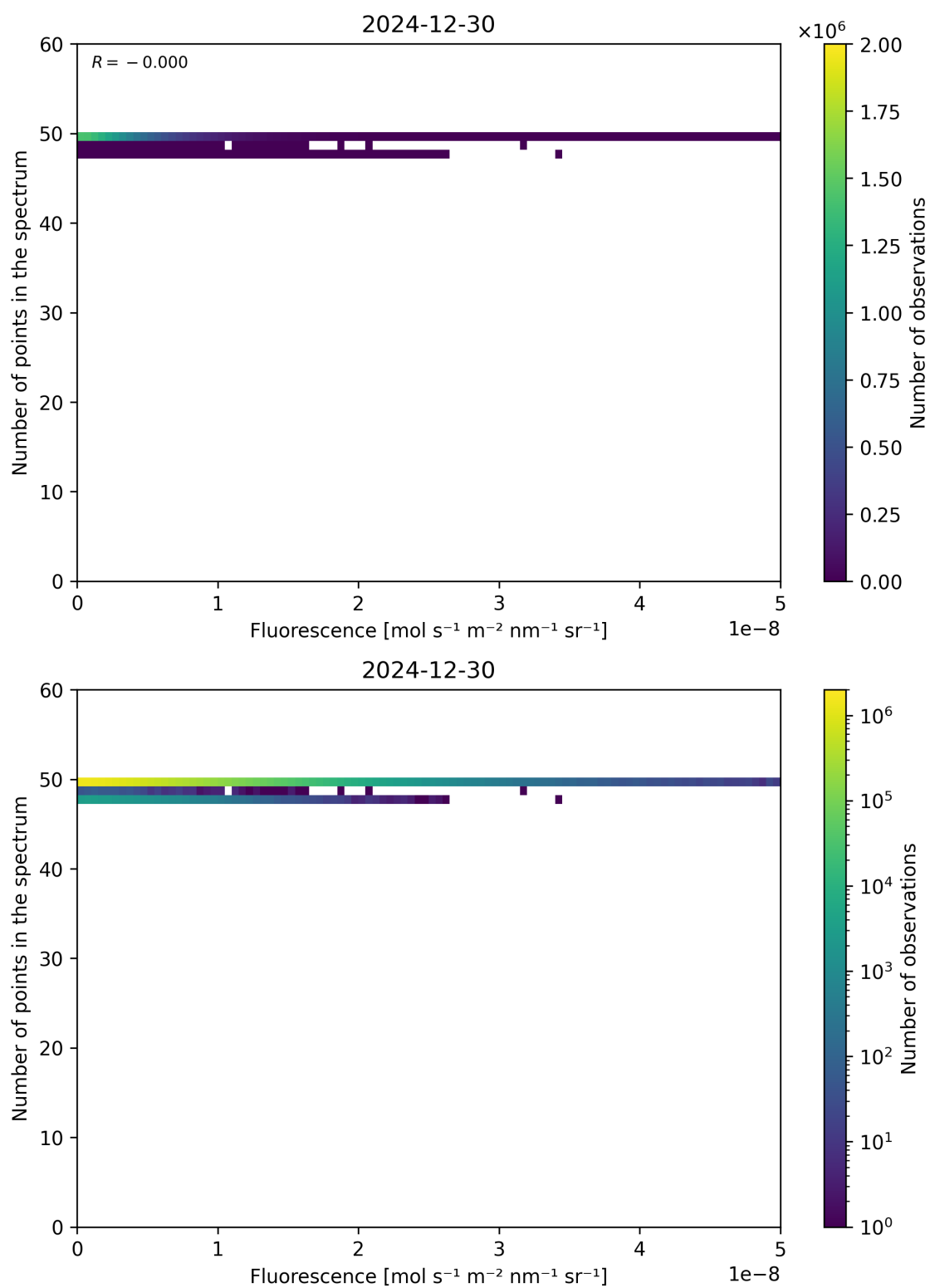
Figure 86: Scatter density plot of “Fluorescence” against “Number of points in the spectrum” for 2024-12-29 to 2024-12-31.
