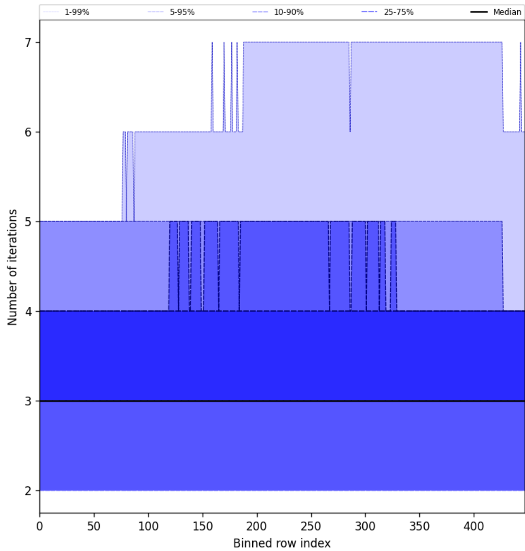
Figure 56: Along track statistics of “Number of iterations” for 2024-12-29 to 2024-12-31
