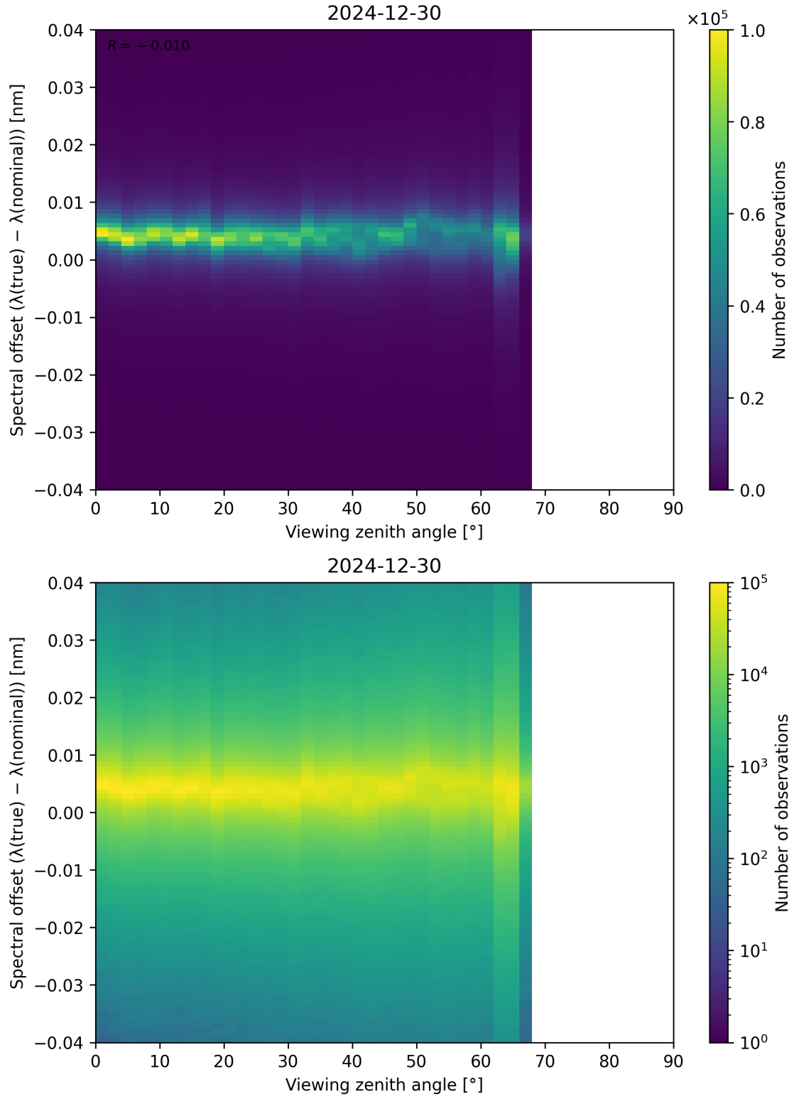
Figure 128: Scatter density plot of “Viewing zenith angle” against “Spectral offset ( \lambda_{\text{true}} - \lambda_{\text{nominal}} )” for 2024-12-29 to 2024-12-31.
