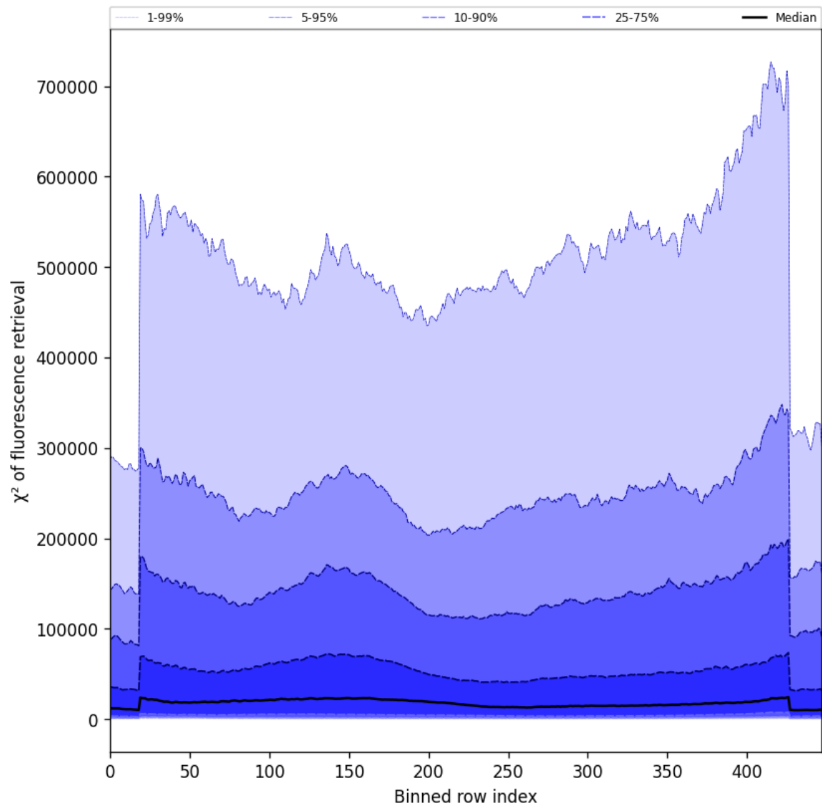
Figure 59: Along track statistics of “ \chi^2 of fluorescence retrieval” for 2024-12-29 to 2024-12-31
