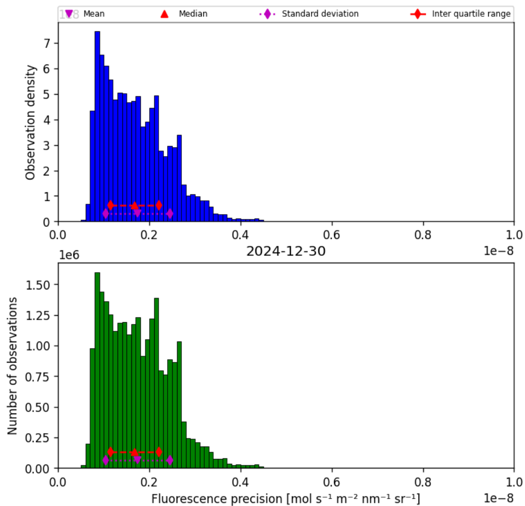
Figure 41: Histogram of “Fluorescence precision” for 2024-12-29 to 2024-12-31
