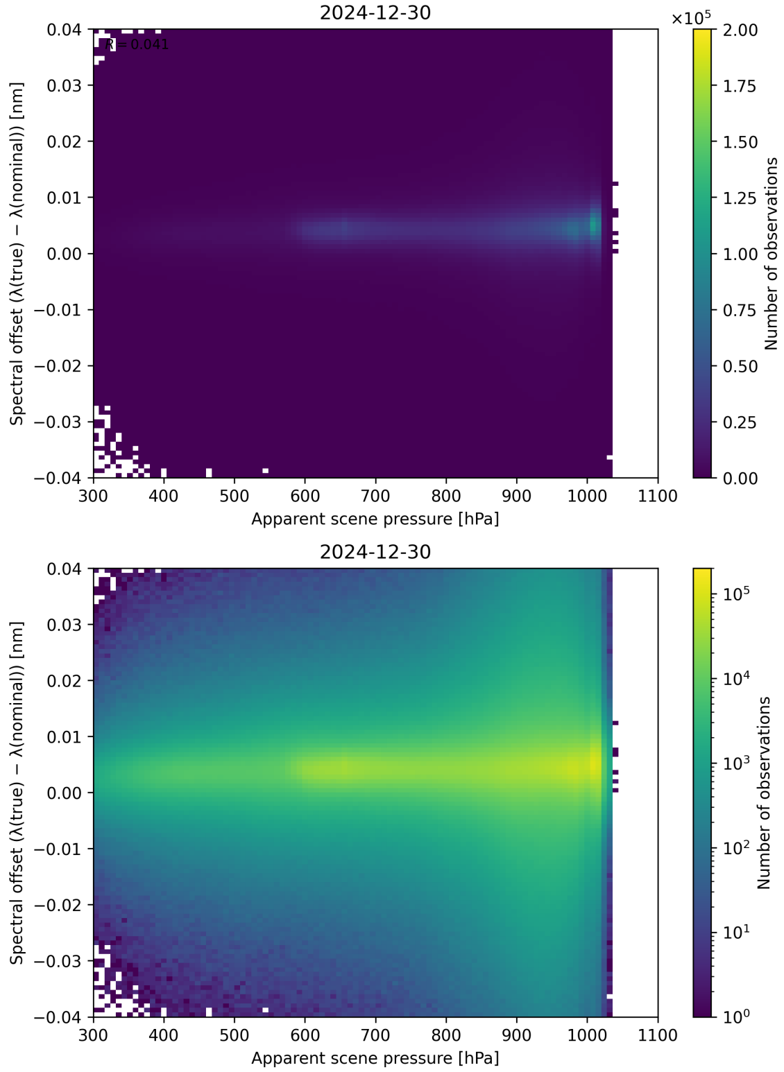
Figure 67: Scatter density plot of “Apparent scene pressure” against “Spectral offset ( \lambda_{\text{true}} - \lambda_{\text{nominal}} )” for 2024-12-29 to 2024-12-31.
