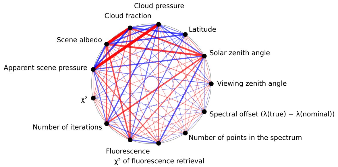
Figure 1: Map of correlation graph for 2024-12-29 to 2024-12-31.
