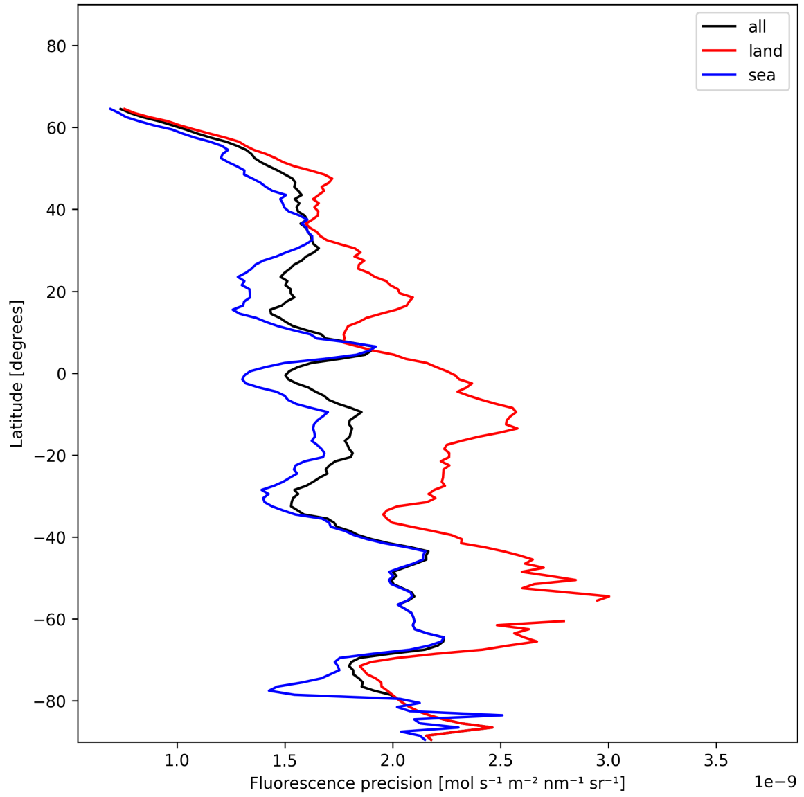
Figure 24: Zonal average of “Fluorescence precision” for 2024-12-29 to 2024-12-31.
