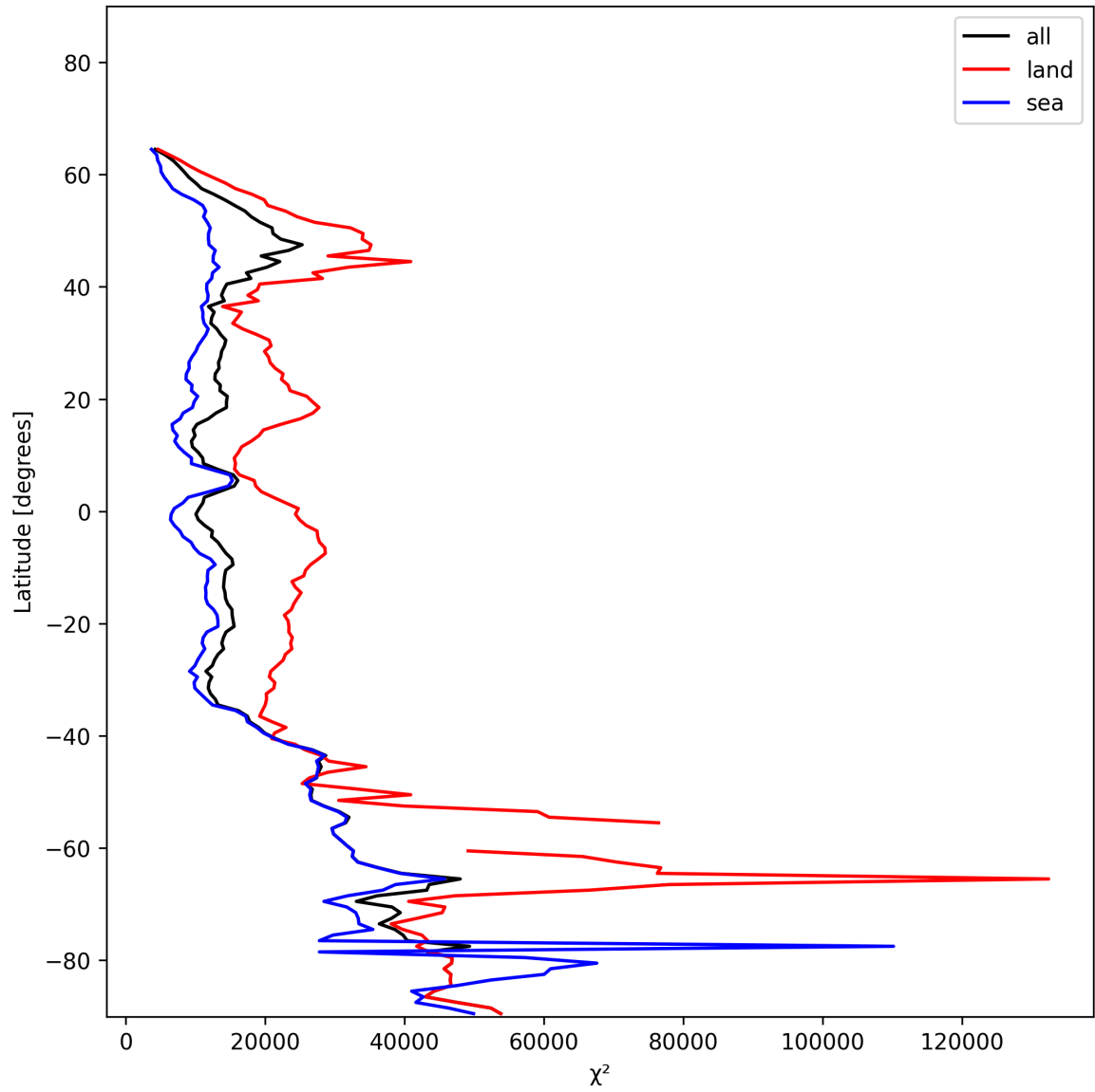
Figure 21: Zonal average of “ \chi^2 ” for 2024-12-29 to 2024-12-31.
