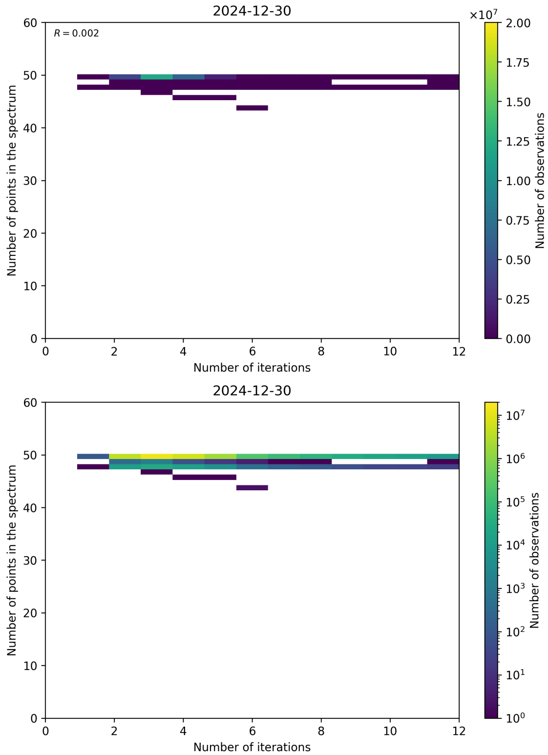
Figure 99: Scatter density plot of “Number of iterations” against “Number of points in the spectrum” for 2024-12-29 to 2024-12-31.
