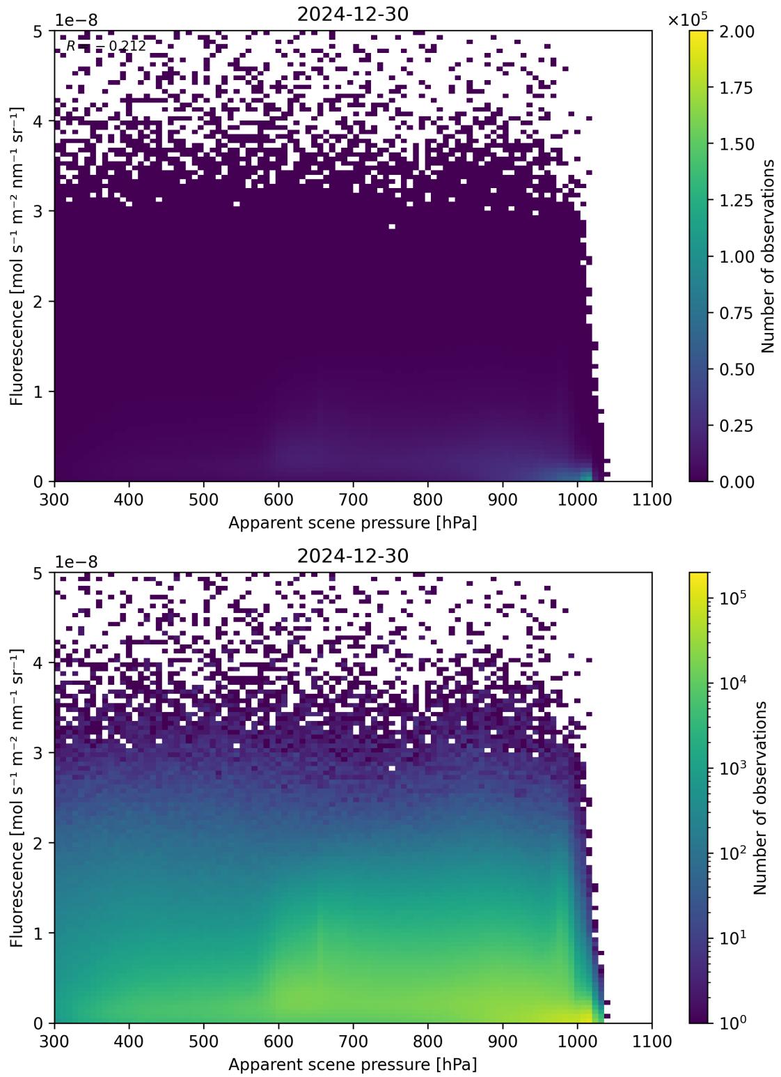
Figure 64: Scatter density plot of “Apparent scene pressure” against “Fluorescence” for 2024-12-29 to 2024-12-31.
