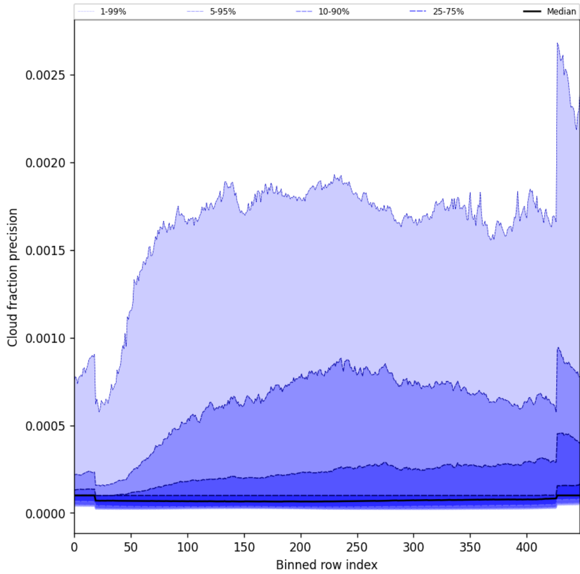
Figure 50: Along track statistics of “Cloud fraction precision” for 2024-12-29 to 2024-12-31
