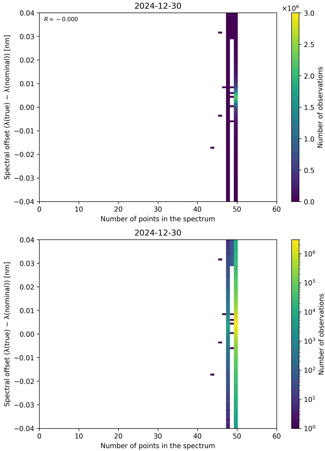
Figure 101: Scatter density plot of “Number of points in the spectrum” against “Spectral offset ( \lambda_{\text{true}} - \lambda_{\text{nominal}} )” for 2024-12-29 to 2024-12-31.
