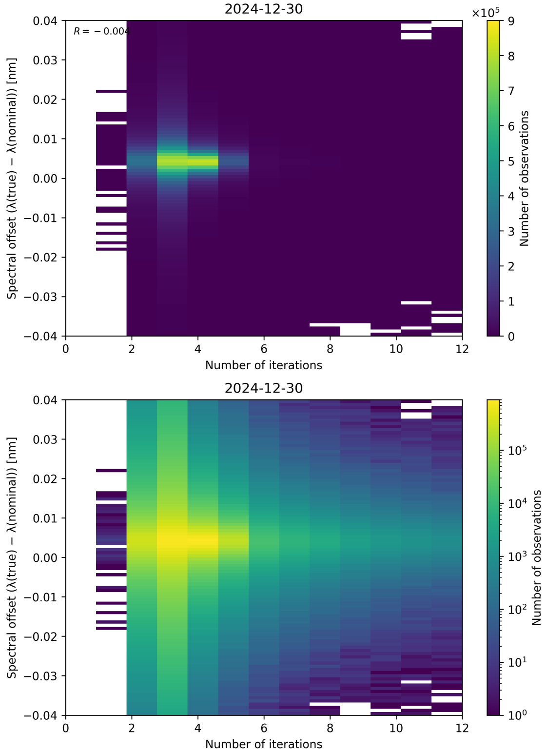
Figure 100: Scatter density plot of “Number of iterations” against “Spectral offset ( \lambda_{\text{true}} - \lambda_{\text{nominal}} )” for 2024-12-29 to 2024-12-31.
