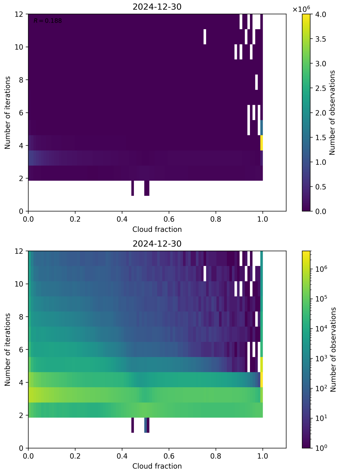
Figure 73: Scatter density plot of “Cloud fraction” against “Number of iterations” for 2024-12-29 to 2024-12-31.
