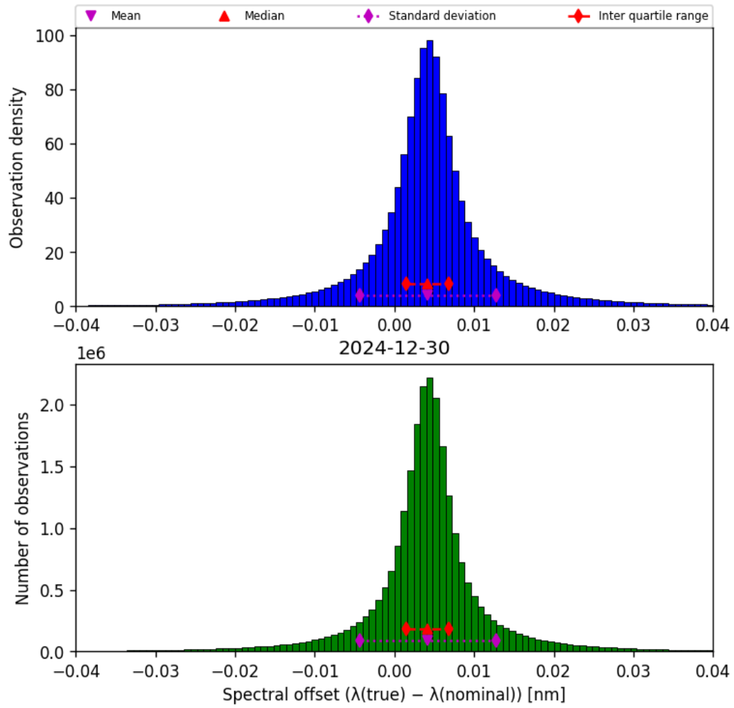
Figure 45: Histogram of “Spectral offset ( \lambda_{\text{true}} - \lambda_{\text{nominal}} )” for 2024-12-29 to 2024-12-31
