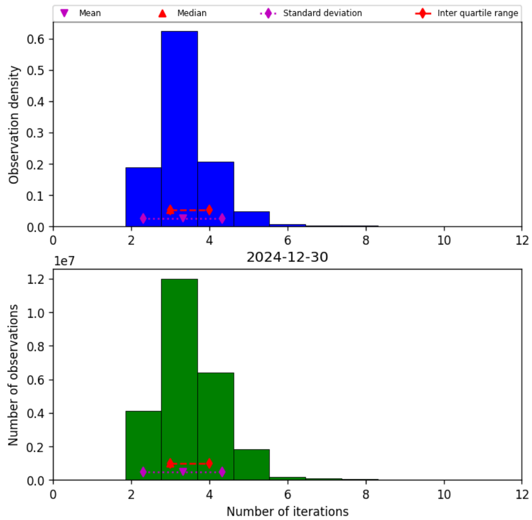
Figure 39: Histogram of “Number of iterations” for 2024-12-29 to 2024-12-31
