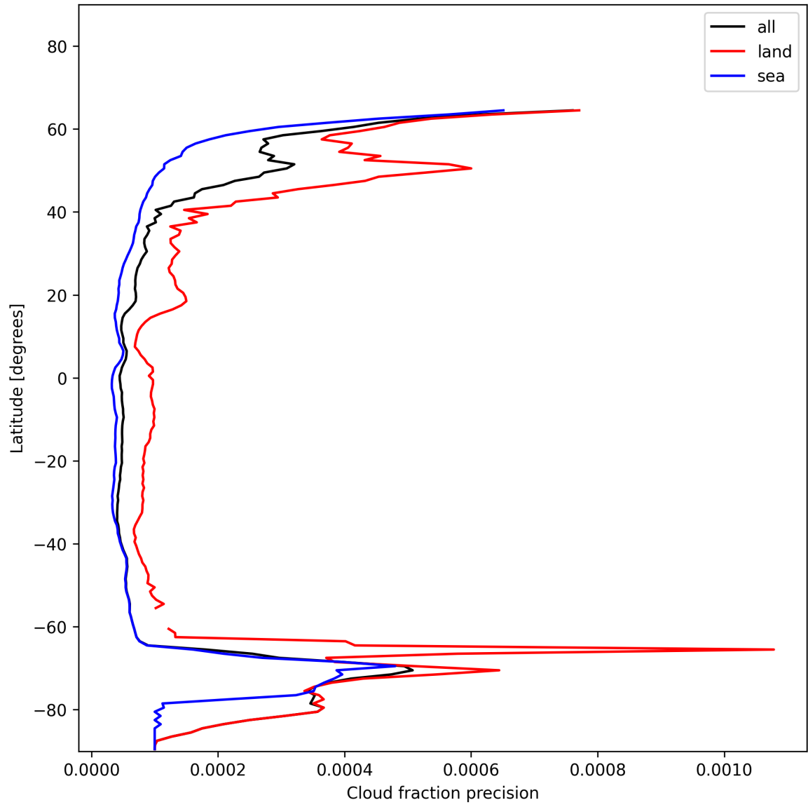
Figure 16: Zonal average of “Cloud fraction precision” for 2024-12-29 to 2024-12-31.
