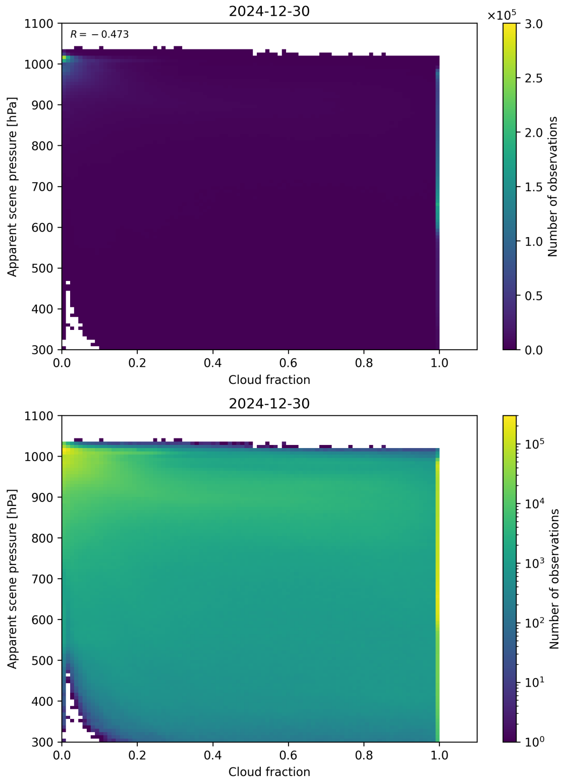
Figure 70: Scatter density plot of “Cloud fraction” against “Apparent scene pressure” for 2024-12-29 to 2024-12-31.
