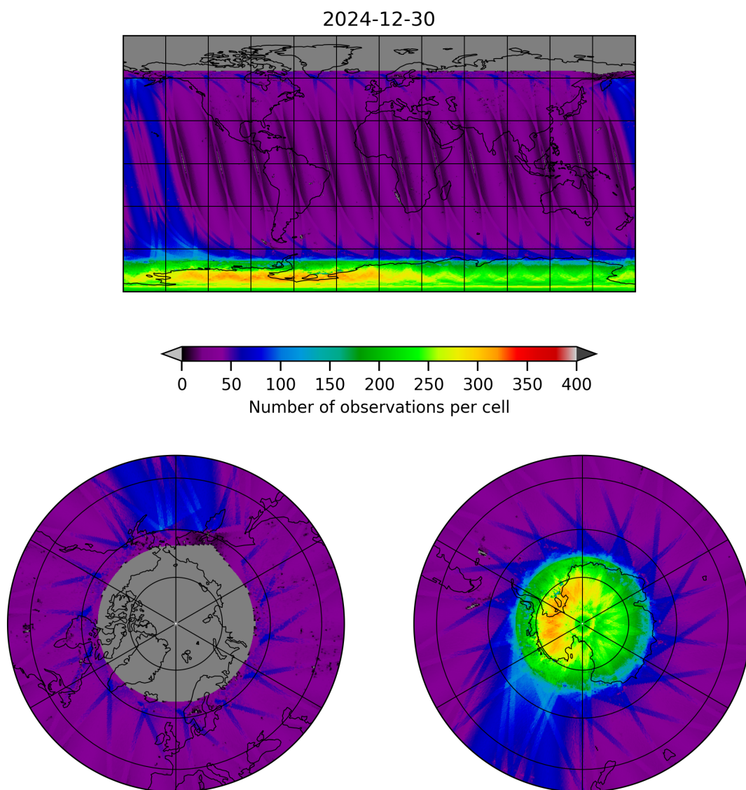
Figure 11: Map of the number of observations for 2024-12-29 to 2024-12-31
