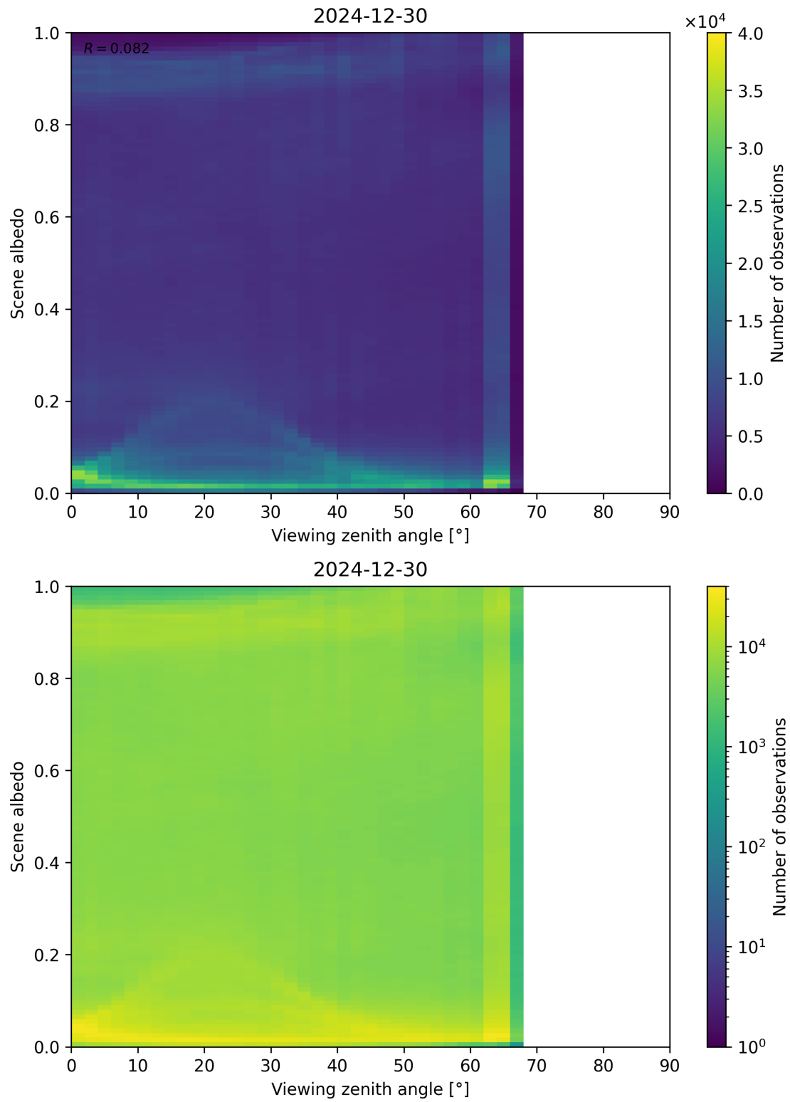
Figure 126: Scatter density plot of “Viewing zenith angle” against “Scene albedo” for 2024-12-29 to 2024-12-31.
