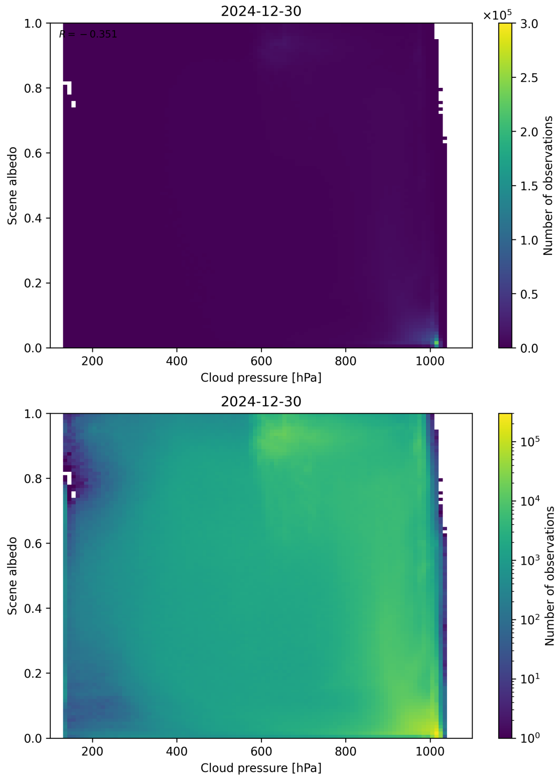
Figure 83: Scatter density plot of “Cloud pressure” against “Scene albedo” for 2024-12-29 to 2024-12-31.
