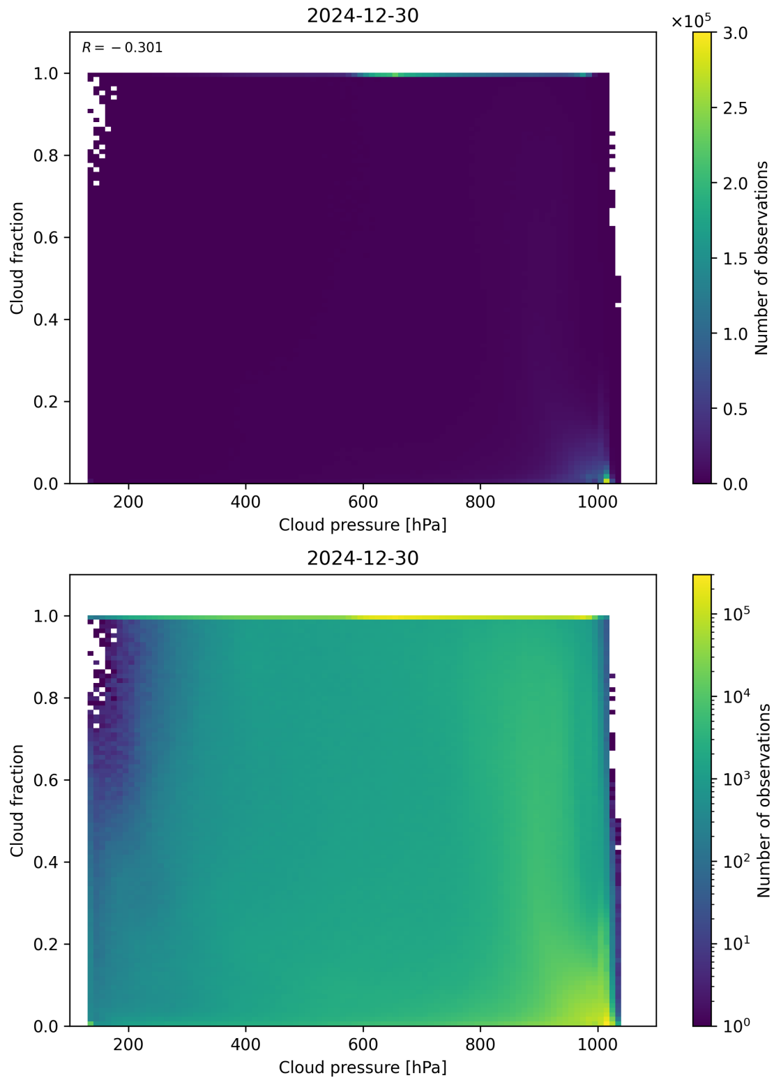
Figure 79: Scatter density plot of “Cloud pressure” against “Cloud fraction” for 2024-12-29 to 2024-12-31.
