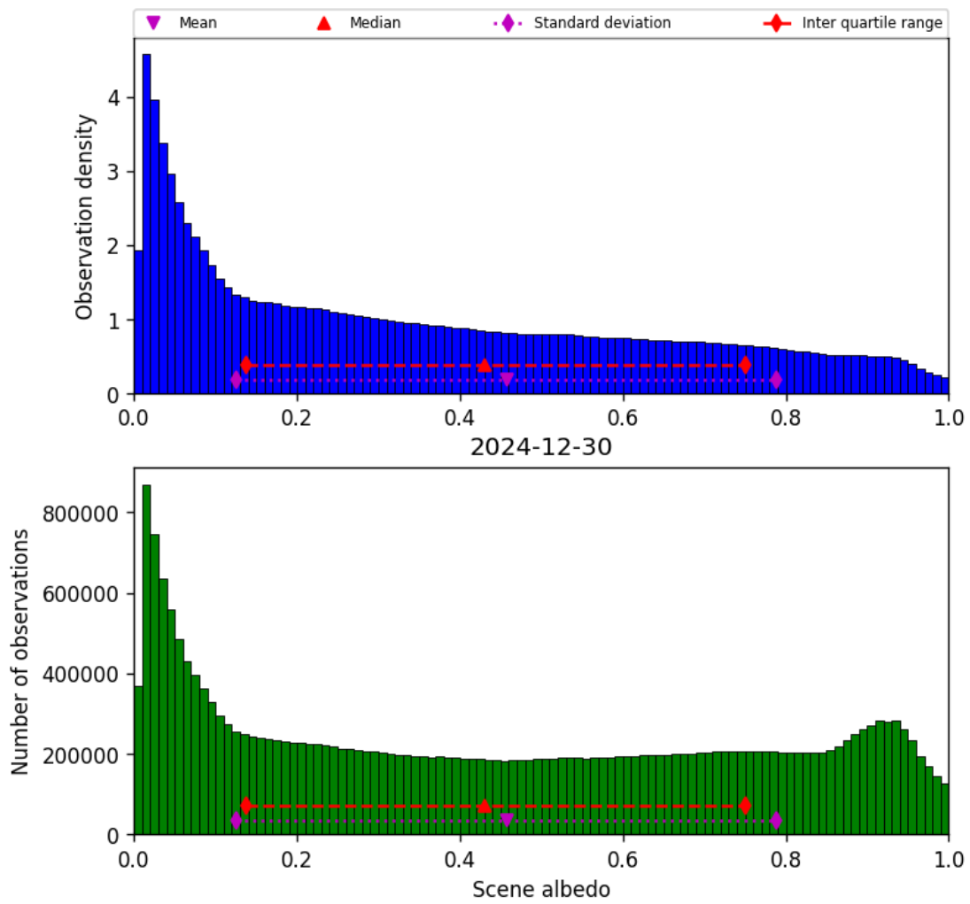
Figure 34: Histogram of “Scene albedo” for 2024-12-29 to 2024-12-31
