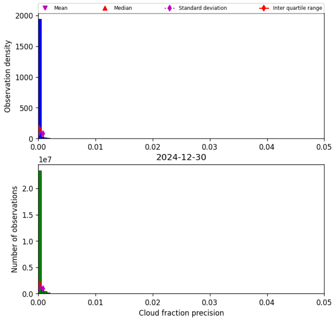
Figure 33: Histogram of “Cloud fraction precision” for 2024-12-29 to 2024-12-31
