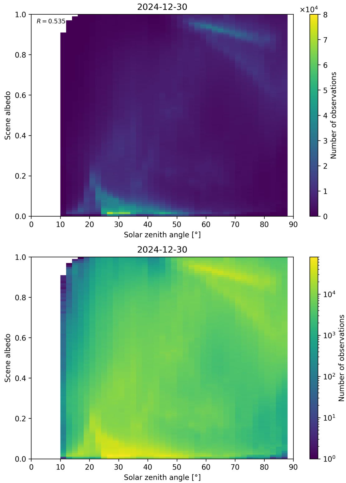
Figure 116: Scatter density plot of “Solar zenith angle” against “Scene albedo” for 2024-12-29 to 2024-12-31.
