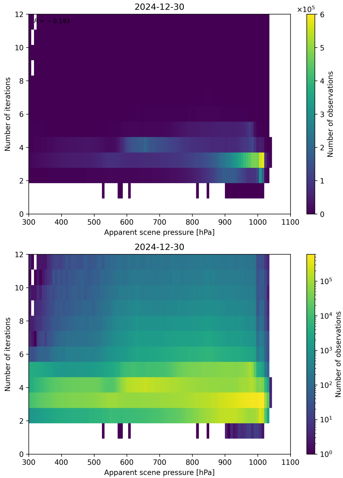
Figure 65: Scatter density plot of “Apparent scene pressure” against “Number of iterations” for 2024-12-29 to 2024-12-31.
