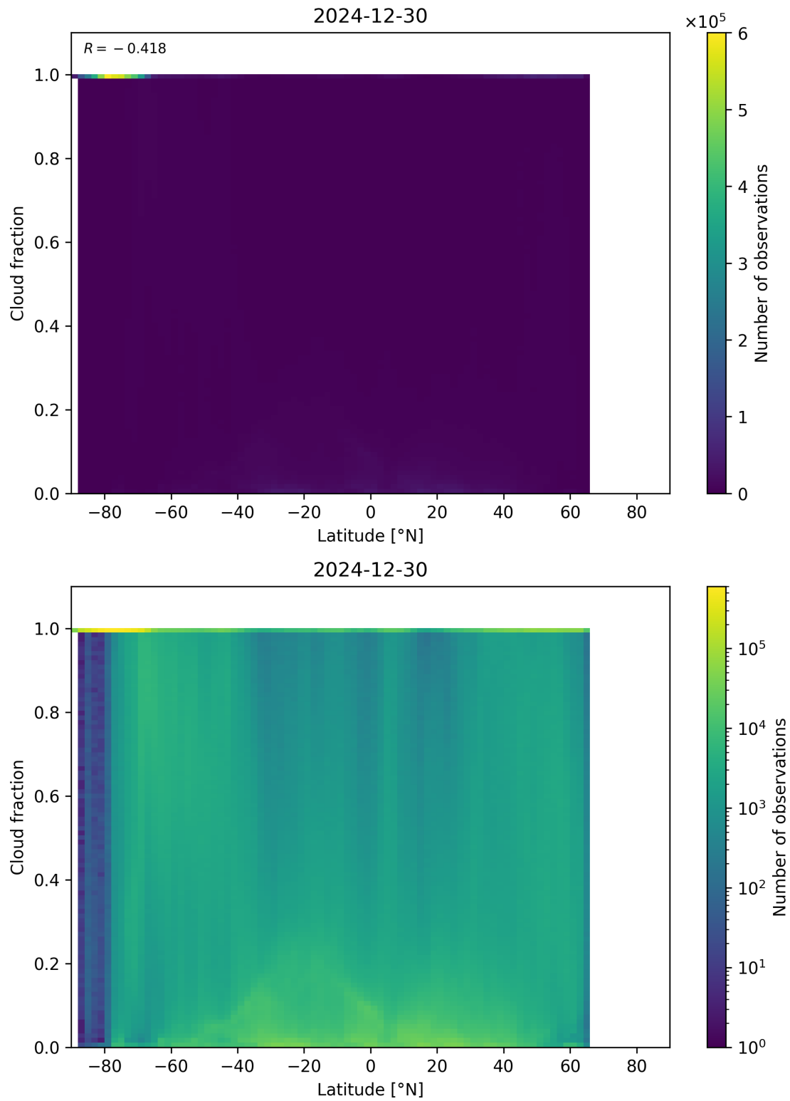
Figure 90: Scatter density plot of “Latitude” against “Cloud fraction” for 2024-12-29 to 2024-12-31.
