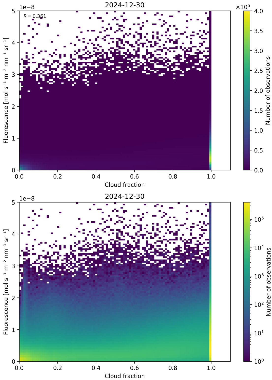
Figure 72: Scatter density plot of “Cloud fraction” against “Fluorescence” for 2024-12-29 to 2024-12-31.
