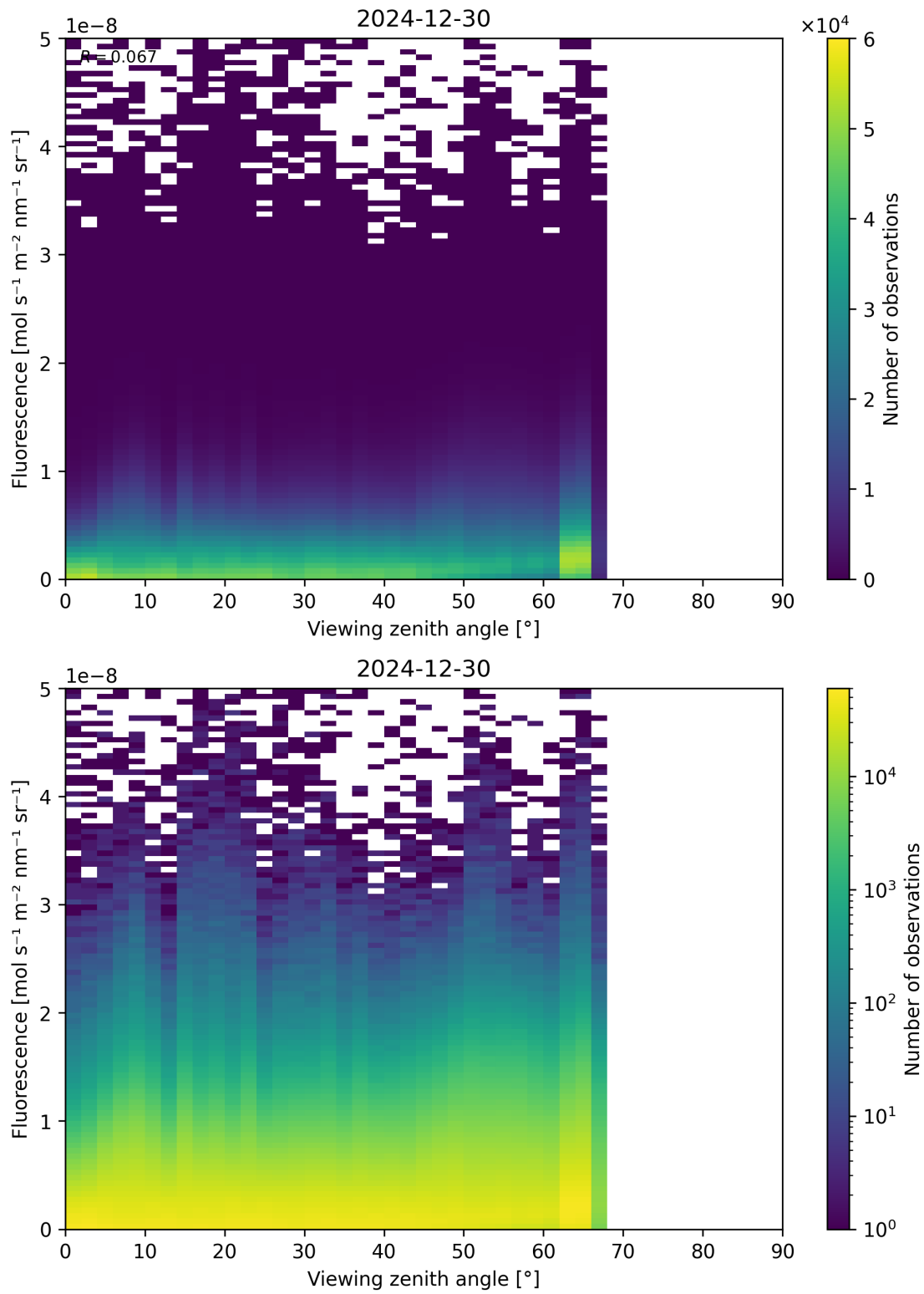
Figure 122: Scatter density plot of “Viewing zenith angle” against “Fluorescence” for 2024-12-29 to 2024-12-31.
