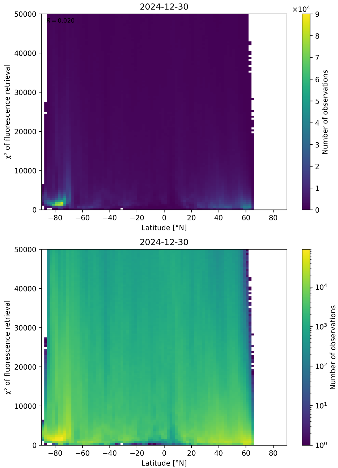
Figure 89: Scatter density plot of “Latitude” against “ \chi^2 of fluorescence retrieval” for 2024-12-29 to 2024-12-31.
