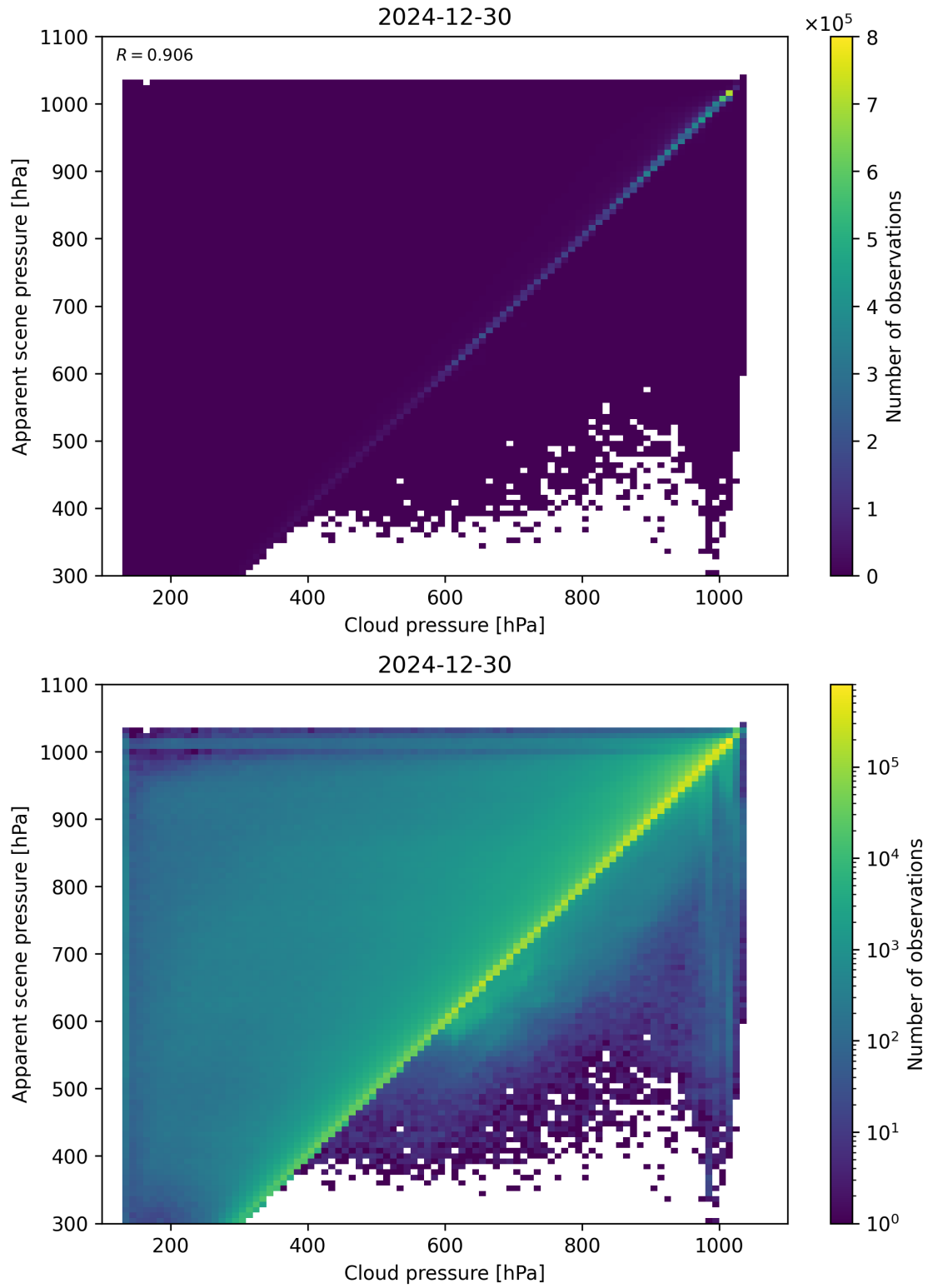
Figure 77: Scatter density plot of “Cloud pressure” against “Apparent scene pressure” for 2024-12-29 to 2024-12-31.
