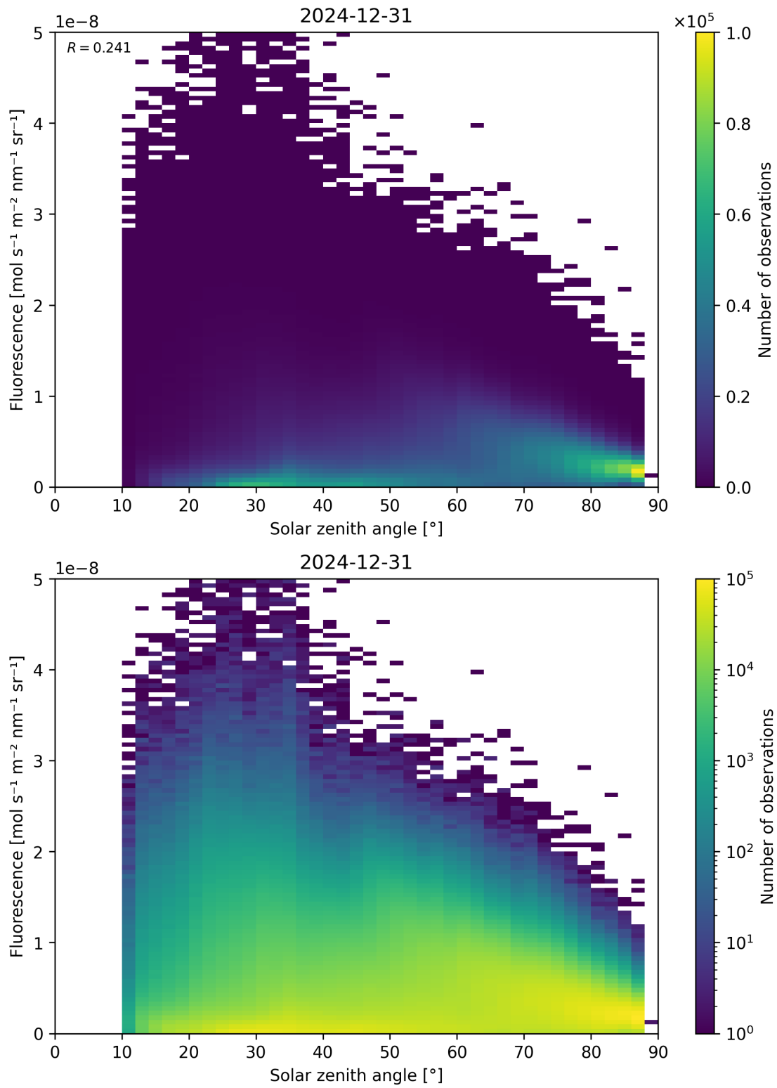
Figure 112: Scatter density plot of “Solar zenith angle” against “Fluorescence” for 2024-12-30 to 2025-01-01.
