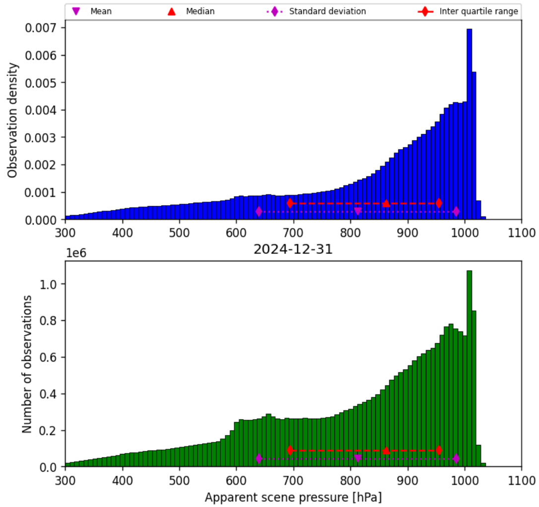
Figure 36: Histogram of “Apparent scene pressure” for 2024-12-30 to 2025-01-01
