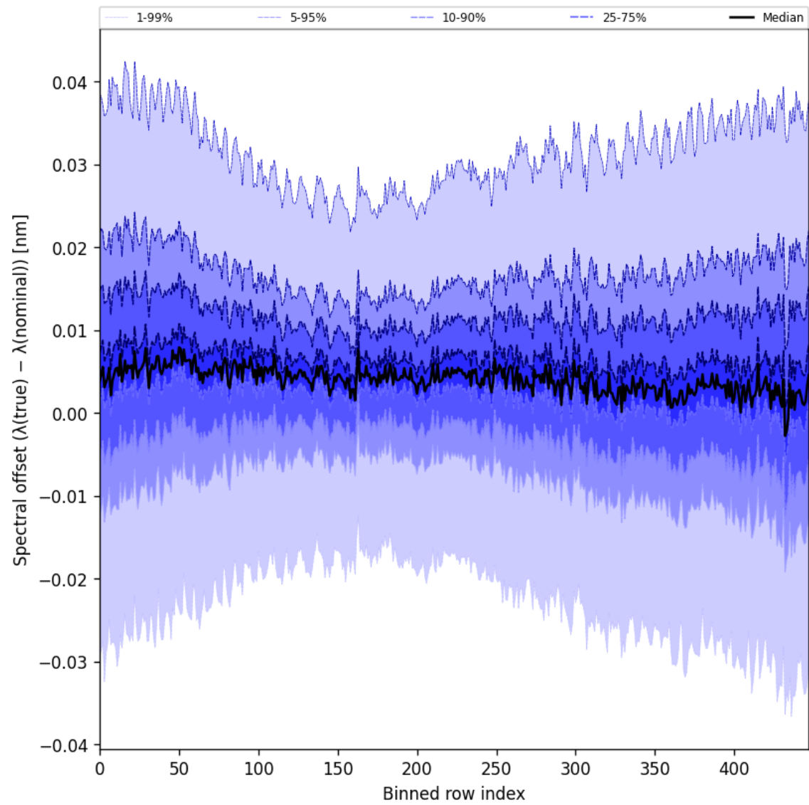
Figure 62: Along track statistics of “Spectral offset ( \lambda_{\text{true}} - \lambda_{\text{nominal}} )” for 2024-12-30 to 2025-01-01
