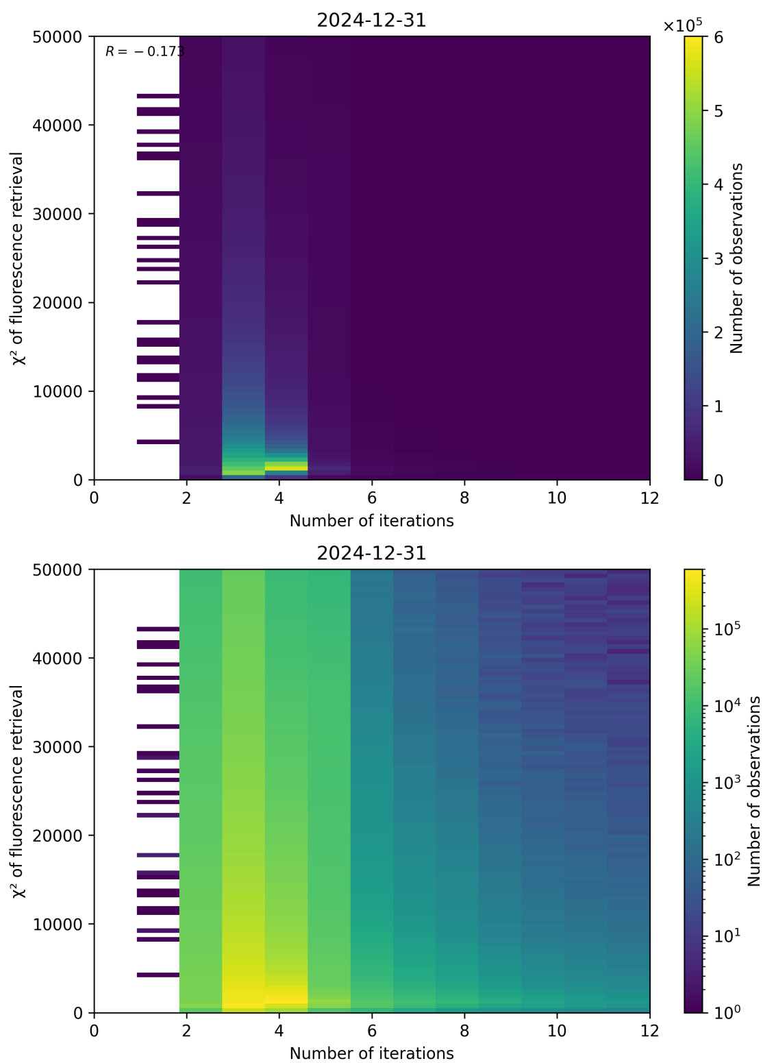
Figure 97: Scatter density plot of “Number of iterations” against “ \chi^2 of fluorescence retrieval” for 2024-12-30 to 2025-01-01.
