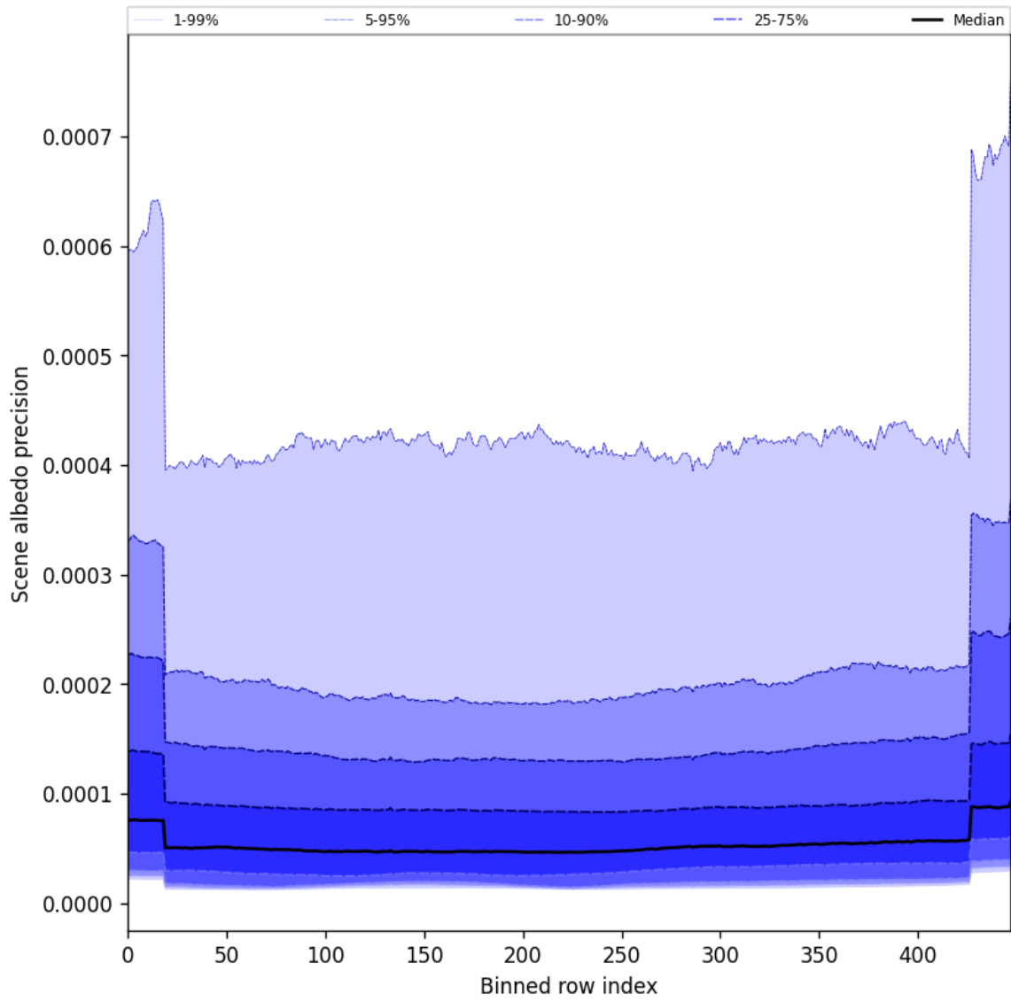
Figure 52: Along track statistics of “Scene albedo precision” for 2024-12-30 to 2025-01-01
