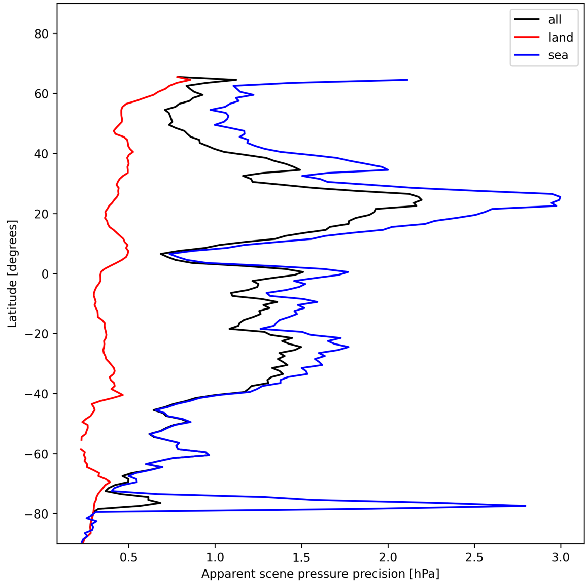
Figure 20: Zonal average of “Apparent scene pressure precision” for 2024-12-30 to 2025-01-01.
