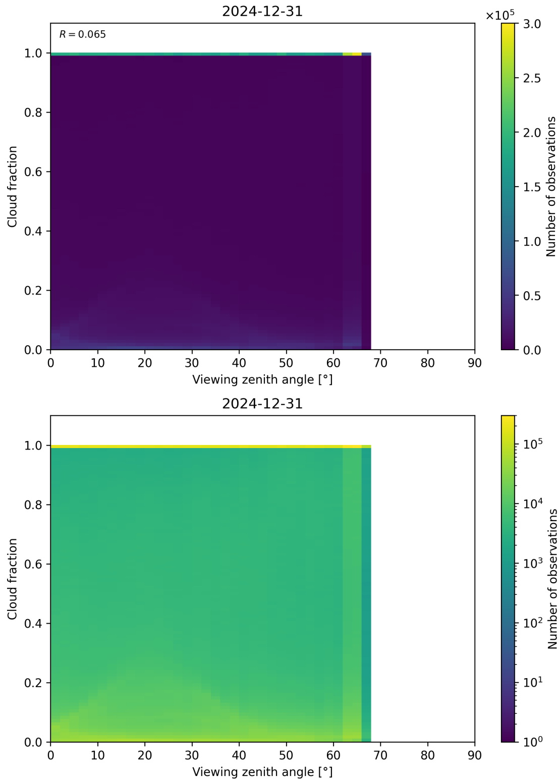
Figure 120: Scatter density plot of “Viewing zenith angle” against “Cloud fraction” for 2024-12-30 to 2025-01-01.
