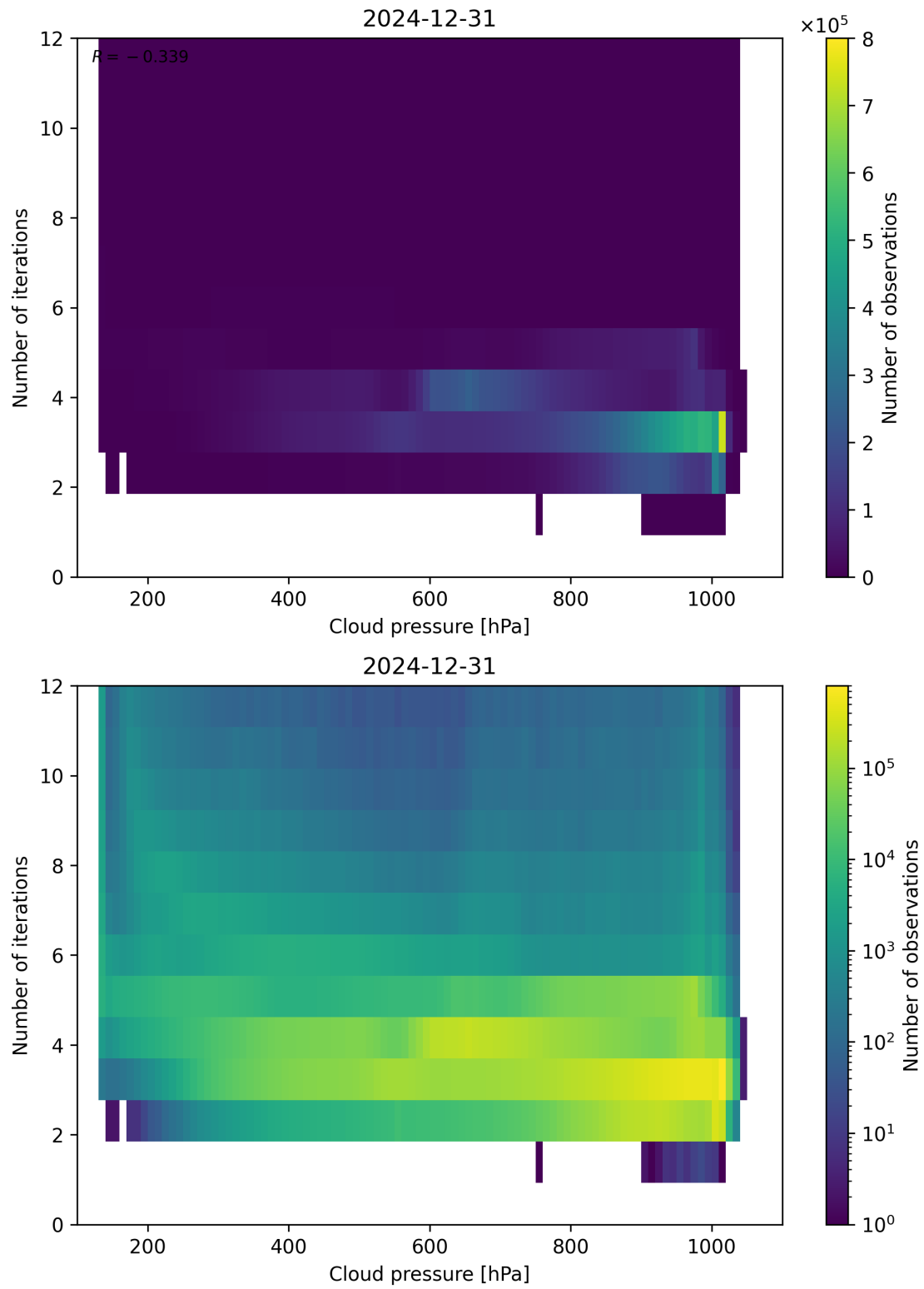
Figure 81: Scatter density plot of “Cloud pressure” against “Number of iterations” for 2024-12-30 to 2025-01-01.
