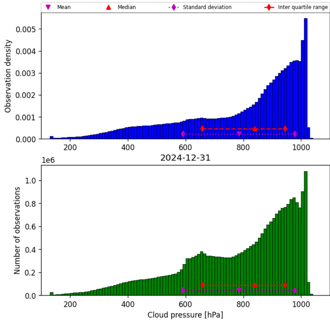
Figure 30: Histogram of “Cloud pressure” for 2024-12-30 to 2025-01-01
