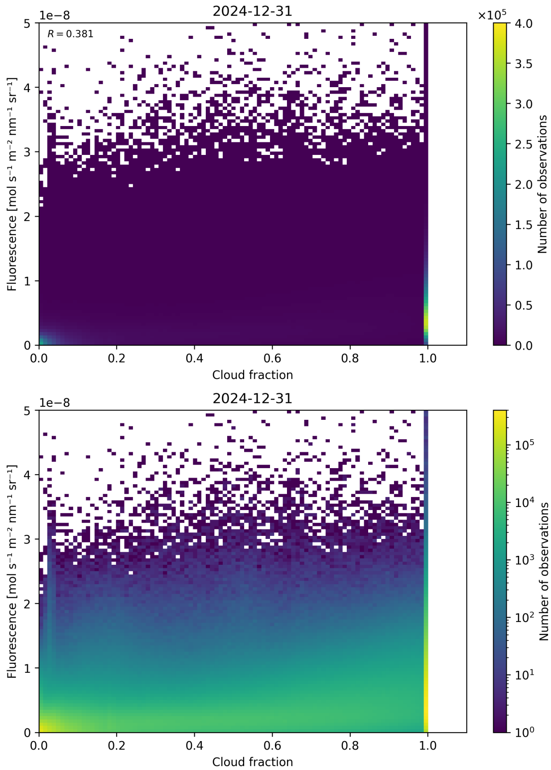
Figure 72: Scatter density plot of “Cloud fraction” against “Fluorescence” for 2024-12-30 to 2025-01-01.
