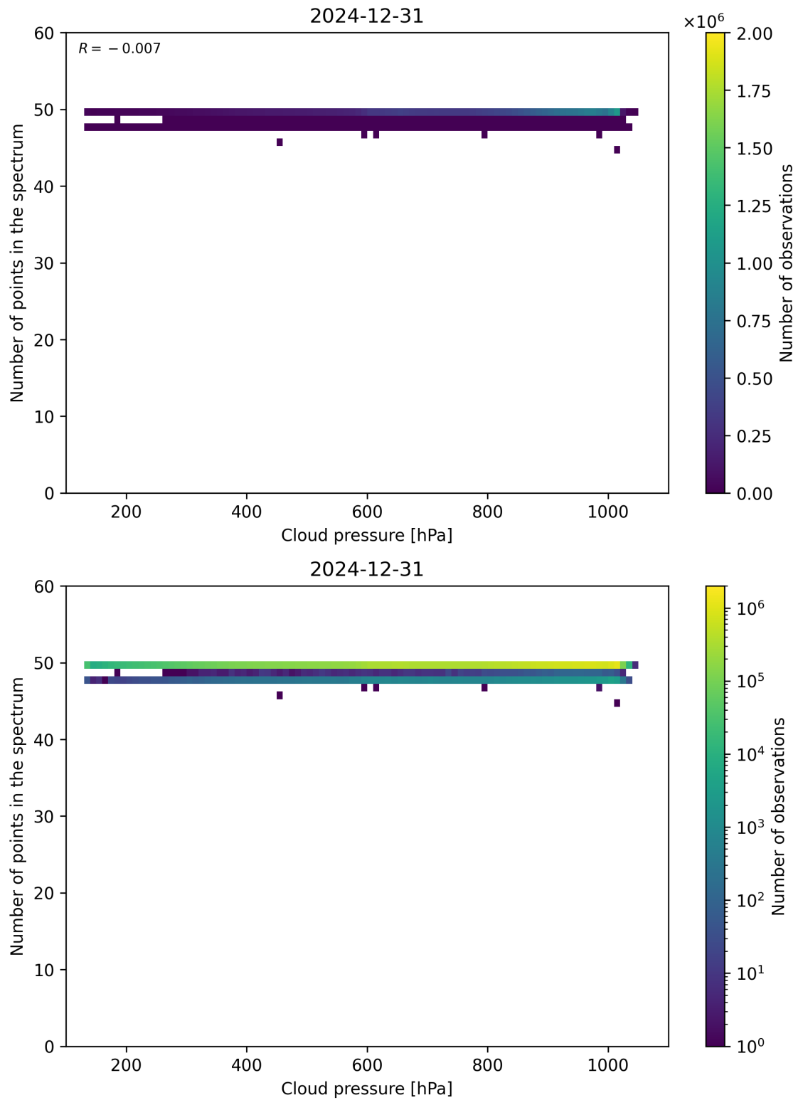
Figure 82: Scatter density plot of “Cloud pressure” against “Number of points in the spectrum” for 2024-12-30 to 2025-01-01.
