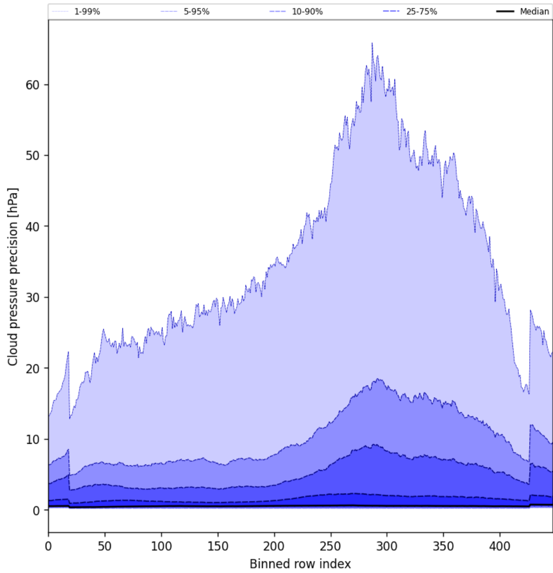
Figure 48: Along track statistics of “Cloud pressure precision” for 2024-12-30 to 2025-01-01
