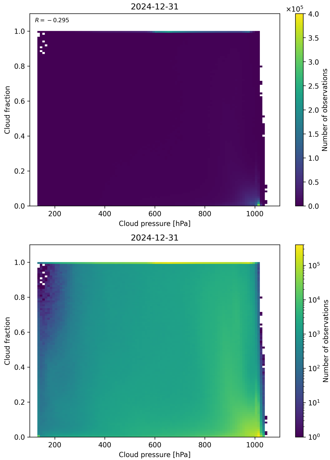
Figure 79: Scatter density plot of “Cloud pressure” against “Cloud fraction” for 2024-12-30 to 2025-01-01.
