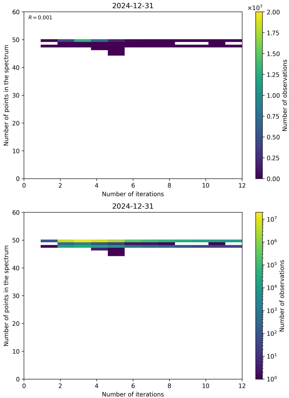
Figure 99: Scatter density plot of “Number of iterations” against “Number of points in the spectrum” for 2024-12-30 to 2025-01-01.
