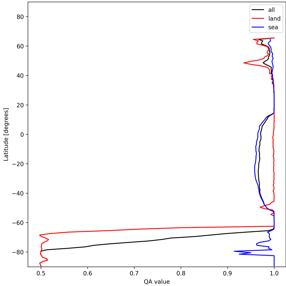
Figure 12: Zonal average of “QA value” for 2024-12-30 to 2025-01-01.
