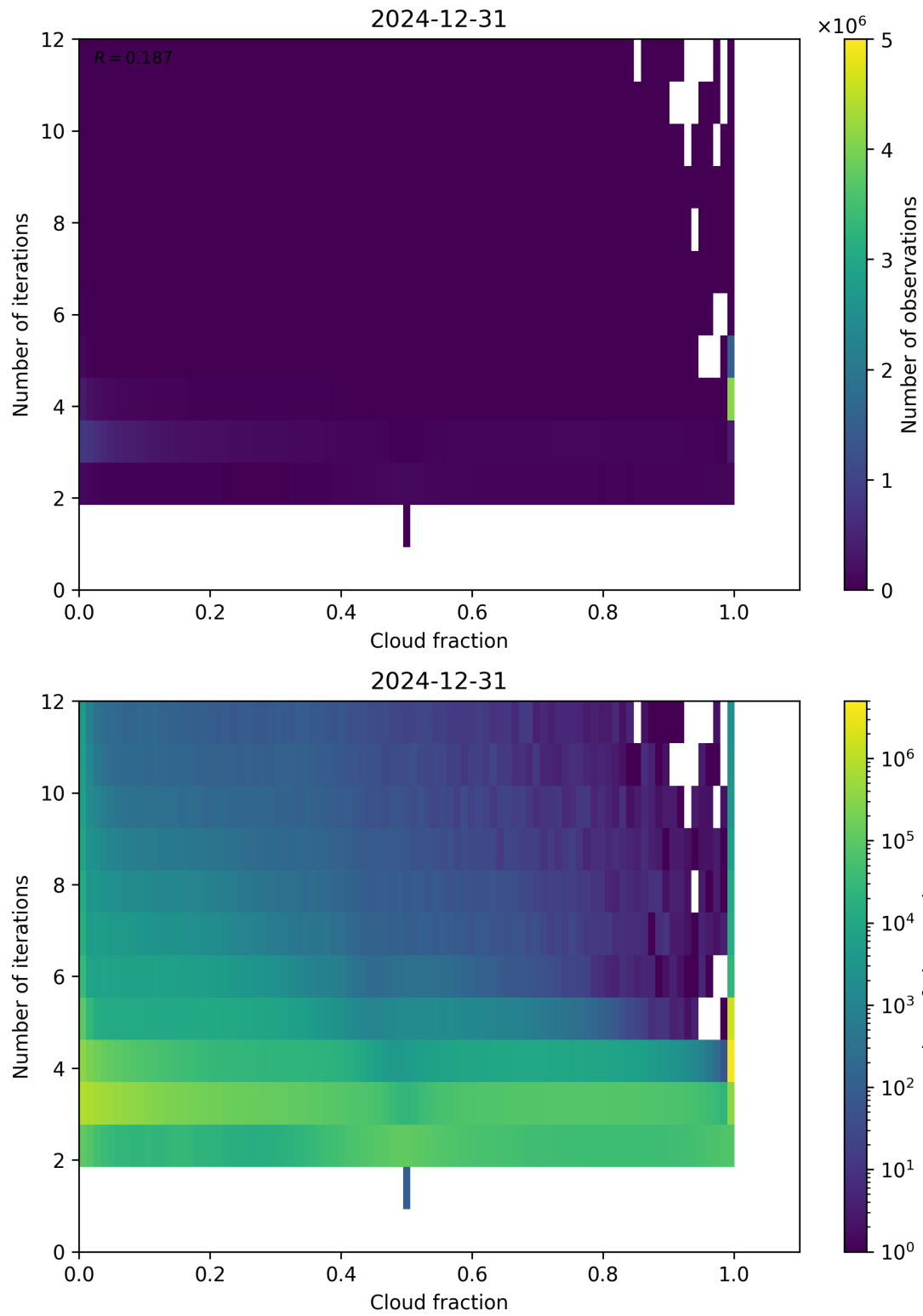
Figure 73: Scatter density plot of “Cloud fraction” against “Number of iterations” for 2024-12-30 to 2025-01-01.
