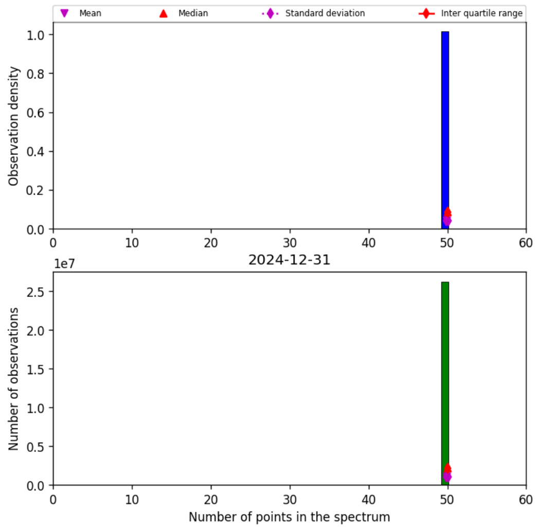
Figure 44: Histogram of “Number of points in the spectrum” for 2024-12-30 to 2025-01-01
