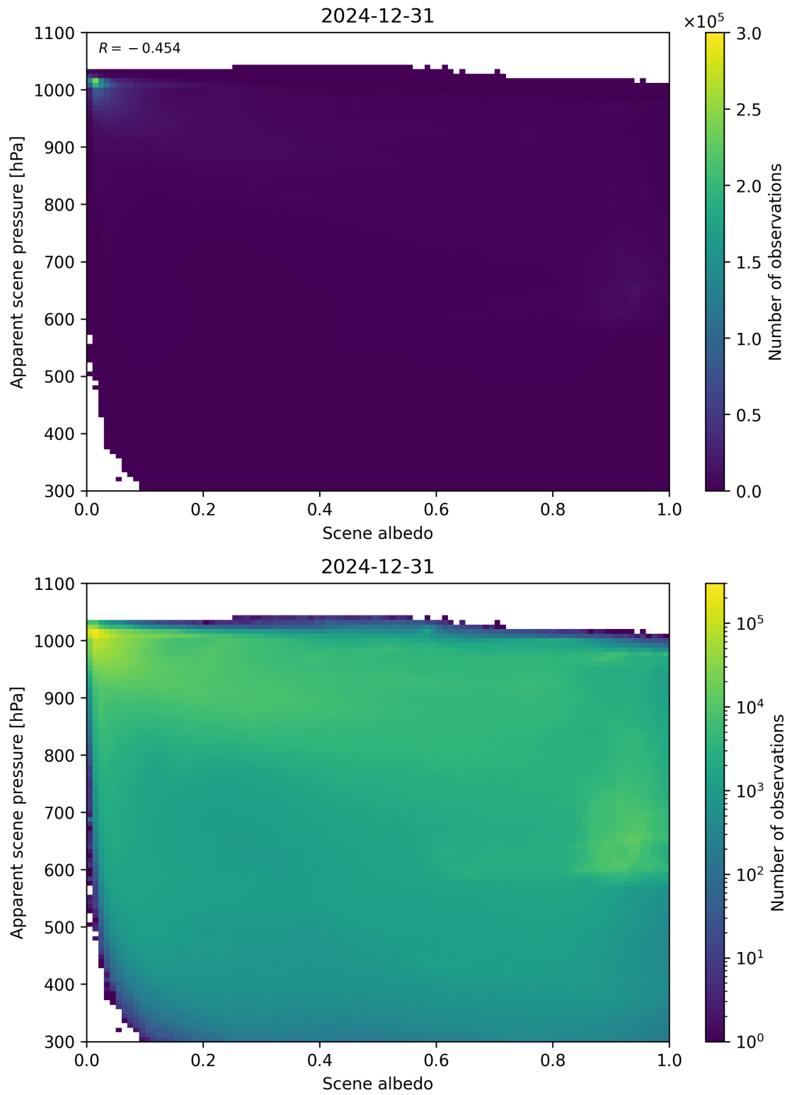
Figure 102: Scatter density plot of “Scene albedo” against “Apparent scene pressure” for 2024-12-30 to 2025-01-01.
