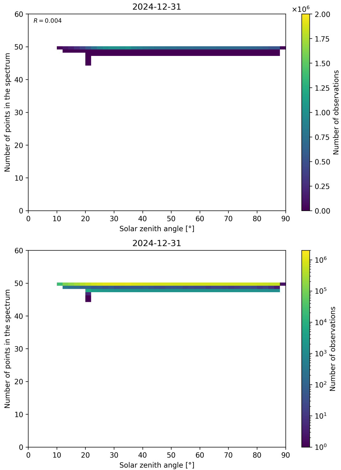
Figure 115: Scatter density plot of “Solar zenith angle” against “Number of points in the spectrum” for 2024-12-30 to 2025-01-01.
