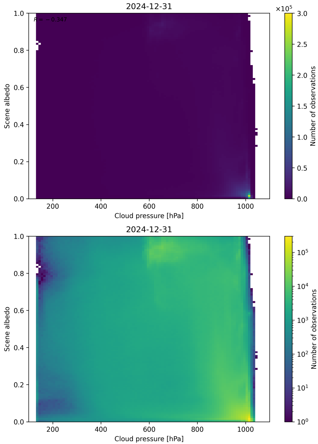
Figure 83: Scatter density plot of “Cloud pressure” against “Scene albedo” for 2024-12-30 to 2025-01-01.
