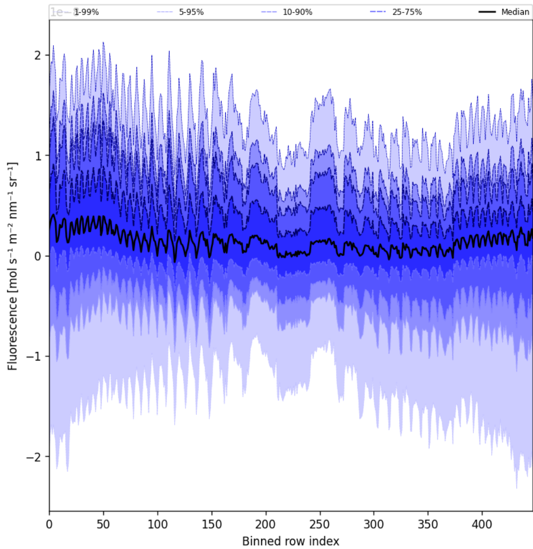
Figure 57: Along track statistics of “Fluorescence” for 2024-12-30 to 2025-01-01
