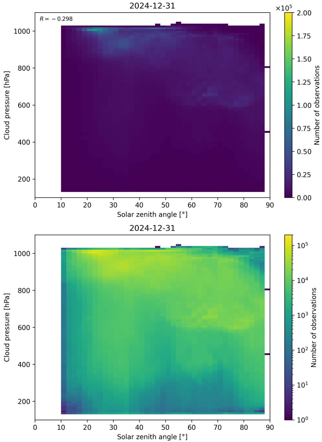
Figure 111: Scatter density plot of “Solar zenith angle” against “Cloud pressure” for 2024-12-30 to 2025-01-01.
