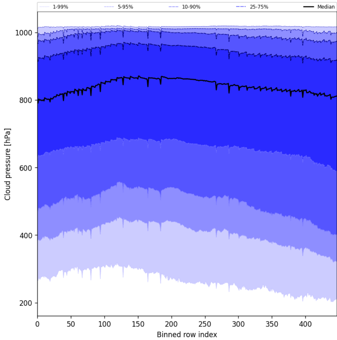
Figure 47: Along track statistics of “Cloud pressure” for 2024-12-30 to 2025-01-01
