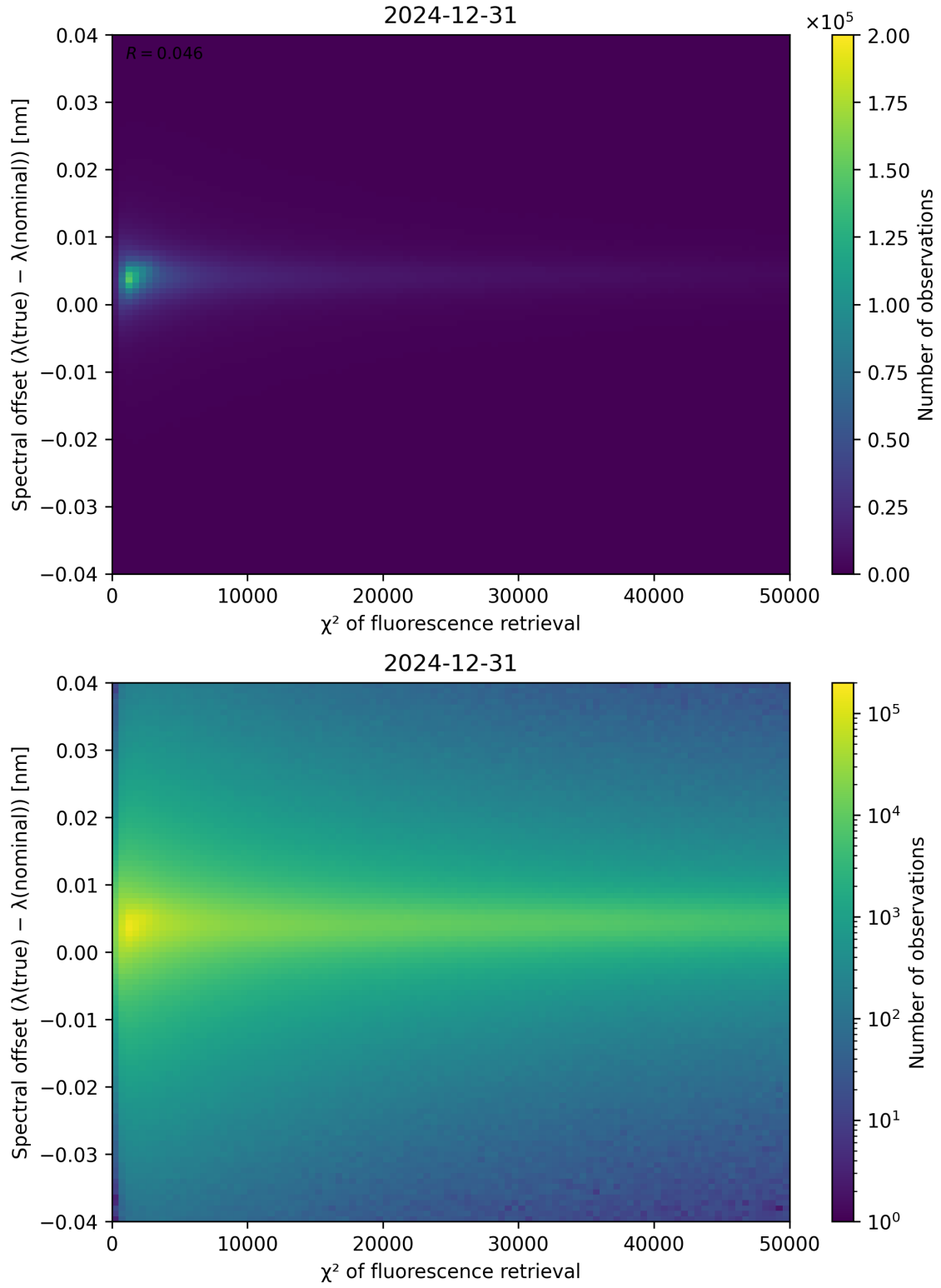
Figure 69: Scatter density plot of “ \chi^2 of fluorescence retrieval” against “Spectral offset ( \lambda_{\text{true}} - \lambda_{\text{nominal}} )” for 2024-12-30 to 2025-01-01.
