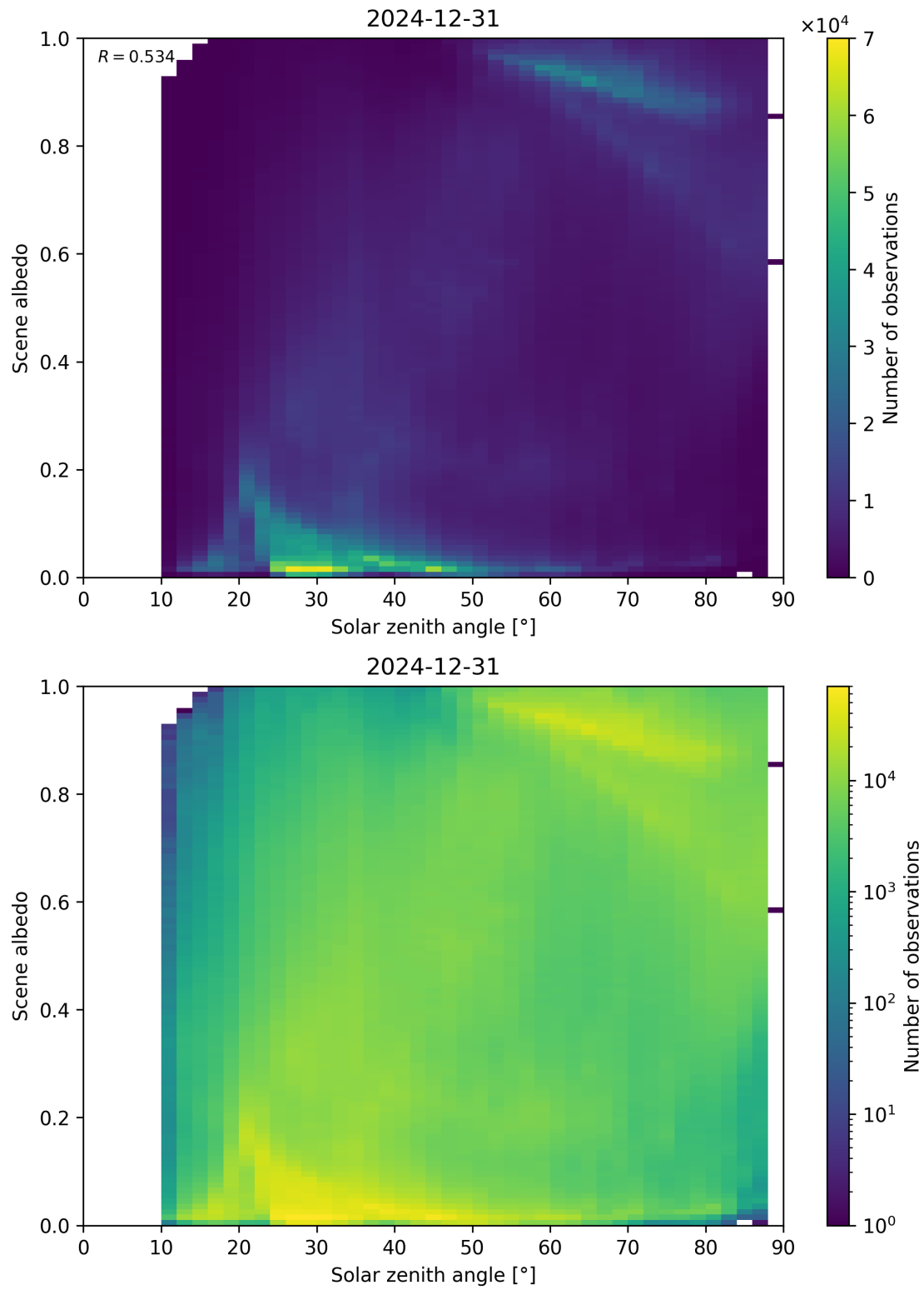
Figure 116: Scatter density plot of “Solar zenith angle” against “Scene albedo” for 2024-12-30 to 2025-01-01.
