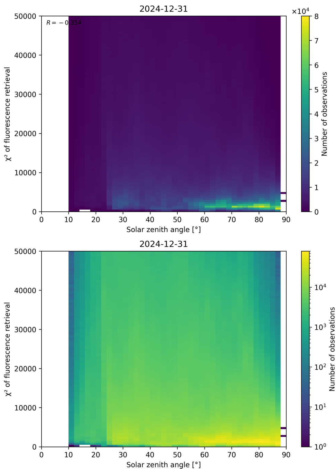
Figure 109: Scatter density plot of “Solar zenith angle” against “ \chi^2 of fluorescence retrieval” for 2024-12-30 to 2025-01-01.
