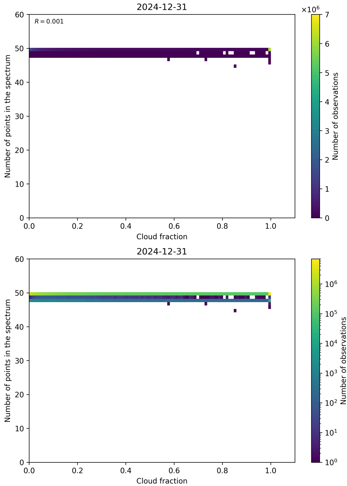
Figure 74: Scatter density plot of “Cloud fraction” against “Number of points in the spectrum” for 2024-12-30 to 2025-01-01.
