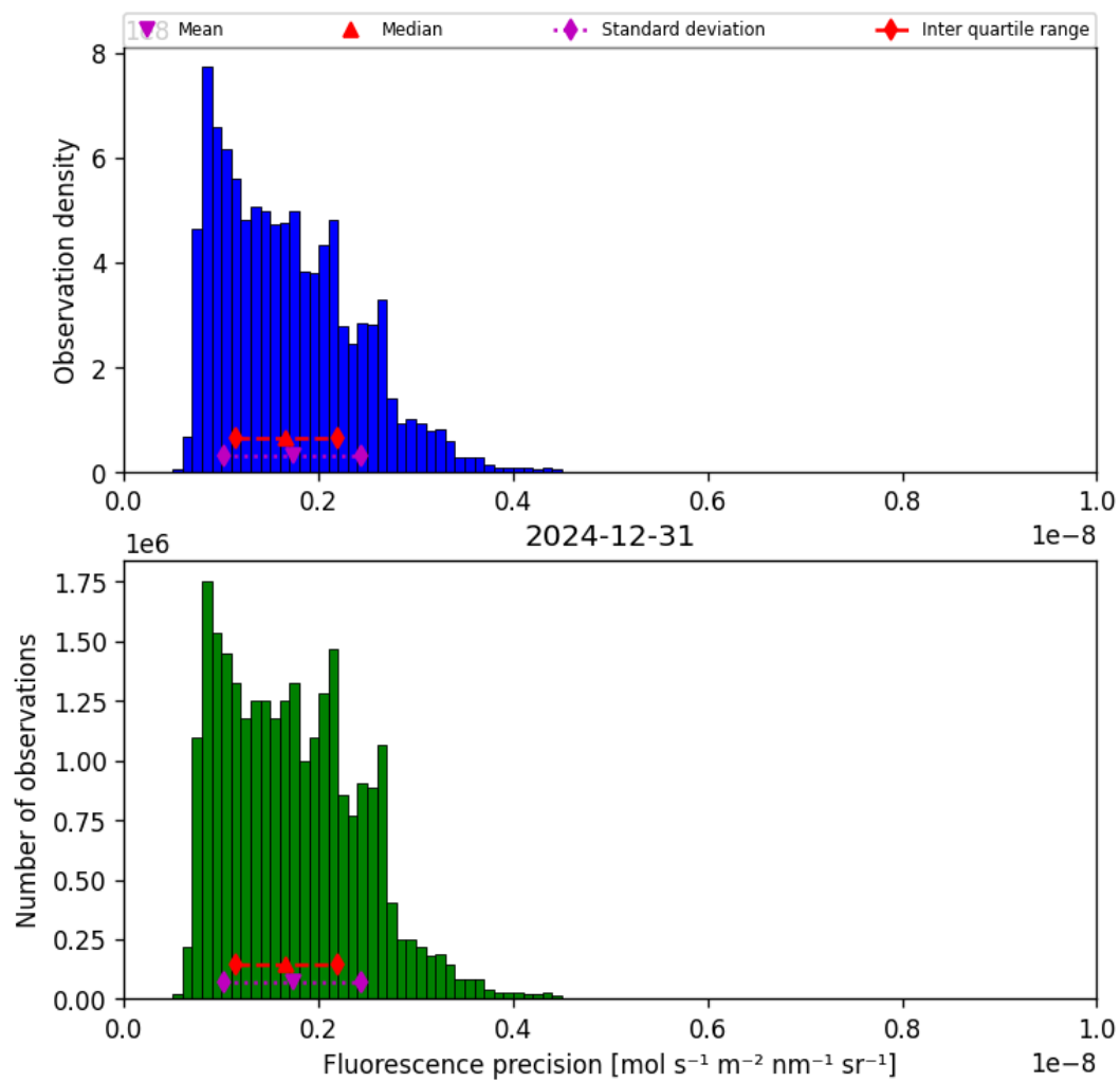
Figure 41: Histogram of “Fluorescence precision” for 2024-12-30 to 2025-01-01
