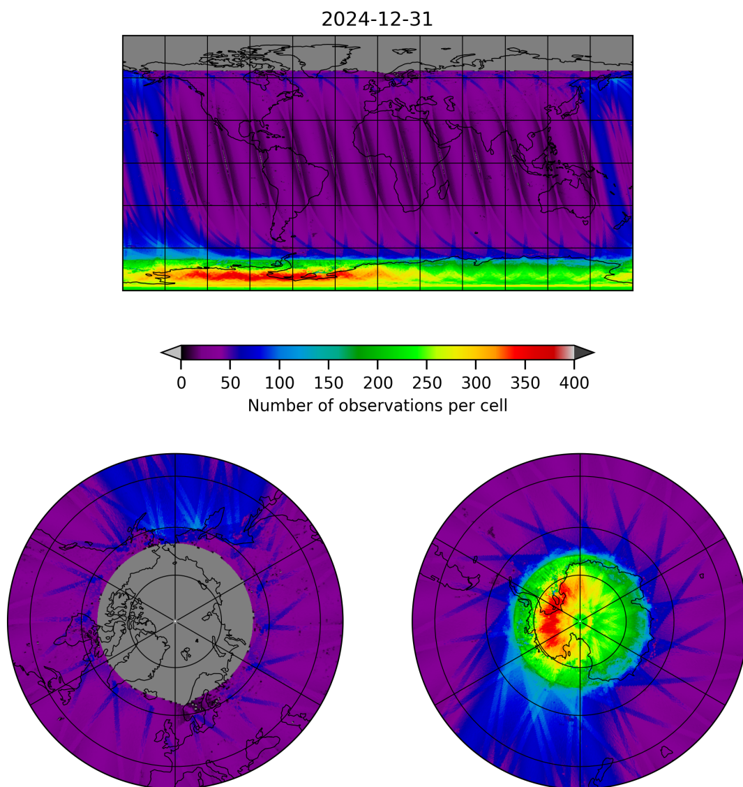
Figure 11: Map of the number of observations for 2024-12-30 to 2025-01-01
