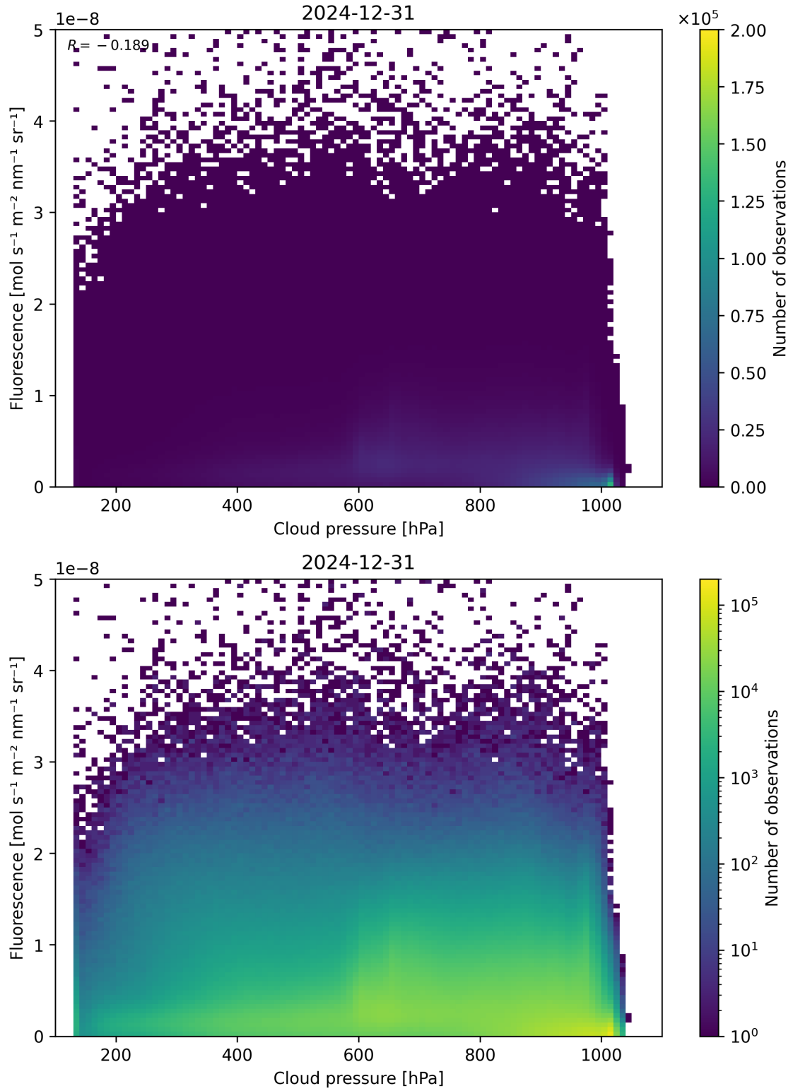
Figure 80: Scatter density plot of “Cloud pressure” against “Fluorescence” for 2024-12-30 to 2025-01-01.
