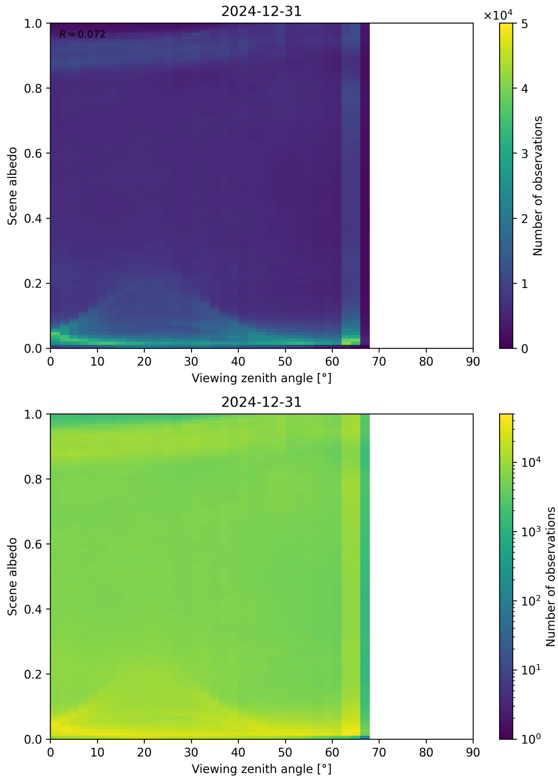
Figure 126: Scatter density plot of “Viewing zenith angle” against “Scene albedo” for 2024-12-30 to 2025-01-01.
