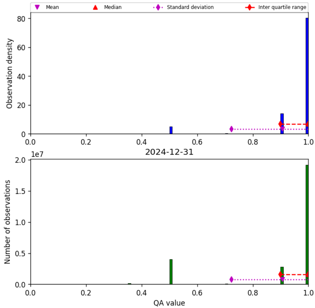
Figure 29: Histogram of “QA value” for 2024-12-30 to 2025-01-01
