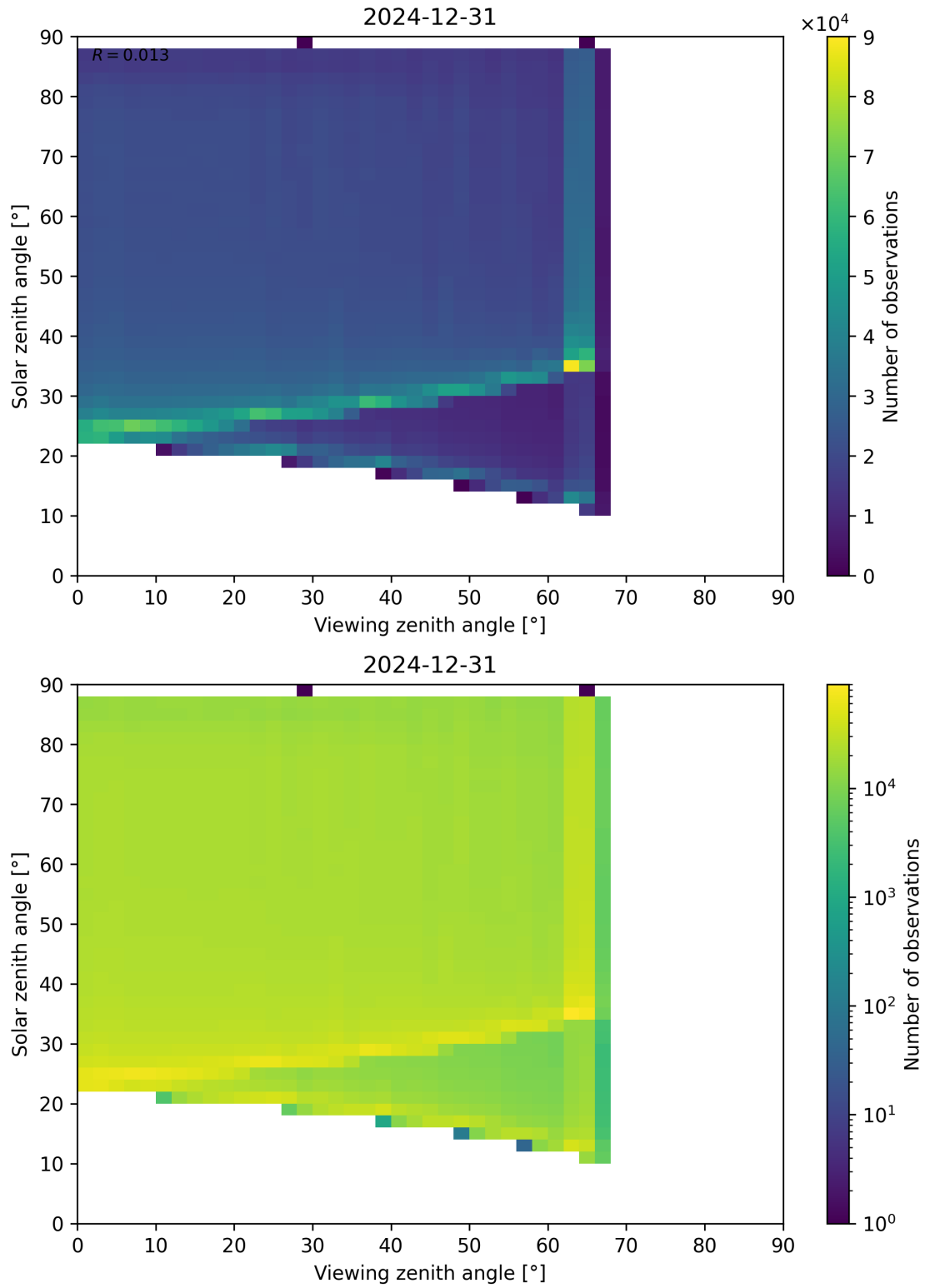
Figure 127: Scatter density plot of “Viewing zenith angle” against “Solar zenith angle” for 2024-12-30 to 2025-01-01.
