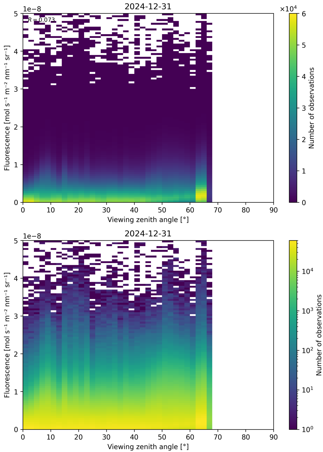
Figure 122: Scatter density plot of “Viewing zenith angle” against “Fluorescence” for 2024-12-30 to 2025-01-01.
