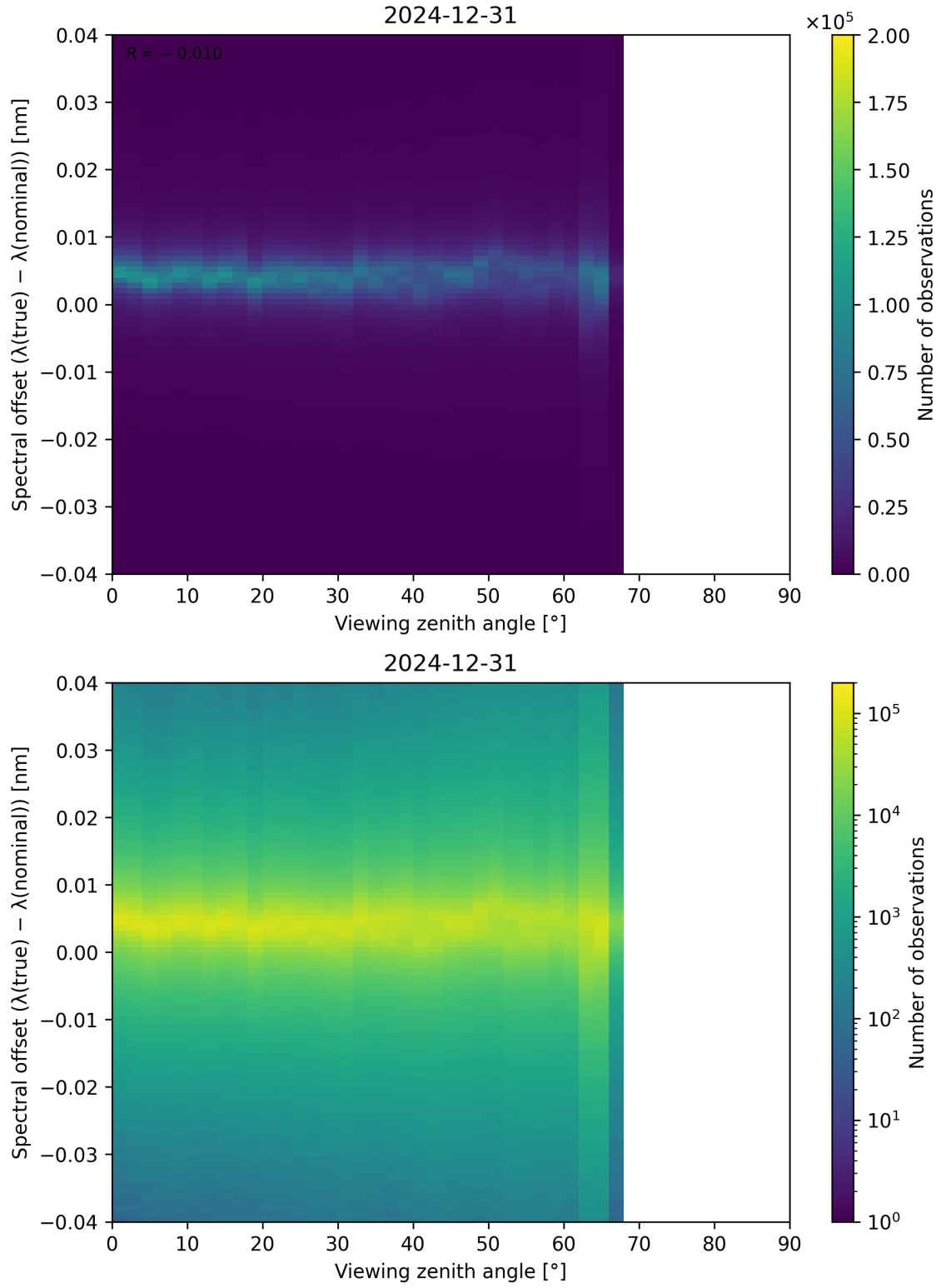
Figure 128: Scatter density plot of “Viewing zenith angle” against “Spectral offset ( \lambda_{\text{true}} - \lambda_{\text{nominal}} )” for 2024-12-30 to 2025-01-01.
