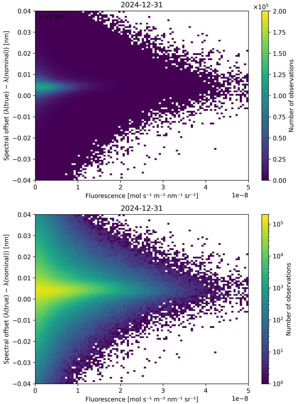
Figure 87: Scatter density plot of “Fluorescence” against “Spectral offset ( \lambda_{\text{true}} - \lambda_{\text{nominal}} )” for 2024-12-30 to 2025-01-01.
