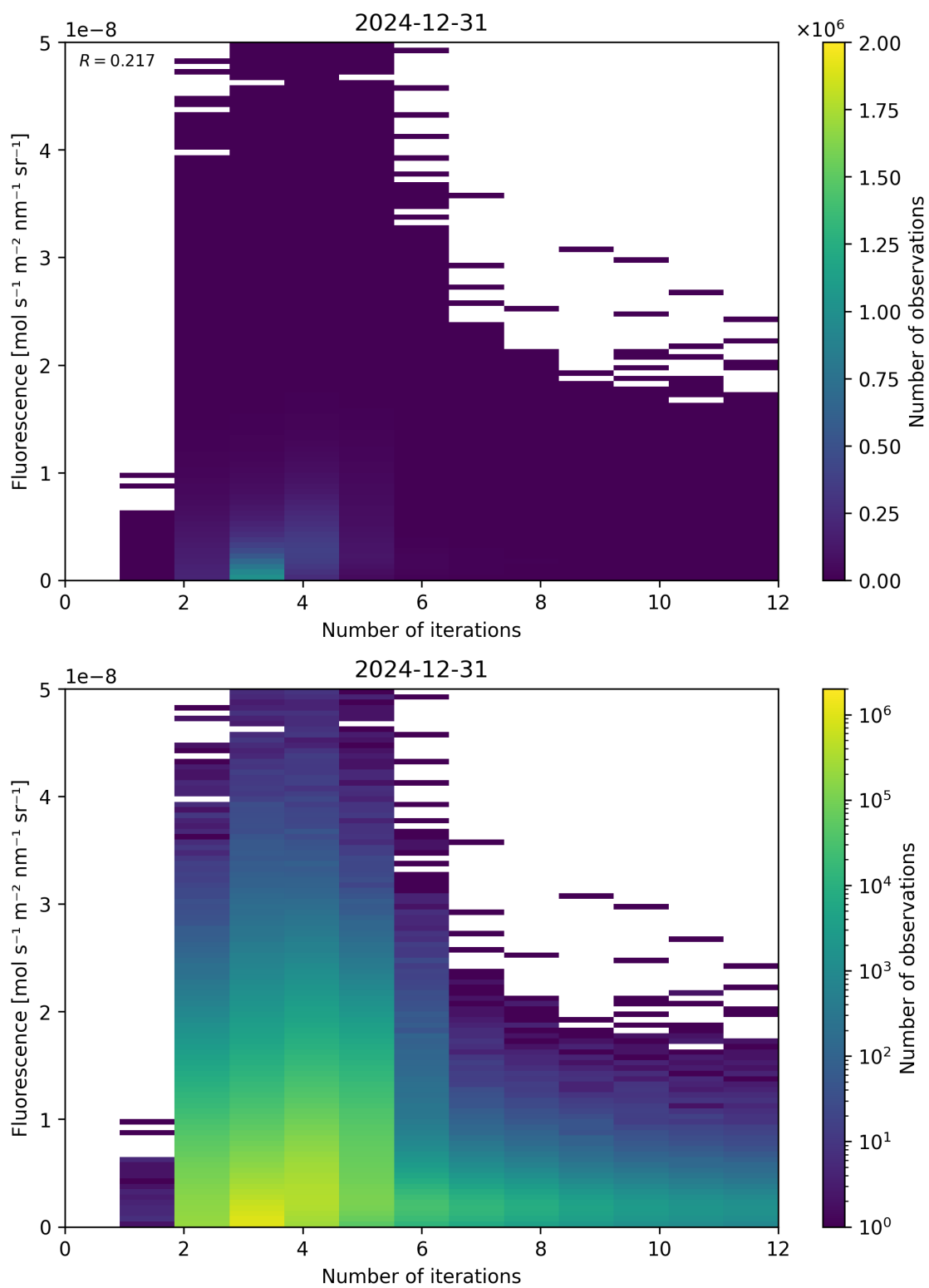
Figure 98: Scatter density plot of “Number of iterations” against “Fluorescence” for 2024-12-30 to 2025-01-01.
