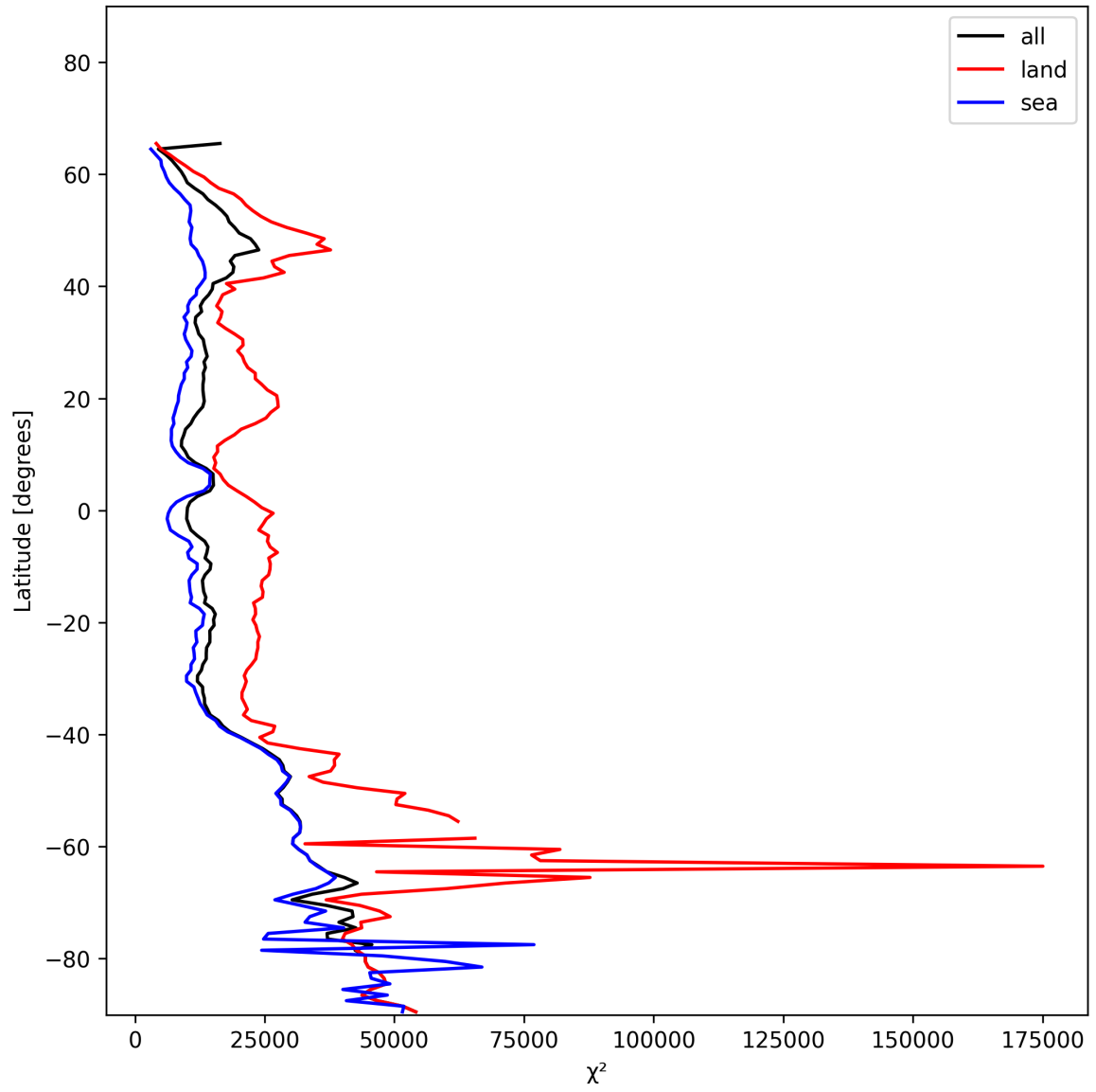
Figure 21: Zonal average of “ \chi^2 ” for 2024-12-30 to 2025-01-01.
