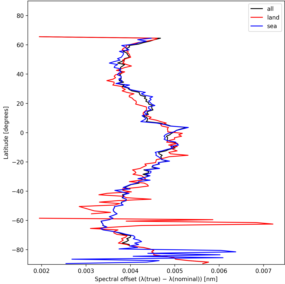
Figure 28: Zonal average of “Spectral offset ( \lambda_{\text{true}} - \lambda_{\text{nominal}} )” for 2024-12-30 to 2025-01-01.
