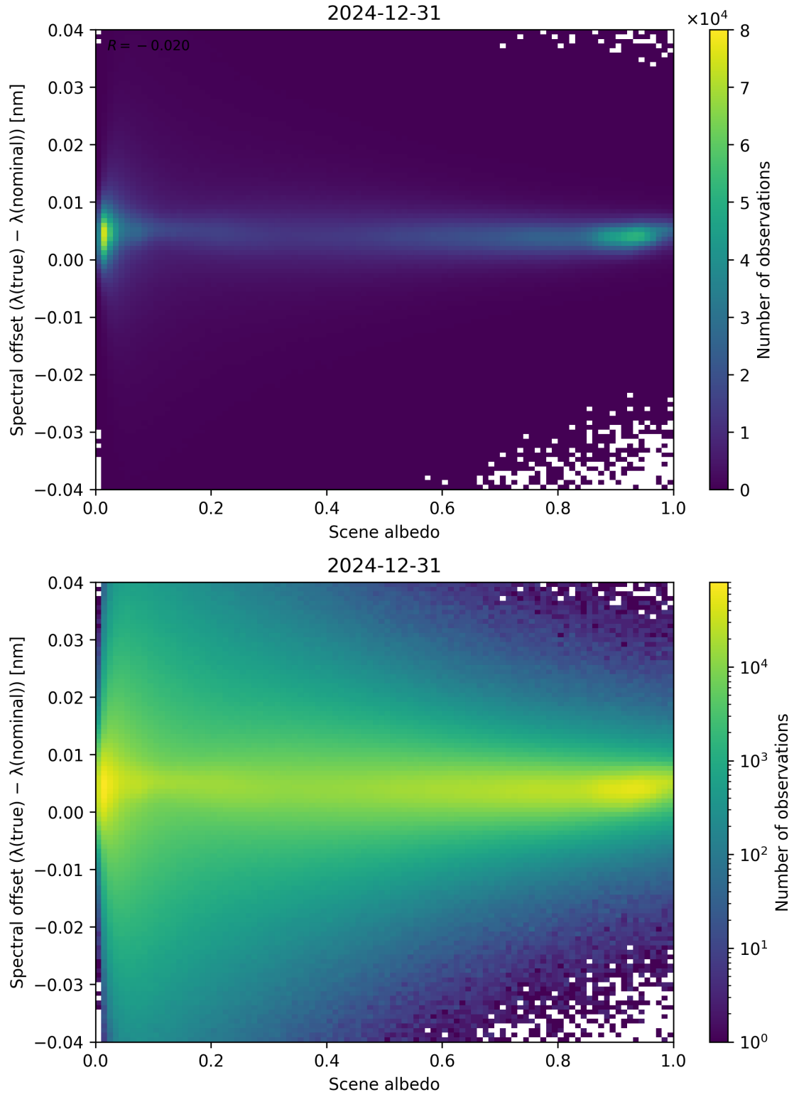
Figure 107: Scatter density plot of “Scene albedo” against “Spectral offset ( \lambda_{\text{true}} - \lambda_{\text{nominal}} )” for 2024-12-30 to 2025-01-01.
