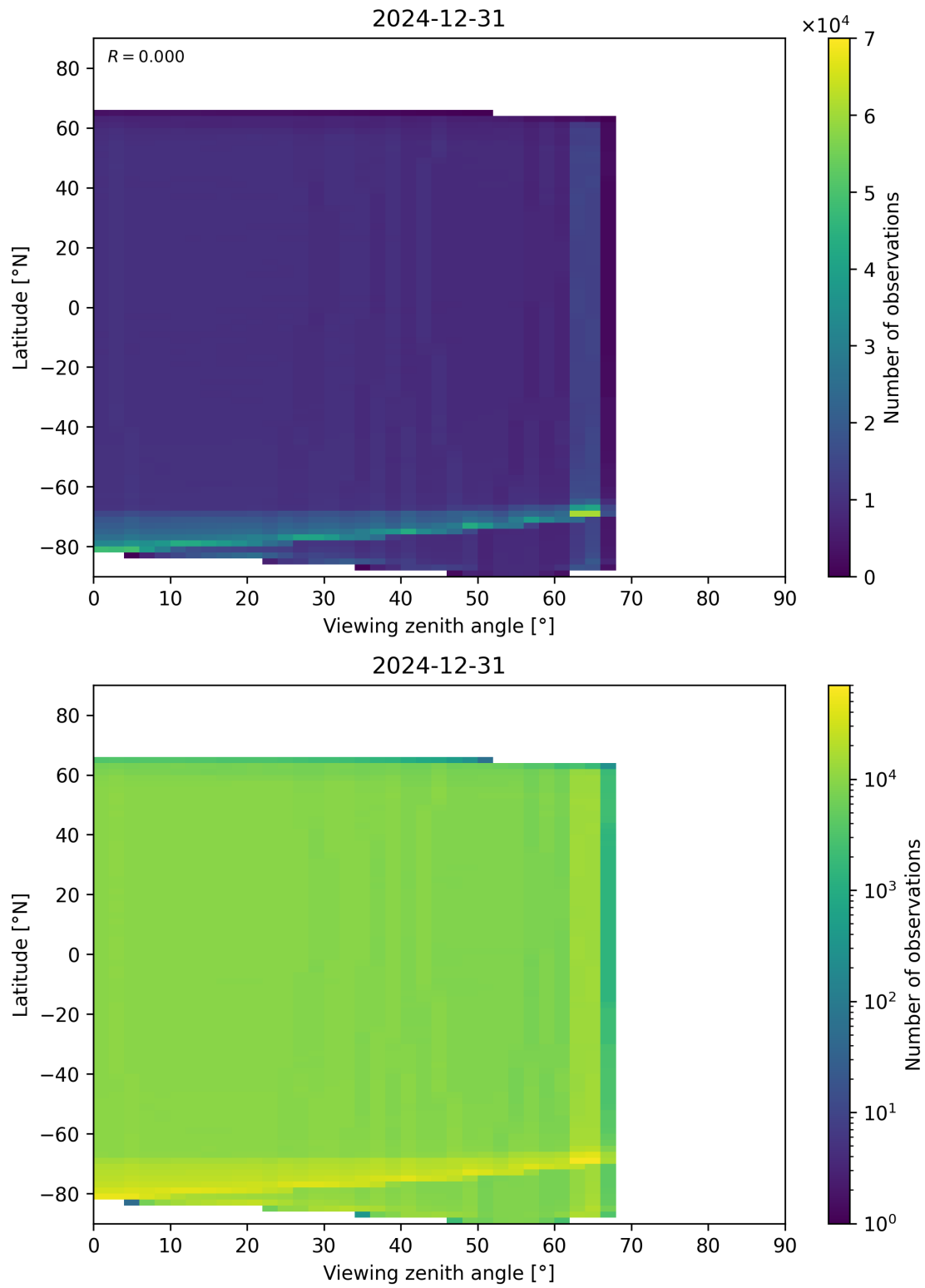
Figure 123: Scatter density plot of “Viewing zenith angle” against “Latitude” for 2024-12-30 to 2025-01-01.
