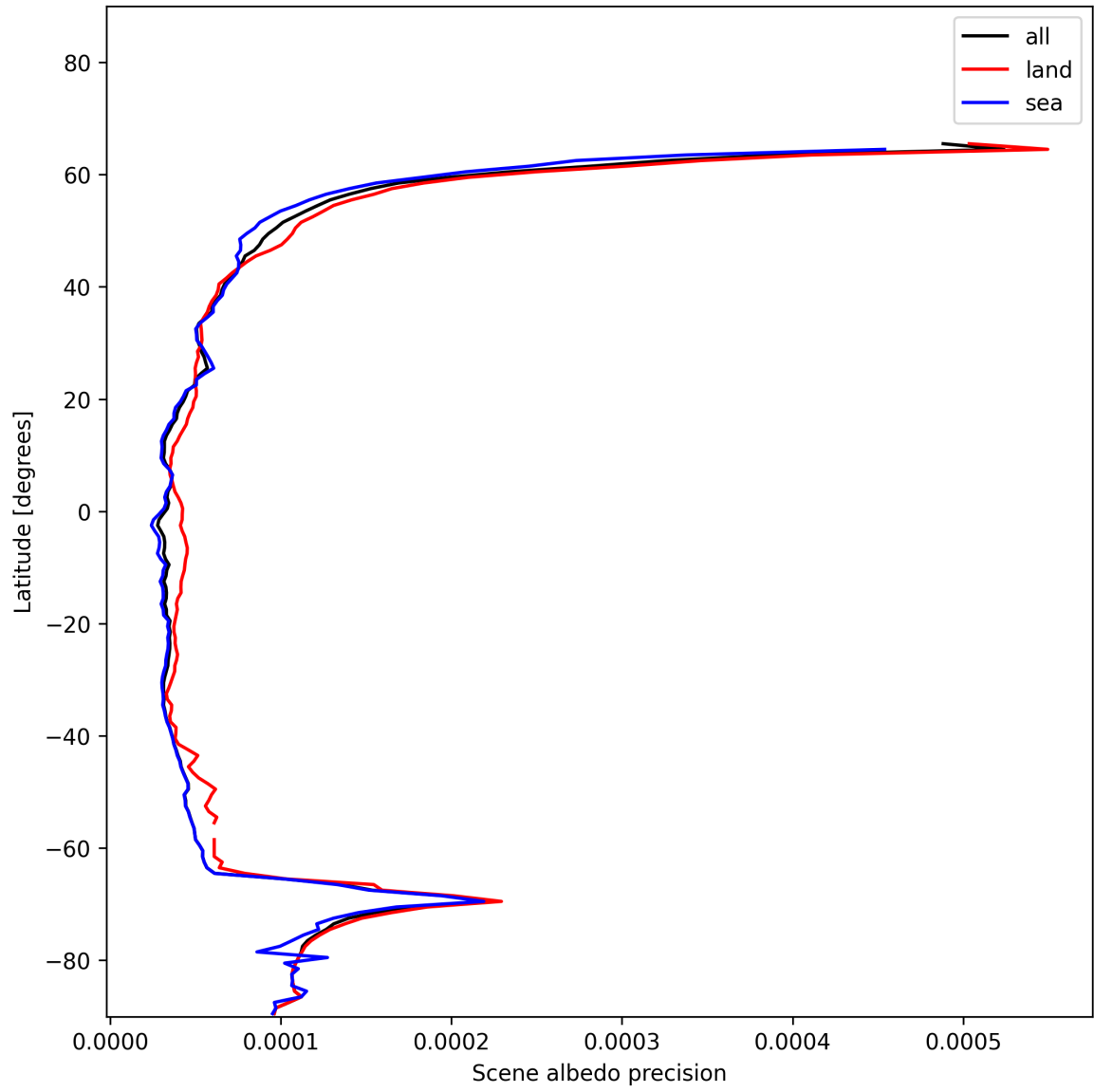
Figure 18: Zonal average of “Scene albedo precision” for 2024-12-30 to 2025-01-01.
