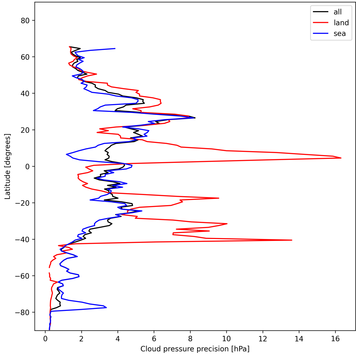
Figure 14: Zonal average of “Cloud pressure precision” for 2024-12-30 to 2025-01-01.
