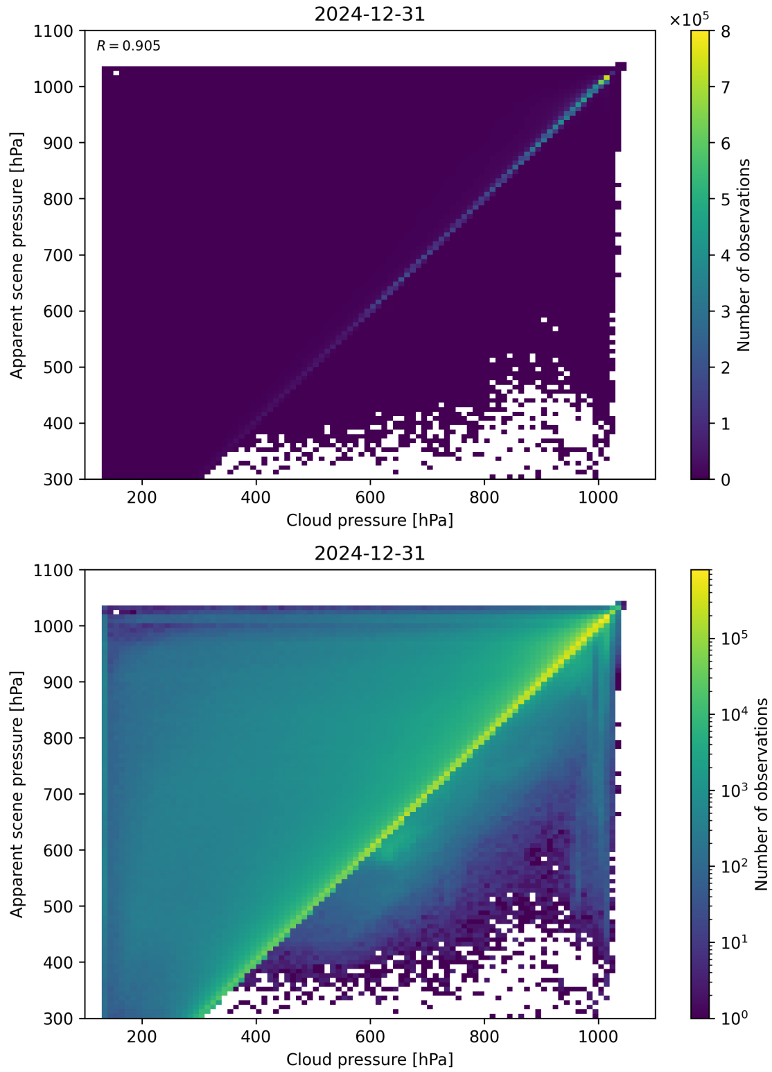
Figure 77: Scatter density plot of “Cloud pressure” against “Apparent scene pressure” for 2024-12-30 to 2025-01-01.
