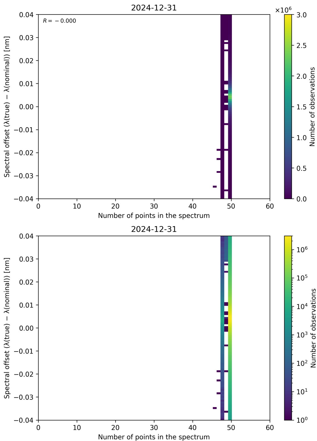
Figure 101: Scatter density plot of “Number of points in the spectrum” against “Spectral offset ( \lambda_{\text{true}} - \lambda_{\text{nominal}} )” for 2024-12-30 to 2025-01-01.
