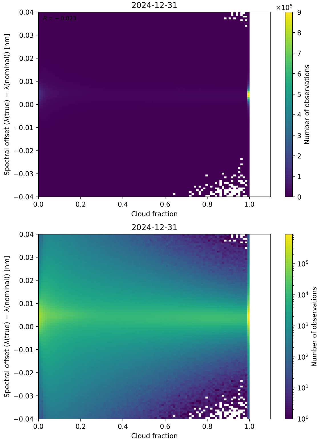
Figure 76: Scatter density plot of “Cloud fraction” against “Spectral offset ( \lambda_{\text{true}} - \lambda_{\text{nominal}} )” for 2024-12-30 to 2025-01-01.
