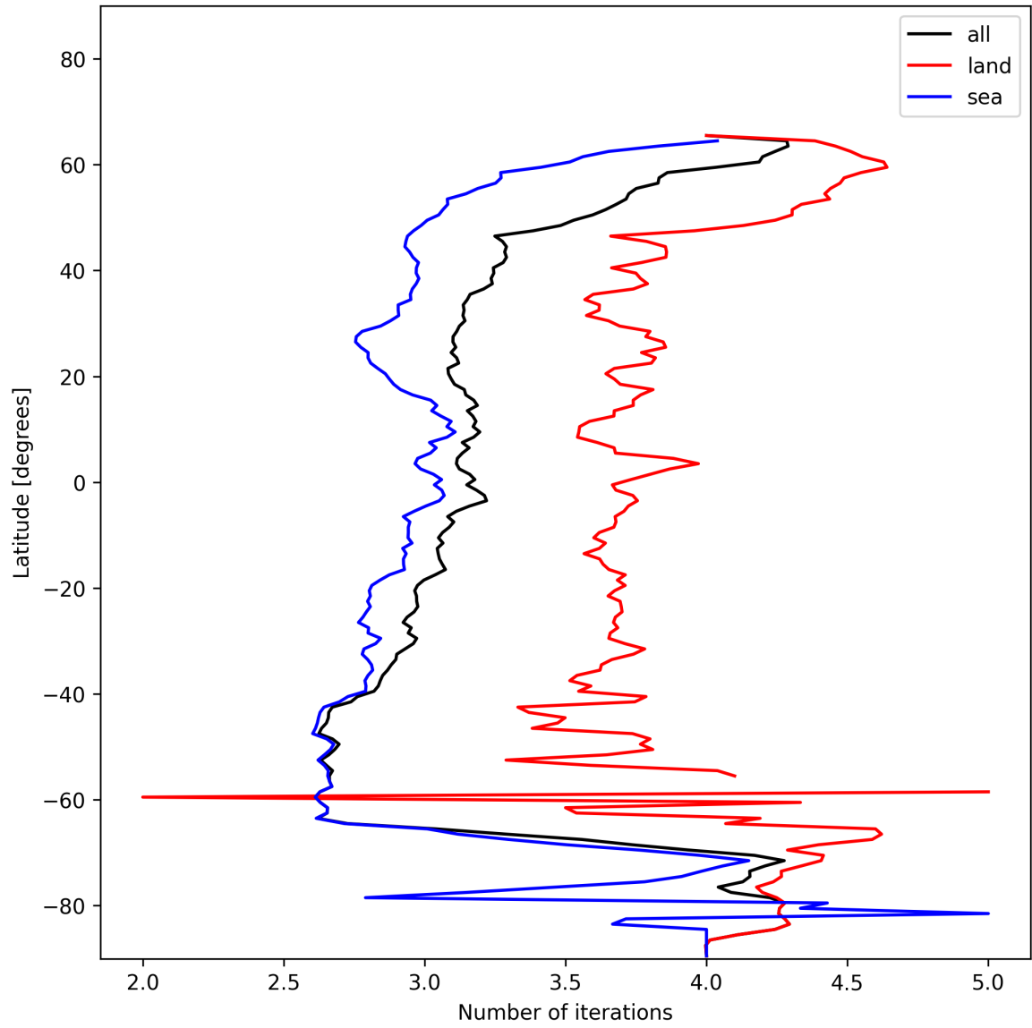
Figure 22: Zonal average of “Number of iterations” for 2024-12-30 to 2025-01-01.
