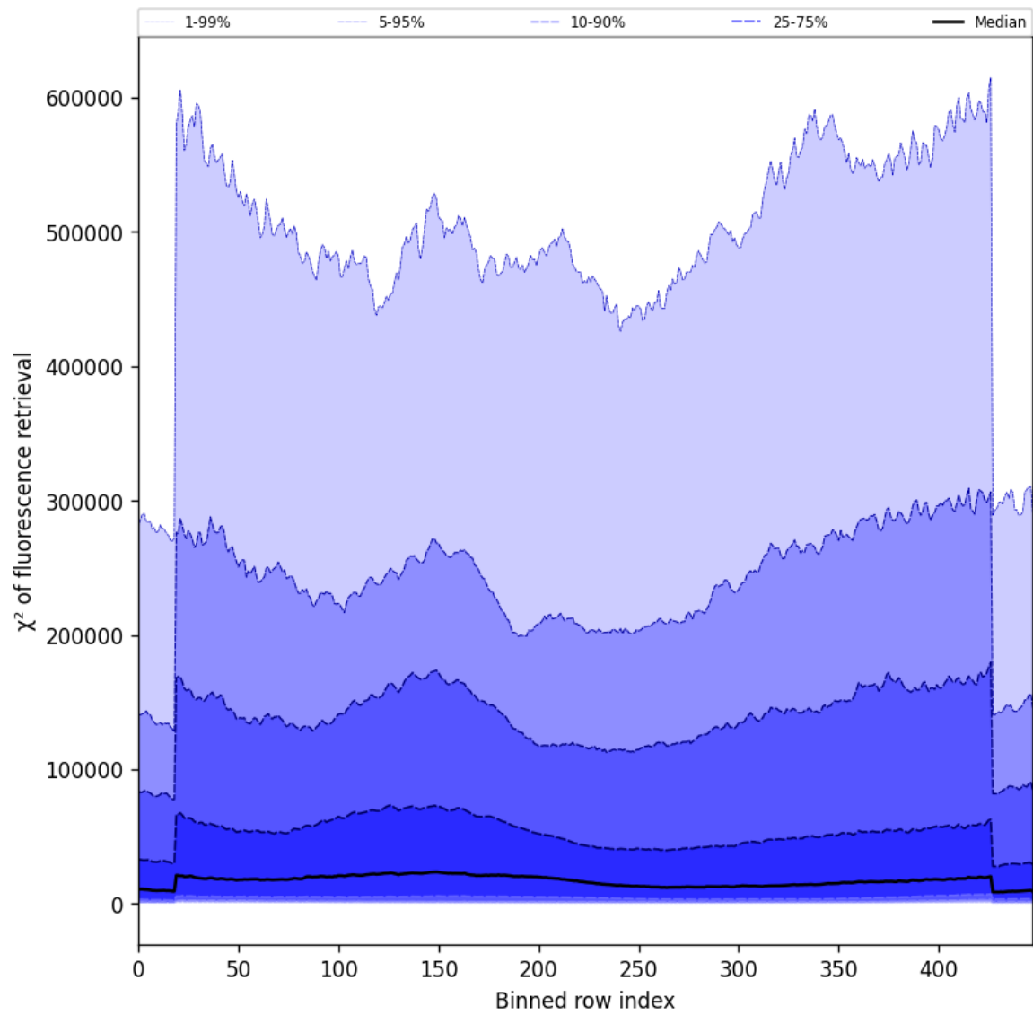
Figure 59: Along track statistics of “ \chi^2 of fluorescence retrieval” for 2024-12-30 to 2025-01-01
