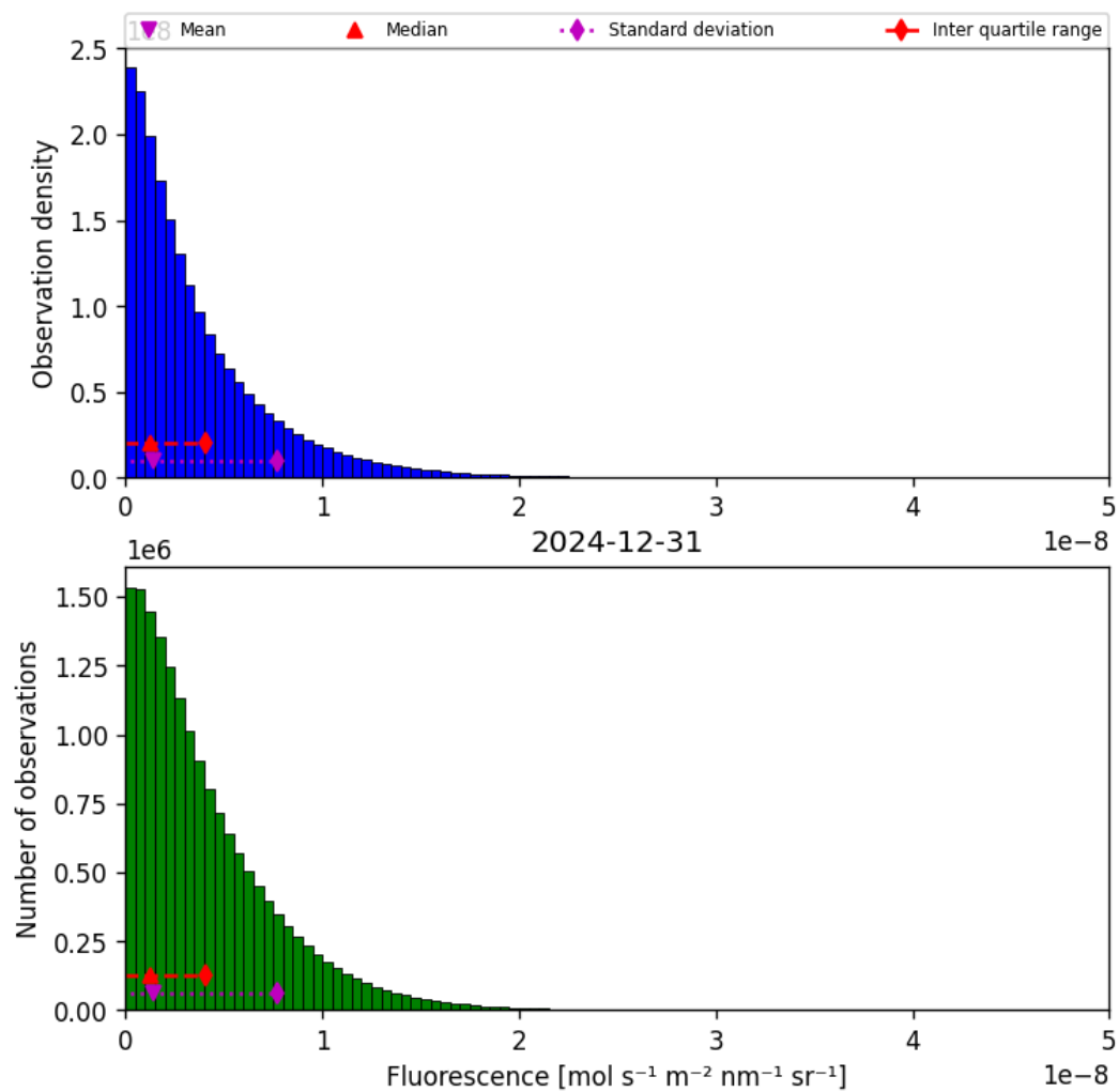
Figure 40: Histogram of “Fluorescence” for 2024-12-30 to 2025-01-01
