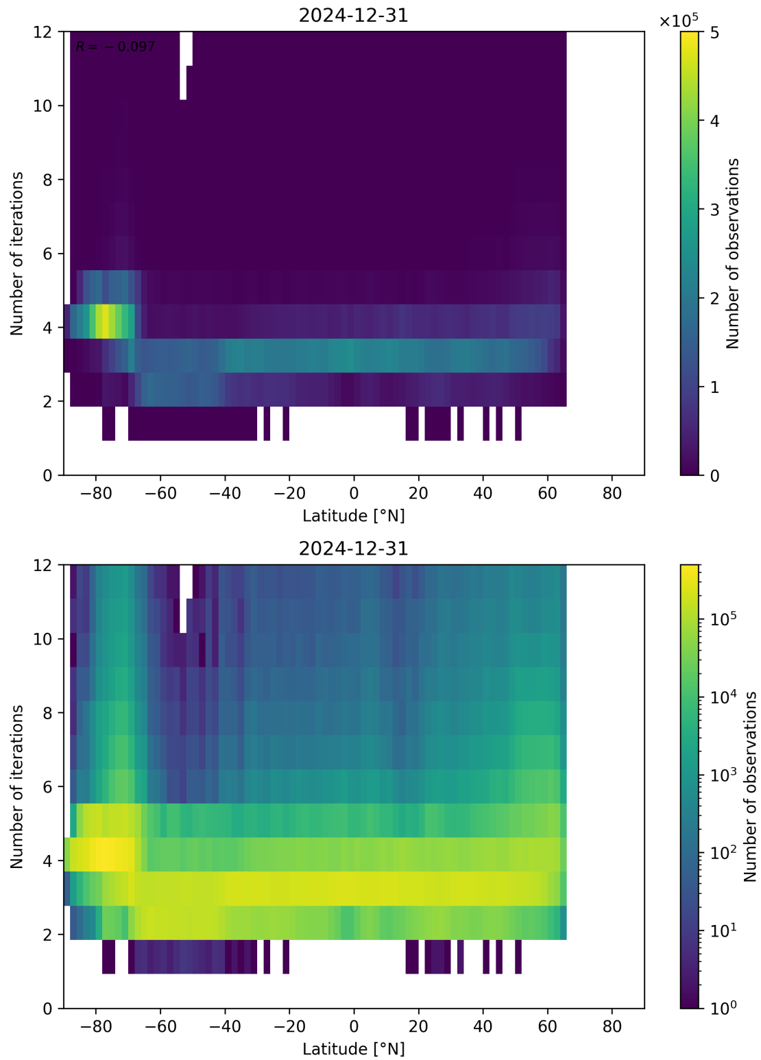
Figure 93: Scatter density plot of “Latitude” against “Number of iterations” for 2024-12-30 to 2025-01-01.
