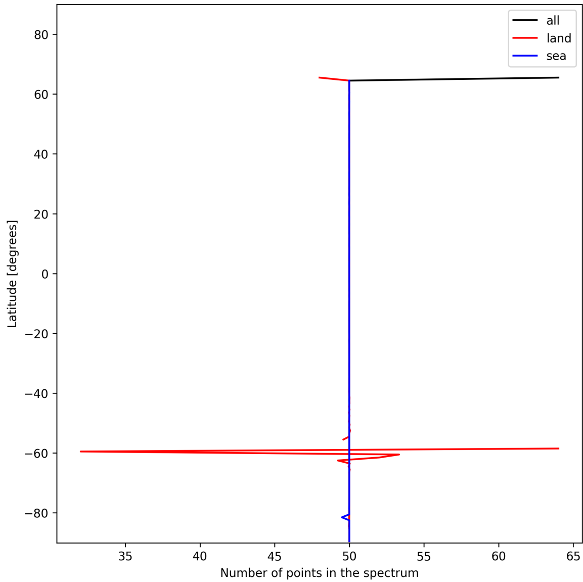
Figure 27: Zonal average of “Number of points in the spectrum” for 2024-12-30 to 2025-01-01.
