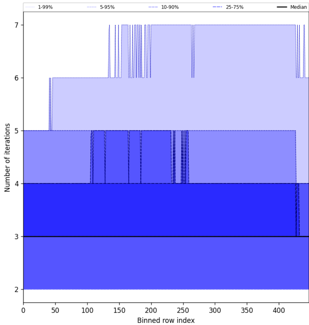
Figure 56: Along track statistics of “Number of iterations” for 2024-12-30 to 2025-01-01
