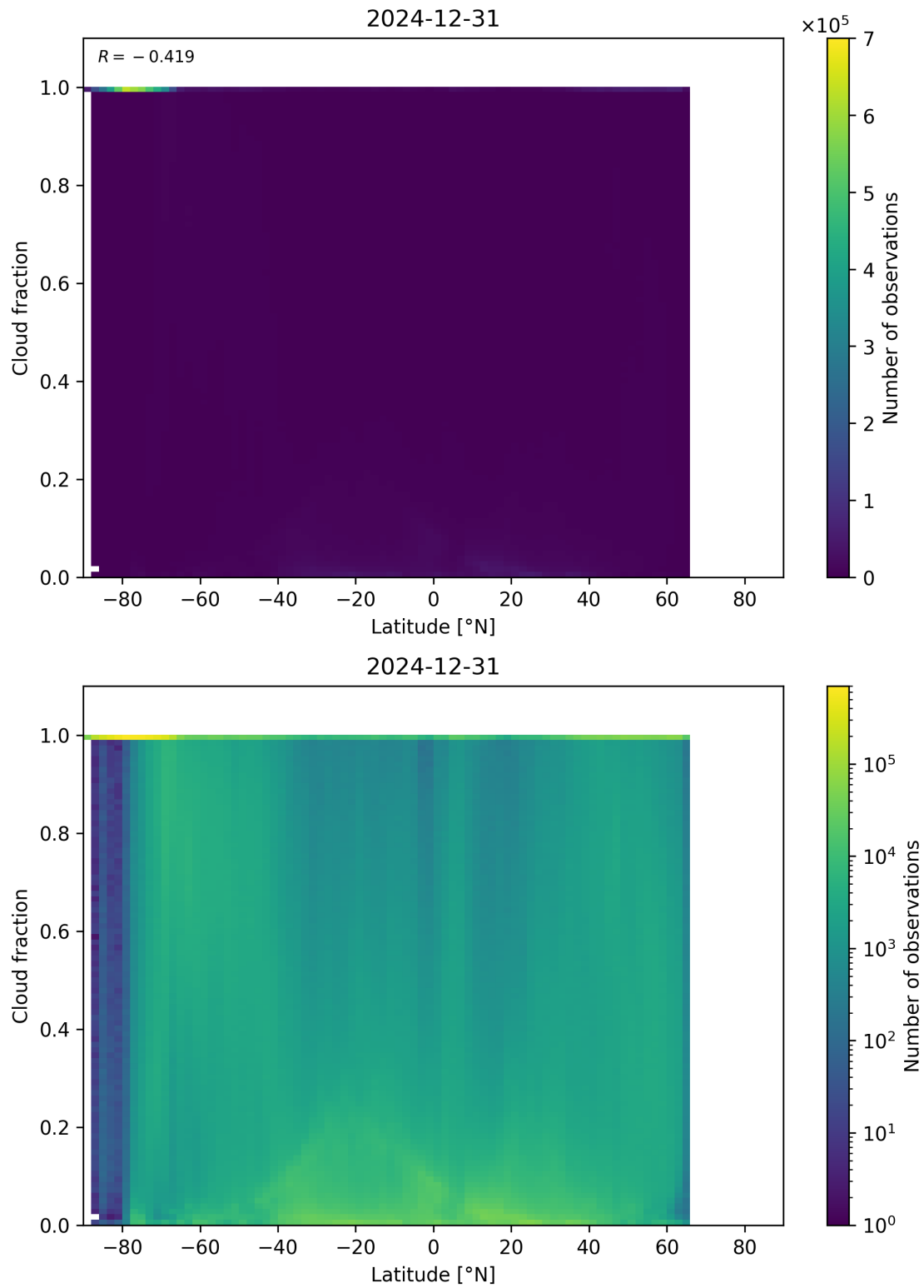
Figure 90: Scatter density plot of “Latitude” against “Cloud fraction” for 2024-12-30 to 2025-01-01.
