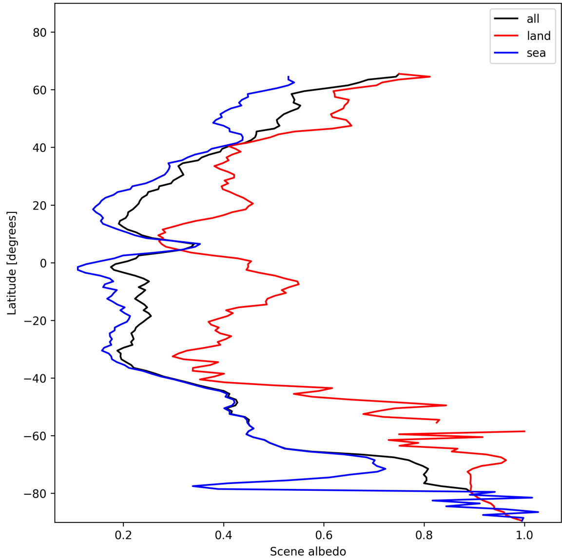
Figure 17: Zonal average of “Scene albedo” for 2024-12-30 to 2025-01-01.
