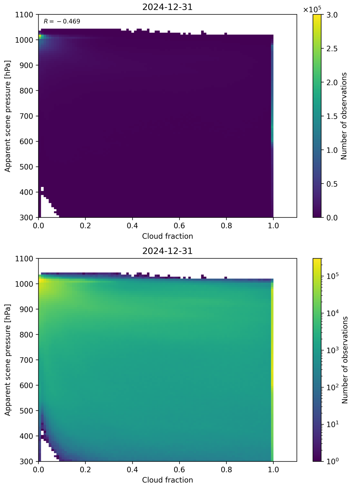
Figure 70: Scatter density plot of “Cloud fraction” against “Apparent scene pressure” for 2024-12-30 to 2025-01-01.
