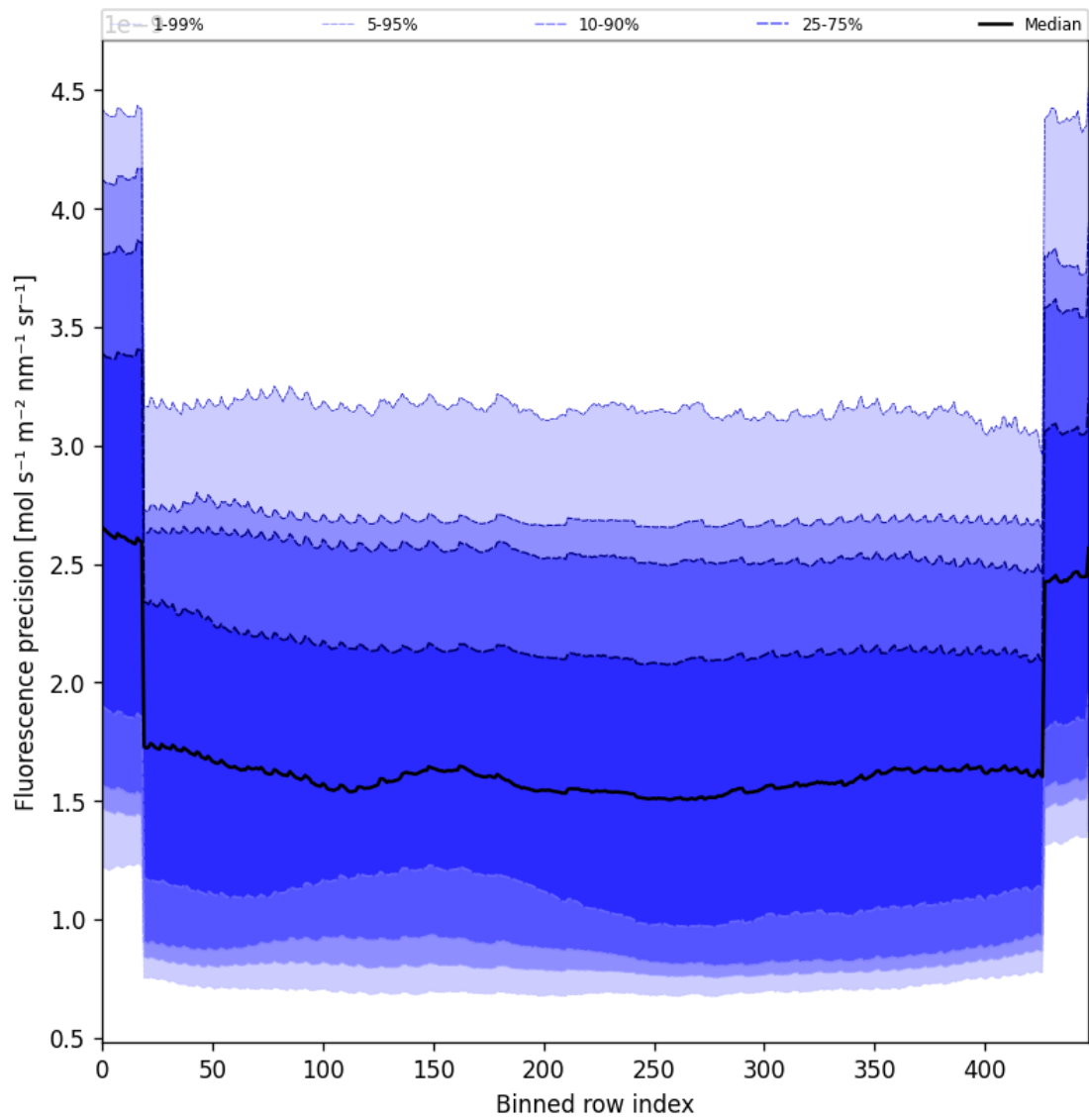
Figure 58: Along track statistics of “Fluorescence precision” for 2024-12-30 to 2025-01-01
