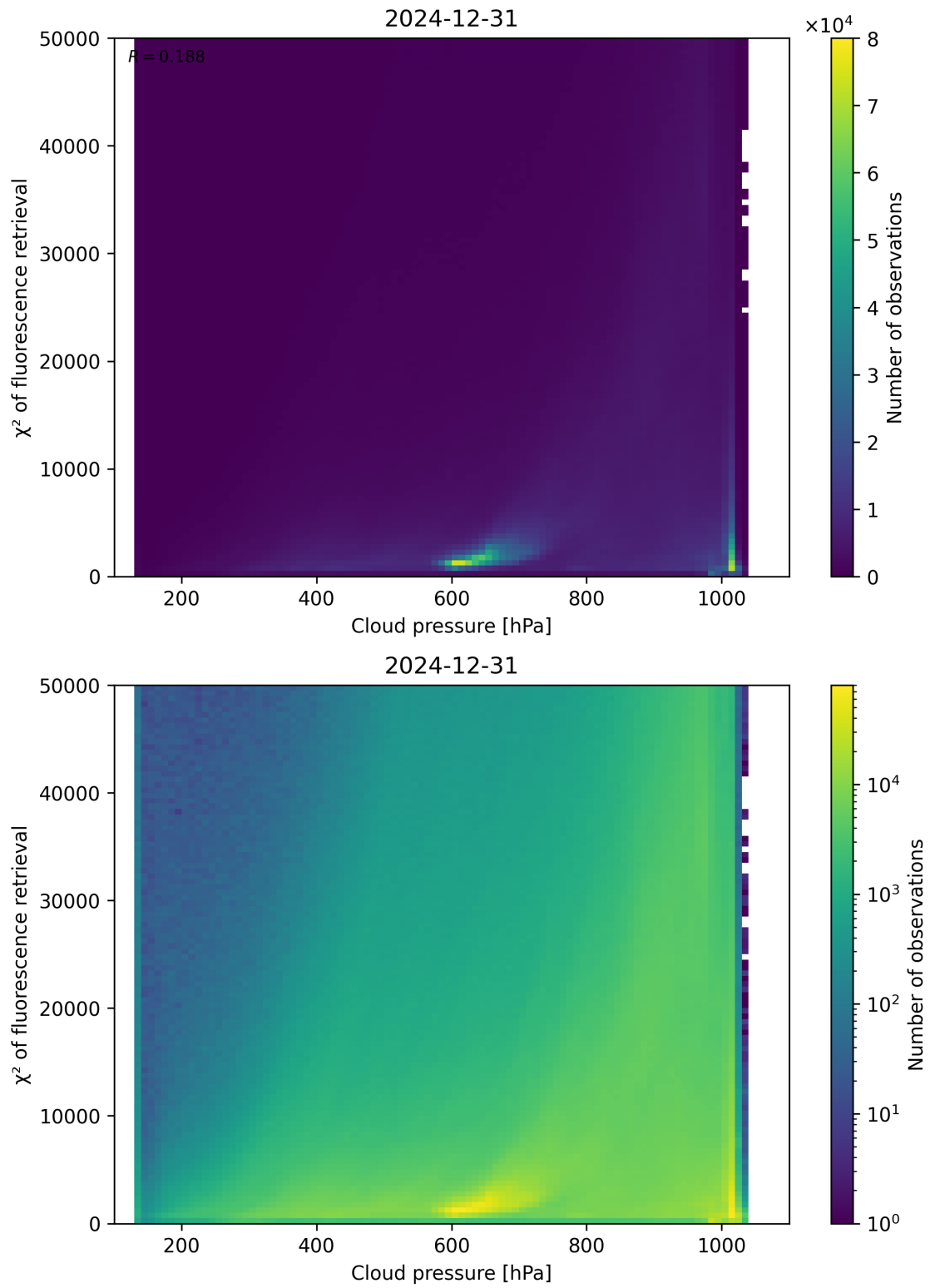
Figure 78: Scatter density plot of “Cloud pressure” against “ \chi^2 of fluorescence retrieval” for 2024-12-30 to 2025-01-01.
