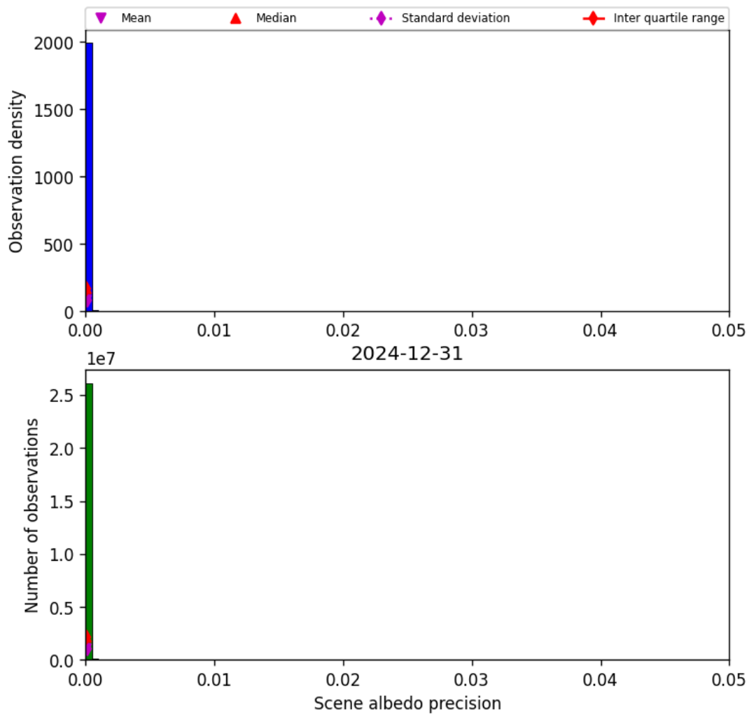
Figure 35: Histogram of “Scene albedo precision” for 2024-12-30 to 2025-01-01
