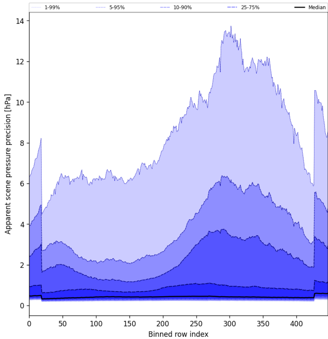
Figure 54: Along track statistics of “Apparent scene pressure precision” for 2024-12-30 to 2025-01-01
