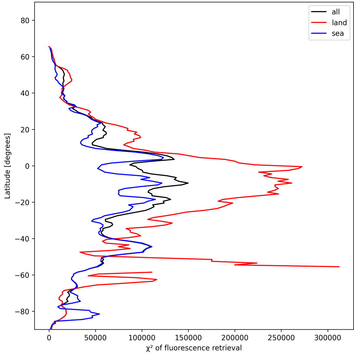
Figure 25: Zonal average of “ \chi^2 of fluorescence retrieval” for 2024-12-30 to 2025-01-01.
