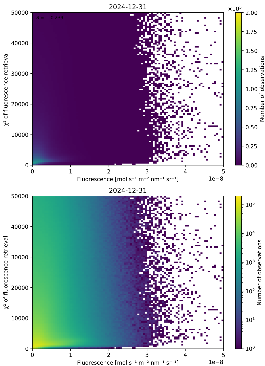
Figure 85: Scatter density plot of “Fluorescence” against “ \chi^2 of fluorescence retrieval” for 2024-12-30 to 2025-01-01.
