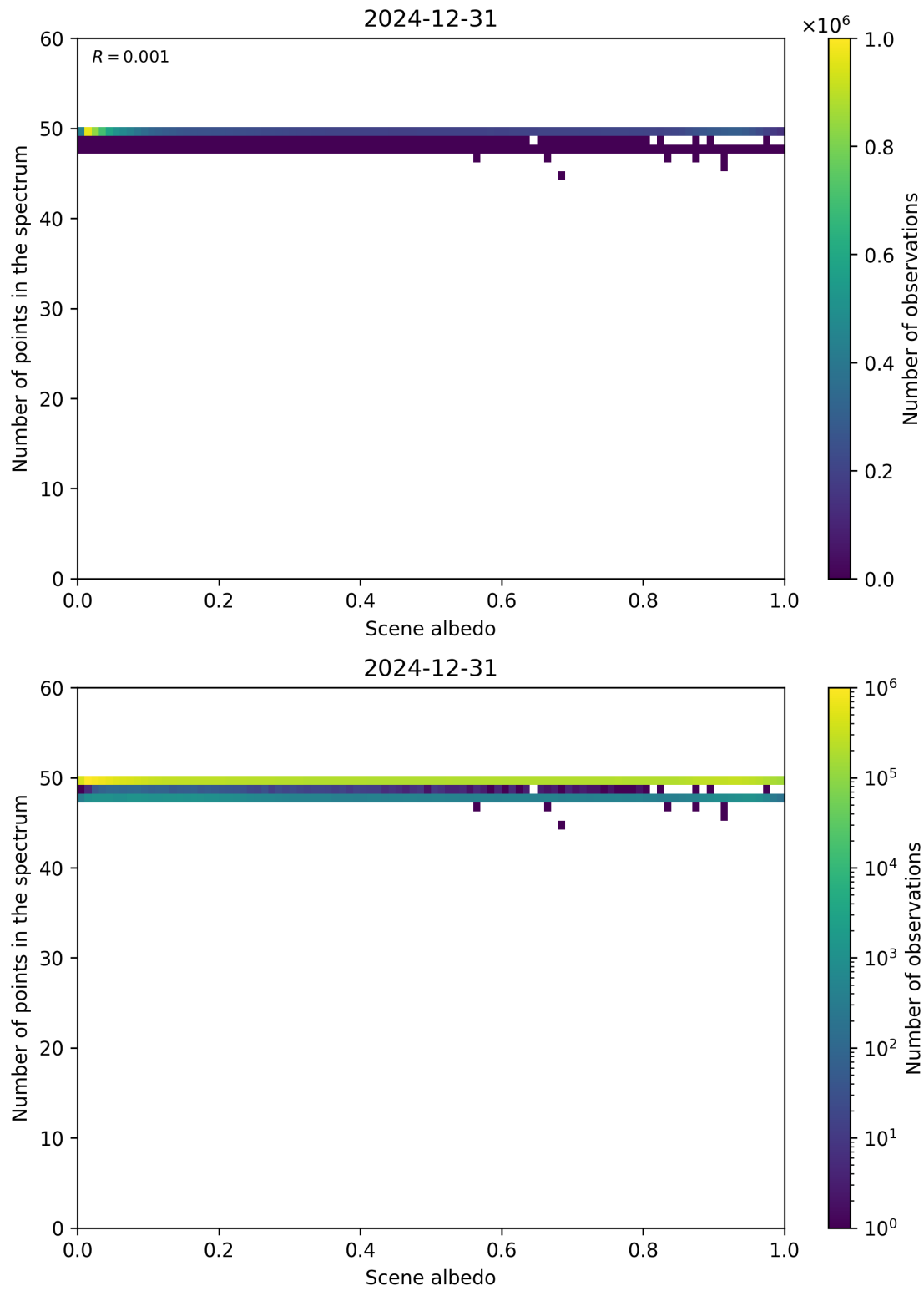
Figure 106: Scatter density plot of “Scene albedo” against “Number of points in the spectrum” for 2024-12-30 to 2025-01-01.
