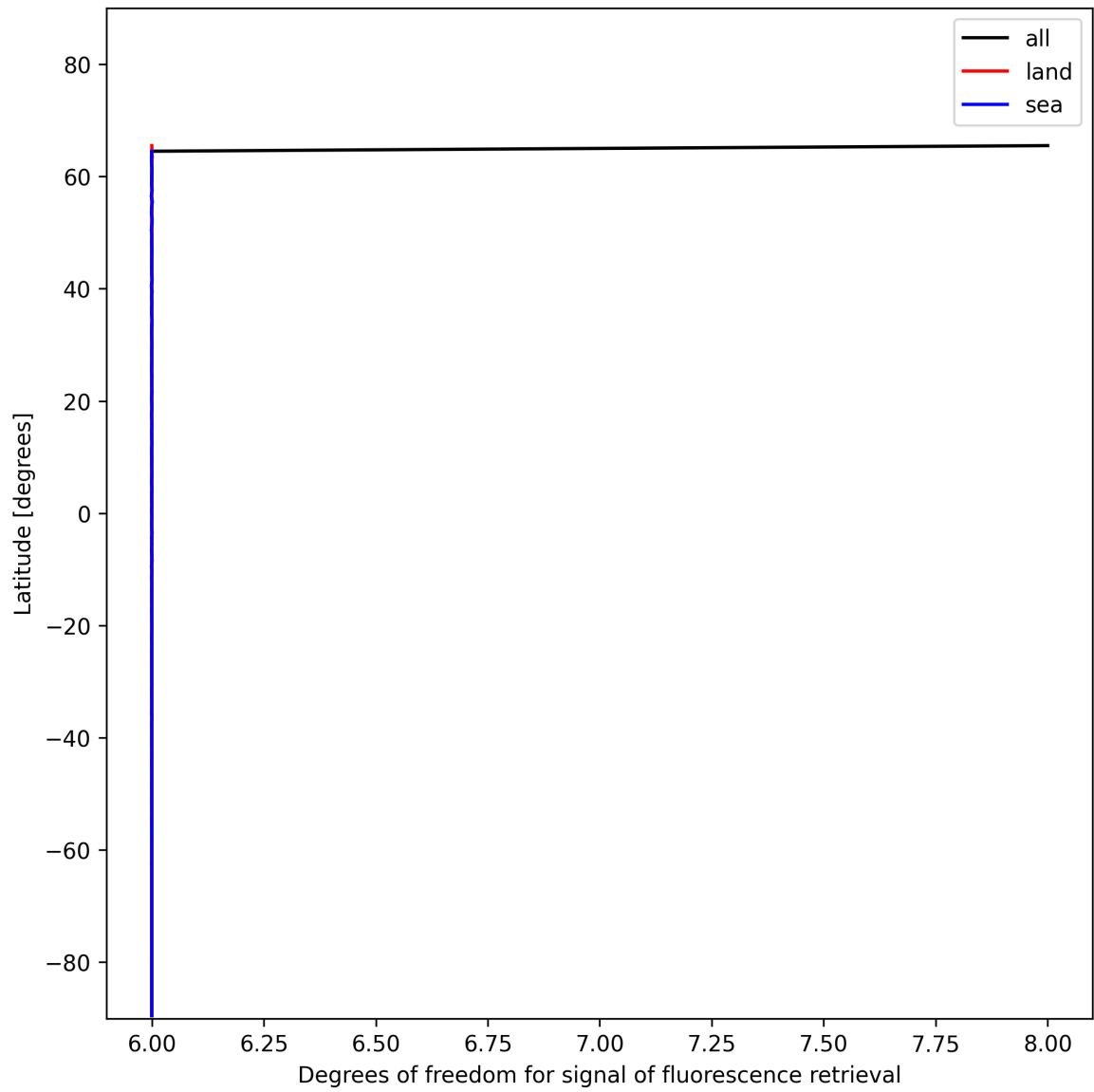
Figure 26: Zonal average of “Degrees of freedom for signal of fluorescence retrieval” for 2024-12-30 to 2025-01-01.
