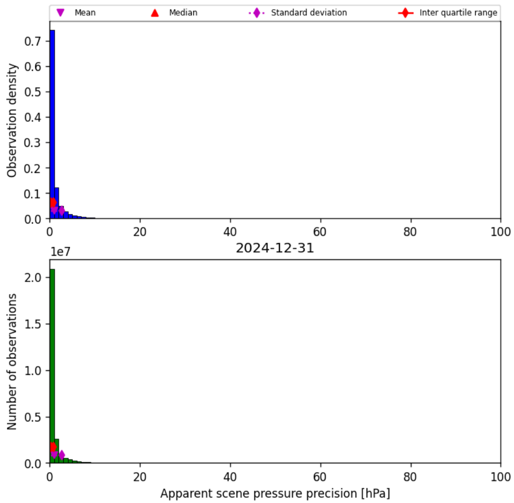
Figure 37: Histogram of “Apparent scene pressure precision” for 2024-12-30 to 2025-01-01
