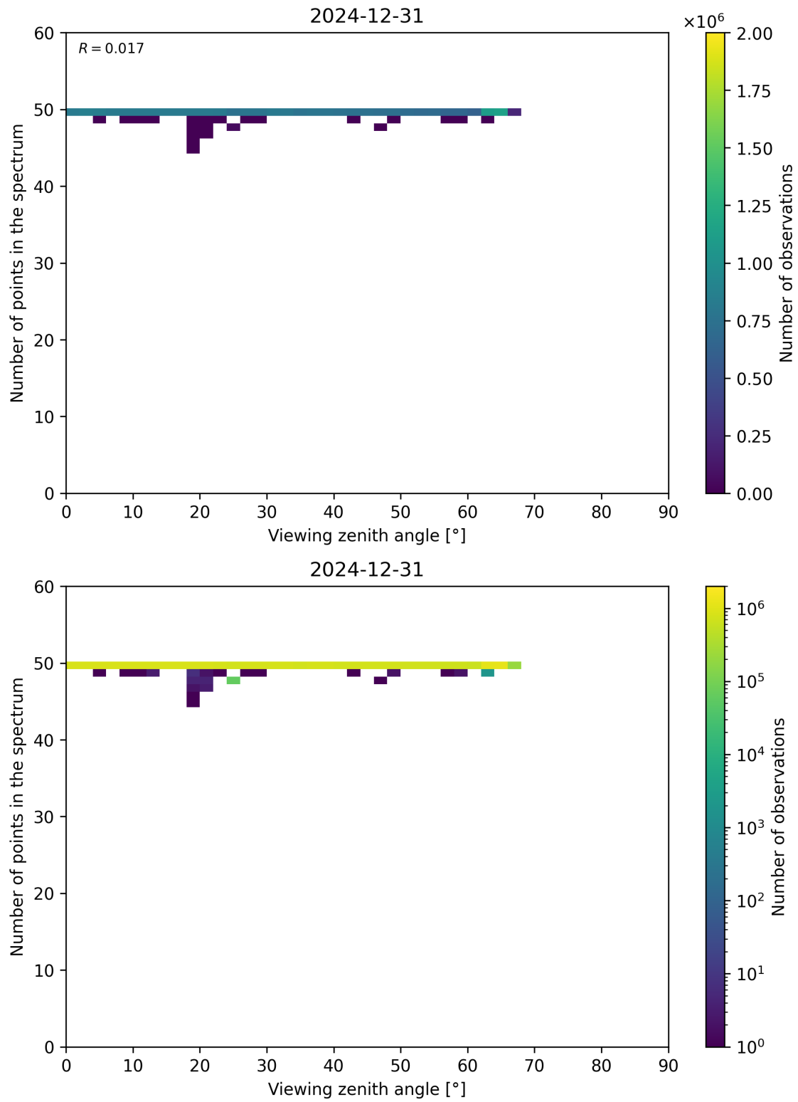
Figure 125: Scatter density plot of “Viewing zenith angle” against “Number of points in the spectrum” for 2024-12-30 to 2025-01-01.
