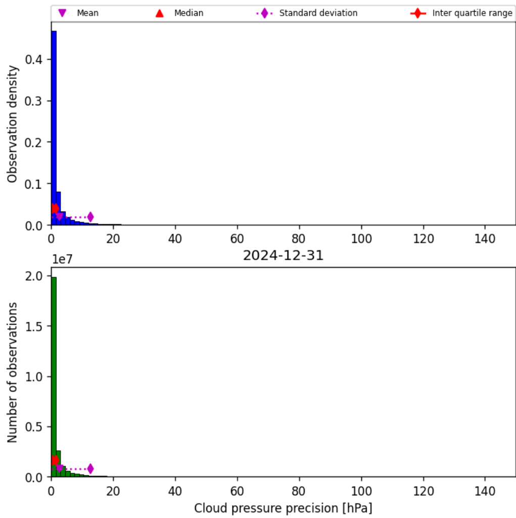
Figure 31: Histogram of “Cloud pressure precision” for 2024-12-30 to 2025-01-01
