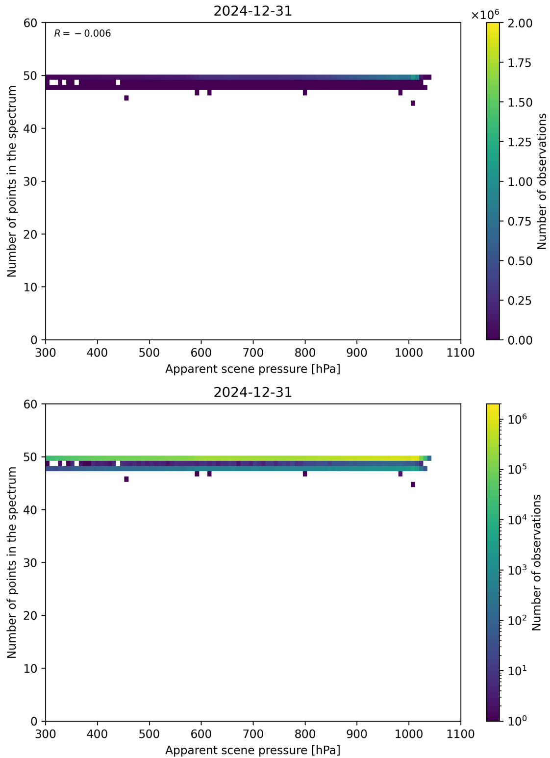
Figure 66: Scatter density plot of “Apparent scene pressure” against “Number of points in the spectrum” for 2024-12-30 to 2025-01-01.
