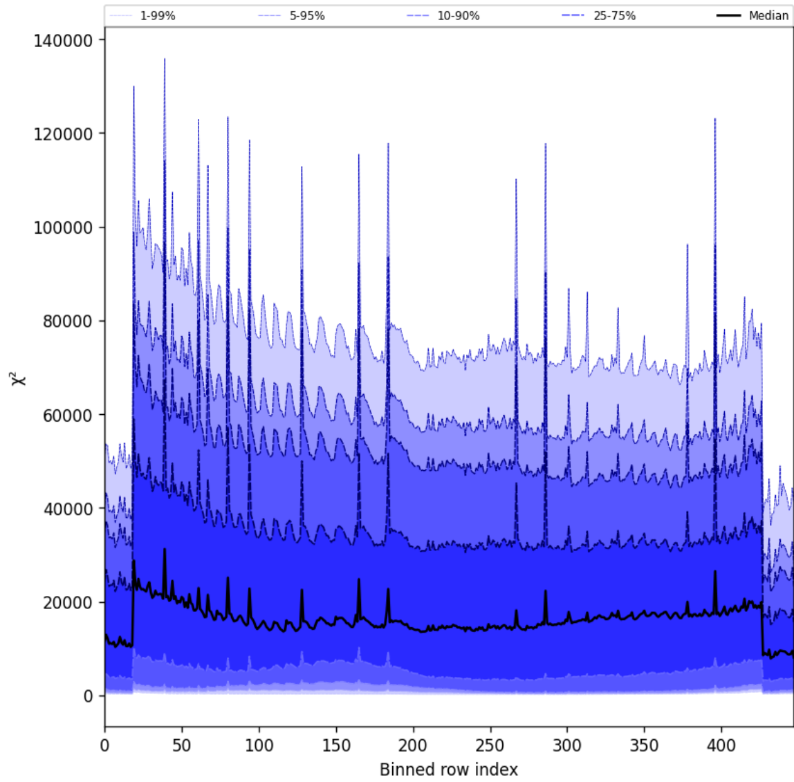
Figure 55: Along track statistics of “ \chi^2 ” for 2024-12-30 to 2025-01-01
