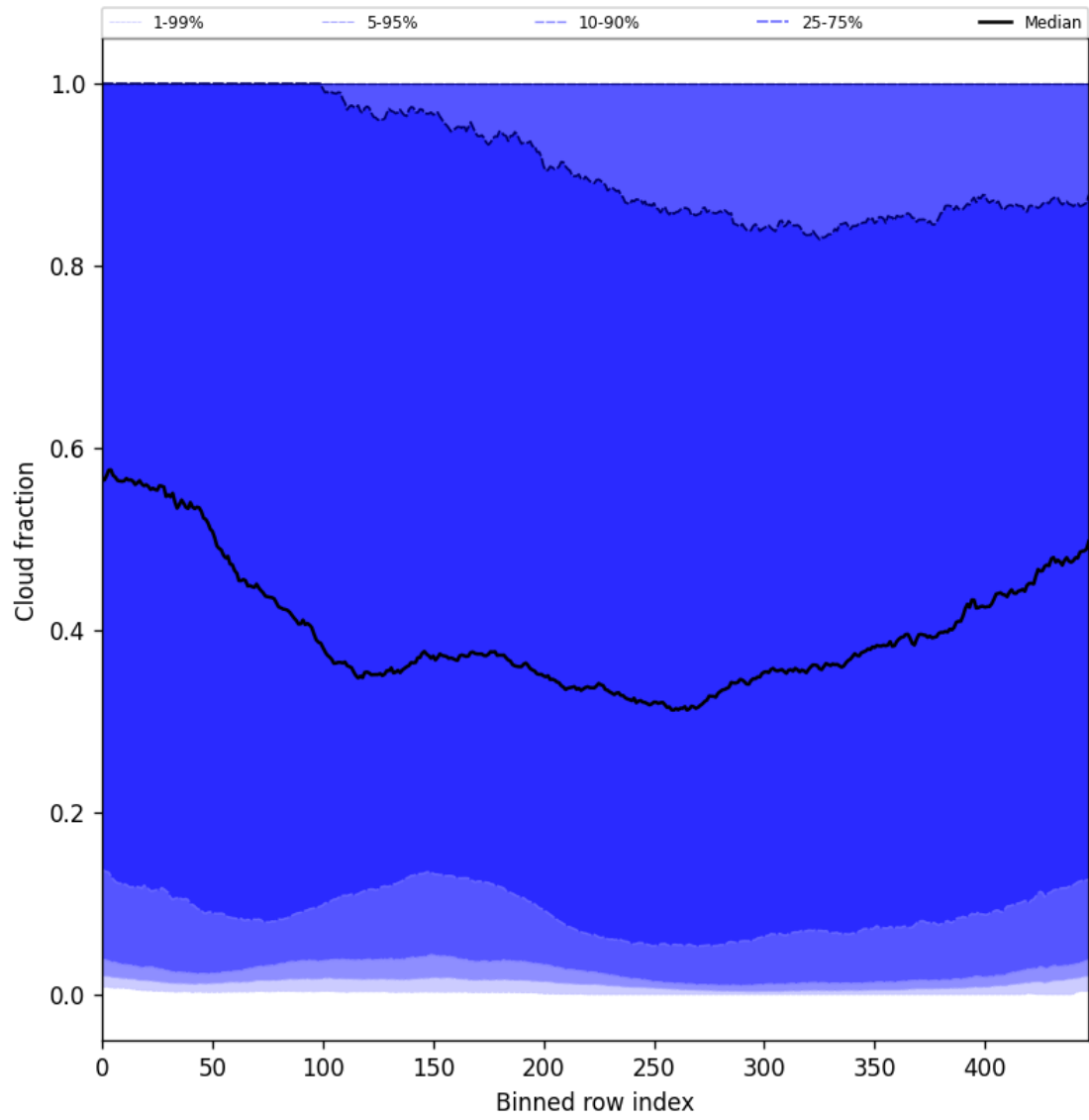
Figure 49: Along track statistics of “Cloud fraction” for 2024-12-30 to 2025-01-01
