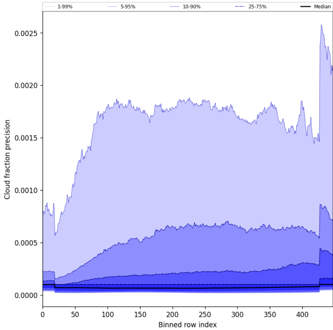
Figure 50: Along track statistics of “Cloud fraction precision” for 2024-12-30 to 2025-01-01
