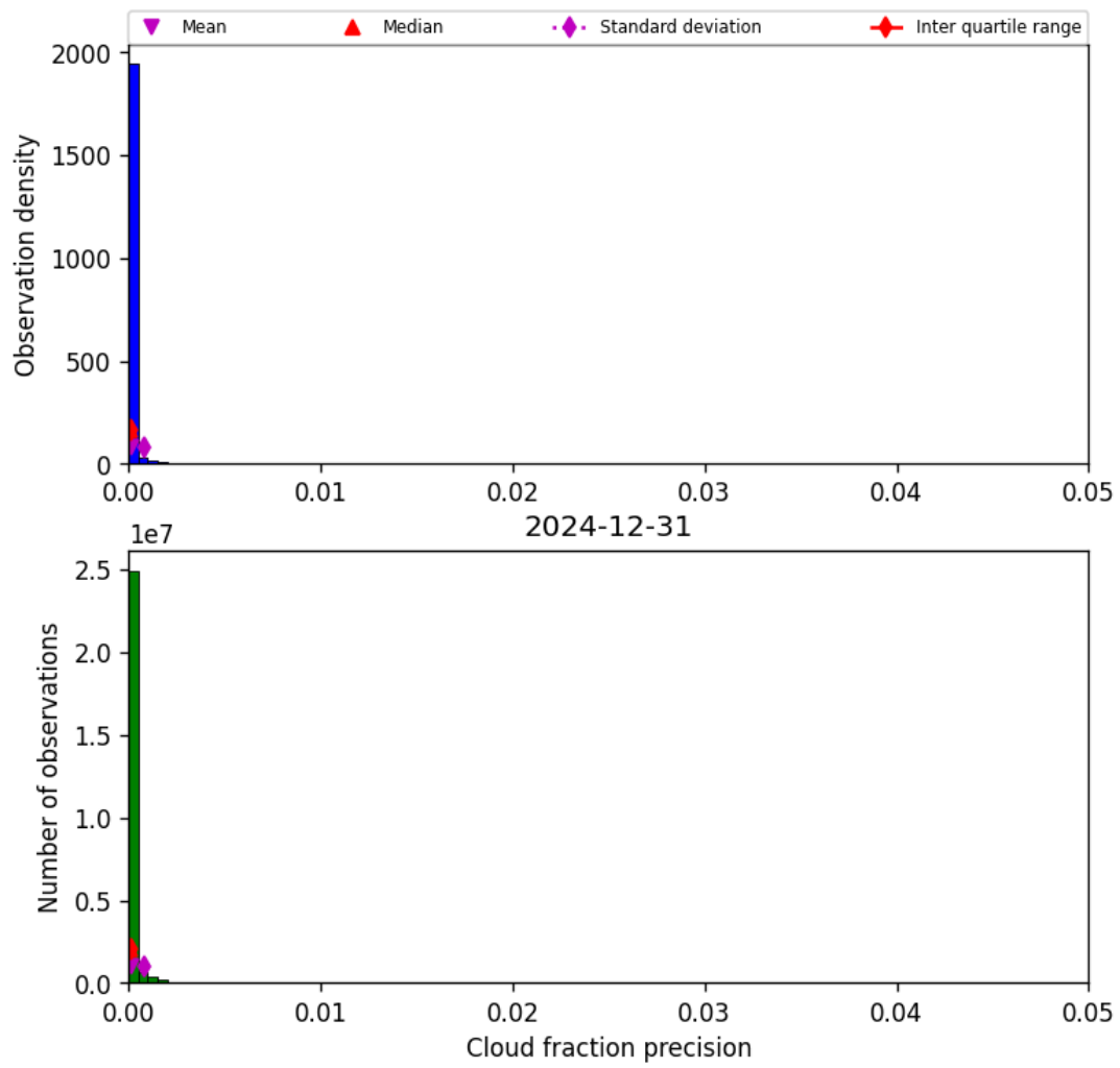
Figure 33: Histogram of “Cloud fraction precision” for 2024-12-30 to 2025-01-01
