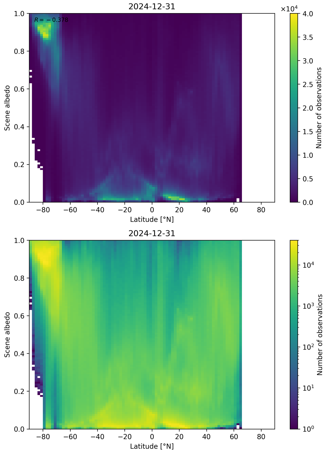
Figure 95: Scatter density plot of “Latitude” against “Scene albedo” for 2024-12-30 to 2025-01-01.
