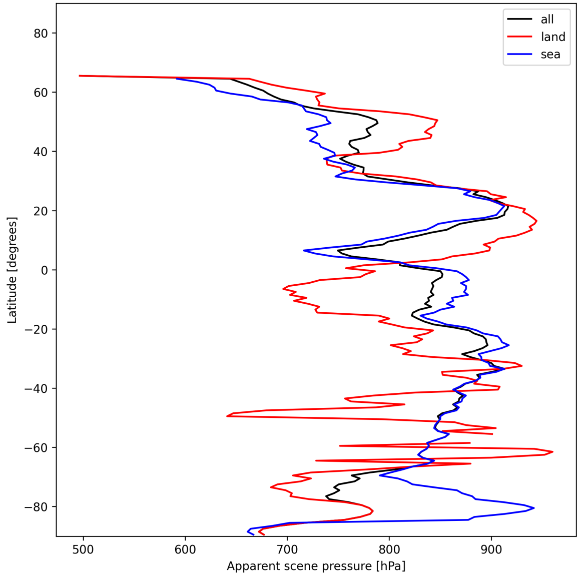
Figure 19: Zonal average of “Apparent scene pressure” for 2024-12-30 to 2025-01-01.
