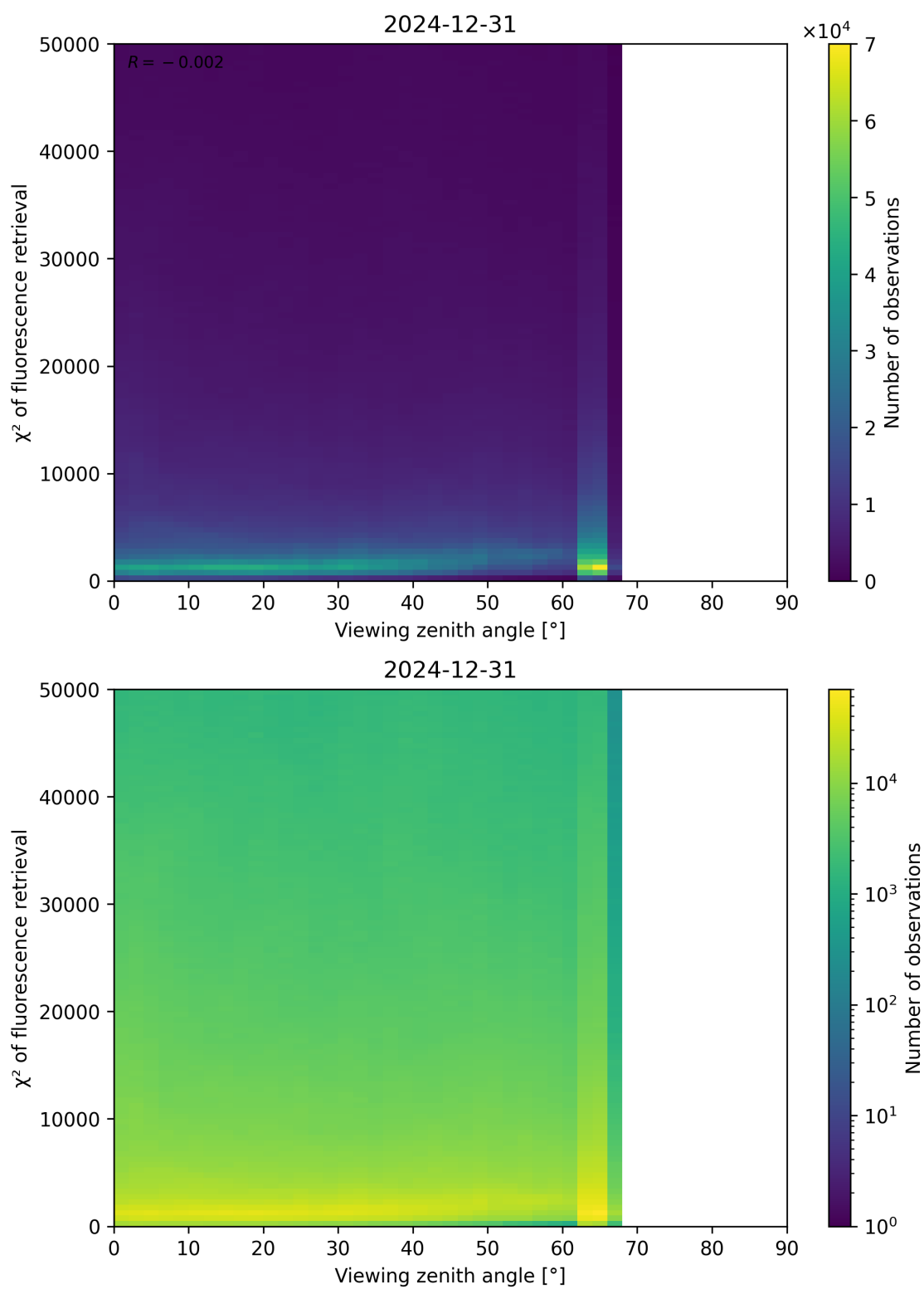
Figure 119: Scatter density plot of “Viewing zenith angle” against “ \chi^2 of fluorescence retrieval” for 2024-12-30 to 2025-01-01.
