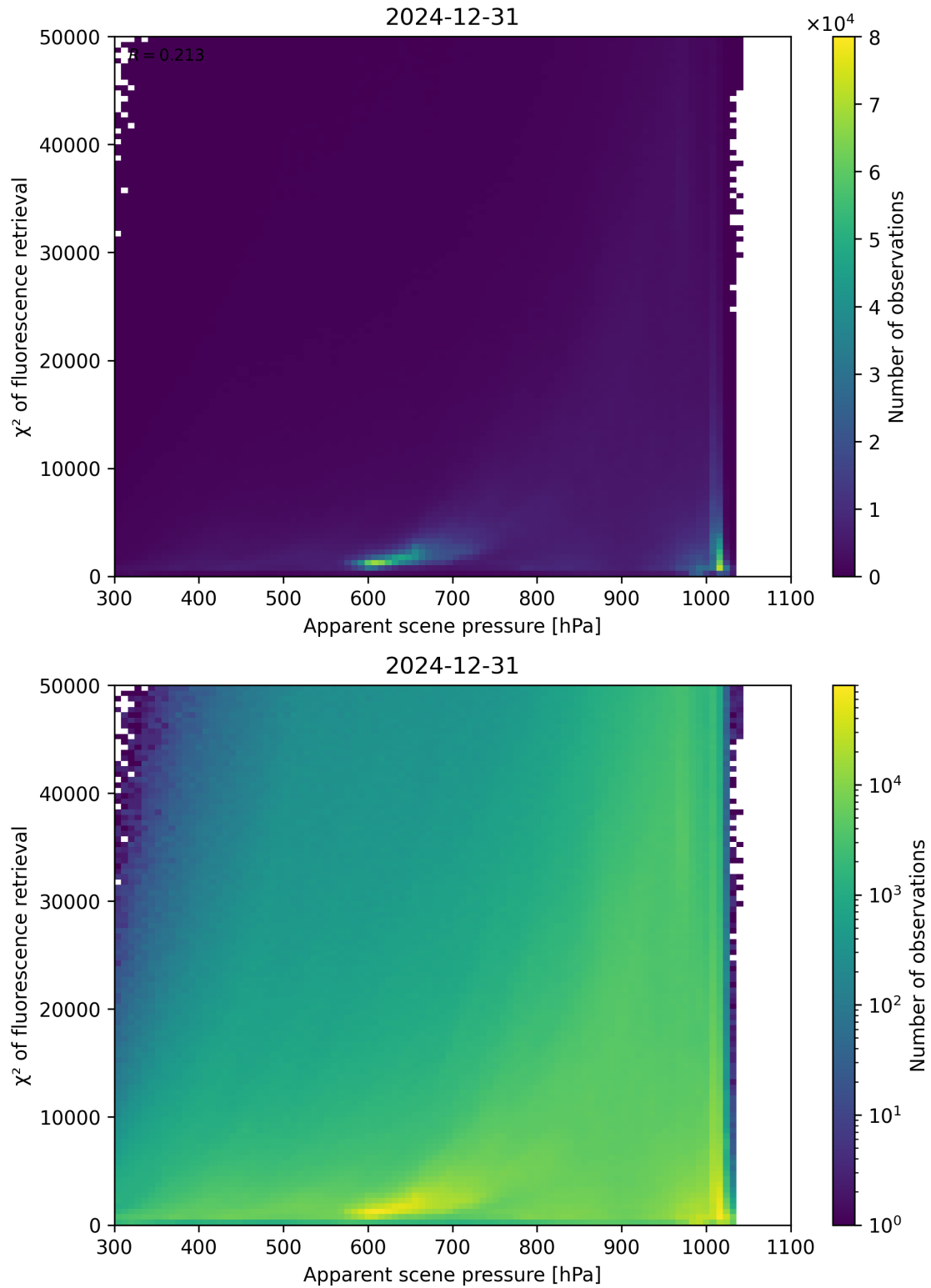
Figure 63: Scatter density plot of “Apparent scene pressure” against “ \chi^2 of fluorescence retrieval” for 2024-12-30 to 2025-01-01.
