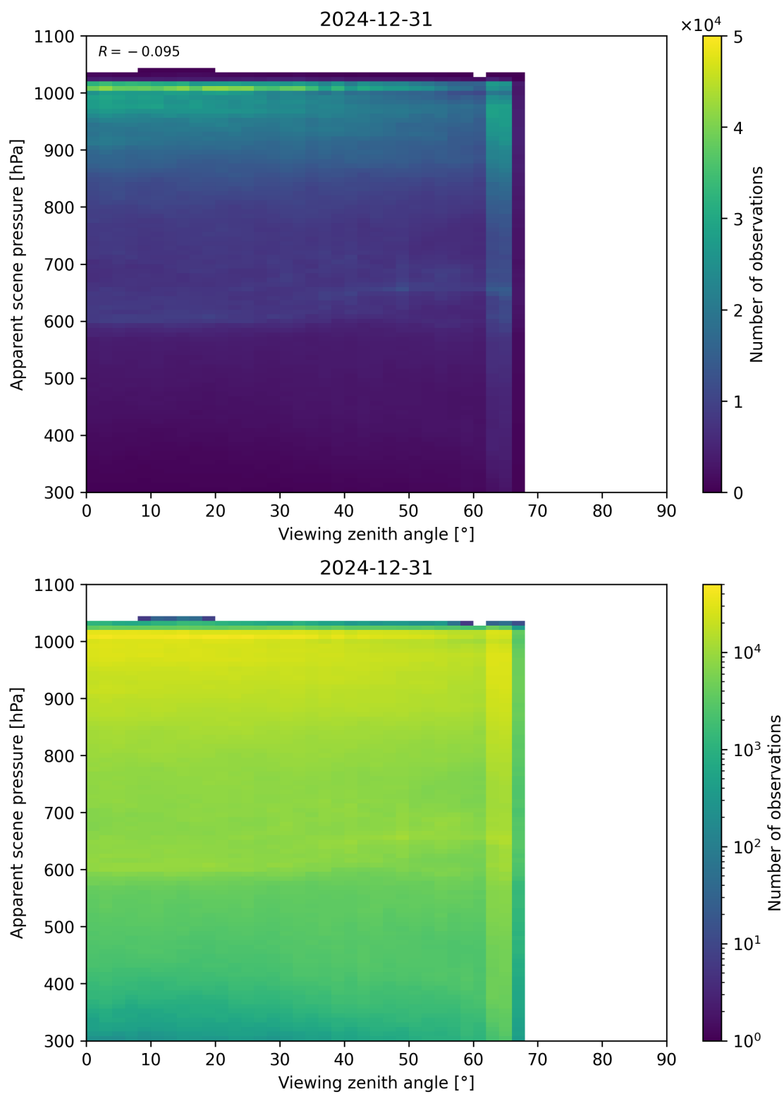
Figure 118: Scatter density plot of “Viewing zenith angle” against “Apparent scene pressure” for 2024-12-30 to 2025-01-01.
