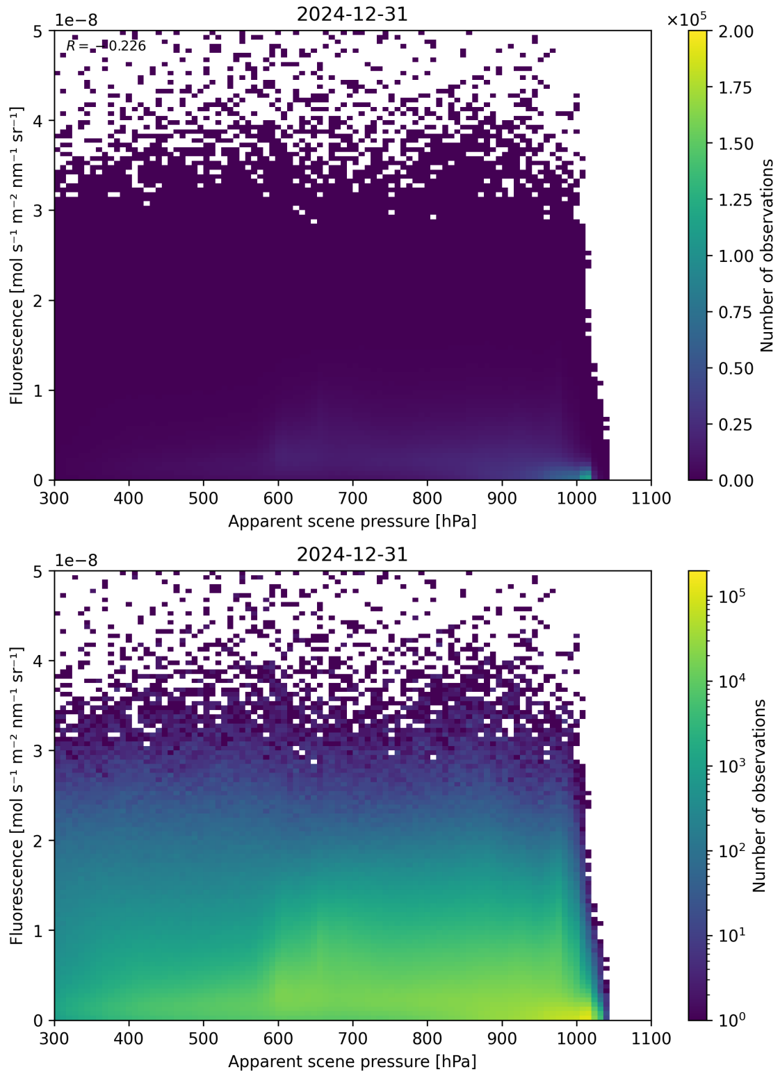
Figure 64: Scatter density plot of “Apparent scene pressure” against “Fluorescence” for 2024-12-30 to 2025-01-01.
