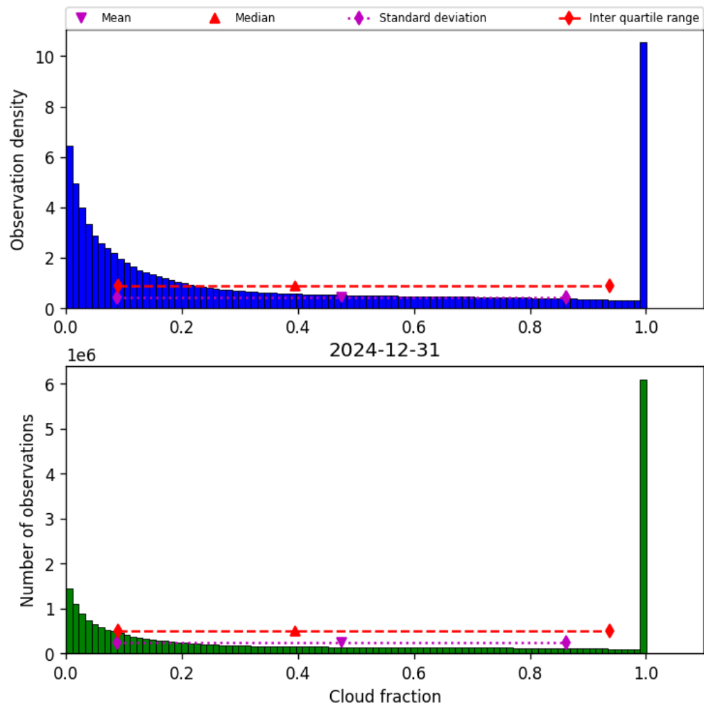
Figure 32: Histogram of “Cloud fraction” for 2024-12-30 to 2025-01-01
