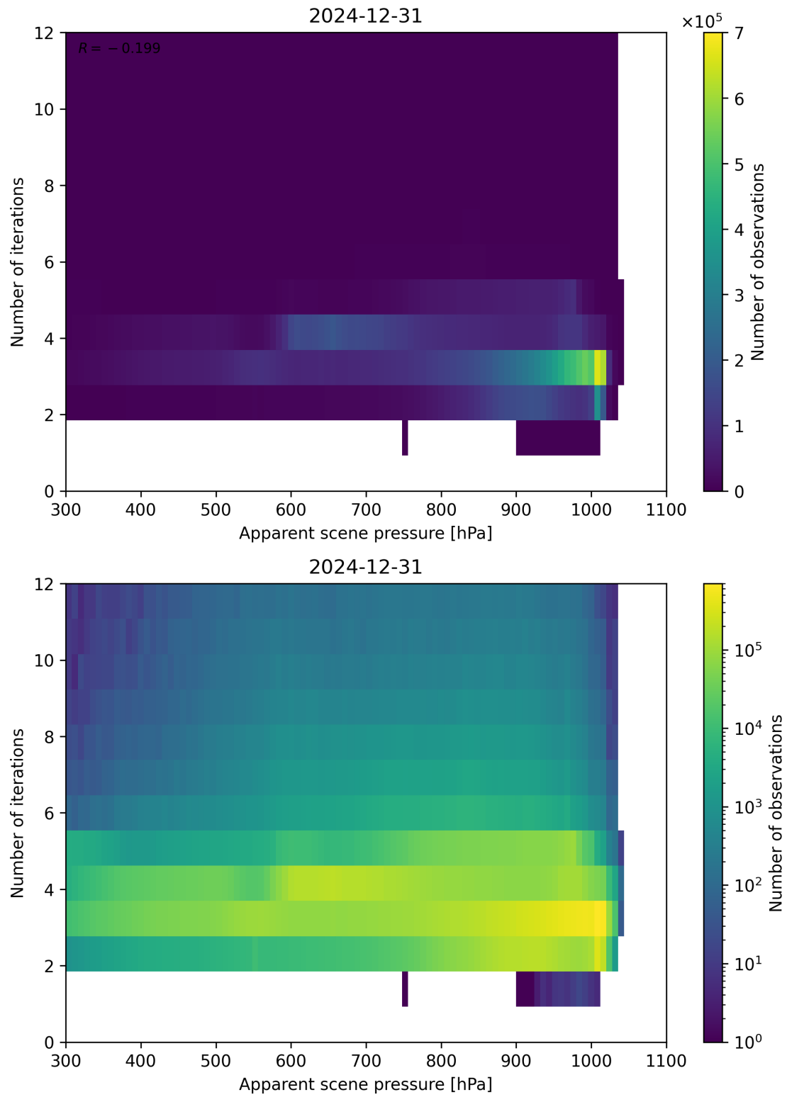
Figure 65: Scatter density plot of “Apparent scene pressure” against “Number of iterations” for 2024-12-30 to 2025-01-01.
