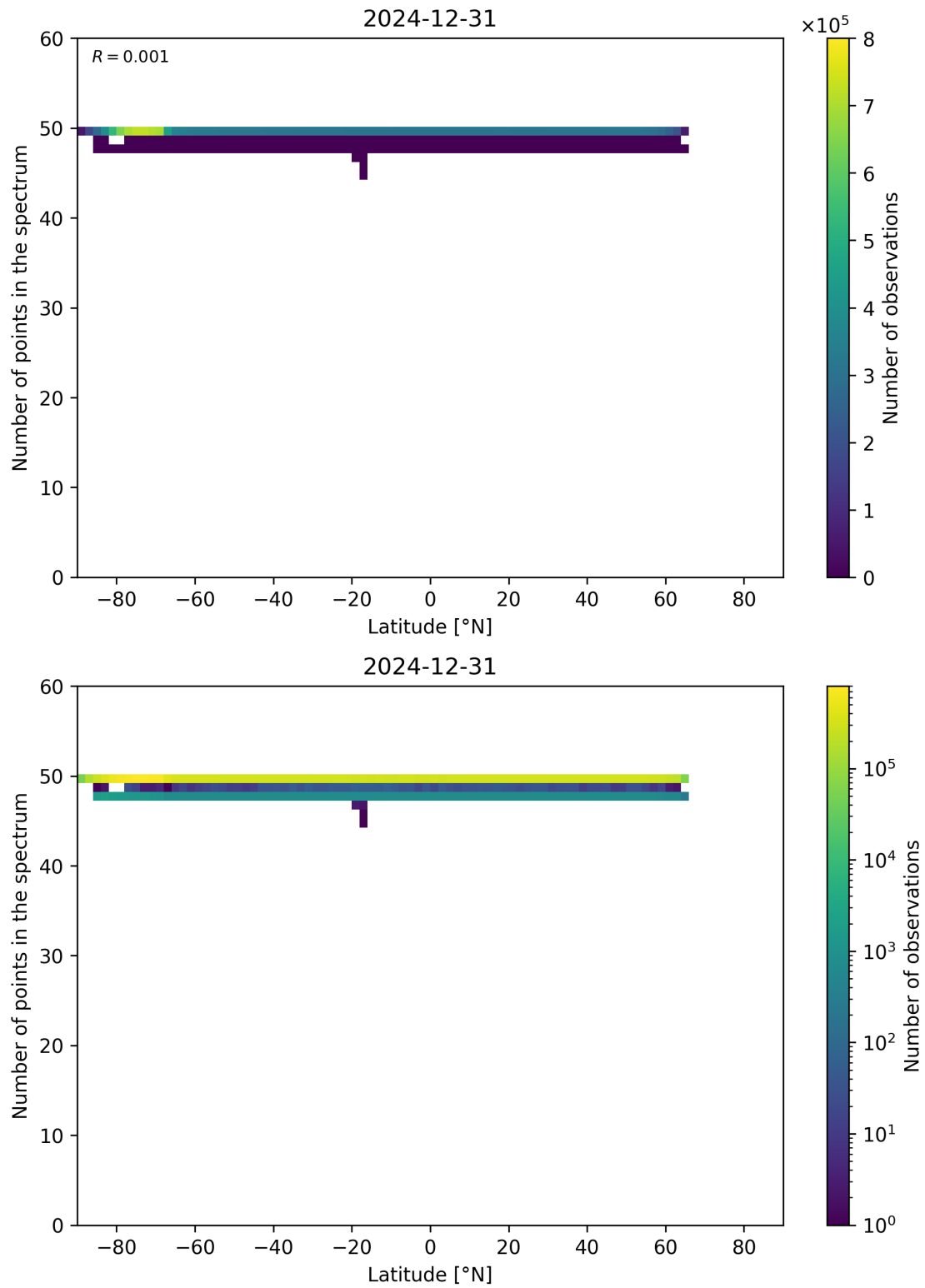
Figure 94: Scatter density plot of “Latitude” against “Number of points in the spectrum” for 2024-12-30 to 2025-01-01.
