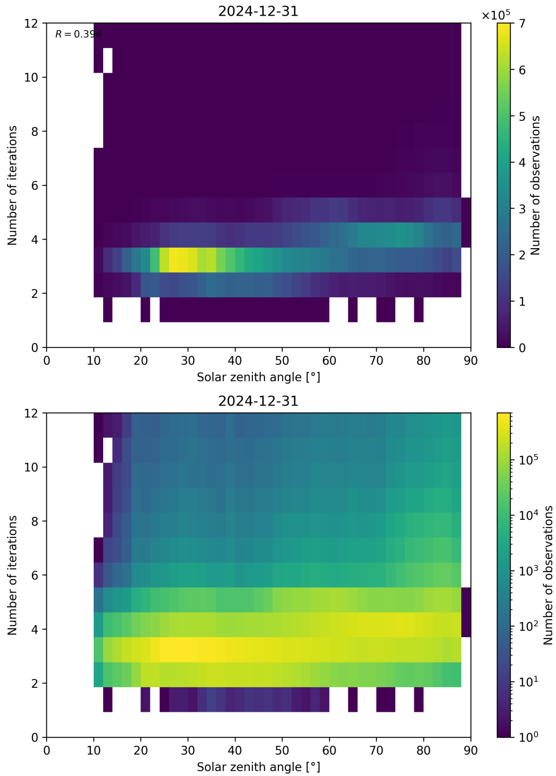
Figure 114: Scatter density plot of “Solar zenith angle” against “Number of iterations” for 2024-12-30 to 2025-01-01.
