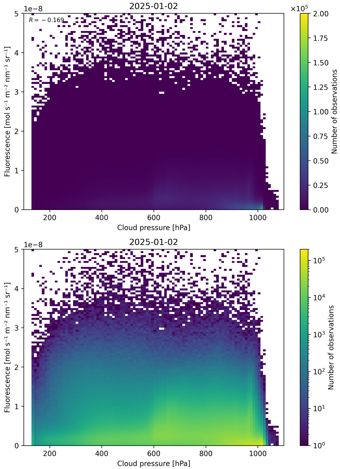
Figure 80: Scatter density plot of “Cloud pressure” against “Fluorescence” for 2025-01-01 to 2025-01-03.
