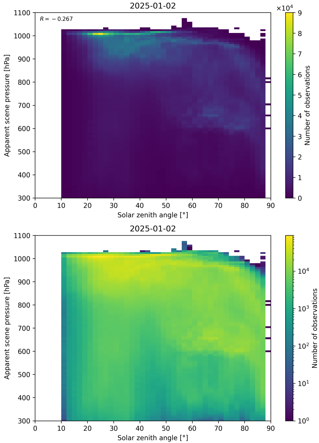
Figure 108: Scatter density plot of “Solar zenith angle” against “Apparent scene pressure” for 2025-01-01 to 2025-01-03.
