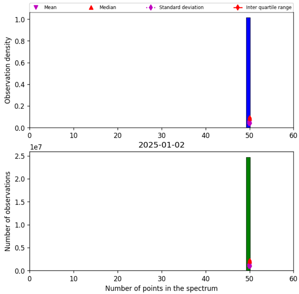
Figure 44: Histogram of “Number of points in the spectrum” for 2025-01-01 to 2025-01-03
