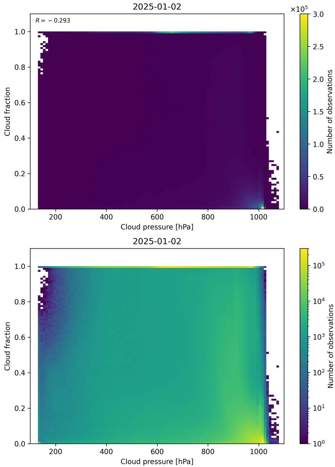
Figure 79: Scatter density plot of “Cloud pressure” against “Cloud fraction” for 2025-01-01 to 2025-01-03.
