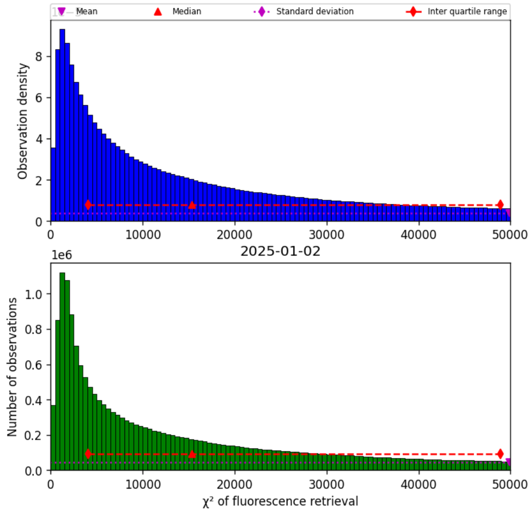
Figure 42: Histogram of “ \chi^2 of fluorescence retrieval” for 2025-01-01 to 2025-01-03
