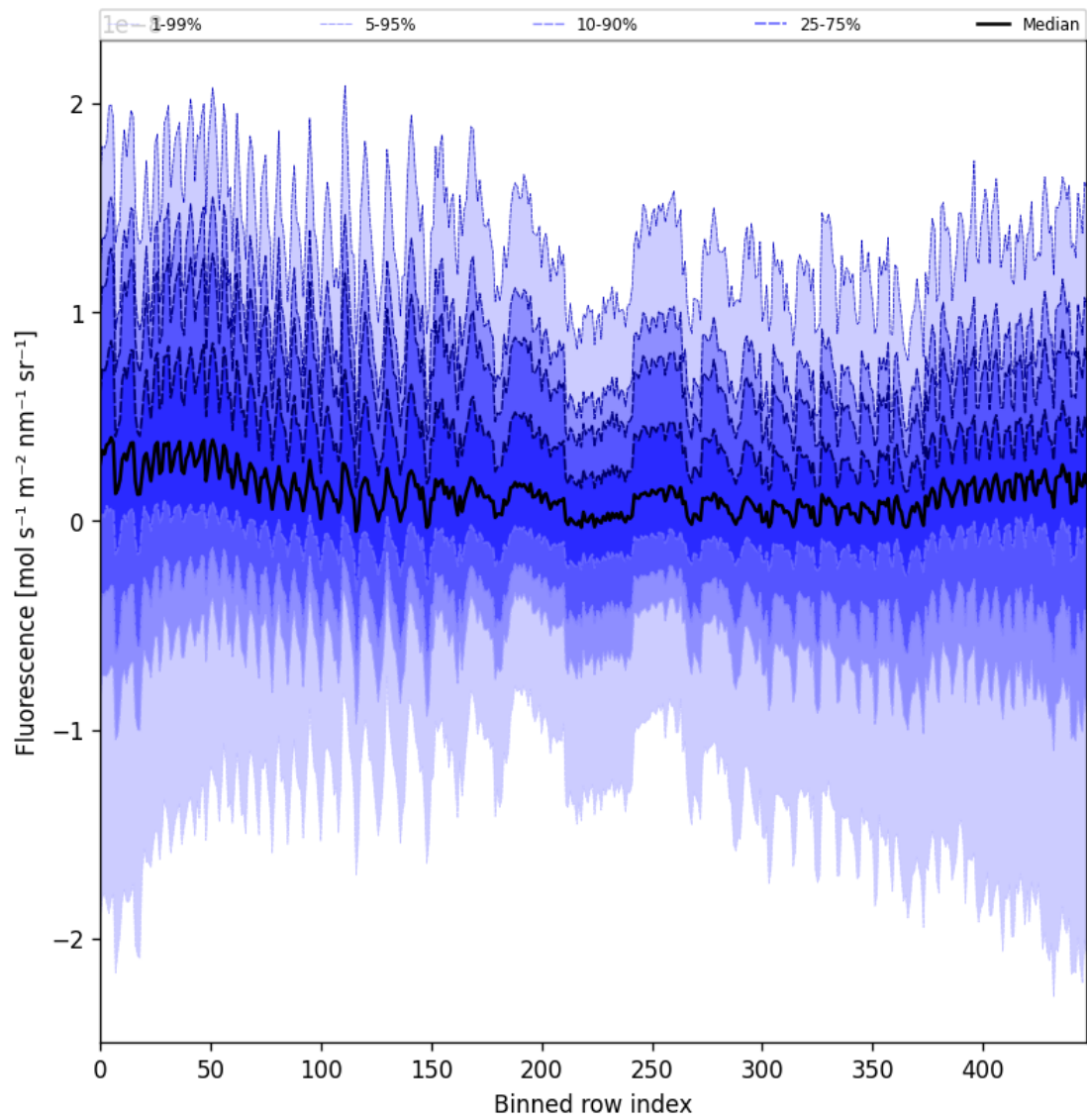
Figure 57: Along track statistics of “Fluorescence” for 2025-01-01 to 2025-01-03
