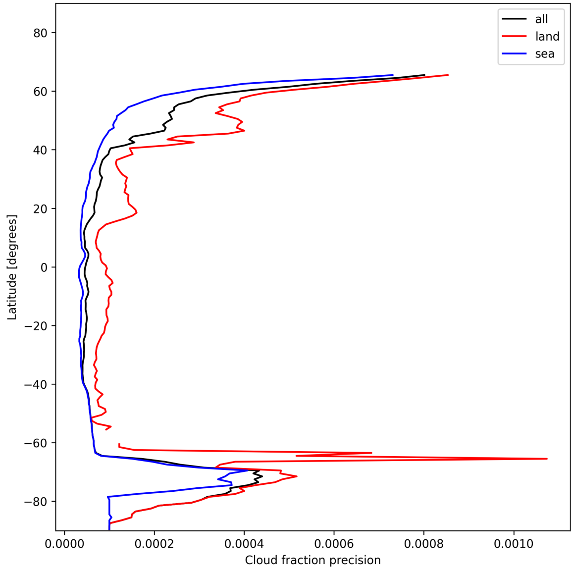
Figure 16: Zonal average of “Cloud fraction precision” for 2025-01-01 to 2025-01-03.
