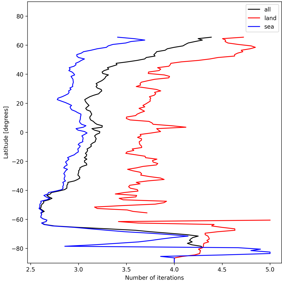
Figure 22: Zonal average of “Number of iterations” for 2025-01-01 to 2025-01-03.
