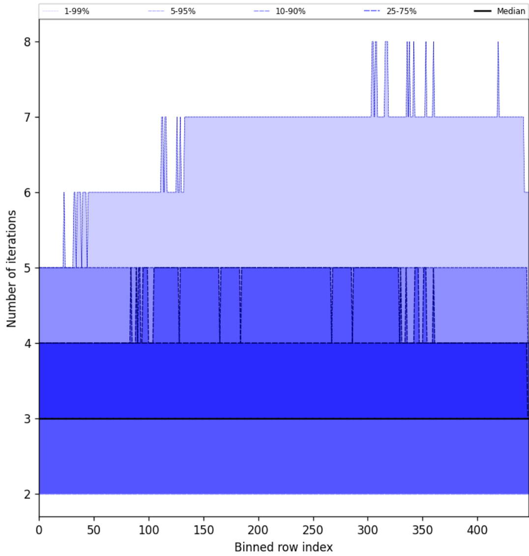
Figure 56: Along track statistics of “Number of iterations” for 2025-01-01 to 2025-01-03
