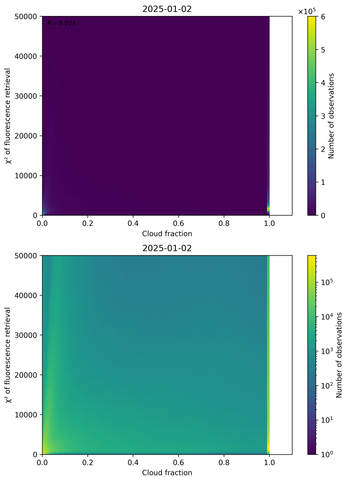
Figure 71: Scatter density plot of “Cloud fraction” against “ \chi^2 of fluorescence retrieval” for 2025-01-01 to 2025-01-03.
