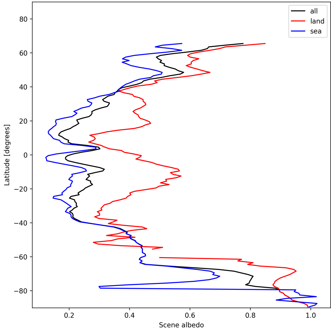
Figure 17: Zonal average of “Scene albedo” for 2025-01-01 to 2025-01-03.
