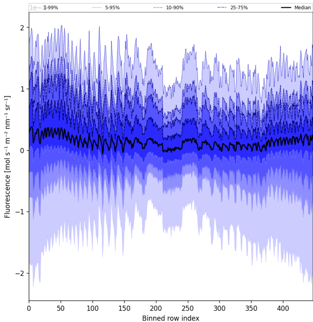
Figure 57: Along track statistics of “Fluorescence” for 2025-01-02 to 2025-01-04
