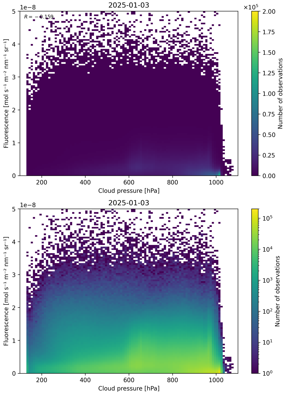
Figure 80: Scatter density plot of “Cloud pressure” against “Fluorescence” for 2025-01-02 to 2025-01-04.
