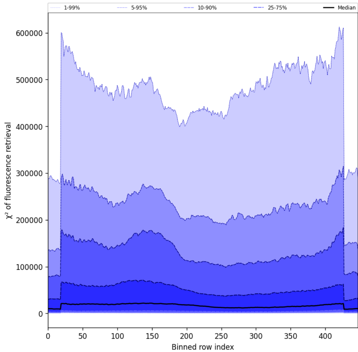
Figure 59: Along track statistics of “ \chi^2 of fluorescence retrieval” for 2025-01-02 to 2025-01-04
