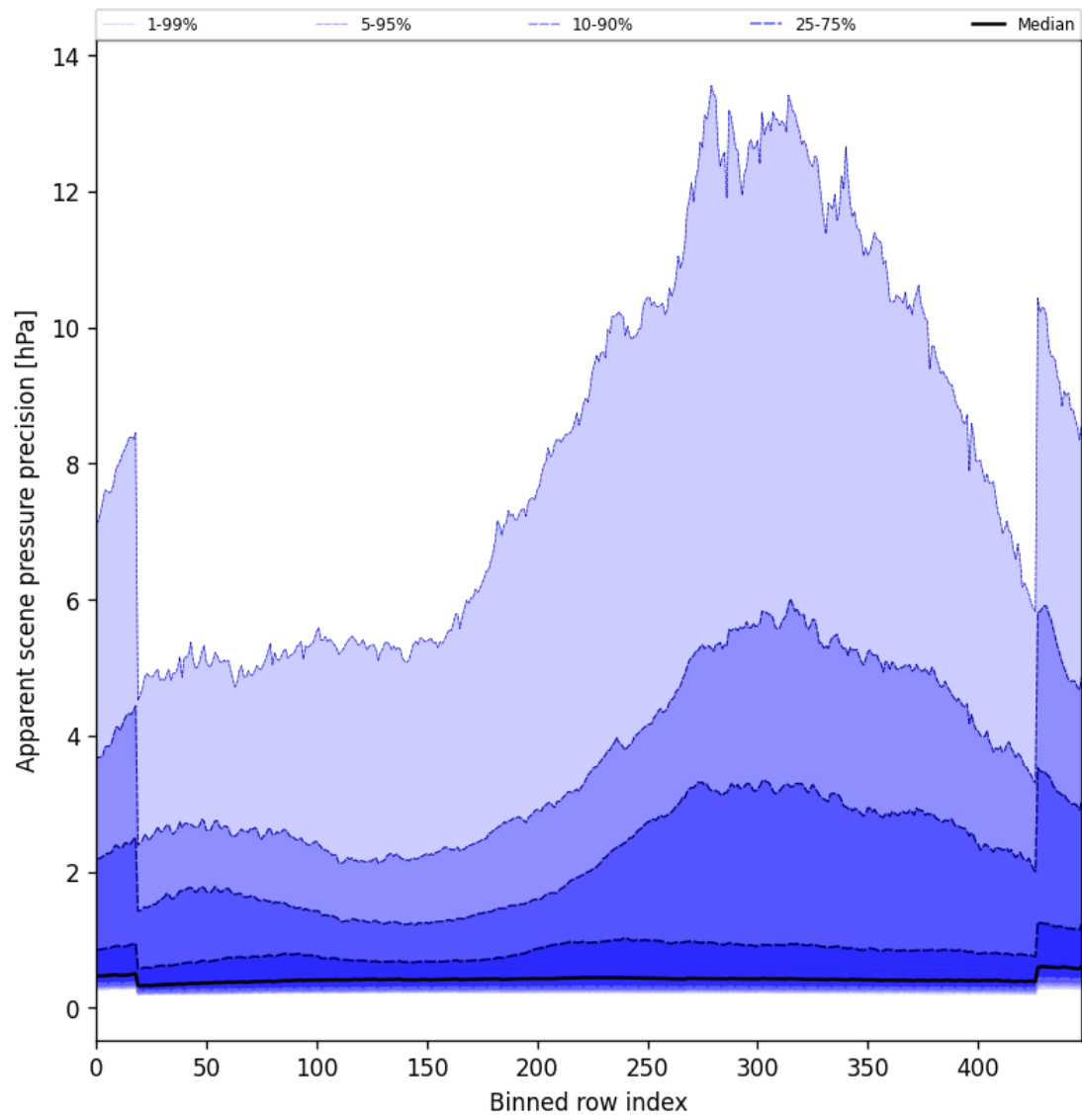
Figure 54: Along track statistics of “Apparent scene pressure precision” for 2025-01-02 to 2025-01-04
