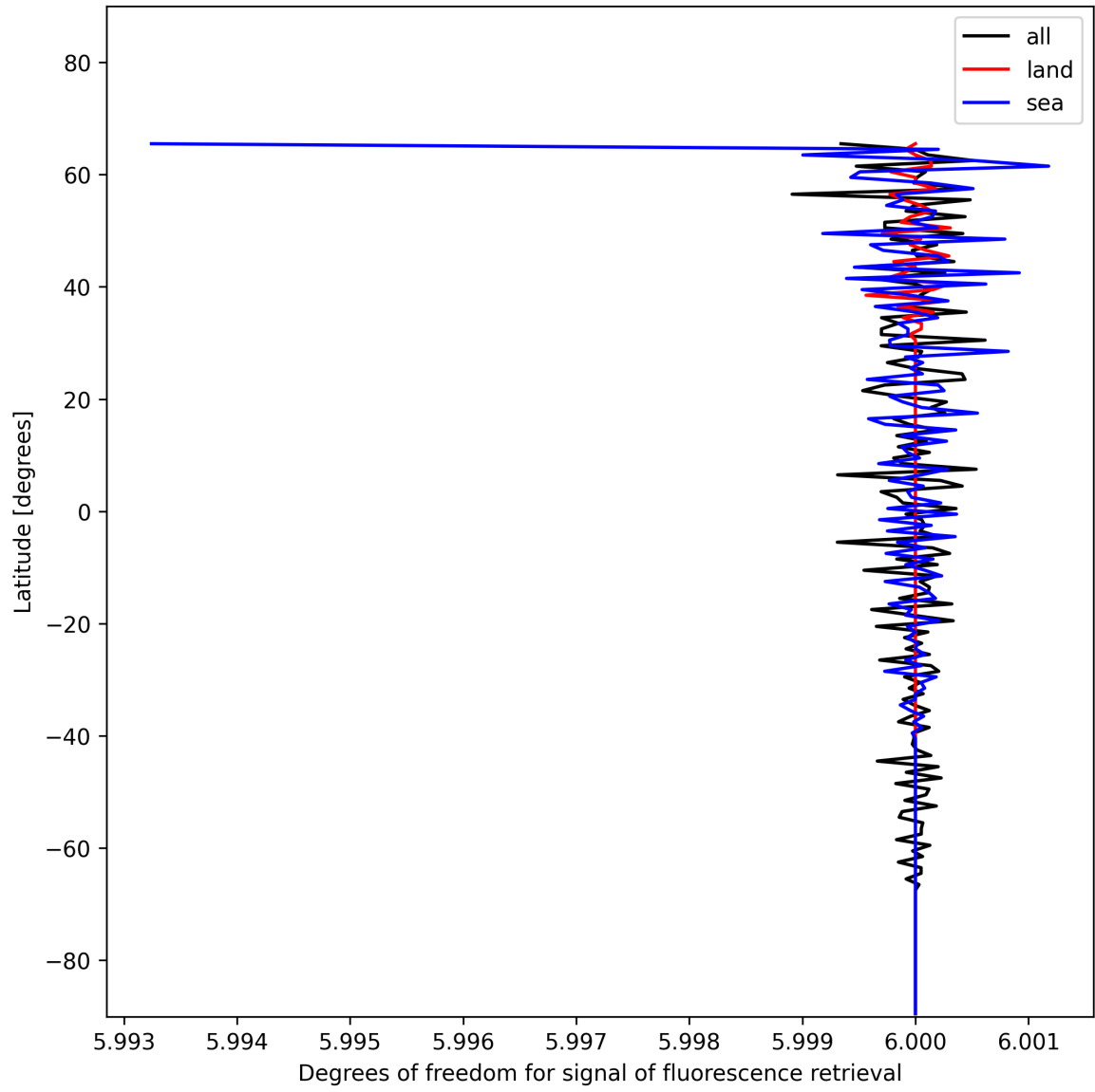
Figure 26: Zonal average of “Degrees of freedom for signal of fluorescence retrieval” for 2025-01-02 to 2025-01-04.
