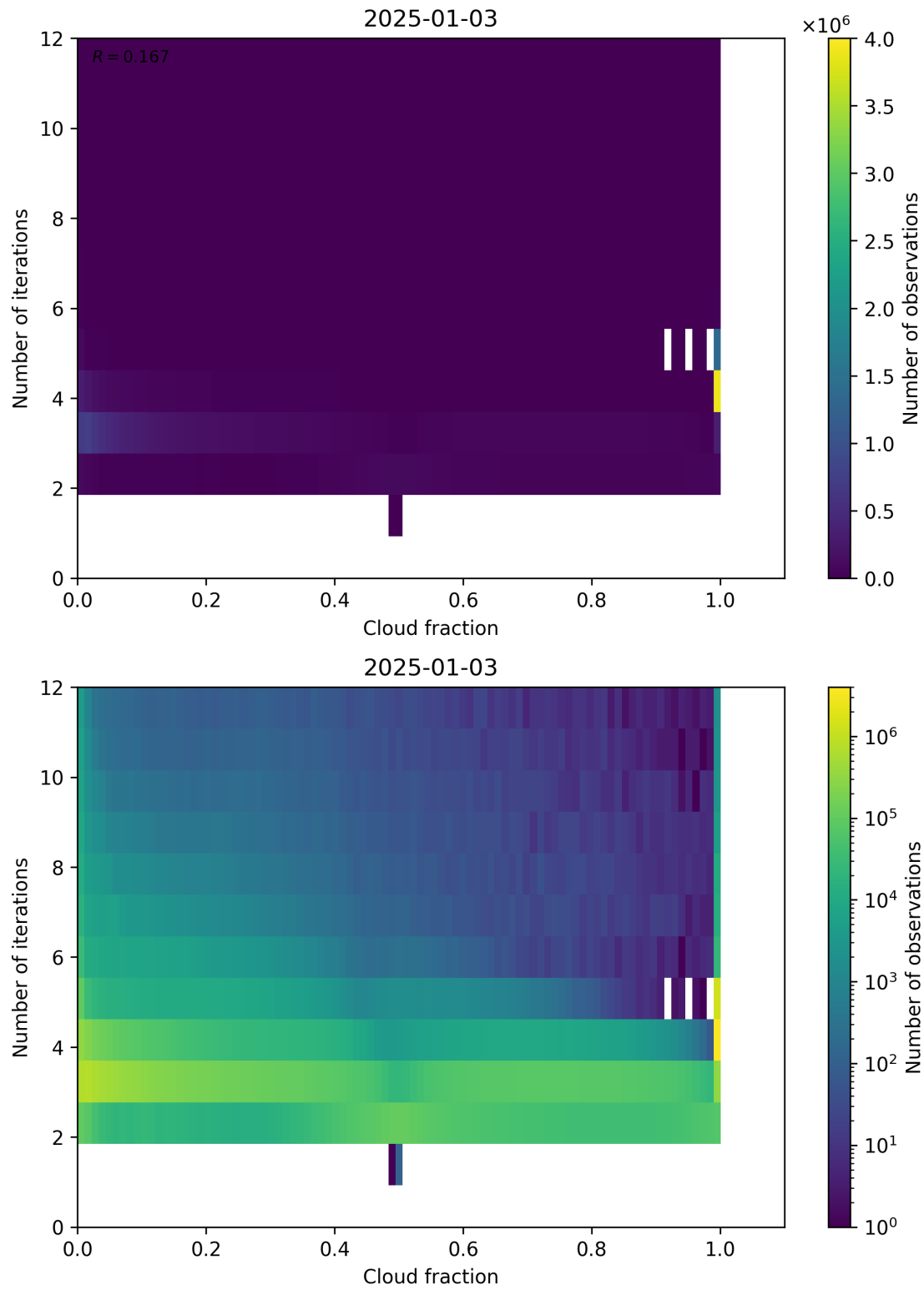
Figure 73: Scatter density plot of “Cloud fraction” against “Number of iterations” for 2025-01-02 to 2025-01-04.
