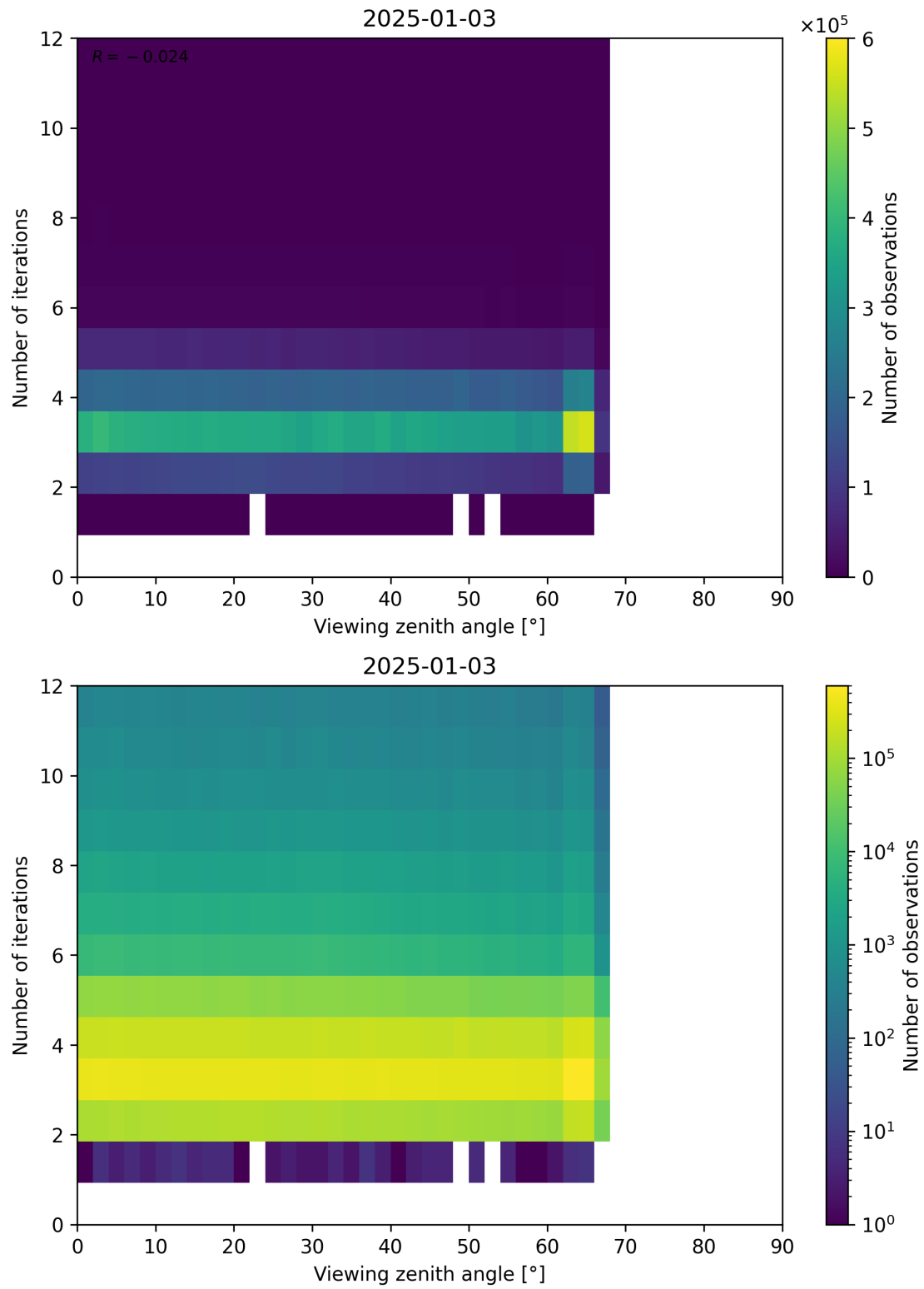
Figure 124: Scatter density plot of “Viewing zenith angle” against “Number of iterations” for 2025-01-02 to 2025-01-04.
