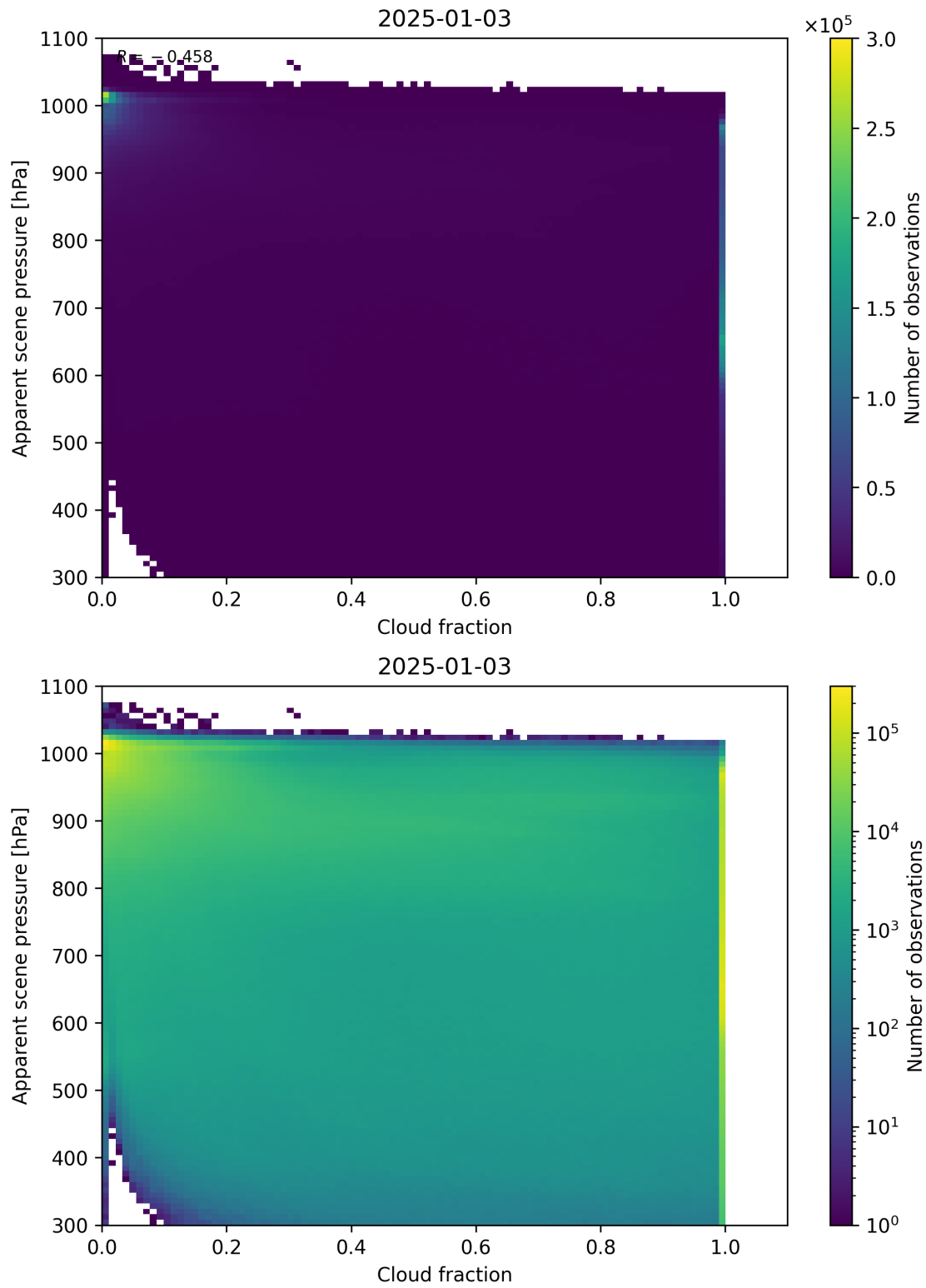
Figure 70: Scatter density plot of “Cloud fraction” against “Apparent scene pressure” for 2025-01-02 to 2025-01-04.
