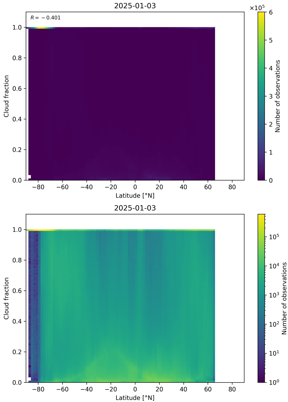
Figure 90: Scatter density plot of “Latitude” against “Cloud fraction” for 2025-01-02 to 2025-01-04.
