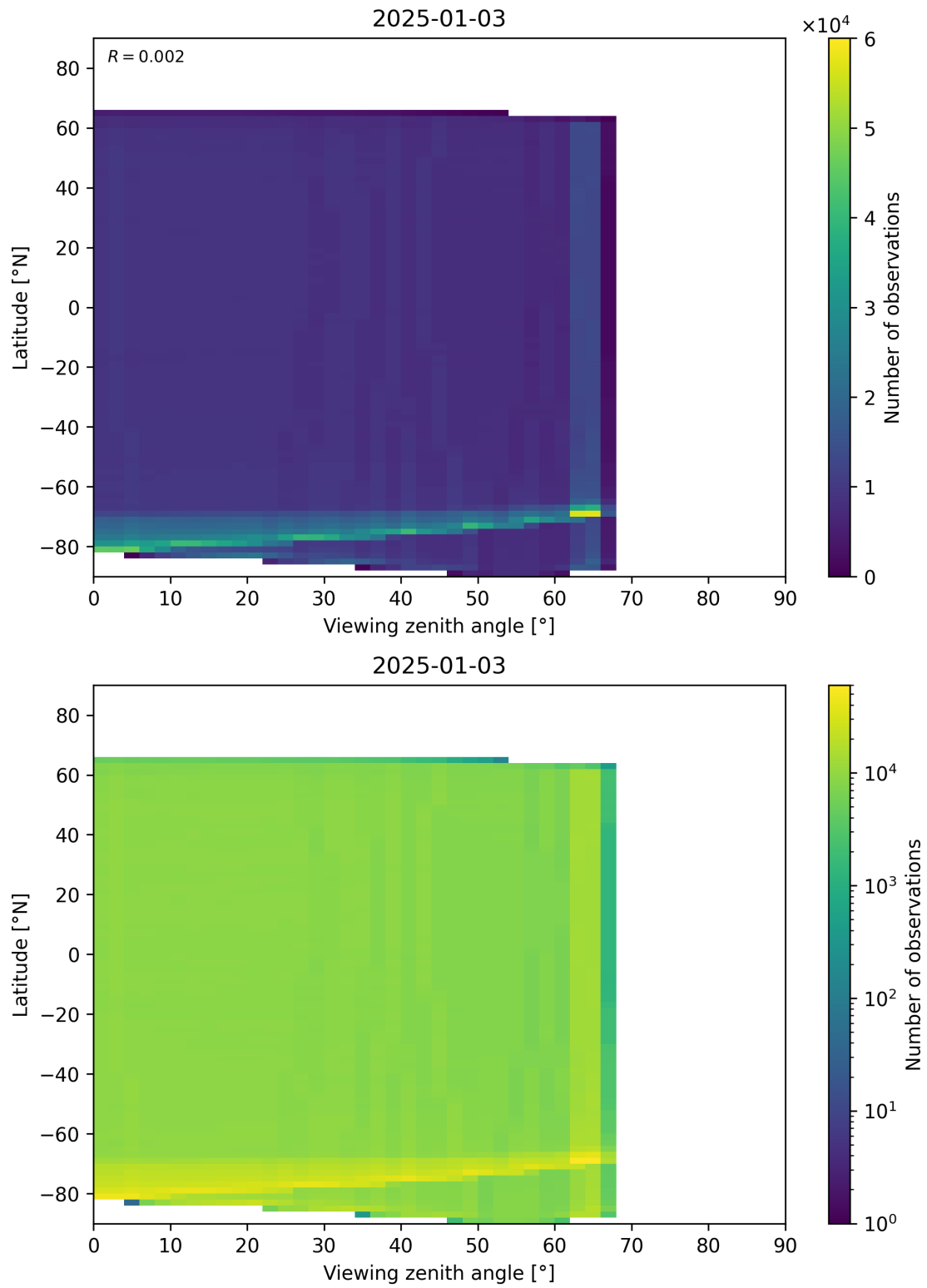
Figure 123: Scatter density plot of “Viewing zenith angle” against “Latitude” for 2025-01-02 to 2025-01-04.
