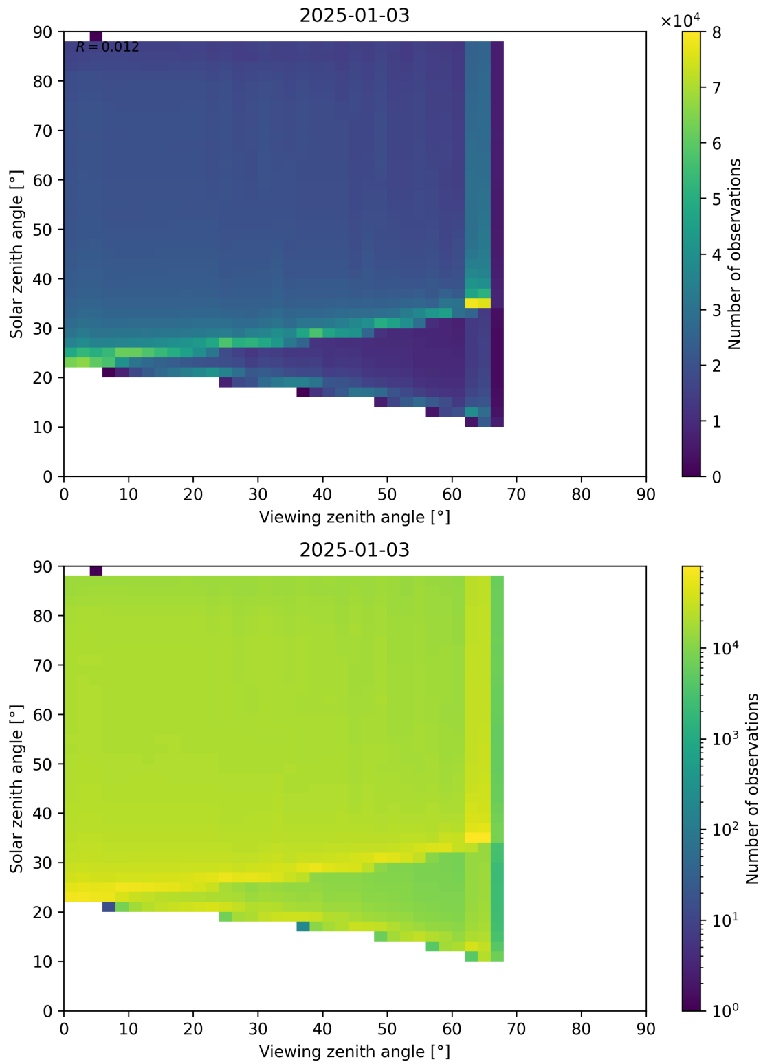
Figure 127: Scatter density plot of “Viewing zenith angle” against “Solar zenith angle” for 2025-01-02 to 2025-01-04.
