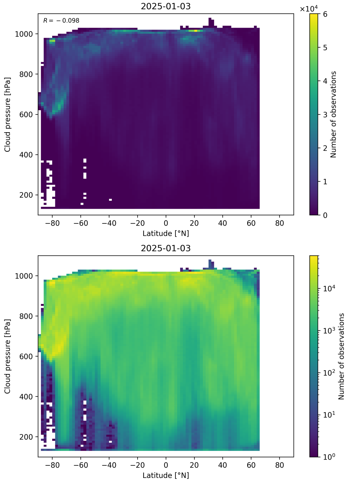
Figure 91: Scatter density plot of “Latitude” against “Cloud pressure” for 2025-01-02 to 2025-01-04.
