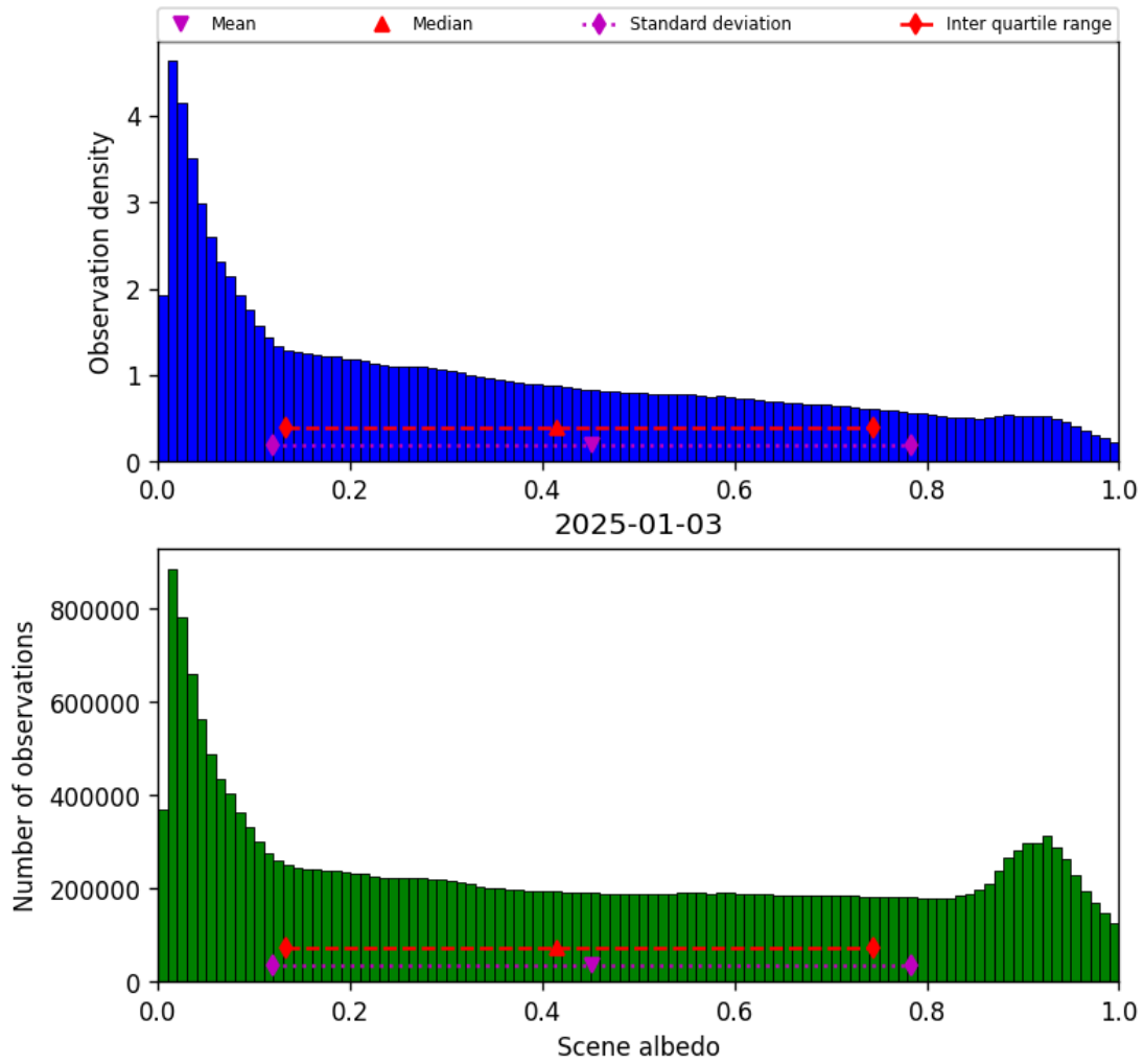
Figure 34: Histogram of “Scene albedo” for 2025-01-02 to 2025-01-04
