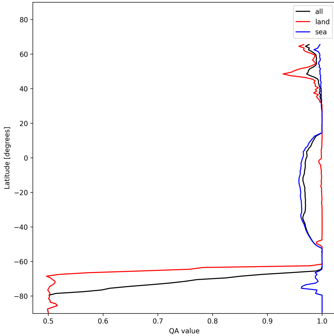
Figure 12: Zonal average of “QA value” for 2025-01-02 to 2025-01-04.
