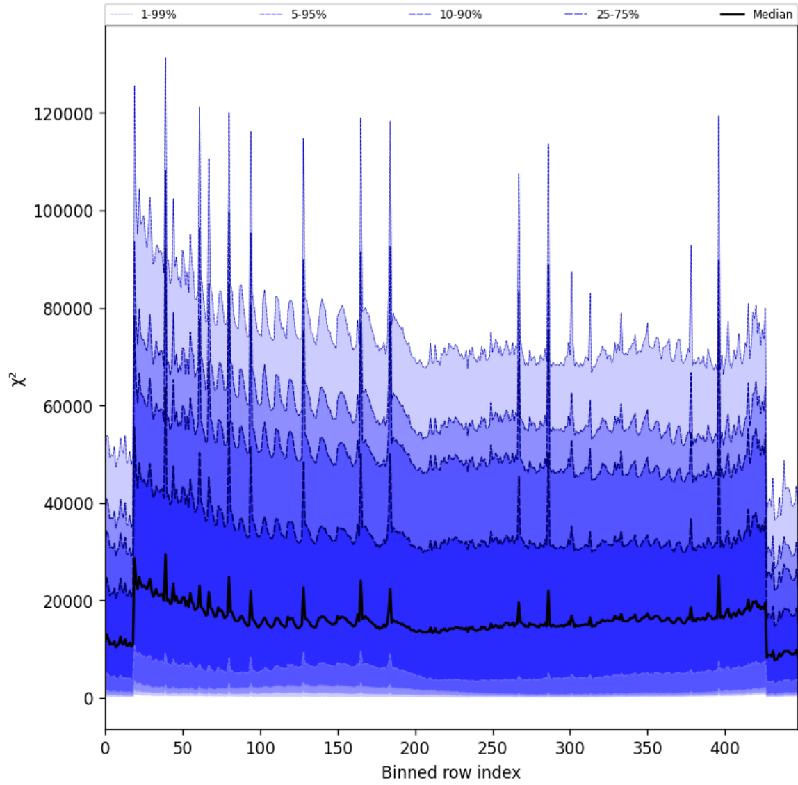
Figure 55: Along track statistics of “ \chi^2 ” for 2025-01-02 to 2025-01-04
