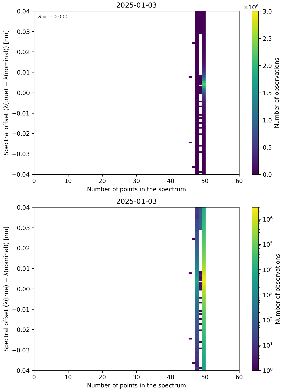
Figure 101: Scatter density plot of “Number of points in the spectrum” against “Spectral offset ( \lambda_{\text{true}} - \lambda_{\text{nominal}} )” for 2025-01-02 to 2025-01-04.
