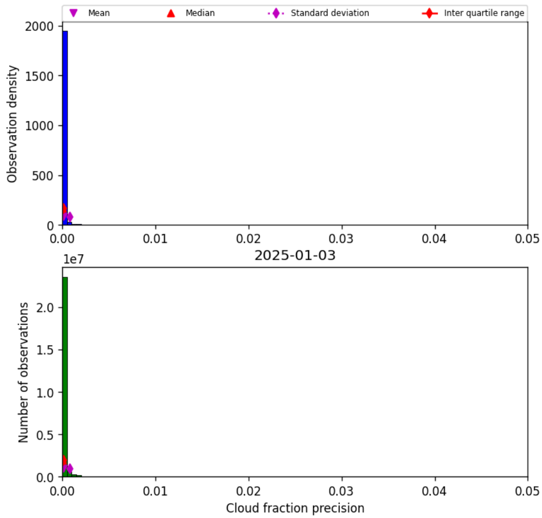
Figure 33: Histogram of “Cloud fraction precision” for 2025-01-02 to 2025-01-04
