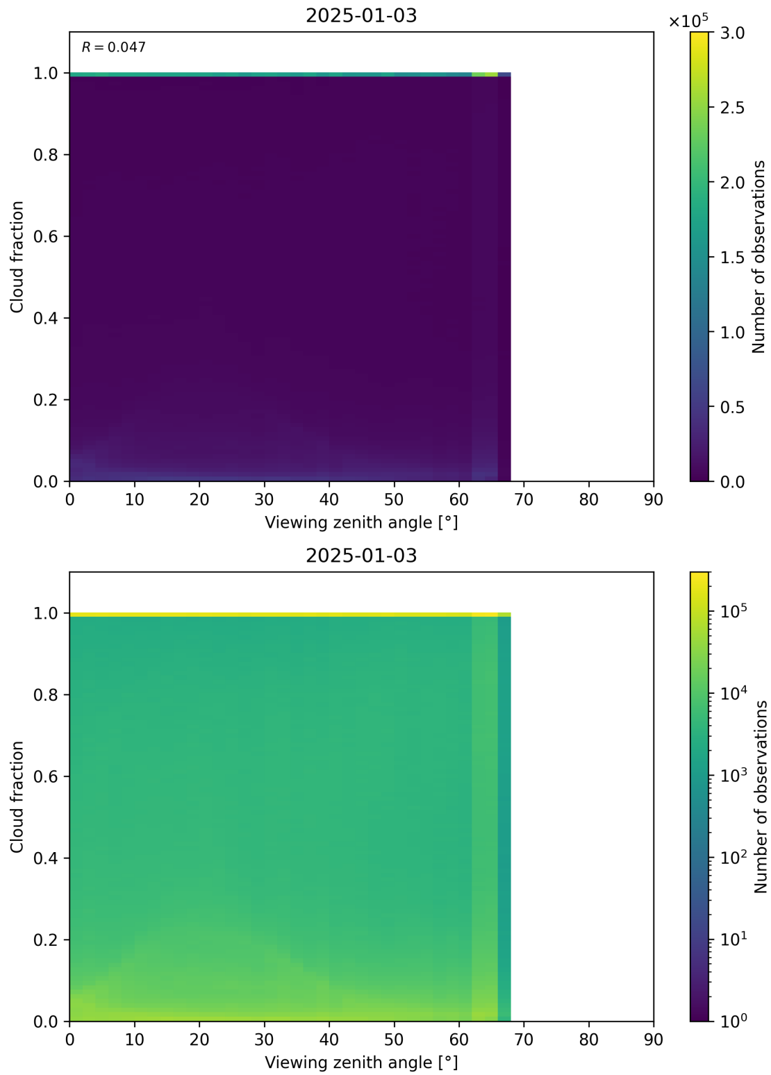
Figure 120: Scatter density plot of “Viewing zenith angle” against “Cloud fraction” for 2025-01-02 to 2025-01-04.
