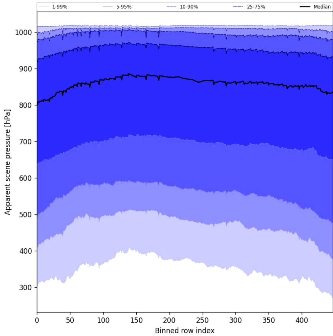
Figure 53: Along track statistics of “Apparent scene pressure” for 2025-01-02 to 2025-01-04
