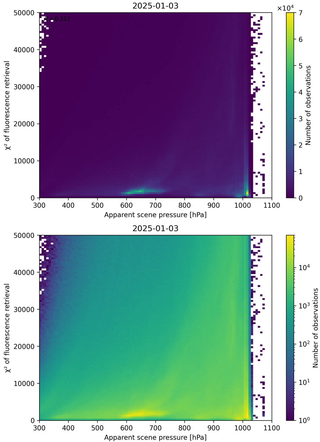
Figure 63: Scatter density plot of “Apparent scene pressure” against “ \chi^2 of fluorescence retrieval” for 2025-01-02 to 2025-01-04.
