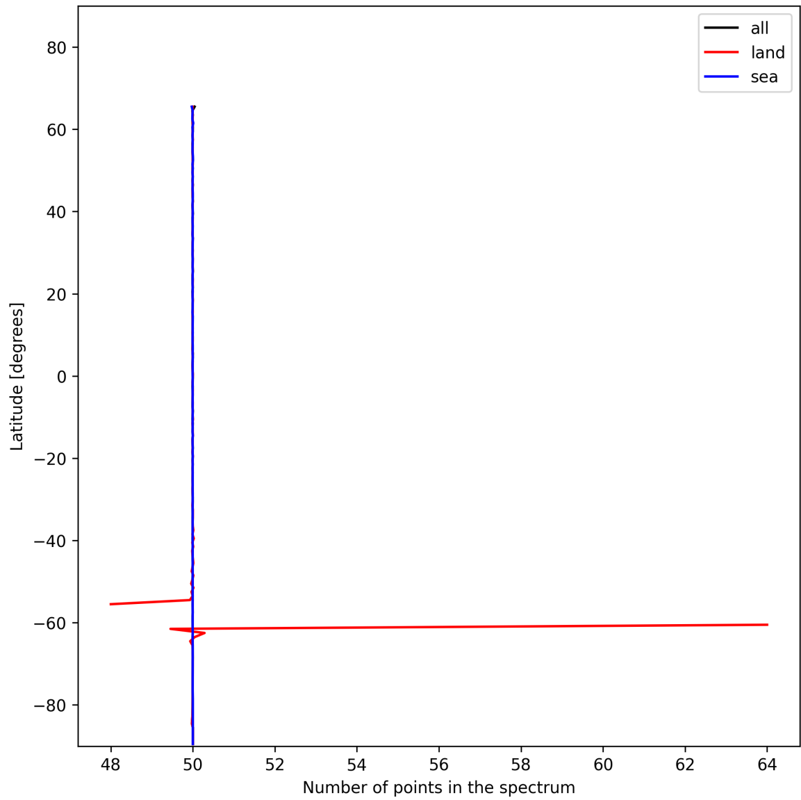
Figure 27: Zonal average of “Number of points in the spectrum” for 2025-01-02 to 2025-01-04.
