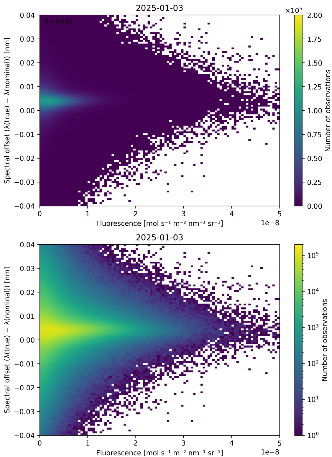
Figure 87: Scatter density plot of “Fluorescence” against “Spectral offset ( \lambda_{\text{true}} - \lambda_{\text{nominal}} )” for 2025-01-02 to 2025-01-04.
