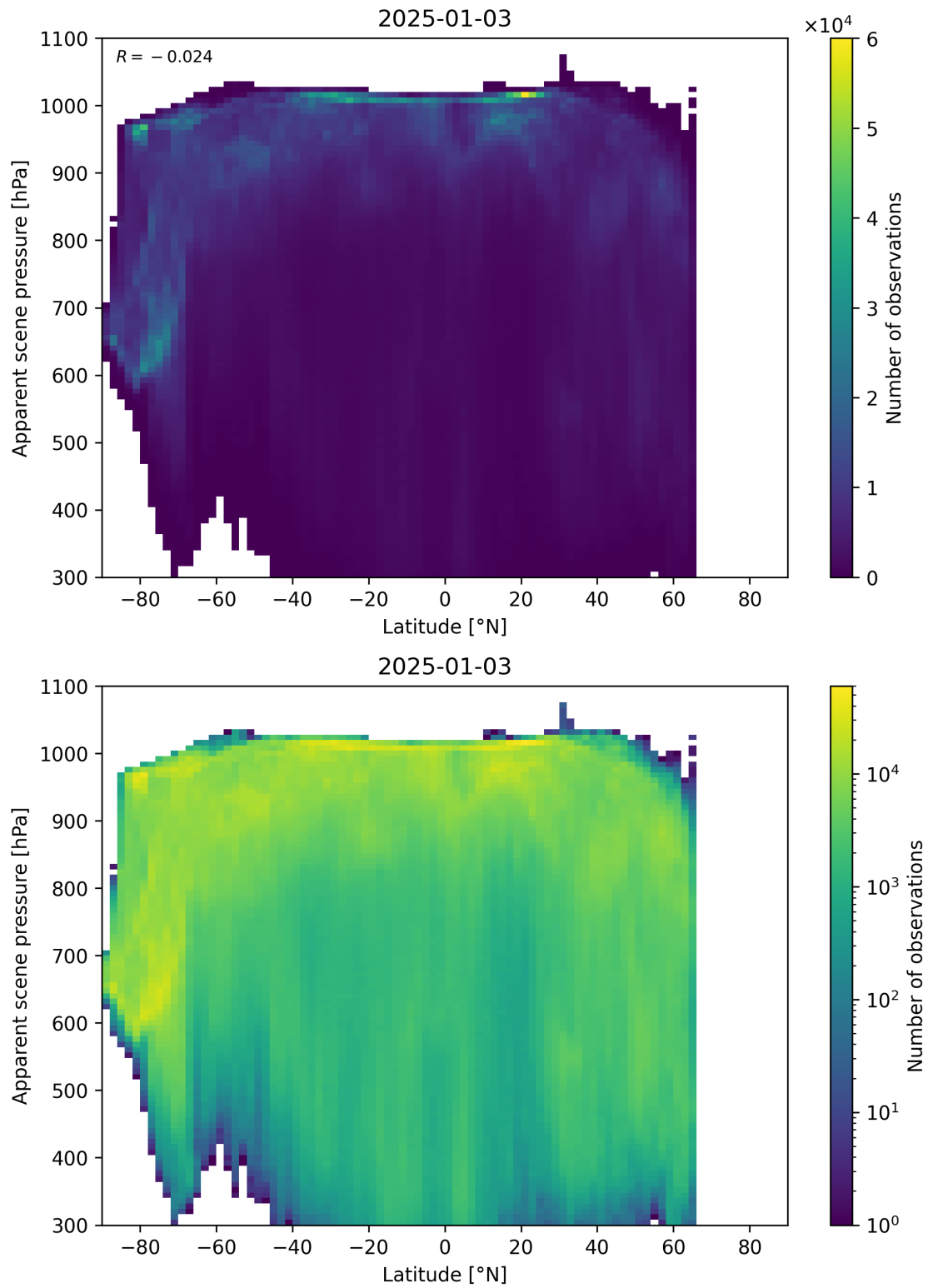
Figure 88: Scatter density plot of “Latitude” against “Apparent scene pressure” for 2025-01-02 to 2025-01-04.
