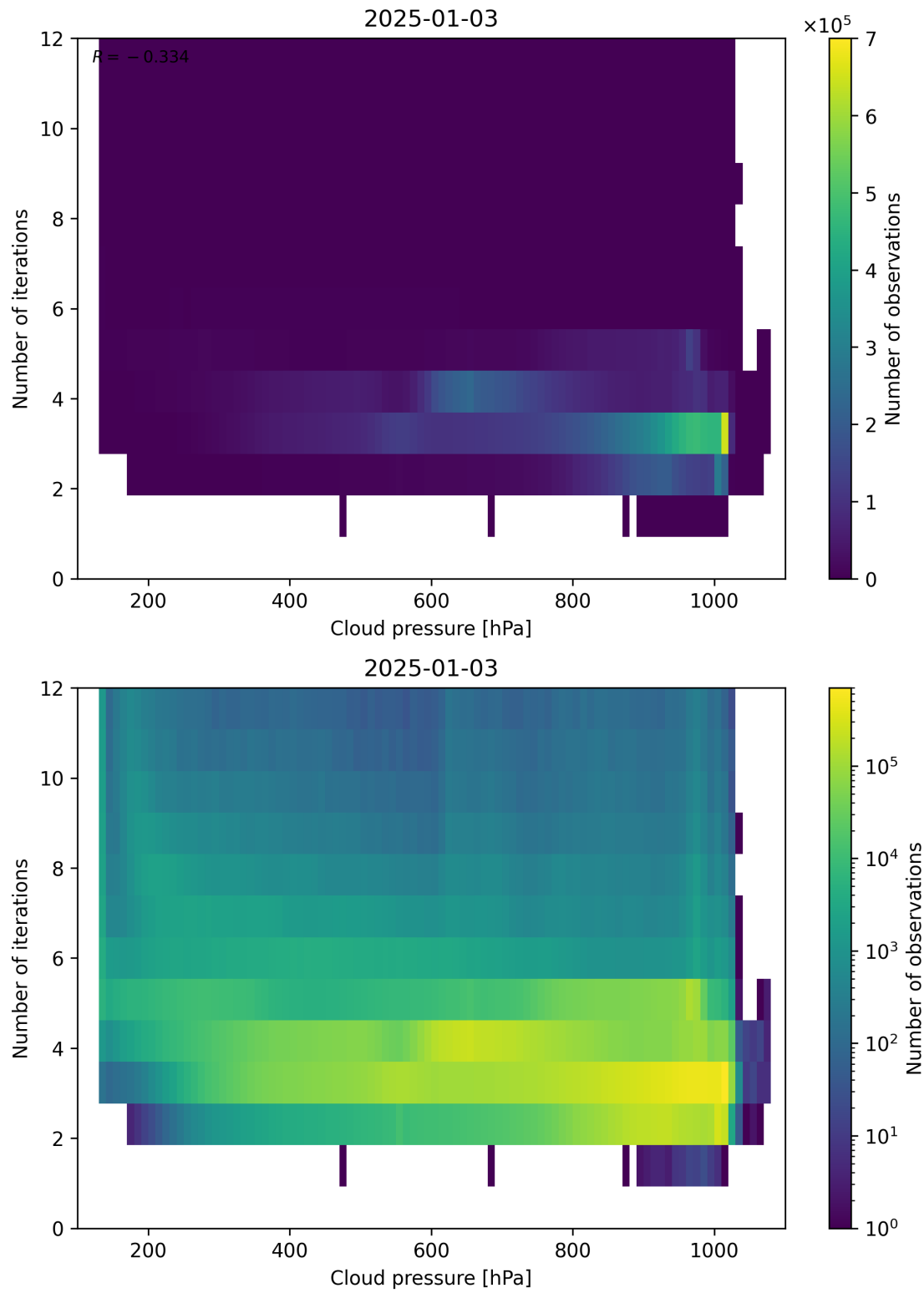
Figure 81: Scatter density plot of “Cloud pressure” against “Number of iterations” for 2025-01-02 to 2025-01-04.
