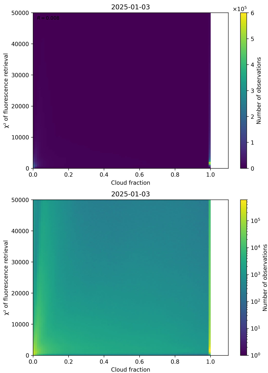
Figure 71: Scatter density plot of “Cloud fraction” against “ \chi^2 of fluorescence retrieval” for 2025-01-02 to 2025-01-04.
