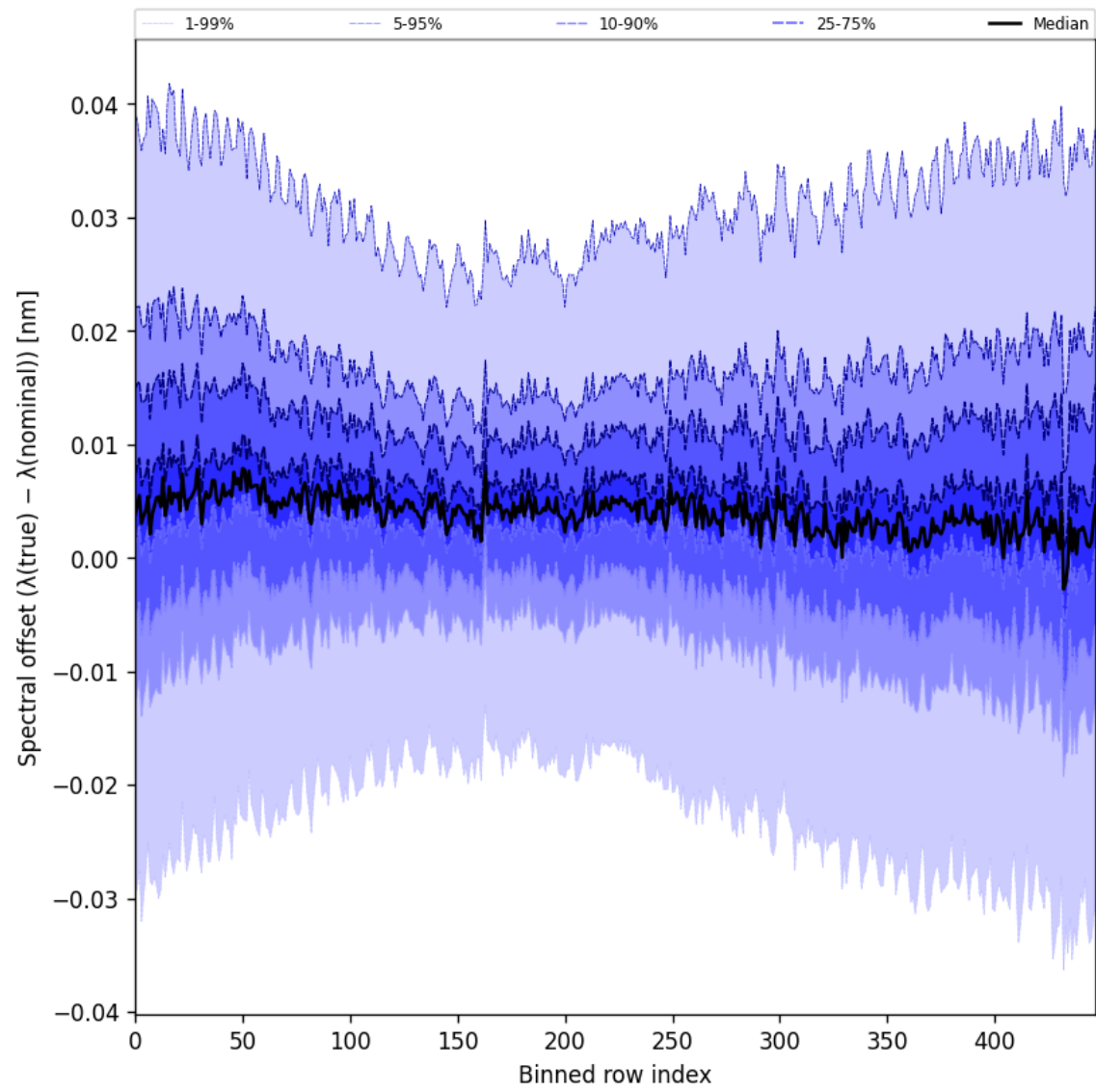
Figure 62: Along track statistics of “Spectral offset ( \lambda_{\text{true}} - \lambda_{\text{nominal}} )” for 2025-01-02 to 2025-01-04
