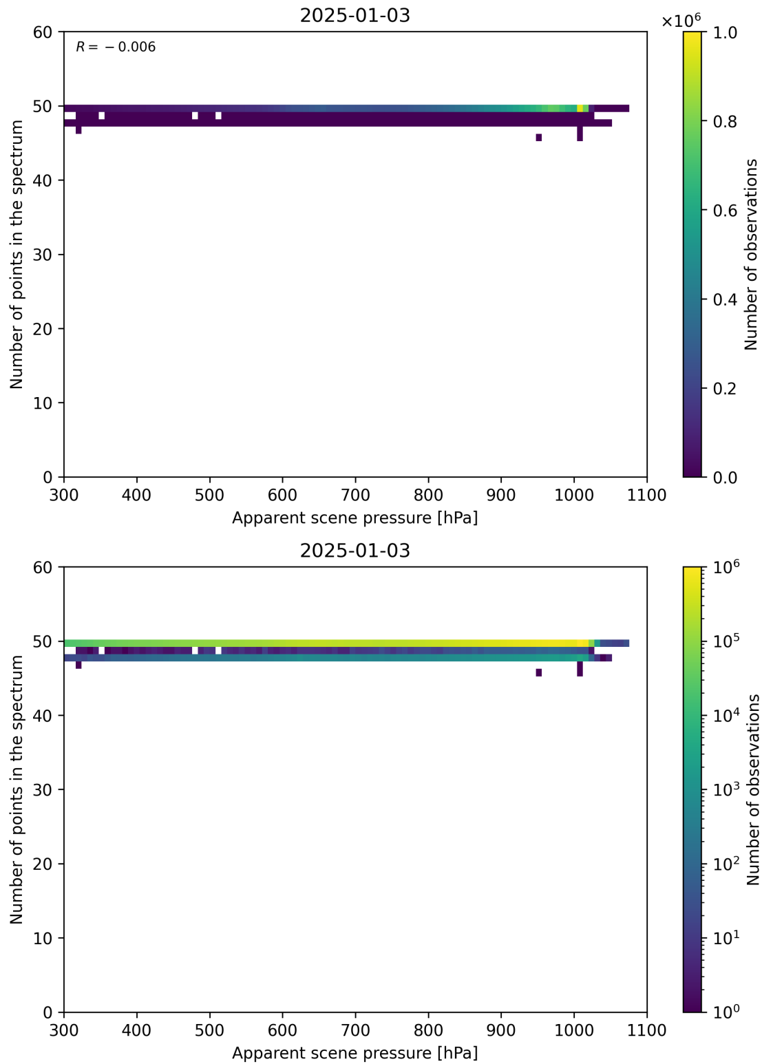
Figure 66: Scatter density plot of “Apparent scene pressure” against “Number of points in the spectrum” for 2025-01-02 to 2025-01-04.
