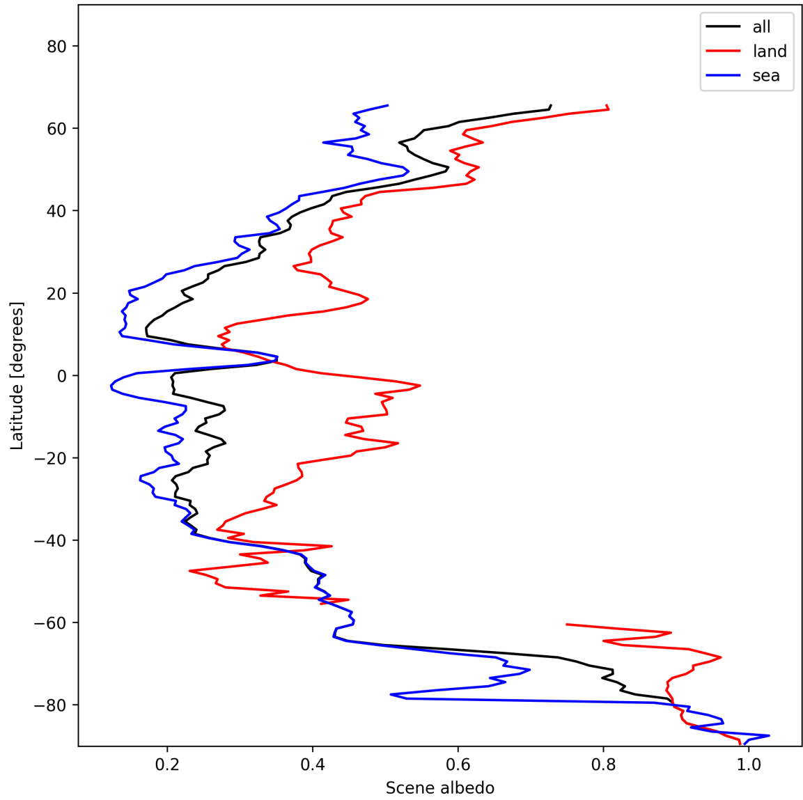
Figure 17: Zonal average of “Scene albedo” for 2025-01-02 to 2025-01-04.
