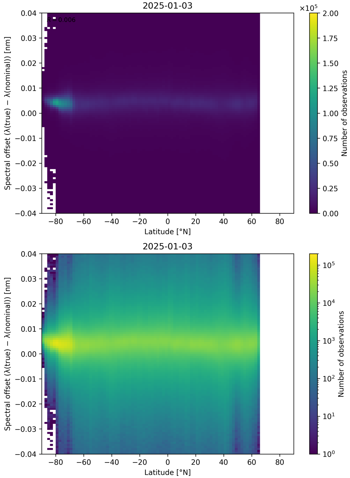
Figure 96: Scatter density plot of “Latitude” against “Spectral offset ( \lambda_{\text{true}} - \lambda_{\text{nominal}} )” for 2025-01-02 to 2025-01-04.
