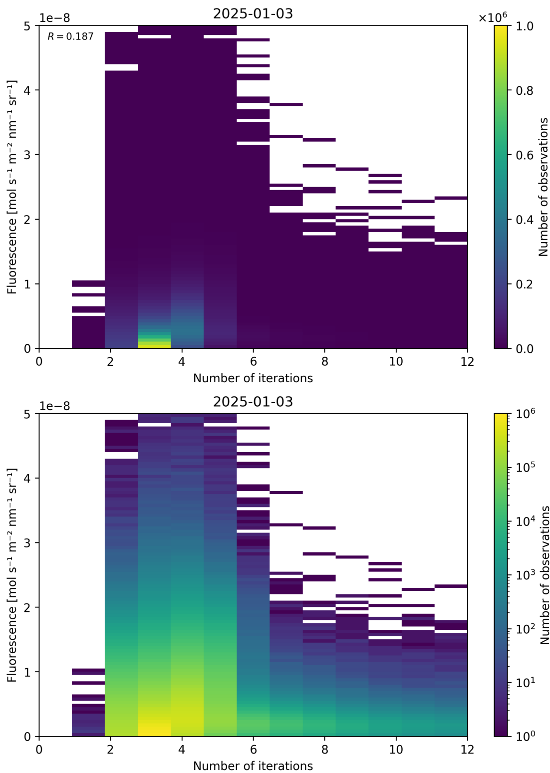
Figure 98: Scatter density plot of “Number of iterations” against “Fluorescence” for 2025-01-02 to 2025-01-04.
