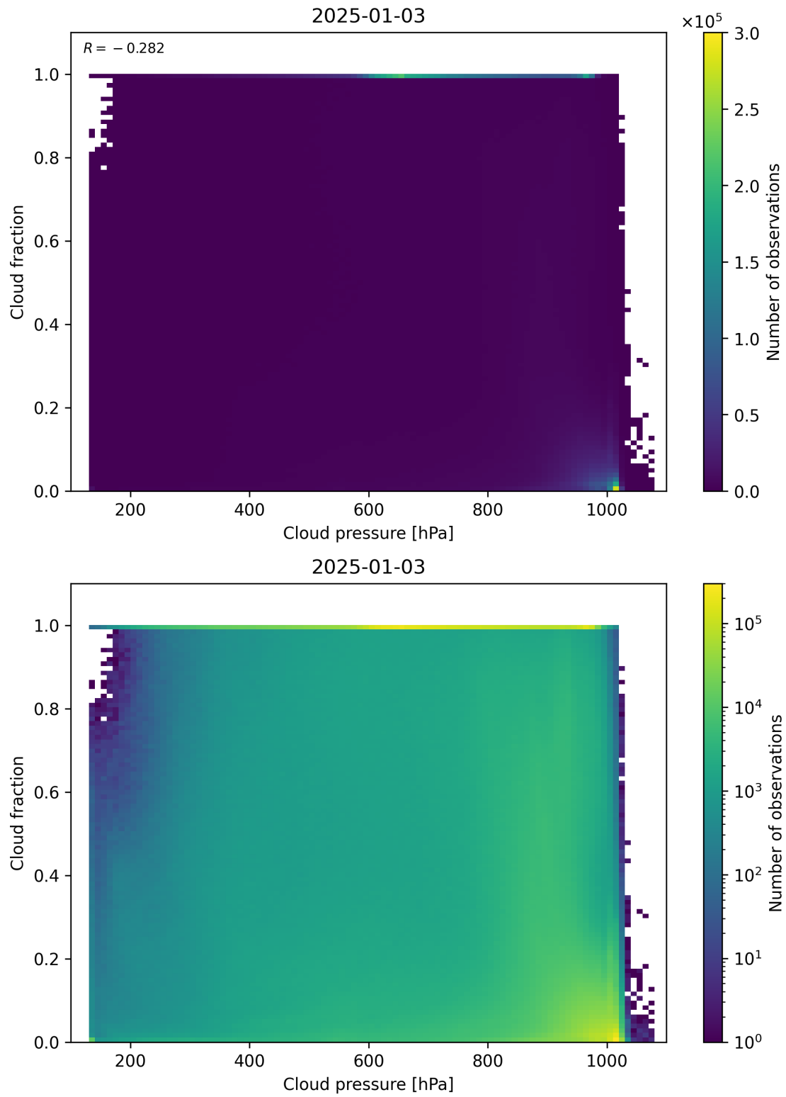
Figure 79: Scatter density plot of “Cloud pressure” against “Cloud fraction” for 2025-01-02 to 2025-01-04.
