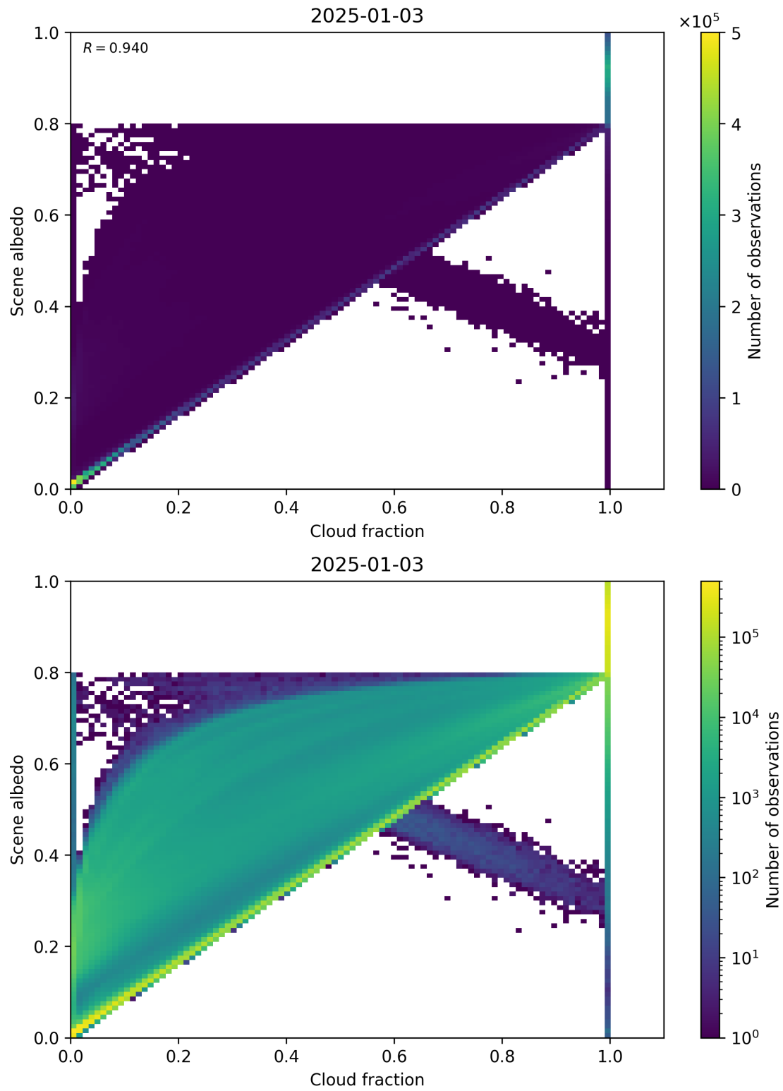
Figure 75: Scatter density plot of “Cloud fraction” against “Scene albedo” for 2025-01-02 to 2025-01-04.
