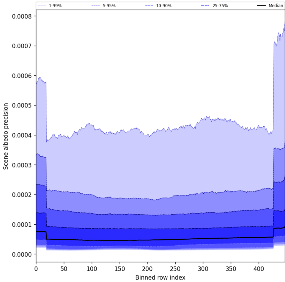
Figure 52: Along track statistics of “Scene albedo precision” for 2025-01-02 to 2025-01-04
