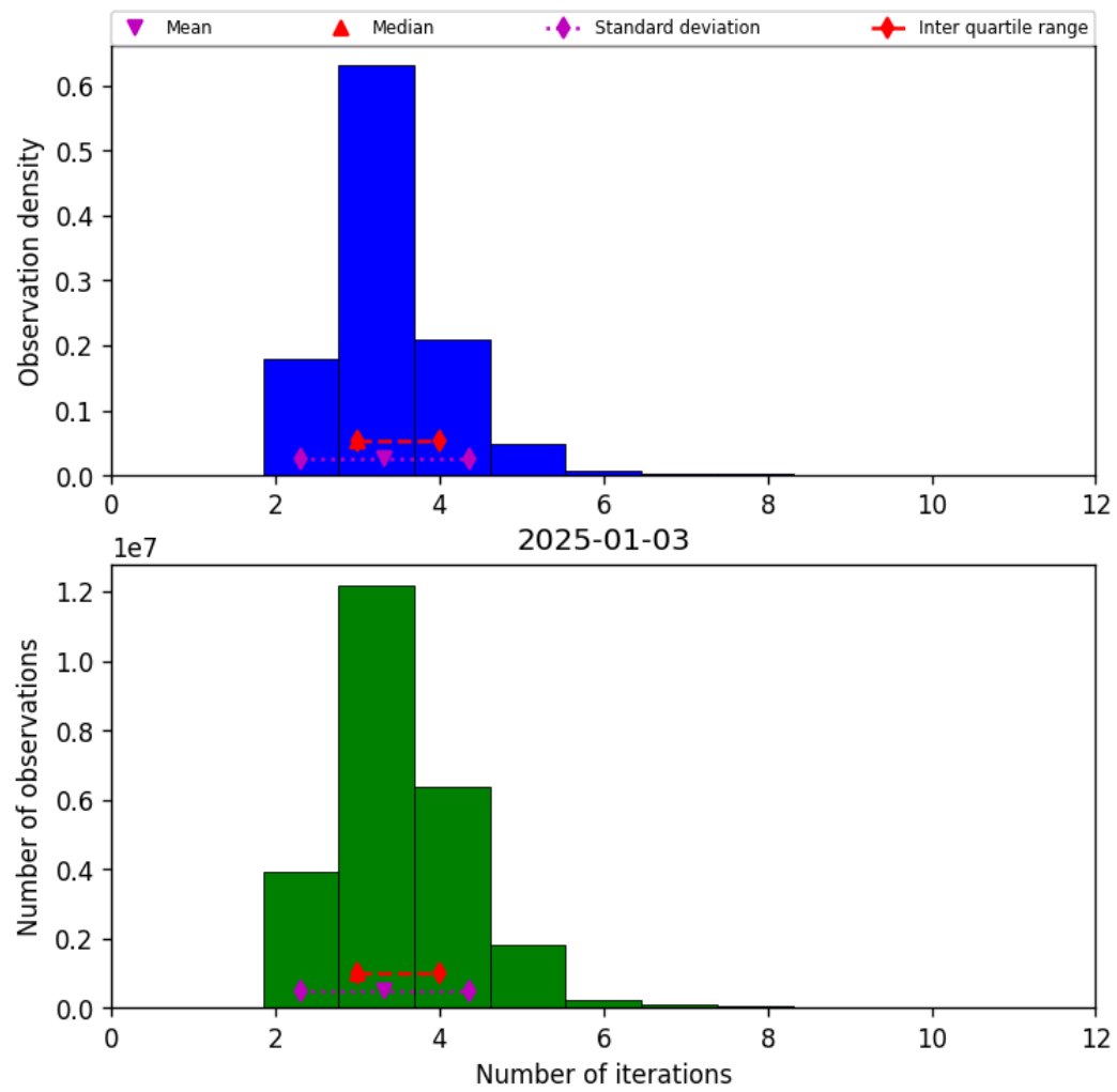
Figure 39: Histogram of “Number of iterations” for 2025-01-02 to 2025-01-04
