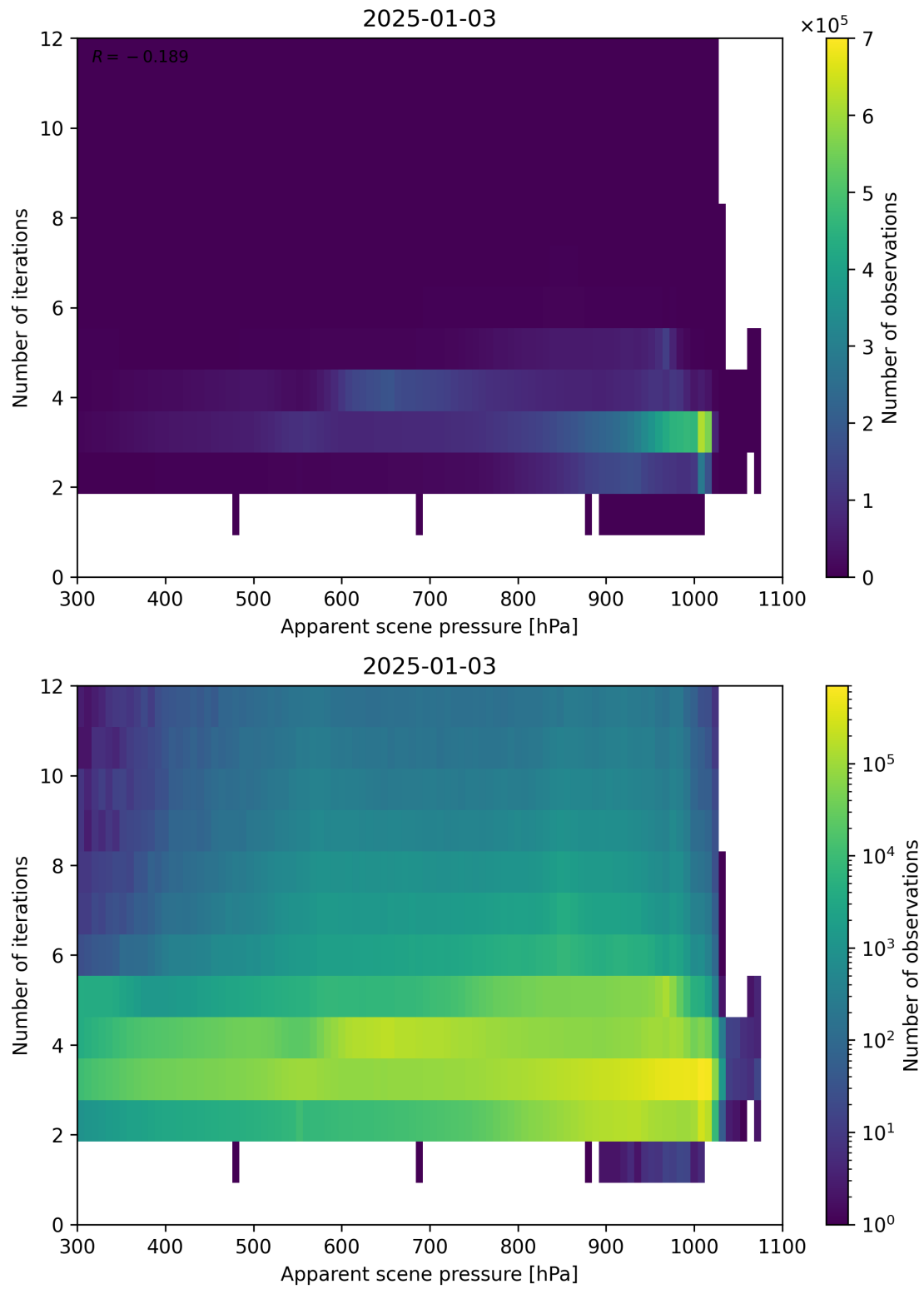
Figure 65: Scatter density plot of “Apparent scene pressure” against “Number of iterations” for 2025-01-02 to 2025-01-04.
