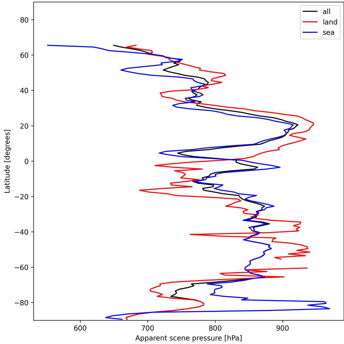
Figure 19: Zonal average of “Apparent scene pressure” for 2025-01-02 to 2025-01-04.
