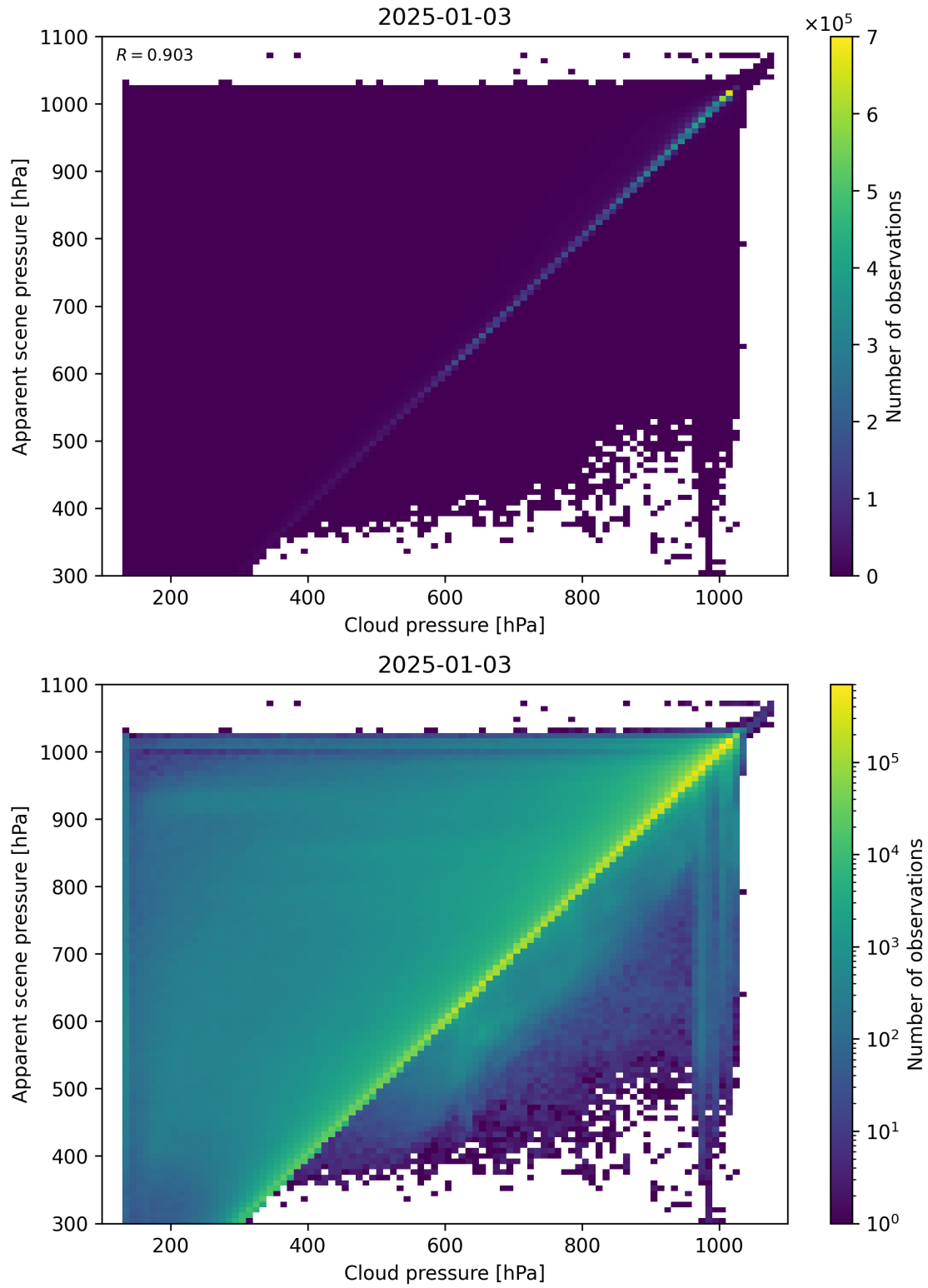
Figure 77: Scatter density plot of “Cloud pressure” against “Apparent scene pressure” for 2025-01-02 to 2025-01-04.
