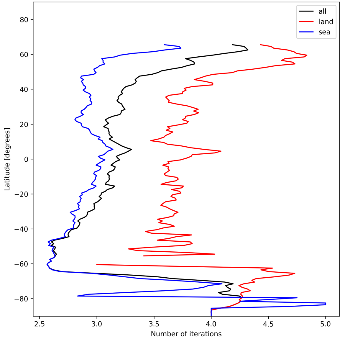
Figure 22: Zonal average of “Number of iterations” for 2025-01-02 to 2025-01-04.
