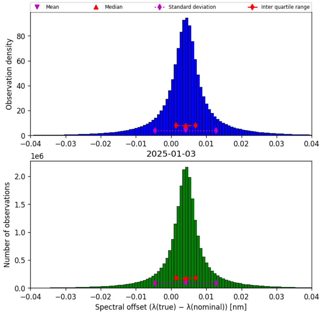
Figure 45: Histogram of “Spectral offset ( \lambda_{\text{true}} - \lambda_{\text{nominal}} )” for 2025-01-02 to 2025-01-04
