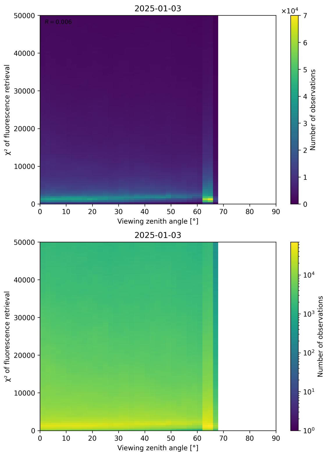
Figure 119: Scatter density plot of “Viewing zenith angle” against “ \chi^2 of fluorescence retrieval” for 2025-01-02 to 2025-01-04.
