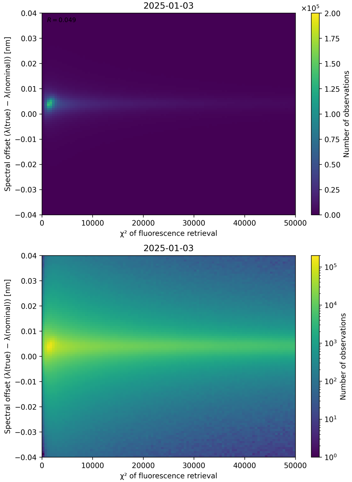
Figure 69: Scatter density plot of “ \chi^2 of fluorescence retrieval” against “Spectral offset ( \lambda_{\text{true}} - \lambda_{\text{nominal}} )” for 2025-01-02 to 2025-01-04.
