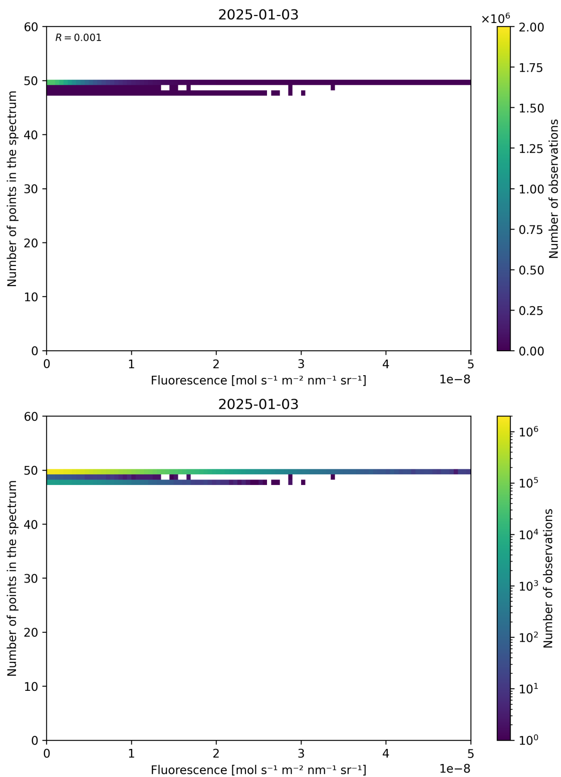
Figure 86: Scatter density plot of “Fluorescence” against “Number of points in the spectrum” for 2025-01-02 to 2025-01-04.
