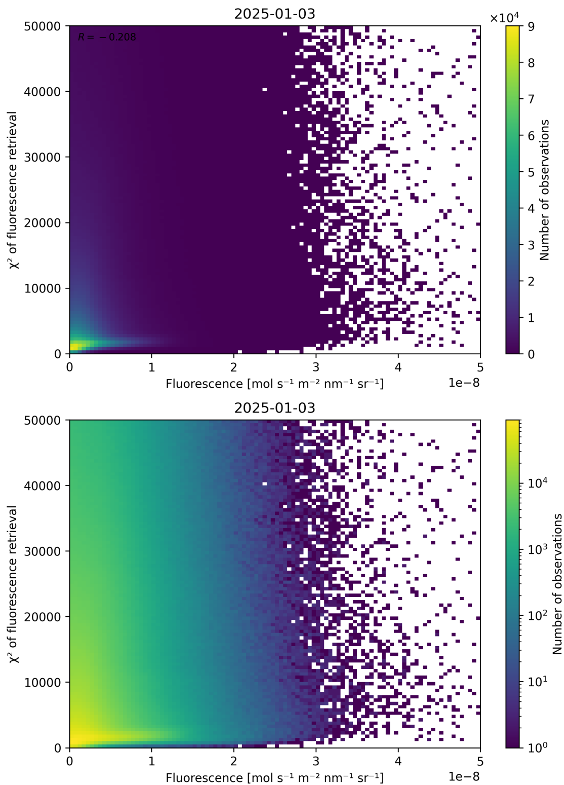
Figure 85: Scatter density plot of “Fluorescence” against “ \chi^2 of fluorescence retrieval” for 2025-01-02 to 2025-01-04.
