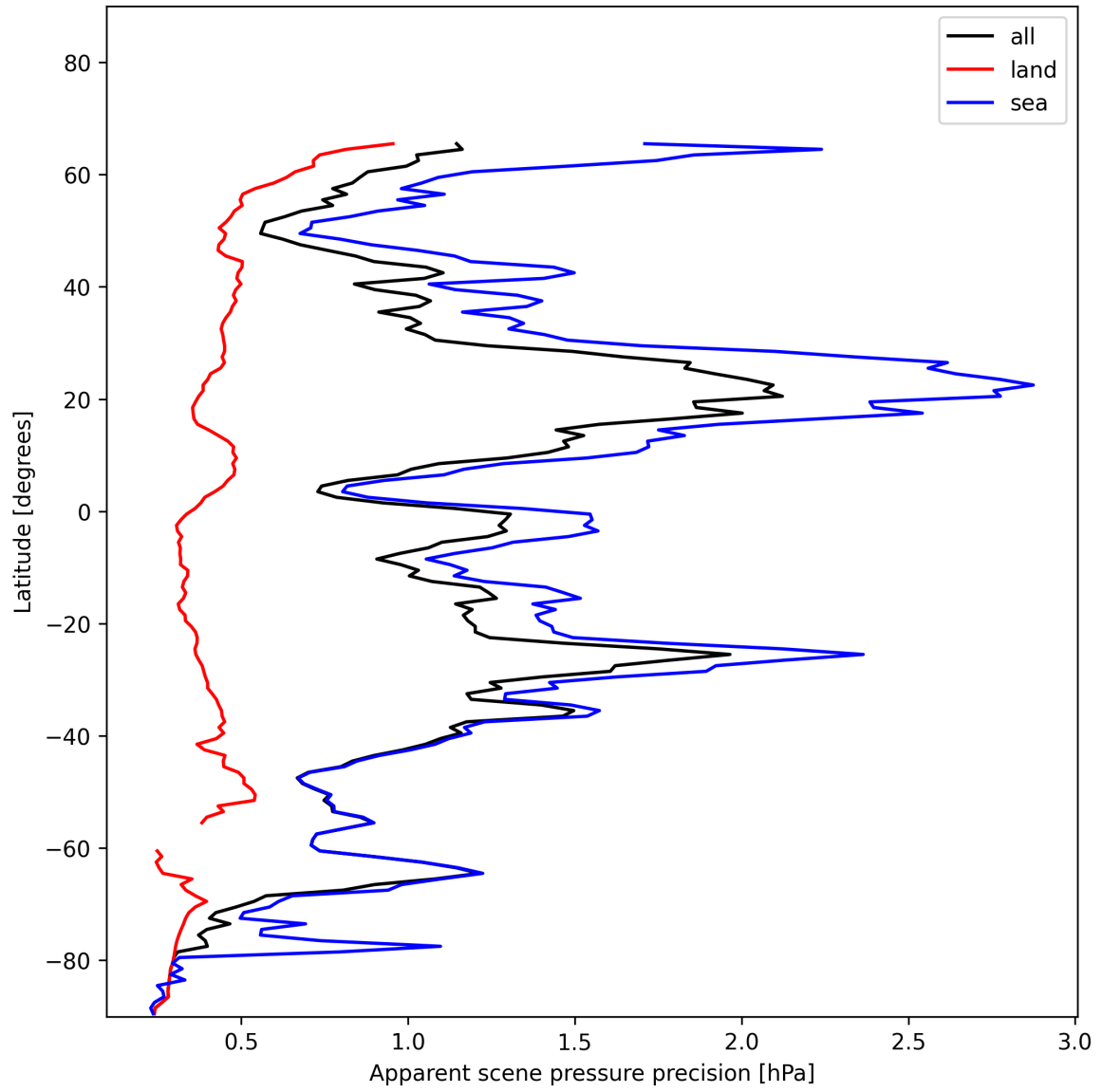
Figure 20: Zonal average of “Apparent scene pressure precision” for 2025-01-02 to 2025-01-04.
