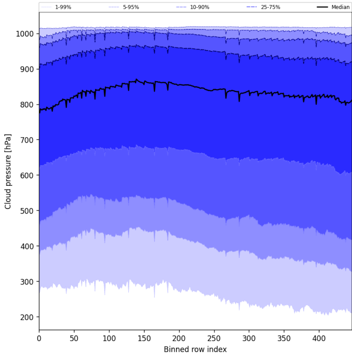
Figure 47: Along track statistics of “Cloud pressure” for 2025-01-02 to 2025-01-04
