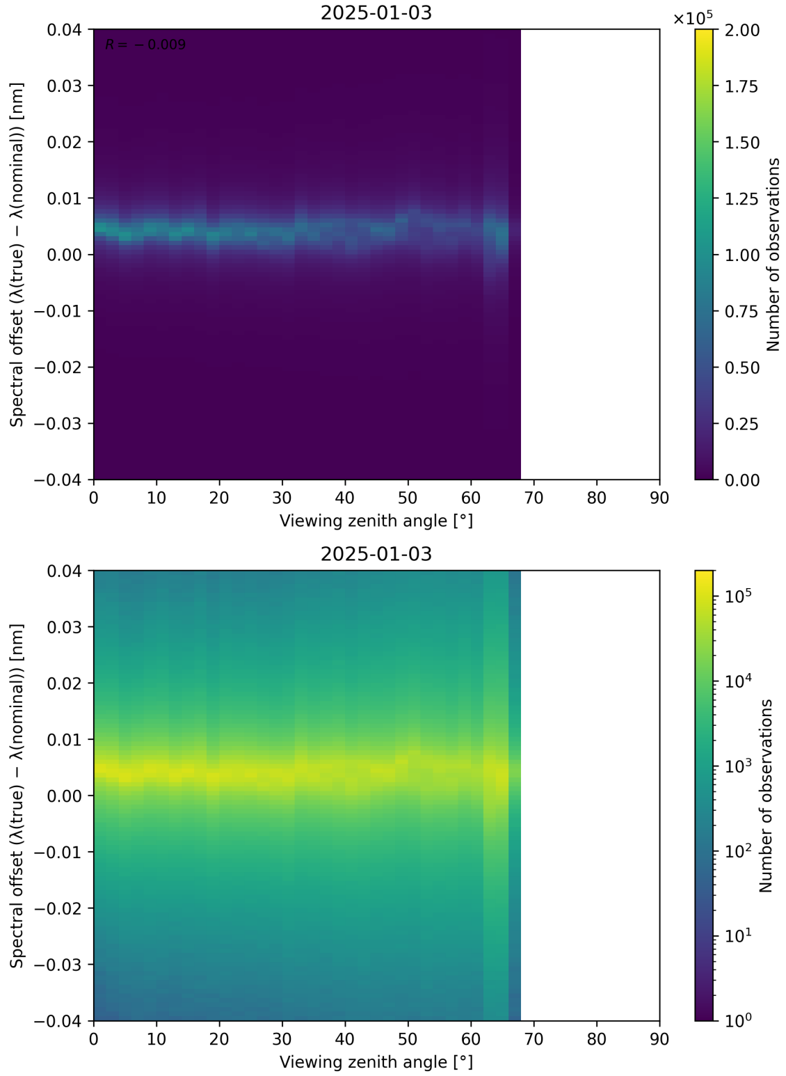
Figure 128: Scatter density plot of “Viewing zenith angle” against “Spectral offset ( \lambda_{\text{true}} - \lambda_{\text{nominal}} )” for 2025-01-02 to 2025-01-04.
