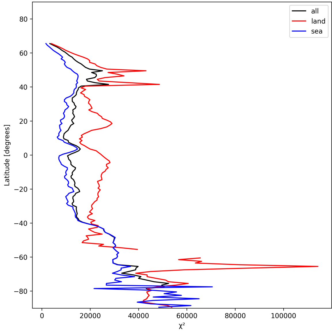
Figure 21: Zonal average of “ \chi^2 ” for 2025-01-02 to 2025-01-04.
