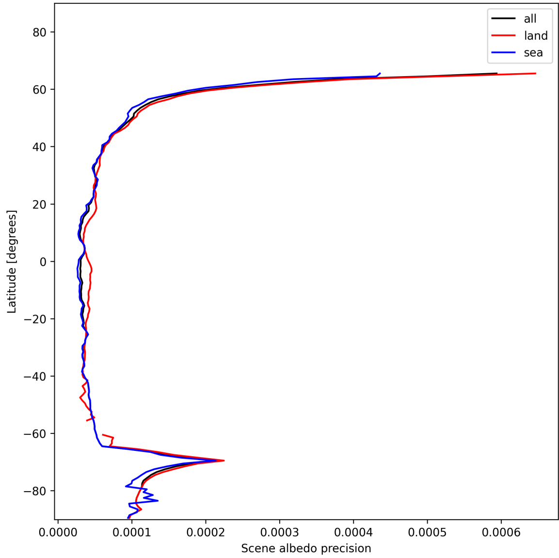
Figure 18: Zonal average of “Scene albedo precision” for 2025-01-02 to 2025-01-04.
