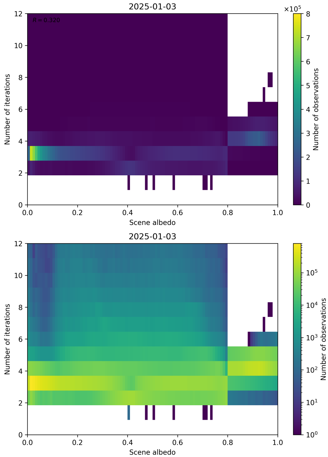
Figure 105: Scatter density plot of “Scene albedo” against “Number of iterations” for 2025-01-02 to 2025-01-04.
