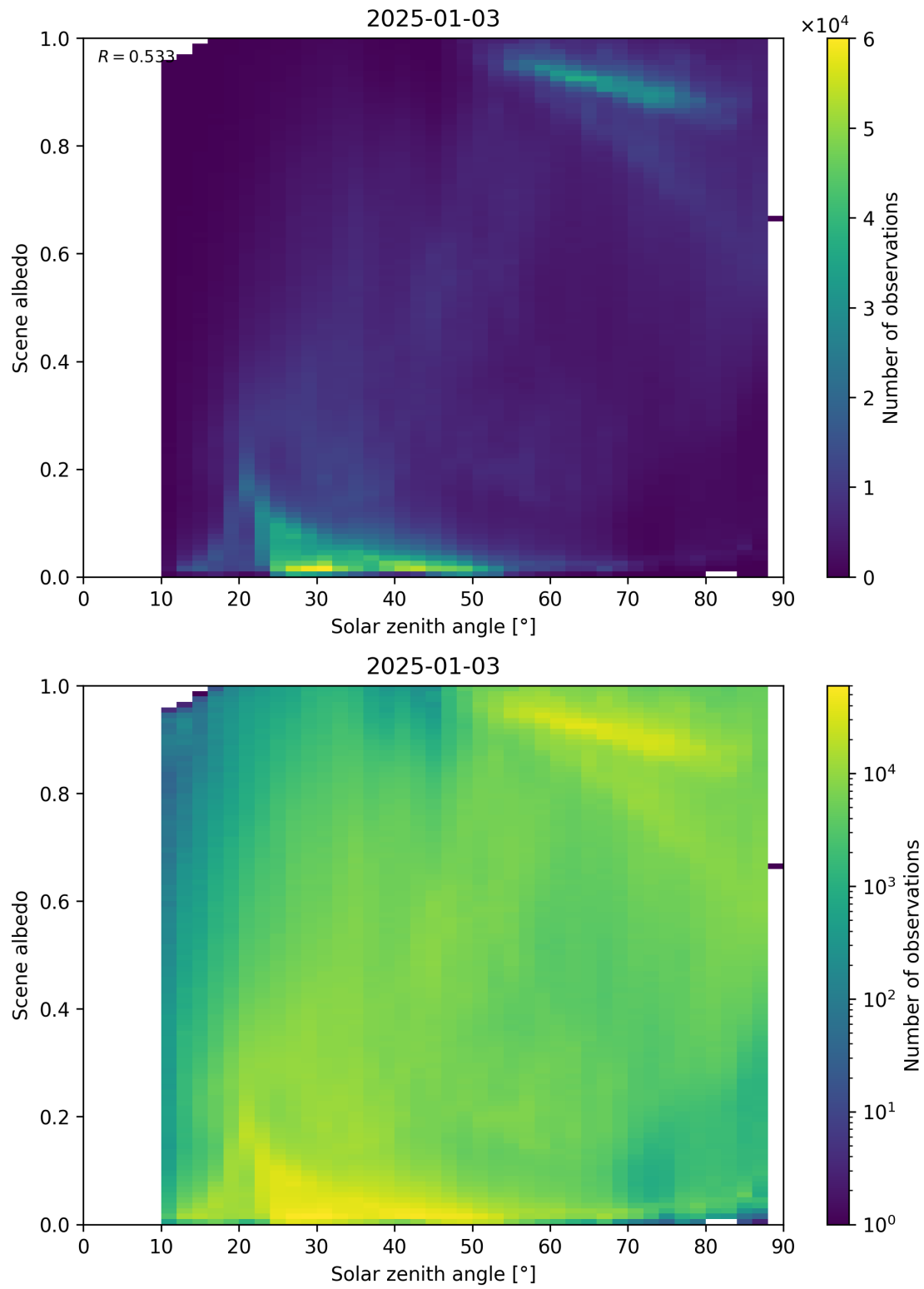
Figure 116: Scatter density plot of “Solar zenith angle” against “Scene albedo” for 2025-01-02 to 2025-01-04.
