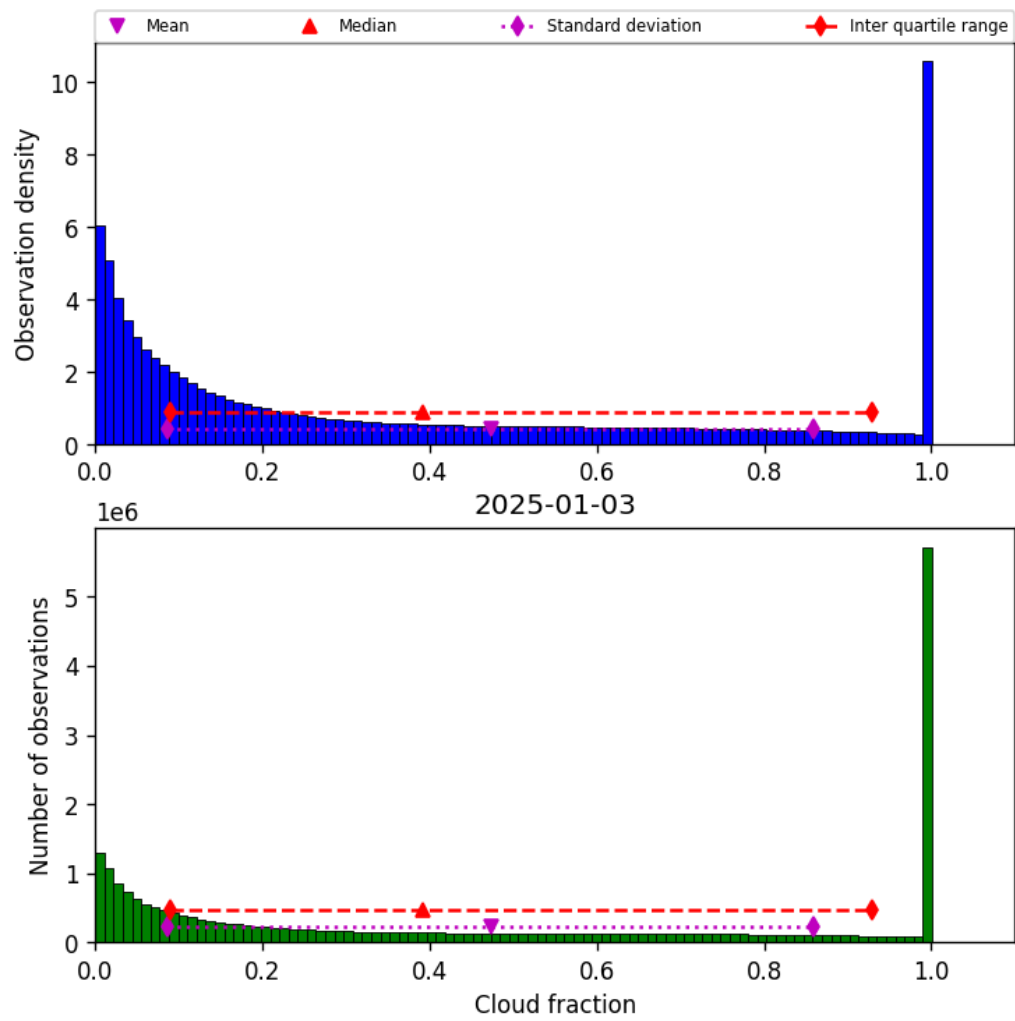
Figure 32: Histogram of “Cloud fraction” for 2025-01-02 to 2025-01-04
