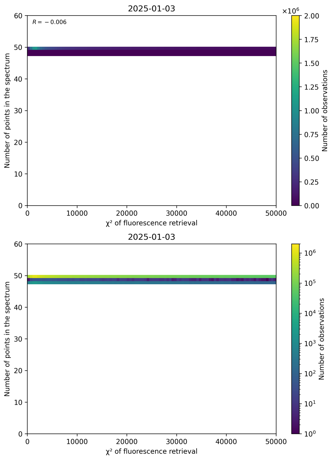
Figure 68: Scatter density plot of “ \chi^2 of fluorescence retrieval” against “Number of points in the spectrum” for 2025-01-02 to 2025-01-04.
