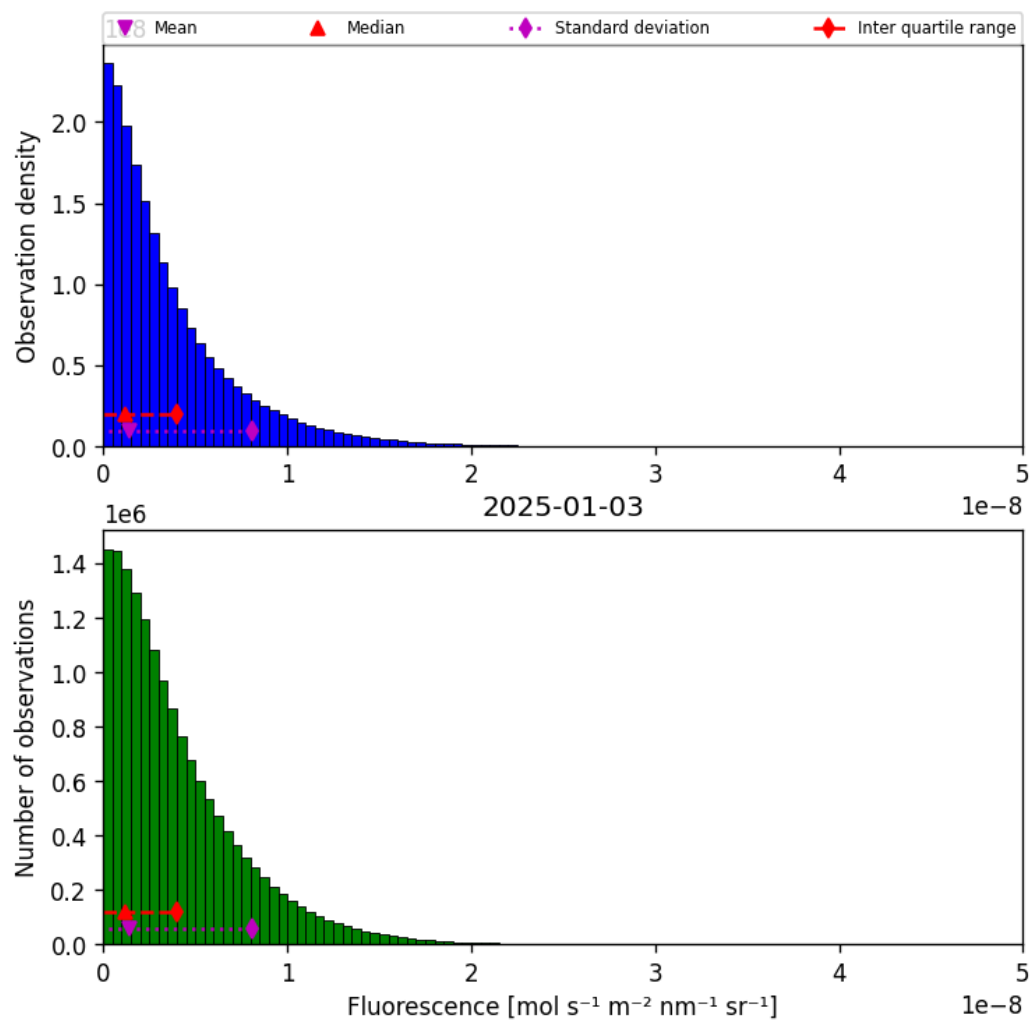
Figure 40: Histogram of “Fluorescence” for 2025-01-02 to 2025-01-04
