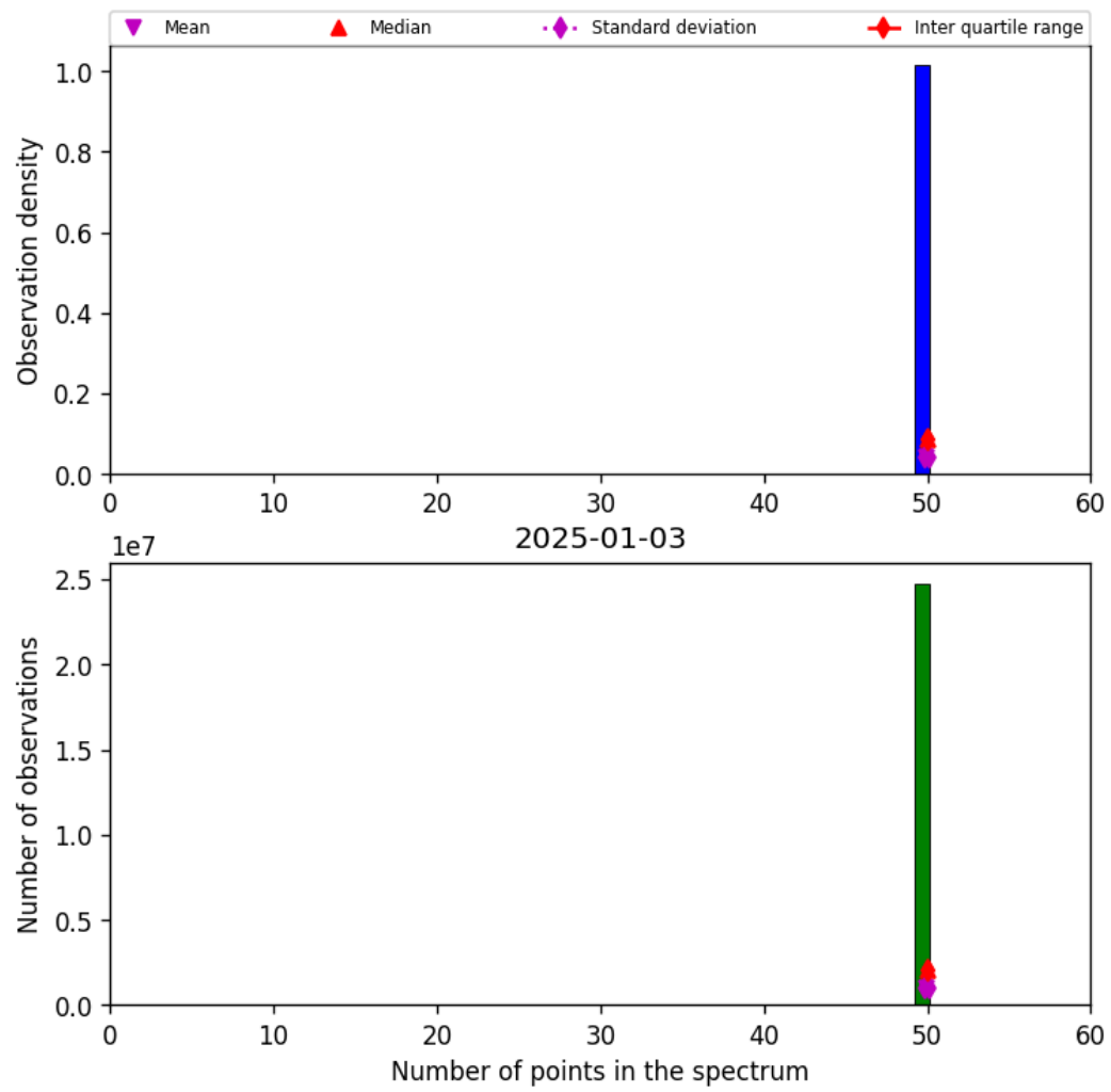
Figure 44: Histogram of “Number of points in the spectrum” for 2025-01-02 to 2025-01-04
