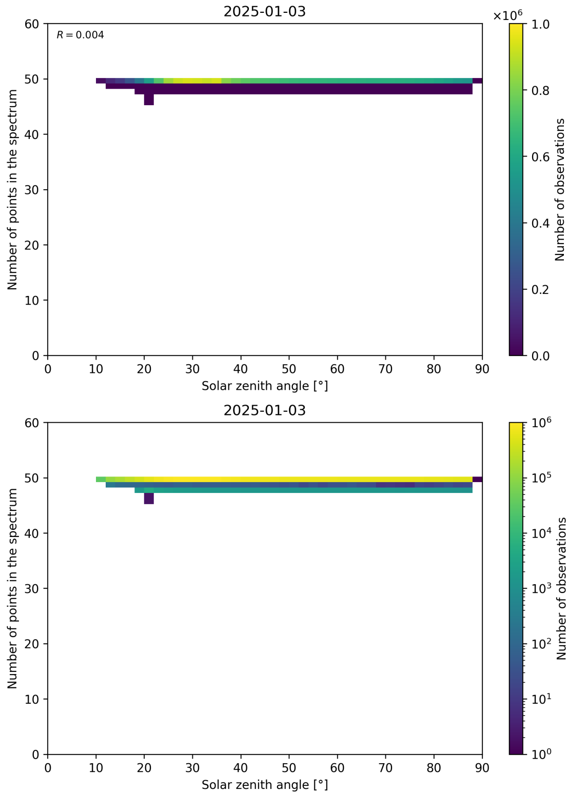
Figure 115: Scatter density plot of “Solar zenith angle” against “Number of points in the spectrum” for 2025-01-02 to 2025-01-04.
