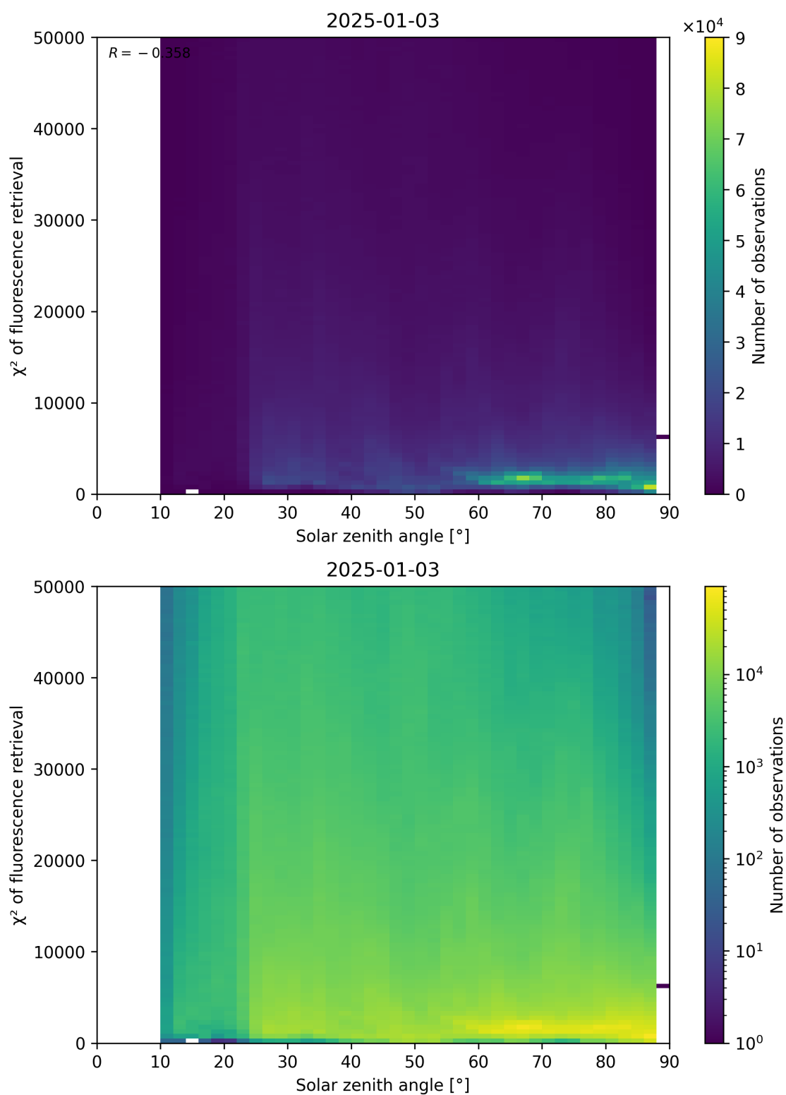
Figure 109: Scatter density plot of “Solar zenith angle” against “ \chi^2 of fluorescence retrieval” for 2025-01-02 to 2025-01-04.
