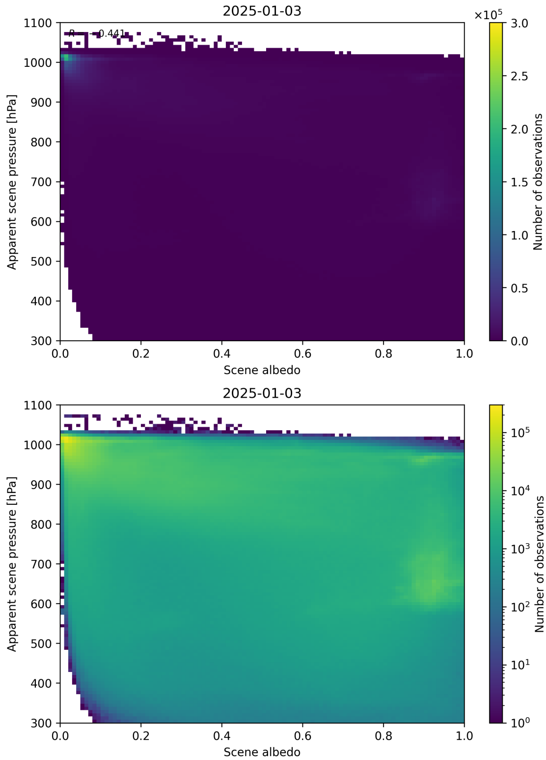
Figure 102: Scatter density plot of “Scene albedo” against “Apparent scene pressure” for 2025-01-02 to 2025-01-04.
