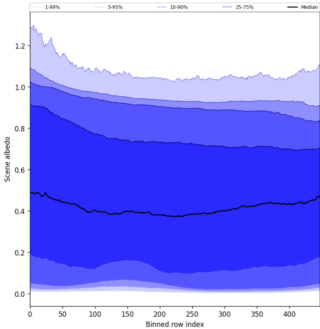
Figure 51: Along track statistics of “Scene albedo” for 2025-01-02 to 2025-01-04
