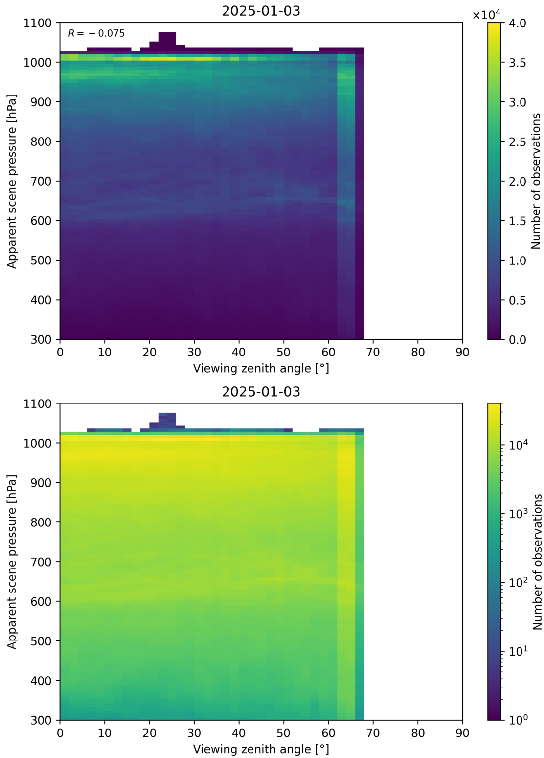
Figure 118: Scatter density plot of “Viewing zenith angle” against “Apparent scene pressure” for 2025-01-02 to 2025-01-04.
