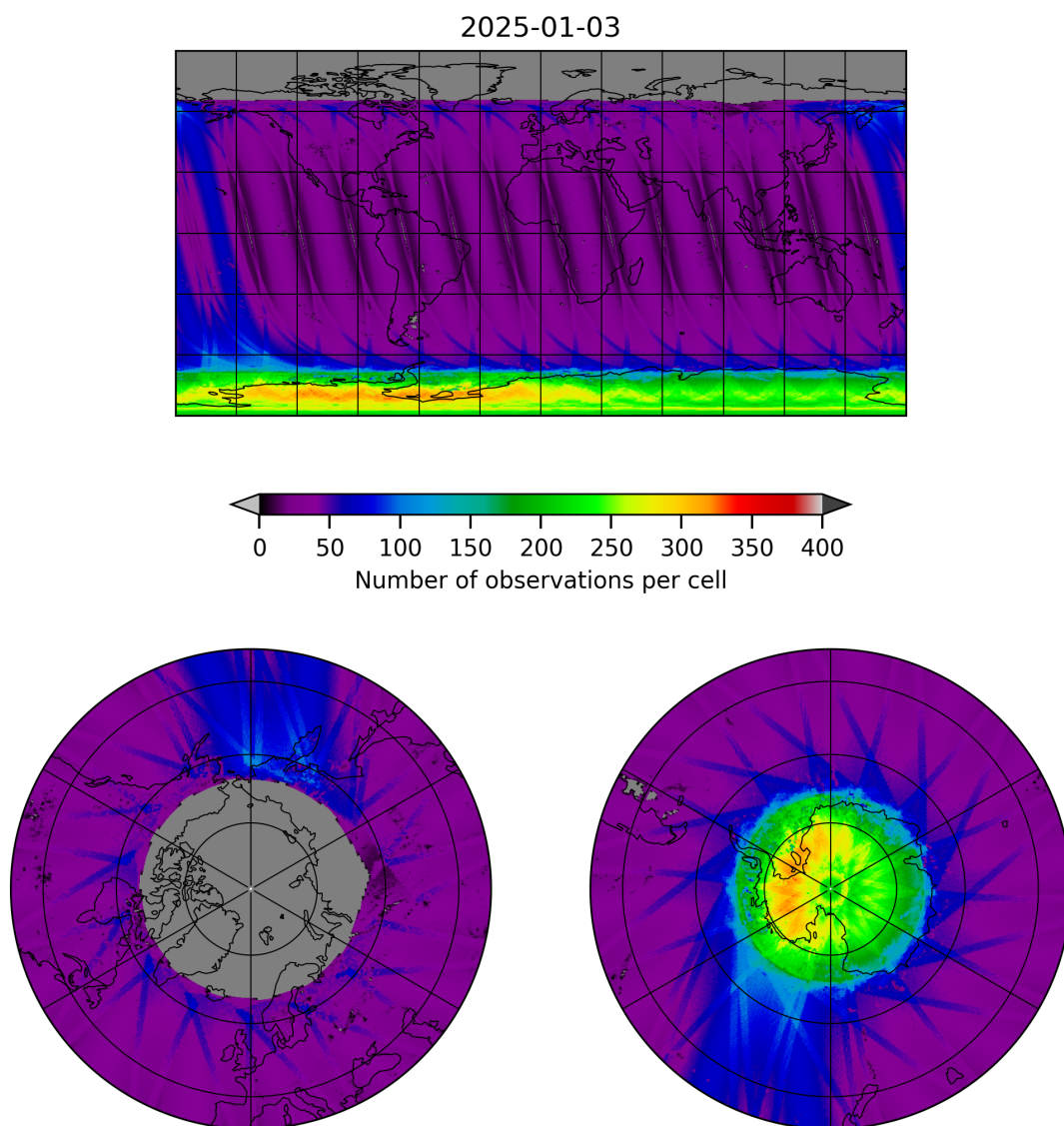
Figure 11: Map of the number of observations for 2025-01-02 to 2025-01-04
