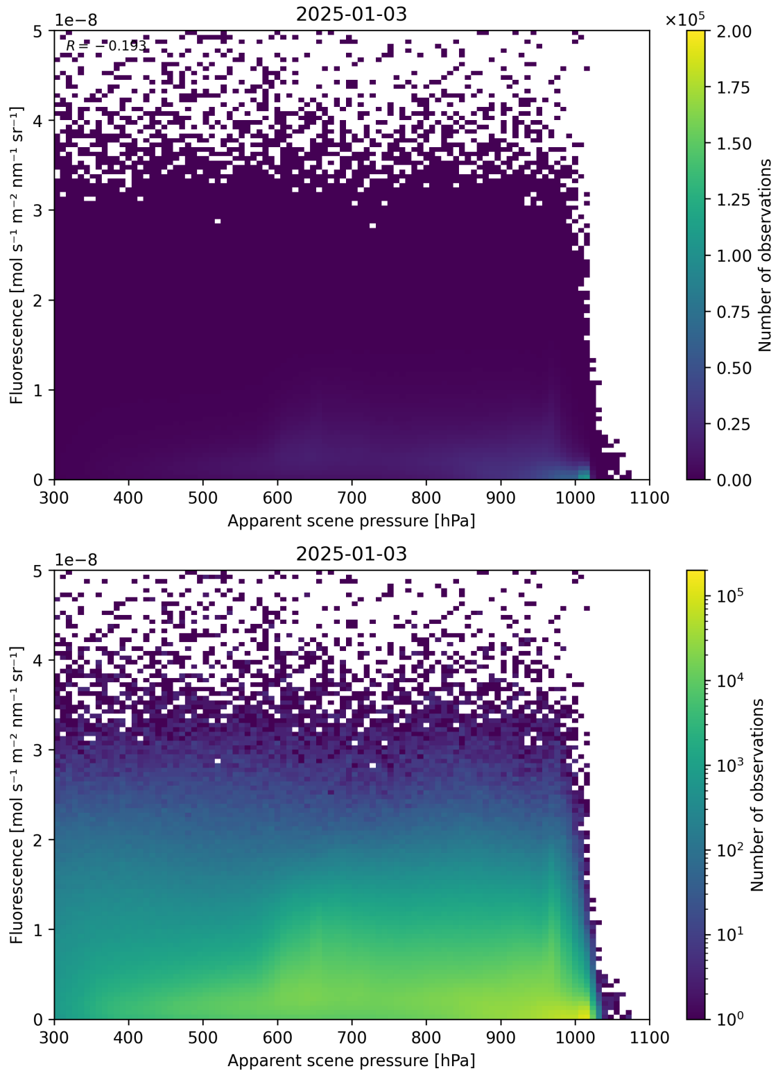
Figure 64: Scatter density plot of “Apparent scene pressure” against “Fluorescence” for 2025-01-02 to 2025-01-04.
