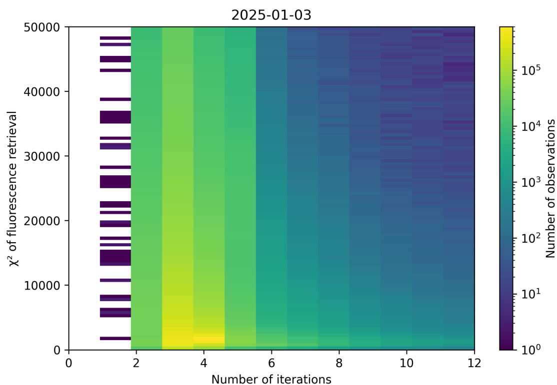
Figure 97: Scatter density plot of “Number of iterations” against “ \chi^2 of fluorescence retrieval” for 2025-01-02 to 2025-01-04.
