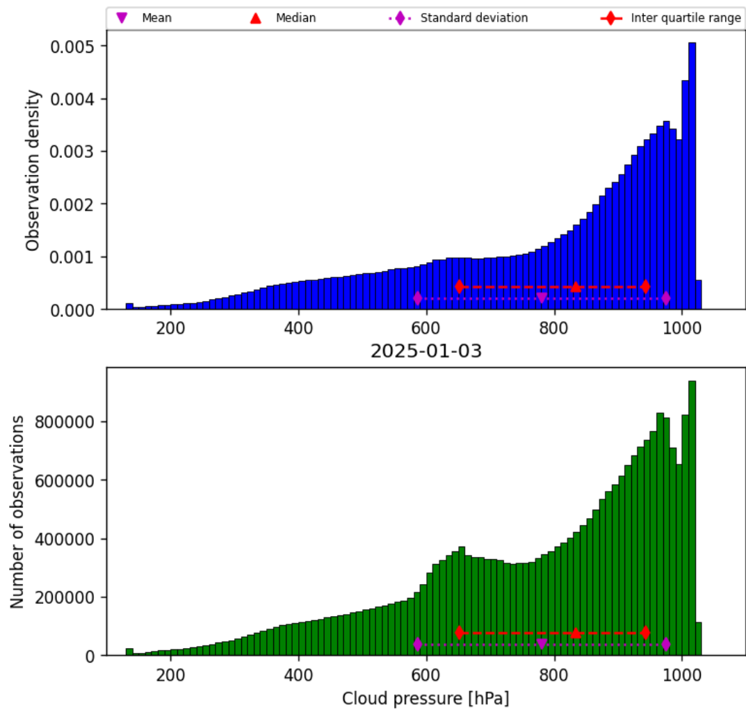
Figure 30: Histogram of “Cloud pressure” for 2025-01-02 to 2025-01-04
