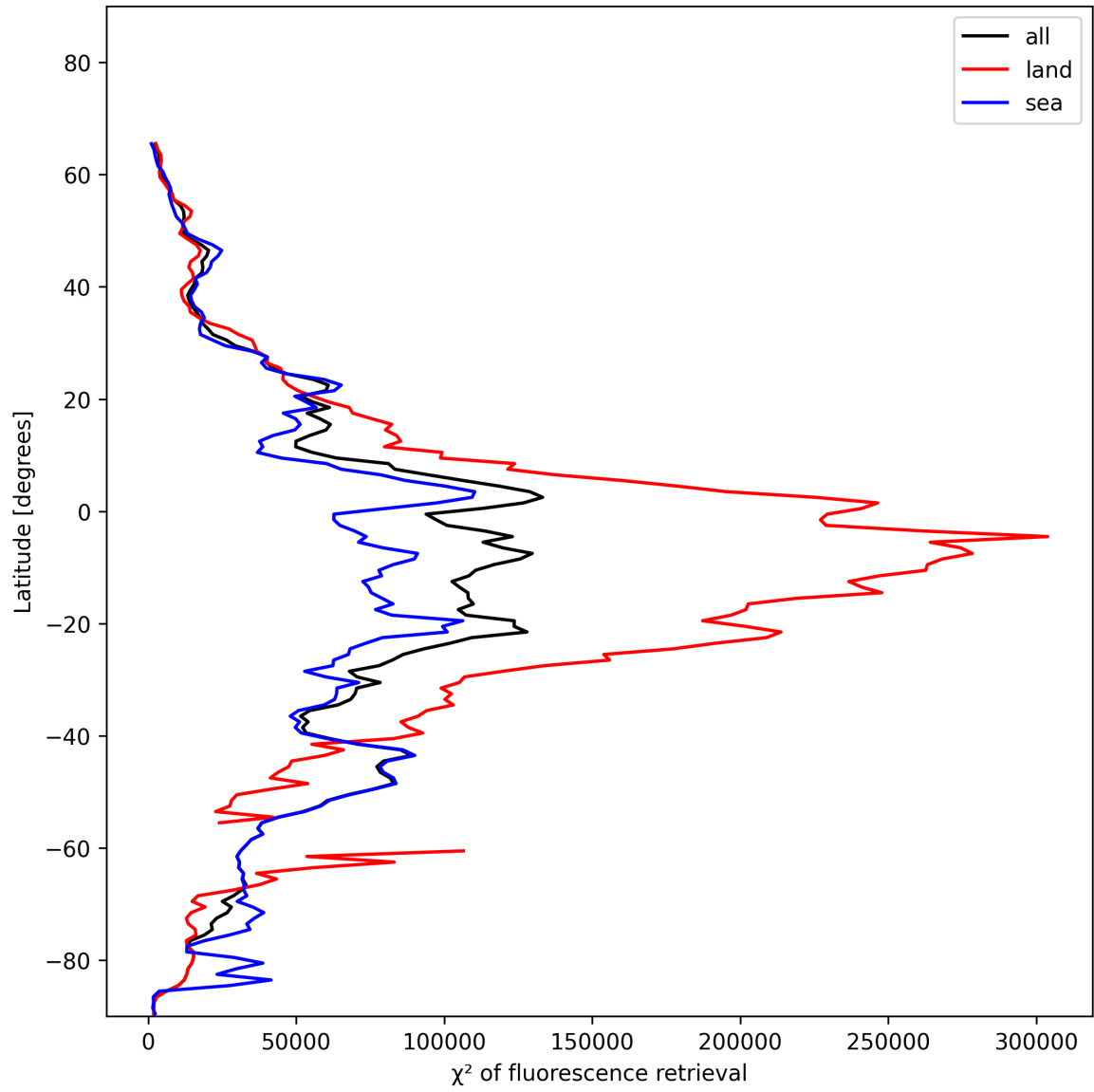
Figure 25: Zonal average of “ \chi^2 of fluorescence retrieval” for 2025-01-02 to 2025-01-04.
