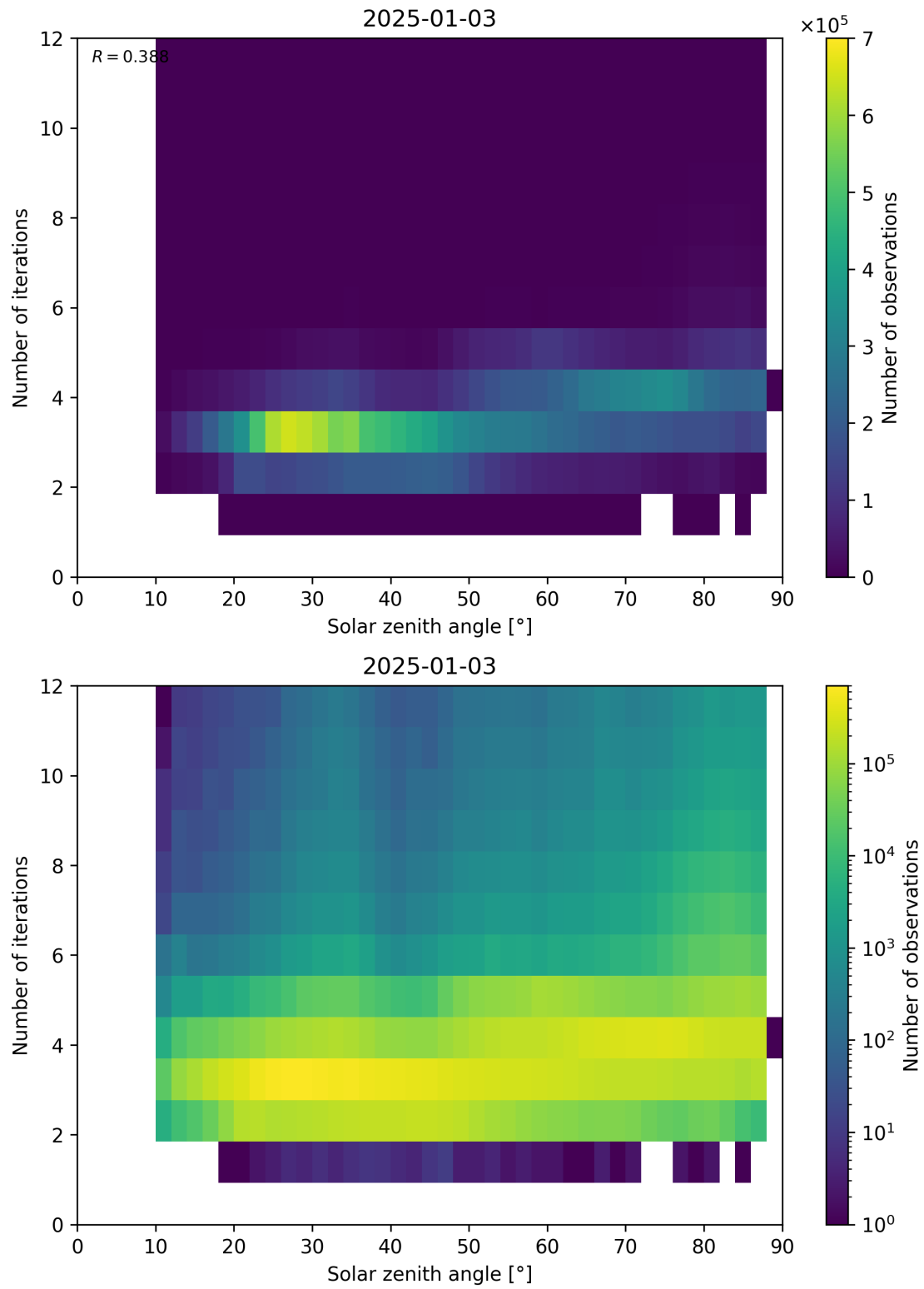
Figure 114: Scatter density plot of “Solar zenith angle” against “Number of iterations” for 2025-01-02 to 2025-01-04.
