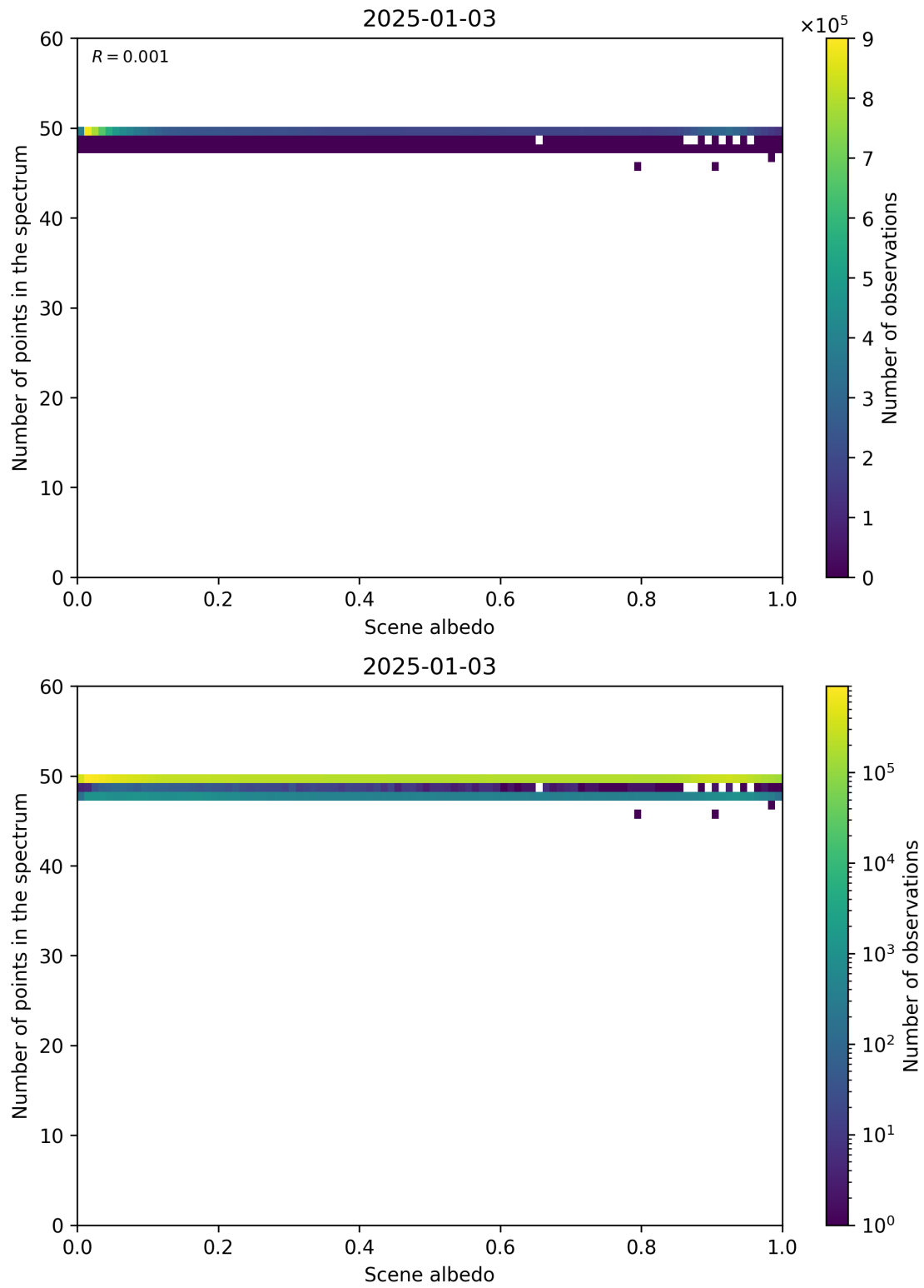
Figure 106: Scatter density plot of “Scene albedo” against “Number of points in the spectrum” for 2025-01-02 to 2025-01-04.
