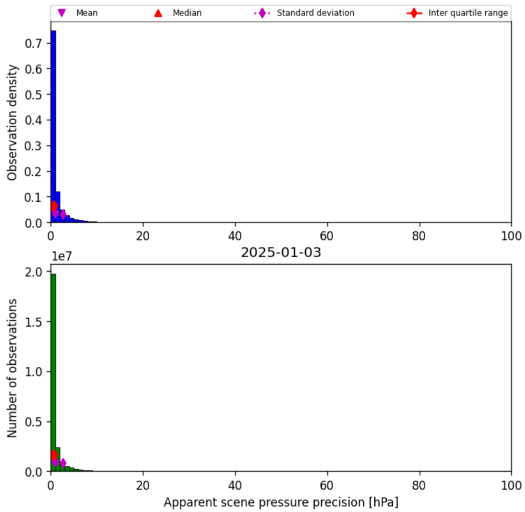
Figure 37: Histogram of “Apparent scene pressure precision” for 2025-01-02 to 2025-01-04
