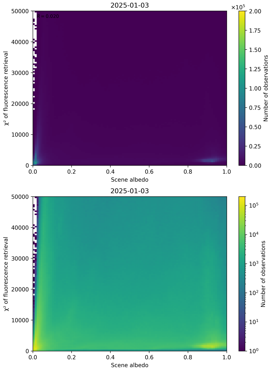
Figure 103: Scatter density plot of “Scene albedo” against “ \chi^2 of fluorescence retrieval” for 2025-01-02 to 2025-01-04.
