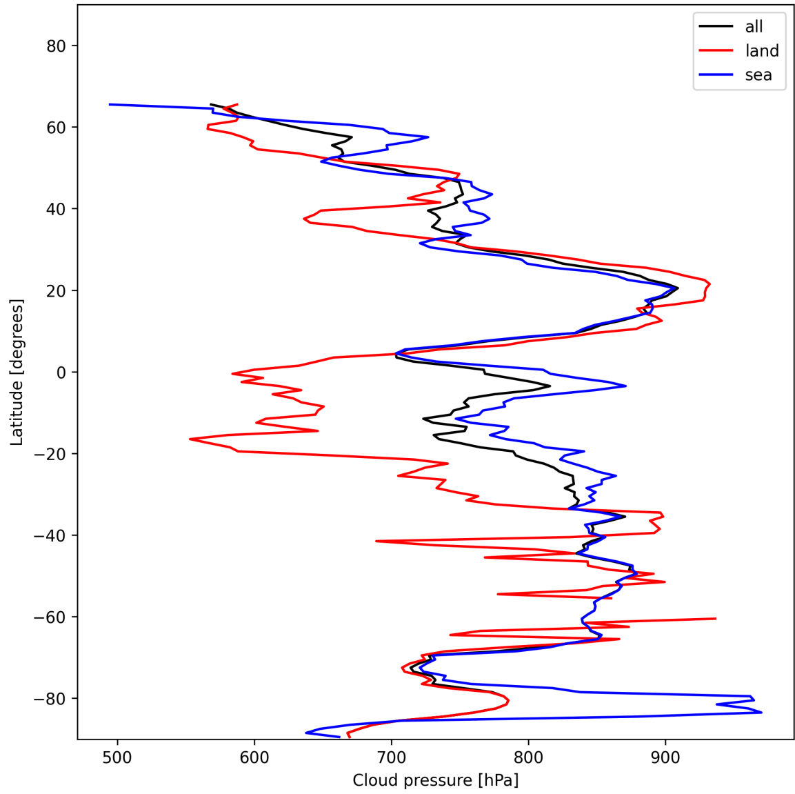
Figure 13: Zonal average of “Cloud pressure” for 2025-01-02 to 2025-01-04.
