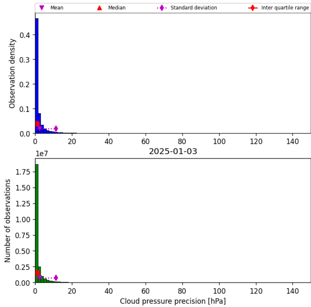
Figure 31: Histogram of “Cloud pressure precision” for 2025-01-02 to 2025-01-04
