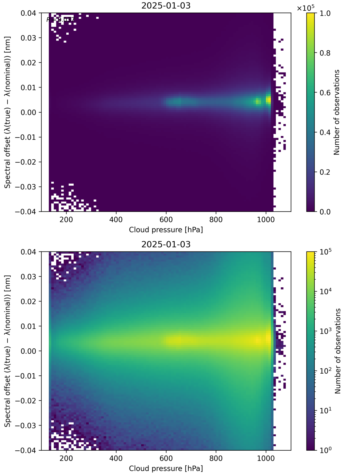
Figure 84: Scatter density plot of “Cloud pressure” against “Spectral offset ( \lambda_{\text{true}} - \lambda_{\text{nominal}} )” for 2025-01-02 to 2025-01-04.
