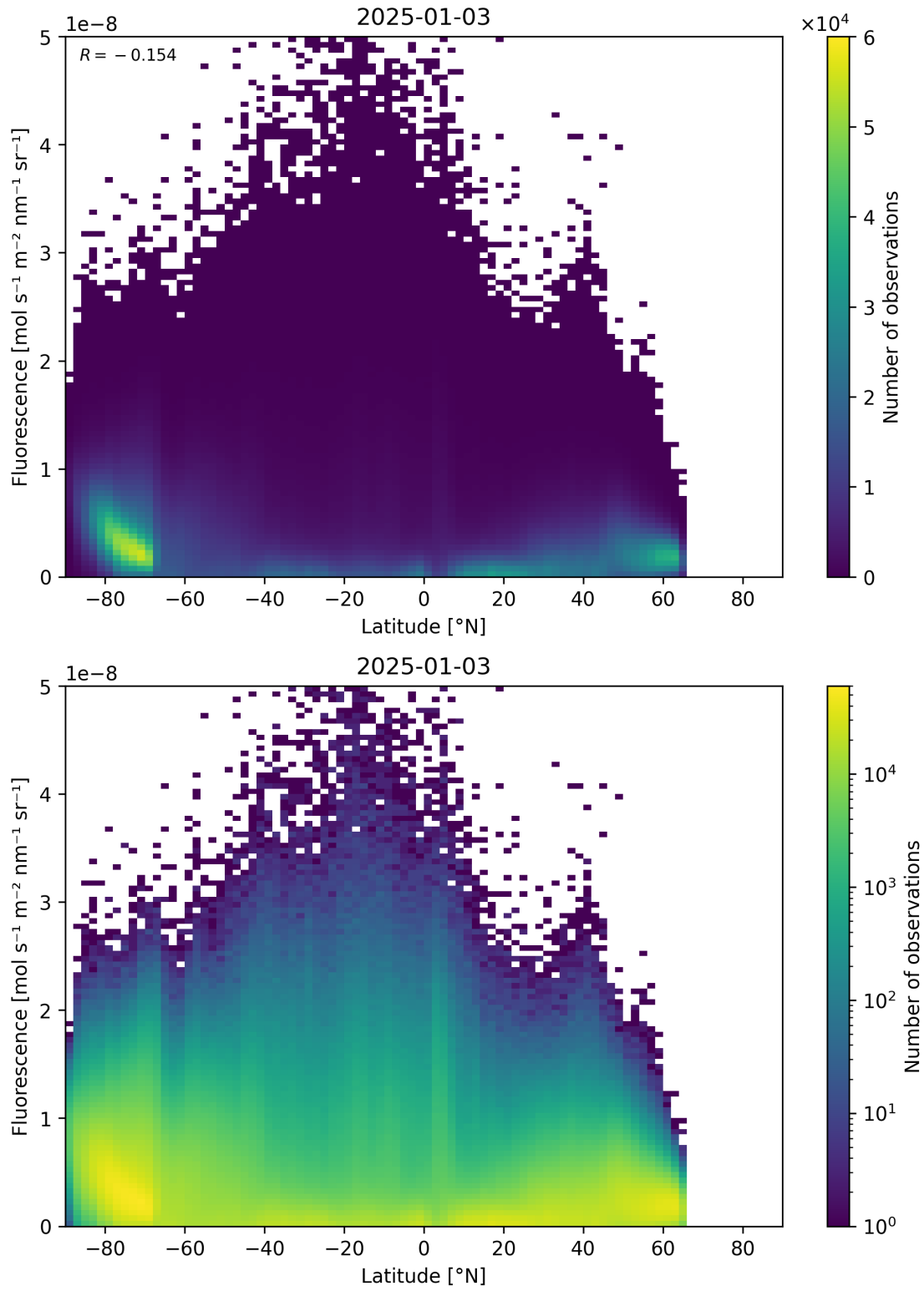
Figure 92: Scatter density plot of “Latitude” against “Fluorescence” for 2025-01-02 to 2025-01-04.
