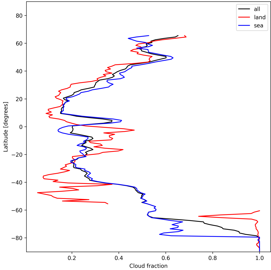
Figure 15: Zonal average of “Cloud fraction” for 2025-01-02 to 2025-01-04.
