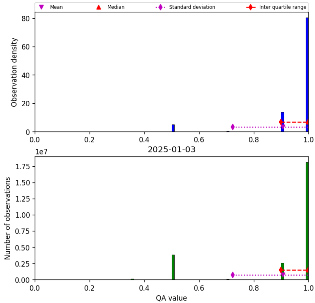
Figure 29: Histogram of “QA value” for 2025-01-02 to 2025-01-04
