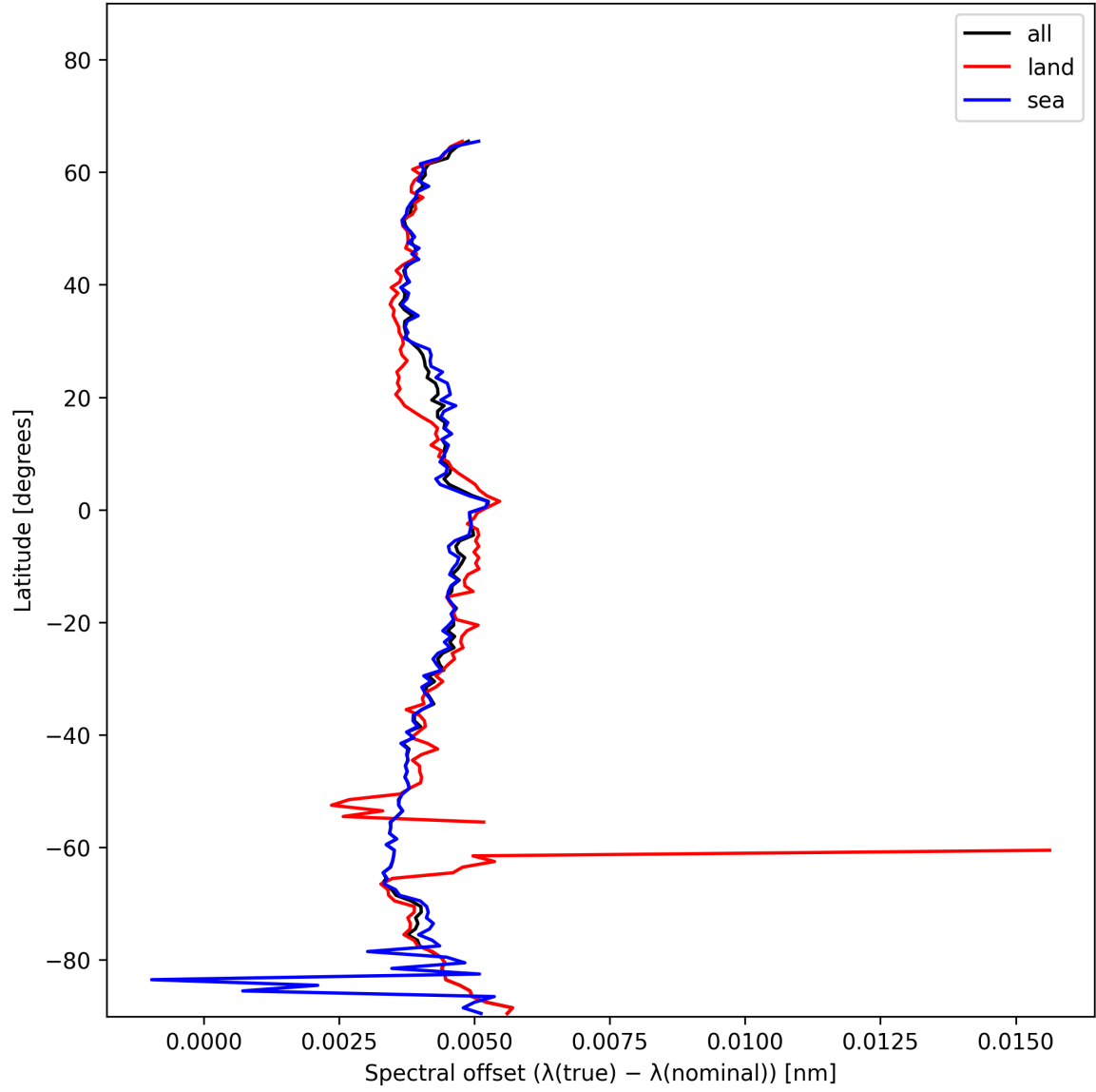
Figure 28: Zonal average of “Spectral offset ( \lambda_{\text{true}} - \lambda_{\text{nominal}} )” for 2025-01-02 to 2025-01-04.
