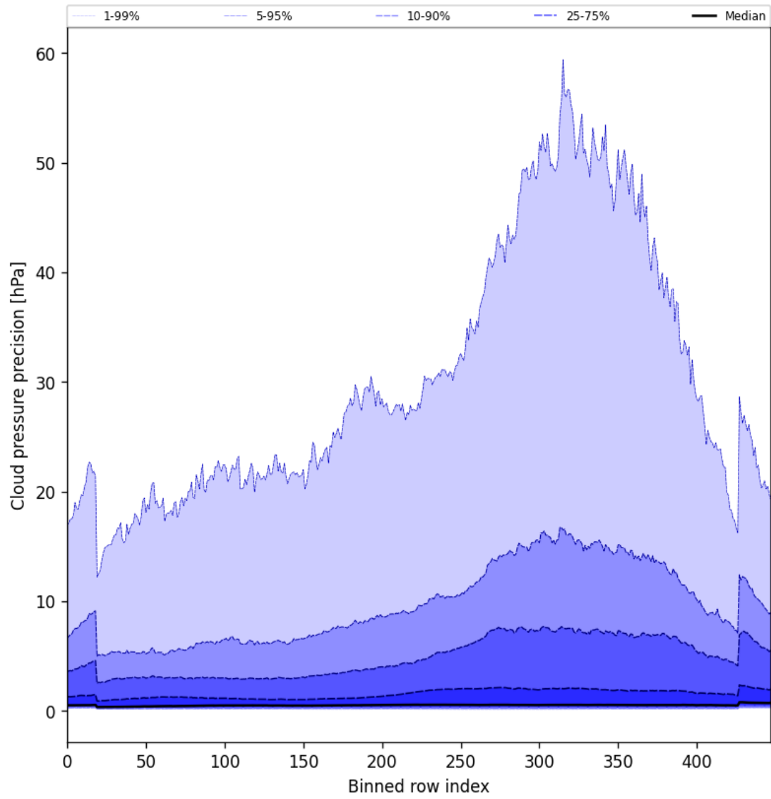
Figure 48: Along track statistics of “Cloud pressure precision” for 2025-01-02 to 2025-01-04
