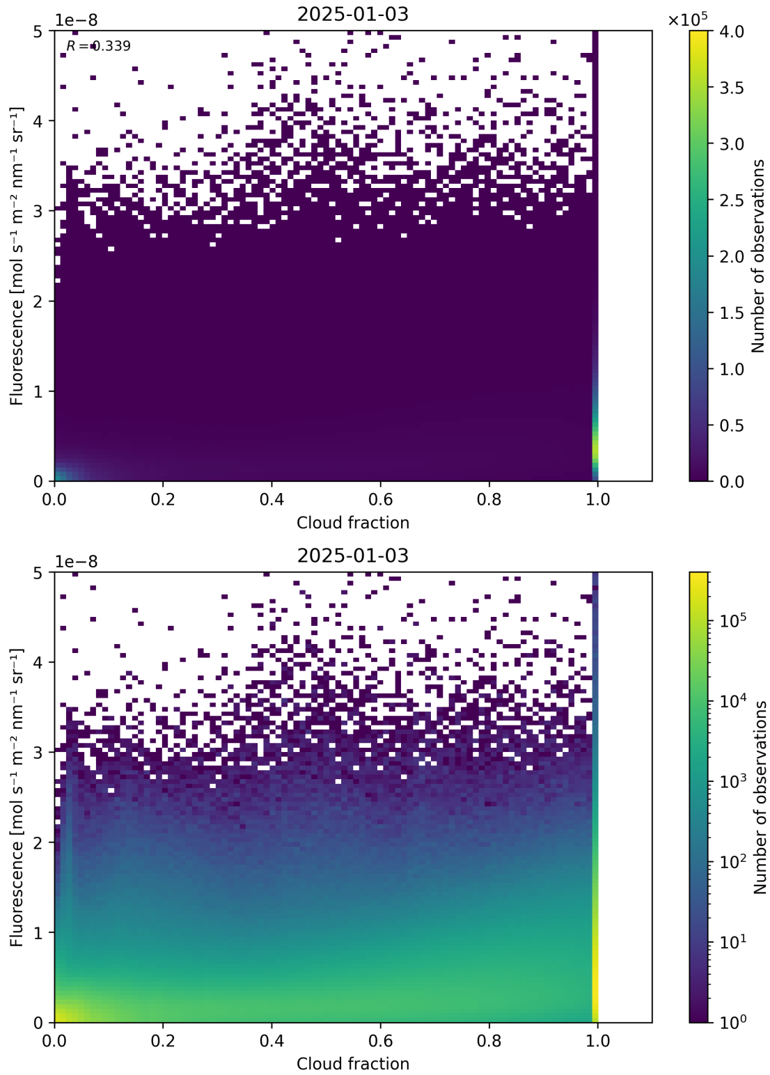
Figure 72: Scatter density plot of “Cloud fraction” against “Fluorescence” for 2025-01-02 to 2025-01-04.
