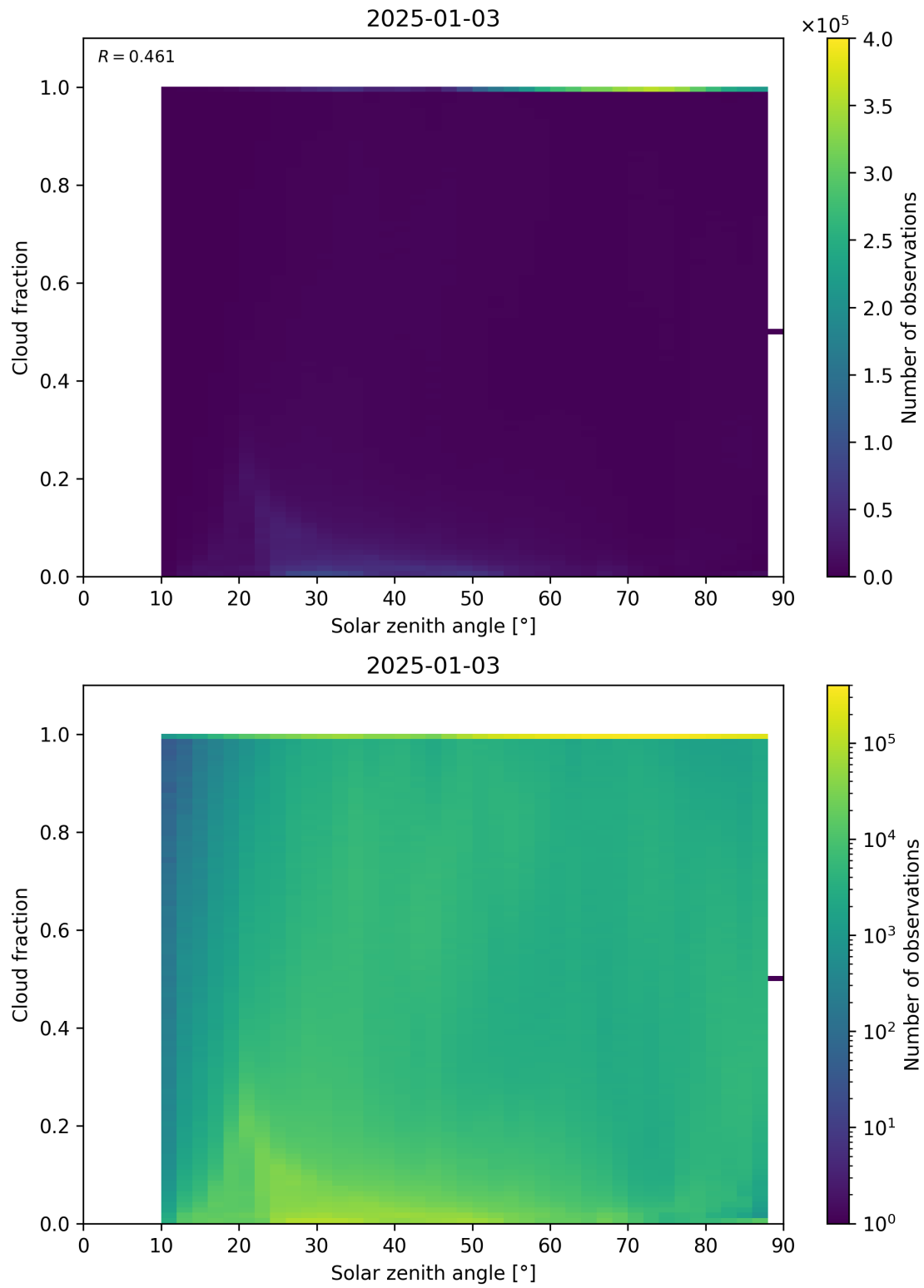
Figure 110: Scatter density plot of “Solar zenith angle” against “Cloud fraction” for 2025-01-02 to 2025-01-04.
