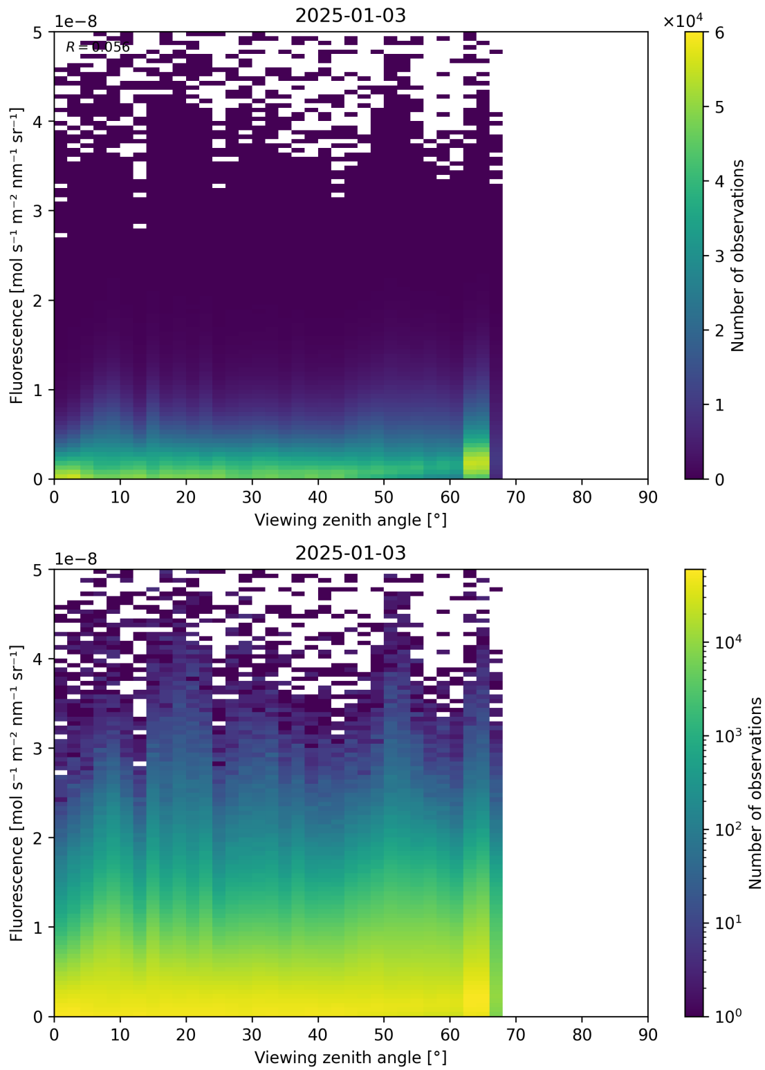
Figure 122: Scatter density plot of “Viewing zenith angle” against “Fluorescence” for 2025-01-02 to 2025-01-04.
