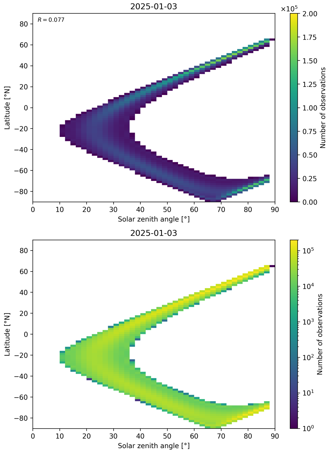
Figure 113: Scatter density plot of “Solar zenith angle” against “Latitude” for 2025-01-02 to 2025-01-04.
