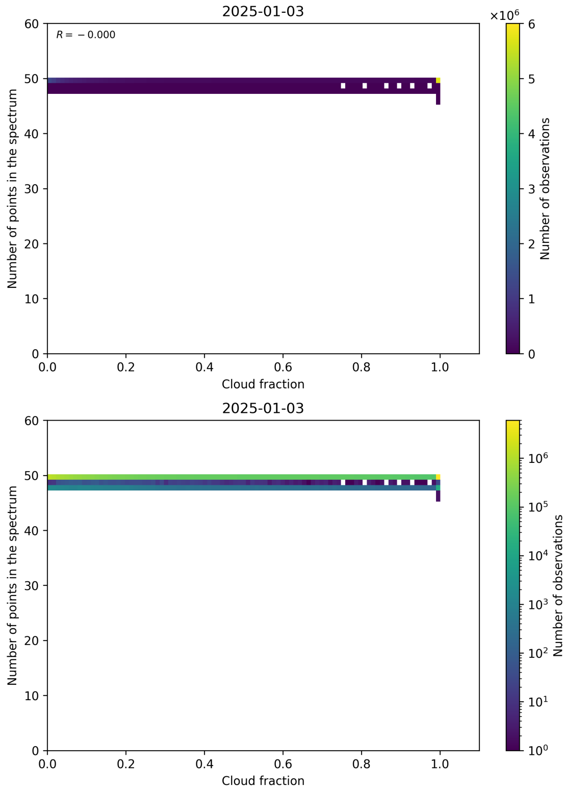
Figure 74: Scatter density plot of “Cloud fraction” against “Number of points in the spectrum” for 2025-01-02 to 2025-01-04.
