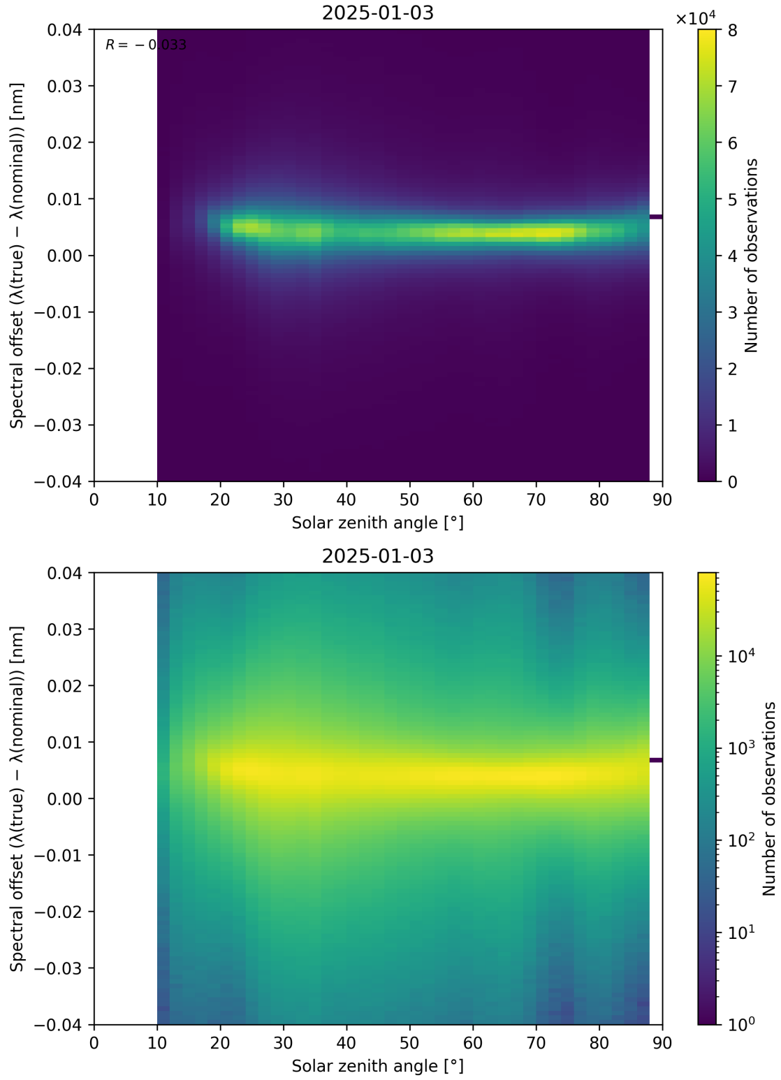
Figure 117: Scatter density plot of “Solar zenith angle” against “Spectral offset ( \lambda_{\text{true}} - \lambda_{\text{nominal}} )” for 2025-01-02 to 2025-01-04.
