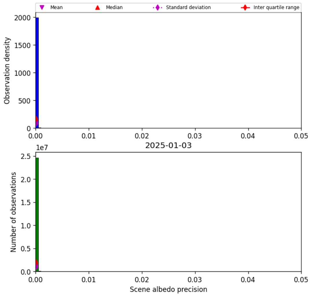
Figure 35: Histogram of “Scene albedo precision” for 2025-01-02 to 2025-01-04
