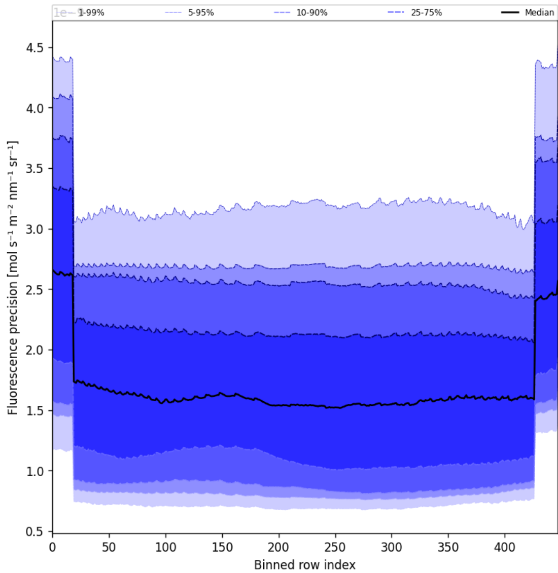
Figure 58: Along track statistics of “Fluorescence precision” for 2025-01-02 to 2025-01-04
