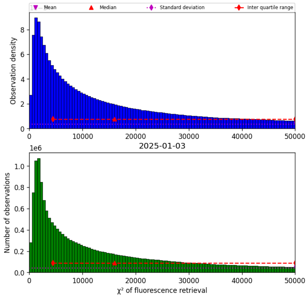
Figure 42: Histogram of “ \chi^2 of fluorescence retrieval” for 2025-01-02 to 2025-01-04
