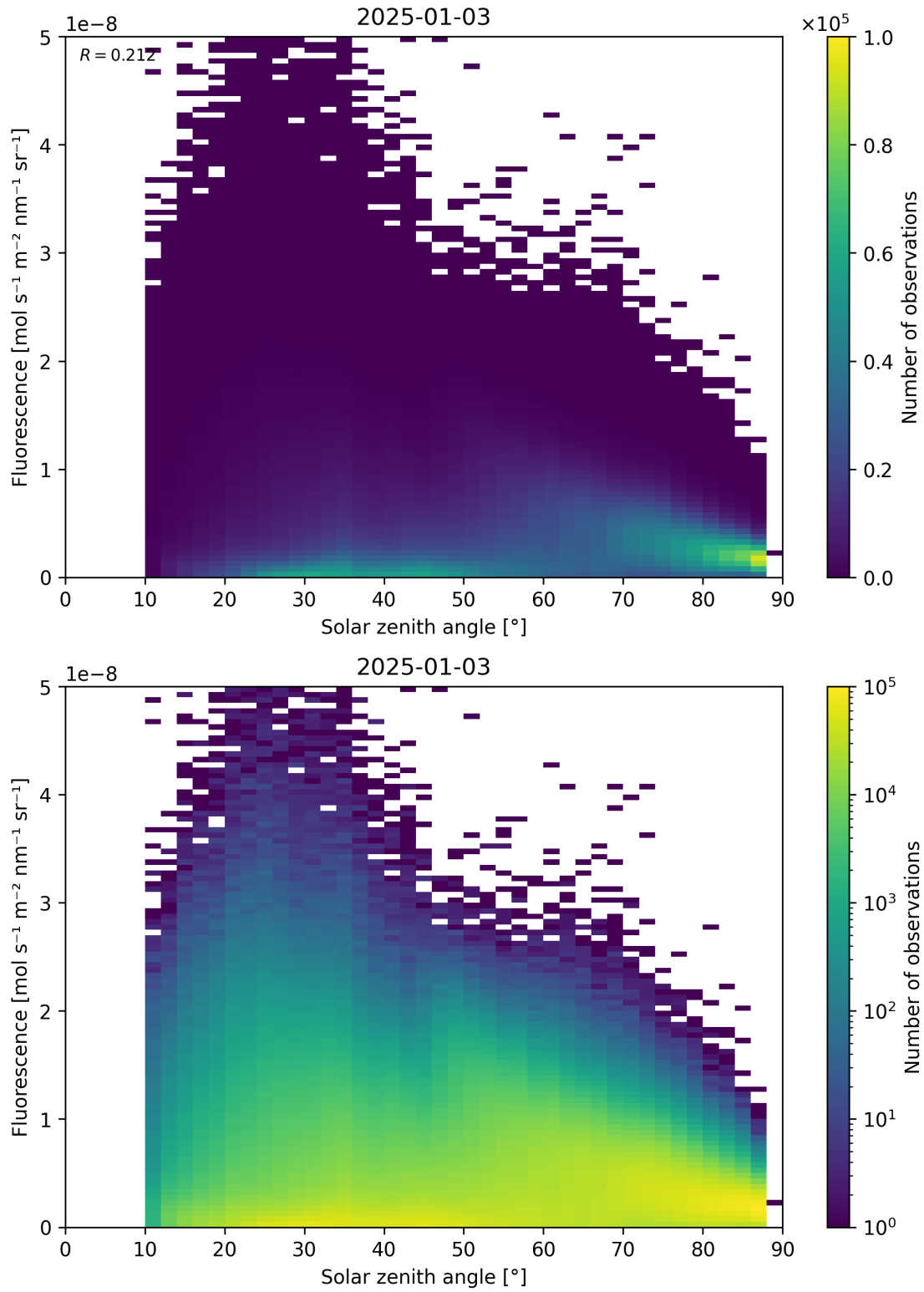
Figure 112: Scatter density plot of “Solar zenith angle” against “Fluorescence” for 2025-01-02 to 2025-01-04.
