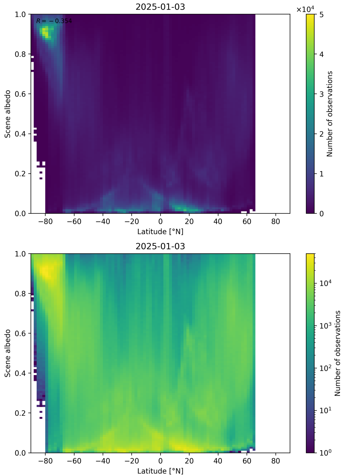
Figure 95: Scatter density plot of “Latitude” against “Scene albedo” for 2025-01-02 to 2025-01-04.
