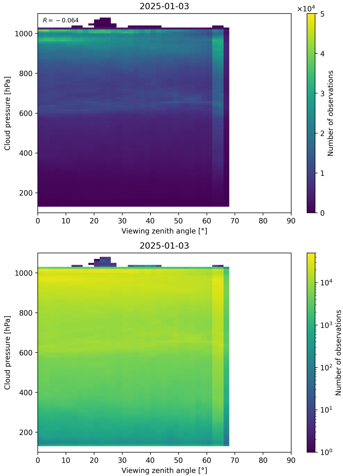
Figure 121: Scatter density plot of “Viewing zenith angle” against “Cloud pressure” for 2025-01-02 to 2025-01-04.
