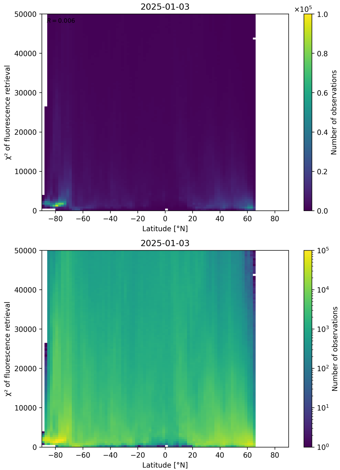
Figure 89: Scatter density plot of “Latitude” against “ \chi^2 of fluorescence retrieval” for 2025-01-02 to 2025-01-04.
