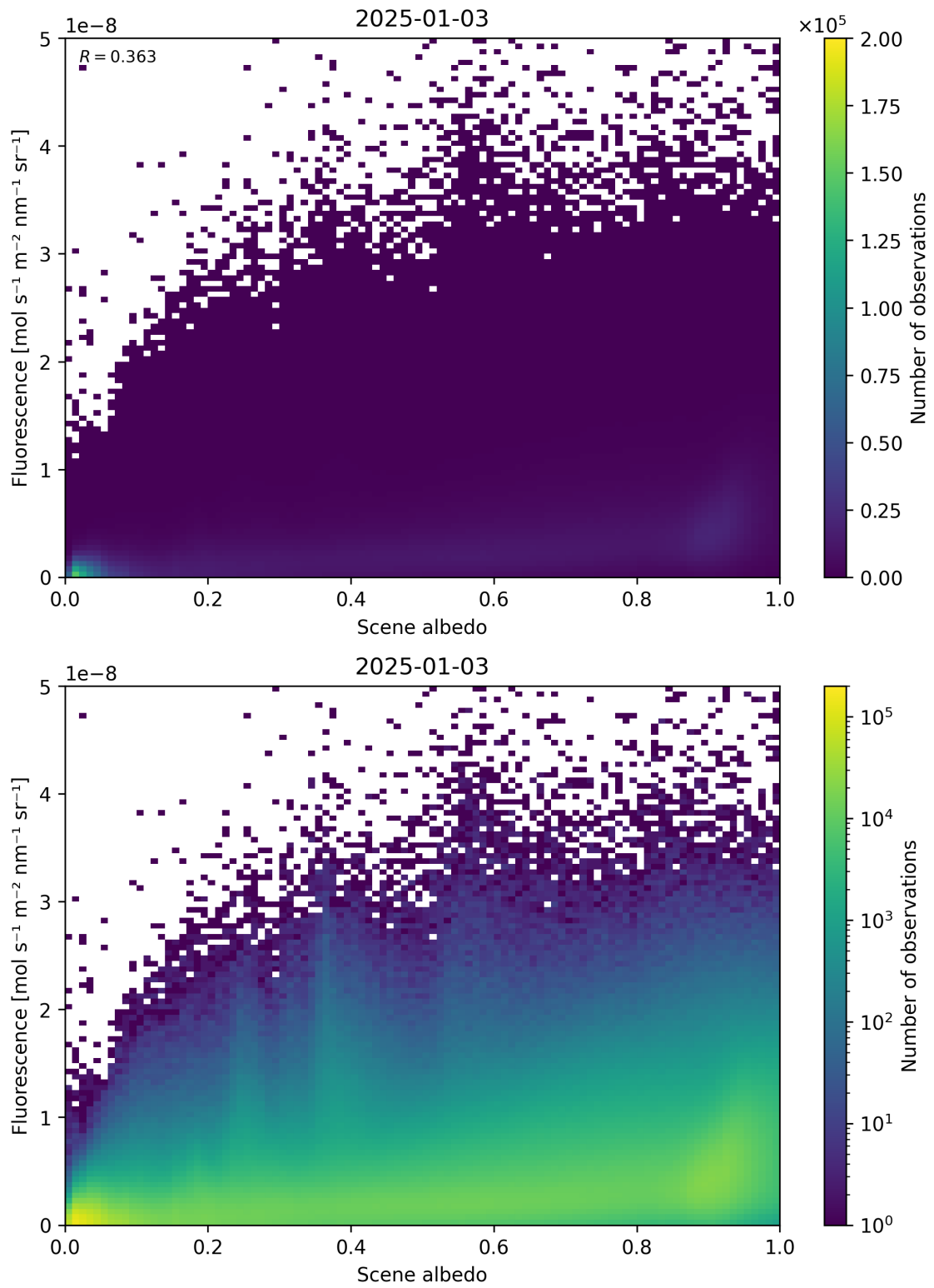
Figure 104: Scatter density plot of “Scene albedo” against “Fluorescence” for 2025-01-02 to 2025-01-04.
