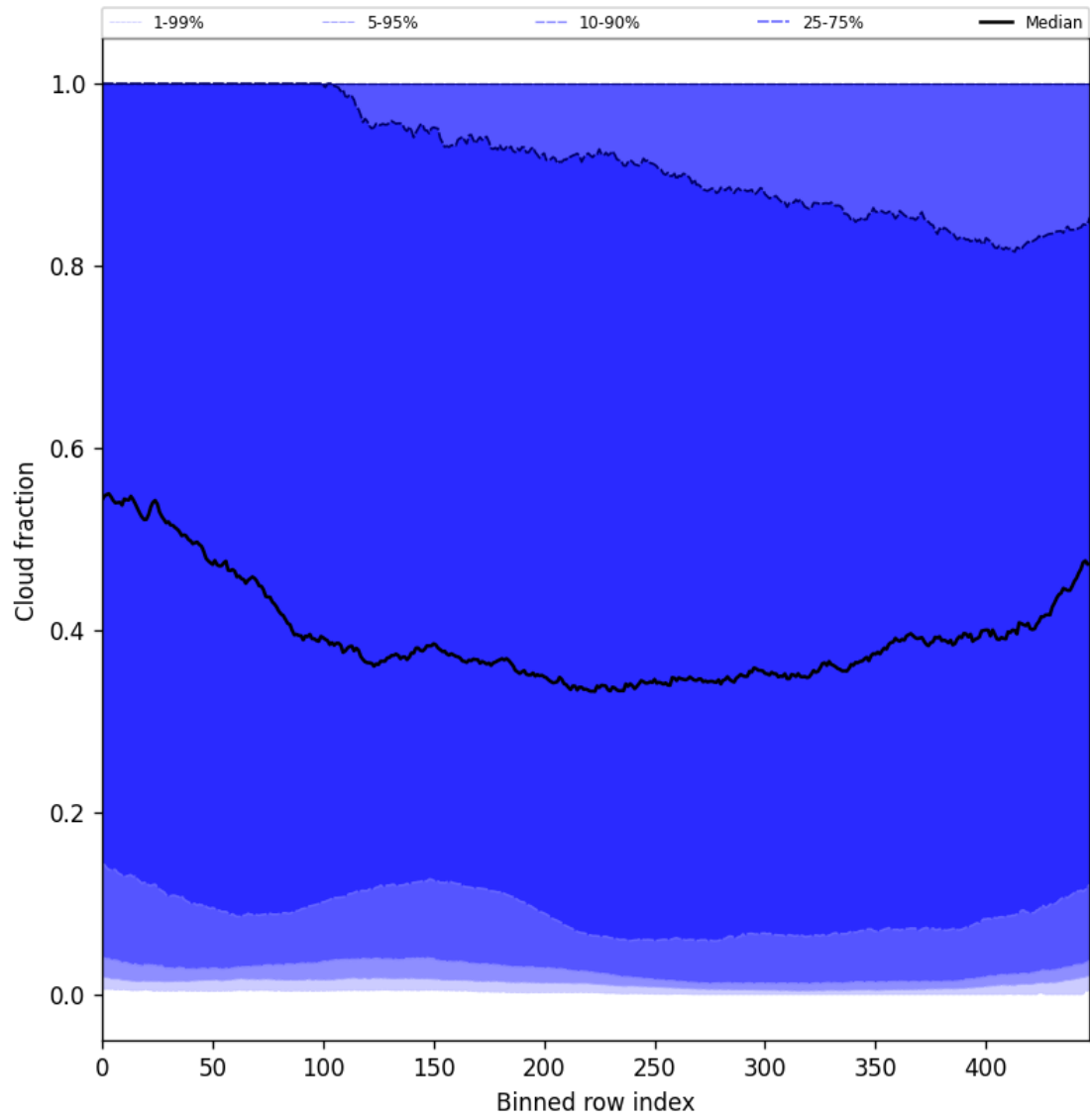
Figure 49: Along track statistics of “Cloud fraction” for 2025-01-02 to 2025-01-04
