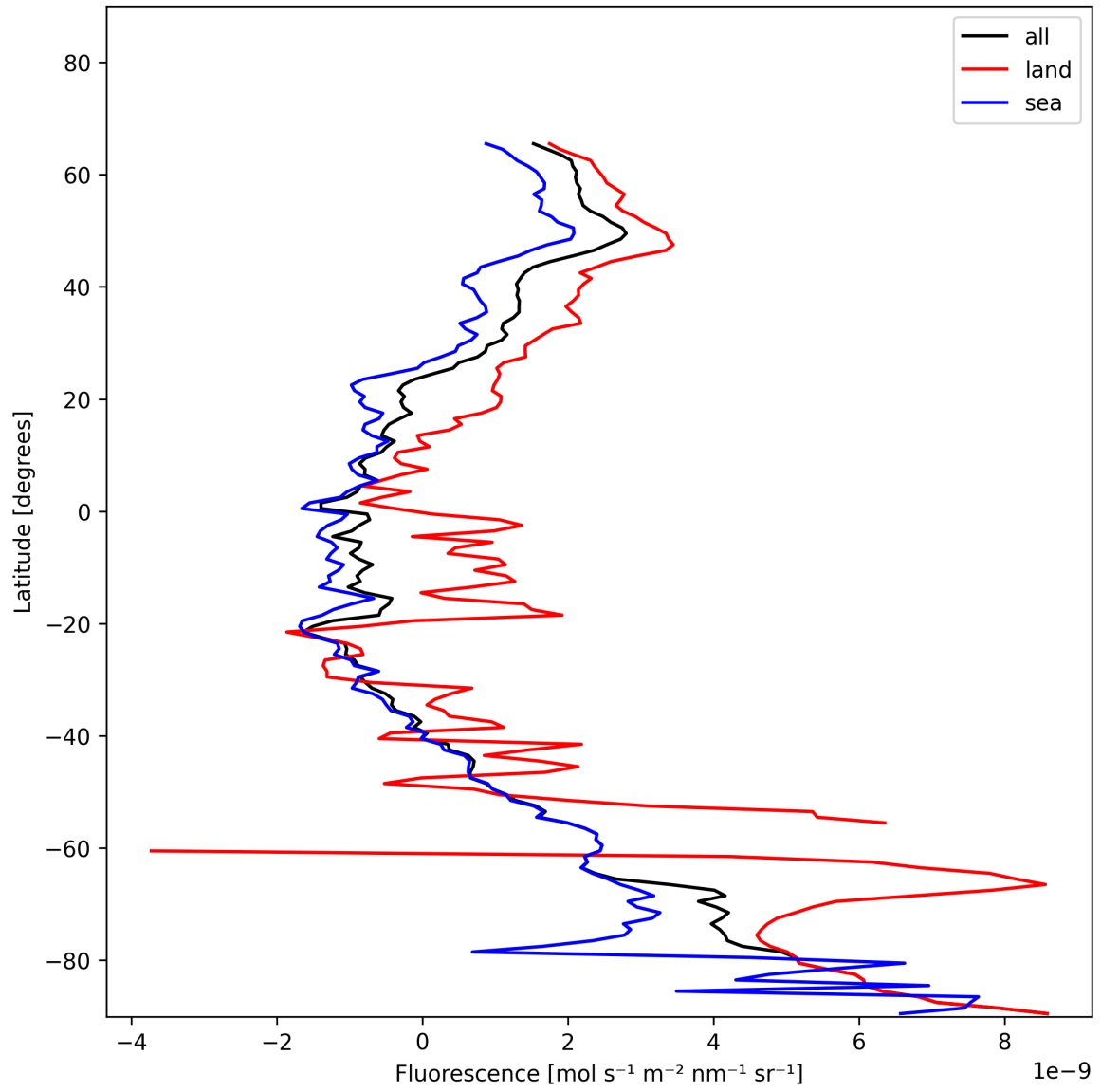
Figure 23: Zonal average of “Fluorescence” for 2025-01-02 to 2025-01-04.
