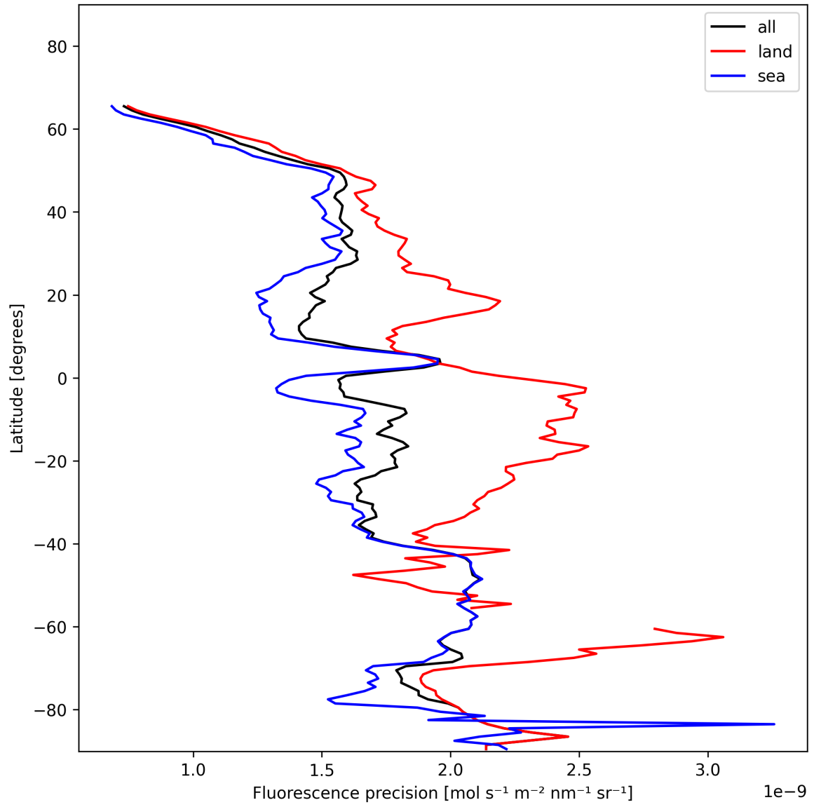
Figure 24: Zonal average of “Fluorescence precision” for 2025-01-02 to 2025-01-04.
