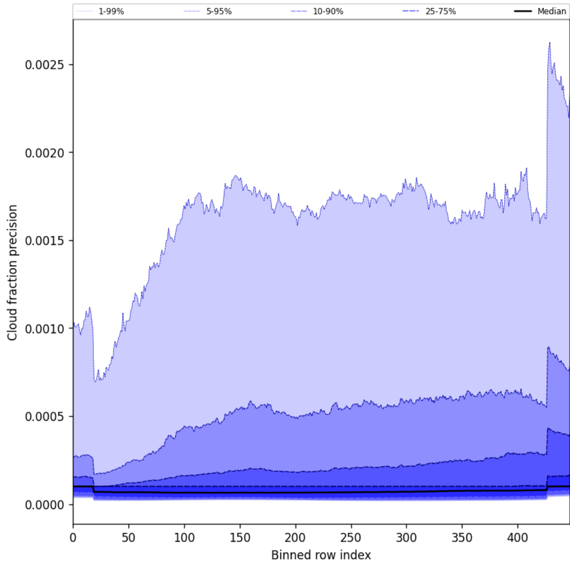
Figure 50: Along track statistics of “Cloud fraction precision” for 2025-01-02 to 2025-01-04
