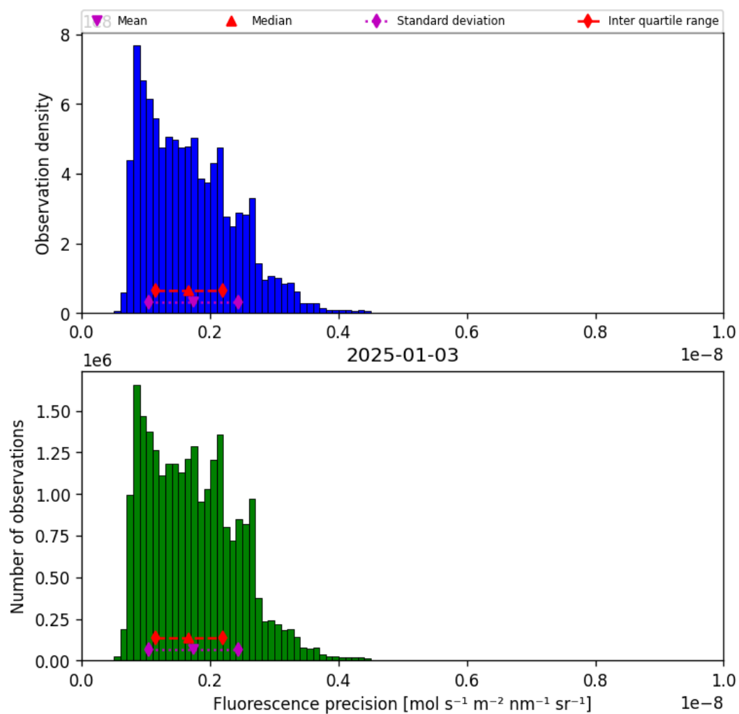
Figure 41: Histogram of “Fluorescence precision” for 2025-01-02 to 2025-01-04
