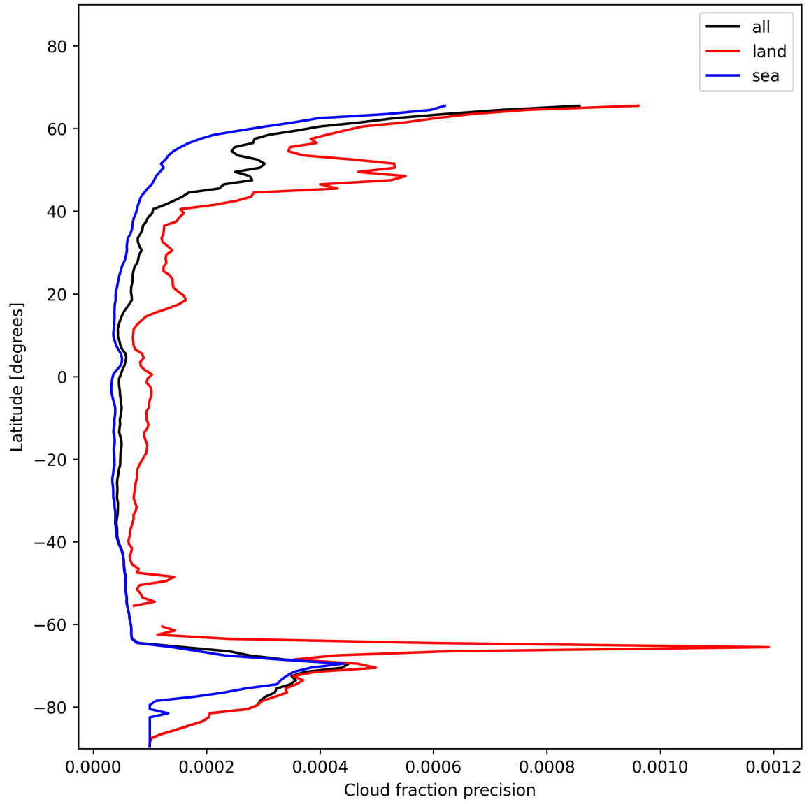
Figure 16: Zonal average of “Cloud fraction precision” for 2025-01-02 to 2025-01-04.
