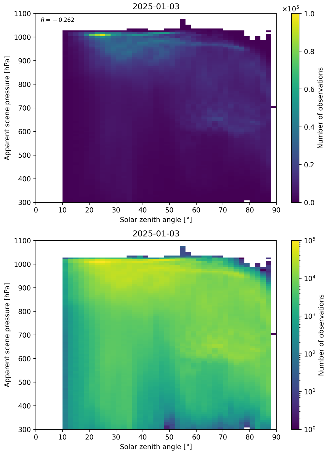
Figure 108: Scatter density plot of “Solar zenith angle” against “Apparent scene pressure” for 2025-01-02 to 2025-01-04.
