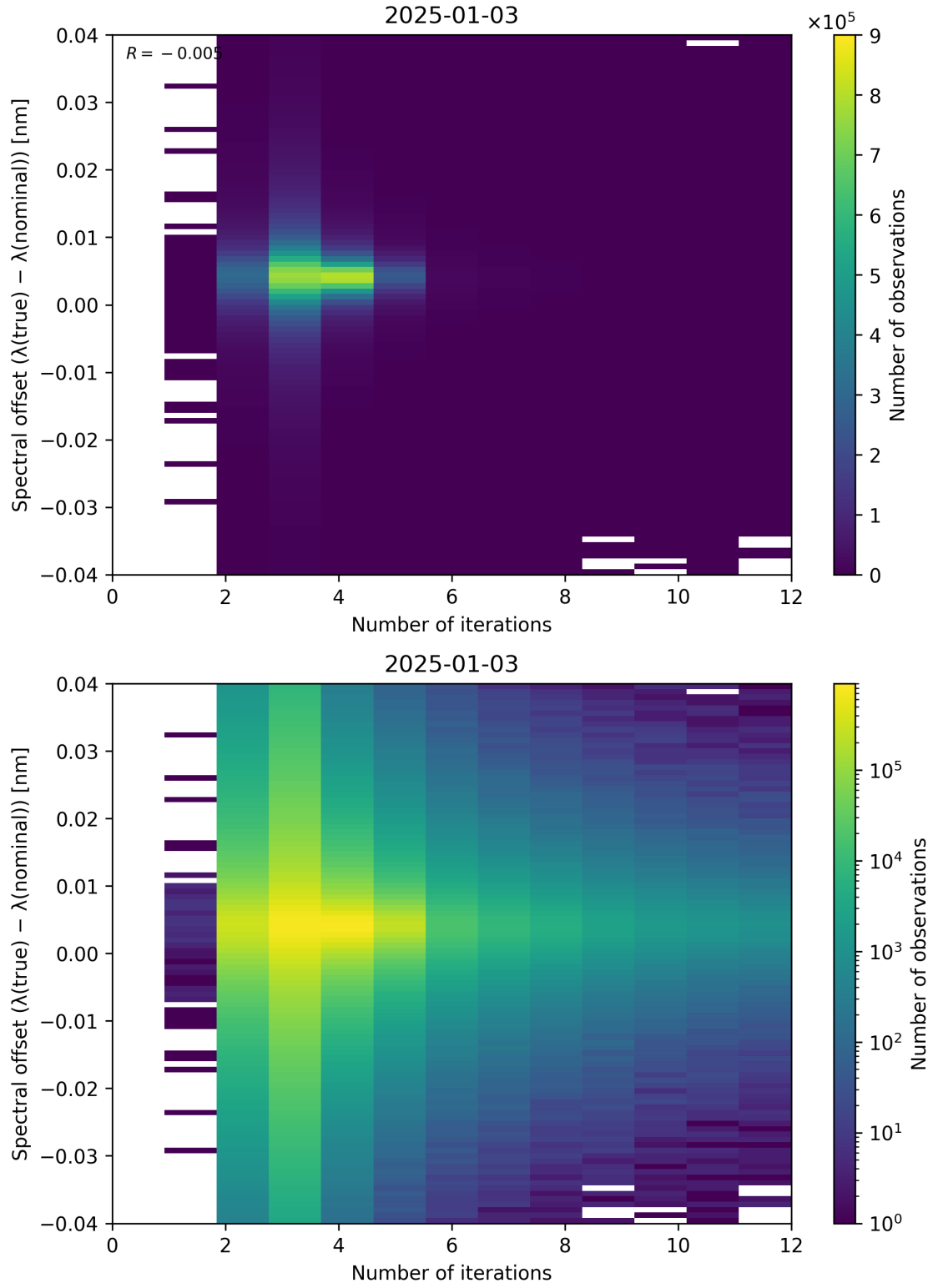
Figure 100: Scatter density plot of “Number of iterations” against “Spectral offset ( \lambda_{\text{true}} - \lambda_{\text{nominal}} )” for 2025-01-02 to 2025-01-04.
