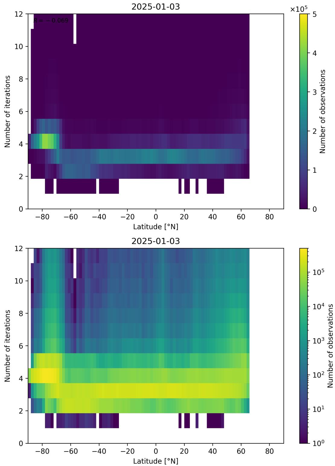
Figure 93: Scatter density plot of “Latitude” against “Number of iterations” for 2025-01-02 to 2025-01-04.
