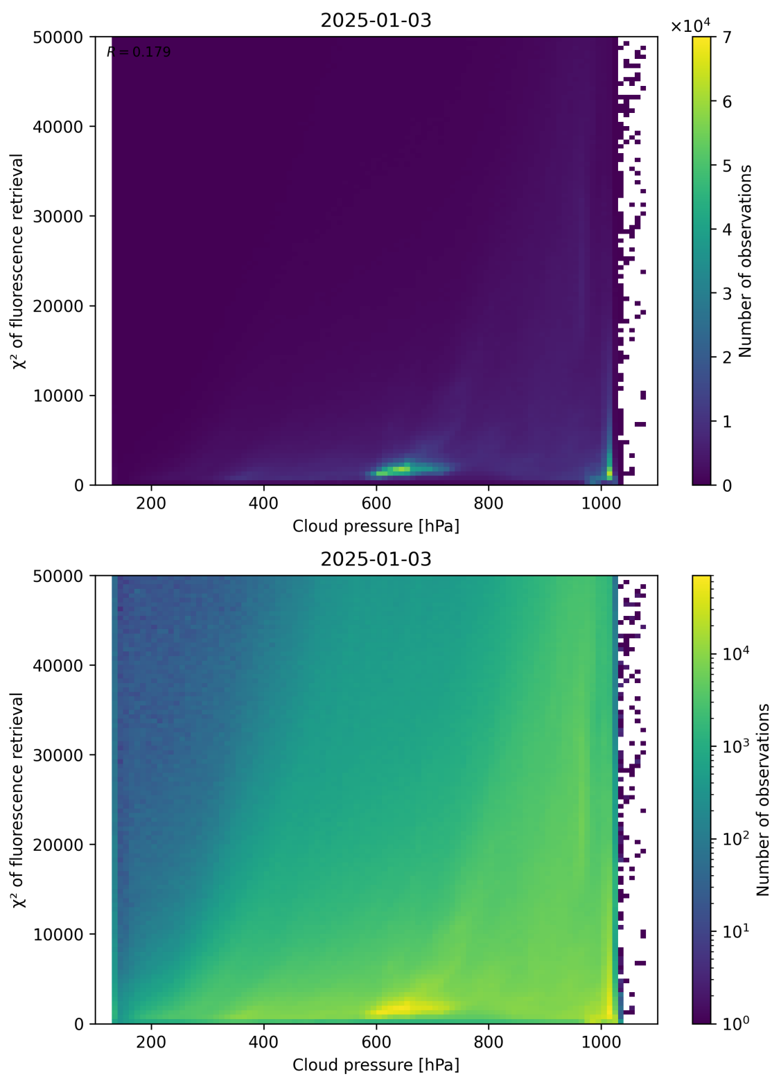
Figure 78: Scatter density plot of “Cloud pressure” against “ \chi^2 of fluorescence retrieval” for 2025-01-02 to 2025-01-04.
