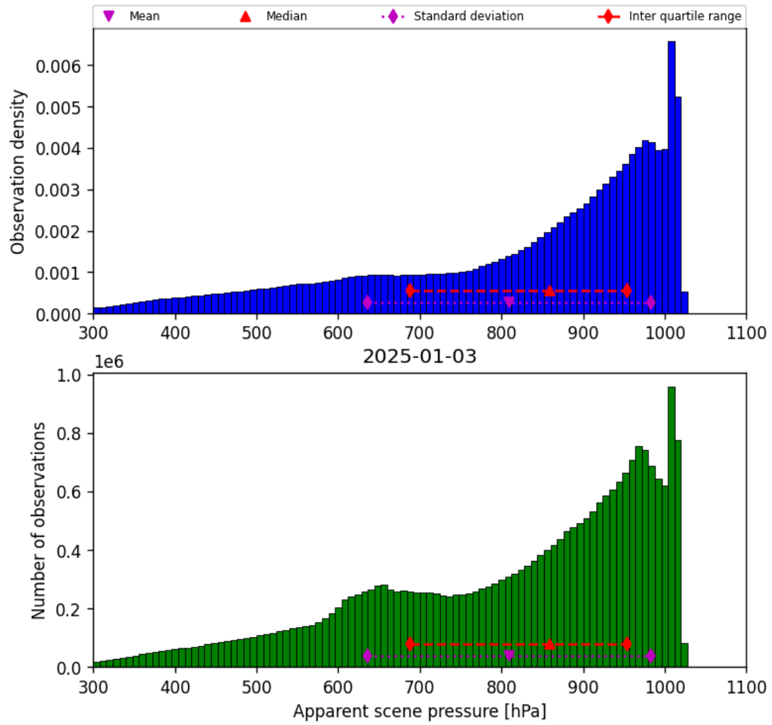
Figure 36: Histogram of “Apparent scene pressure” for 2025-01-02 to 2025-01-04
