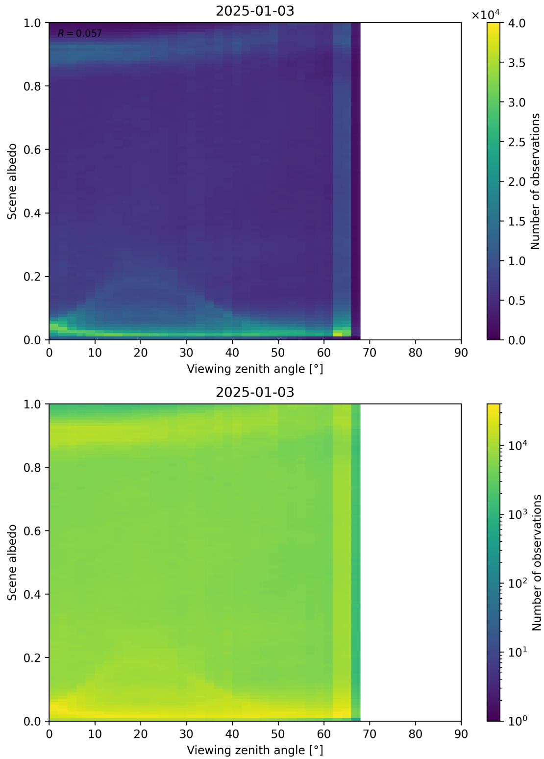
Figure 126: Scatter density plot of “Viewing zenith angle” against “Scene albedo” for 2025-01-02 to 2025-01-04.
