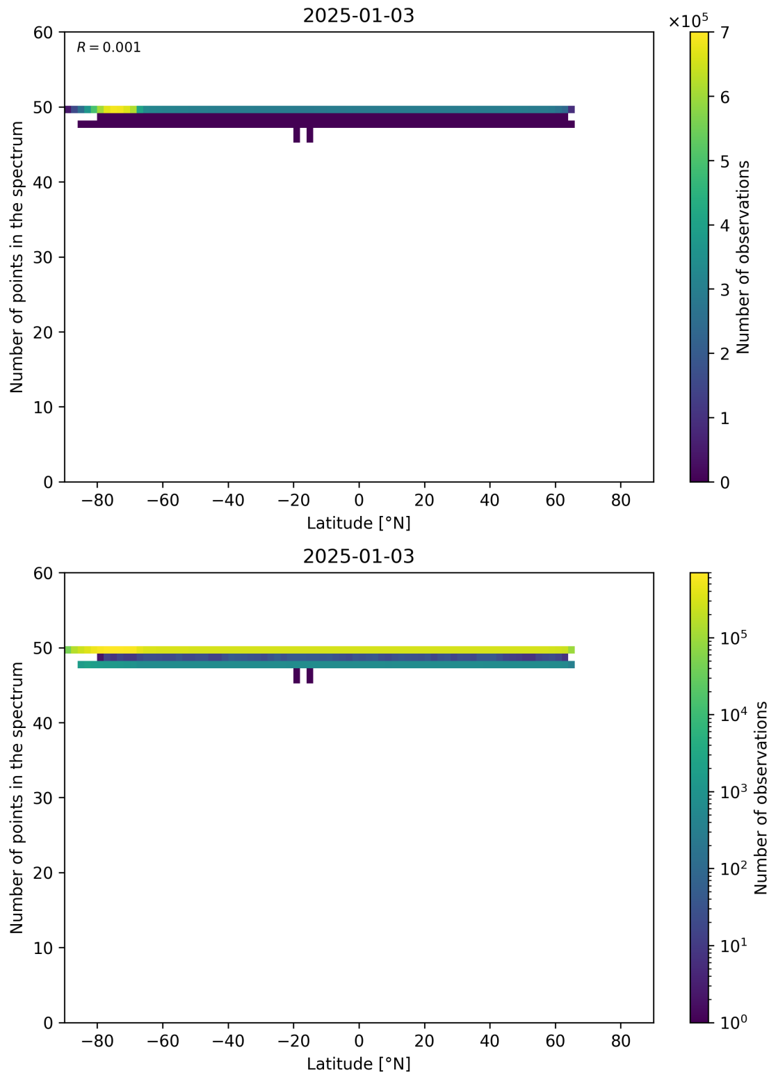
Figure 94: Scatter density plot of “Latitude” against “Number of points in the spectrum” for 2025-01-02 to 2025-01-04.
