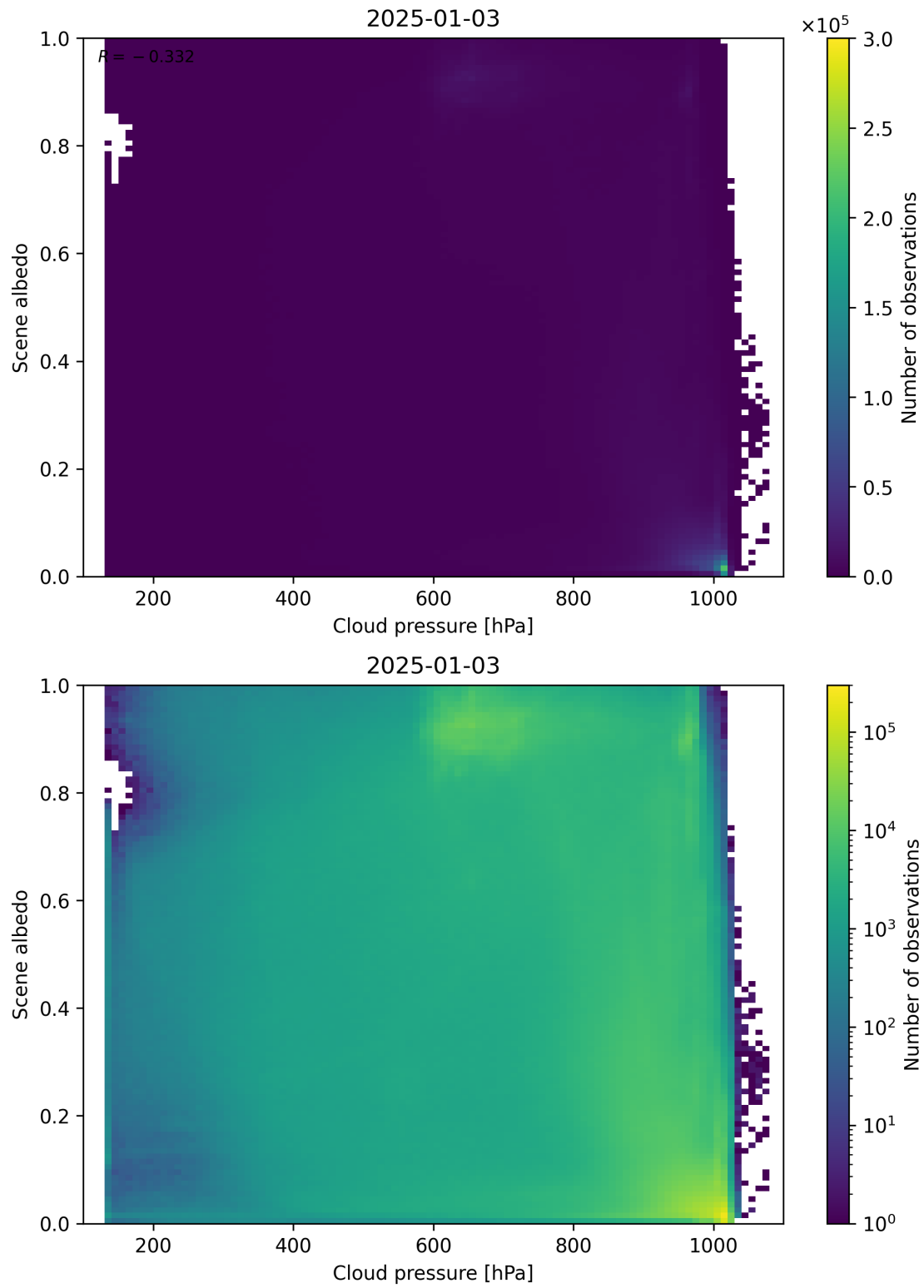
Figure 83: Scatter density plot of “Cloud pressure” against “Scene albedo” for 2025-01-02 to 2025-01-04.
