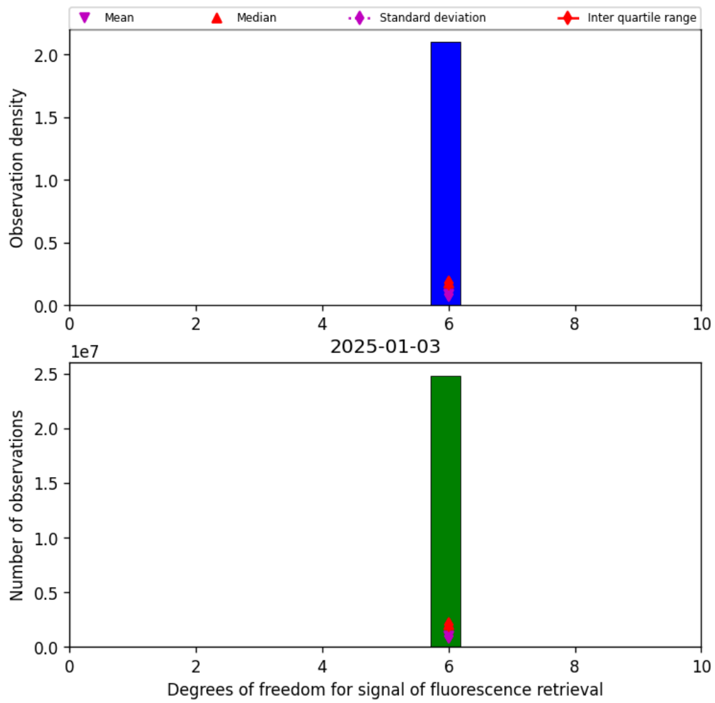
Figure 43: Histogram of “Degrees of freedom for signal of fluorescence retrieval” for 2025-01-02 to 2025-01-04
