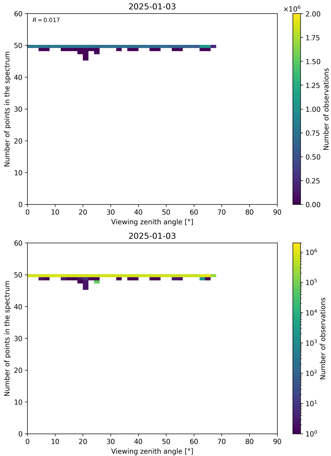
Figure 125: Scatter density plot of “Viewing zenith angle” against “Number of points in the spectrum” for 2025-01-02 to 2025-01-04.
