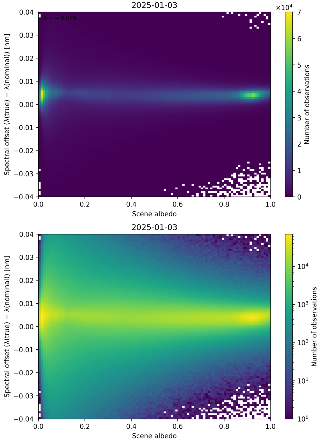
Figure 107: Scatter density plot of “Scene albedo” against “Spectral offset ( \lambda_{\text{true}} - \lambda_{\text{nominal}} )” for 2025-01-02 to 2025-01-04.
