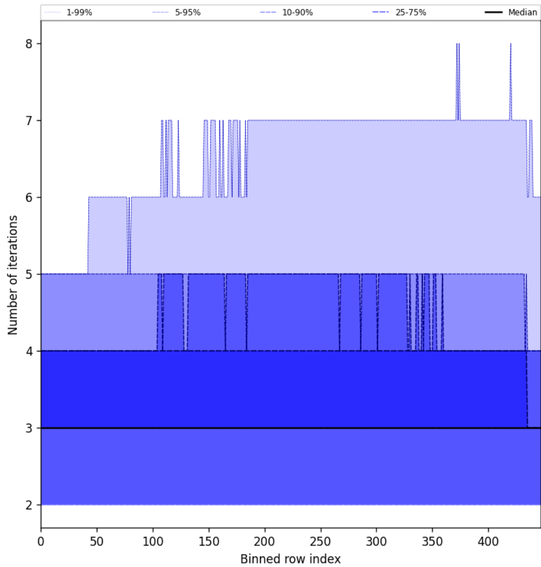
Figure 56: Along track statistics of “Number of iterations” for 2025-01-02 to 2025-01-04
