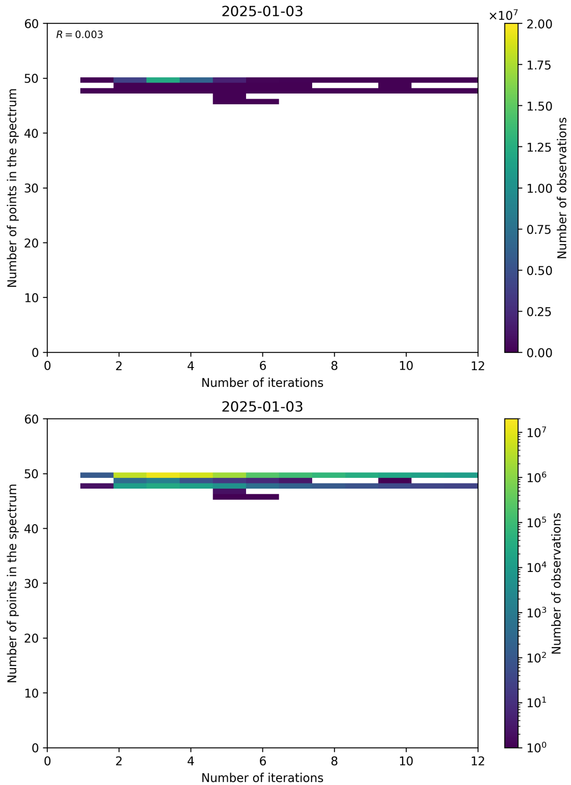
Figure 99: Scatter density plot of “Number of iterations” against “Number of points in the spectrum” for 2025-01-02 to 2025-01-04.
