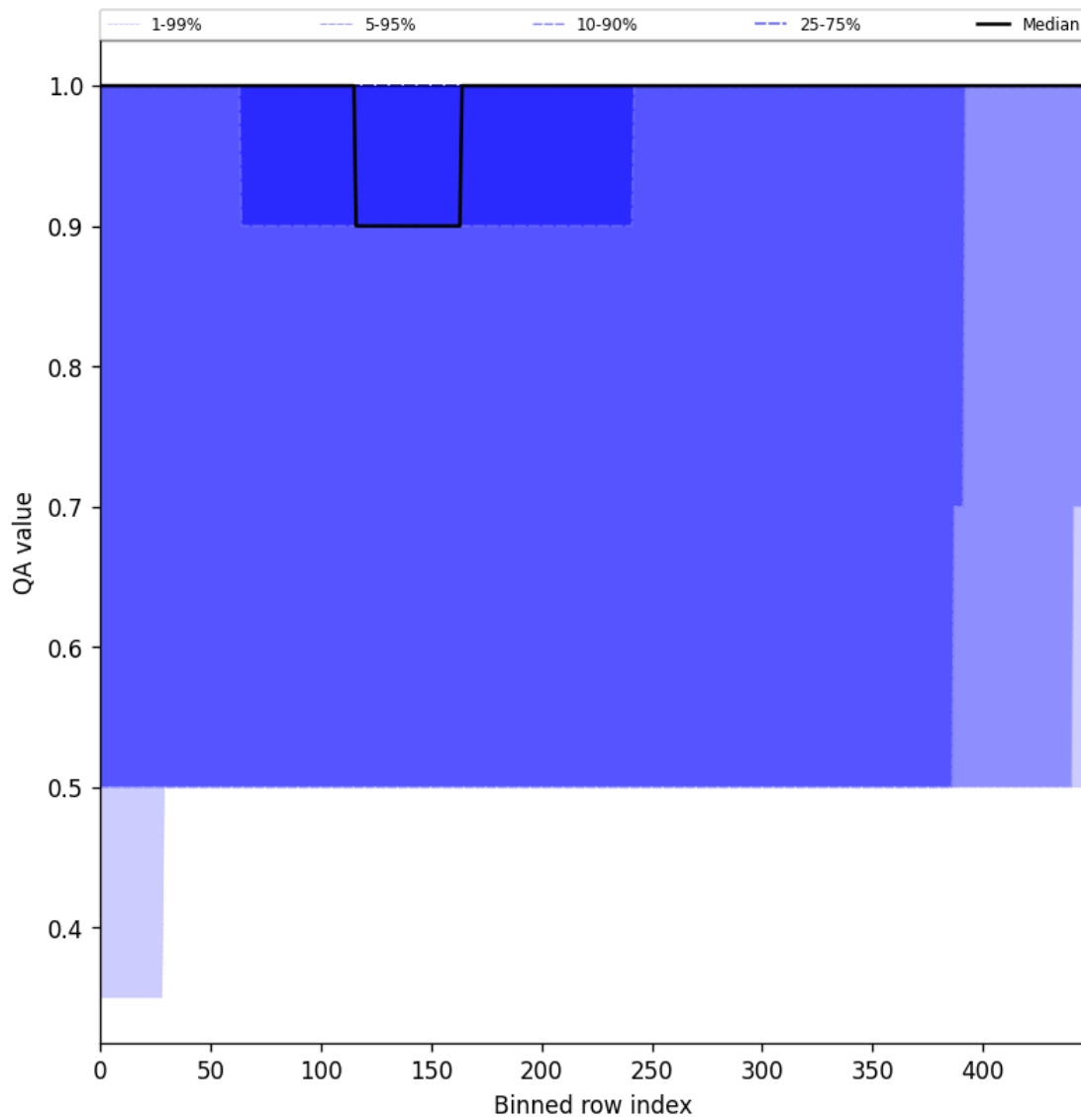
Figure 46: Along track statistics of “QA value” for 2025-01-02 to 2025-01-04
