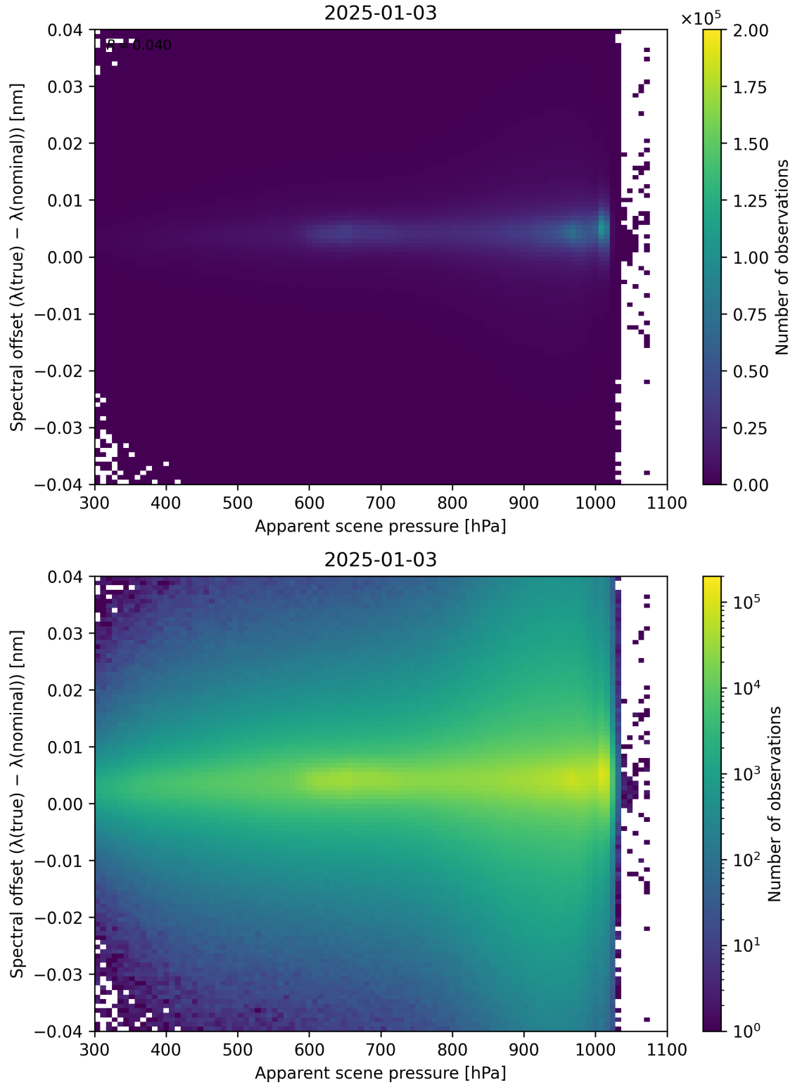
Figure 67: Scatter density plot of “Apparent scene pressure” against “Spectral offset ( \lambda_{\text{true}} - \lambda_{\text{nominal}} )” for 2025-01-02 to 2025-01-04.
