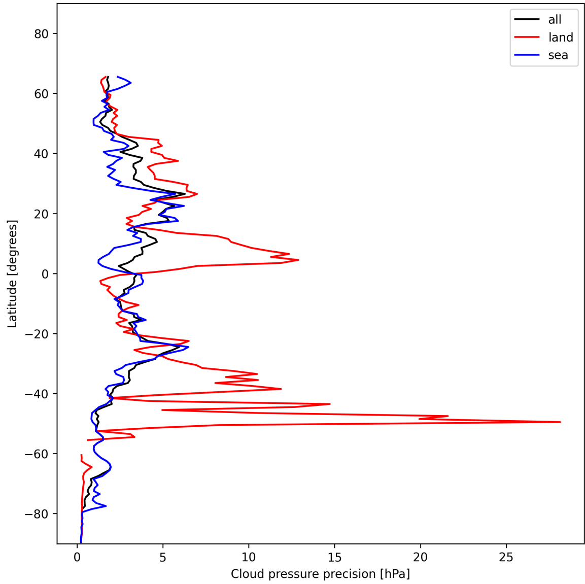
Figure 14: Zonal average of “Cloud pressure precision” for 2025-01-02 to 2025-01-04.
