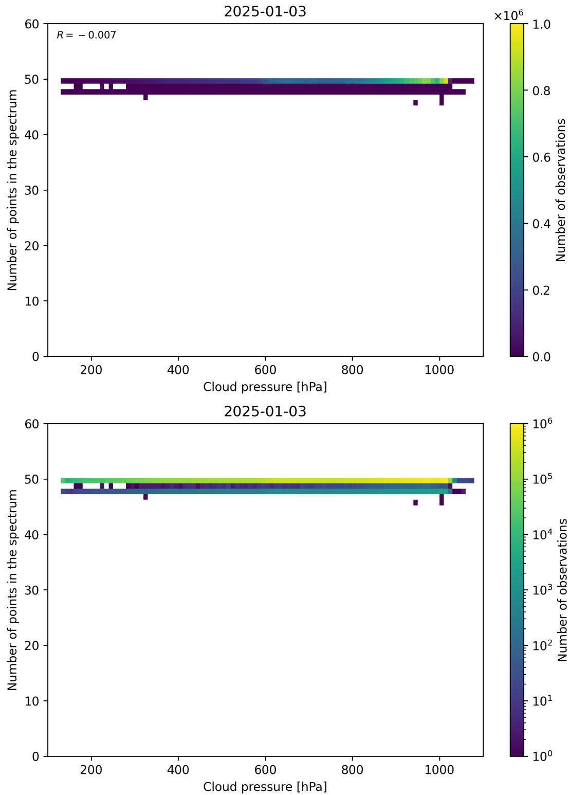
Figure 82: Scatter density plot of “Cloud pressure” against “Number of points in the spectrum” for 2025-01-02 to 2025-01-04.
