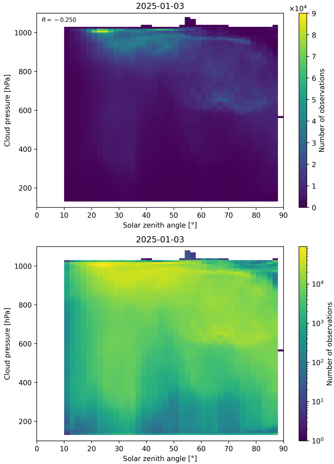
Figure 111: Scatter density plot of “Solar zenith angle” against “Cloud pressure” for 2025-01-02 to 2025-01-04.
