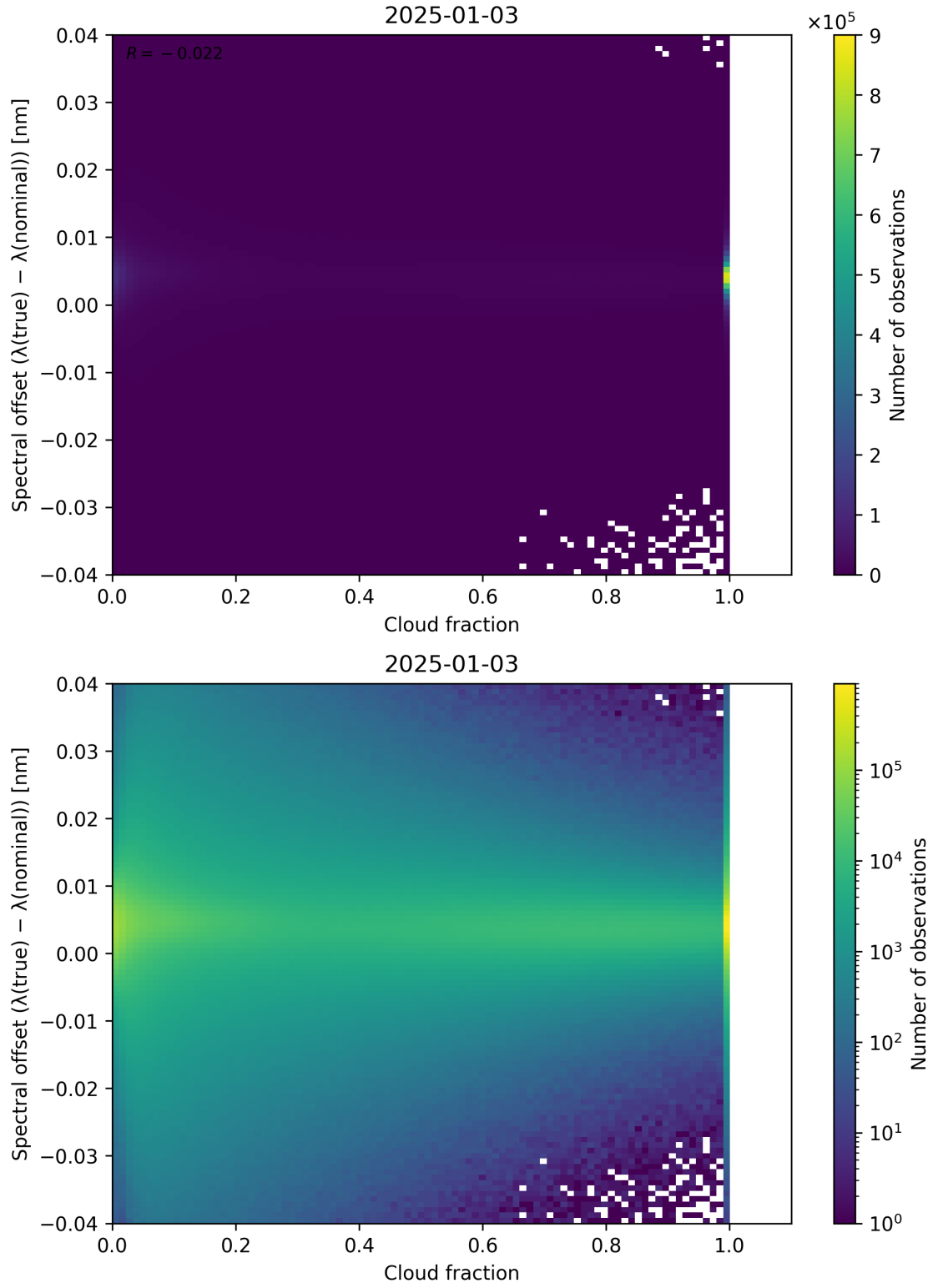
Figure 76: Scatter density plot of “Cloud fraction” against “Spectral offset ( \lambda_{\text{true}} - \lambda_{\text{nominal}} )” for 2025-01-02 to 2025-01-04.
