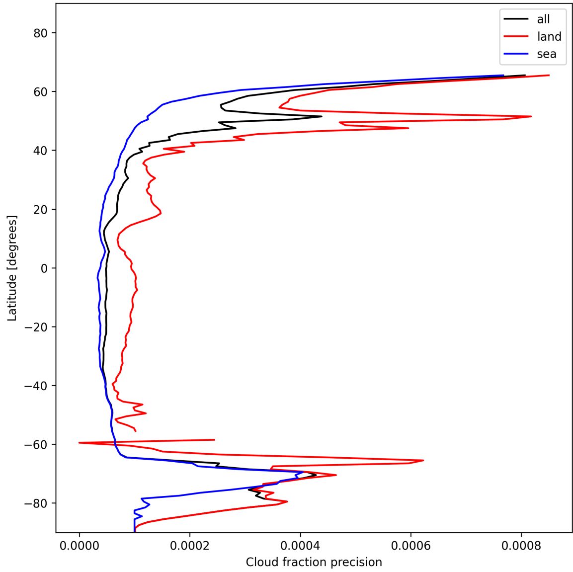
Figure 16: Zonal average of “Cloud fraction precision” for 2025-01-03 to 2025-01-05.
