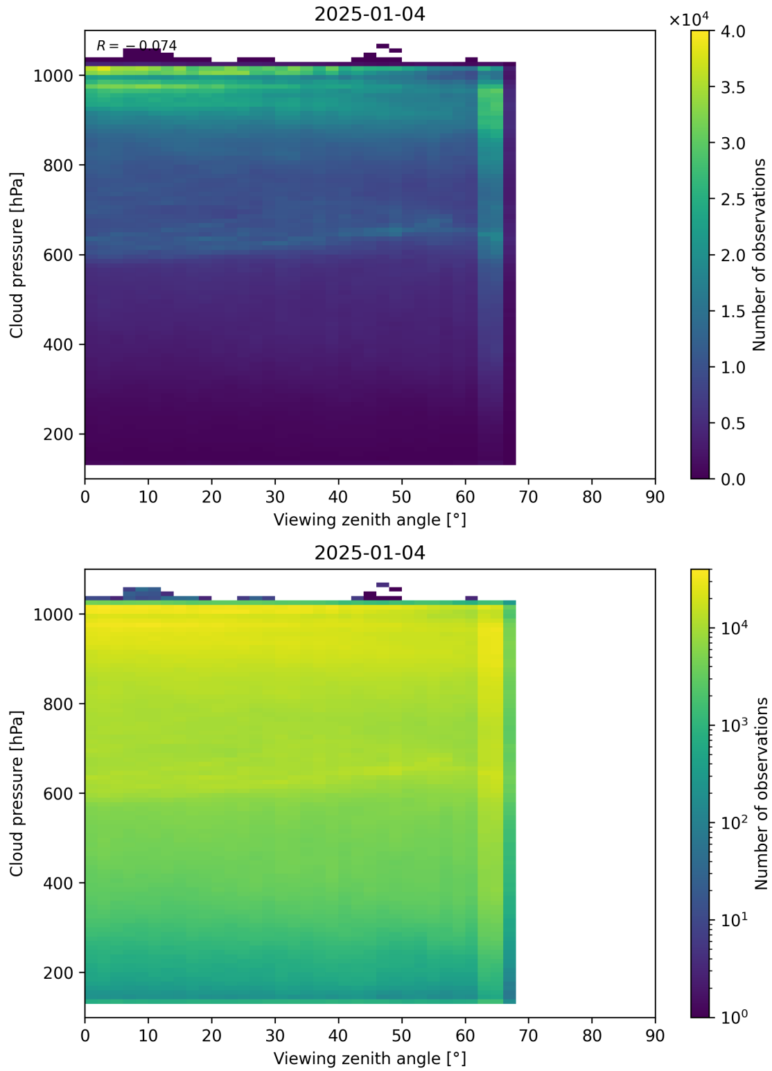
Figure 121: Scatter density plot of “Viewing zenith angle” against “Cloud pressure” for 2025-01-03 to 2025-01-05.
