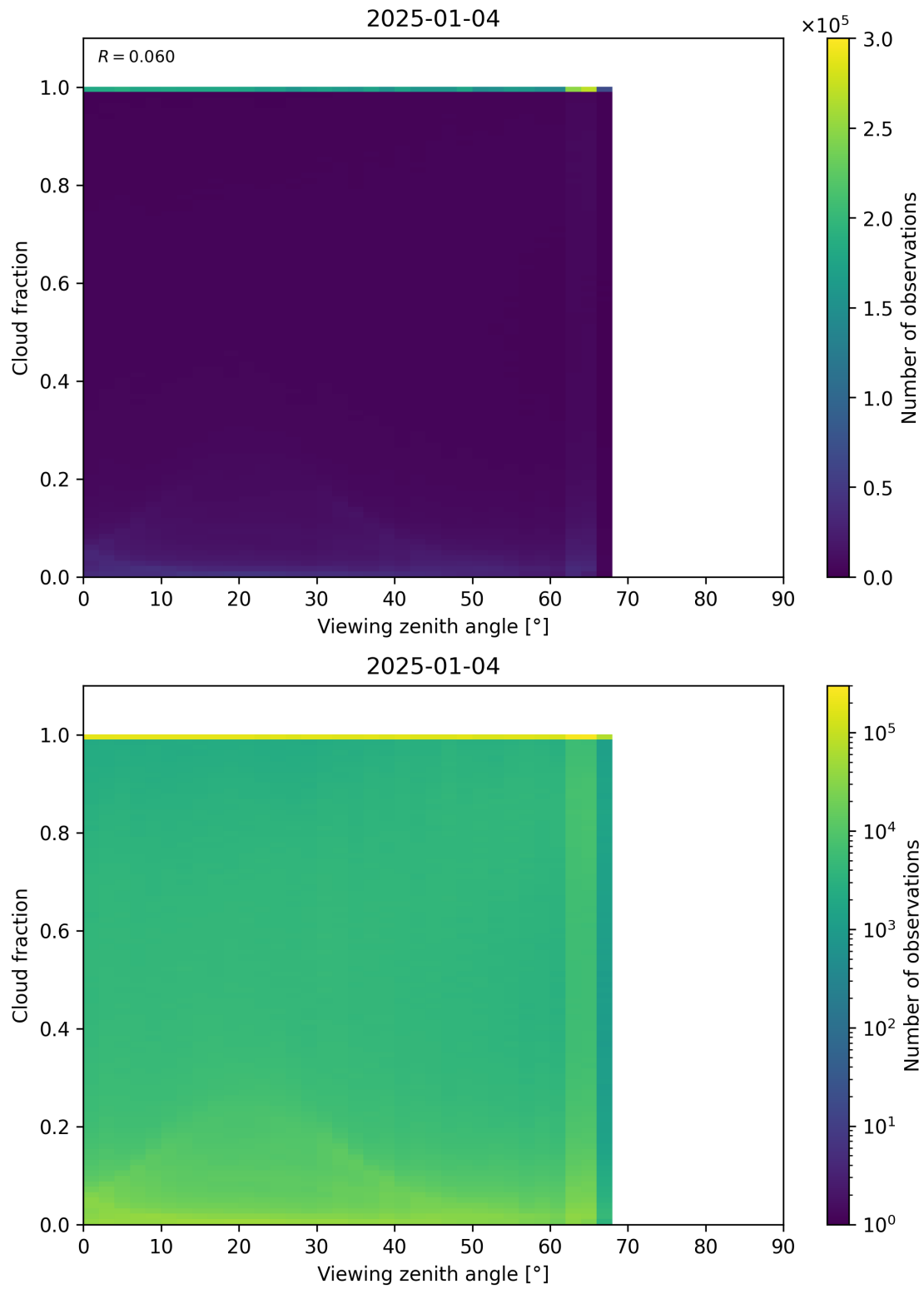
Figure 120: Scatter density plot of “Viewing zenith angle” against “Cloud fraction” for 2025-01-03 to 2025-01-05.
