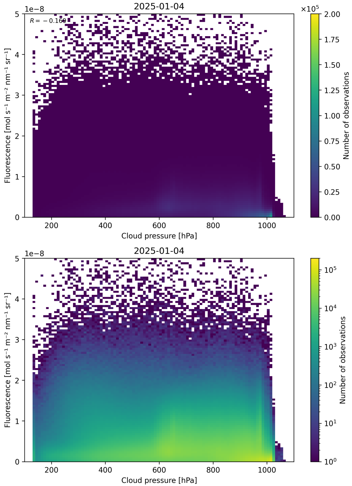
Figure 80: Scatter density plot of “Cloud pressure” against “Fluorescence” for 2025-01-03 to 2025-01-05.
