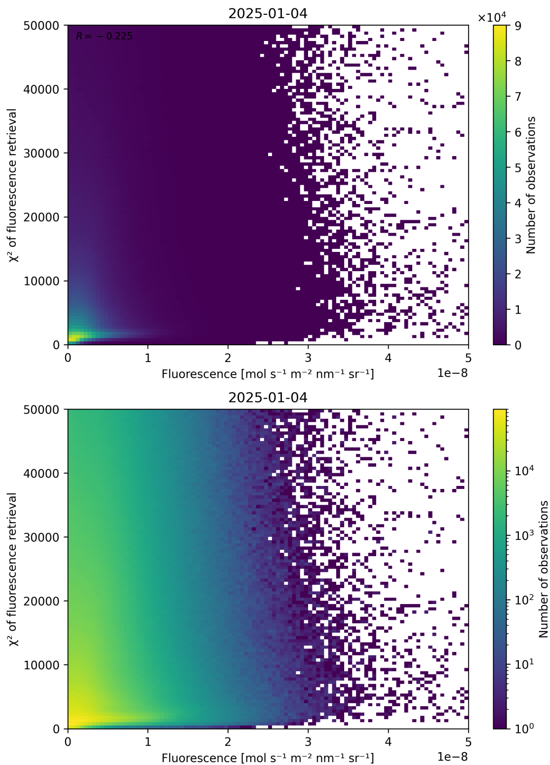
Figure 85: Scatter density plot of “Fluorescence” against “ \chi^2 of fluorescence retrieval” for 2025-01-03 to 2025-01-05.
