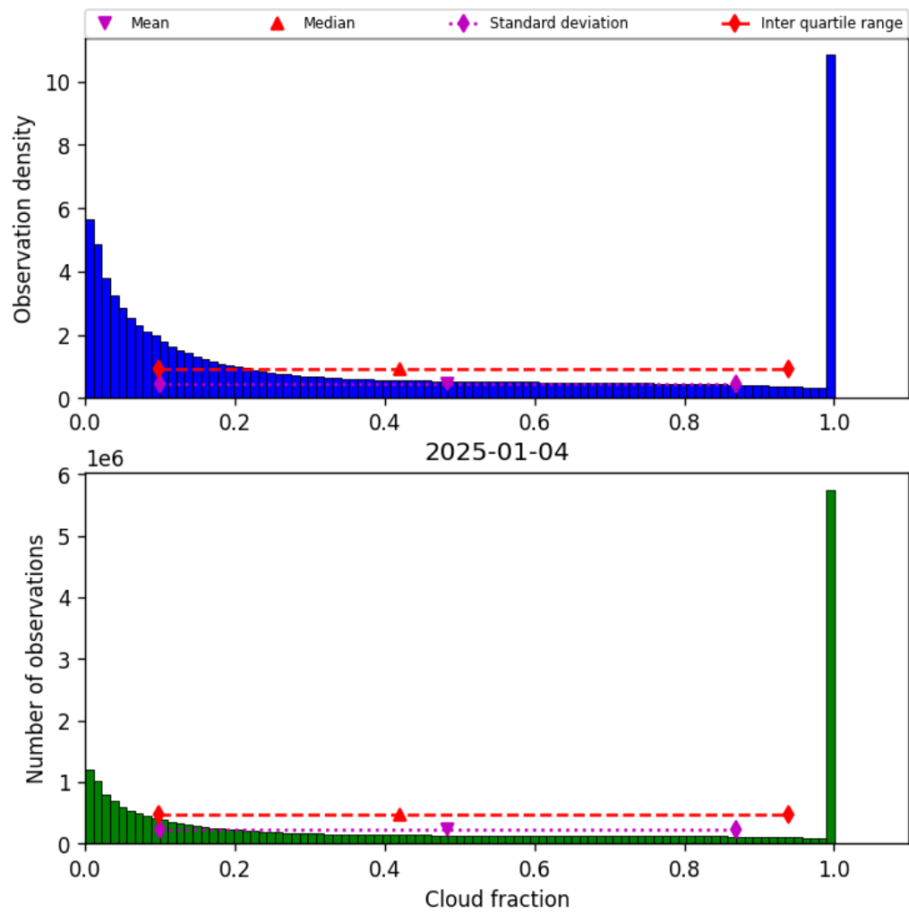
Figure 32: Histogram of “Cloud fraction” for 2025-01-03 to 2025-01-05
