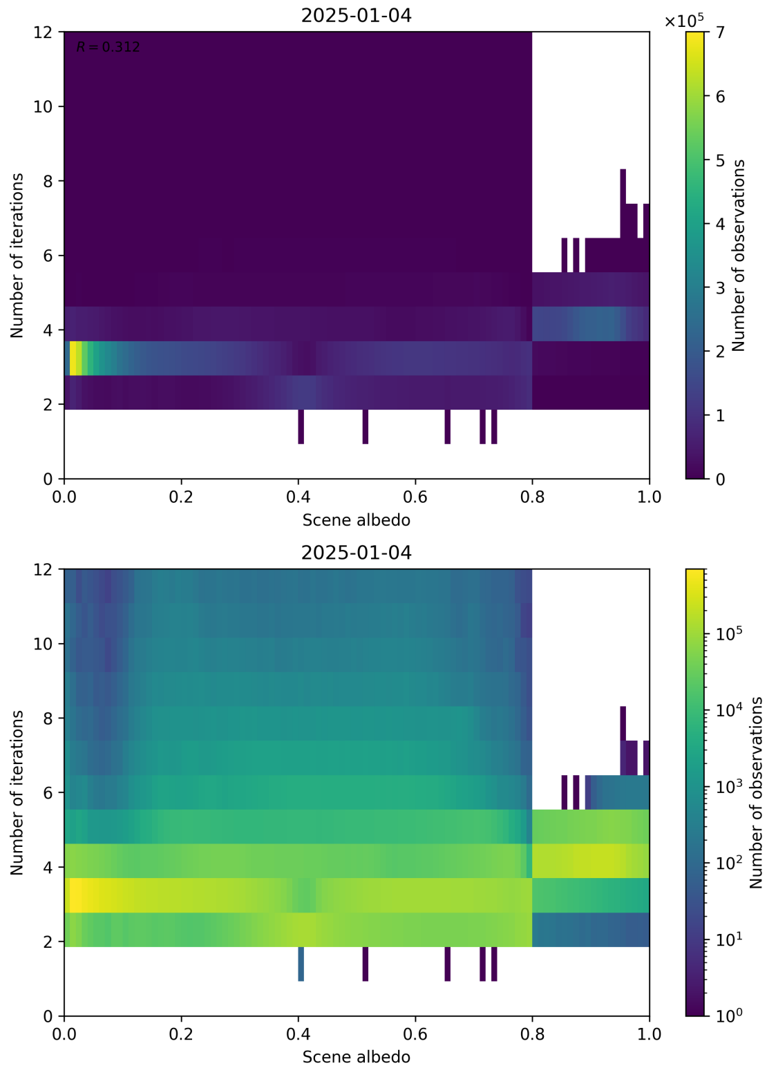
Figure 105: Scatter density plot of “Scene albedo” against “Number of iterations” for 2025-01-03 to 2025-01-05.
