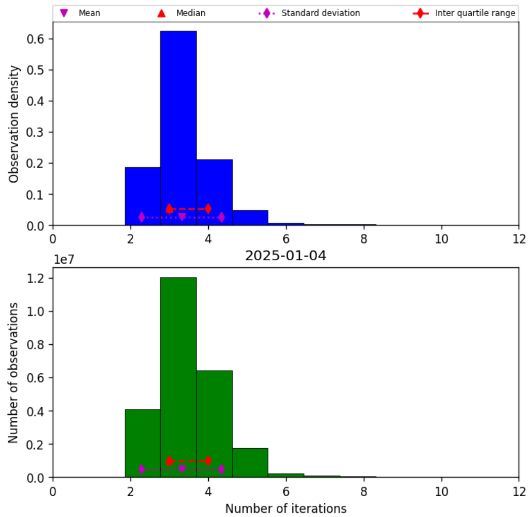
Figure 39: Histogram of “Number of iterations” for 2025-01-03 to 2025-01-05
