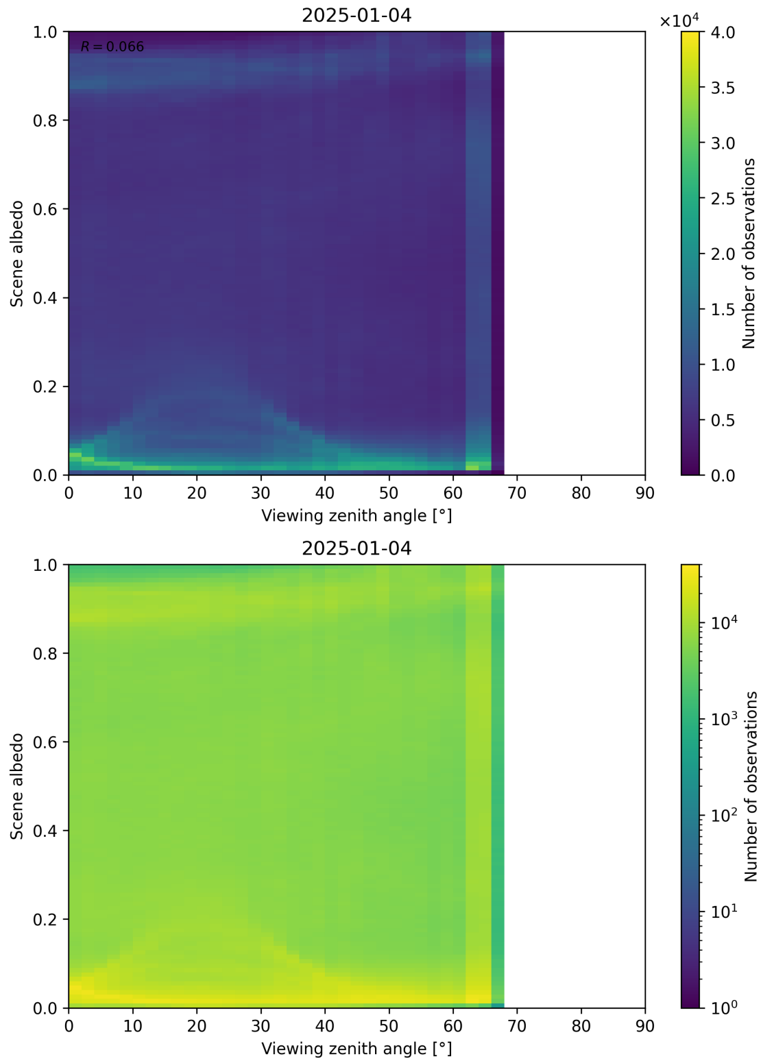
Figure 126: Scatter density plot of “Viewing zenith angle” against “Scene albedo” for 2025-01-03 to 2025-01-05.
