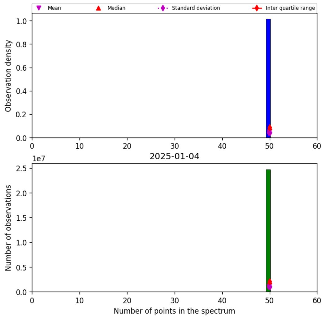
Figure 44: Histogram of “Number of points in the spectrum” for 2025-01-03 to 2025-01-05
