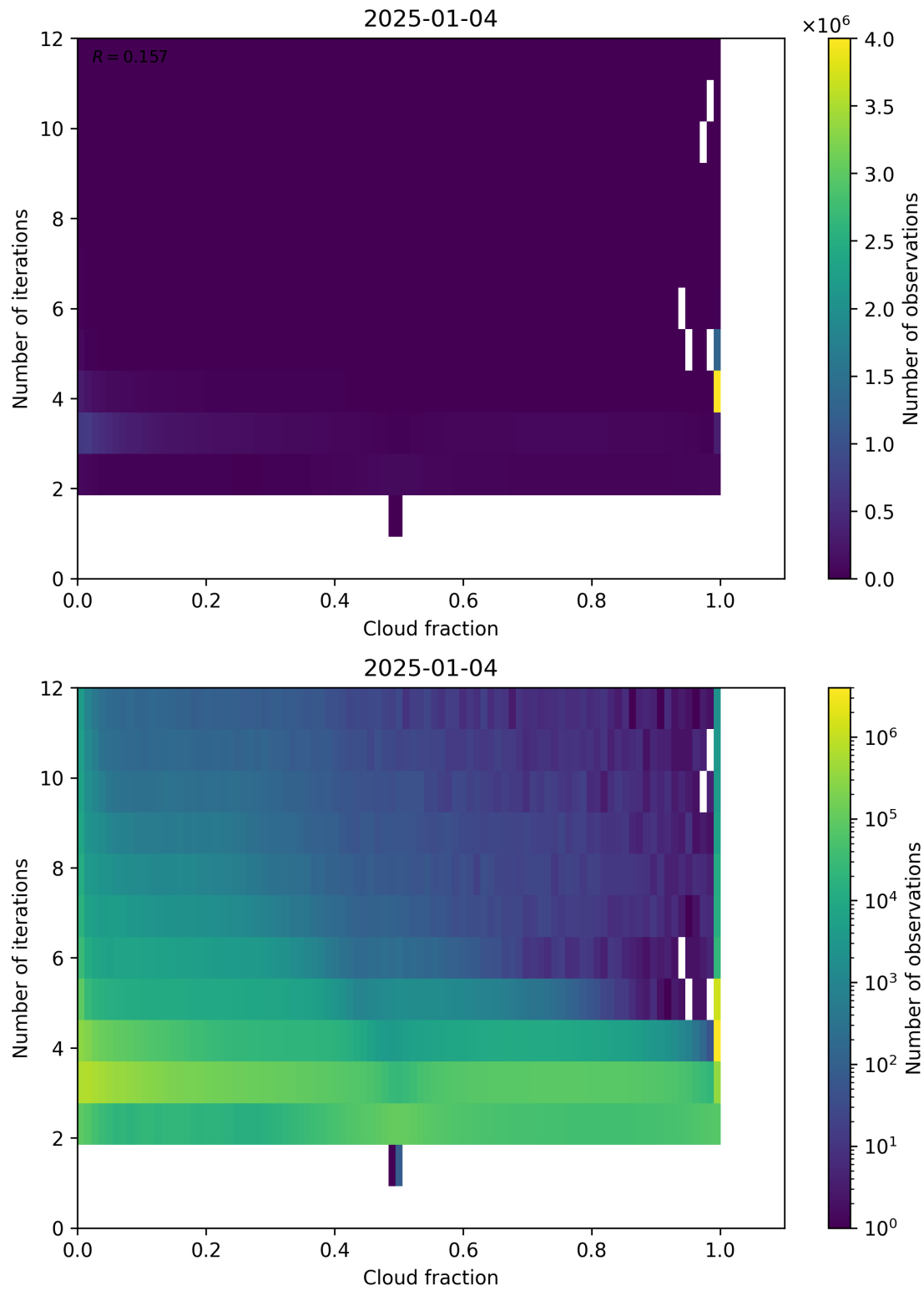
Figure 73: Scatter density plot of “Cloud fraction” against “Number of iterations” for 2025-01-03 to 2025-01-05.
