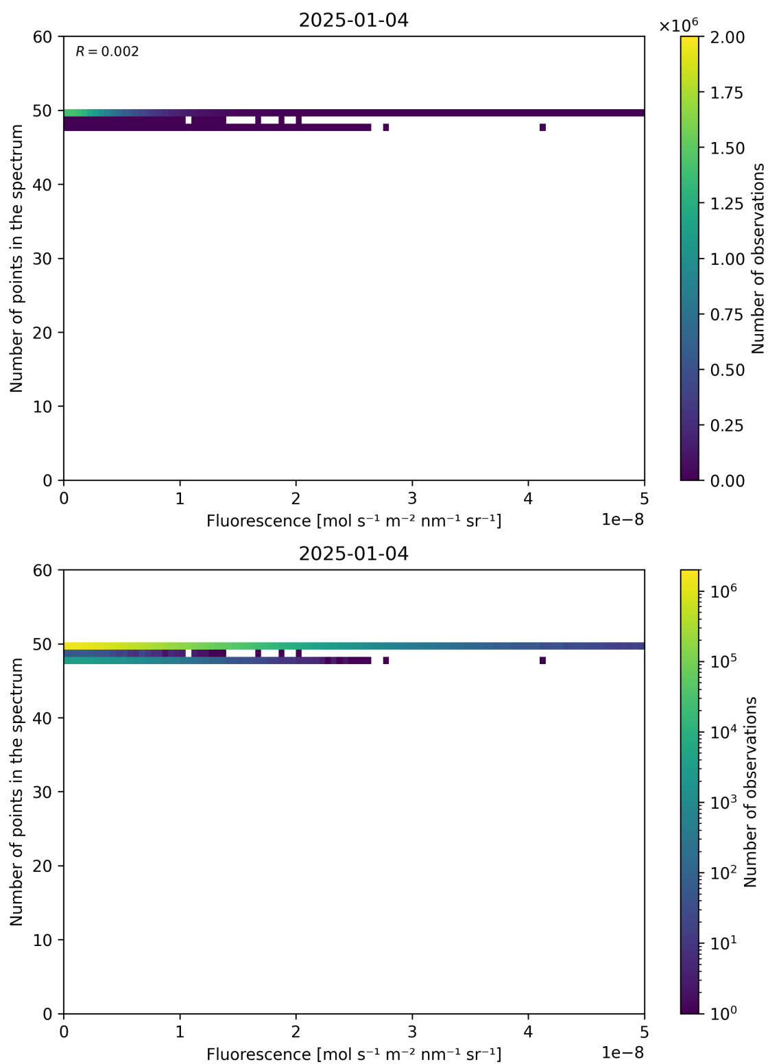
Figure 86: Scatter density plot of “Fluorescence” against “Number of points in the spectrum” for 2025-01-03 to 2025-01-05.
