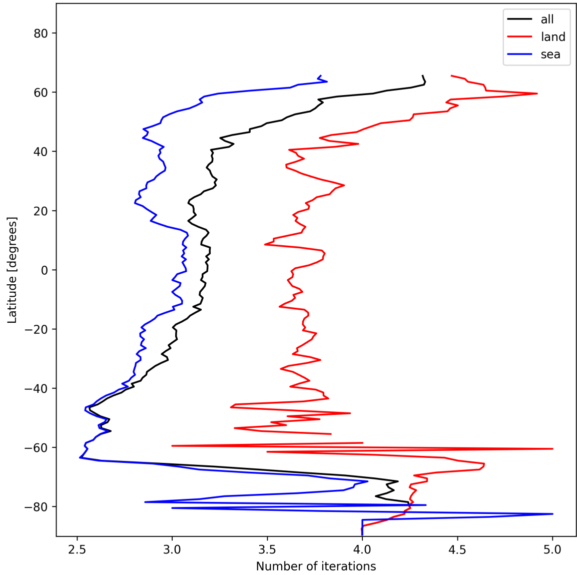
Figure 22: Zonal average of “Number of iterations” for 2025-01-03 to 2025-01-05.
