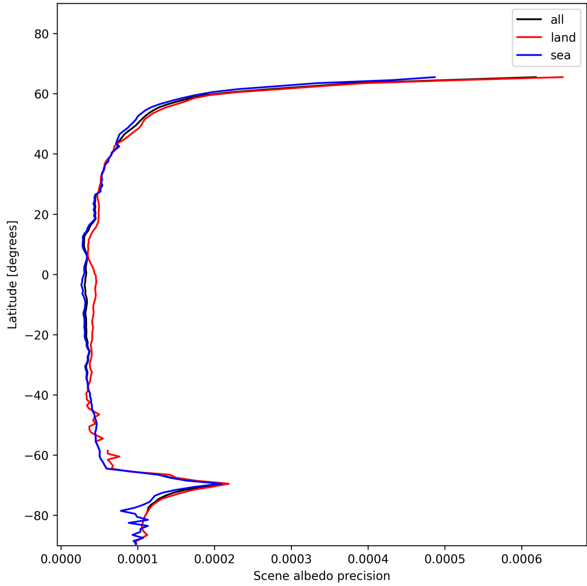
Figure 18: Zonal average of “Scene albedo precision” for 2025-01-03 to 2025-01-05.
