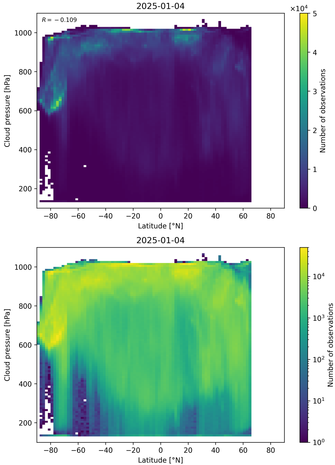
Figure 91: Scatter density plot of “Latitude” against “Cloud pressure” for 2025-01-03 to 2025-01-05.
