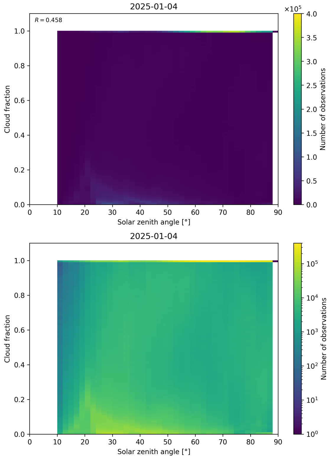
Figure 110: Scatter density plot of “Solar zenith angle” against “Cloud fraction” for 2025-01-03 to 2025-01-05.
