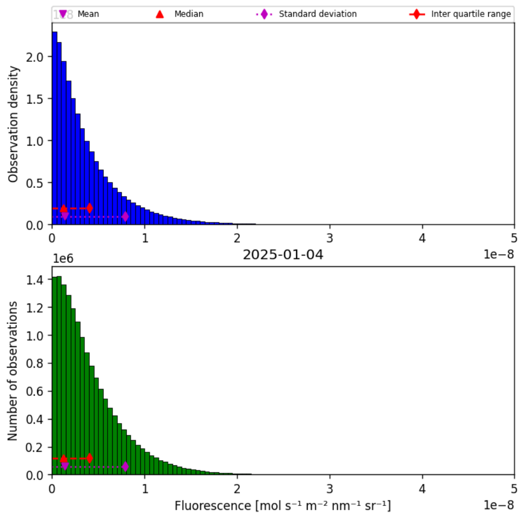
Figure 40: Histogram of “Fluorescence” for 2025-01-03 to 2025-01-05
