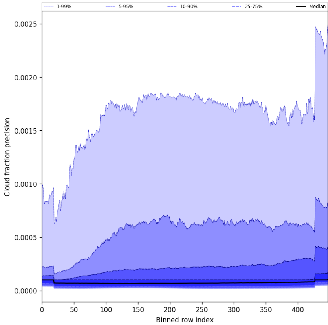
Figure 50: Along track statistics of “Cloud fraction precision” for 2025-01-03 to 2025-01-05
