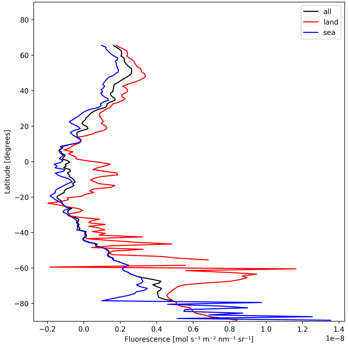
Figure 23: Zonal average of “Fluorescence” for 2025-01-03 to 2025-01-05.
