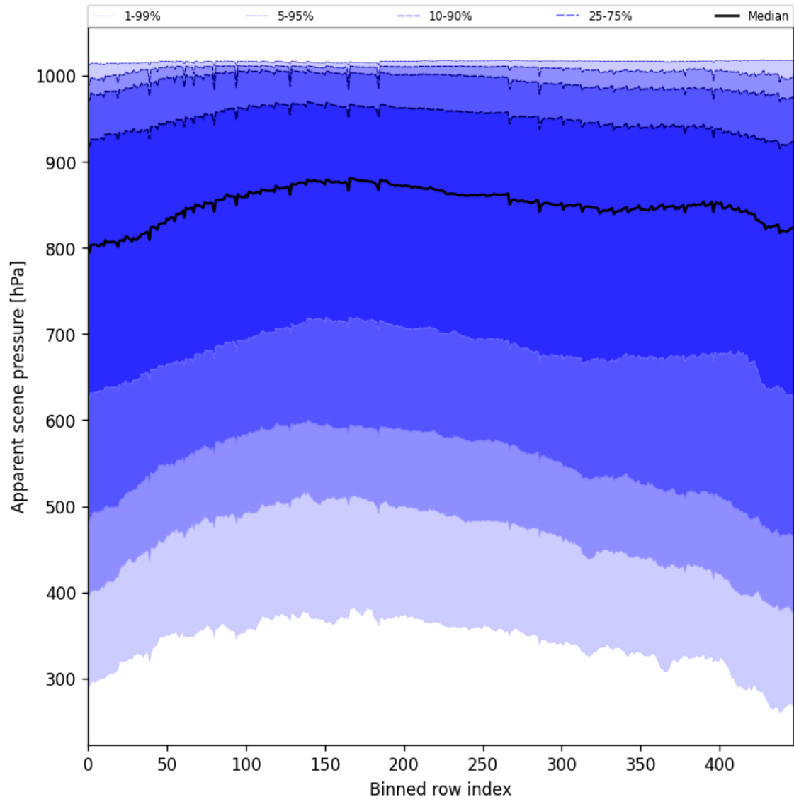
Figure 53: Along track statistics of “Apparent scene pressure” for 2025-01-03 to 2025-01-05
