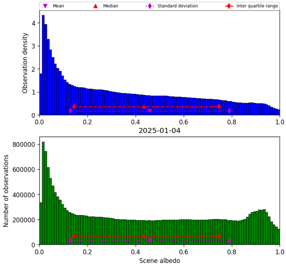
Figure 34: Histogram of “Scene albedo” for 2025-01-03 to 2025-01-05
