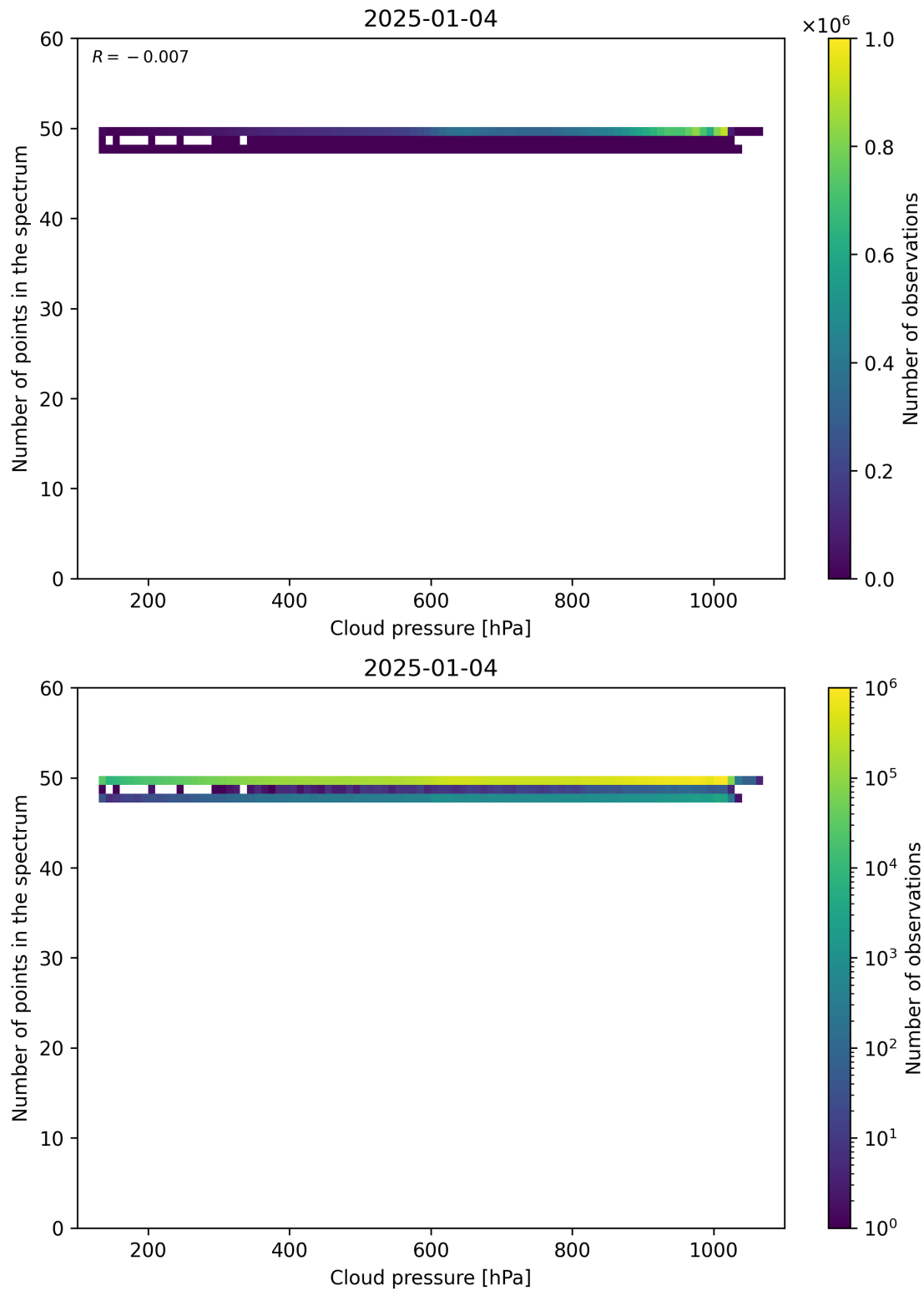
Figure 82: Scatter density plot of “Cloud pressure” against “Number of points in the spectrum” for 2025-01-03 to 2025-01-05.
