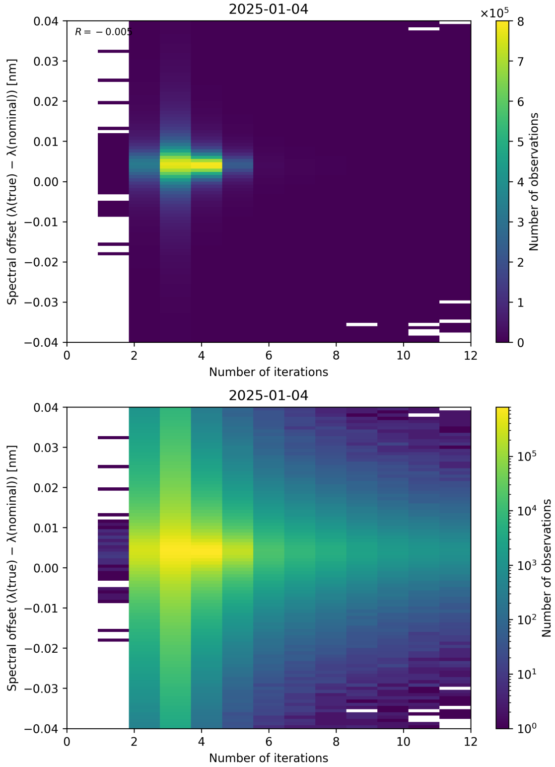
Figure 100: Scatter density plot of “Number of iterations” against “Spectral offset ( \lambda_{\text{true}} - \lambda_{\text{nominal}} )” for 2025-01-03 to 2025-01-05.
