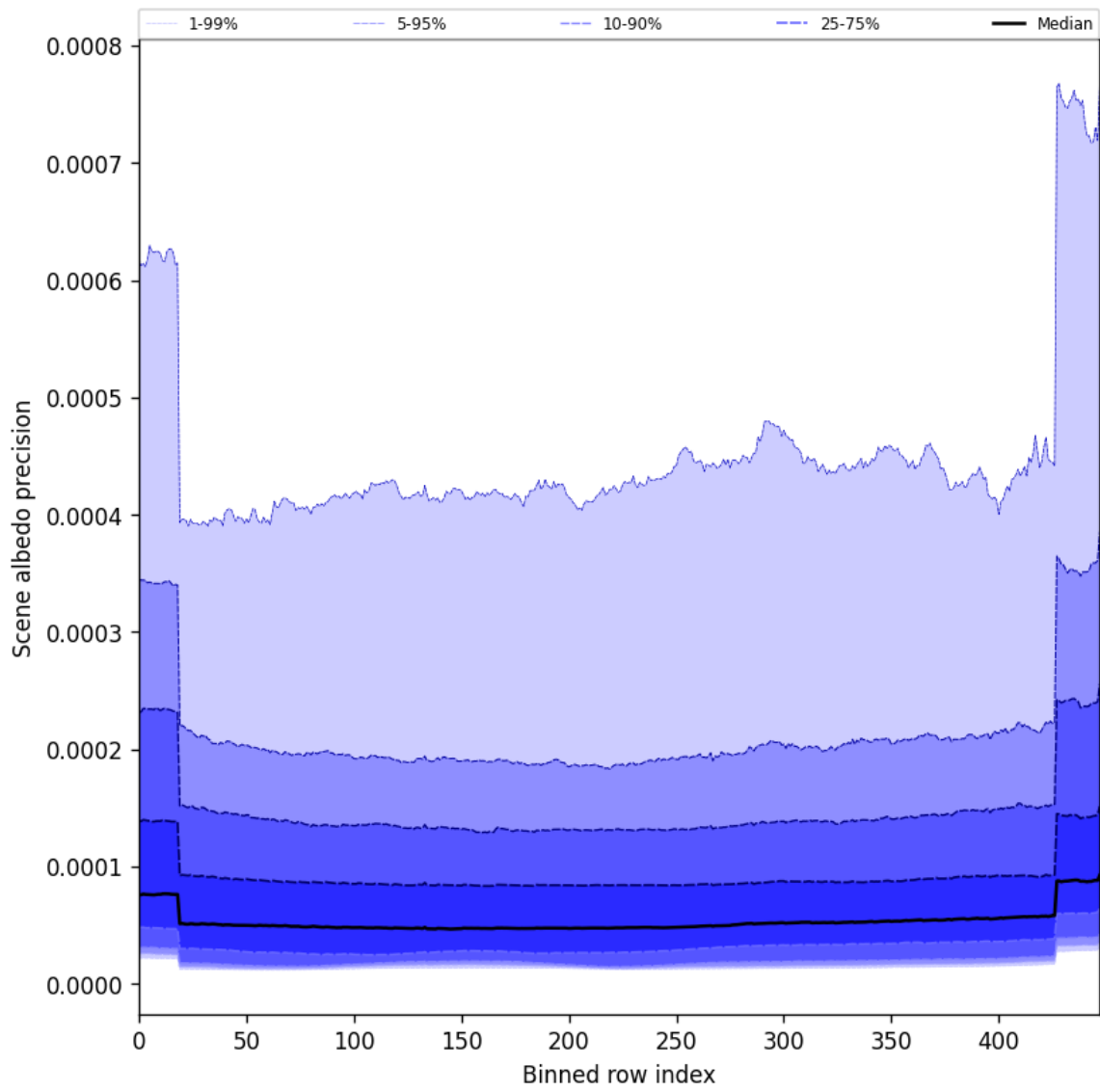
Figure 52: Along track statistics of “Scene albedo precision” for 2025-01-03 to 2025-01-05
