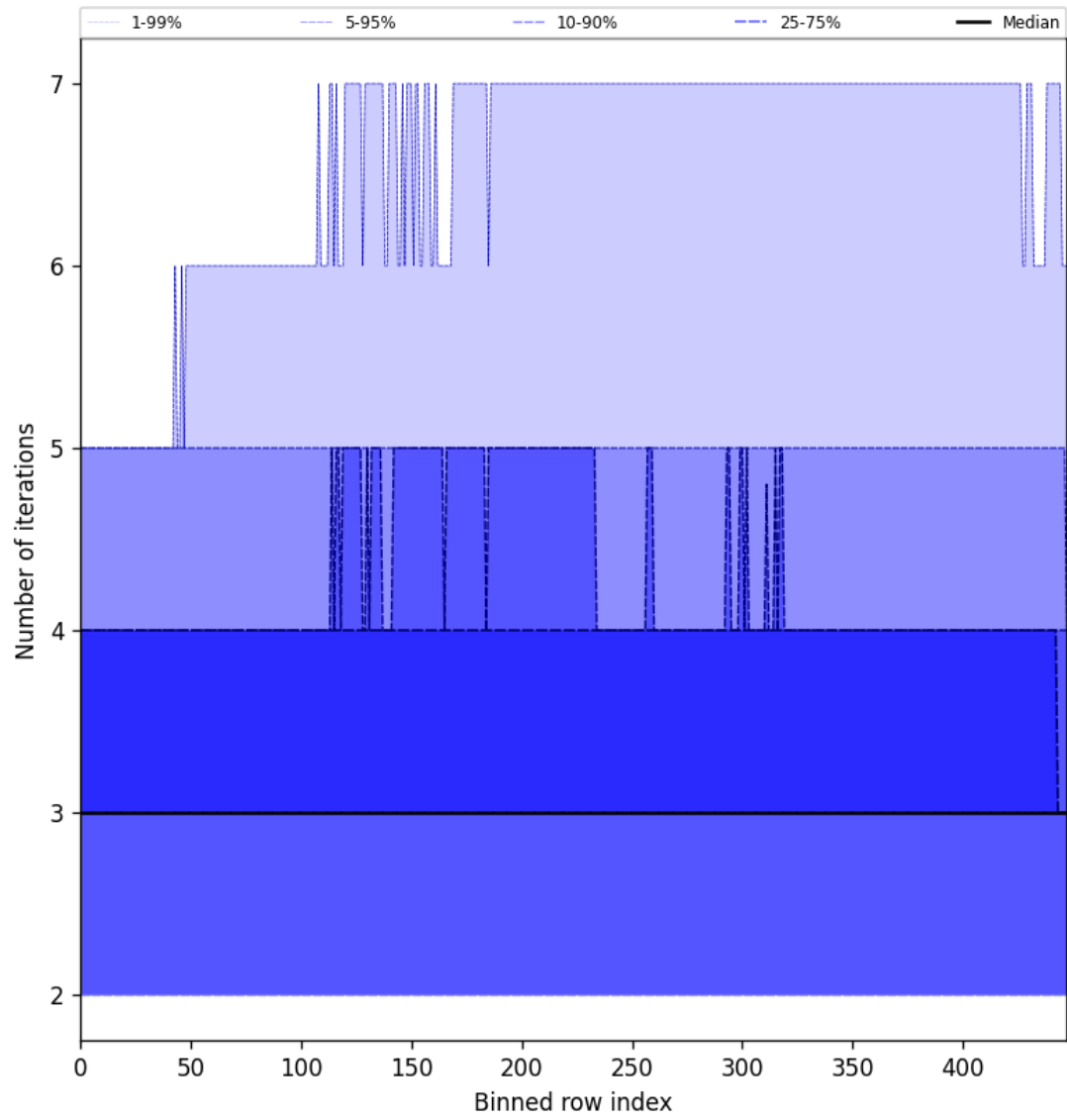
Figure 56: Along track statistics of “Number of iterations” for 2025-01-03 to 2025-01-05
