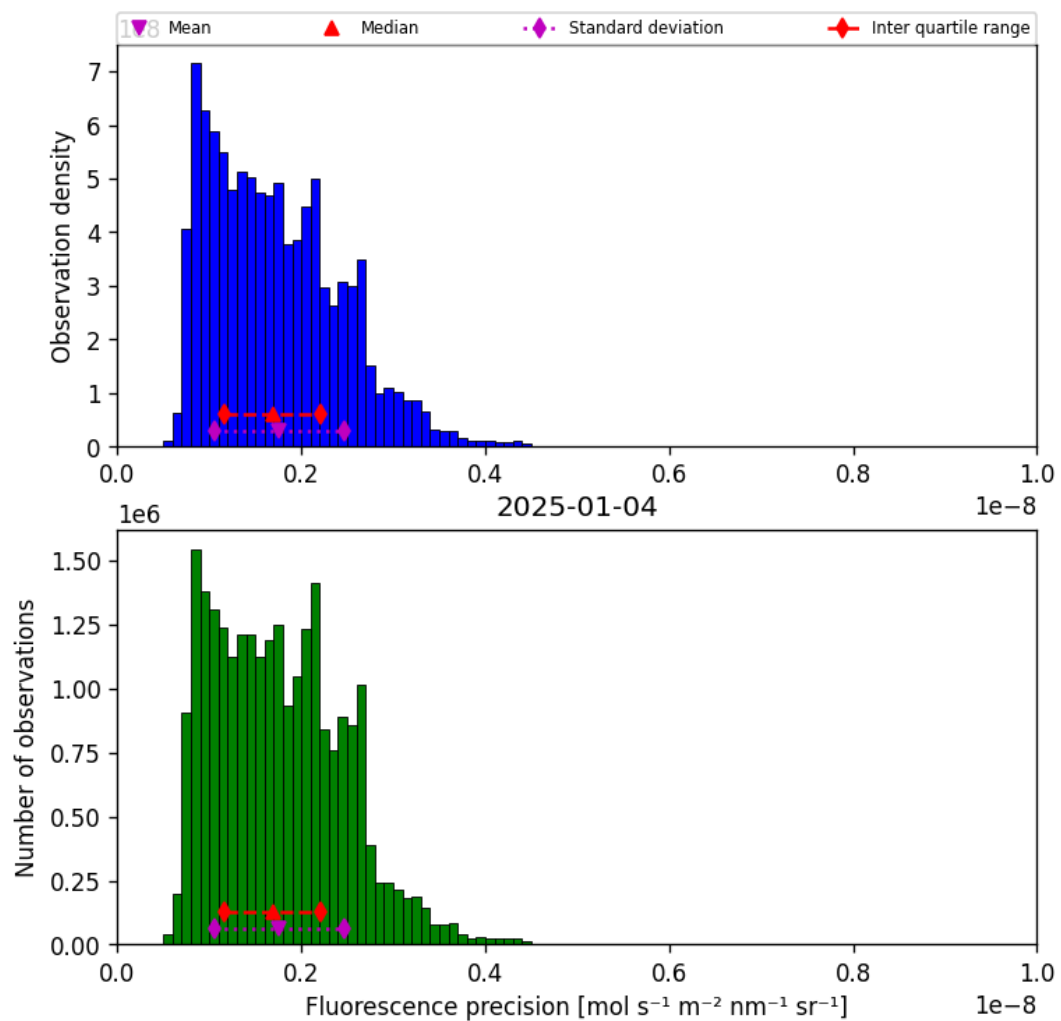
Figure 41: Histogram of “Fluorescence precision” for 2025-01-03 to 2025-01-05
