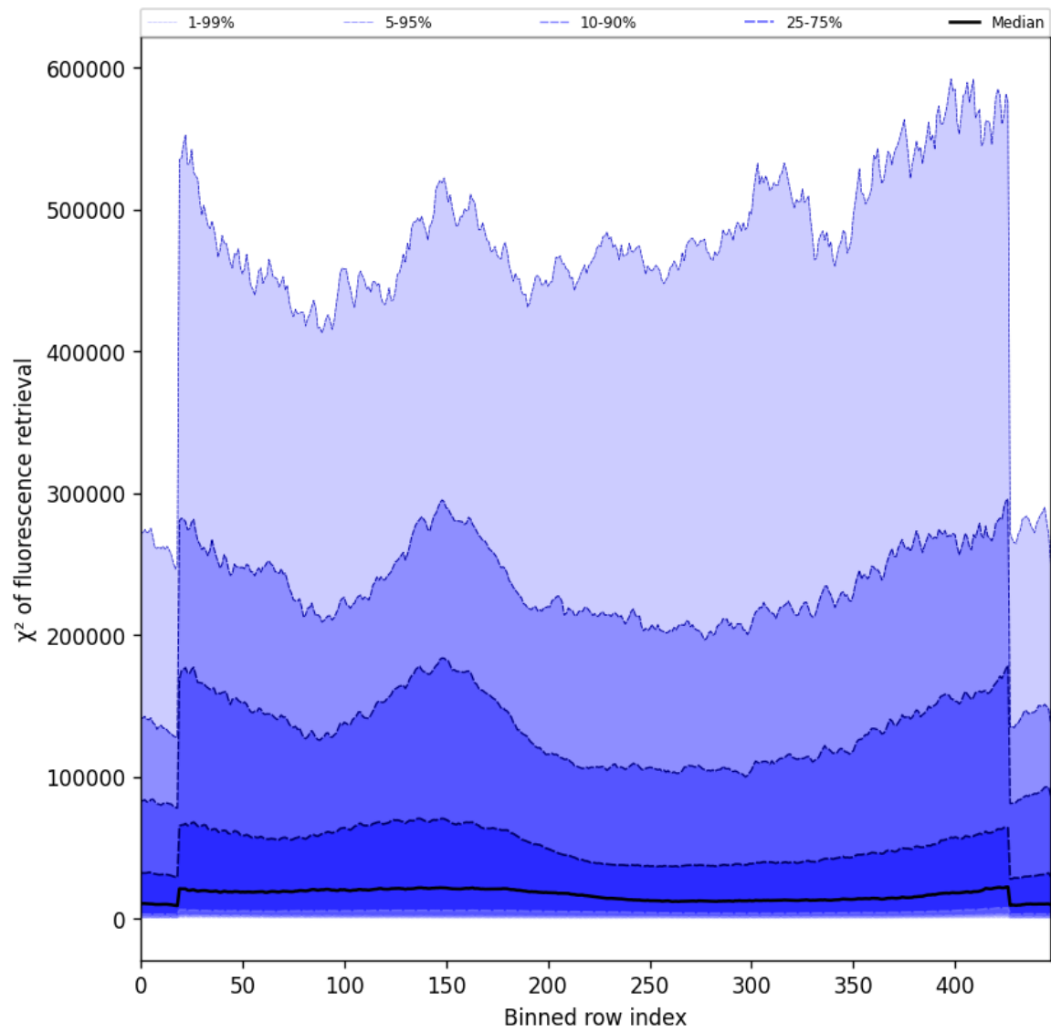
Figure 59: Along track statistics of “ \chi^2 of fluorescence retrieval” for 2025-01-03 to 2025-01-05
