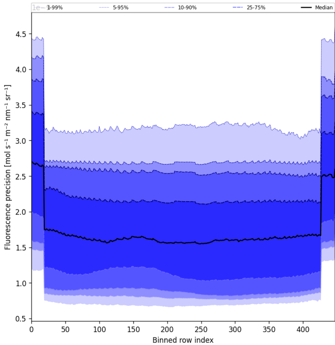
Figure 58: Along track statistics of "Fluorescence precision" for 2025-01-03 to 2025-01-05
