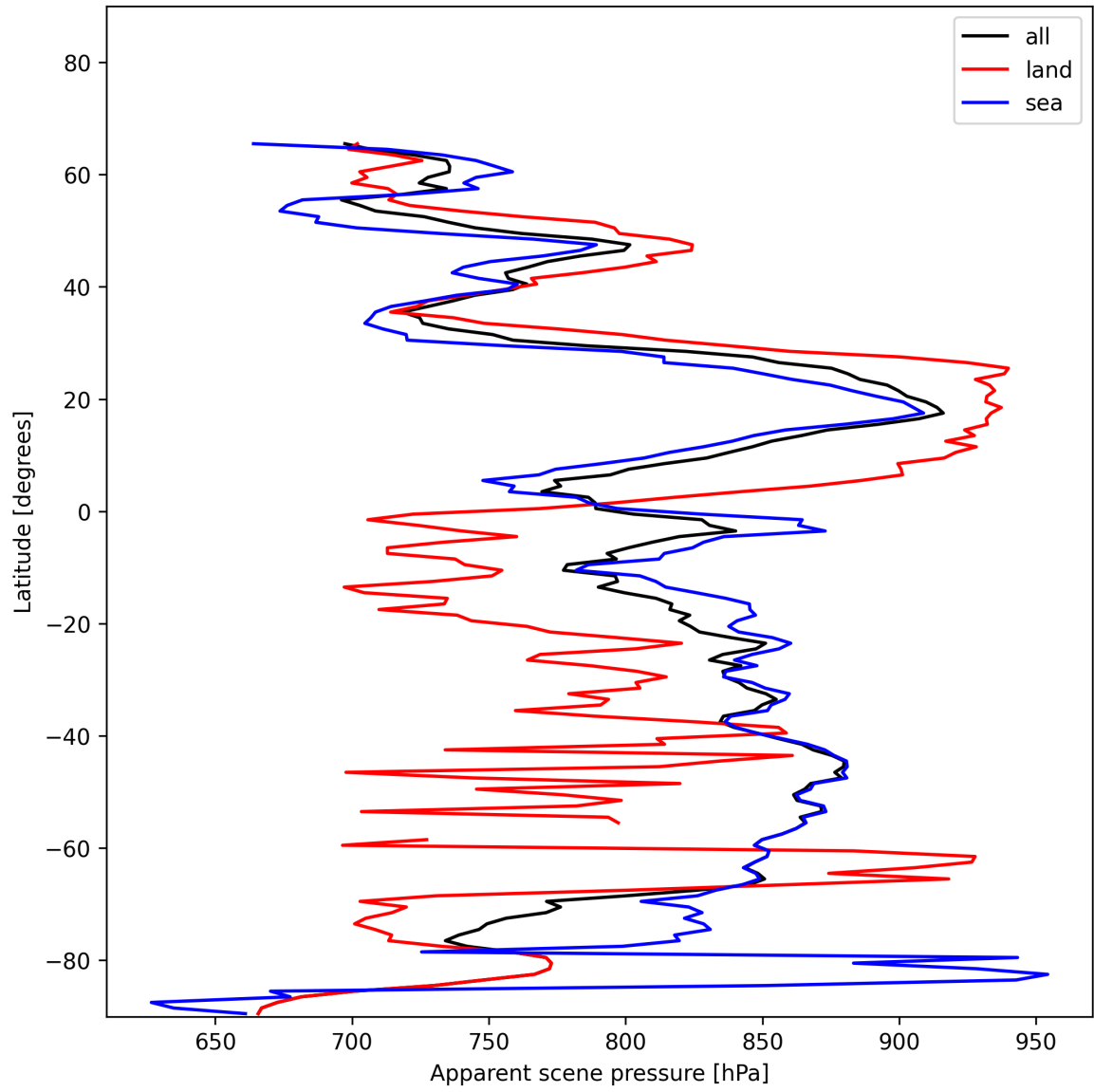
Figure 19: Zonal average of “Apparent scene pressure” for 2025-01-03 to 2025-01-05.
