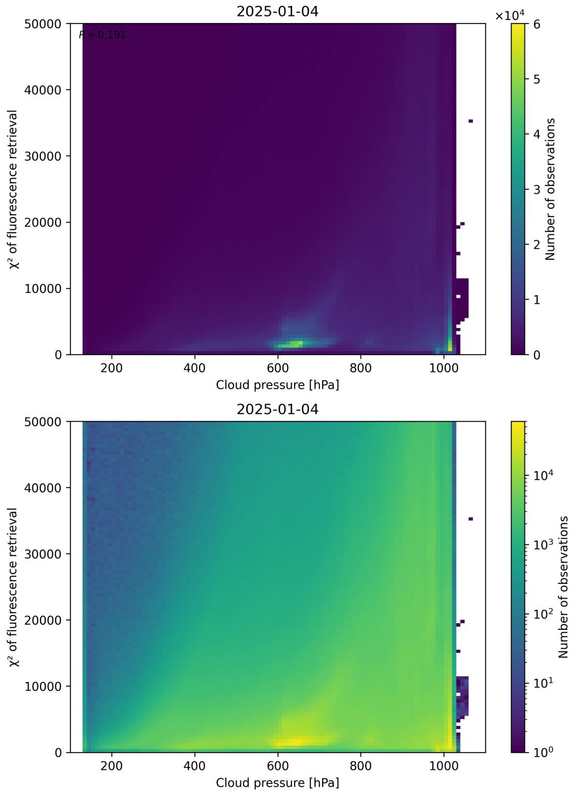
Figure 78: Scatter density plot of “Cloud pressure” against “ \chi^2 of fluorescence retrieval” for 2025-01-03 to 2025-01-05.
