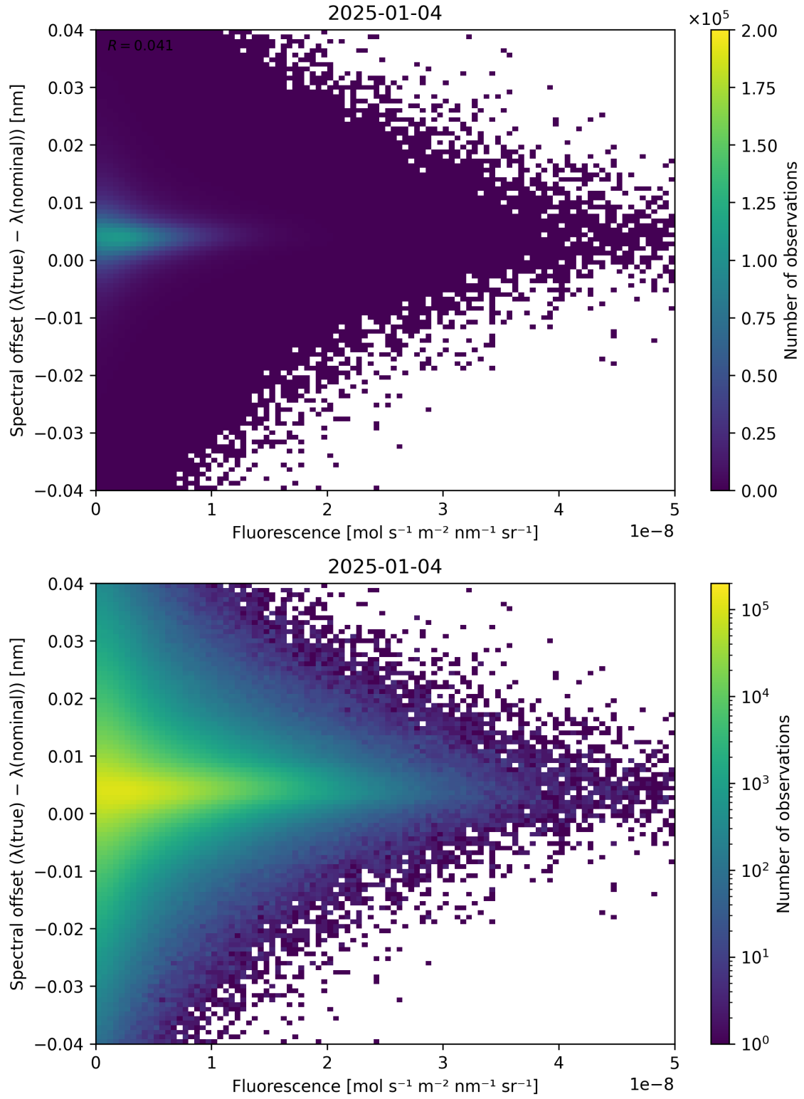
Figure 87: Scatter density plot of “Fluorescence” against “Spectral offset ( \lambda_{\text{true}} - \lambda_{\text{nominal}} )” for 2025-01-03 to 2025-01-05.
