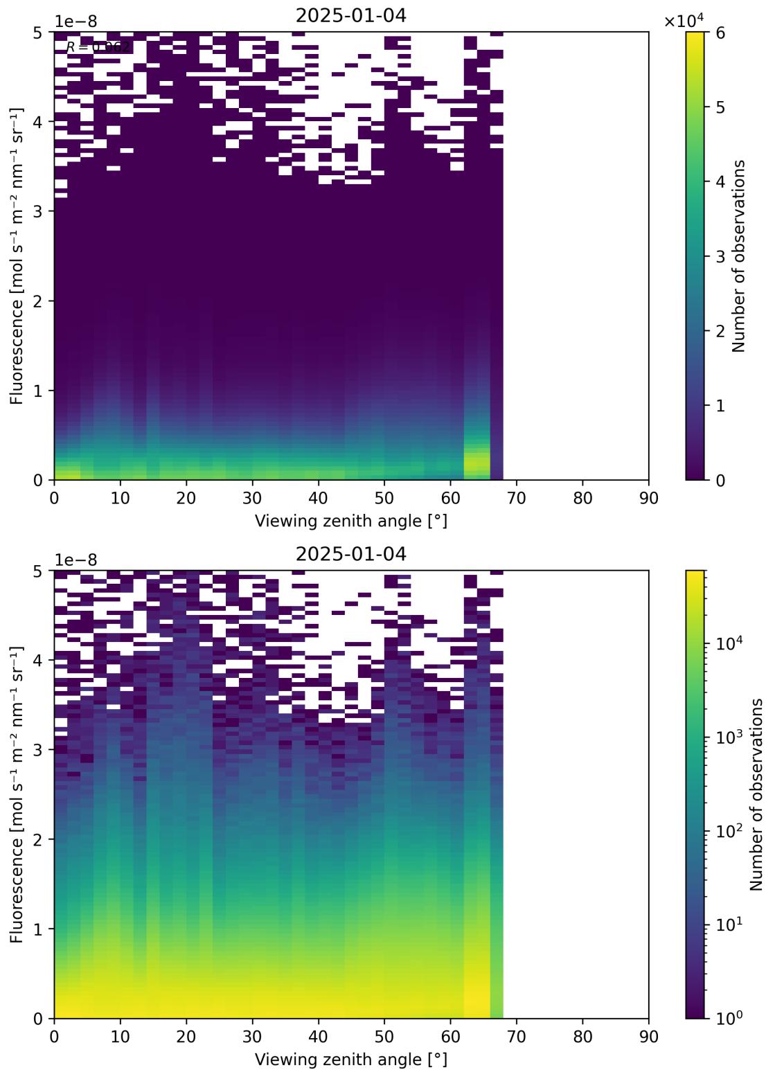
Figure 122: Scatter density plot of “Viewing zenith angle” against “Fluorescence” for 2025-01-03 to 2025-01-05.
