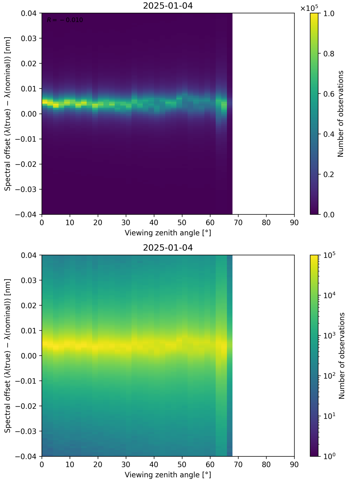
Figure 128: Scatter density plot of “Viewing zenith angle” against “Spectral offset ( \lambda_{\text{true}} - \lambda_{\text{nominal}} )” for 2025-01-03 to 2025-01-05.
