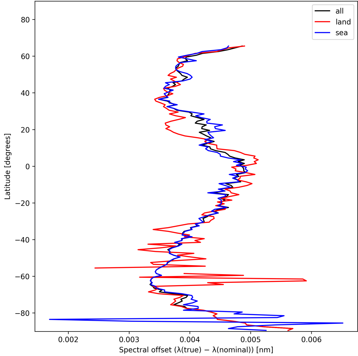
Figure 28: Zonal average of “Spectral offset ( \lambda_{\text{true}} - \lambda_{\text{nominal}} )” for 2025-01-03 to 2025-01-05.
