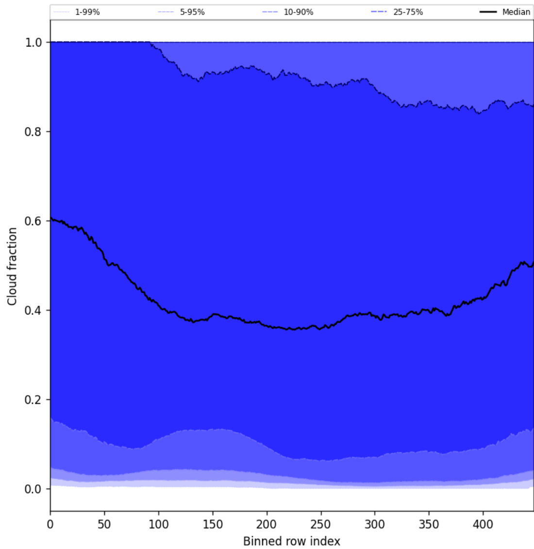
Figure 49: Along track statistics of “Cloud fraction” for 2025-01-03 to 2025-01-05
