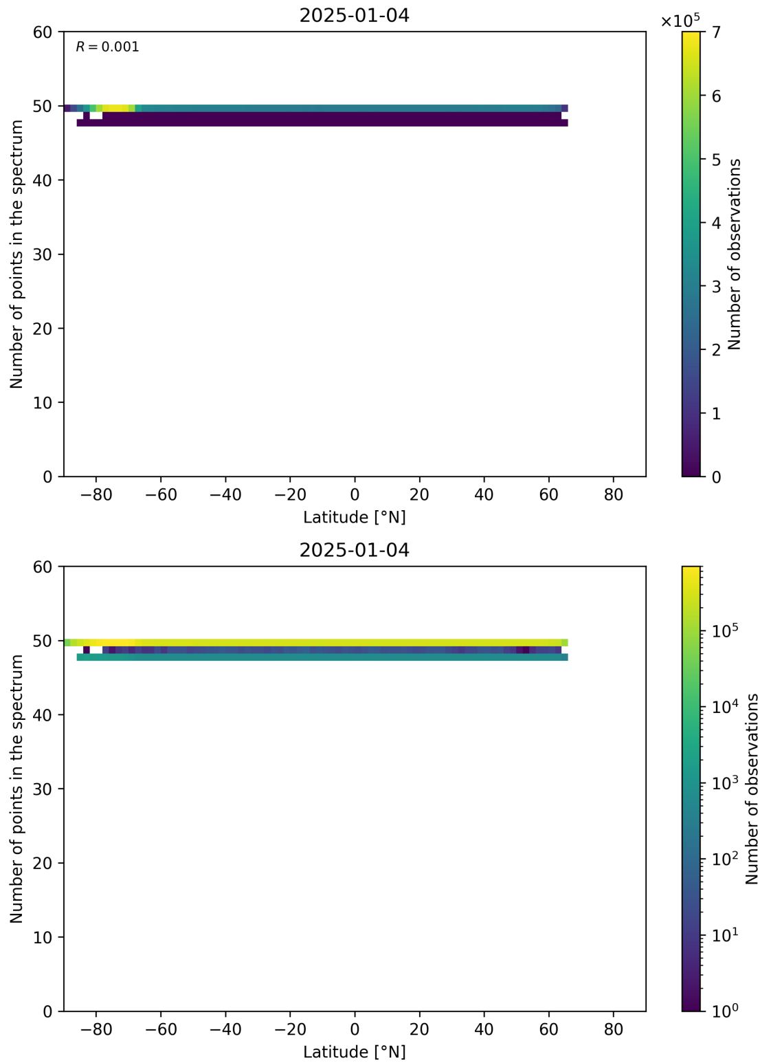
Figure 94: Scatter density plot of “Latitude” against “Number of points in the spectrum” for 2025-01-03 to 2025-01-05.
