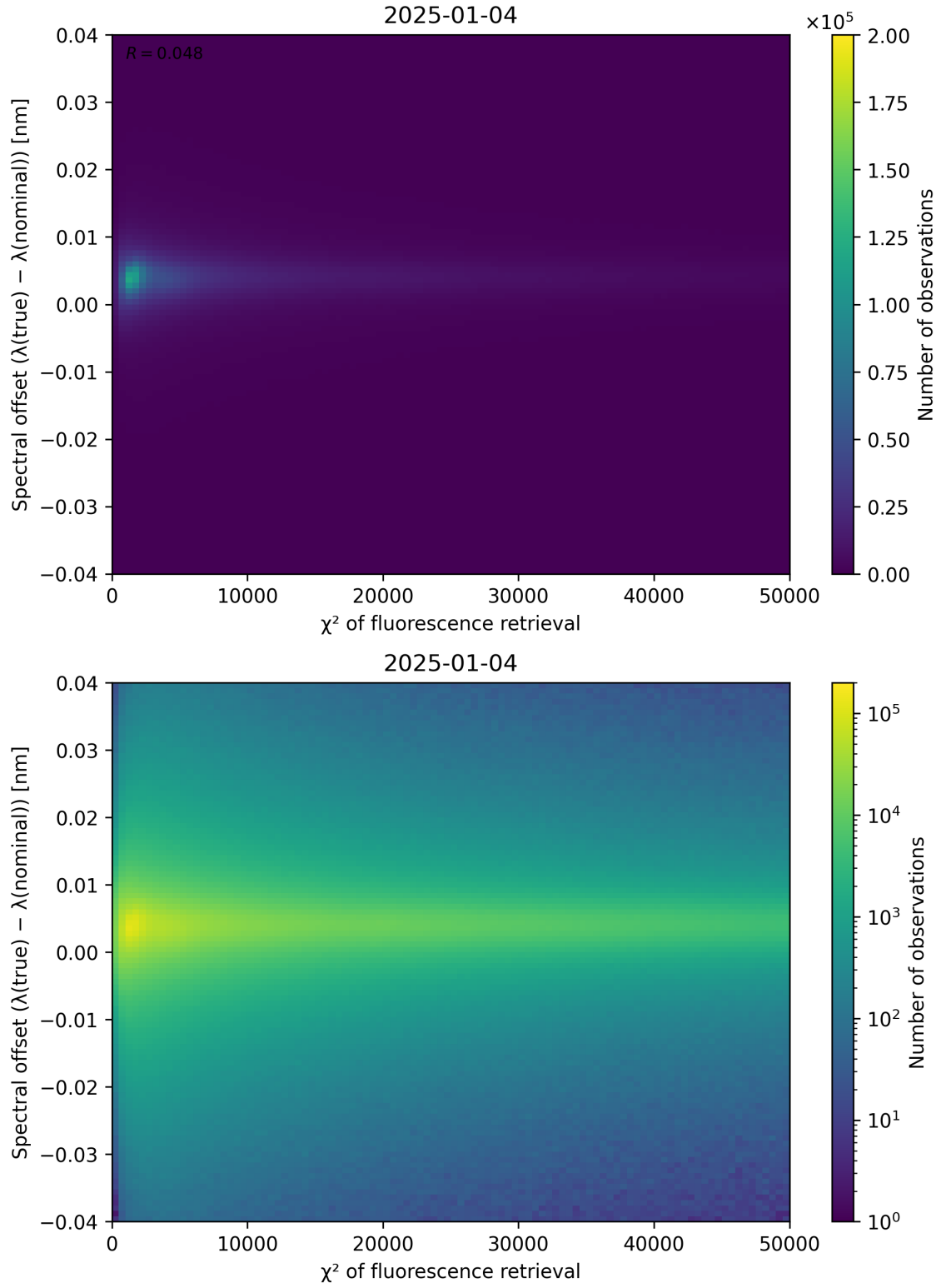
Figure 69: Scatter density plot of “ \chi^2 of fluorescence retrieval” against “Spectral offset ( \lambda_{\text{true}} - \lambda_{\text{nominal}} )” for 2025-01-03 to 2025-01-05.
