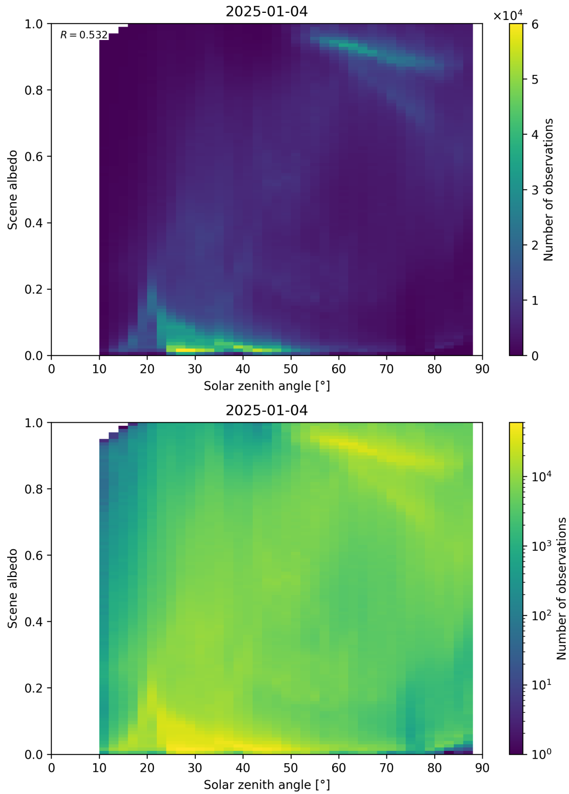
Figure 116: Scatter density plot of “Solar zenith angle” against “Scene albedo” for 2025-01-03 to 2025-01-05.
