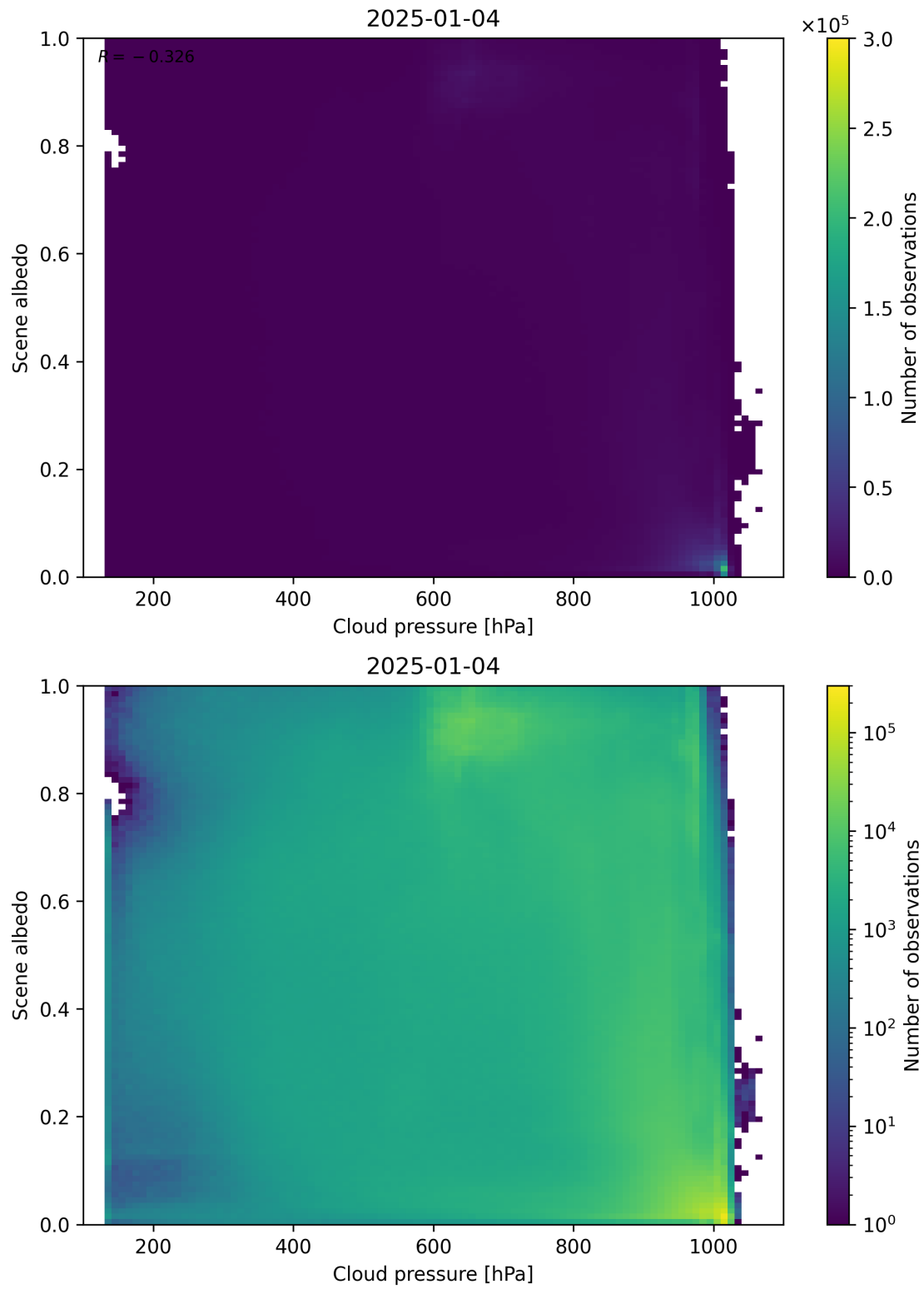
Figure 83: Scatter density plot of “Cloud pressure” against “Scene albedo” for 2025-01-03 to 2025-01-05.
