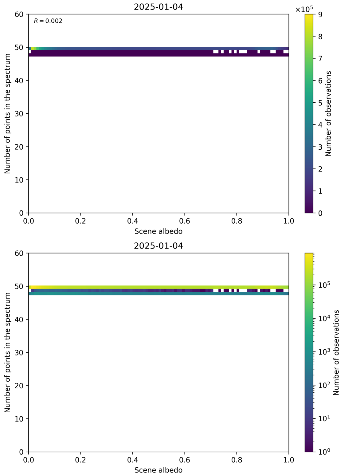
Figure 106: Scatter density plot of “Scene albedo” against “Number of points in the spectrum” for 2025-01-03 to 2025-01-05.
