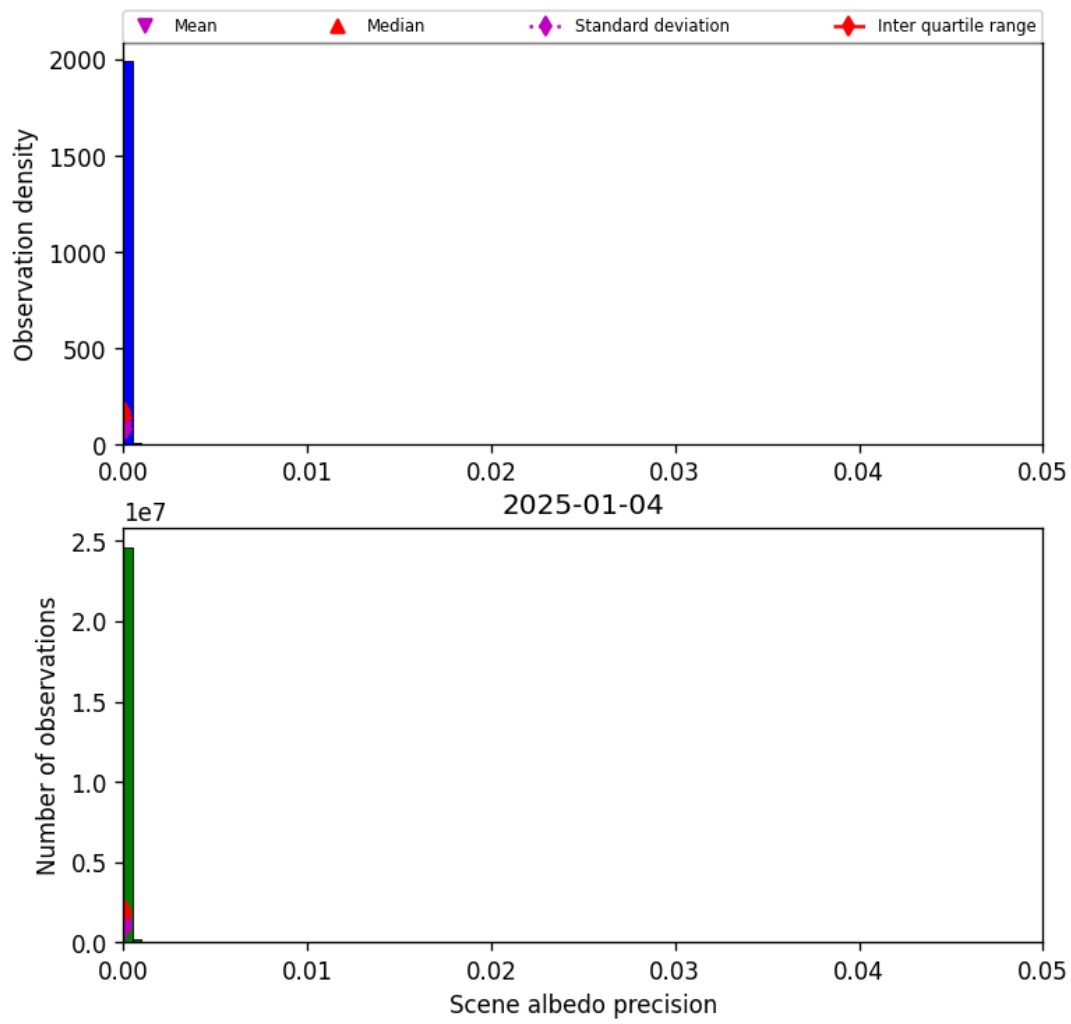
Figure 35: Histogram of “Scene albedo precision” for 2025-01-03 to 2025-01-05
