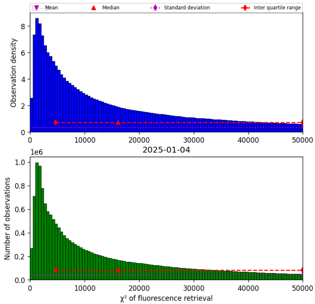
Figure 42: Histogram of “ \chi^2 of fluorescence retrieval” for 2025-01-03 to 2025-01-05
