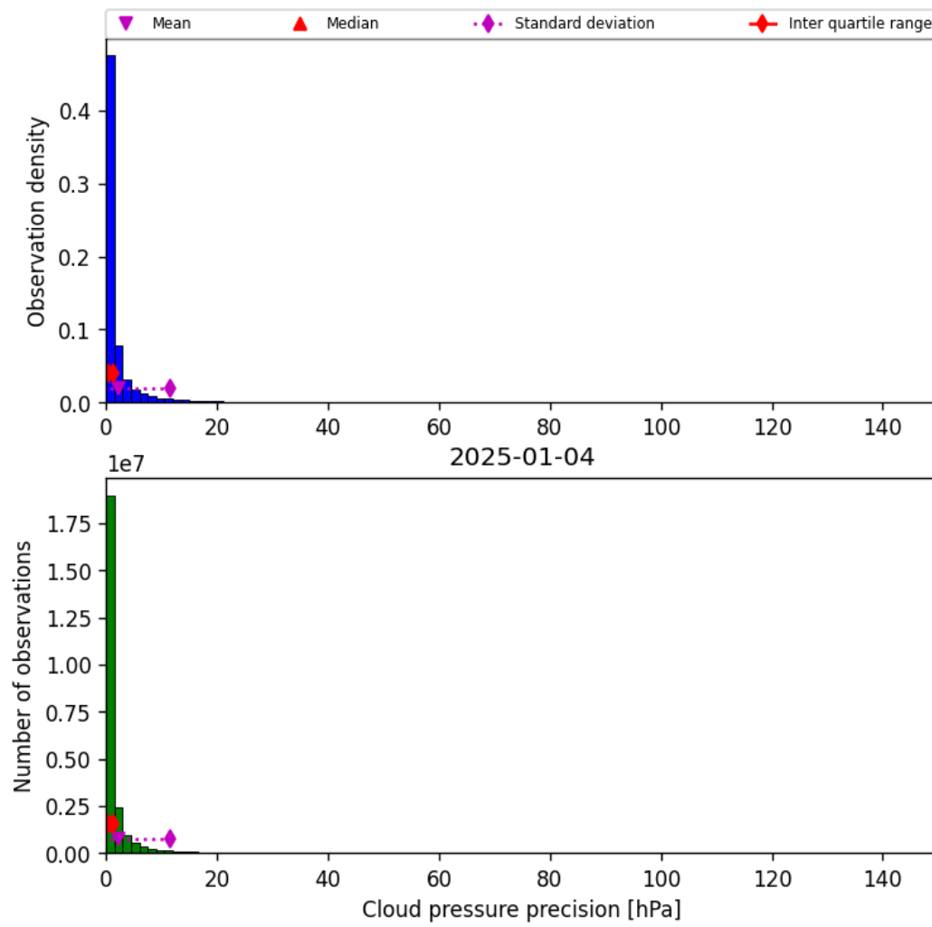
Figure 31: Histogram of “Cloud pressure precision” for 2025-01-03 to 2025-01-05
