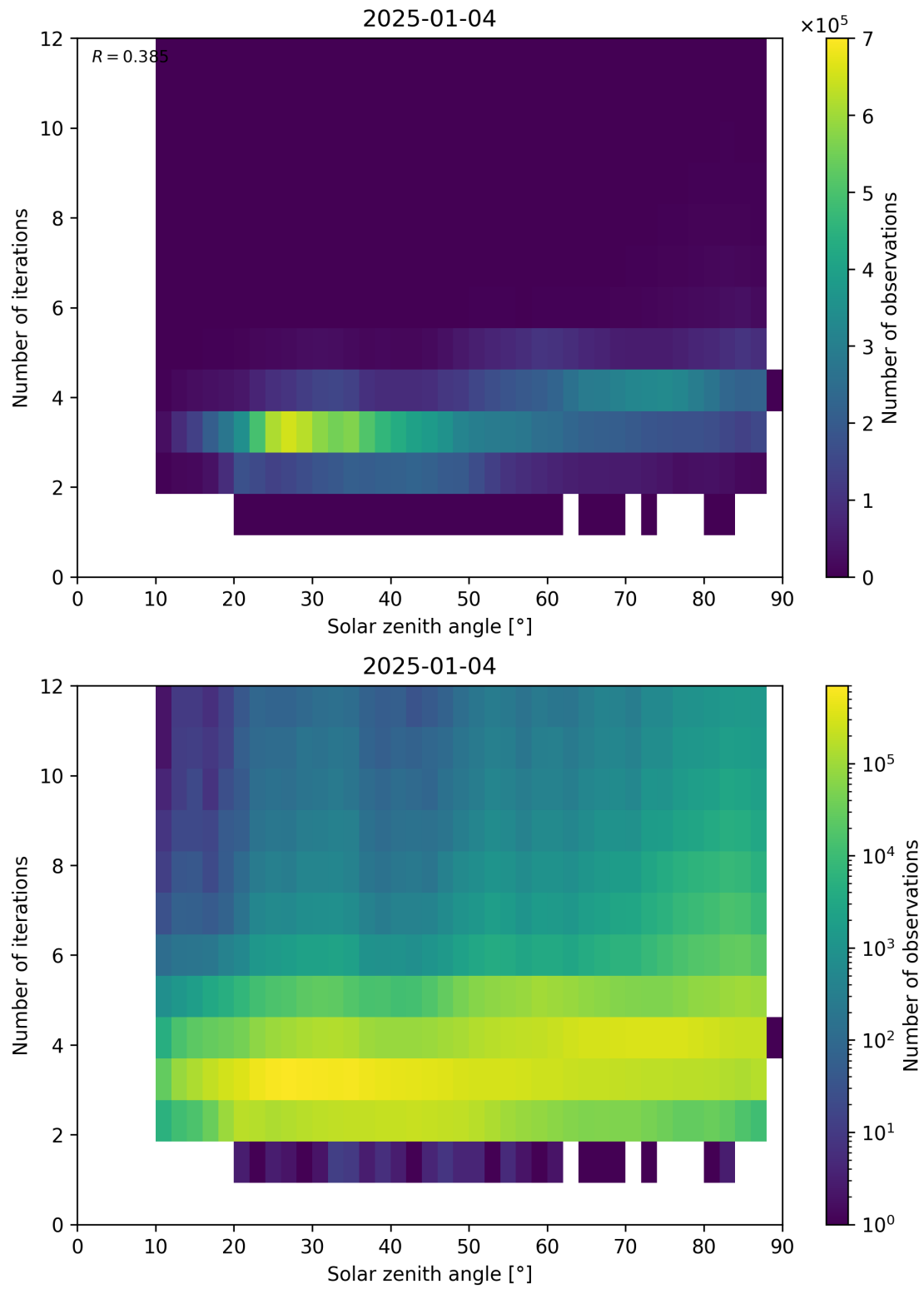
Figure 114: Scatter density plot of “Solar zenith angle” against “Number of iterations” for 2025-01-03 to 2025-01-05.
