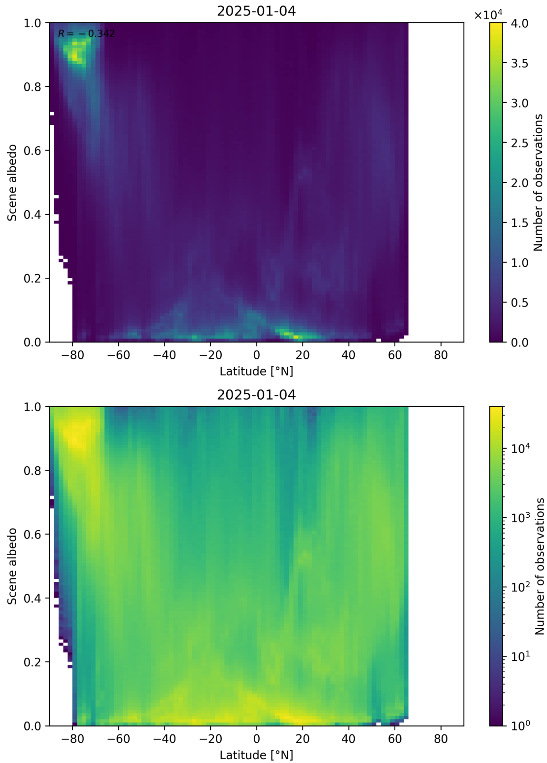
Figure 95: Scatter density plot of “Latitude” against “Scene albedo” for 2025-01-03 to 2025-01-05.
