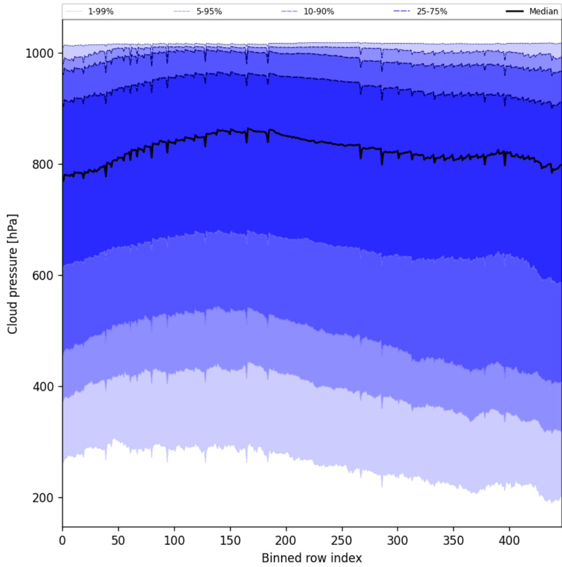
Figure 47: Along track statistics of “Cloud pressure” for 2025-01-03 to 2025-01-05
