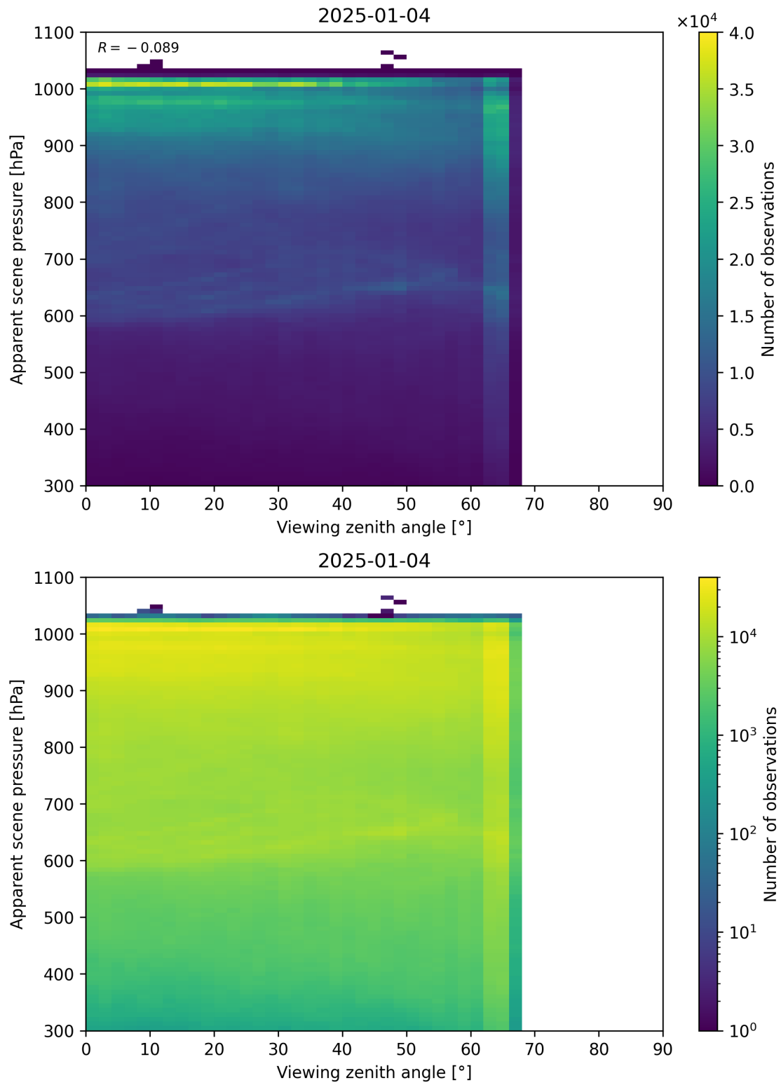
Figure 118: Scatter density plot of “Viewing zenith angle” against “Apparent scene pressure” for 2025-01-03 to 2025-01-05.
