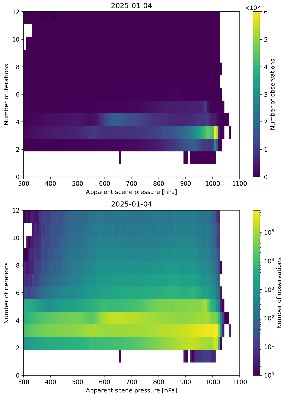
Figure 65: Scatter density plot of “Apparent scene pressure” against “Number of iterations” for 2025-01-03 to 2025-01-05.
