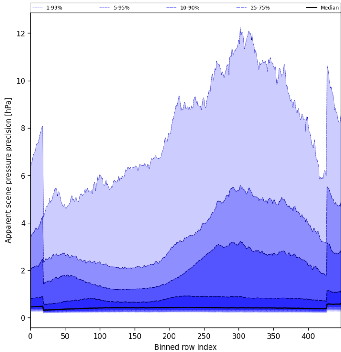
Figure 54: Along track statistics of “Apparent scene pressure precision” for 2025-01-03 to 2025-01-05
