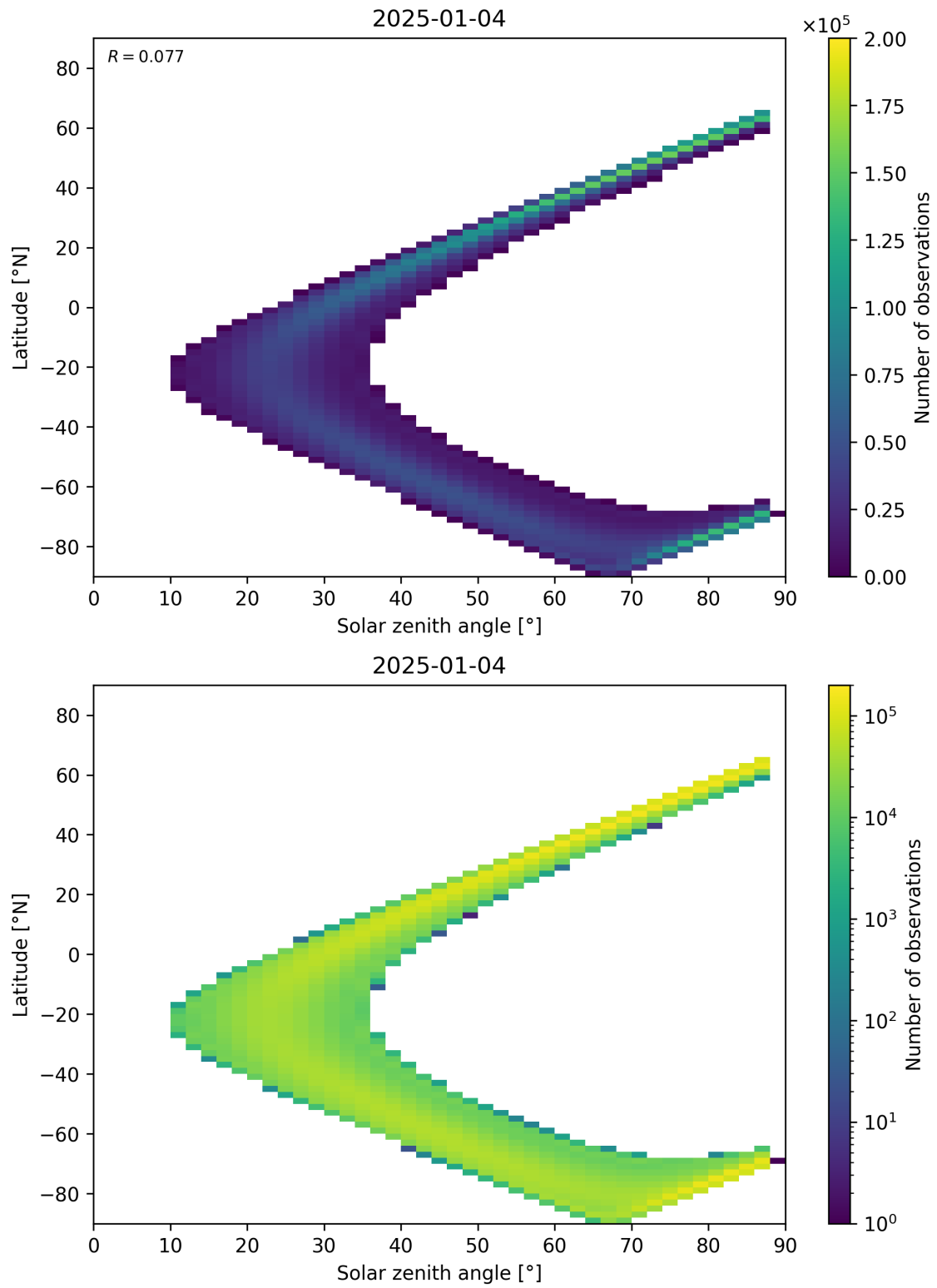
Figure 113: Scatter density plot of “Solar zenith angle” against “Latitude” for 2025-01-03 to 2025-01-05.
