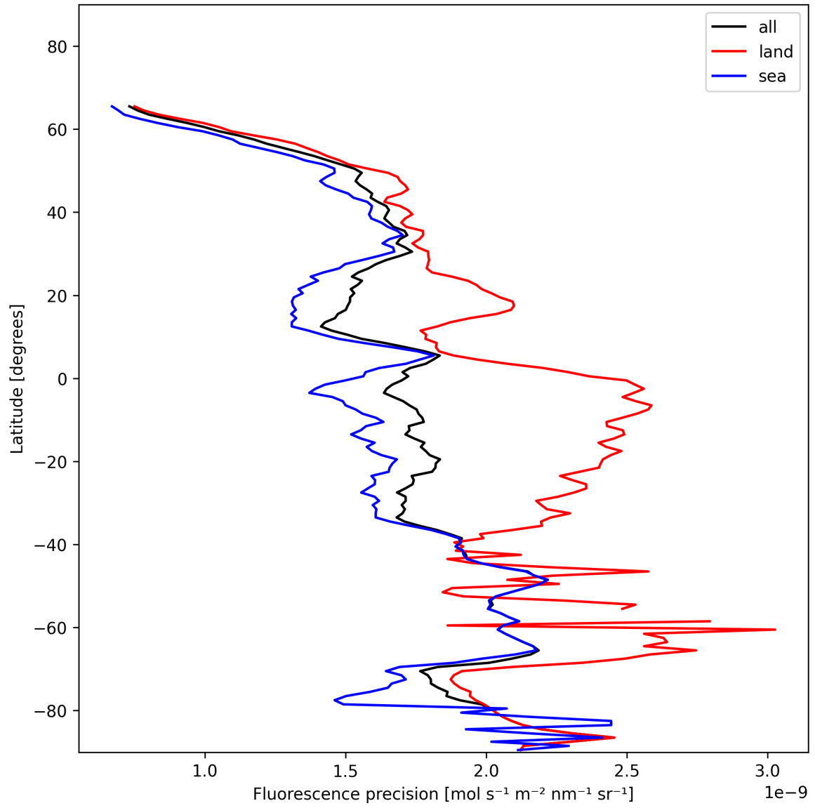
Figure 24: Zonal average of “Fluorescence precision” for 2025-01-03 to 2025-01-05.
