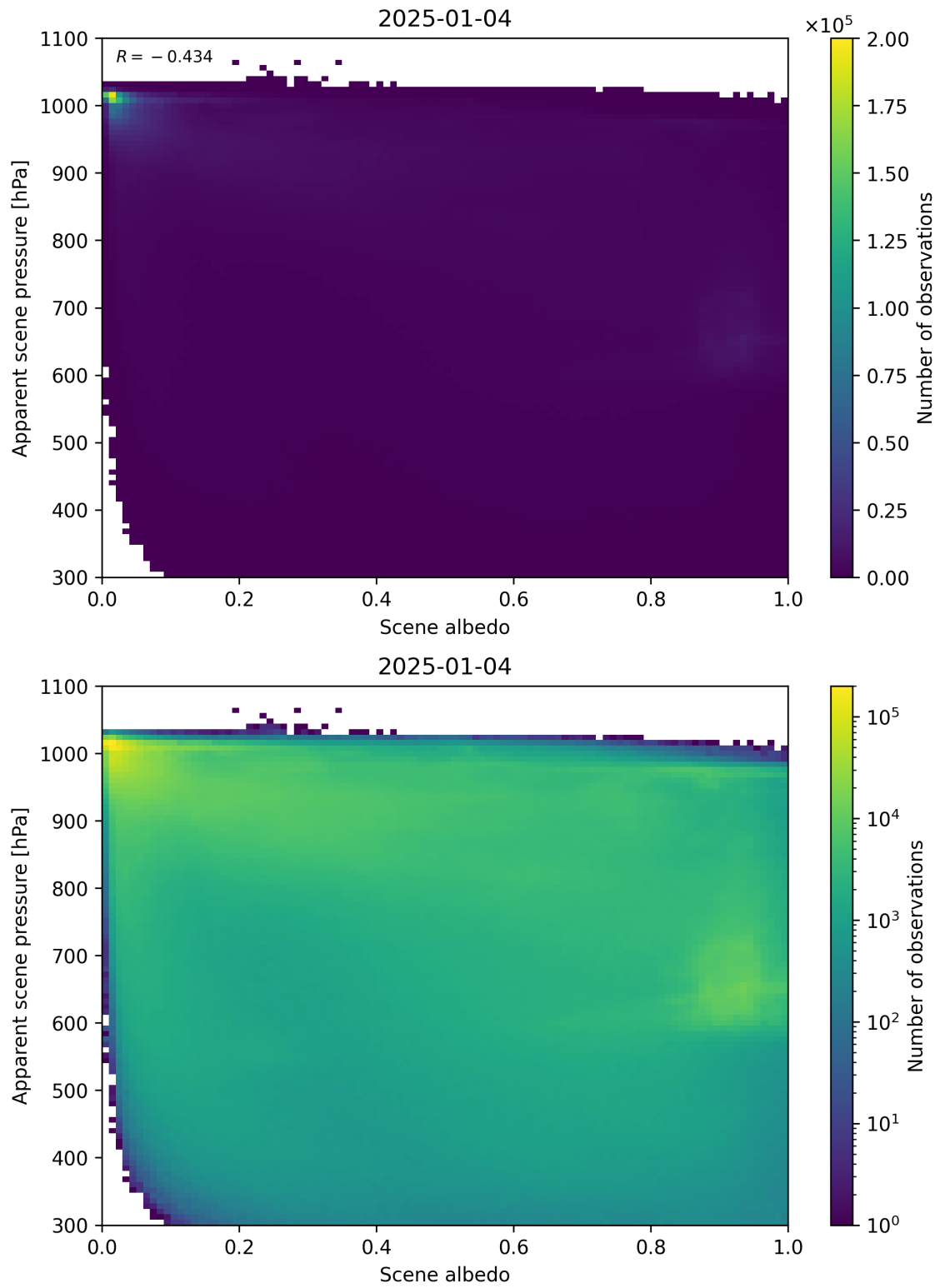
Figure 102: Scatter density plot of “Scene albedo” against “Apparent scene pressure” for 2025-01-03 to 2025-01-05.
