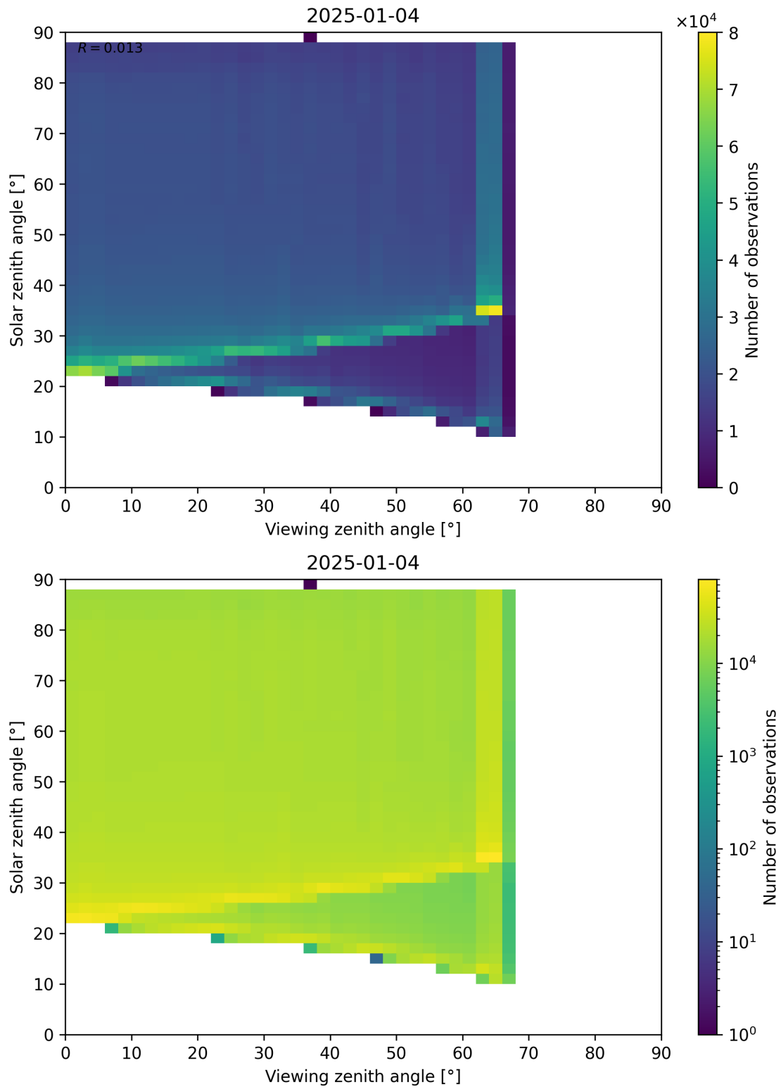
Figure 127: Scatter density plot of “Viewing zenith angle” against “Solar zenith angle” for 2025-01-03 to 2025-01-05.
