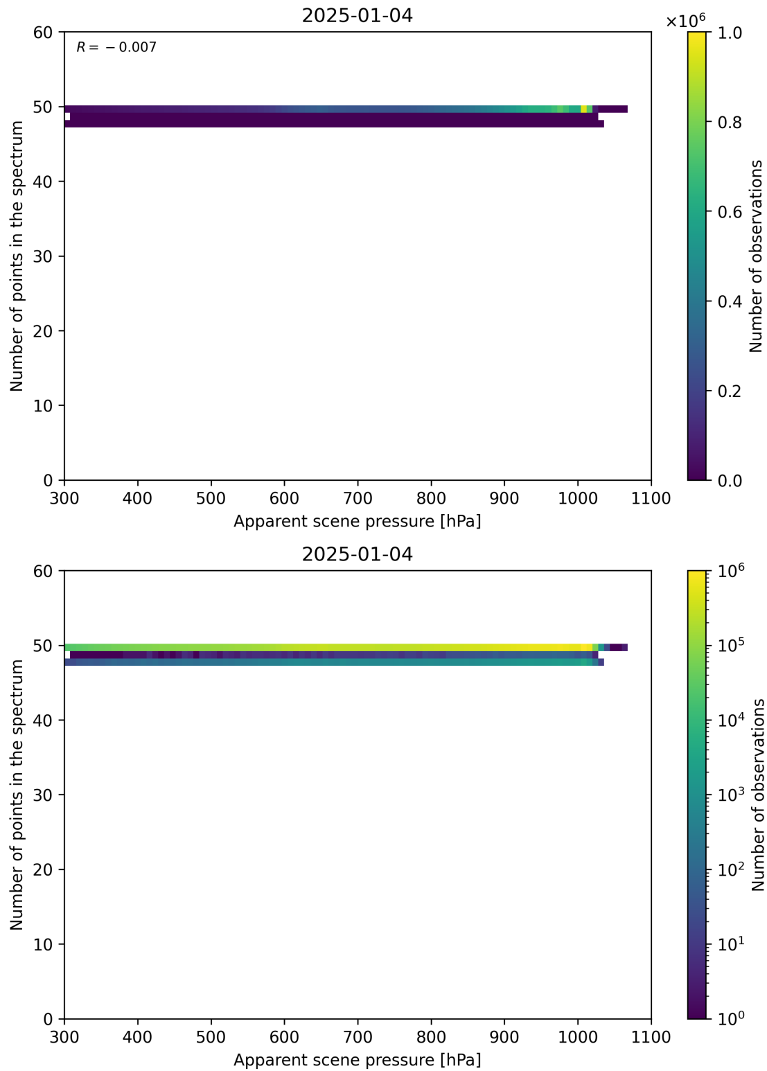
Figure 66: Scatter density plot of “Apparent scene pressure” against “Number of points in the spectrum” for 2025-01-03 to 2025-01-05.
