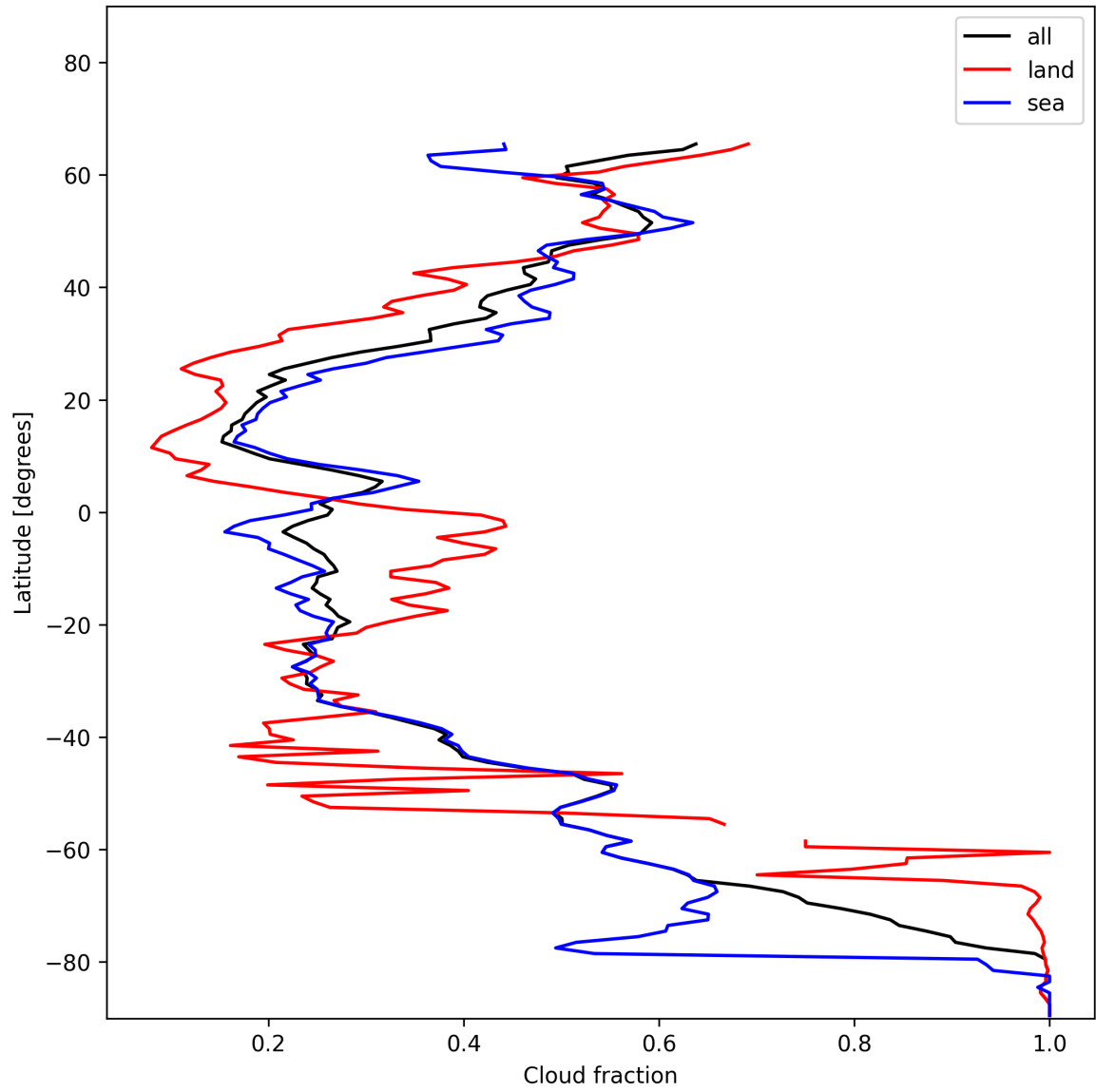
Figure 15: Zonal average of “Cloud fraction” for 2025-01-03 to 2025-01-05.
