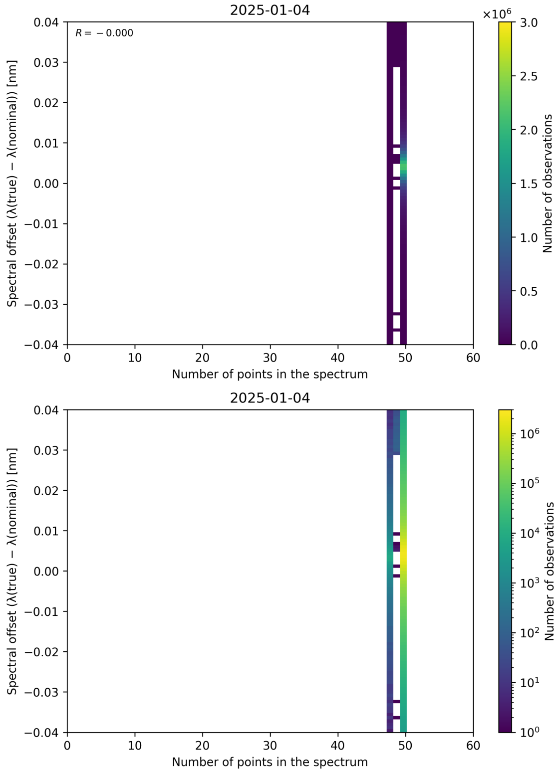
Figure 101: Scatter density plot of “Number of points in the spectrum” against “Spectral offset ( \lambda_{\text{true}} - \lambda_{\text{nominal}} )” for 2025-01-03 to 2025-01-05.
