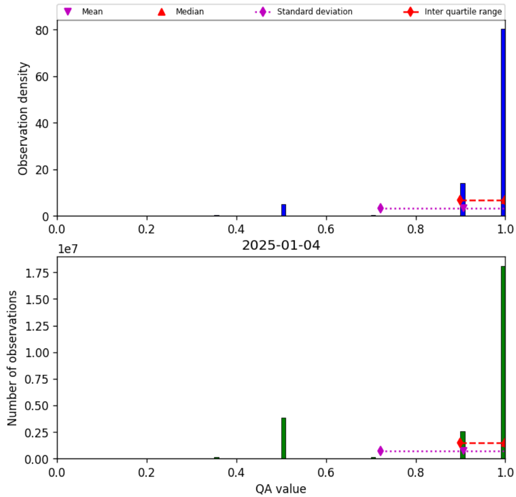
Figure 29: Histogram of “QA value” for 2025-01-03 to 2025-01-05
