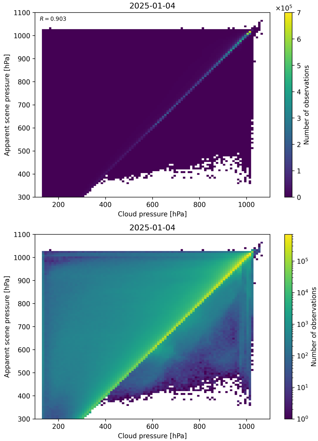
Figure 77: Scatter density plot of “Cloud pressure” against “Apparent scene pressure” for 2025-01-03 to 2025-01-05.
