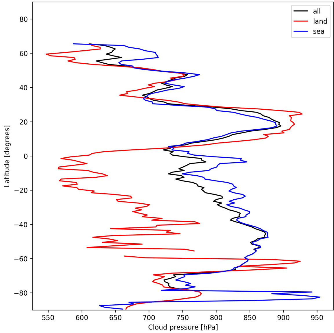
Figure 13: Zonal average of “Cloud pressure” for 2025-01-03 to 2025-01-05.
