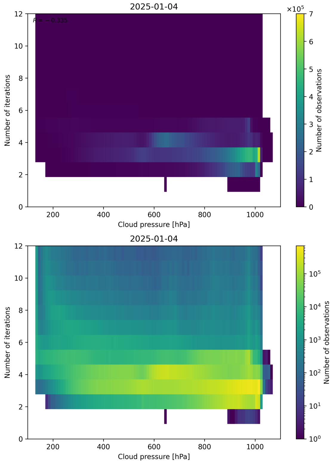
Figure 81: Scatter density plot of “Cloud pressure” against “Number of iterations” for 2025-01-03 to 2025-01-05.
