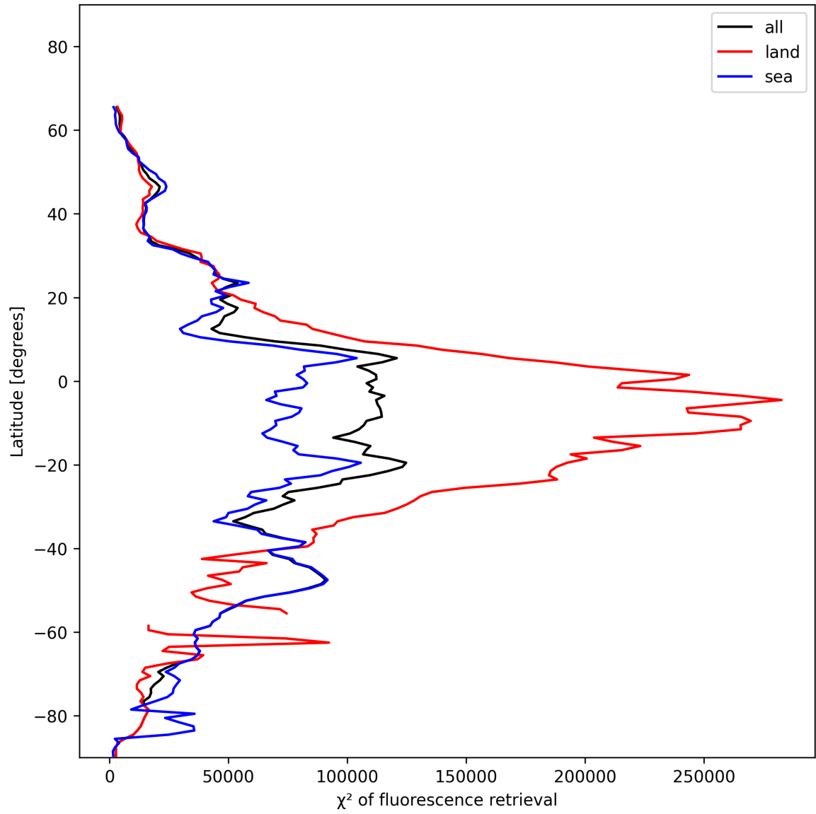
Figure 25: Zonal average of “ \chi^2 of fluorescence retrieval” for 2025-01-03 to 2025-01-05.
