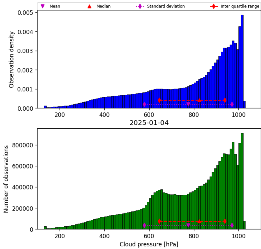
Figure 30: Histogram of “Cloud pressure” for 2025-01-03 to 2025-01-05
