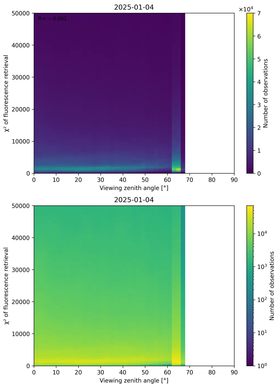
Figure 119: Scatter density plot of “Viewing zenith angle” against “ \chi^2 of fluorescence retrieval” for 2025-01-03 to 2025-01-05.
