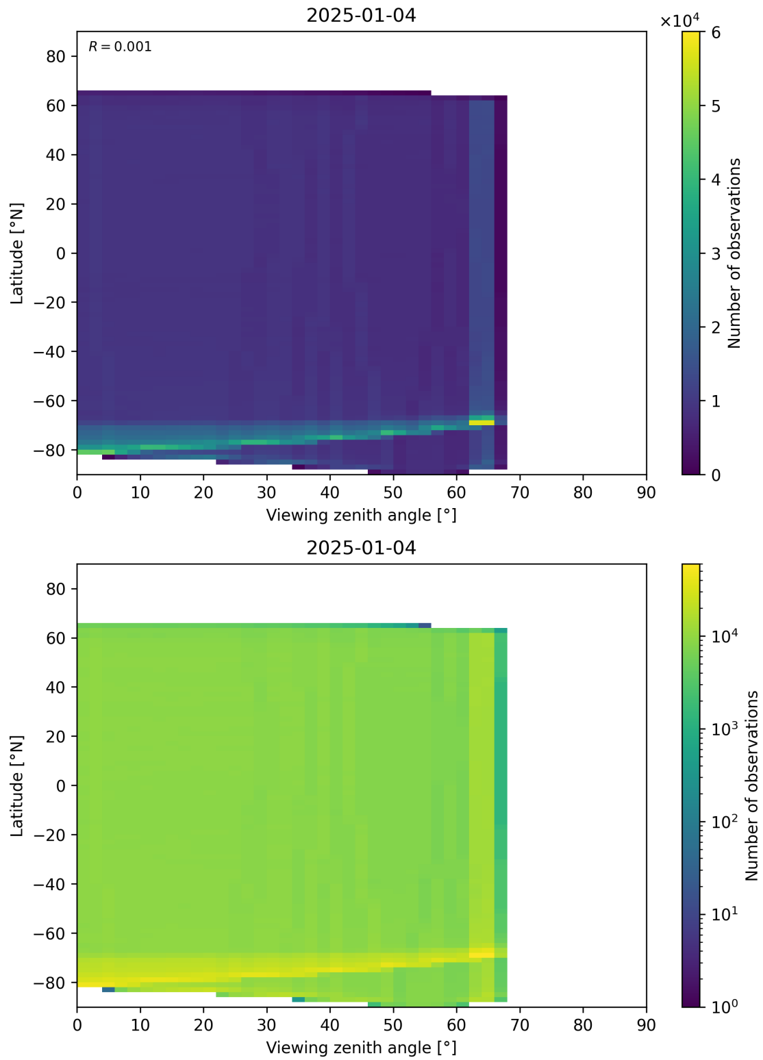
Figure 123: Scatter density plot of “Viewing zenith angle” against “Latitude” for 2025-01-03 to 2025-01-05.
