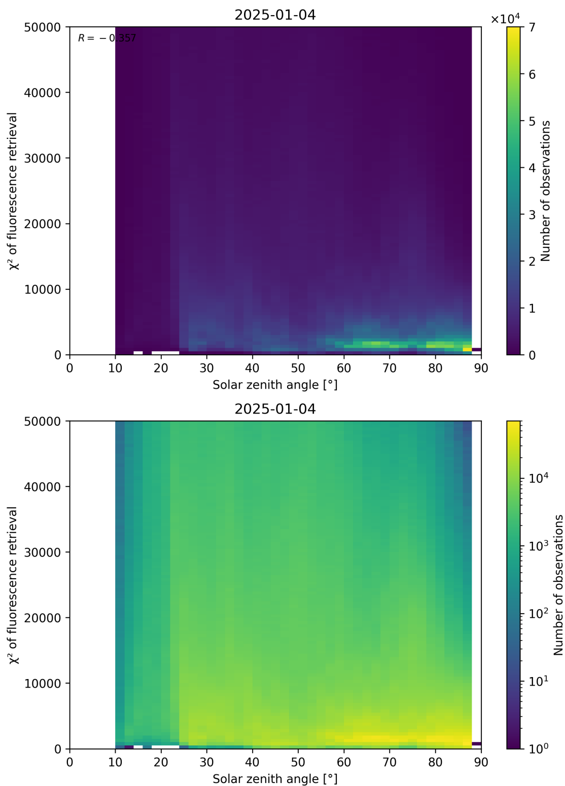
Figure 109: Scatter density plot of “Solar zenith angle” against “ \chi^2 of fluorescence retrieval” for 2025-01-03 to 2025-01-05.
