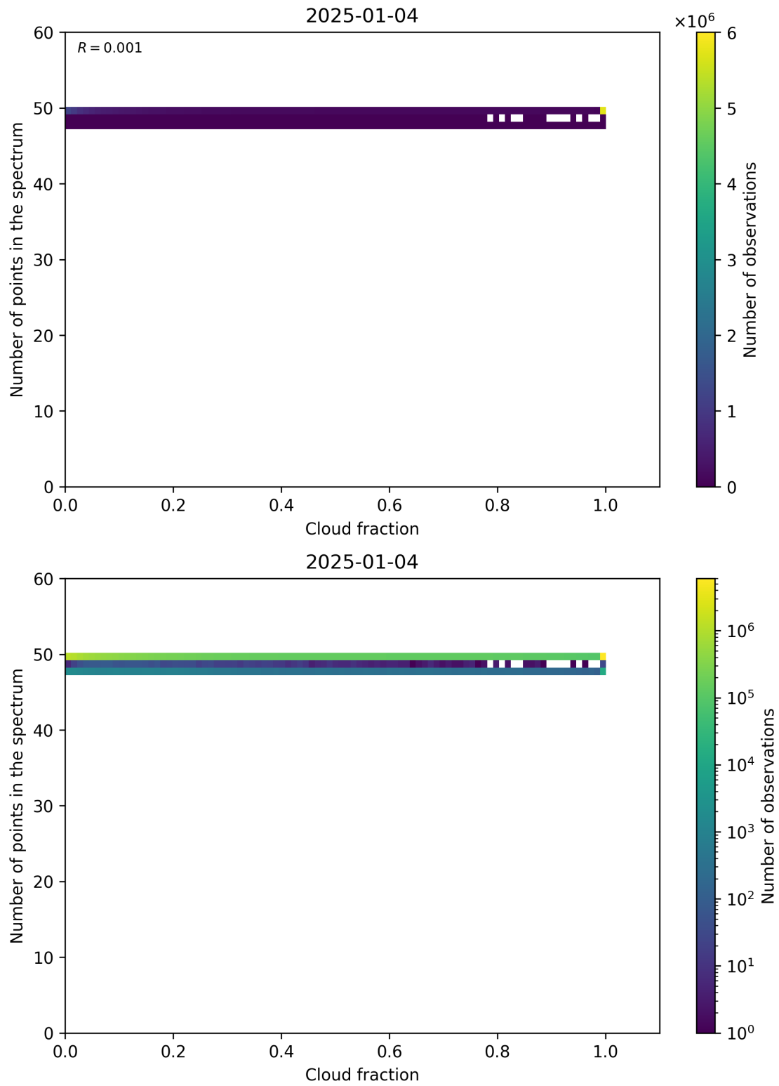
Figure 74: Scatter density plot of “Cloud fraction” against “Number of points in the spectrum” for 2025-01-03 to 2025-01-05.
