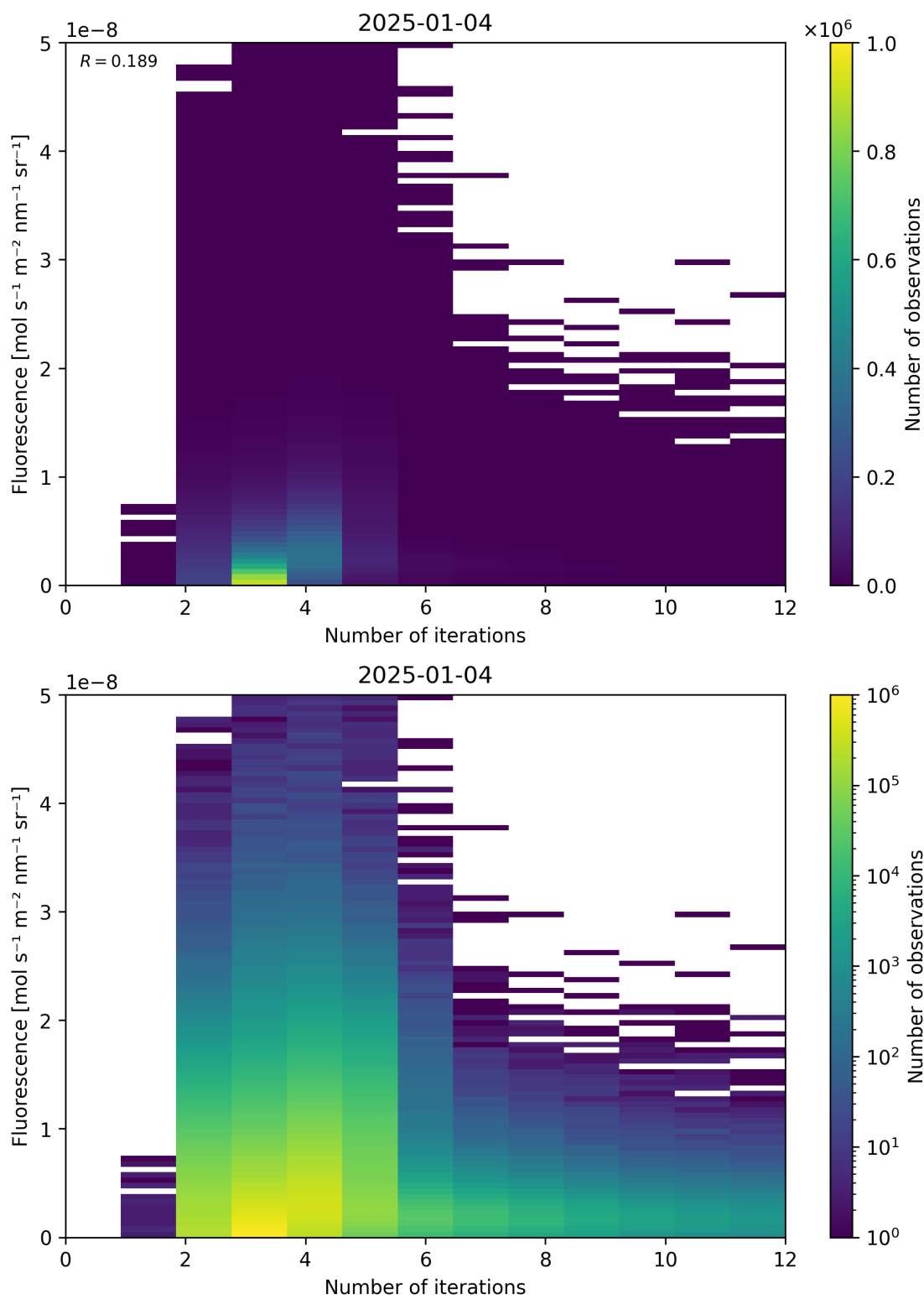
Figure 98: Scatter density plot of “Number of iterations” against “Fluorescence” for 2025-01-03 to 2025-01-05.
