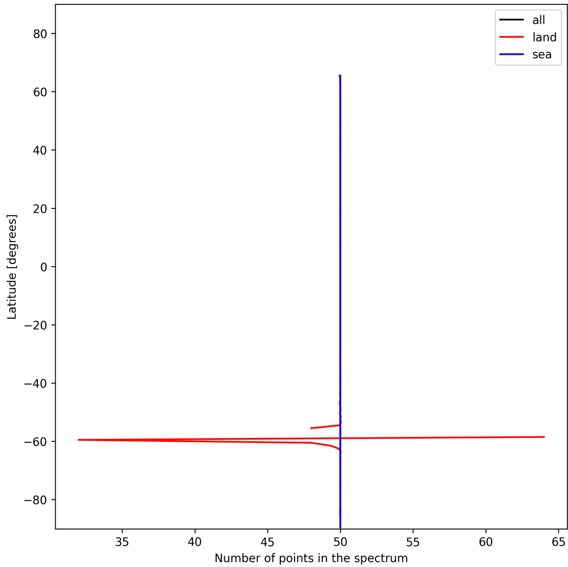
Figure 27: Zonal average of “Number of points in the spectrum” for 2025-01-03 to 2025-01-05.
