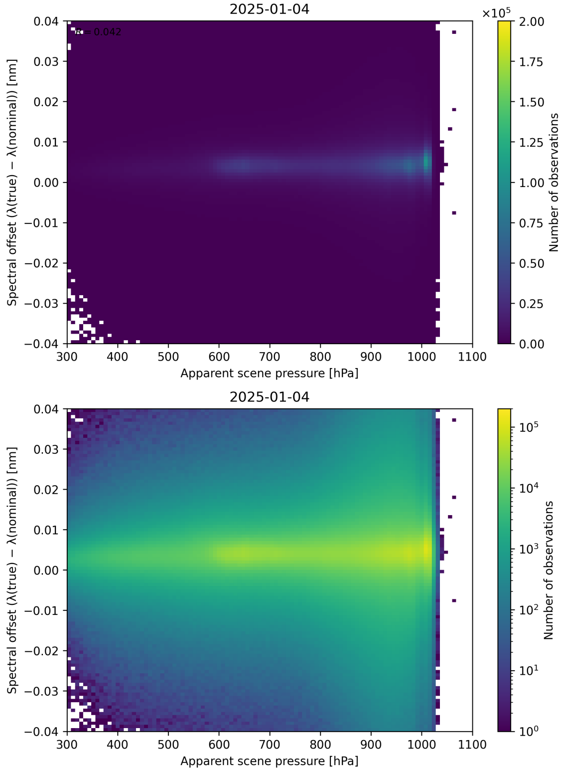
Figure 67: Scatter density plot of “Apparent scene pressure” against “Spectral offset ( \lambda_{\text{true}} - \lambda_{\text{nominal}} )” for 2025-01-03 to 2025-01-05.
