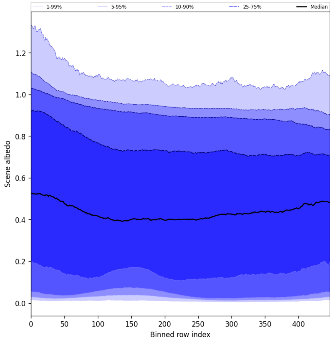
Figure 51: Along track statistics of “Scene albedo” for 2025-01-03 to 2025-01-05
