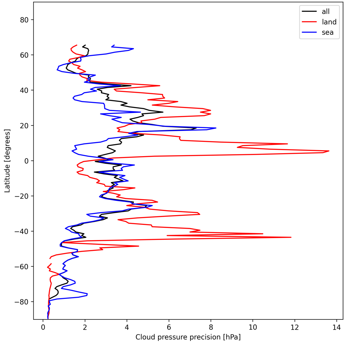
Figure 14: Zonal average of "Cloud pressure precision" for 2025-01-03 to 2025-01-05.
