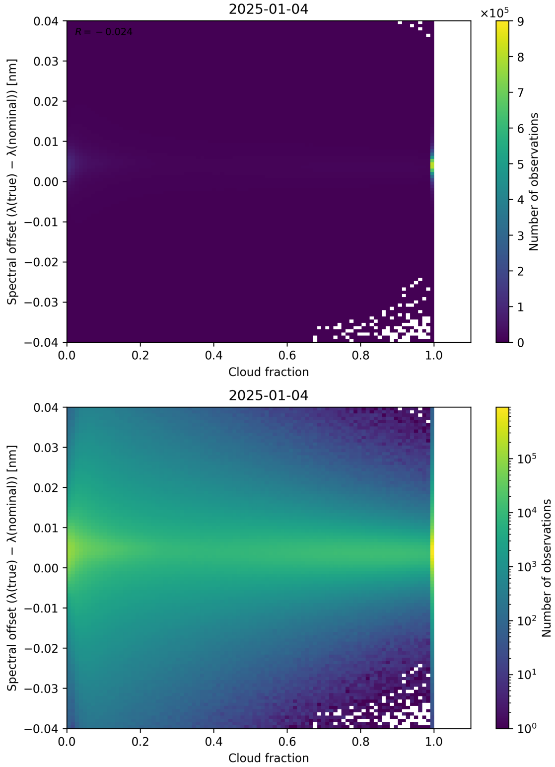
Figure 76: Scatter density plot of “Cloud fraction” against “Spectral offset ( \lambda_{\text{true}} - \lambda_{\text{nominal}} )” for 2025-01-03 to 2025-01-05.
