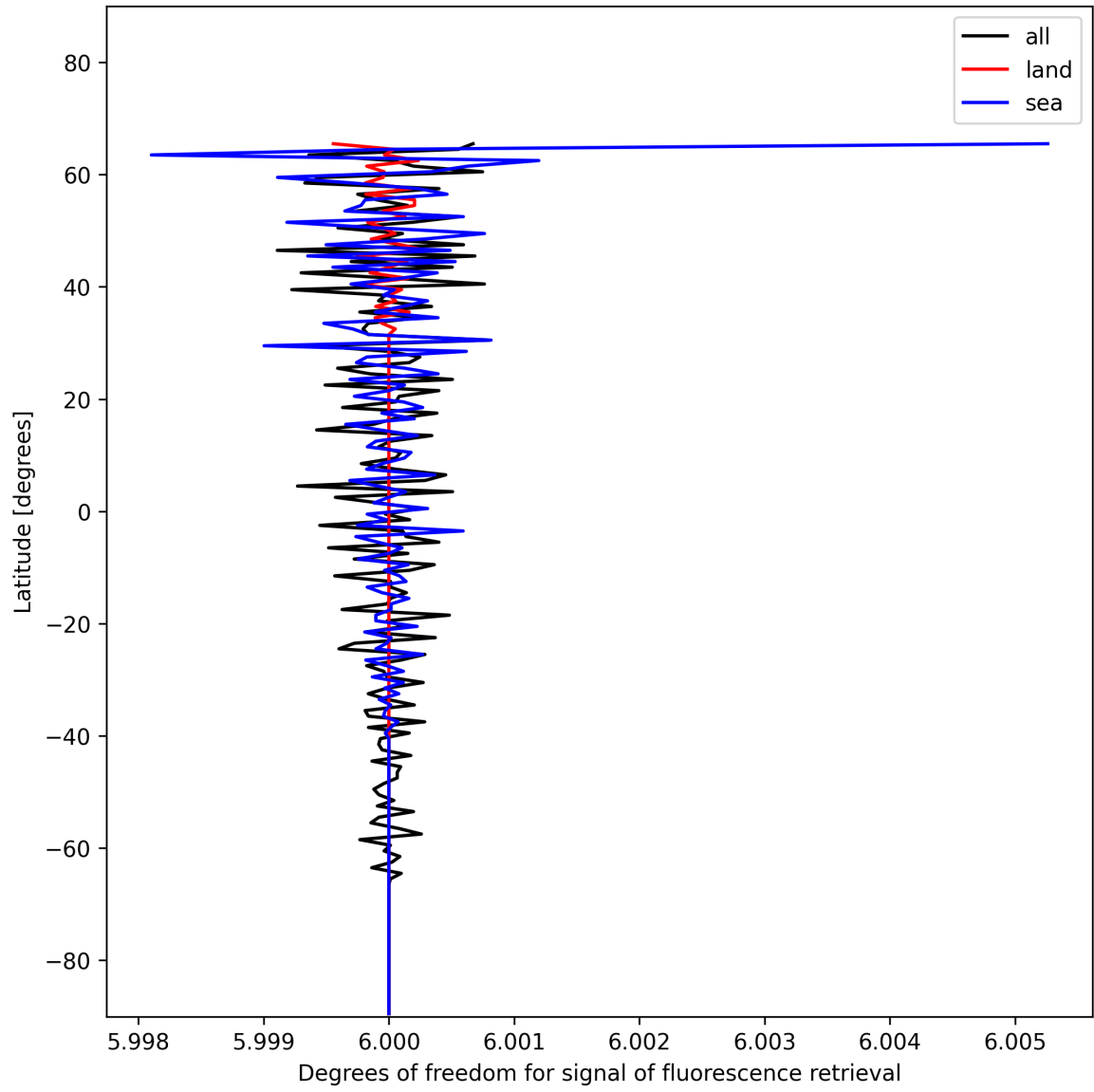
Figure 26: Zonal average of “Degrees of freedom for signal of fluorescence retrieval” for 2025-01-03 to 2025-01-05.
