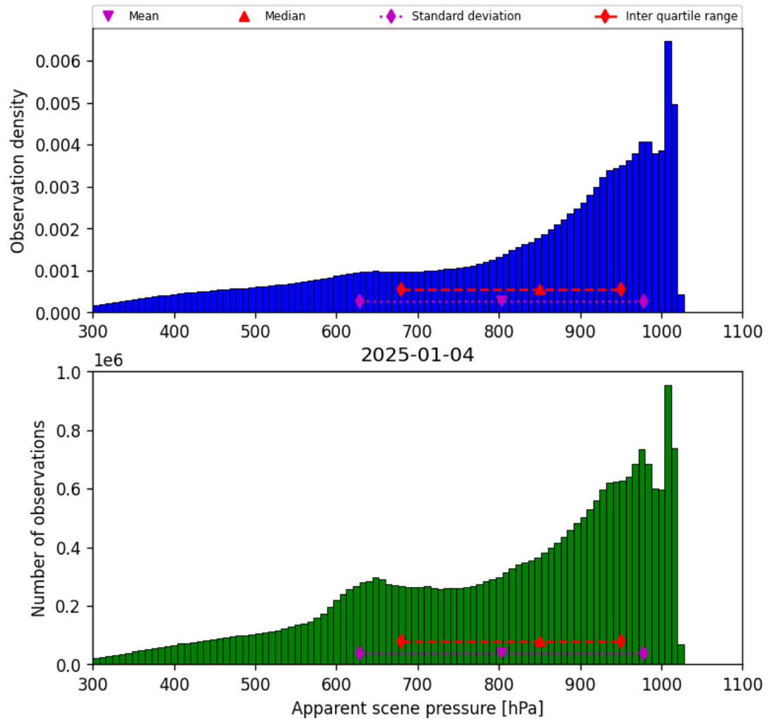
Figure 36: Histogram of “Apparent scene pressure” for 2025-01-03 to 2025-01-05
