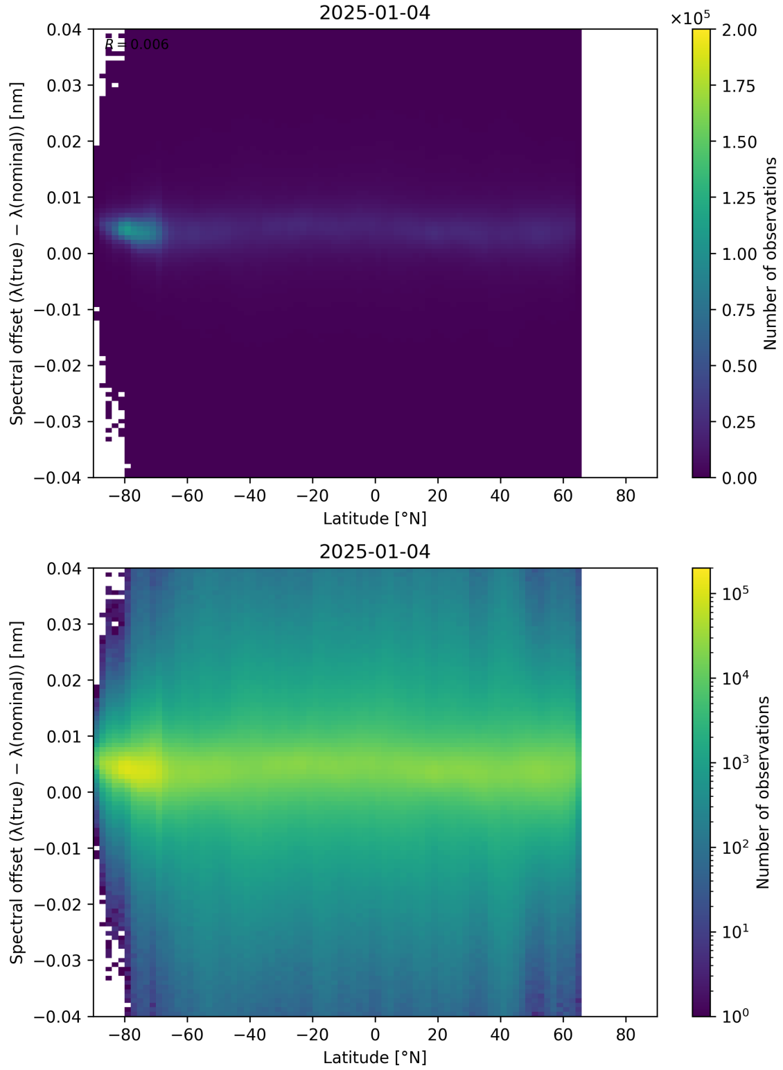
Figure 96: Scatter density plot of “Latitude” against “Spectral offset ( \lambda_{\text{true}} - \lambda_{\text{nominal}} )” for 2025-01-03 to 2025-01-05.
