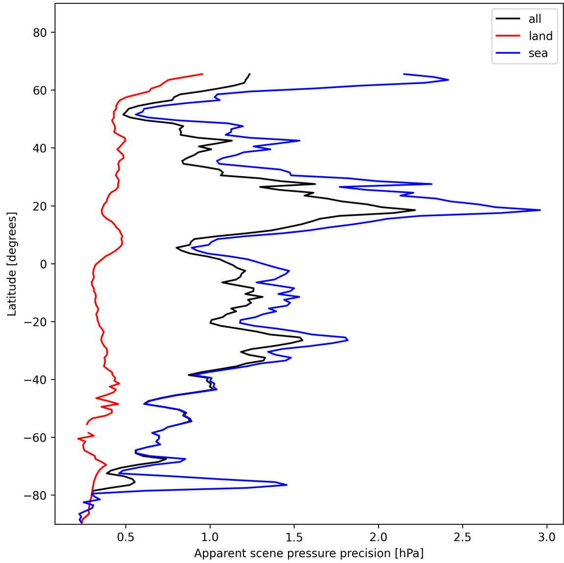
Figure 20: Zonal average of “Apparent scene pressure precision” for 2025-01-03 to 2025-01-05.
