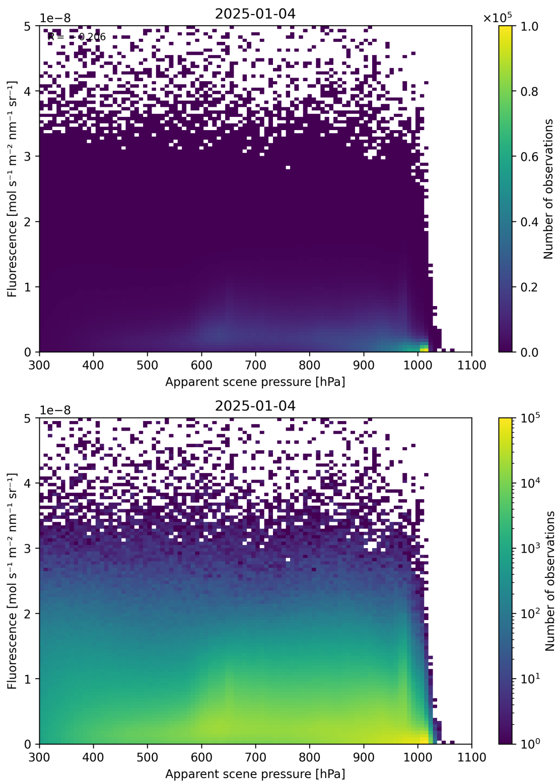
Figure 64: Scatter density plot of “Apparent scene pressure” against “Fluorescence” for 2025-01-03 to 2025-01-05.
