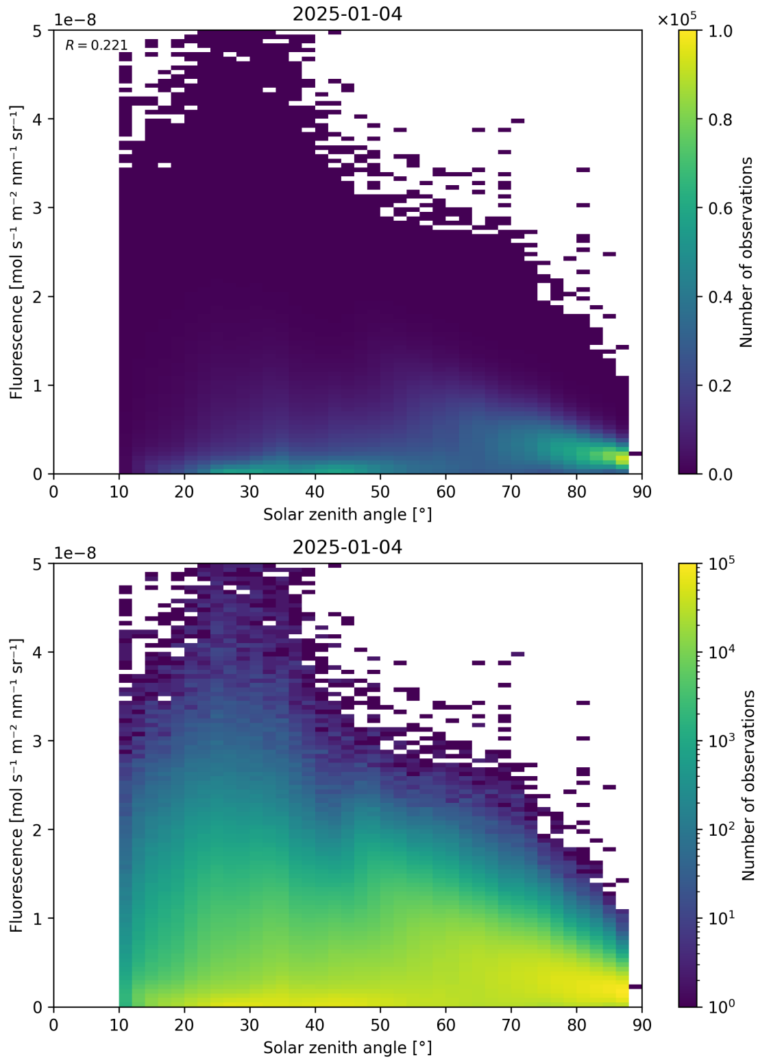
Figure 112: Scatter density plot of “Solar zenith angle” against “Fluorescence” for 2025-01-03 to 2025-01-05.
