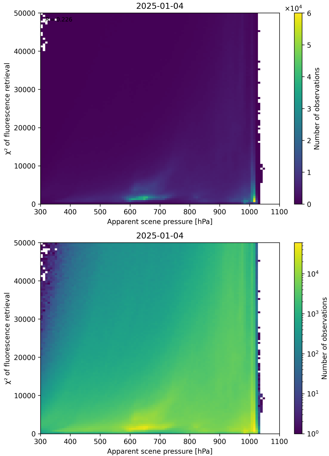
Figure 63: Scatter density plot of “Apparent scene pressure” against “ \chi^2 of fluorescence retrieval” for 2025-01-03 to 2025-01-05.
