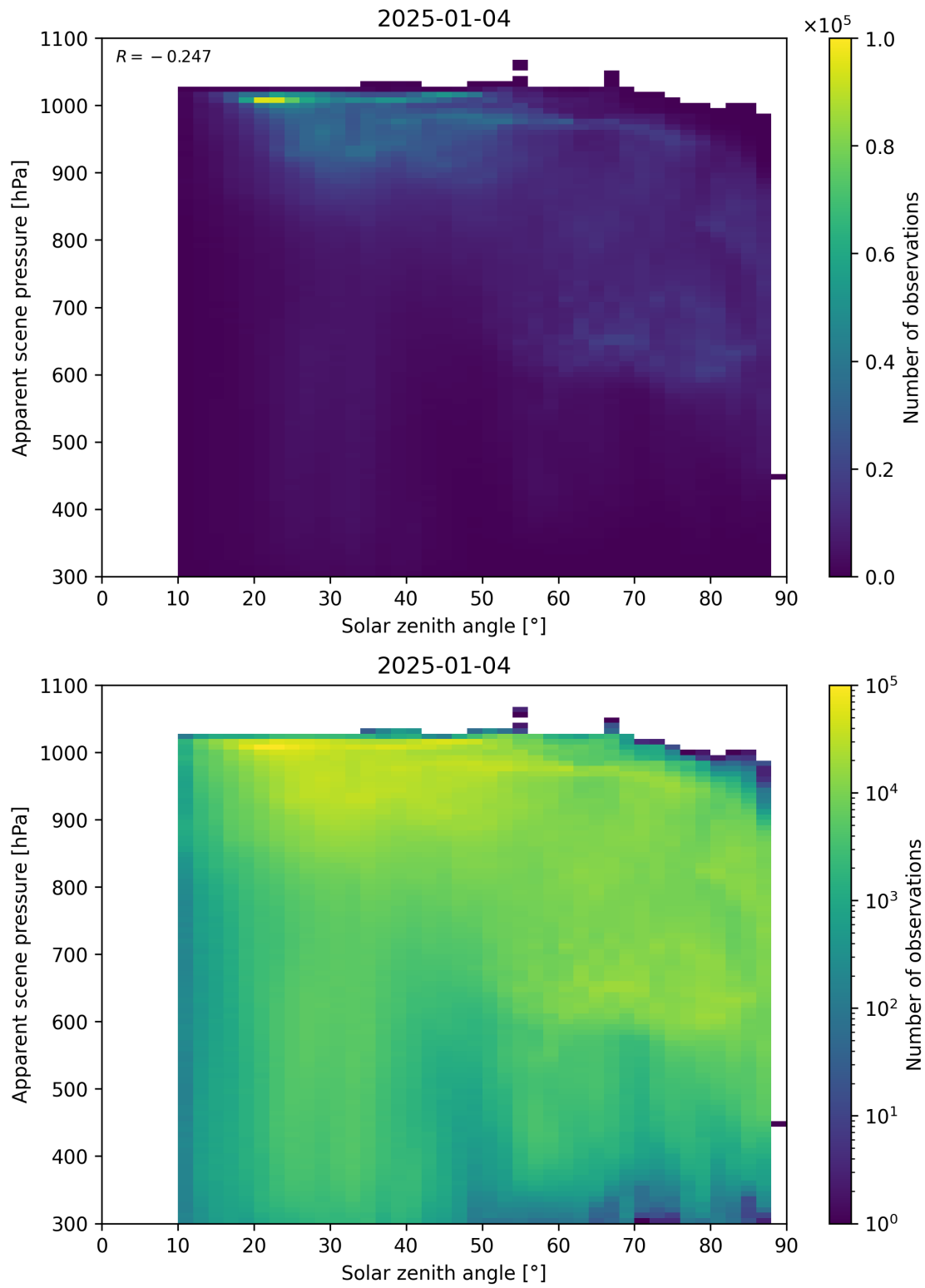
Figure 108: Scatter density plot of “Solar zenith angle” against “Apparent scene pressure” for 2025-01-03 to 2025-01-05.
