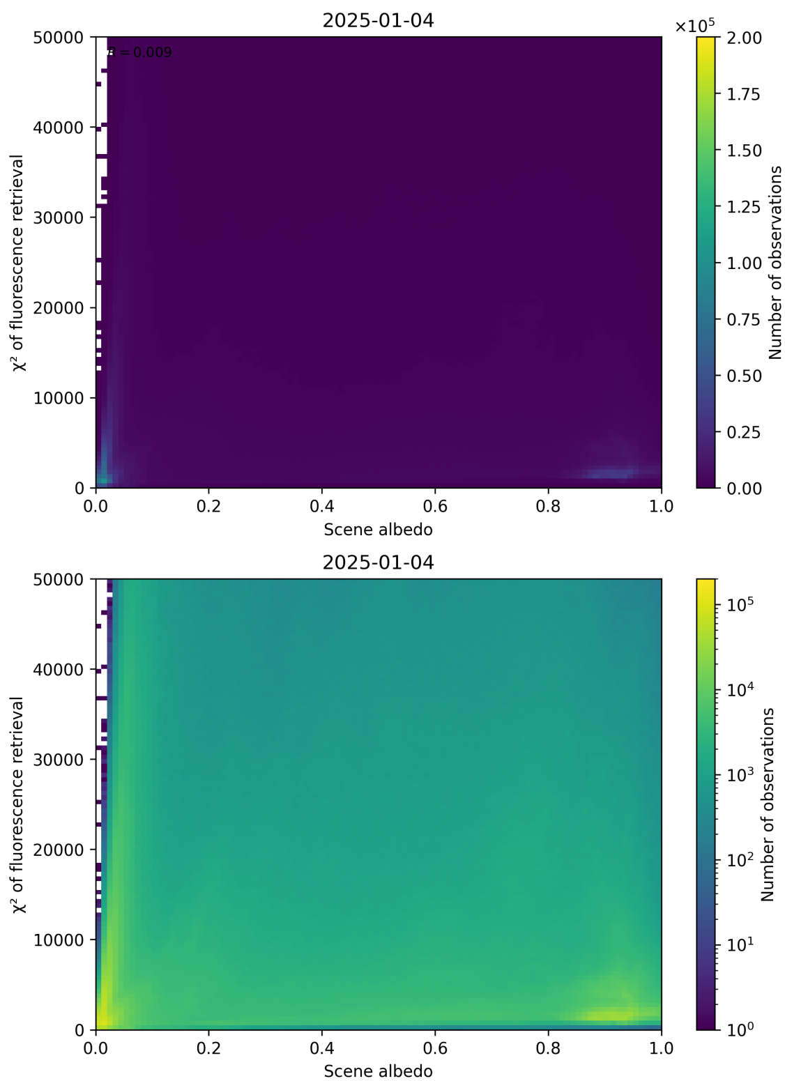
Figure 103: Scatter density plot of “Scene albedo” against “ \chi^2 of fluorescence retrieval” for 2025-01-03 to 2025-01-05.
