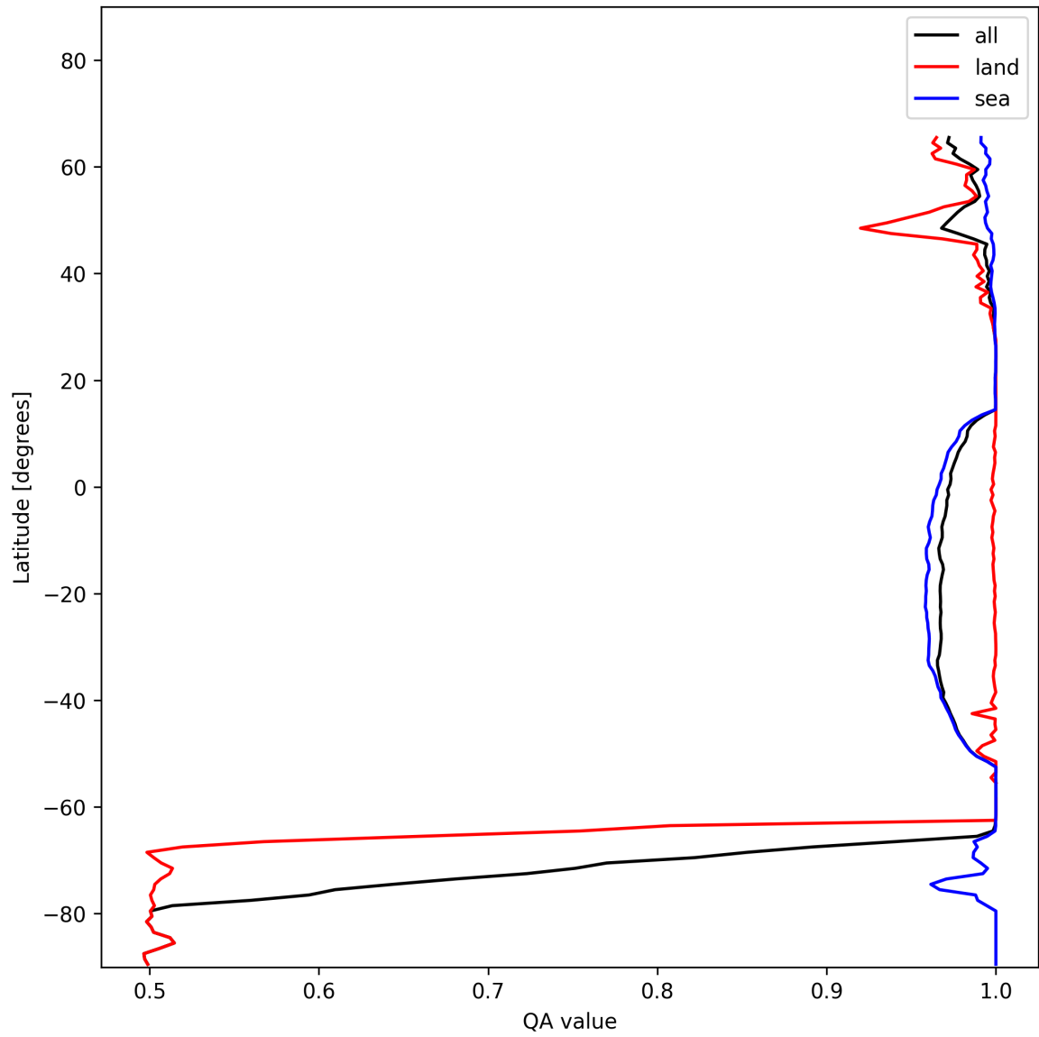
Figure 12: Zonal average of “QA value” for 2025-01-03 to 2025-01-05.
