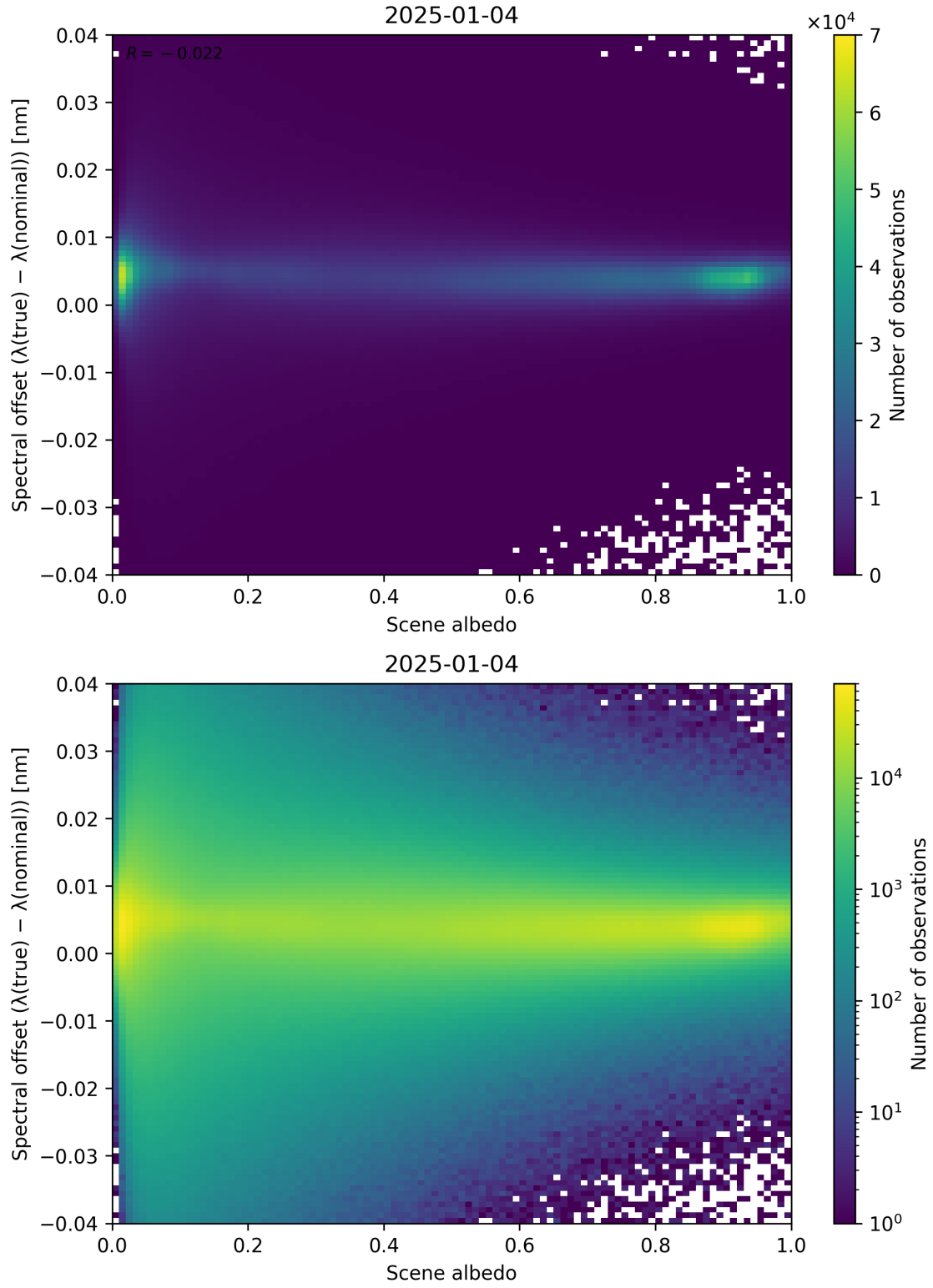
Figure 107: Scatter density plot of “Scene albedo” against “Spectral offset ( \lambda_{\text{true}} - \lambda_{\text{nominal}} )” for 2025-01-03 to 2025-01-05.
