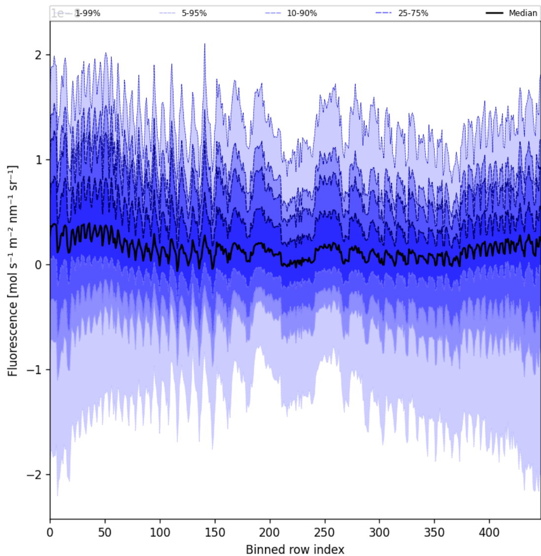
Figure 57: Along track statistics of “Fluorescence” for 2025-01-03 to 2025-01-05
