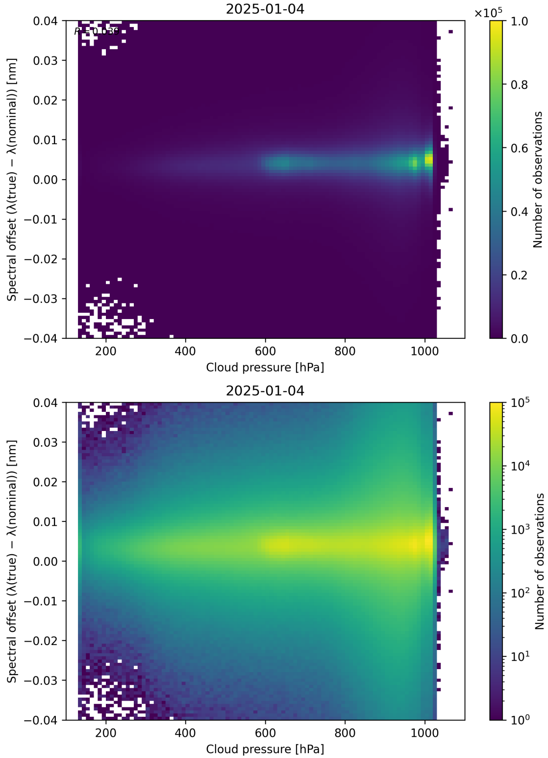
Figure 84: Scatter density plot of “Cloud pressure” against “Spectral offset ( \lambda_{\text{true}} - \lambda_{\text{nominal}} )” for 2025-01-03 to 2025-01-05.
