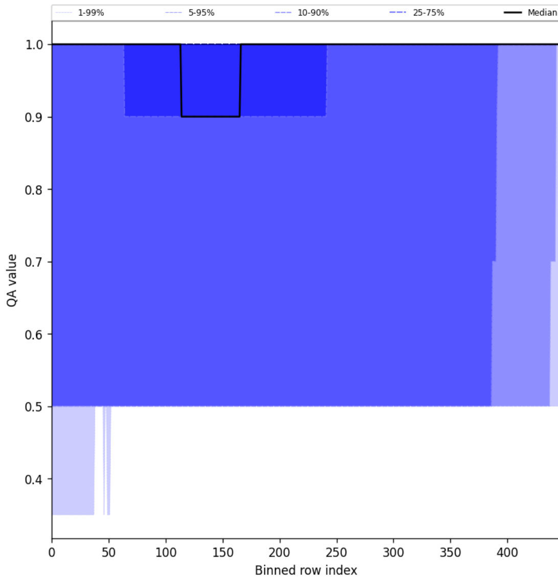
Figure 46: Along track statistics of “QA value” for 2025-01-03 to 2025-01-05
