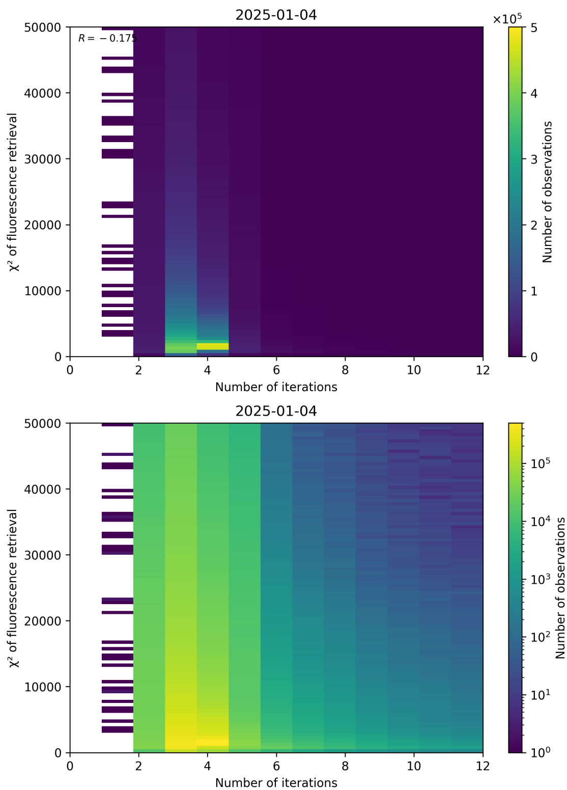
Figure 97: Scatter density plot of “Number of iterations” against “ \chi^2 of fluorescence retrieval” for 2025-01-03 to 2025-01-05.
