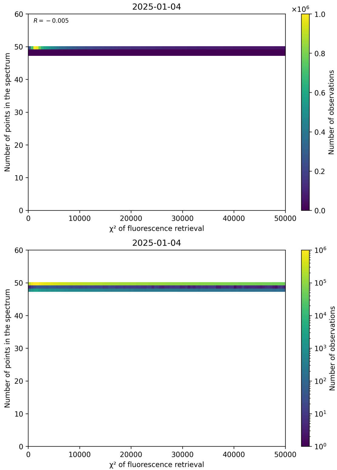
Figure 68: Scatter density plot of “ \chi^2 of fluorescence retrieval” against “Number of points in the spectrum” for 2025-01-03 to 2025-01-05.
