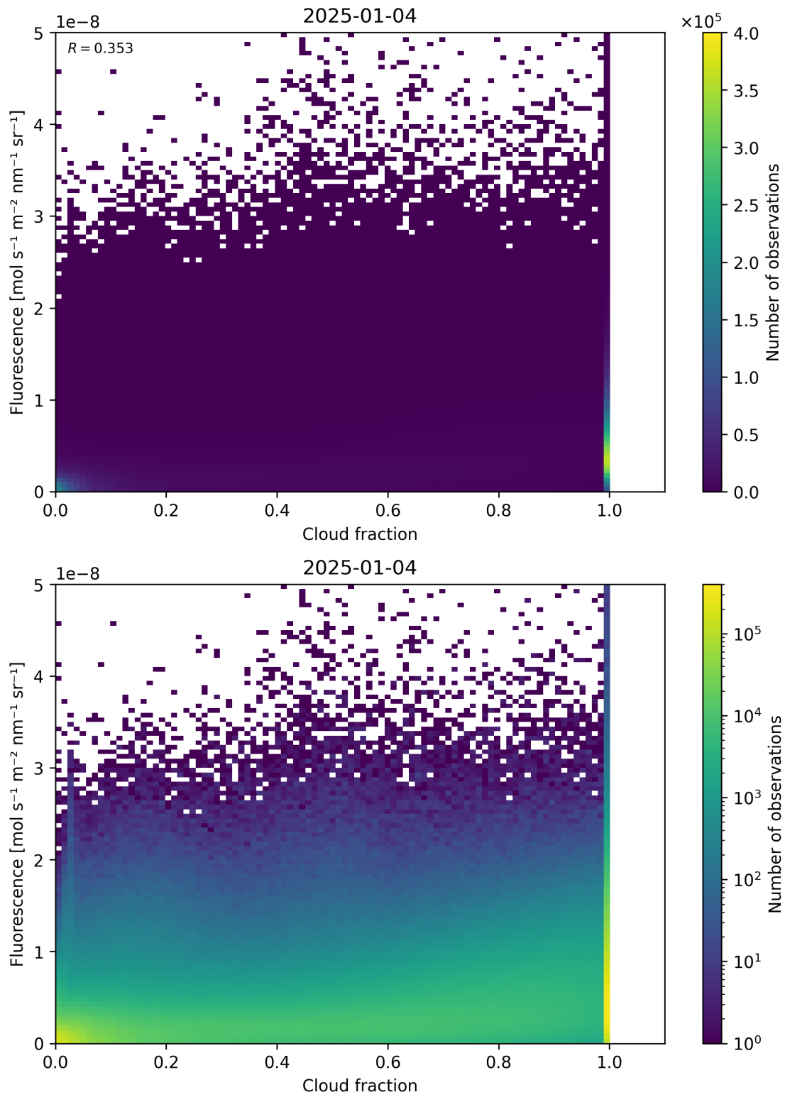
Figure 72: Scatter density plot of “Cloud fraction” against “Fluorescence” for 2025-01-03 to 2025-01-05.
