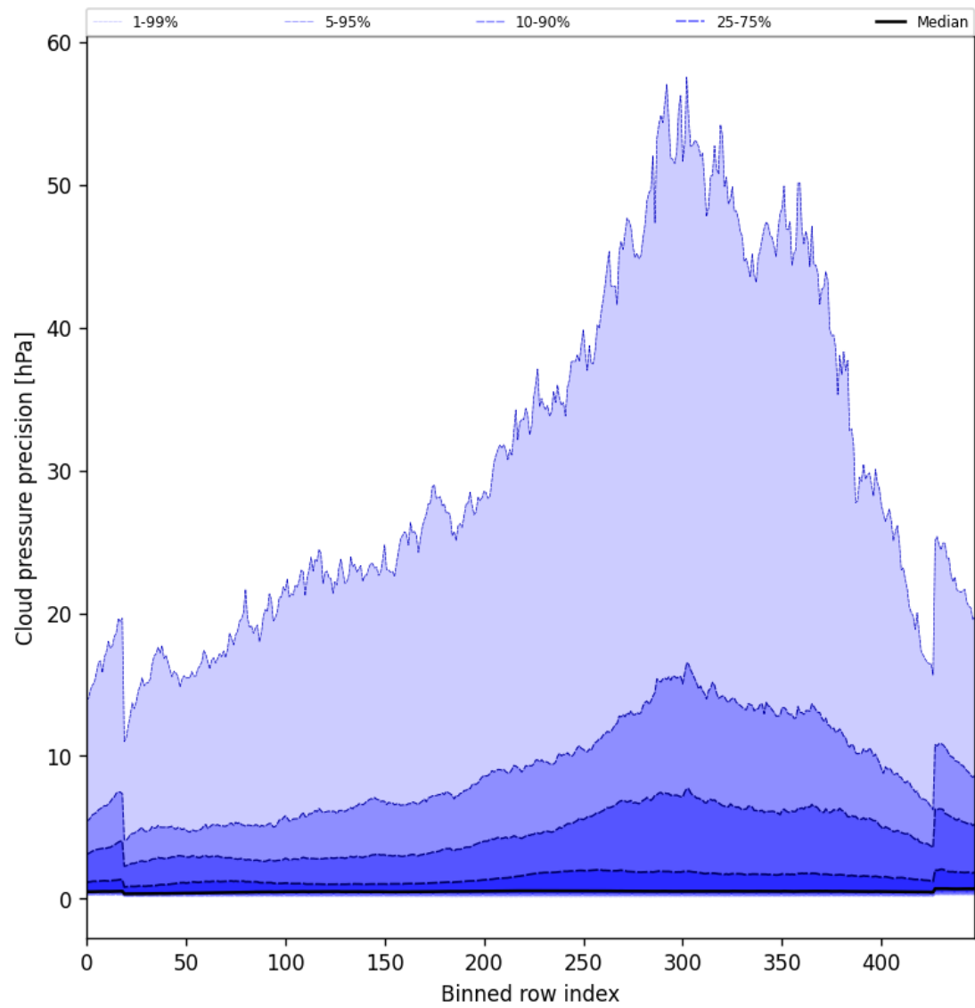
Figure 48: Along track statistics of “Cloud pressure precision” for 2025-01-03 to 2025-01-05
