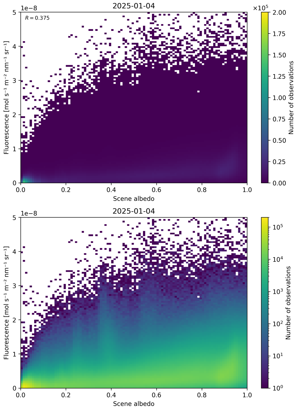
Figure 104: Scatter density plot of “Scene albedo” against “Fluorescence” for 2025-01-03 to 2025-01-05.
