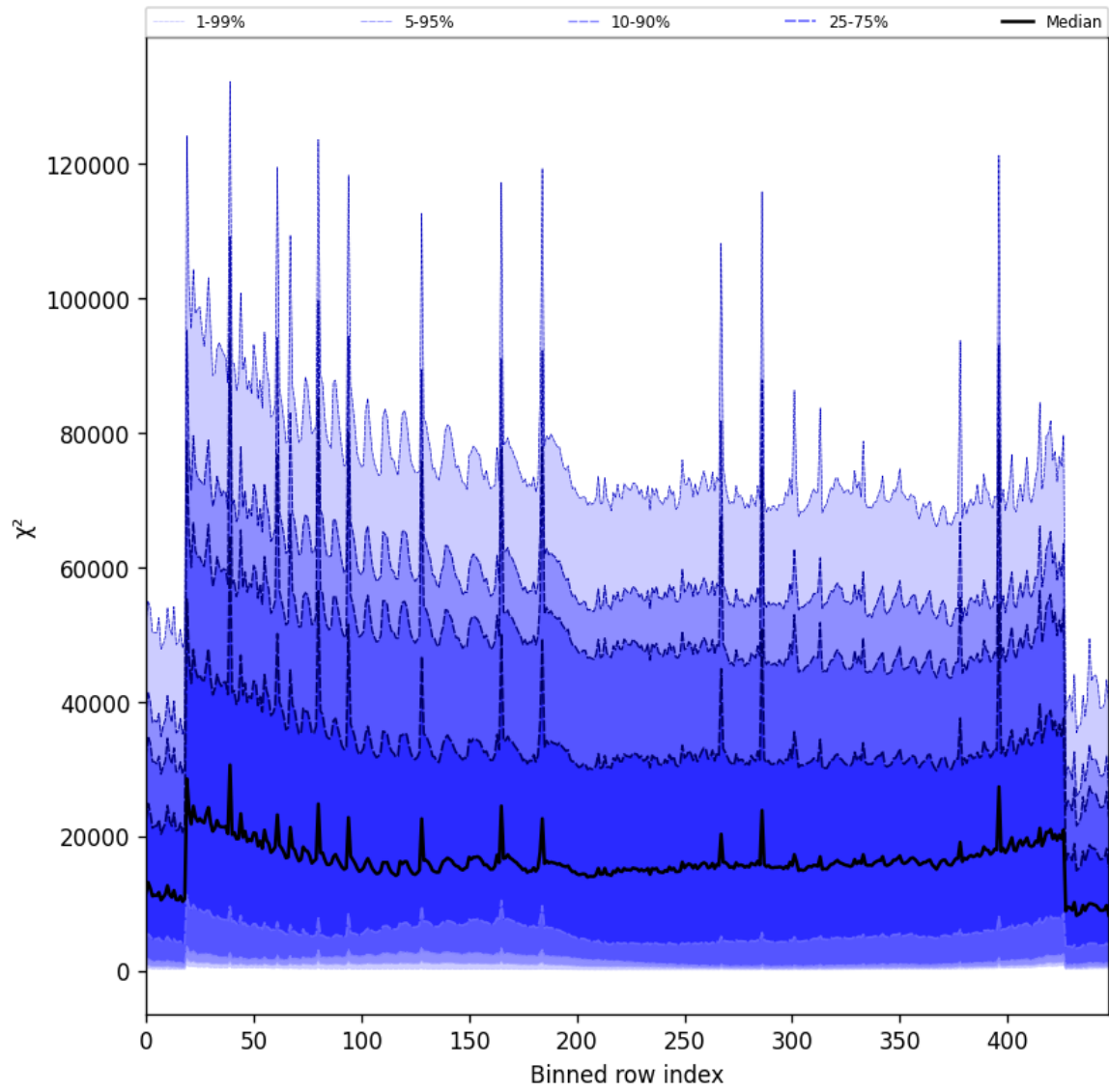
Figure 55: Along track statistics of “ \chi^2 ” for 2025-01-03 to 2025-01-05
