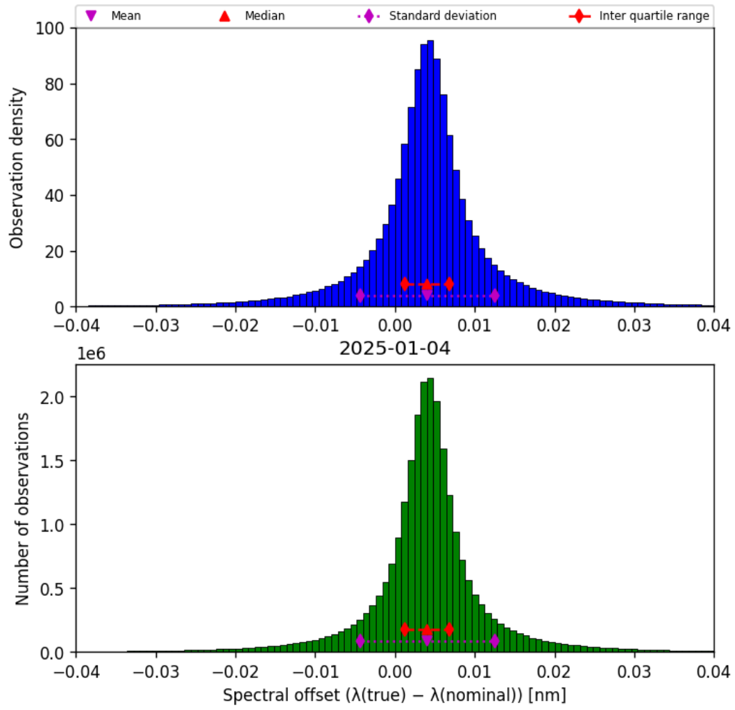
Figure 45: Histogram of “Spectral offset ( \lambda_{\text{true}} - \lambda_{\text{nominal}} )” for 2025-01-03 to 2025-01-05
