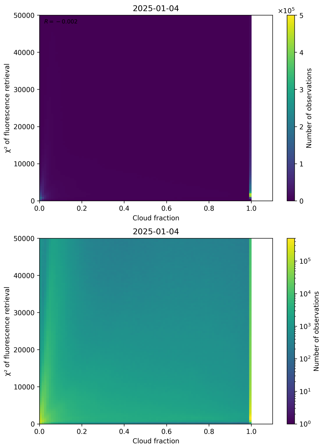
Figure 71: Scatter density plot of “Cloud fraction” against “ \chi^2 of fluorescence retrieval” for 2025-01-03 to 2025-01-05.
