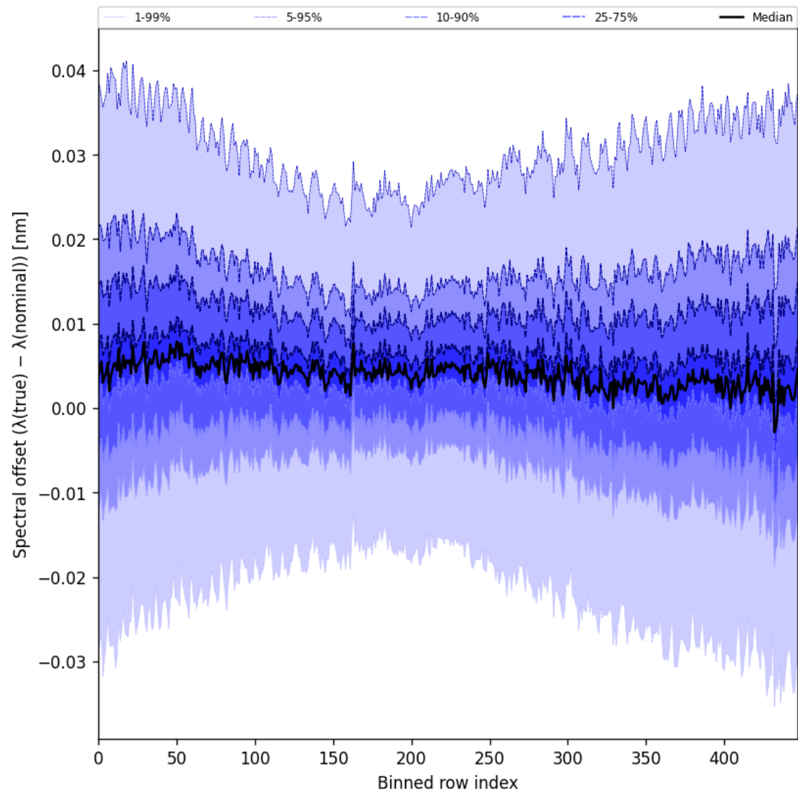
Figure 62: Along track statistics of “Spectral offset ( \lambda_{\text{true}} - \lambda_{\text{nominal}} )” for 2025-01-03 to 2025-01-05
