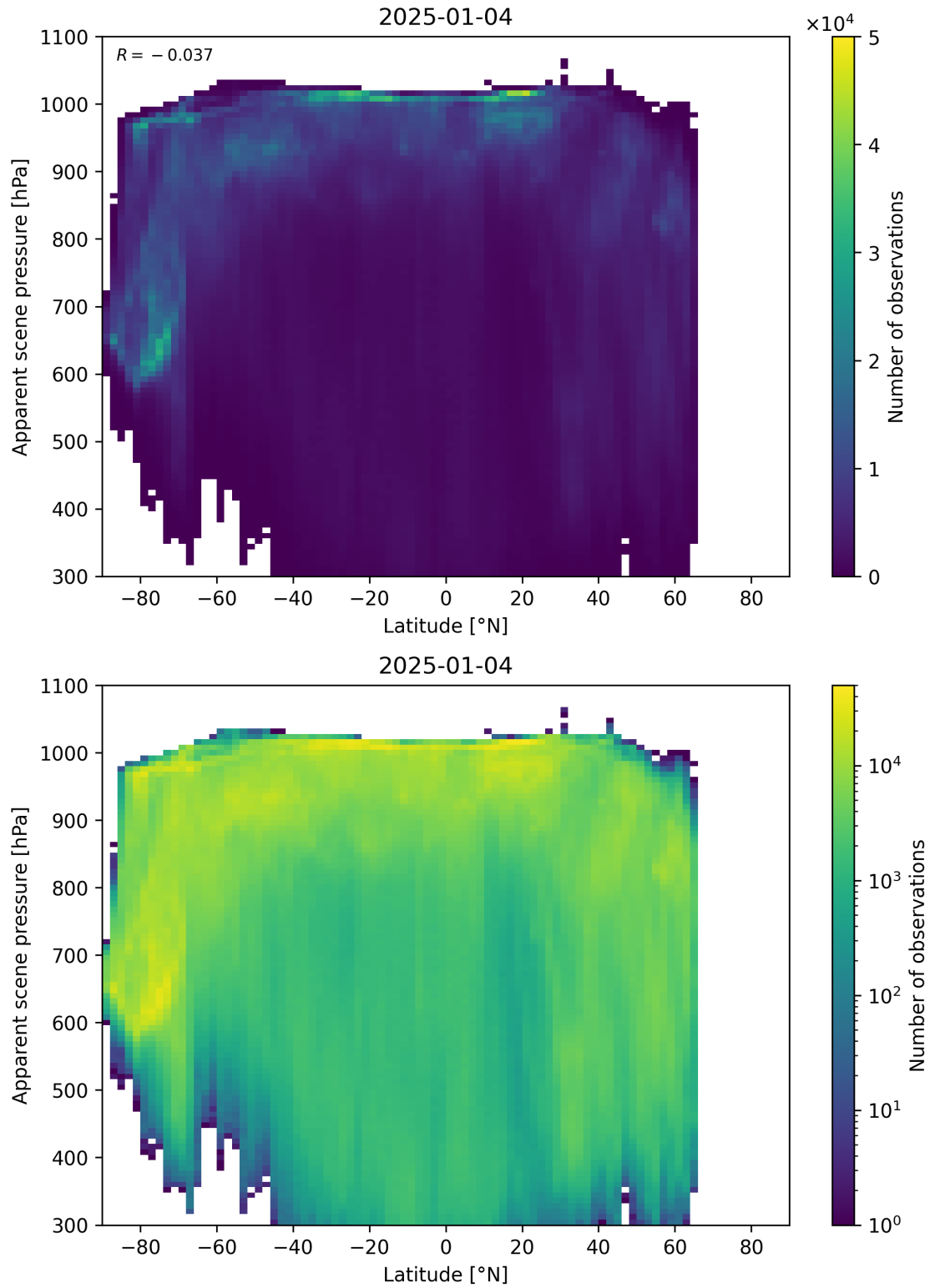
Figure 88: Scatter density plot of “Latitude” against “Apparent scene pressure” for 2025-01-03 to 2025-01-05.
