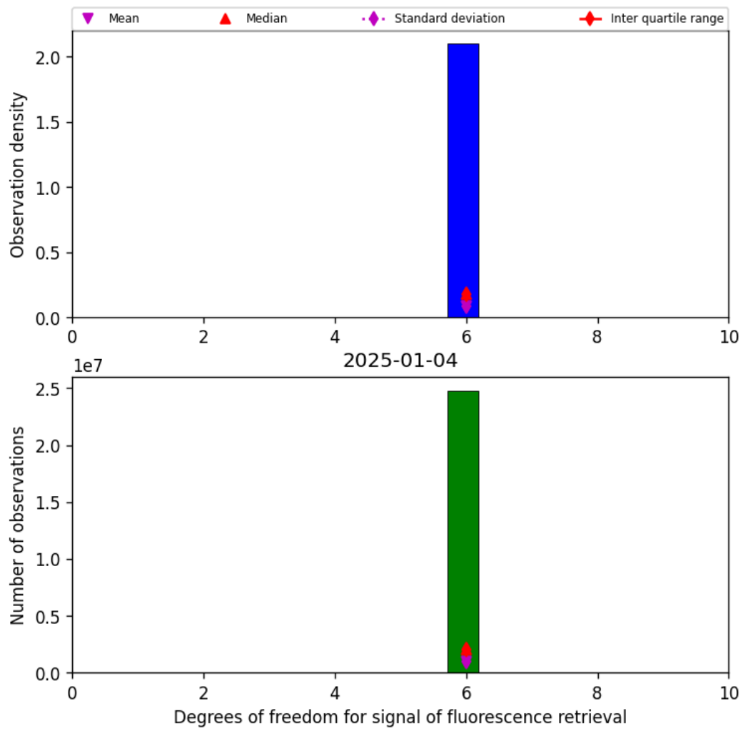
Figure 43: Histogram of "Degrees of freedom for signal of fluorescence retrieval" for 2025-01-03 to 2025-01-05
