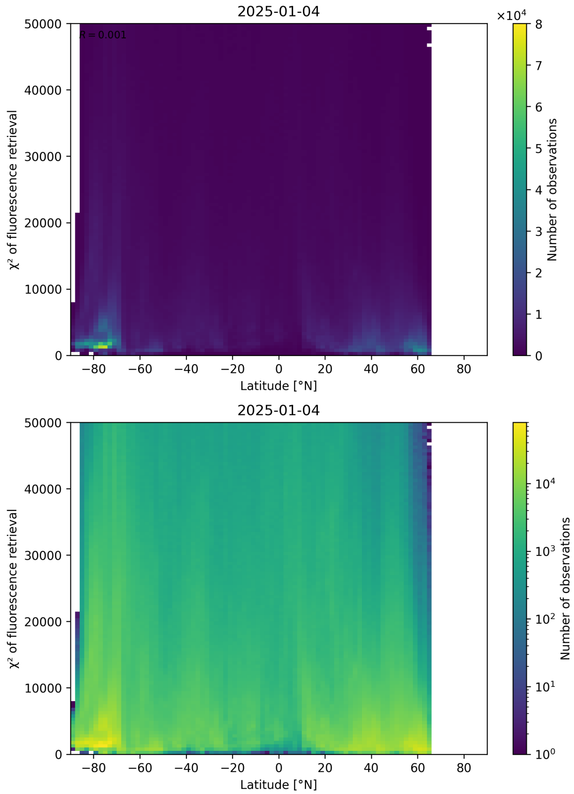
Figure 89: Scatter density plot of “Latitude” against “ \chi^2 of fluorescence retrieval” for 2025-01-03 to 2025-01-05.
