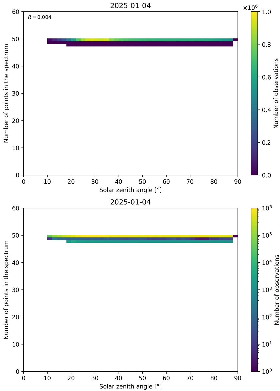
Figure 115: Scatter density plot of “Solar zenith angle” against “Number of points in the spectrum” for 2025-01-03 to 2025-01-05.
