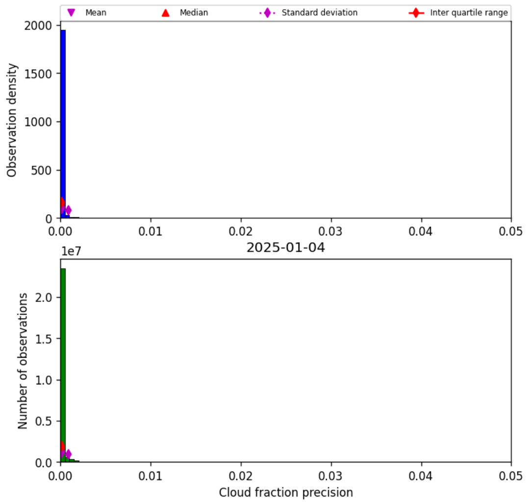
Figure 33: Histogram of “Cloud fraction precision” for 2025-01-03 to 2025-01-05
