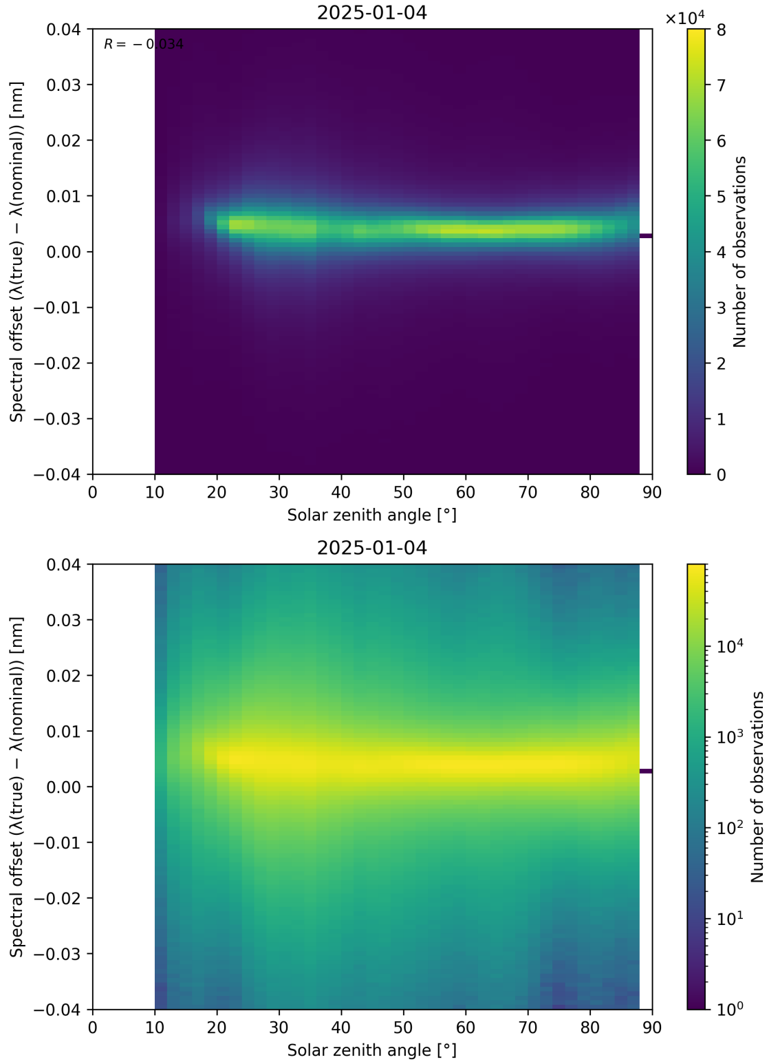
Figure 117: Scatter density plot of “Solar zenith angle” against “Spectral offset ( \lambda_{\text{true}} - \lambda_{\text{nominal}} )” for 2025-01-03 to 2025-01-05.
