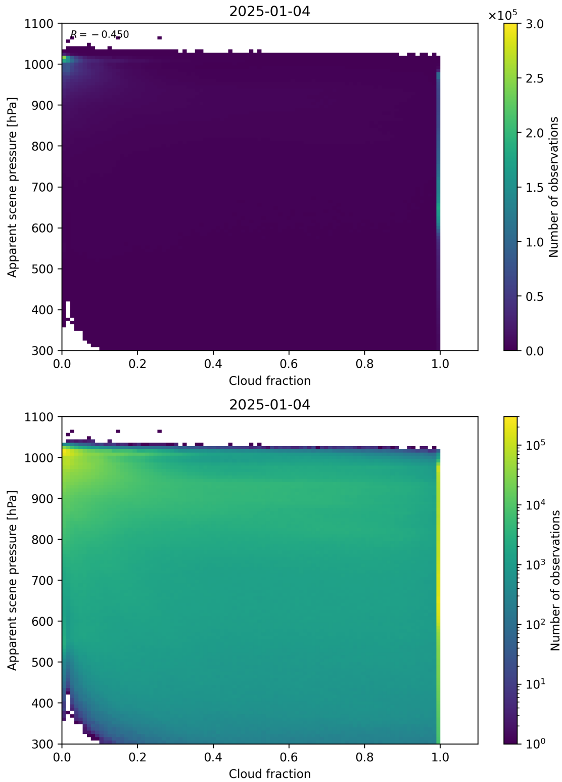
Figure 70: Scatter density plot of “Cloud fraction” against “Apparent scene pressure” for 2025-01-03 to 2025-01-05.
