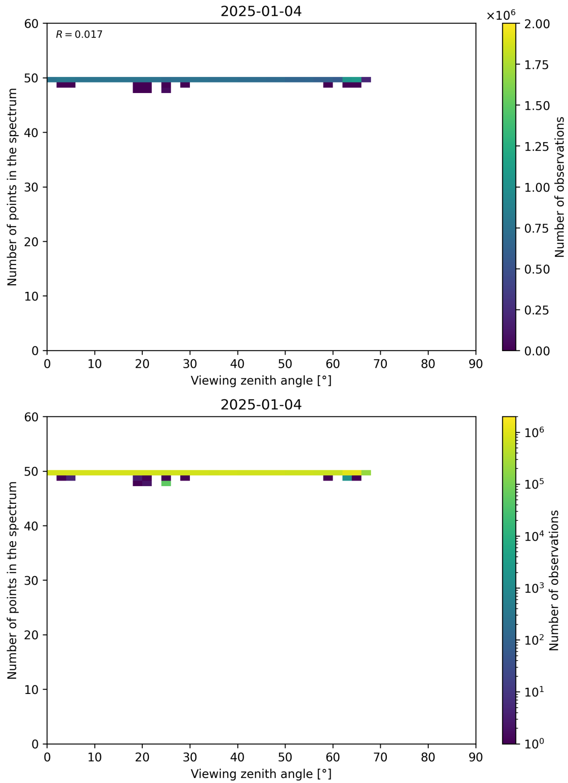
Figure 125: Scatter density plot of “Viewing zenith angle” against “Number of points in the spectrum” for 2025-01-03 to 2025-01-05.
