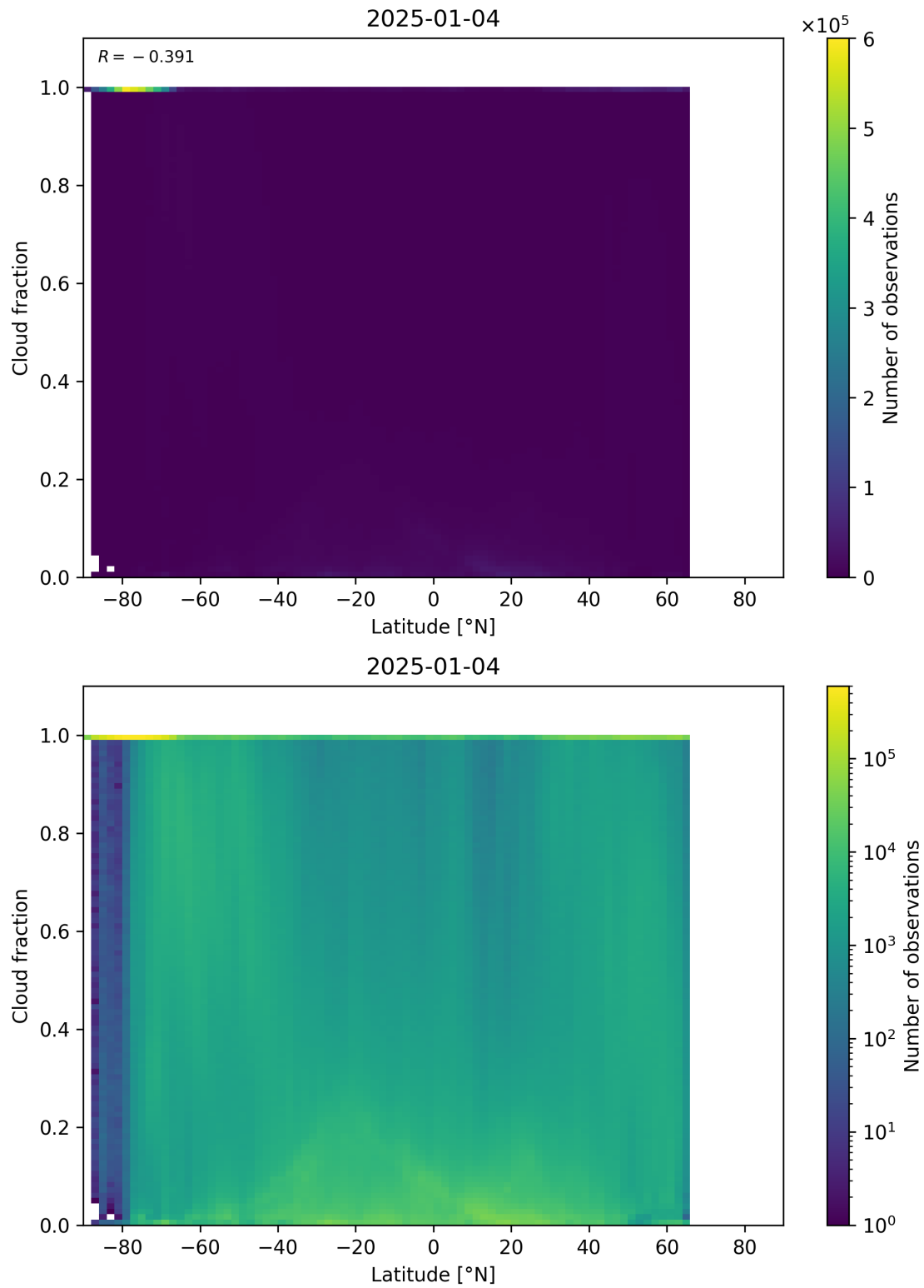
Figure 90: Scatter density plot of “Latitude” against “Cloud fraction” for 2025-01-03 to 2025-01-05.
