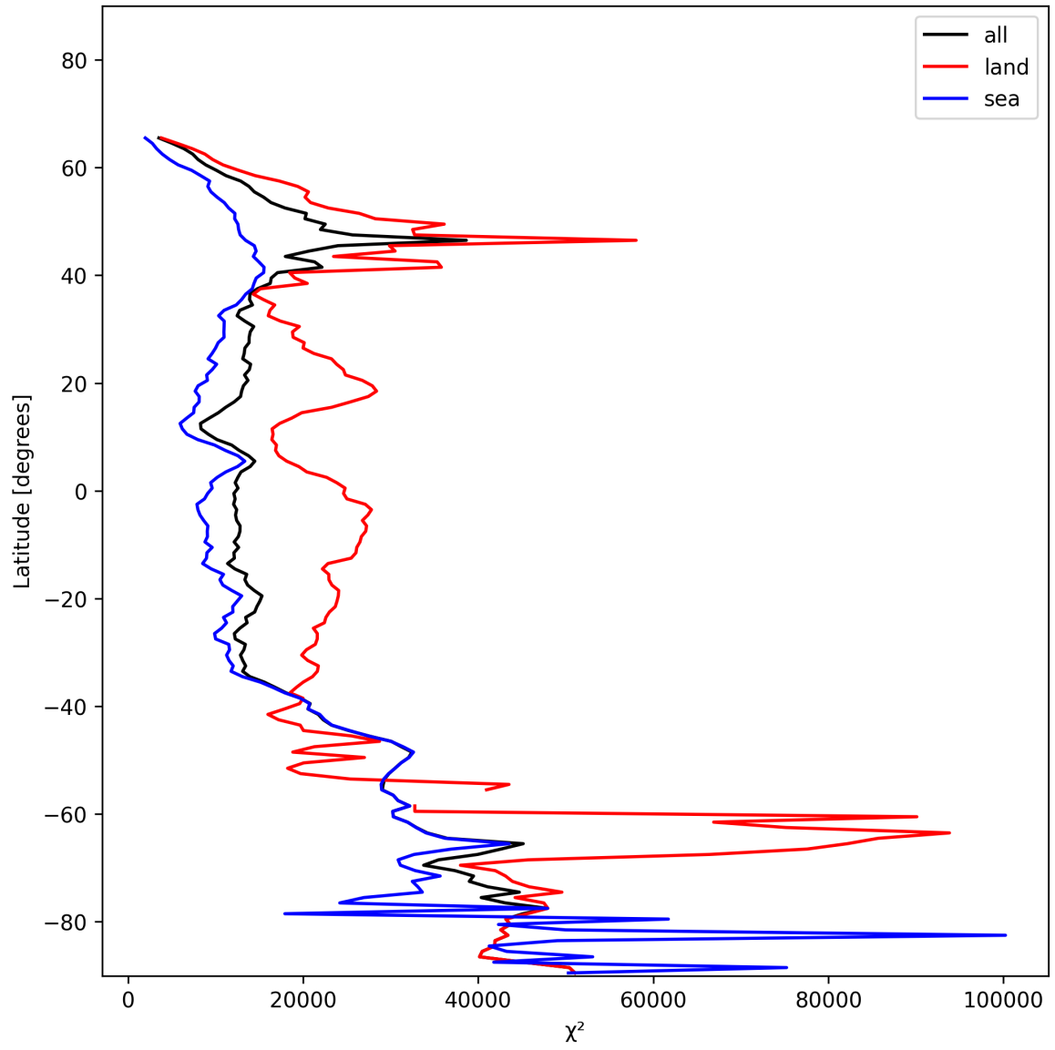
Figure 21: Zonal average of “ \chi^2 ” for 2025-01-03 to 2025-01-05.
