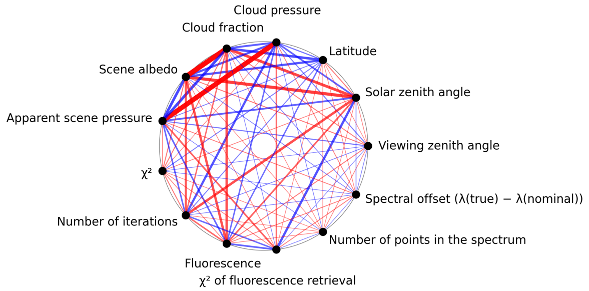
Figure 1: Map of correlation graph for 2025-01-03 to 2025-01-05.
