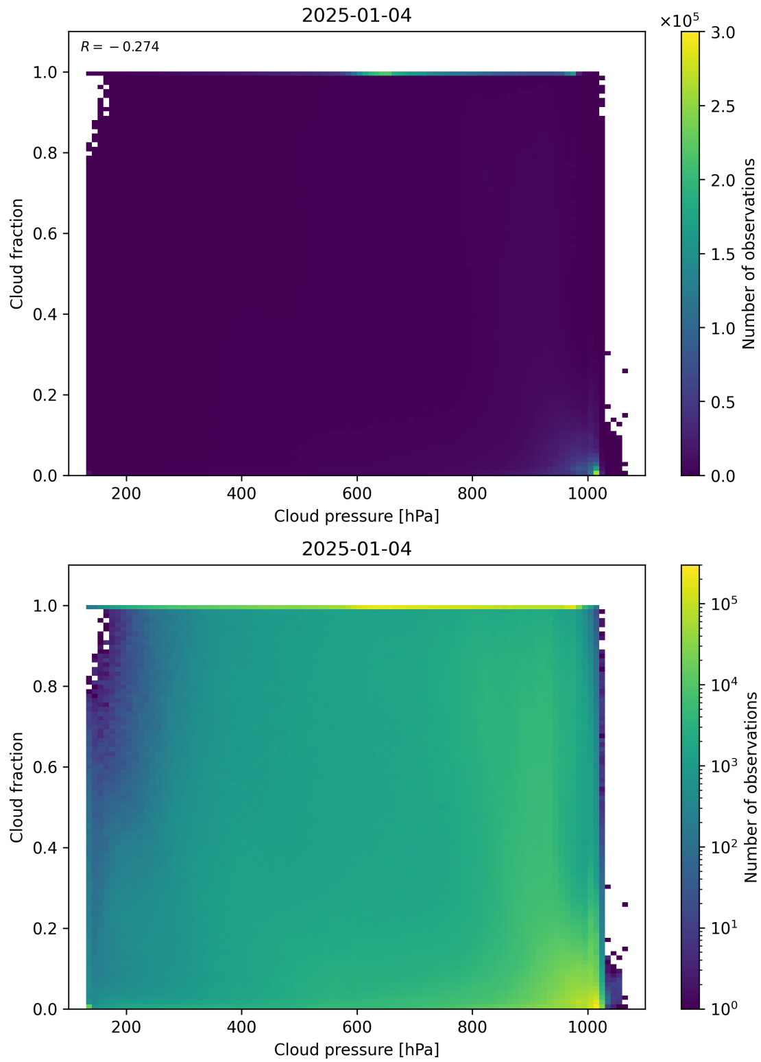
Figure 79: Scatter density plot of “Cloud pressure” against “Cloud fraction” for 2025-01-03 to 2025-01-05.
