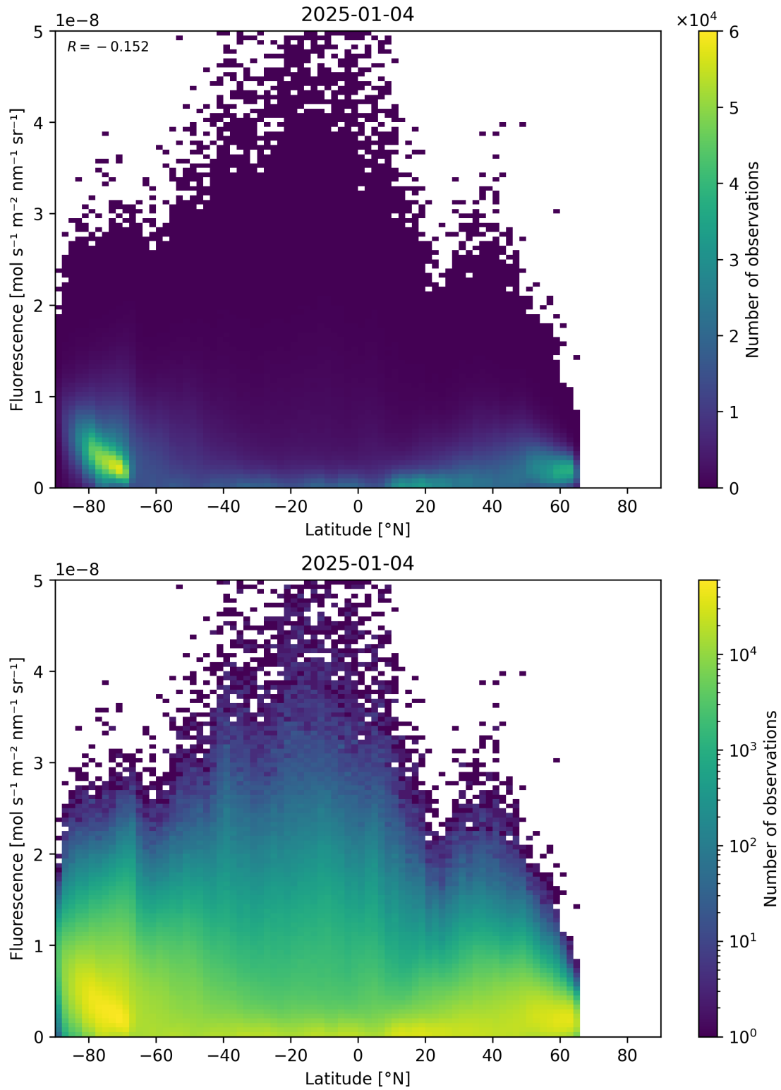
Figure 92: Scatter density plot of “Latitude” against “Fluorescence” for 2025-01-03 to 2025-01-05.
