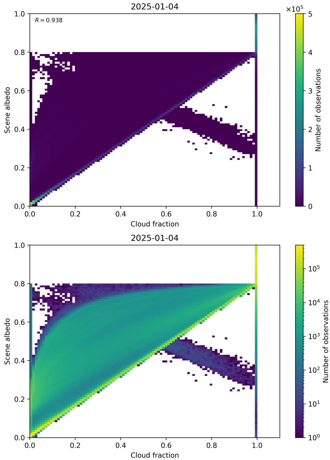
Figure 75: Scatter density plot of “Cloud fraction” against “Scene albedo” for 2025-01-03 to 2025-01-05.
