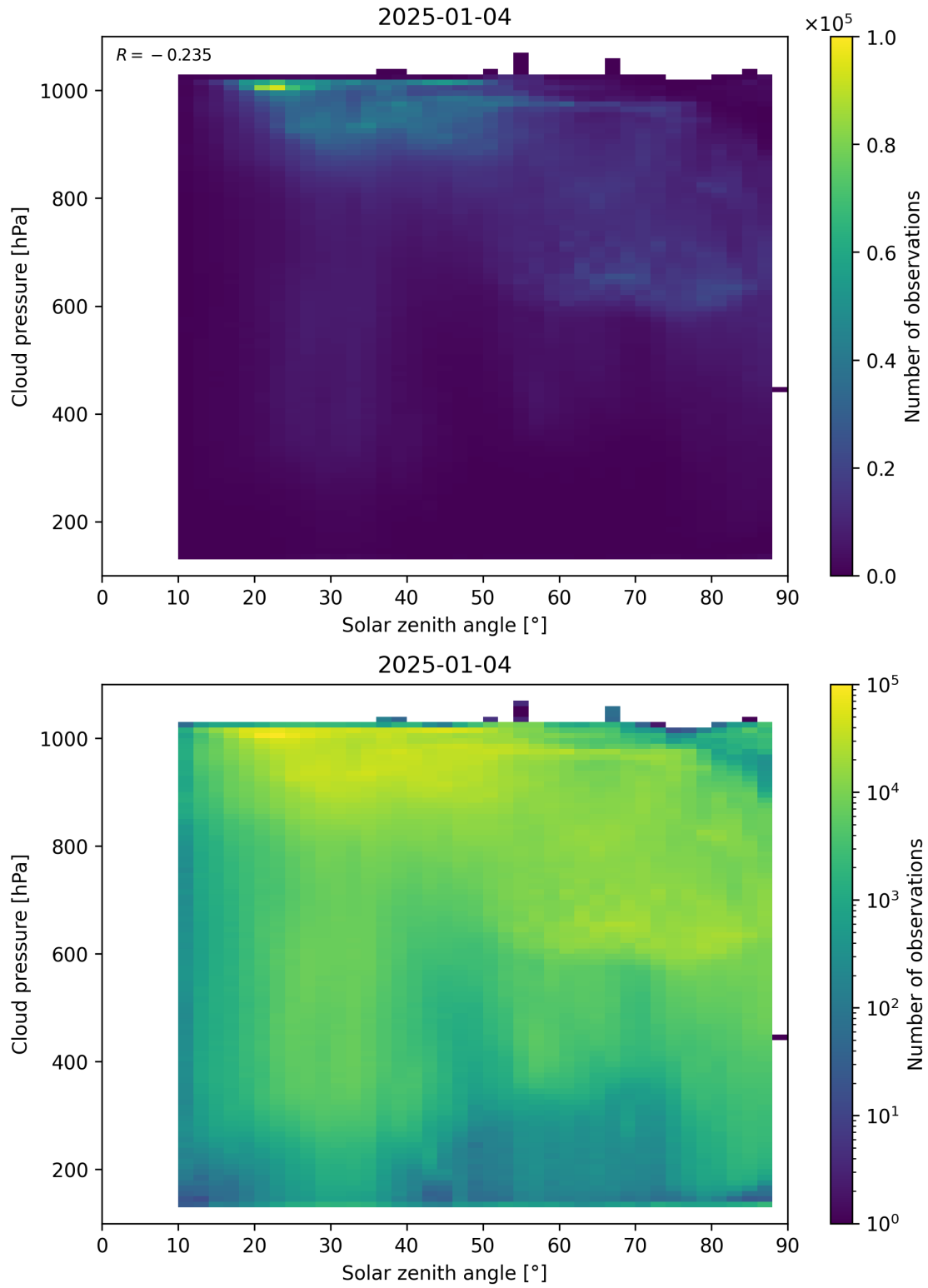
Figure 111: Scatter density plot of “Solar zenith angle” against “Cloud pressure” for 2025-01-03 to 2025-01-05.
