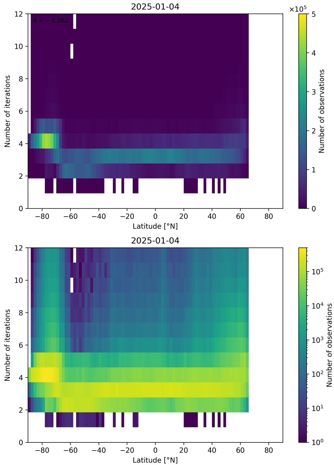
Figure 93: Scatter density plot of “Latitude” against “Number of iterations” for 2025-01-03 to 2025-01-05.
