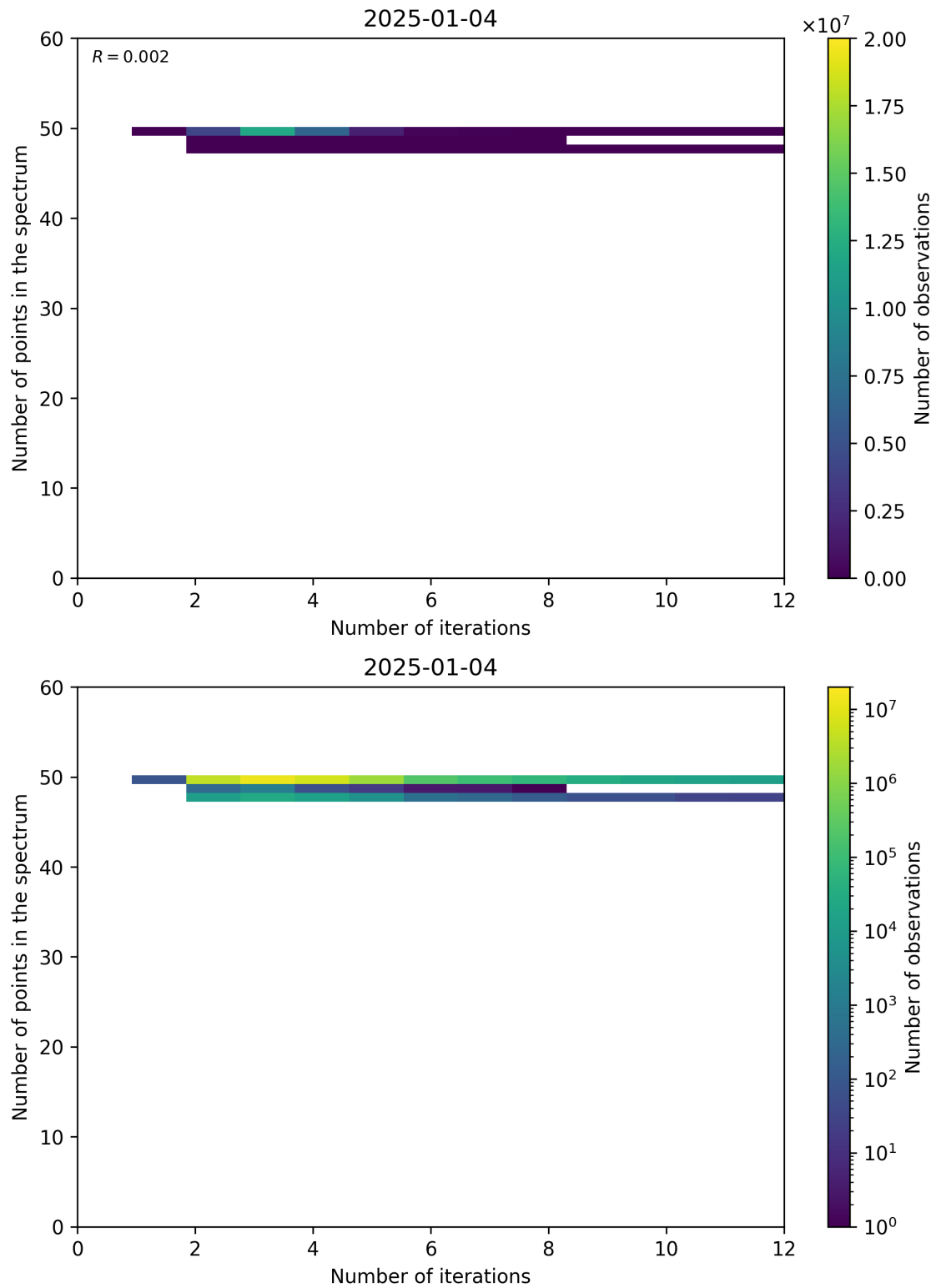
Figure 99: Scatter density plot of “Number of iterations” against “Number of points in the spectrum” for 2025-01-03 to 2025-01-05.
