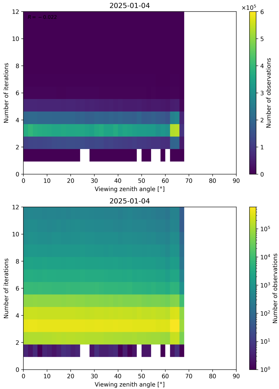
Figure 124: Scatter density plot of “Viewing zenith angle” against “Number of iterations” for 2025-01-03 to 2025-01-05.
