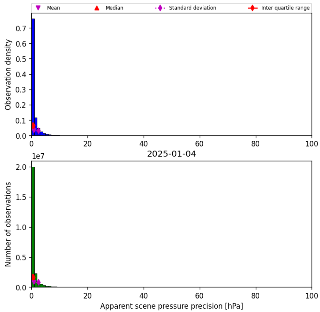
Figure 37: Histogram of “Apparent scene pressure precision” for 2025-01-03 to 2025-01-05
