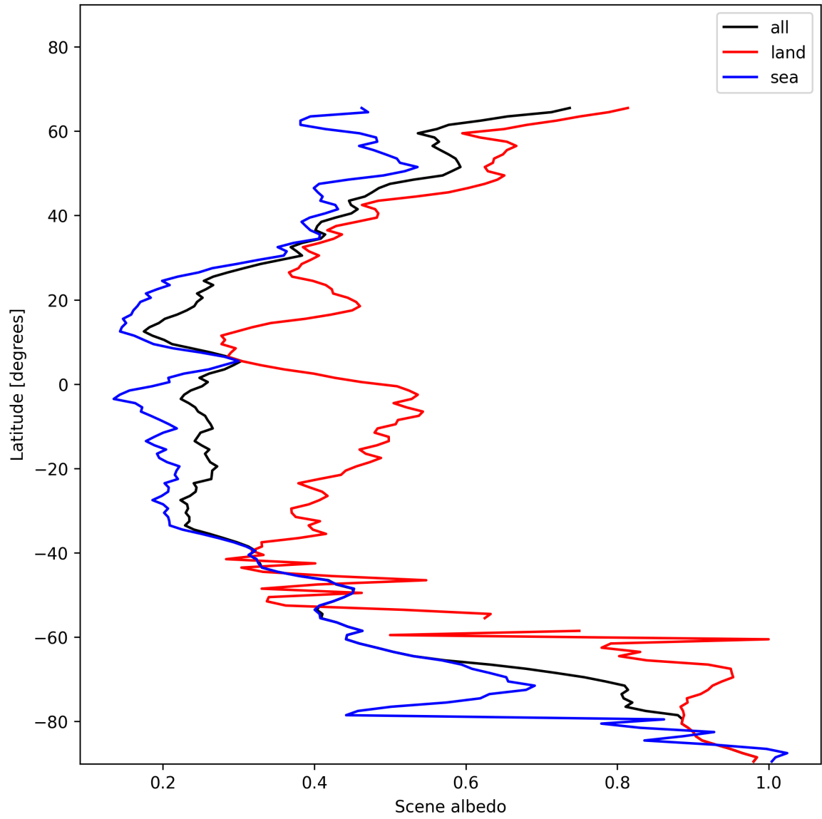
Figure 17: Zonal average of “Scene albedo” for 2025-01-03 to 2025-01-05.
