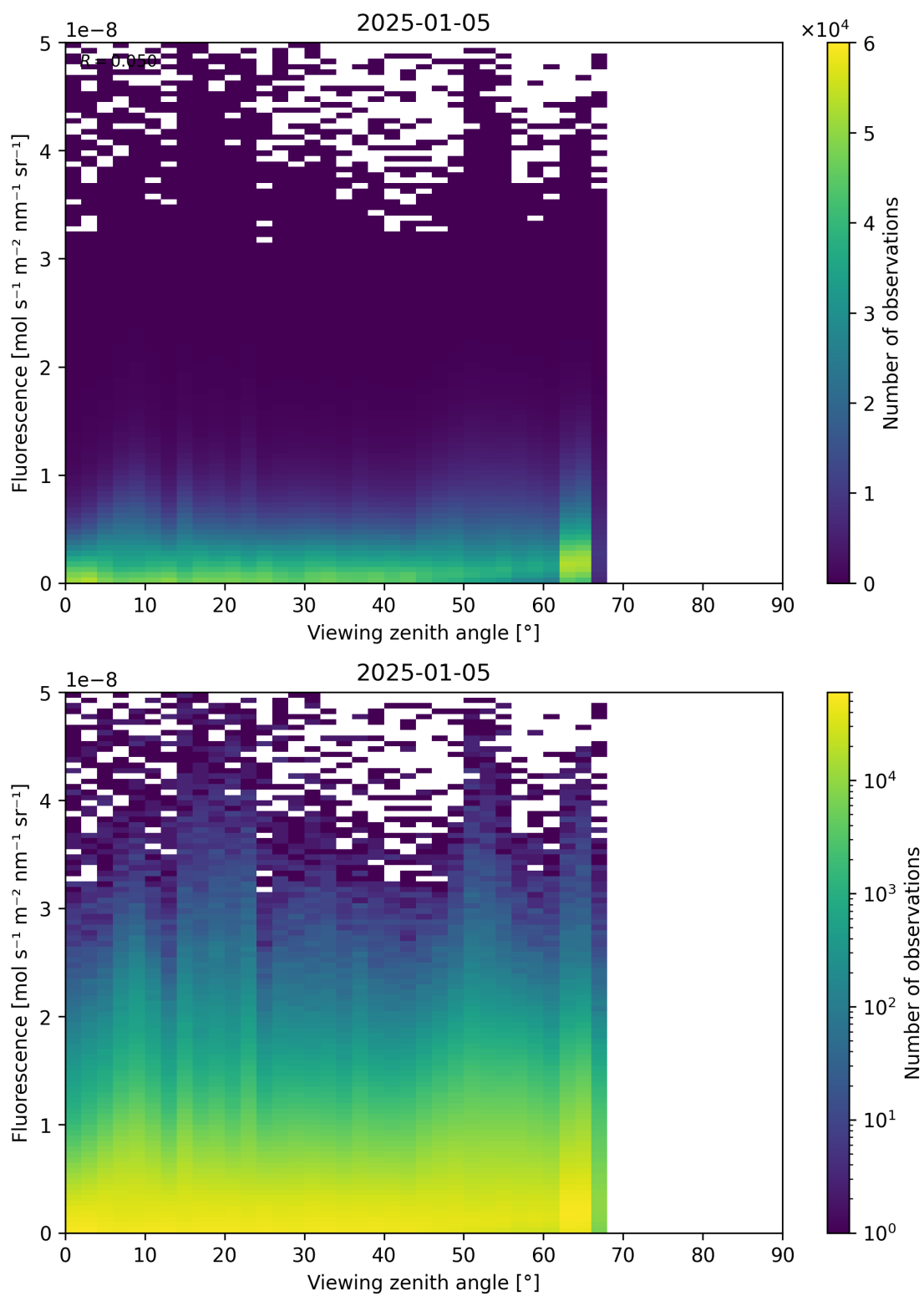
Figure 122: Scatter density plot of “Viewing zenith angle” against “Fluorescence” for 2025-01-04 to 2025-01-06.
