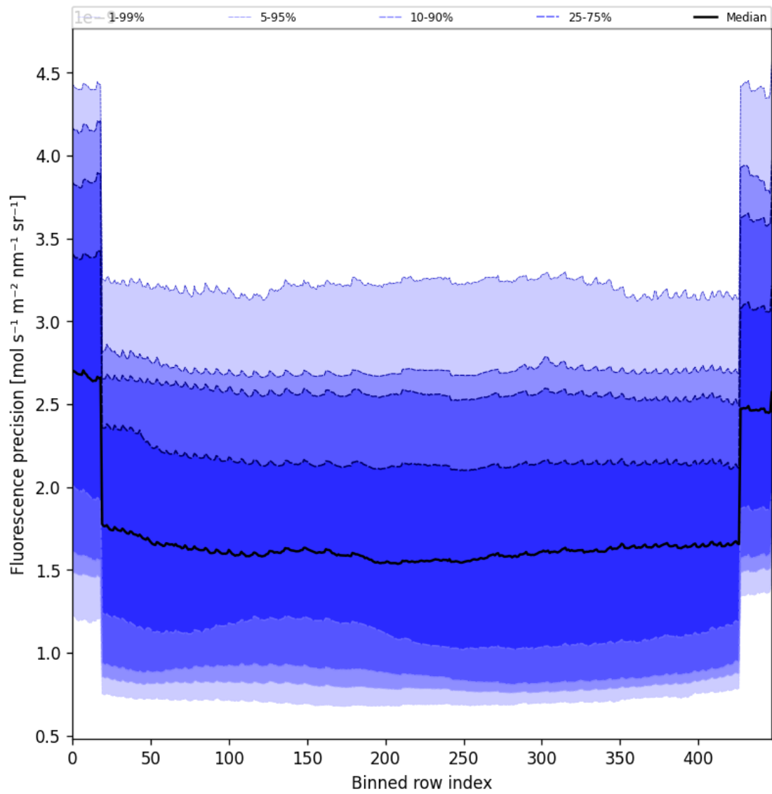
Figure 58: Along track statistics of “Fluorescence precision” for 2025-01-04 to 2025-01-06
