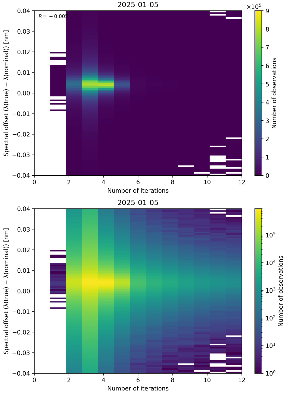
Figure 100: Scatter density plot of “Number of iterations” against “Spectral offset ( \lambda_{\text{true}} - \lambda_{\text{nominal}} )” for 2025-01-04 to 2025-01-06.
