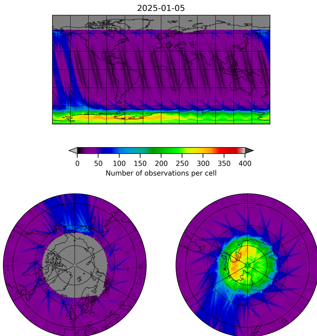
Figure 11: Map of the number of observations for 2025-01-04 to 2025-01-06
