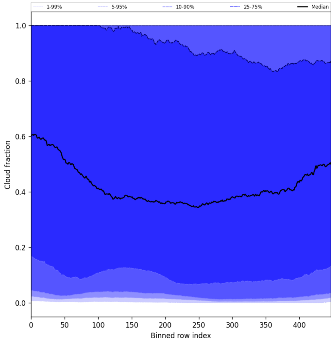
Figure 49: Along track statistics of “Cloud fraction” for 2025-01-04 to 2025-01-06
