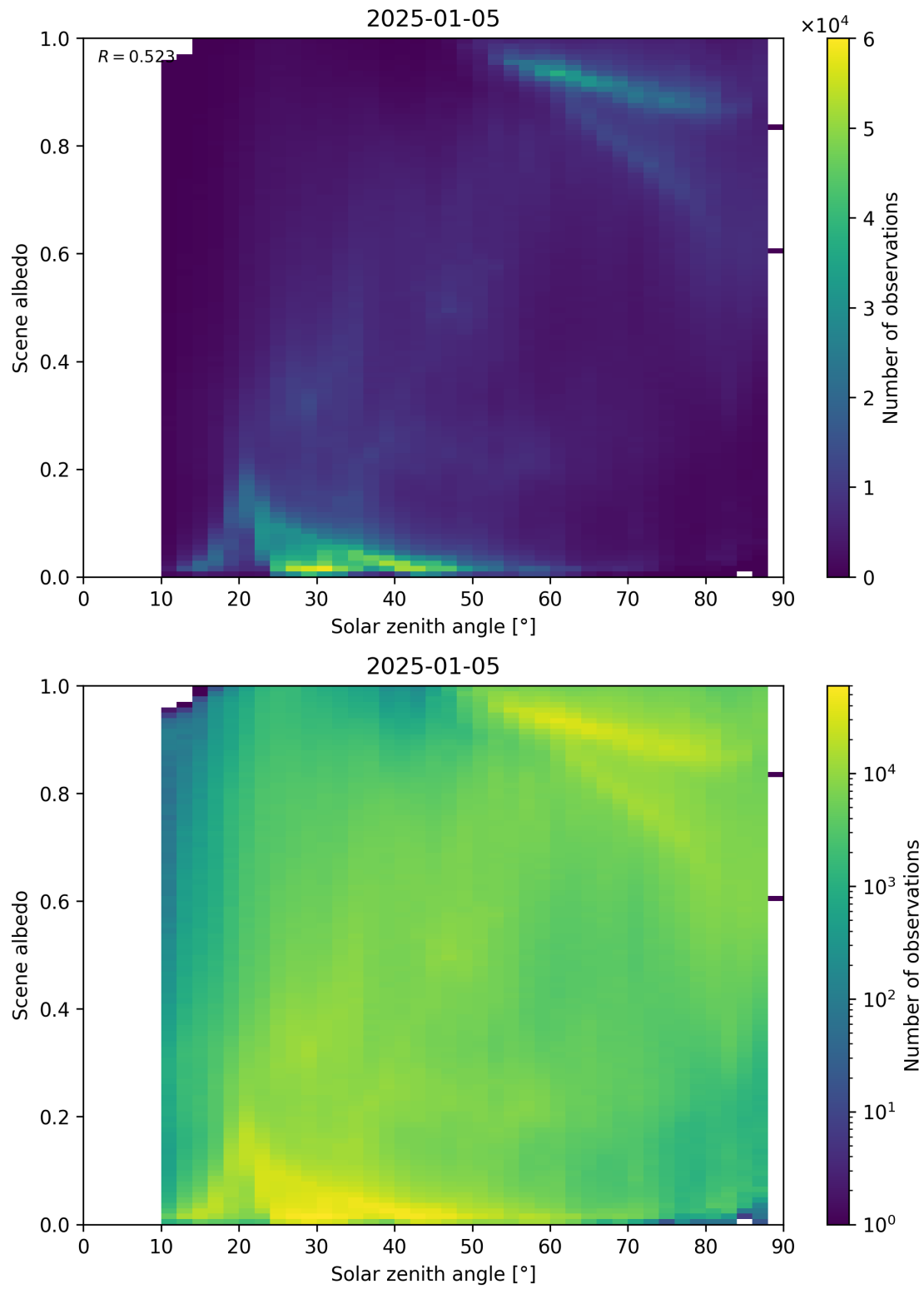
Figure 116: Scatter density plot of “Solar zenith angle” against “Scene albedo” for 2025-01-04 to 2025-01-06.
