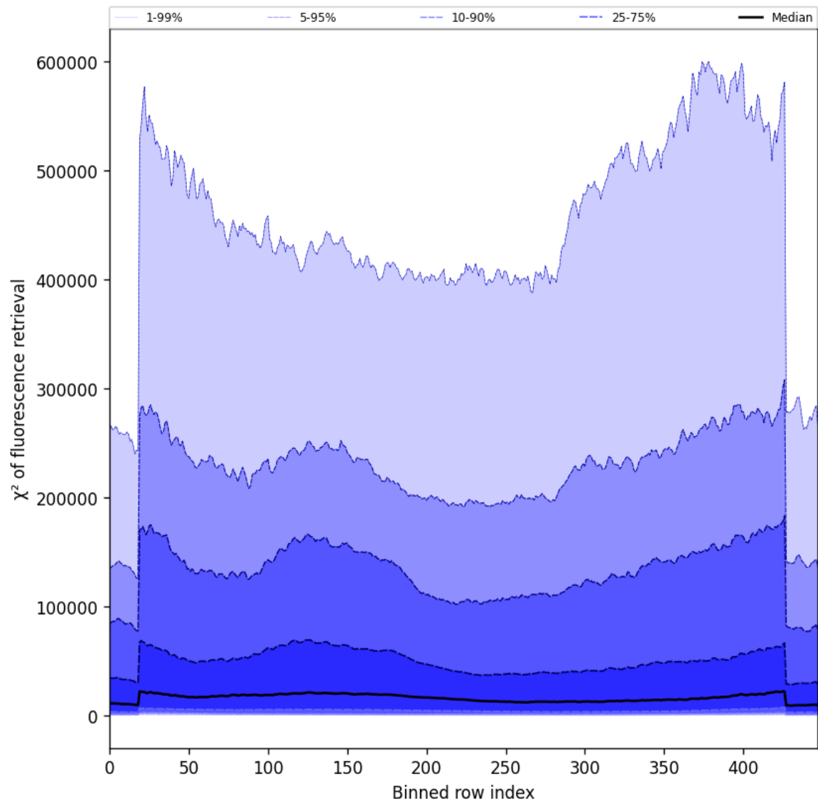
Figure 59: Along track statistics of “ \chi^2 of fluorescence retrieval” for 2025-01-04 to 2025-01-06
