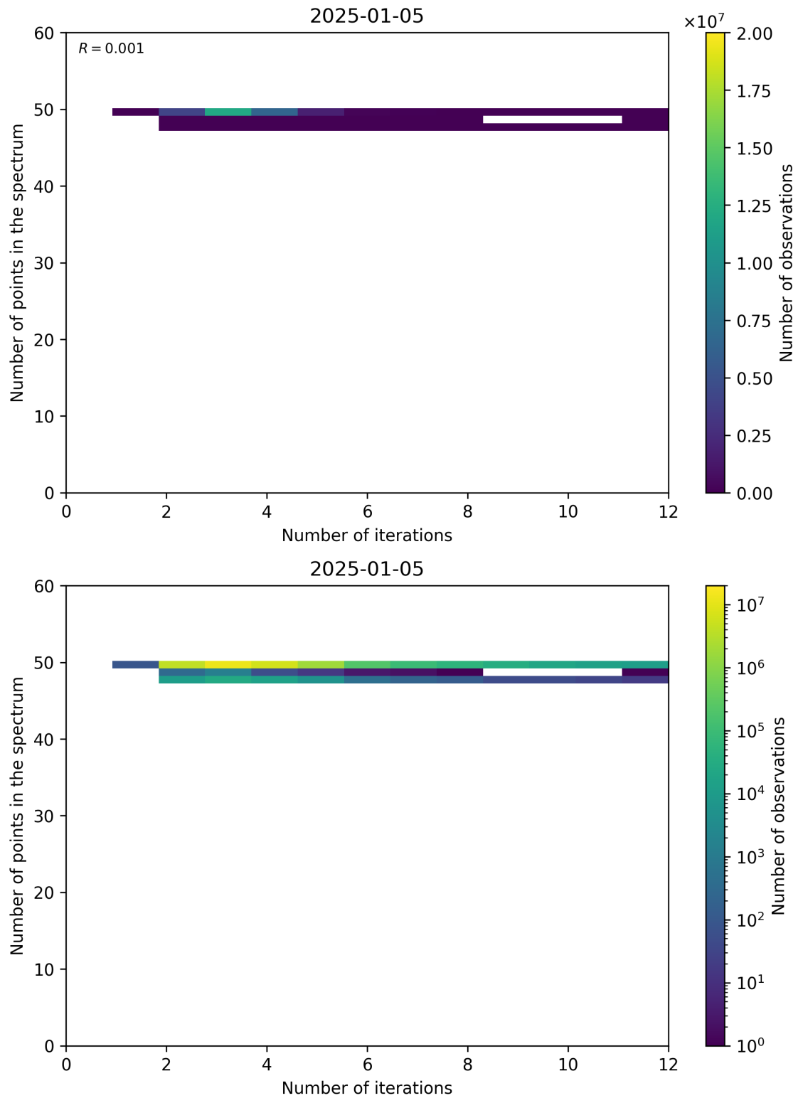
Figure 99: Scatter density plot of “Number of iterations” against “Number of points in the spectrum” for 2025-01-04 to 2025-01-06.
