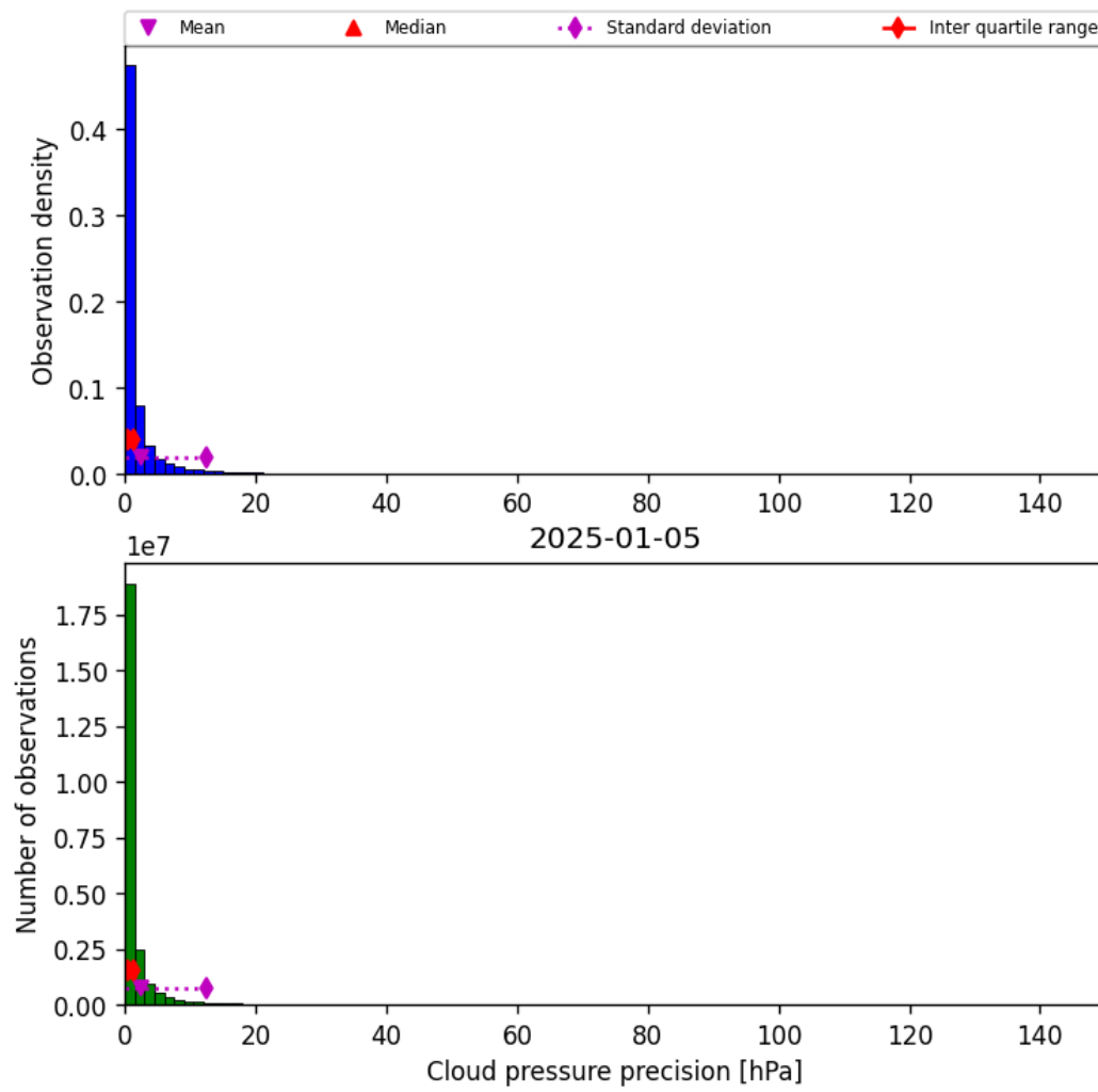
Figure 31: Histogram of “Cloud pressure precision” for 2025-01-04 to 2025-01-06
