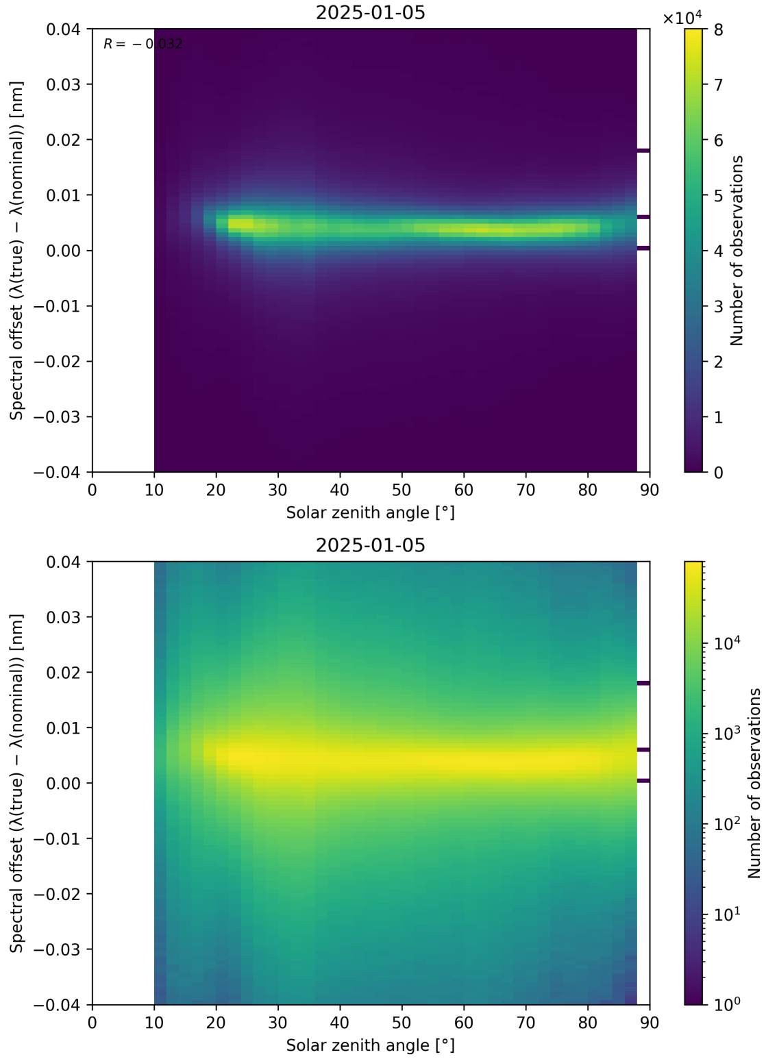
Figure 117: Scatter density plot of “Solar zenith angle” against “Spectral offset ( \lambda_{\text{true}} - \lambda_{\text{nominal}} )” for 2025-01-04 to 2025-01-06.
