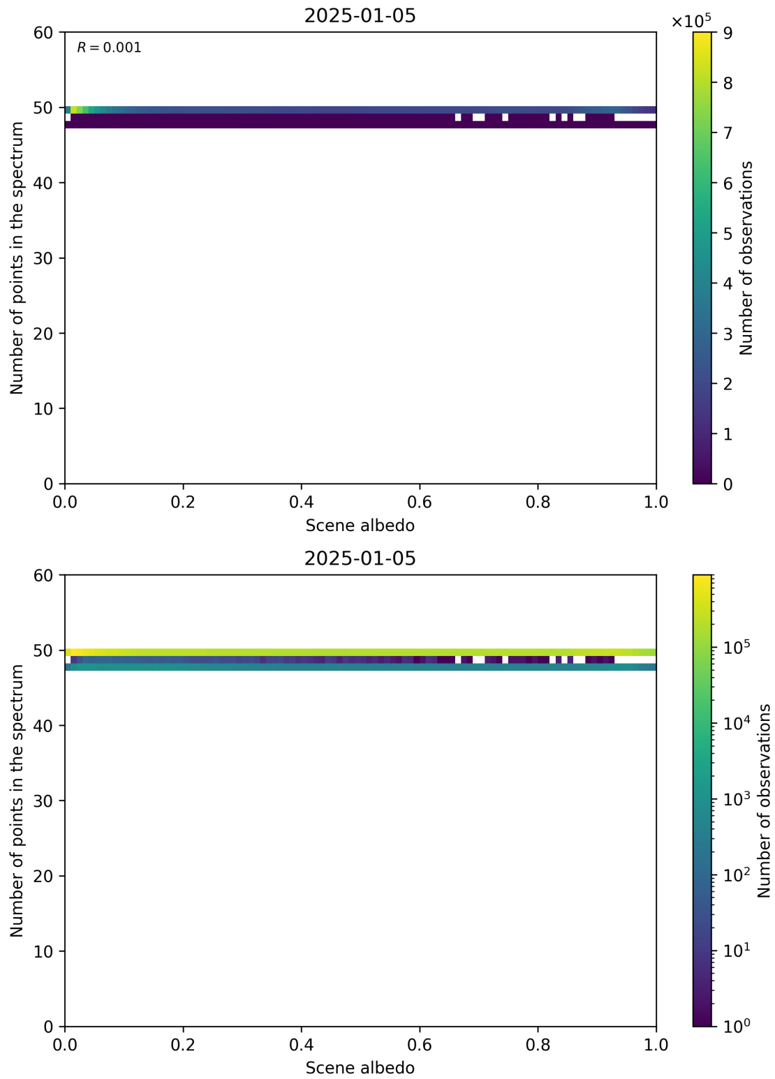
Figure 106: Scatter density plot of “Scene albedo” against “Number of points in the spectrum” for 2025-01-04 to 2025-01-06.
