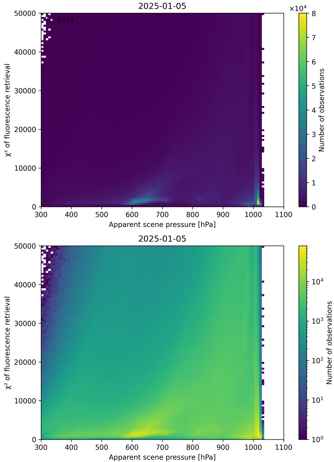
Figure 63: Scatter density plot of “Apparent scene pressure” against “ \chi^2 of fluorescence retrieval” for 2025-01-04 to 2025-01-06.
