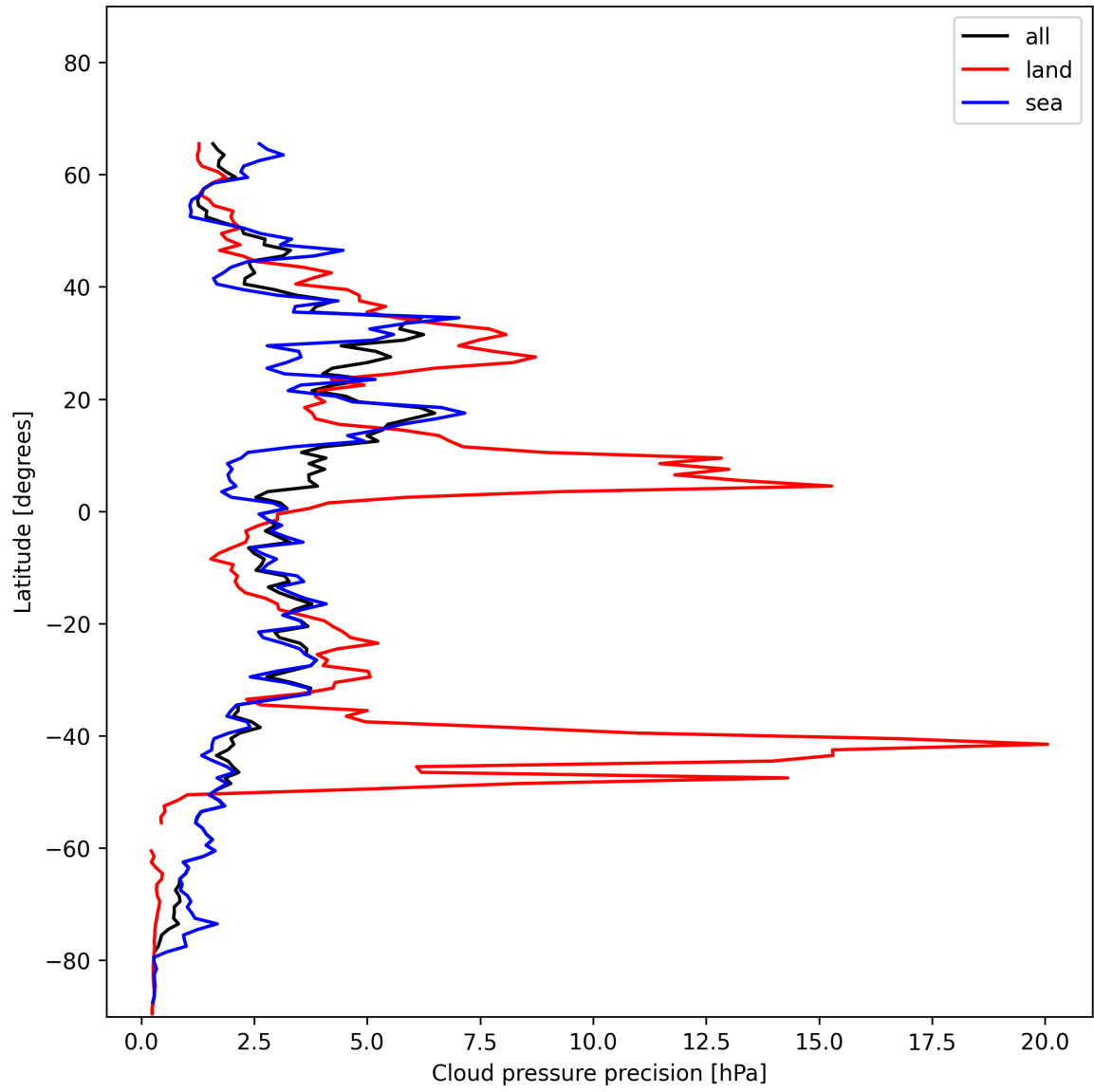
Figure 14: Zonal average of “Cloud pressure precision” for 2025-01-04 to 2025-01-06.
