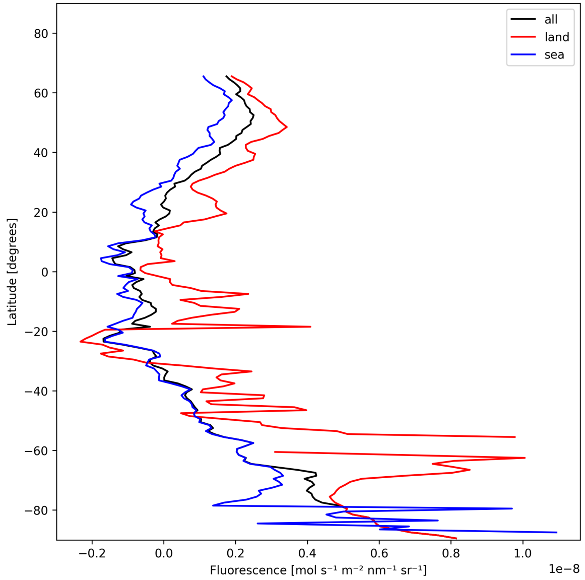
Figure 23: Zonal average of “Fluorescence” for 2025-01-04 to 2025-01-06.
