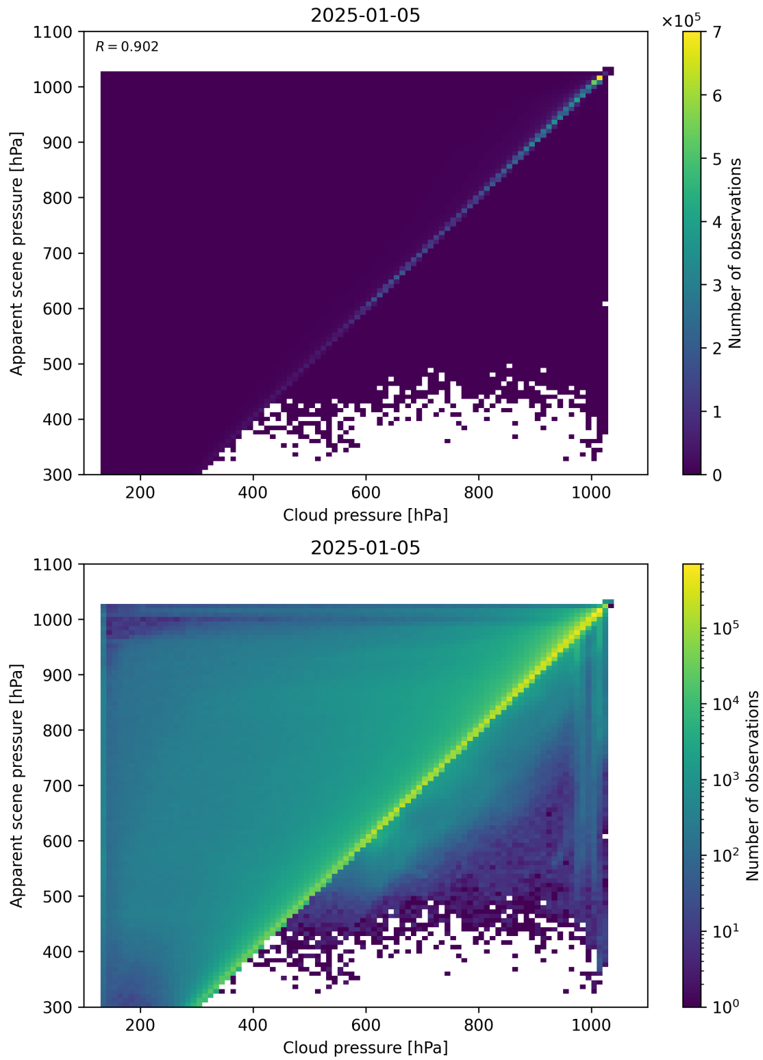
Figure 77: Scatter density plot of “Cloud pressure” against “Apparent scene pressure” for 2025-01-04 to 2025-01-06.
