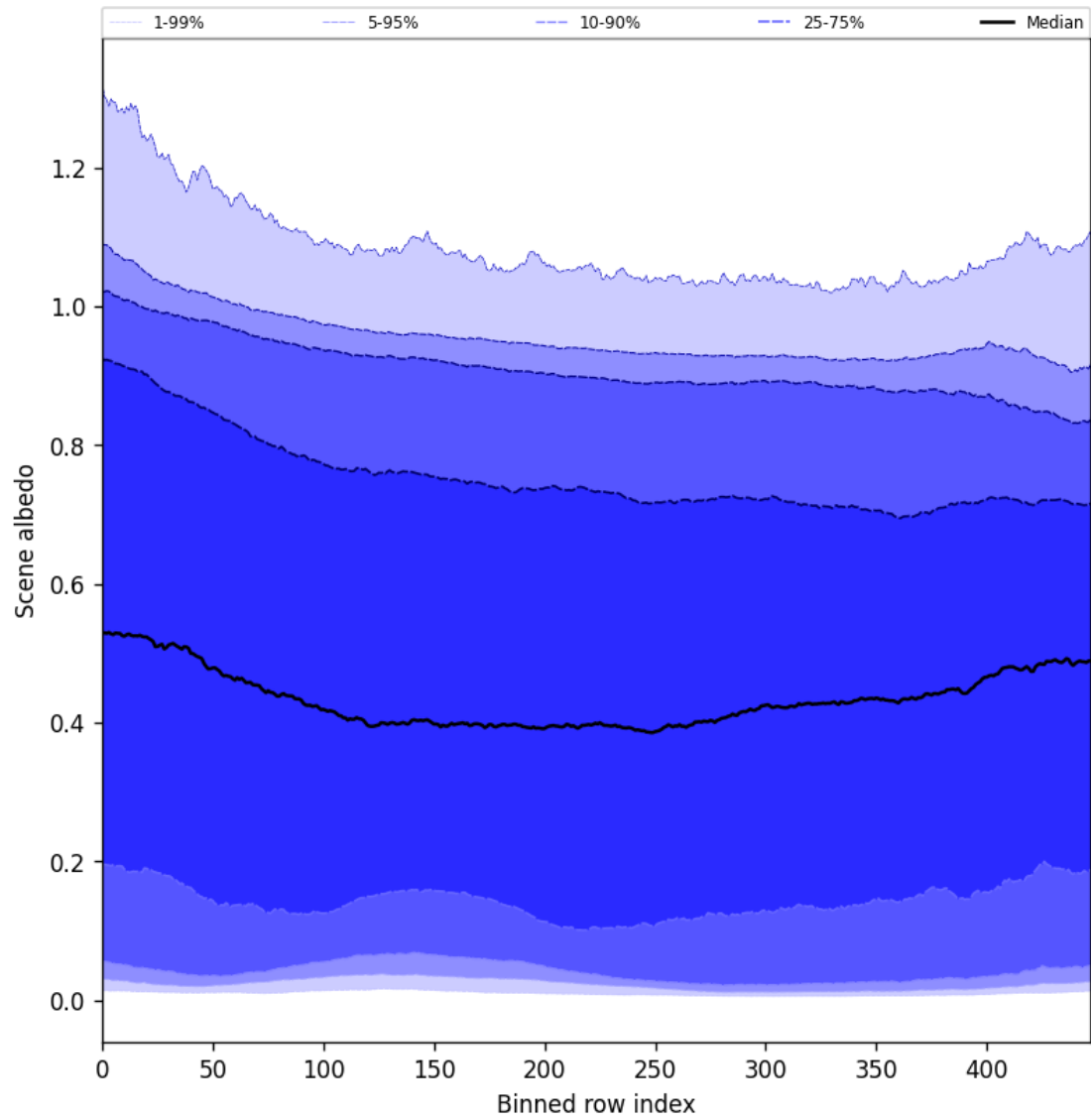
Figure 51: Along track statistics of “Scene albedo” for 2025-01-04 to 2025-01-06
