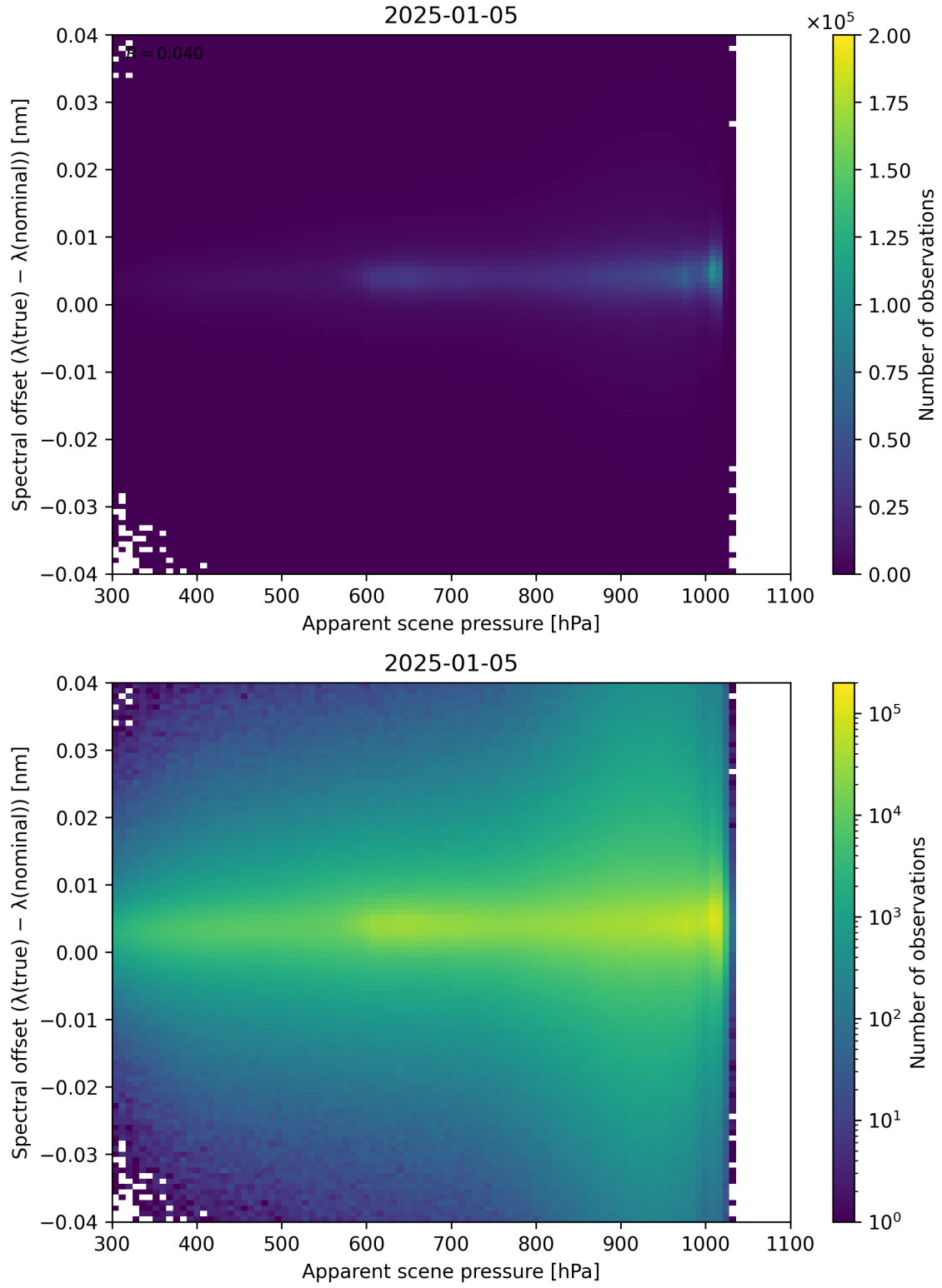
Figure 67: Scatter density plot of “Apparent scene pressure” against “Spectral offset ( \lambda_{\text{true}} - \lambda_{\text{nominal}} )” for 2025-01-04 to 2025-01-06.
