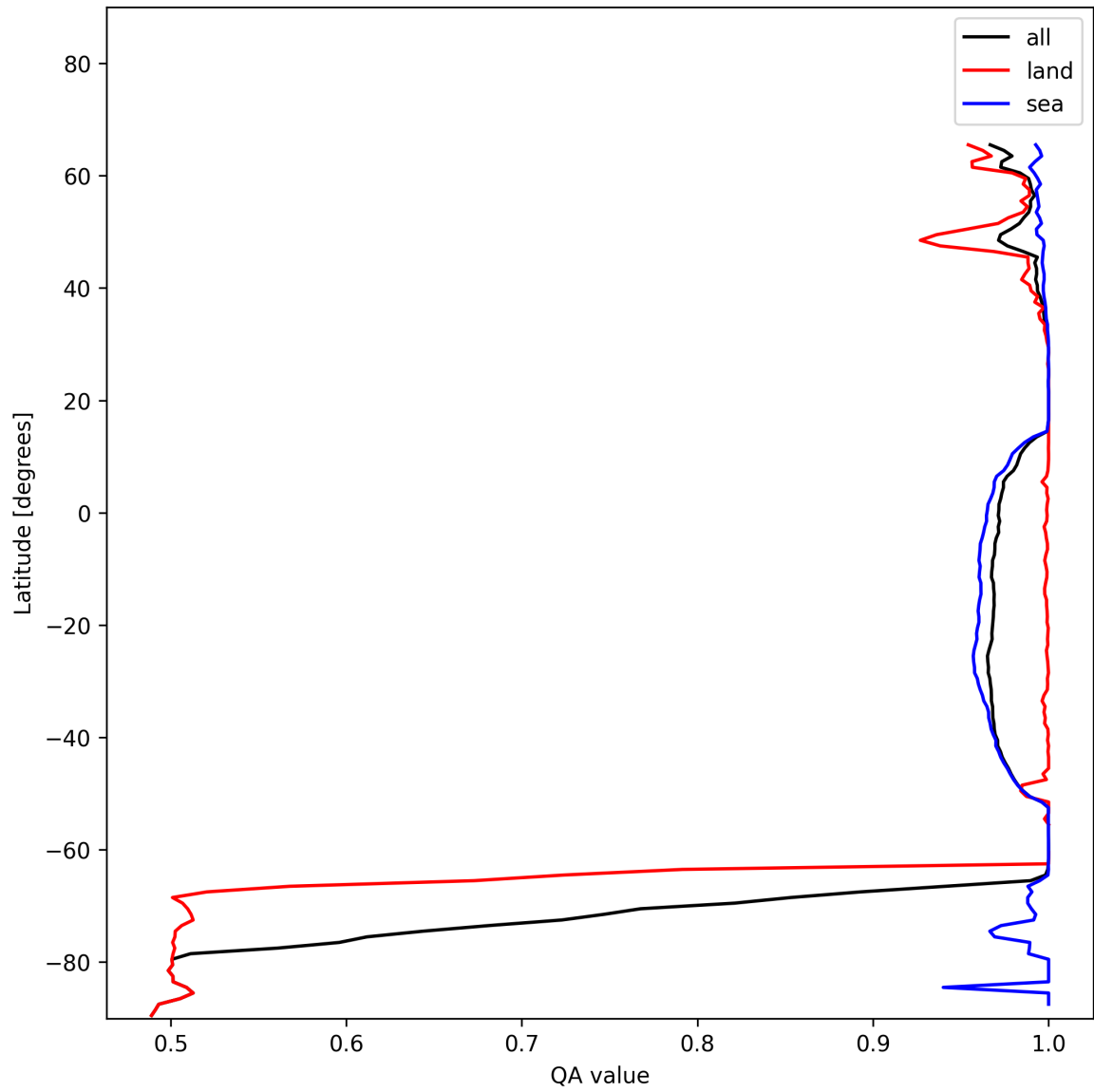
Figure 12: Zonal average of “QA value” for 2025-01-04 to 2025-01-06.
