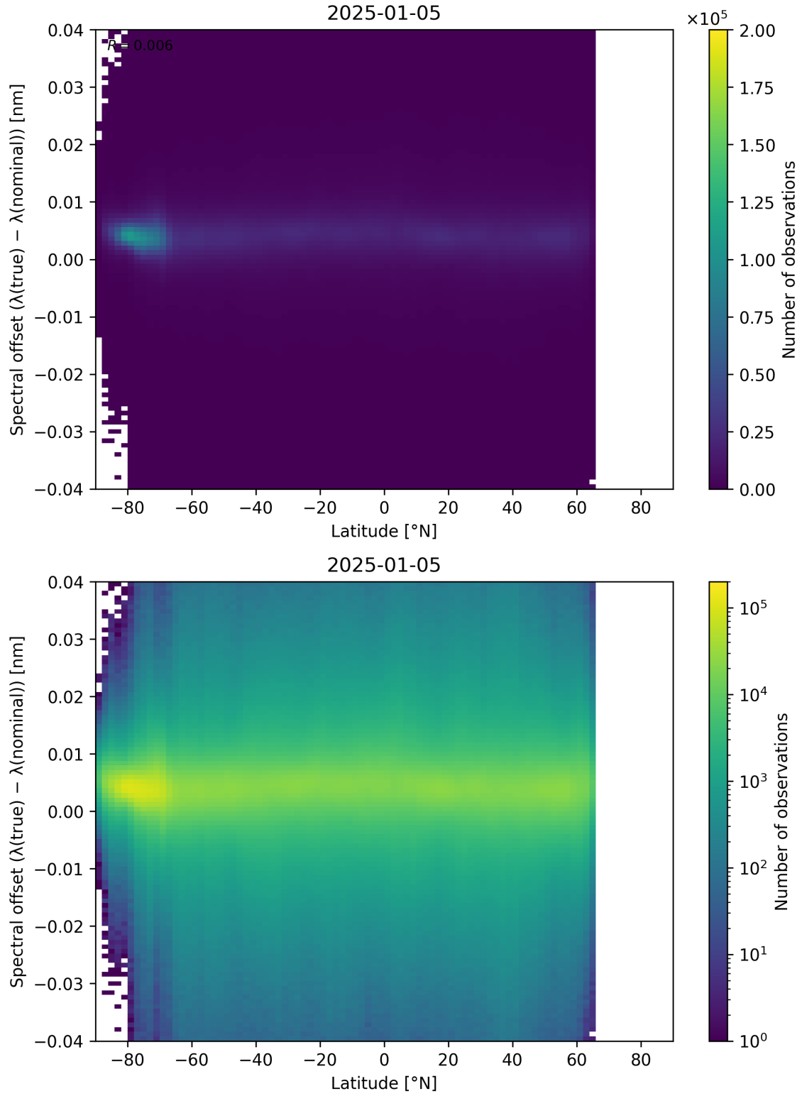
Figure 96: Scatter density plot of “Latitude” against “Spectral offset ( \lambda_{\text{true}} - \lambda_{\text{nominal}} )” for 2025-01-04 to 2025-01-06.
