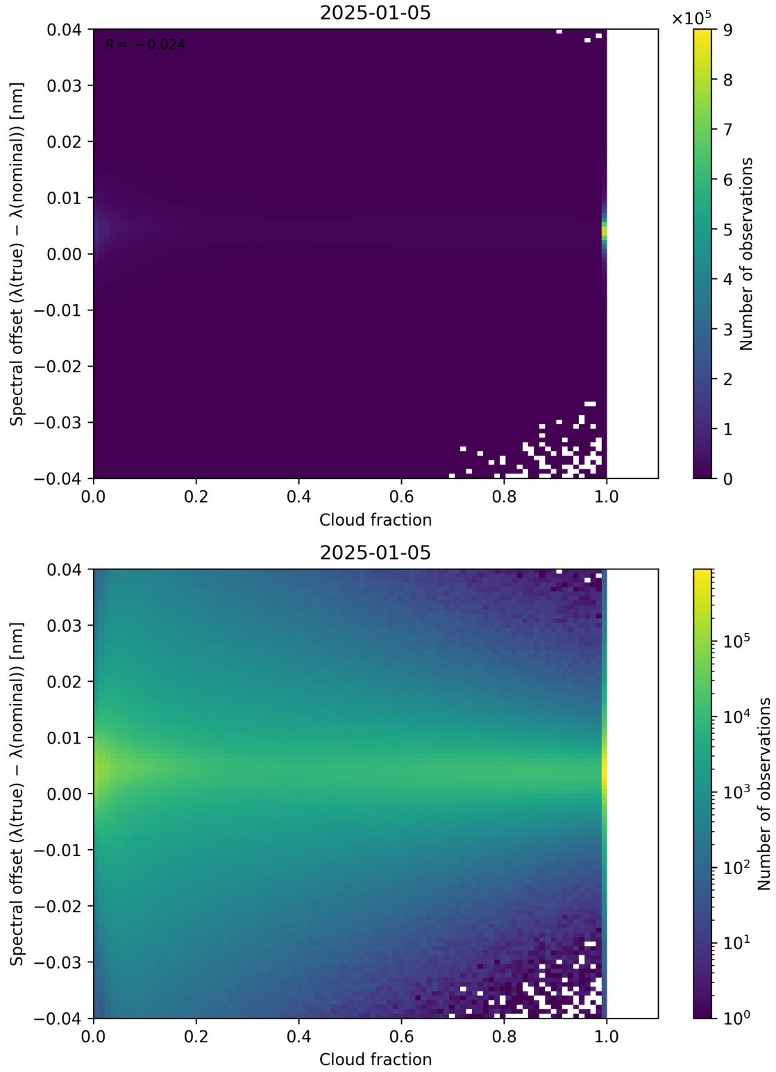
Figure 76: Scatter density plot of “Cloud fraction” against “Spectral offset ( \lambda_{\text{true}} - \lambda_{\text{nominal}} )” for 2025-01-04 to 2025-01-06.
