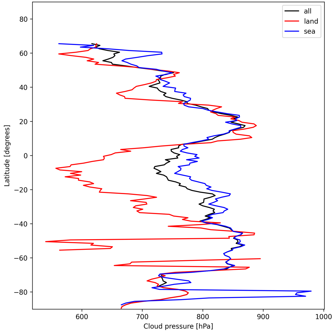
Figure 13: Zonal average of “Cloud pressure” for 2025-01-04 to 2025-01-06.
