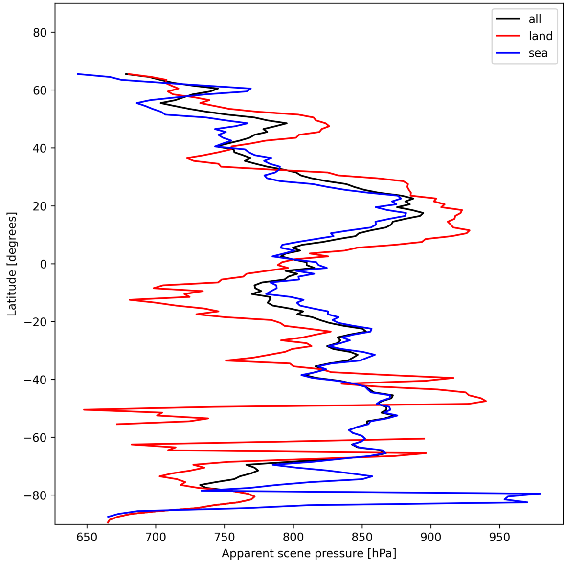
Figure 19: Zonal average of “Apparent scene pressure” for 2025-01-04 to 2025-01-06.
