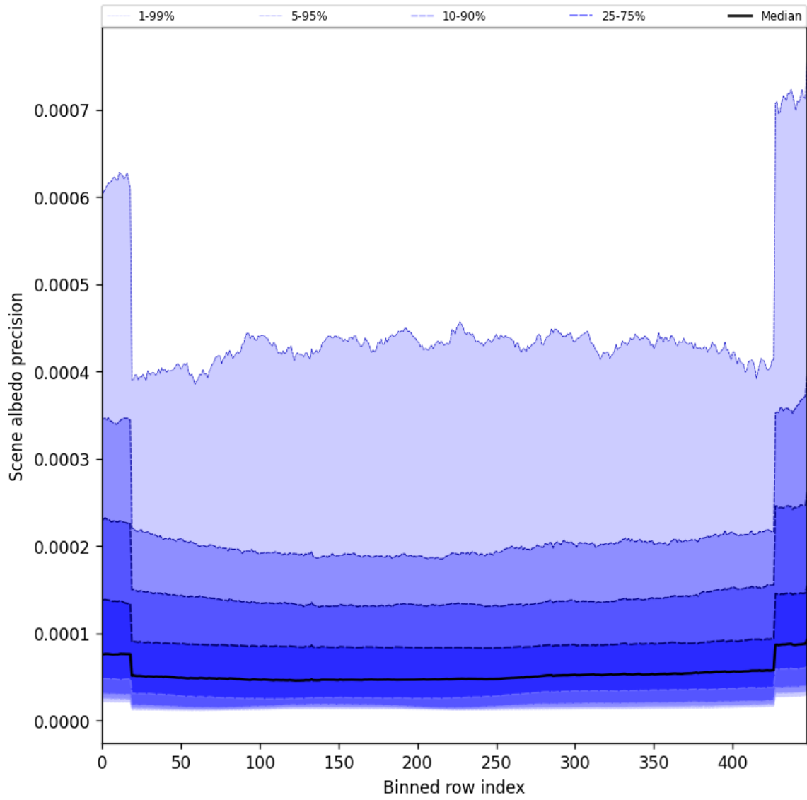
Figure 52: Along track statistics of “Scene albedo precision” for 2025-01-04 to 2025-01-06
