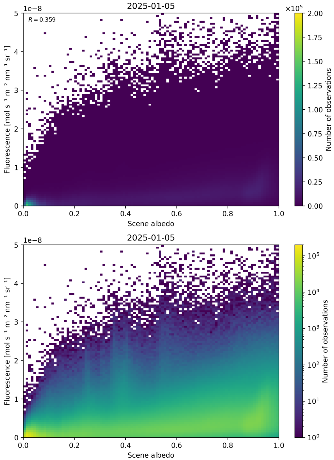
Figure 104: Scatter density plot of “Scene albedo” against “Fluorescence” for 2025-01-04 to 2025-01-06.
