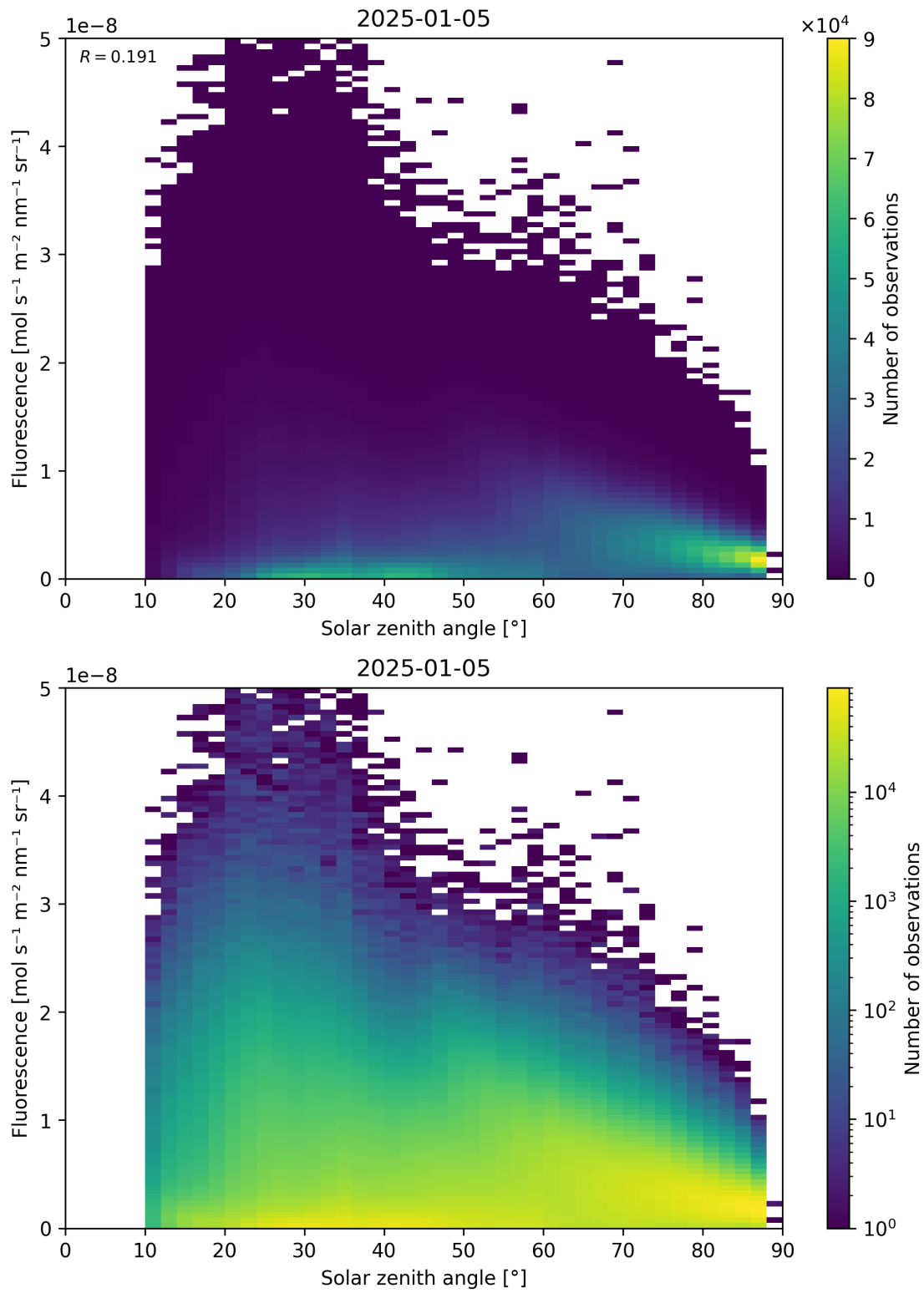
Figure 112: Scatter density plot of “Solar zenith angle” against “Fluorescence” for 2025-01-04 to 2025-01-06.
