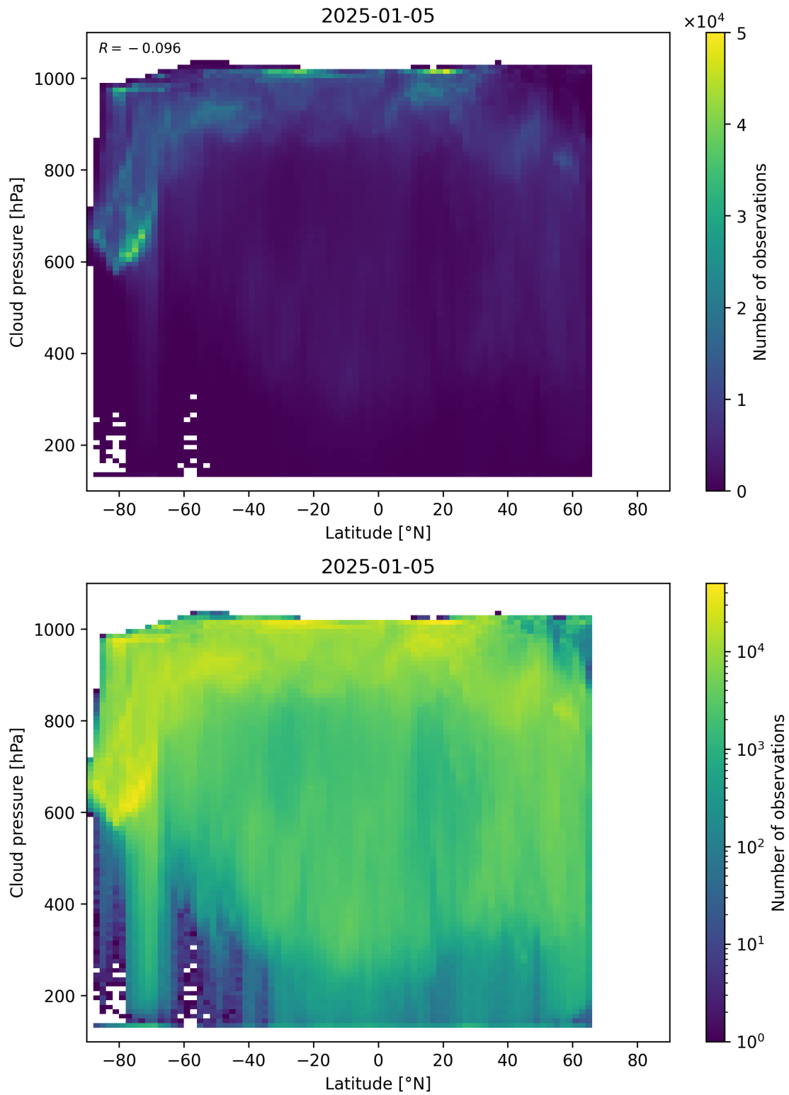
Figure 91: Scatter density plot of “Latitude” against “Cloud pressure” for 2025-01-04 to 2025-01-06.
