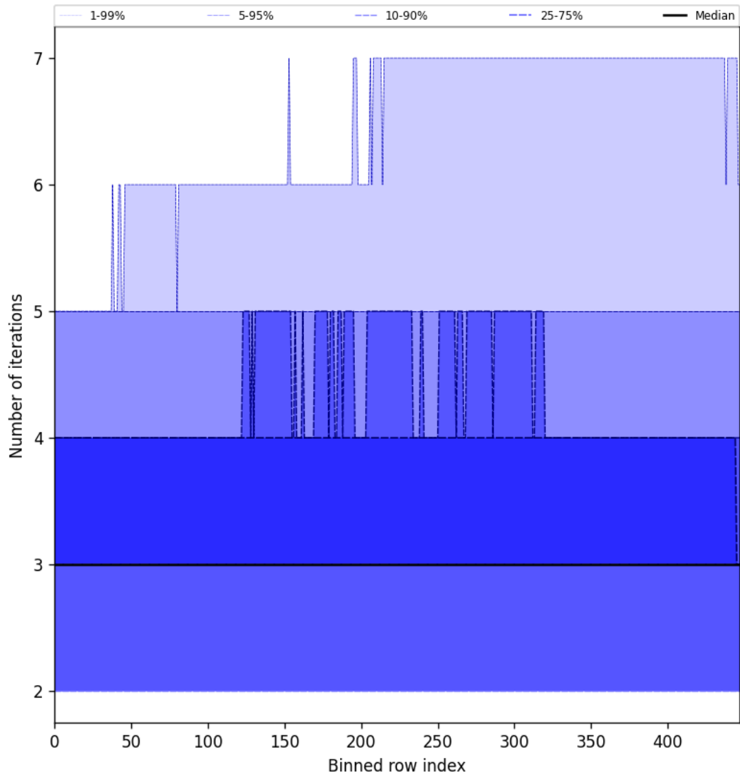
Figure 56: Along track statistics of “Number of iterations” for 2025-01-04 to 2025-01-06
