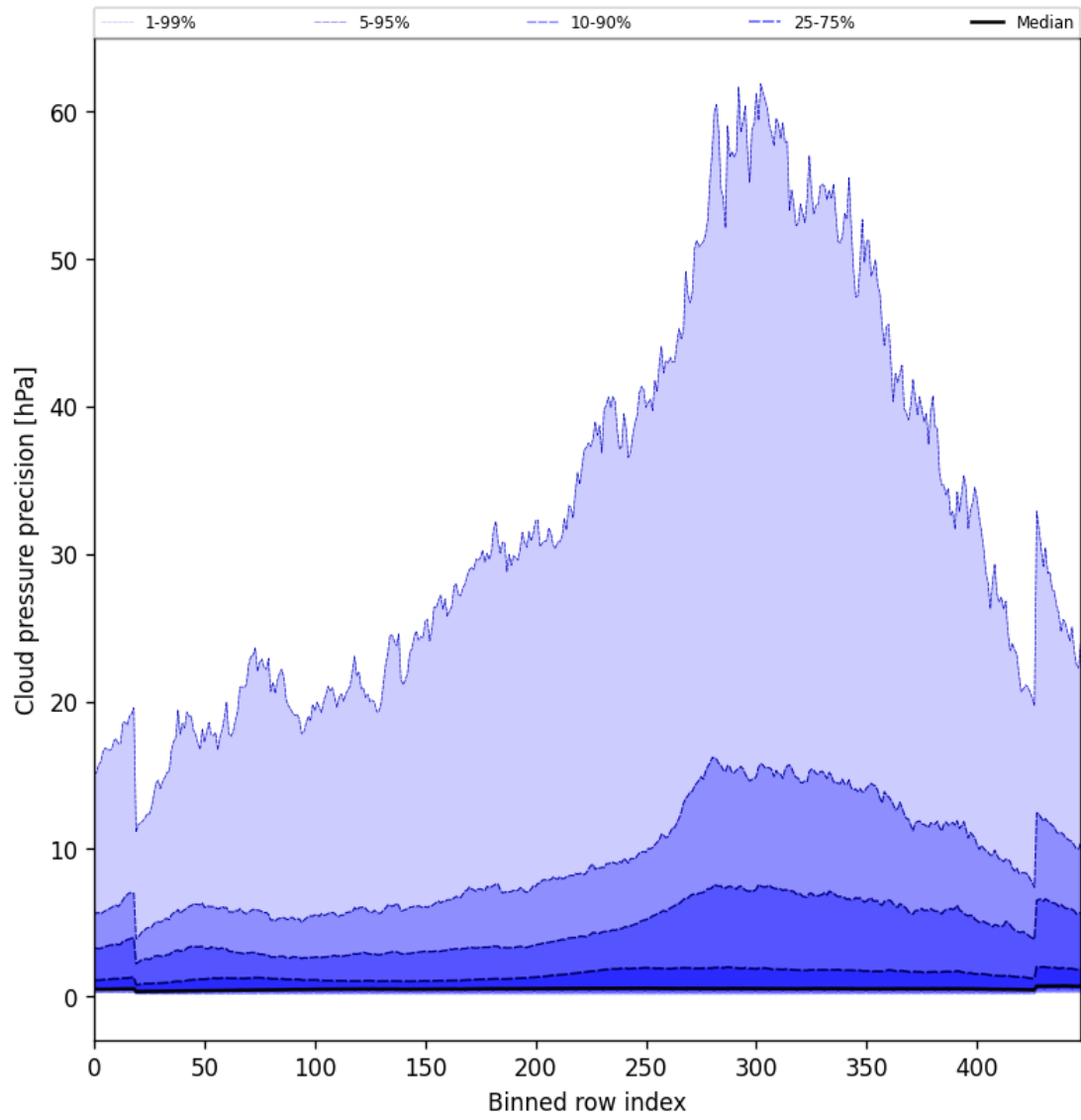
Figure 48: Along track statistics of “Cloud pressure precision” for 2025-01-04 to 2025-01-06
