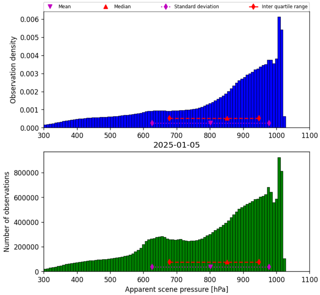
Figure 36: Histogram of “Apparent scene pressure” for 2025-01-04 to 2025-01-06
