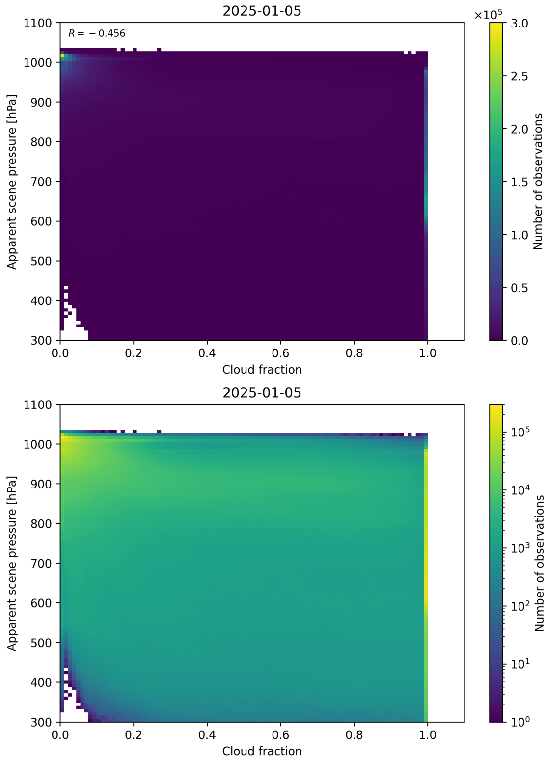
Figure 70: Scatter density plot of “Cloud fraction” against “Apparent scene pressure” for 2025-01-04 to 2025-01-06.
