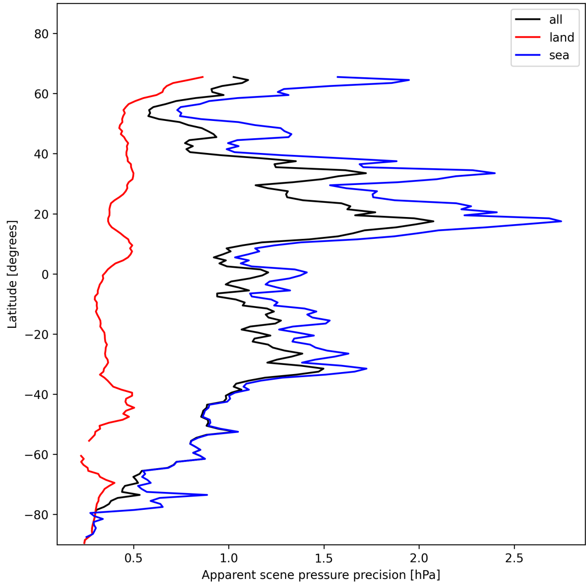
Figure 20: Zonal average of “Apparent scene pressure precision” for 2025-01-04 to 2025-01-06.
