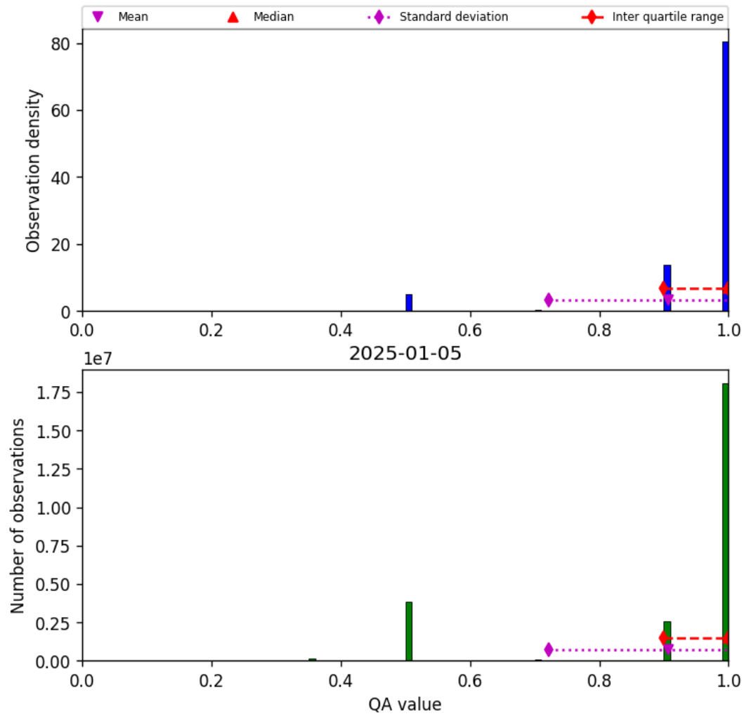
Figure 29: Histogram of “QA value” for 2025-01-04 to 2025-01-06
