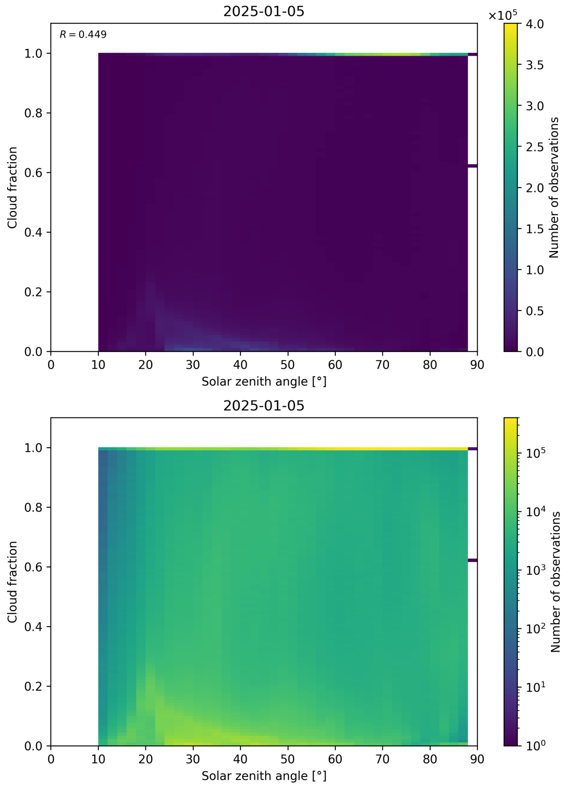
Figure 110: Scatter density plot of “Solar zenith angle” against “Cloud fraction” for 2025-01-04 to 2025-01-06.
