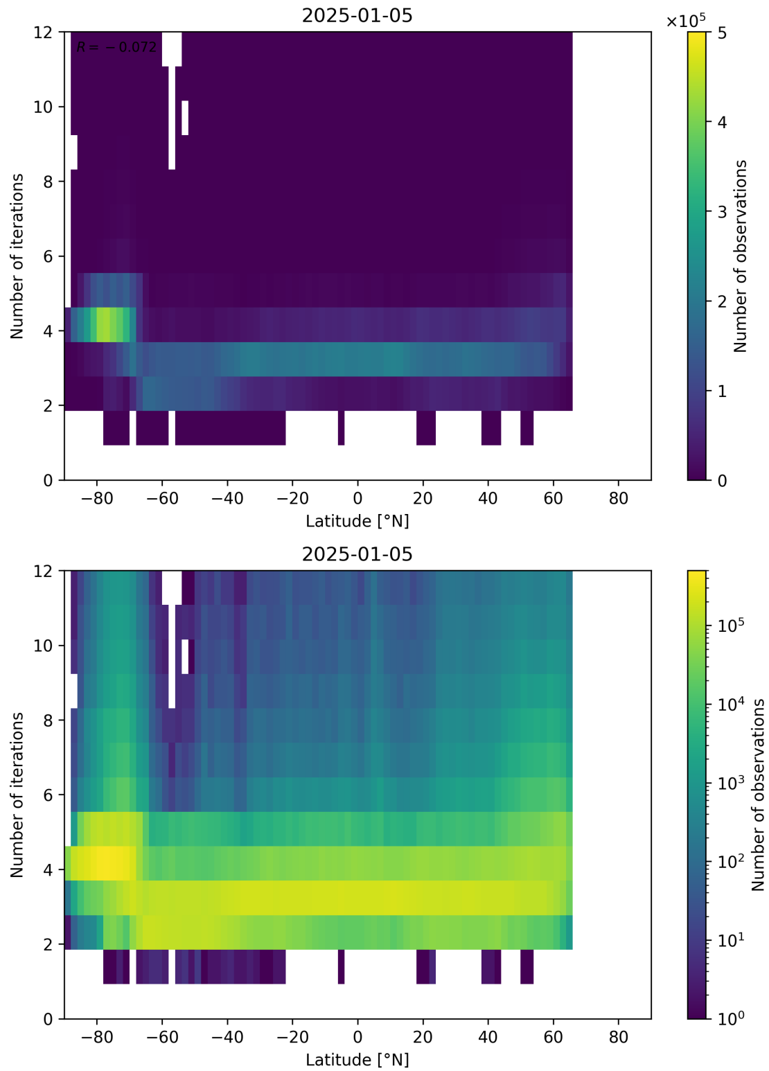
Figure 93: Scatter density plot of “Latitude” against “Number of iterations” for 2025-01-04 to 2025-01-06.
