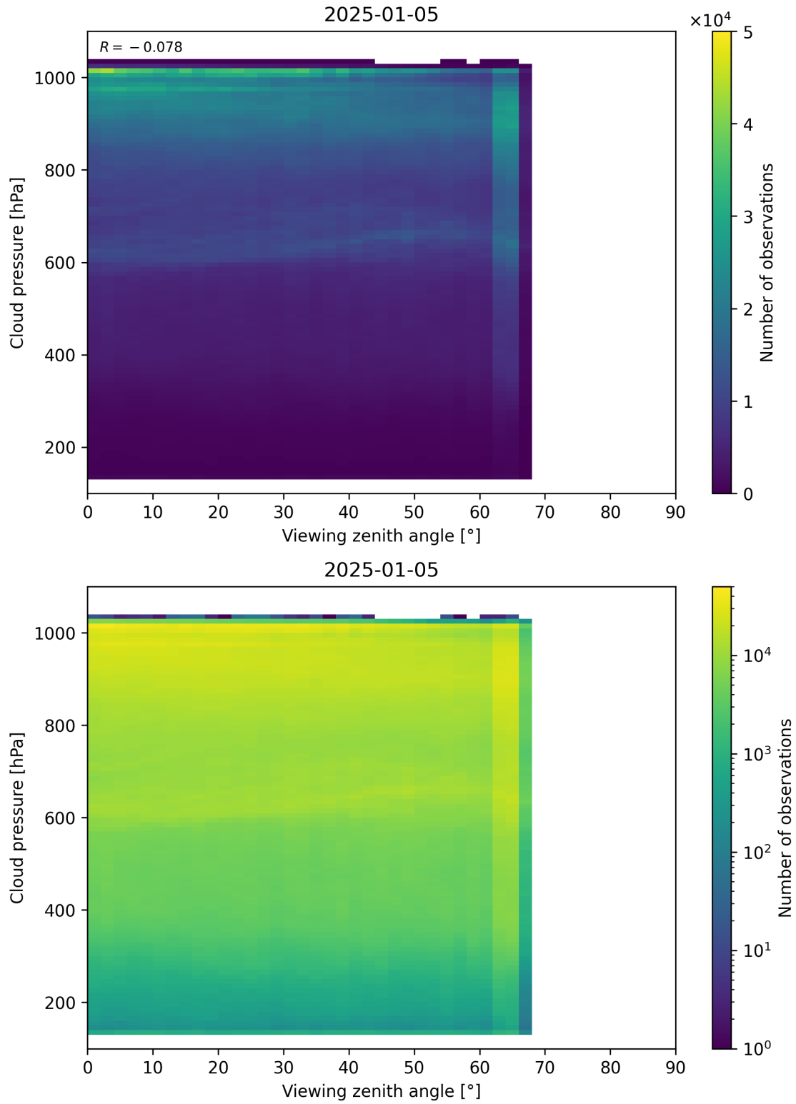
Figure 121: Scatter density plot of “Viewing zenith angle” against “Cloud pressure” for 2025-01-04 to 2025-01-06.
