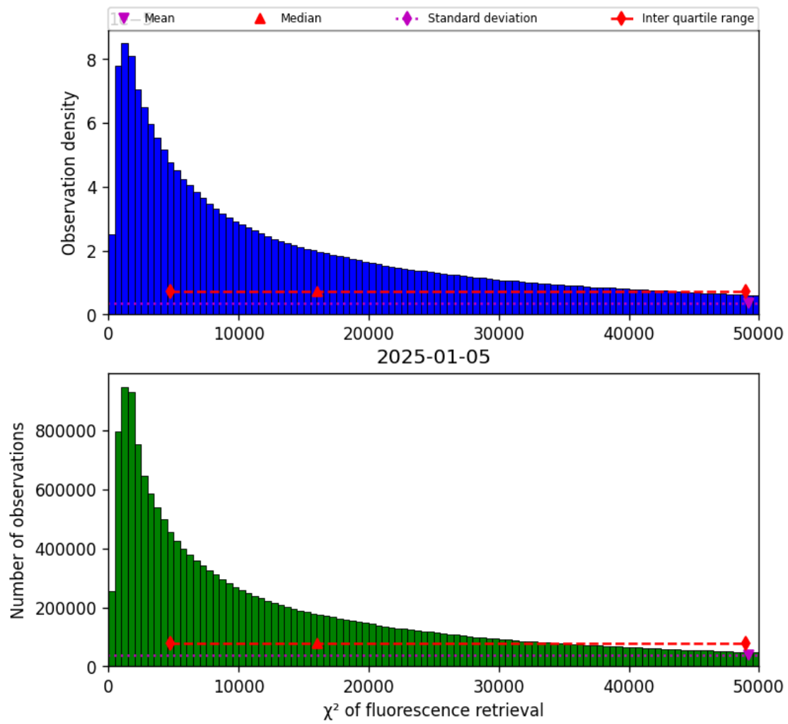
Figure 42: Histogram of “ \chi^2 of fluorescence retrieval” for 2025-01-04 to 2025-01-06
