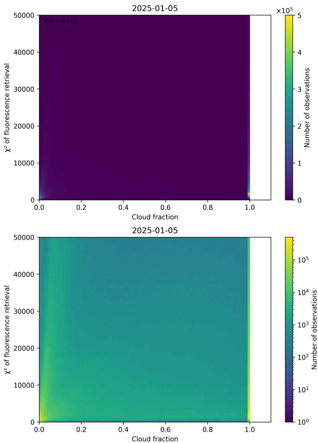
Figure 71: Scatter density plot of “Cloud fraction” against “ \chi^2 of fluorescence retrieval” for 2025-01-04 to 2025-01-06.
