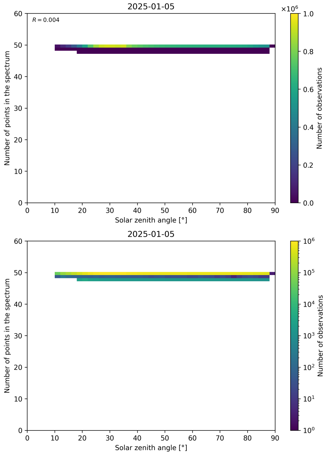
Figure 115: Scatter density plot of “Solar zenith angle” against “Number of points in the spectrum” for 2025-01-04 to 2025-01-06.
