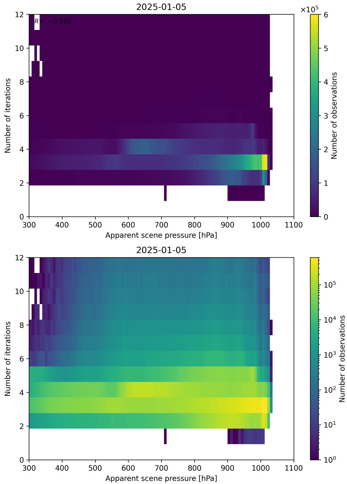
Figure 65: Scatter density plot of “Apparent scene pressure” against “Number of iterations” for 2025-01-04 to 2025-01-06.
