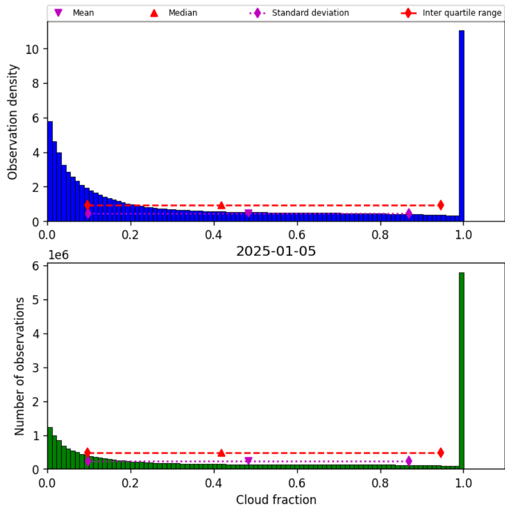
Figure 32: Histogram of “Cloud fraction” for 2025-01-04 to 2025-01-06
