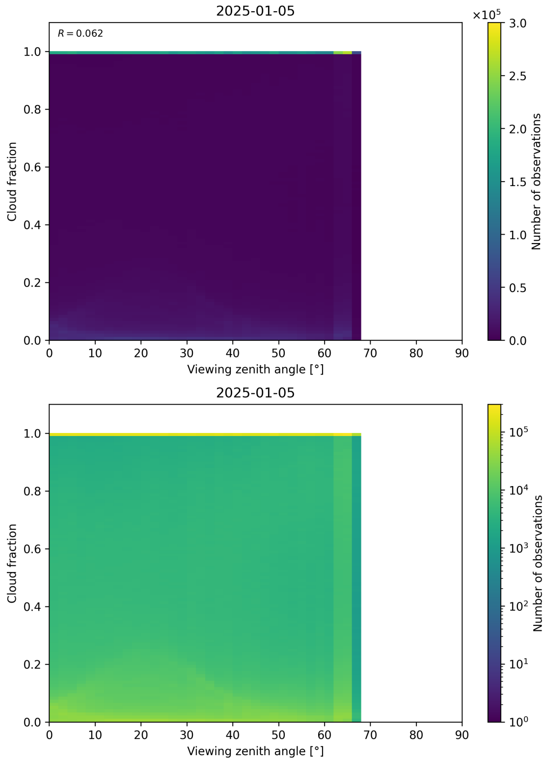
Figure 120: Scatter density plot of “Viewing zenith angle” against “Cloud fraction” for 2025-01-04 to 2025-01-06.
