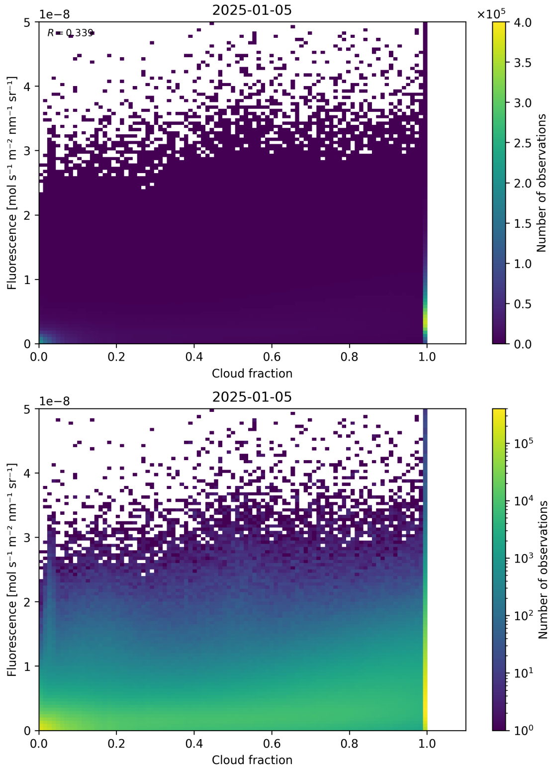
Figure 72: Scatter density plot of “Cloud fraction” against “Fluorescence” for 2025-01-04 to 2025-01-06.
