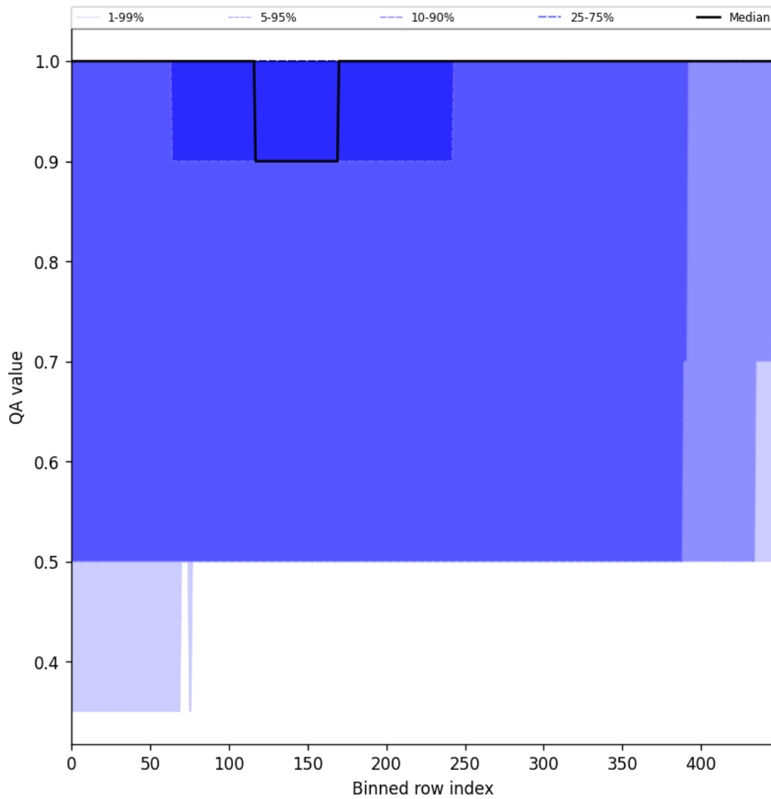
Figure 46: Along track statistics of “QA value” for 2025-01-04 to 2025-01-06
