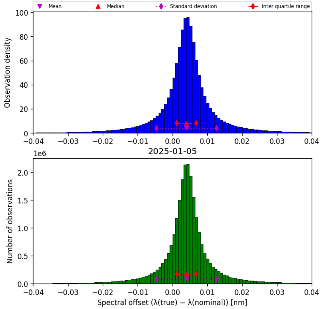
Figure 45: Histogram of “Spectral offset ( \lambda_{\text{true}} - \lambda_{\text{nominal}} )” for 2025-01-04 to 2025-01-06
