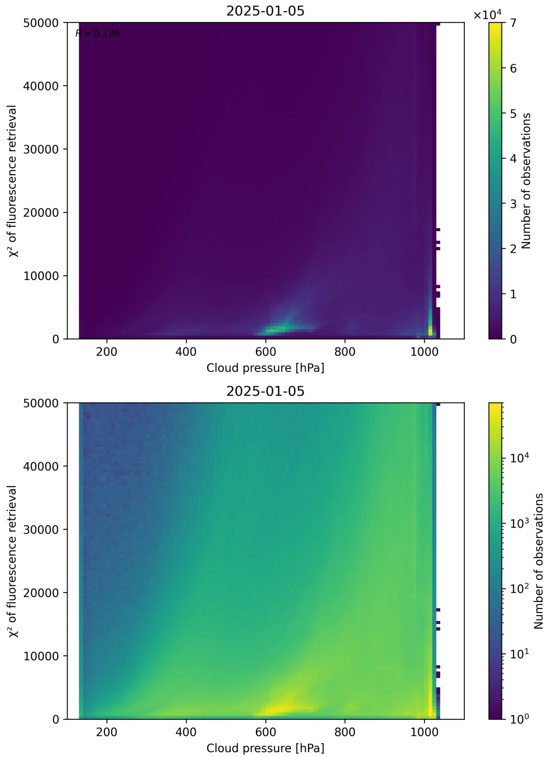
Figure 78: Scatter density plot of “Cloud pressure” against “ \chi^2 of fluorescence retrieval” for 2025-01-04 to 2025-01-06.
