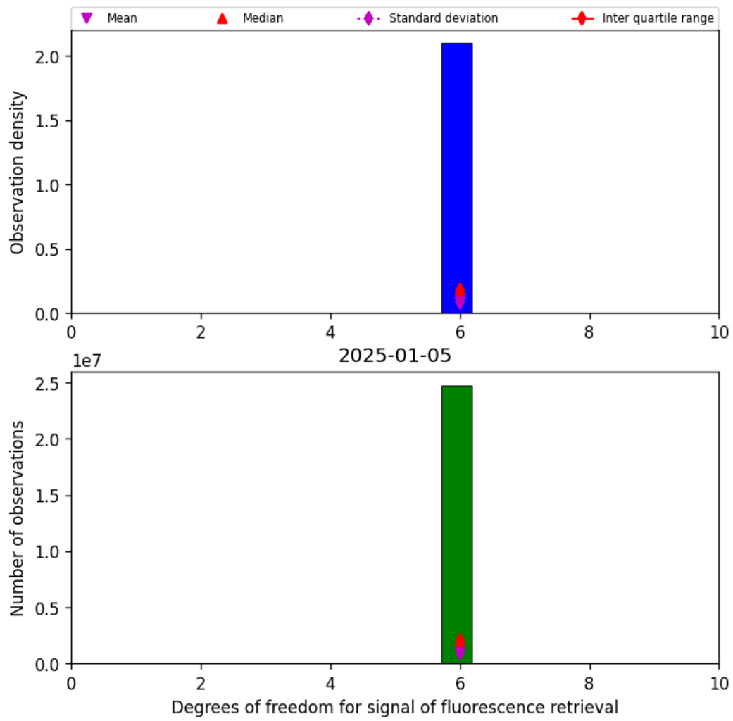
Figure 43: Histogram of “Degrees of freedom for signal of fluorescence retrieval” for 2025-01-04 to 2025-01-06
