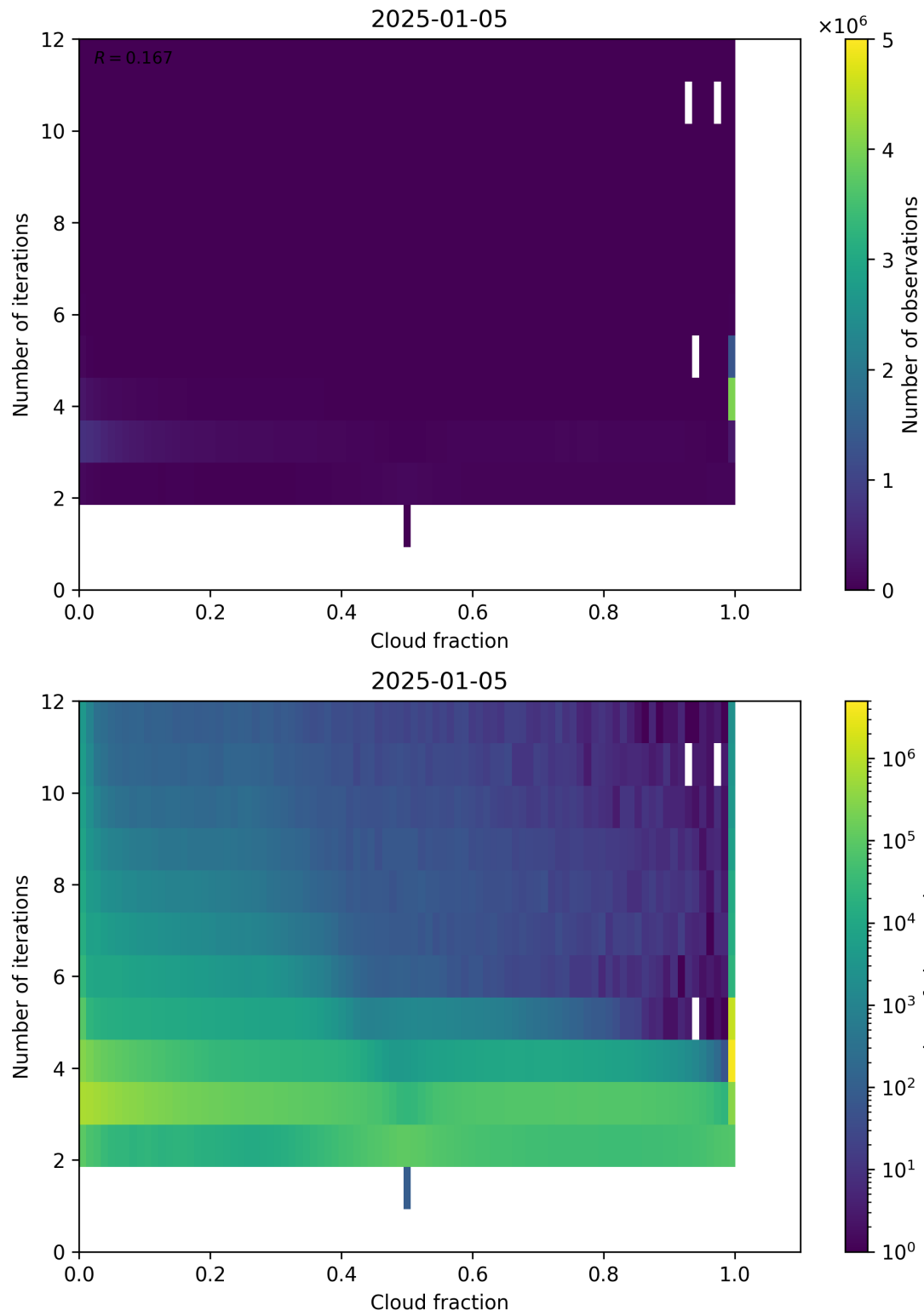
Figure 73: Scatter density plot of “Cloud fraction” against “Number of iterations” for 2025-01-04 to 2025-01-06.
