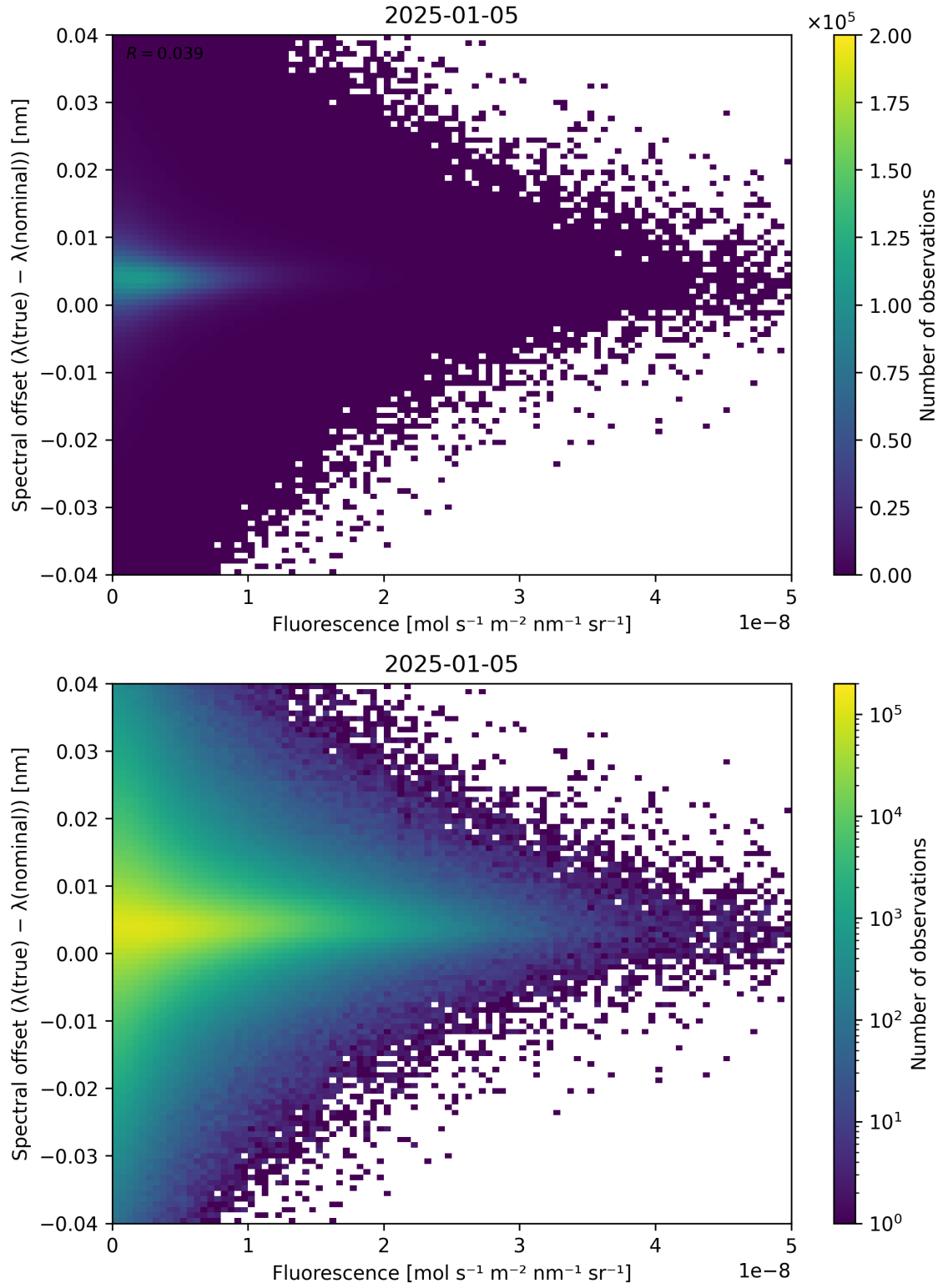
Figure 87: Scatter density plot of “Fluorescence” against “Spectral offset ( \lambda_{\text{true}} - \lambda_{\text{nominal}} )” for 2025-01-04 to 2025-01-06.
