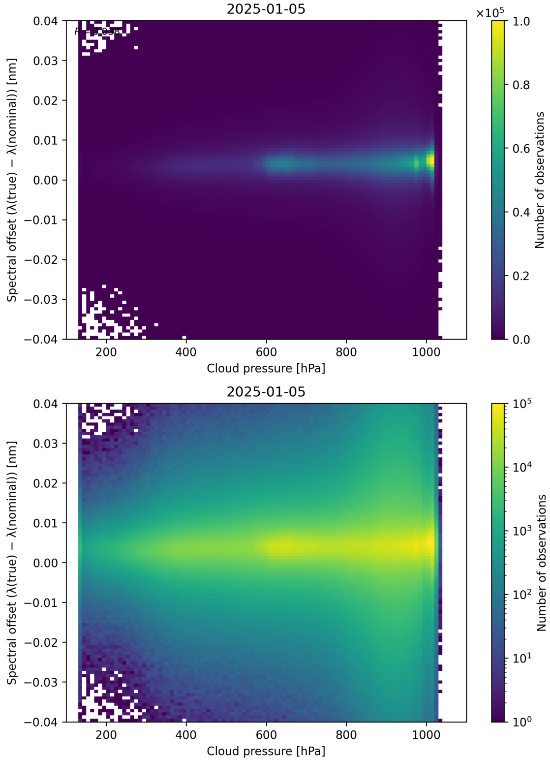
Figure 84: Scatter density plot of “Cloud pressure” against “Spectral offset ( \lambda_{\text{true}} - \lambda_{\text{nominal}} )” for 2025-01-04 to 2025-01-06.
