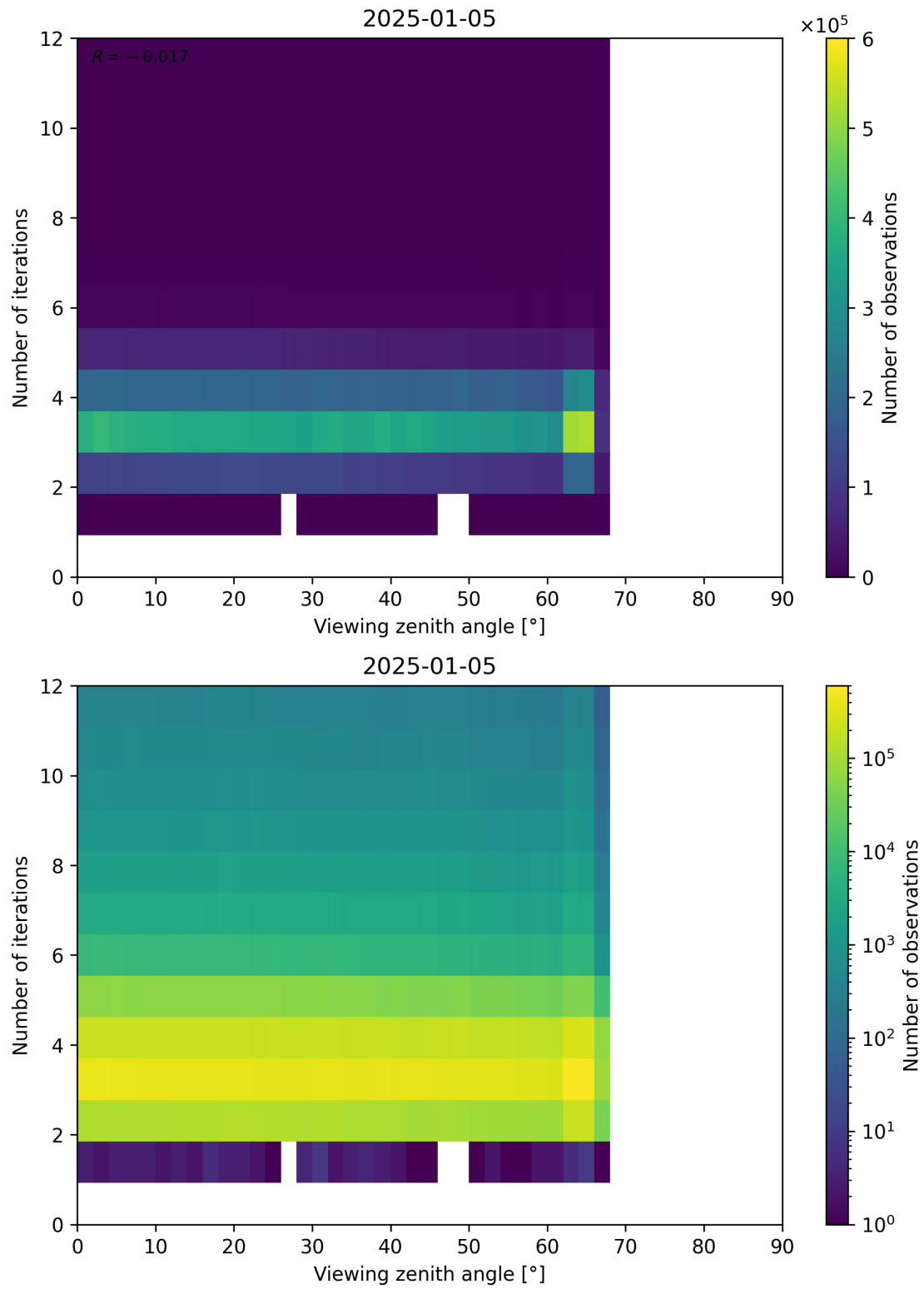
Figure 124: Scatter density plot of “Viewing zenith angle” against “Number of iterations” for 2025-01-04 to 2025-01-06.
