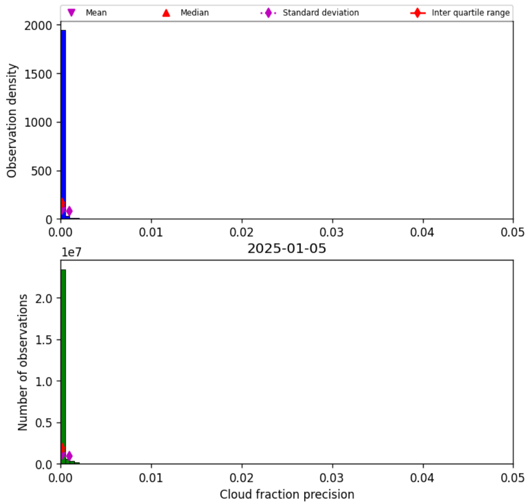
Figure 33: Histogram of “Cloud fraction precision” for 2025-01-04 to 2025-01-06
