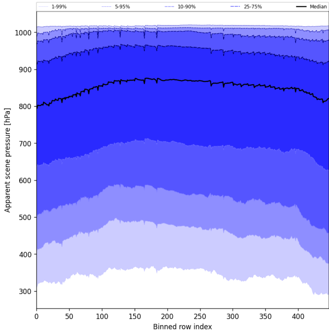
Figure 53: Along track statistics of “Apparent scene pressure” for 2025-01-04 to 2025-01-06
