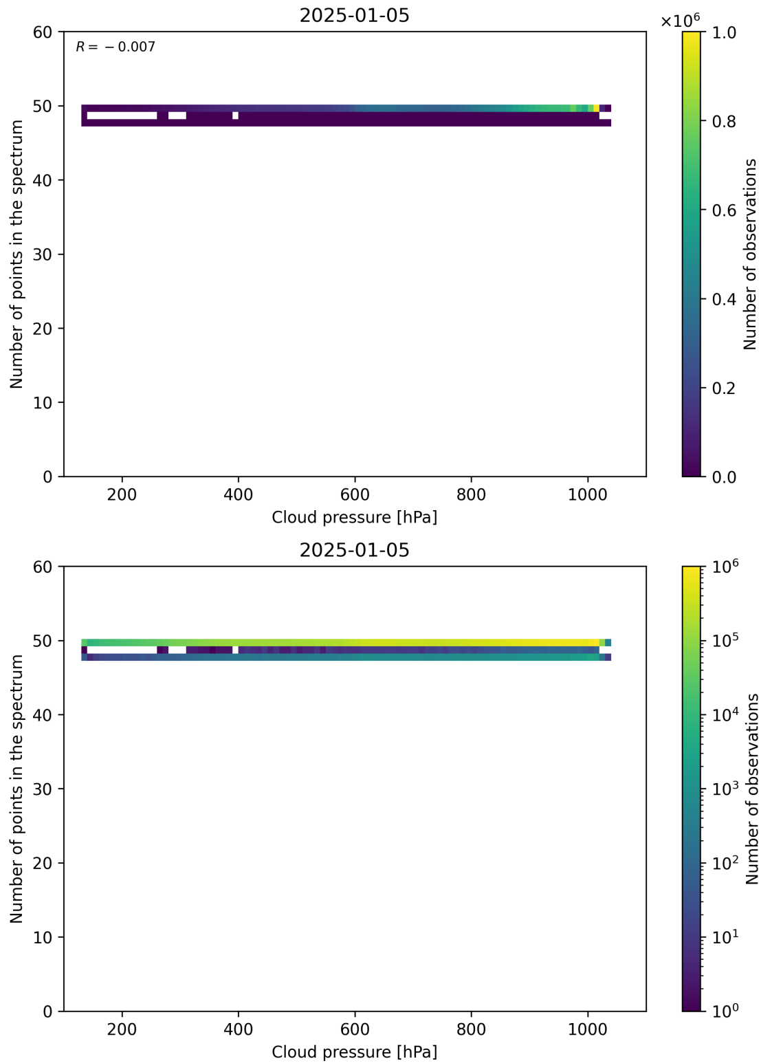
Figure 82: Scatter density plot of “Cloud pressure” against “Number of points in the spectrum” for 2025-01-04 to 2025-01-06.
