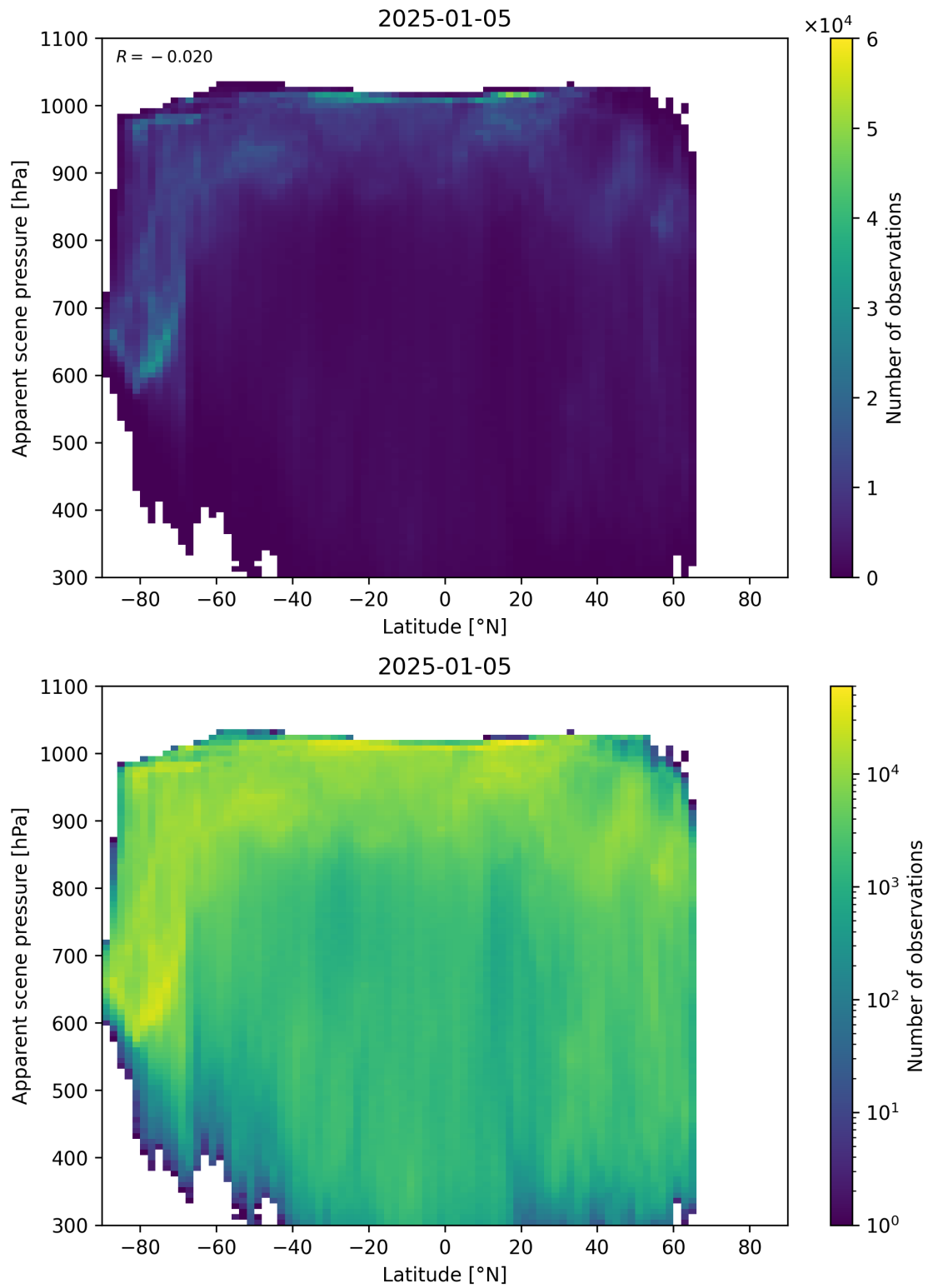
Figure 88: Scatter density plot of “Latitude” against “Apparent scene pressure” for 2025-01-04 to 2025-01-06.
