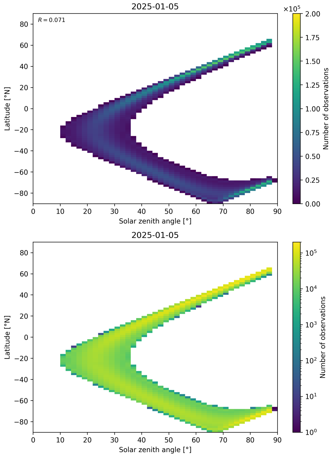
Figure 113: Scatter density plot of “Solar zenith angle” against “Latitude” for 2025-01-04 to 2025-01-06.
