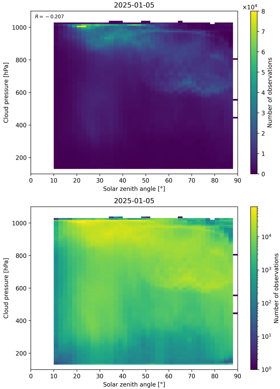
Figure 111: Scatter density plot of “Solar zenith angle” against “Cloud pressure” for 2025-01-04 to 2025-01-06.
