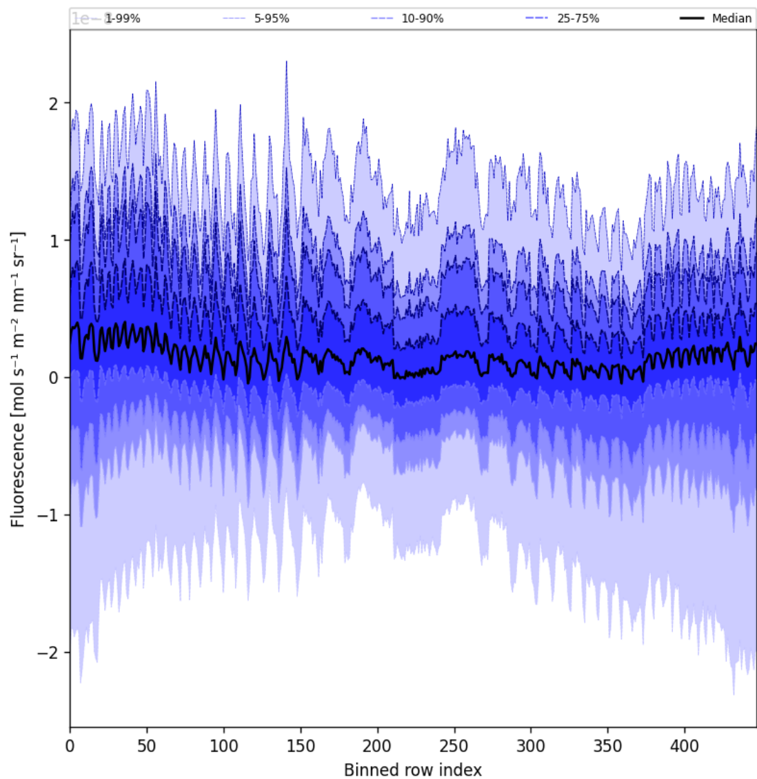
Figure 57: Along track statistics of “Fluorescence” for 2025-01-04 to 2025-01-06
