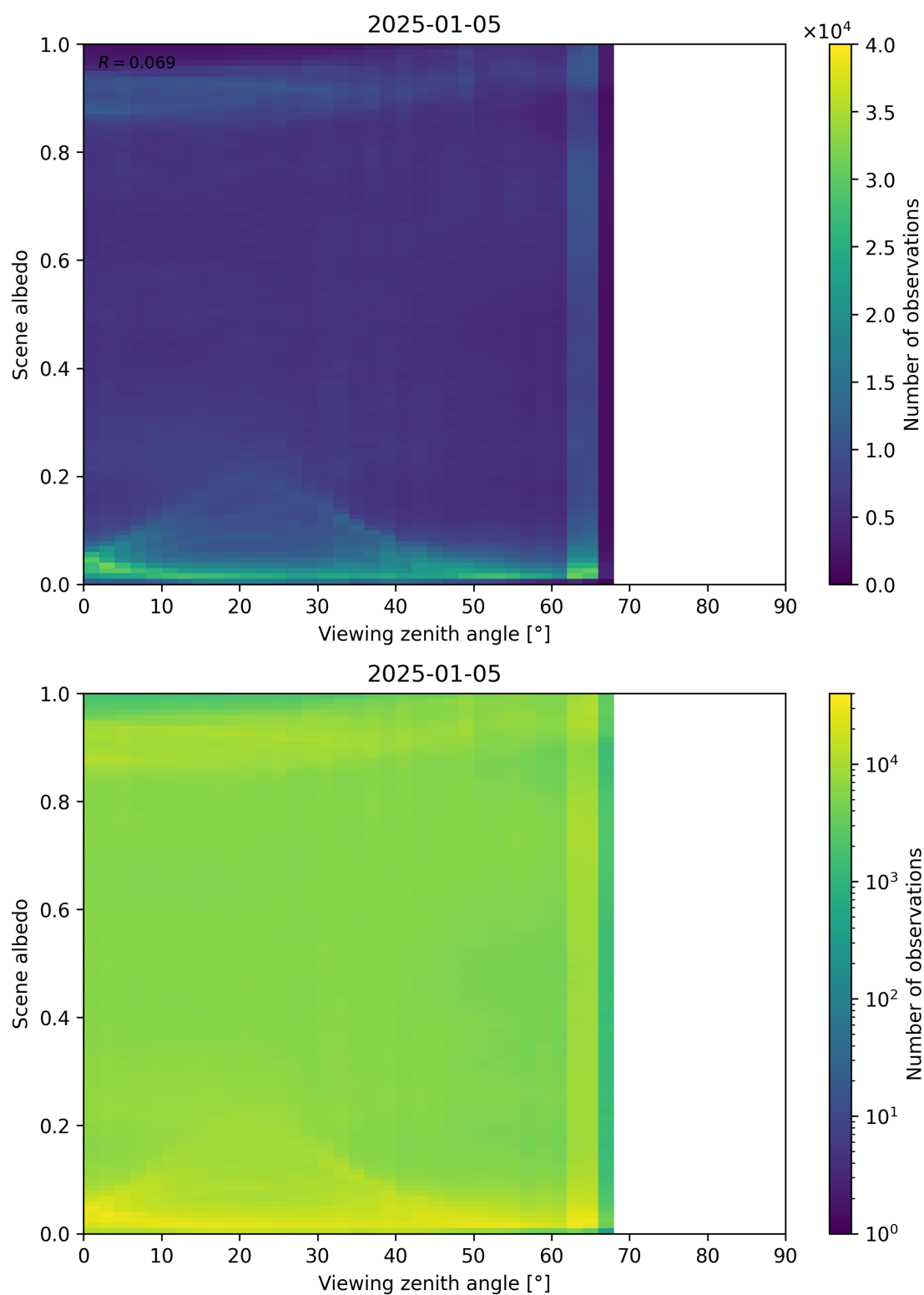
Figure 126: Scatter density plot of “Viewing zenith angle” against “Scene albedo” for 2025-01-04 to 2025-01-06.
