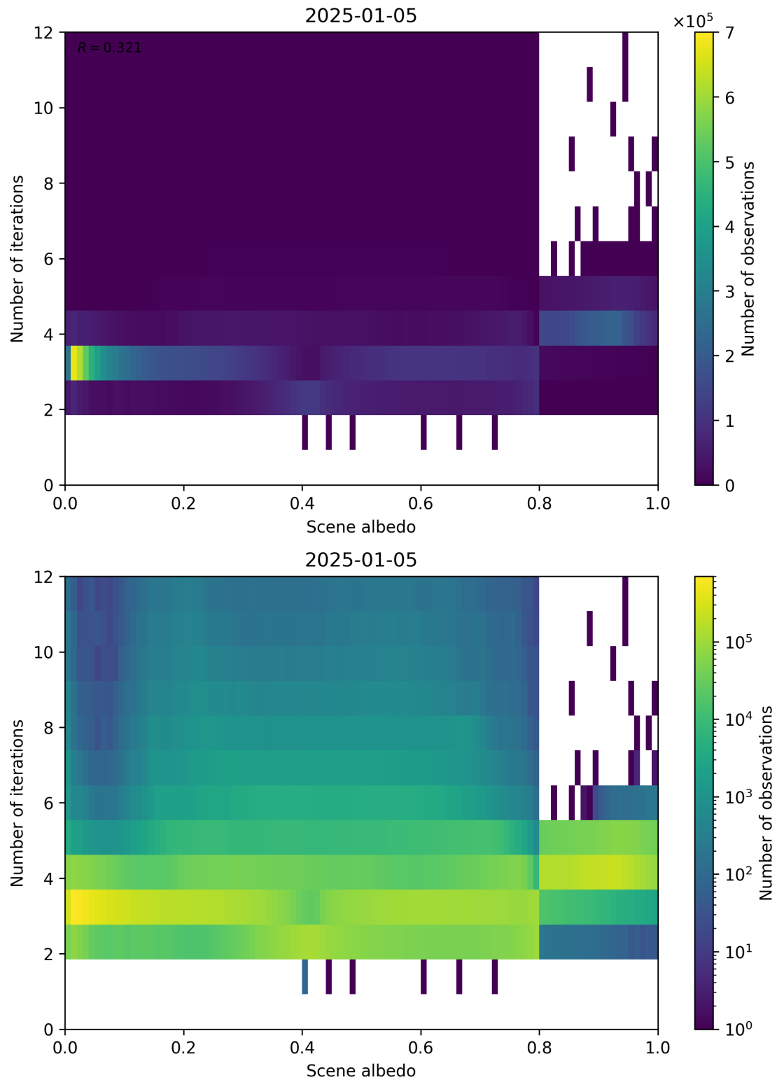
Figure 105: Scatter density plot of “Scene albedo” against “Number of iterations” for 2025-01-04 to 2025-01-06.
