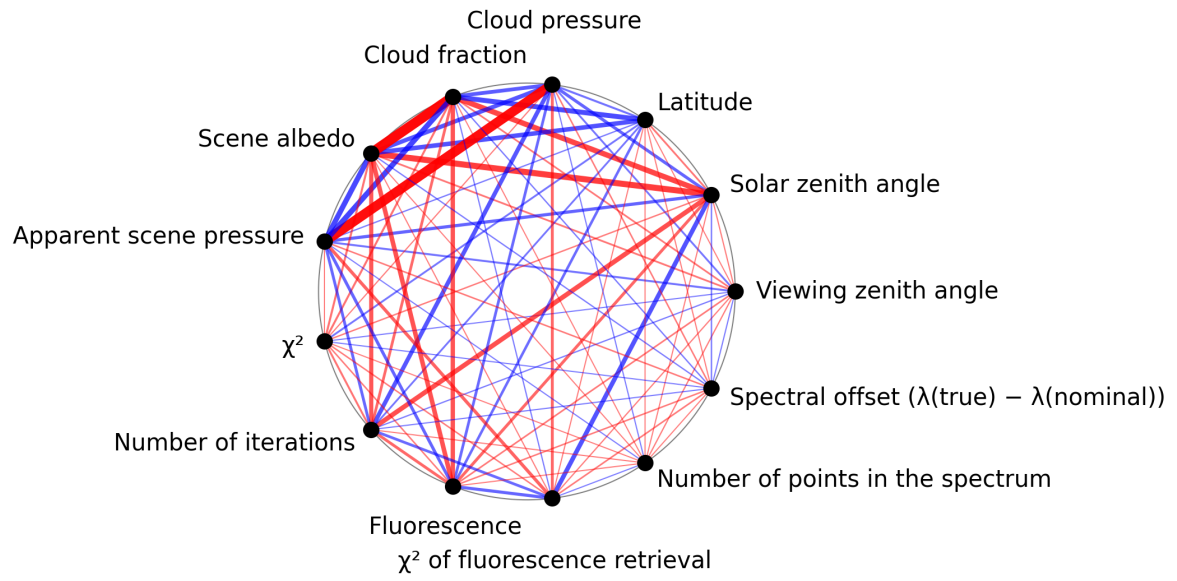
Figure 1: Map of correlation graph for 2025-01-04 to 2025-01-06.
