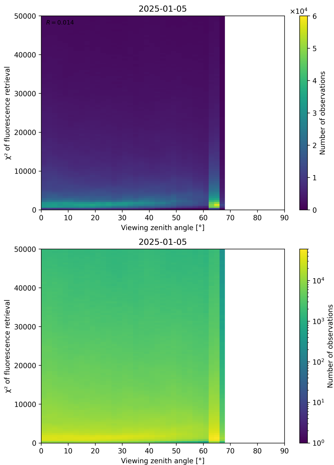
Figure 119: Scatter density plot of “Viewing zenith angle” against “ \chi^2 of fluorescence retrieval” for 2025-01-04 to 2025-01-06.
