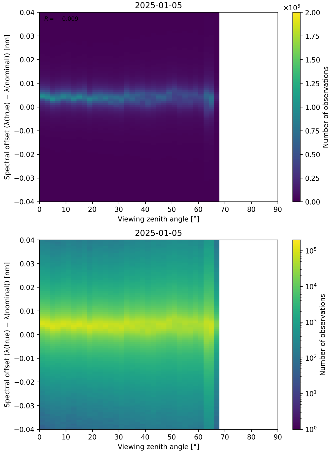
Figure 128: Scatter density plot of “Viewing zenith angle” against “Spectral offset ( \lambda_{\text{true}} - \lambda_{\text{nominal}} )” for 2025-01-04 to 2025-01-06.
