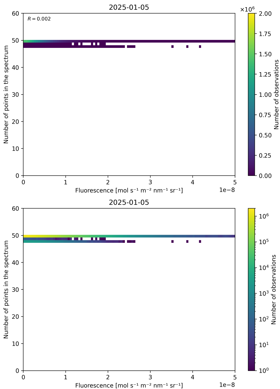
Figure 86: Scatter density plot of “Fluorescence” against “Number of points in the spectrum” for 2025-01-04 to 2025-01-06.
