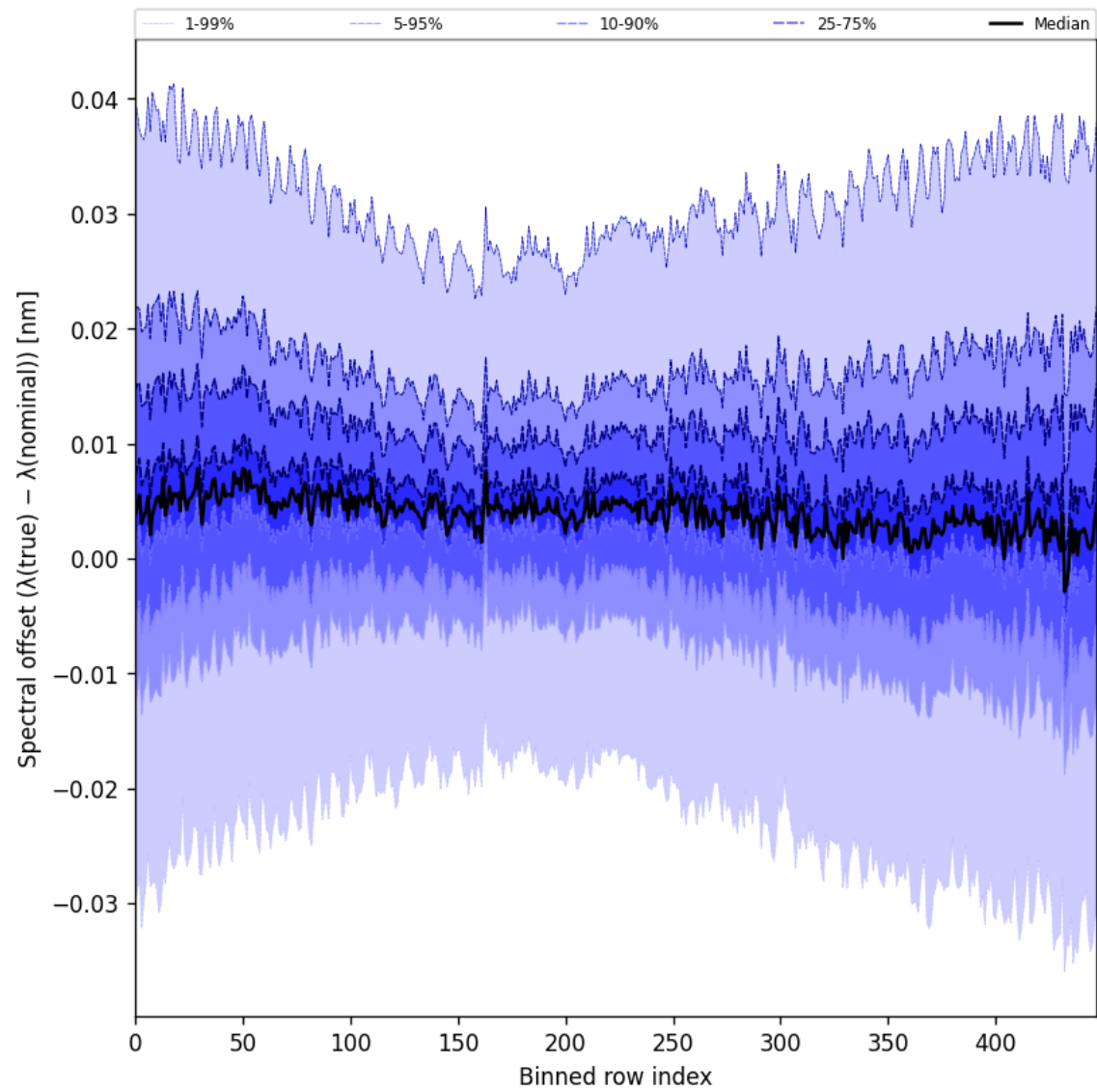
Figure 62: Along track statistics of “Spectral offset ( \lambda_{\text{true}} - \lambda_{\text{nominal}} )” for 2025-01-04 to 2025-01-06
