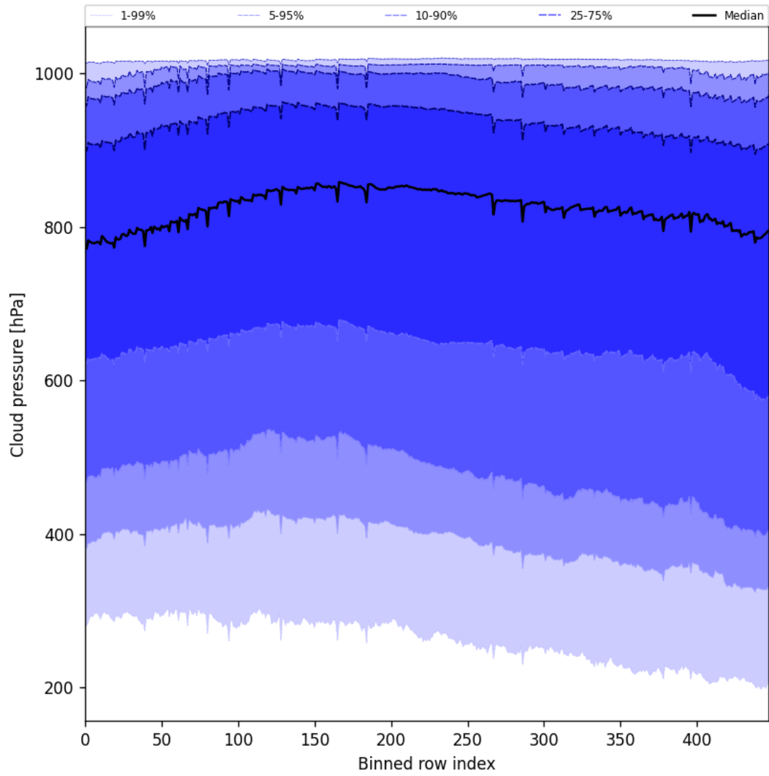
Figure 47: Along track statistics of “Cloud pressure” for 2025-01-04 to 2025-01-06
