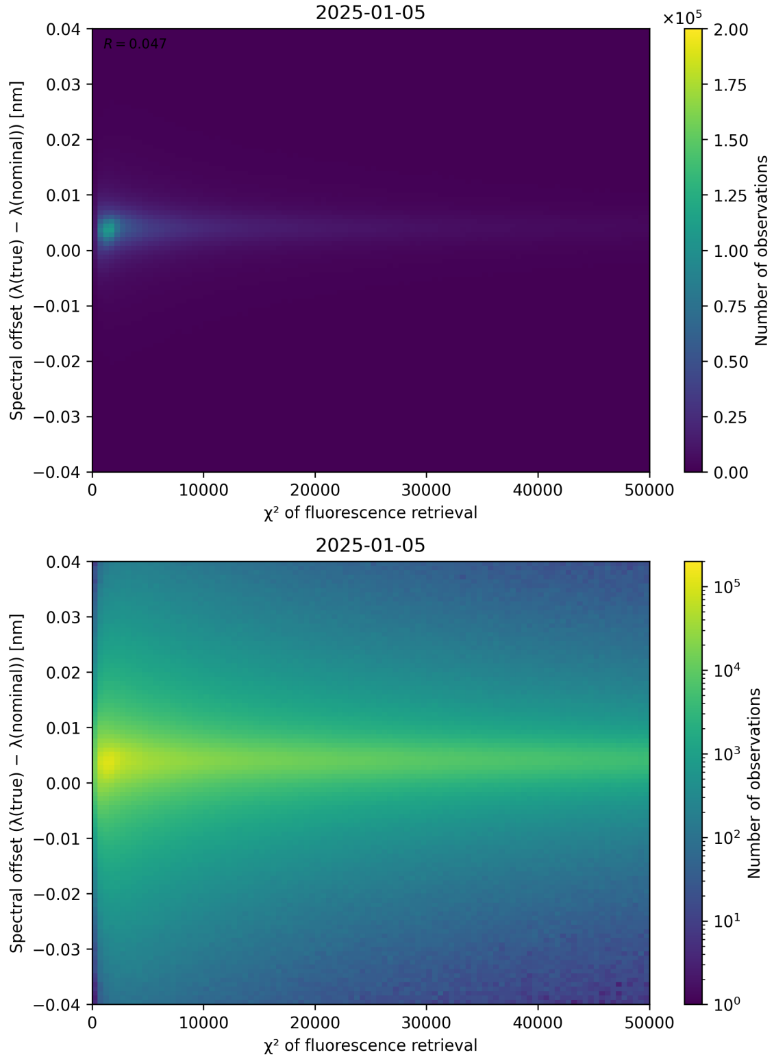
Figure 69: Scatter density plot of “ \chi^2 of fluorescence retrieval” against “Spectral offset ( \lambda_{\text{true}} - \lambda_{\text{nominal}} )” for 2025-01-04 to 2025-01-06.
