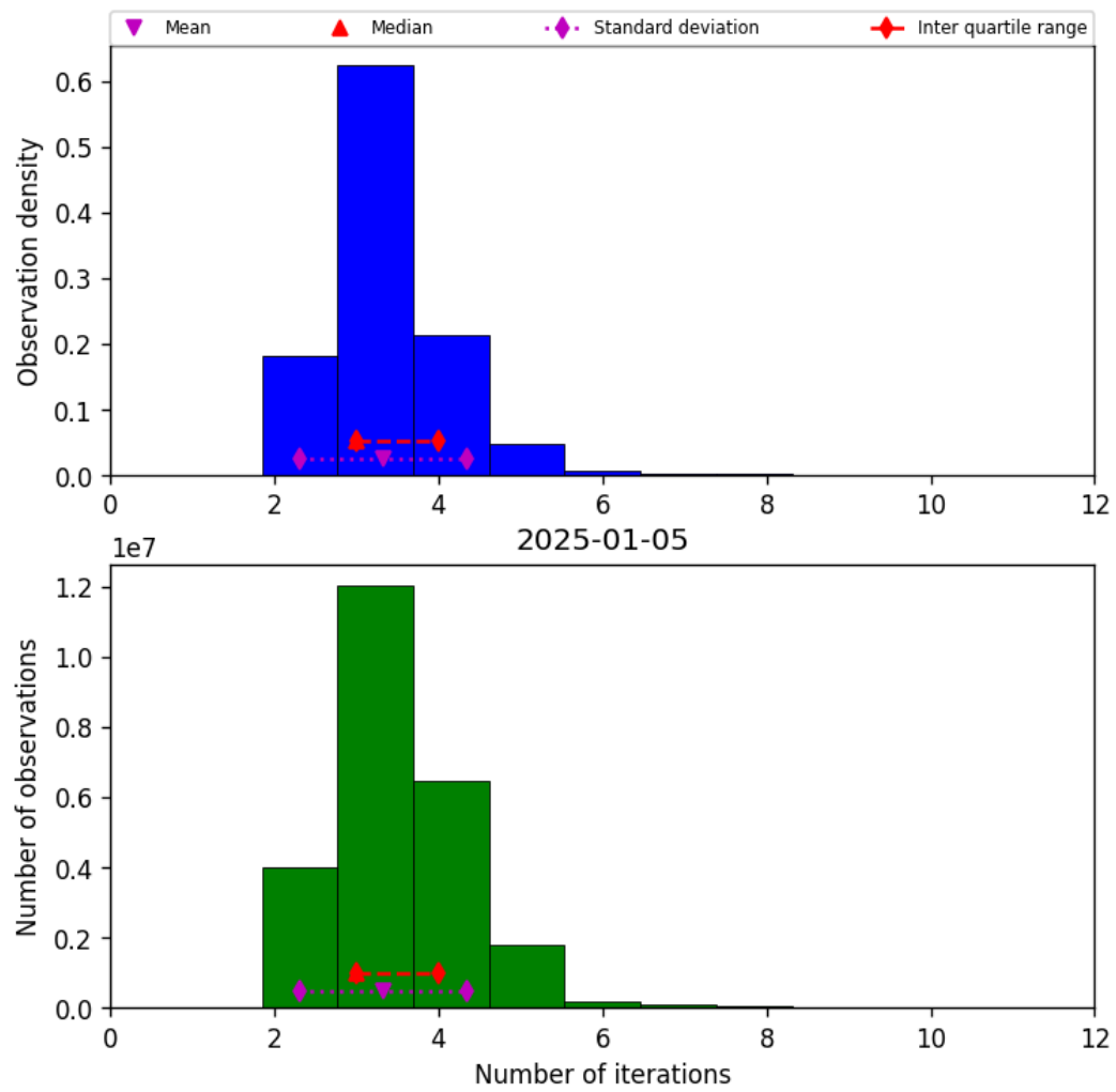
Figure 39: Histogram of “Number of iterations” for 2025-01-04 to 2025-01-06
