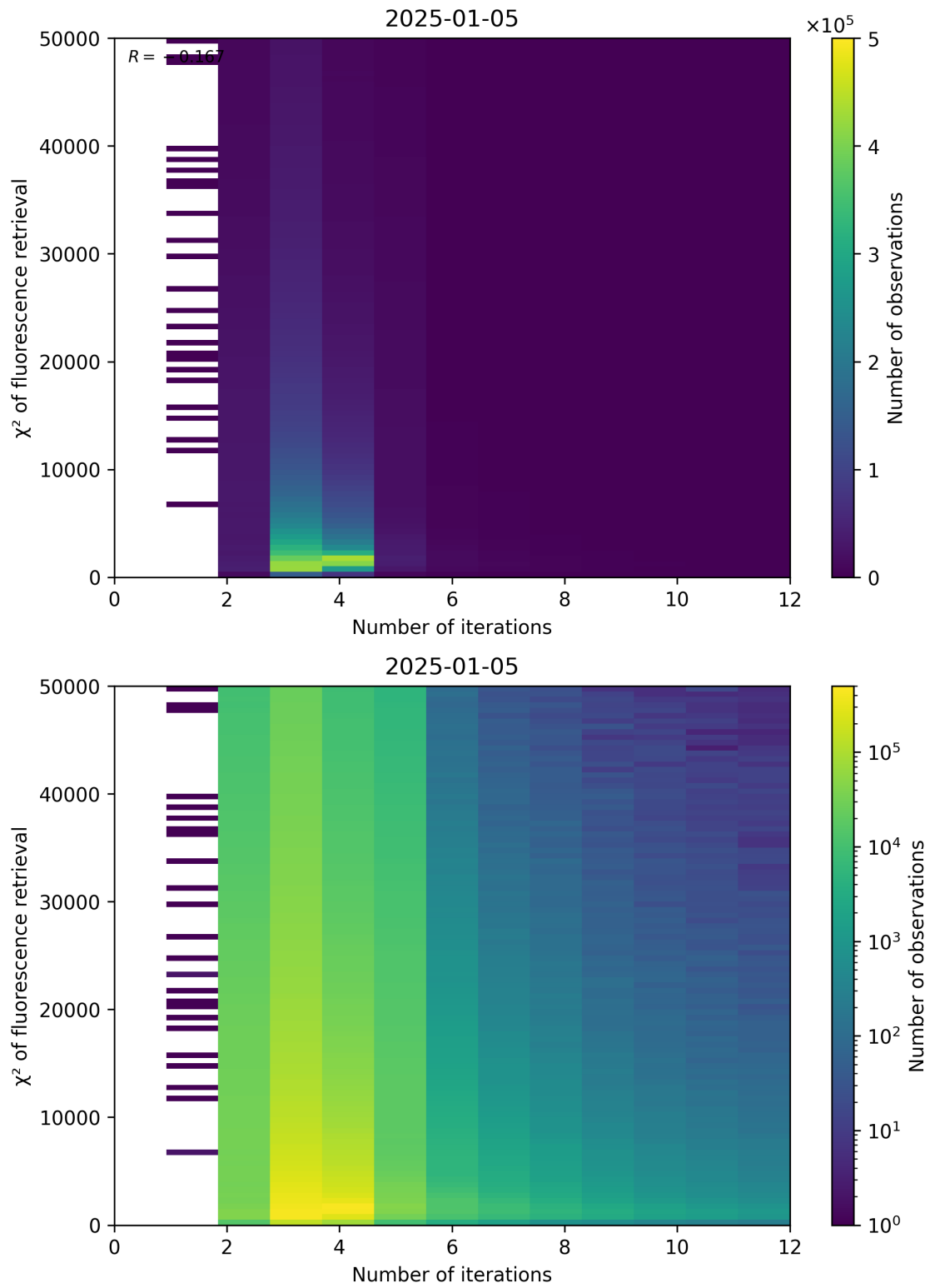
Figure 97: Scatter density plot of “Number of iterations” against “ \chi^2 of fluorescence retrieval” for 2025-01-04 to 2025-01-06.
