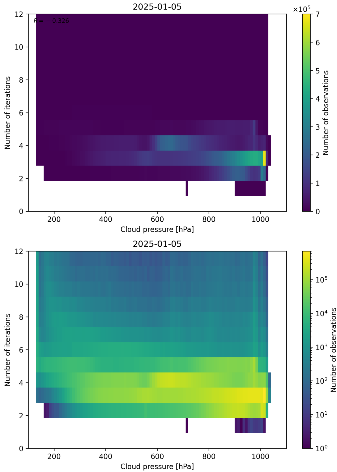
Figure 81: Scatter density plot of “Cloud pressure” against “Number of iterations” for 2025-01-04 to 2025-01-06.
