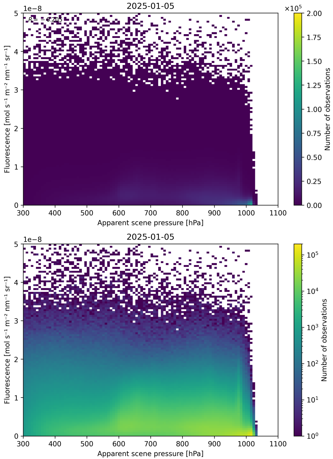
Figure 64: Scatter density plot of “Apparent scene pressure” against “Fluorescence” for 2025-01-04 to 2025-01-06.
