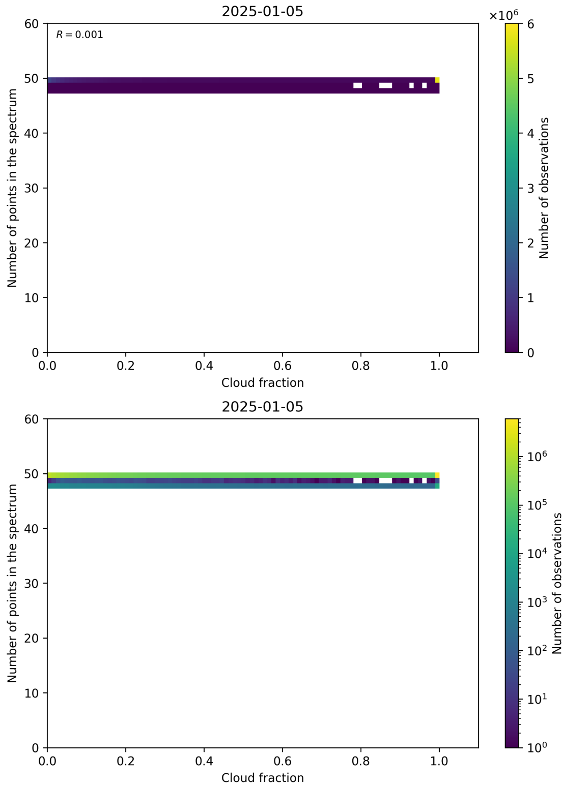
Figure 74: Scatter density plot of “Cloud fraction” against “Number of points in the spectrum” for 2025-01-04 to 2025-01-06.
