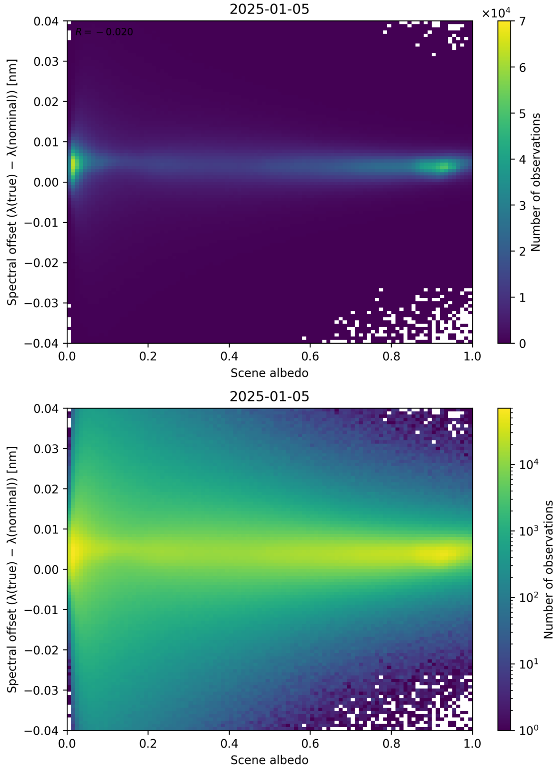
Figure 107: Scatter density plot of “Scene albedo” against “Spectral offset ( \lambda_{\text{true}} - \lambda_{\text{nominal}} )” for 2025-01-04 to 2025-01-06.
