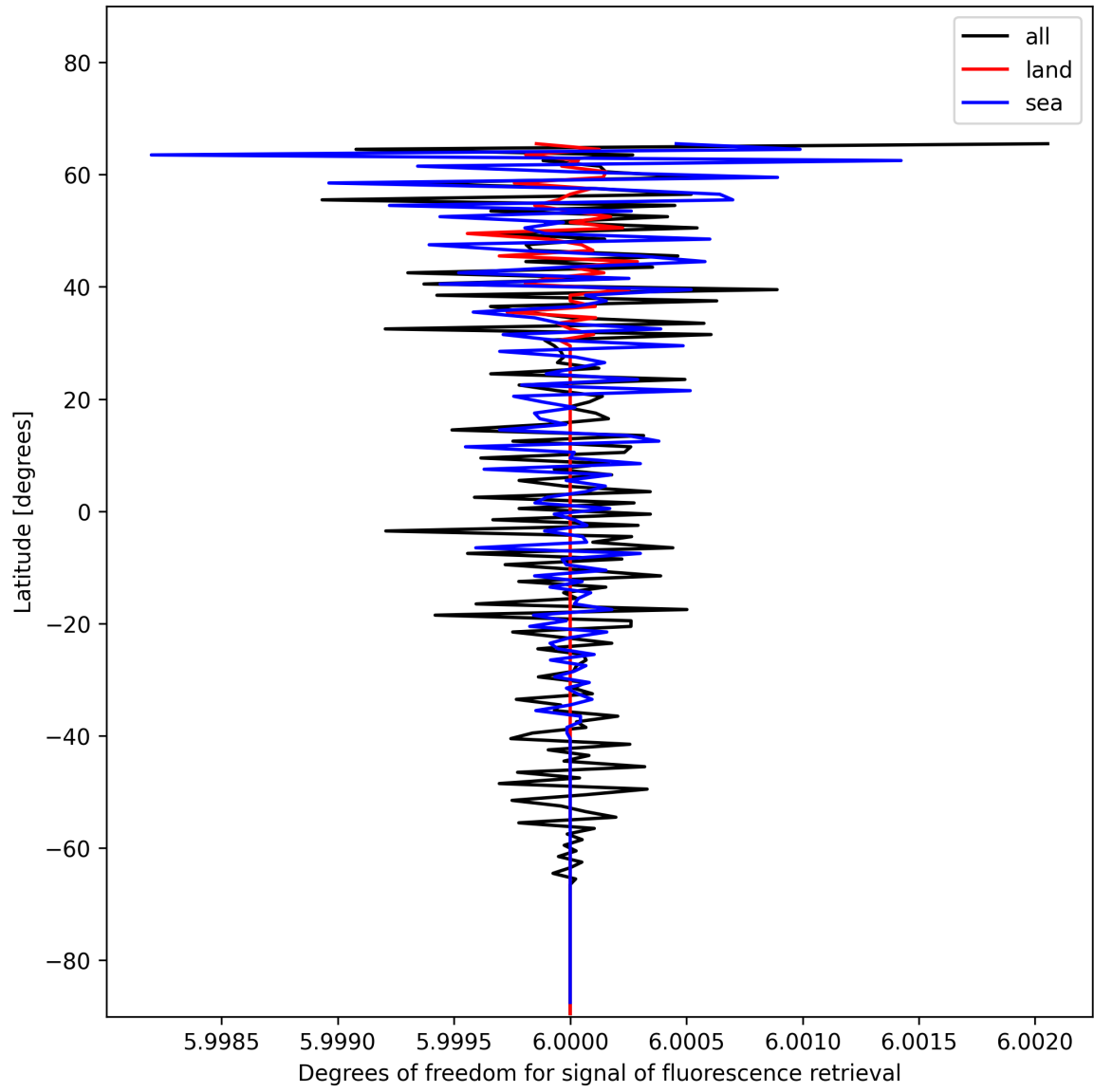
Figure 26: Zonal average of “Degrees of freedom for signal of fluorescence retrieval” for 2025-01-04 to 2025-01-06.
