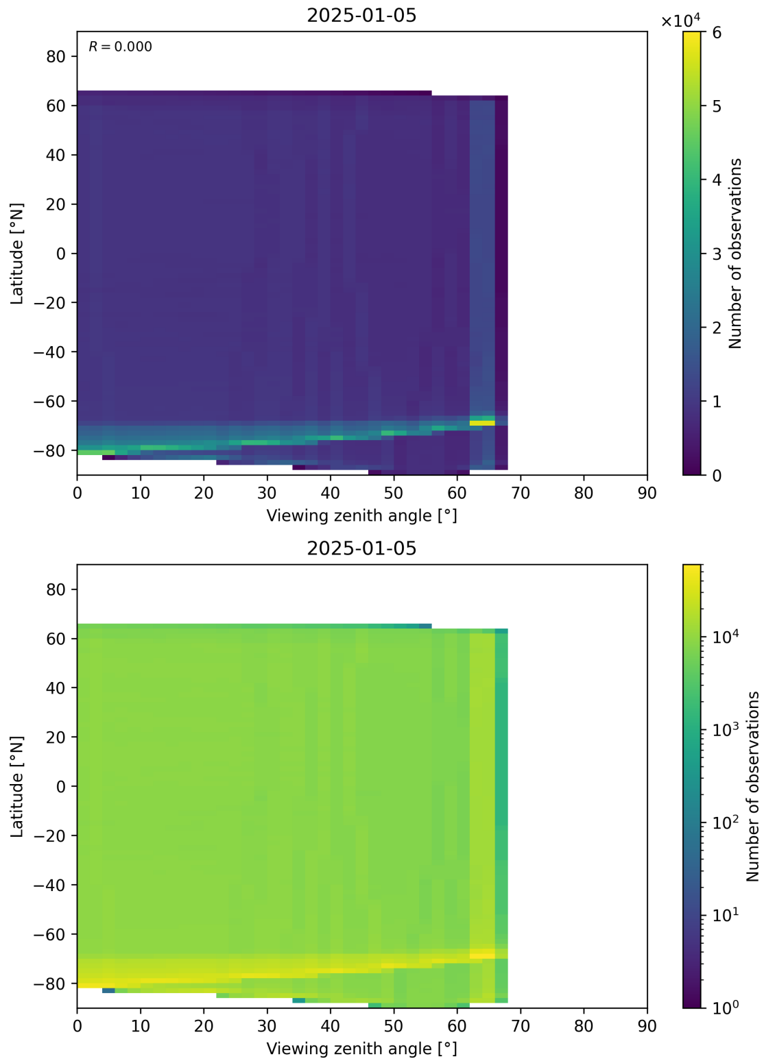
Figure 123: Scatter density plot of “Viewing zenith angle” against “Latitude” for 2025-01-04 to 2025-01-06.
