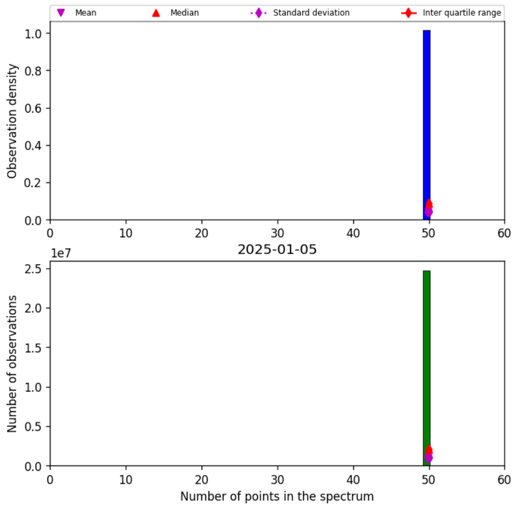
Figure 44: Histogram of “Number of points in the spectrum” for 2025-01-04 to 2025-01-06
