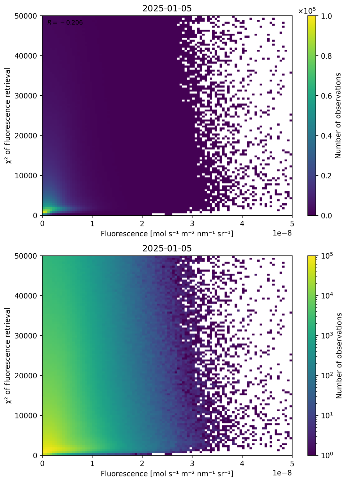
Figure 85: Scatter density plot of “Fluorescence” against “ \chi^2 of fluorescence retrieval” for 2025-01-04 to 2025-01-06.
