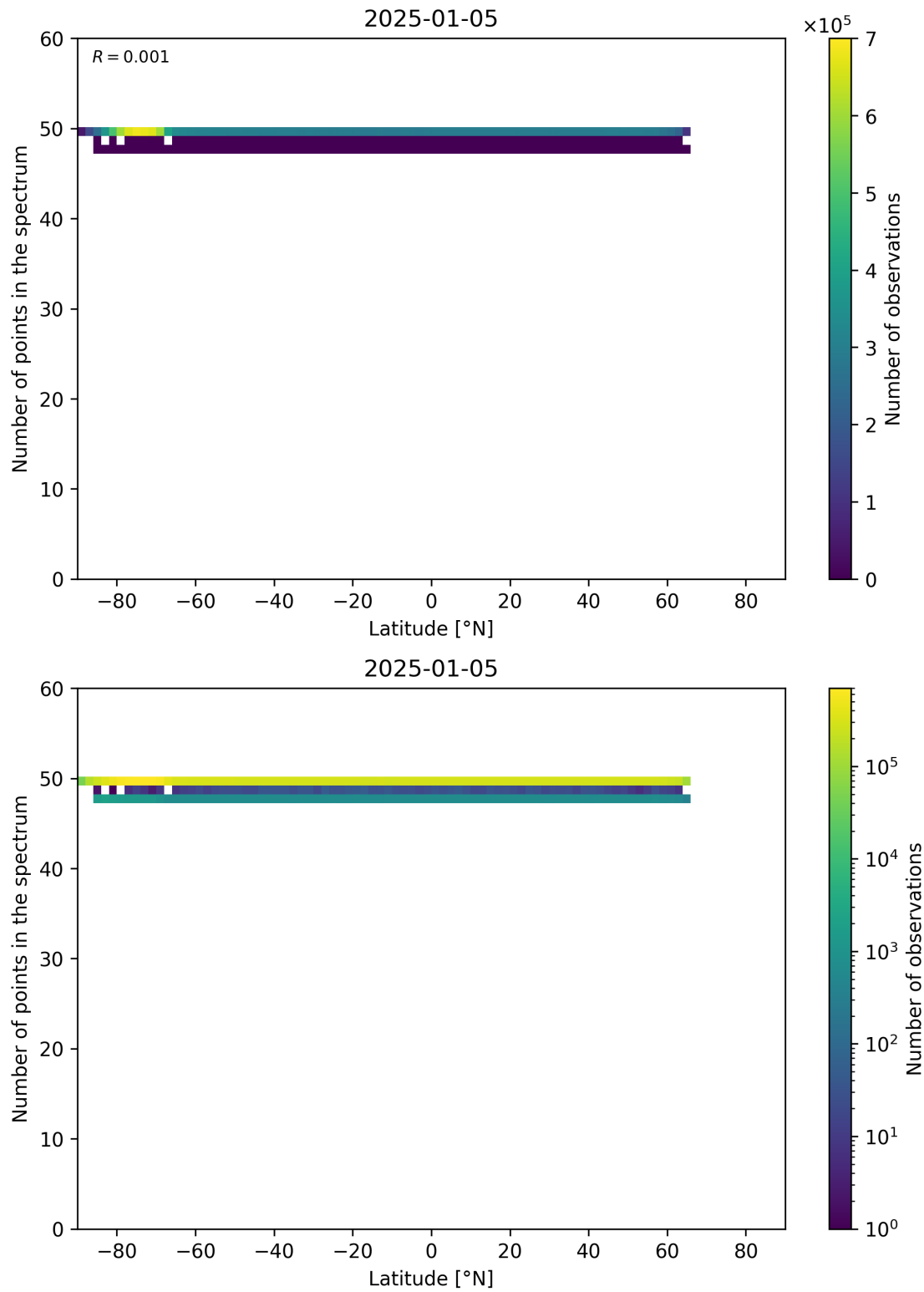
Figure 94: Scatter density plot of “Latitude” against “Number of points in the spectrum” for 2025-01-04 to 2025-01-06.
