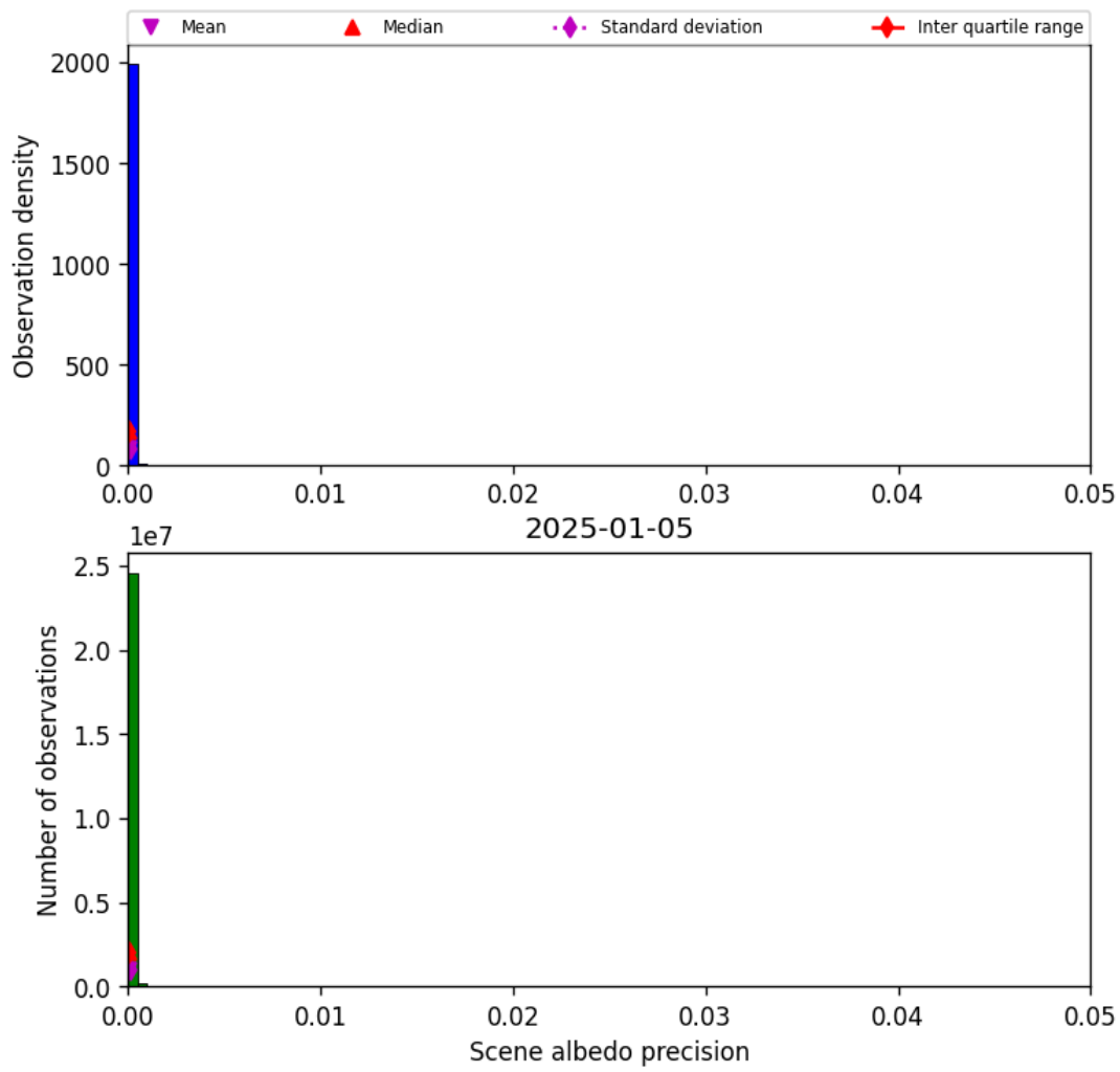
Figure 35: Histogram of “Scene albedo precision” for 2025-01-04 to 2025-01-06
