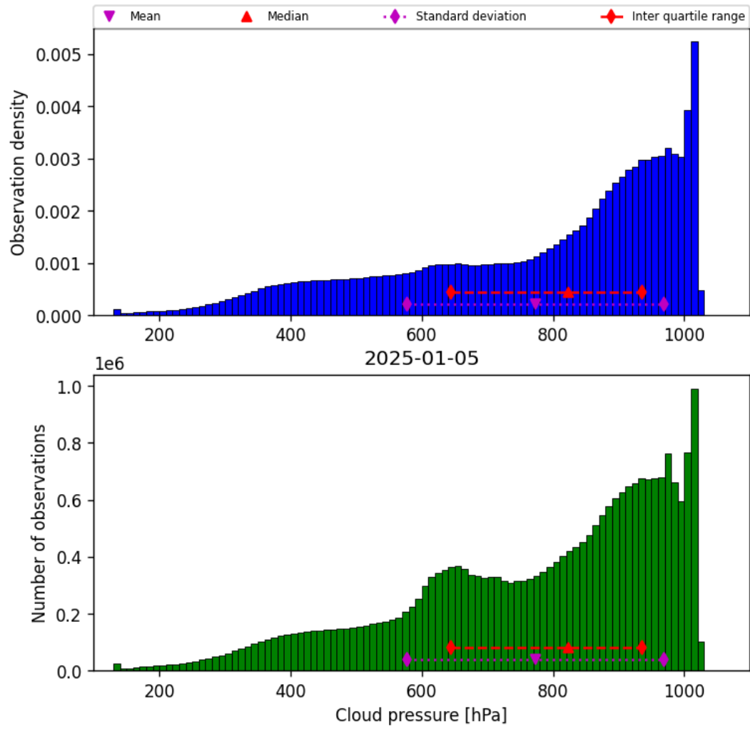
Figure 30: Histogram of “Cloud pressure” for 2025-01-04 to 2025-01-06
