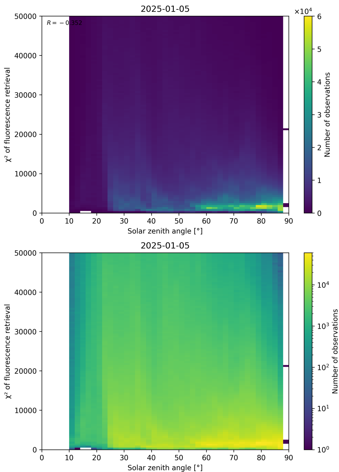
Figure 109: Scatter density plot of “Solar zenith angle” against “ \chi^2 of fluorescence retrieval” for 2025-01-04 to 2025-01-06.
