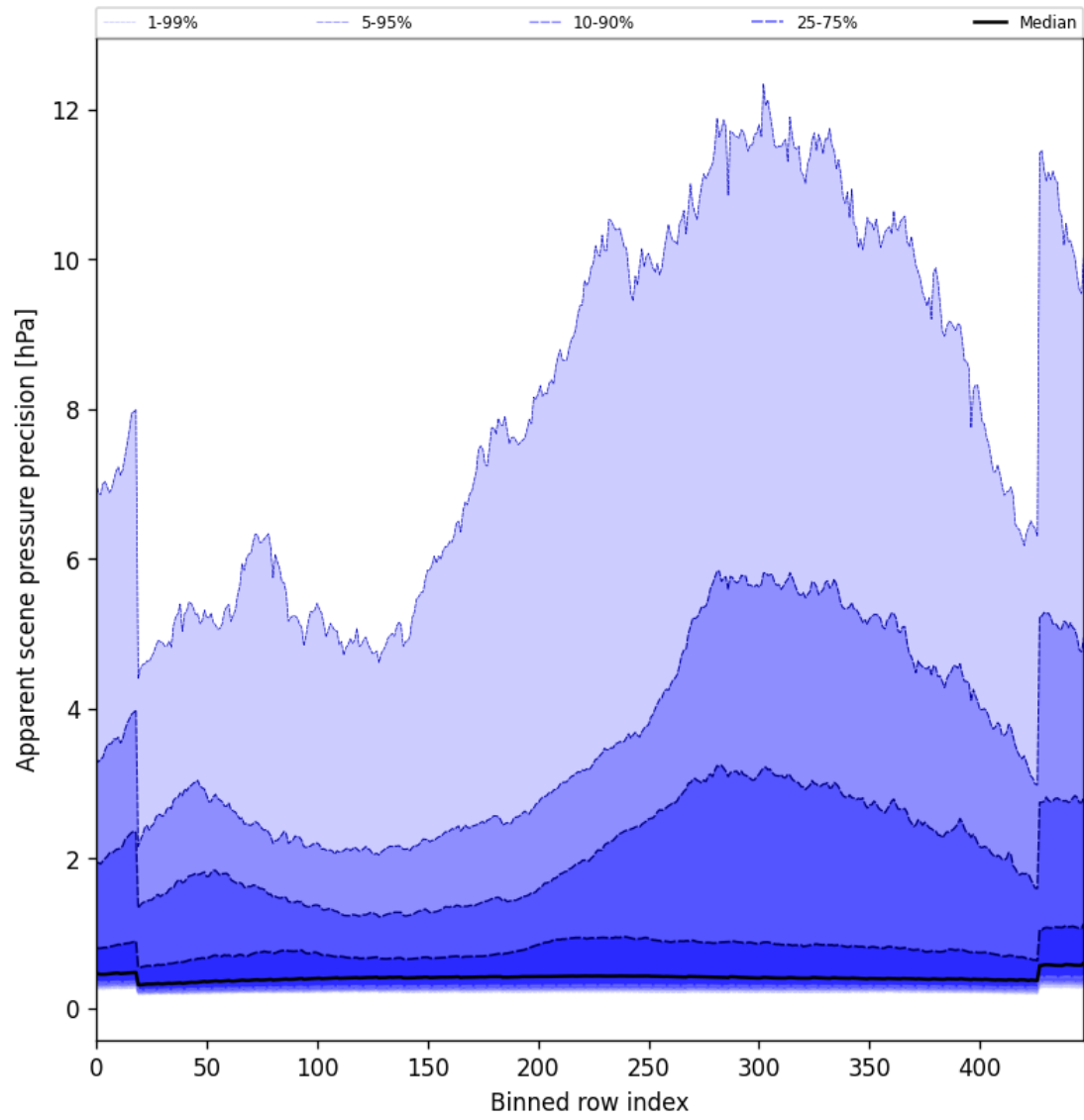
Figure 54: Along track statistics of “Apparent scene pressure precision” for 2025-01-04 to 2025-01-06
