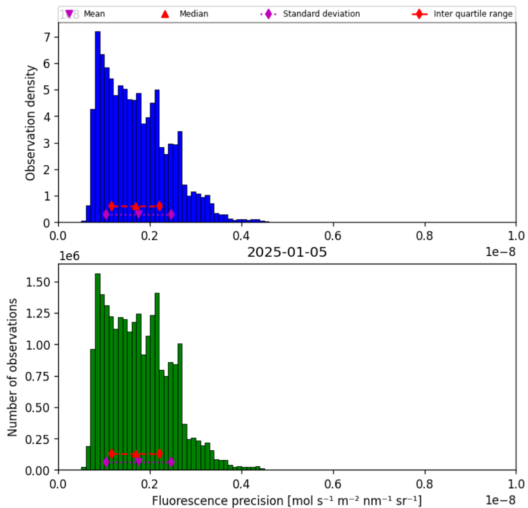
Figure 41: Histogram of “Fluorescence precision” for 2025-01-04 to 2025-01-06
