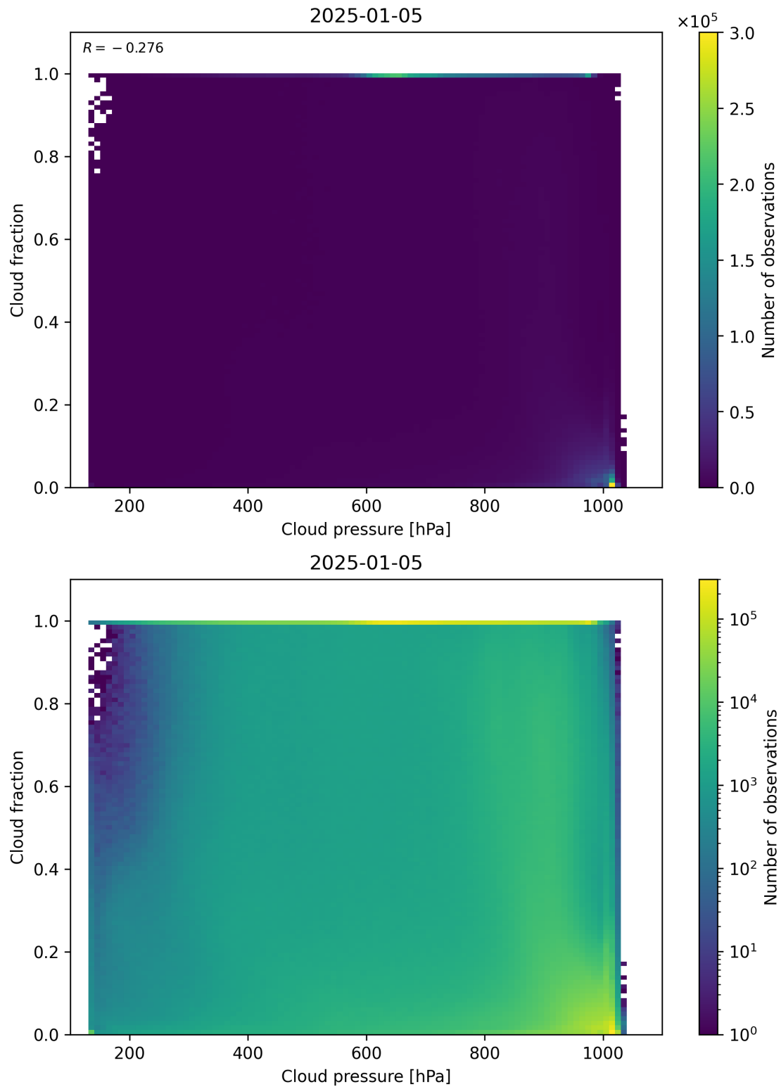
Figure 79: Scatter density plot of “Cloud pressure” against “Cloud fraction” for 2025-01-04 to 2025-01-06.
