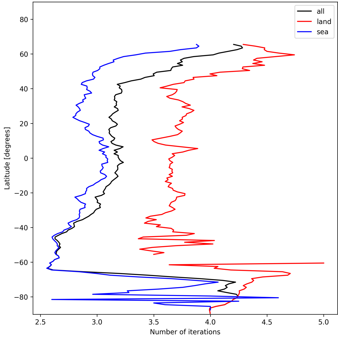
Figure 22: Zonal average of “Number of iterations” for 2025-01-04 to 2025-01-06.
