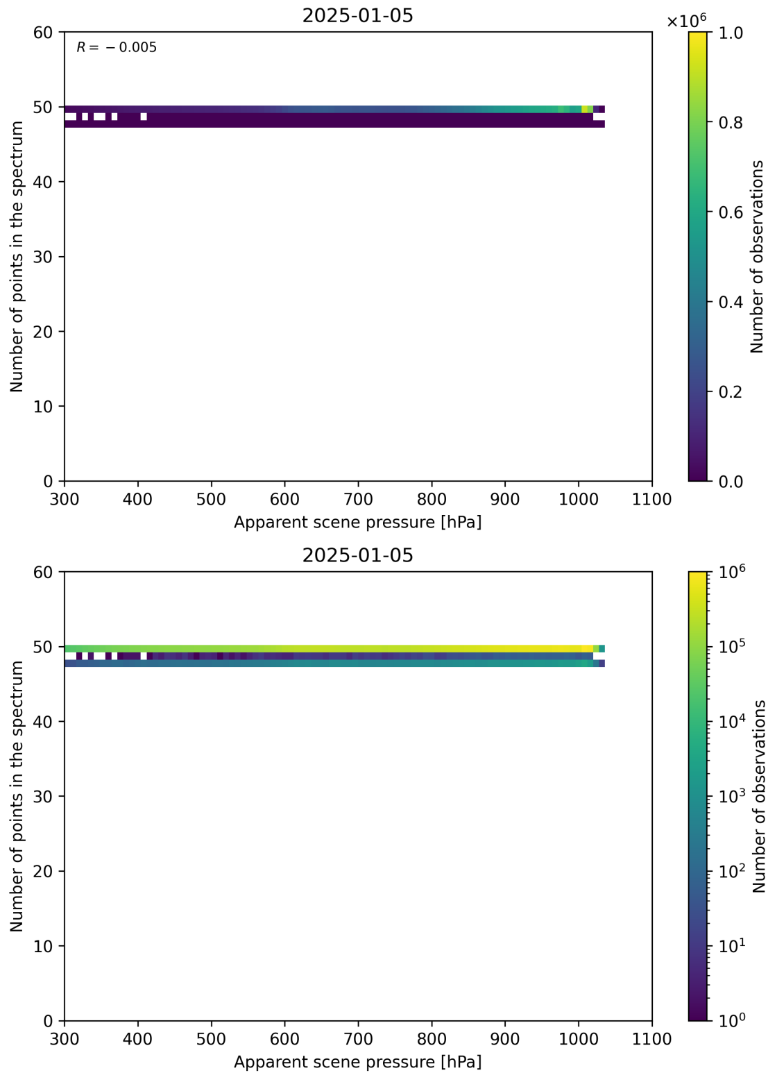
Figure 66: Scatter density plot of “Apparent scene pressure” against “Number of points in the spectrum” for 2025-01-04 to 2025-01-06.
