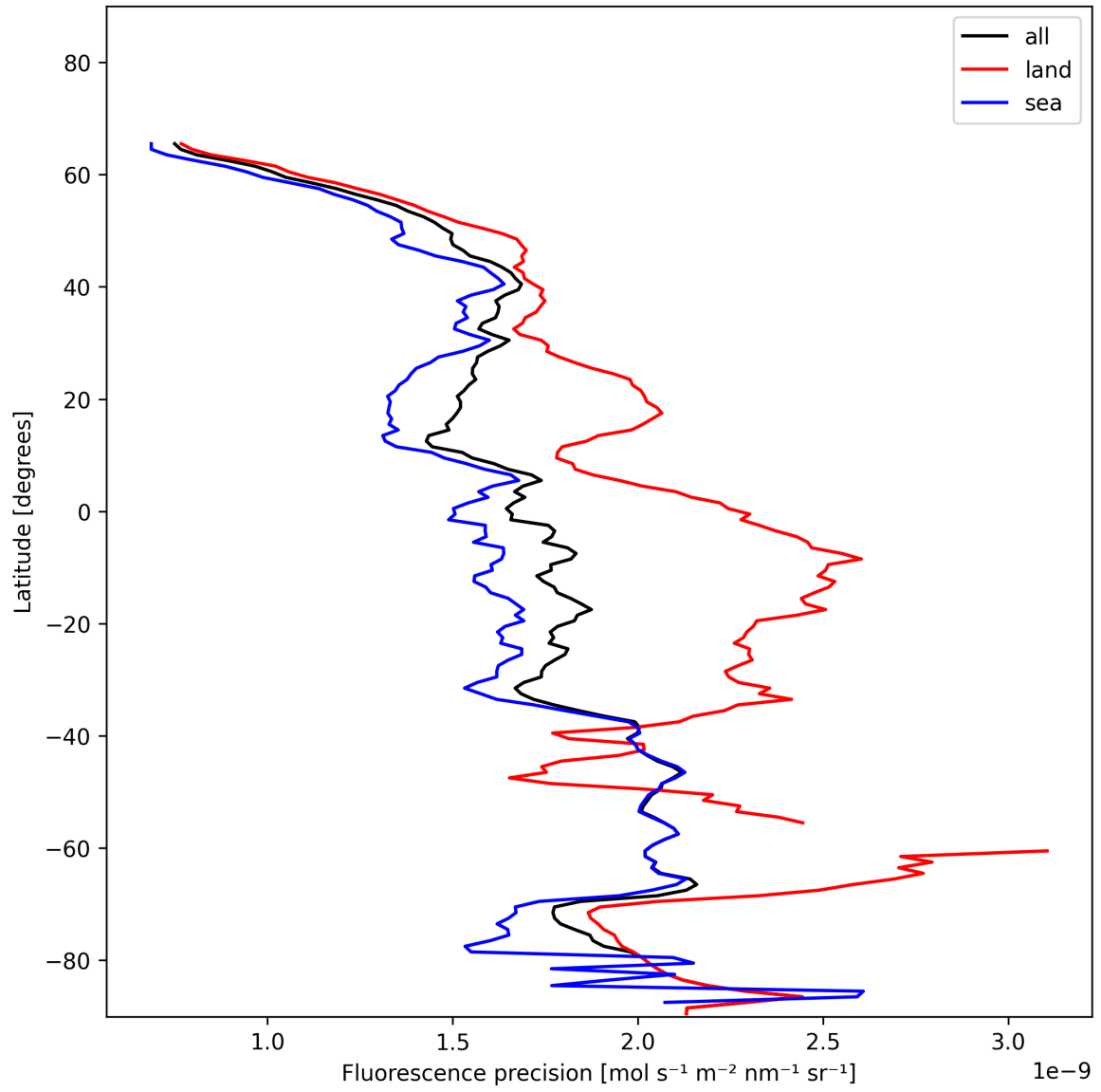
Figure 24: Zonal average of “Fluorescence precision” for 2025-01-04 to 2025-01-06.
