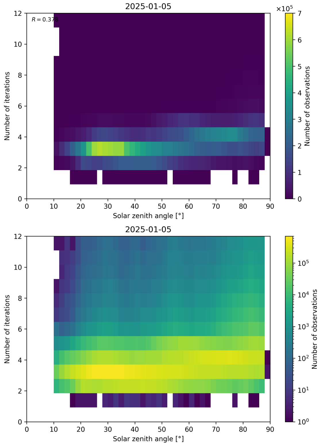
Figure 114: Scatter density plot of “Solar zenith angle” against “Number of iterations” for 2025-01-04 to 2025-01-06.
