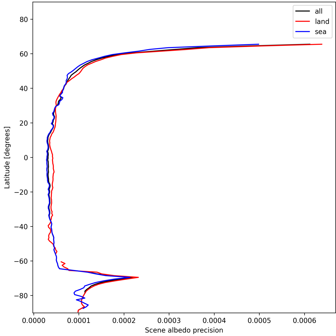
Figure 18: Zonal average of “Scene albedo precision” for 2025-01-04 to 2025-01-06.
