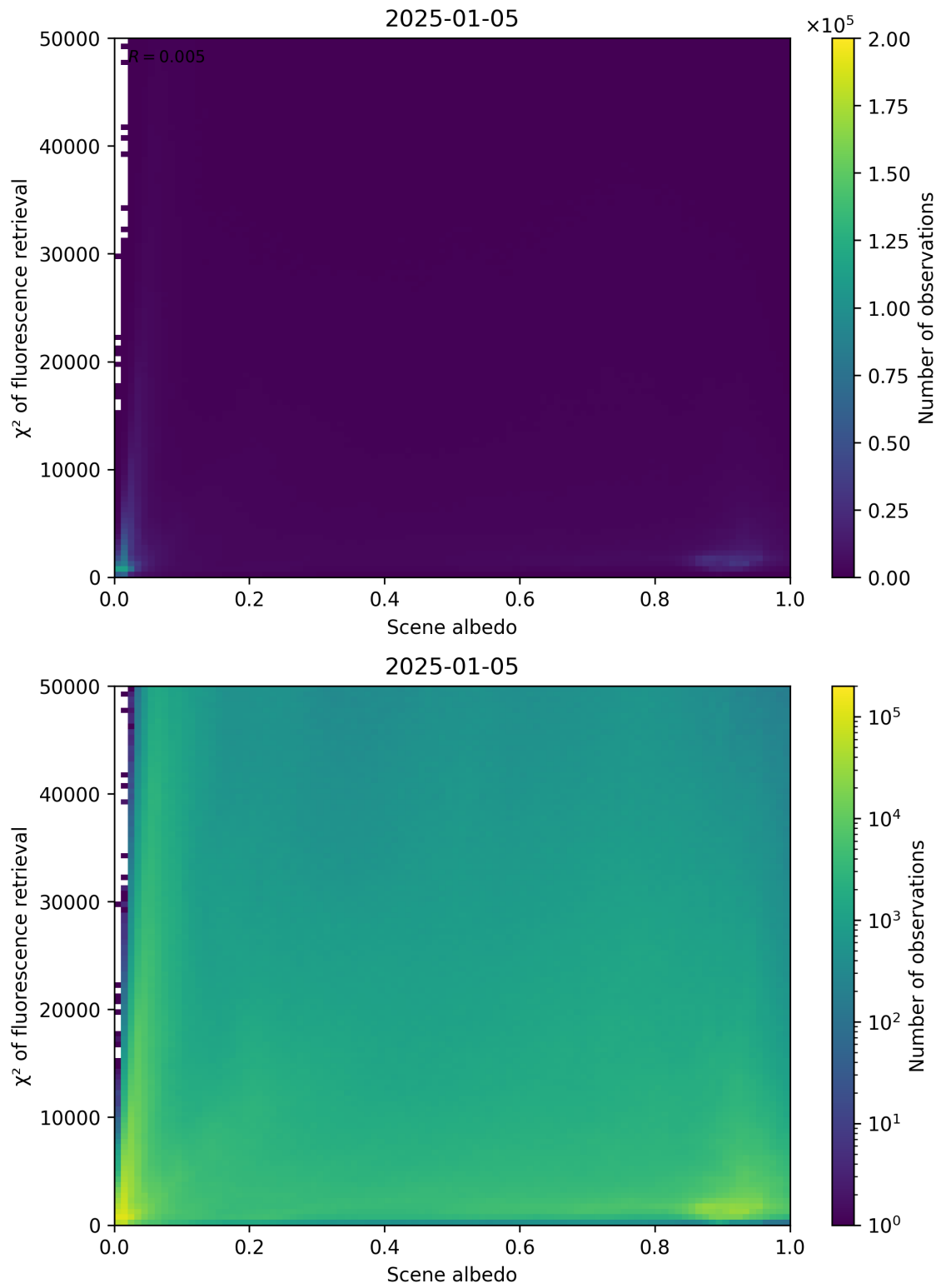
Figure 103: Scatter density plot of “Scene albedo” against “ \chi^2 of fluorescence retrieval” for 2025-01-04 to 2025-01-06.
