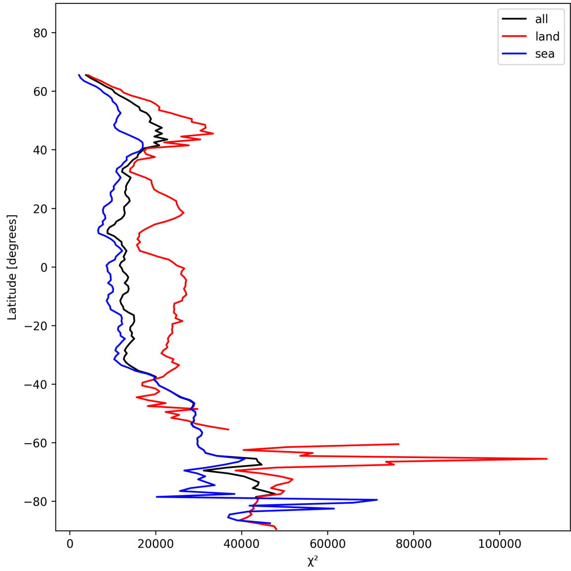
Figure 21: Zonal average of “ \chi^2 ” for 2025-01-04 to 2025-01-06.
