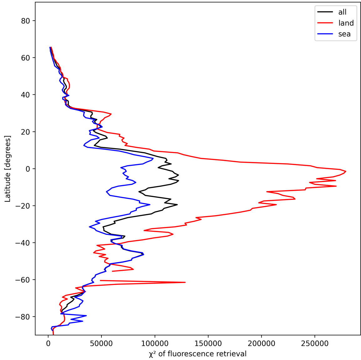
Figure 25: Zonal average of “ \chi^2 of fluorescence retrieval” for 2025-01-04 to 2025-01-06.
