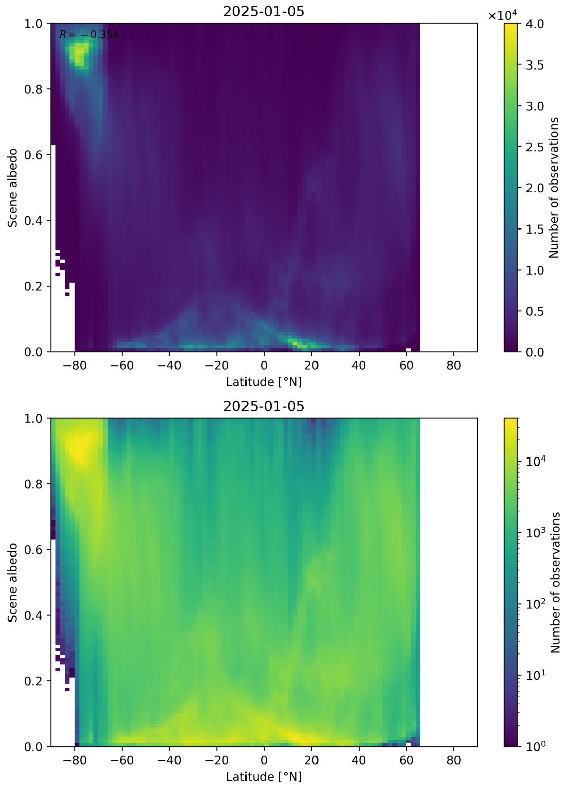
Figure 95: Scatter density plot of “Latitude” against “Scene albedo” for 2025-01-04 to 2025-01-06.
