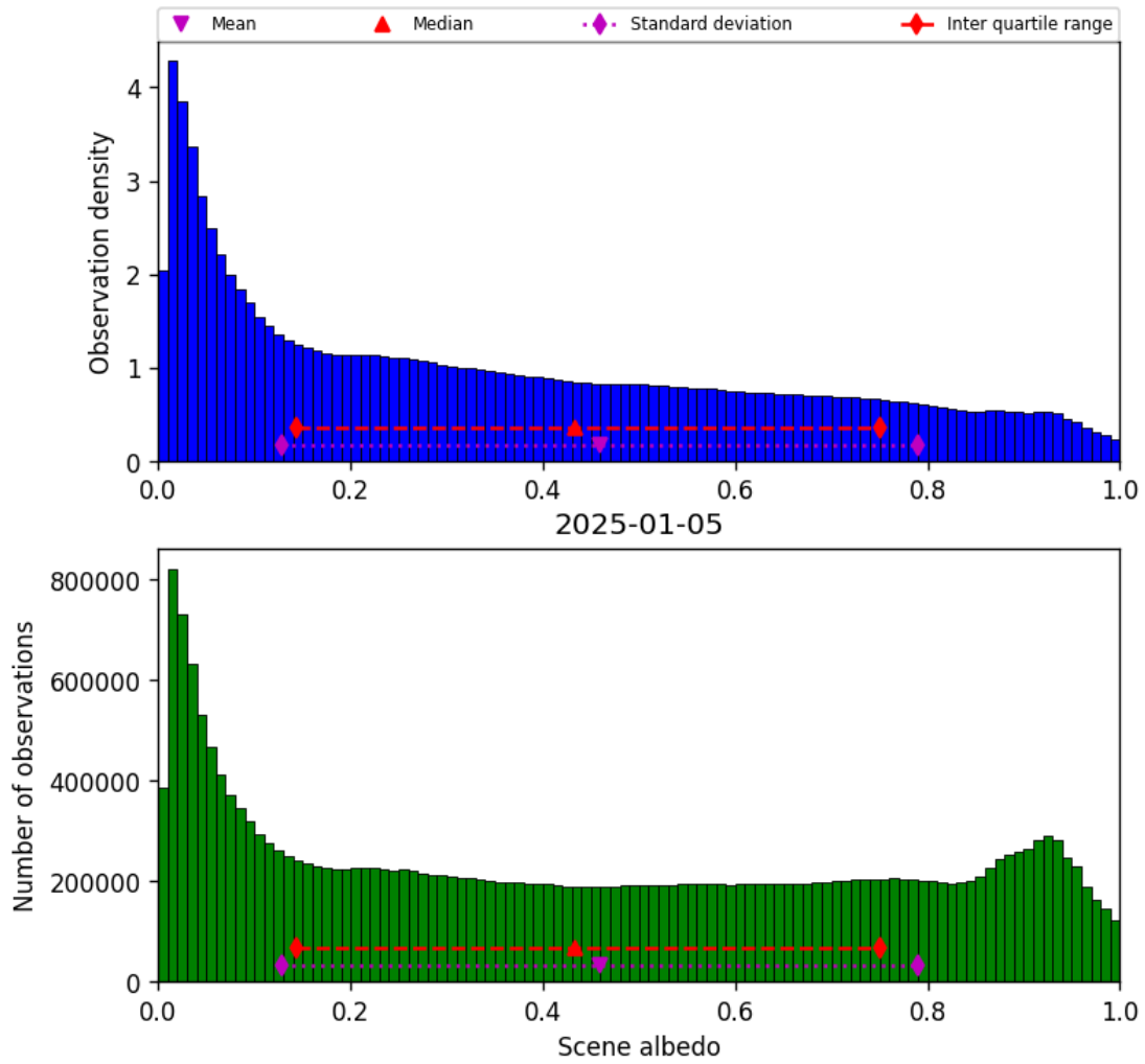
Figure 34: Histogram of “Scene albedo” for 2025-01-04 to 2025-01-06
