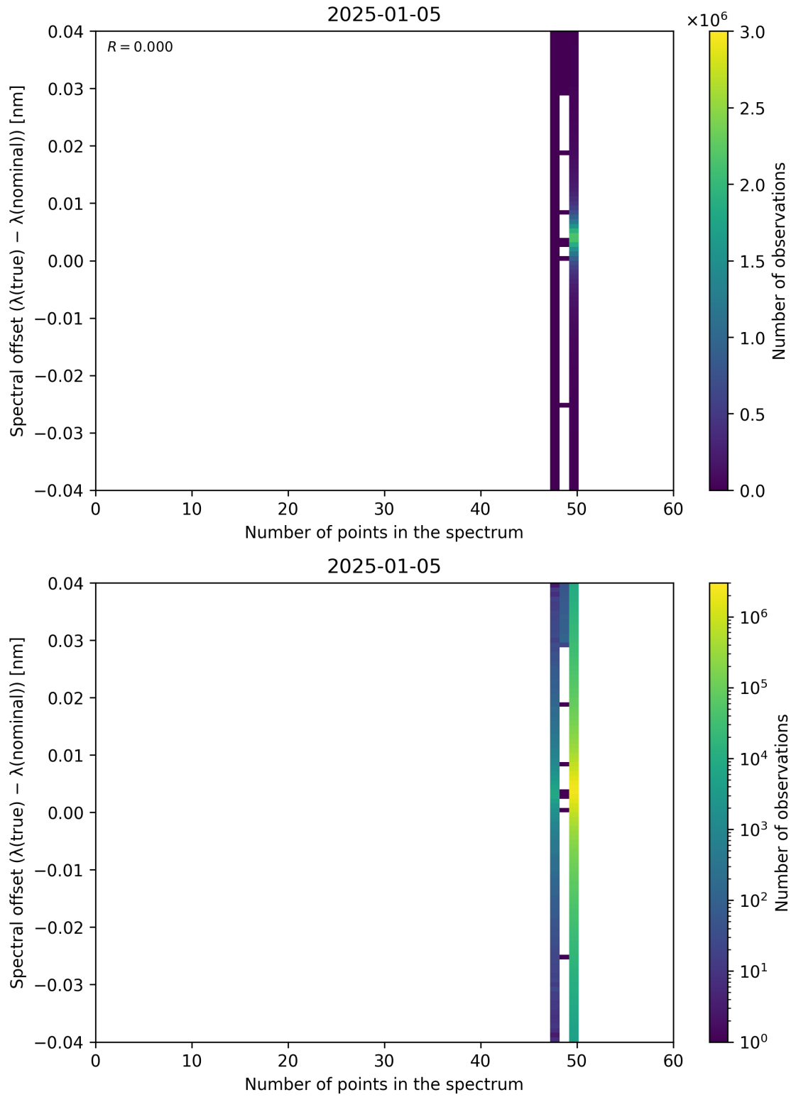
Figure 101: Scatter density plot of “Number of points in the spectrum” against “Spectral offset ( \lambda_{\text{true}} - \lambda_{\text{nominal}} )” for 2025-01-04 to 2025-01-06.
