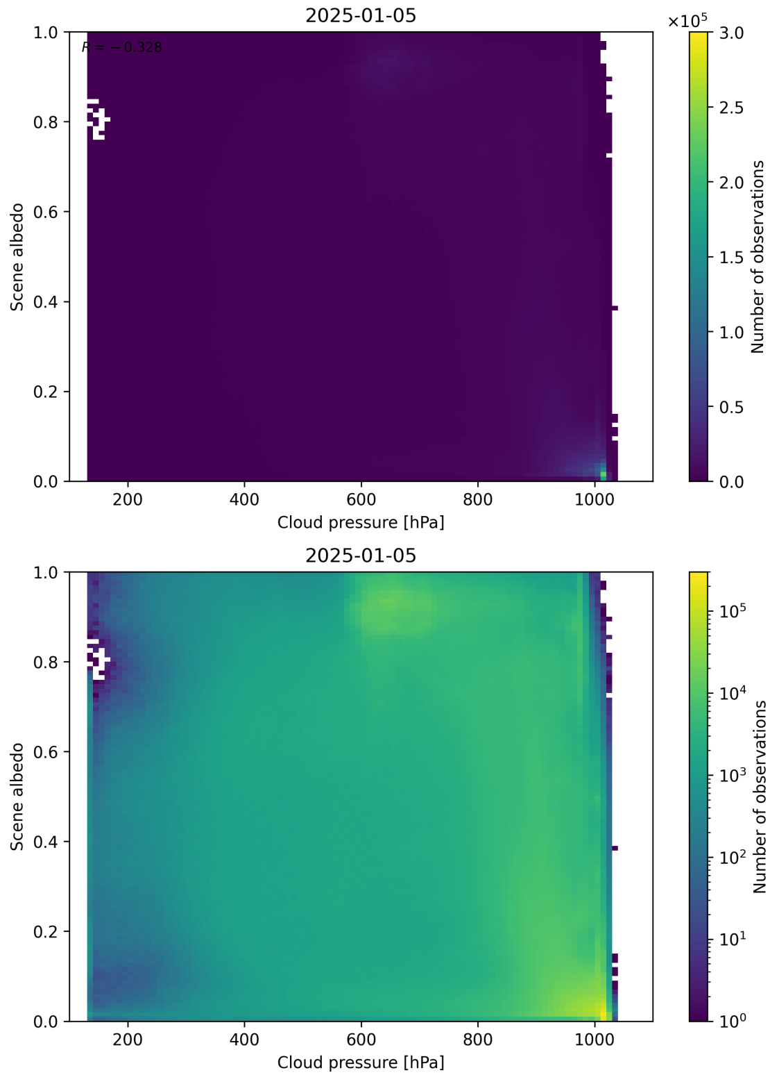
Figure 83: Scatter density plot of “Cloud pressure” against “Scene albedo” for 2025-01-04 to 2025-01-06.
