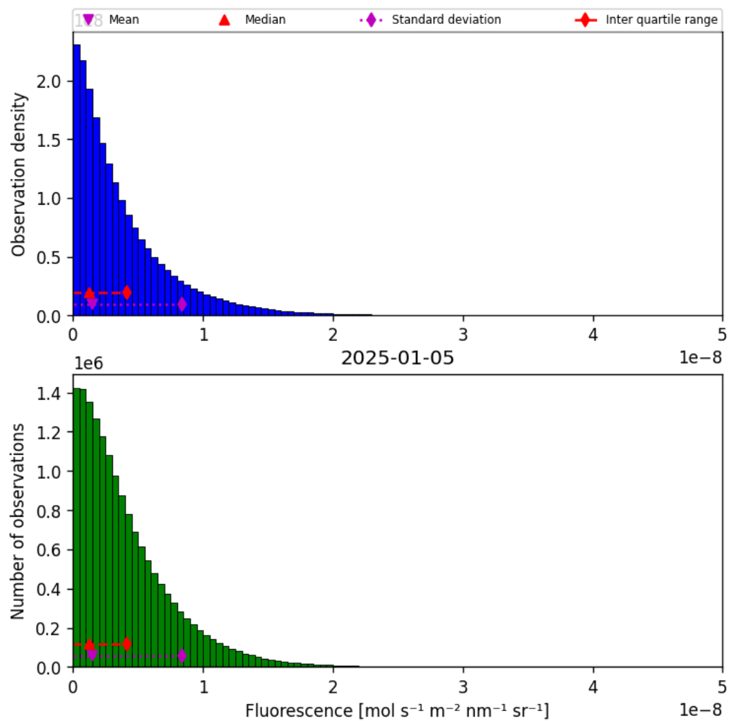
Figure 40: Histogram of “Fluorescence” for 2025-01-04 to 2025-01-06
