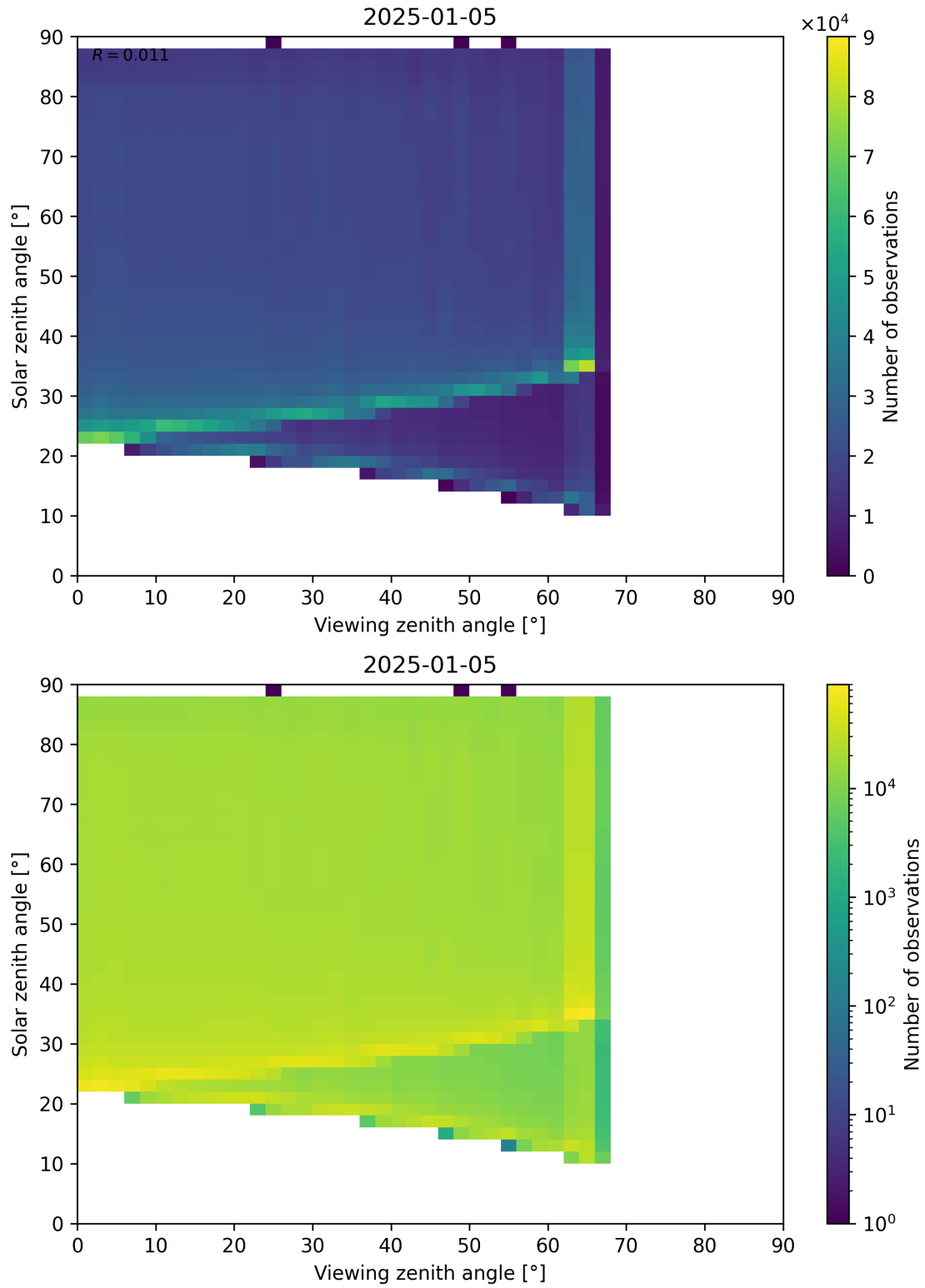
Figure 127: Scatter density plot of “Viewing zenith angle” against “Solar zenith angle” for 2025-01-04 to 2025-01-06.
