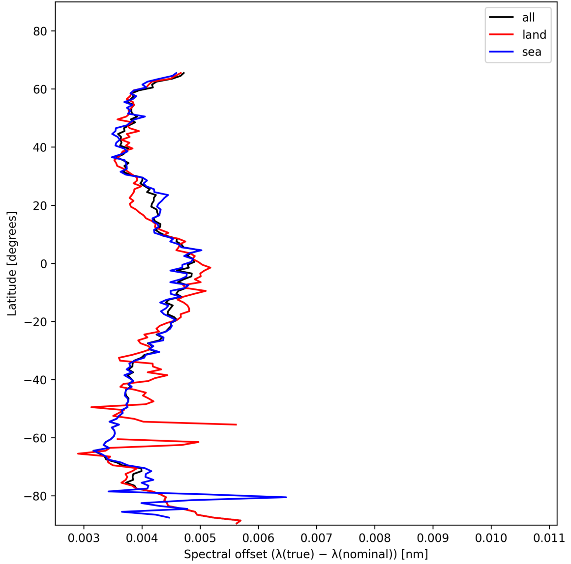
Figure 28: Zonal average of “Spectral offset ( \lambda_{\text{true}} - \lambda_{\text{nominal}} )” for 2025-01-04 to 2025-01-06.
