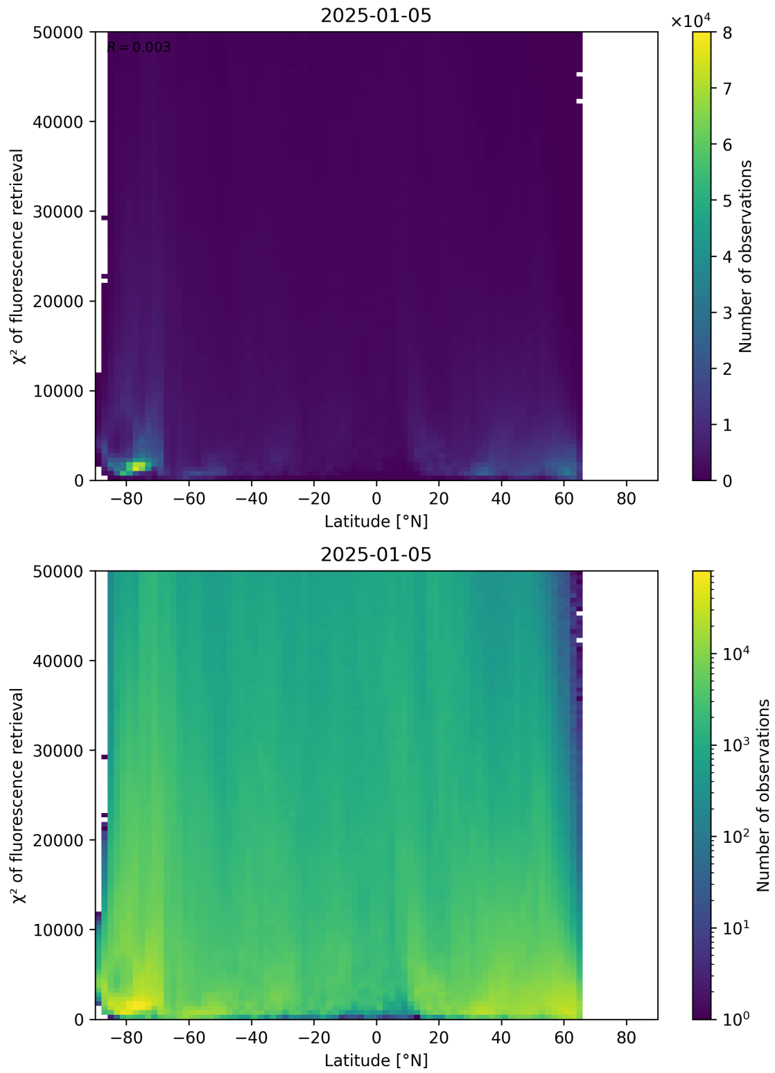
Figure 89: Scatter density plot of “Latitude” against “ \chi^2 of fluorescence retrieval” for 2025-01-04 to 2025-01-06.
