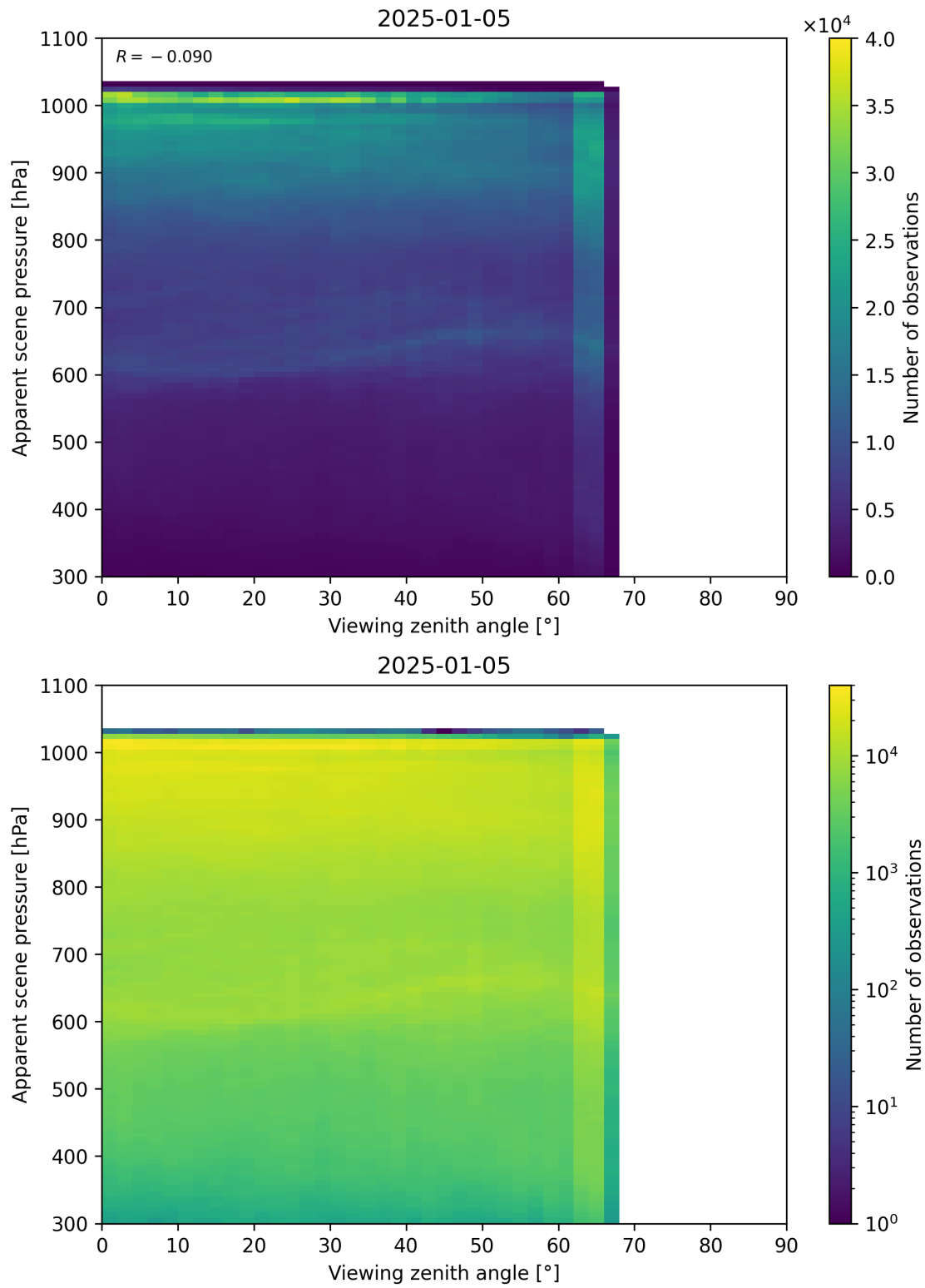
Figure 118: Scatter density plot of “Viewing zenith angle” against “Apparent scene pressure” for 2025-01-04 to 2025-01-06.
