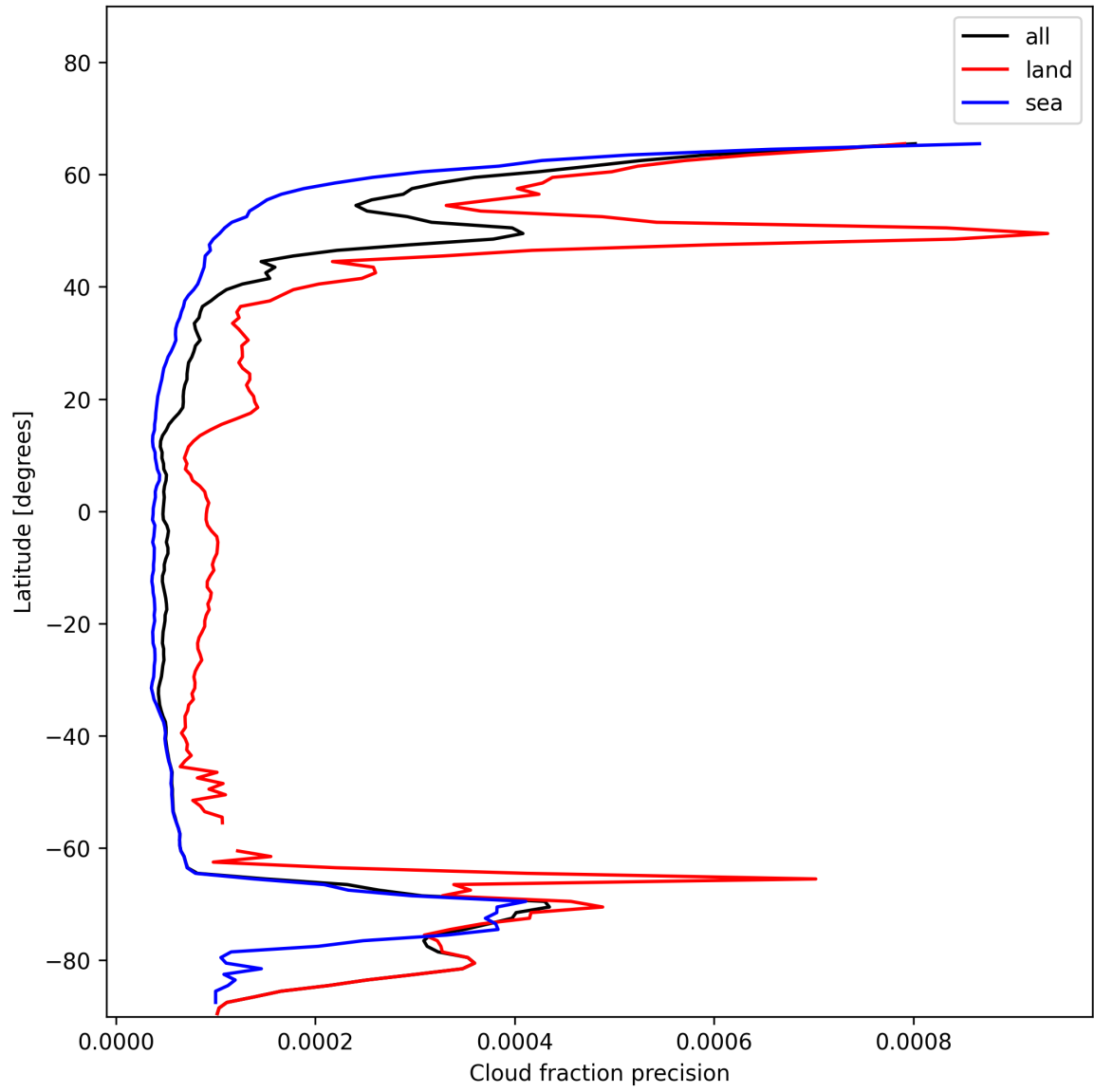
Figure 16: Zonal average of “Cloud fraction precision” for 2025-01-04 to 2025-01-06.
