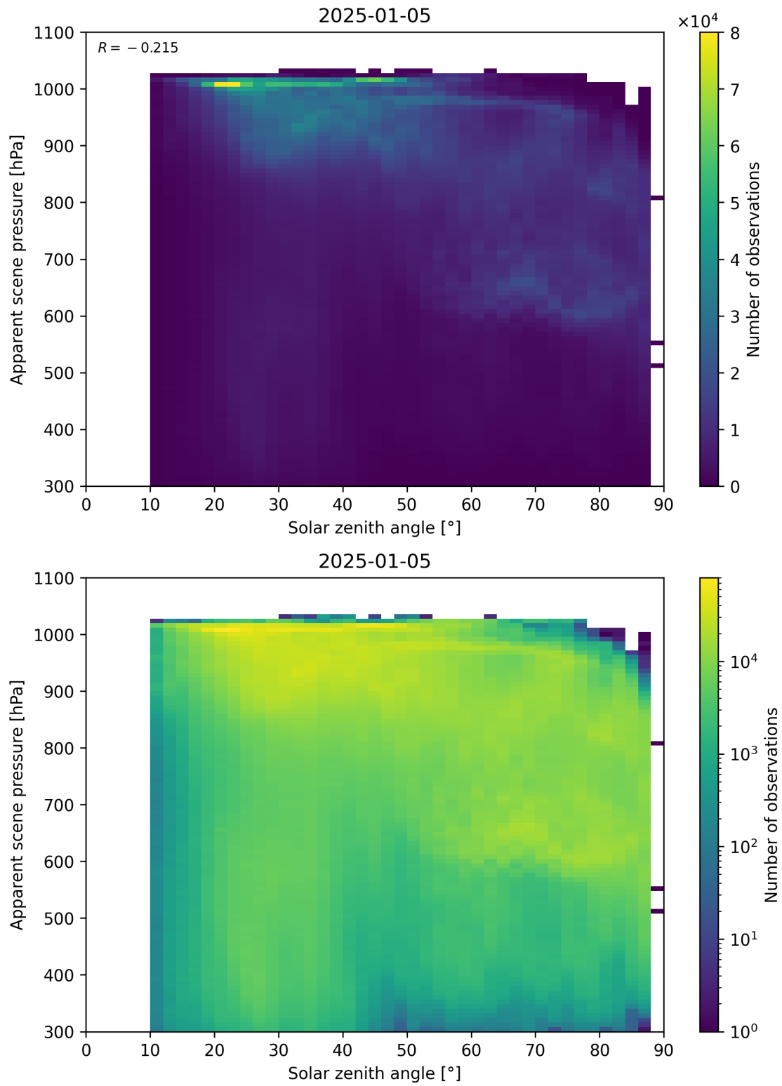
Figure 108: Scatter density plot of “Solar zenith angle” against “Apparent scene pressure” for 2025-01-04 to 2025-01-06.
