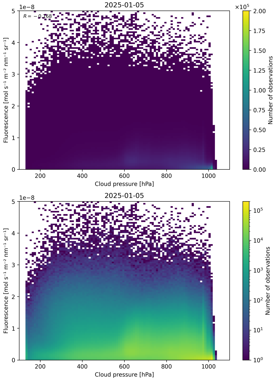
Figure 80: Scatter density plot of “Cloud pressure” against “Fluorescence” for 2025-01-04 to 2025-01-06.
