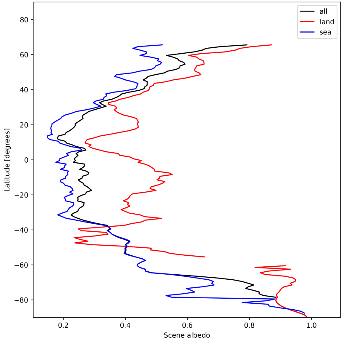
Figure 17: Zonal average of “Scene albedo” for 2025-01-04 to 2025-01-06.
