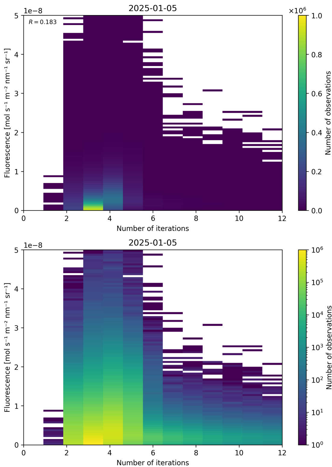
Figure 98: Scatter density plot of “Number of iterations” against “Fluorescence” for 2025-01-04 to 2025-01-06.
