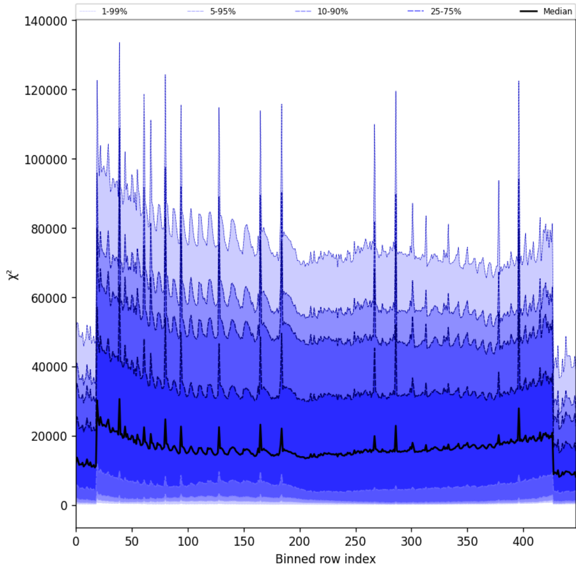
Figure 55: Along track statistics of “ \chi^2 ” for 2025-01-04 to 2025-01-06
