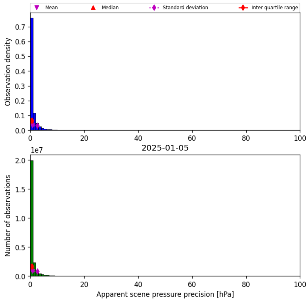
Figure 37: Histogram of “Apparent scene pressure precision” for 2025-01-04 to 2025-01-06
