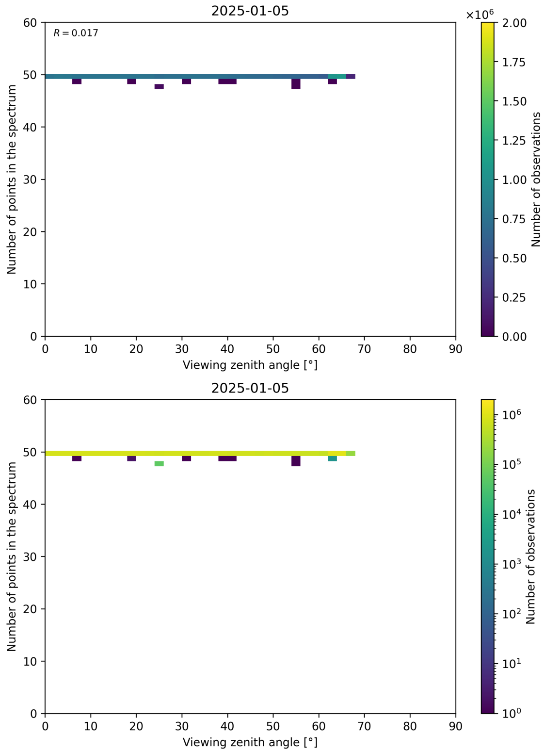
Figure 125: Scatter density plot of “Viewing zenith angle” against “Number of points in the spectrum” for 2025-01-04 to 2025-01-06.
