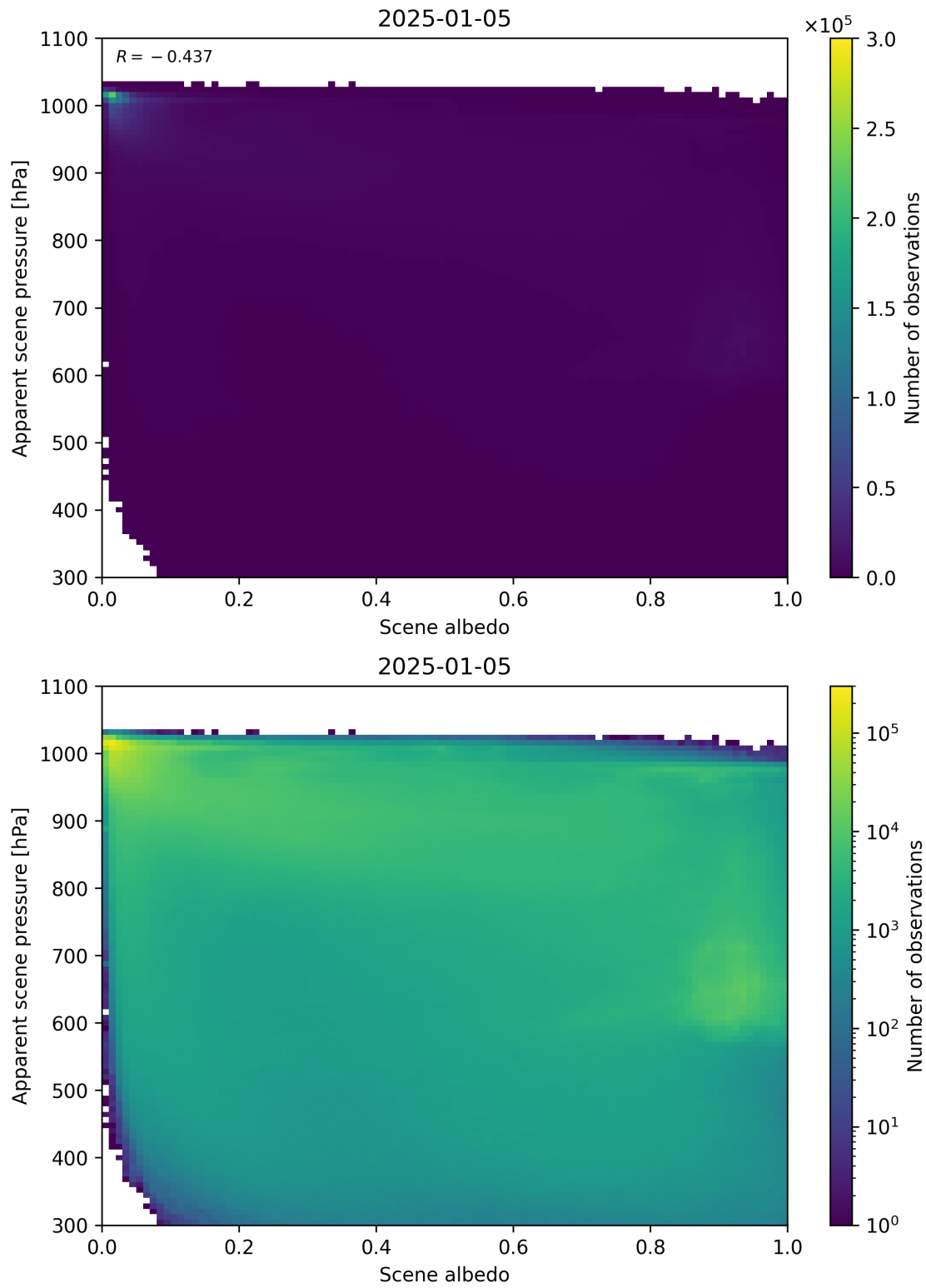
Figure 102: Scatter density plot of “Scene albedo” against “Apparent scene pressure” for 2025-01-04 to 2025-01-06.
