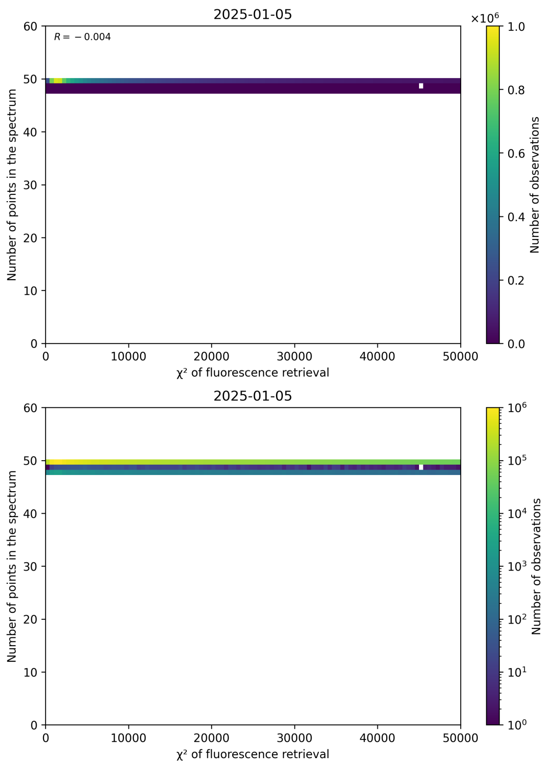
Figure 68: Scatter density plot of " \chi^2 of fluorescence retrieval" against "Number of points in the spectrum" for 2025-01-04 to 2025-01-06.
