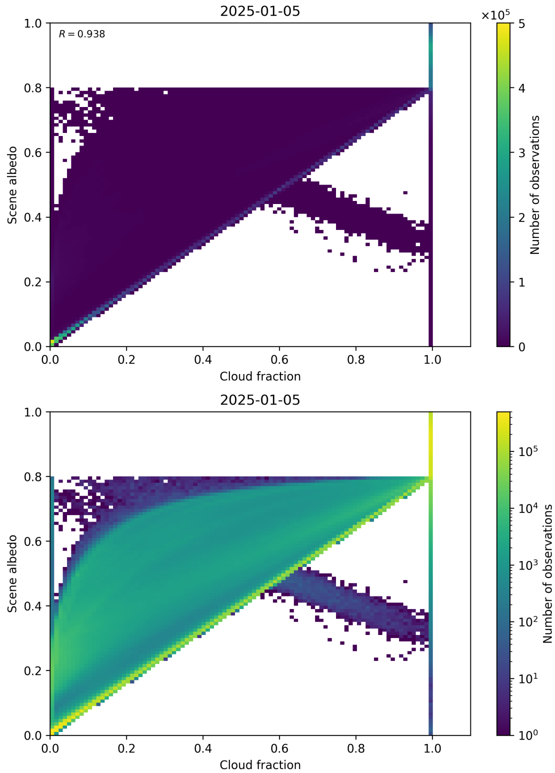
Figure 75: Scatter density plot of “Cloud fraction” against “Scene albedo” for 2025-01-04 to 2025-01-06.
