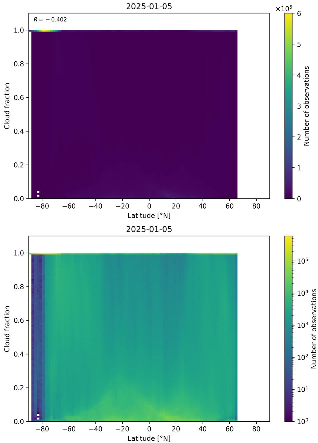
Figure 90: Scatter density plot of “Latitude” against “Cloud fraction” for 2025-01-04 to 2025-01-06.
