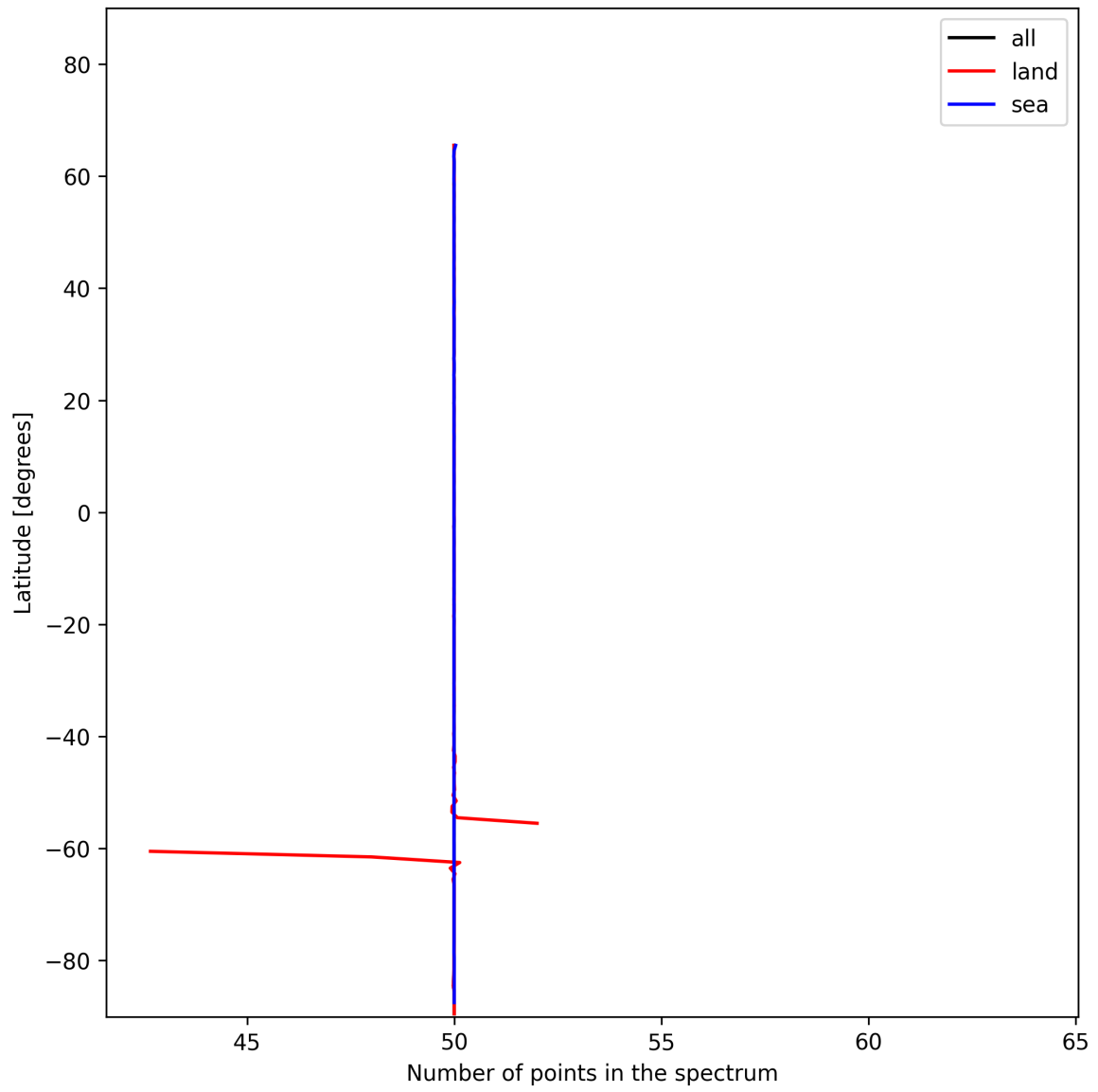
Figure 27: Zonal average of “Number of points in the spectrum” for 2025-01-04 to 2025-01-06.
