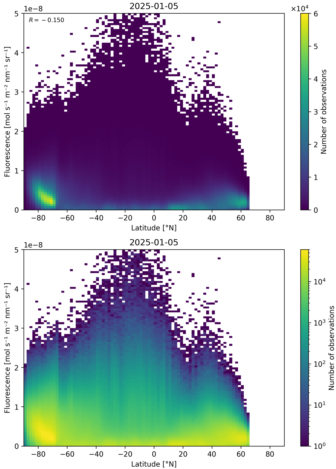
Figure 92: Scatter density plot of “Latitude” against “Fluorescence” for 2025-01-04 to 2025-01-06.
