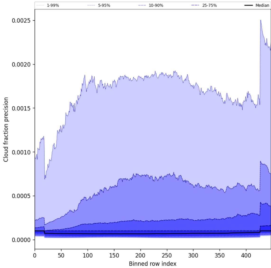
Figure 50: Along track statistics of “Cloud fraction precision” for 2025-01-04 to 2025-01-06
