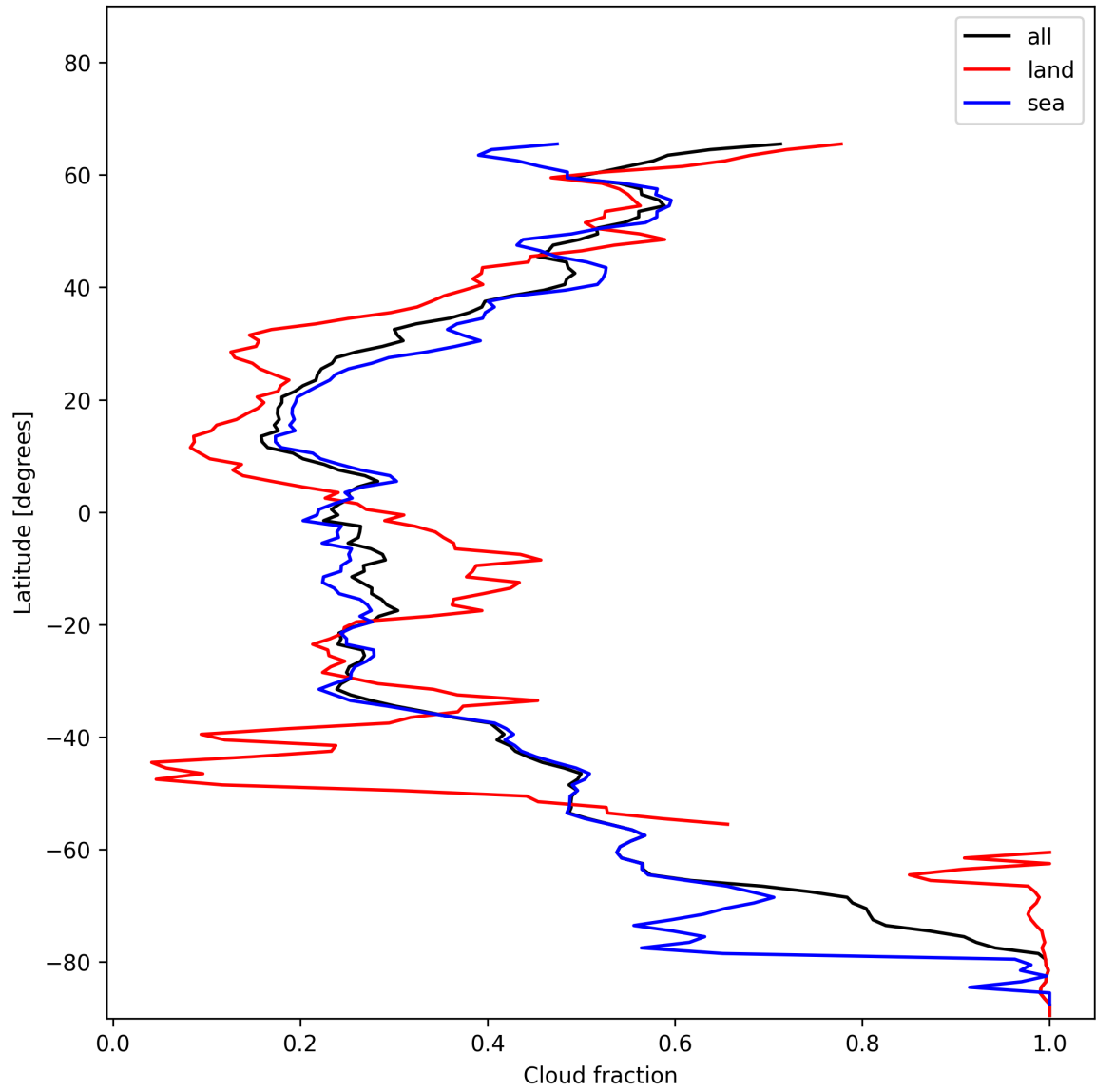
Figure 15: Zonal average of “Cloud fraction” for 2025-01-04 to 2025-01-06.
