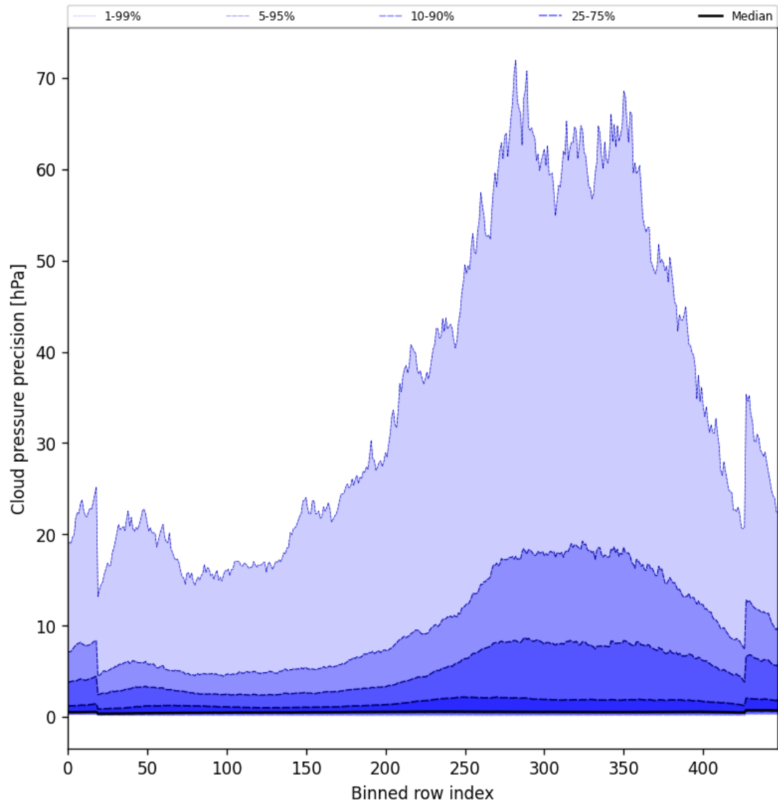
Figure 48: Along track statistics of “Cloud pressure precision” for 2025-01-05 to 2025-01-07
