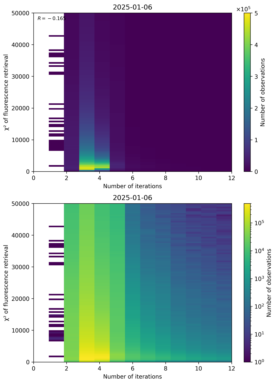
Figure 97: Scatter density plot of “Number of iterations” against “ \chi^2 of fluorescence retrieval” for 2025-01-05 to 2025-01-07.
