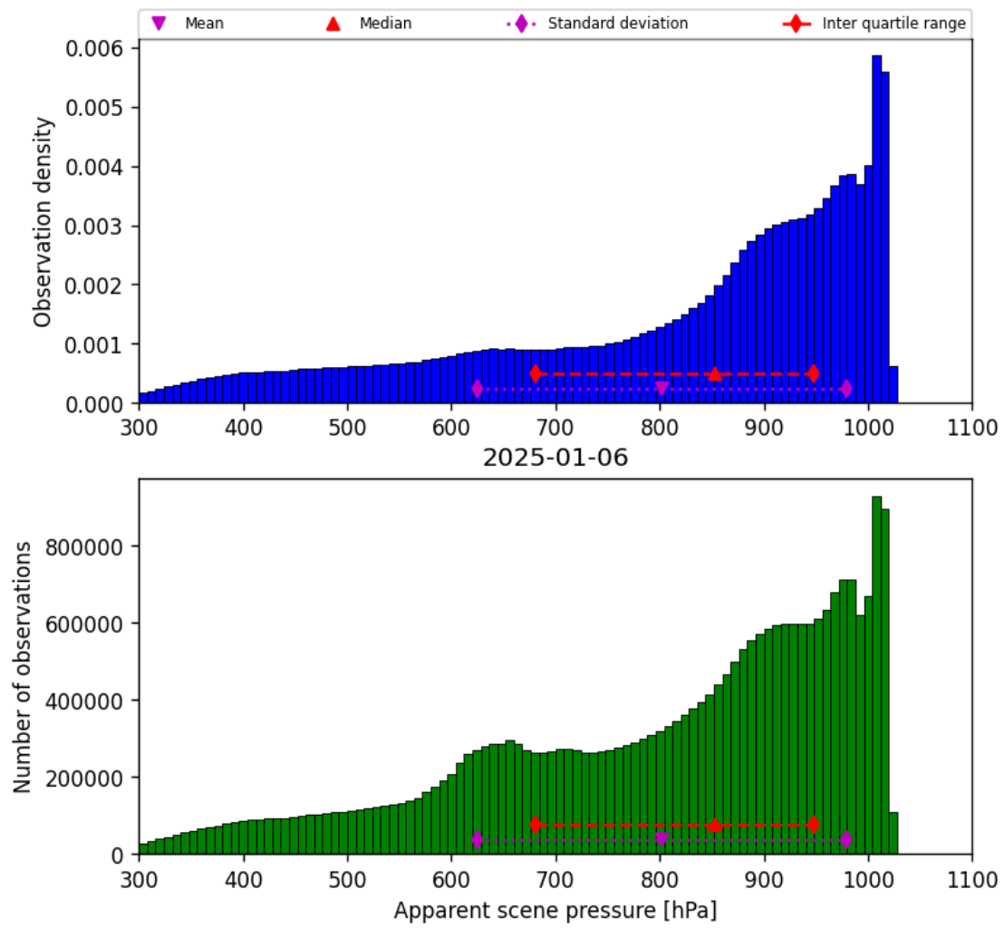
Figure 36: Histogram of “Apparent scene pressure” for 2025-01-05 to 2025-01-07
