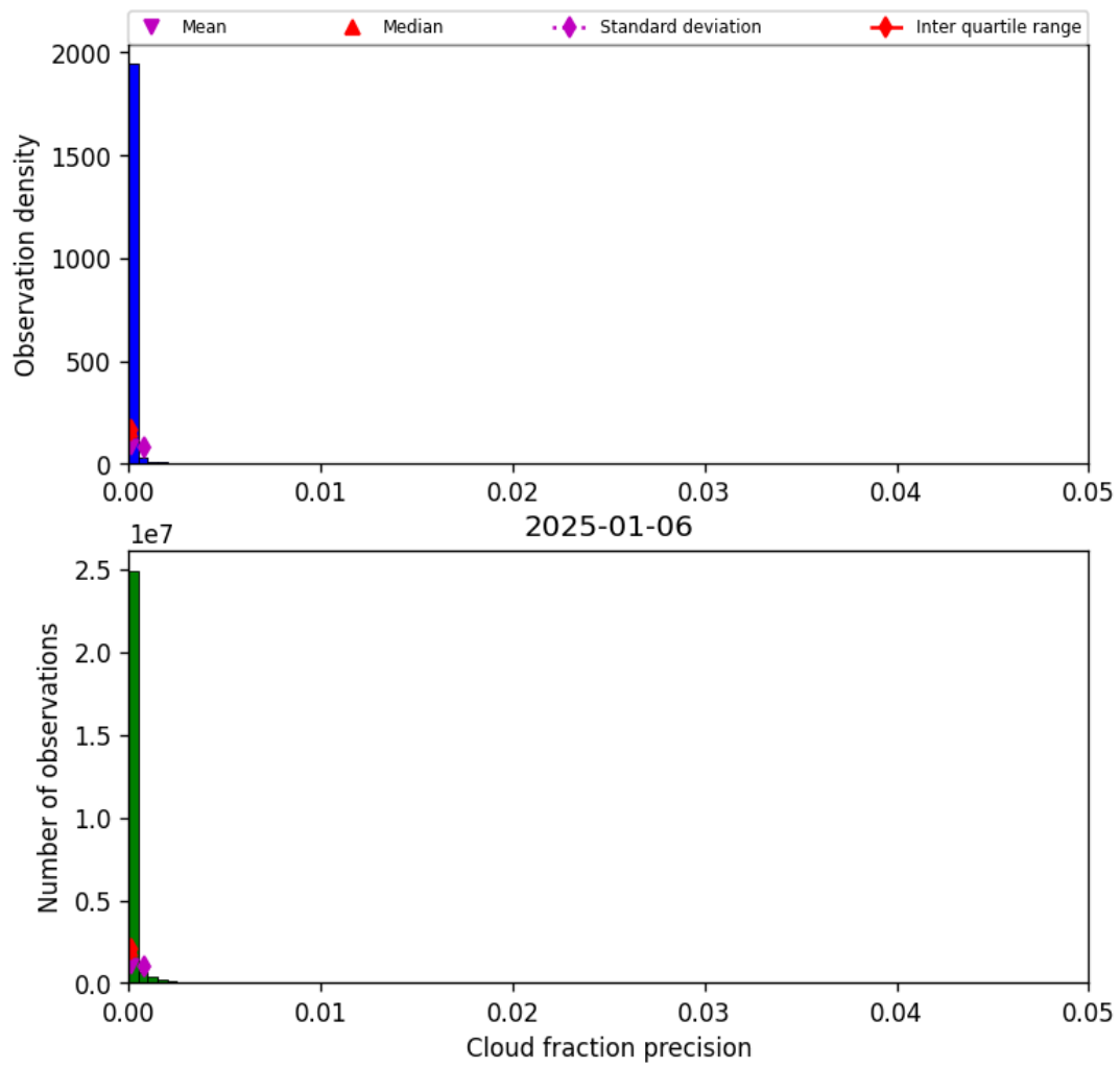
Figure 33: Histogram of “Cloud fraction precision” for 2025-01-05 to 2025-01-07
