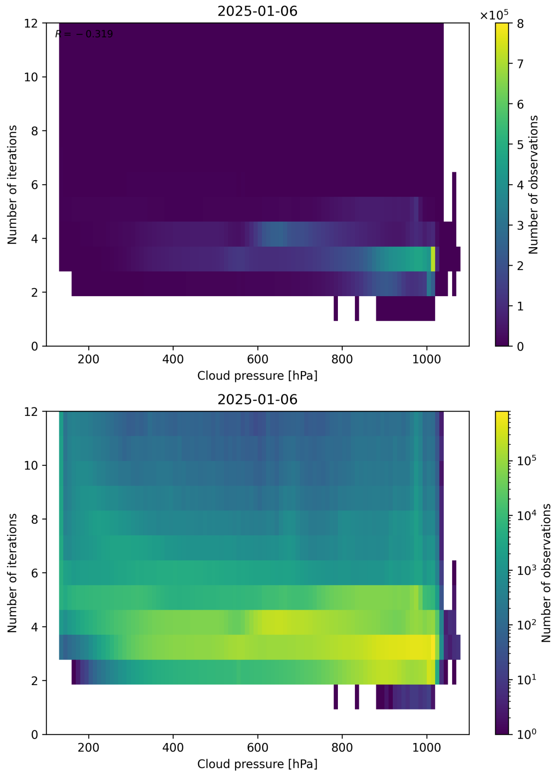
Figure 81: Scatter density plot of “Cloud pressure” against “Number of iterations” for 2025-01-05 to 2025-01-07.
