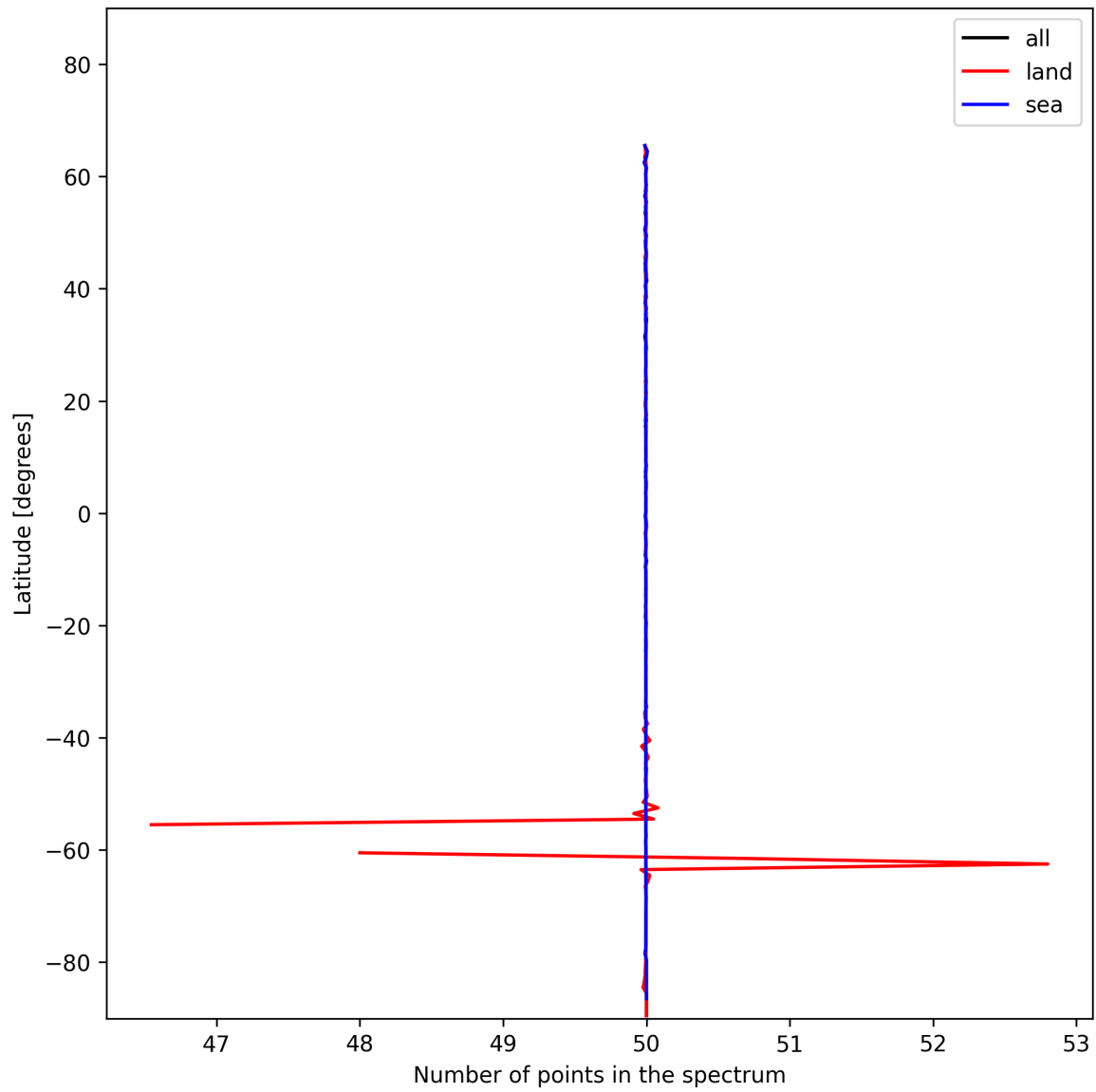
Figure 27: Zonal average of “Number of points in the spectrum” for 2025-01-05 to 2025-01-07.
