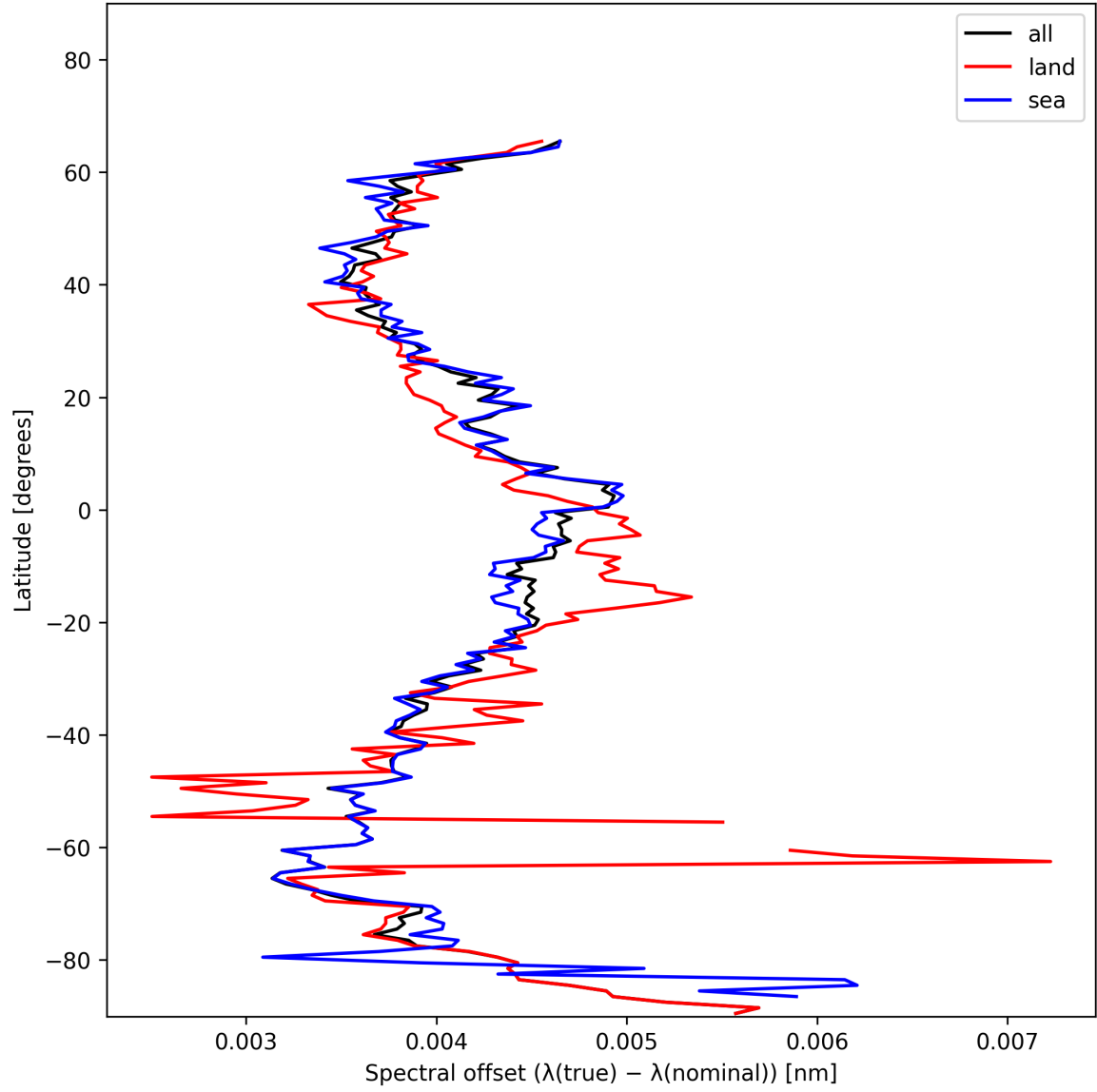
Figure 28: Zonal average of “Spectral offset ( \lambda_{\text{true}} - \lambda_{\text{nominal}} )” for 2025-01-05 to 2025-01-07.
