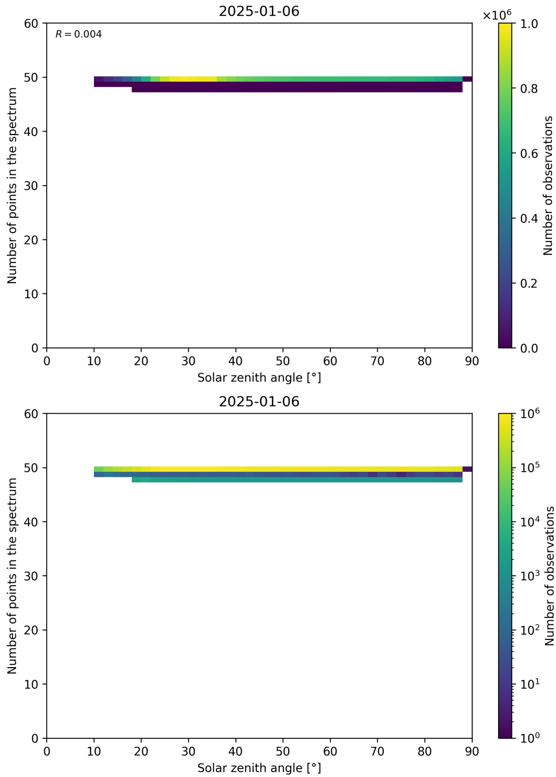
Figure 115: Scatter density plot of “Solar zenith angle” against “Number of points in the spectrum” for 2025-01-05 to 2025-01-07.
