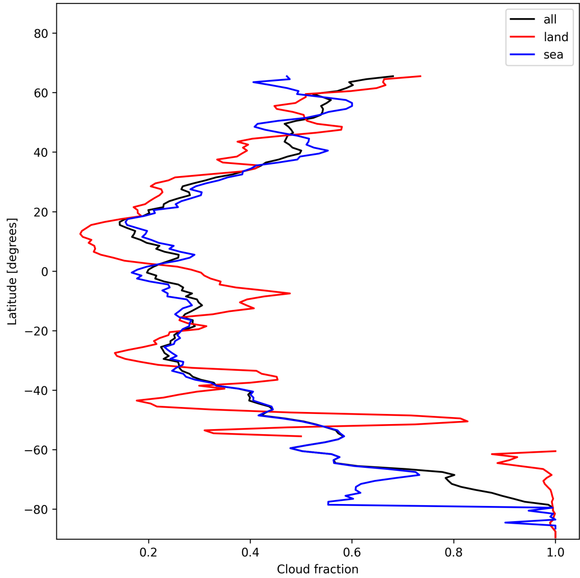
Figure 15: Zonal average of “Cloud fraction” for 2025-01-05 to 2025-01-07.
