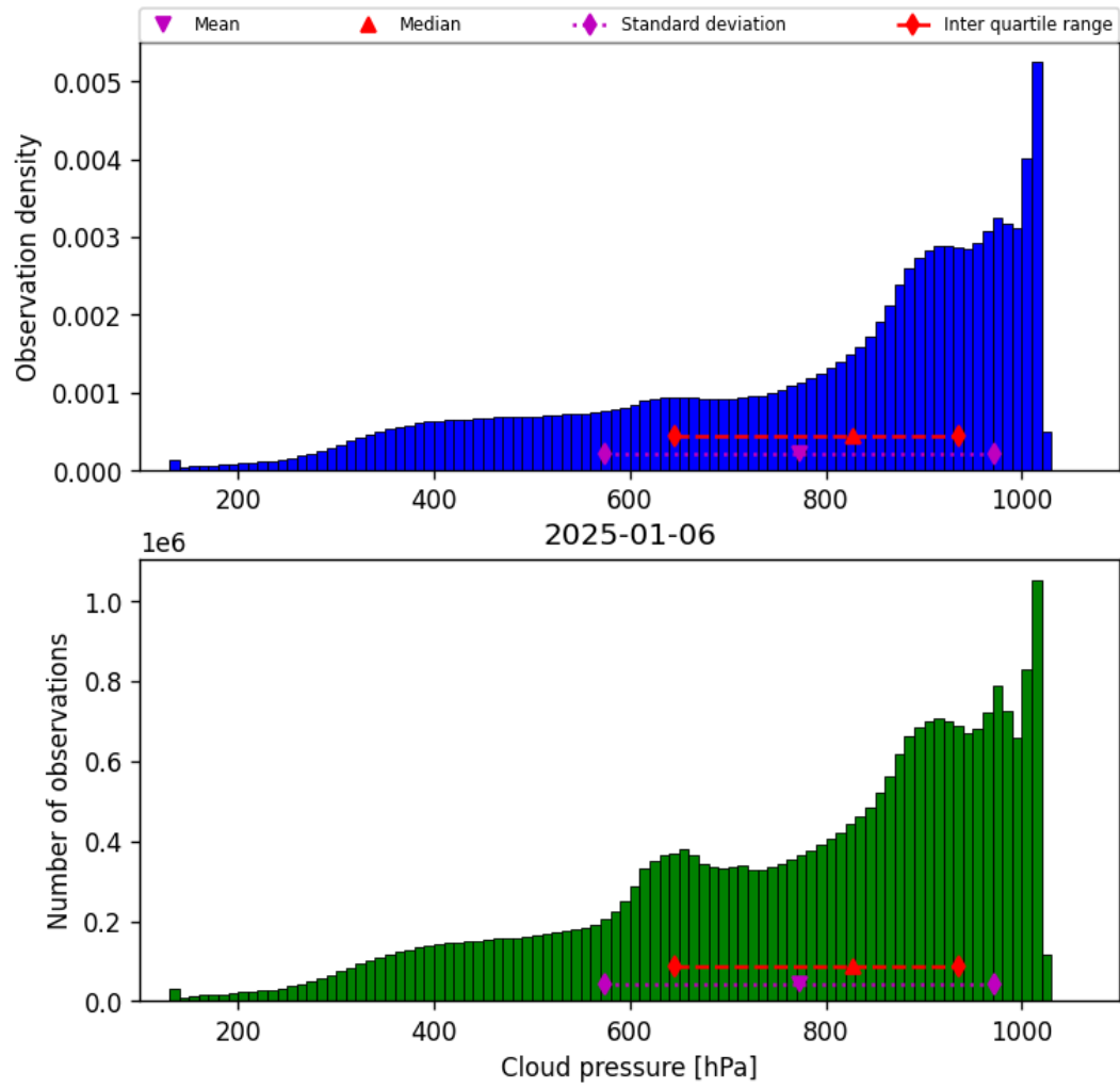
Figure 30: Histogram of “Cloud pressure” for 2025-01-05 to 2025-01-07
