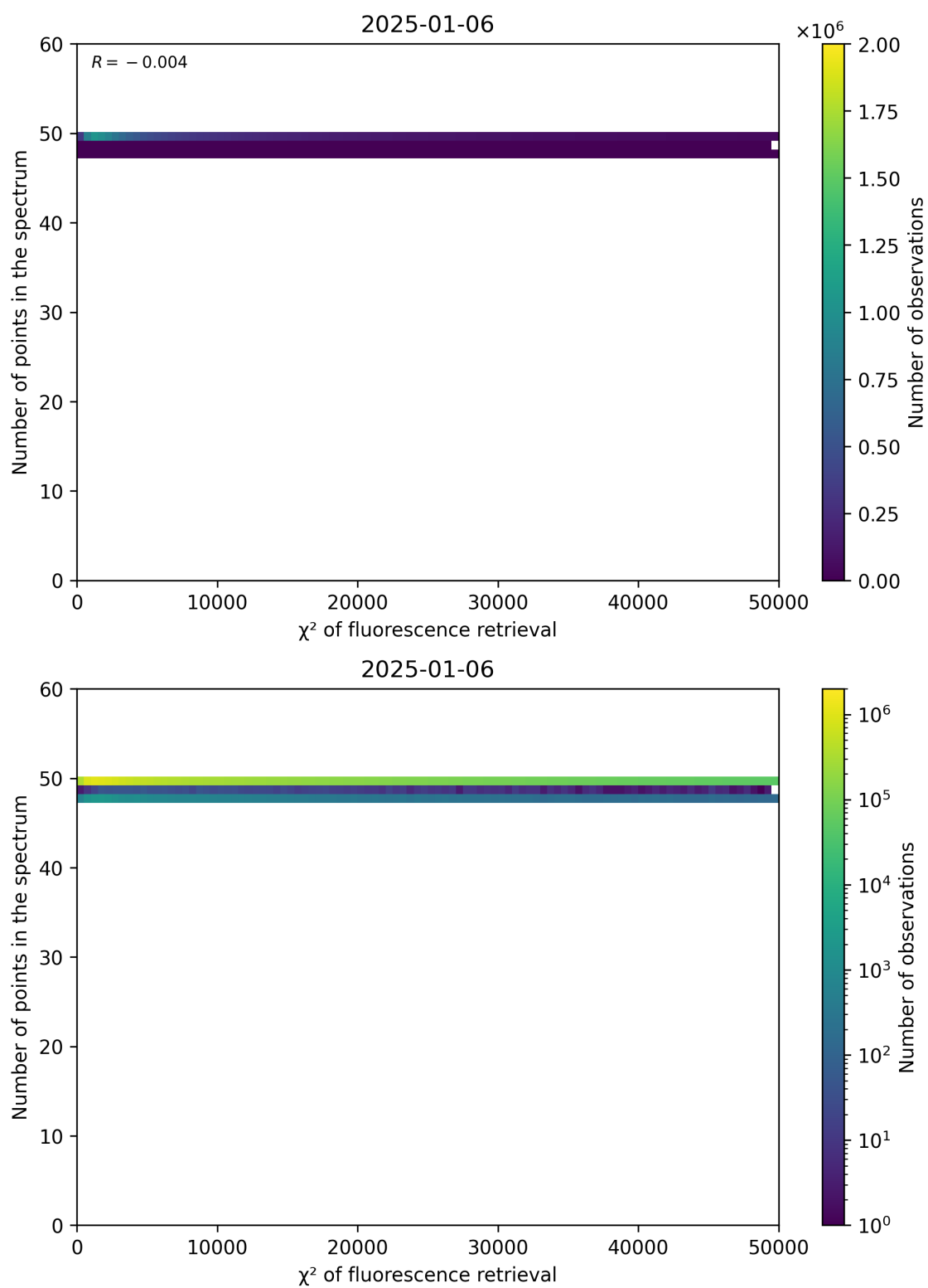
Figure 68: Scatter density plot of “ \chi^2 of fluorescence retrieval” against “Number of points in the spectrum” for 2025-01-05 to 2025-01-07.
