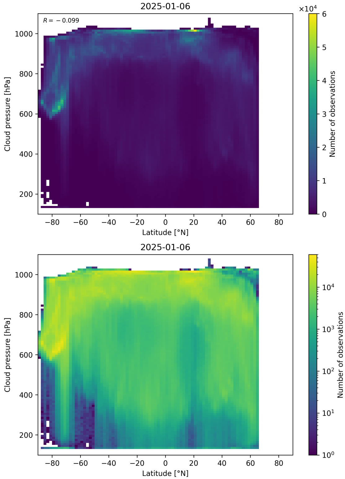
Figure 91: Scatter density plot of “Latitude” against “Cloud pressure” for 2025-01-05 to 2025-01-07.
