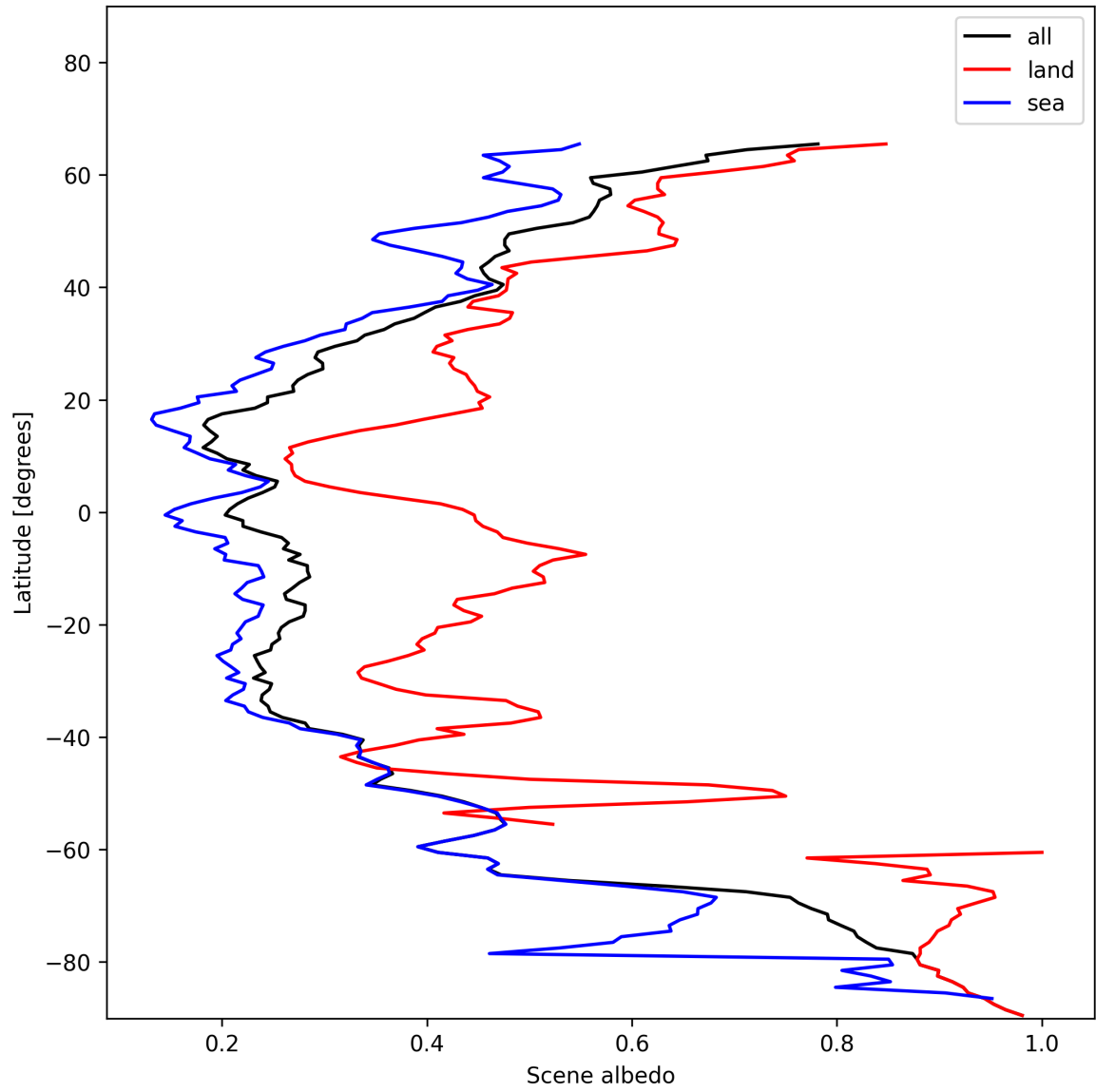
Figure 17: Zonal average of “Scene albedo” for 2025-01-05 to 2025-01-07.
