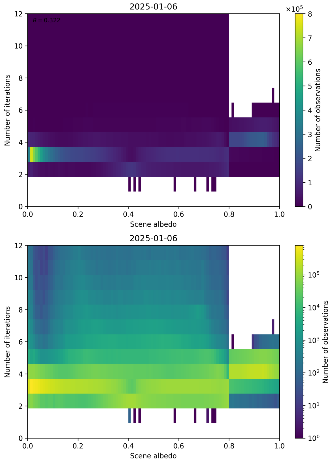
Figure 105: Scatter density plot of “Scene albedo” against “Number of iterations” for 2025-01-05 to 2025-01-07.
