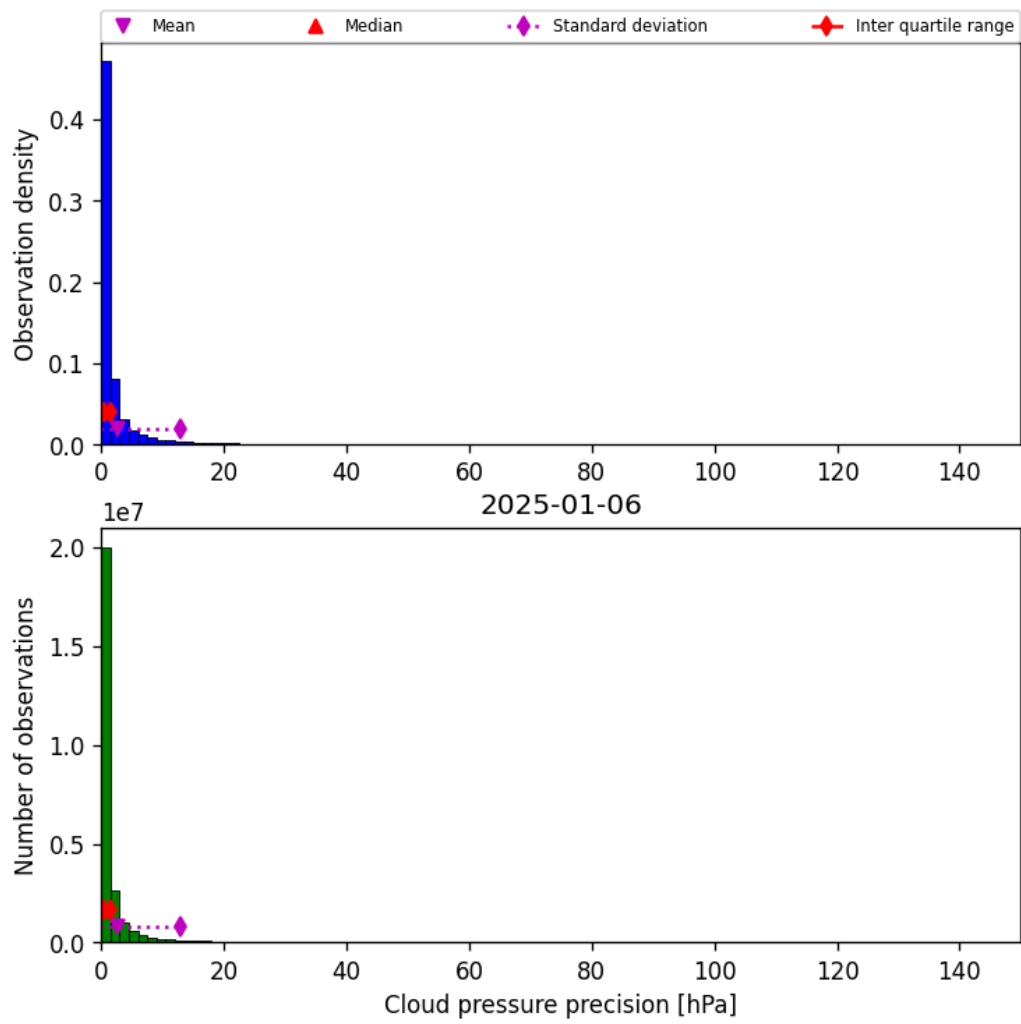
Figure 31: Histogram of “Cloud pressure precision” for 2025-01-05 to 2025-01-07
