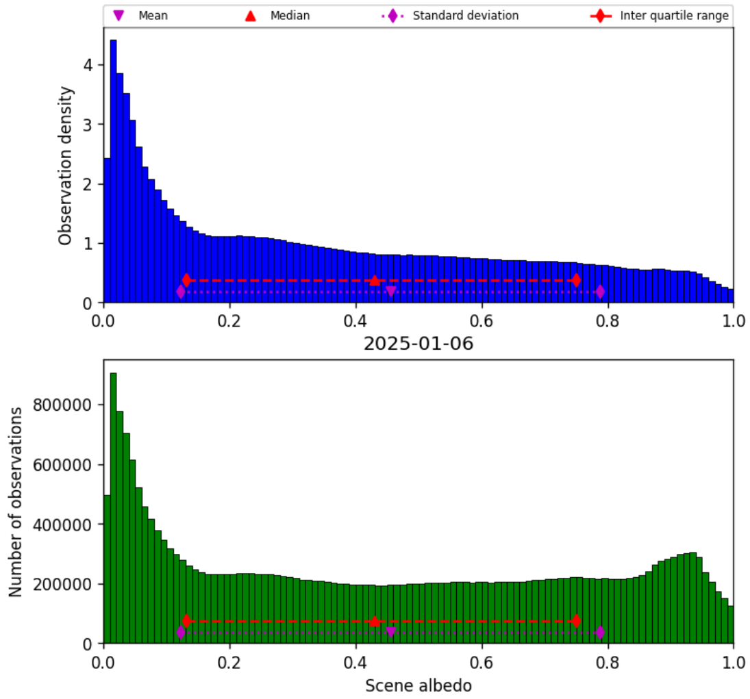
Figure 34: Histogram of “Scene albedo” for 2025-01-05 to 2025-01-07
