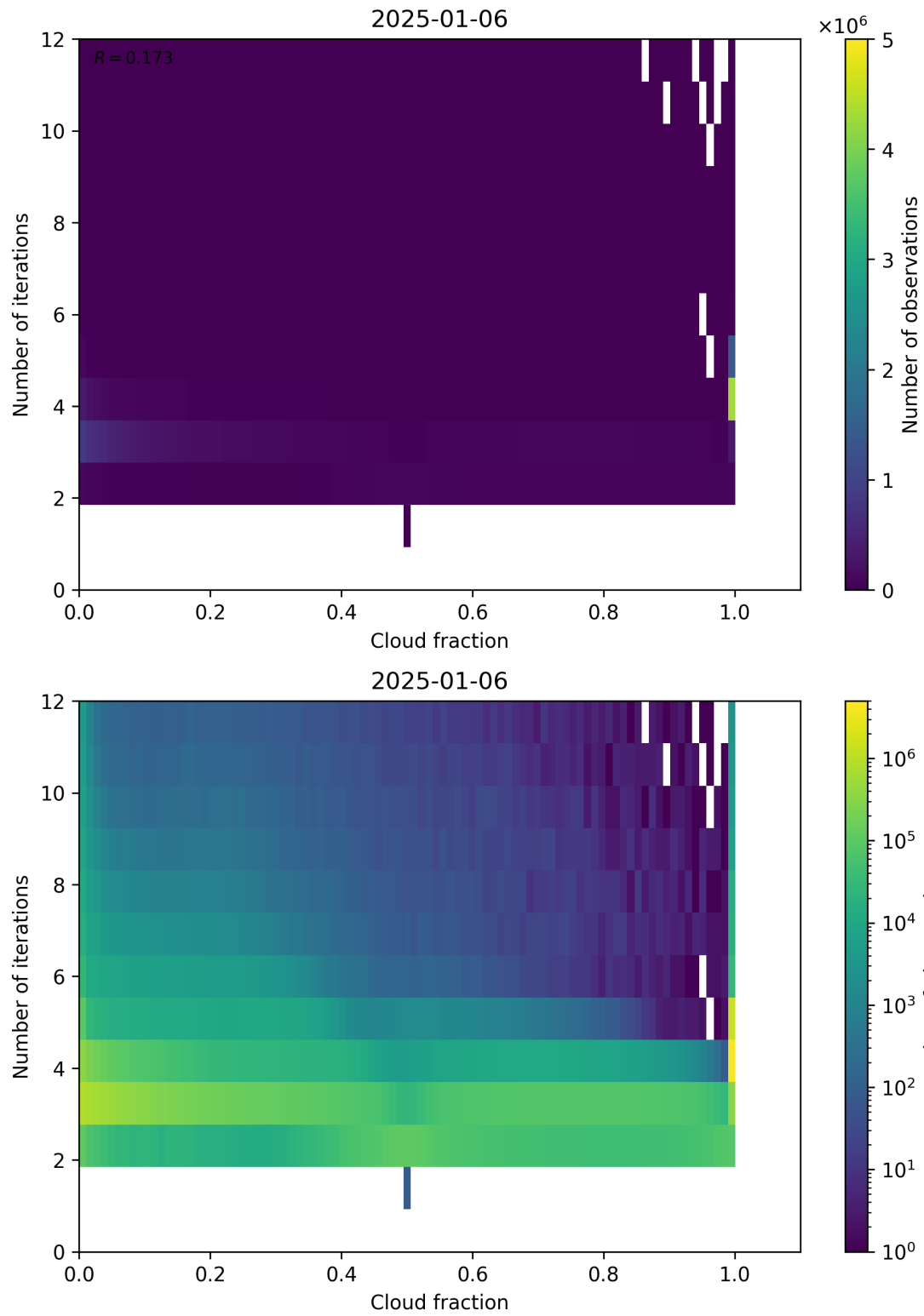
Figure 73: Scatter density plot of “Cloud fraction” against “Number of iterations” for 2025-01-05 to 2025-01-07.
