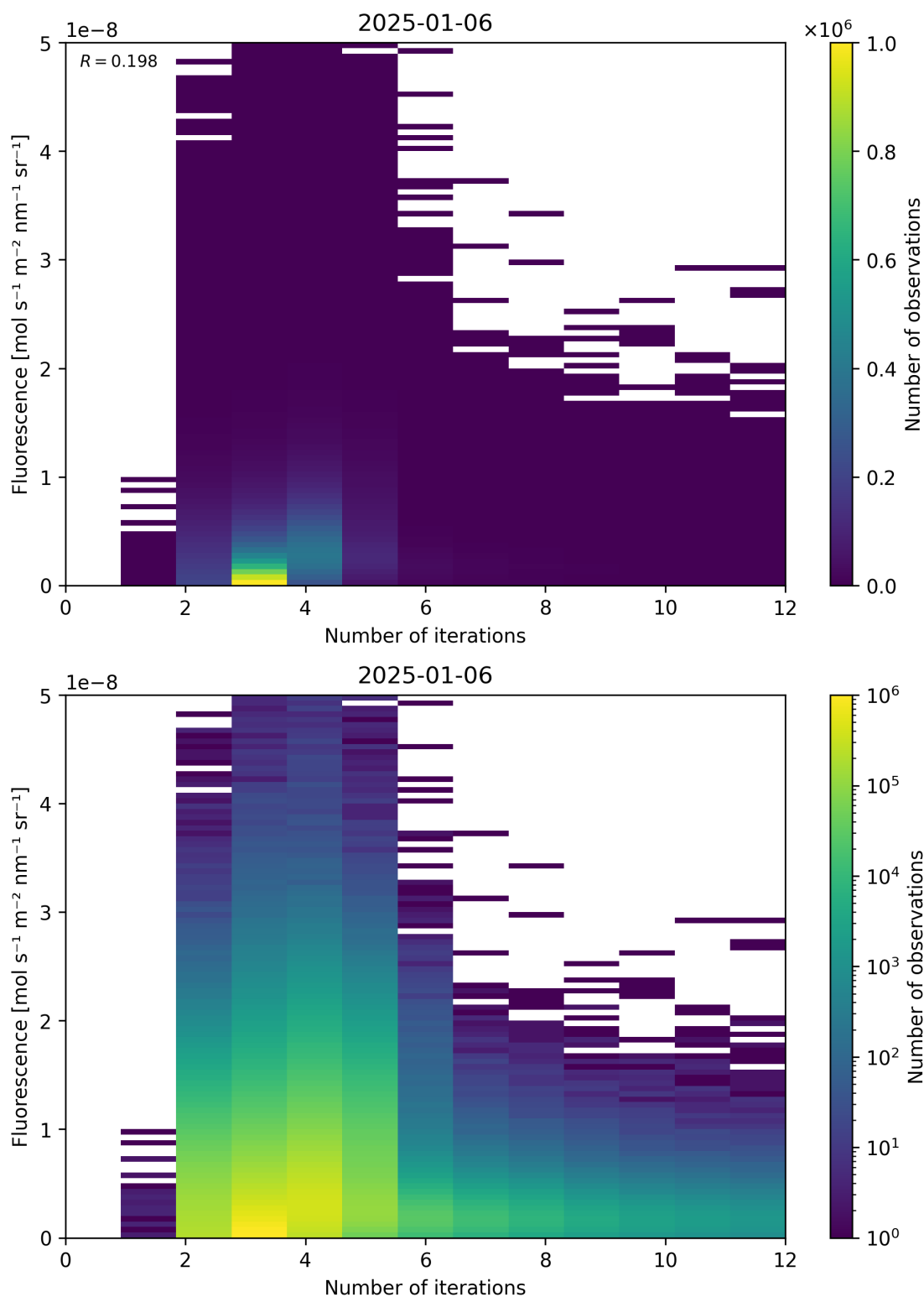
Figure 98: Scatter density plot of “Number of iterations” against “Fluorescence” for 2025-01-05 to 2025-01-07.
