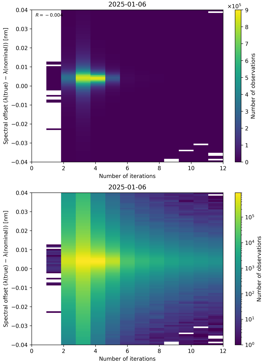
Figure 100: Scatter density plot of “Number of iterations” against “Spectral offset ( \lambda_{\text{true}} - \lambda_{\text{nominal}} )” for 2025-01-05 to 2025-01-07.
