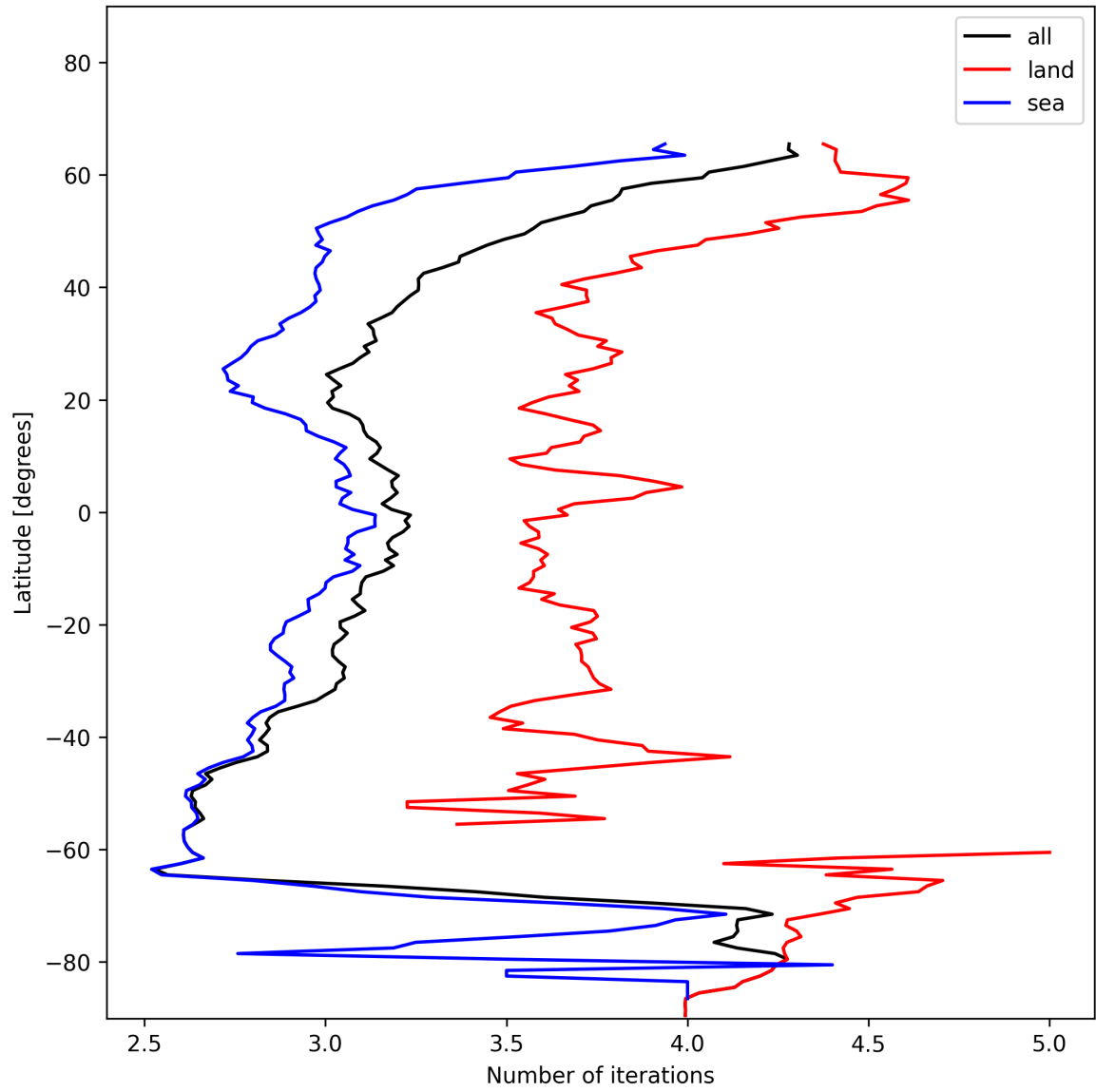
Figure 22: Zonal average of “Number of iterations” for 2025-01-05 to 2025-01-07.
