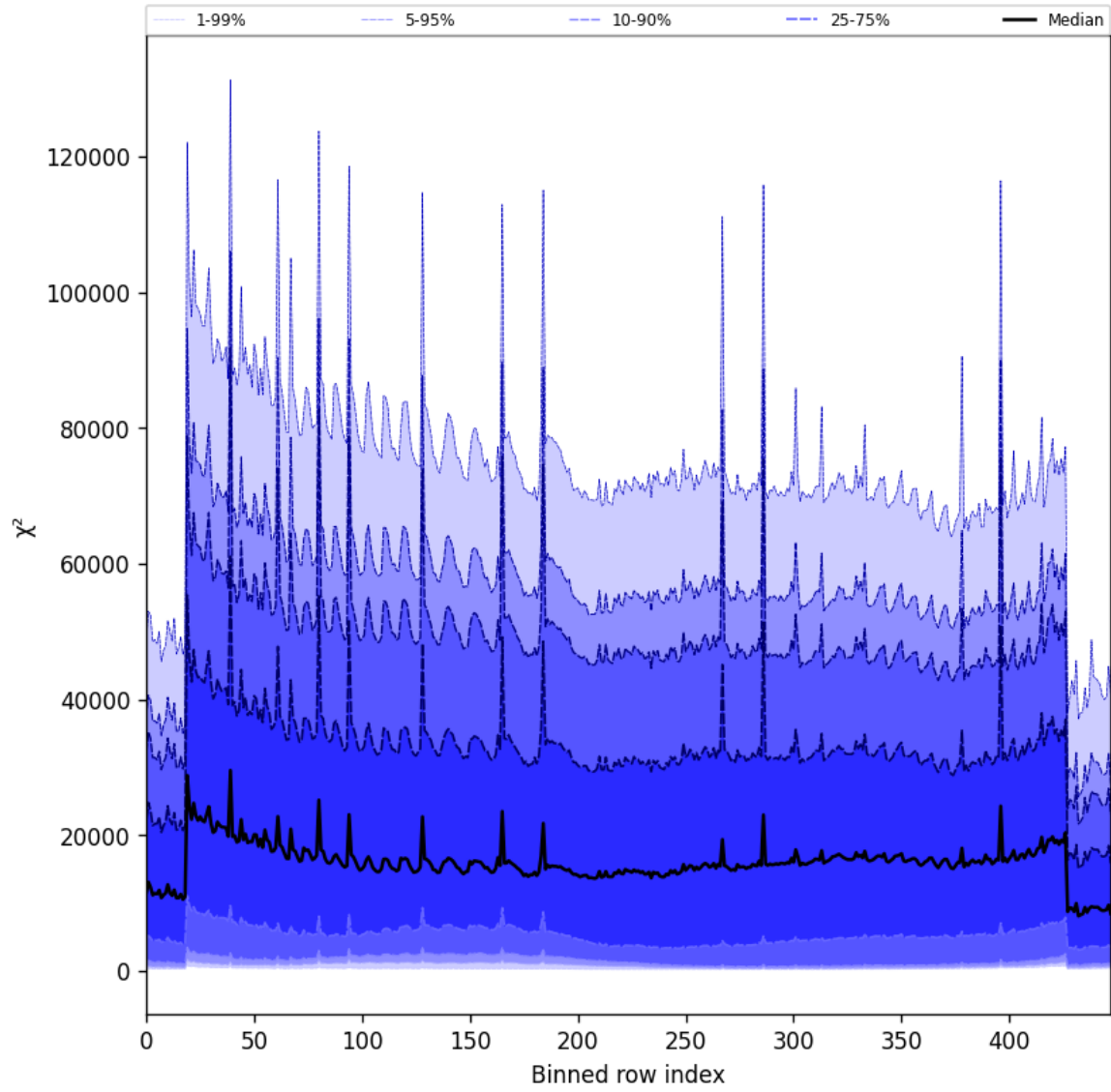
Figure 55: Along track statistics of “ \chi^2 ” for 2025-01-05 to 2025-01-07
