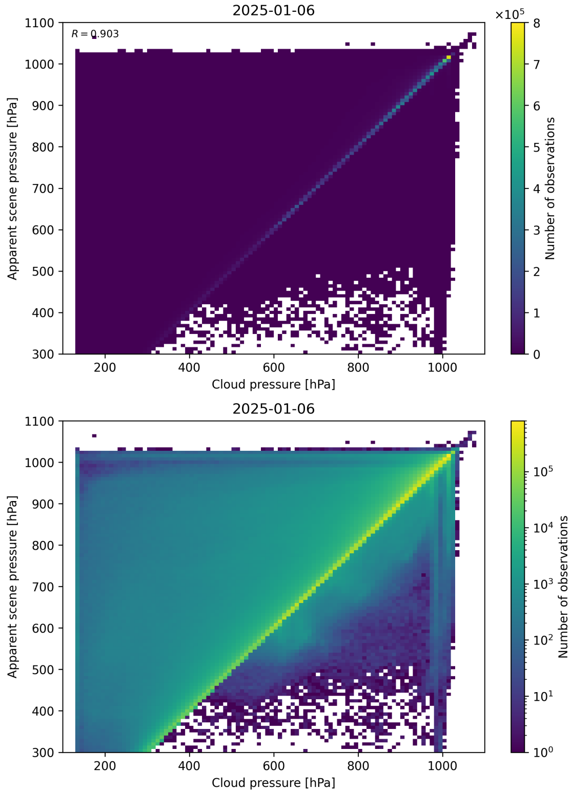
Figure 77: Scatter density plot of “Cloud pressure” against “Apparent scene pressure” for 2025-01-05 to 2025-01-07.
