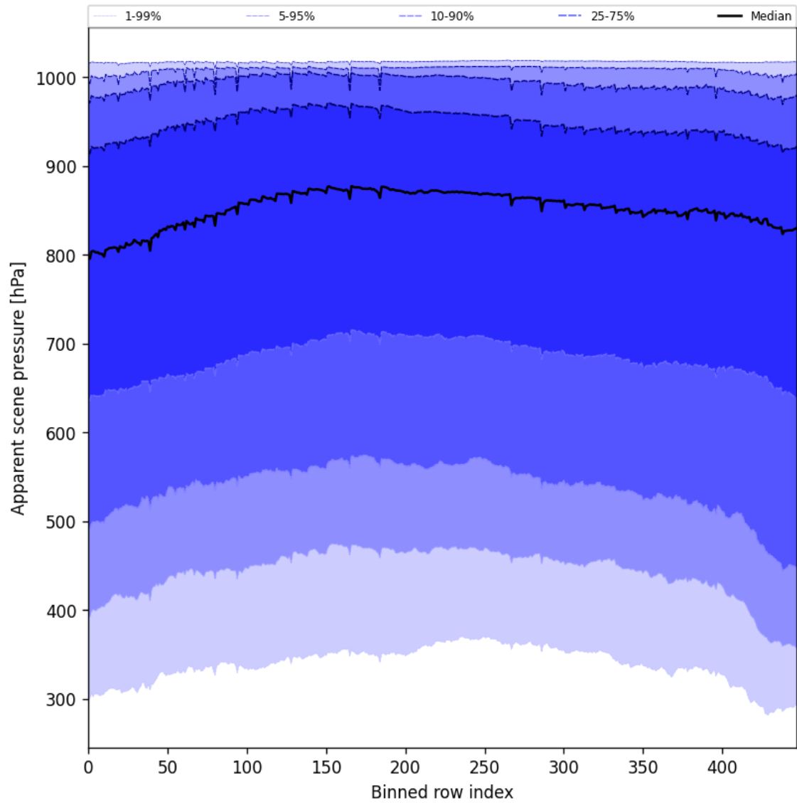
Figure 53: Along track statistics of “Apparent scene pressure” for 2025-01-05 to 2025-01-07
