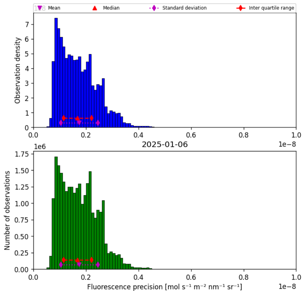
Figure 41: Histogram of “Fluorescence precision” for 2025-01-05 to 2025-01-07
