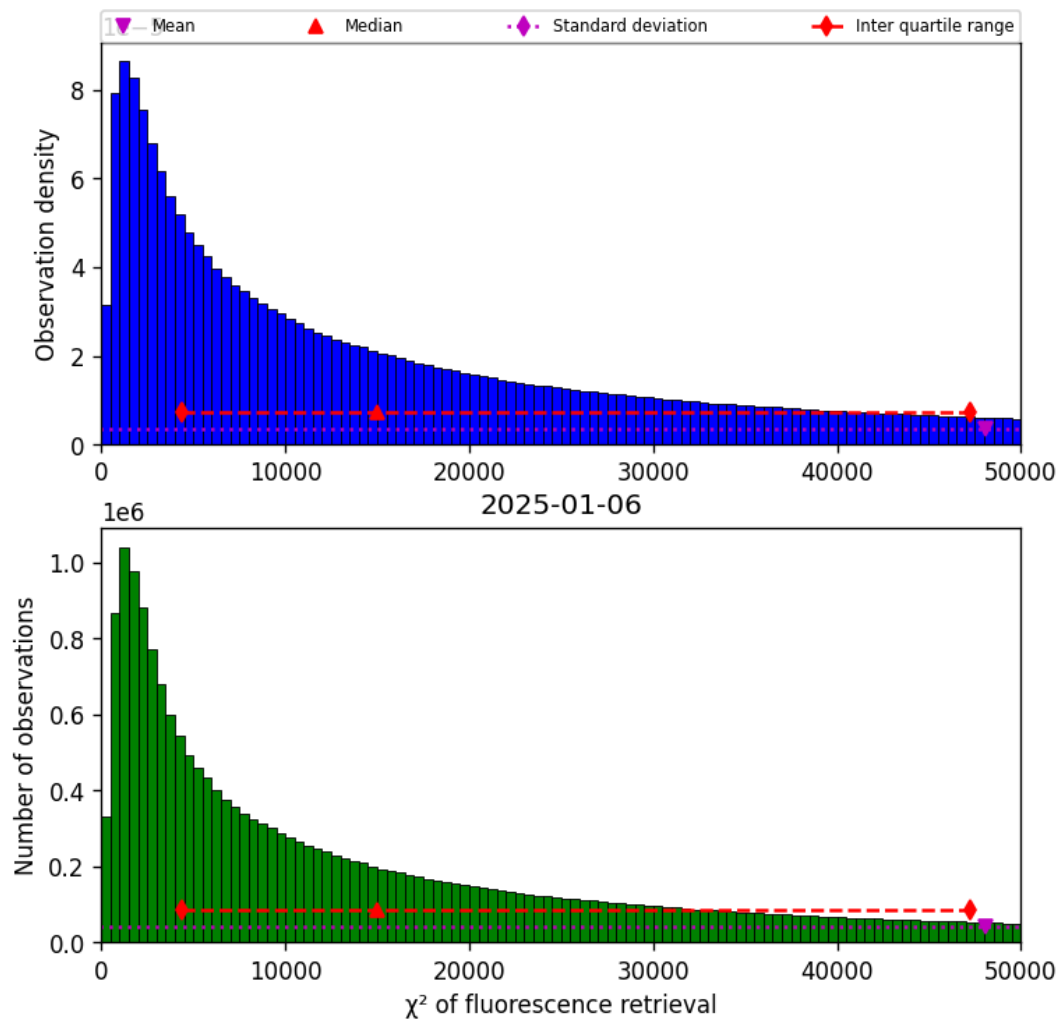
Figure 42: Histogram of “ \chi^2 of fluorescence retrieval” for 2025-01-05 to 2025-01-07
