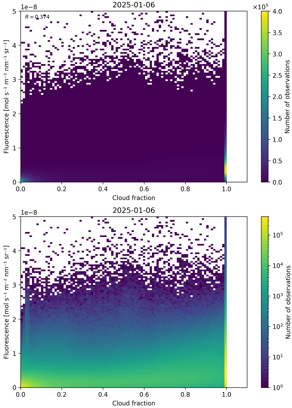
Figure 72: Scatter density plot of “Cloud fraction” against “Fluorescence” for 2025-01-05 to 2025-01-07.
