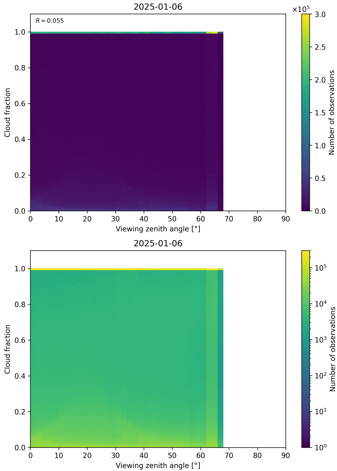
Figure 120: Scatter density plot of “Viewing zenith angle” against “Cloud fraction” for 2025-01-05 to 2025-01-07.
