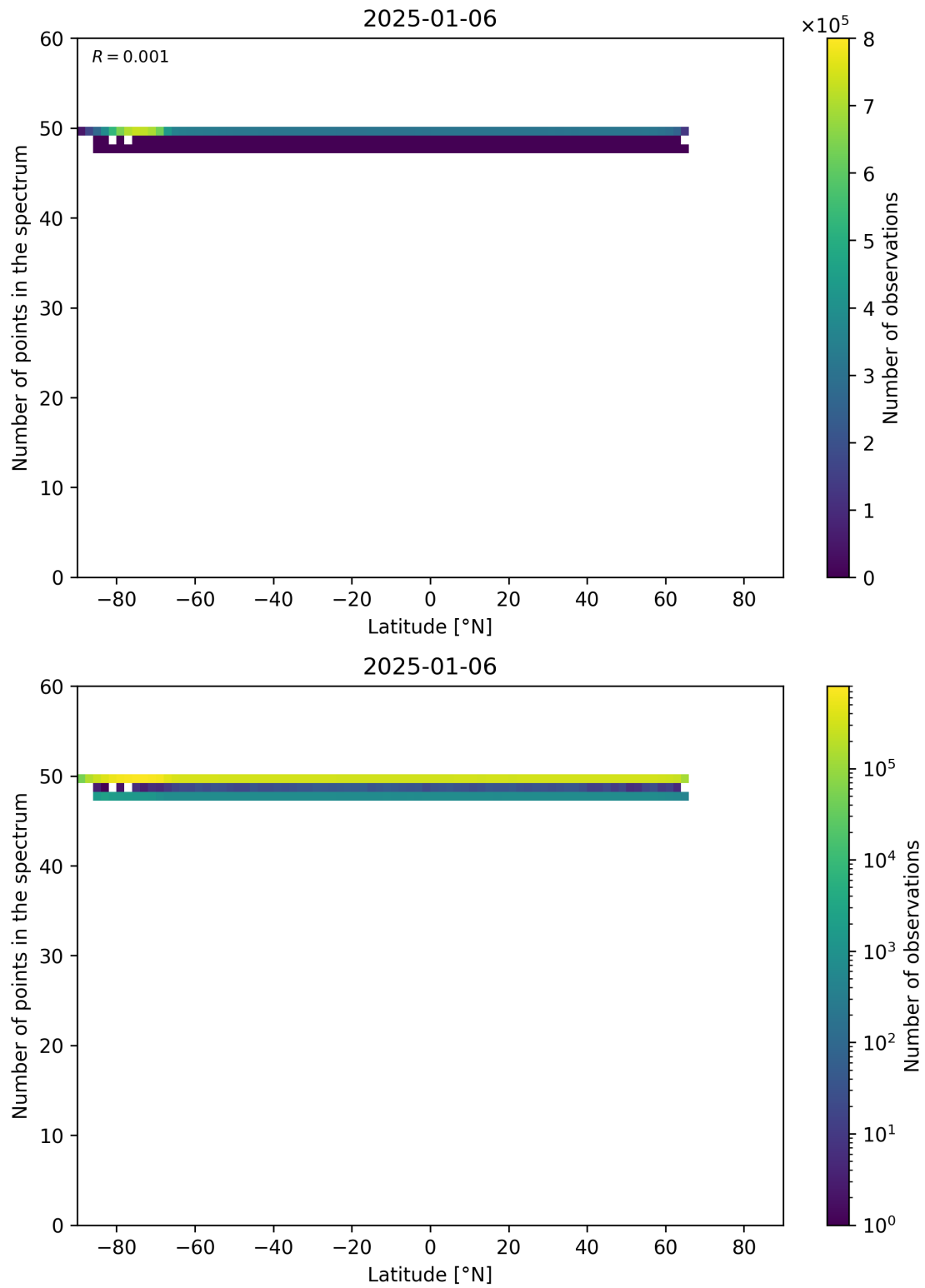
Figure 94: Scatter density plot of “Latitude” against “Number of points in the spectrum” for 2025-01-05 to 2025-01-07.
