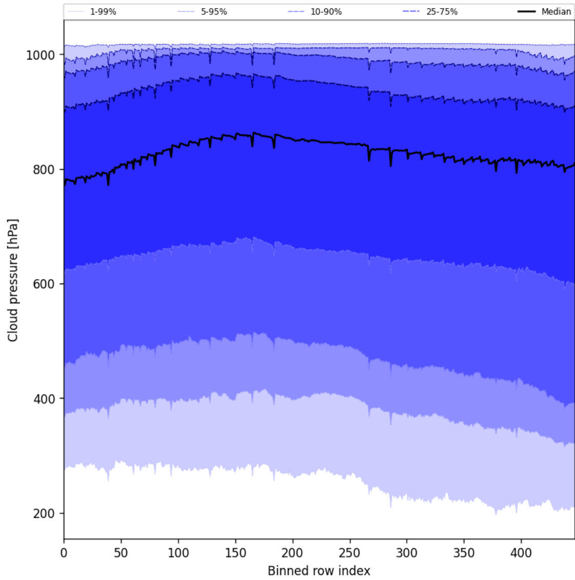
Figure 47: Along track statistics of “Cloud pressure” for 2025-01-05 to 2025-01-07
