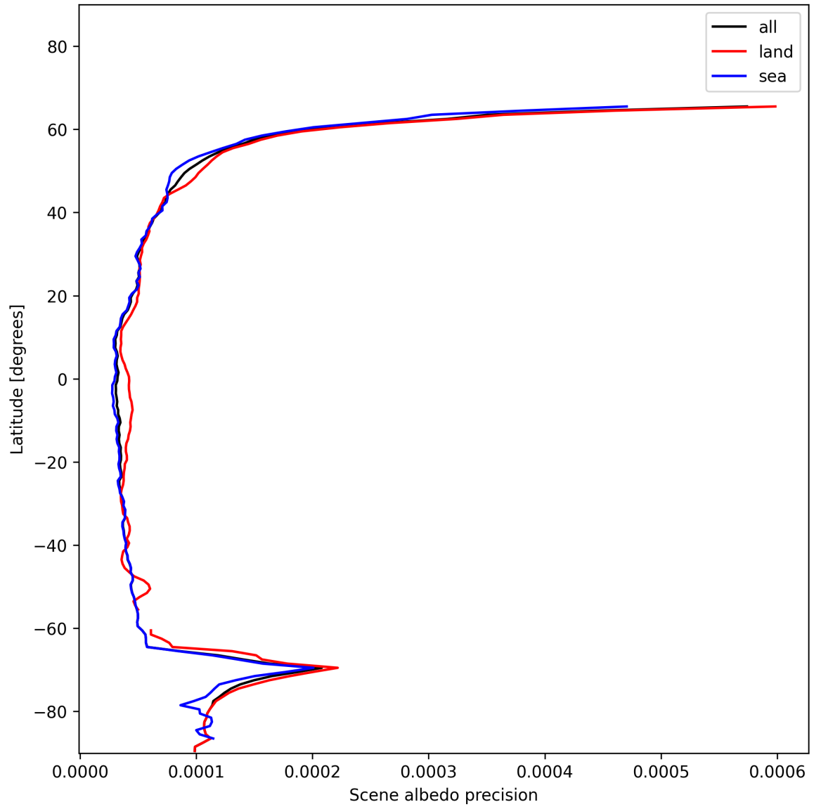
Figure 18: Zonal average of “Scene albedo precision” for 2025-01-05 to 2025-01-07.
