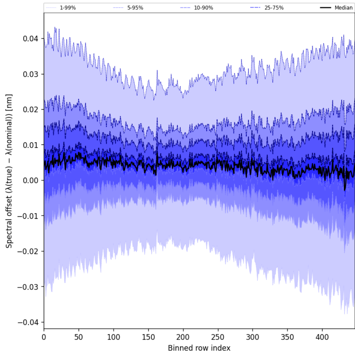
Figure 62: Along track statistics of “Spectral offset ( \lambda_{\text{true}} - \lambda_{\text{nominal}} )” for 2025-01-05 to 2025-01-07
