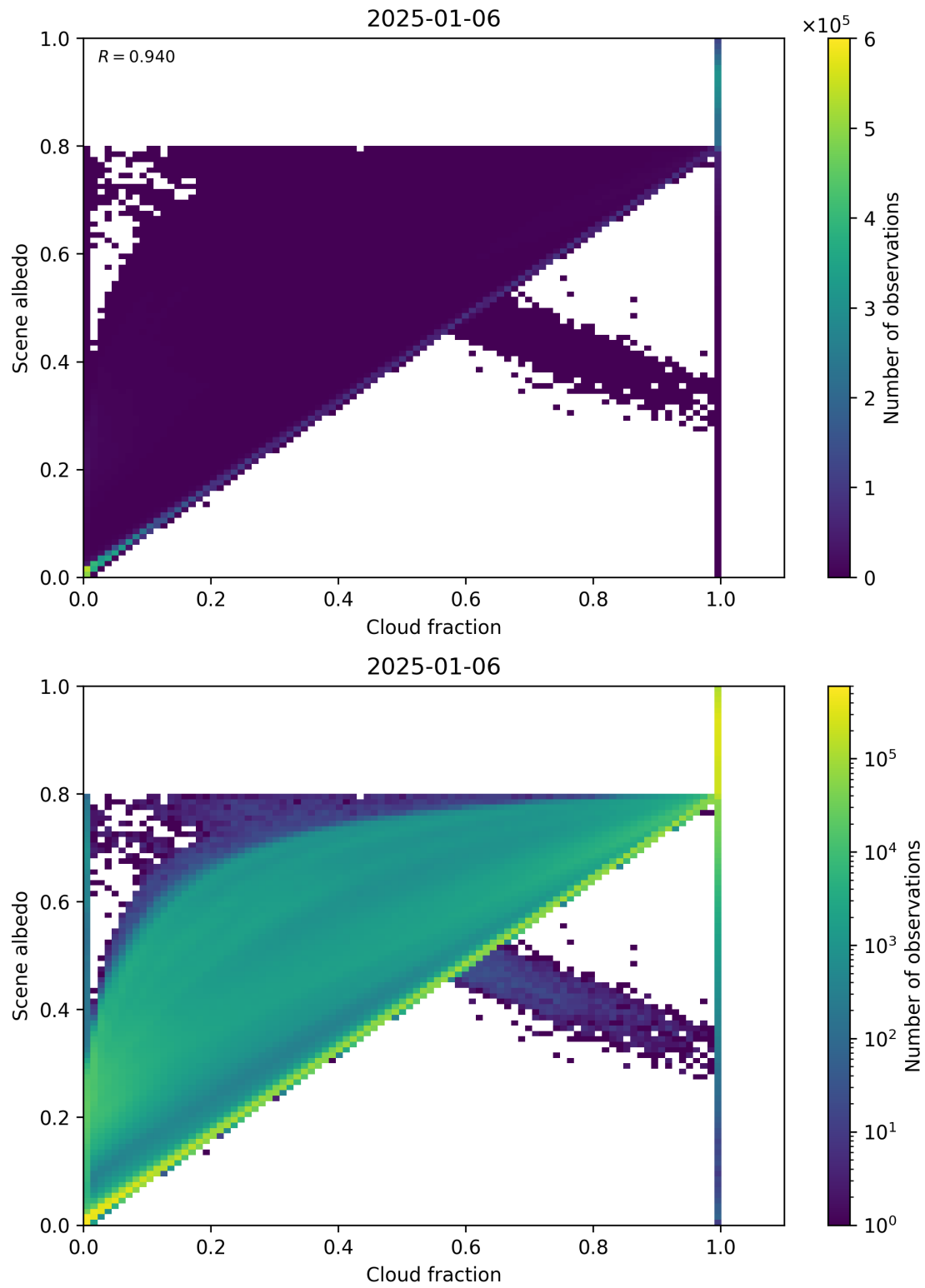
Figure 75: Scatter density plot of “Cloud fraction” against “Scene albedo” for 2025-01-05 to 2025-01-07.
