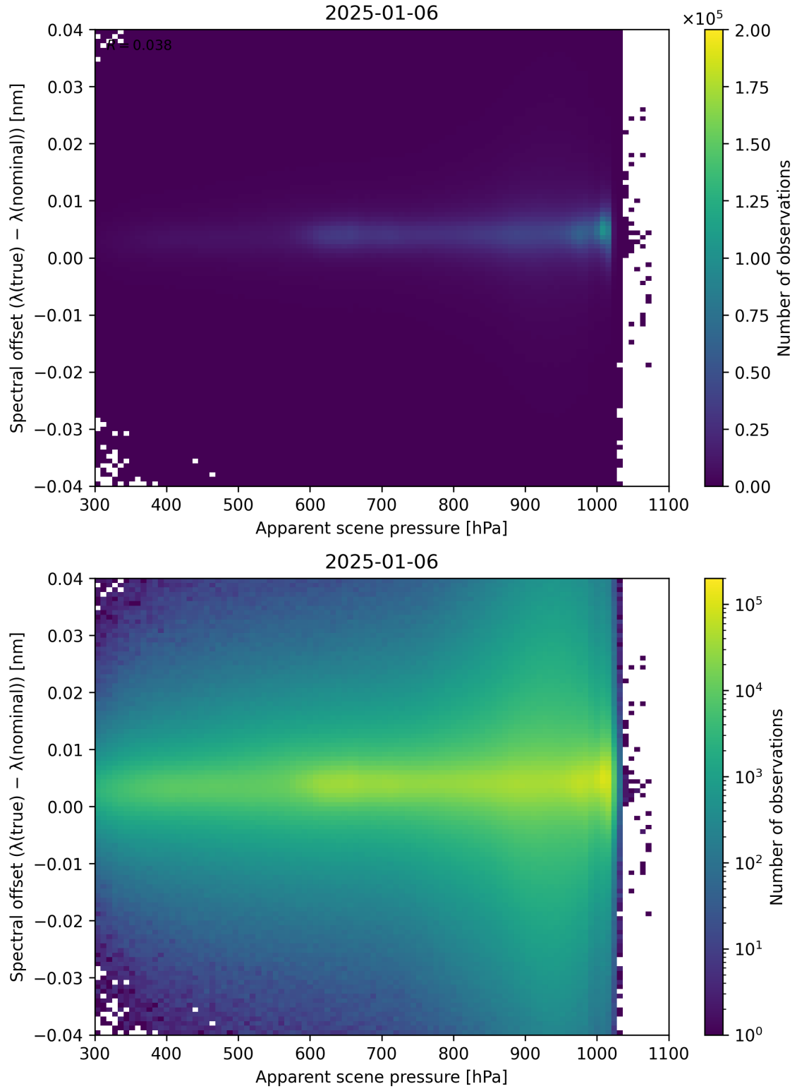
Figure 67: Scatter density plot of “Apparent scene pressure” against “Spectral offset ( \lambda_{\text{true}} - \lambda_{\text{nominal}} )” for 2025-01-05 to 2025-01-07.
