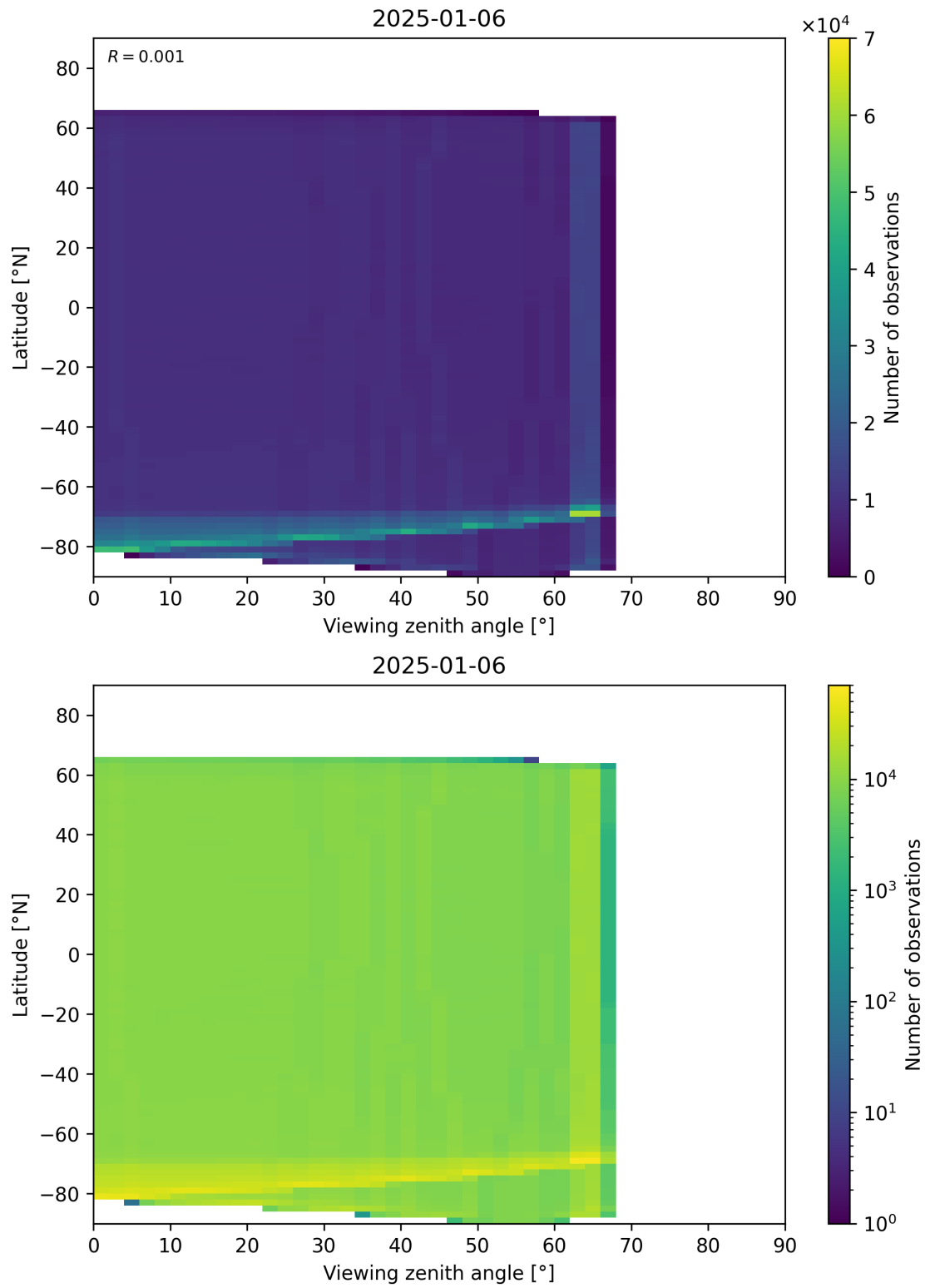
Figure 123: Scatter density plot of “Viewing zenith angle” against “Latitude” for 2025-01-05 to 2025-01-07.
