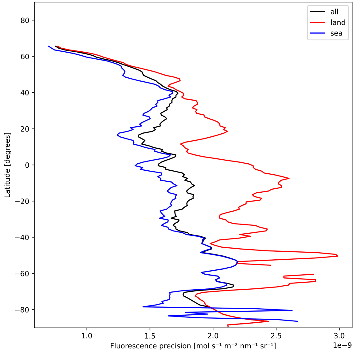
Figure 24: Zonal average of “Fluorescence precision” for 2025-01-05 to 2025-01-07.
