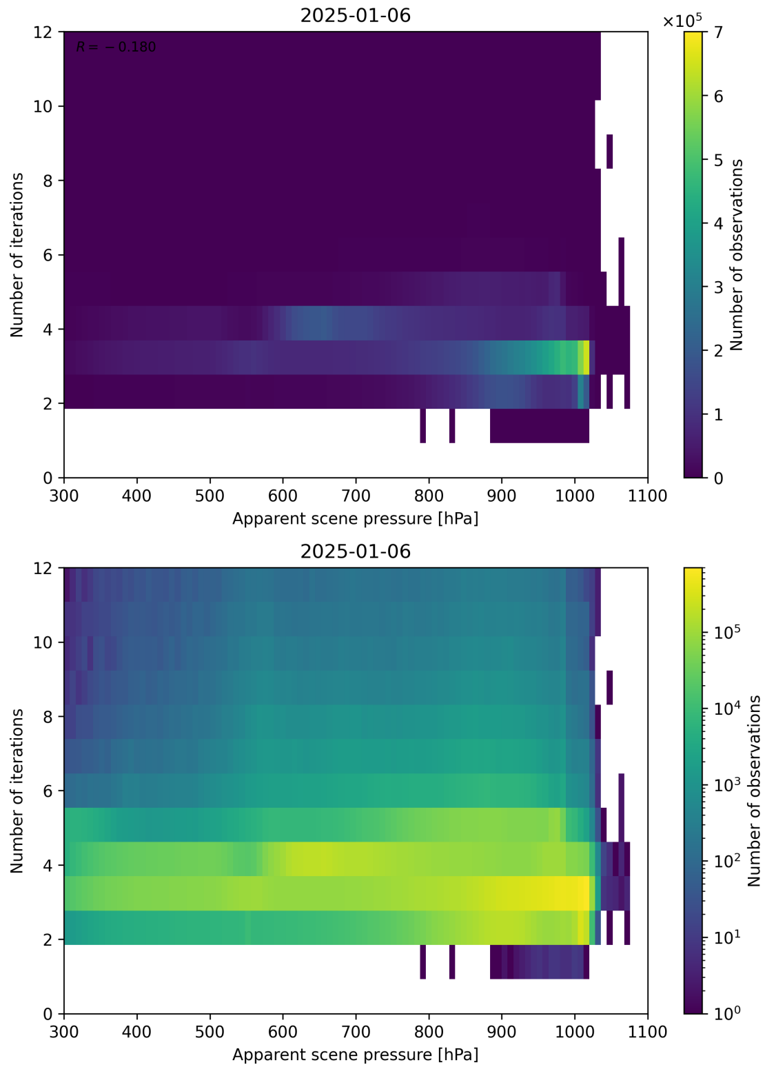
Figure 65: Scatter density plot of “Apparent scene pressure” against “Number of iterations” for 2025-01-05 to 2025-01-07.
