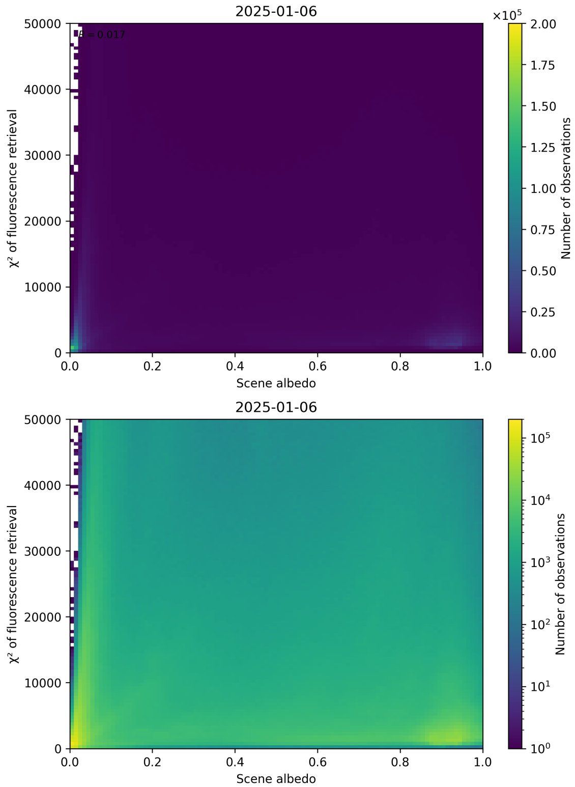
Figure 103: Scatter density plot of “Scene albedo” against “ \chi^2 of fluorescence retrieval” for 2025-01-05 to 2025-01-07.
