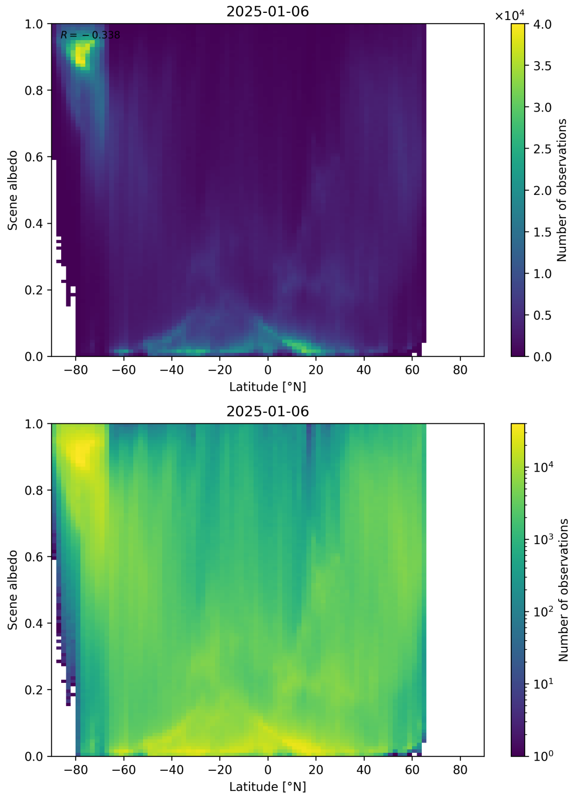
Figure 95: Scatter density plot of “Latitude” against “Scene albedo” for 2025-01-05 to 2025-01-07.
