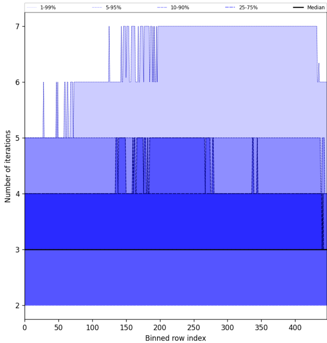
Figure 56: Along track statistics of “Number of iterations” for 2025-01-05 to 2025-01-07
