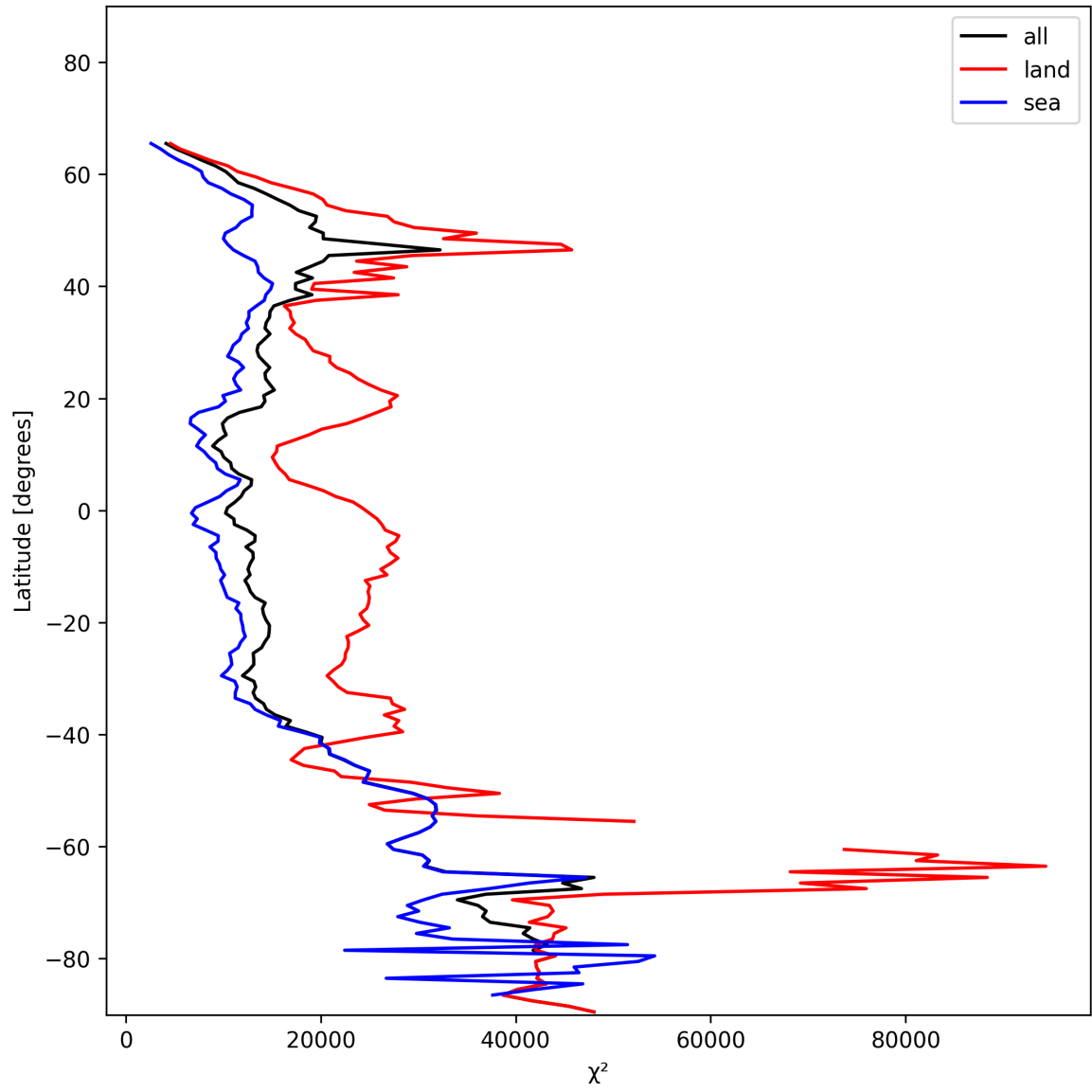
Figure 21: Zonal average of “ \chi^2 ” for 2025-01-05 to 2025-01-07.
