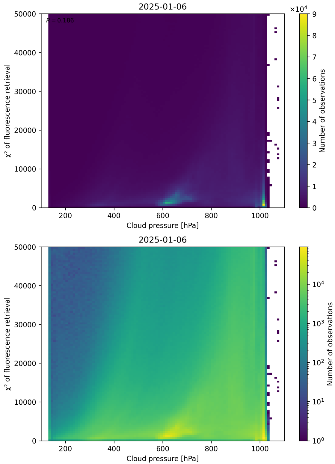
Figure 78: Scatter density plot of “Cloud pressure” against “ \chi^2 of fluorescence retrieval” for 2025-01-05 to 2025-01-07.
