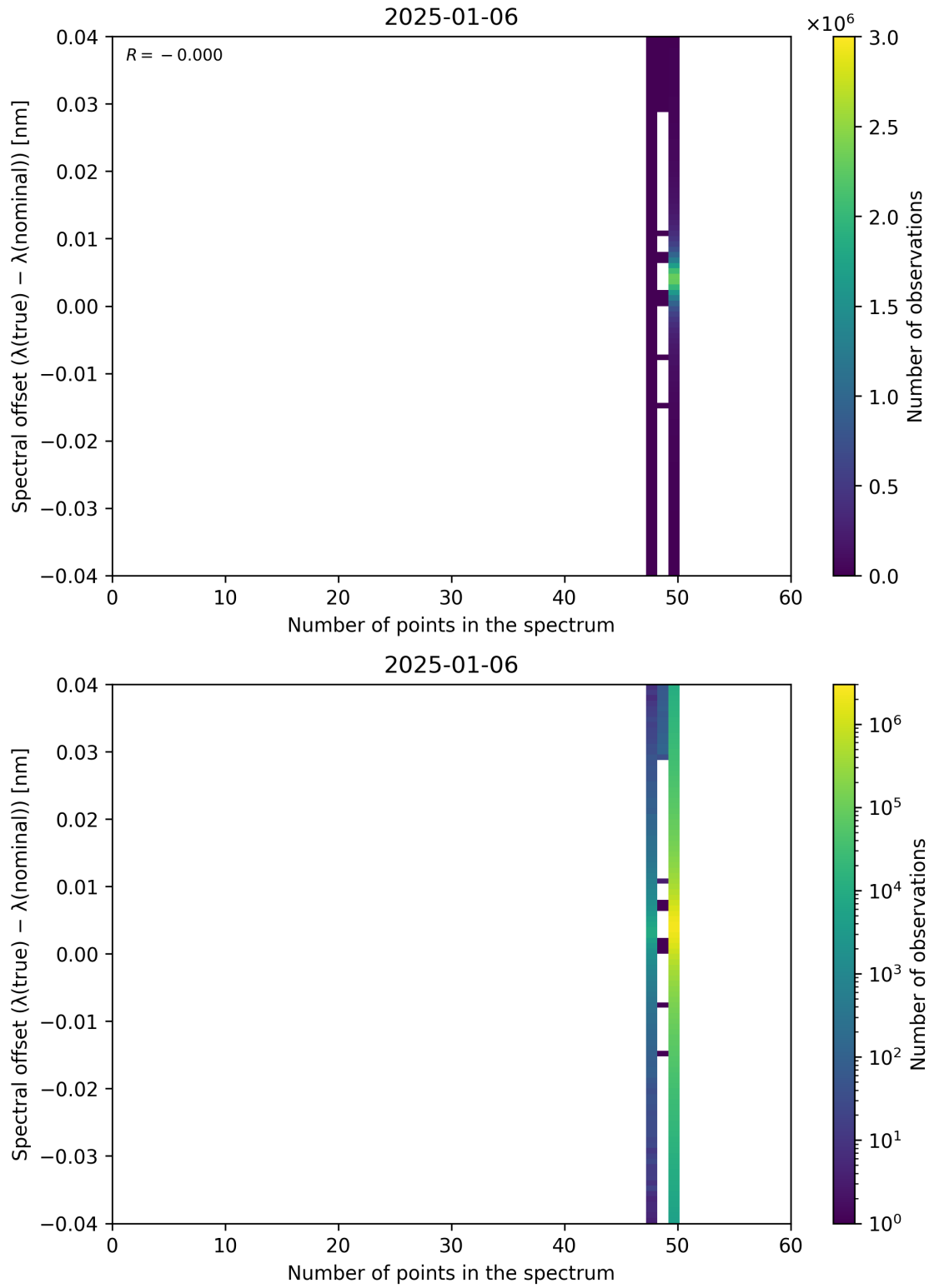
Figure 101: Scatter density plot of “Number of points in the spectrum” against “Spectral offset ( \lambda_{\text{true}} - \lambda_{\text{nominal}} )” for 2025-01-05 to 2025-01-07.
