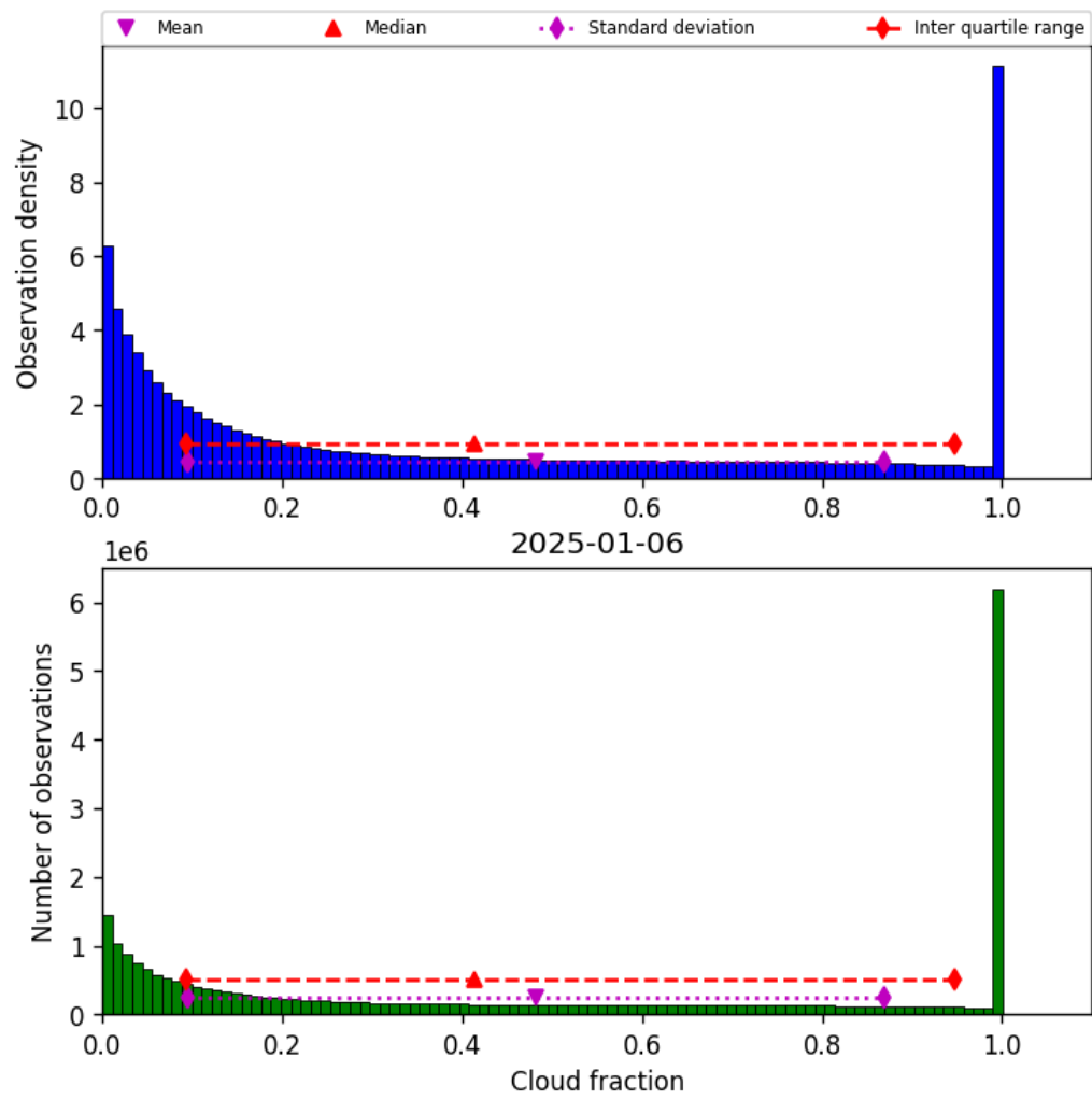
Figure 32: Histogram of “Cloud fraction” for 2025-01-05 to 2025-01-07
