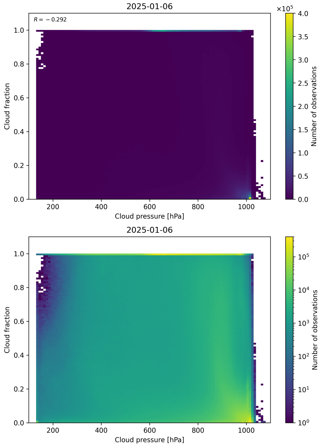
Figure 79: Scatter density plot of “Cloud pressure” against “Cloud fraction” for 2025-01-05 to 2025-01-07.
