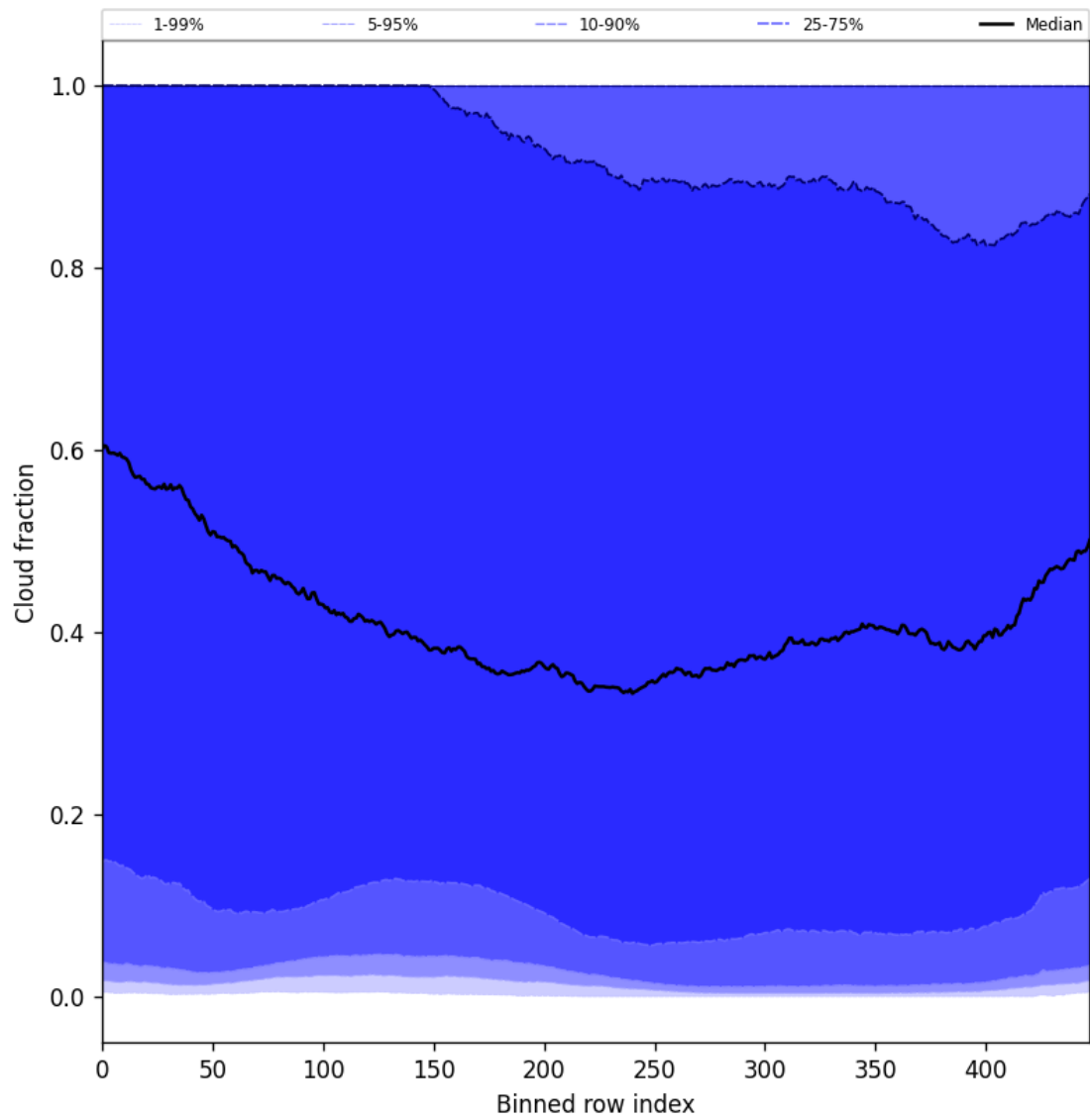
Figure 49: Along track statistics of “Cloud fraction” for 2025-01-05 to 2025-01-07
