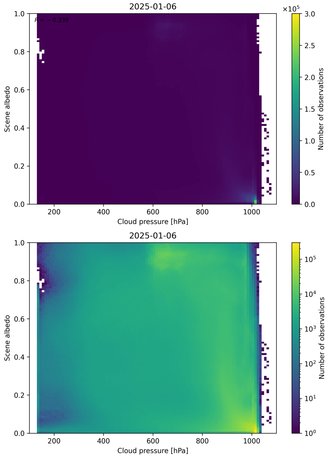
Figure 83: Scatter density plot of “Cloud pressure” against “Scene albedo” for 2025-01-05 to 2025-01-07.
