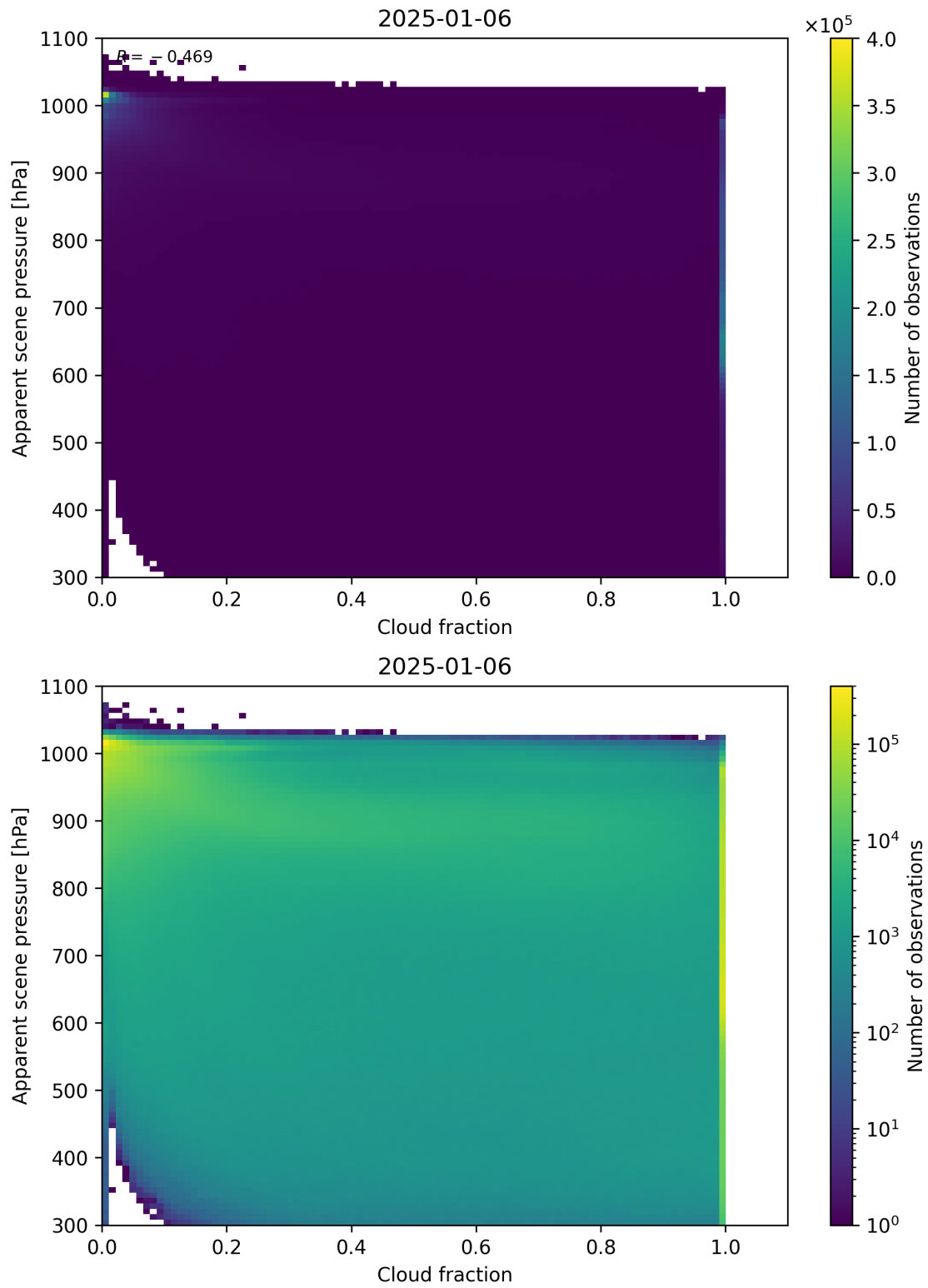
Figure 70: Scatter density plot of “Cloud fraction” against “Apparent scene pressure” for 2025-01-05 to 2025-01-07.
