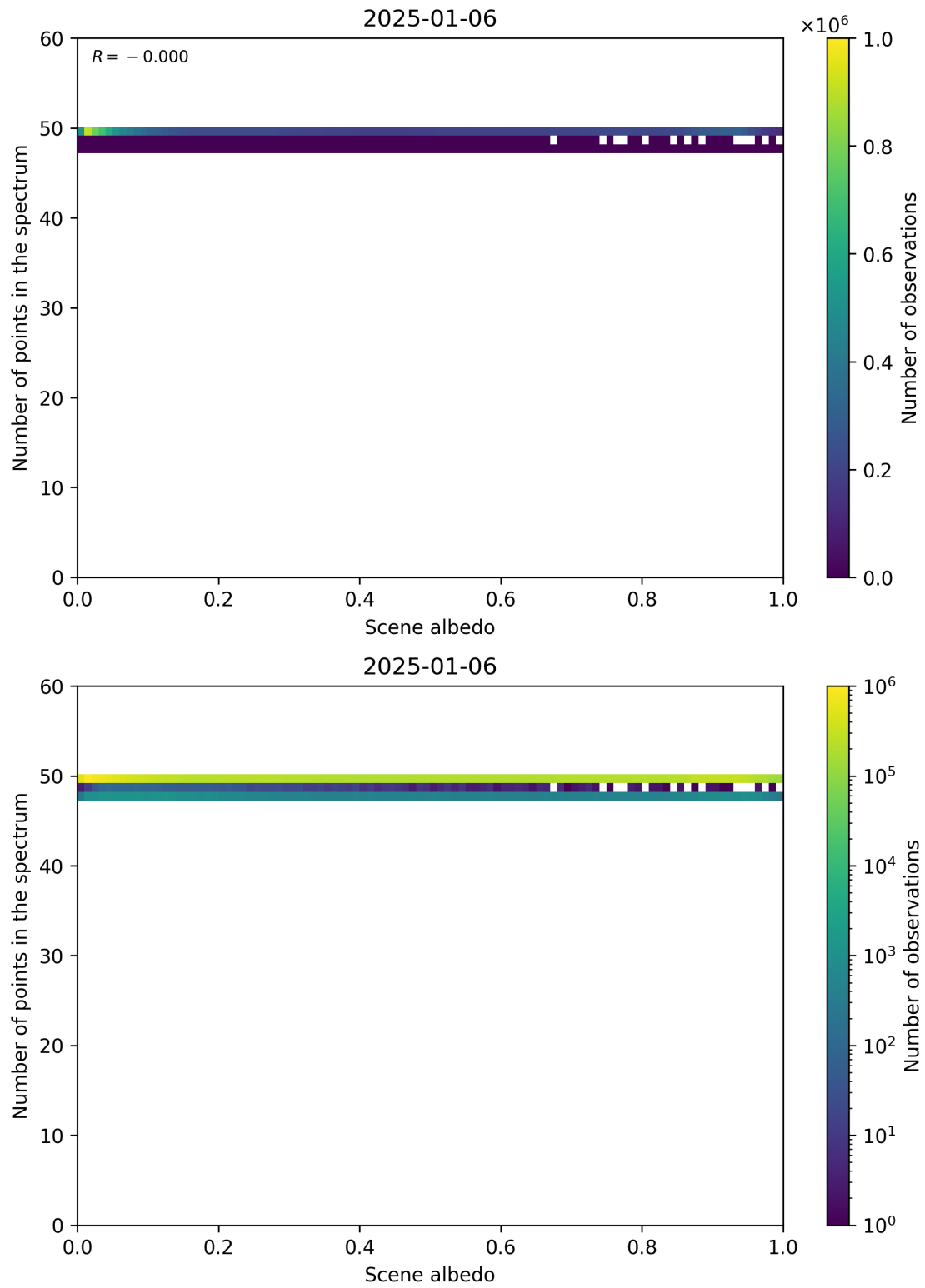
Figure 106: Scatter density plot of “Scene albedo” against “Number of points in the spectrum” for 2025-01-05 to 2025-01-07.
