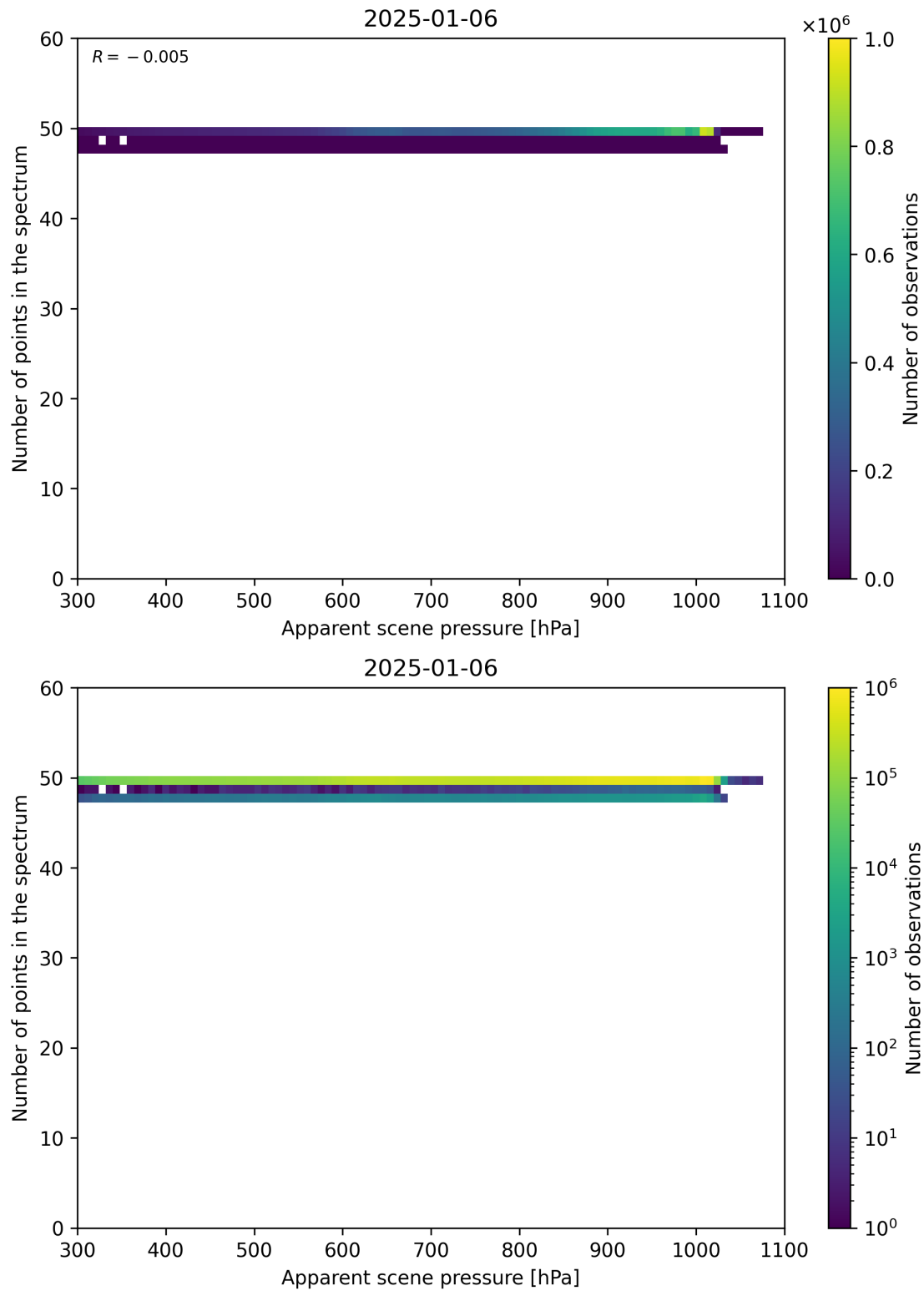
Figure 66: Scatter density plot of “Apparent scene pressure” against “Number of points in the spectrum” for 2025-01-05 to 2025-01-07.
