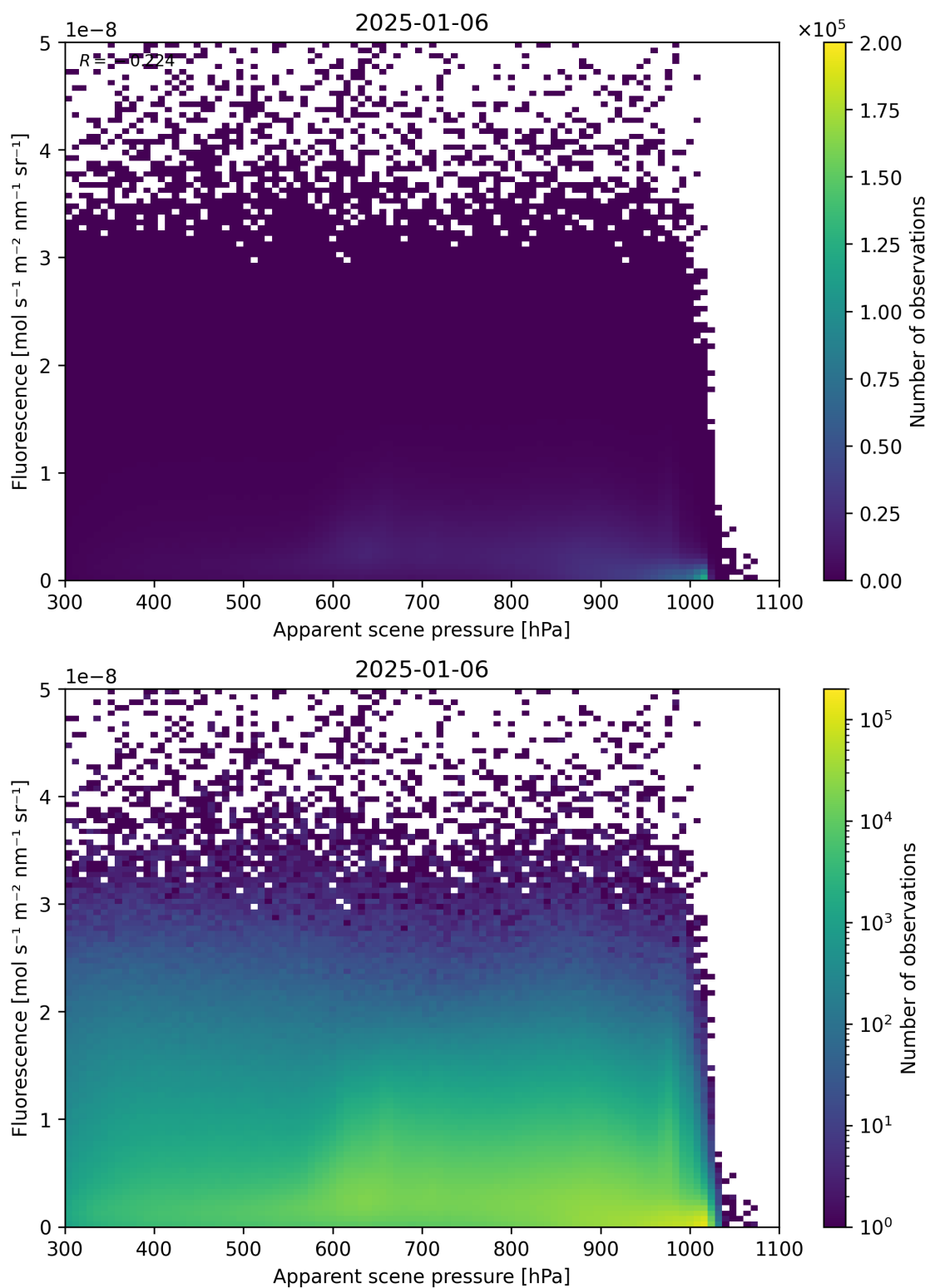
Figure 64: Scatter density plot of “Apparent scene pressure” against “Fluorescence” for 2025-01-05 to 2025-01-07.
