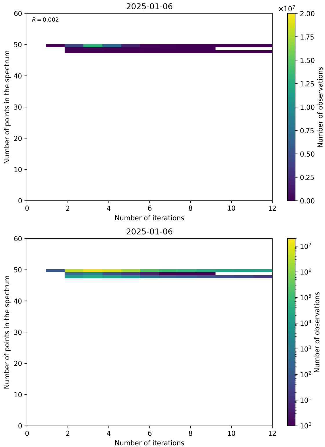
Figure 99: Scatter density plot of “Number of iterations” against “Number of points in the spectrum” for 2025-01-05 to 2025-01-07.
