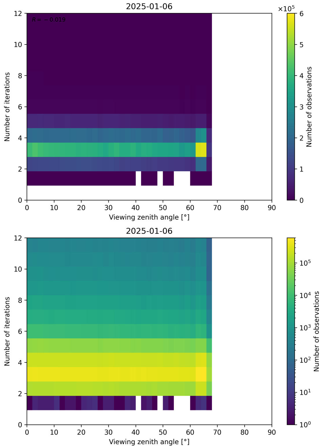
Figure 124: Scatter density plot of “Viewing zenith angle” against “Number of iterations” for 2025-01-05 to 2025-01-07.
