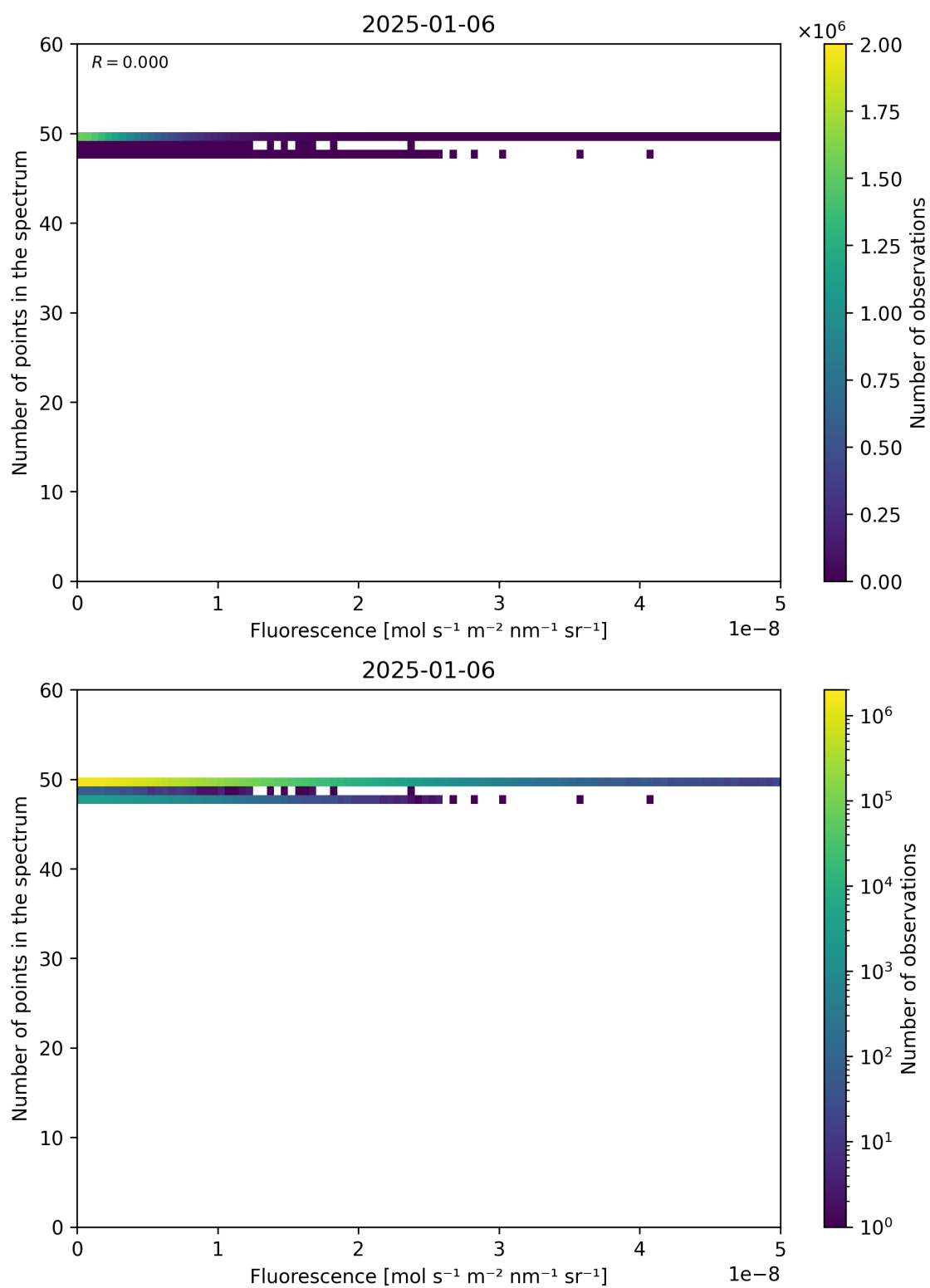
Figure 86: Scatter density plot of “Fluorescence” against “Number of points in the spectrum” for 2025-01-05 to 2025-01-07.
