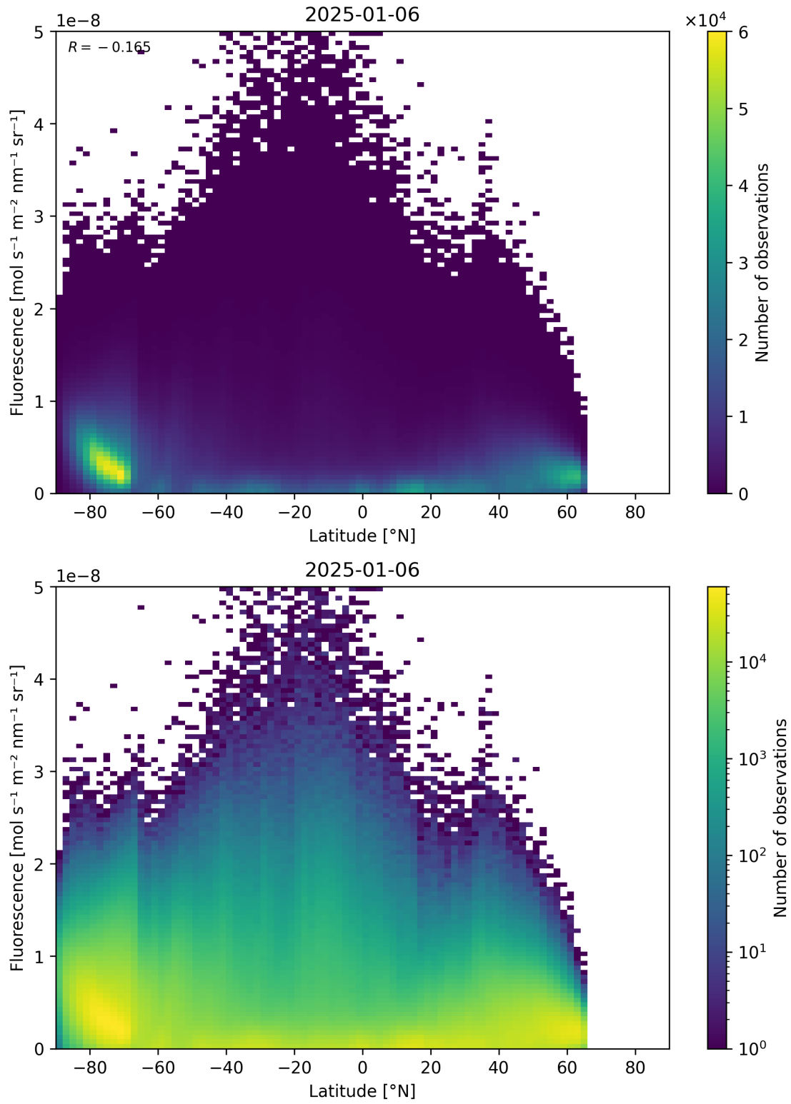
Figure 92: Scatter density plot of “Latitude” against “Fluorescence” for 2025-01-05 to 2025-01-07.
