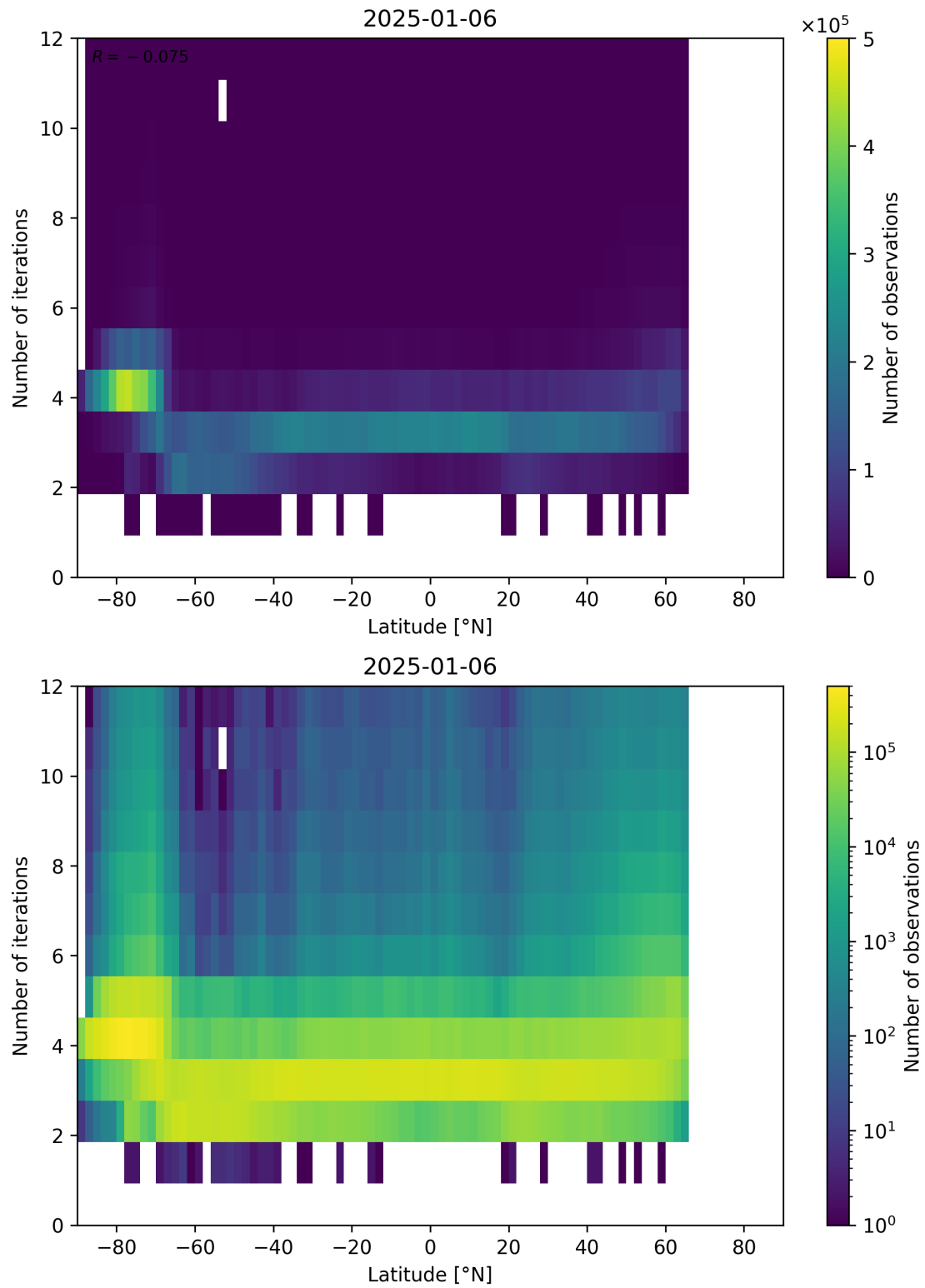
Figure 93: Scatter density plot of “Latitude” against “Number of iterations” for 2025-01-05 to 2025-01-07.
