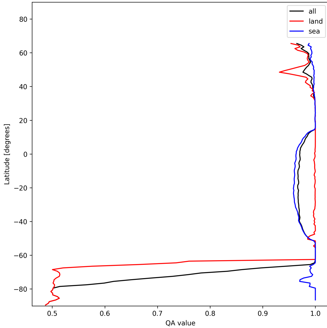
Figure 12: Zonal average of “QA value” for 2025-01-05 to 2025-01-07.
