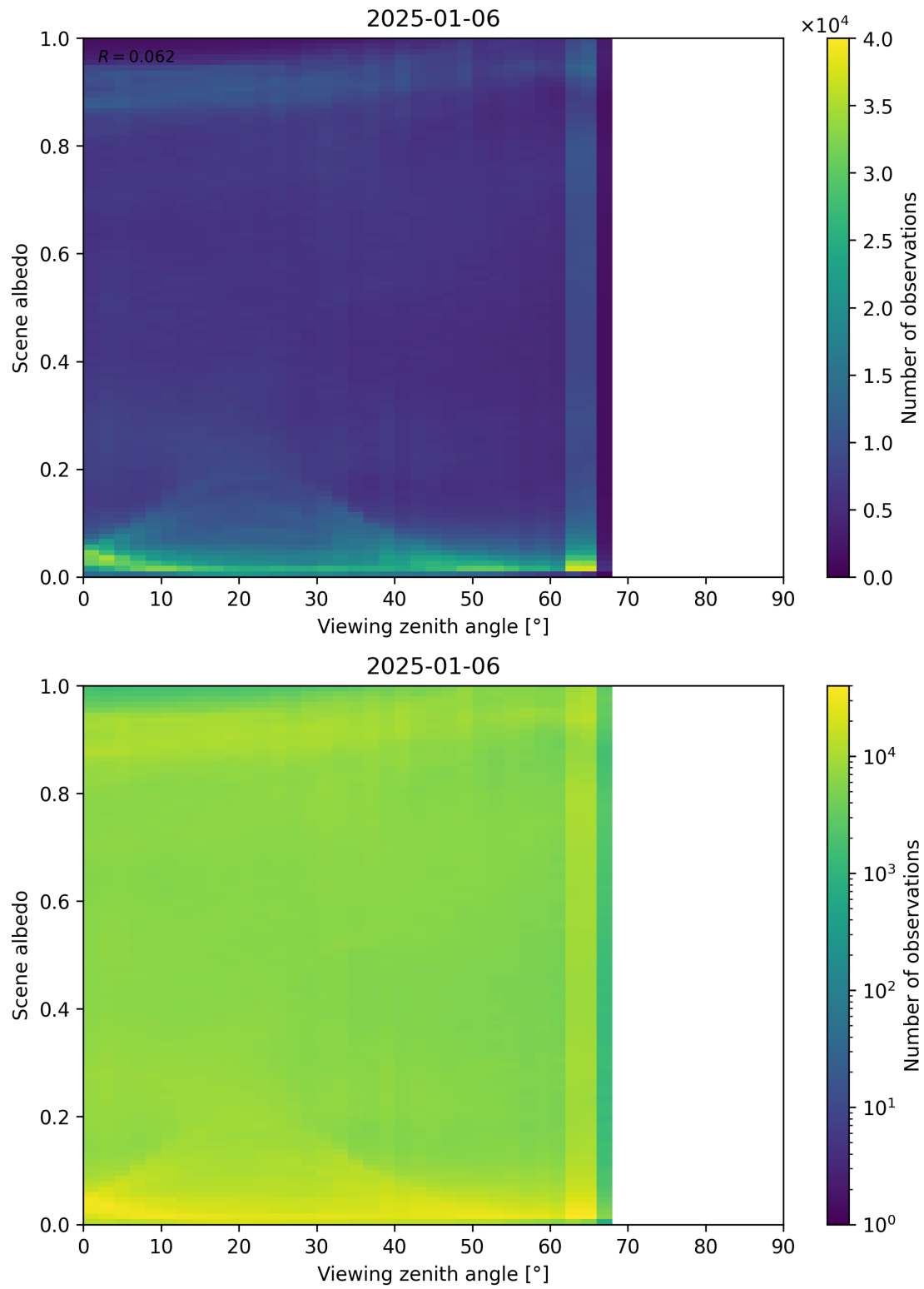
Figure 126: Scatter density plot of “Viewing zenith angle” against “Scene albedo” for 2025-01-05 to 2025-01-07.
