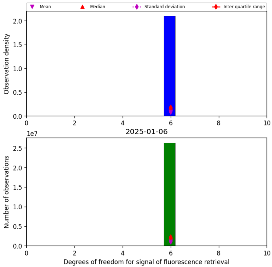
Figure 43: Histogram of “Degrees of freedom for signal of fluorescence retrieval” for 2025-01-05 to 2025-01-07
