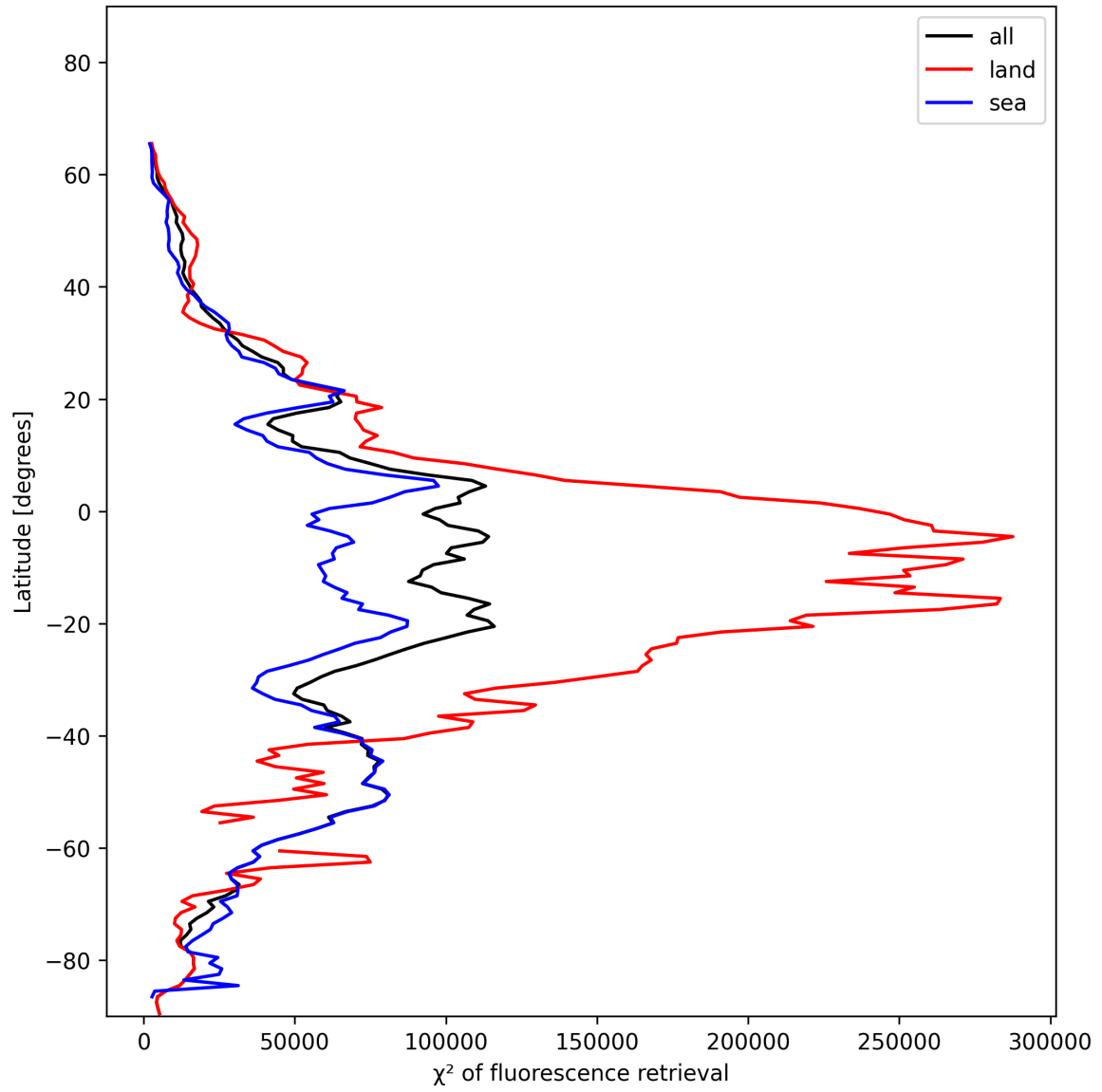
Figure 25: Zonal average of “ \chi^2 of fluorescence retrieval” for 2025-01-05 to 2025-01-07.
