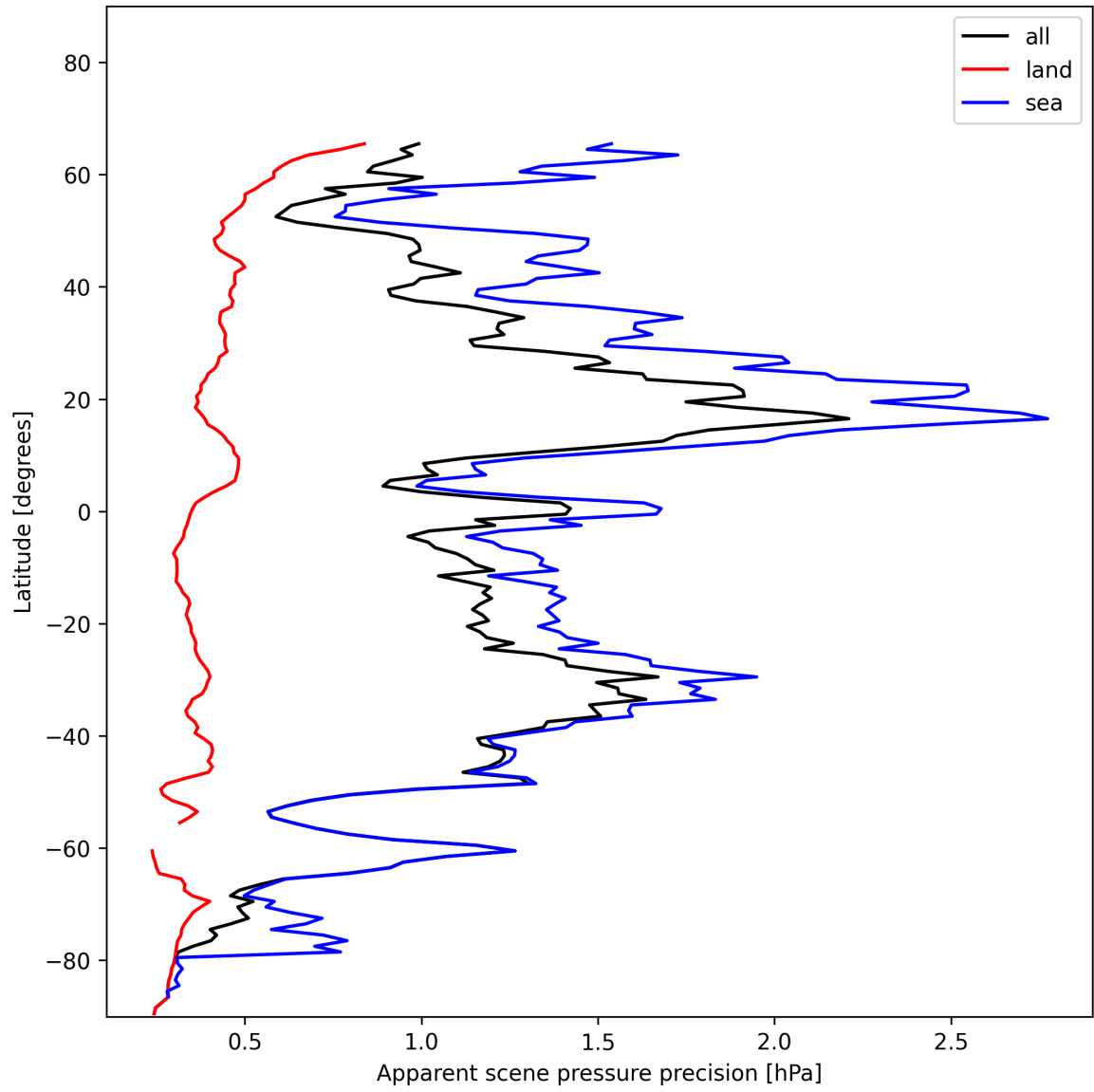
Figure 20: Zonal average of “Apparent scene pressure precision” for 2025-01-05 to 2025-01-07.
