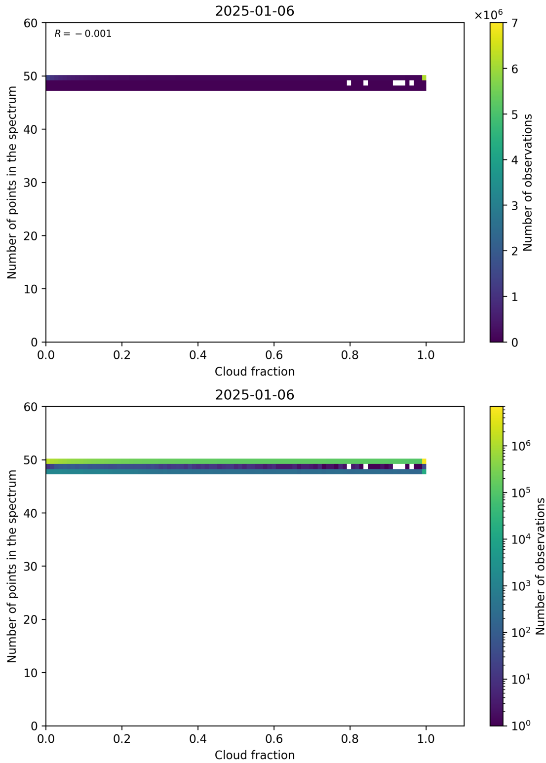
Figure 74: Scatter density plot of “Cloud fraction” against “Number of points in the spectrum” for 2025-01-05 to 2025-01-07.
