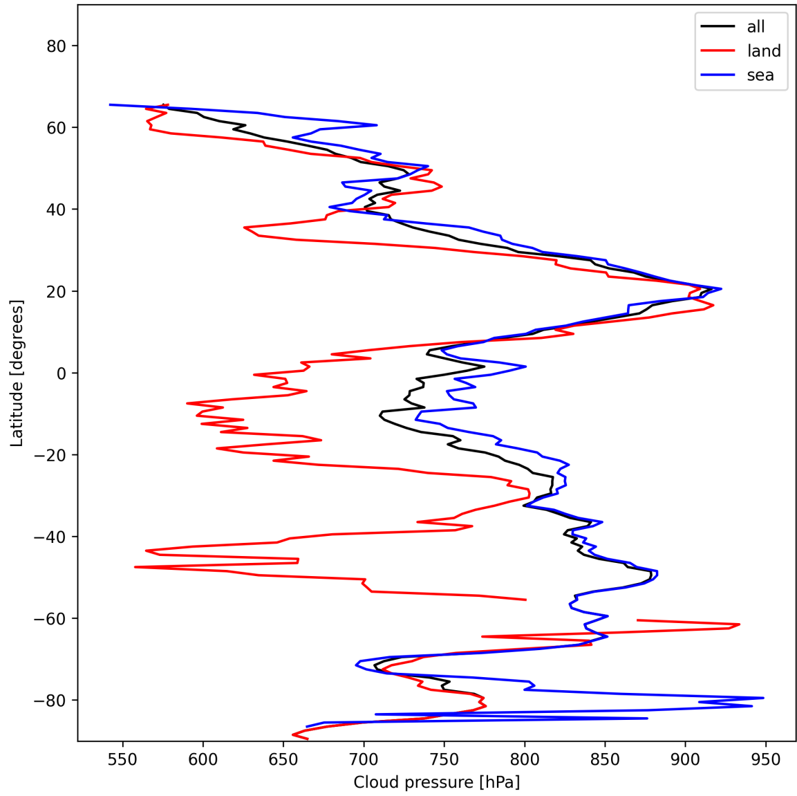
Figure 13: Zonal average of “Cloud pressure” for 2025-01-05 to 2025-01-07.
