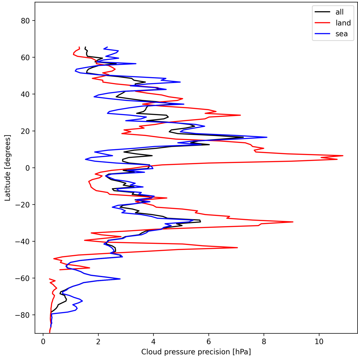
Figure 14: Zonal average of “Cloud pressure precision” for 2025-01-05 to 2025-01-07.
