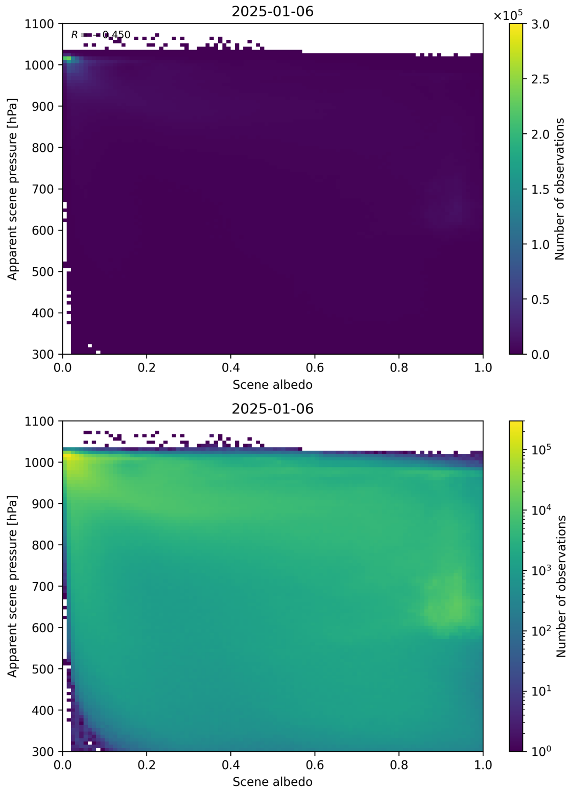
Figure 102: Scatter density plot of “Scene albedo” against “Apparent scene pressure” for 2025-01-05 to 2025-01-07.
