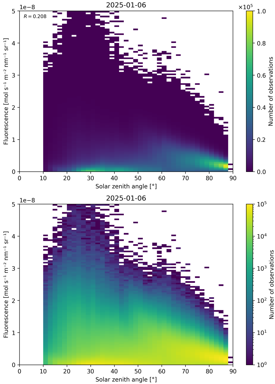
Figure 112: Scatter density plot of “Solar zenith angle” against “Fluorescence” for 2025-01-05 to 2025-01-07.
