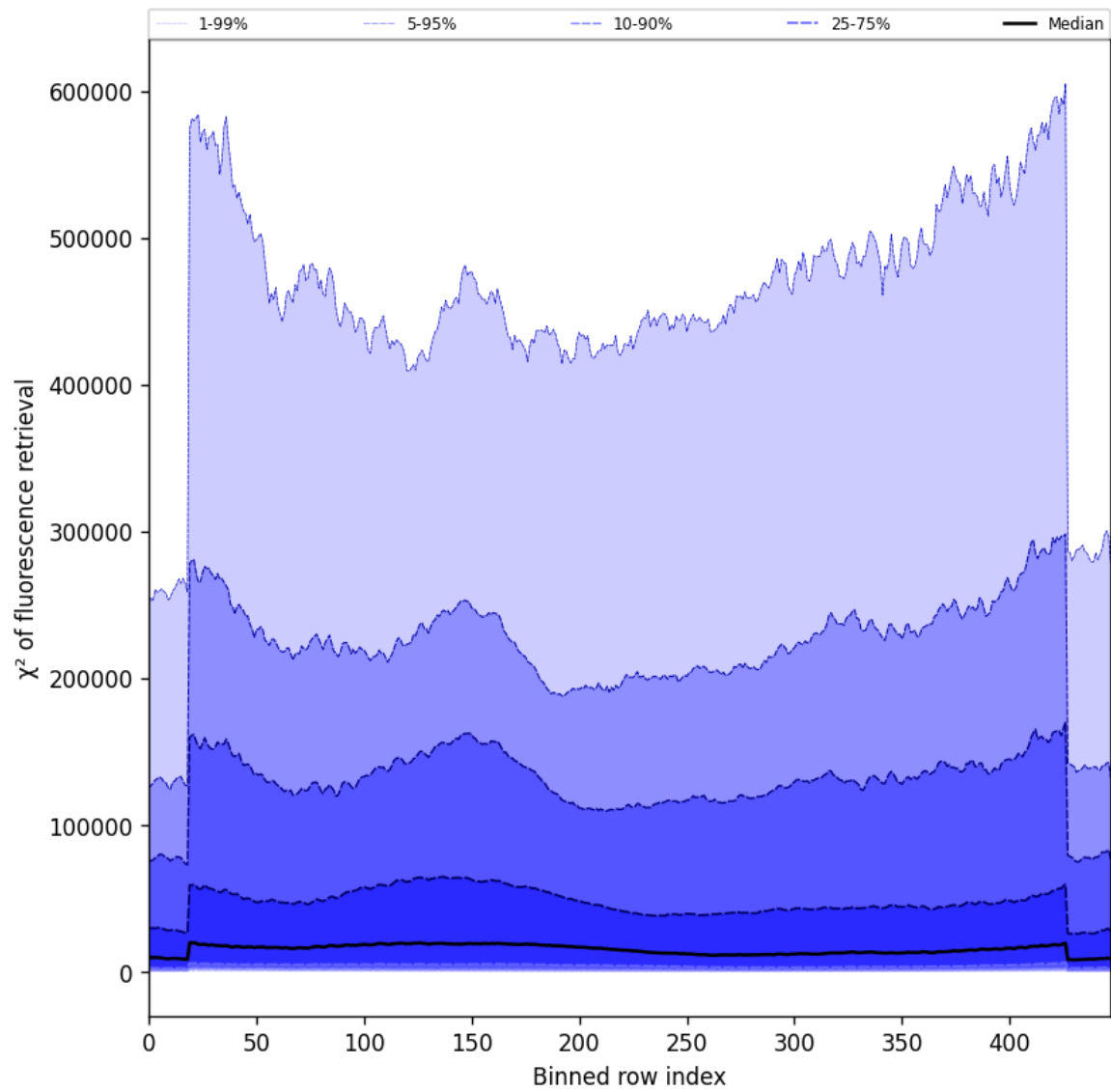
Figure 59: Along track statistics of “ \chi^2 of fluorescence retrieval” for 2025-01-05 to 2025-01-07
