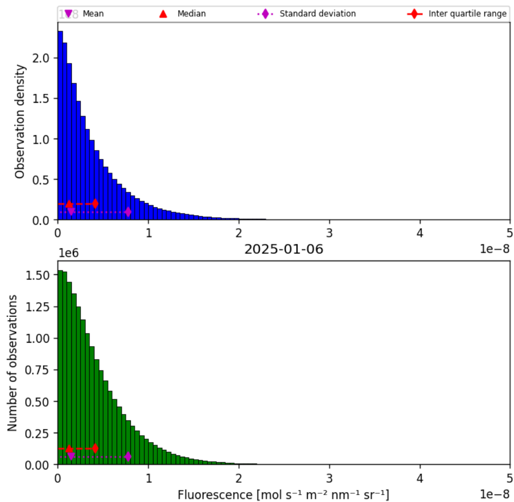
Figure 40: Histogram of “Fluorescence” for 2025-01-05 to 2025-01-07
