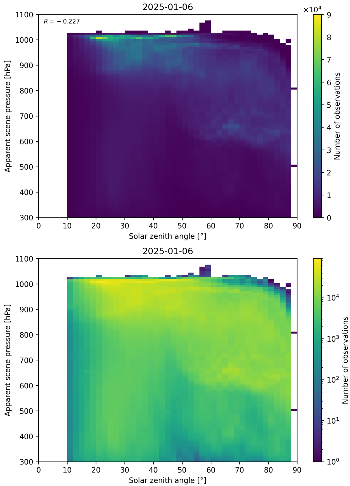
Figure 108: Scatter density plot of “Solar zenith angle” against “Apparent scene pressure” for 2025-01-05 to 2025-01-07.
