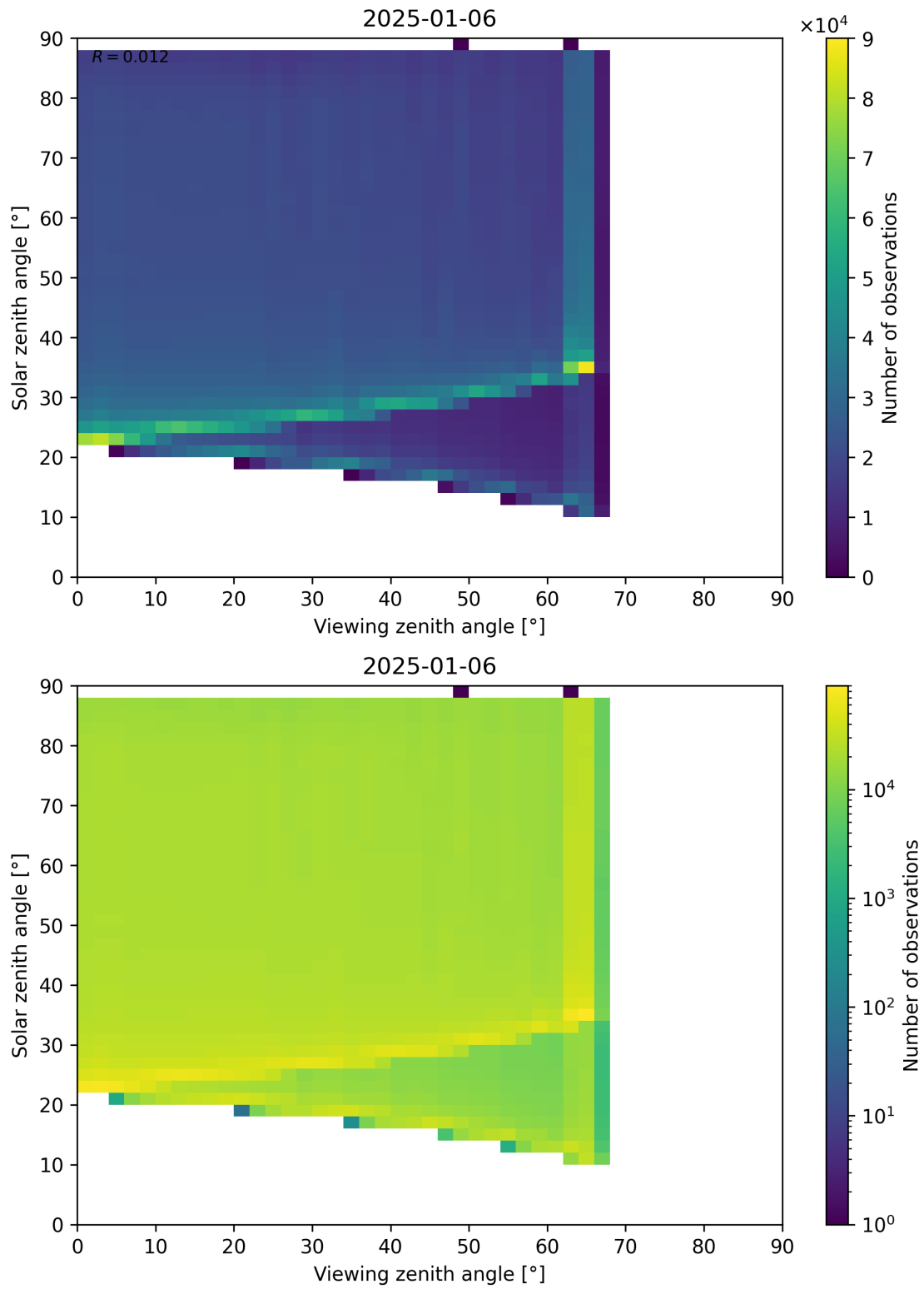
Figure 127: Scatter density plot of “Viewing zenith angle” against “Solar zenith angle” for 2025-01-05 to 2025-01-07.
