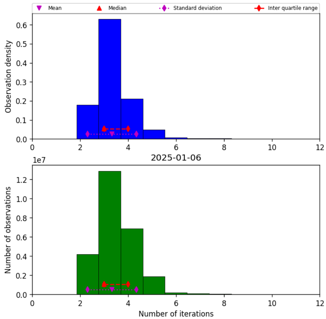
Figure 39: Histogram of “Number of iterations” for 2025-01-05 to 2025-01-07
