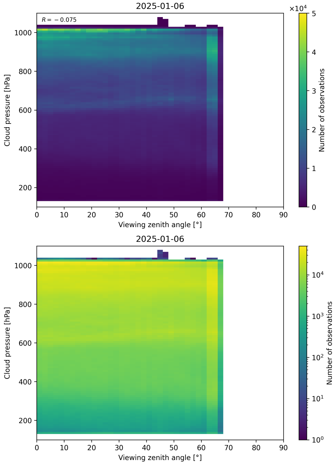
Figure 121: Scatter density plot of “Viewing zenith angle” against “Cloud pressure” for 2025-01-05 to 2025-01-07.
