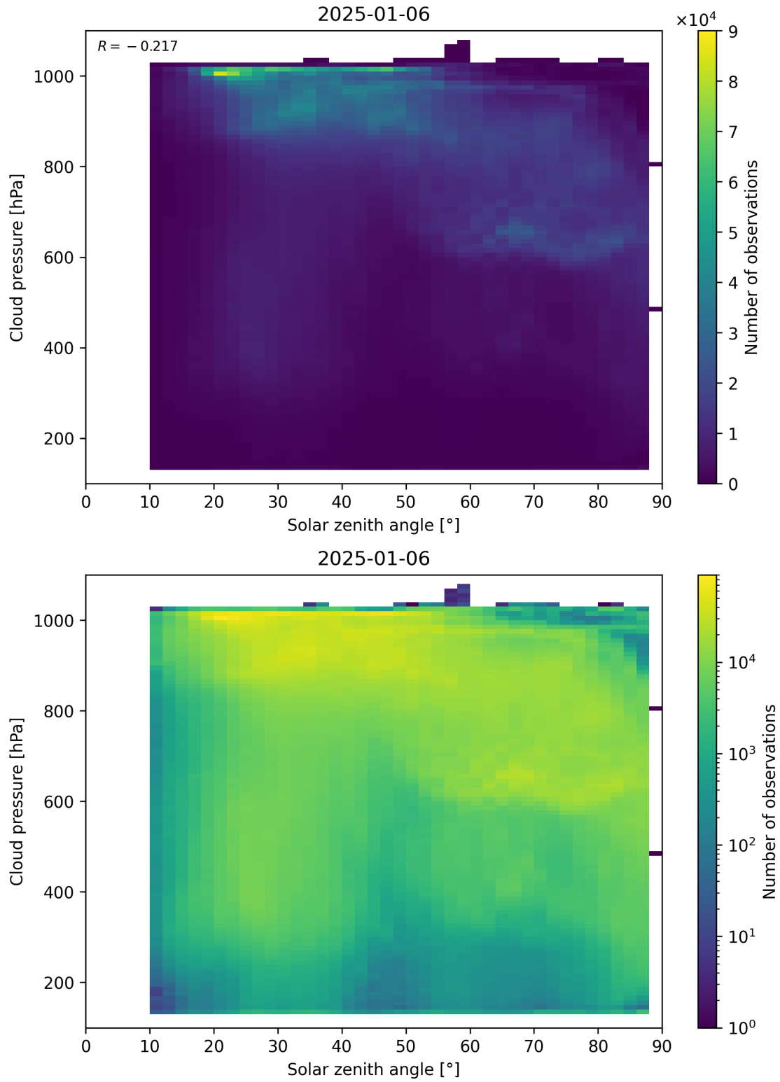
Figure 111: Scatter density plot of “Solar zenith angle” against “Cloud pressure” for 2025-01-05 to 2025-01-07.
