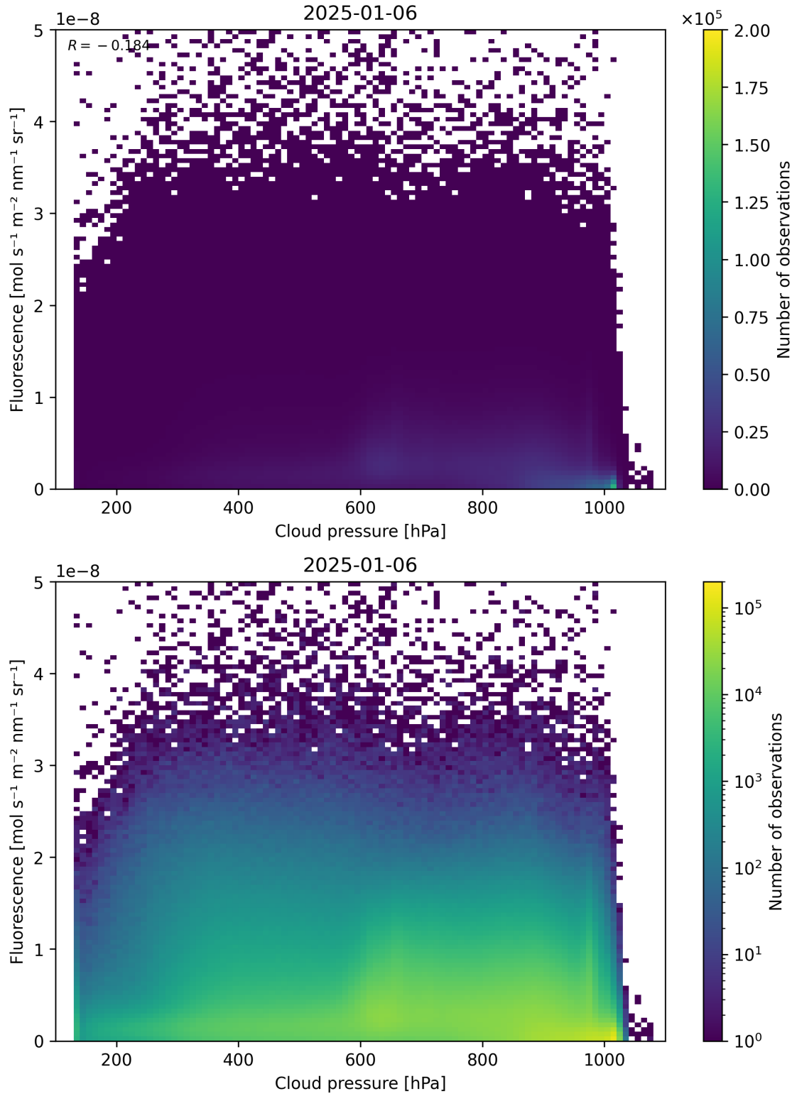
Figure 80: Scatter density plot of “Cloud pressure” against “Fluorescence” for 2025-01-05 to 2025-01-07.
