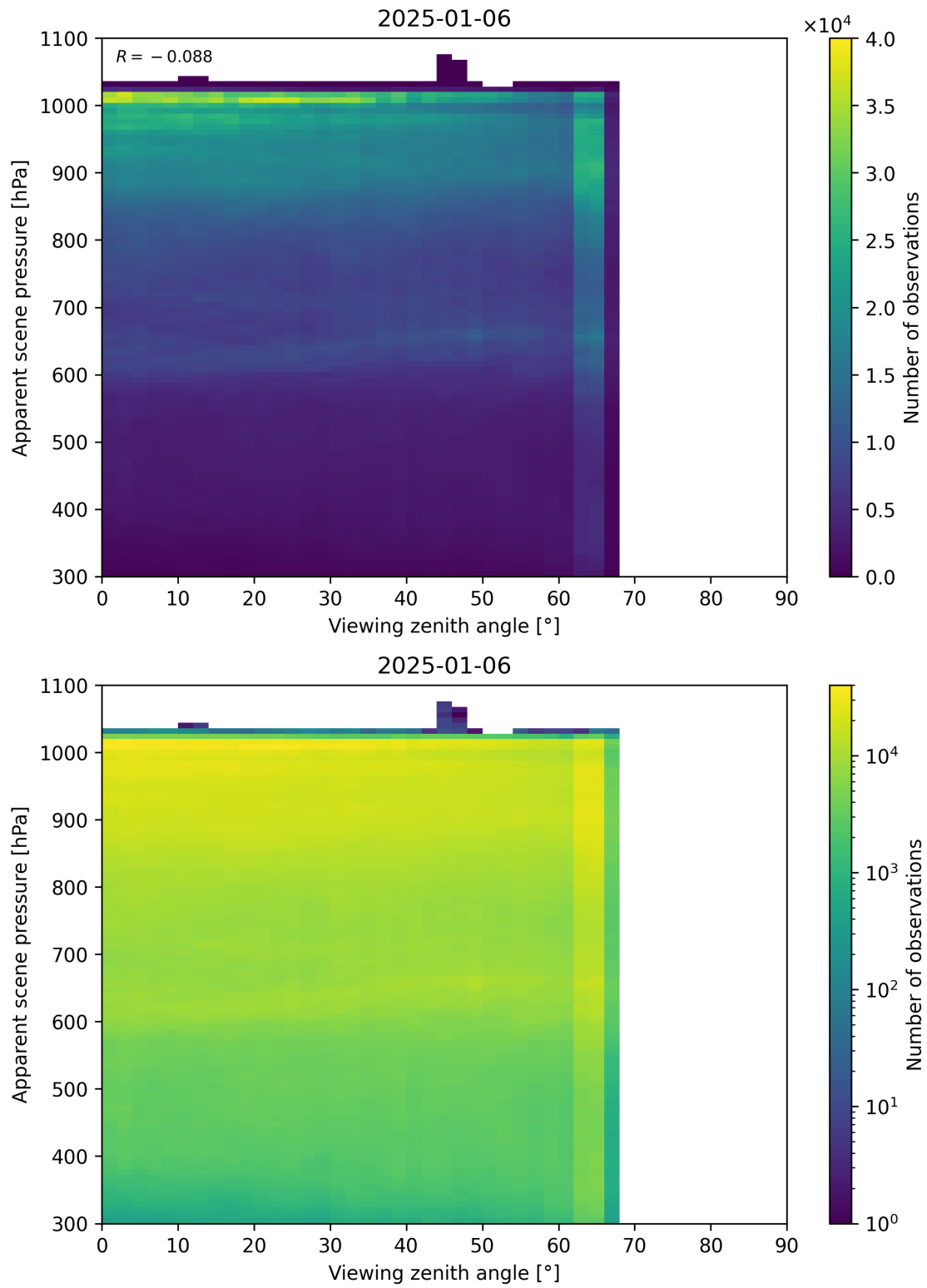
Figure 118: Scatter density plot of “Viewing zenith angle” against “Apparent scene pressure” for 2025-01-05 to 2025-01-07.
