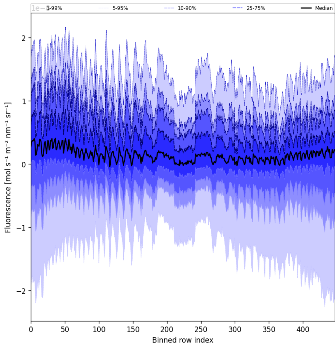
Figure 57: Along track statistics of “Fluorescence” for 2025-01-05 to 2025-01-07
