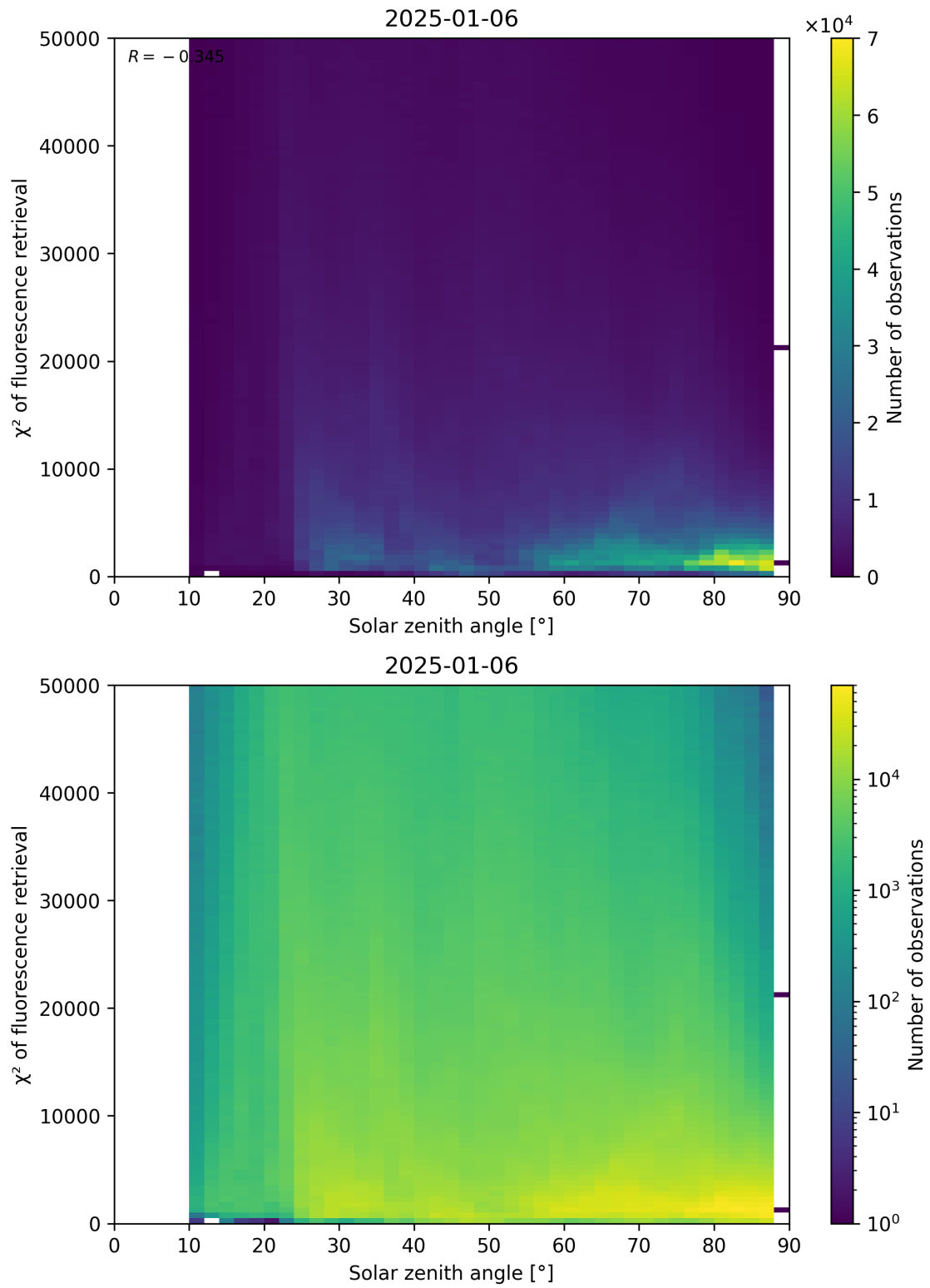
Figure 109: Scatter density plot of “Solar zenith angle” against “ \chi^2 of fluorescence retrieval” for 2025-01-05 to 2025-01-07.
