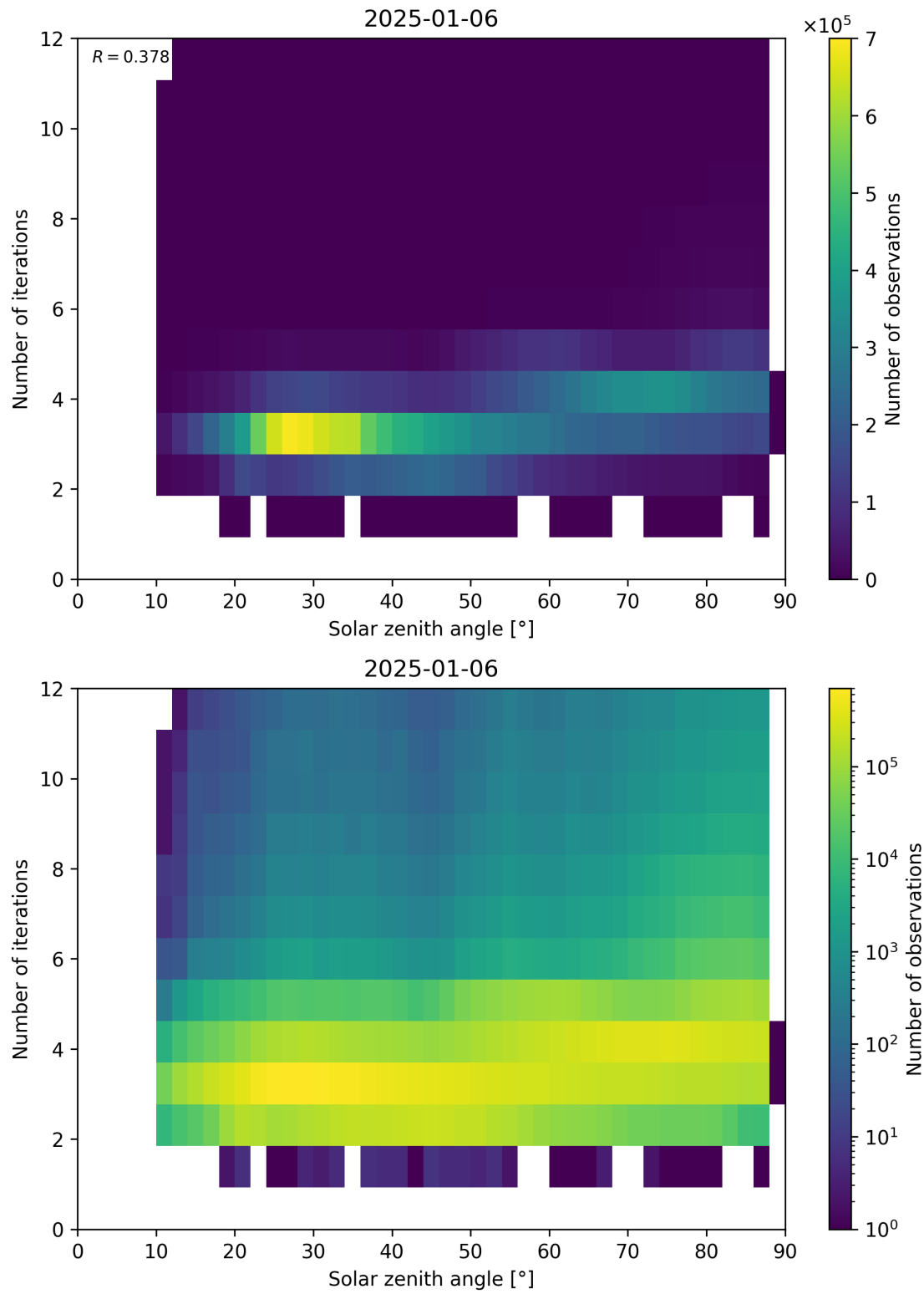
Figure 114: Scatter density plot of “Solar zenith angle” against “Number of iterations” for 2025-01-05 to 2025-01-07.
