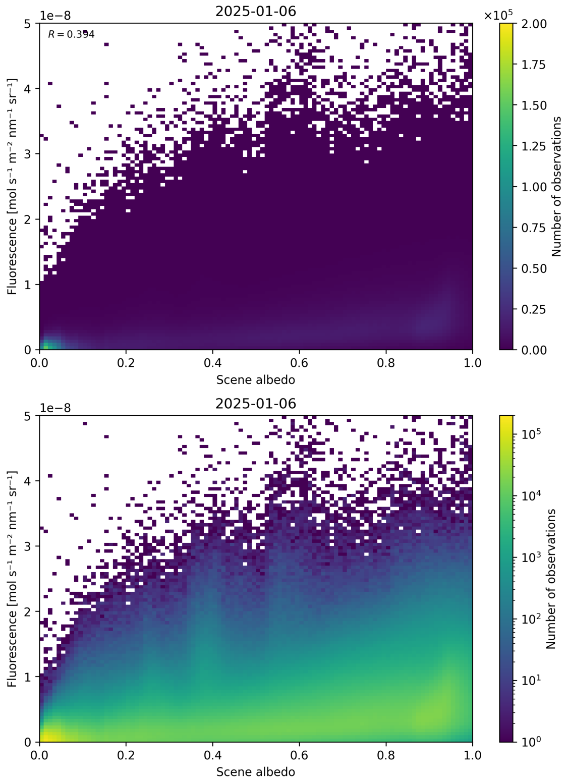
Figure 104: Scatter density plot of “Scene albedo” against “Fluorescence” for 2025-01-05 to 2025-01-07.
