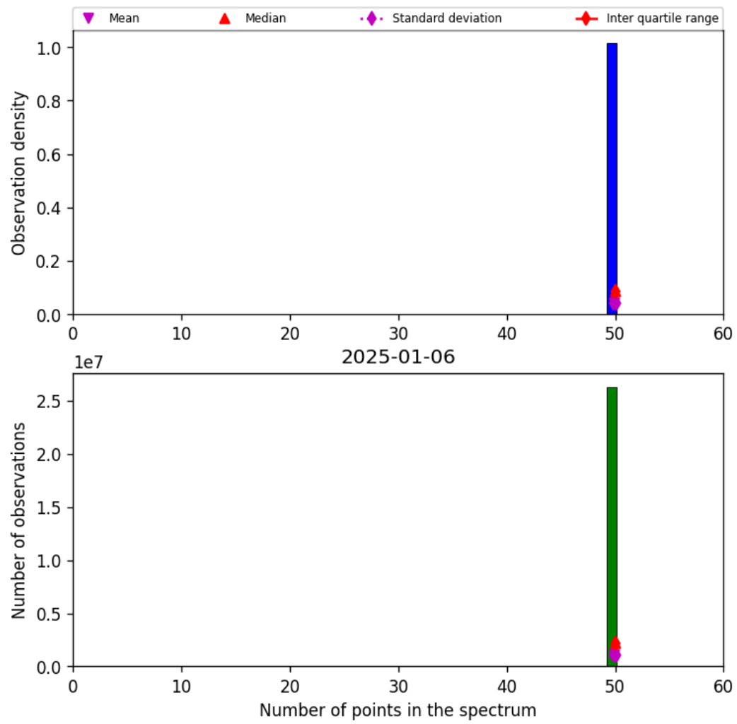
Figure 44: Histogram of “Number of points in the spectrum” for 2025-01-05 to 2025-01-07
