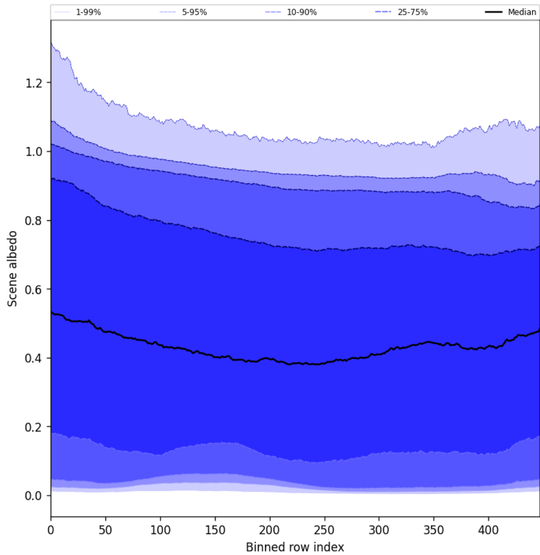
Figure 51: Along track statistics of “Scene albedo” for 2025-01-05 to 2025-01-07
