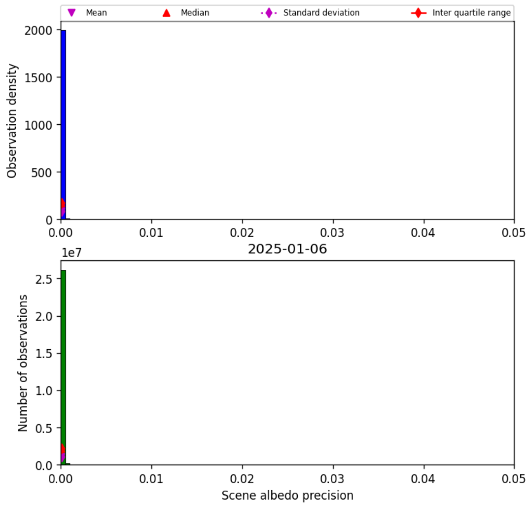
Figure 35: Histogram of “Scene albedo precision” for 2025-01-05 to 2025-01-07
