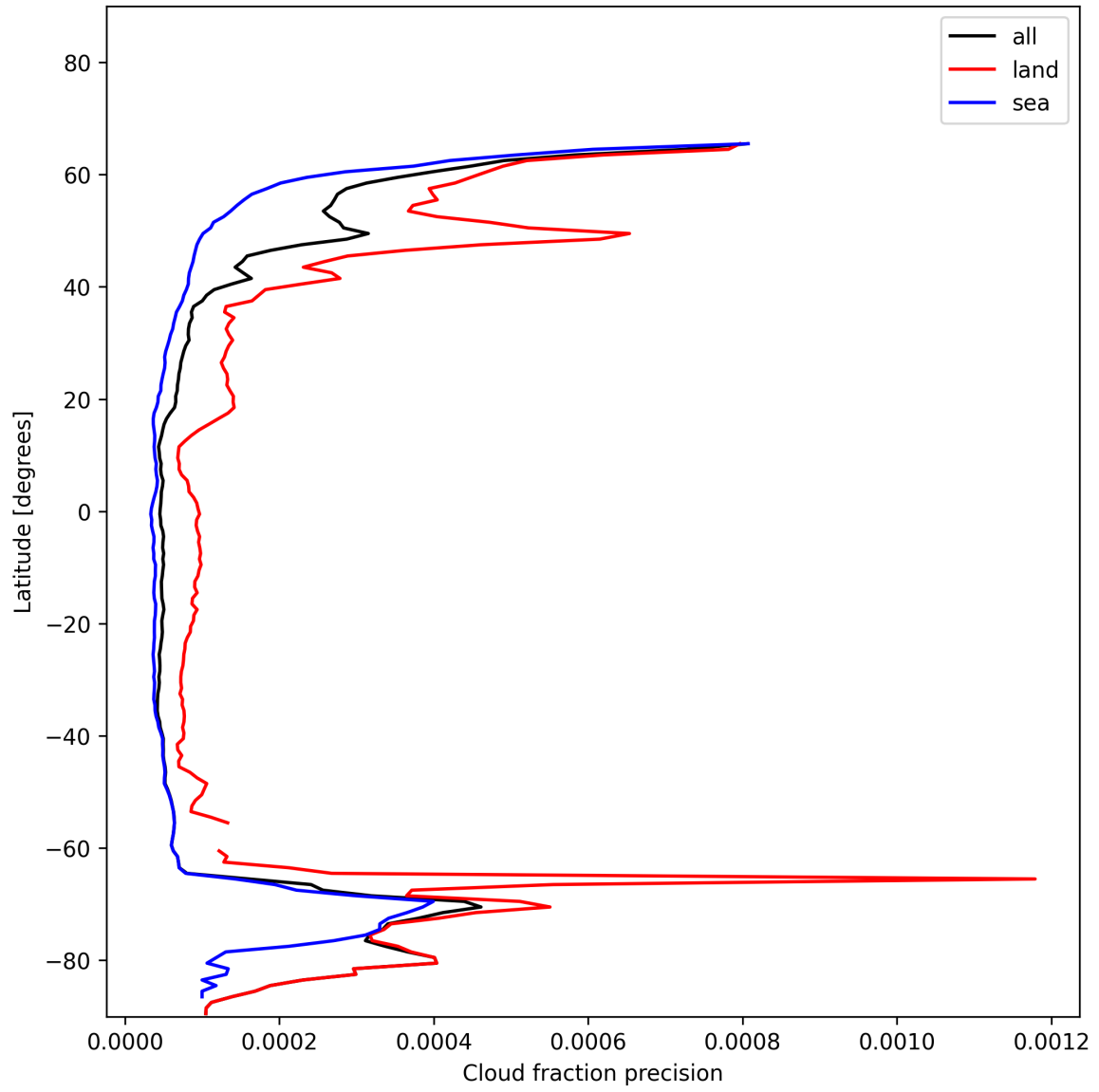
Figure 16: Zonal average of “Cloud fraction precision” for 2025-01-05 to 2025-01-07.
