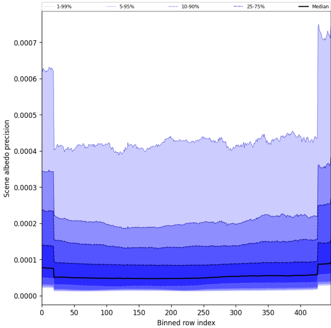
Figure 52: Along track statistics of “Scene albedo precision” for 2025-01-05 to 2025-01-07
