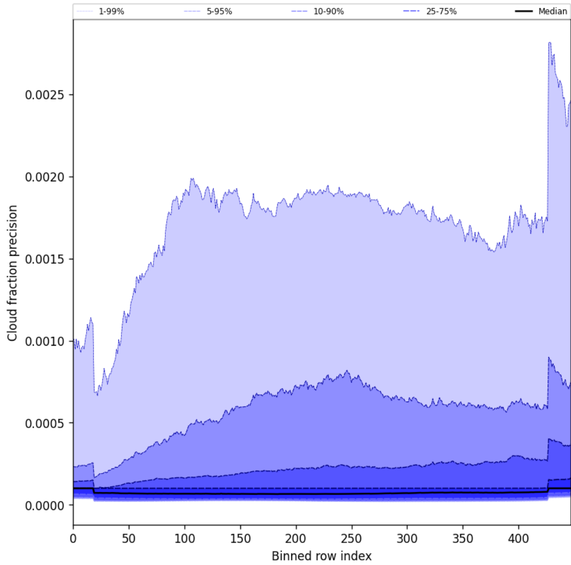
Figure 50: Along track statistics of “Cloud fraction precision” for 2025-01-05 to 2025-01-07
