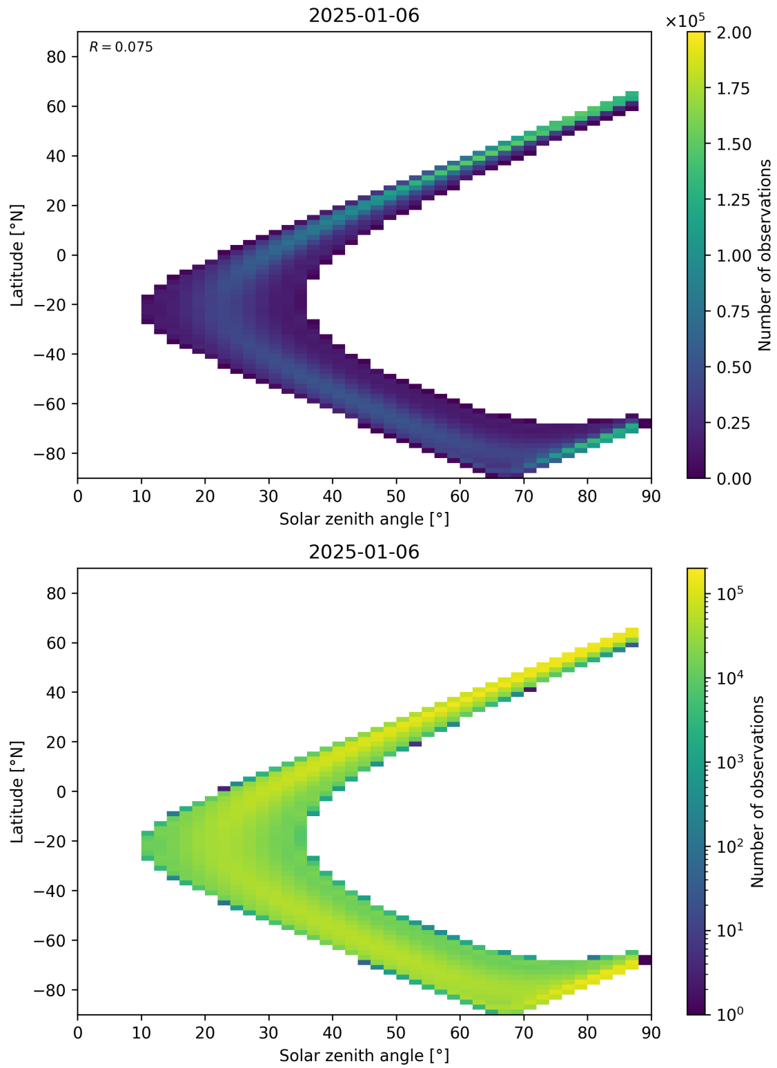
Figure 113: Scatter density plot of “Solar zenith angle” against “Latitude” for 2025-01-05 to 2025-01-07.
