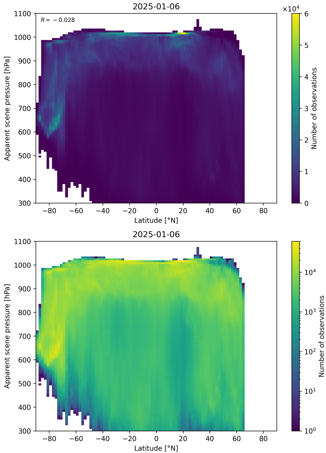
Figure 88: Scatter density plot of “Latitude” against “Apparent scene pressure” for 2025-01-05 to 2025-01-07.
