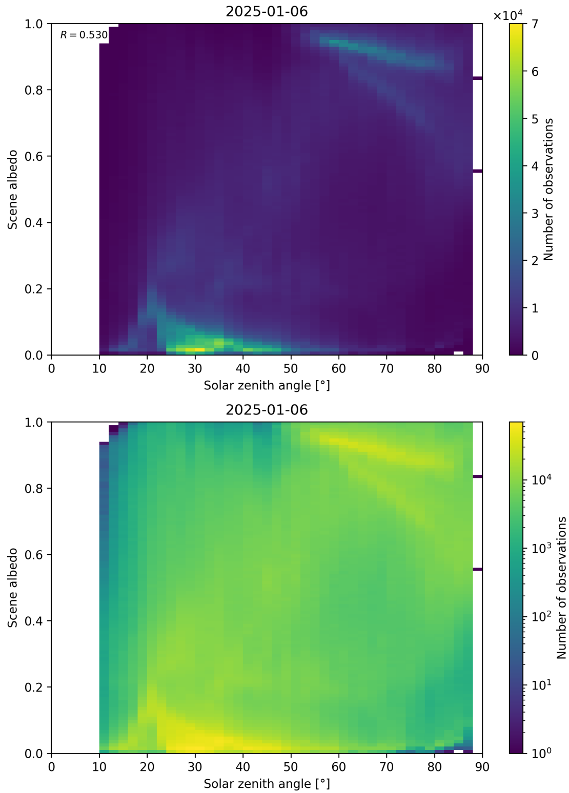
Figure 116: Scatter density plot of “Solar zenith angle” against “Scene albedo” for 2025-01-05 to 2025-01-07.
