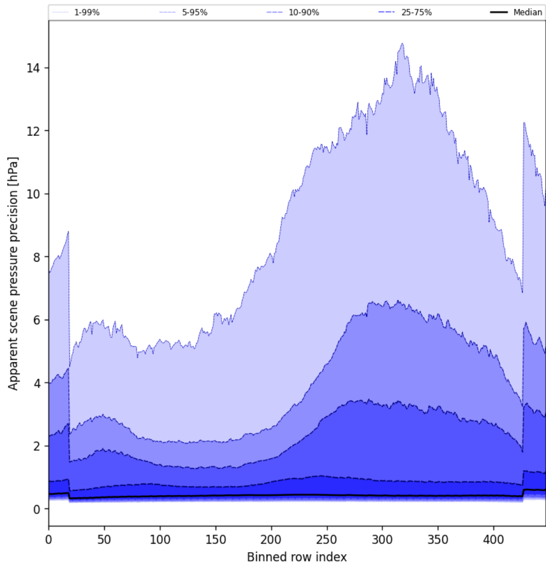
Figure 54: Along track statistics of “Apparent scene pressure precision” for 2025-01-05 to 2025-01-07
