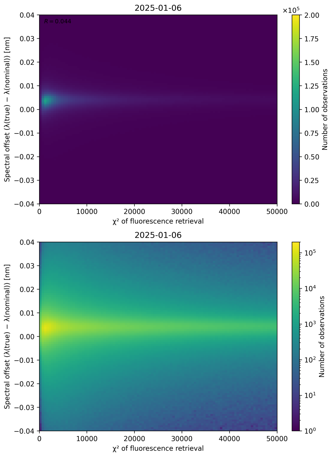
Figure 69: Scatter density plot of “ \chi^2 of fluorescence retrieval” against “Spectral offset ( \lambda_{\text{true}} - \lambda_{\text{nominal}} )” for 2025-01-05 to 2025-01-07.
