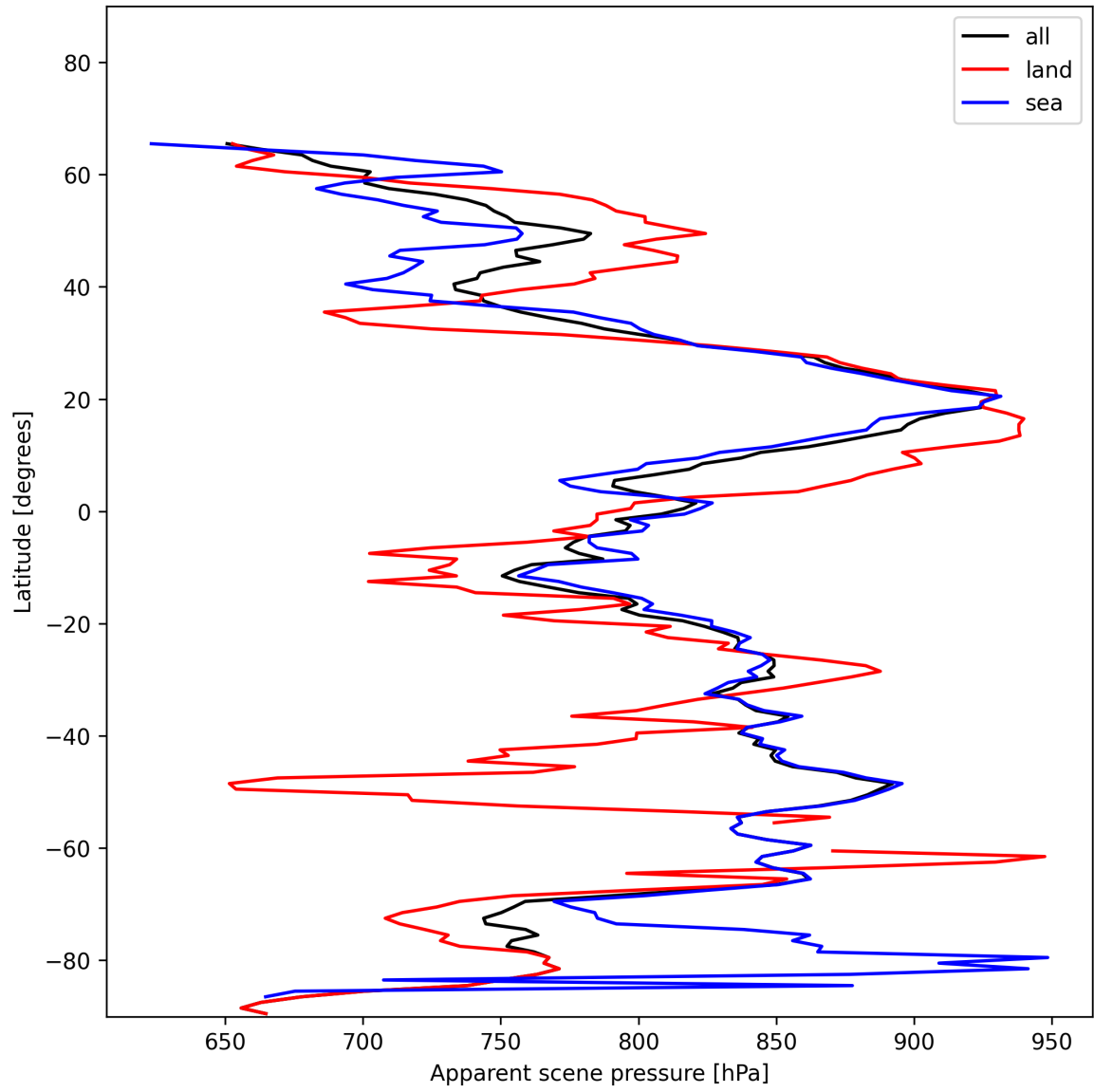
Figure 19: Zonal average of “Apparent scene pressure” for 2025-01-05 to 2025-01-07.
