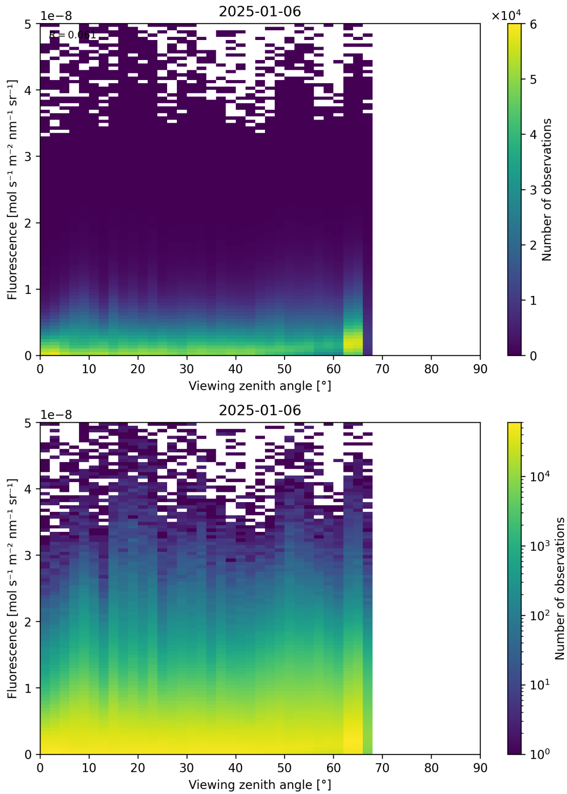
Figure 122: Scatter density plot of “Viewing zenith angle” against “Fluorescence” for 2025-01-05 to 2025-01-07.
