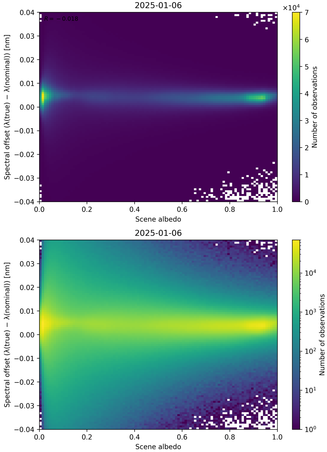
Figure 107: Scatter density plot of “Scene albedo” against “Spectral offset ( \lambda_{\text{true}} - \lambda_{\text{nominal}} )” for 2025-01-05 to 2025-01-07.
