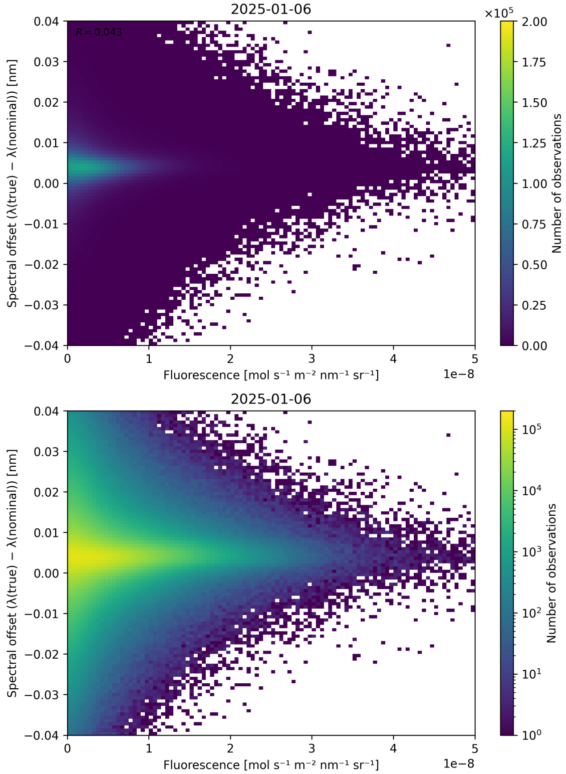
Figure 87: Scatter density plot of “Fluorescence” against “Spectral offset ( \lambda_{\text{true}} - \lambda_{\text{nominal}} )” for 2025-01-05 to 2025-01-07.
