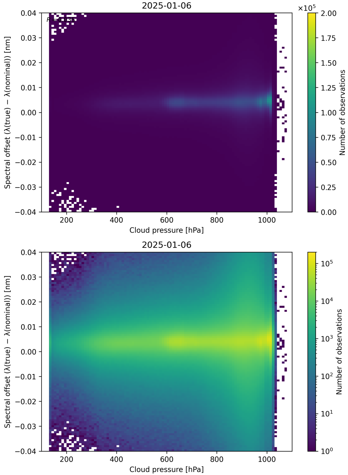
Figure 84: Scatter density plot of “Cloud pressure” against “Spectral offset ( \lambda_{\text{true}} - \lambda_{\text{nominal}} )” for 2025-01-05 to 2025-01-07.
