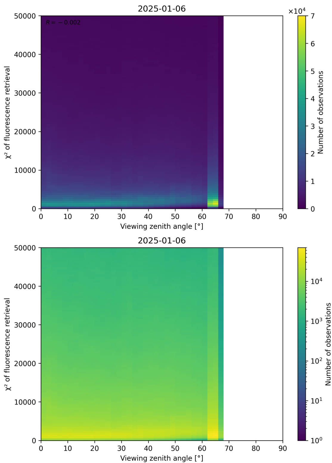
Figure 119: Scatter density plot of “Viewing zenith angle” against “ \chi^2 of fluorescence retrieval” for 2025-01-05 to 2025-01-07.
