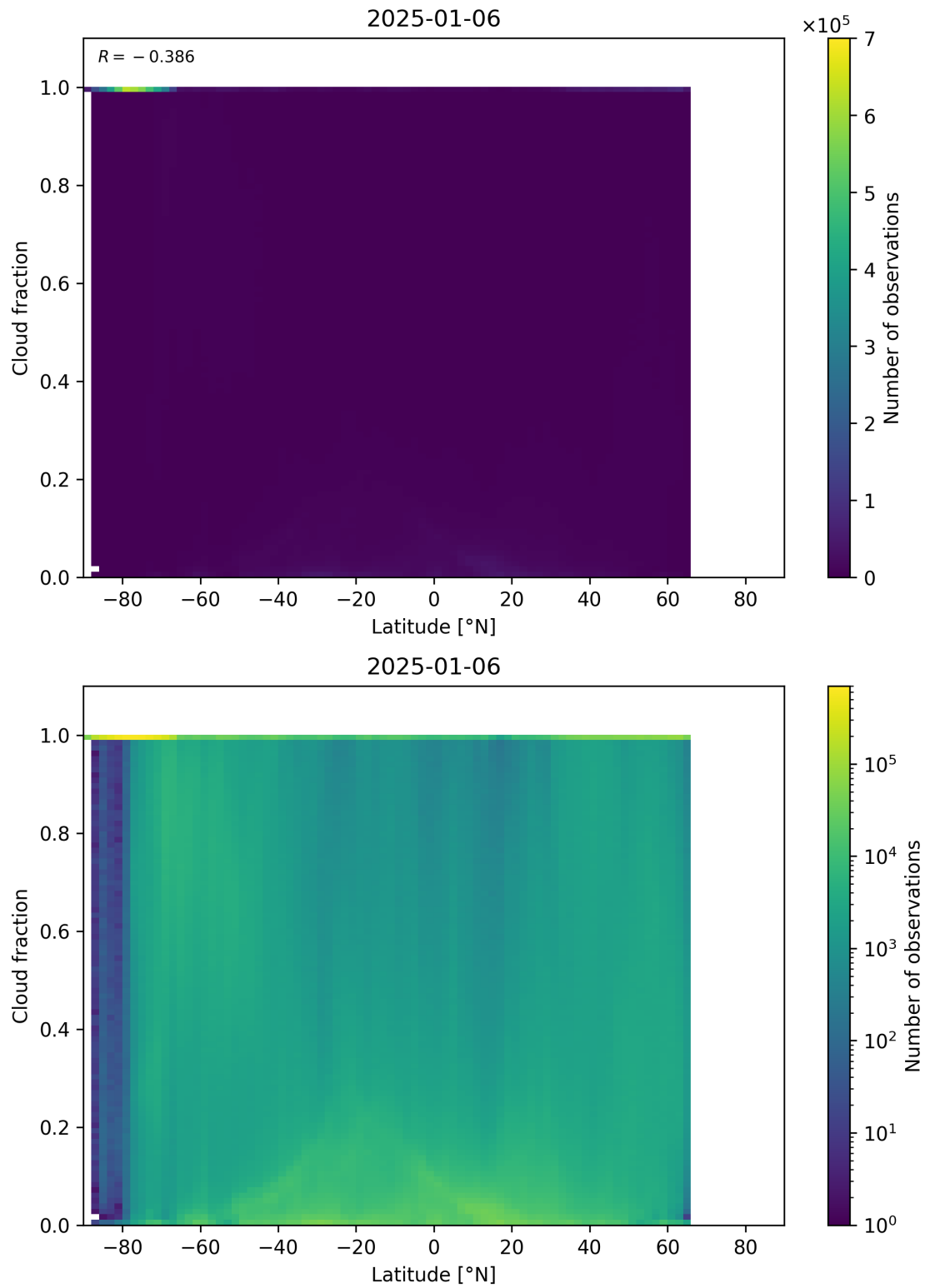
Figure 90: Scatter density plot of “Latitude” against “Cloud fraction” for 2025-01-05 to 2025-01-07.
