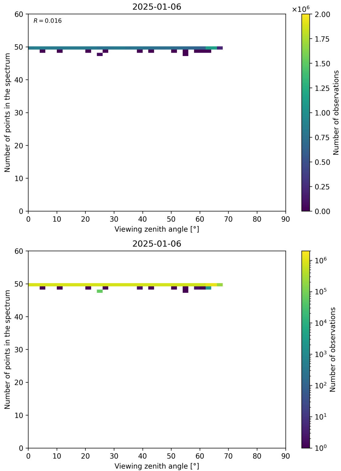
Figure 125: Scatter density plot of “Viewing zenith angle” against “Number of points in the spectrum” for 2025-01-05 to 2025-01-07.
