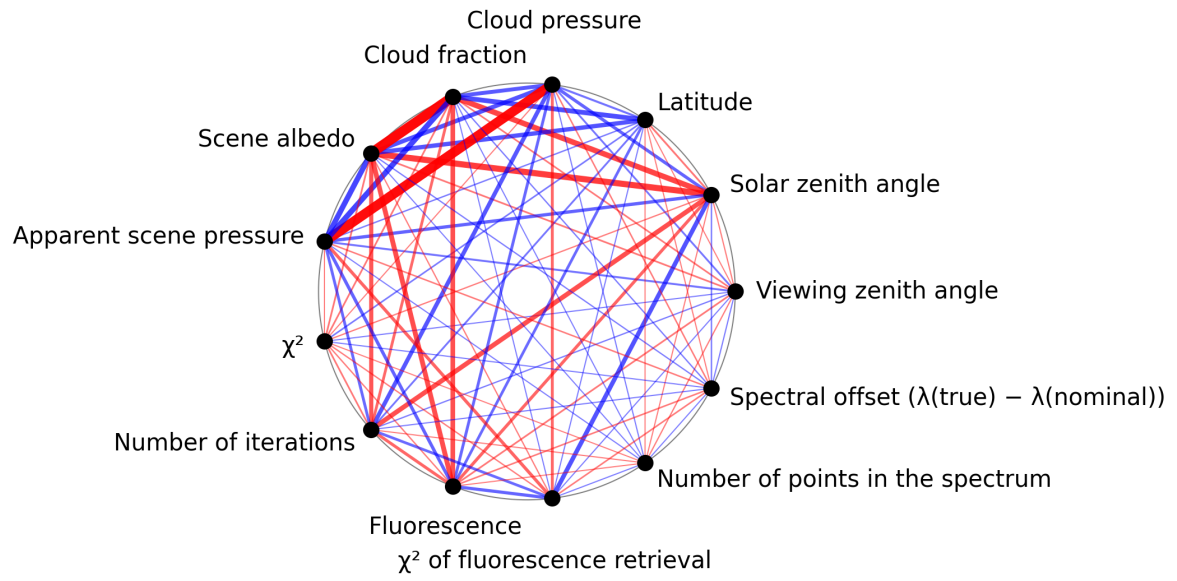
Figure 1: Map of correlation graph for 2025-01-05 to 2025-01-07.
