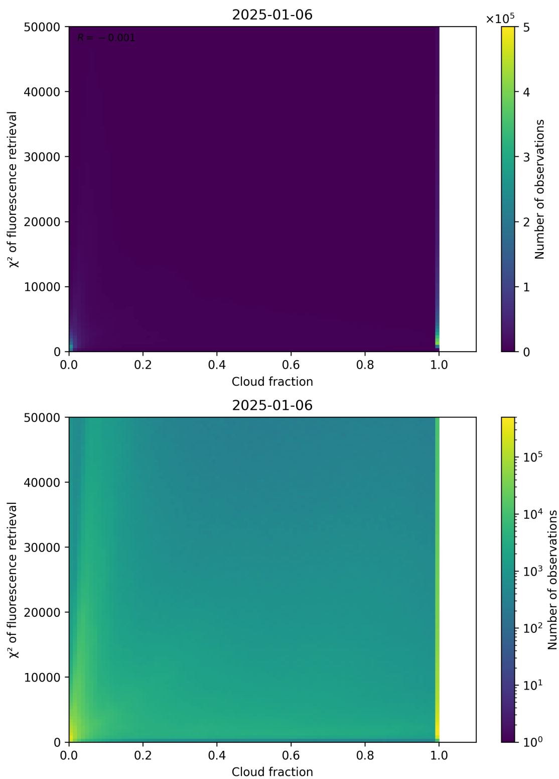
Figure 71: Scatter density plot of “Cloud fraction” against “ \chi^2 of fluorescence retrieval” for 2025-01-05 to 2025-01-07.
