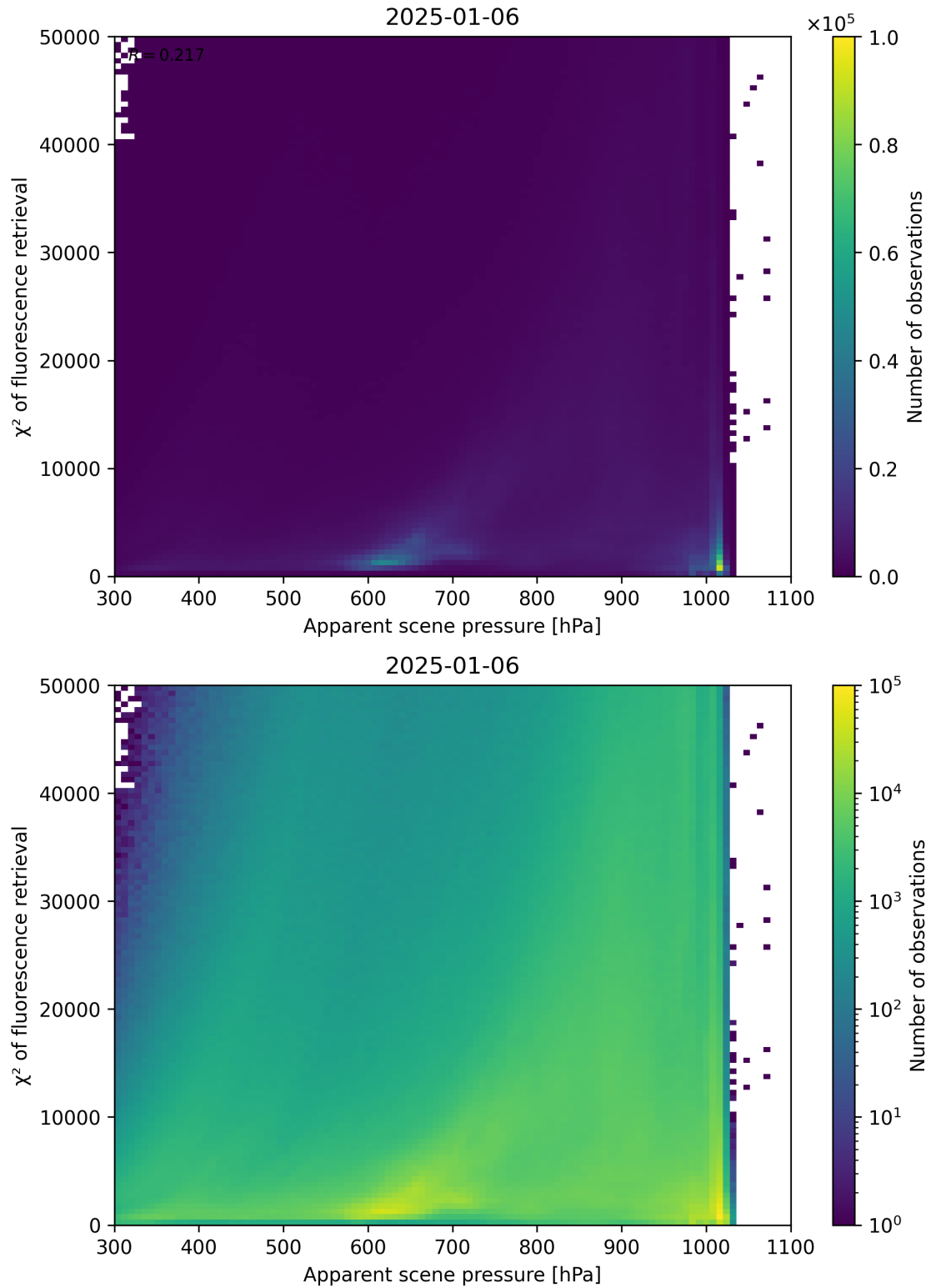
Figure 63: Scatter density plot of “Apparent scene pressure” against “ \chi^2 of fluorescence retrieval” for 2025-01-05 to 2025-01-07.
