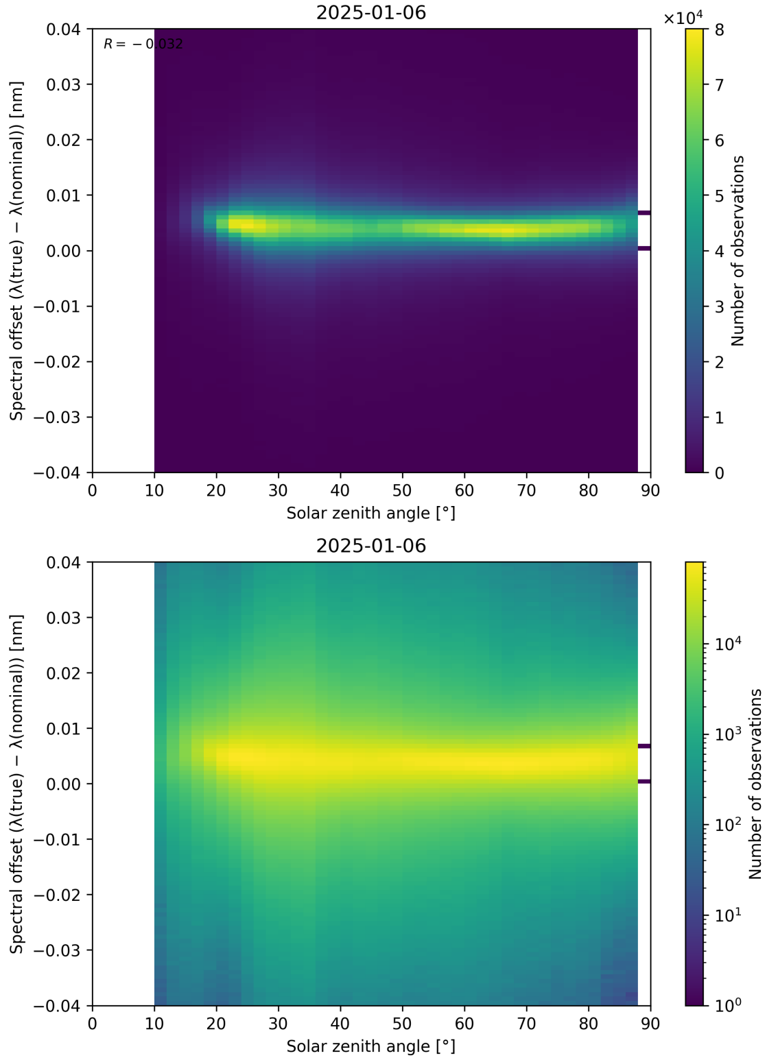
Figure 117: Scatter density plot of “Solar zenith angle” against “Spectral offset ( \lambda_{\text{true}} - \lambda_{\text{nominal}} )” for 2025-01-05 to 2025-01-07.
