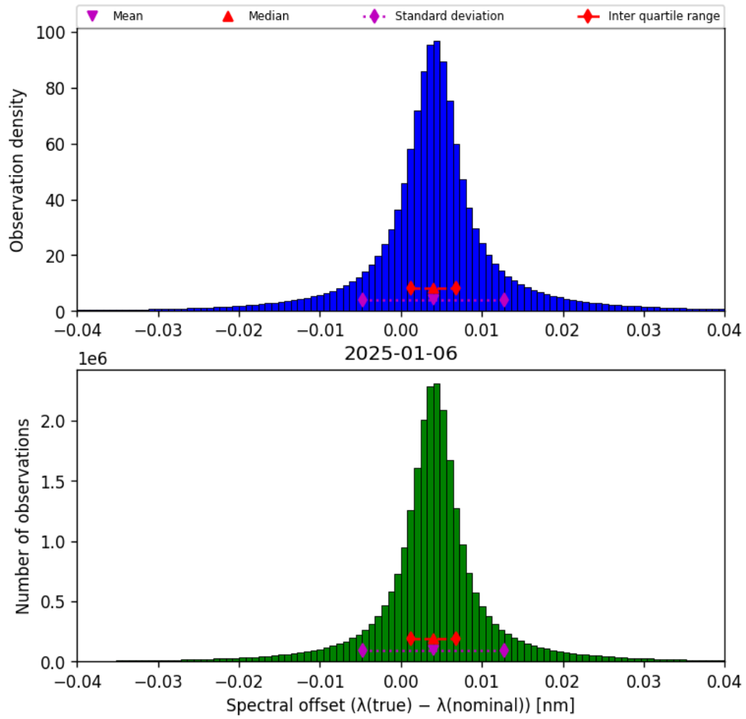
Figure 45: Histogram of “Spectral offset ( \lambda_{\text{true}} - \lambda_{\text{nominal}} )” for 2025-01-05 to 2025-01-07
