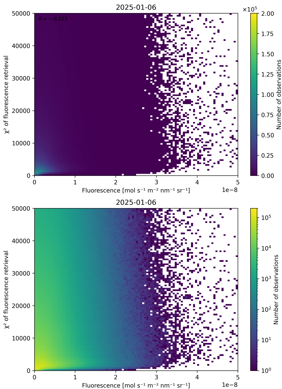
Figure 85: Scatter density plot of “Fluorescence” against “ \chi^2 of fluorescence retrieval” for 2025-01-05 to 2025-01-07.
