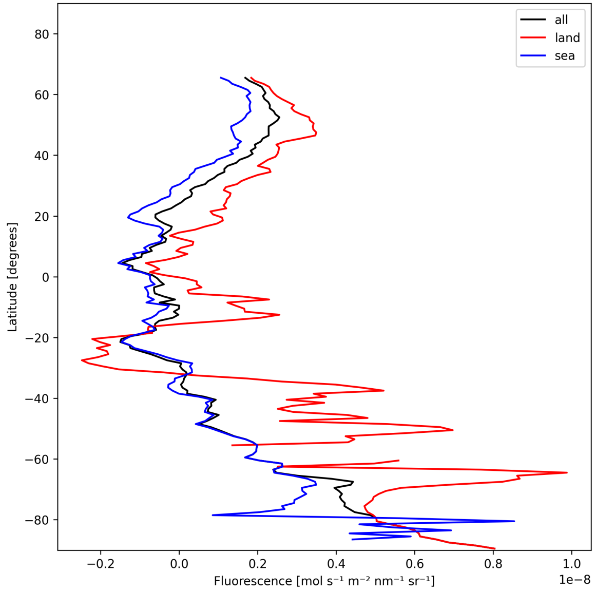
Figure 23: Zonal average of “Fluorescence” for 2025-01-05 to 2025-01-07.
