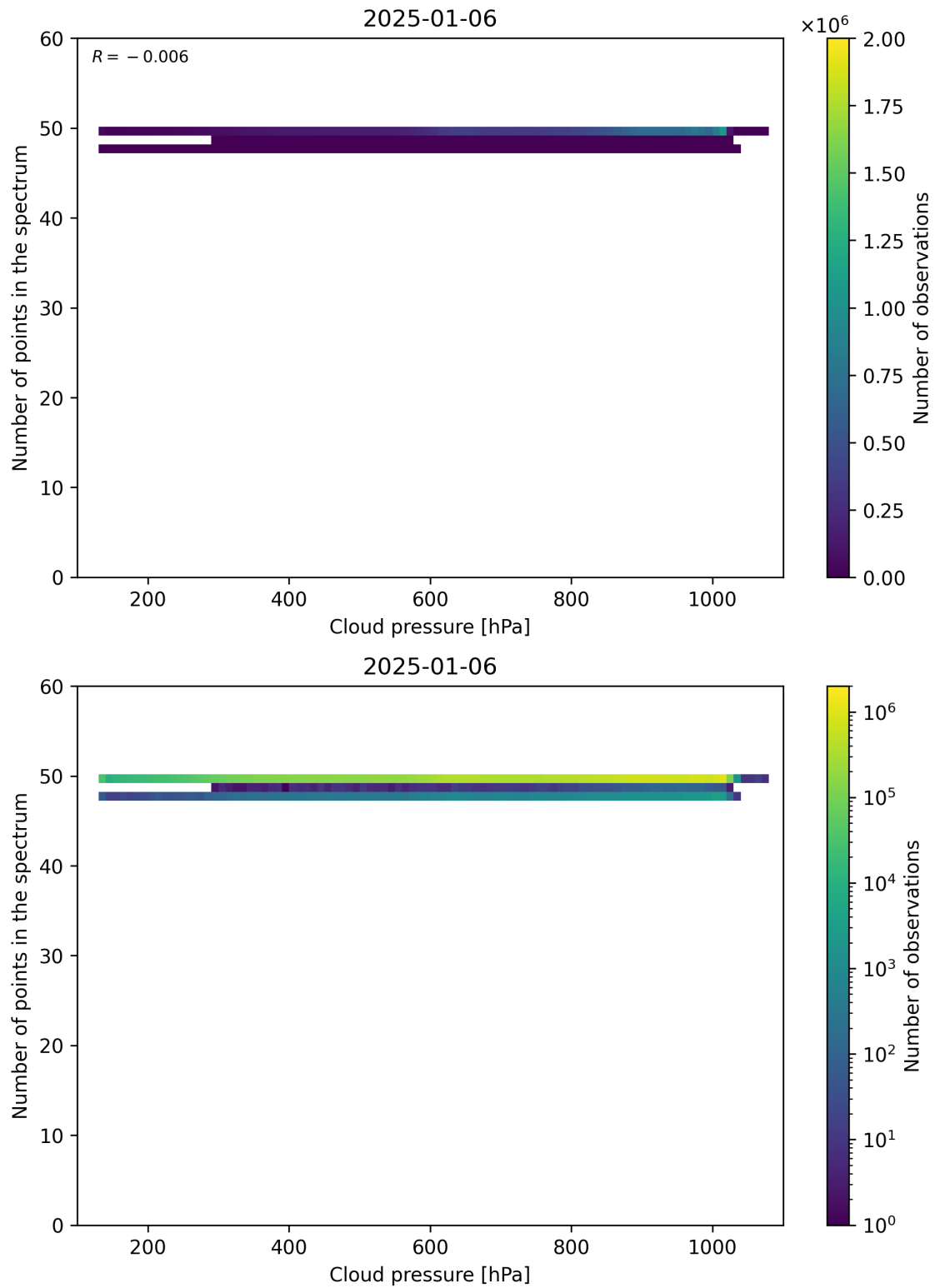
Figure 82: Scatter density plot of “Cloud pressure” against “Number of points in the spectrum” for 2025-01-05 to 2025-01-07.
