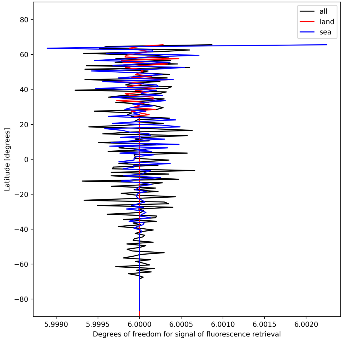
Figure 26: Zonal average of “Degrees of freedom for signal of fluorescence retrieval” for 2025-01-05 to 2025-01-07.
