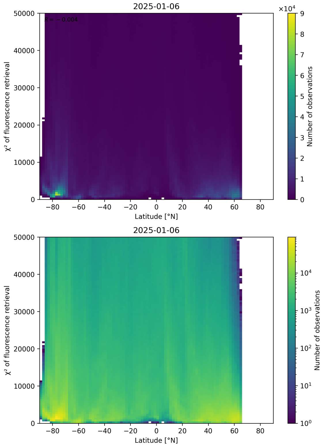
Figure 89: Scatter density plot of “Latitude” against “ \chi^2 of fluorescence retrieval” for 2025-01-05 to 2025-01-07.
