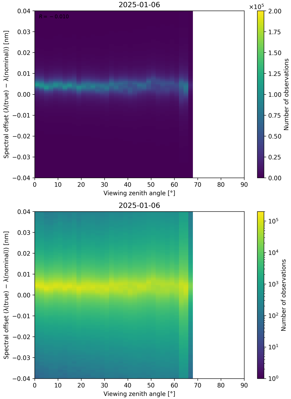
Figure 128: Scatter density plot of “Viewing zenith angle” against “Spectral offset ( \lambda_{\text{true}} - \lambda_{\text{nominal}} )” for 2025-01-05 to 2025-01-07.
