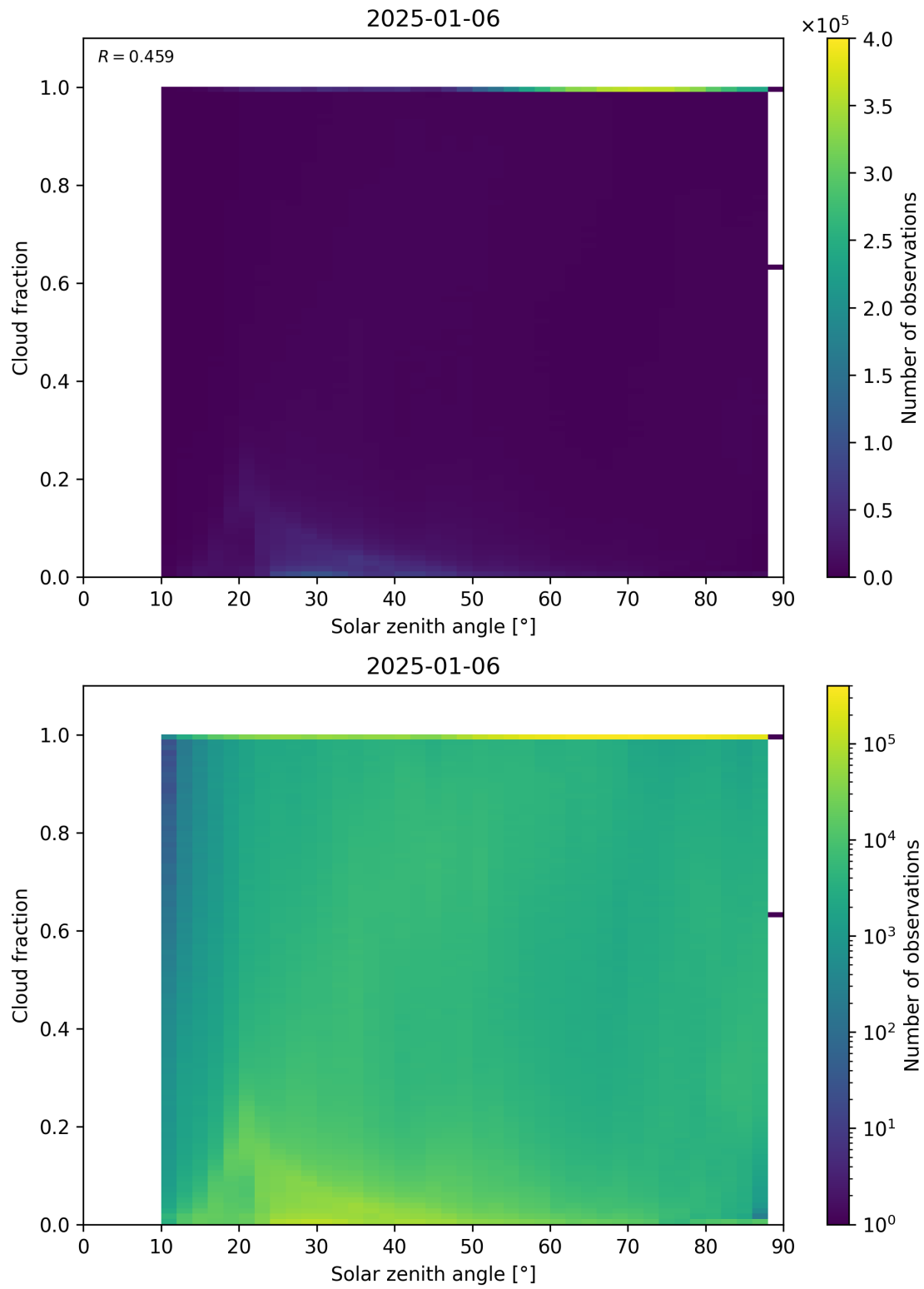
Figure 110: Scatter density plot of “Solar zenith angle” against “Cloud fraction” for 2025-01-05 to 2025-01-07.
