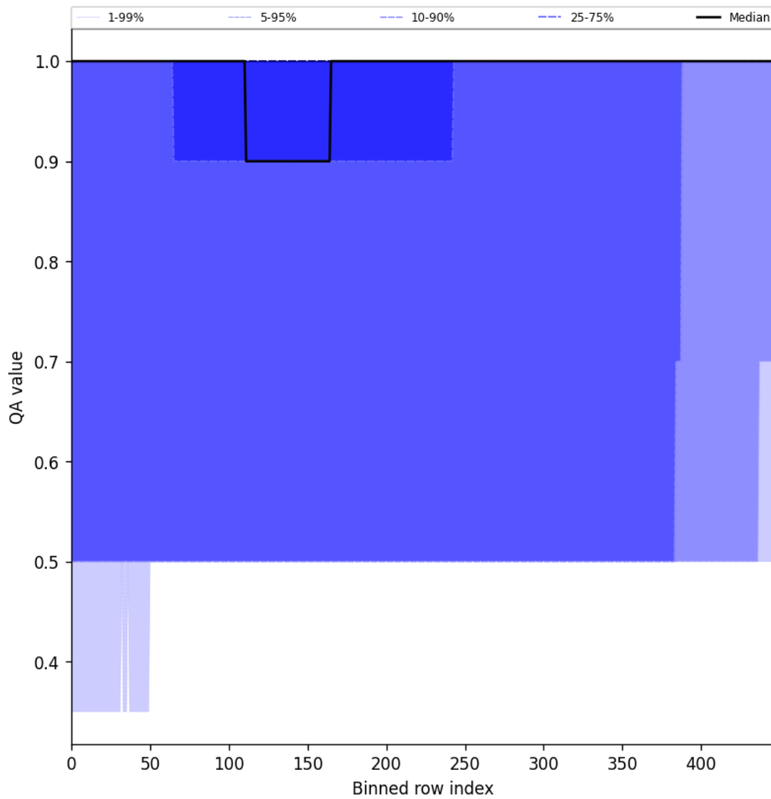
Figure 46: Along track statistics of “QA value” for 2025-01-05 to 2025-01-07
