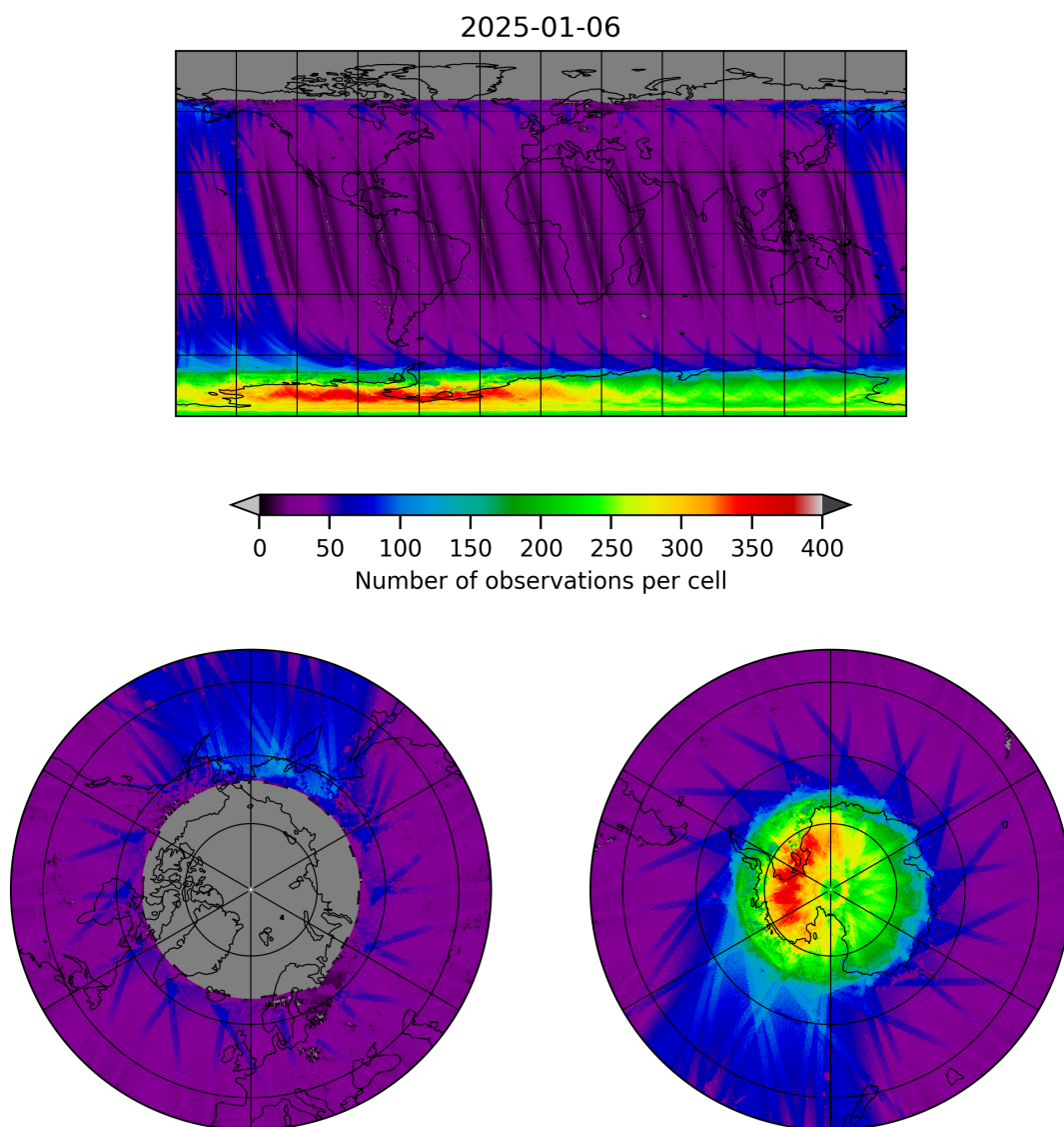
Figure 11: Map of the number of observations for 2025-01-05 to 2025-01-07
