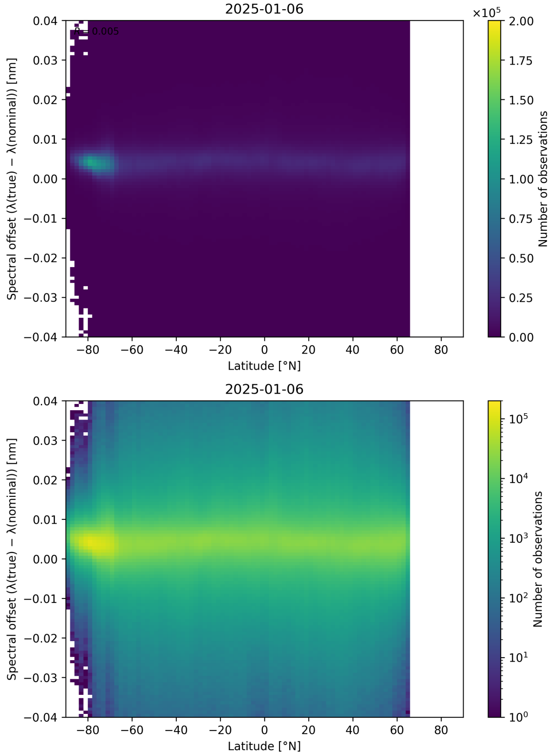
Figure 96: Scatter density plot of “Latitude” against “Spectral offset ( \lambda_{\text{true}} - \lambda_{\text{nominal}} )” for 2025-01-05 to 2025-01-07.
