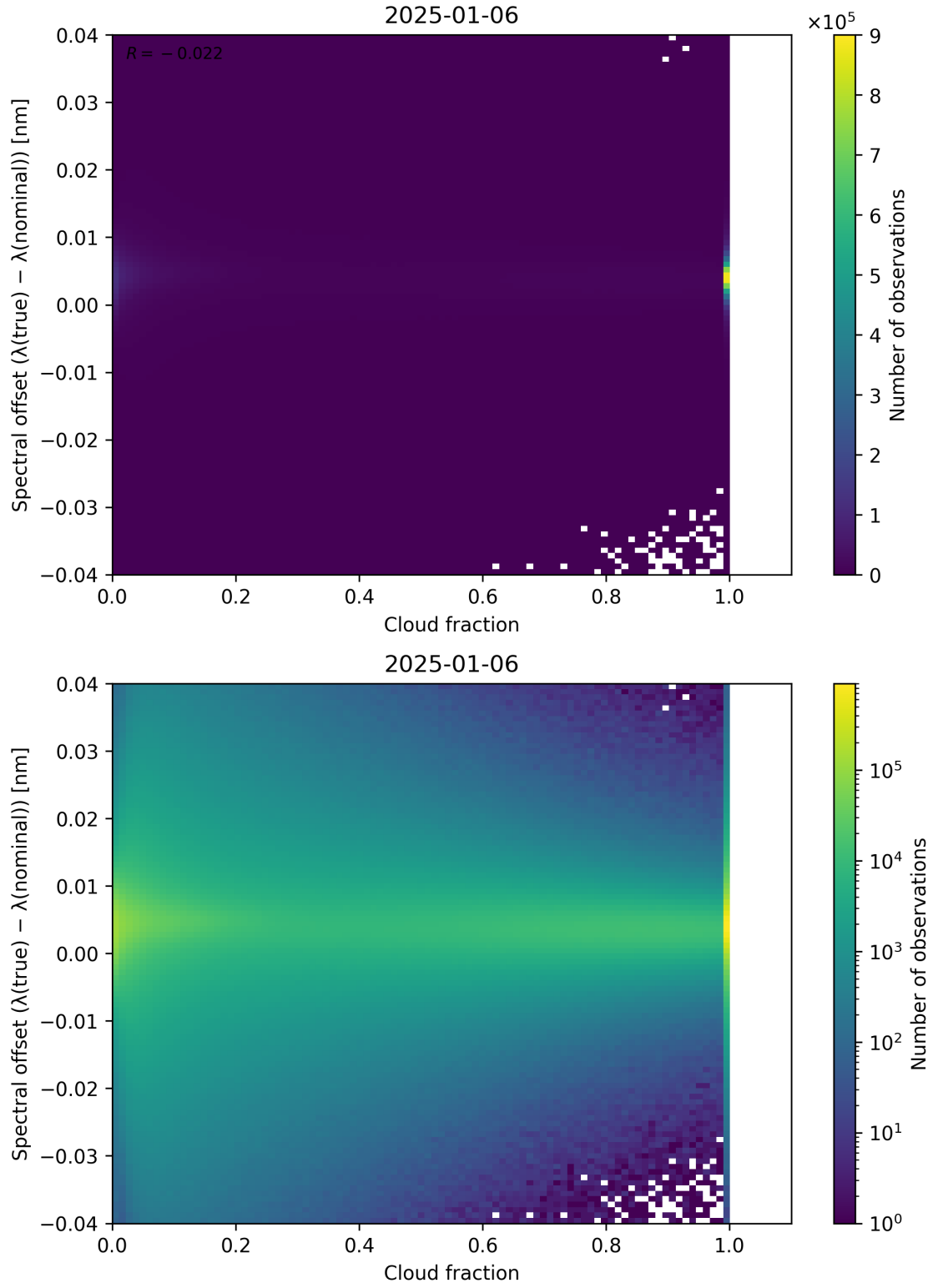
Figure 76: Scatter density plot of “Cloud fraction” against “Spectral offset ( \lambda_{\text{true}} - \lambda_{\text{nominal}} )” for 2025-01-05 to 2025-01-07.
