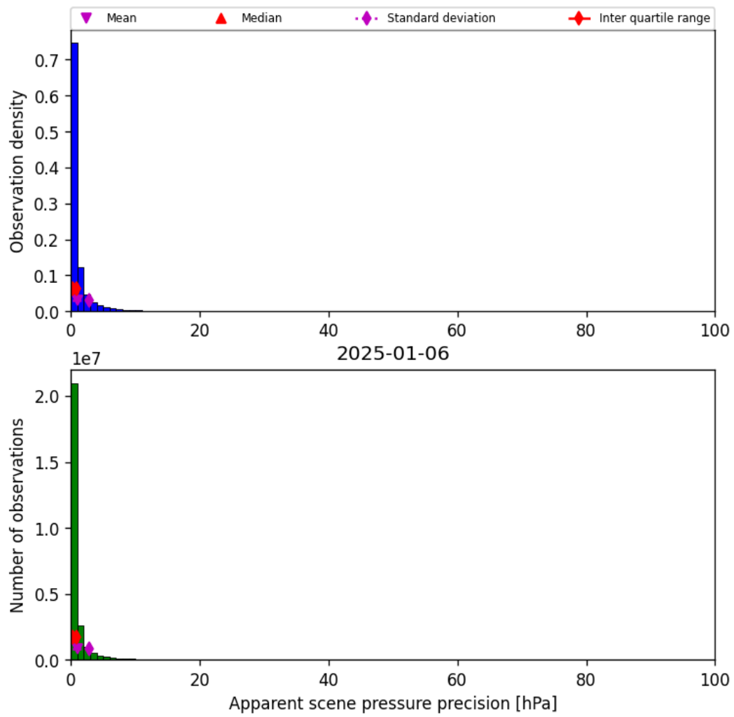
Figure 37: Histogram of “Apparent scene pressure precision” for 2025-01-05 to 2025-01-07
