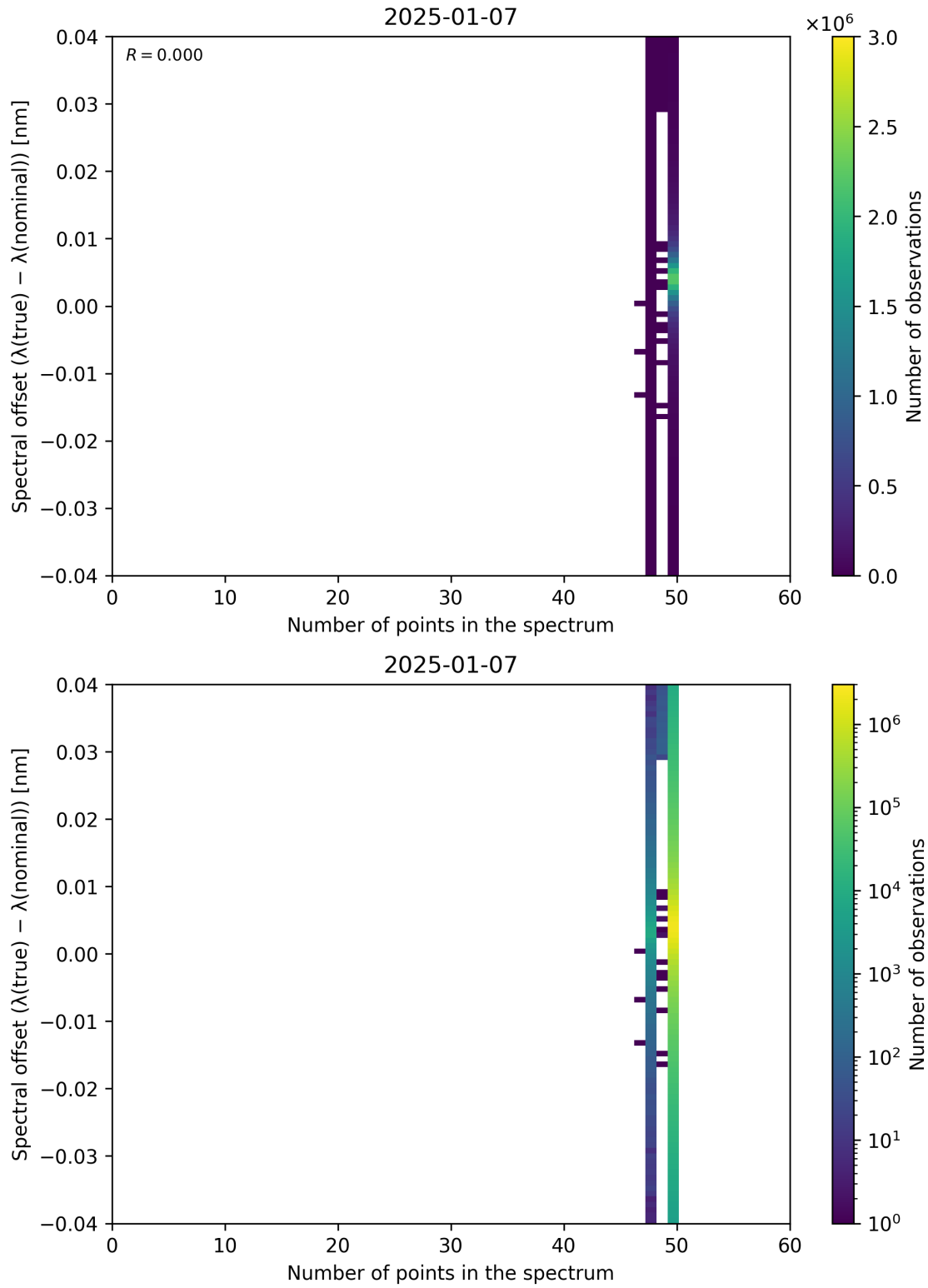
Figure 101: Scatter density plot of “Number of points in the spectrum” against “Spectral offset ( \lambda_{\text{true}} - \lambda_{\text{nominal}} )” for 2025-01-07 to 2025-01-08.
