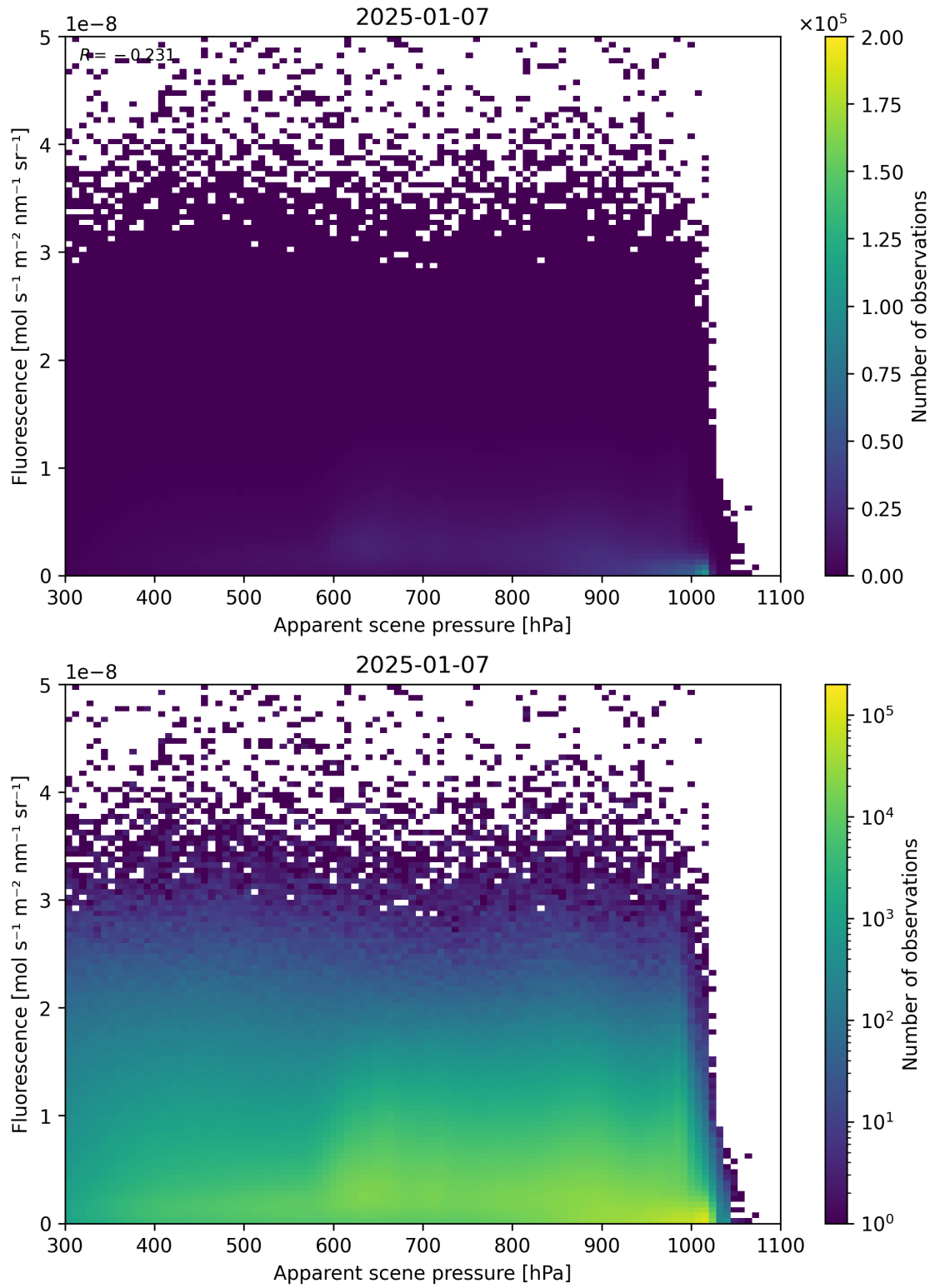
Figure 64: Scatter density plot of “Apparent scene pressure” against “Fluorescence” for 2025-01-07 to 2025-01-08.
