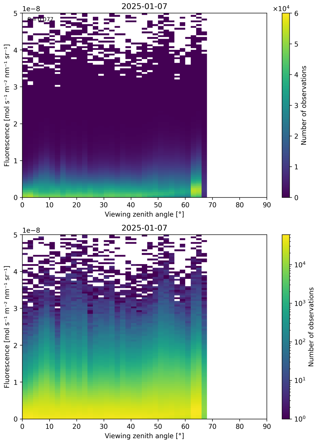
Figure 122: Scatter density plot of “Viewing zenith angle” against “Fluorescence” for 2025-01-07 to 2025-01-08.
