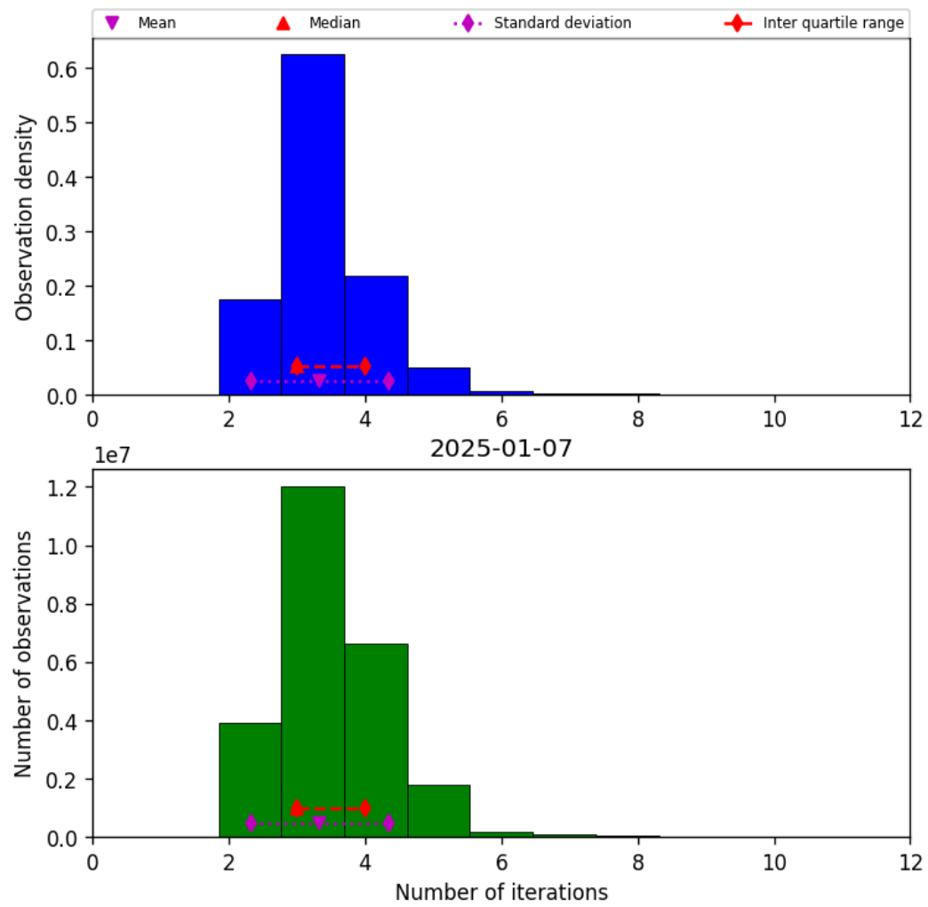
Figure 39: Histogram of “Number of iterations” for 2025-01-07 to 2025-01-08
