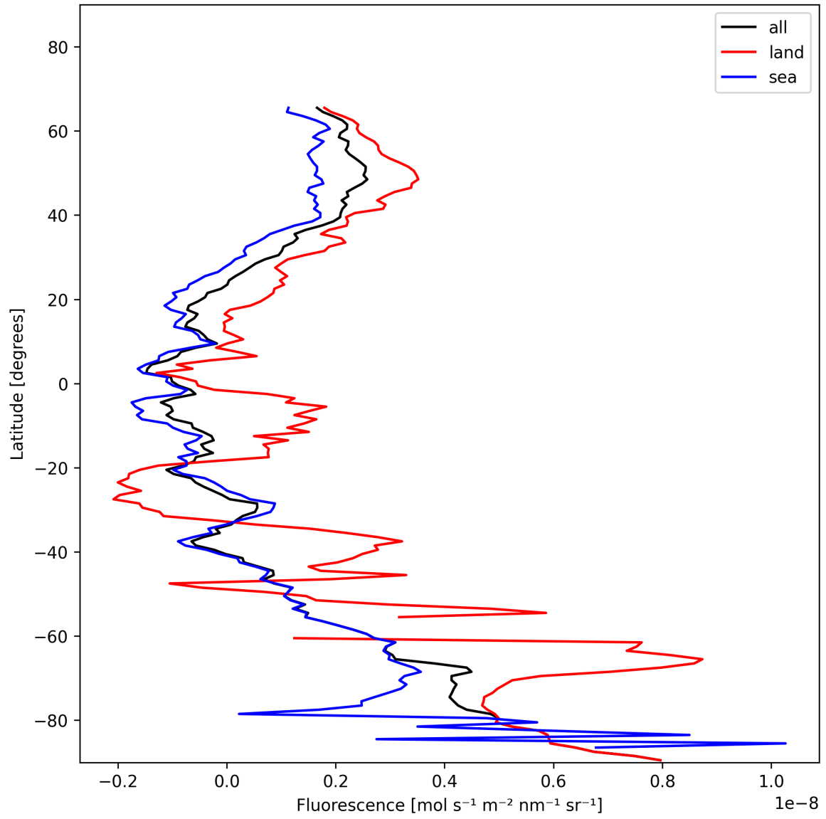
Figure 23: Zonal average of “Fluorescence” for 2025-01-07 to 2025-01-08.
