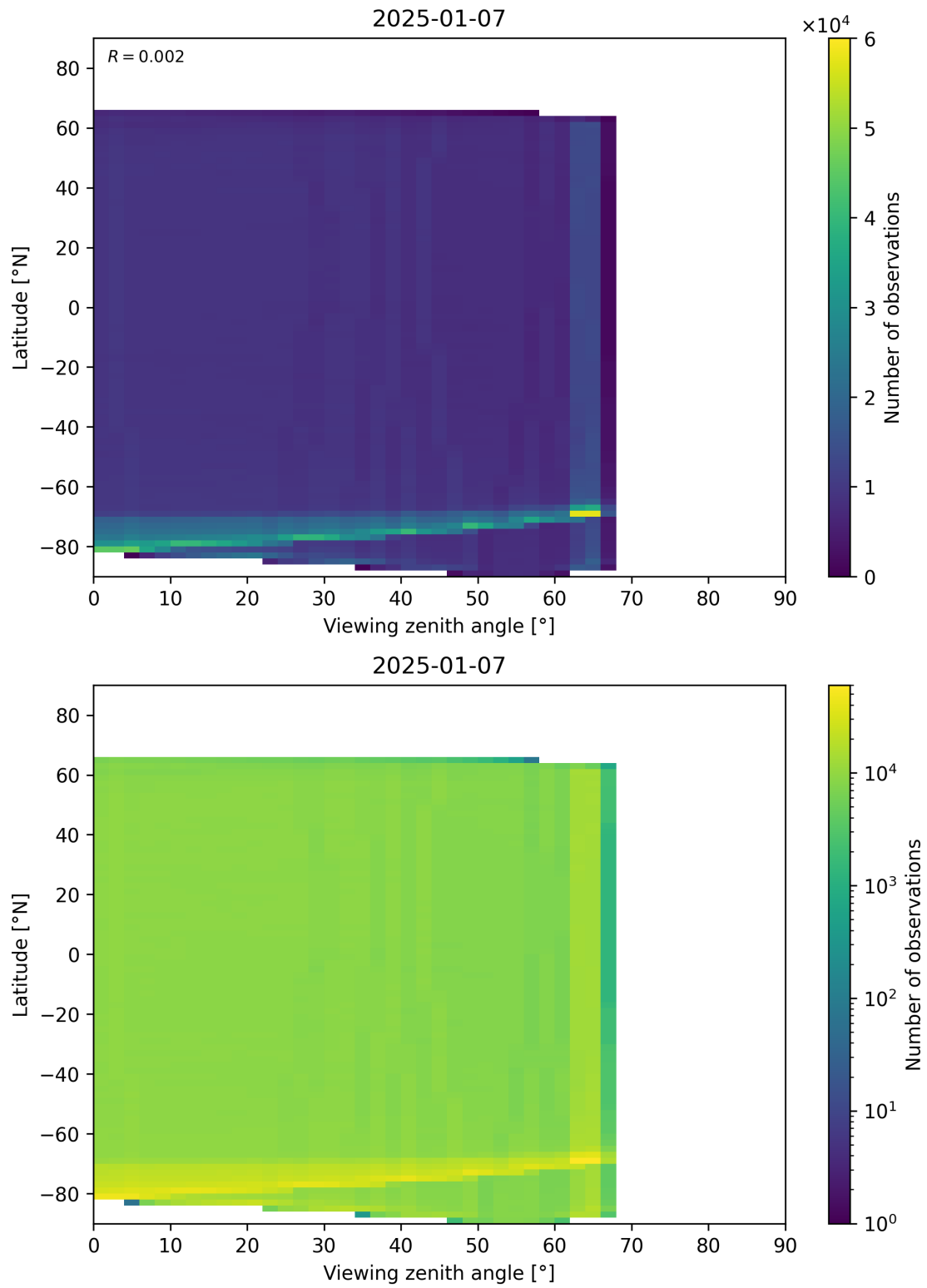
Figure 123: Scatter density plot of “Viewing zenith angle” against “Latitude” for 2025-01-07 to 2025-01-08.
