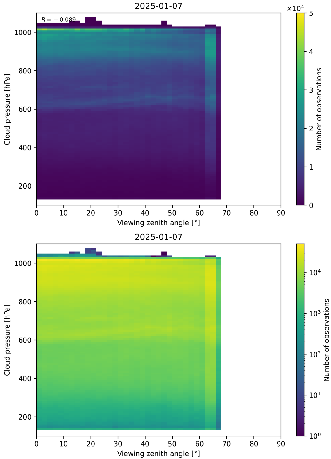
Figure 121: Scatter density plot of “Viewing zenith angle” against “Cloud pressure” for 2025-01-07 to 2025-01-08.
