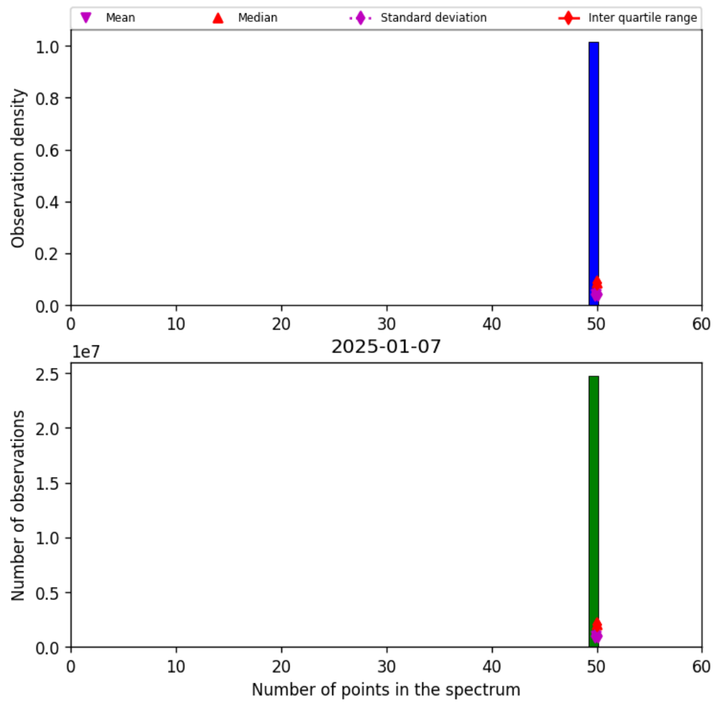
Figure 44: Histogram of “Number of points in the spectrum” for 2025-01-07 to 2025-01-08
