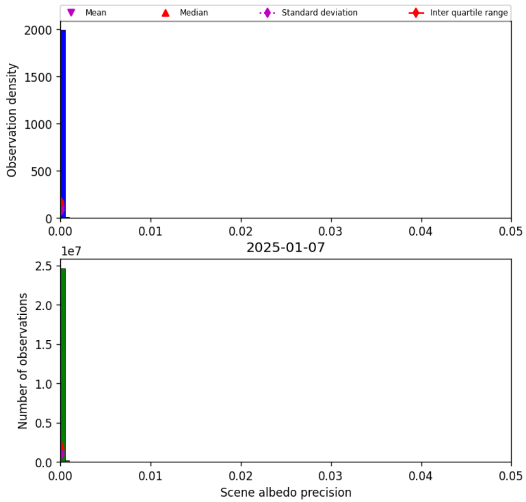
Figure 35: Histogram of “Scene albedo precision” for 2025-01-07 to 2025-01-08
