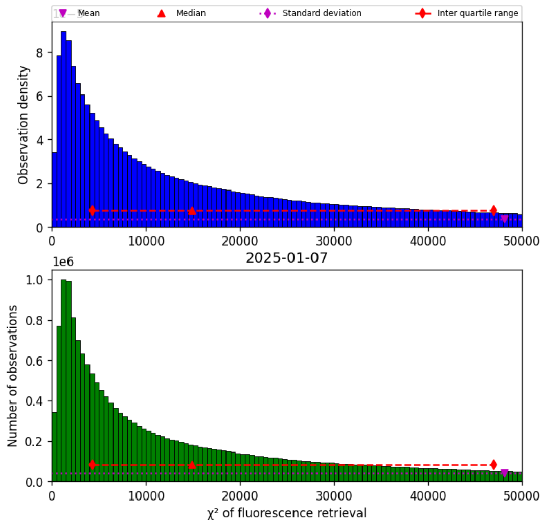
Figure 42: Histogram of “ \chi^2 of fluorescence retrieval” for 2025-01-07 to 2025-01-08
