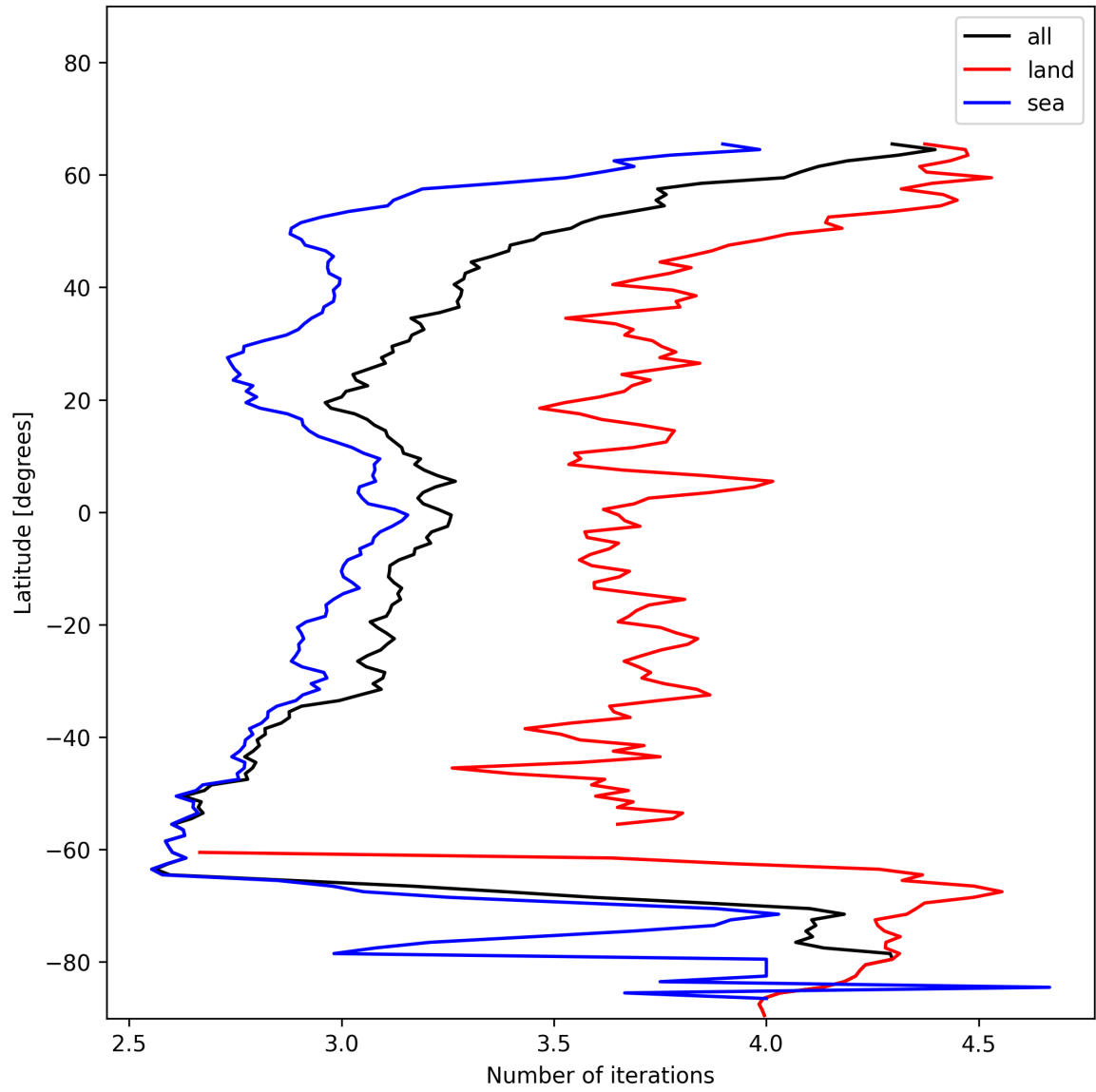
Figure 22: Zonal average of “Number of iterations” for 2025-01-07 to 2025-01-08.
