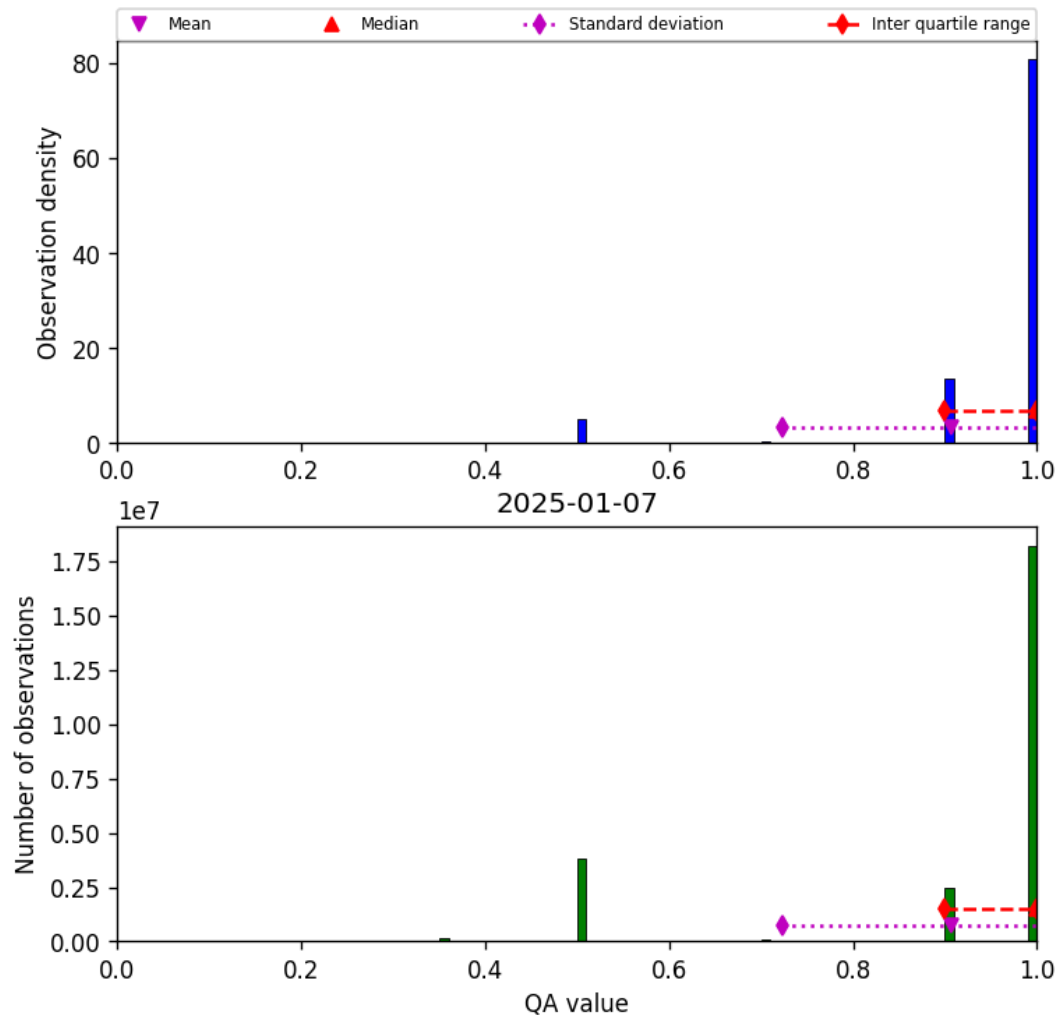
Figure 29: Histogram of “QA value” for 2025-01-07 to 2025-01-08
