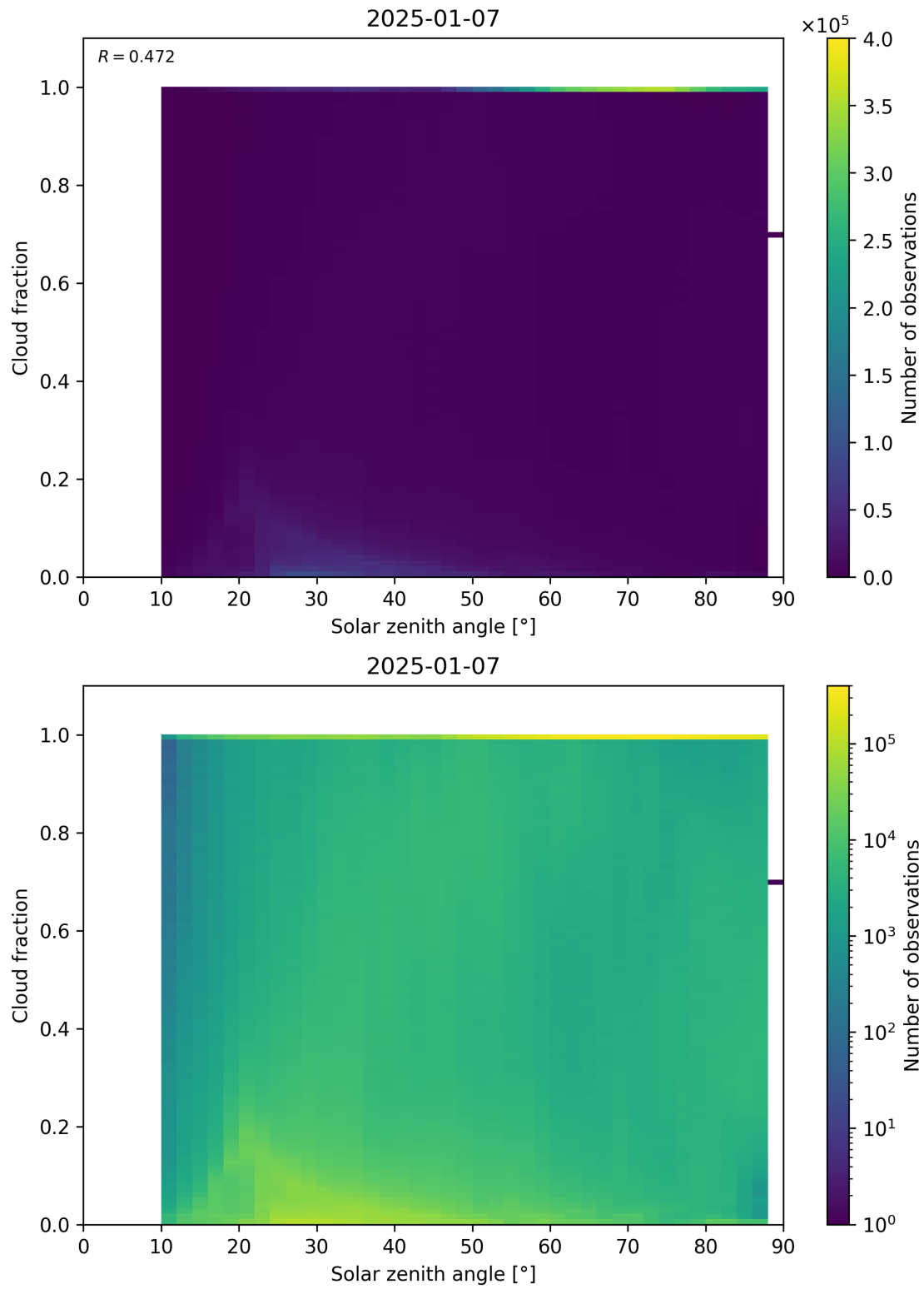
Figure 110: Scatter density plot of “Solar zenith angle” against “Cloud fraction” for 2025-01-07 to 2025-01-08.
