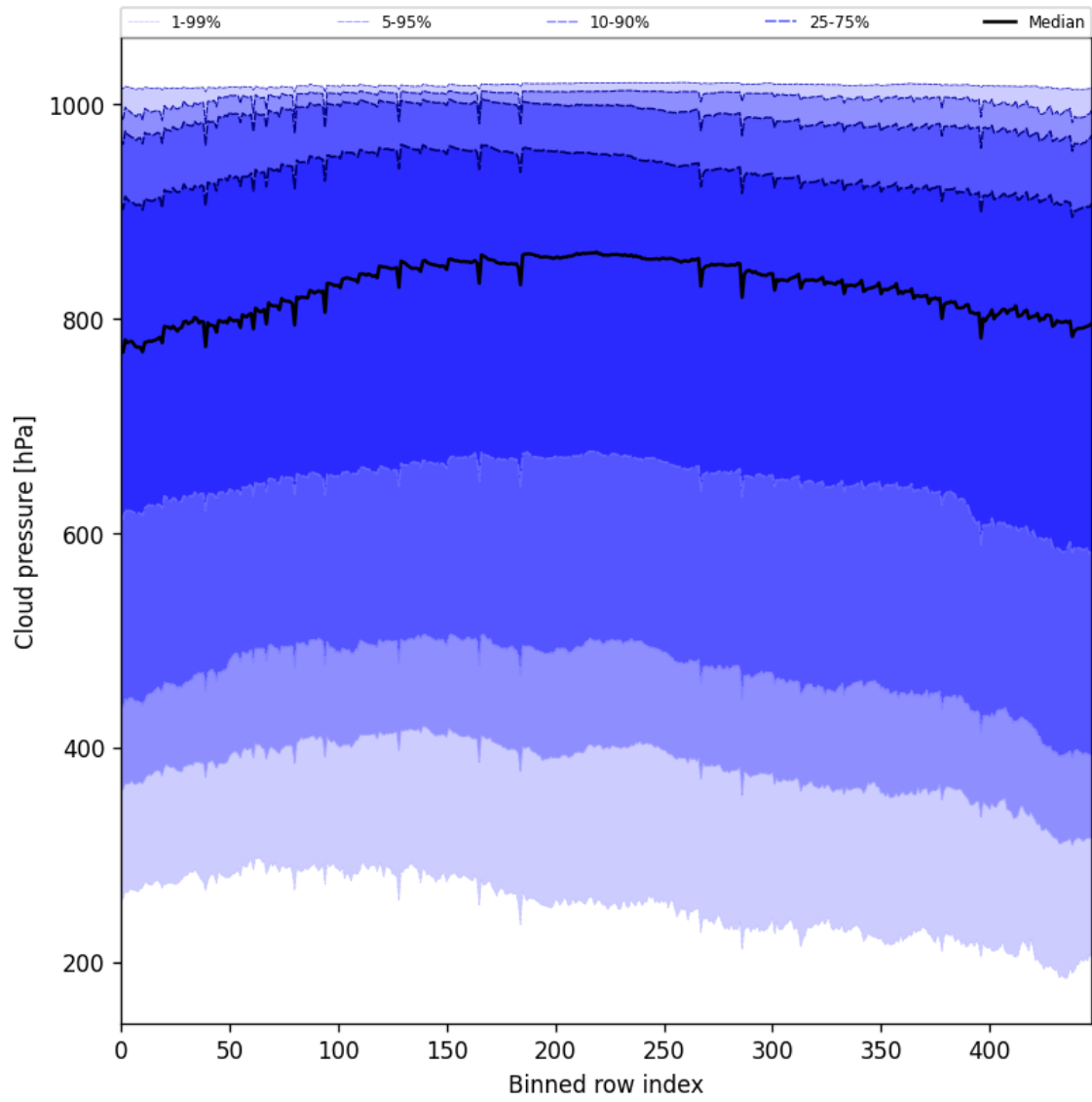
Figure 47: Along track statistics of “Cloud pressure” for 2025-01-07 to 2025-01-08
