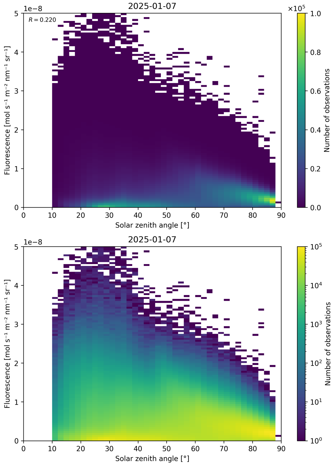
Figure 112: Scatter density plot of “Solar zenith angle” against “Fluorescence” for 2025-01-07 to 2025-01-08.
