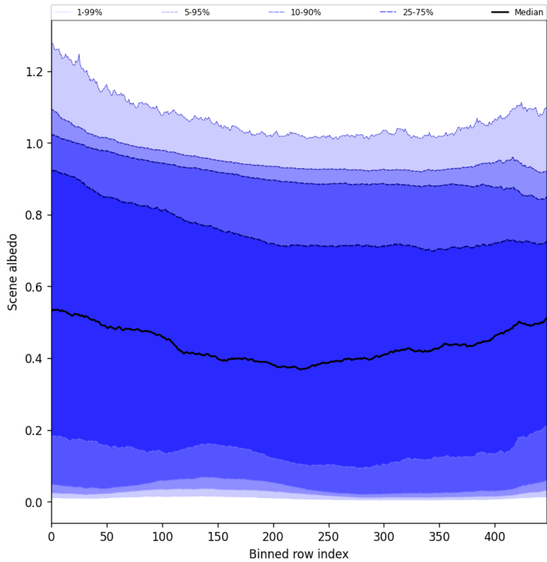
Figure 51: Along track statistics of “Scene albedo” for 2025-01-07 to 2025-01-08
