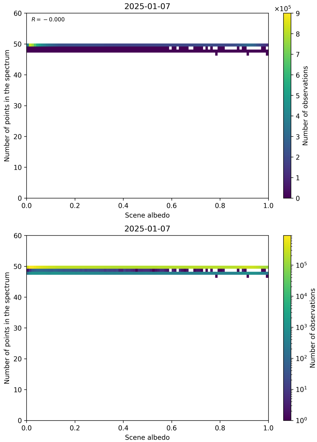
Figure 106: Scatter density plot of “Scene albedo” against “Number of points in the spectrum” for 2025-01-07 to 2025-01-08.
