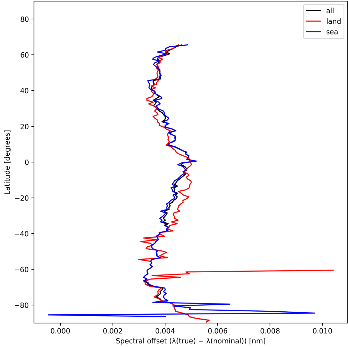
Figure 28: Zonal average of “Spectral offset ( \lambda_{\text{true}} - \lambda_{\text{nominal}} )” for 2025-01-07 to 2025-01-08.
