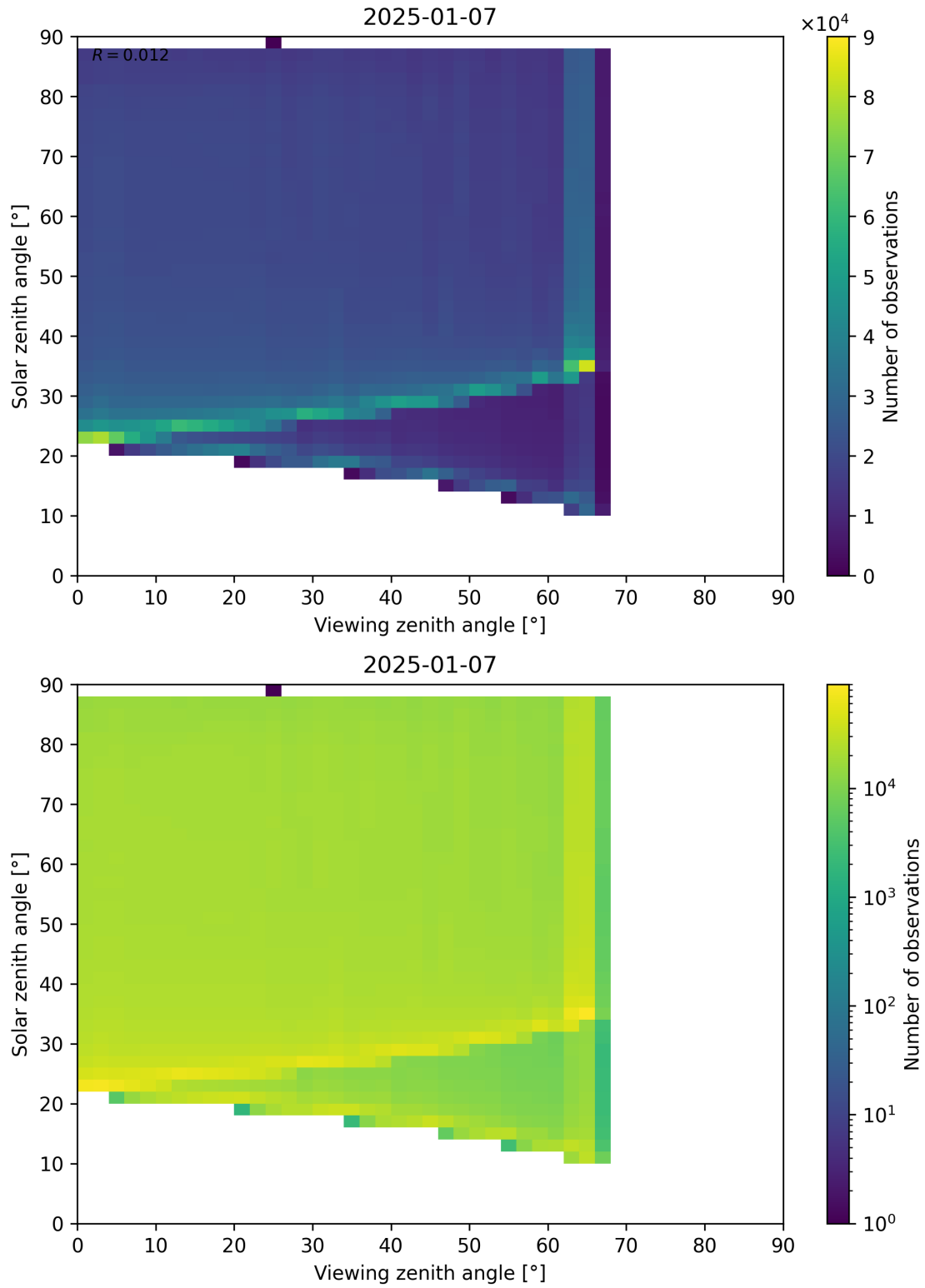
Figure 127: Scatter density plot of “Viewing zenith angle” against “Solar zenith angle” for 2025-01-07 to 2025-01-08.
