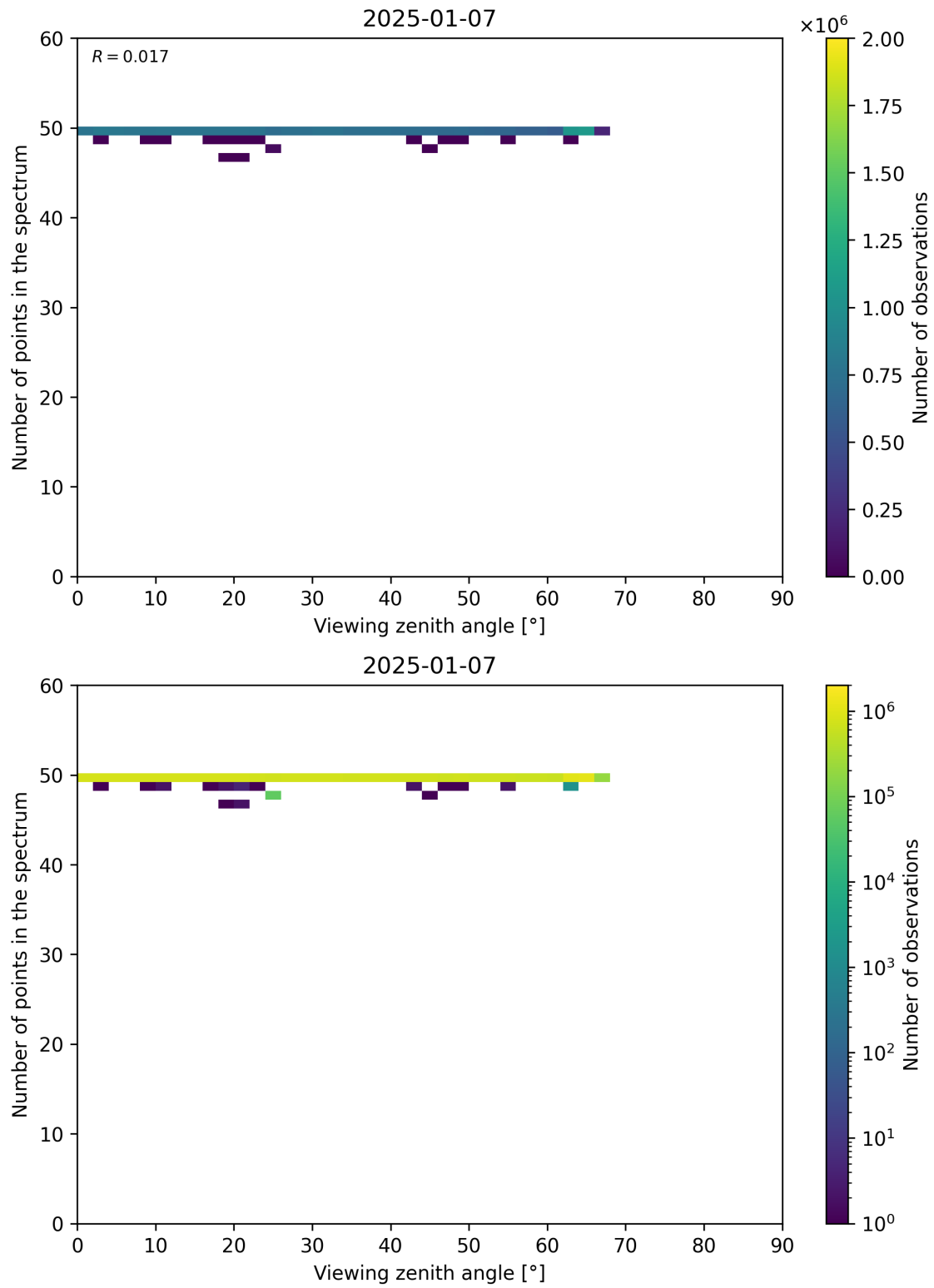
Figure 125: Scatter density plot of “Viewing zenith angle” against “Number of points in the spectrum” for 2025-01-07 to 2025-01-08.
