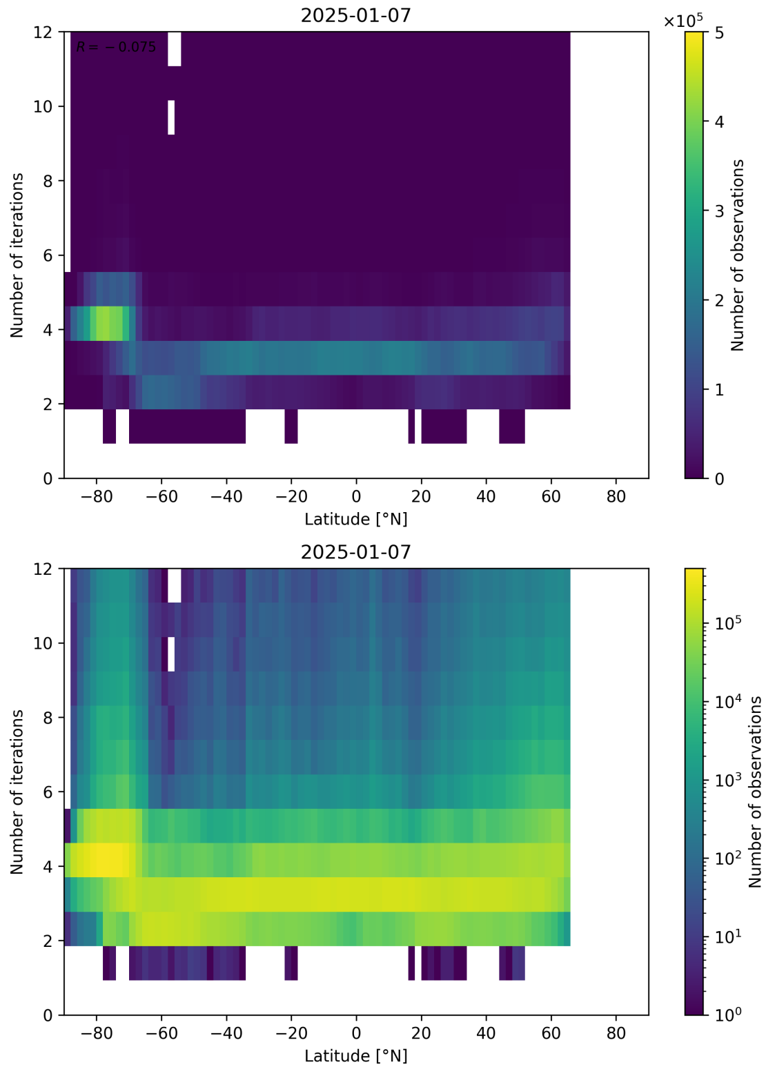
Figure 93: Scatter density plot of “Latitude” against “Number of iterations” for 2025-01-07 to 2025-01-08.
