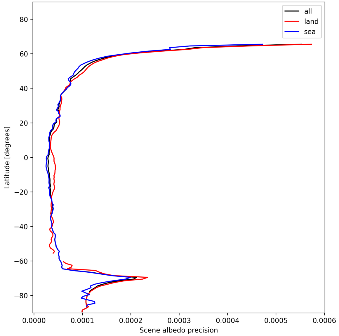
Figure 18: Zonal average of “Scene albedo precision” for 2025-01-07 to 2025-01-08.
