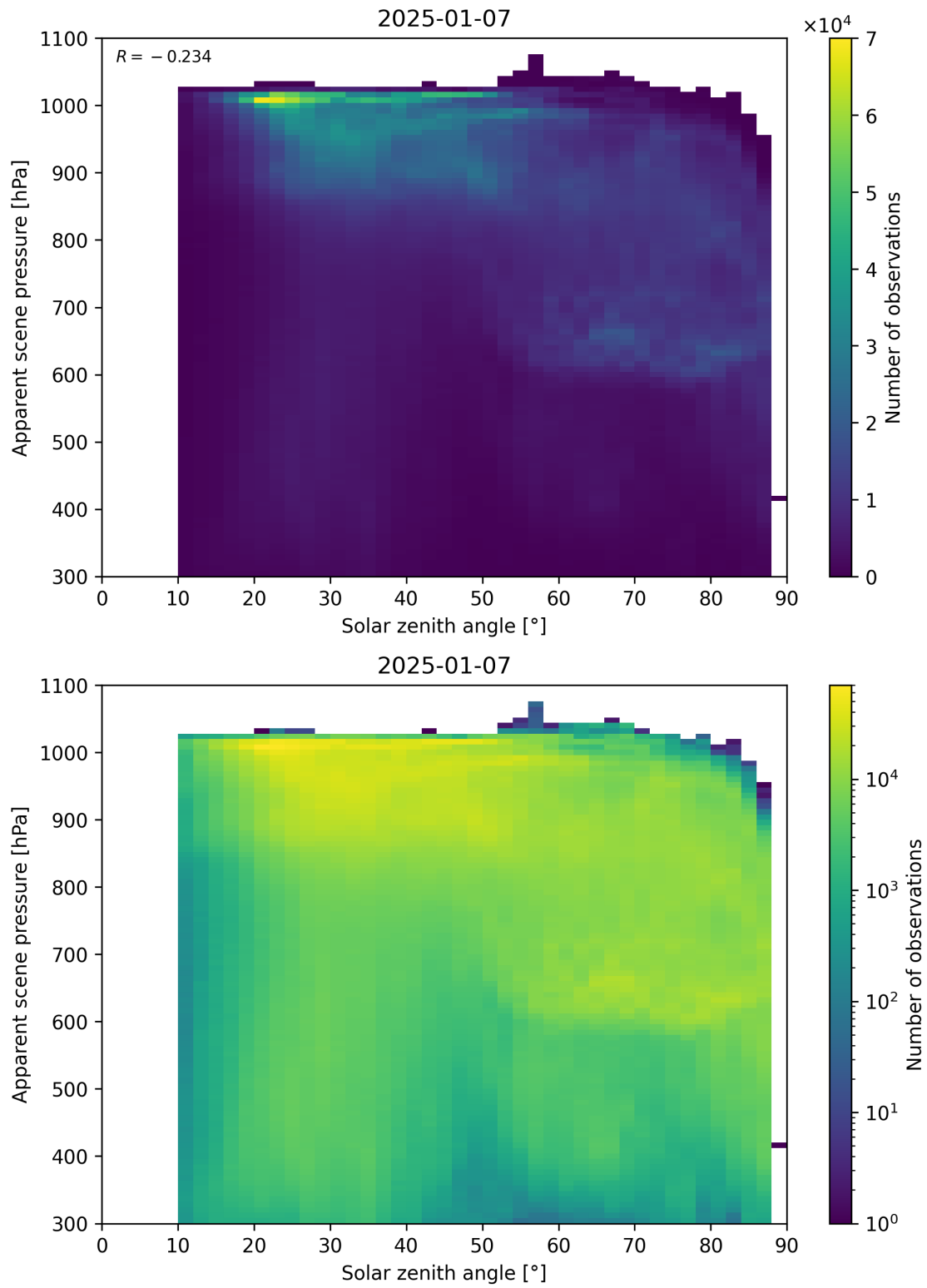
Figure 108: Scatter density plot of “Solar zenith angle” against “Apparent scene pressure” for 2025-01-07 to 2025-01-08.
