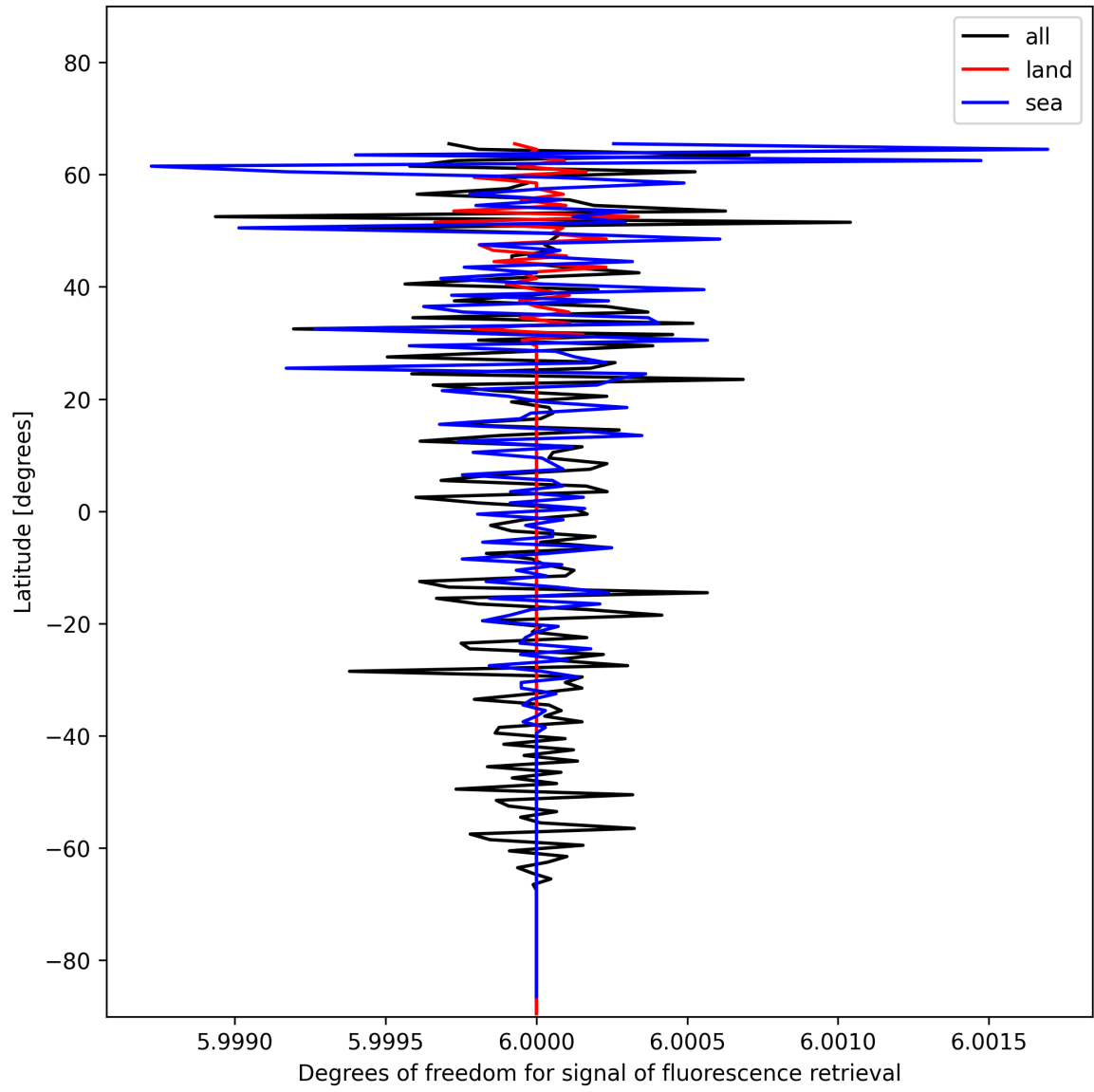
Figure 26: Zonal average of “Degrees of freedom for signal of fluorescence retrieval” for 2025-01-07 to 2025-01-08.
