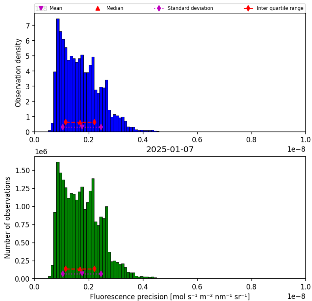
Figure 41: Histogram of “Fluorescence precision” for 2025-01-07 to 2025-01-08
