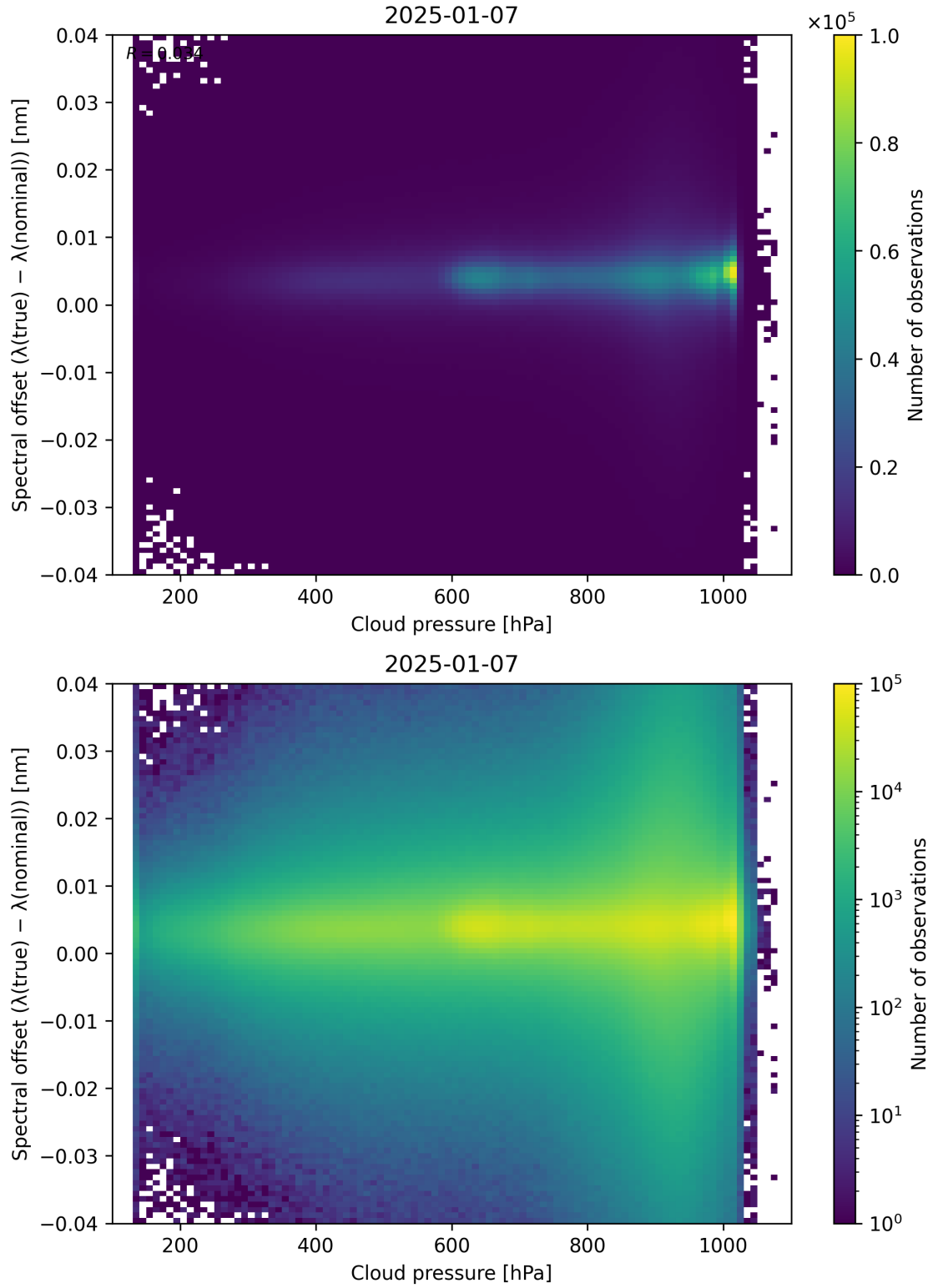
Figure 84: Scatter density plot of “Cloud pressure” against “Spectral offset ( \lambda_{\text{true}} - \lambda_{\text{nominal}} )” for 2025-01-07 to 2025-01-08.
