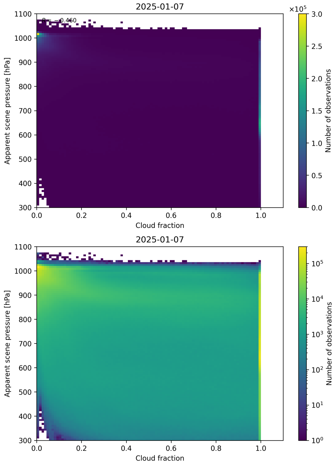
Figure 70: Scatter density plot of “Cloud fraction” against “Apparent scene pressure” for 2025-01-07 to 2025-01-08.
