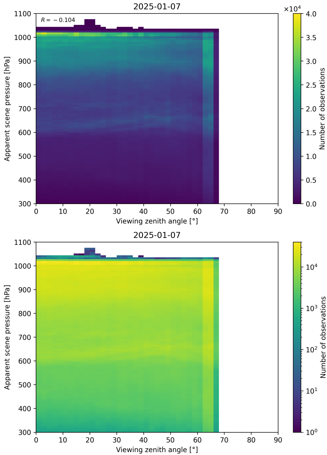
Figure 118: Scatter density plot of “Viewing zenith angle” against “Apparent scene pressure” for 2025-01-07 to 2025-01-08.
