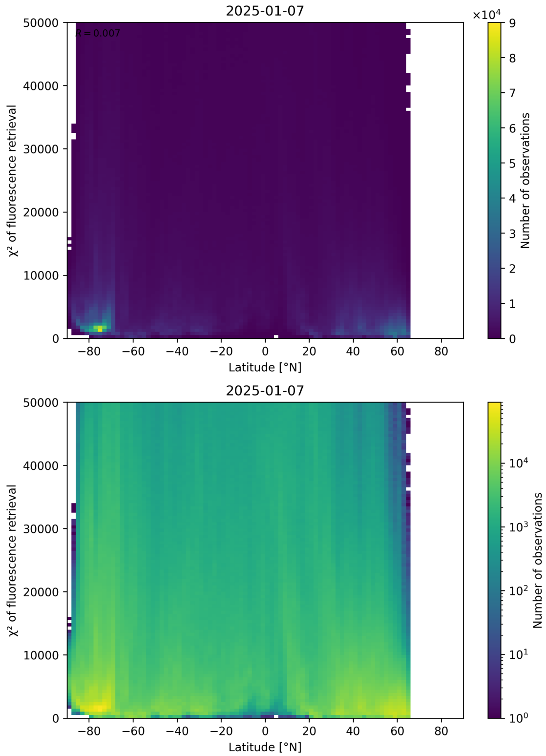
Figure 89: Scatter density plot of “Latitude” against “ \chi^2 of fluorescence retrieval” for 2025-01-07 to 2025-01-08.
