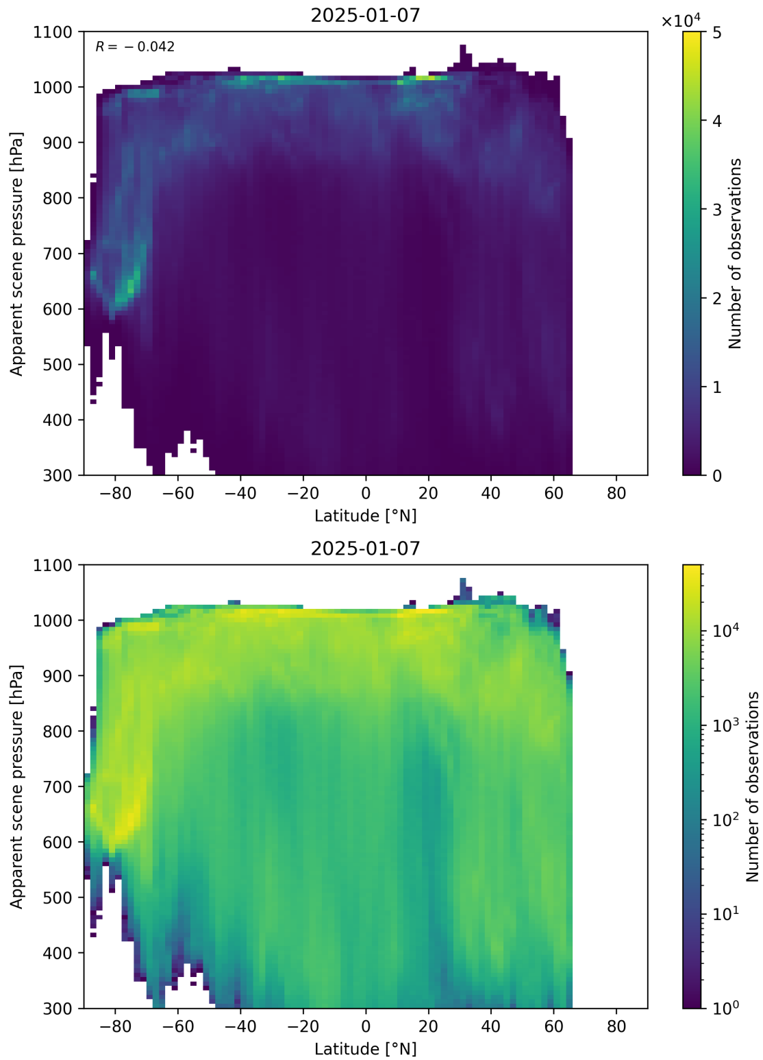
Figure 88: Scatter density plot of “Latitude” against “Apparent scene pressure” for 2025-01-07 to 2025-01-08.
