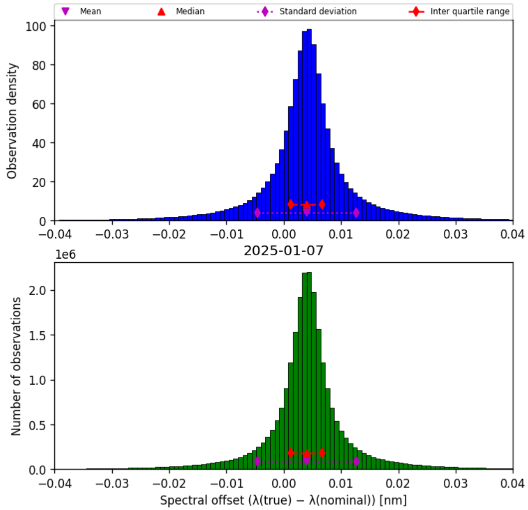
Figure 45: Histogram of “Spectral offset ( \lambda_{\text{true}} - \lambda_{\text{nominal}} )” for 2025-01-07 to 2025-01-08
