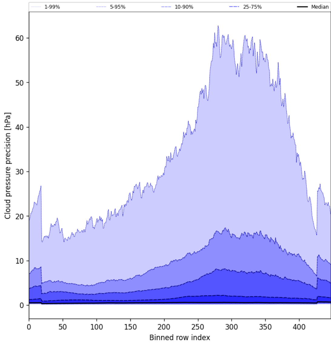
Figure 48: Along track statistics of “Cloud pressure precision” for 2025-01-07 to 2025-01-08
