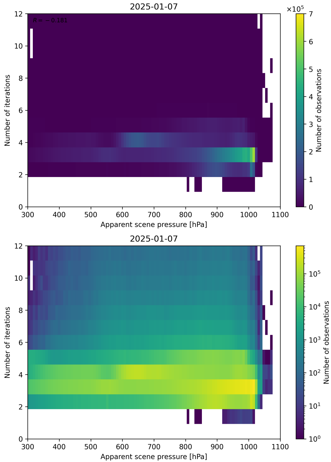
Figure 65: Scatter density plot of “Apparent scene pressure” against “Number of iterations” for 2025-01-07 to 2025-01-08.
