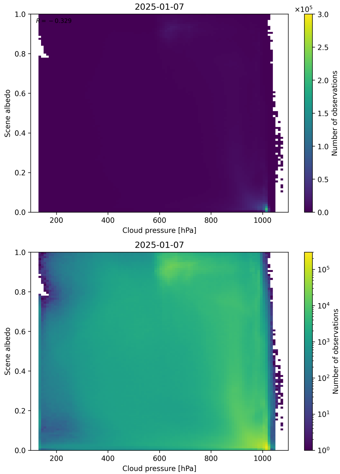
Figure 83: Scatter density plot of “Cloud pressure” against “Scene albedo” for 2025-01-07 to 2025-01-08.
