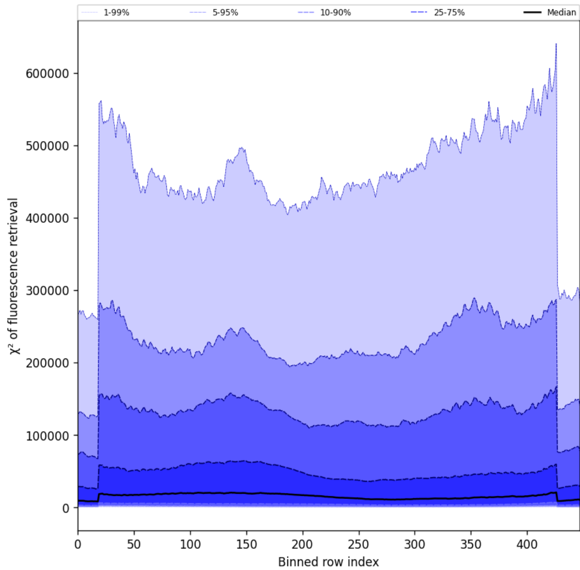
Figure 59: Along track statistics of “ \chi^2 of fluorescence retrieval” for 2025-01-07 to 2025-01-08
