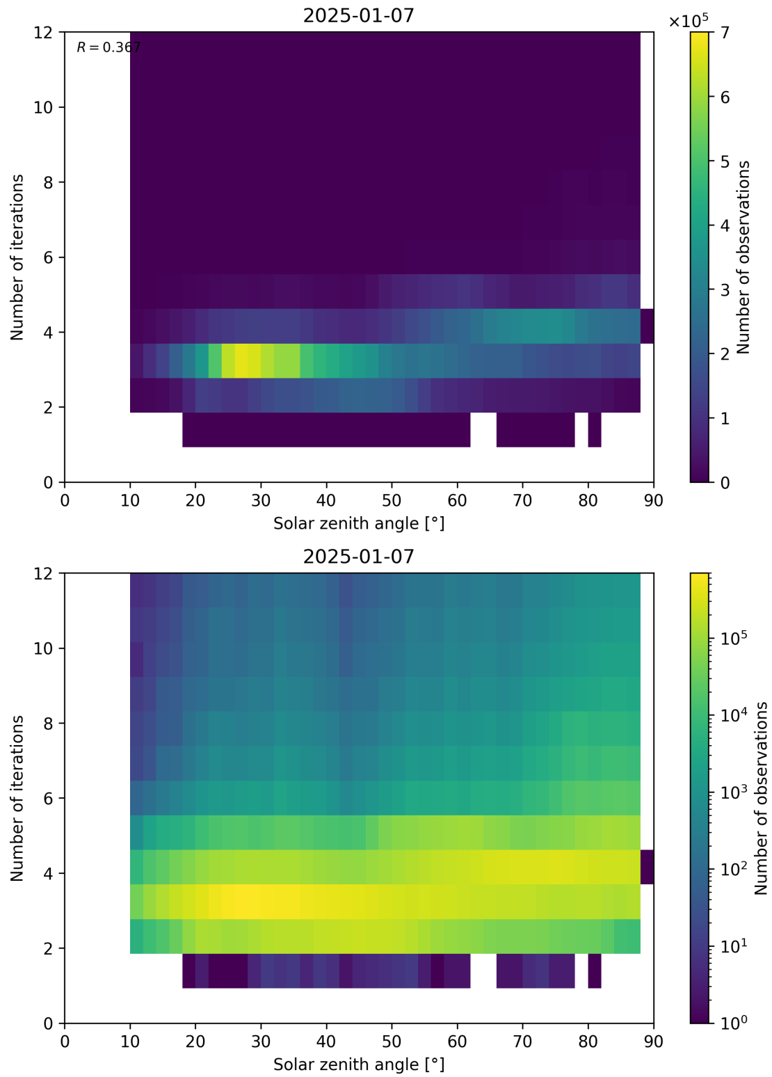
Figure 114: Scatter density plot of “Solar zenith angle” against “Number of iterations” for 2025-01-07 to 2025-01-08.
