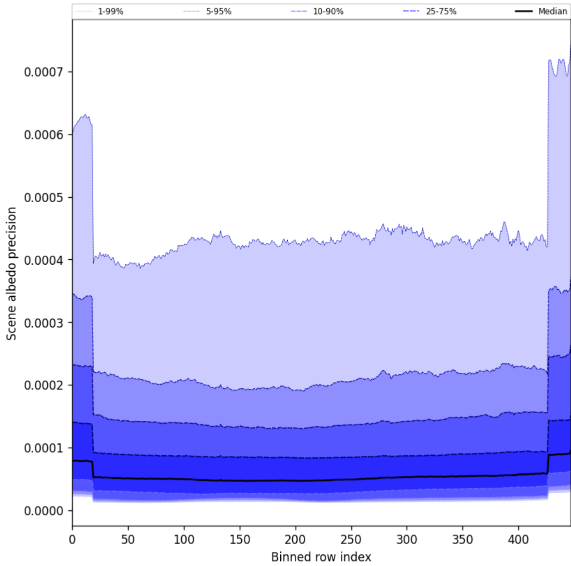
Figure 52: Along track statistics of “Scene albedo precision” for 2025-01-07 to 2025-01-08
