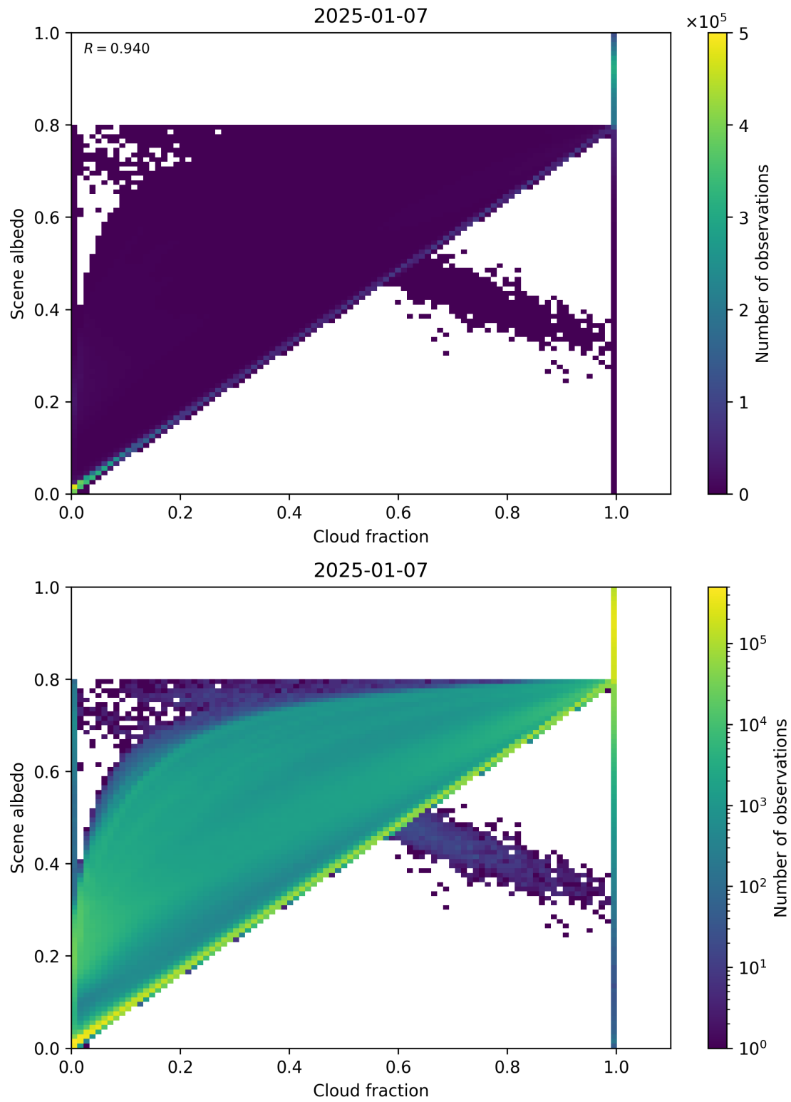
Figure 75: Scatter density plot of “Cloud fraction” against “Scene albedo” for 2025-01-07 to 2025-01-08.
