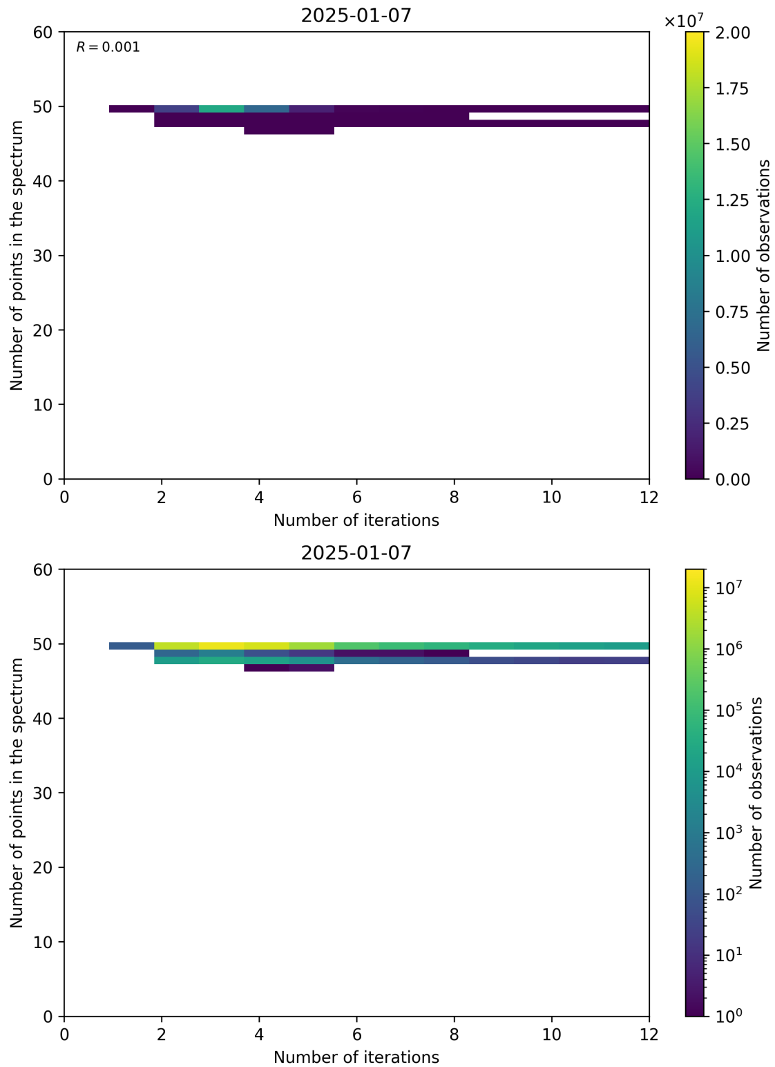
Figure 99: Scatter density plot of “Number of iterations” against “Number of points in the spectrum” for 2025-01-07 to 2025-01-08.
