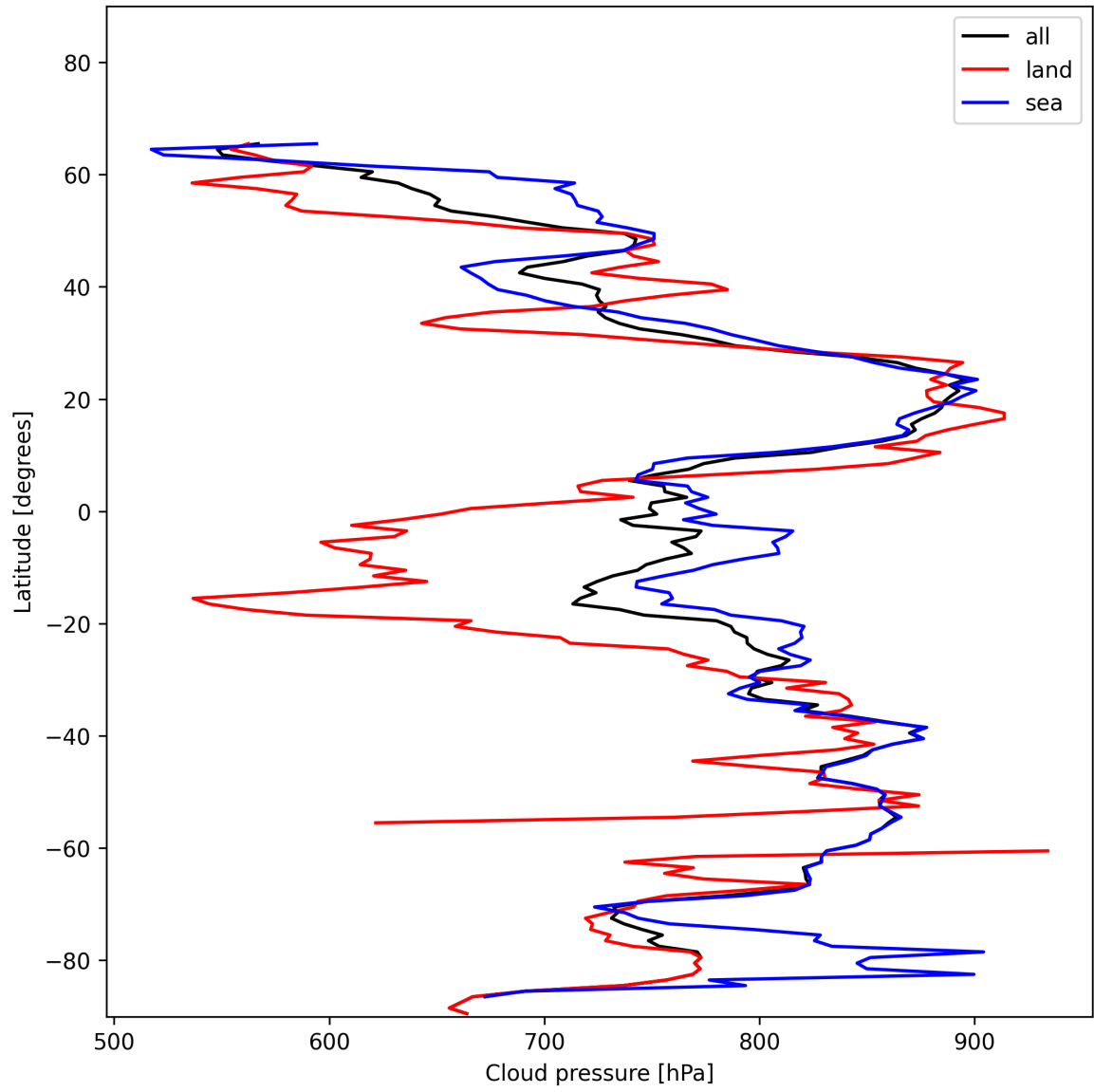
Figure 13: Zonal average of “Cloud pressure” for 2025-01-07 to 2025-01-08.
