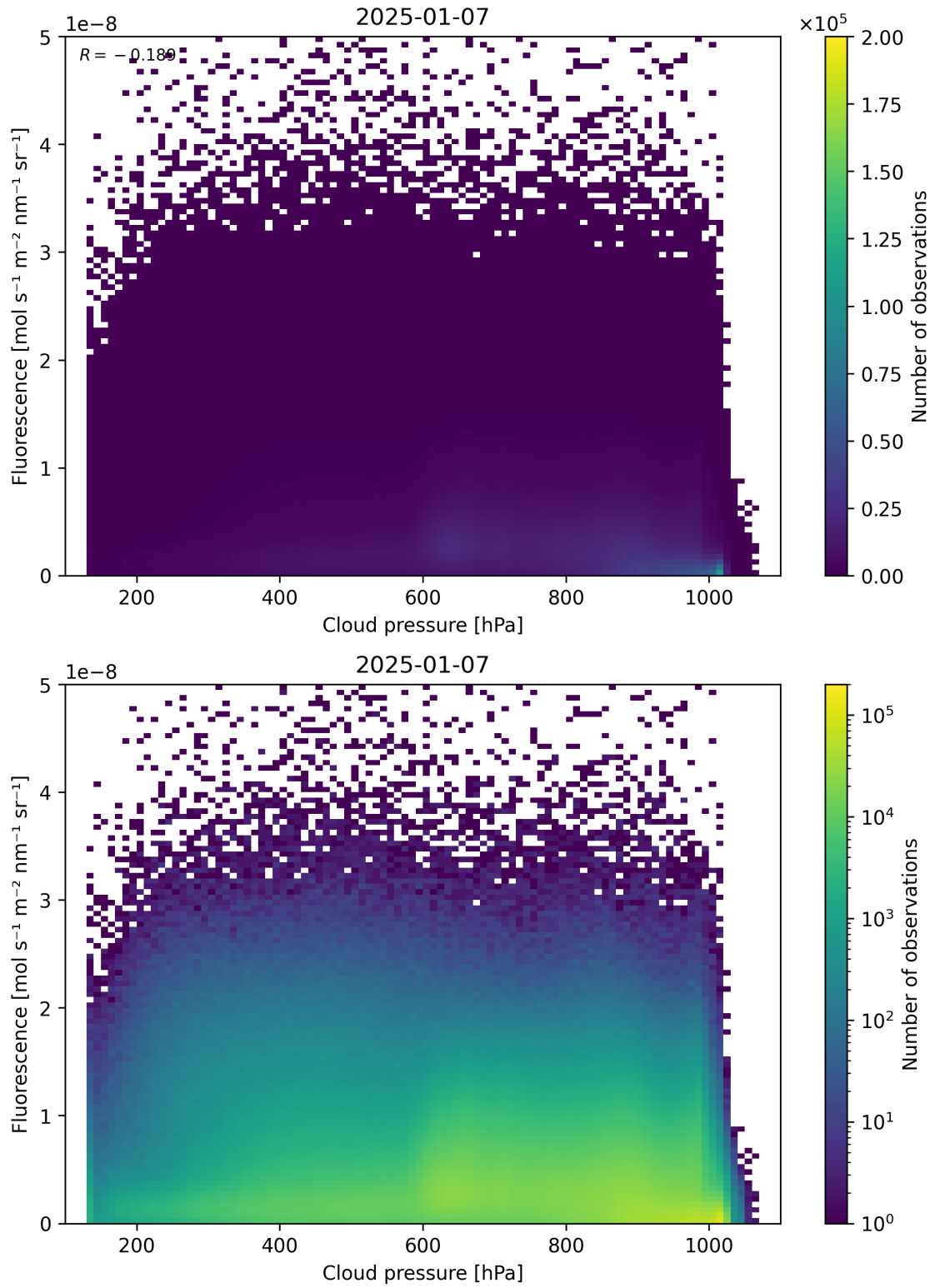
Figure 80: Scatter density plot of “Cloud pressure” against “Fluorescence” for 2025-01-07 to 2025-01-08.
