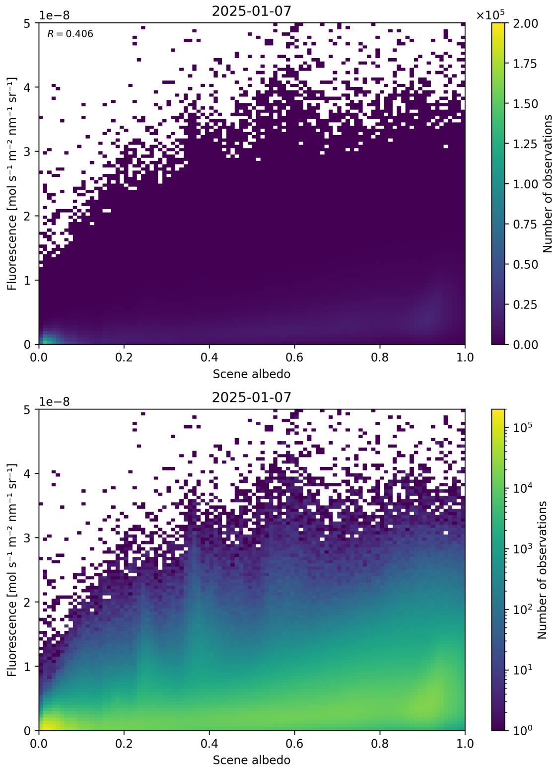
Figure 104: Scatter density plot of “Scene albedo” against “Fluorescence” for 2025-01-07 to 2025-01-08.
