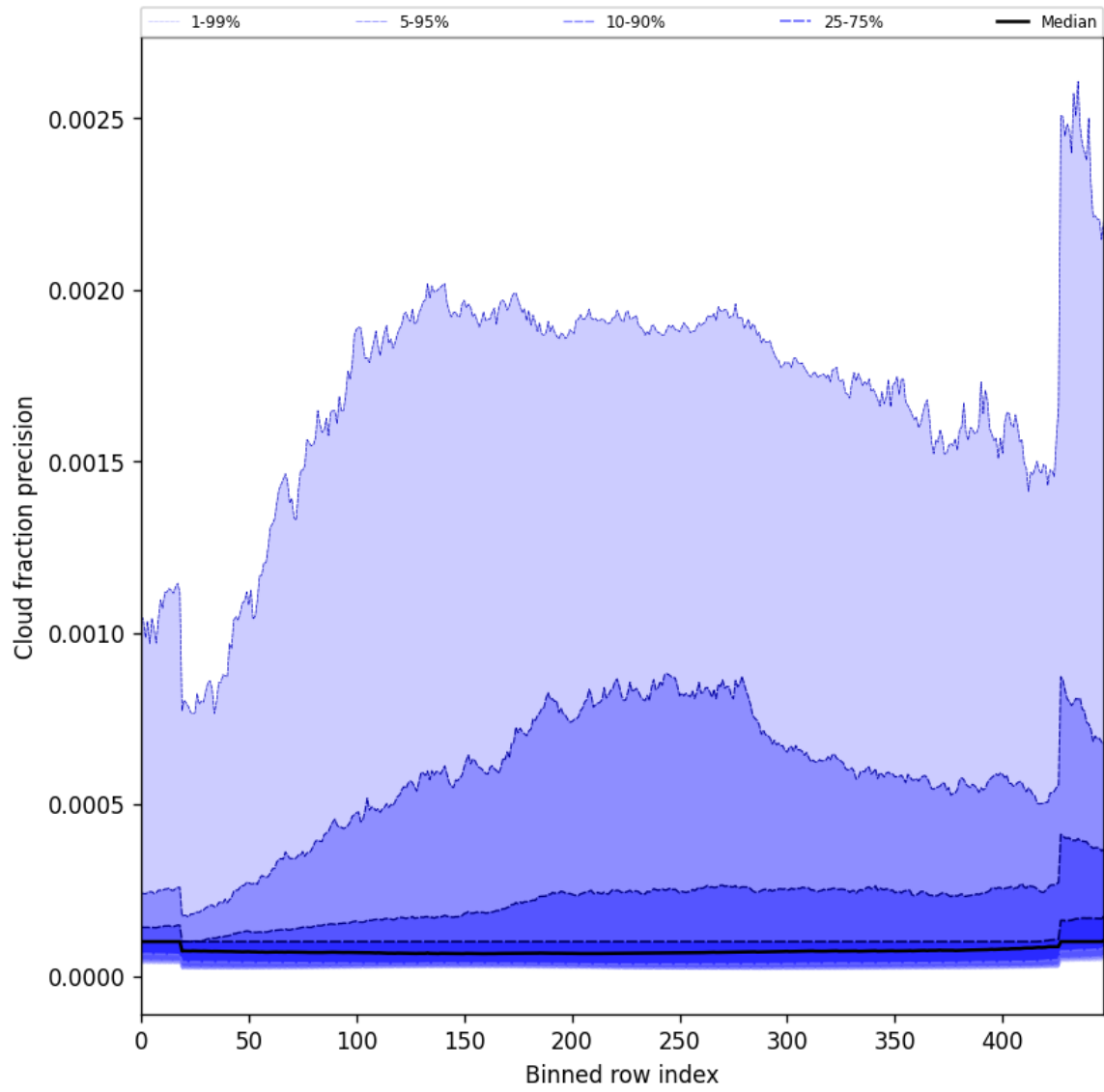
Figure 50: Along track statistics of “Cloud fraction precision” for 2025-01-07 to 2025-01-08
