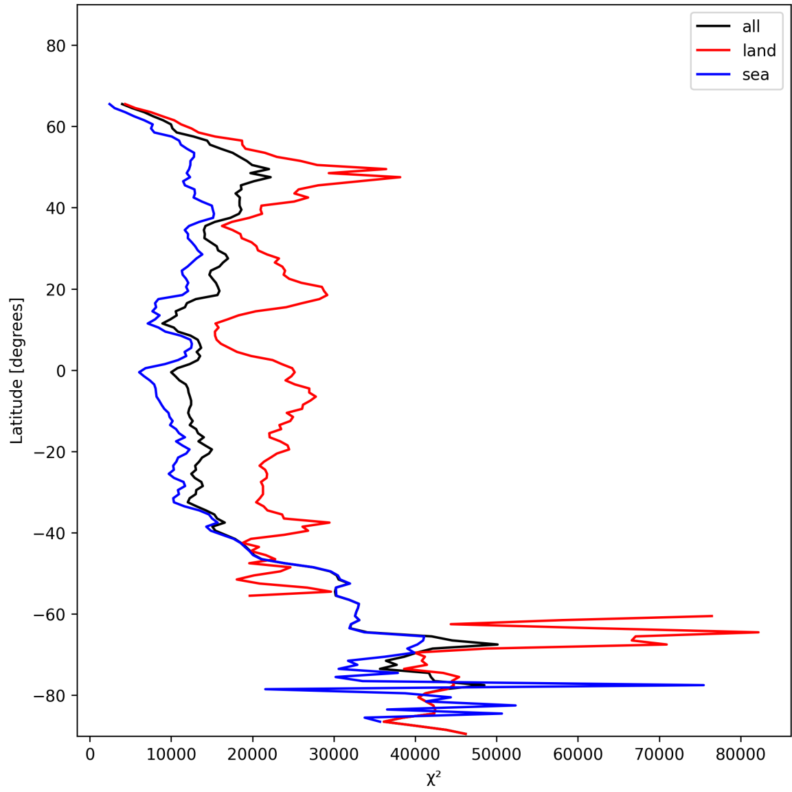
Figure 21: Zonal average of “ \chi^2 ” for 2025-01-07 to 2025-01-08.
