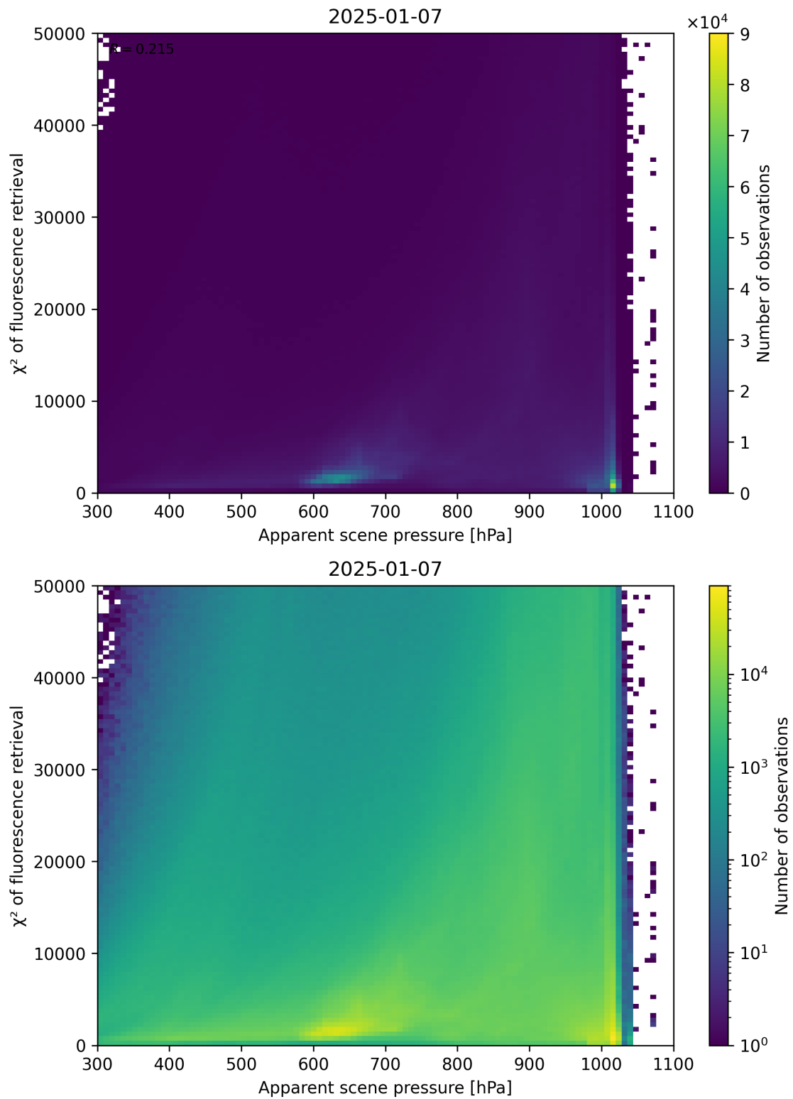
Figure 63: Scatter density plot of “Apparent scene pressure” against “ \chi^2 of fluorescence retrieval” for 2025-01-07 to 2025-01-08.
