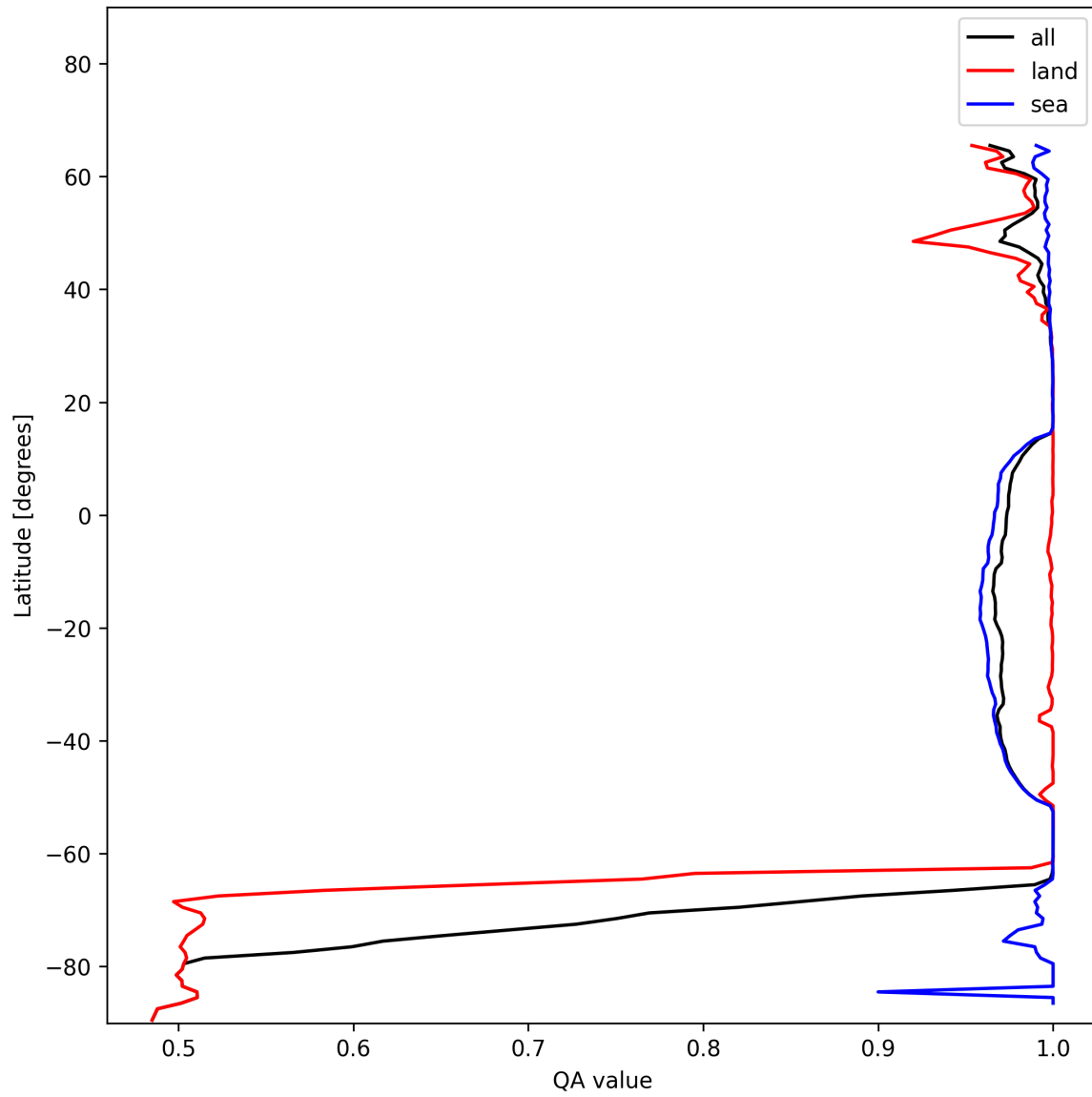
Figure 12: Zonal average of “QA value” for 2025-01-07 to 2025-01-08.
