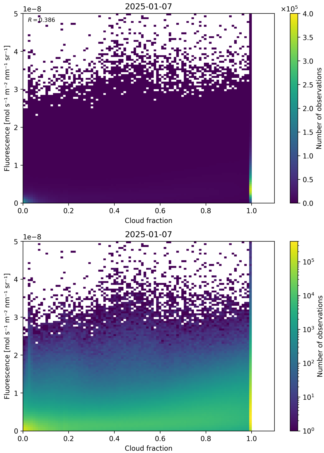
Figure 72: Scatter density plot of “Cloud fraction” against “Fluorescence” for 2025-01-07 to 2025-01-08.
