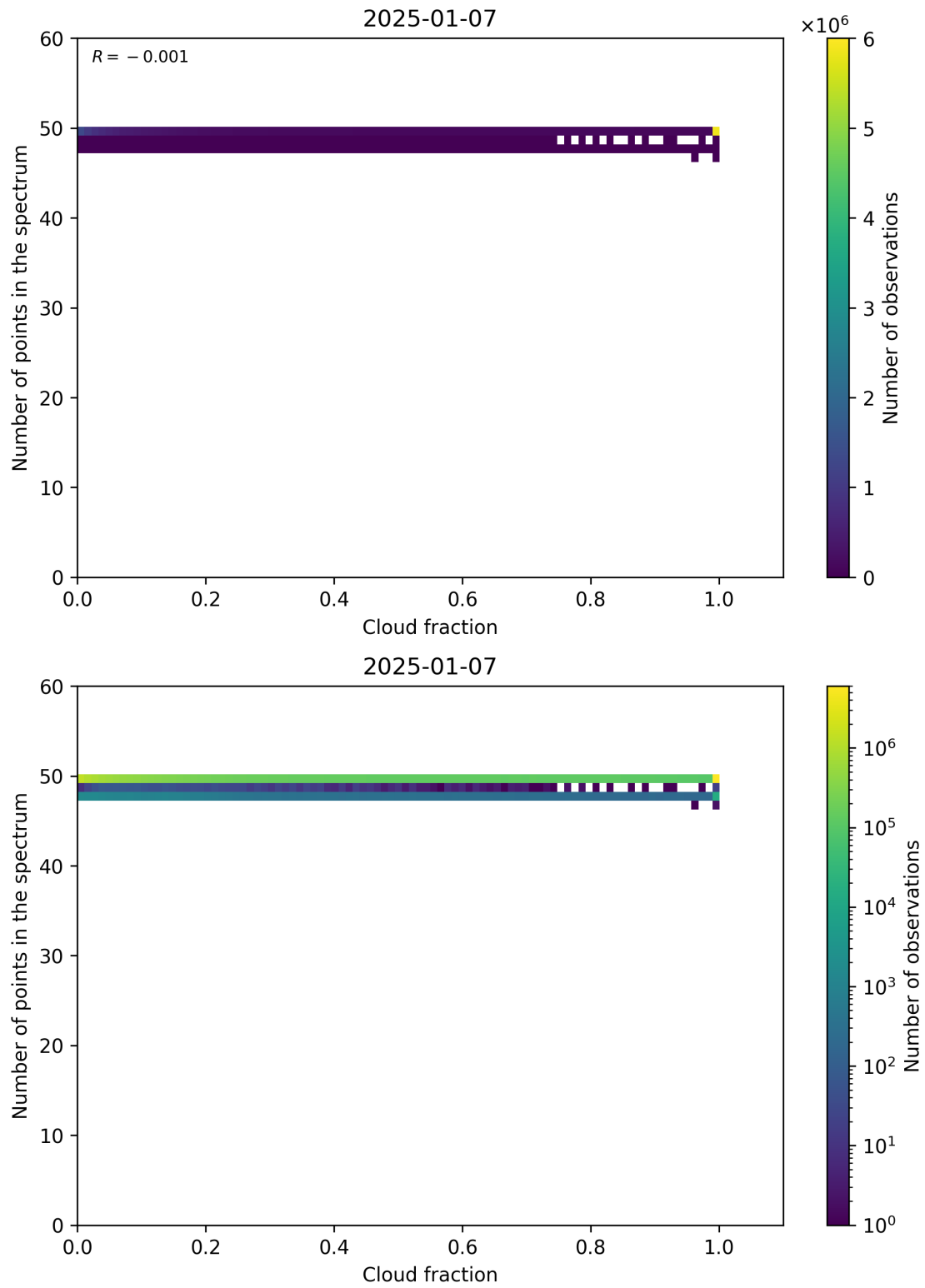
Figure 74: Scatter density plot of “Cloud fraction” against “Number of points in the spectrum” for 2025-01-07 to 2025-01-08.
