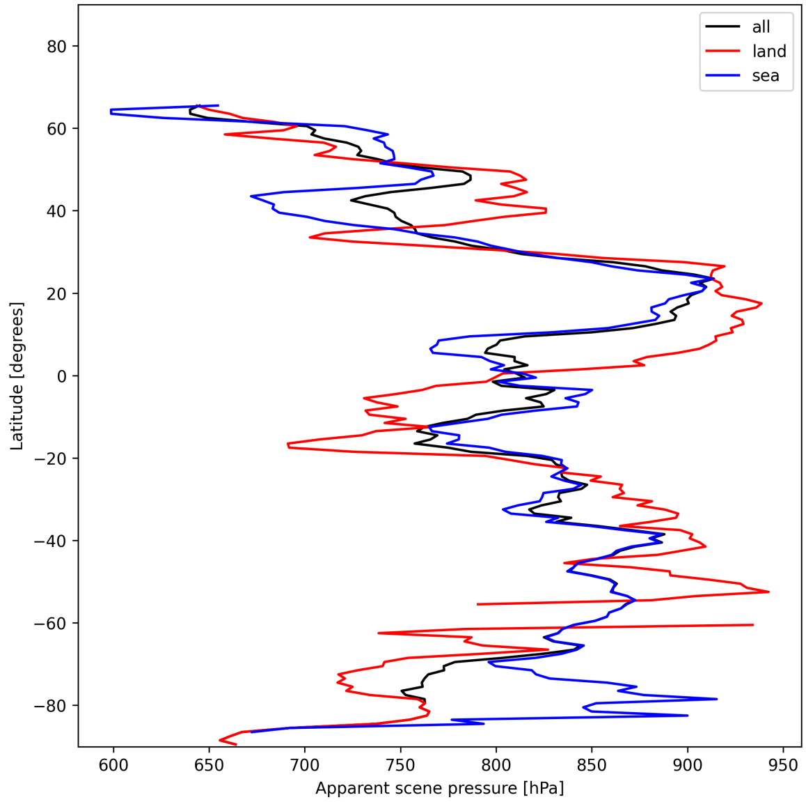
Figure 19: Zonal average of “Apparent scene pressure” for 2025-01-07 to 2025-01-08.
