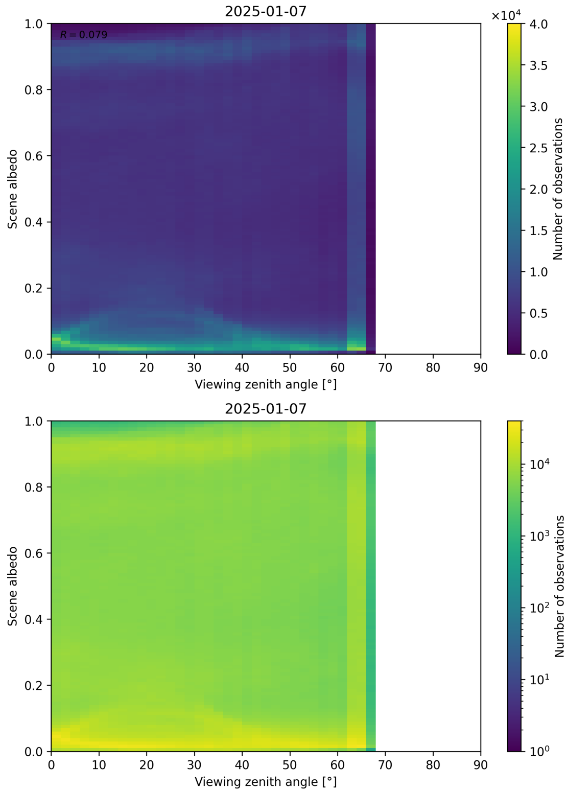
Figure 126: Scatter density plot of “Viewing zenith angle” against “Scene albedo” for 2025-01-07 to 2025-01-08.
