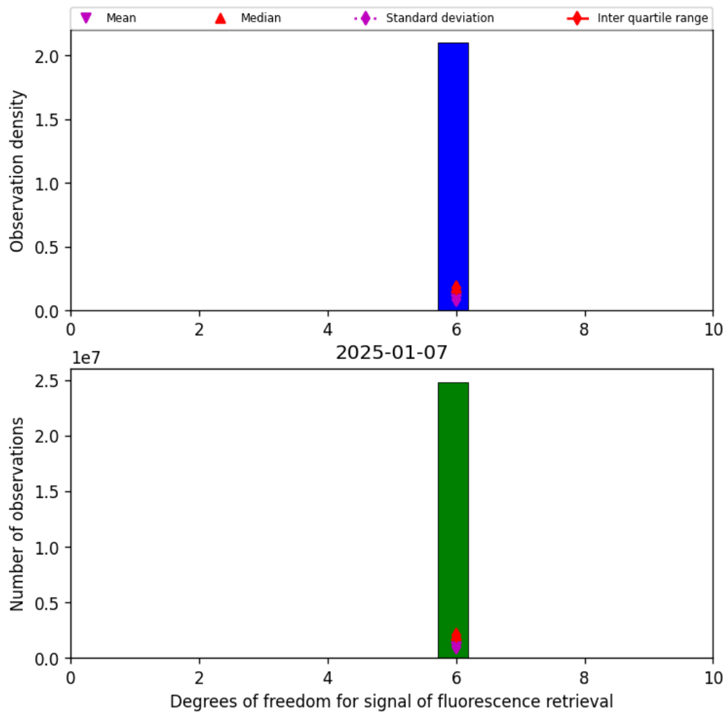
Figure 43: Histogram of “Degrees of freedom for signal of fluorescence retrieval” for 2025-01-07 to 2025-01-08
