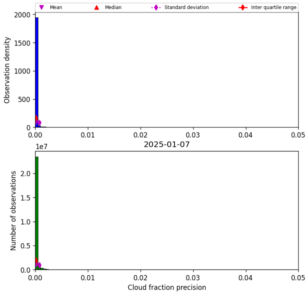
Figure 33: Histogram of “Cloud fraction precision” for 2025-01-07 to 2025-01-08
