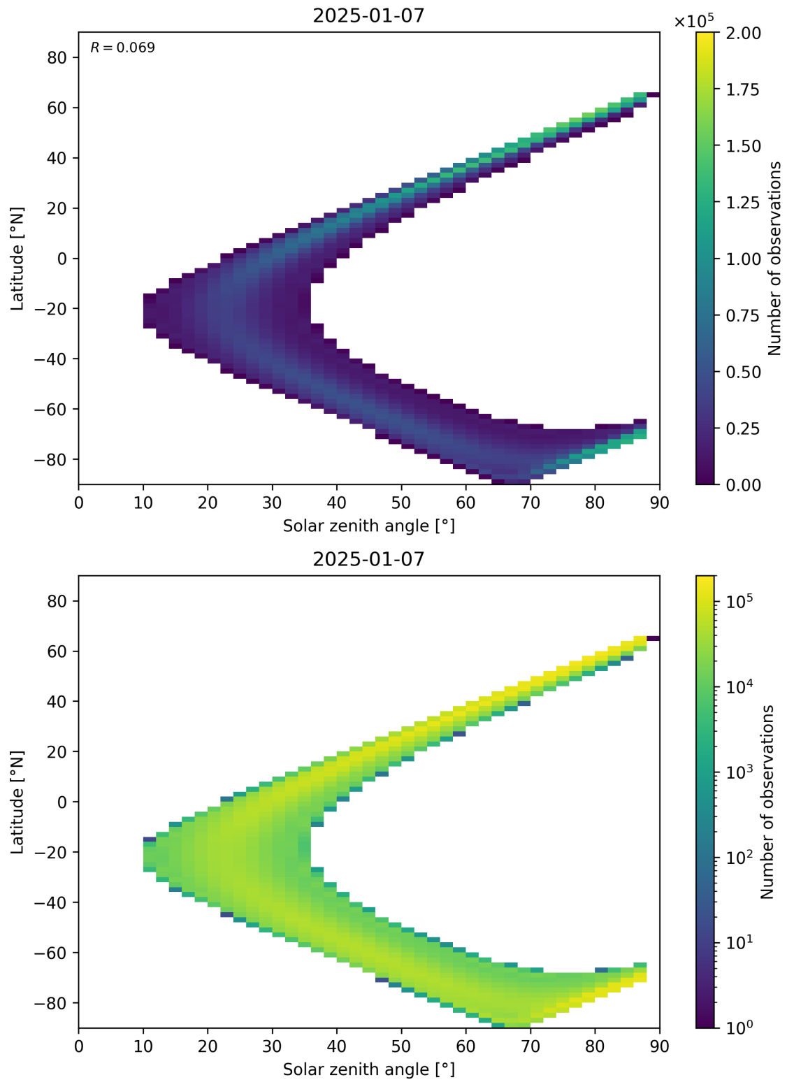
Figure 113: Scatter density plot of “Solar zenith angle” against “Latitude” for 2025-01-07 to 2025-01-08.
