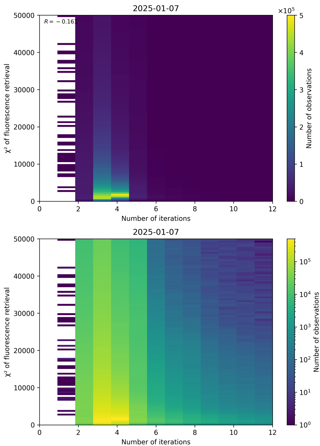
Figure 97: Scatter density plot of “Number of iterations” against “ \chi^2 of fluorescence retrieval” for 2025-01-07 to 2025-01-08.
