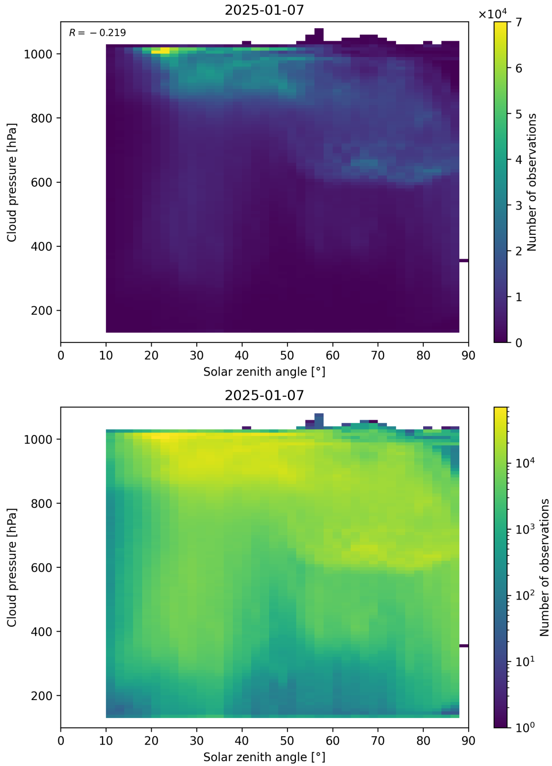
Figure 111: Scatter density plot of “Solar zenith angle” against “Cloud pressure” for 2025-01-07 to 2025-01-08.
