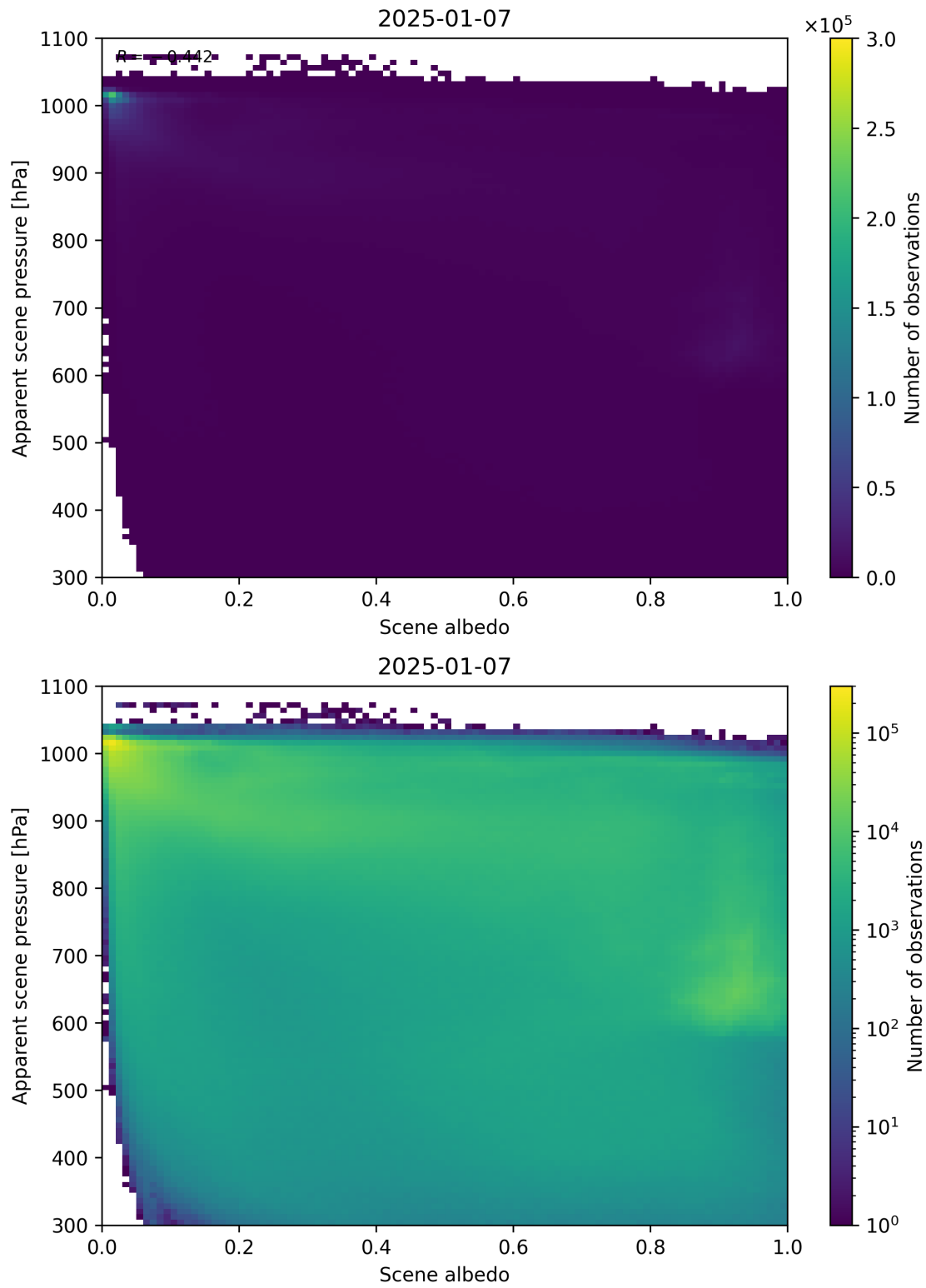
Figure 102: Scatter density plot of “Scene albedo” against “Apparent scene pressure” for 2025-01-07 to 2025-01-08.
