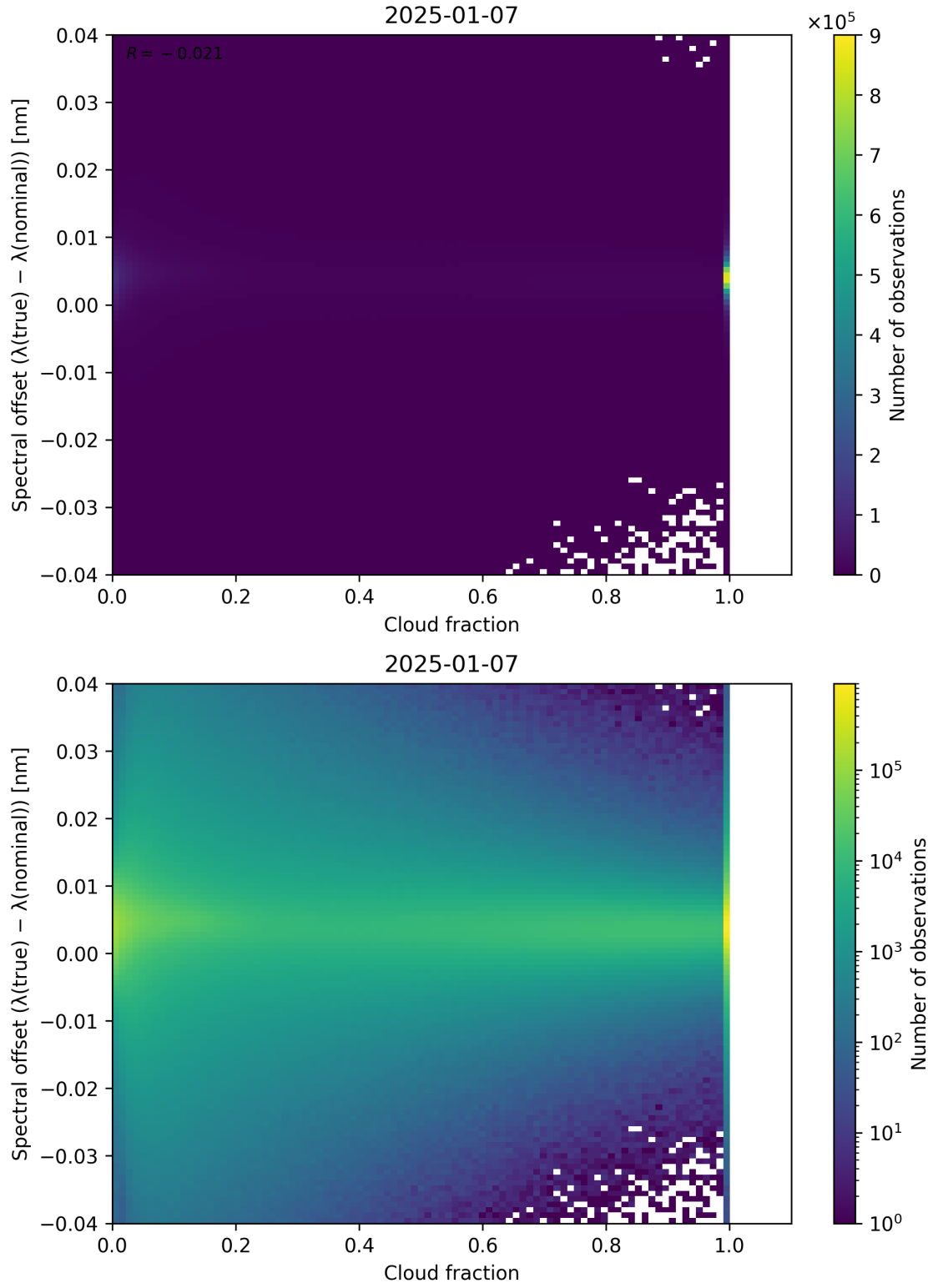
Figure 76: Scatter density plot of “Cloud fraction” against “Spectral offset ( \lambda_{\text{true}} - \lambda_{\text{nominal}} )” for 2025-01-07 to 2025-01-08.
