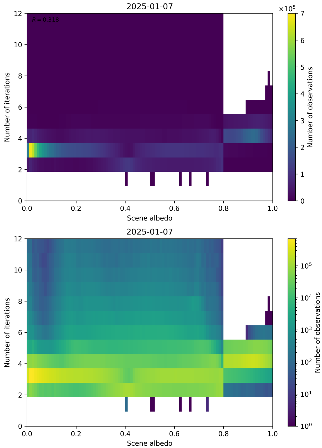
Figure 105: Scatter density plot of “Scene albedo” against “Number of iterations” for 2025-01-07 to 2025-01-08.
