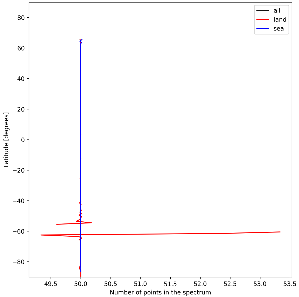
Figure 27: Zonal average of “Number of points in the spectrum” for 2025-01-07 to 2025-01-08.
