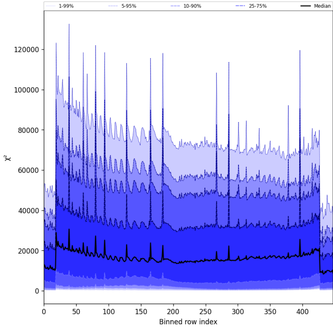
Figure 55: Along track statistics of “ \chi^2 ” for 2025-01-07 to 2025-01-08
