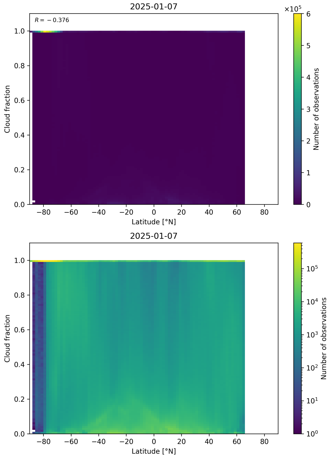
Figure 90: Scatter density plot of “Latitude” against “Cloud fraction” for 2025-01-07 to 2025-01-08.
