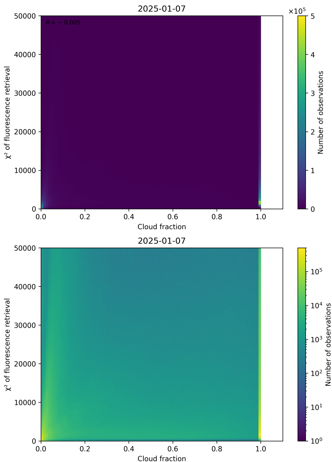
Figure 71: Scatter density plot of “Cloud fraction” against “ \chi^2 of fluorescence retrieval” for 2025-01-07 to 2025-01-08.
