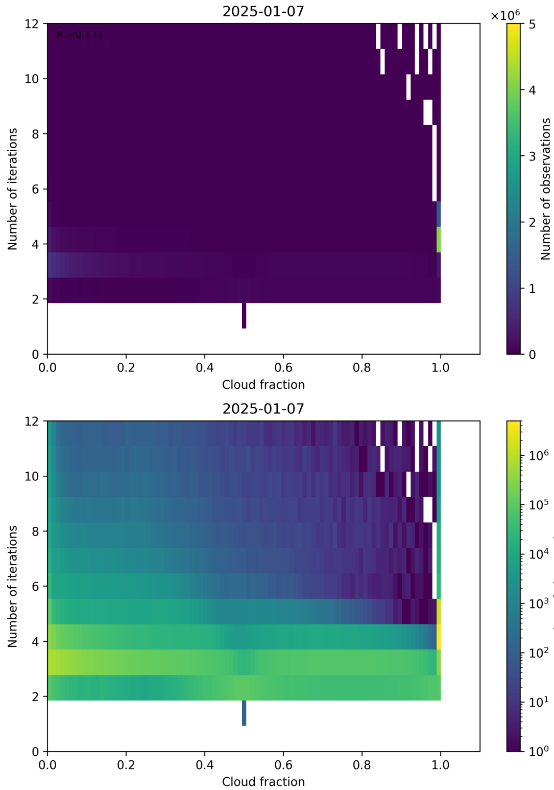
Figure 73: Scatter density plot of “Cloud fraction” against “Number of iterations” for 2025-01-07 to 2025-01-08.
