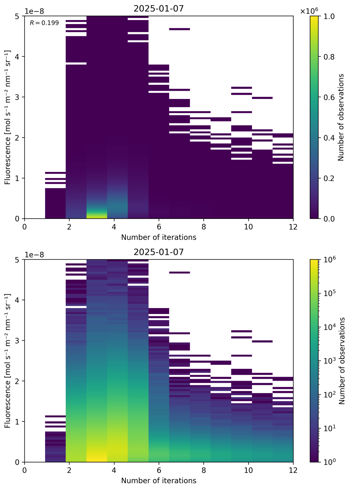
Figure 98: Scatter density plot of “Number of iterations” against “Fluorescence” for 2025-01-07 to 2025-01-08.
