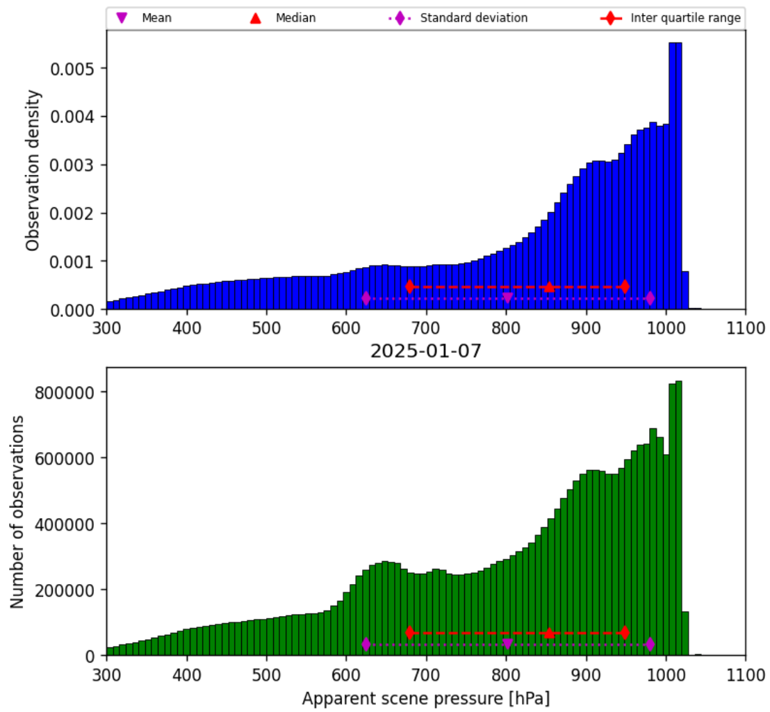
Figure 36: Histogram of “Apparent scene pressure” for 2025-01-07 to 2025-01-08
