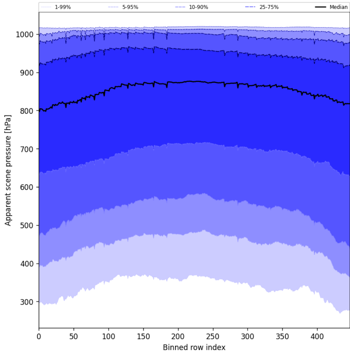
Figure 53: Along track statistics of “Apparent scene pressure” for 2025-01-07 to 2025-01-08
