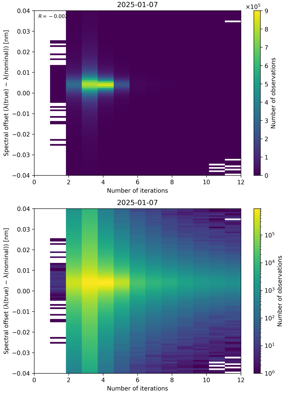
Figure 100: Scatter density plot of “Number of iterations” against “Spectral offset ( \lambda_{\text{true}} - \lambda_{\text{nominal}} )” for 2025-01-07 to 2025-01-08.
