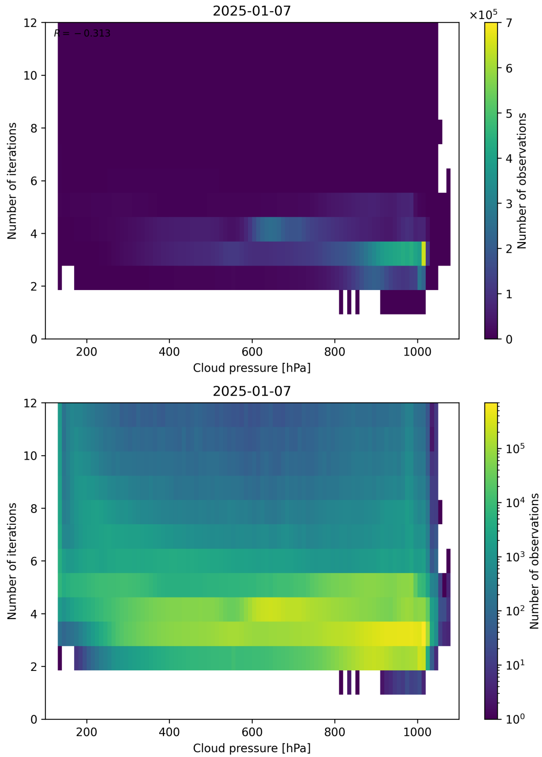
Figure 81: Scatter density plot of “Cloud pressure” against “Number of iterations” for 2025-01-07 to 2025-01-08.
