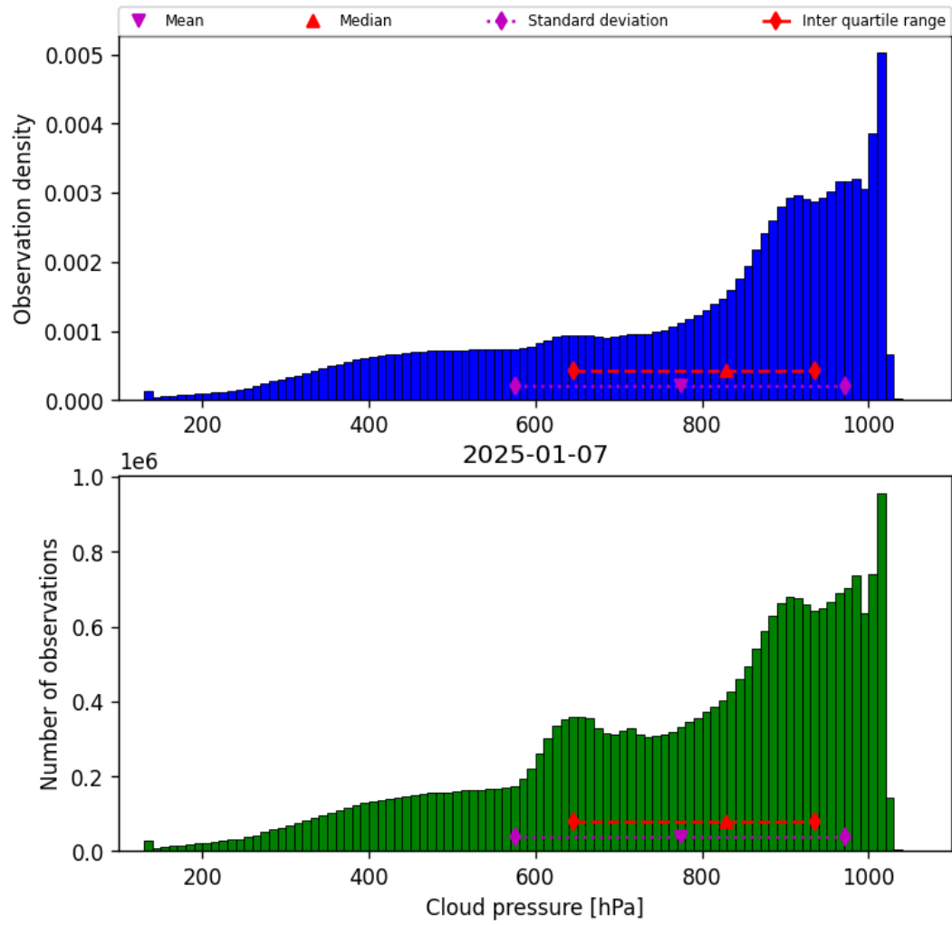
Figure 30: Histogram of “Cloud pressure” for 2025-01-07 to 2025-01-08
