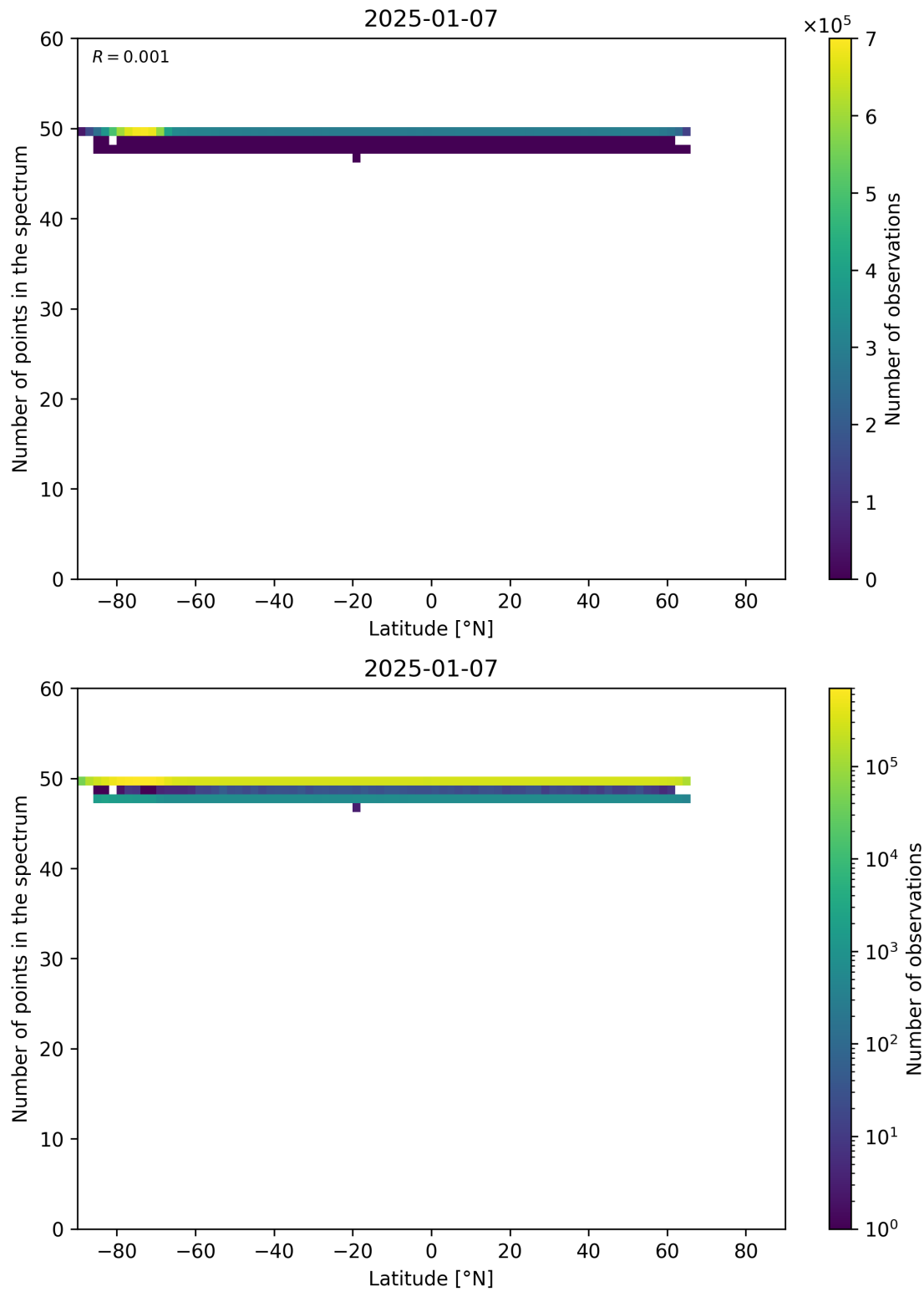
Figure 94: Scatter density plot of “Latitude” against “Number of points in the spectrum” for 2025-01-07 to 2025-01-08.
