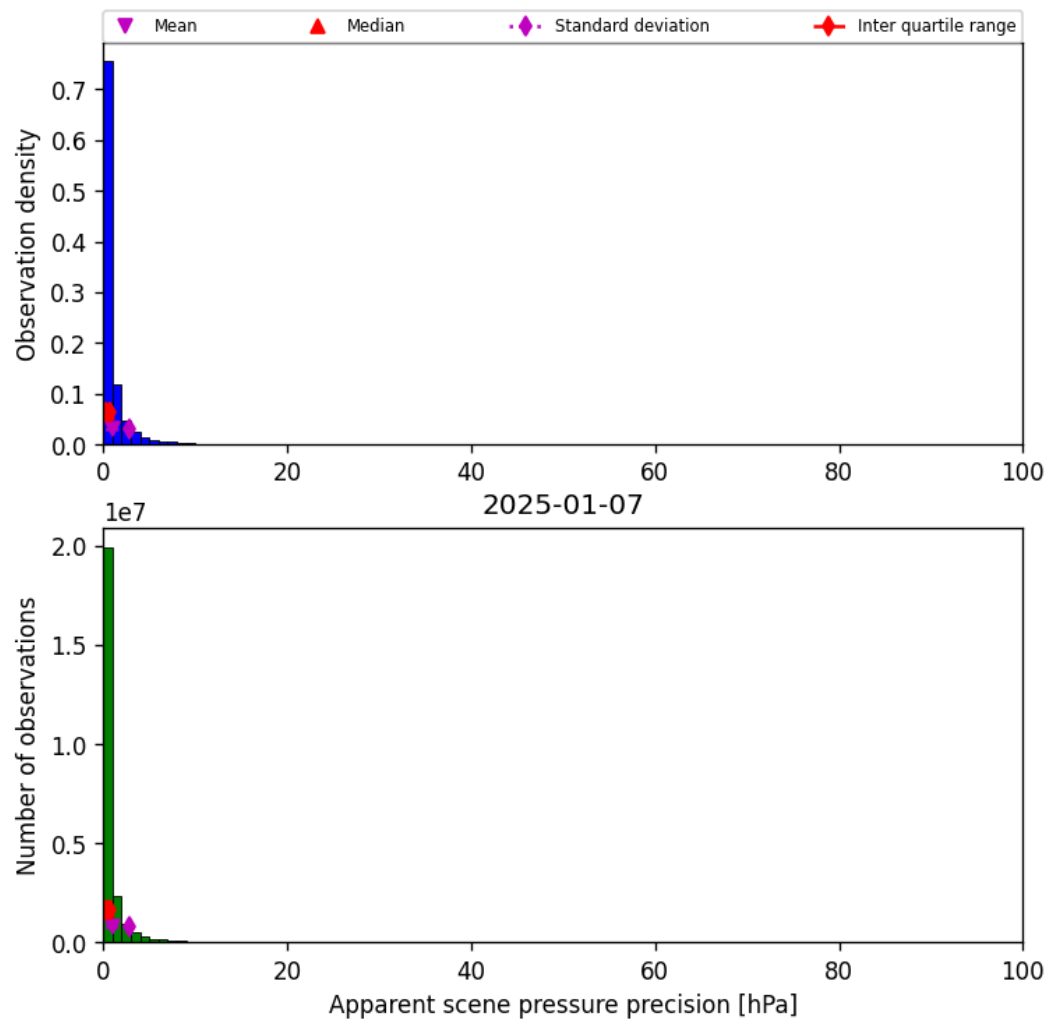
Figure 37: Histogram of “Apparent scene pressure precision” for 2025-01-07 to 2025-01-08
