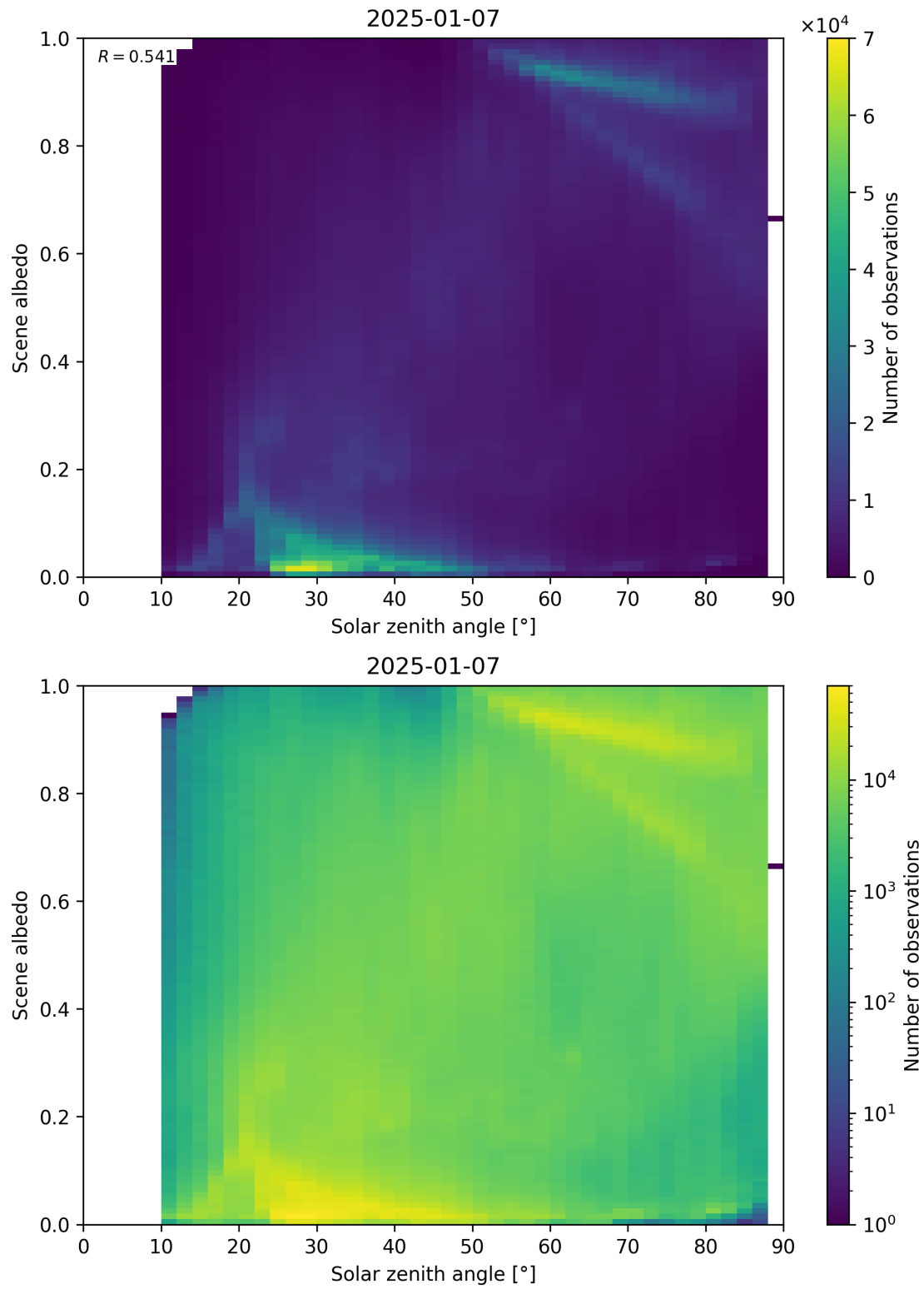
Figure 116: Scatter density plot of “Solar zenith angle” against “Scene albedo” for 2025-01-07 to 2025-01-08.
