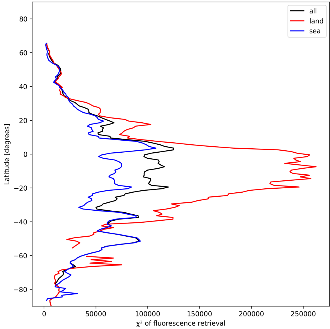
Figure 25: Zonal average of “ \chi^2 of fluorescence retrieval” for 2025-01-07 to 2025-01-08.
