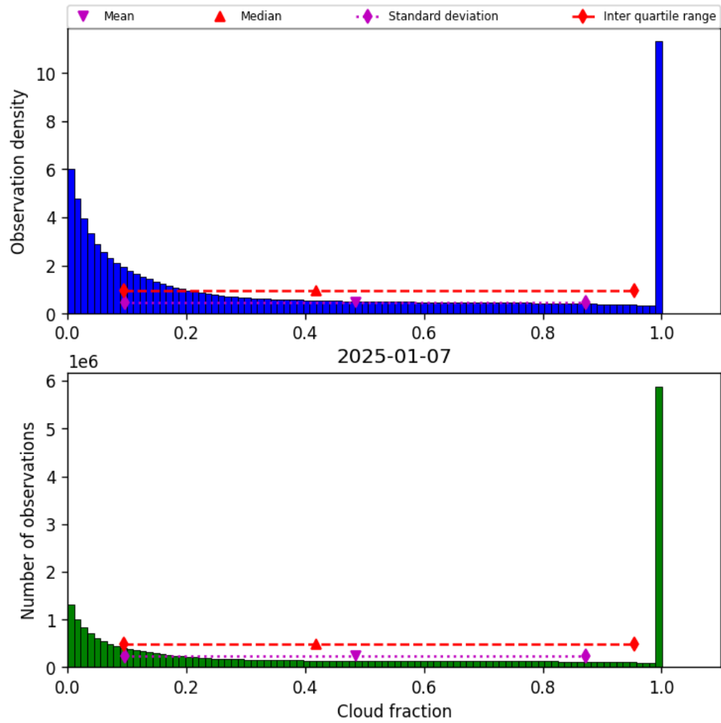
Figure 32: Histogram of “Cloud fraction” for 2025-01-07 to 2025-01-08
