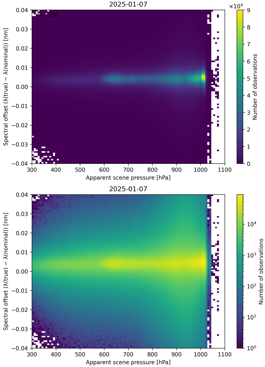
Figure 67: Scatter density plot of “Apparent scene pressure” against “Spectral offset ( \lambda_{\text{true}} - \lambda_{\text{nominal}} )” for 2025-01-07 to 2025-01-08.
