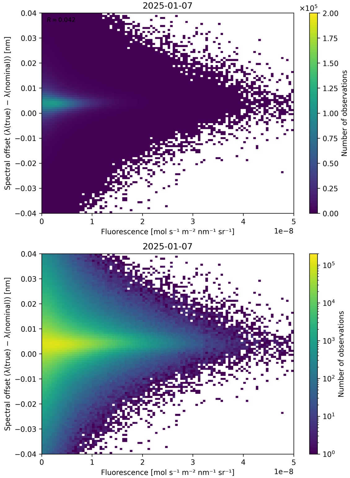
Figure 87: Scatter density plot of “Fluorescence” against “Spectral offset ( \lambda_{\text{true}} - \lambda_{\text{nominal}} )” for 2025-01-07 to 2025-01-08.
