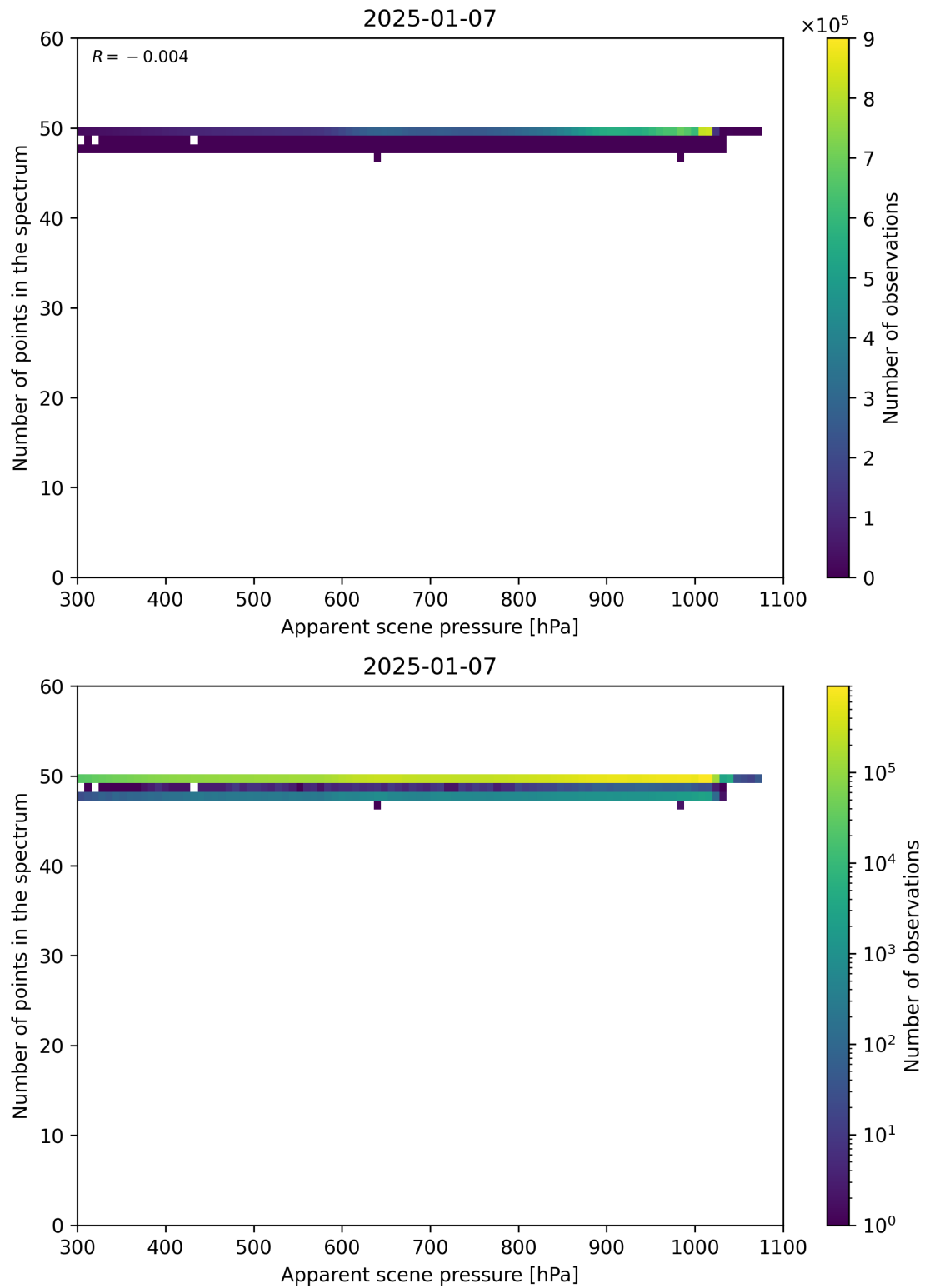
Figure 66: Scatter density plot of “Apparent scene pressure” against “Number of points in the spectrum” for 2025-01-07 to 2025-01-08.
