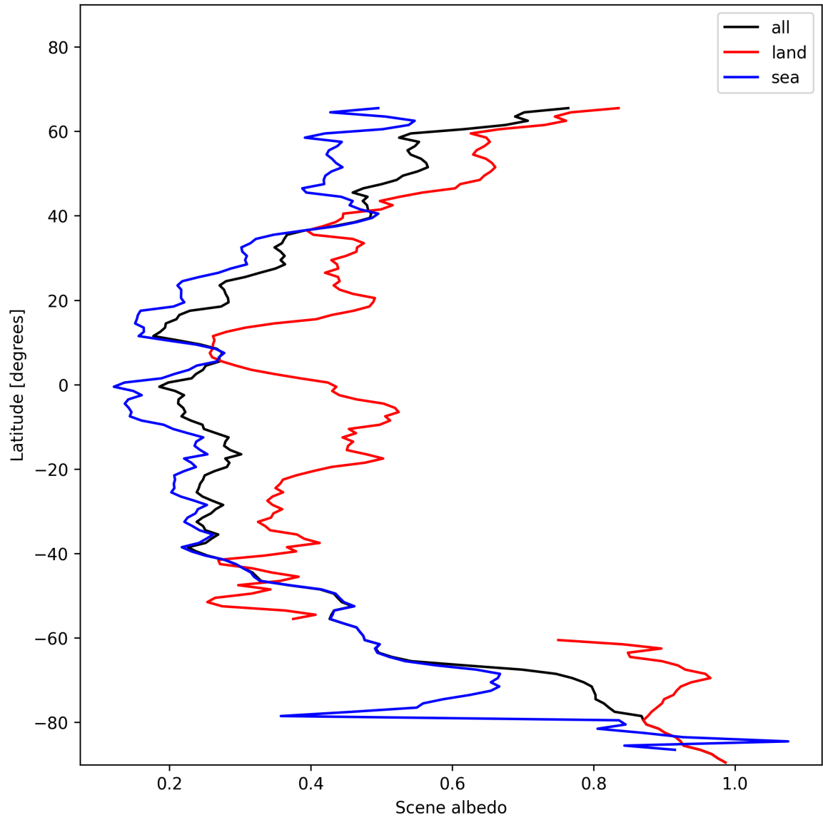
Figure 17: Zonal average of “Scene albedo” for 2025-01-07 to 2025-01-08.
