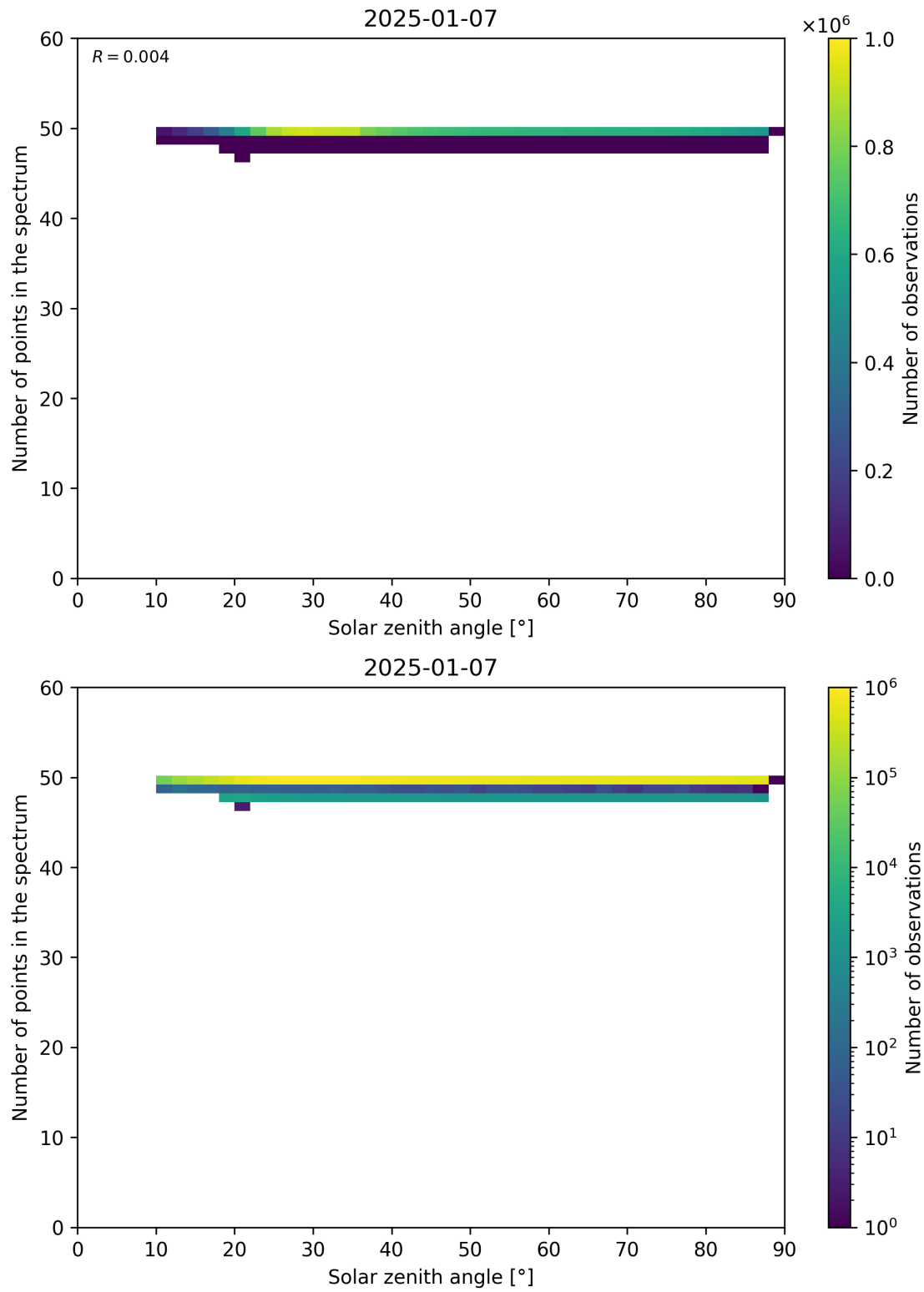
Figure 115: Scatter density plot of “Solar zenith angle” against “Number of points in the spectrum” for 2025-01-07 to 2025-01-08.
