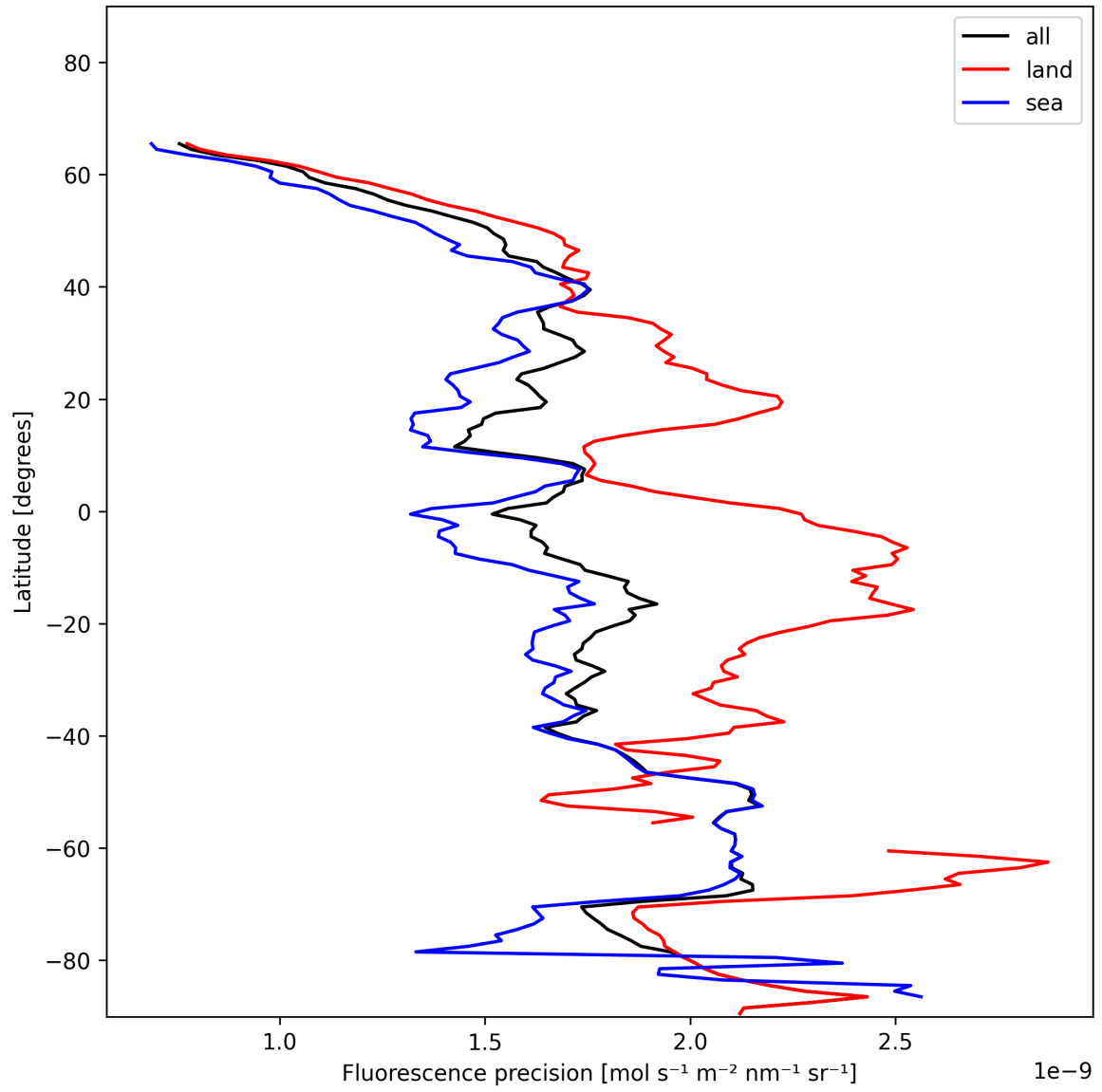
Figure 24: Zonal average of “Fluorescence precision” for 2025-01-07 to 2025-01-08.
