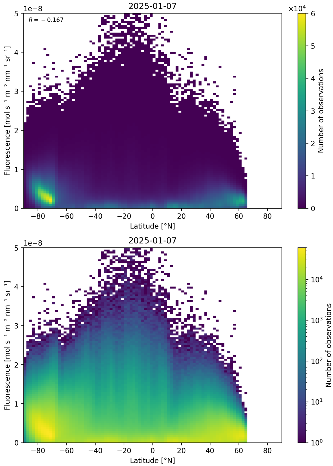
Figure 92: Scatter density plot of “Latitude” against “Fluorescence” for 2025-01-07 to 2025-01-08.
