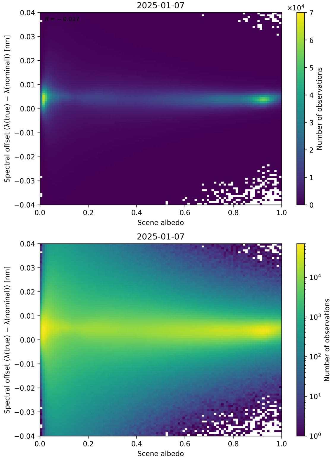
Figure 107: Scatter density plot of “Scene albedo” against “Spectral offset ( \lambda_{\text{true}} - \lambda_{\text{nominal}} )” for 2025-01-07 to 2025-01-08.
