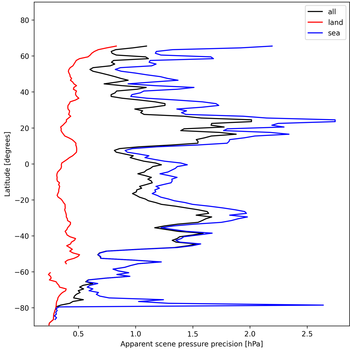
Figure 20: Zonal average of “Apparent scene pressure precision” for 2025-01-07 to 2025-01-08.
