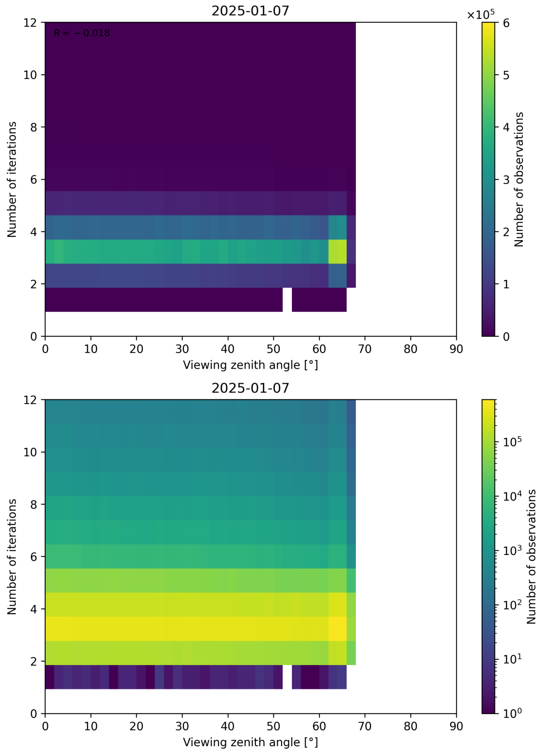
Figure 124: Scatter density plot of “Viewing zenith angle” against “Number of iterations” for 2025-01-07 to 2025-01-08.
