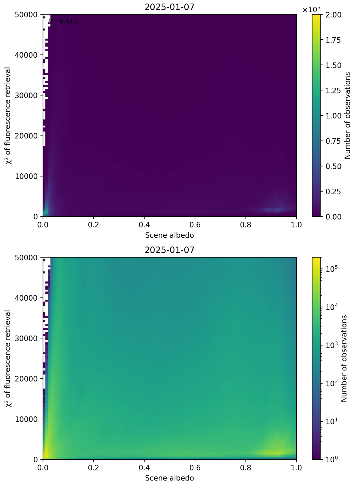
Figure 103: Scatter density plot of “Scene albedo” against “ \chi^2 of fluorescence retrieval” for 2025-01-07 to 2025-01-08.
