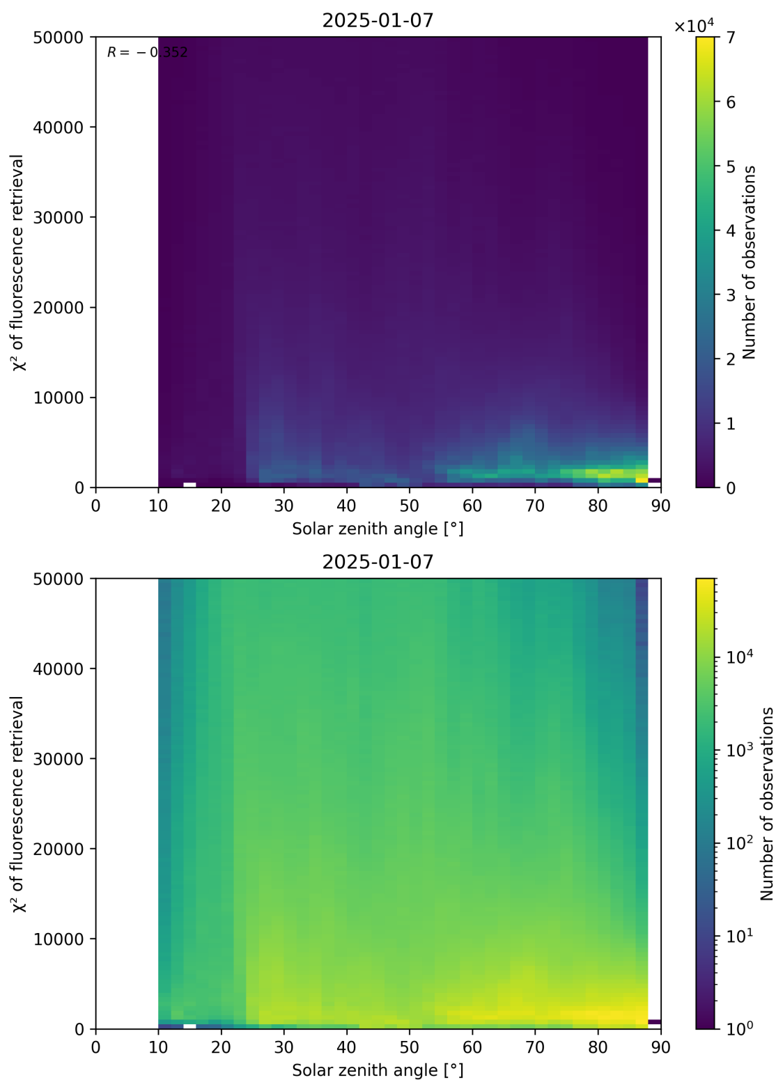
Figure 109: Scatter density plot of “Solar zenith angle” against “ \chi^2 of fluorescence retrieval” for 2025-01-07 to 2025-01-08.
