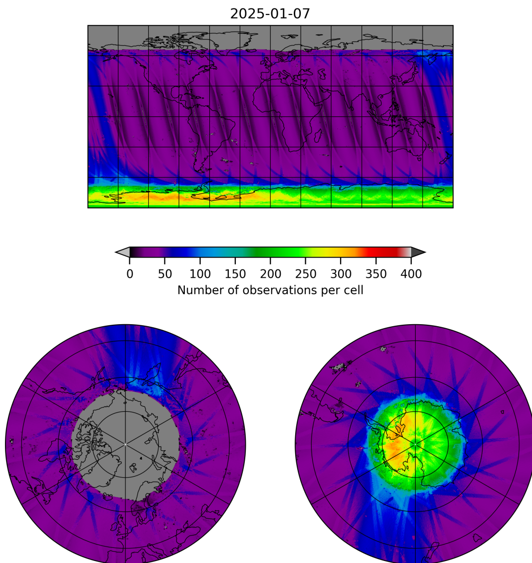
Figure 11: Map of the number of observations for 2025-01-07 to 2025-01-08
