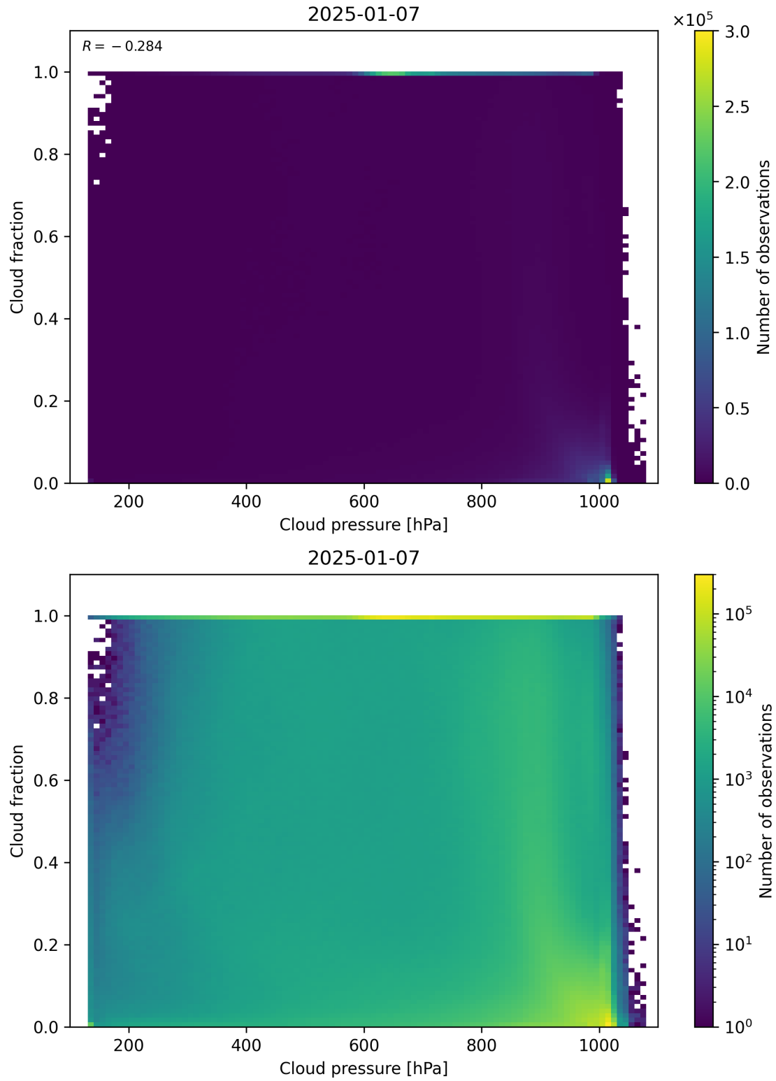
Figure 79: Scatter density plot of “Cloud pressure” against “Cloud fraction” for 2025-01-07 to 2025-01-08.
