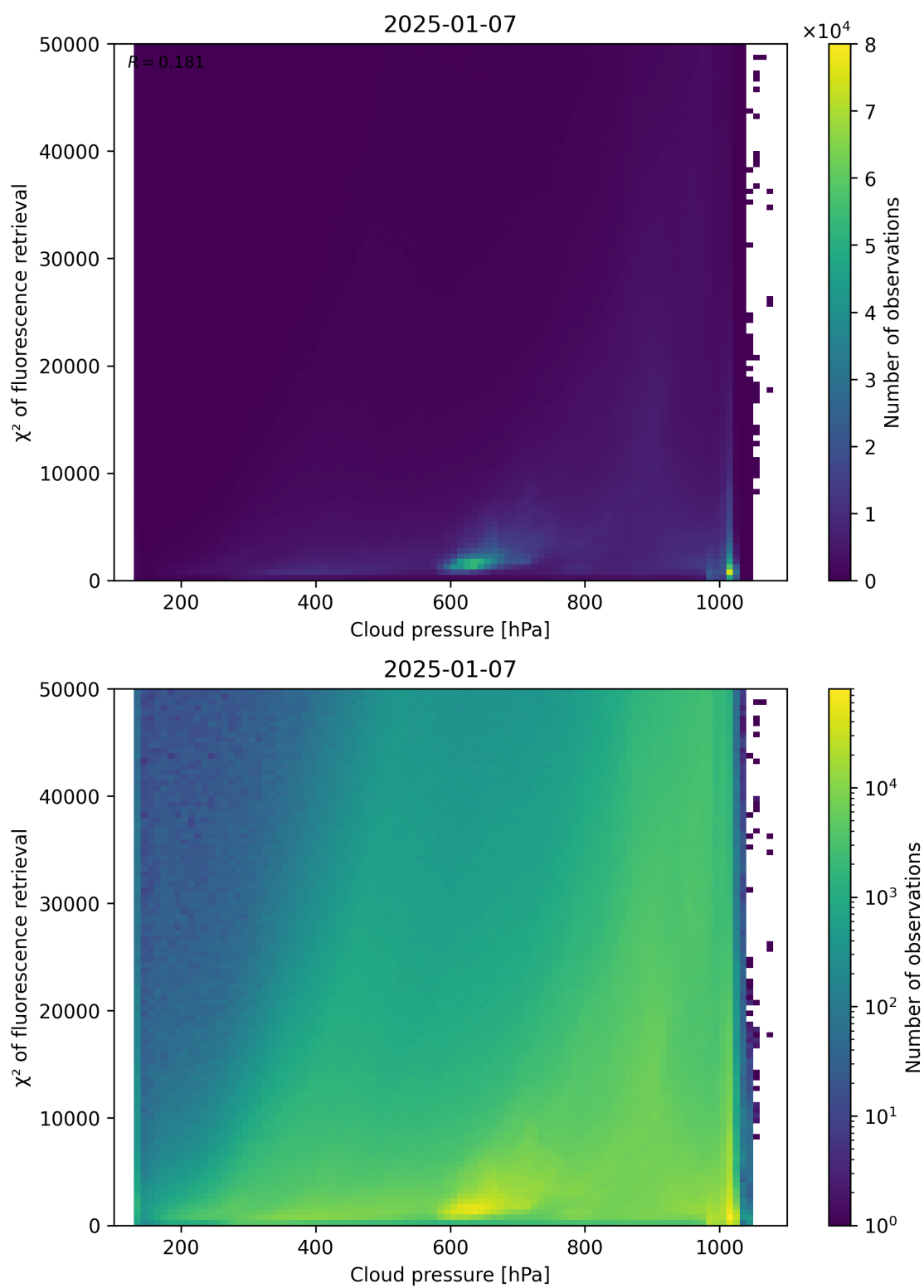
Figure 78: Scatter density plot of “Cloud pressure” against “ \chi^2 of fluorescence retrieval” for 2025-01-07 to 2025-01-08.
