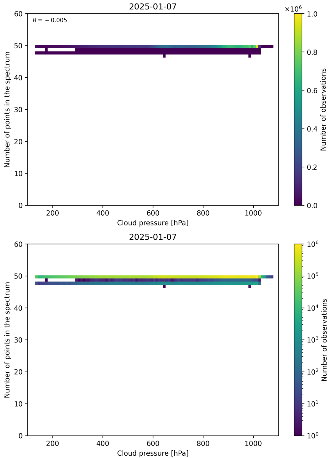
Figure 82: Scatter density plot of “Cloud pressure” against “Number of points in the spectrum” for 2025-01-07 to 2025-01-08.
