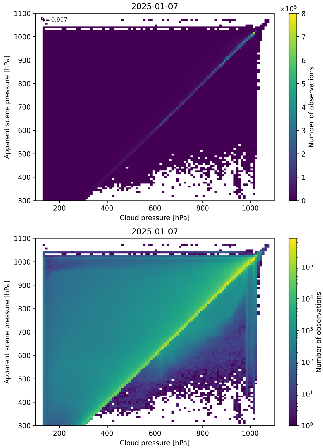
Figure 77: Scatter density plot of “Cloud pressure” against “Apparent scene pressure” for 2025-01-07 to 2025-01-08.
