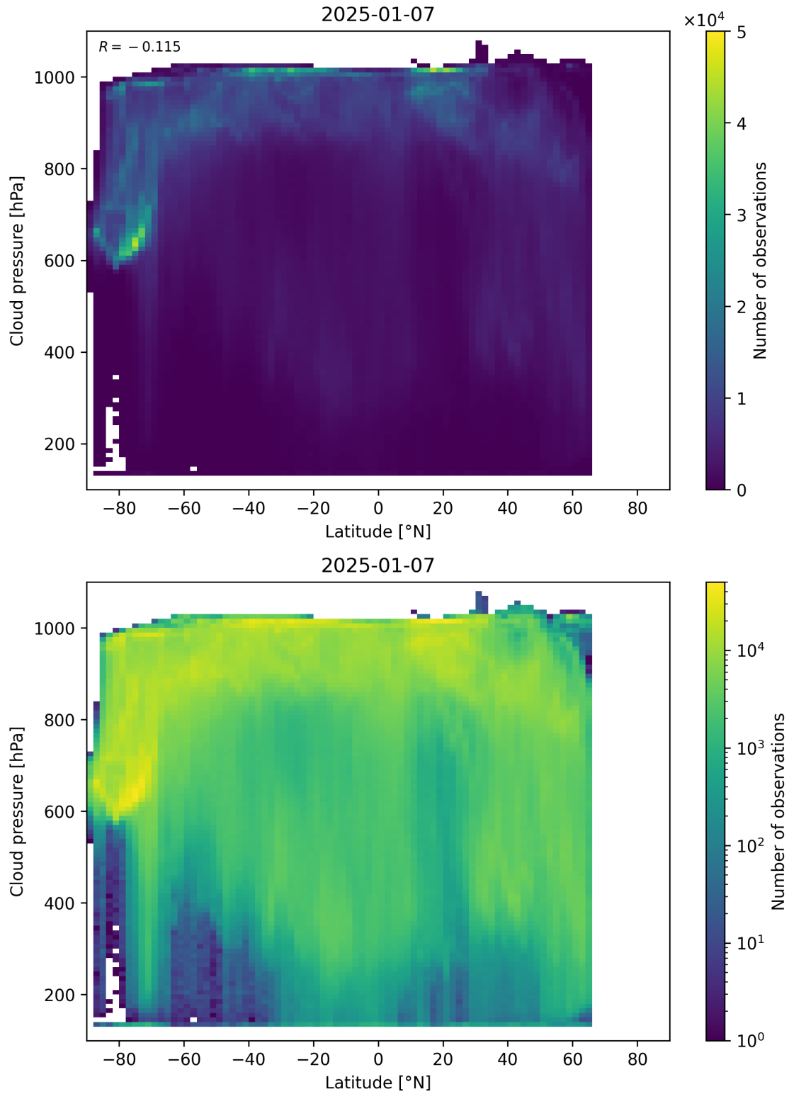
Figure 91: Scatter density plot of “Latitude” against “Cloud pressure” for 2025-01-07 to 2025-01-08.
