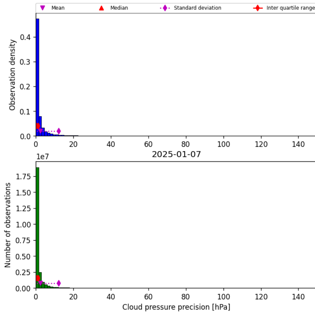
Figure 31: Histogram of “Cloud pressure precision” for 2025-01-07 to 2025-01-08
