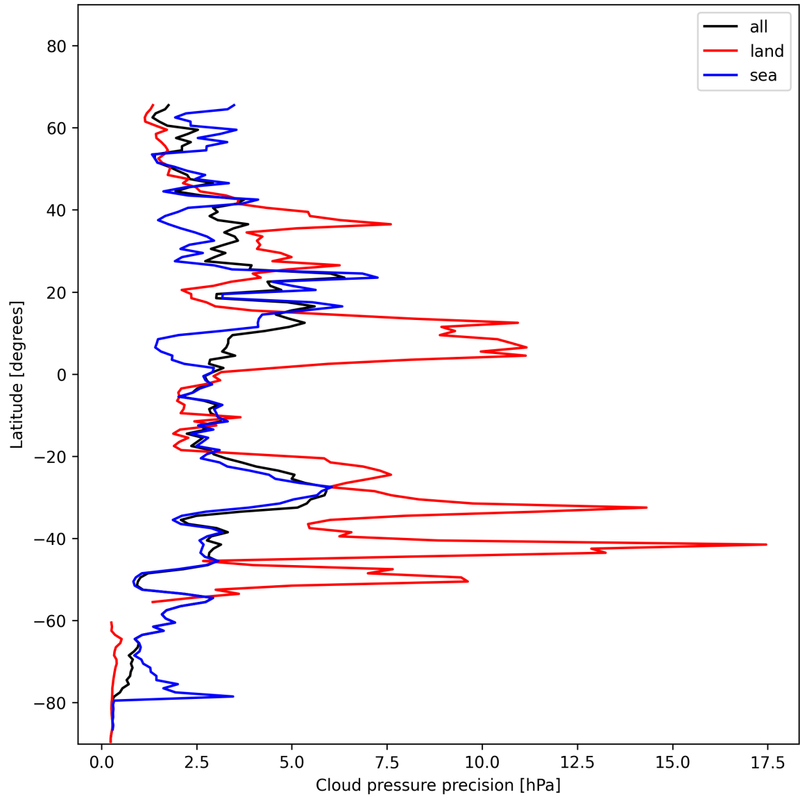
Figure 14: Zonal average of "Cloud pressure precision" for 2025-01-07 to 2025-01-08.
