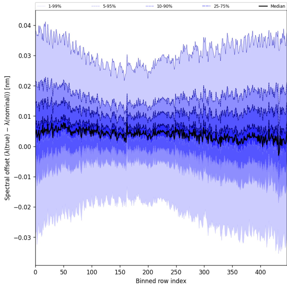
Figure 62: Along track statistics of “Spectral offset ( \lambda_{\text{true}} - \lambda_{\text{nominal}} )” for 2025-01-07 to 2025-01-08
