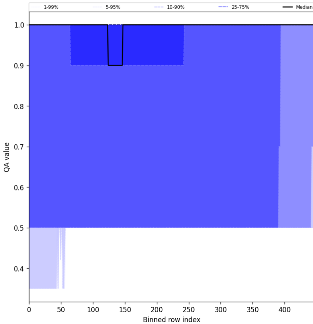
Figure 46: Along track statistics of “QA value” for 2025-01-07 to 2025-01-08
