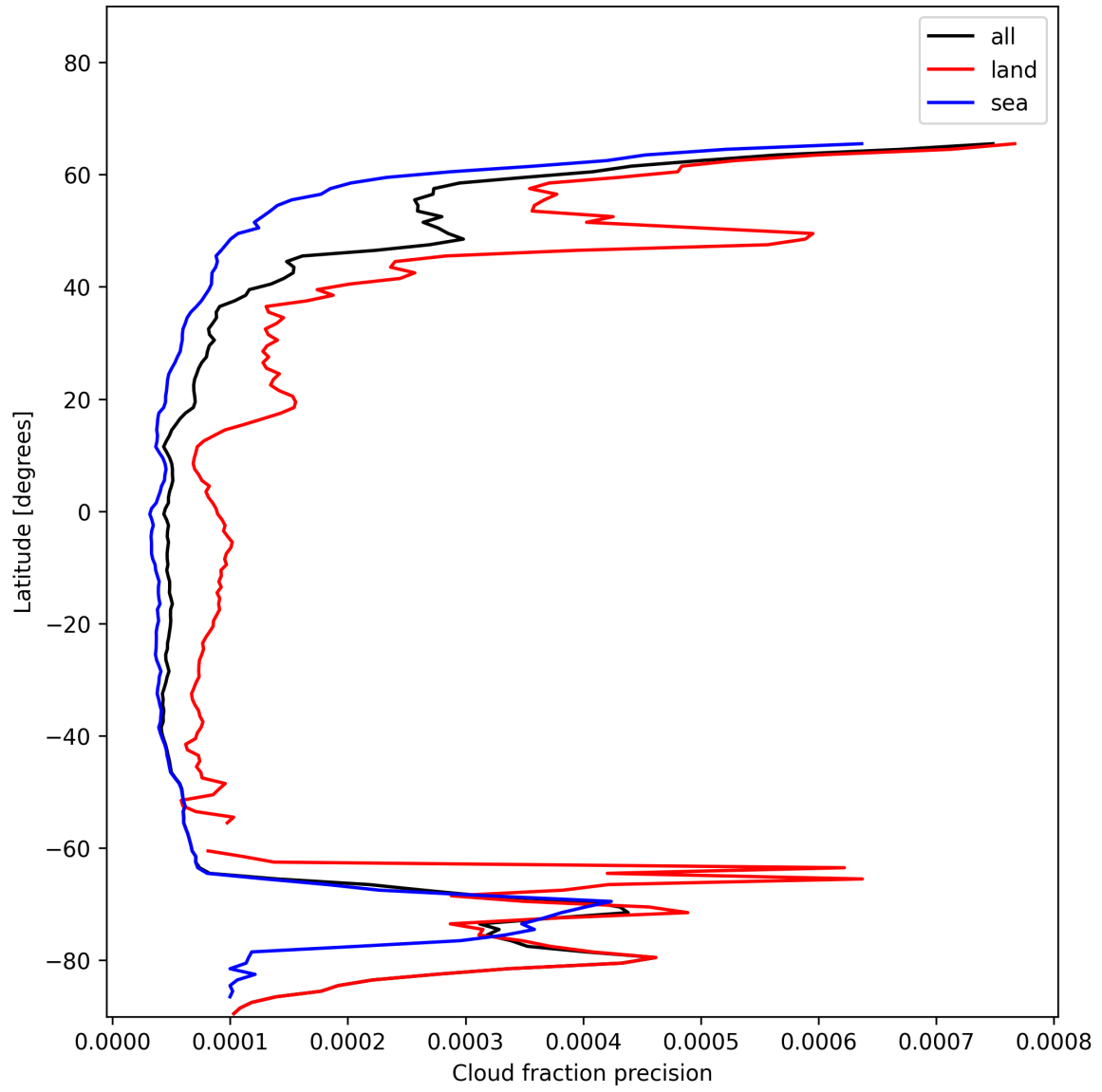
Figure 16: Zonal average of “Cloud fraction precision” for 2025-01-07 to 2025-01-08.
