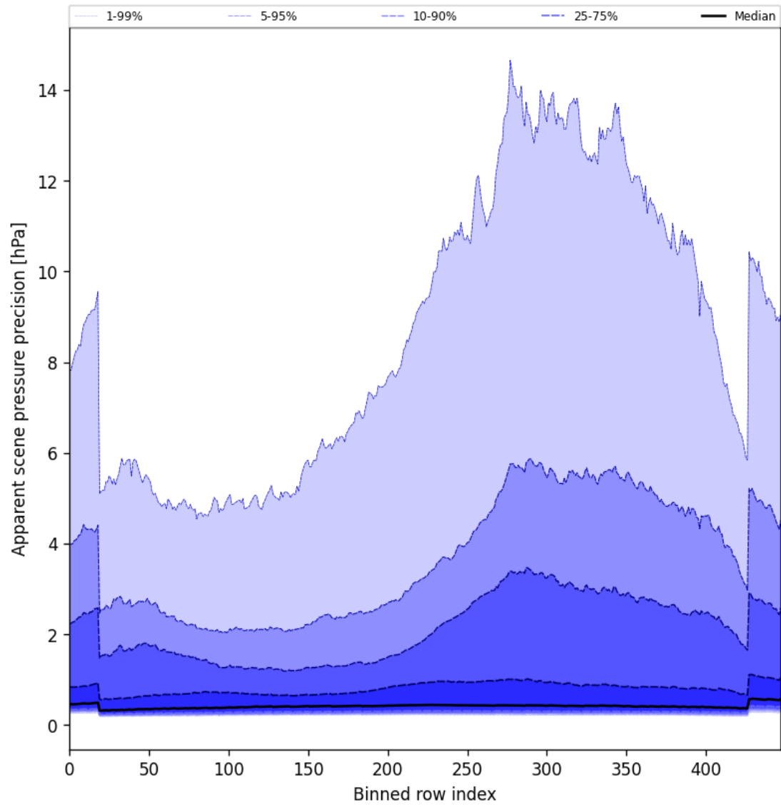
Figure 54: Along track statistics of “Apparent scene pressure precision” for 2025-01-07 to 2025-01-08
