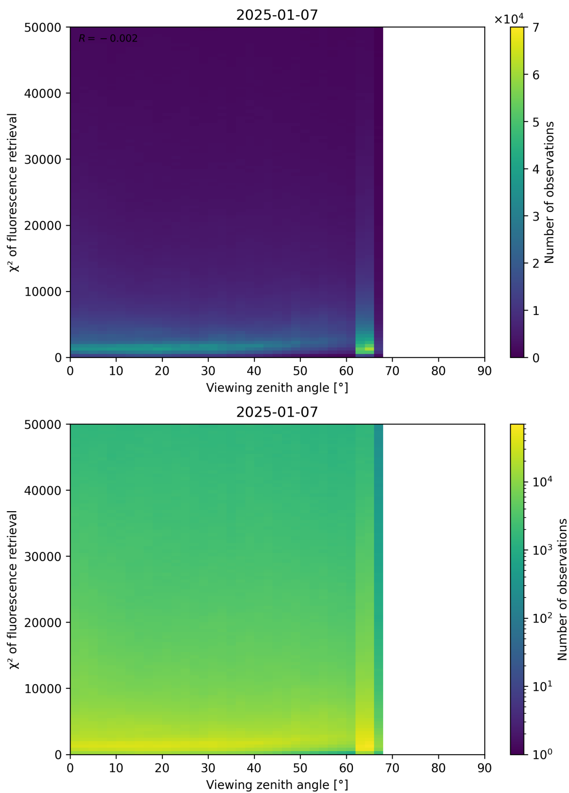
Figure 119: Scatter density plot of “Viewing zenith angle” against “ \chi^2 of fluorescence retrieval” for 2025-01-07 to 2025-01-08.
