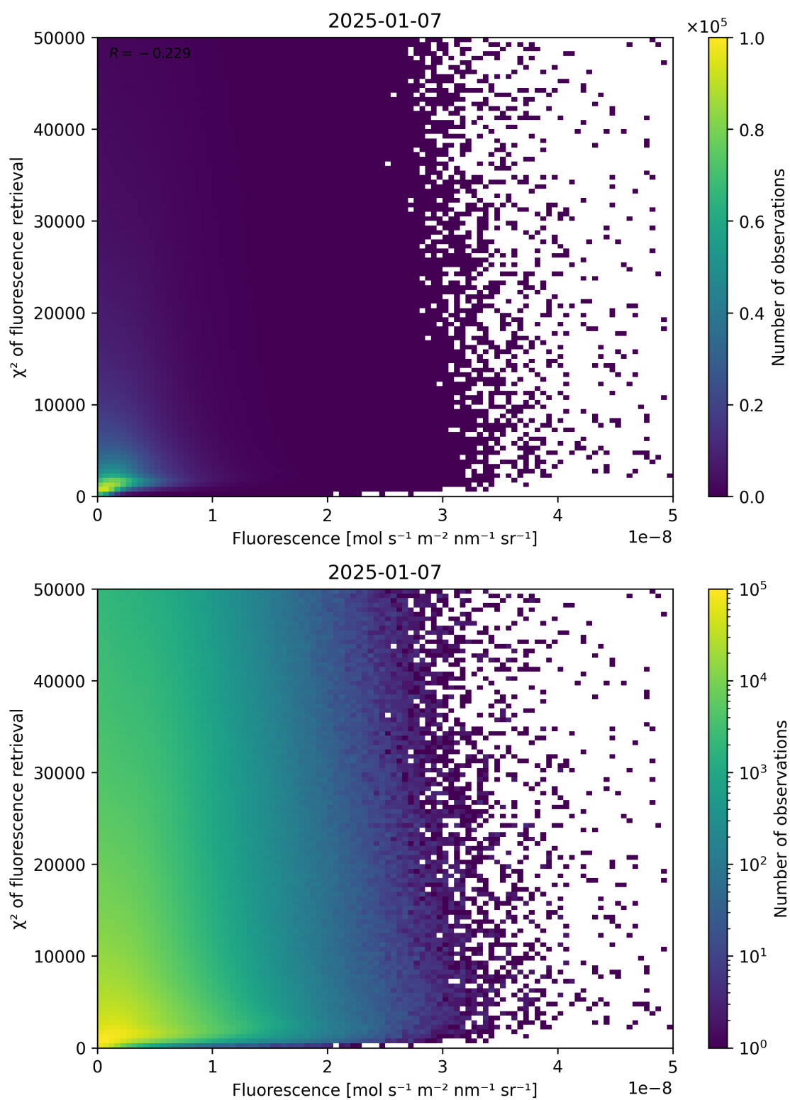
Figure 85: Scatter density plot of “Fluorescence” against “ \chi^2 of fluorescence retrieval” for 2025-01-07 to 2025-01-08.
