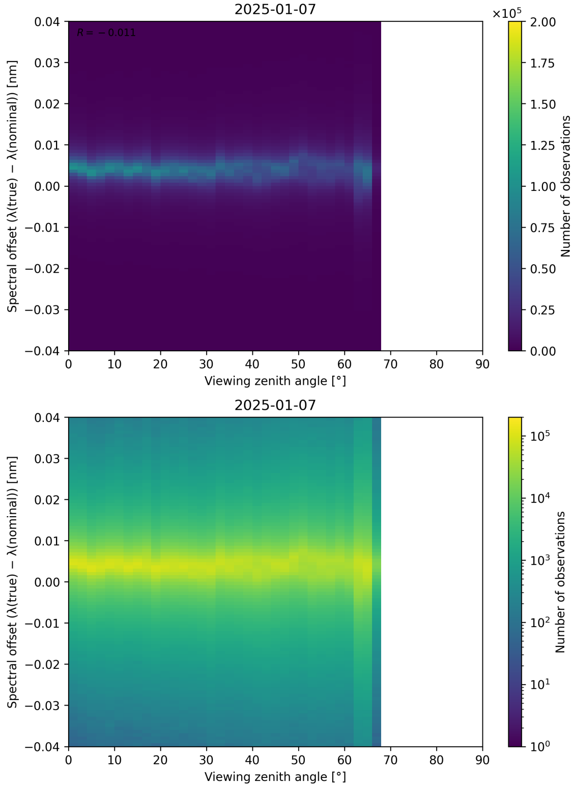
Figure 128: Scatter density plot of “Viewing zenith angle” against “Spectral offset ( \lambda_{\text{true}} - \lambda_{\text{nominal}} )” for 2025-01-07 to 2025-01-08.
