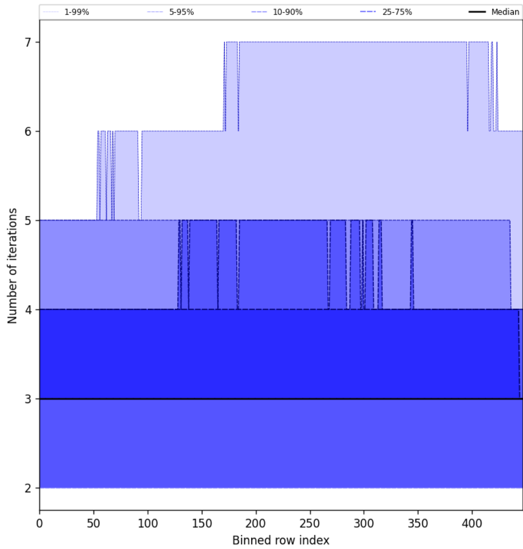
Figure 56: Along track statistics of “Number of iterations” for 2025-01-07 to 2025-01-08
