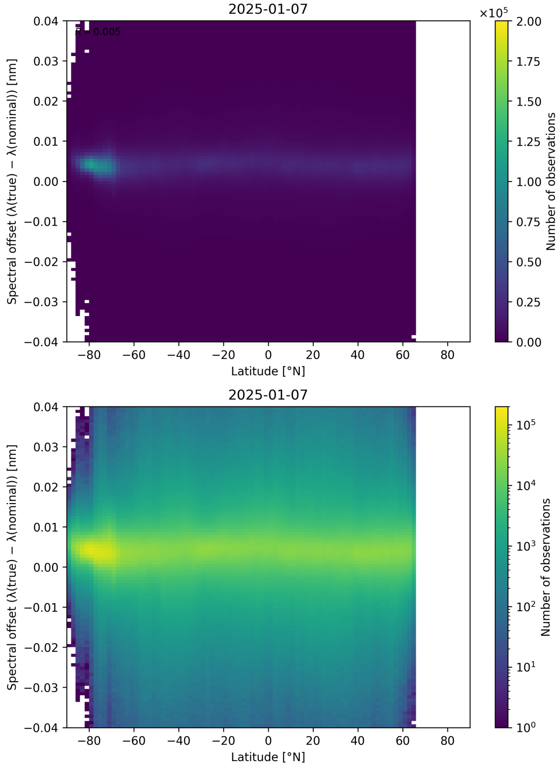
Figure 96: Scatter density plot of “Latitude” against “Spectral offset ( \lambda_{\text{true}} - \lambda_{\text{nominal}} )” for 2025-01-07 to 2025-01-08.
