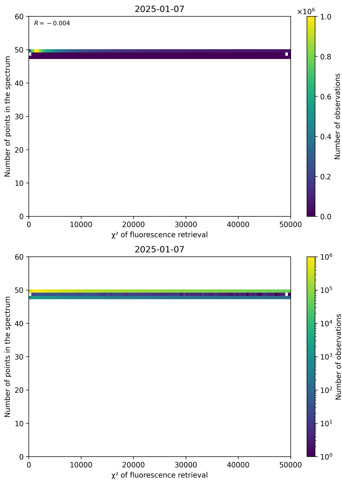
Figure 68: Scatter density plot of " \chi^2 of fluorescence retrieval" against "Number of points in the spectrum" for 2025-01-07 to 2025-01-08.
