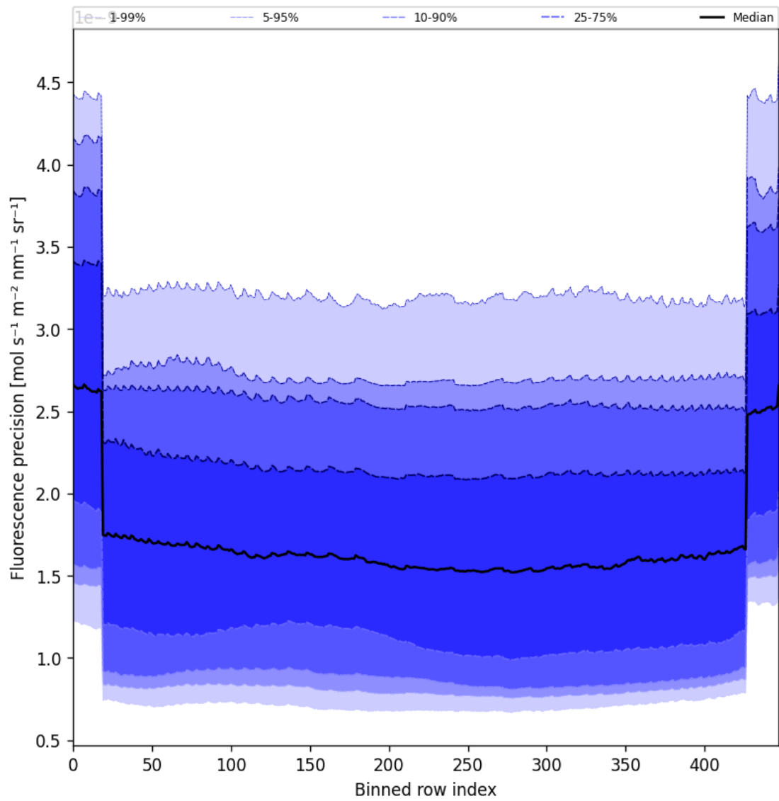
Figure 58: Along track statistics of “Fluorescence precision” for 2025-01-07 to 2025-01-08
