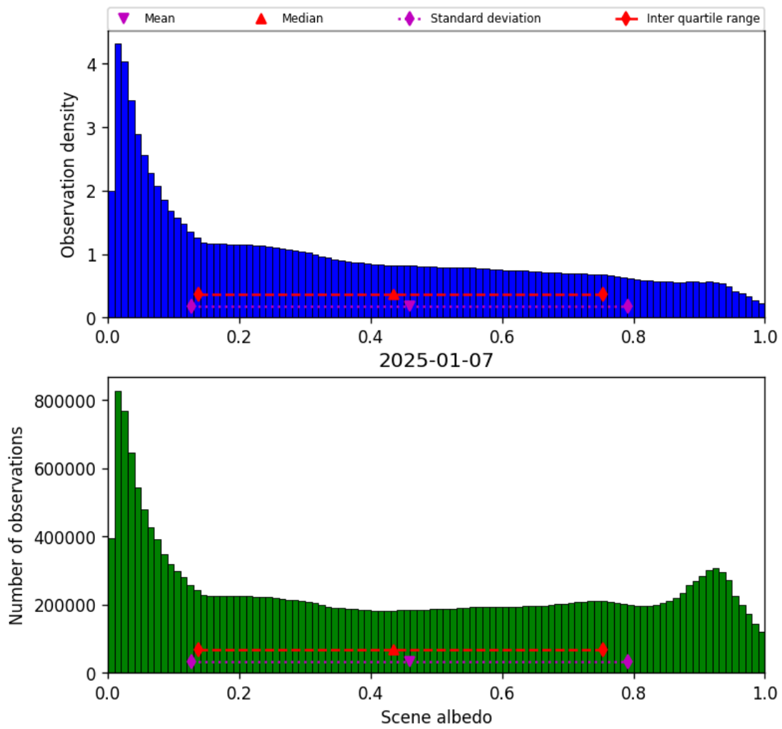
Figure 34: Histogram of “Scene albedo” for 2025-01-07 to 2025-01-08
