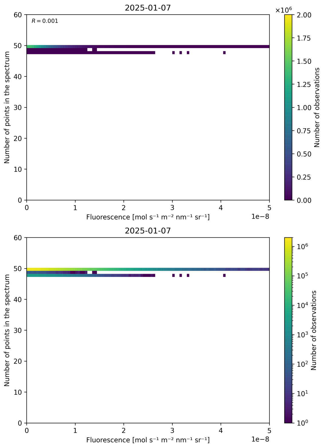
Figure 86: Scatter density plot of “Fluorescence” against “Number of points in the spectrum” for 2025-01-07 to 2025-01-08.
