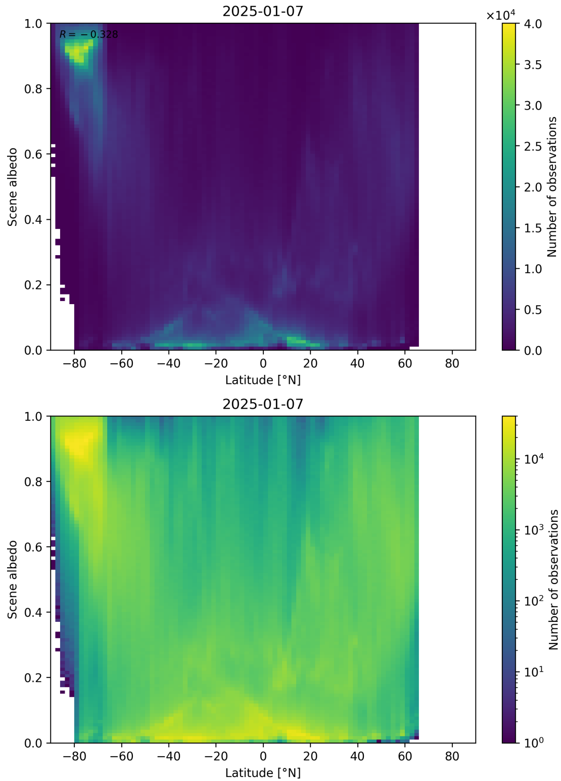
Figure 95: Scatter density plot of “Latitude” against “Scene albedo” for 2025-01-07 to 2025-01-08.
