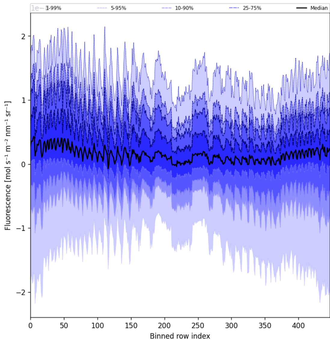
Figure 57: Along track statistics of “Fluorescence” for 2025-01-07 to 2025-01-08
