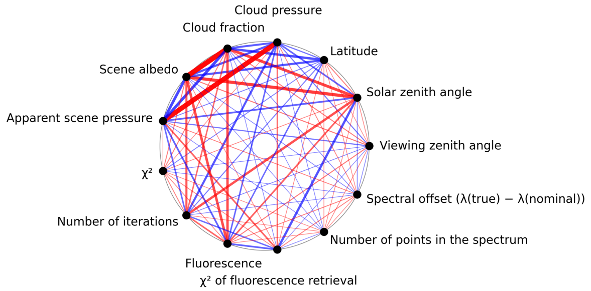
Figure 1: Map of correlation graph for 2025-01-07 to 2025-01-08.
