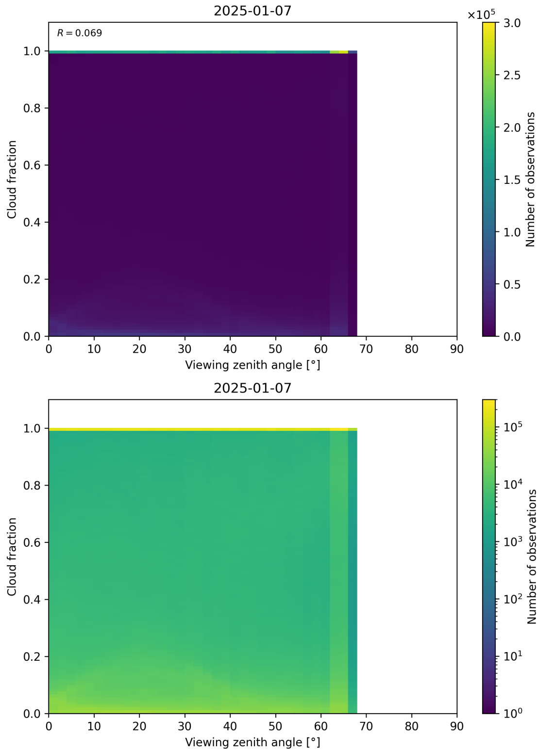
Figure 120: Scatter density plot of “Viewing zenith angle” against “Cloud fraction” for 2025-01-07 to 2025-01-08.
