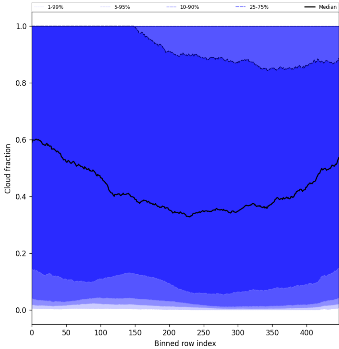
Figure 49: Along track statistics of “Cloud fraction” for 2025-01-07 to 2025-01-08
