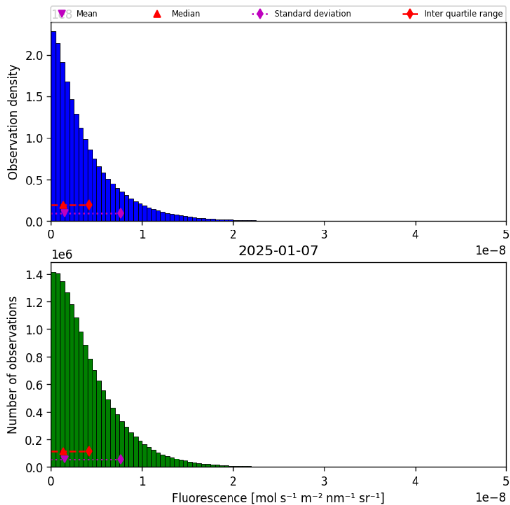
Figure 40: Histogram of “Fluorescence” for 2025-01-07 to 2025-01-08
