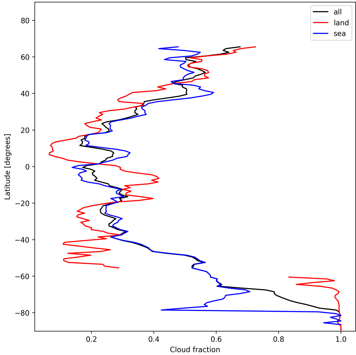
Figure 15: Zonal average of “Cloud fraction” for 2025-01-07 to 2025-01-08.
