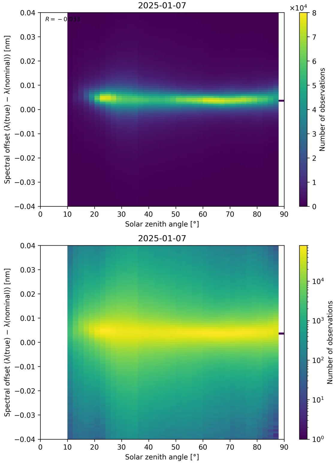
Figure 117: Scatter density plot of “Solar zenith angle” against “Spectral offset ( \lambda_{\text{true}} - \lambda_{\text{nominal}} )” for 2025-01-07 to 2025-01-08.
