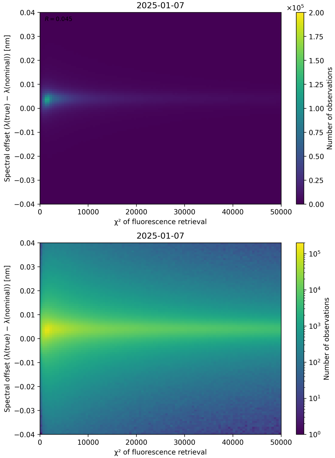
Figure 69: Scatter density plot of “ \chi^2 of fluorescence retrieval” against “Spectral offset ( \lambda_{\text{true}} - \lambda_{\text{nominal}} )” for 2025-01-07 to 2025-01-08.
