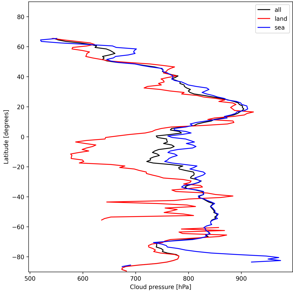
Figure 13: Zonal average of “Cloud pressure” for 2025-01-07 to 2025-01-09.
