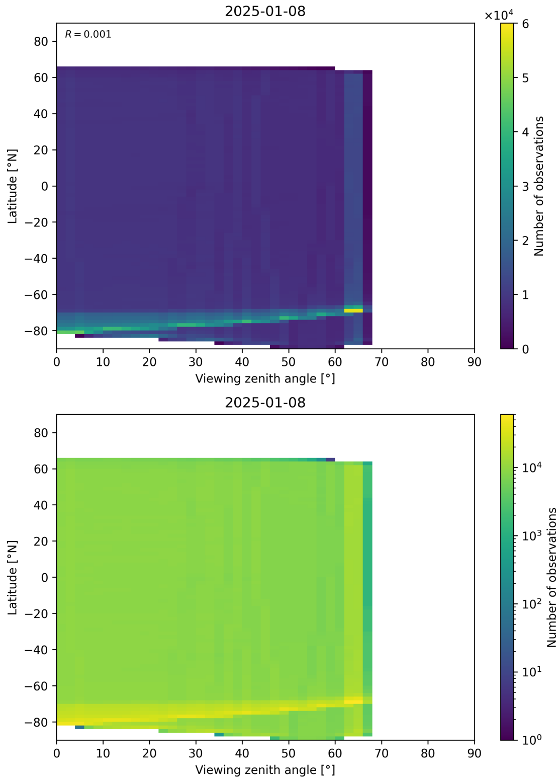
Figure 123: Scatter density plot of “Viewing zenith angle” against “Latitude” for 2025-01-07 to 2025-01-09.
