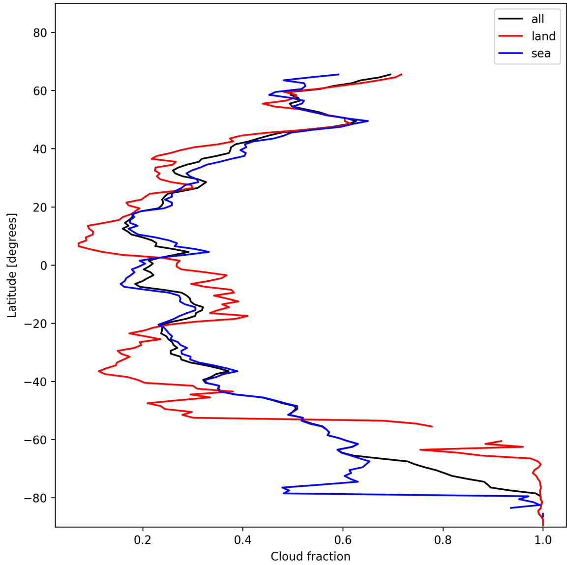
Figure 15: Zonal average of “Cloud fraction” for 2025-01-07 to 2025-01-09.
