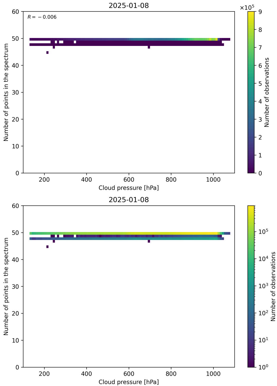
Figure 82: Scatter density plot of “Cloud pressure” against “Number of points in the spectrum” for 2025-01-07 to 2025-01-09.
