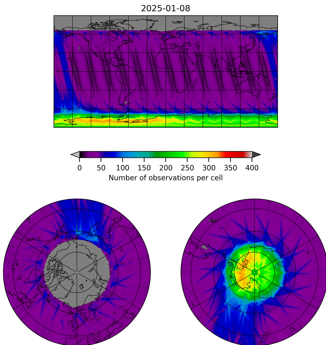
Figure 11: Map of the number of observations for 2025-01-07 to 2025-01-09
