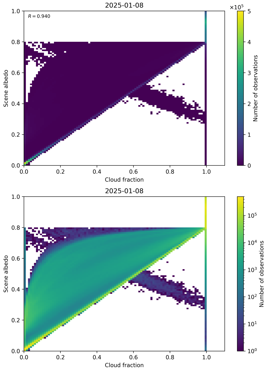
Figure 75: Scatter density plot of “Cloud fraction” against “Scene albedo” for 2025-01-07 to 2025-01-09.
