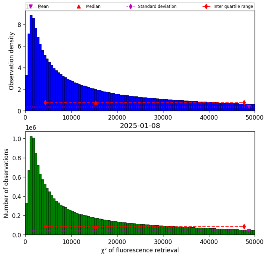
Figure 42: Histogram of “ \chi^2 of fluorescence retrieval” for 2025-01-07 to 2025-01-09
