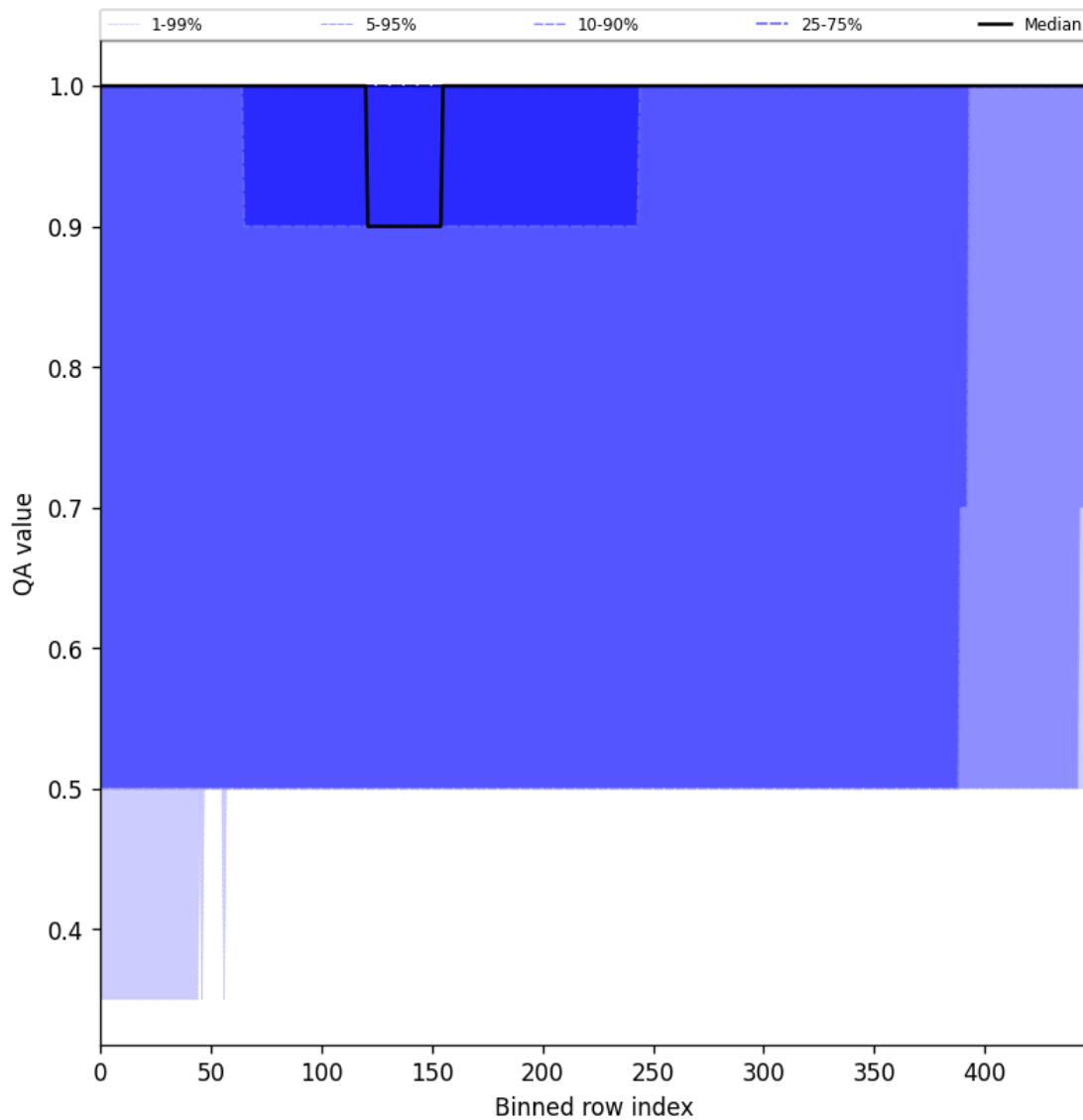
Figure 46: Along track statistics of “QA value” for 2025-01-07 to 2025-01-09
