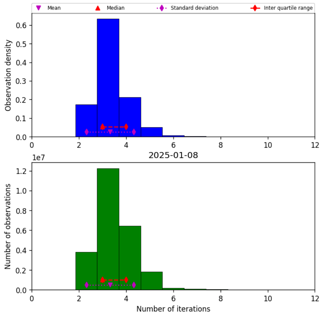
Figure 39: Histogram of “Number of iterations” for 2025-01-07 to 2025-01-09
