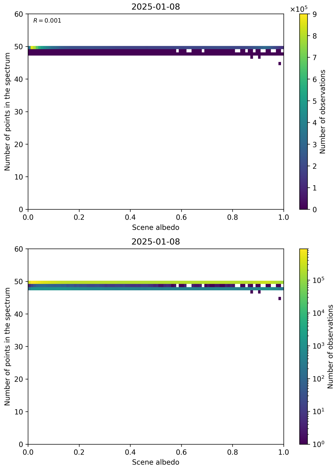
Figure 106: Scatter density plot of “Scene albedo” against “Number of points in the spectrum” for 2025-01-07 to 2025-01-09.
