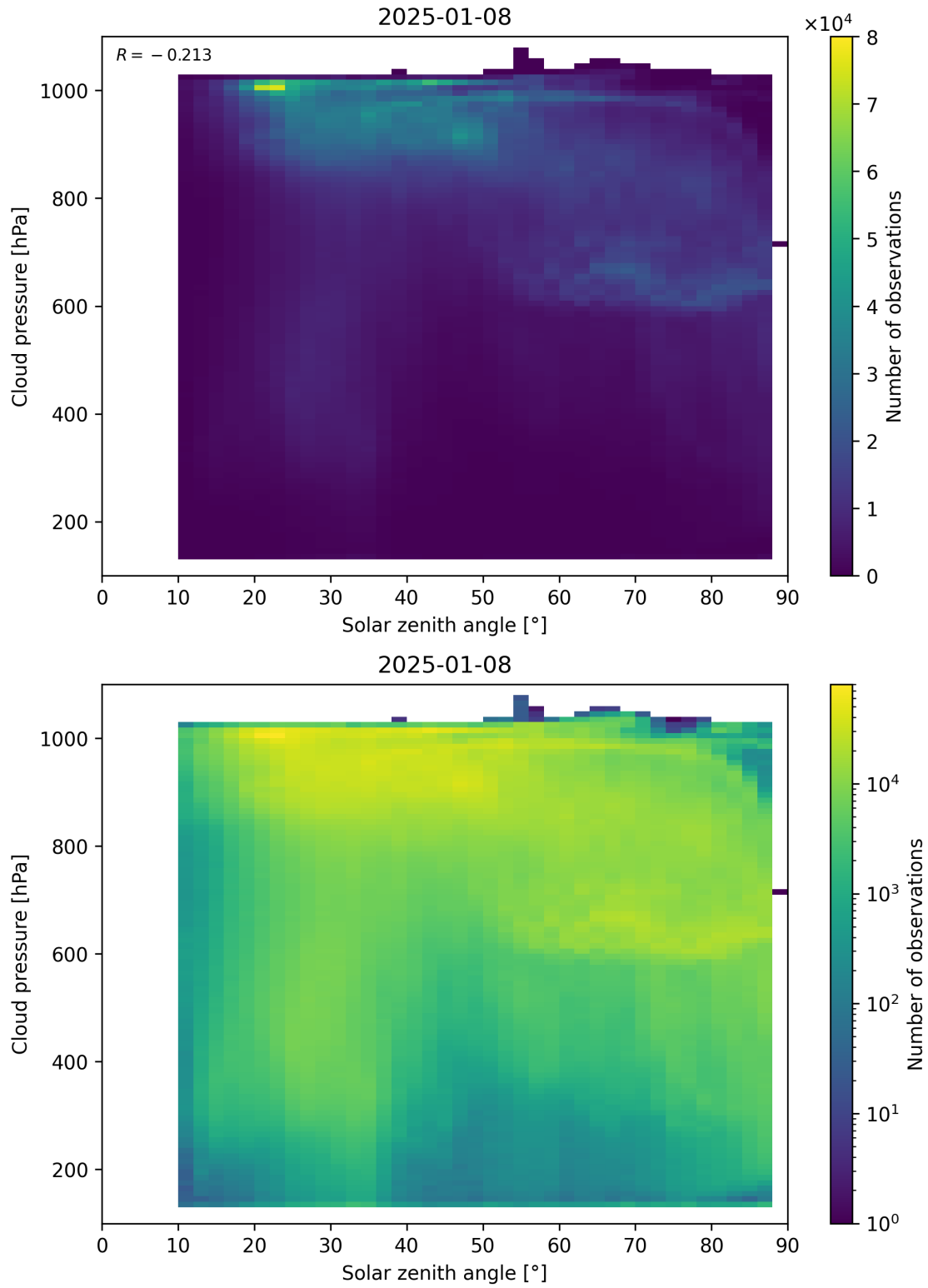
Figure 111: Scatter density plot of “Solar zenith angle” against “Cloud pressure” for 2025-01-07 to 2025-01-09.
