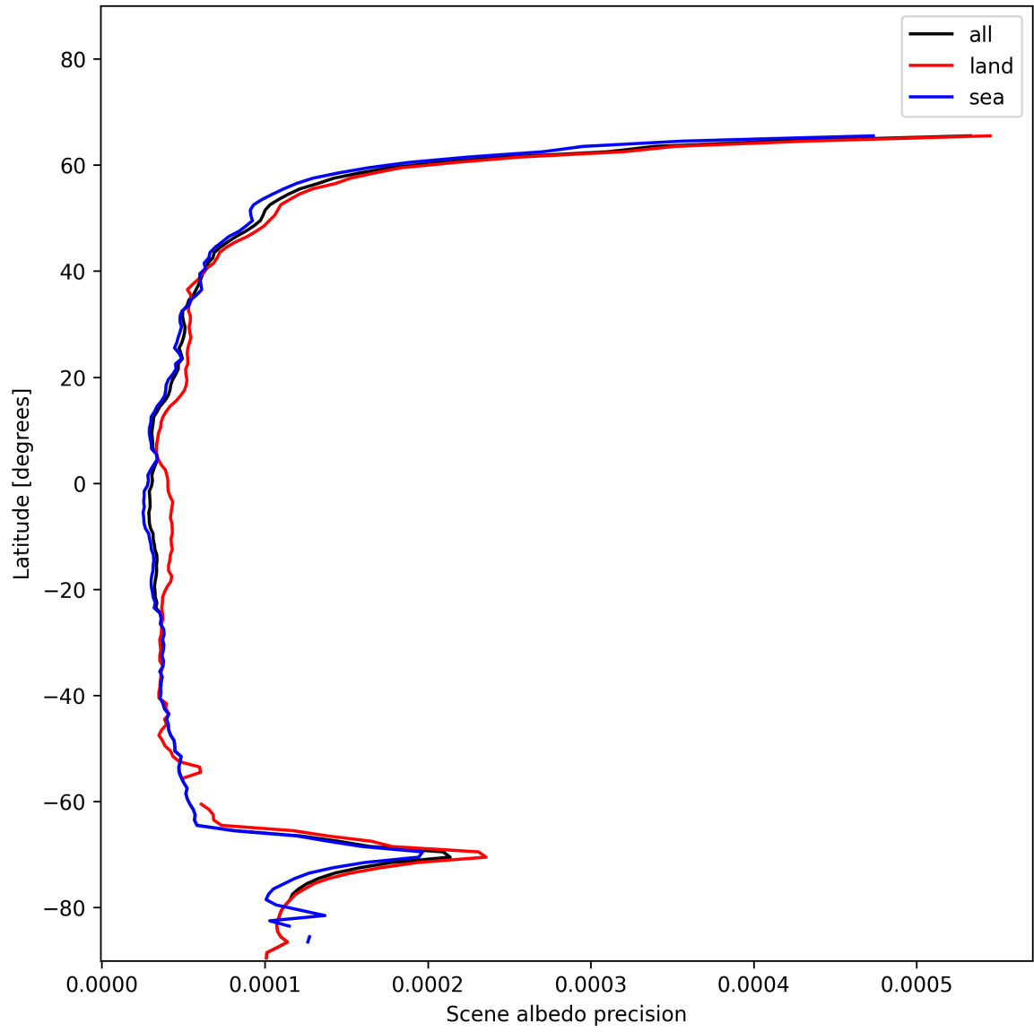
Figure 18: Zonal average of “Scene albedo precision” for 2025-01-07 to 2025-01-09.
