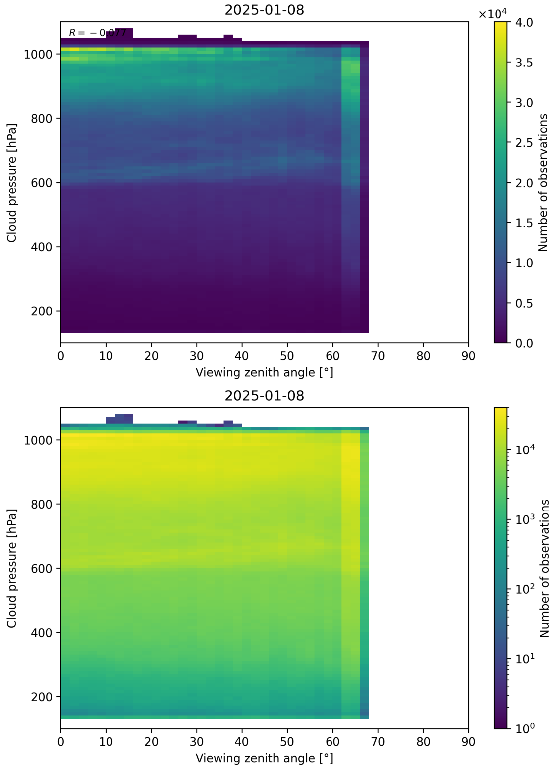
Figure 121: Scatter density plot of “Viewing zenith angle” against “Cloud pressure” for 2025-01-07 to 2025-01-09.
