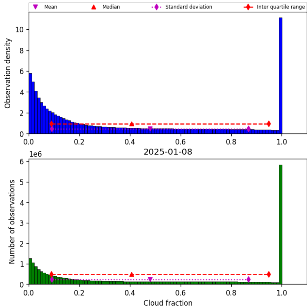
Figure 32: Histogram of “Cloud fraction” for 2025-01-07 to 2025-01-09
