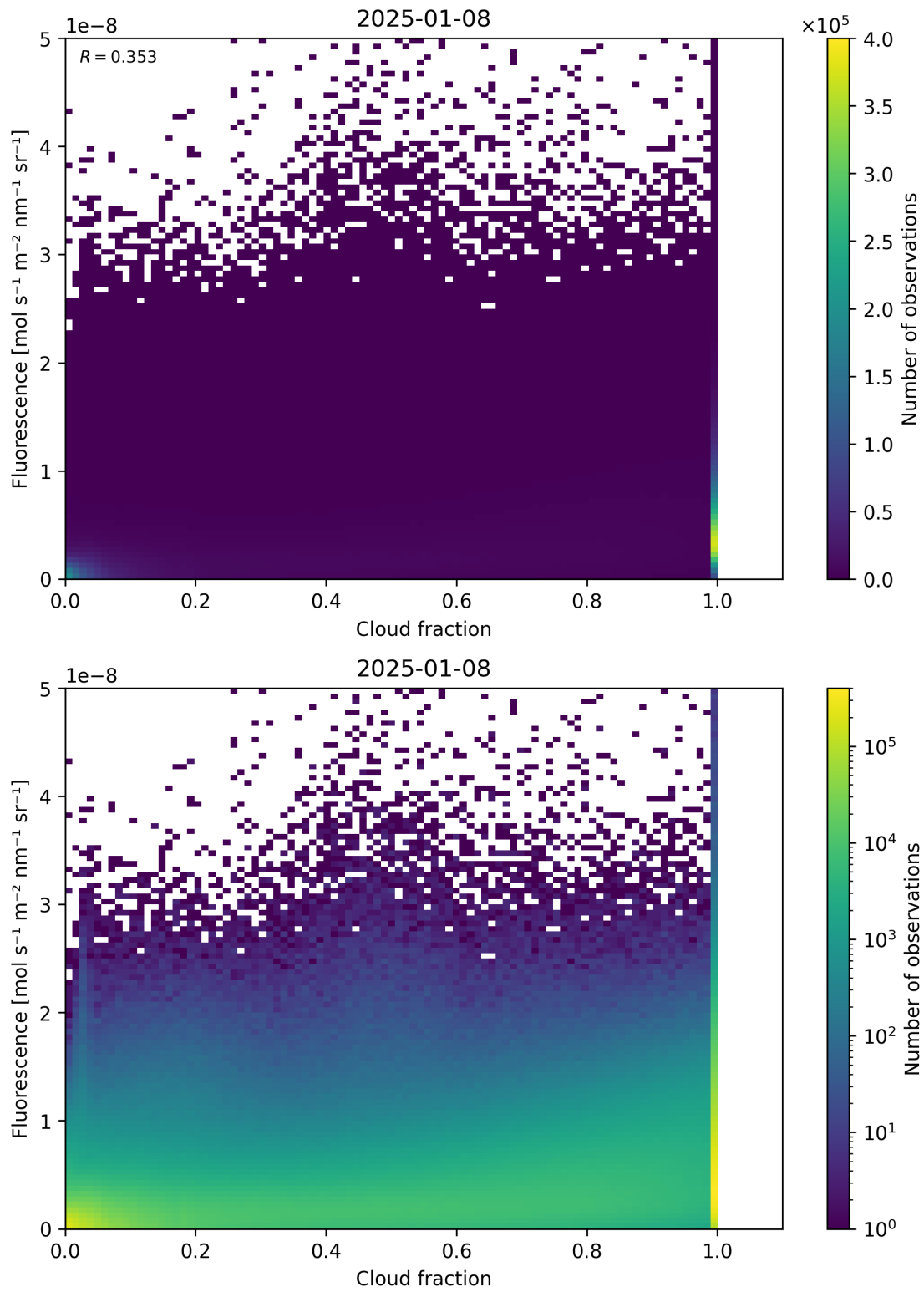
Figure 72: Scatter density plot of “Cloud fraction” against “Fluorescence” for 2025-01-07 to 2025-01-09.
