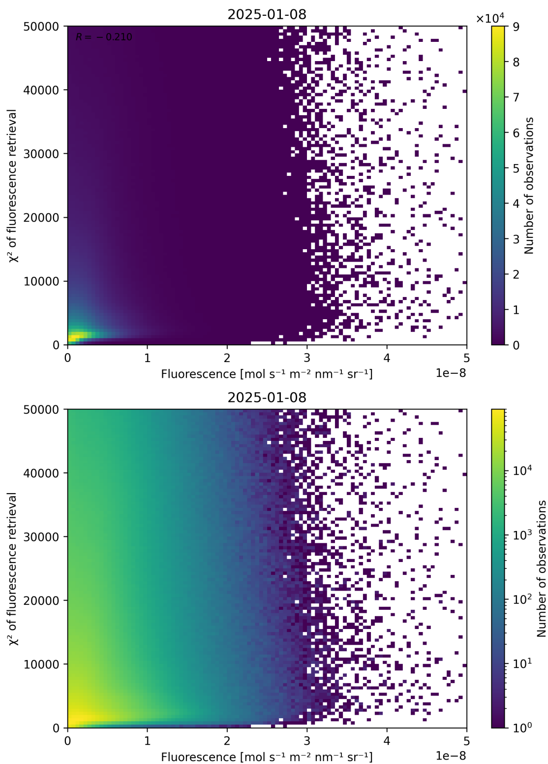
Figure 85: Scatter density plot of “Fluorescence” against “ \chi^2 of fluorescence retrieval” for 2025-01-07 to 2025-01-09.
