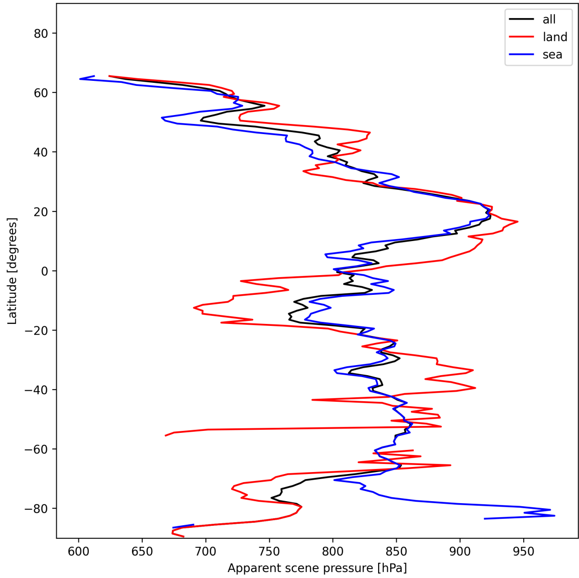
Figure 19: Zonal average of “Apparent scene pressure” for 2025-01-07 to 2025-01-09.
