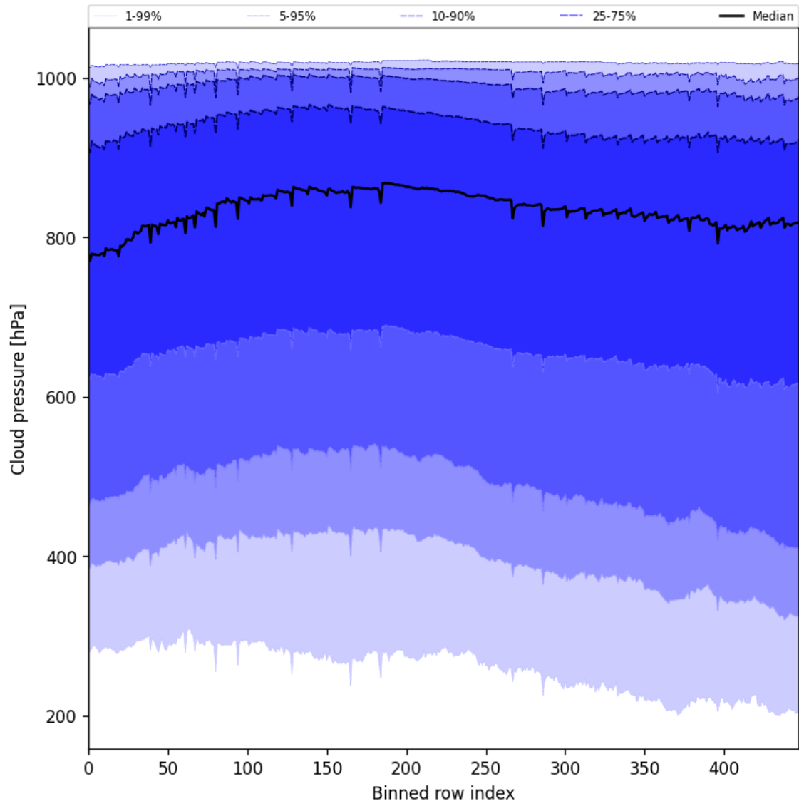
Figure 47: Along track statistics of “Cloud pressure” for 2025-01-07 to 2025-01-09
