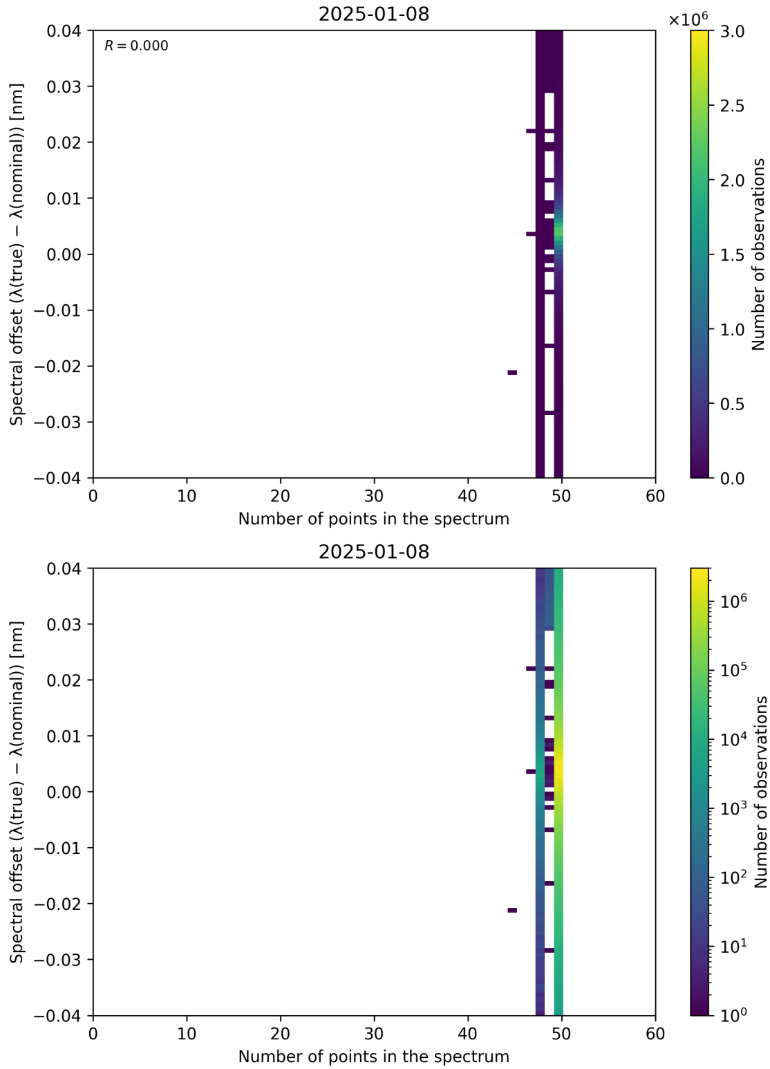
Figure 101: Scatter density plot of “Number of points in the spectrum” against “Spectral offset ( \lambda_{\text{true}} - \lambda_{\text{nominal}} )” for 2025-01-07 to 2025-01-09.
