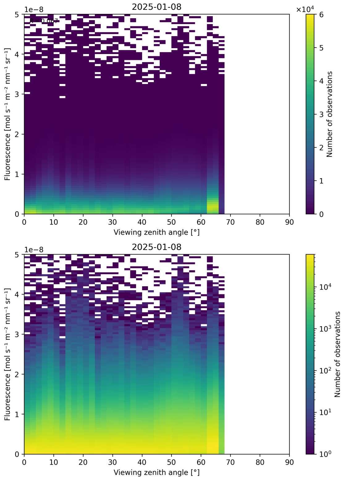
Figure 122: Scatter density plot of “Viewing zenith angle” against “Fluorescence” for 2025-01-07 to 2025-01-09.
