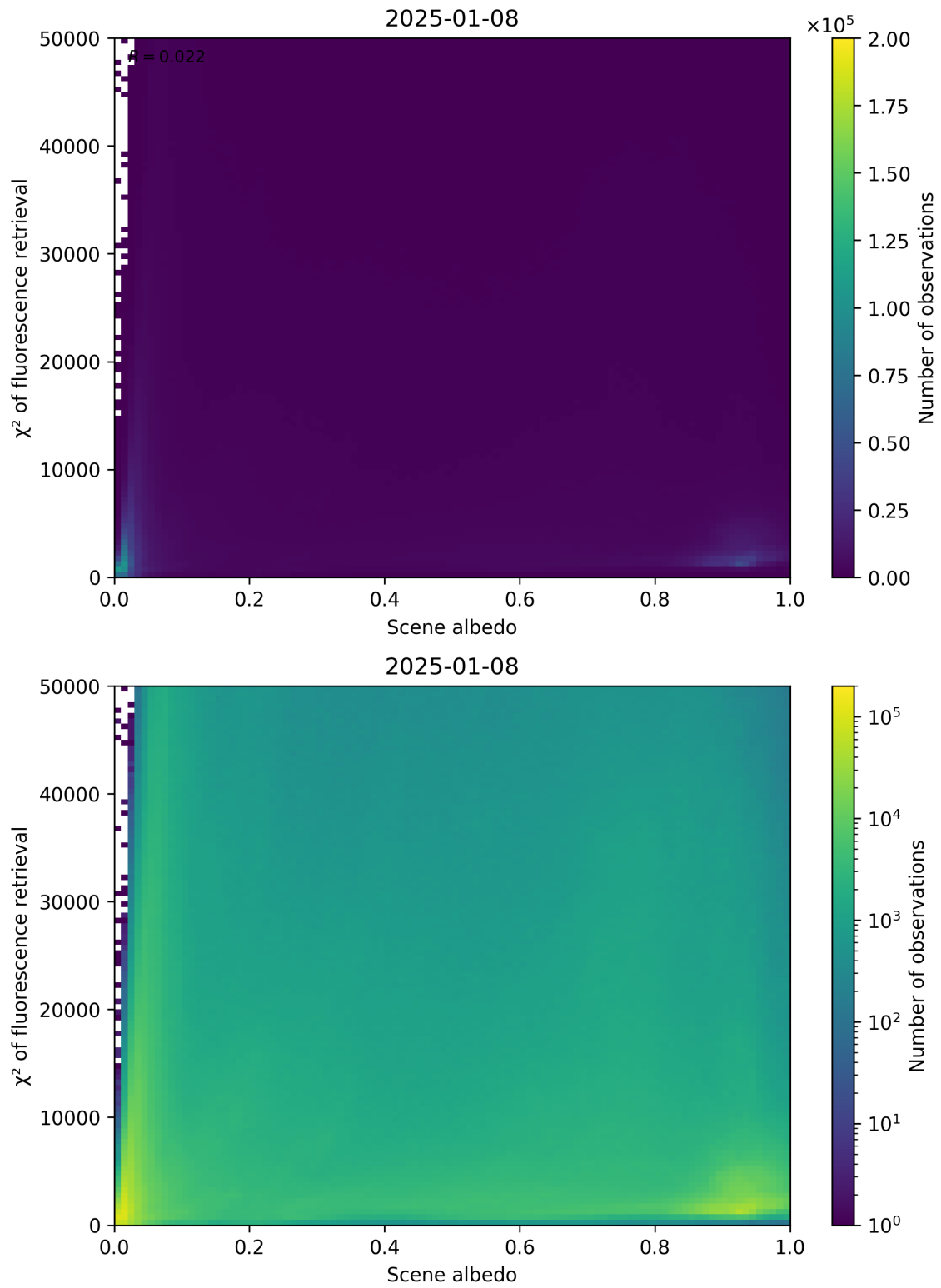
Figure 103: Scatter density plot of “Scene albedo” against “ \chi^2 of fluorescence retrieval” for 2025-01-07 to 2025-01-09.
