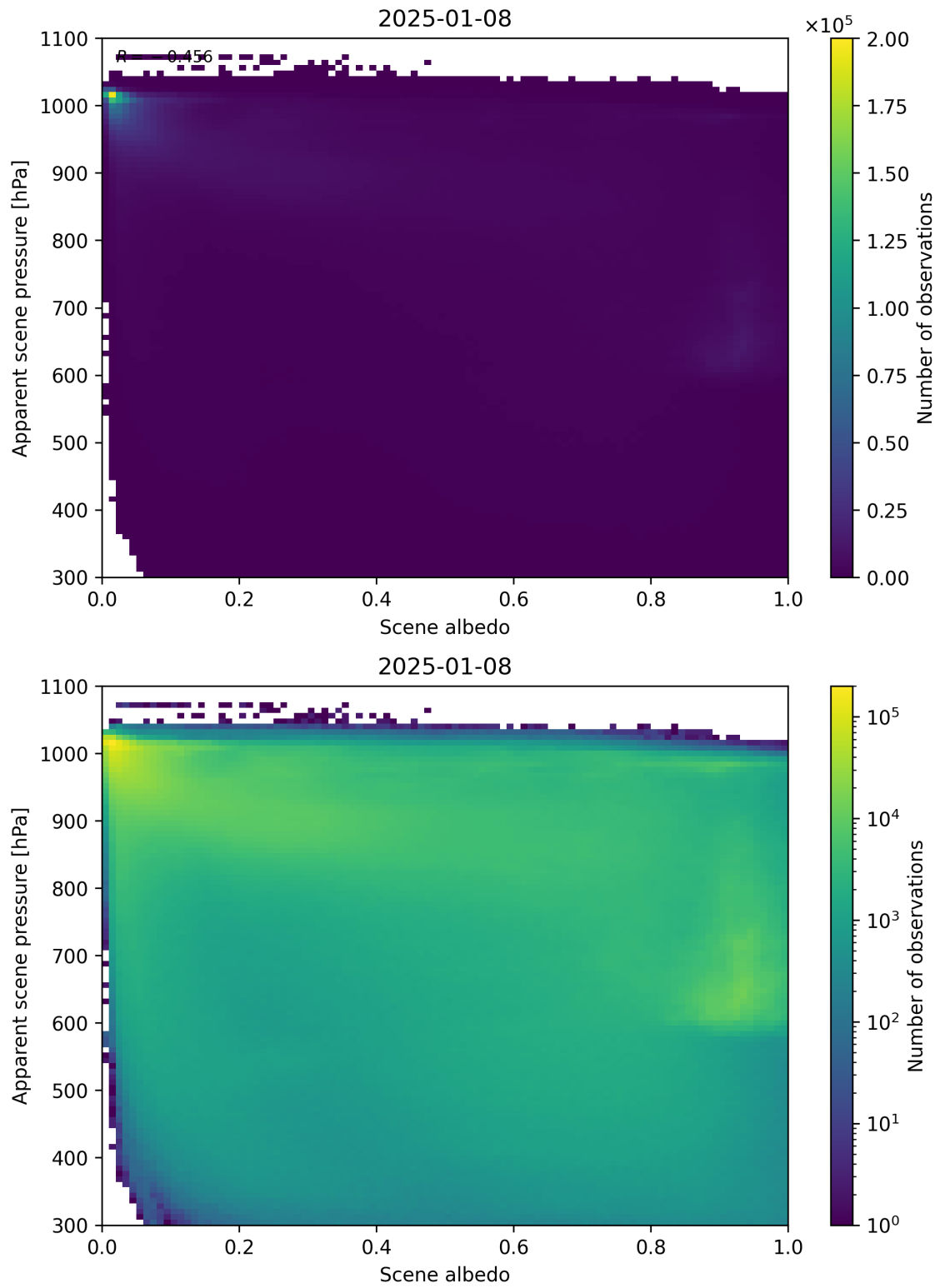
Figure 102: Scatter density plot of “Scene albedo” against “Apparent scene pressure” for 2025-01-07 to 2025-01-09.
