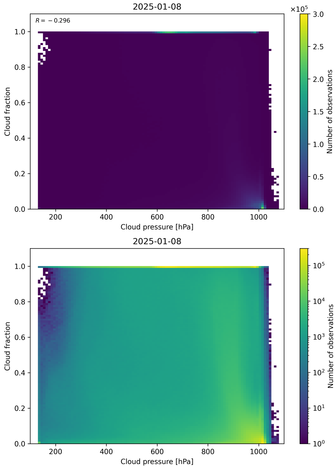
Figure 79: Scatter density plot of “Cloud pressure” against “Cloud fraction” for 2025-01-07 to 2025-01-09.
