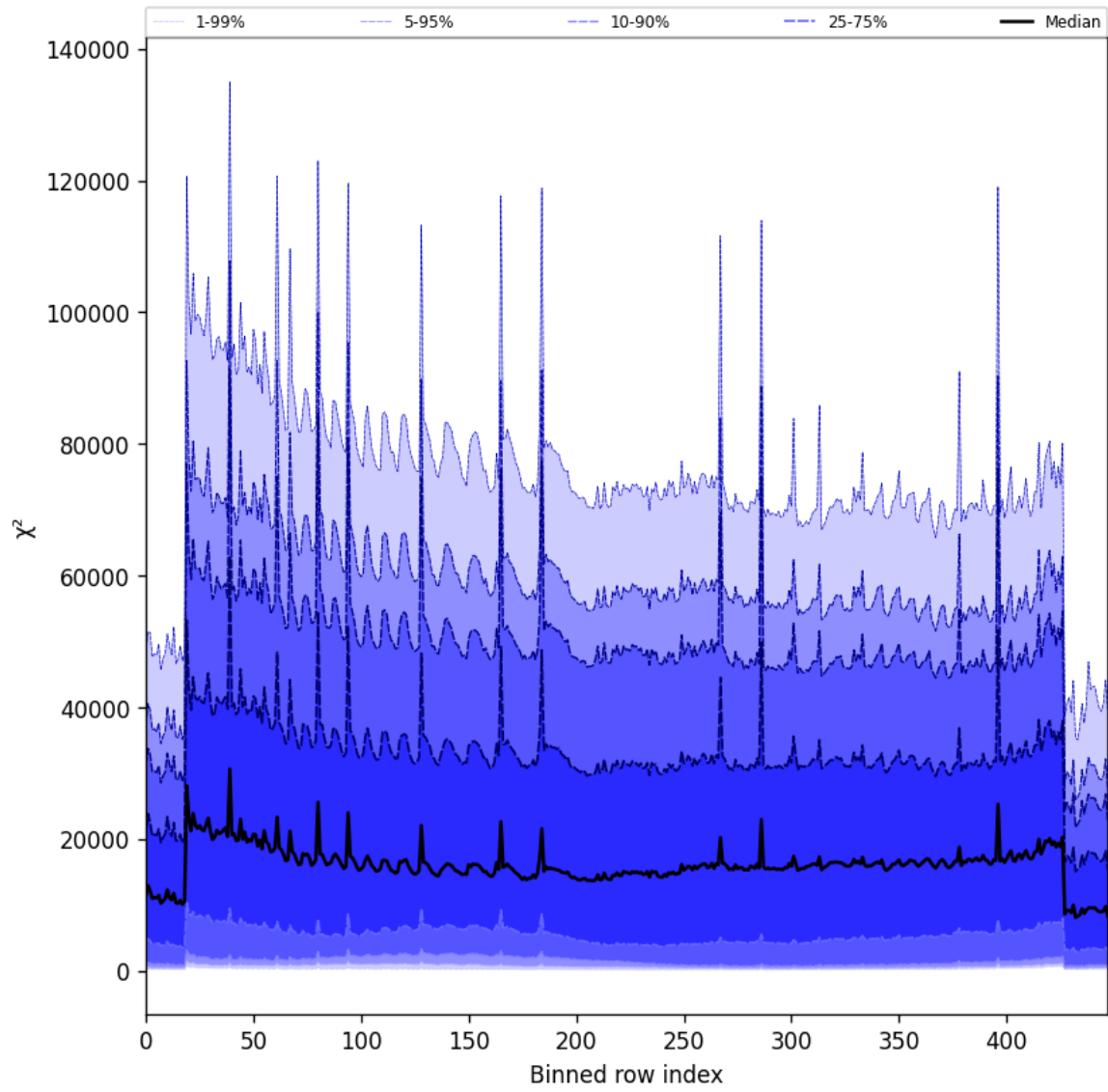
Figure 55: Along track statistics of “ \chi^2 ” for 2025-01-07 to 2025-01-09
