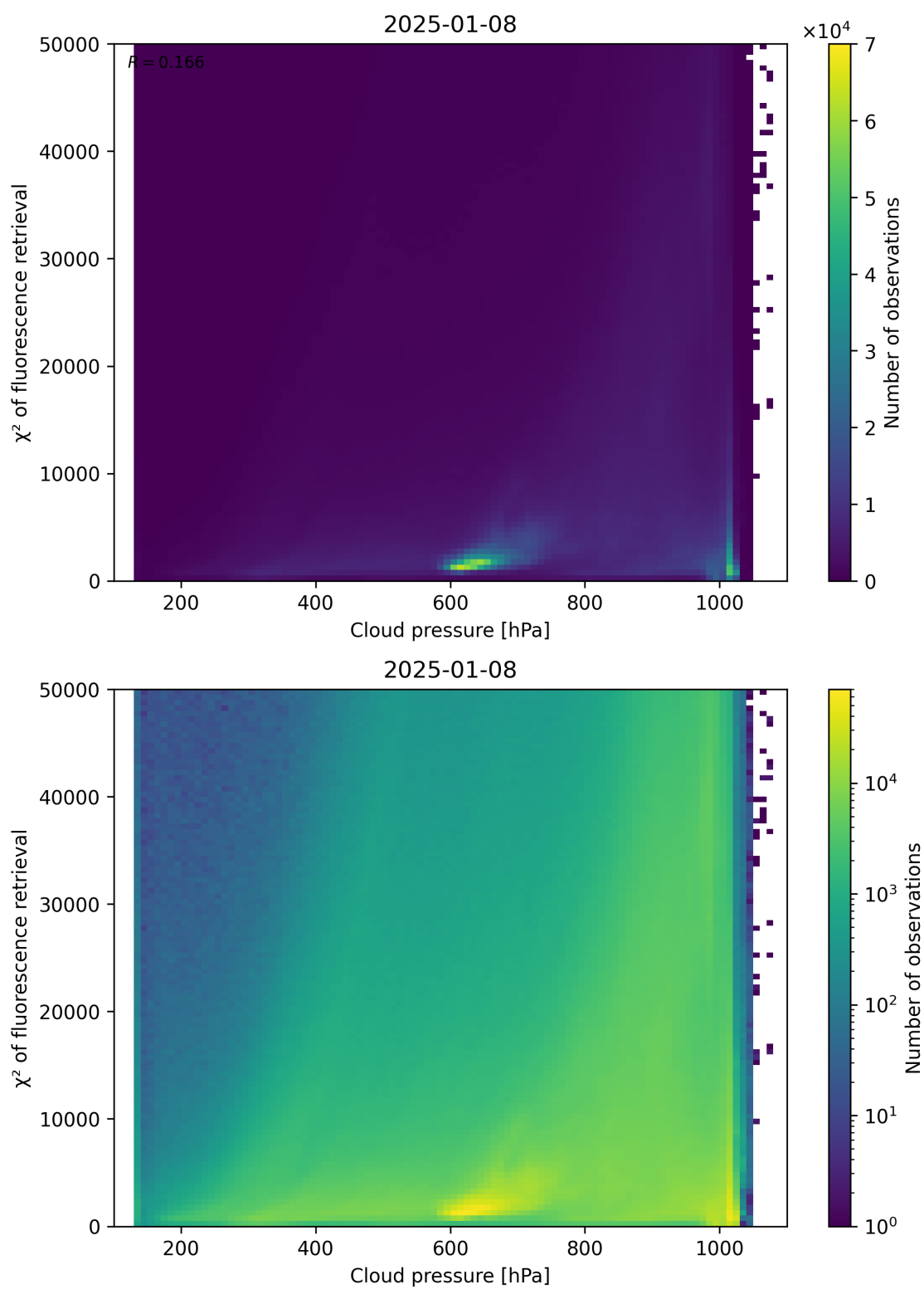
Figure 78: Scatter density plot of “Cloud pressure” against “ \chi^2 of fluorescence retrieval” for 2025-01-07 to 2025-01-09.
