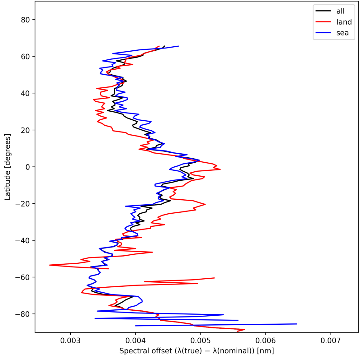
Figure 28: Zonal average of “Spectral offset ( \lambda_{\text{true}} - \lambda_{\text{nominal}} )” for 2025-01-07 to 2025-01-09.
