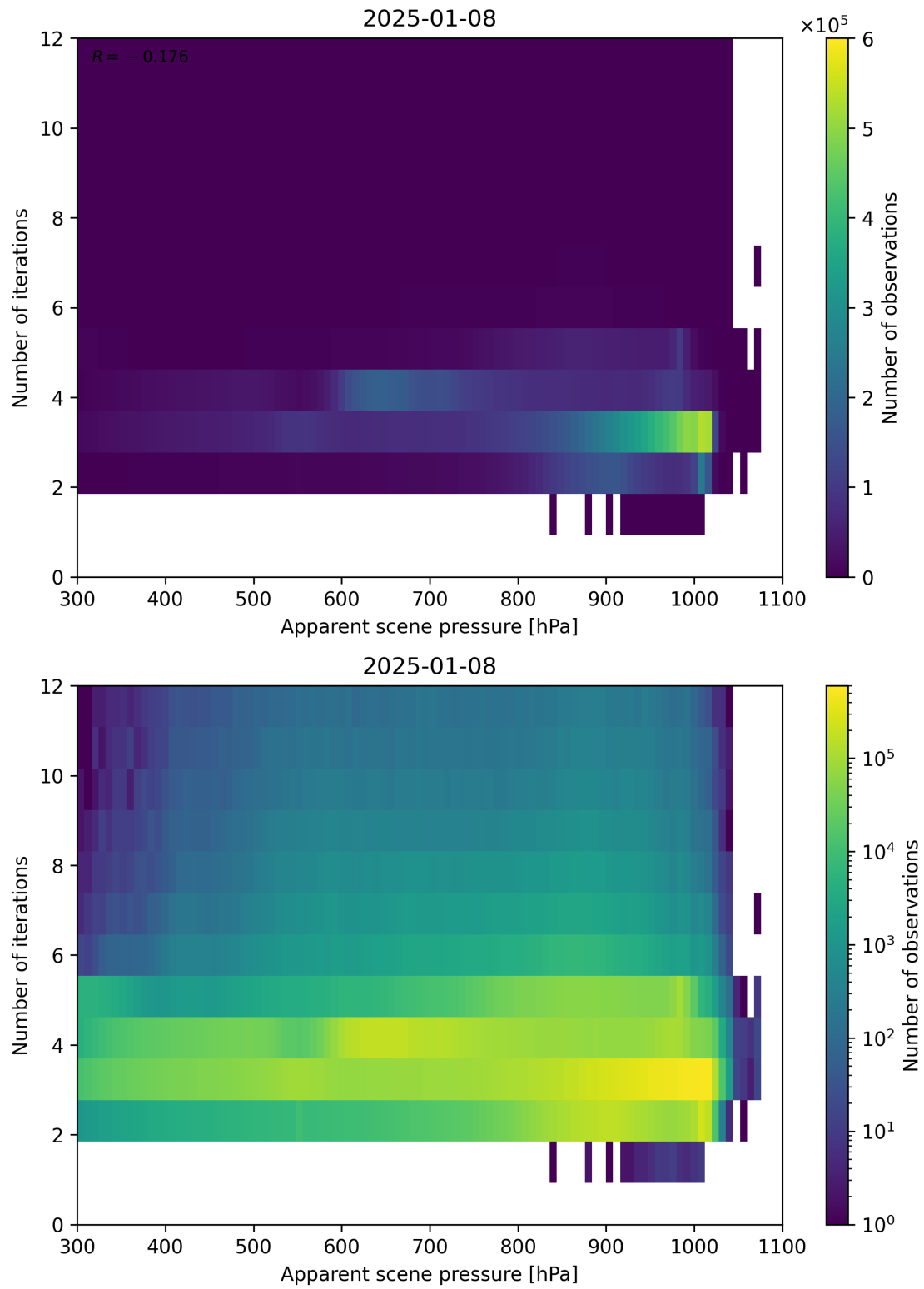
Figure 65: Scatter density plot of “Apparent scene pressure” against “Number of iterations” for 2025-01-07 to 2025-01-09.
