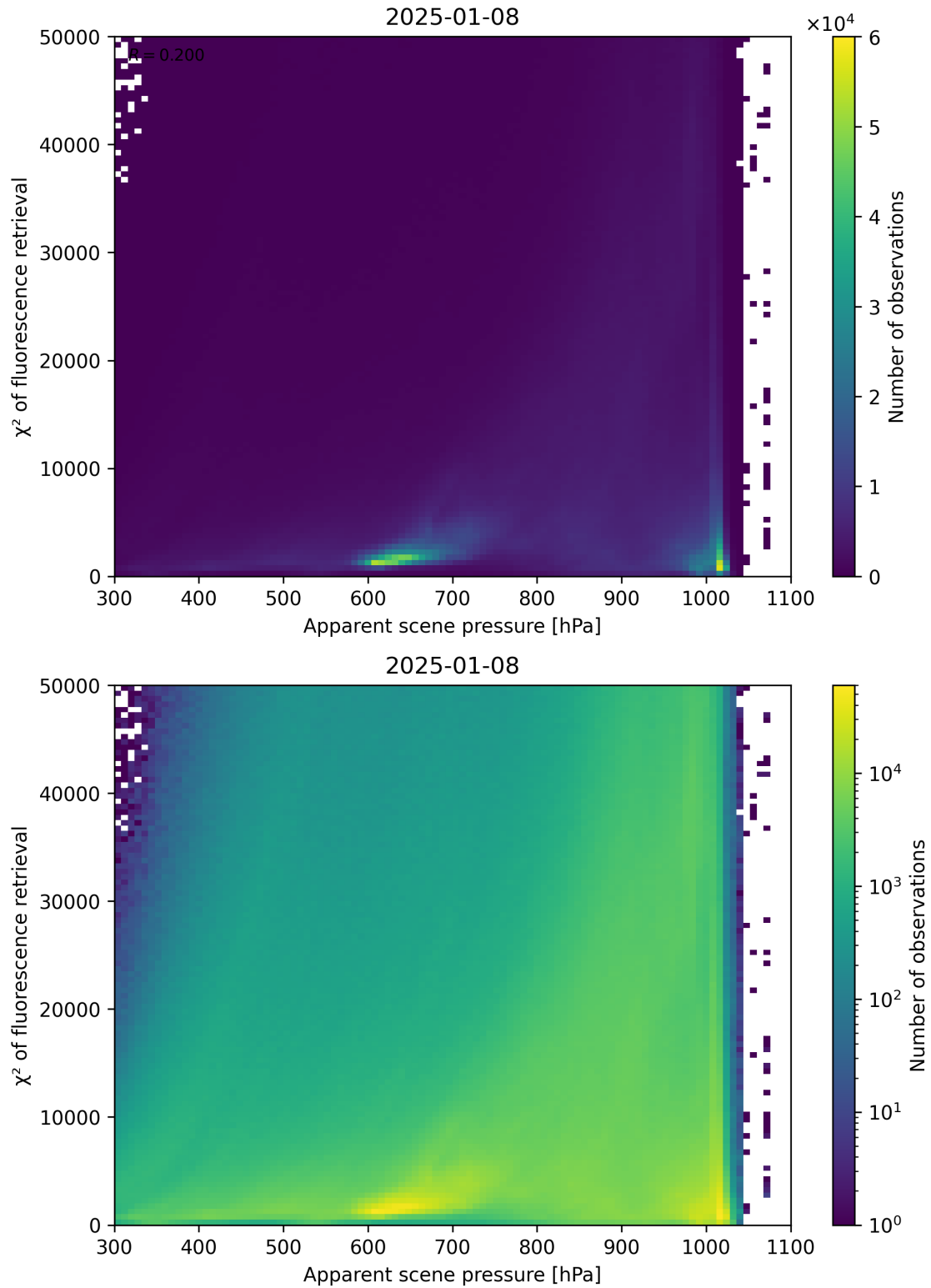
Figure 63: Scatter density plot of “Apparent scene pressure” against “ \chi^2 of fluorescence retrieval” for 2025-01-07 to 2025-01-09.
