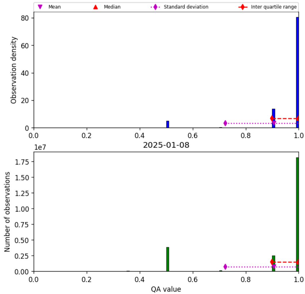
Figure 29: Histogram of “QA value” for 2025-01-07 to 2025-01-09
