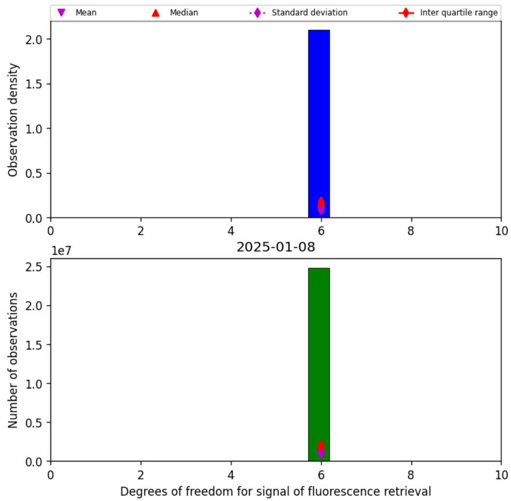
Figure 43: Histogram of “Degrees of freedom for signal of fluorescence retrieval” for 2025-01-07 to 2025-01-09
