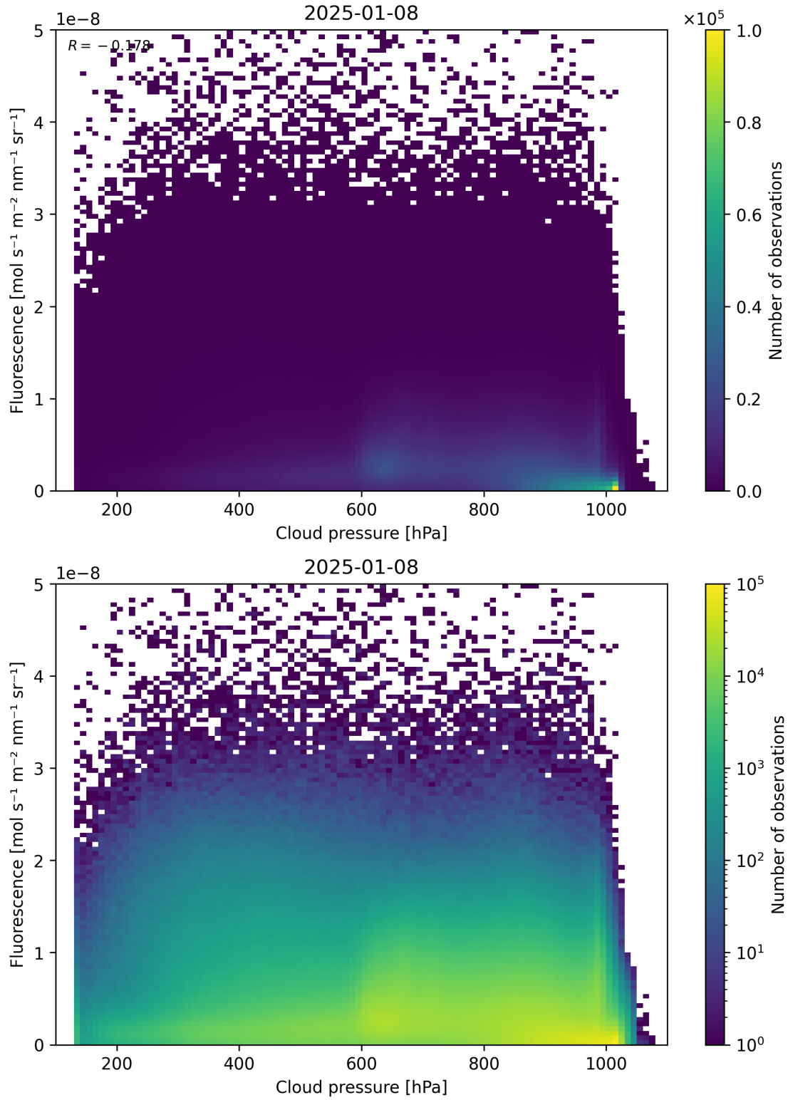
Figure 80: Scatter density plot of “Cloud pressure” against “Fluorescence” for 2025-01-07 to 2025-01-09.
