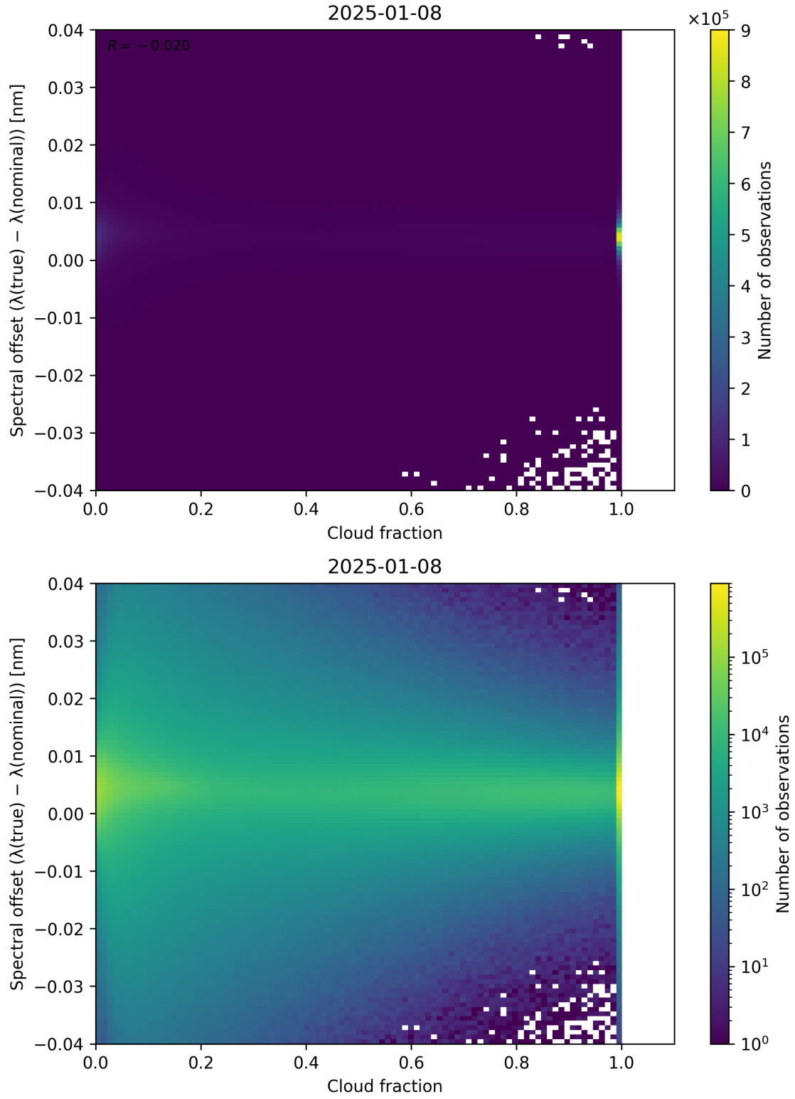
Figure 76: Scatter density plot of “Cloud fraction” against “Spectral offset ( \lambda_{\text{true}} - \lambda_{\text{nominal}} )” for 2025-01-07 to 2025-01-09.
