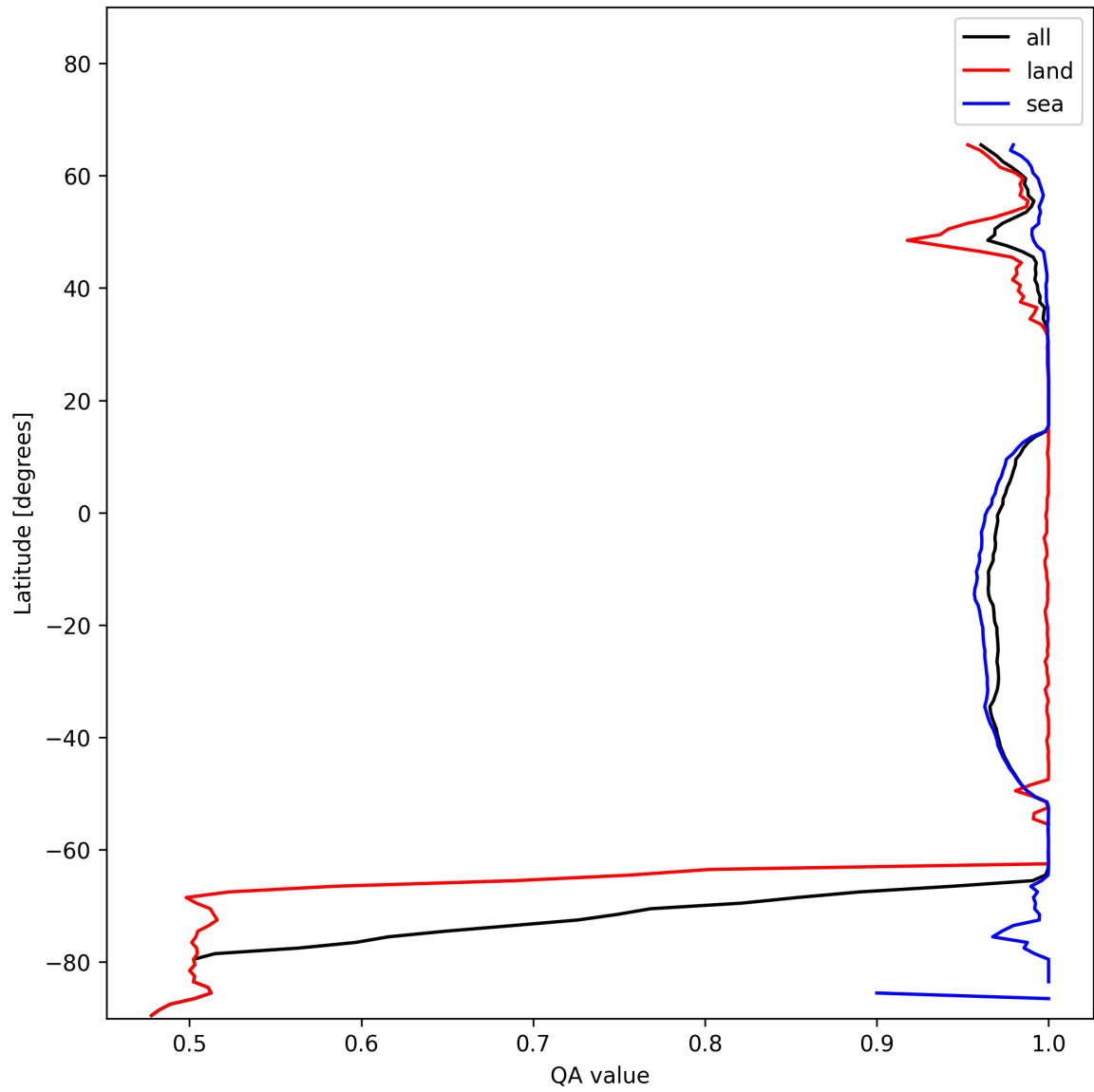
Figure 12: Zonal average of “QA value” for 2025-01-07 to 2025-01-09.
