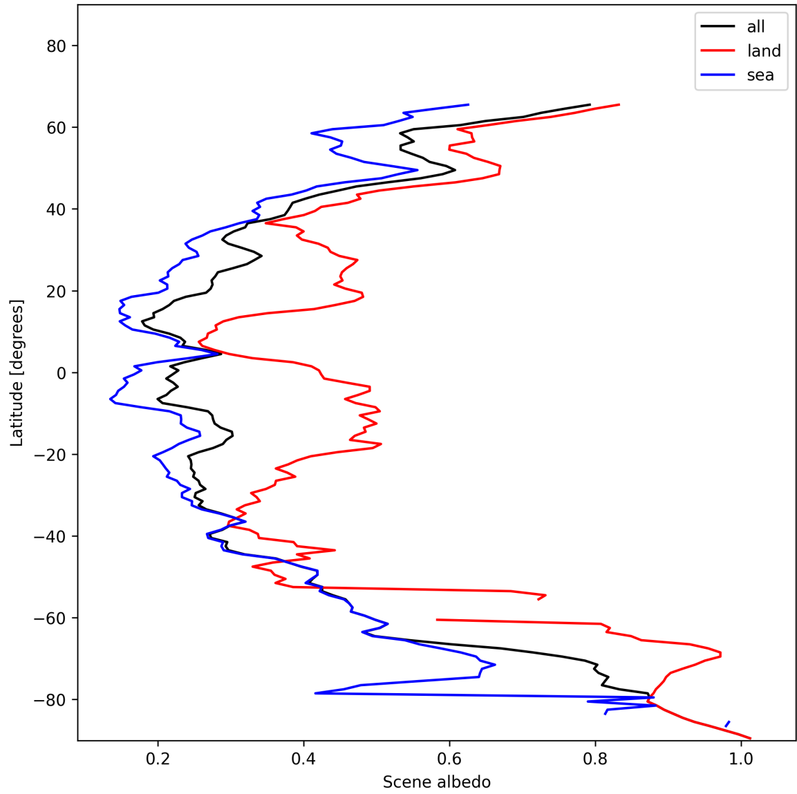
Figure 17: Zonal average of “Scene albedo” for 2025-01-07 to 2025-01-09.
