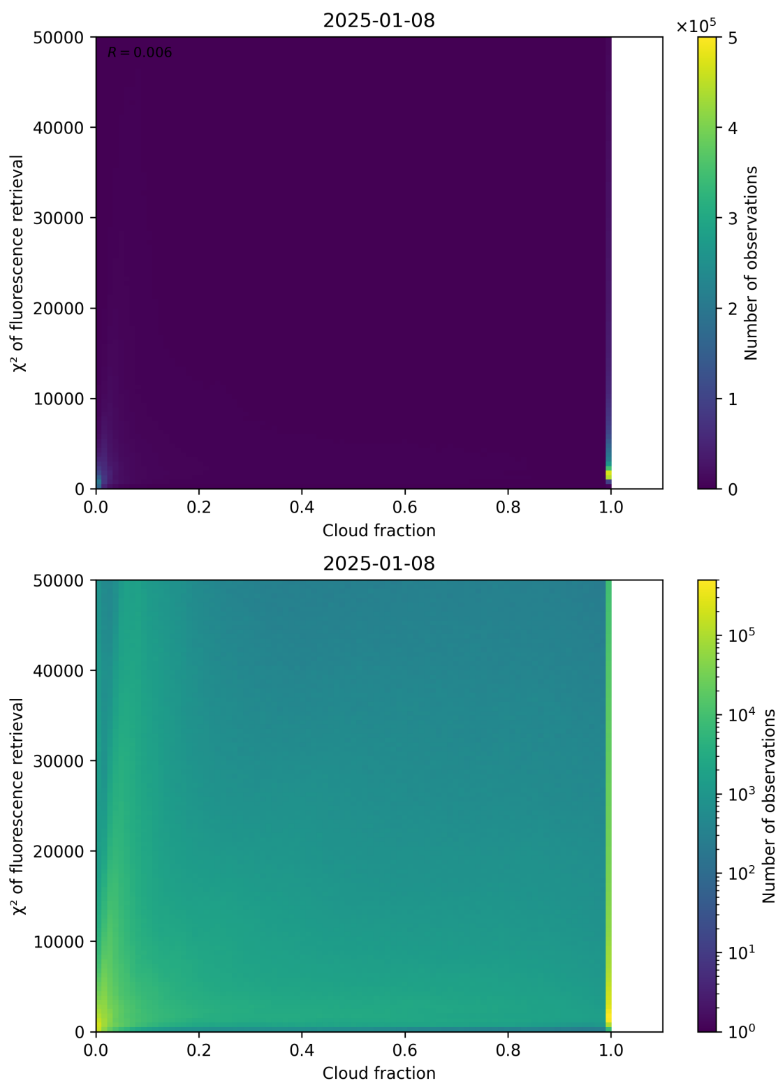
Figure 71: Scatter density plot of “Cloud fraction” against “ \chi^2 of fluorescence retrieval” for 2025-01-07 to 2025-01-09.
