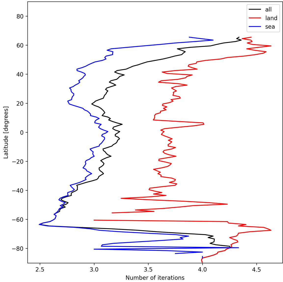
Figure 22: Zonal average of “Number of iterations” for 2025-01-07 to 2025-01-09.
