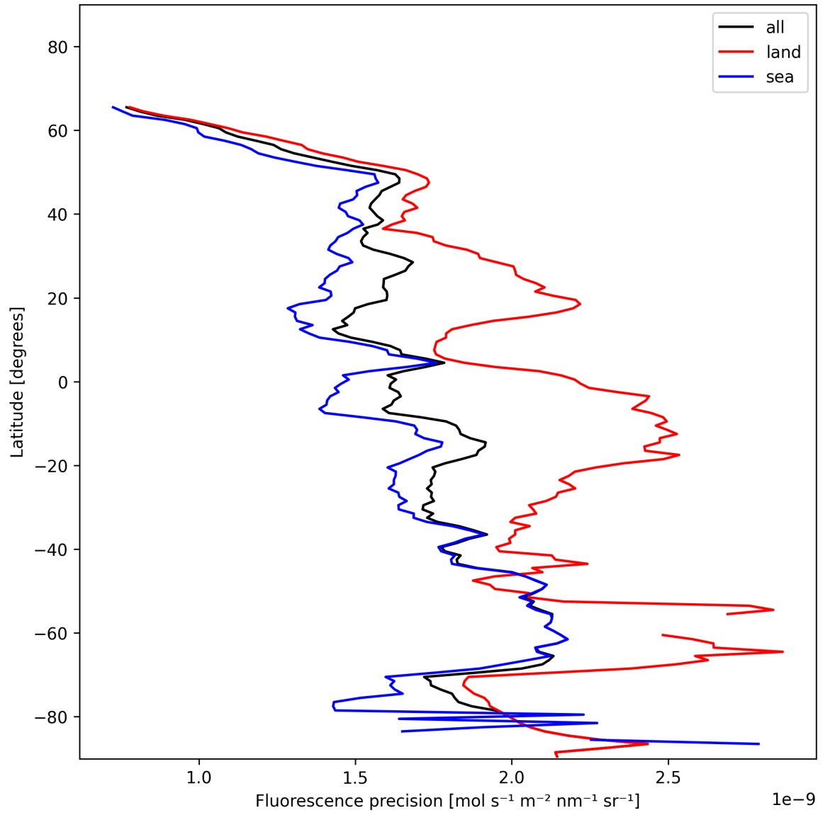
Figure 24: Zonal average of “Fluorescence precision” for 2025-01-07 to 2025-01-09.
