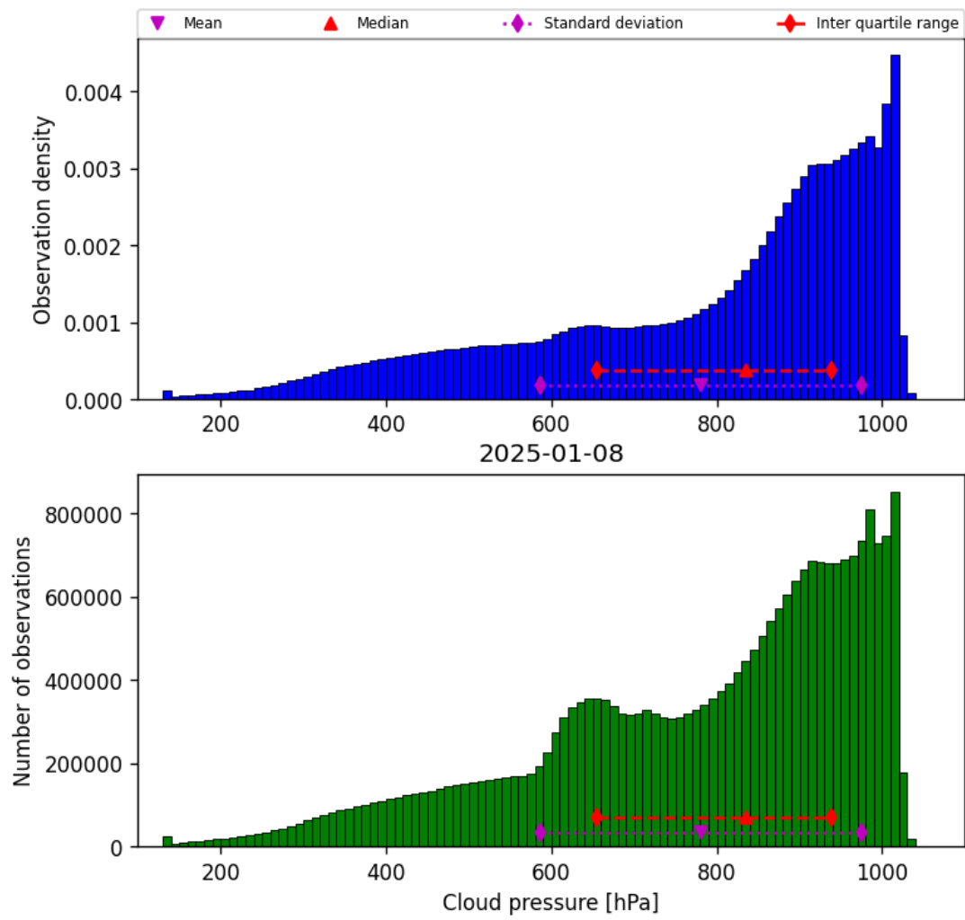
Figure 30: Histogram of “Cloud pressure” for 2025-01-07 to 2025-01-09
