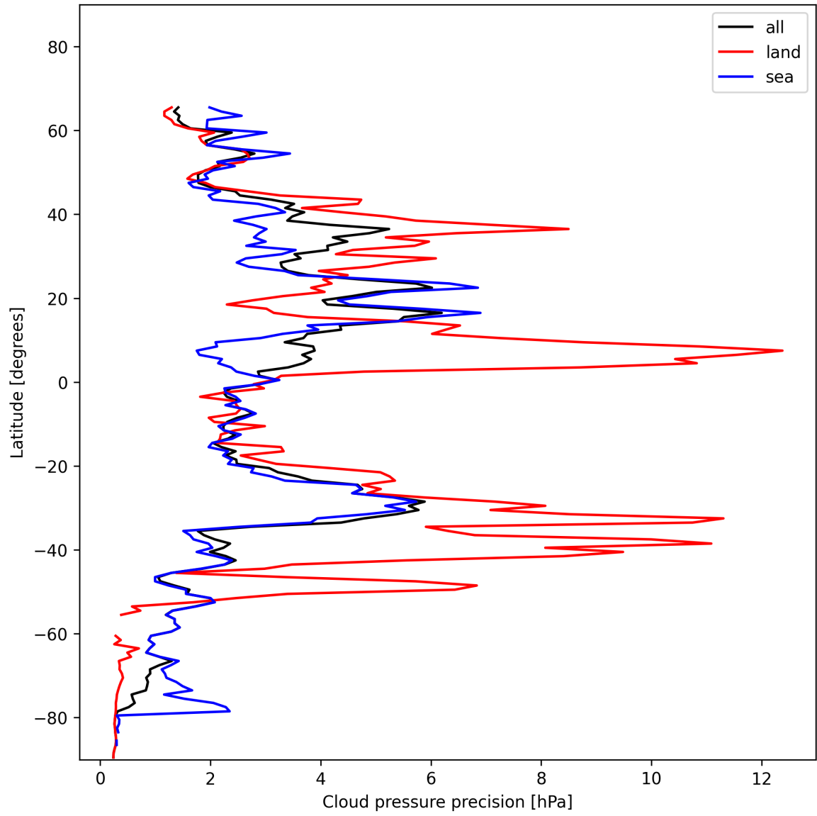
Figure 14: Zonal average of “Cloud pressure precision” for 2025-01-07 to 2025-01-09.
