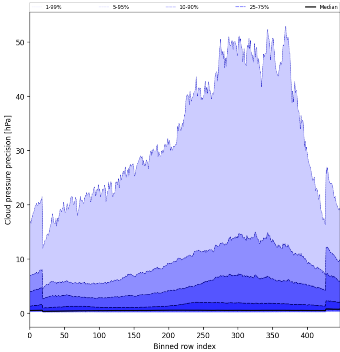
Figure 48: Along track statistics of “Cloud pressure precision” for 2025-01-07 to 2025-01-09
