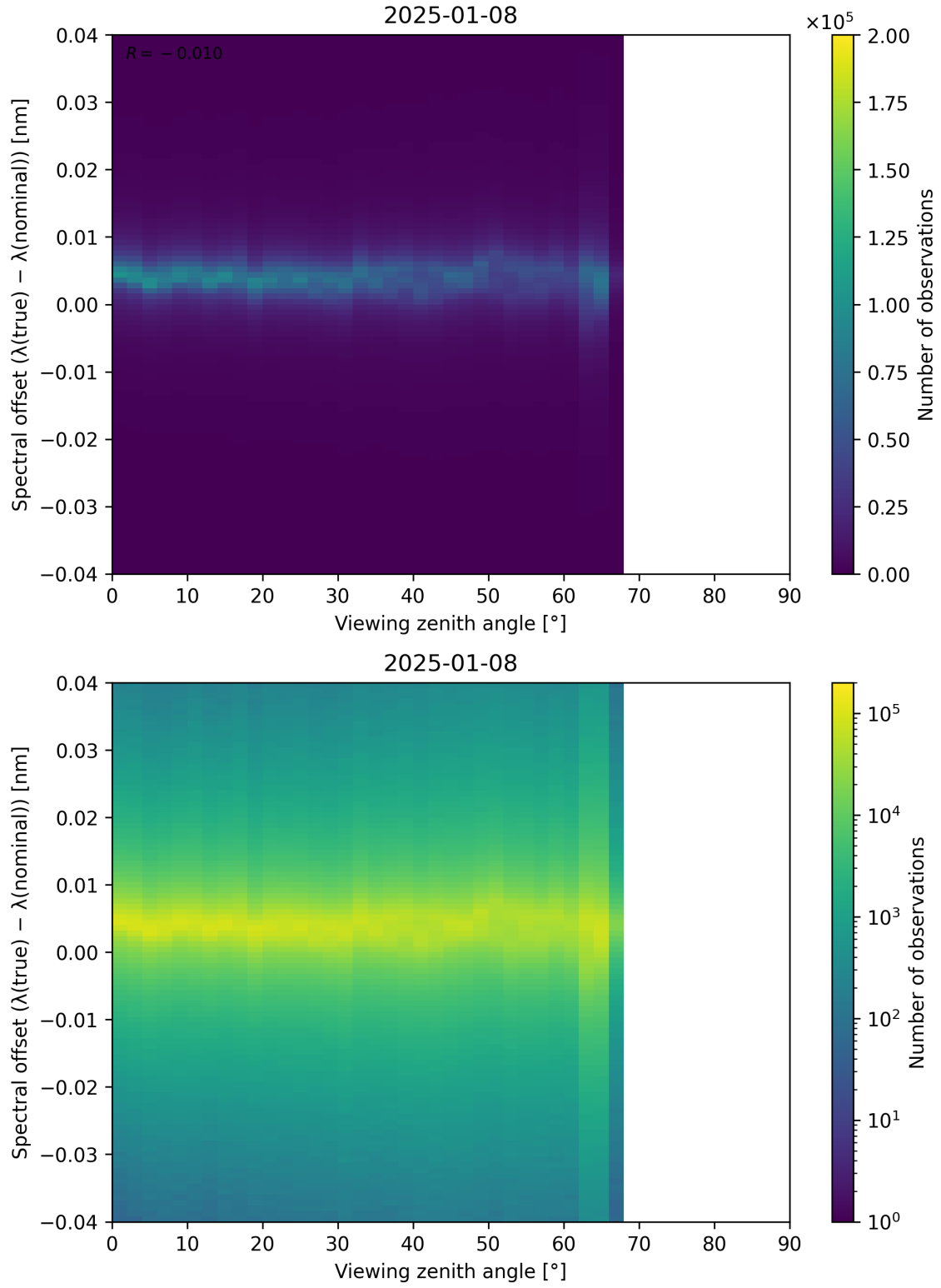
Figure 128: Scatter density plot of “Viewing zenith angle” against “Spectral offset ( \lambda_{\text{true}} - \lambda_{\text{nominal}} )” for 2025-01-07 to 2025-01-09.
