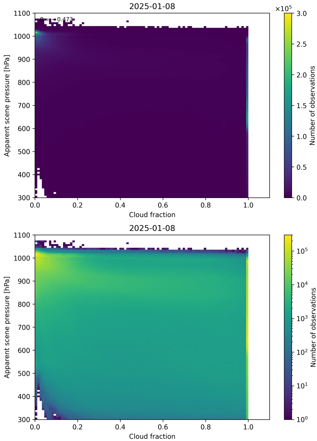
Figure 70: Scatter density plot of “Cloud fraction” against “Apparent scene pressure” for 2025-01-07 to 2025-01-09.
