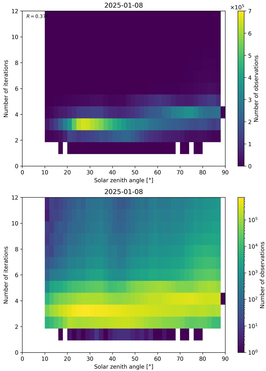
Figure 114: Scatter density plot of “Solar zenith angle” against “Number of iterations” for 2025-01-07 to 2025-01-09.
