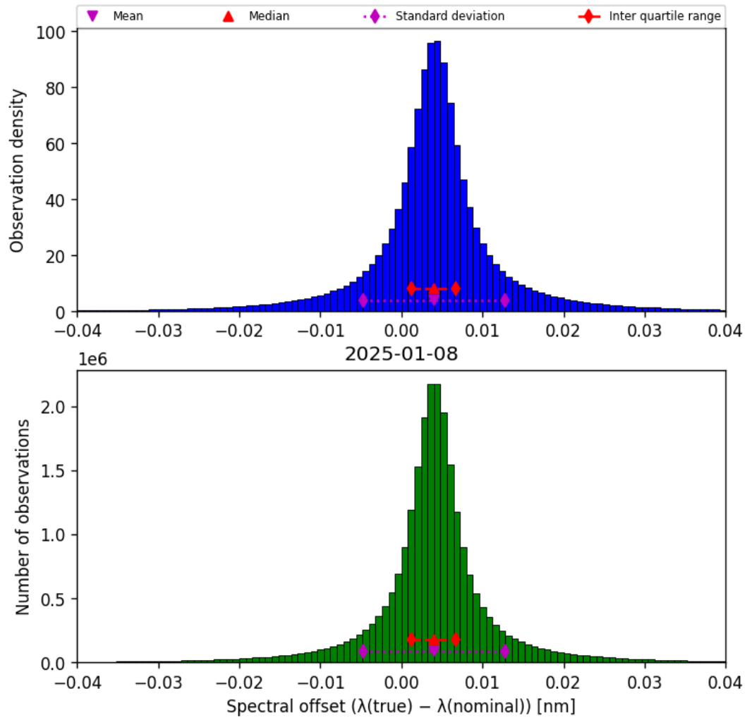
Figure 45: Histogram of “Spectral offset ( \lambda_{\text{true}} - \lambda_{\text{nominal}} )” for 2025-01-07 to 2025-01-09
