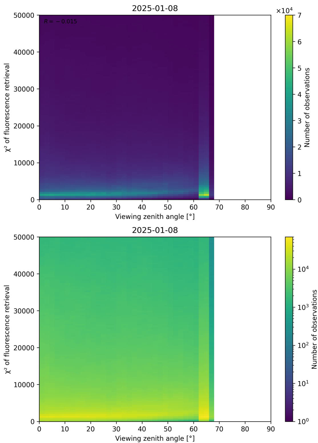
Figure 119: Scatter density plot of “Viewing zenith angle” against “ \chi^2 of fluorescence retrieval” for 2025-01-07 to 2025-01-09.
