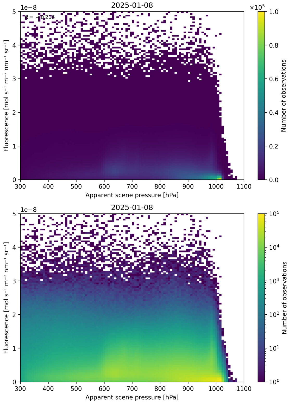
Figure 64: Scatter density plot of “Apparent scene pressure” against “Fluorescence” for 2025-01-07 to 2025-01-09.
