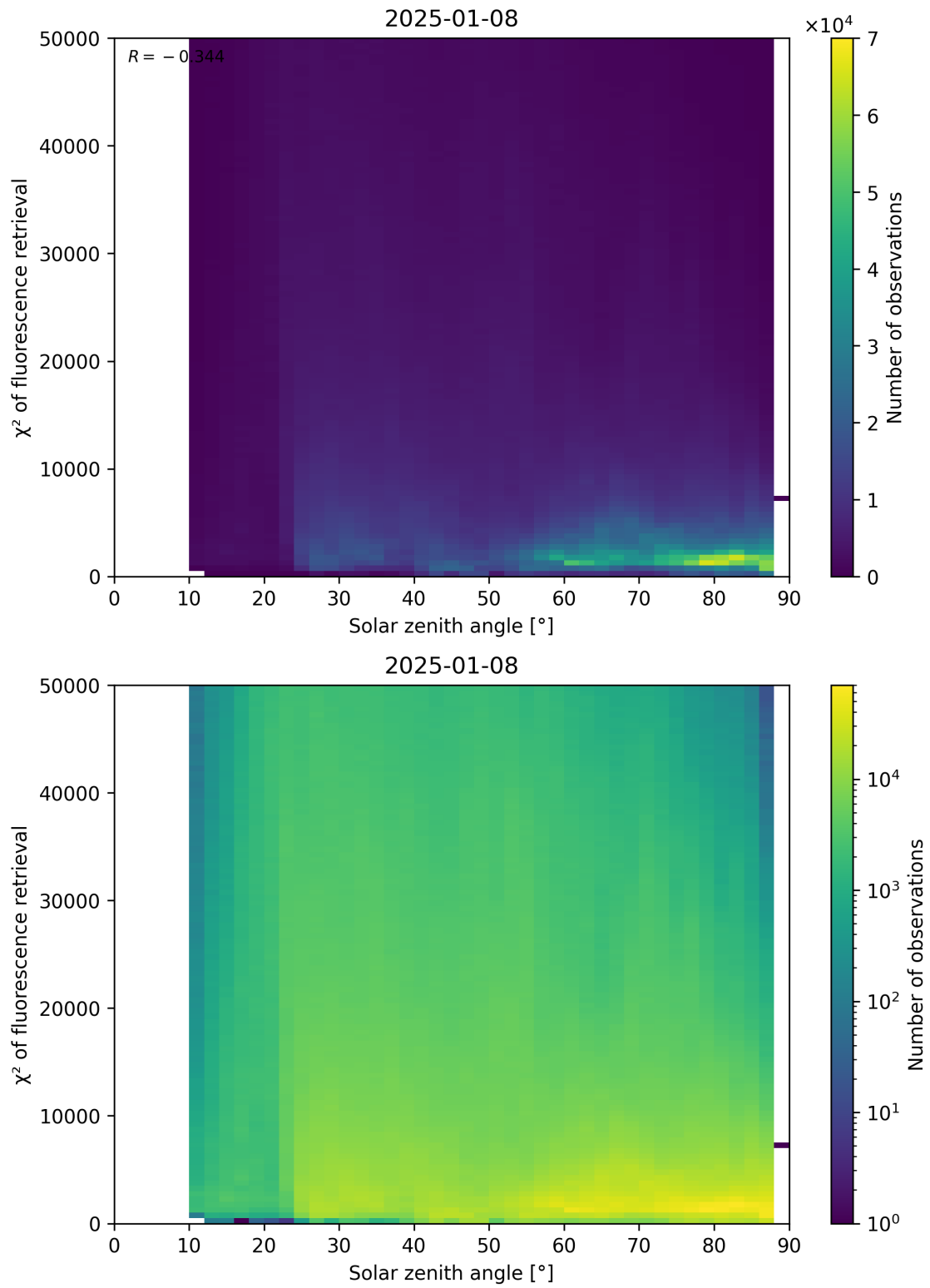
Figure 109: Scatter density plot of “Solar zenith angle” against “ \chi^2 of fluorescence retrieval” for 2025-01-07 to 2025-01-09.
