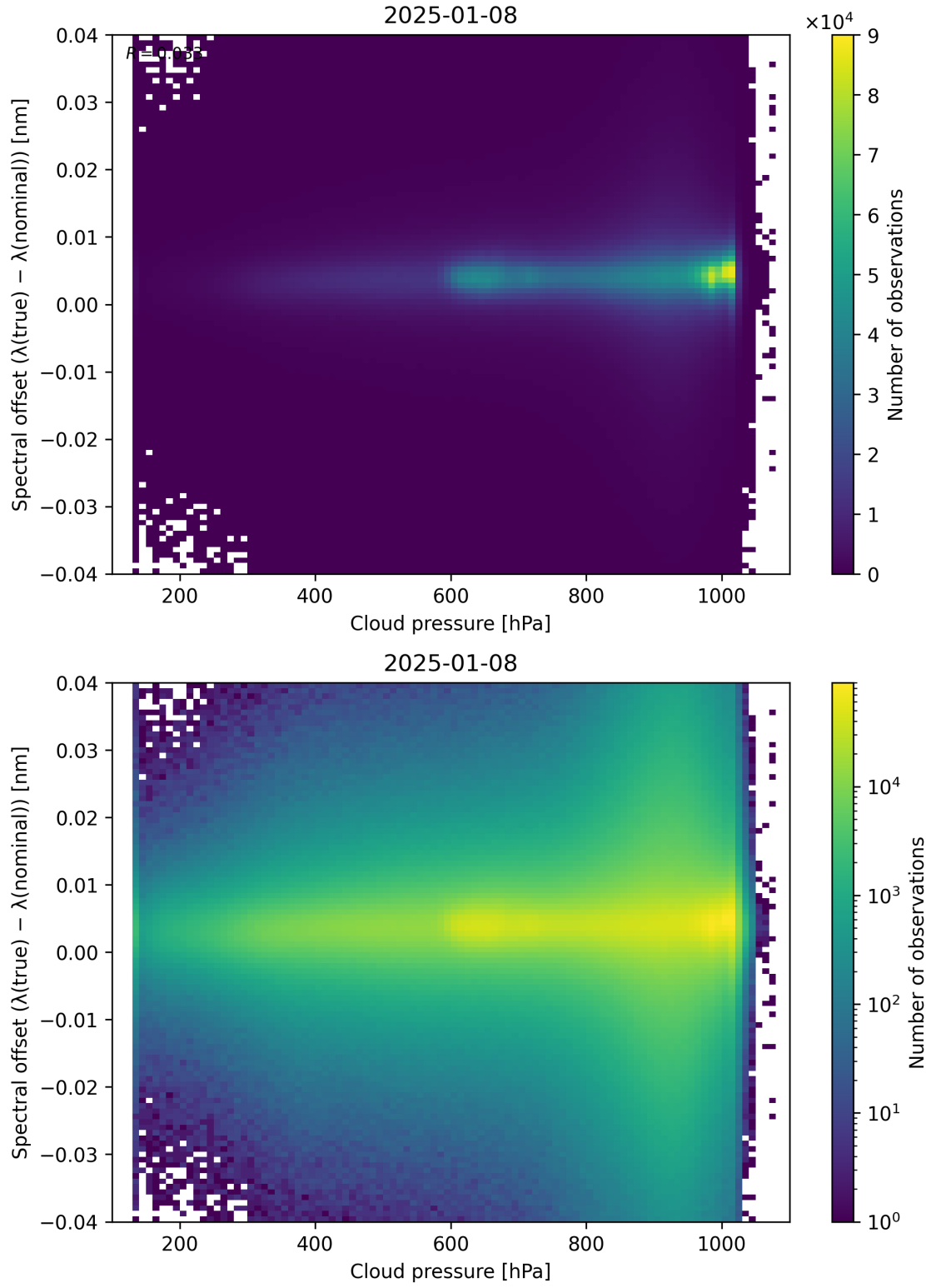
Figure 84: Scatter density plot of “Cloud pressure” against “Spectral offset ( \lambda_{\text{true}} - \lambda_{\text{nominal}} )” for 2025-01-07 to 2025-01-09.
