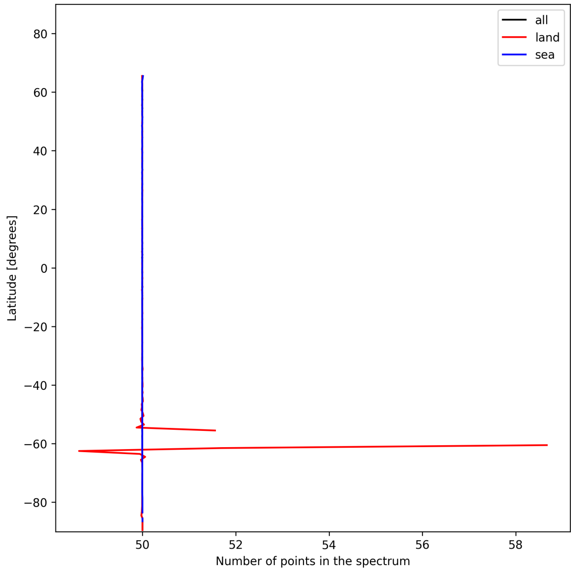
Figure 27: Zonal average of “Number of points in the spectrum” for 2025-01-07 to 2025-01-09.
