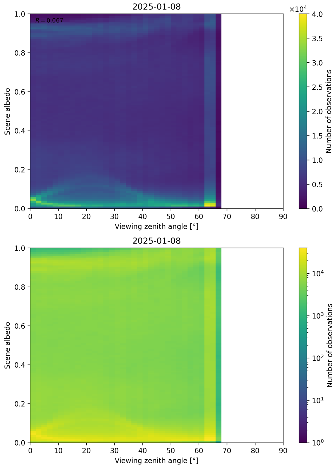
Figure 126: Scatter density plot of “Viewing zenith angle” against “Scene albedo” for 2025-01-07 to 2025-01-09.
