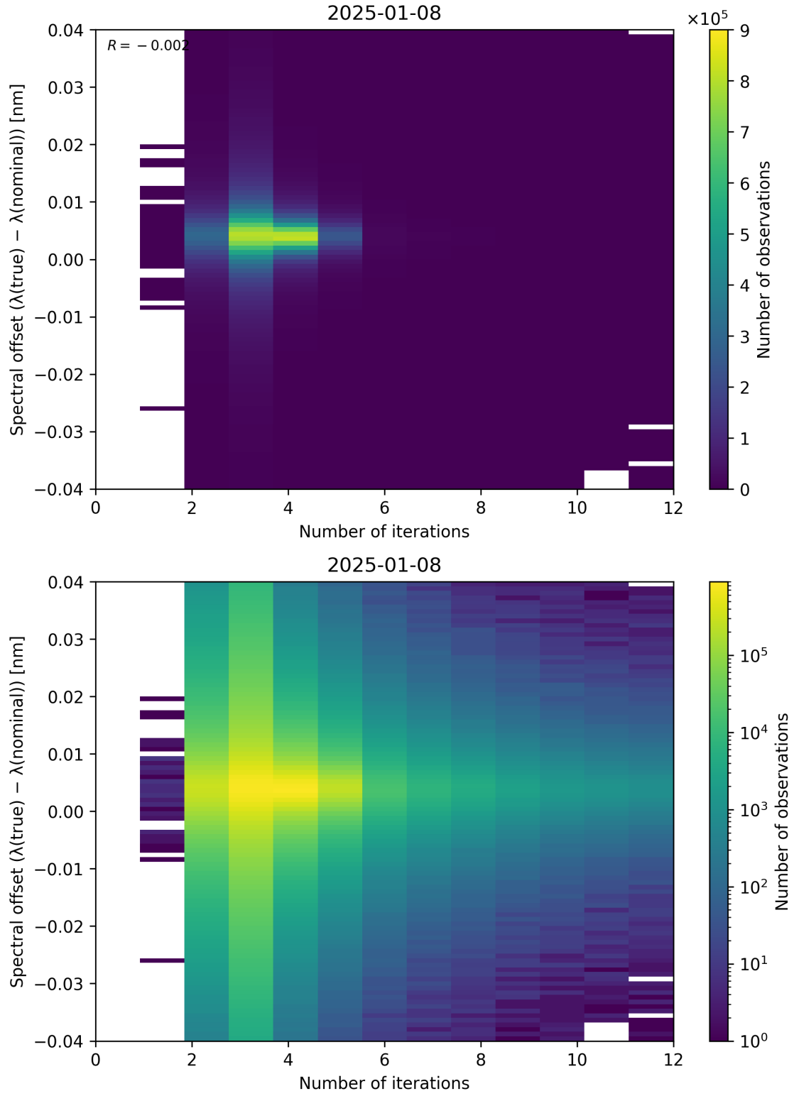
Figure 100: Scatter density plot of “Number of iterations” against “Spectral offset ( \lambda_{\text{true}} - \lambda_{\text{nominal}} )” for 2025-01-07 to 2025-01-09.
