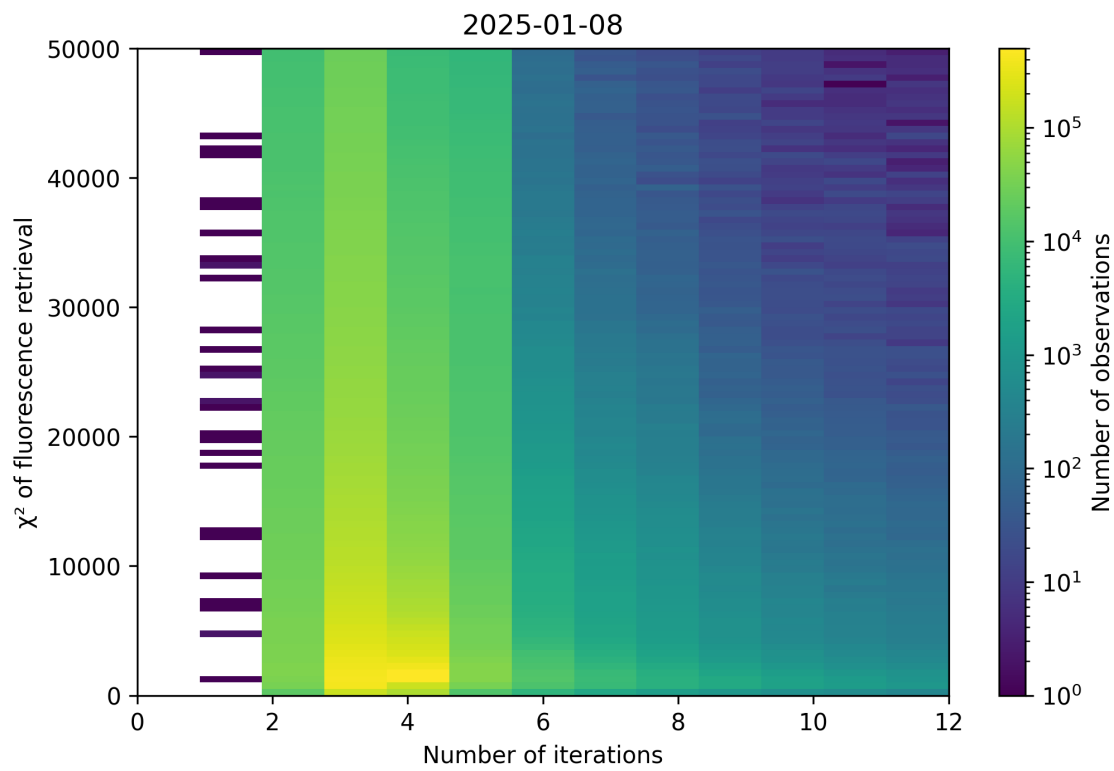
Figure 97: Scatter density plot of “Number of iterations” against “ \chi^2 of fluorescence retrieval” for 2025-01-07 to 2025-01-09.
