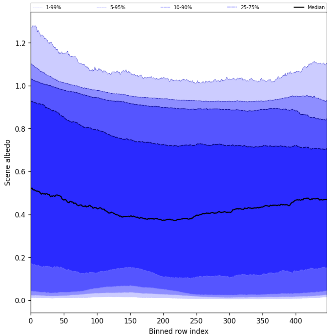
Figure 51: Along track statistics of “Scene albedo” for 2025-01-07 to 2025-01-09
