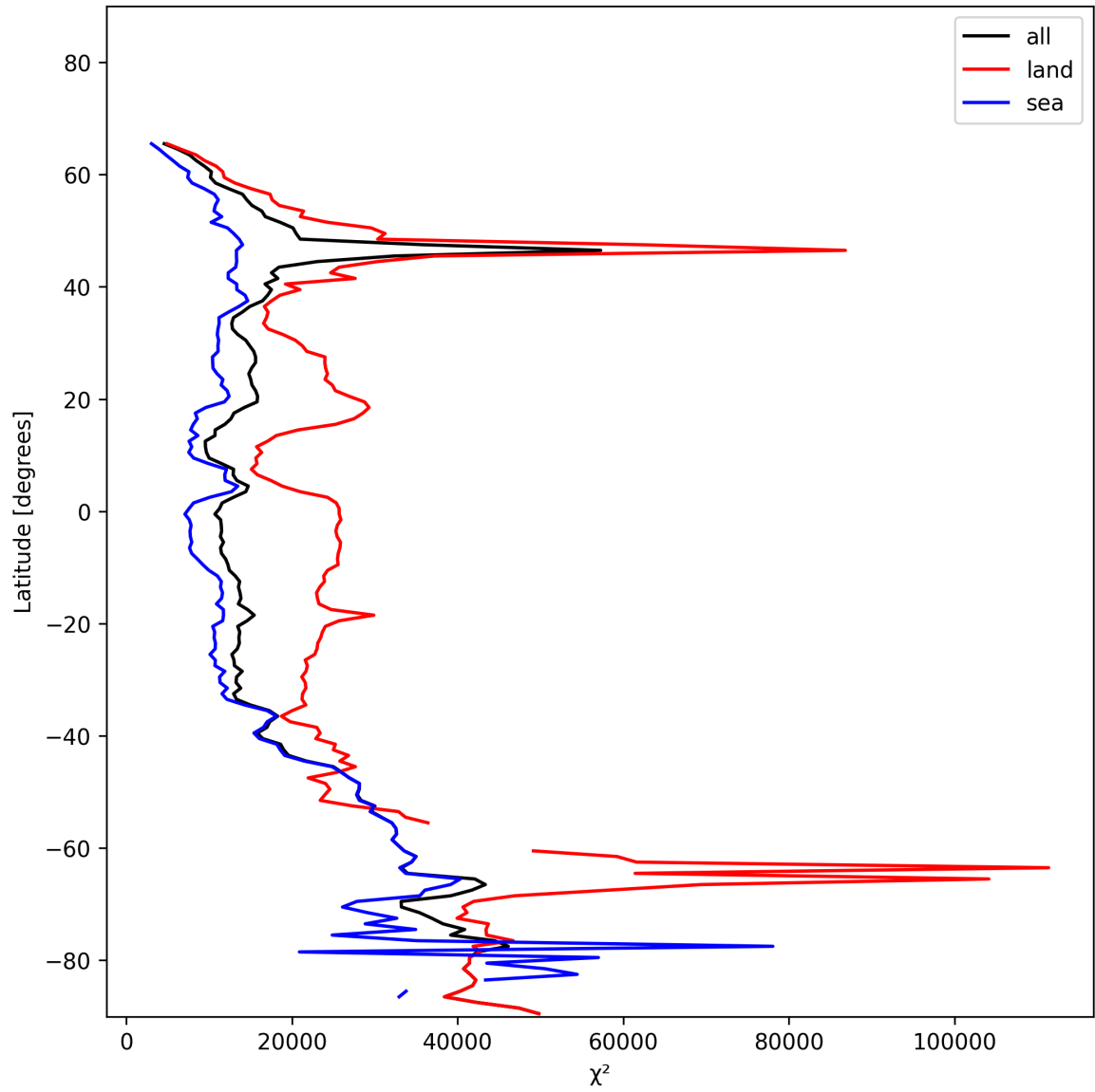
Figure 21: Zonal average of “ \chi^2 ” for 2025-01-07 to 2025-01-09.
