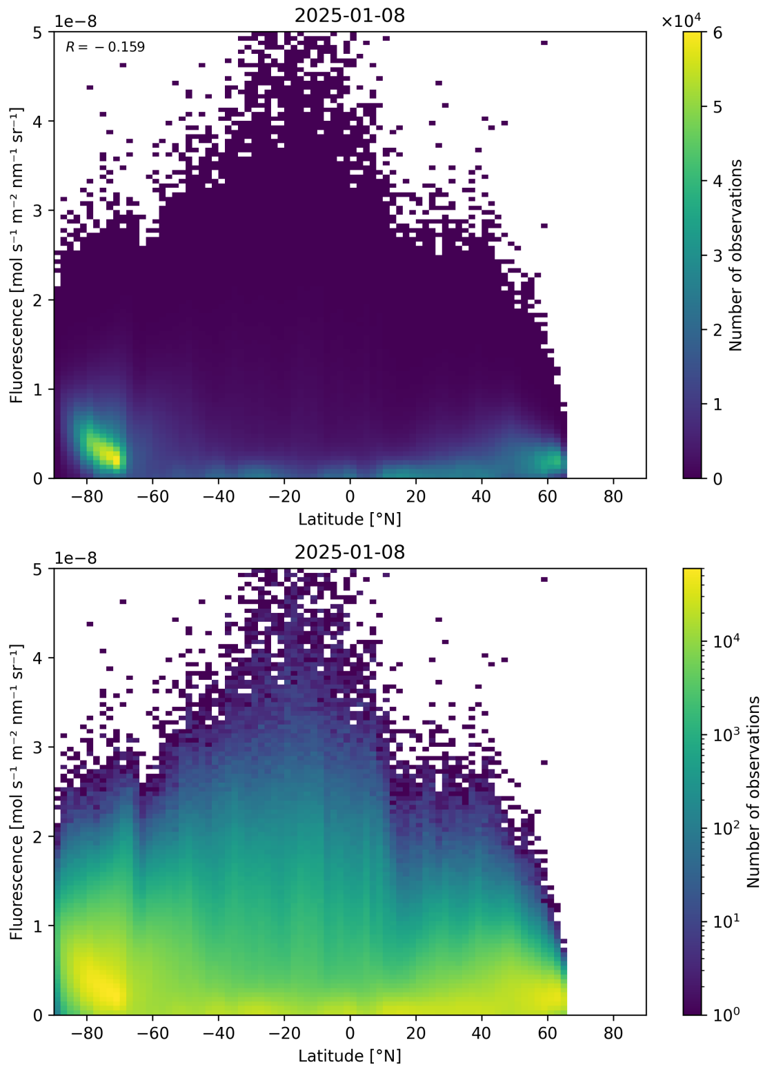
Figure 92: Scatter density plot of “Latitude” against “Fluorescence” for 2025-01-07 to 2025-01-09.
