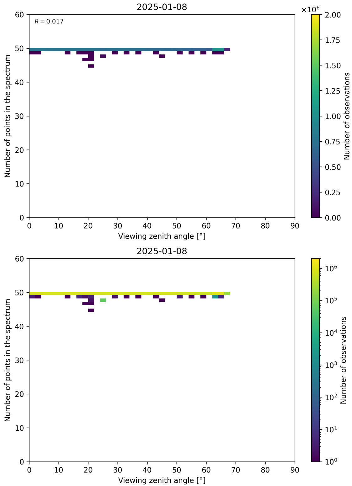
Figure 125: Scatter density plot of “Viewing zenith angle” against “Number of points in the spectrum” for 2025-01-07 to 2025-01-09.
