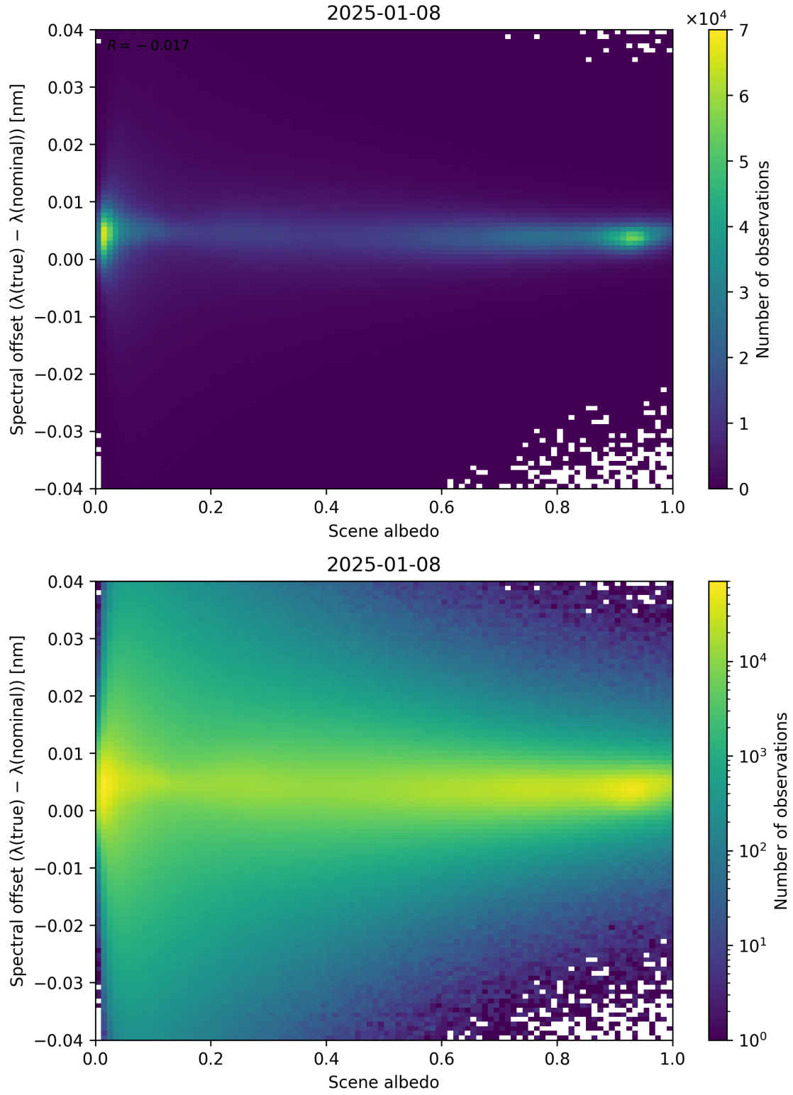
Figure 107: Scatter density plot of “Scene albedo” against “Spectral offset ( \lambda_{\text{true}} - \lambda_{\text{nominal}} )” for 2025-01-07 to 2025-01-09.
