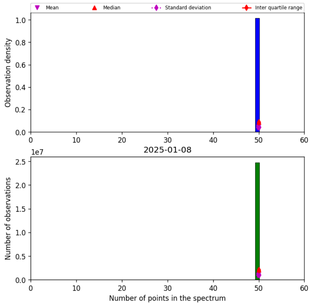
Figure 44: Histogram of “Number of points in the spectrum” for 2025-01-07 to 2025-01-09
