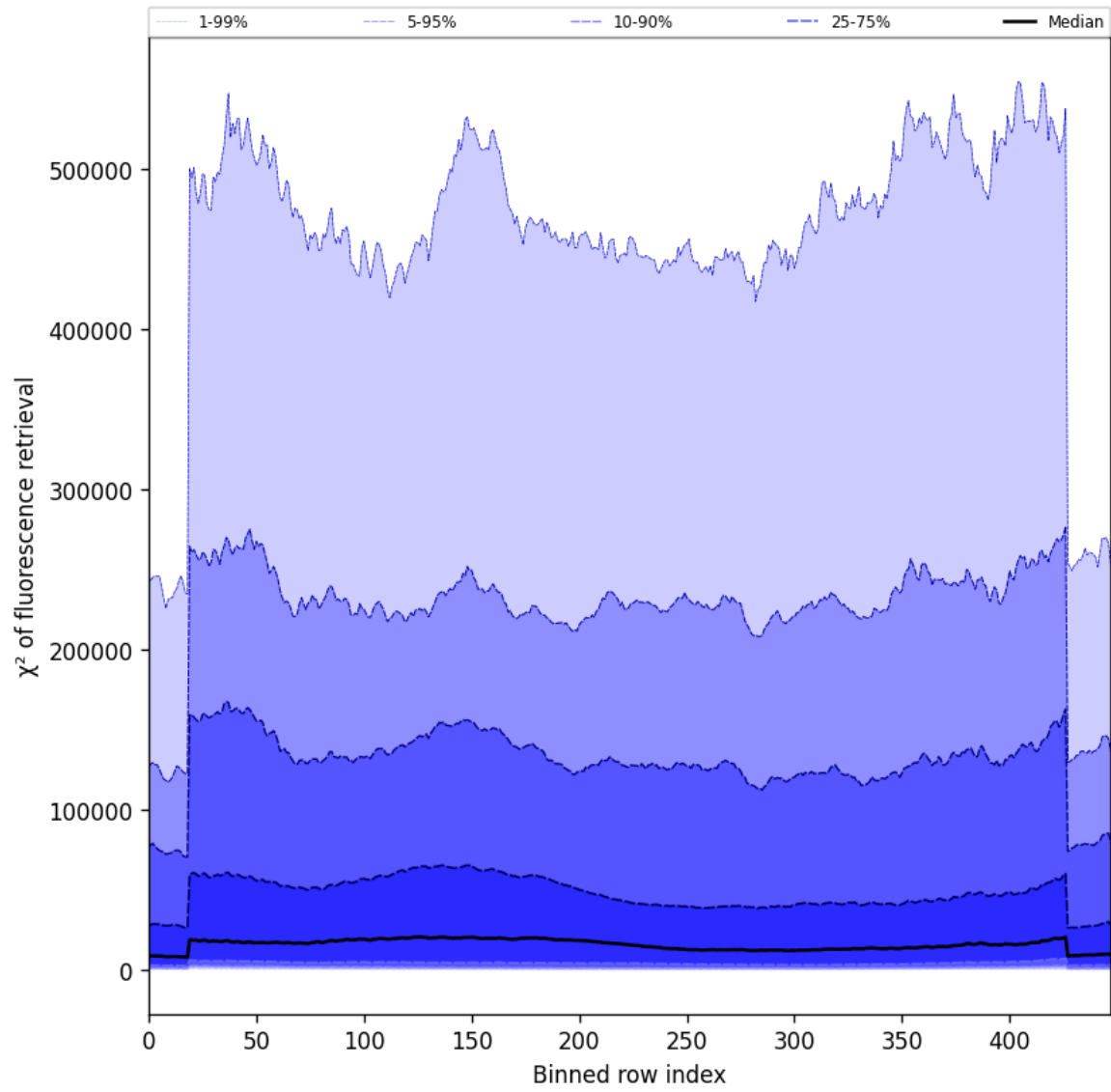
Figure 59: Along track statistics of “ \chi^2 of fluorescence retrieval” for 2025-01-07 to 2025-01-09
