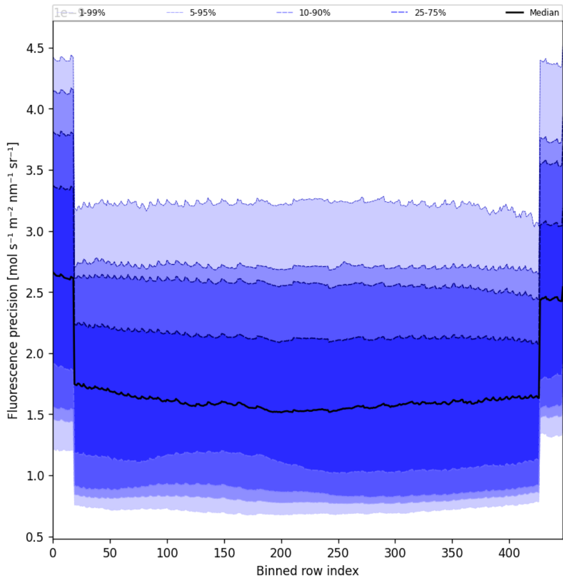
Figure 58: Along track statistics of “Fluorescence precision” for 2025-01-07 to 2025-01-09
