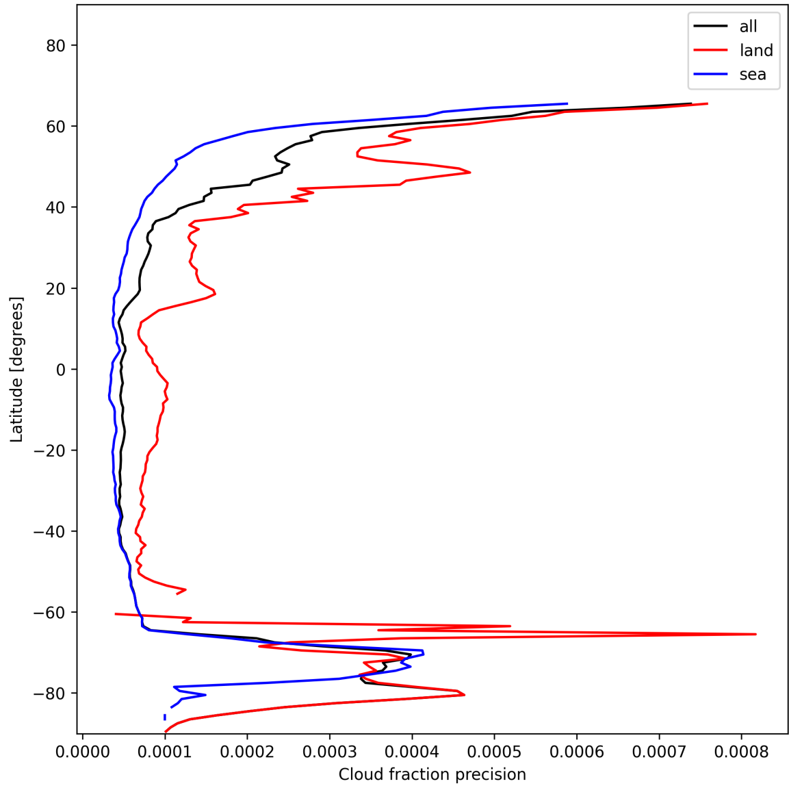
Figure 16: Zonal average of “Cloud fraction precision” for 2025-01-07 to 2025-01-09.
