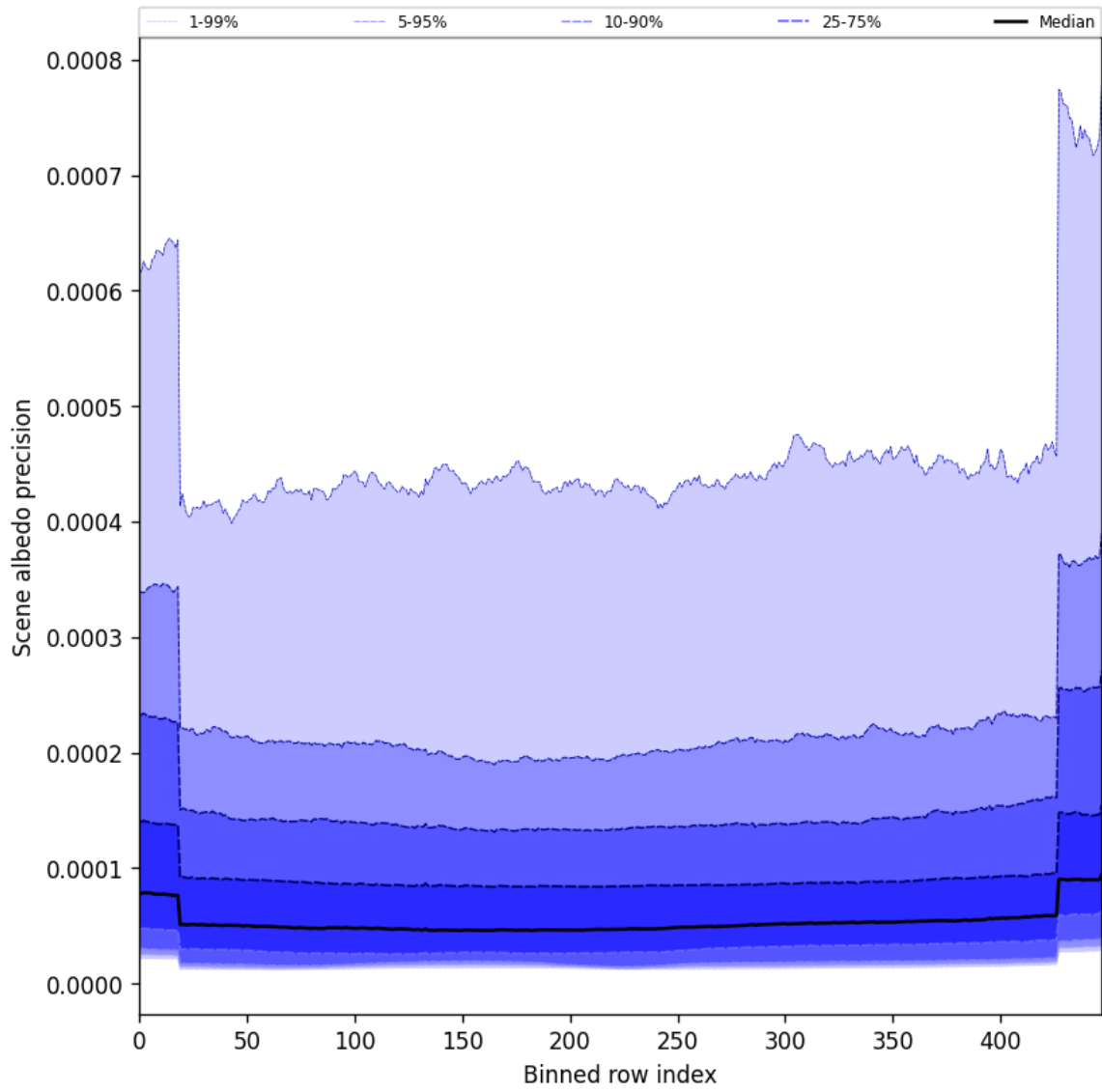
Figure 52: Along track statistics of “Scene albedo precision” for 2025-01-07 to 2025-01-09
