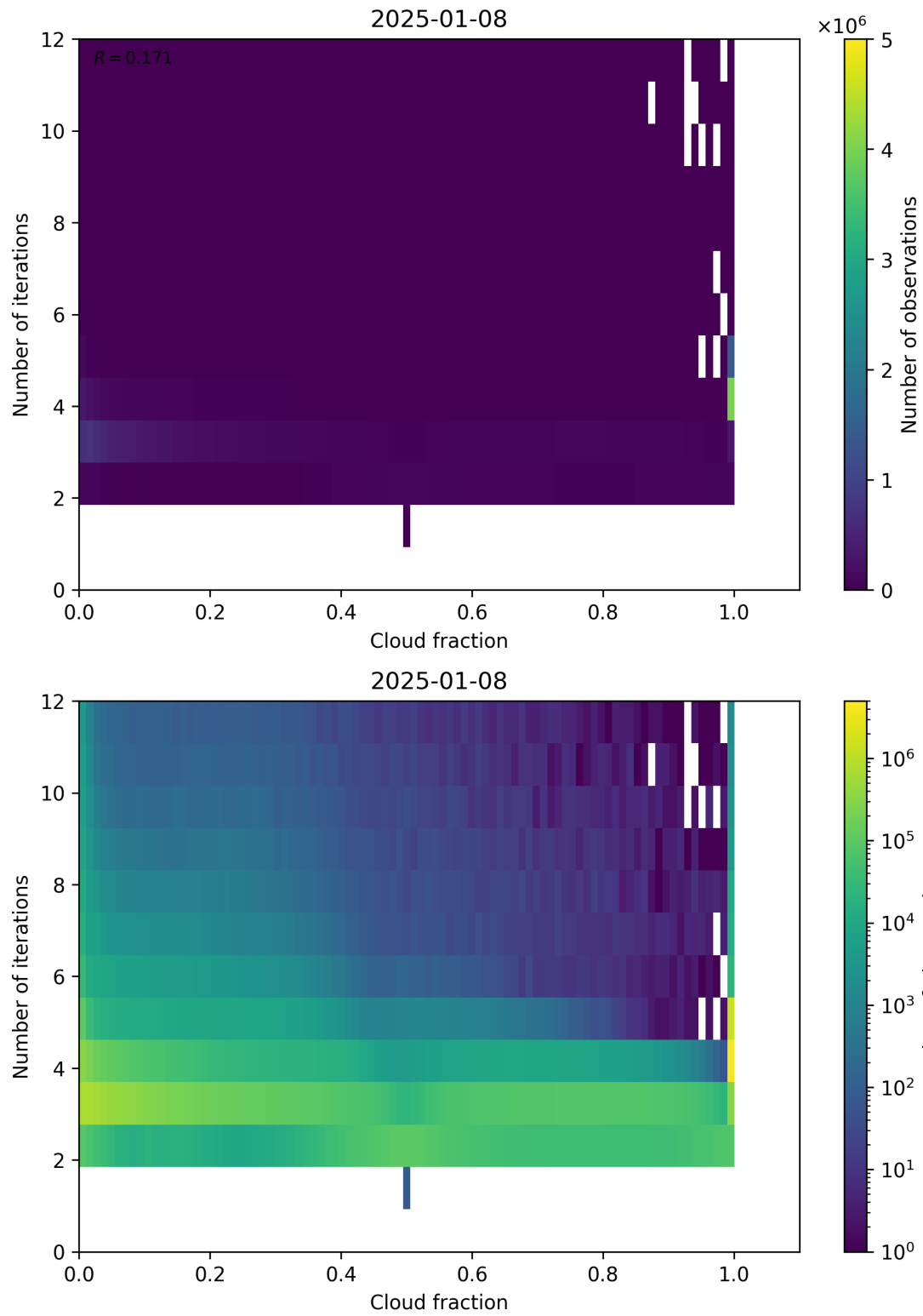
Figure 73: Scatter density plot of “Cloud fraction” against “Number of iterations” for 2025-01-07 to 2025-01-09.
