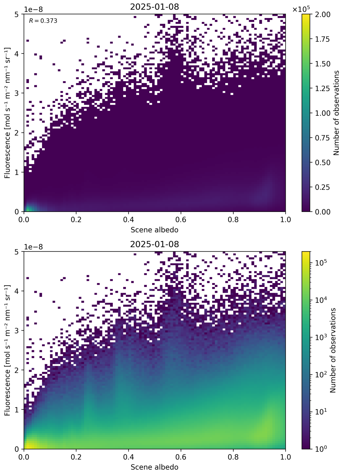
Figure 104: Scatter density plot of “Scene albedo” against “Fluorescence” for 2025-01-07 to 2025-01-09.
