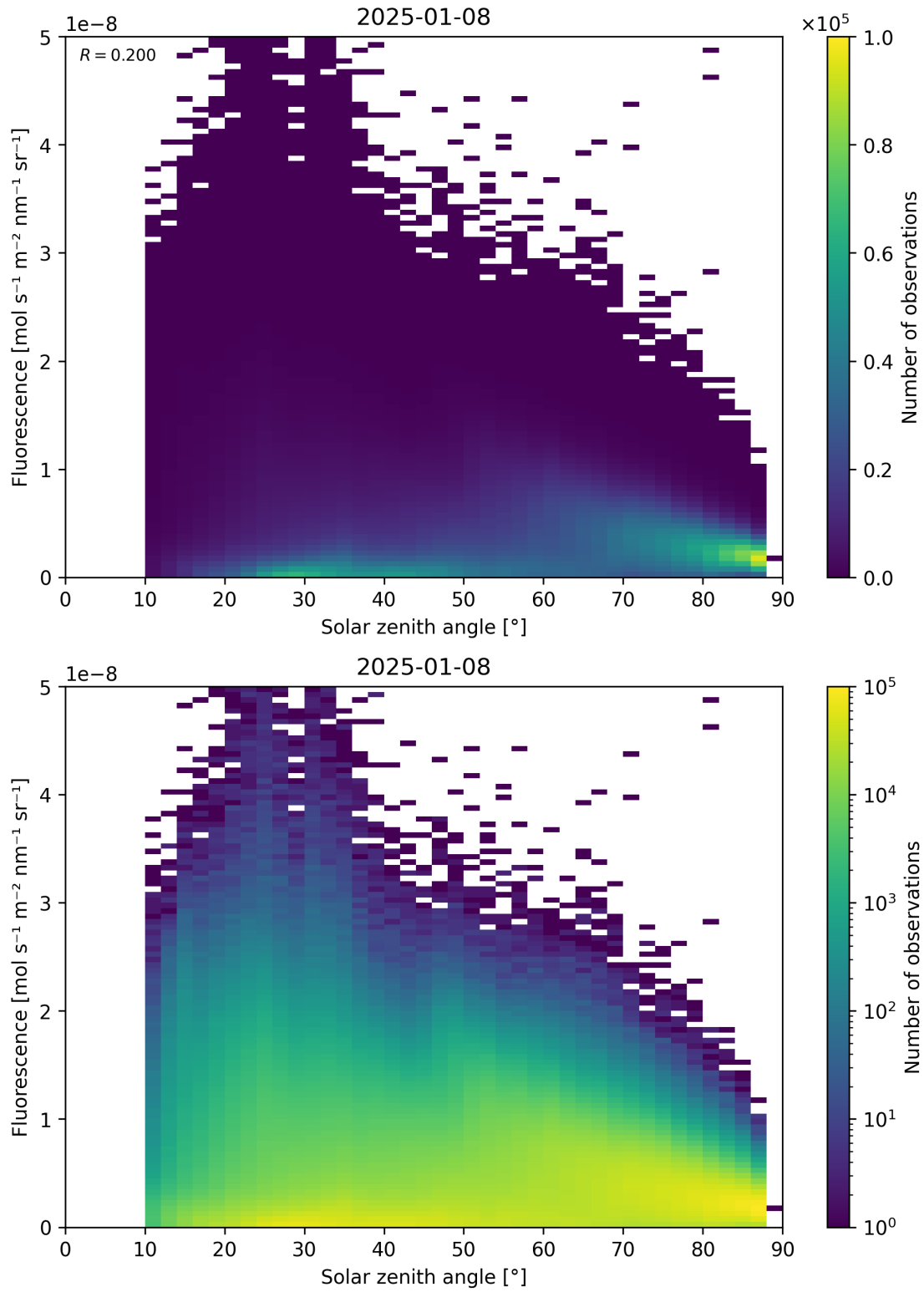
Figure 112: Scatter density plot of “Solar zenith angle” against “Fluorescence” for 2025-01-07 to 2025-01-09.
