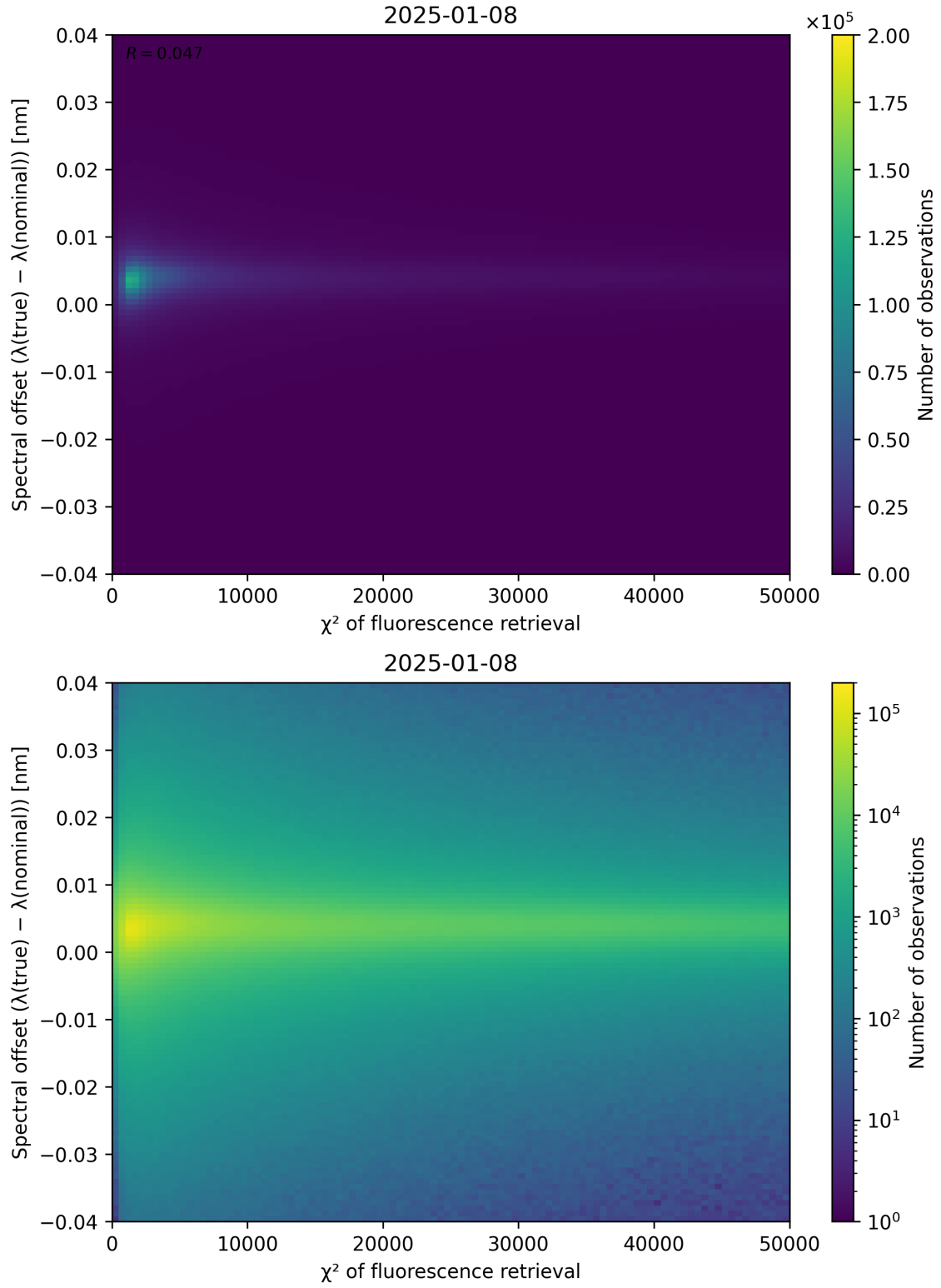
Figure 69: Scatter density plot of “ \chi^2 of fluorescence retrieval” against “Spectral offset ( \lambda_{\text{true}} - \lambda_{\text{nominal}} )” for 2025-01-07 to 2025-01-09.
