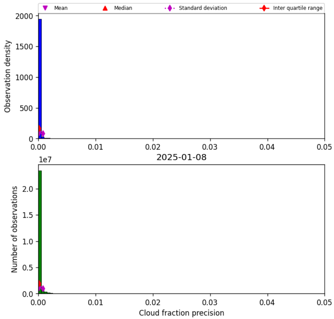
Figure 33: Histogram of “Cloud fraction precision” for 2025-01-07 to 2025-01-09
