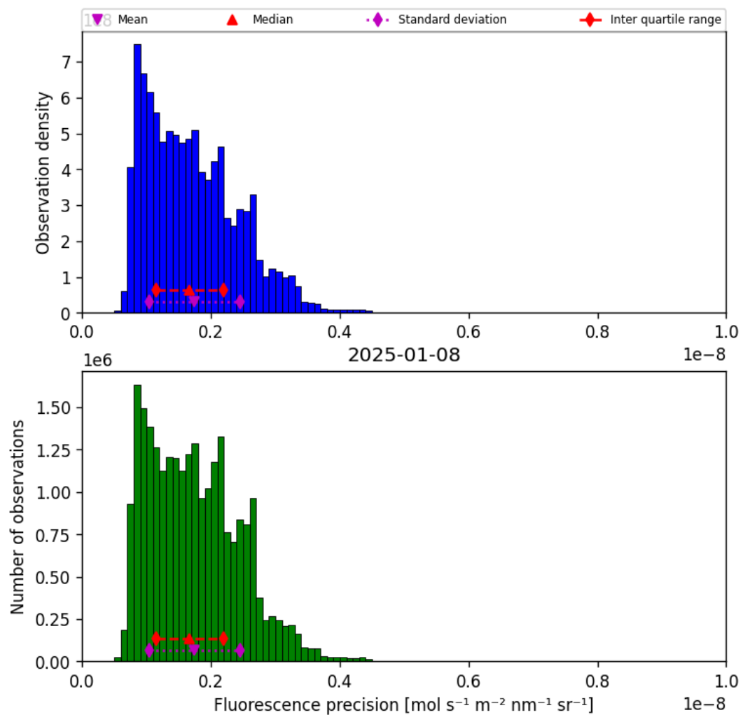
Figure 41: Histogram of “Fluorescence precision” for 2025-01-07 to 2025-01-09
