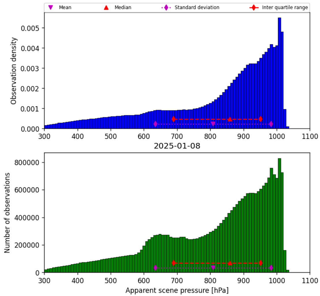
Figure 36: Histogram of “Apparent scene pressure” for 2025-01-07 to 2025-01-09
