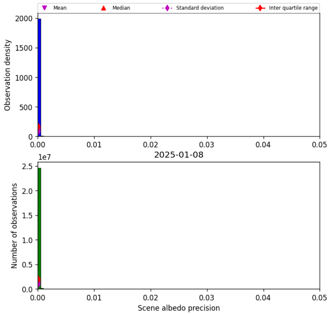
Figure 35: Histogram of “Scene albedo precision” for 2025-01-07 to 2025-01-09
