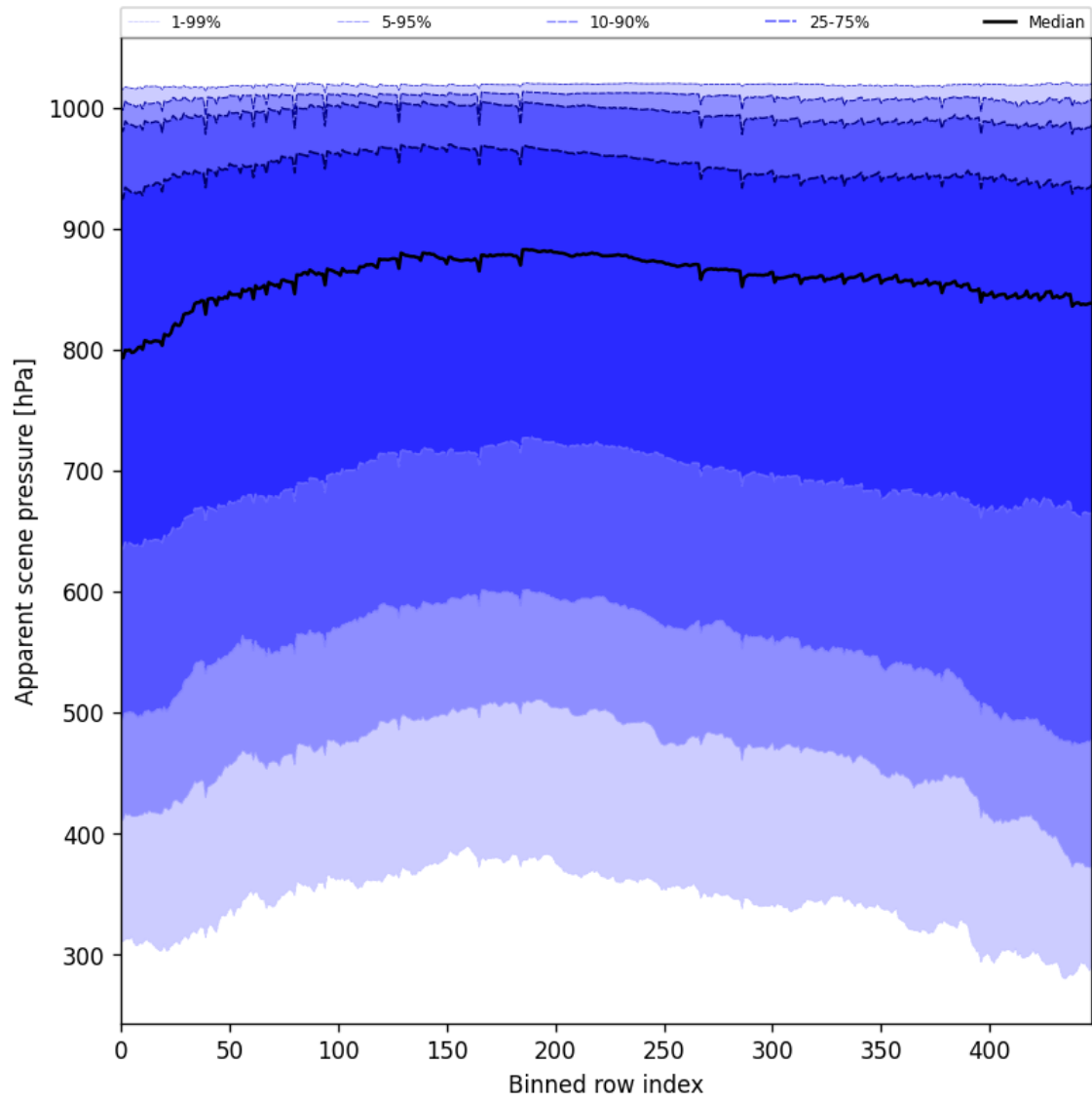
Figure 53: Along track statistics of “Apparent scene pressure” for 2025-01-07 to 2025-01-09
