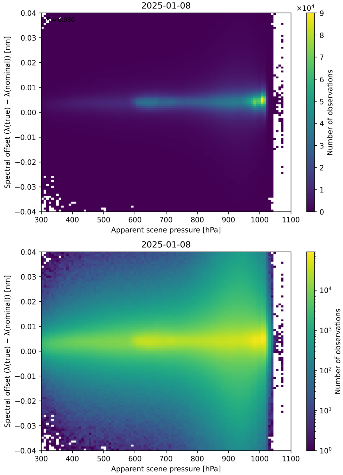
Figure 67: Scatter density plot of “Apparent scene pressure” against “Spectral offset ( \lambda_{\text{true}} - \lambda_{\text{nominal}} )” for 2025-01-07 to 2025-01-09.
