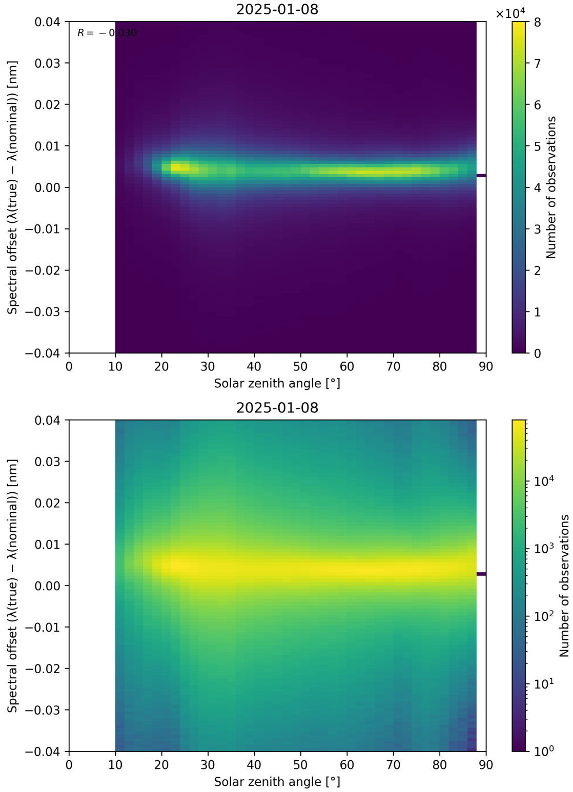
Figure 117: Scatter density plot of “Solar zenith angle” against “Spectral offset ( \lambda_{\text{true}} - \lambda_{\text{nominal}} )” for 2025-01-07 to 2025-01-09.
