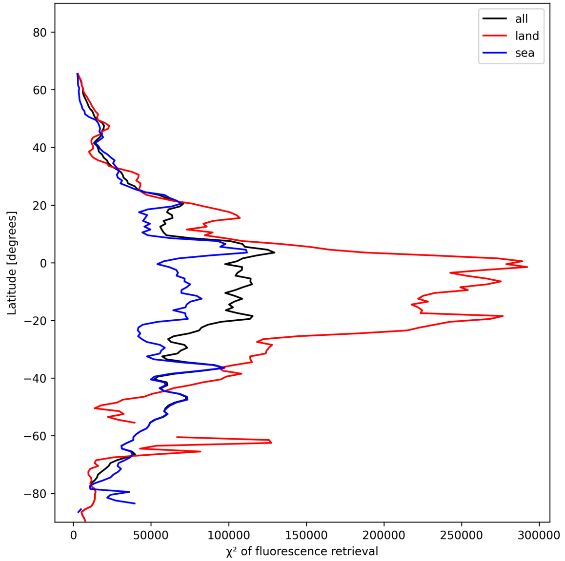
Figure 25: Zonal average of “ \chi^2 of fluorescence retrieval” for 2025-01-07 to 2025-01-09.
