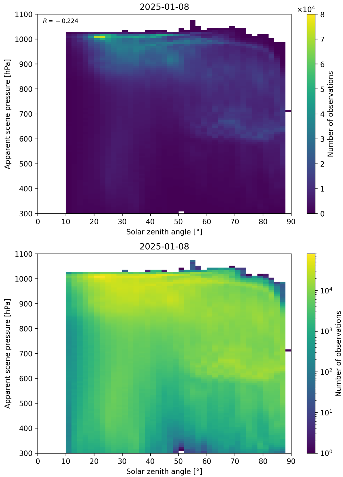
Figure 108: Scatter density plot of “Solar zenith angle” against “Apparent scene pressure” for 2025-01-07 to 2025-01-09.
