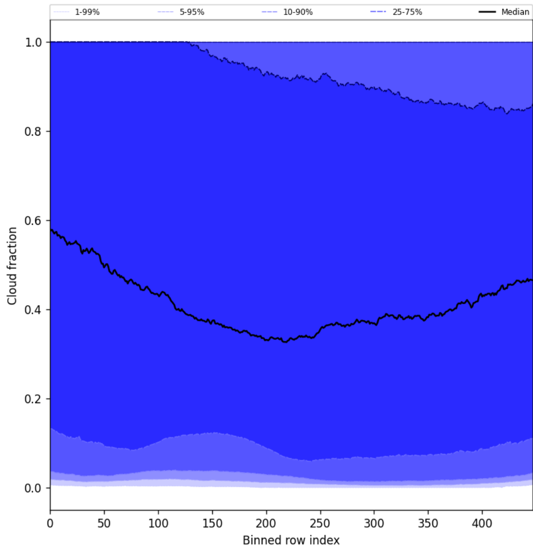
Figure 49: Along track statistics of “Cloud fraction” for 2025-01-07 to 2025-01-09
