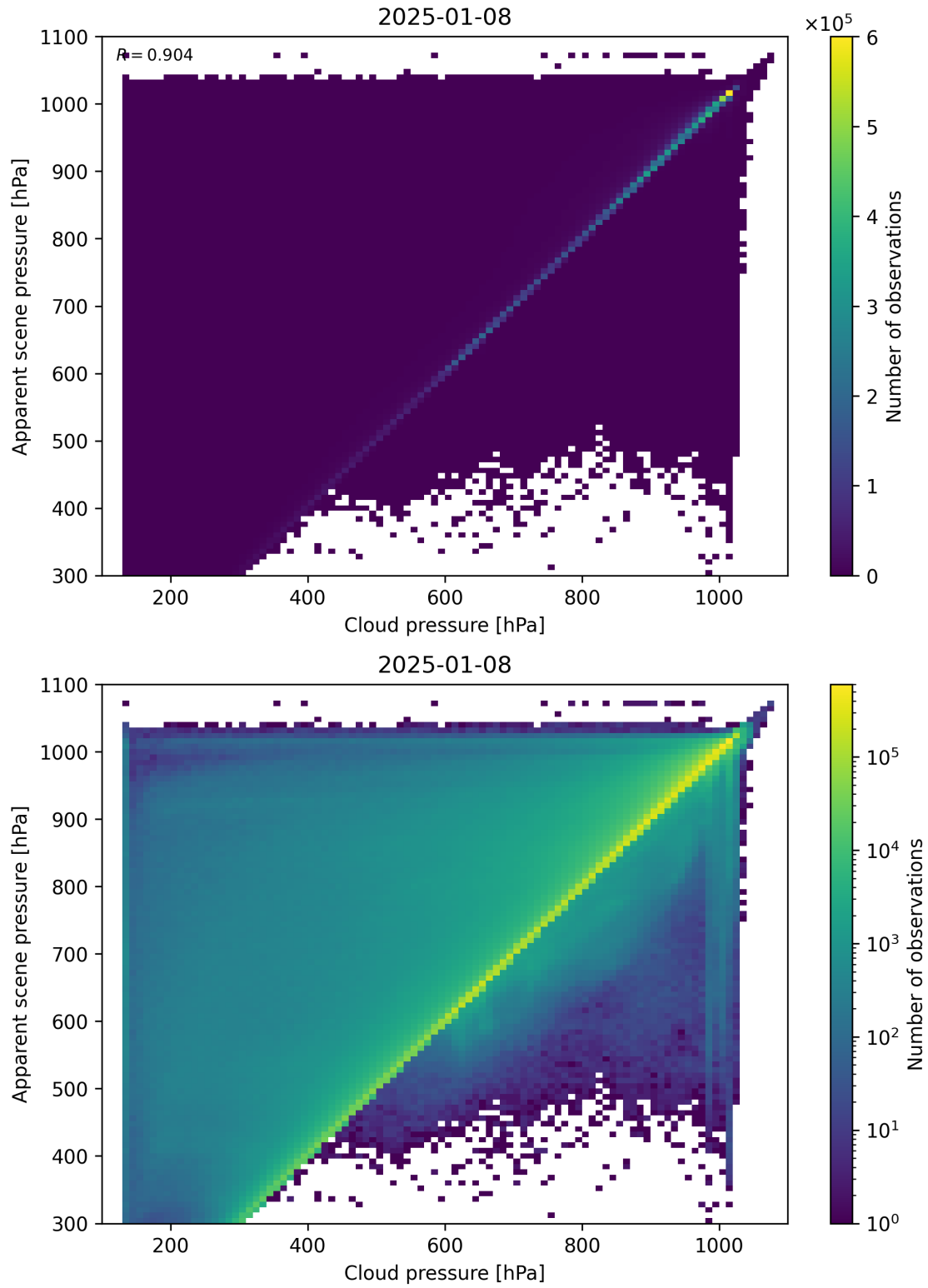
Figure 77: Scatter density plot of “Cloud pressure” against “Apparent scene pressure” for 2025-01-07 to 2025-01-09.
