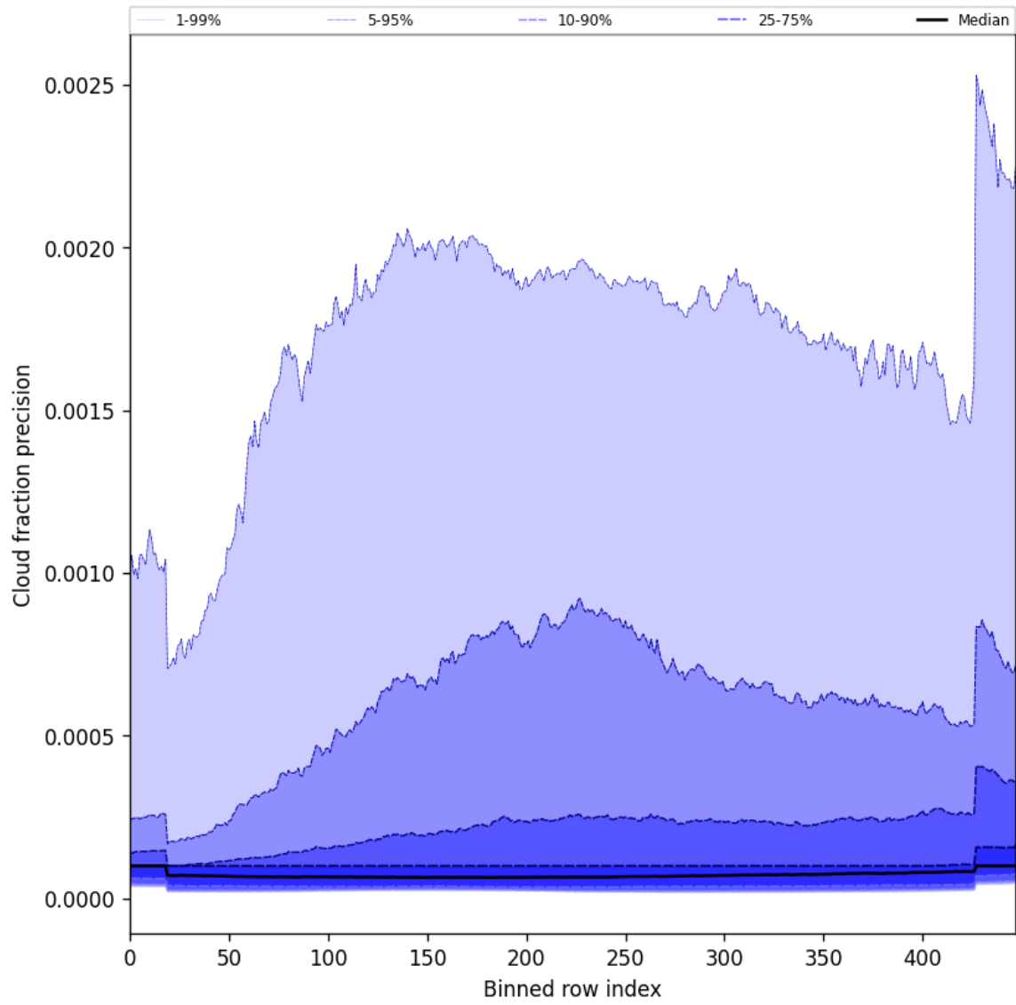
Figure 50: Along track statistics of “Cloud fraction precision” for 2025-01-07 to 2025-01-09
