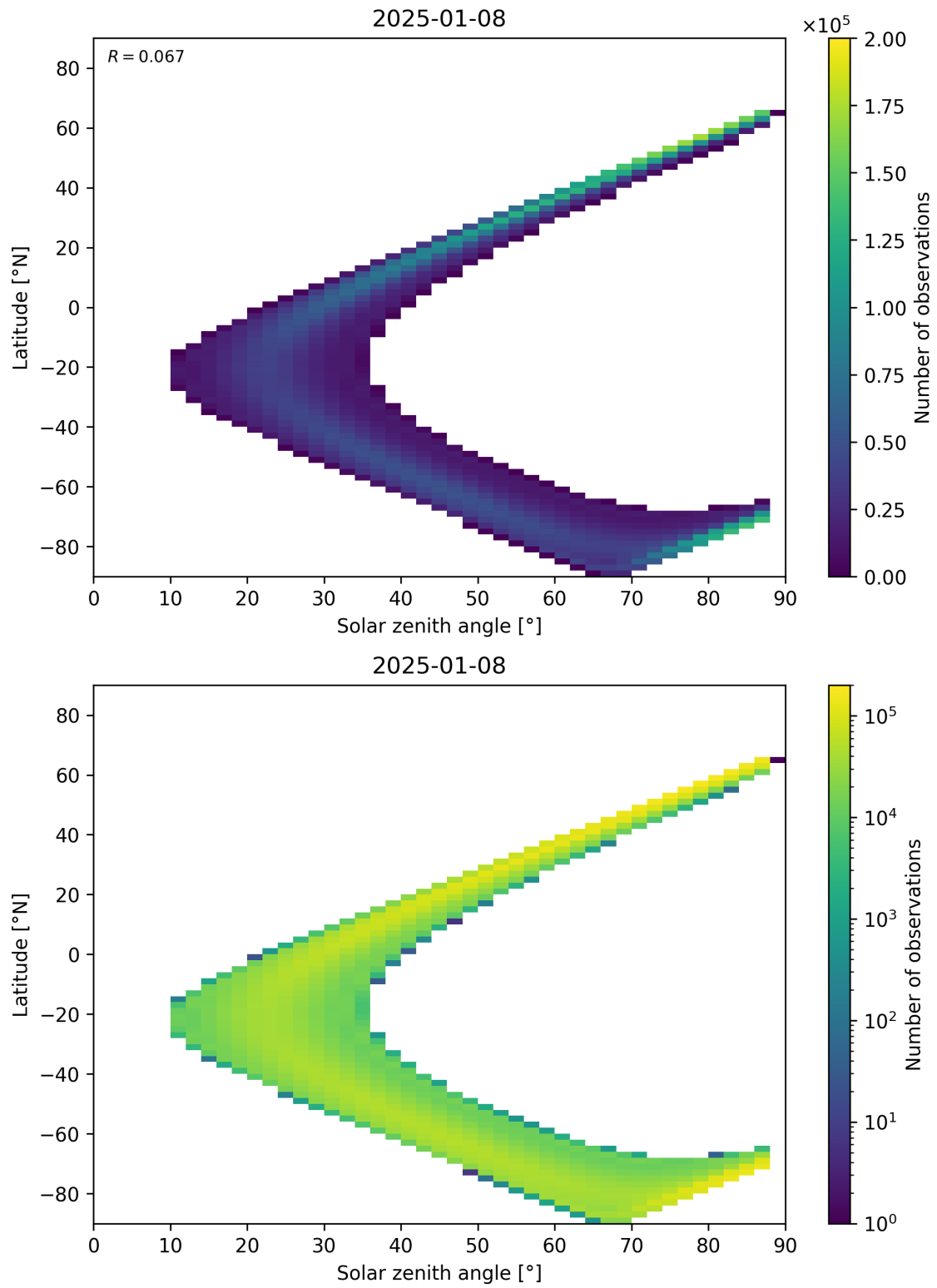
Figure 113: Scatter density plot of “Solar zenith angle” against “Latitude” for 2025-01-07 to 2025-01-09.
