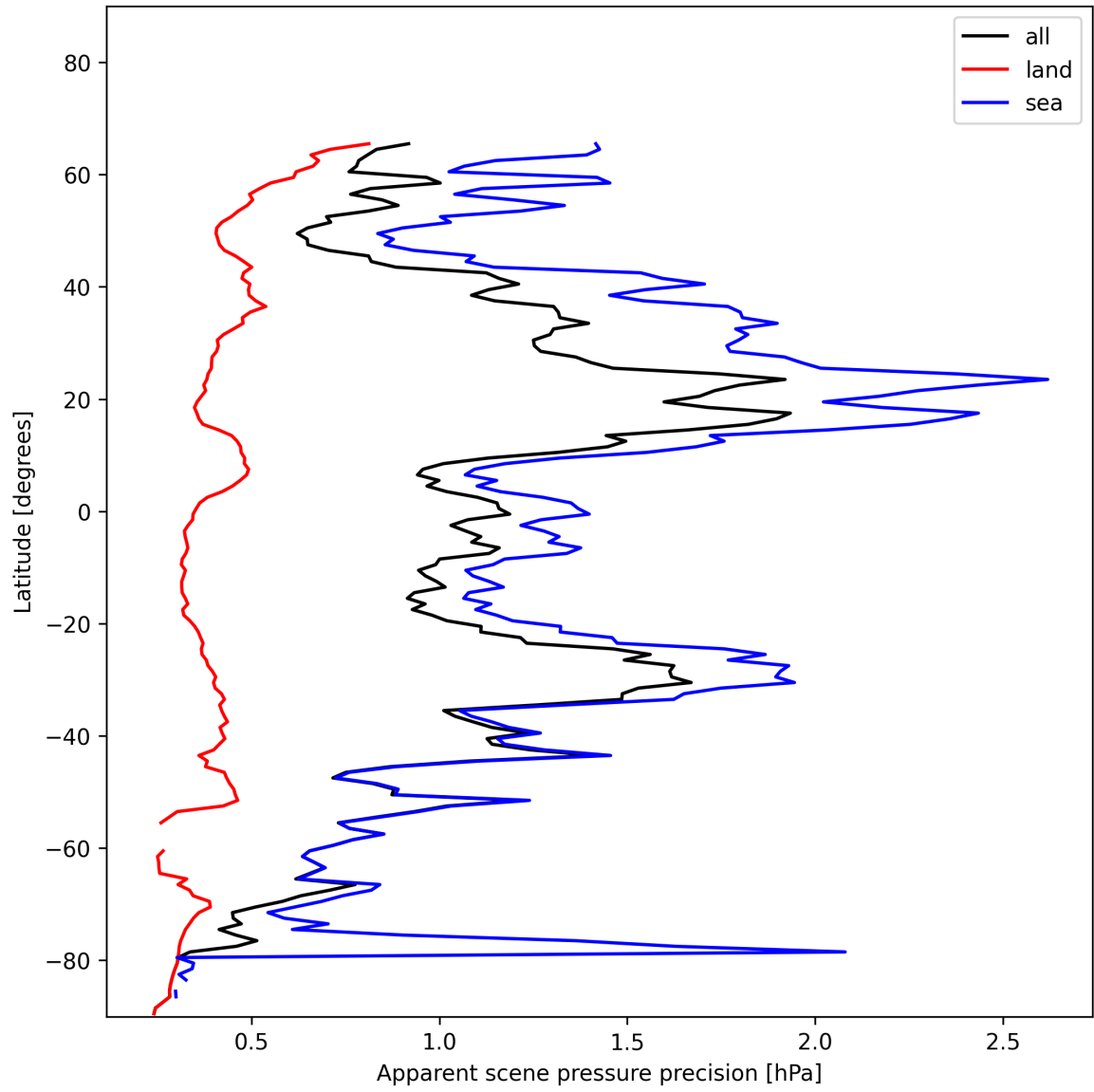
Figure 20: Zonal average of “Apparent scene pressure precision” for 2025-01-07 to 2025-01-09.
