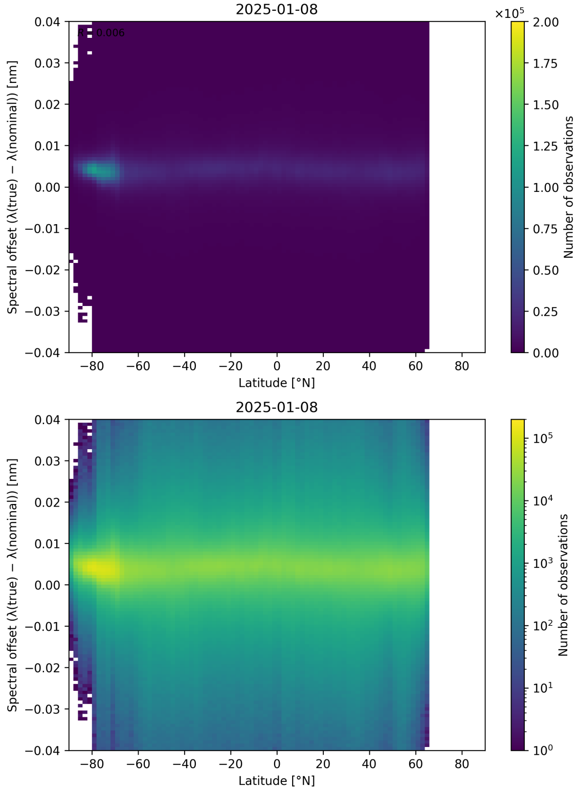
Figure 96: Scatter density plot of “Latitude” against “Spectral offset ( \lambda_{\text{true}} - \lambda_{\text{nominal}} )” for 2025-01-07 to 2025-01-09.
