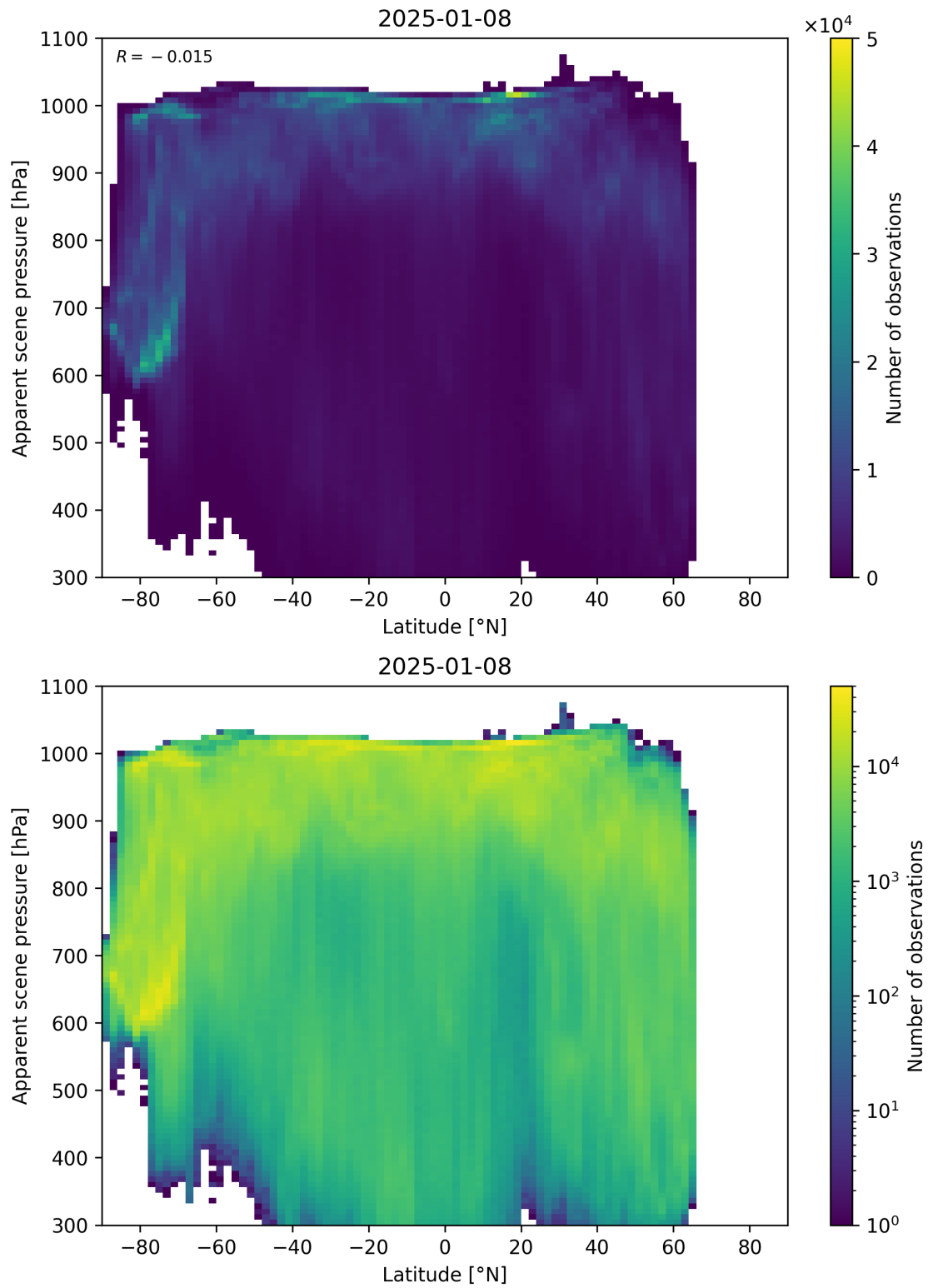
Figure 88: Scatter density plot of “Latitude” against “Apparent scene pressure” for 2025-01-07 to 2025-01-09.
