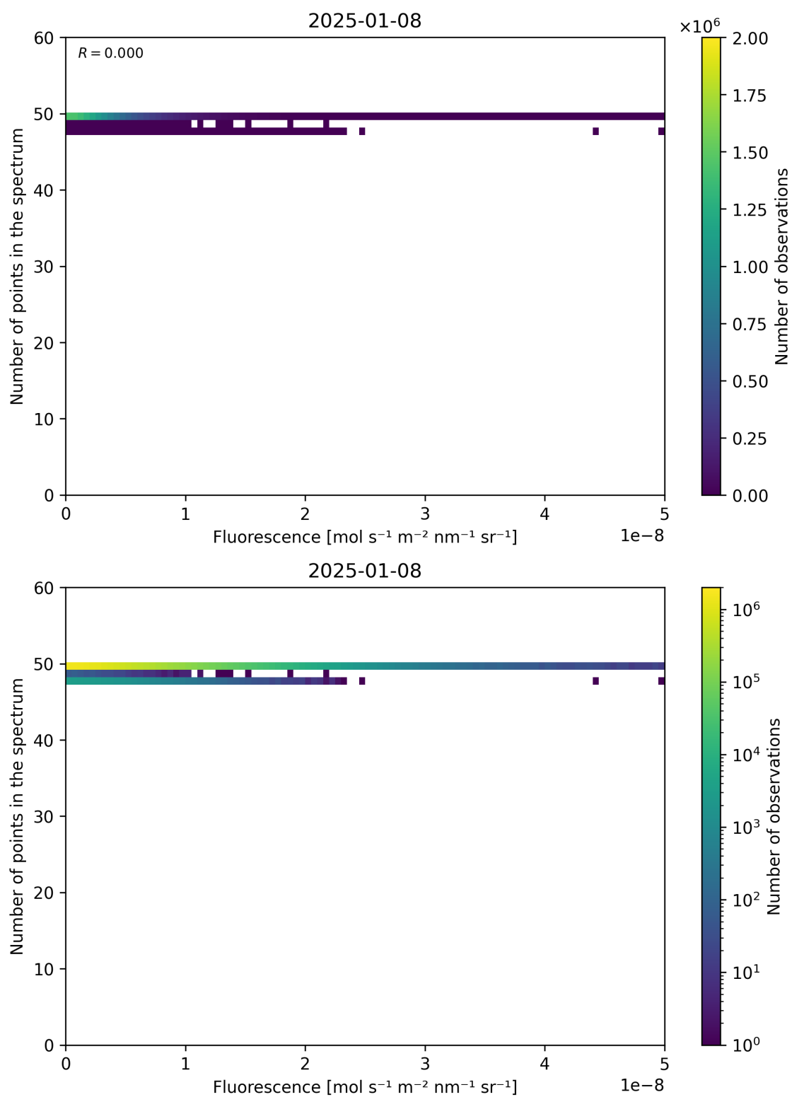
Figure 86: Scatter density plot of “Fluorescence” against “Number of points in the spectrum” for 2025-01-07 to 2025-01-09.
