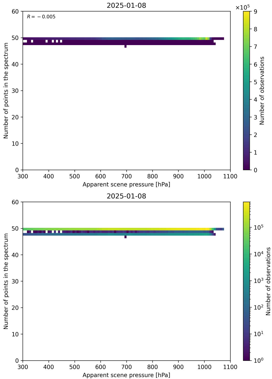
Figure 66: Scatter density plot of “Apparent scene pressure” against “Number of points in the spectrum” for 2025-01-07 to 2025-01-09.
