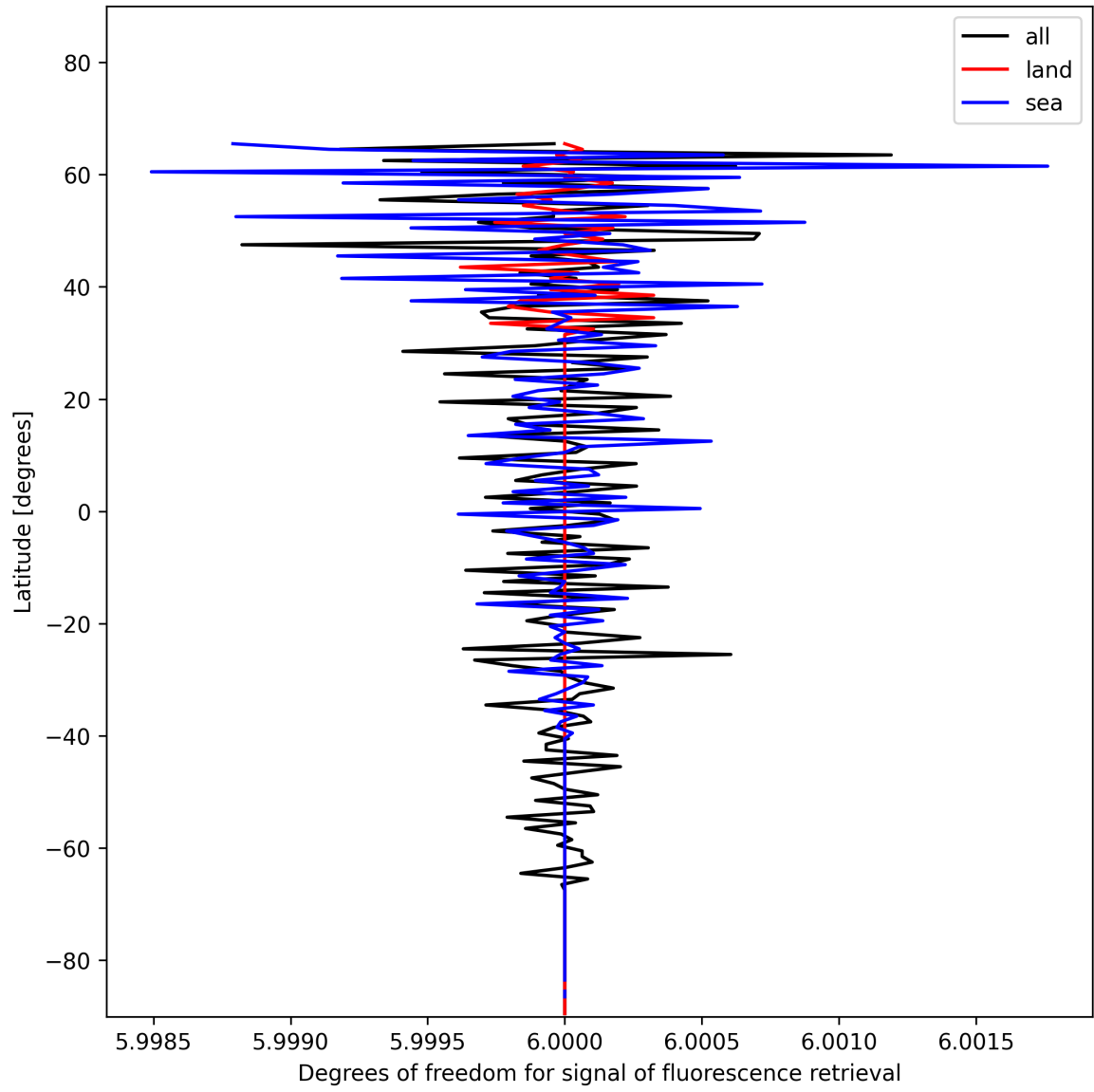
Figure 26: Zonal average of “Degrees of freedom for signal of fluorescence retrieval” for 2025-01-07 to 2025-01-09.
