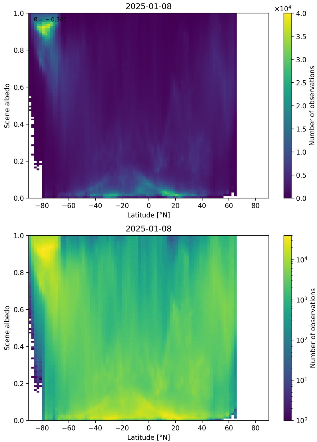
Figure 95: Scatter density plot of “Latitude” against “Scene albedo” for 2025-01-07 to 2025-01-09.
