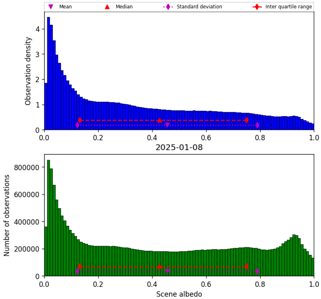
Figure 34: Histogram of “Scene albedo” for 2025-01-07 to 2025-01-09
