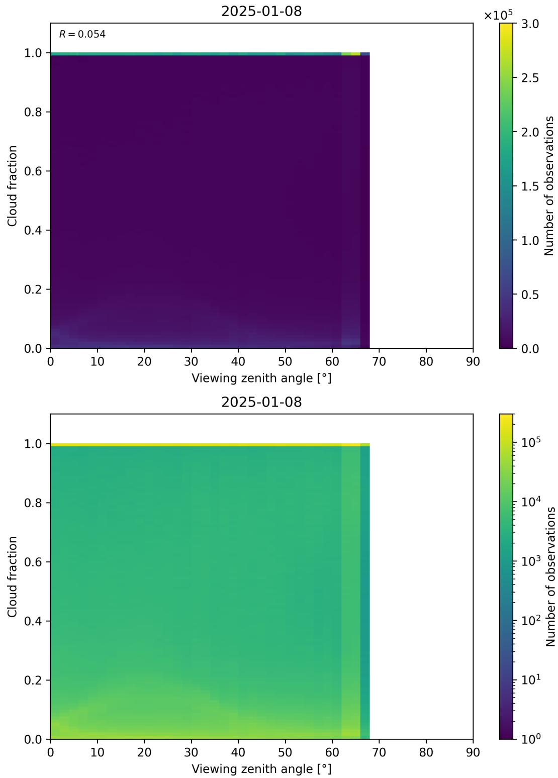
Figure 120: Scatter density plot of “Viewing zenith angle” against “Cloud fraction” for 2025-01-07 to 2025-01-09.
