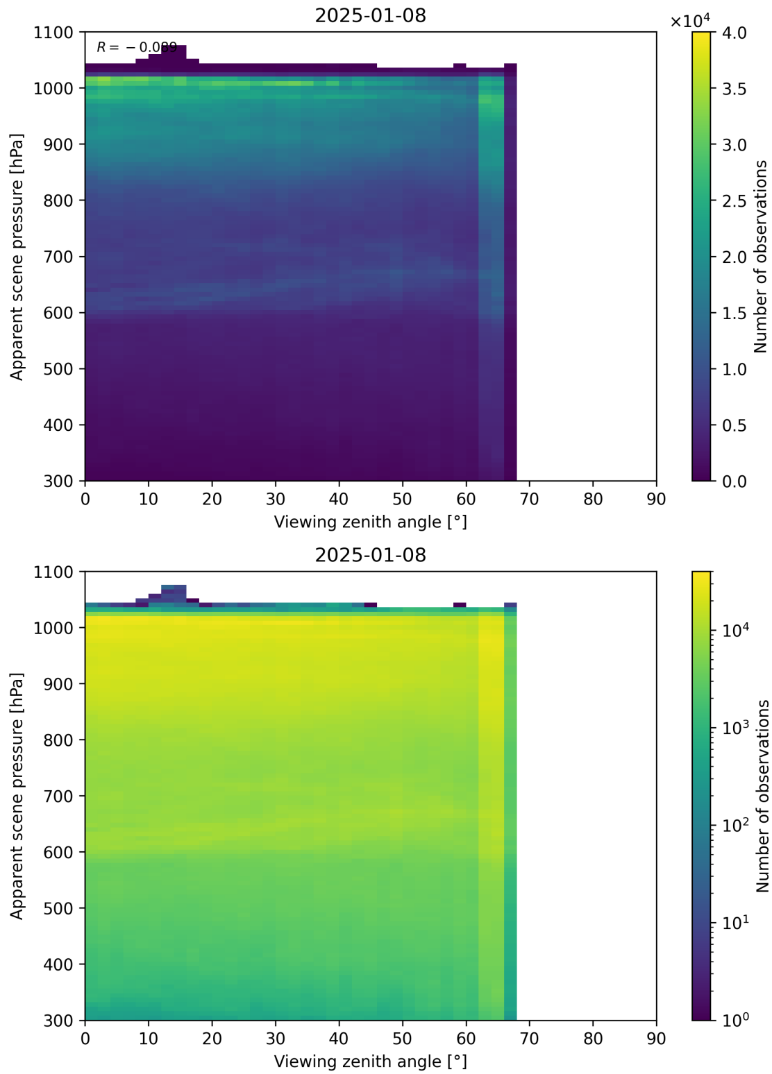
Figure 118: Scatter density plot of “Viewing zenith angle” against “Apparent scene pressure” for 2025-01-07 to 2025-01-09.
