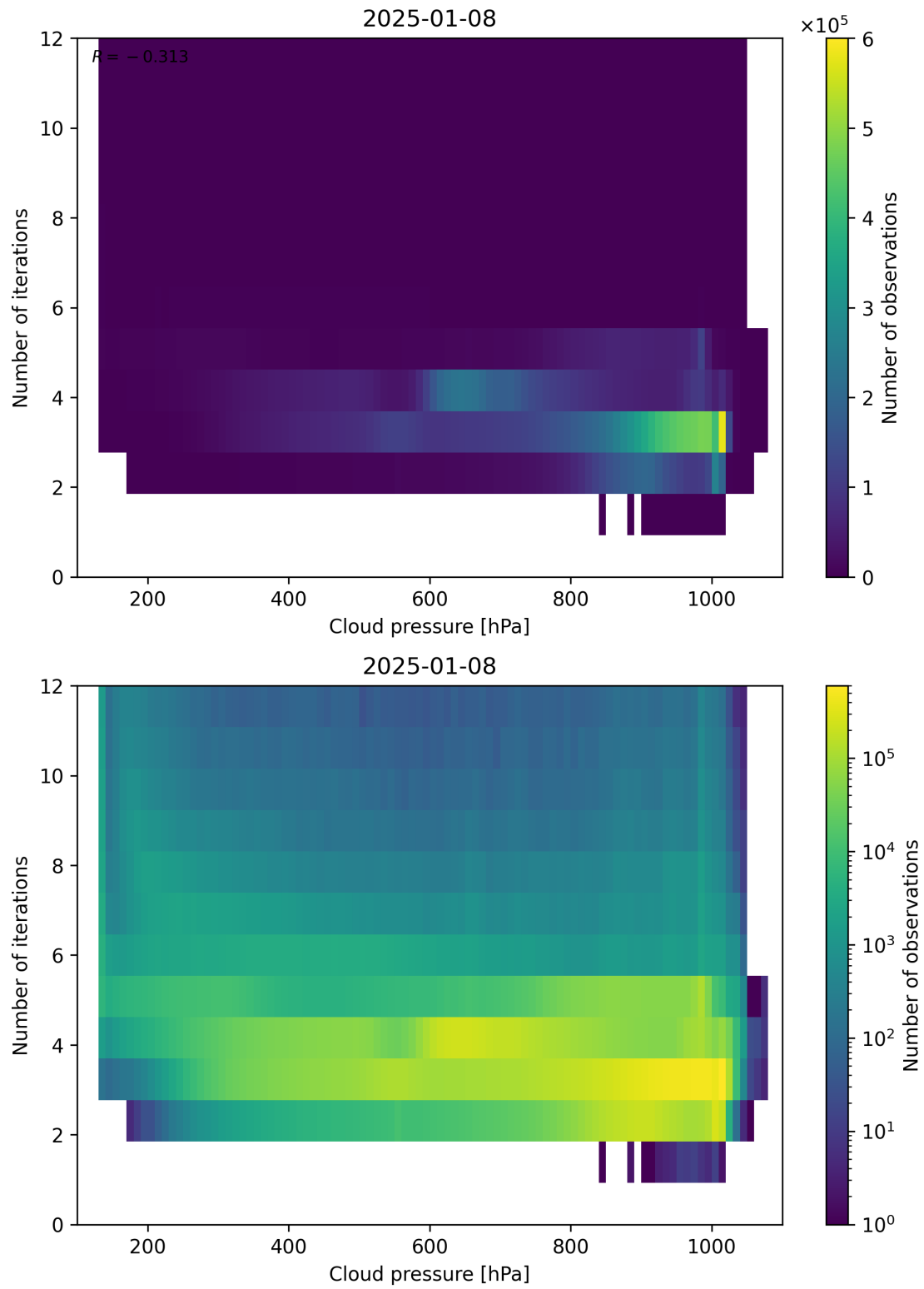
Figure 81: Scatter density plot of “Cloud pressure” against “Number of iterations” for 2025-01-07 to 2025-01-09.
