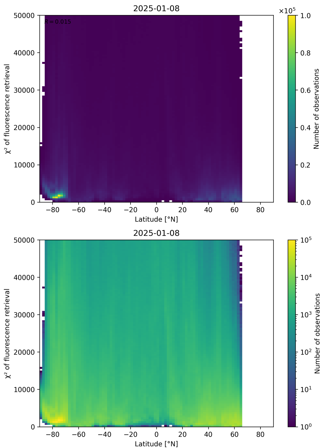
Figure 89: Scatter density plot of “Latitude” against “ \chi^2 of fluorescence retrieval” for 2025-01-07 to 2025-01-09.
