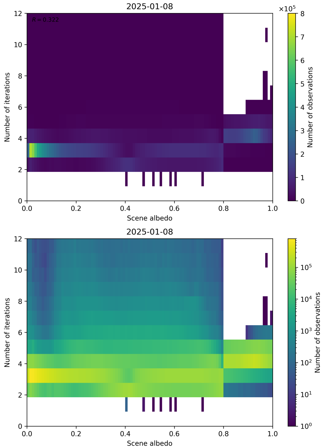
Figure 105: Scatter density plot of “Scene albedo” against “Number of iterations” for 2025-01-07 to 2025-01-09.
