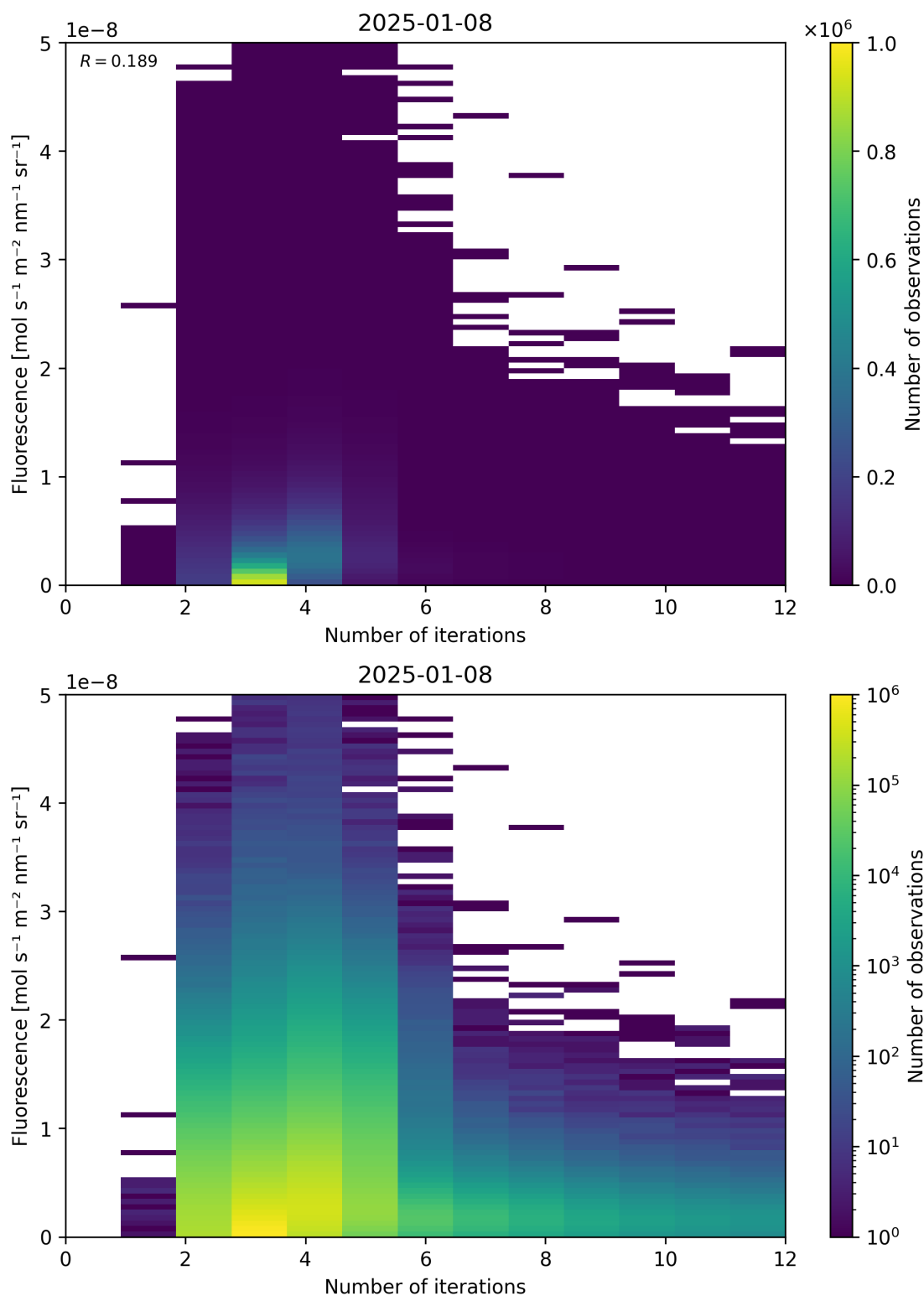
Figure 98: Scatter density plot of "Number of iterations" against "Fluorescence" for 2025-01-07 to 2025-01-09.
