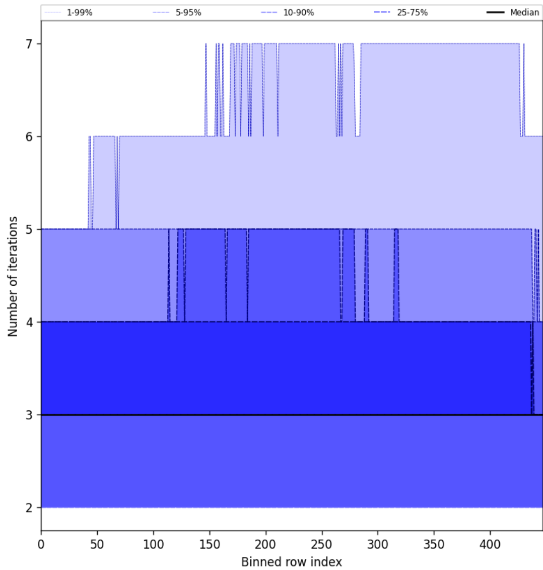
Figure 56: Along track statistics of “Number of iterations” for 2025-01-07 to 2025-01-09
