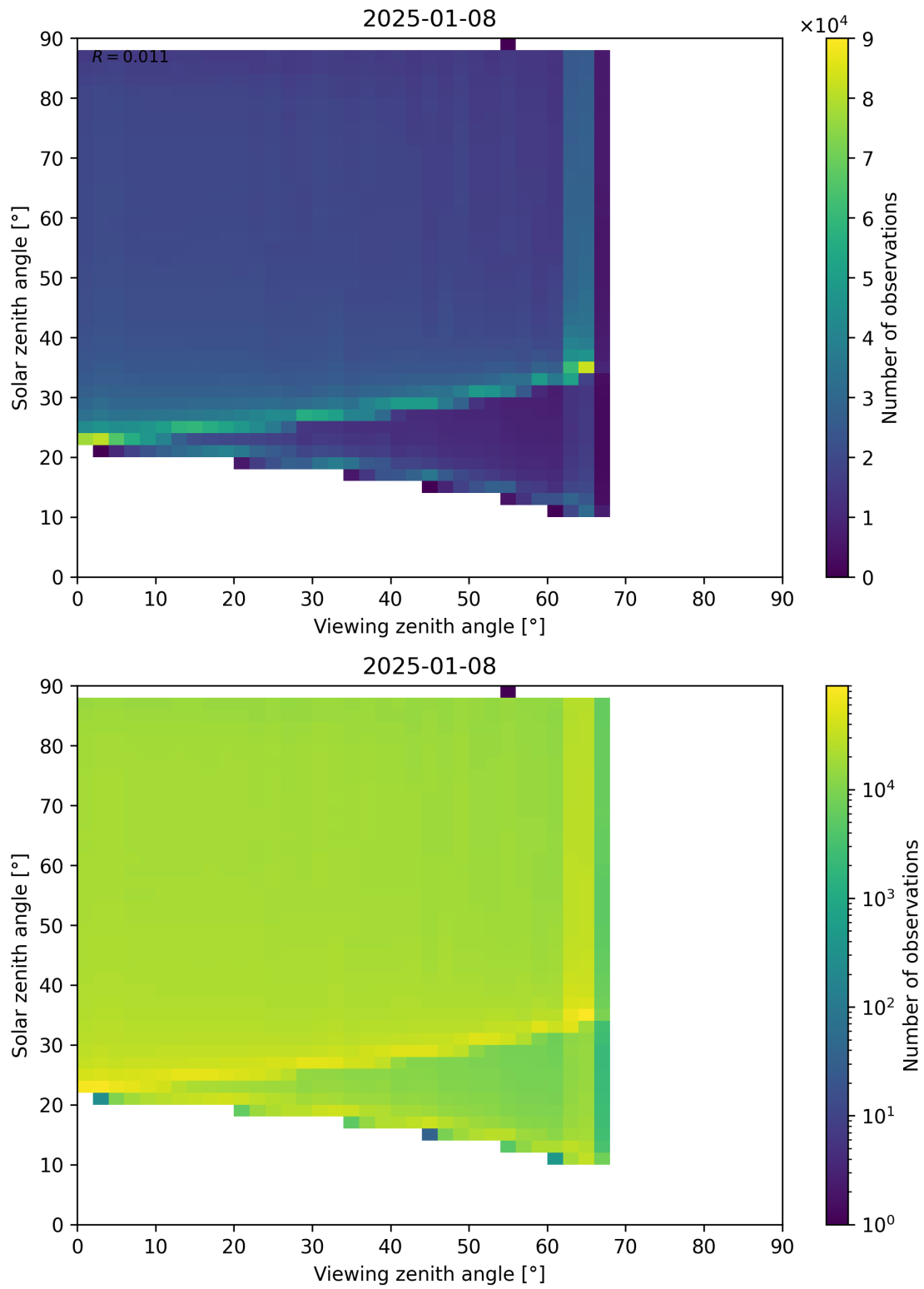
Figure 127: Scatter density plot of “Viewing zenith angle” against “Solar zenith angle” for 2025-01-07 to 2025-01-09.
