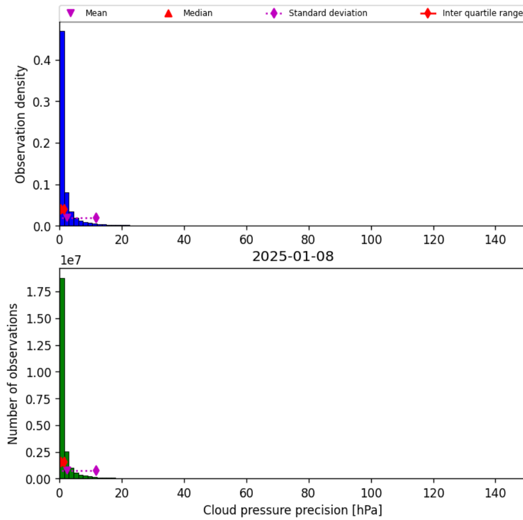
Figure 31: Histogram of “Cloud pressure precision” for 2025-01-07 to 2025-01-09
