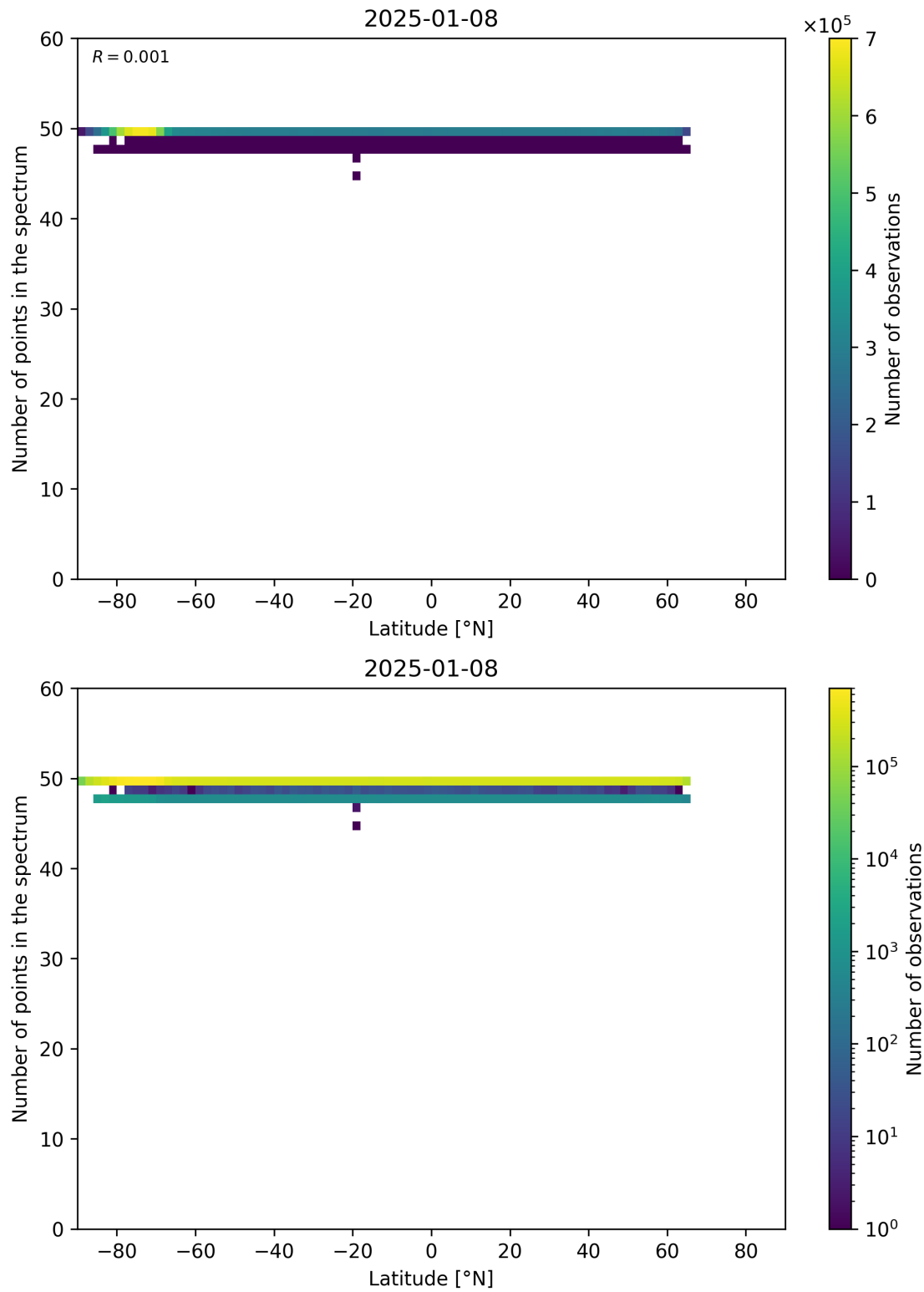
Figure 94: Scatter density plot of “Latitude” against “Number of points in the spectrum” for 2025-01-07 to 2025-01-09.
