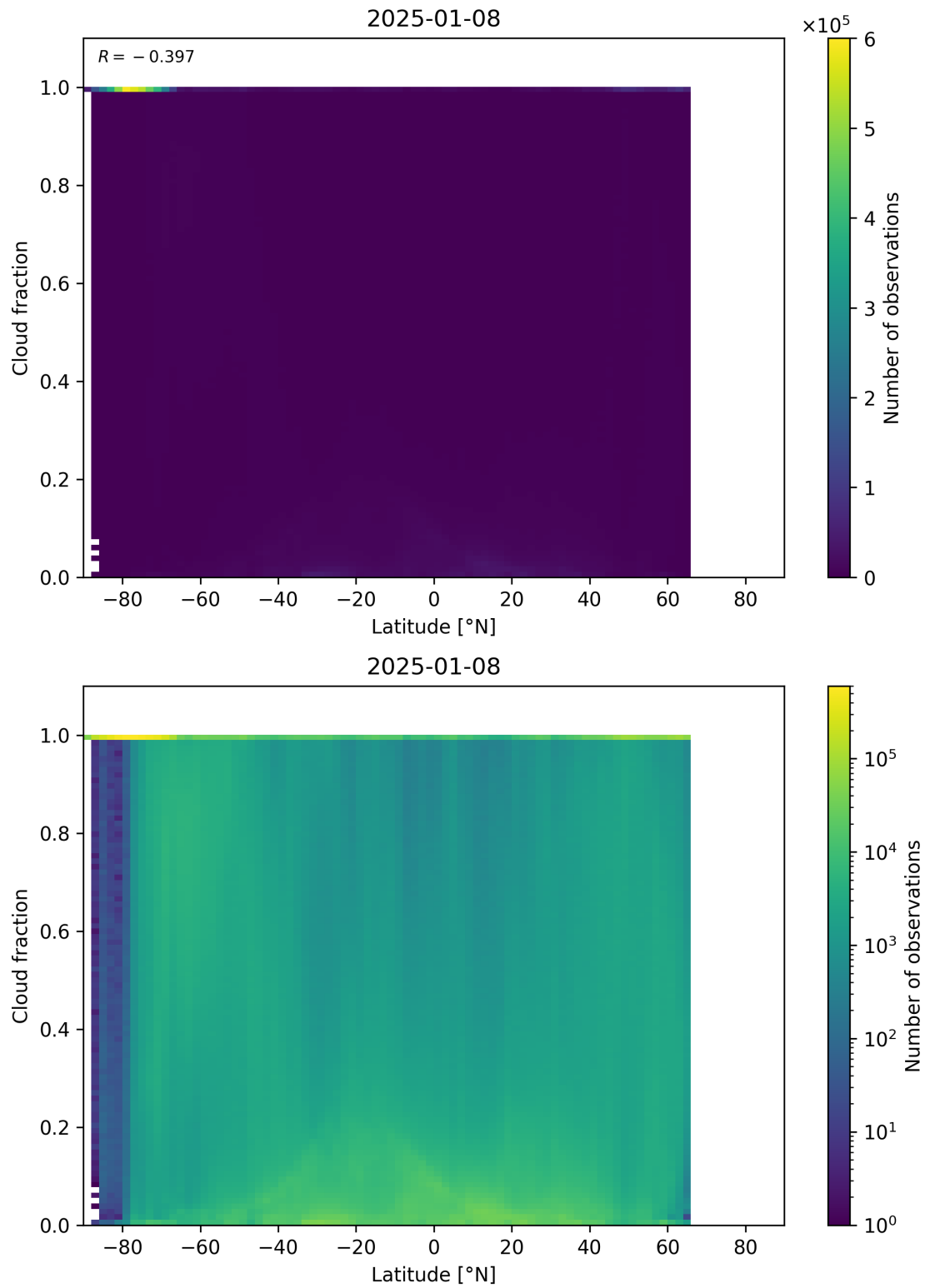
Figure 90: Scatter density plot of “Latitude” against “Cloud fraction” for 2025-01-07 to 2025-01-09.
