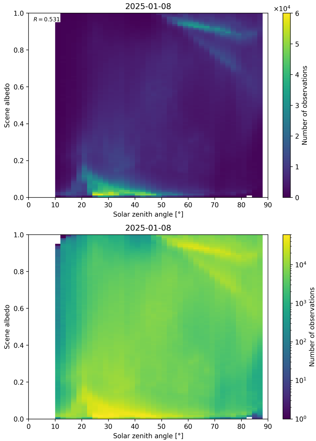
Figure 116: Scatter density plot of “Solar zenith angle” against “Scene albedo” for 2025-01-07 to 2025-01-09.
