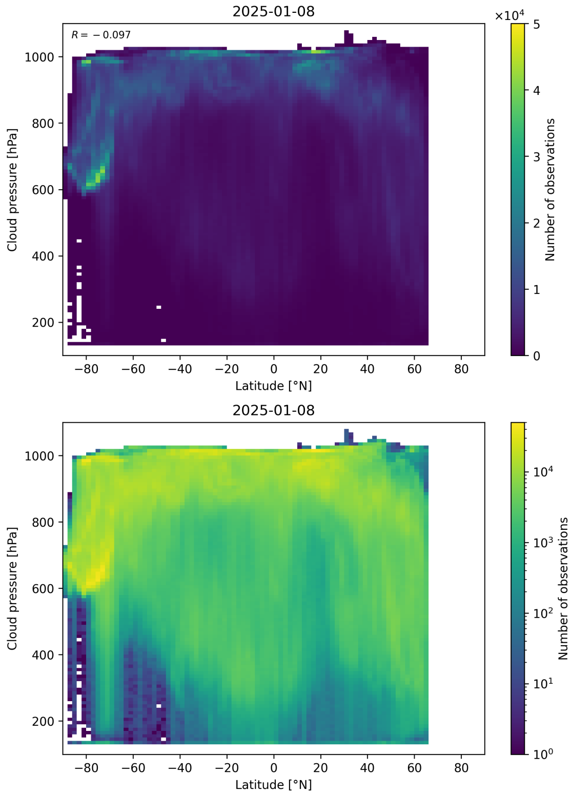
Figure 91: Scatter density plot of “Latitude” against “Cloud pressure” for 2025-01-07 to 2025-01-09.
