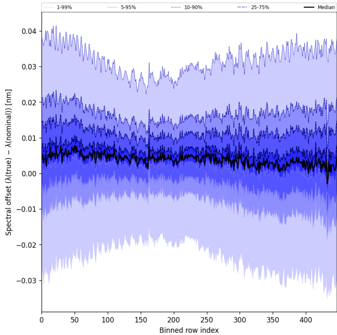
Figure 62: Along track statistics of “Spectral offset ( \lambda_{\text{true}} - \lambda_{\text{nominal}} )” for 2025-01-07 to 2025-01-09
