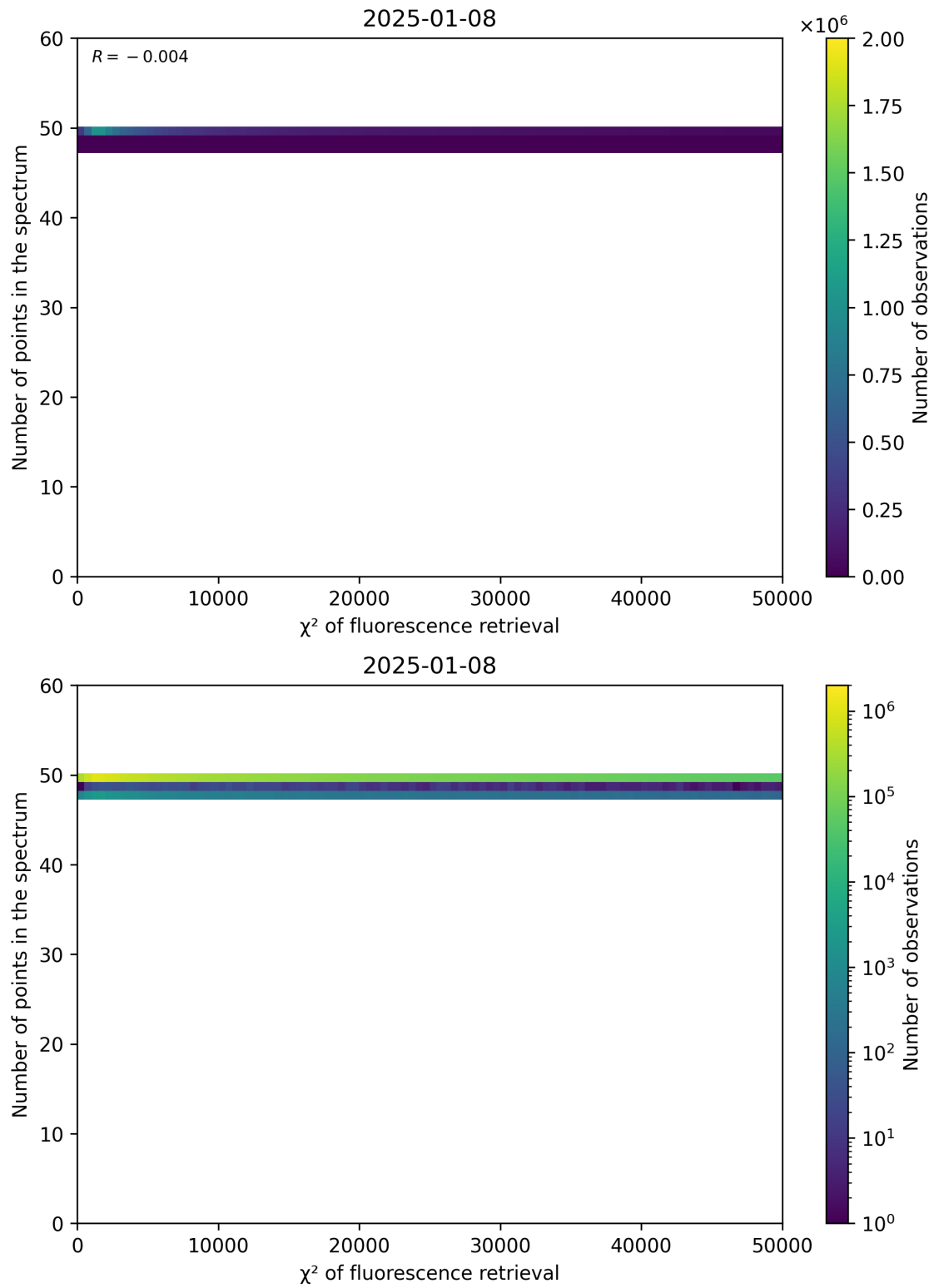
Figure 68: Scatter density plot of “ \chi^2 of fluorescence retrieval” against “Number of points in the spectrum” for 2025-01-07 to 2025-01-09.
