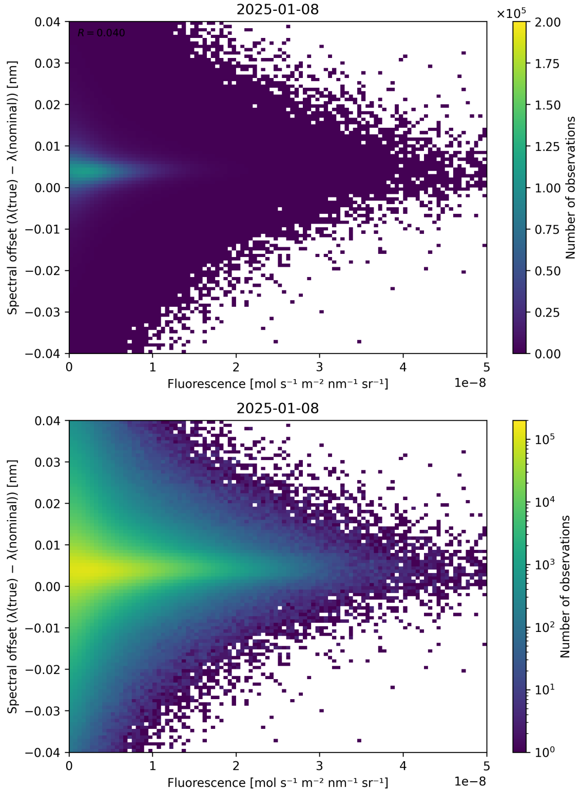
Figure 87: Scatter density plot of “Fluorescence” against “Spectral offset ( \lambda_{\text{true}} - \lambda_{\text{nominal}} )” for 2025-01-07 to 2025-01-09.
