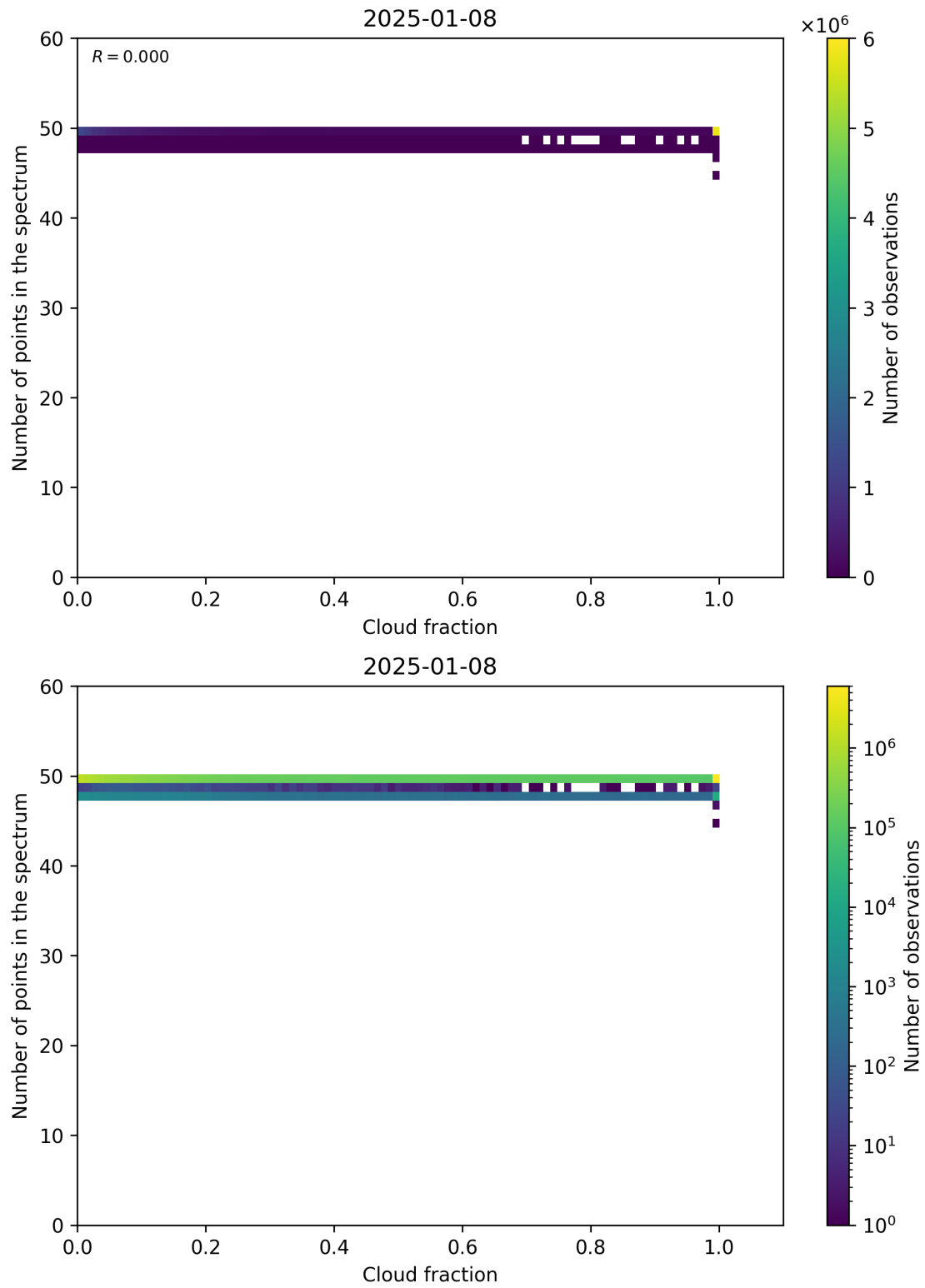
Figure 74: Scatter density plot of “Cloud fraction” against “Number of points in the spectrum” for 2025-01-07 to 2025-01-09.
