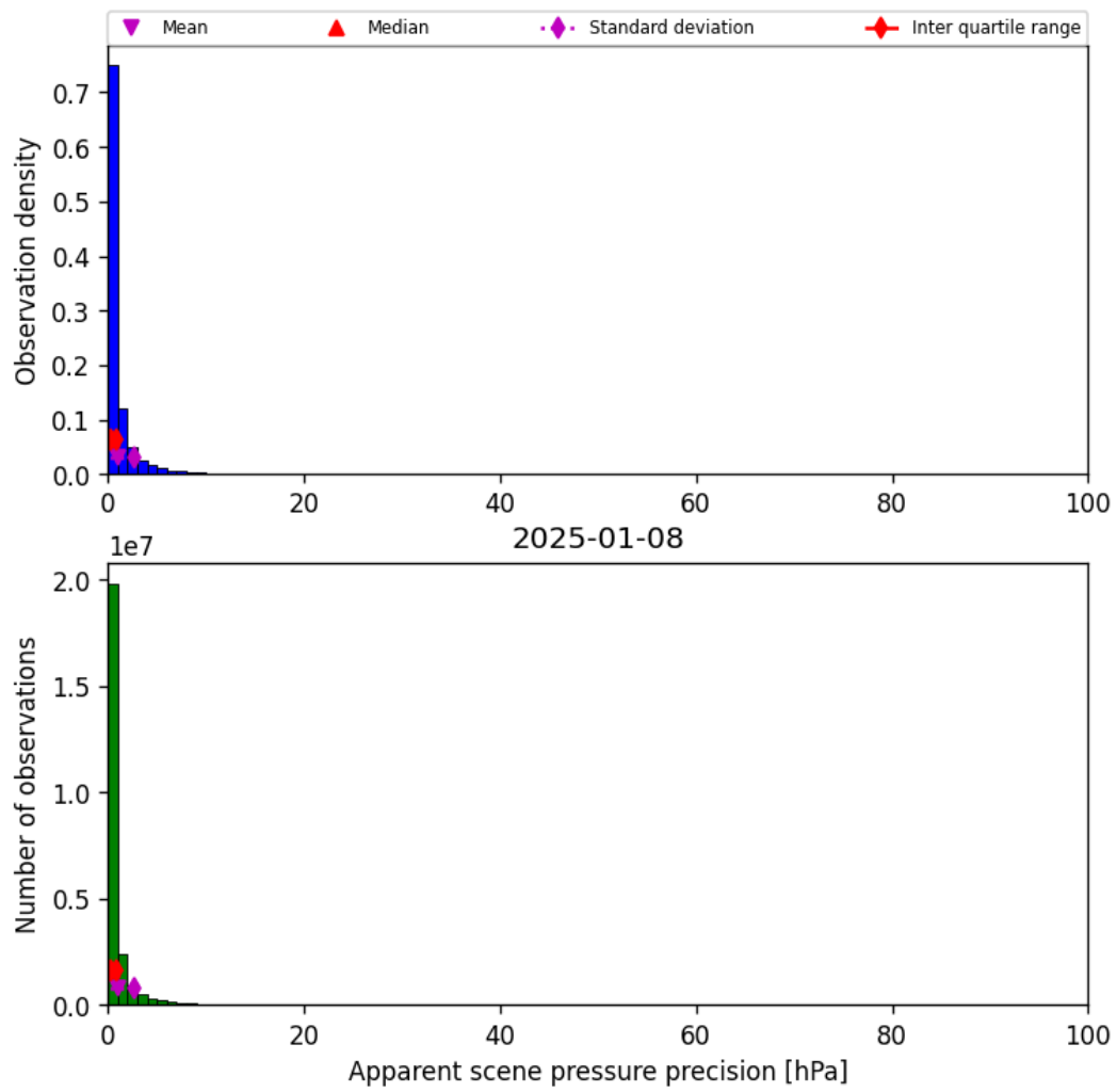
Figure 37: Histogram of “Apparent scene pressure precision” for 2025-01-07 to 2025-01-09
