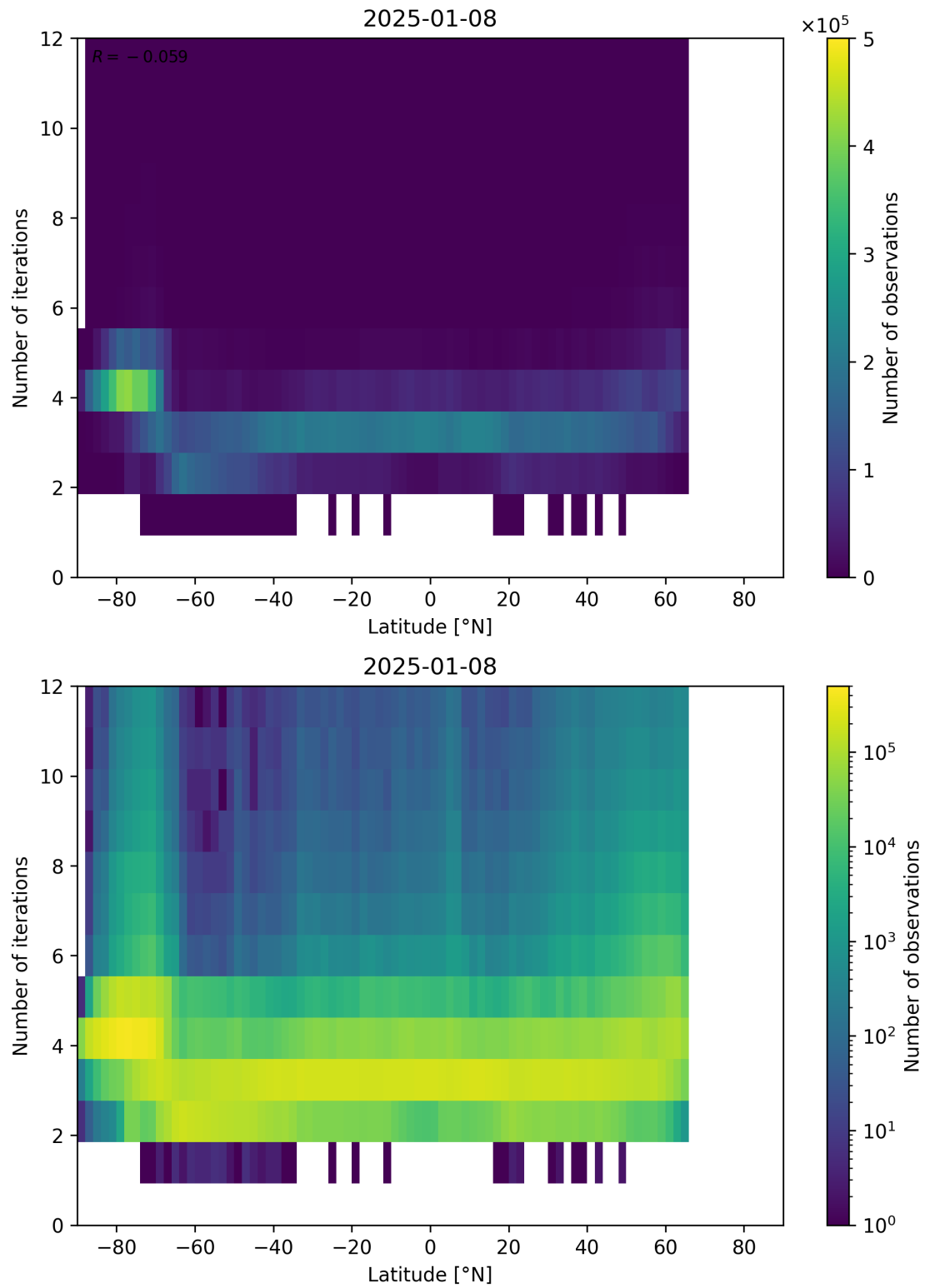
Figure 93: Scatter density plot of “Latitude” against “Number of iterations” for 2025-01-07 to 2025-01-09.
