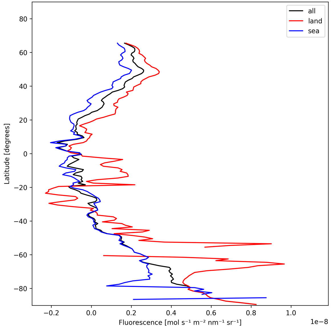
Figure 23: Zonal average of “Fluorescence” for 2025-01-07 to 2025-01-09.
