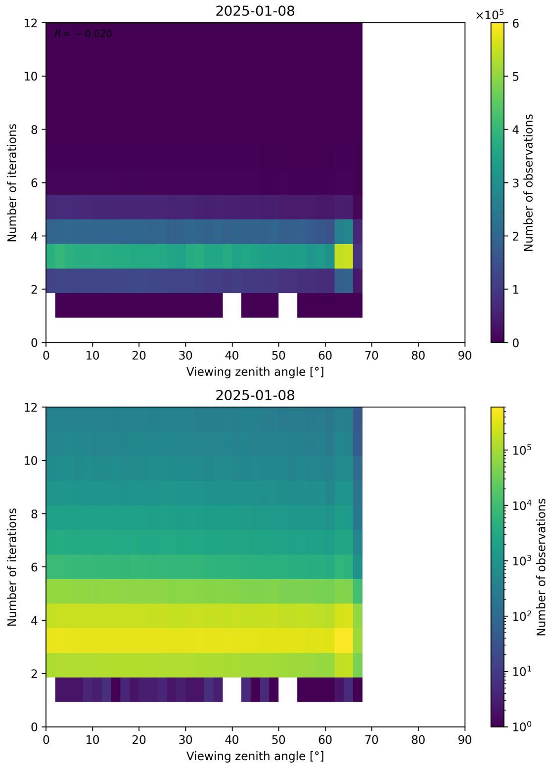
Figure 124: Scatter density plot of “Viewing zenith angle” against “Number of iterations” for 2025-01-07 to 2025-01-09.
