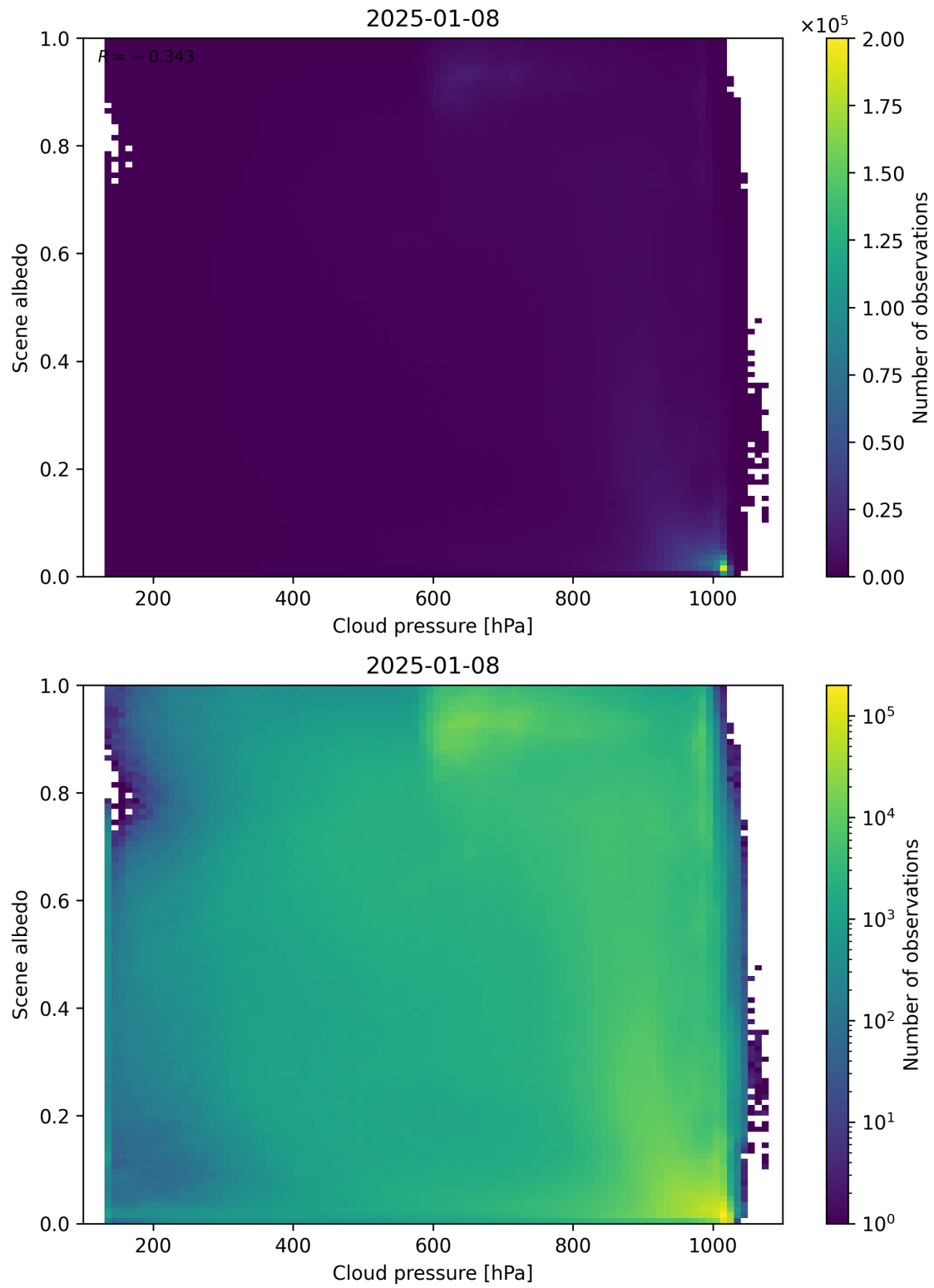
Figure 83: Scatter density plot of “Cloud pressure” against “Scene albedo” for 2025-01-07 to 2025-01-09.
