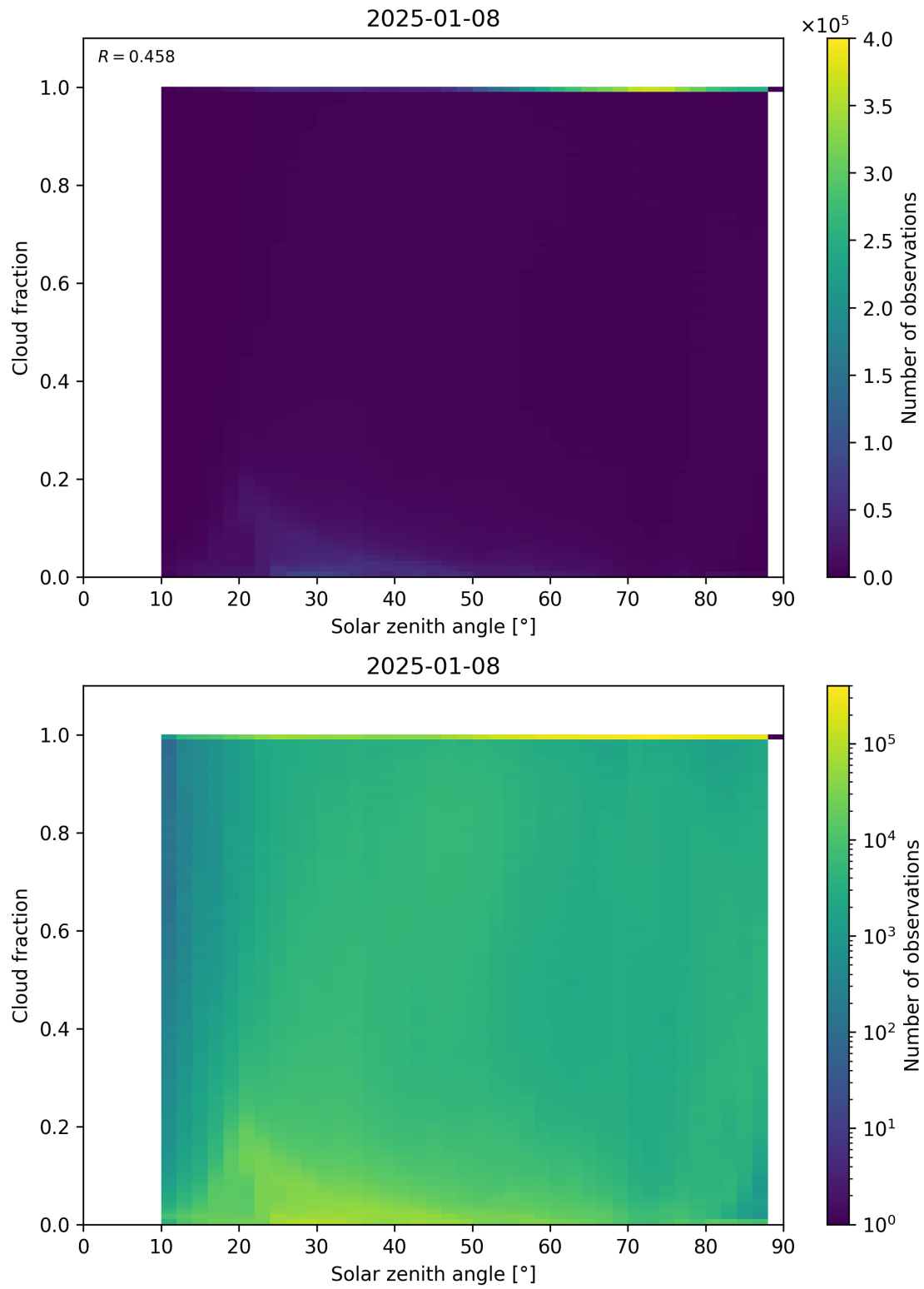
Figure 110: Scatter density plot of “Solar zenith angle” against “Cloud fraction” for 2025-01-07 to 2025-01-09.
