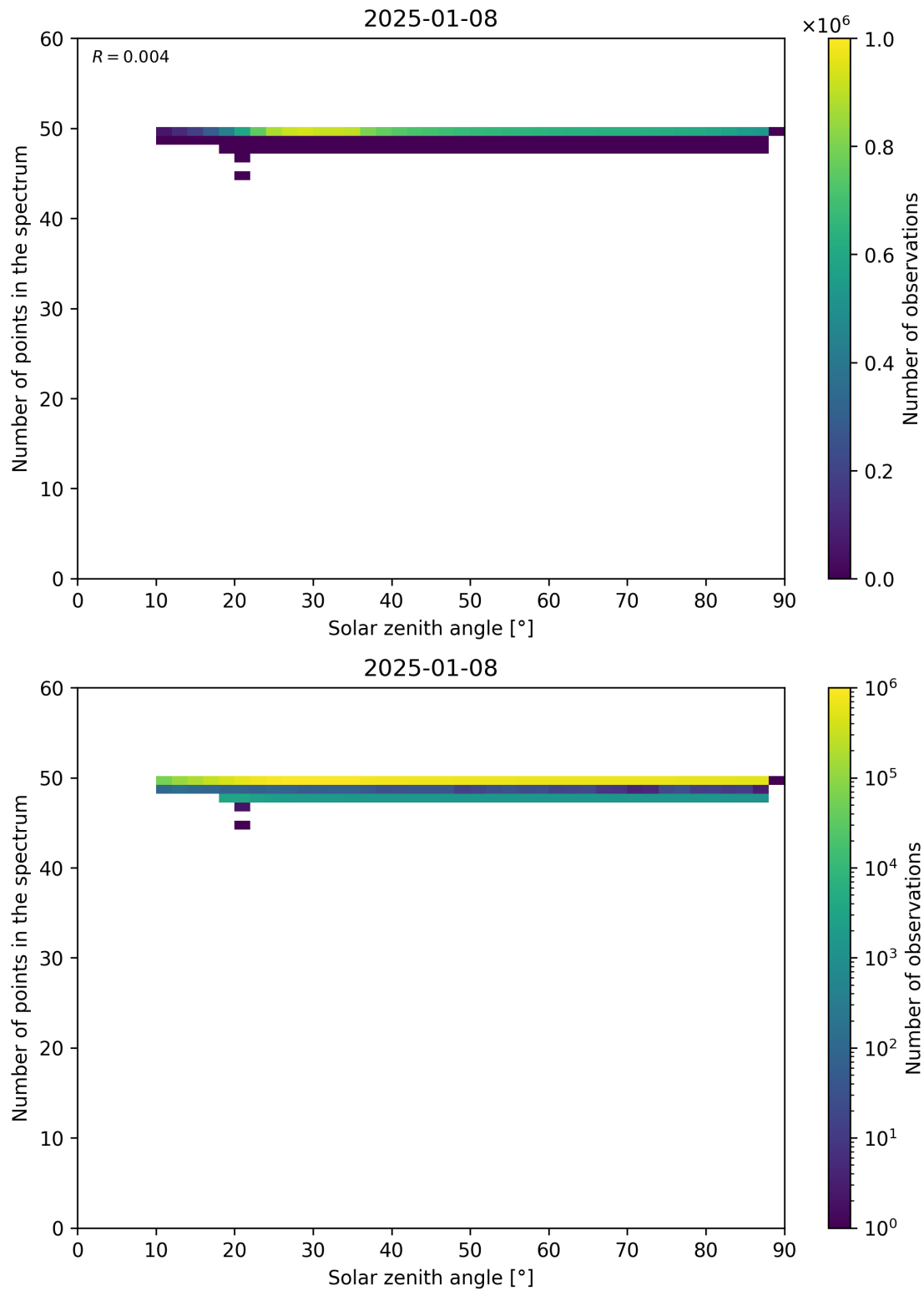
Figure 115: Scatter density plot of “Solar zenith angle” against “Number of points in the spectrum” for 2025-01-07 to 2025-01-09.
