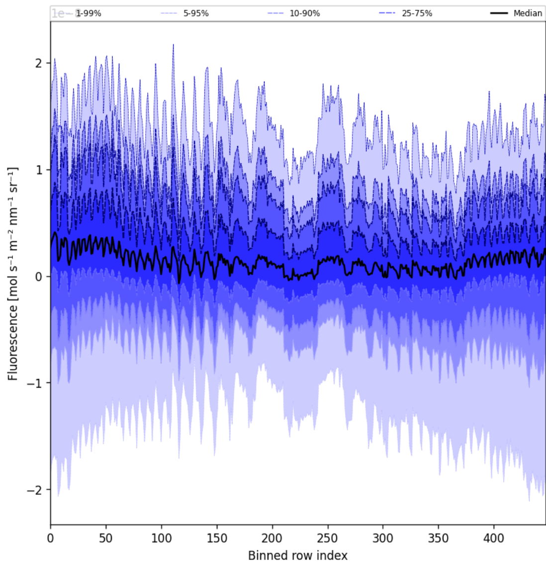
Figure 57: Along track statistics of “Fluorescence” for 2025-01-07 to 2025-01-09
