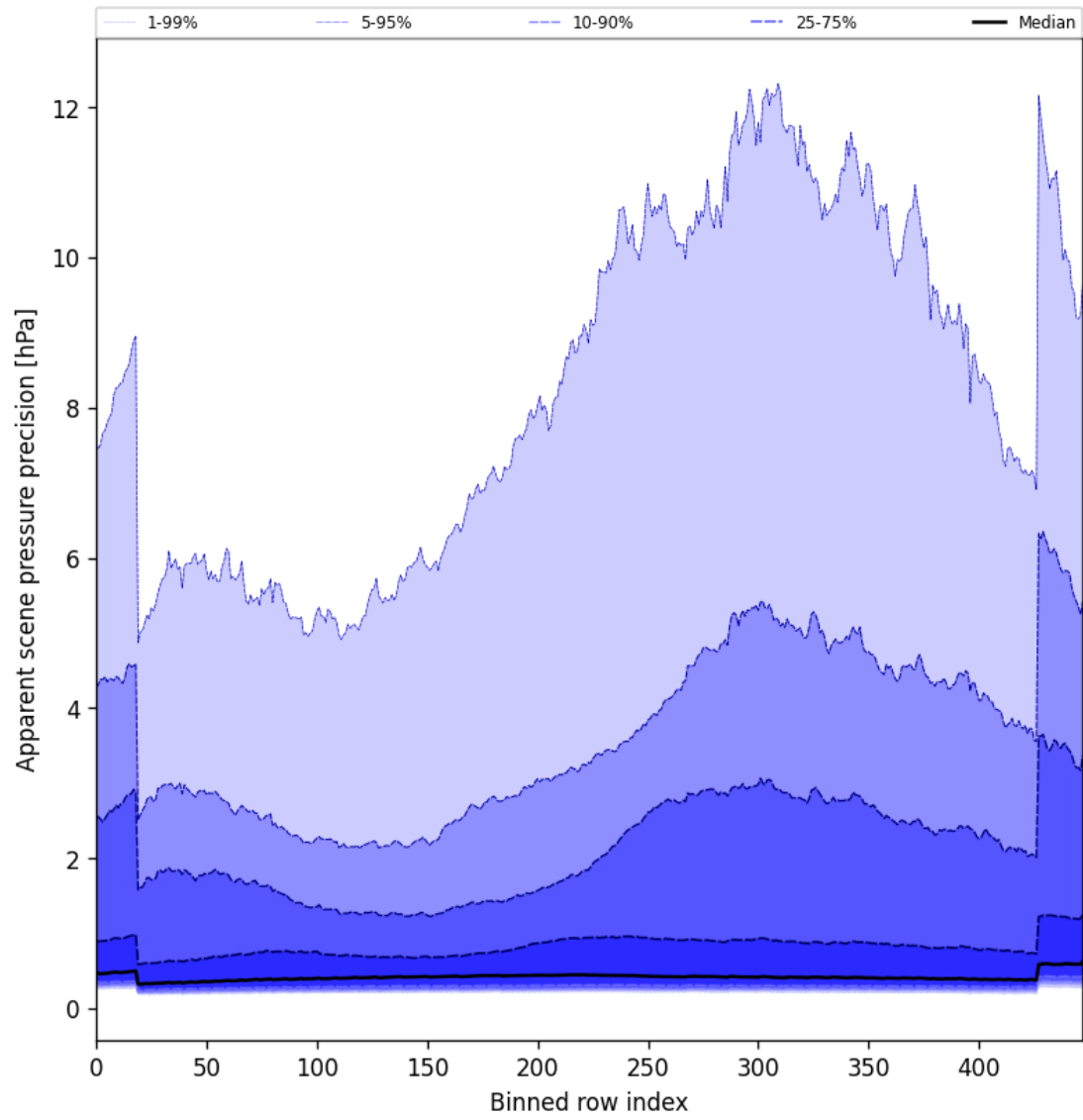
Figure 54: Along track statistics of “Apparent scene pressure precision” for 2025-01-07 to 2025-01-09
