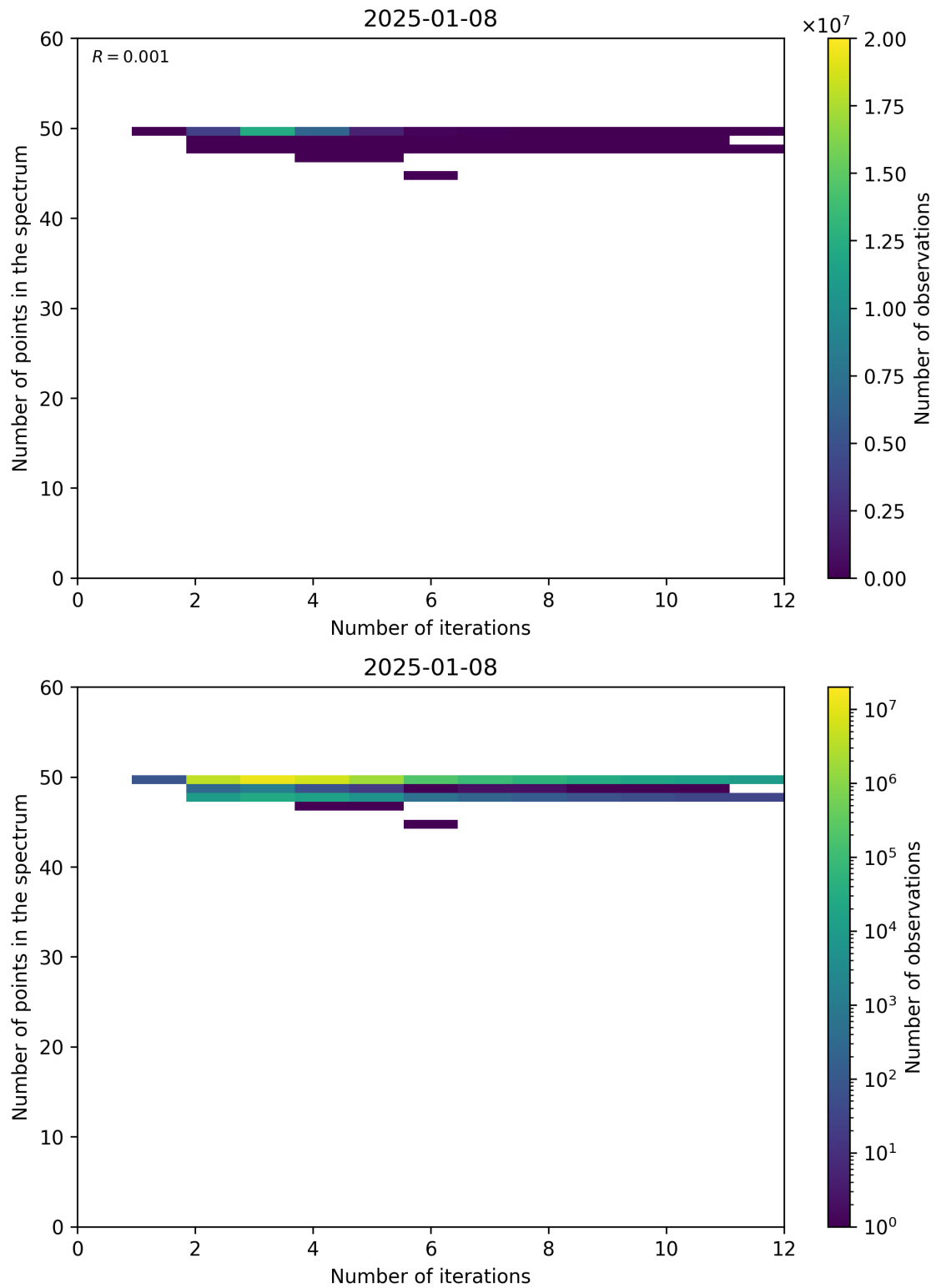
Figure 99: Scatter density plot of “Number of iterations” against “Number of points in the spectrum” for 2025-01-07 to 2025-01-09.
