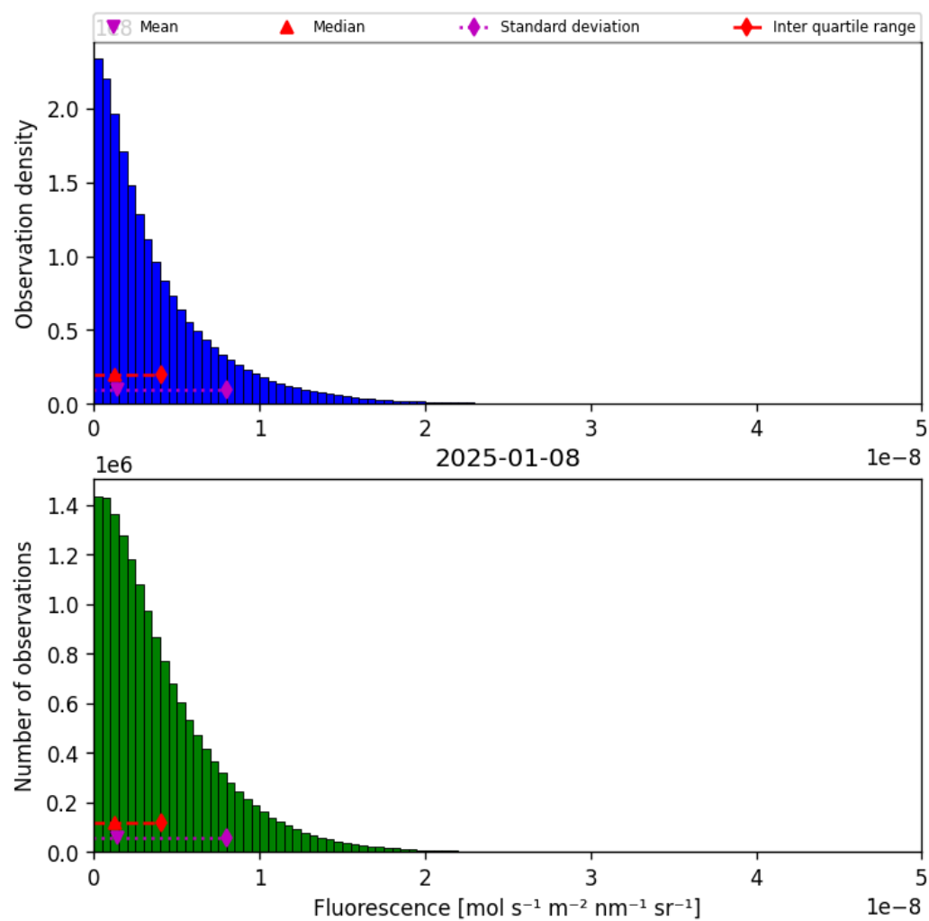
Figure 40: Histogram of “Fluorescence” for 2025-01-07 to 2025-01-09
