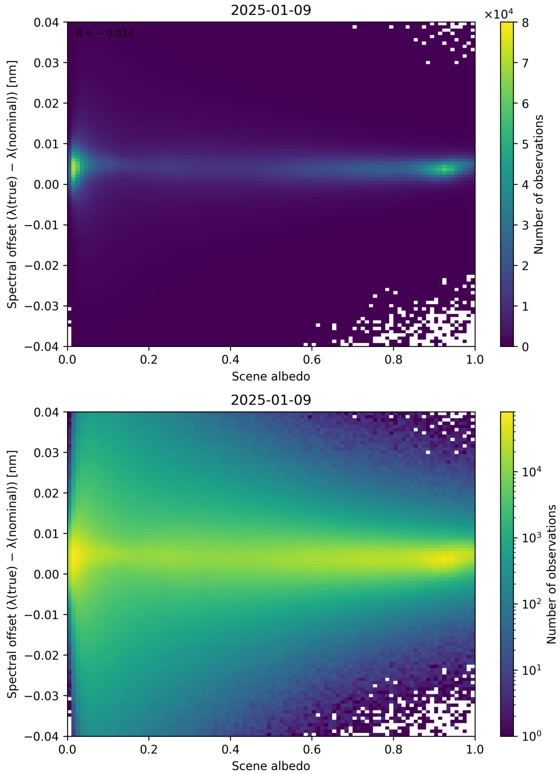
Figure 107: Scatter density plot of “Scene albedo” against “Spectral offset ( \lambda_{\text{true}} - \lambda_{\text{nominal}} )” for 2025-01-08 to 2025-01-10.
