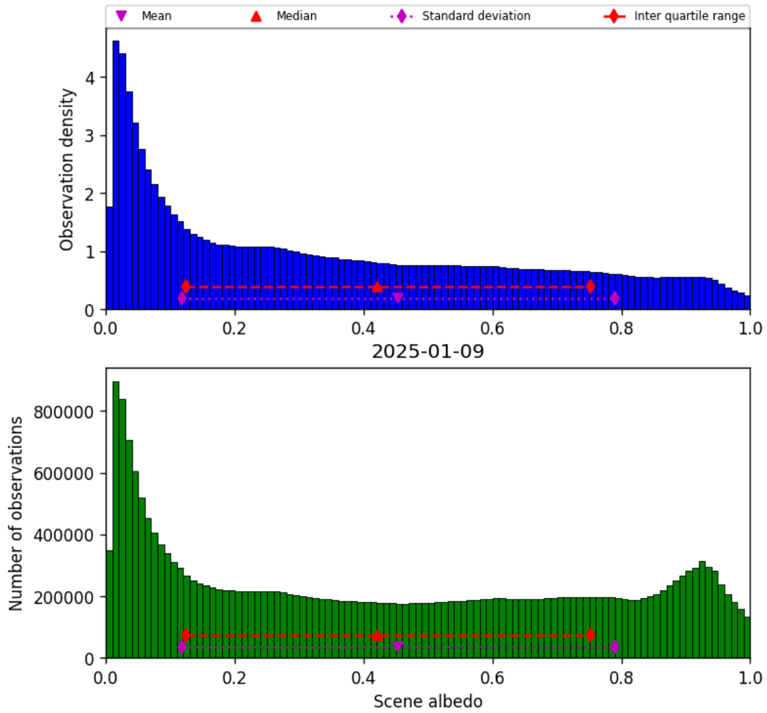
Figure 34: Histogram of “Scene albedo” for 2025-01-08 to 2025-01-10
