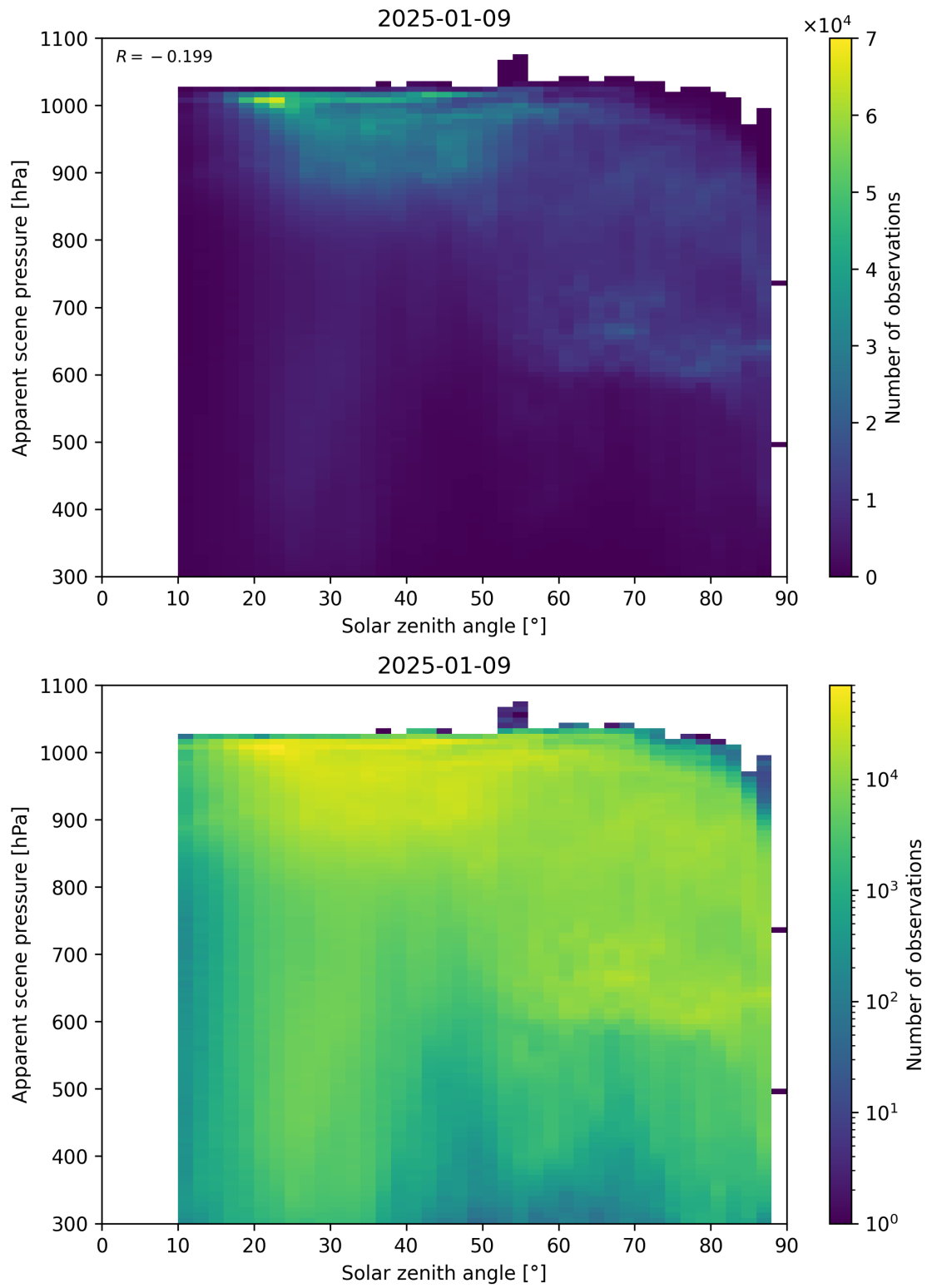
Figure 108: Scatter density plot of “Solar zenith angle” against “Apparent scene pressure” for 2025-01-08 to 2025-01-10.
