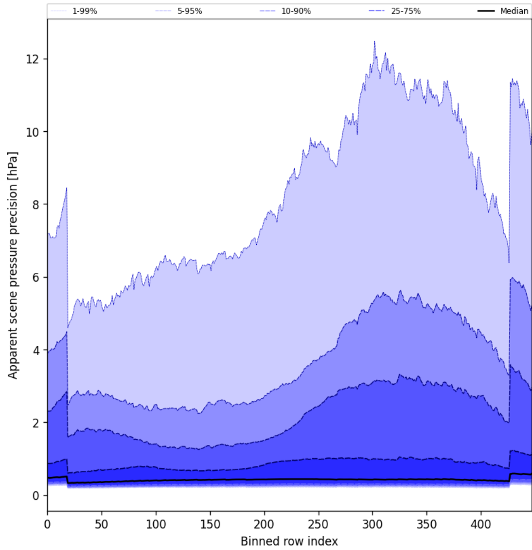
Figure 54: Along track statistics of “Apparent scene pressure precision” for 2025-01-08 to 2025-01-10
