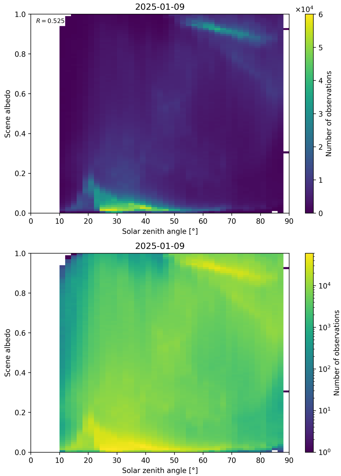
Figure 116: Scatter density plot of “Solar zenith angle” against “Scene albedo” for 2025-01-08 to 2025-01-10.
