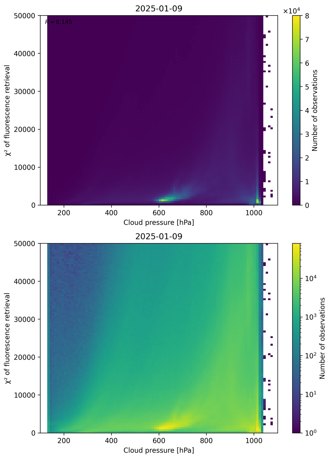
Figure 78: Scatter density plot of “Cloud pressure” against “ \chi^2 of fluorescence retrieval” for 2025-01-08 to 2025-01-10.
