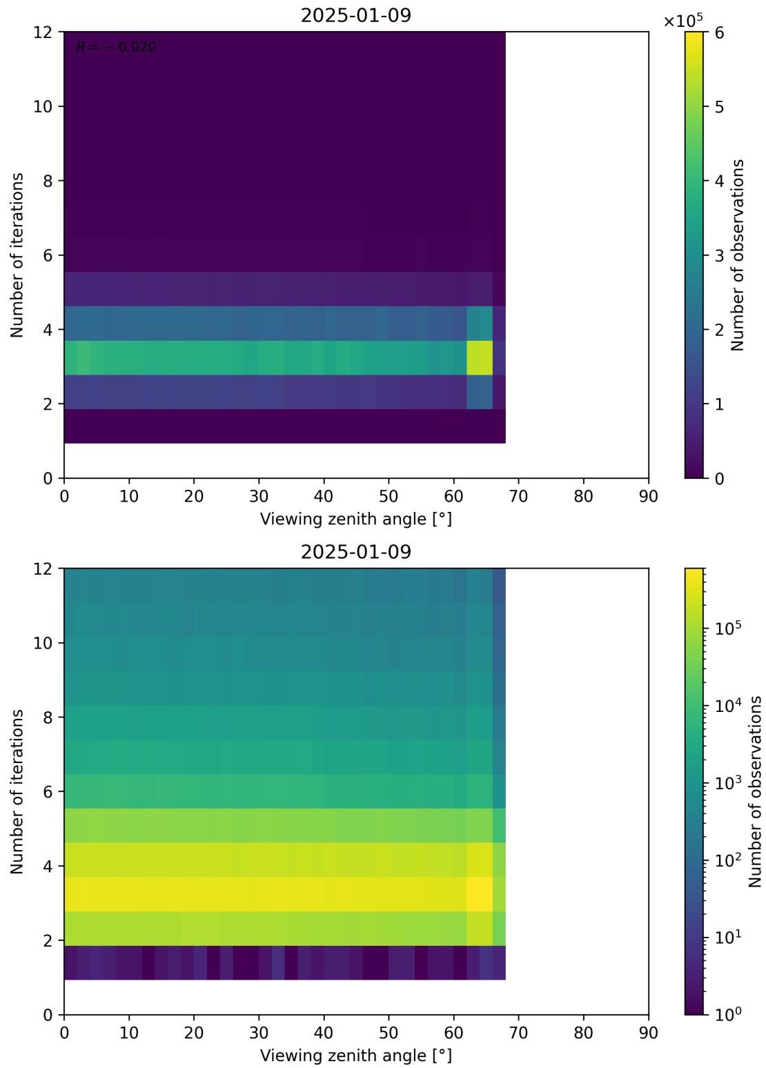
Figure 124: Scatter density plot of “Viewing zenith angle” against “Number of iterations” for 2025-01-08 to 2025-01-10.
