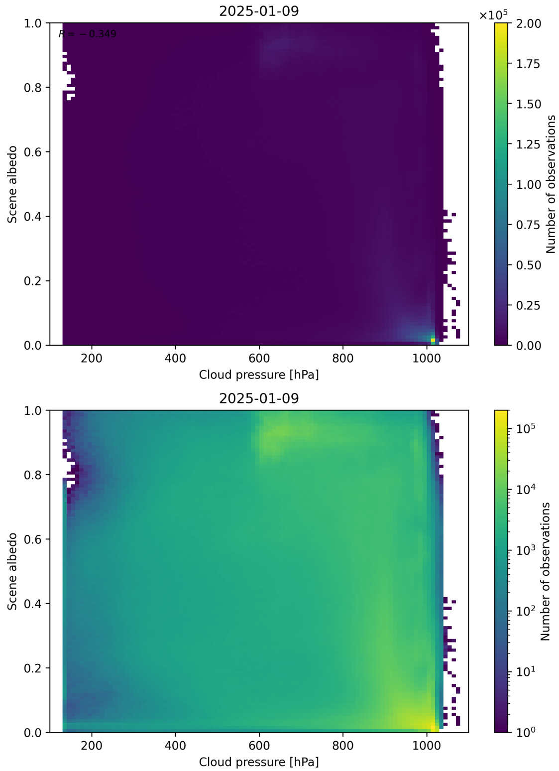
Figure 83: Scatter density plot of “Cloud pressure” against “Scene albedo” for 2025-01-08 to 2025-01-10.
