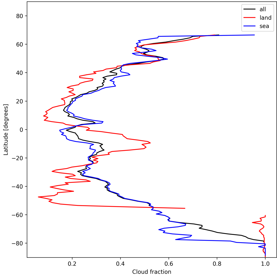
Figure 15: Zonal average of “Cloud fraction” for 2025-01-08 to 2025-01-10.
