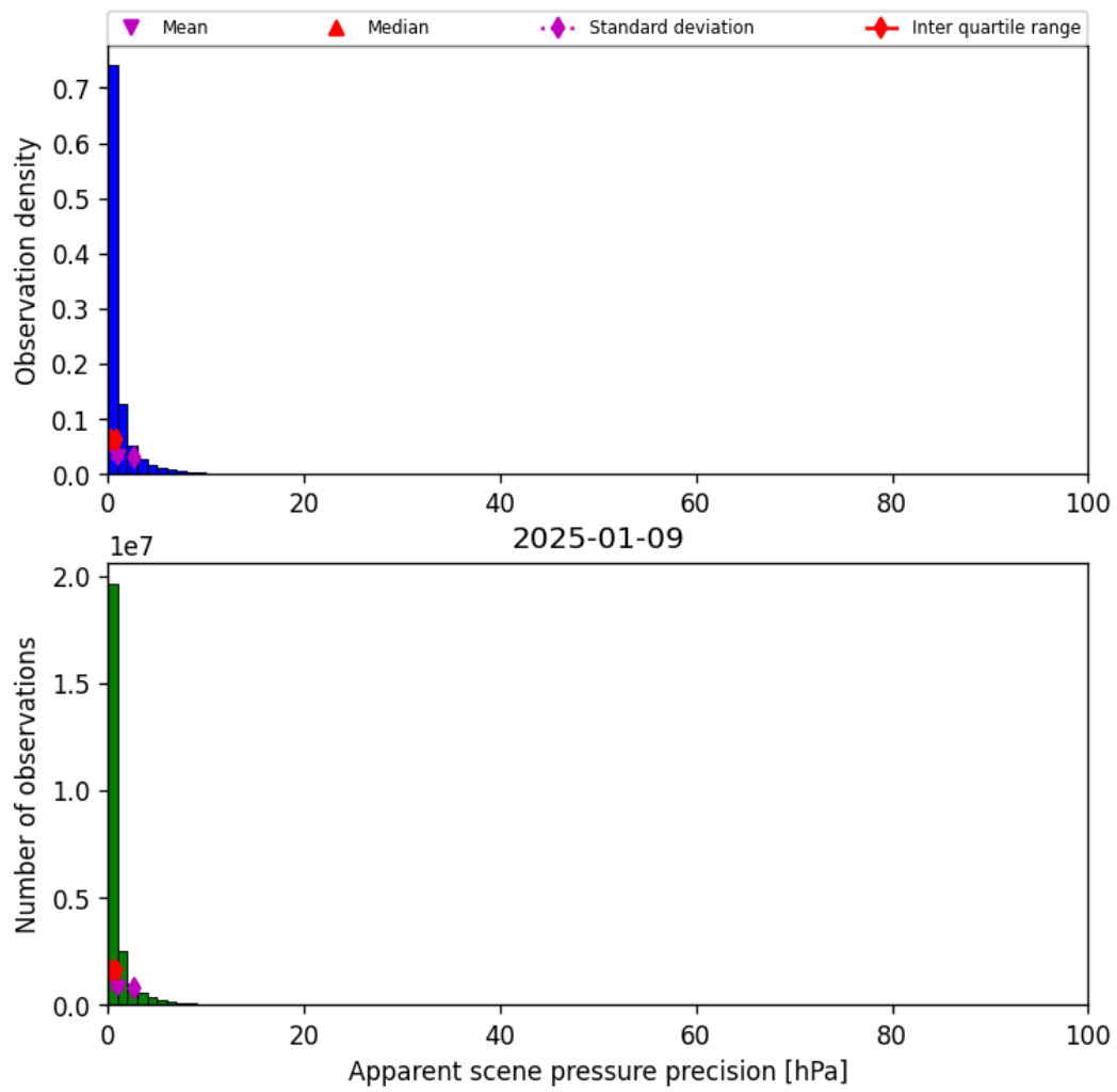
Figure 37: Histogram of “Apparent scene pressure precision” for 2025-01-08 to 2025-01-10
