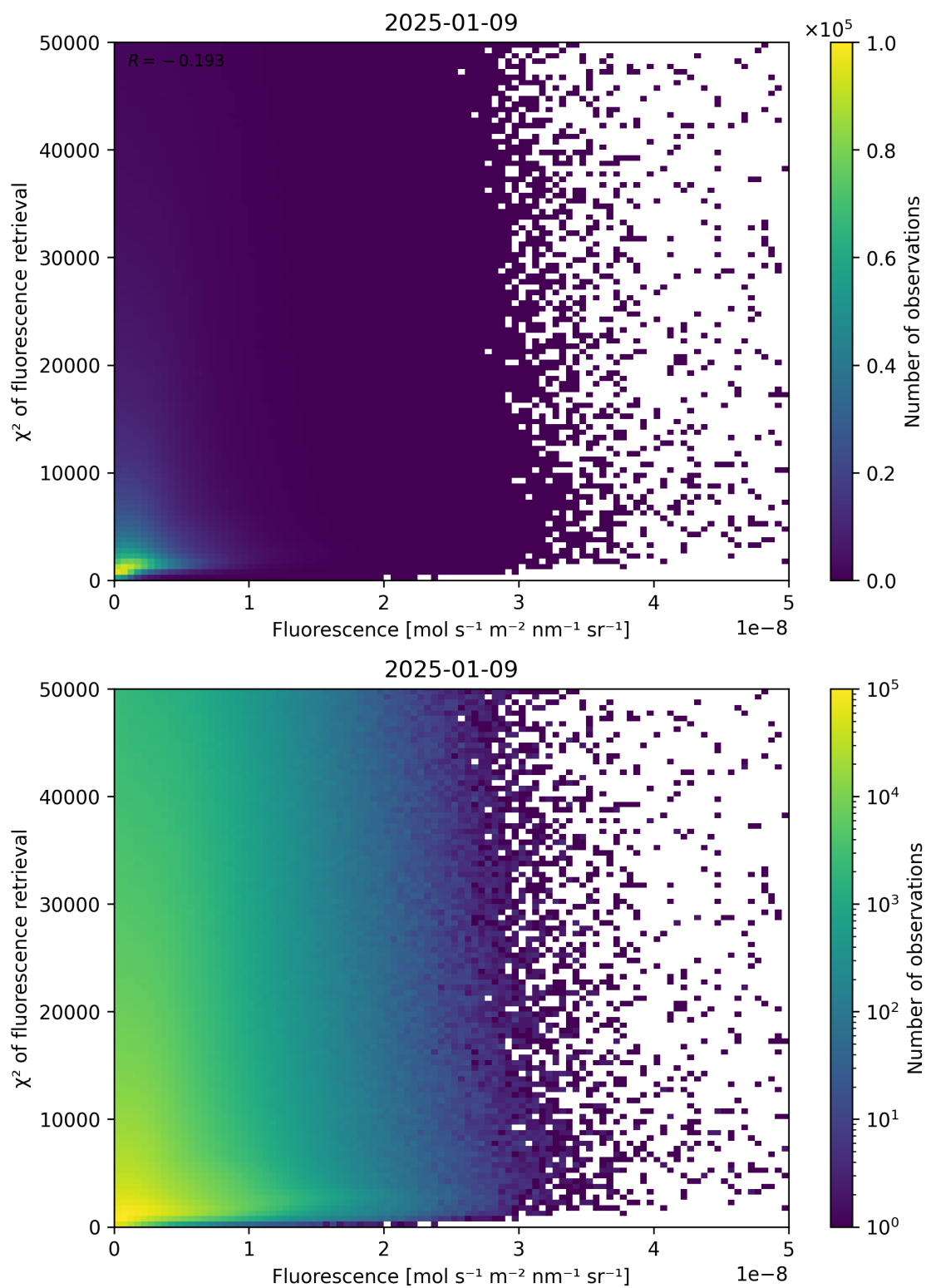
Figure 85: Scatter density plot of “Fluorescence” against “ \chi^2 of fluorescence retrieval” for 2025-01-08 to 2025-01-10.
