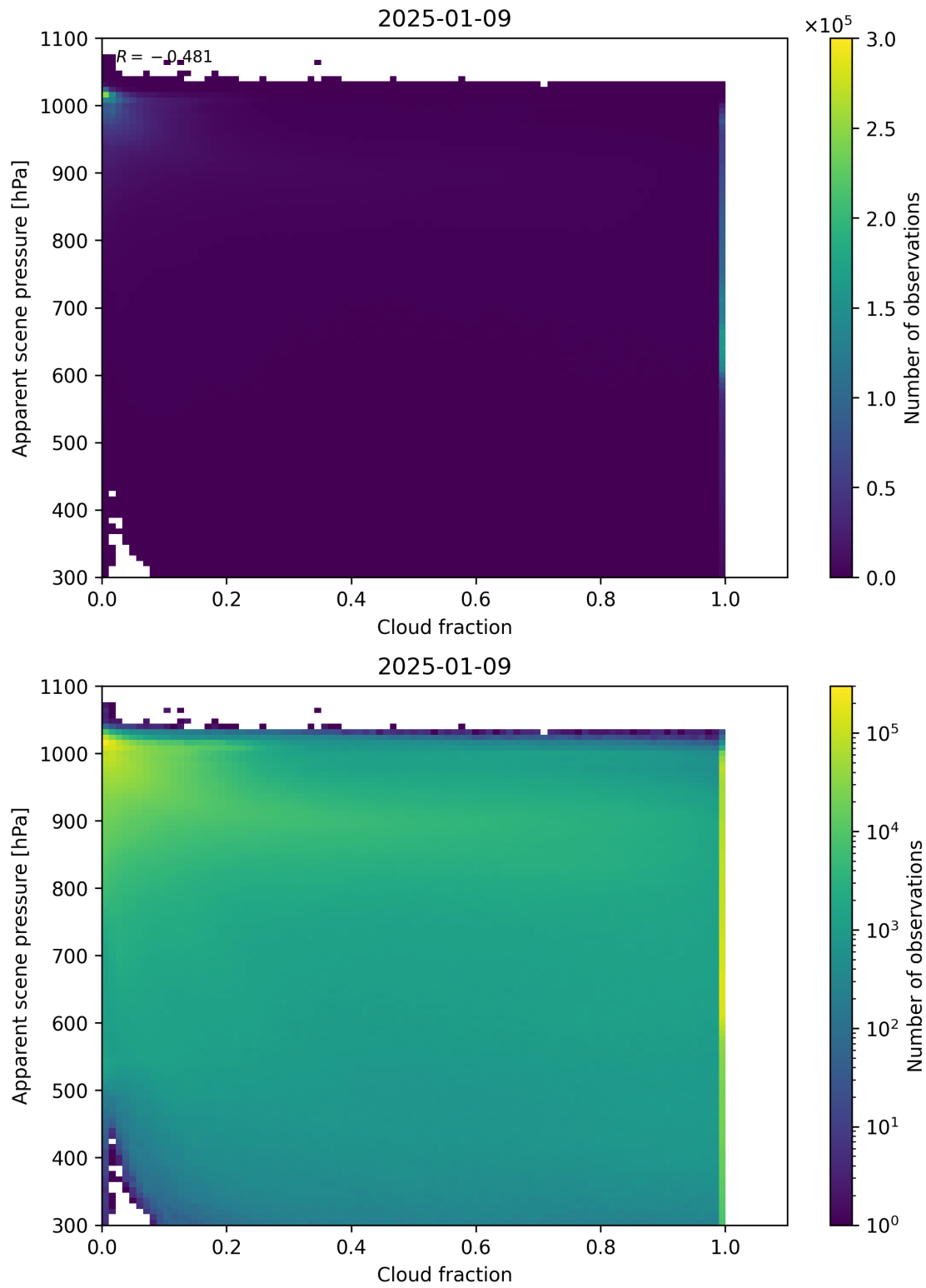
Figure 70: Scatter density plot of “Cloud fraction” against “Apparent scene pressure” for 2025-01-08 to 2025-01-10.
