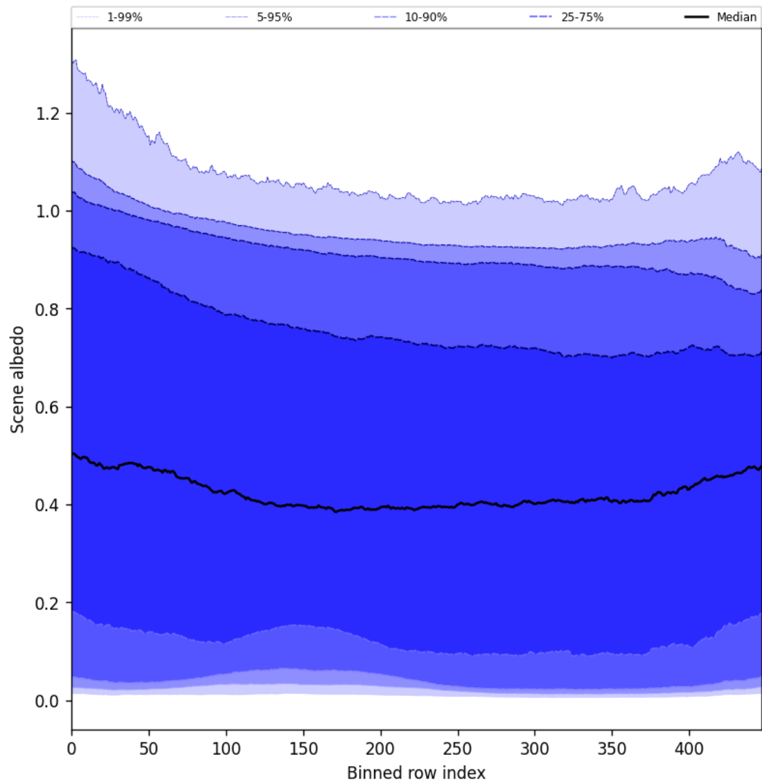
Figure 51: Along track statistics of “Scene albedo” for 2025-01-08 to 2025-01-10
