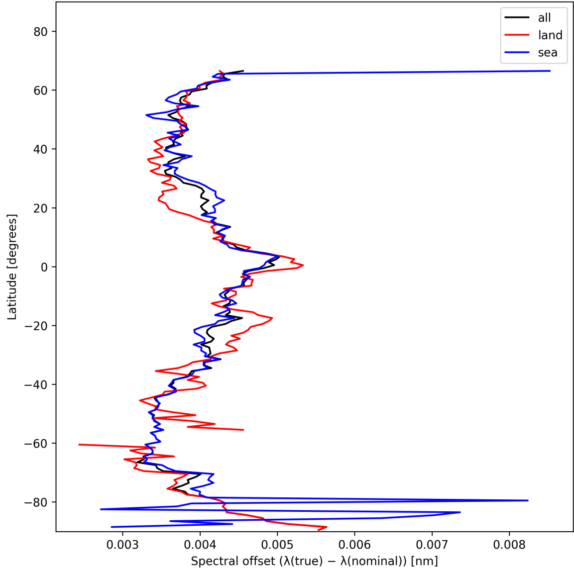
Figure 28: Zonal average of “Spectral offset ( \lambda_{\text{true}} - \lambda_{\text{nominal}} )” for 2025-01-08 to 2025-01-10.
