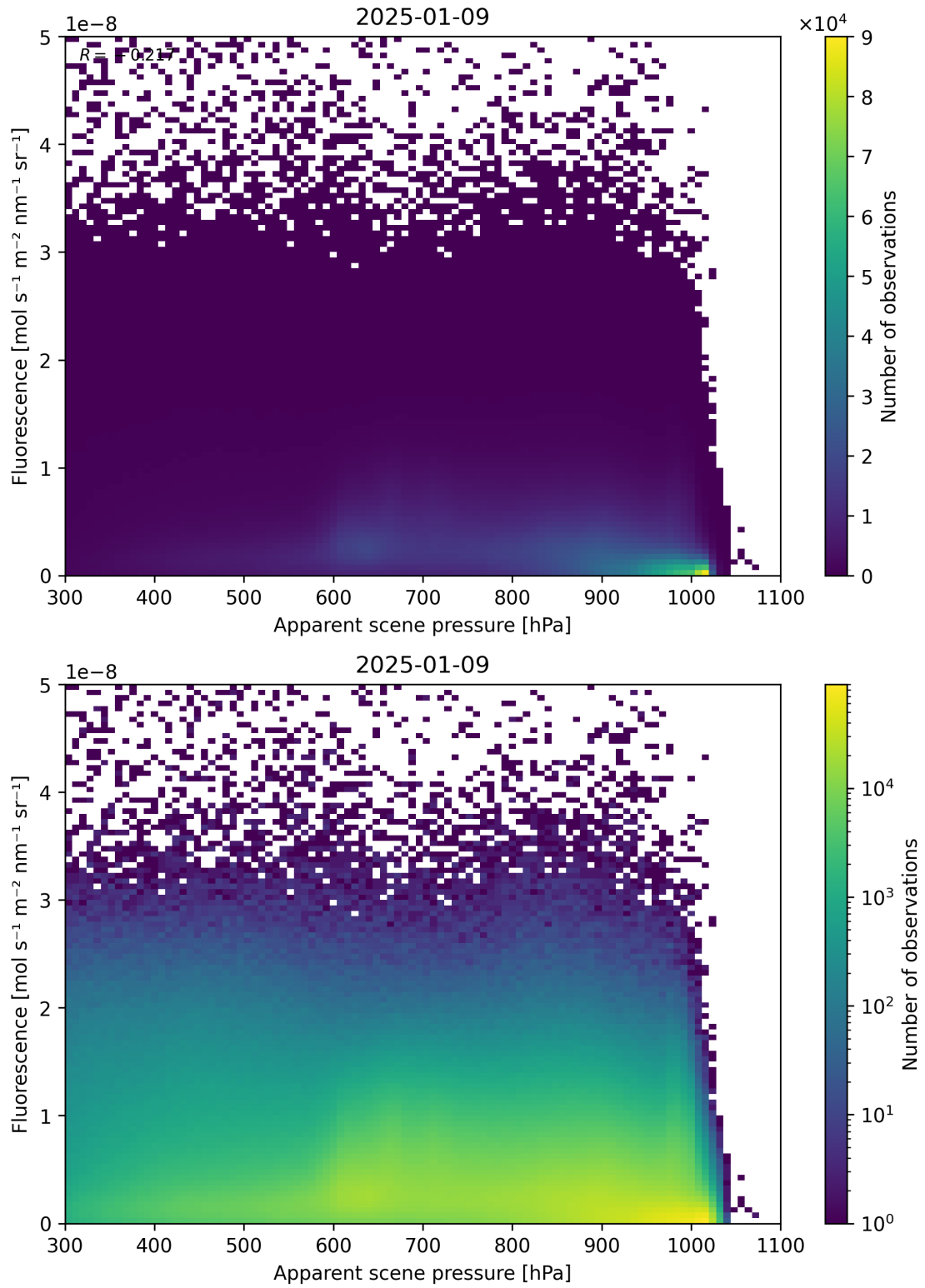
Figure 64: Scatter density plot of “Apparent scene pressure” against “Fluorescence” for 2025-01-08 to 2025-01-10.
