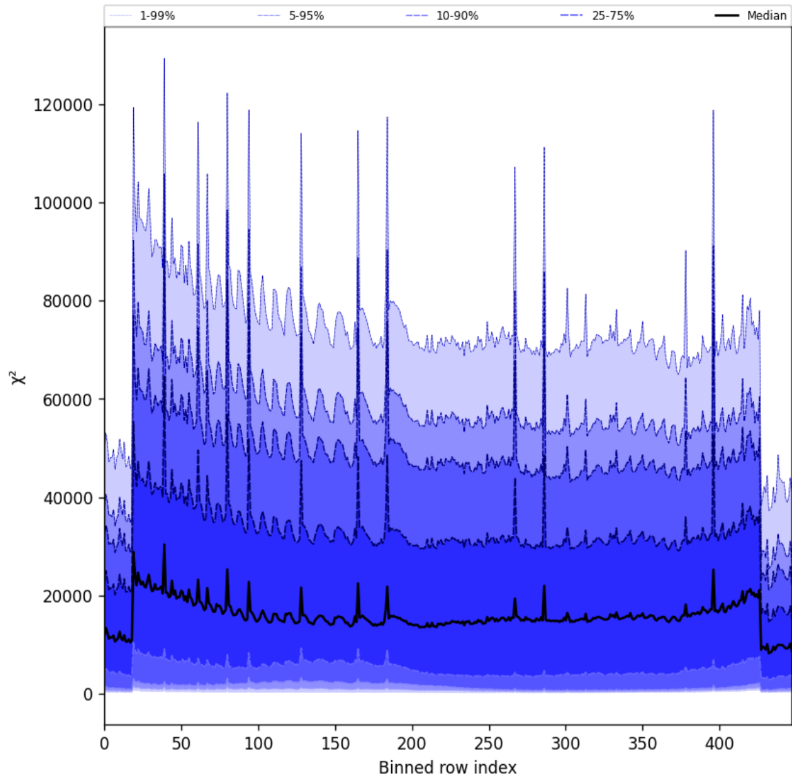
Figure 55: Along track statistics of “ \chi^2 ” for 2025-01-08 to 2025-01-10
