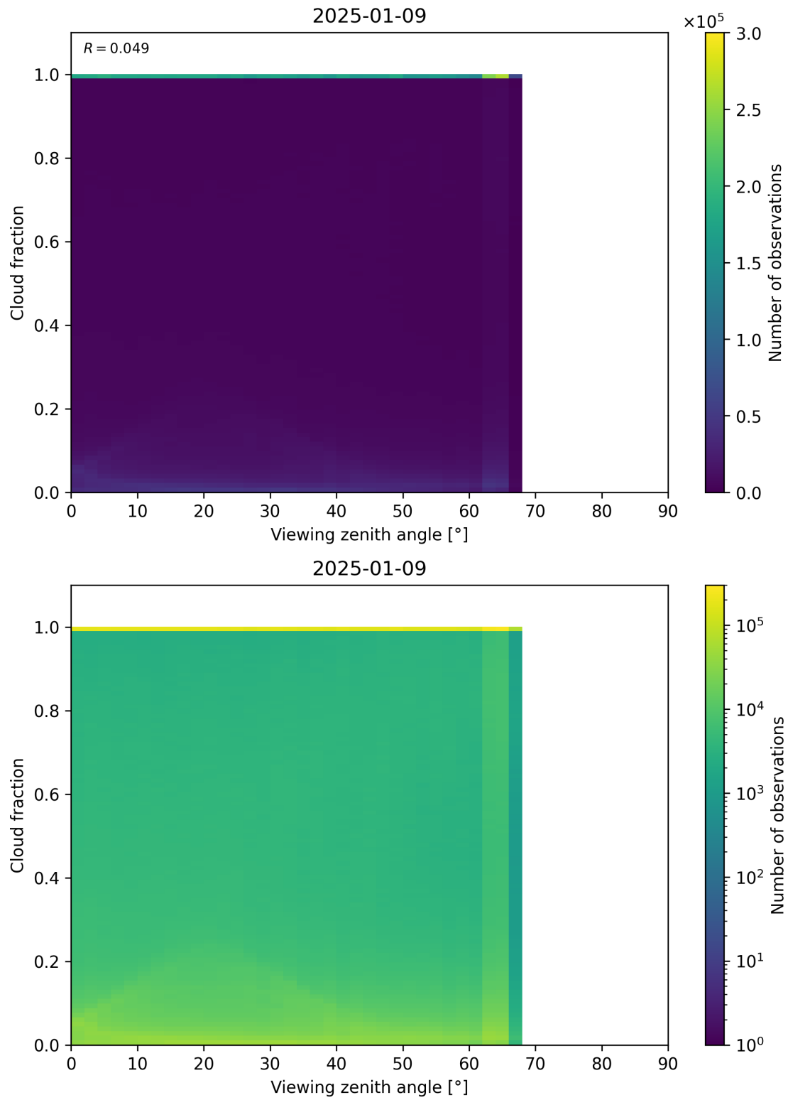
Figure 120: Scatter density plot of “Viewing zenith angle” against “Cloud fraction” for 2025-01-08 to 2025-01-10.
