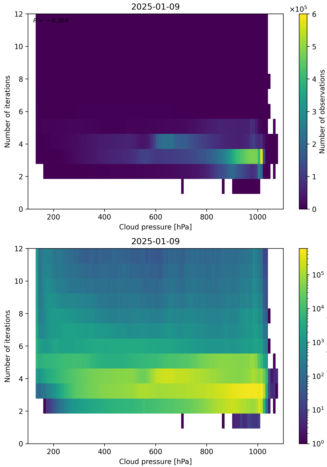
Figure 81: Scatter density plot of “Cloud pressure” against “Number of iterations” for 2025-01-08 to 2025-01-10.
