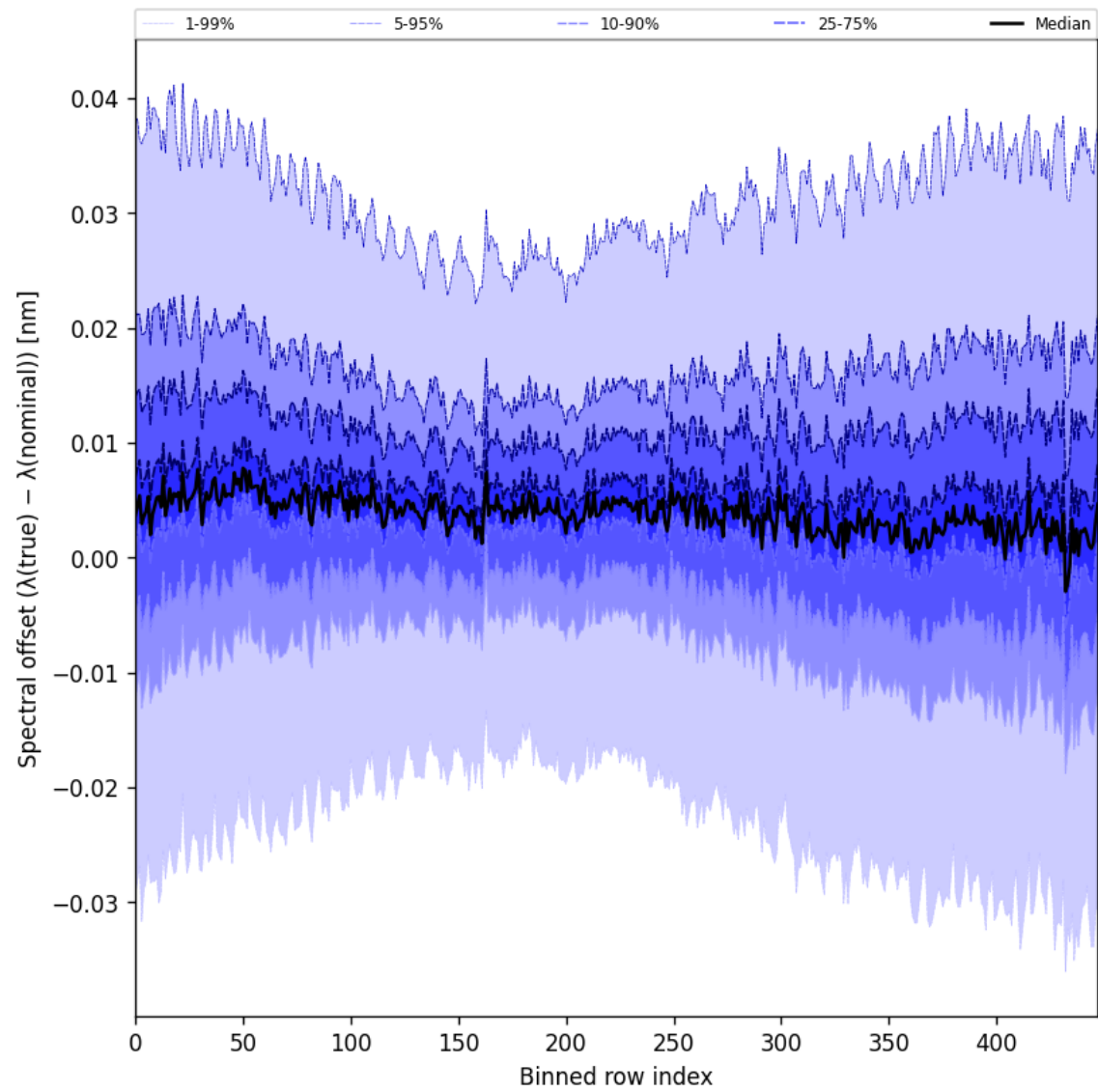
Figure 62: Along track statistics of “Spectral offset ( \lambda_{\text{true}} - \lambda_{\text{nominal}} )” for 2025-01-08 to 2025-01-10
