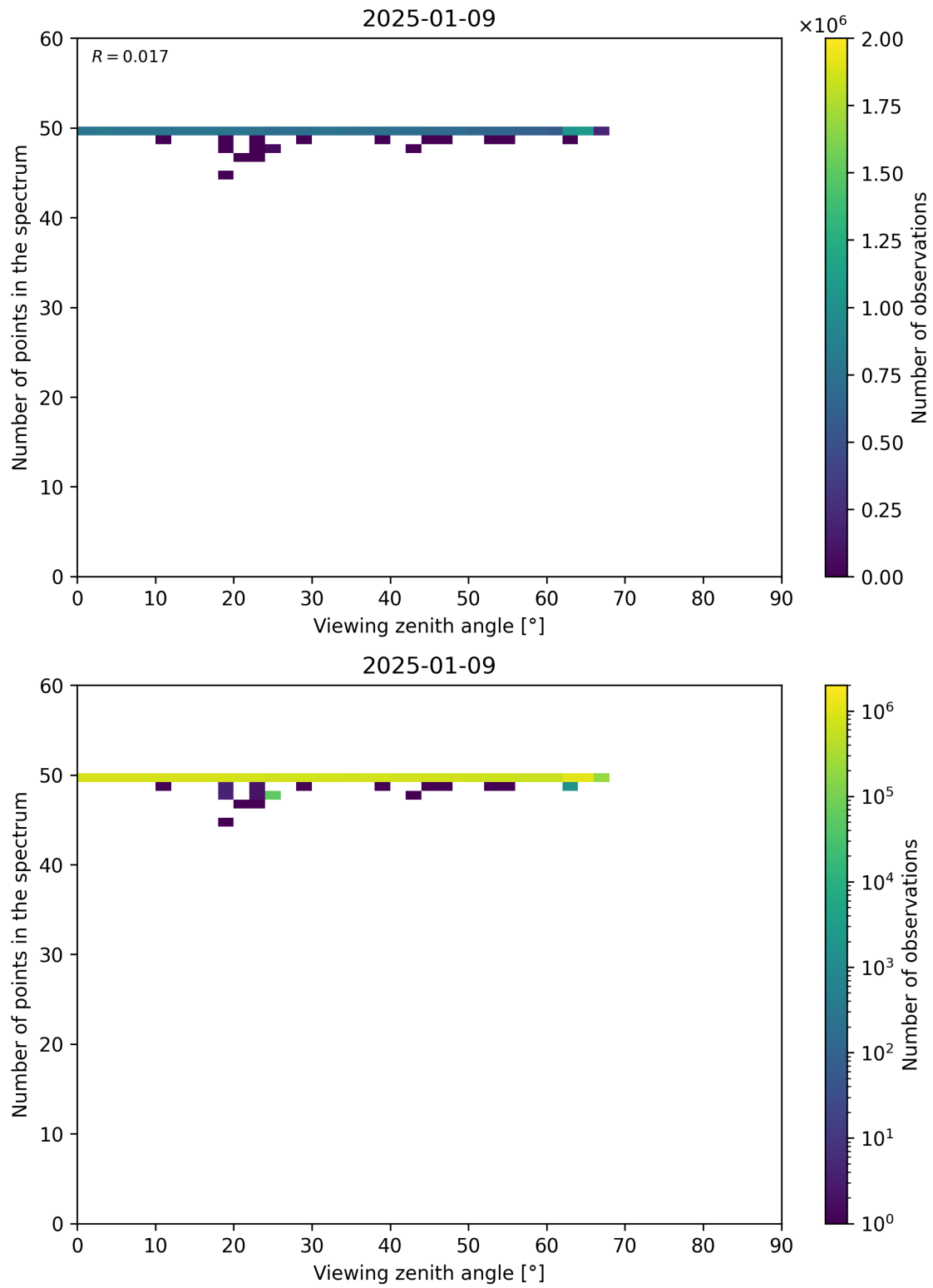
Figure 125: Scatter density plot of “Viewing zenith angle” against “Number of points in the spectrum” for 2025-01-08 to 2025-01-10.
