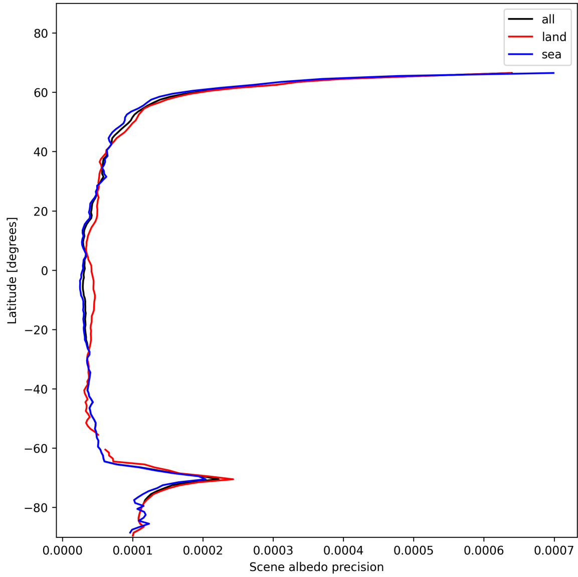
Figure 18: Zonal average of “Scene albedo precision” for 2025-01-08 to 2025-01-10.
