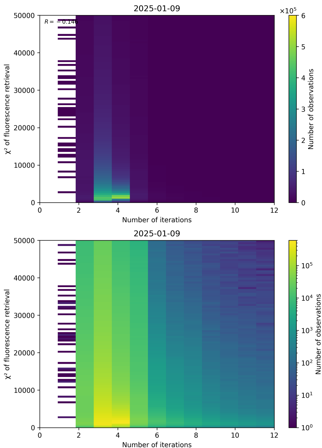
Figure 97: Scatter density plot of “Number of iterations” against “ \chi^2 of fluorescence retrieval” for 2025-01-08 to 2025-01-10.
