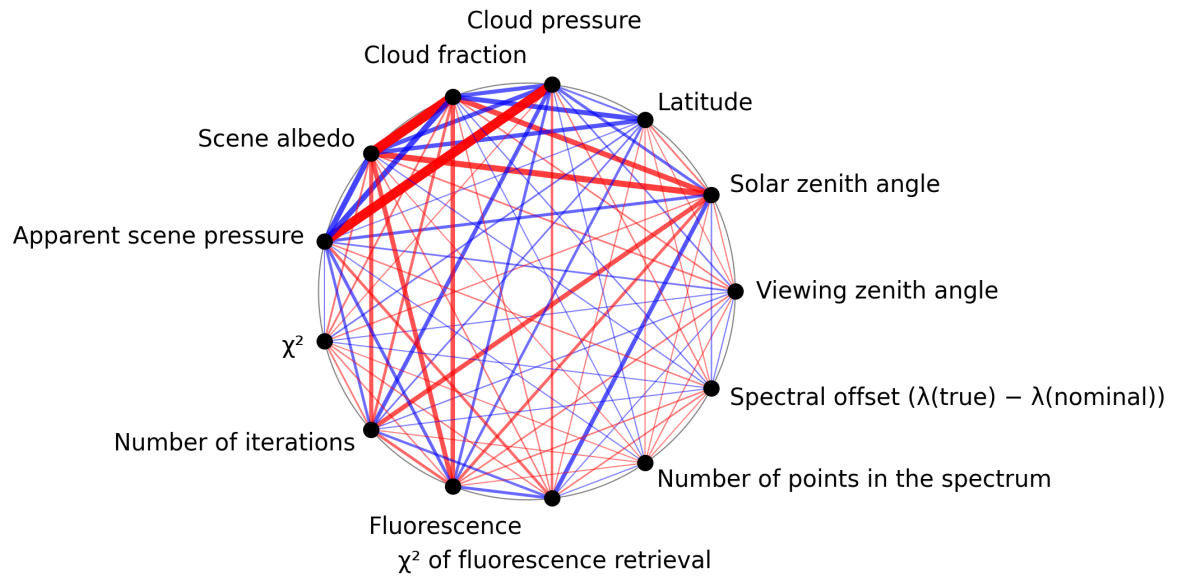
Figure 1: Map of correlation graph for 2025-01-08 to 2025-01-10.
