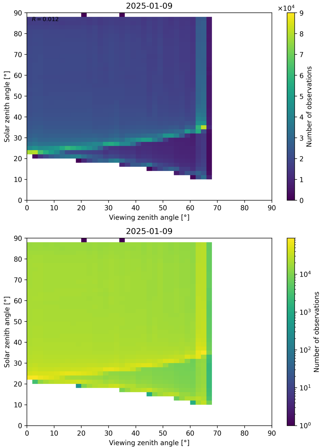
Figure 127: Scatter density plot of “Viewing zenith angle” against “Solar zenith angle” for 2025-01-08 to 2025-01-10.
