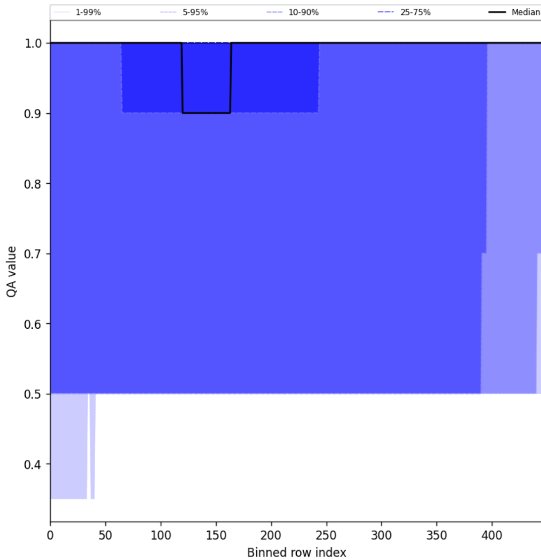
Figure 46: Along track statistics of “QA value” for 2025-01-08 to 2025-01-10
