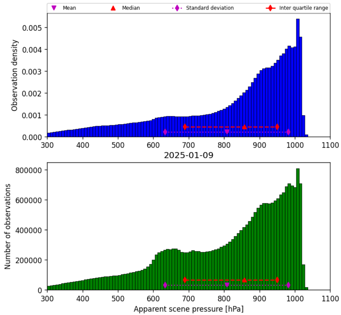
Figure 36: Histogram of “Apparent scene pressure” for 2025-01-08 to 2025-01-10
