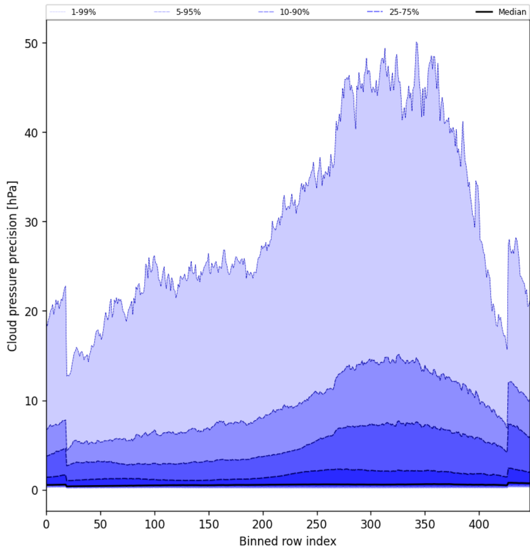
Figure 48: Along track statistics of “Cloud pressure precision” for 2025-01-08 to 2025-01-10
