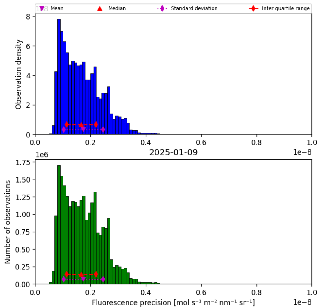
Figure 41: Histogram of “Fluorescence precision” for 2025-01-08 to 2025-01-10
