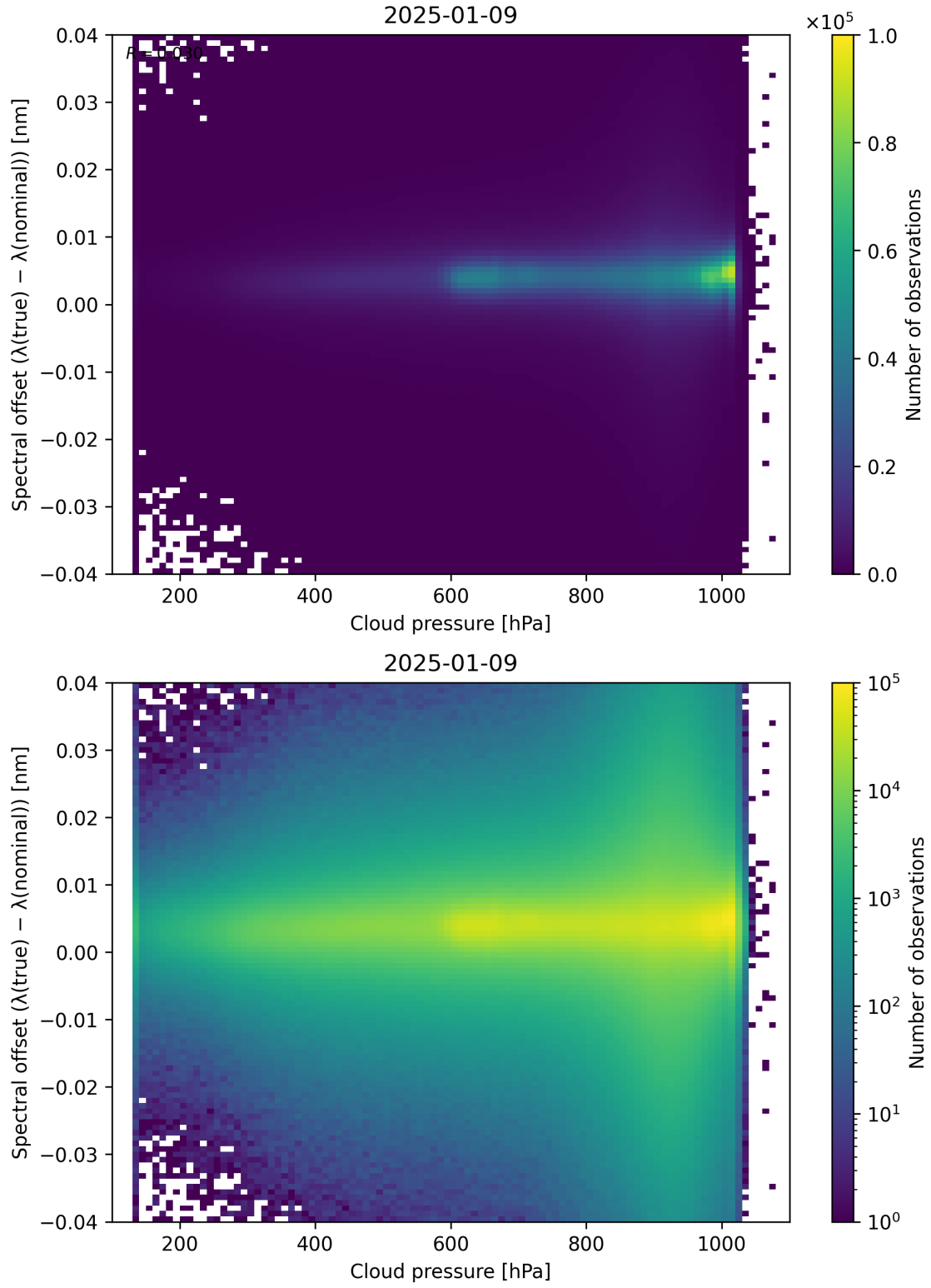
Figure 84: Scatter density plot of “Cloud pressure” against “Spectral offset ( \lambda_{\text{true}} - \lambda_{\text{nominal}} )” for 2025-01-08 to 2025-01-10.
