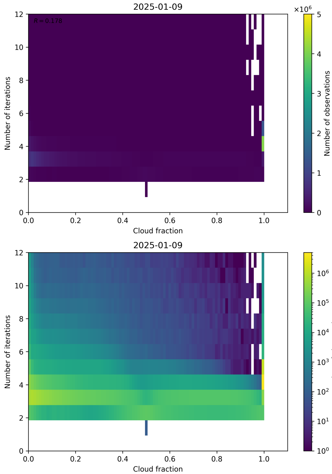
Figure 73: Scatter density plot of “Cloud fraction” against “Number of iterations” for 2025-01-08 to 2025-01-10.
