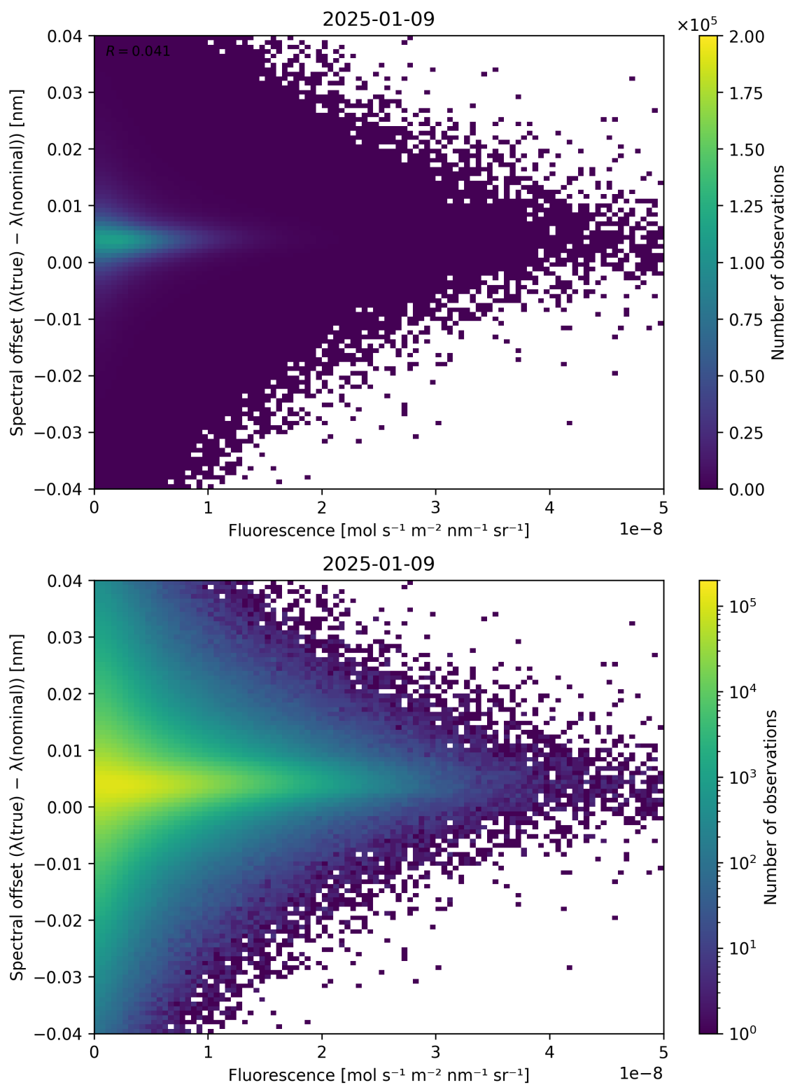
Figure 87: Scatter density plot of “Fluorescence” against “Spectral offset ( \lambda_{\text{true}} - \lambda_{\text{nominal}} )” for 2025-01-08 to 2025-01-10.
