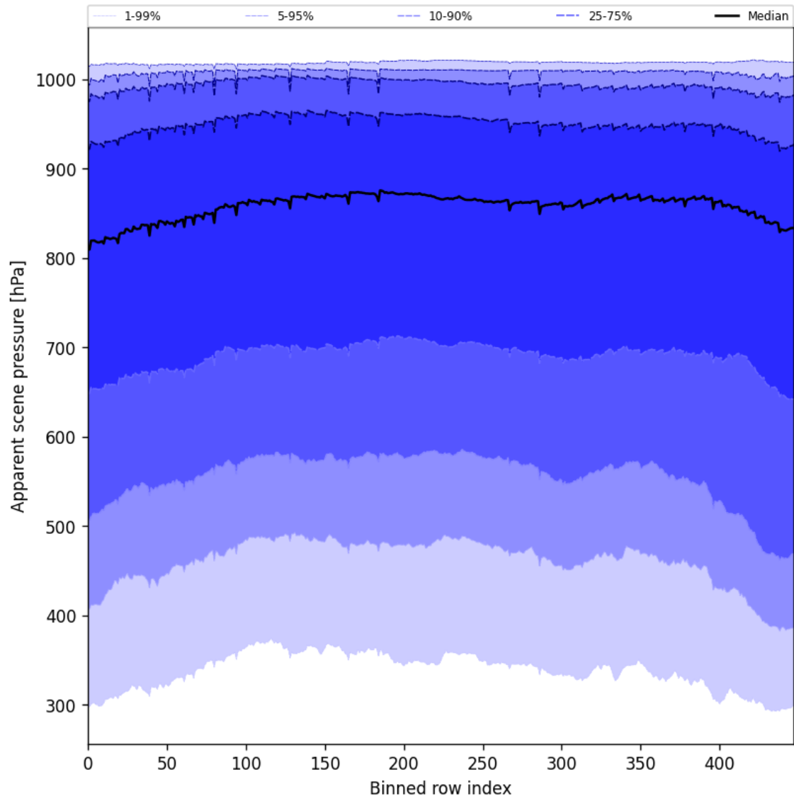
Figure 53: Along track statistics of “Apparent scene pressure” for 2025-01-08 to 2025-01-10
