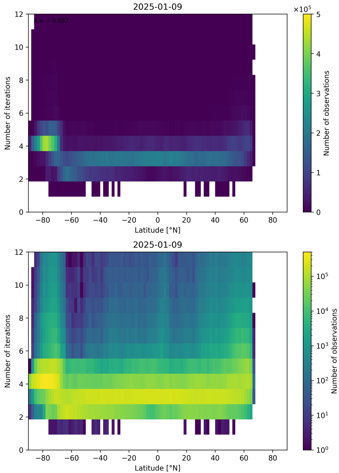
Figure 93: Scatter density plot of “Latitude” against “Number of iterations” for 2025-01-08 to 2025-01-10.
