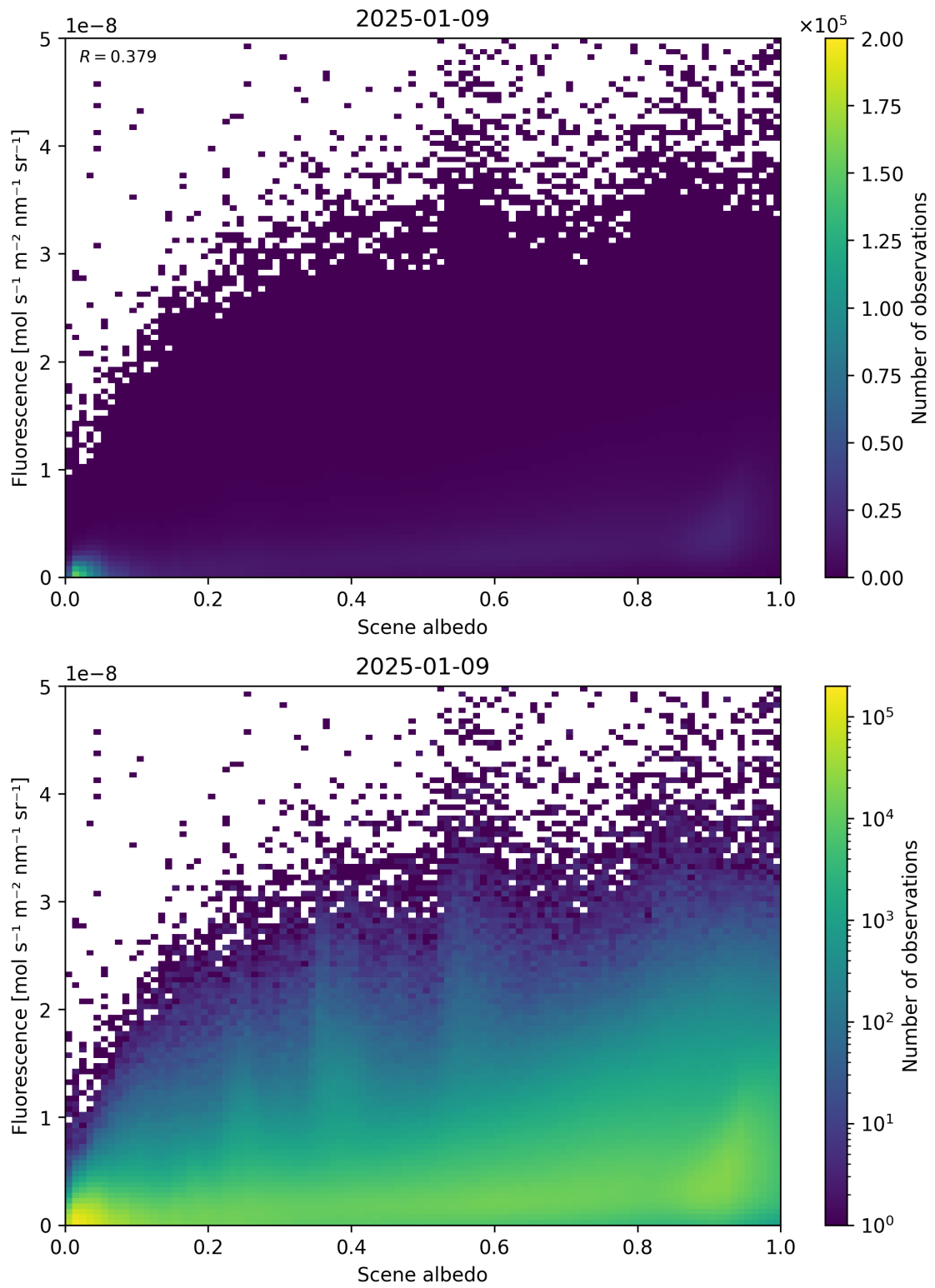
Figure 104: Scatter density plot of “Scene albedo” against “Fluorescence” for 2025-01-08 to 2025-01-10.
