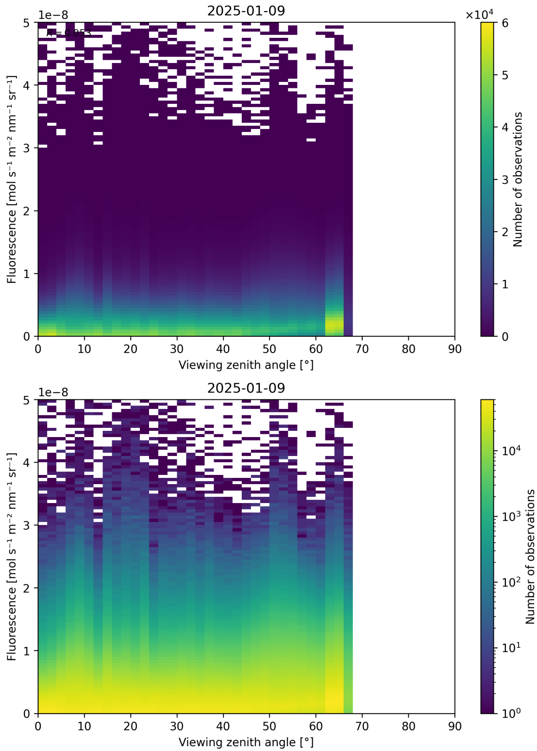
Figure 122: Scatter density plot of “Viewing zenith angle” against “Fluorescence” for 2025-01-08 to 2025-01-10.
