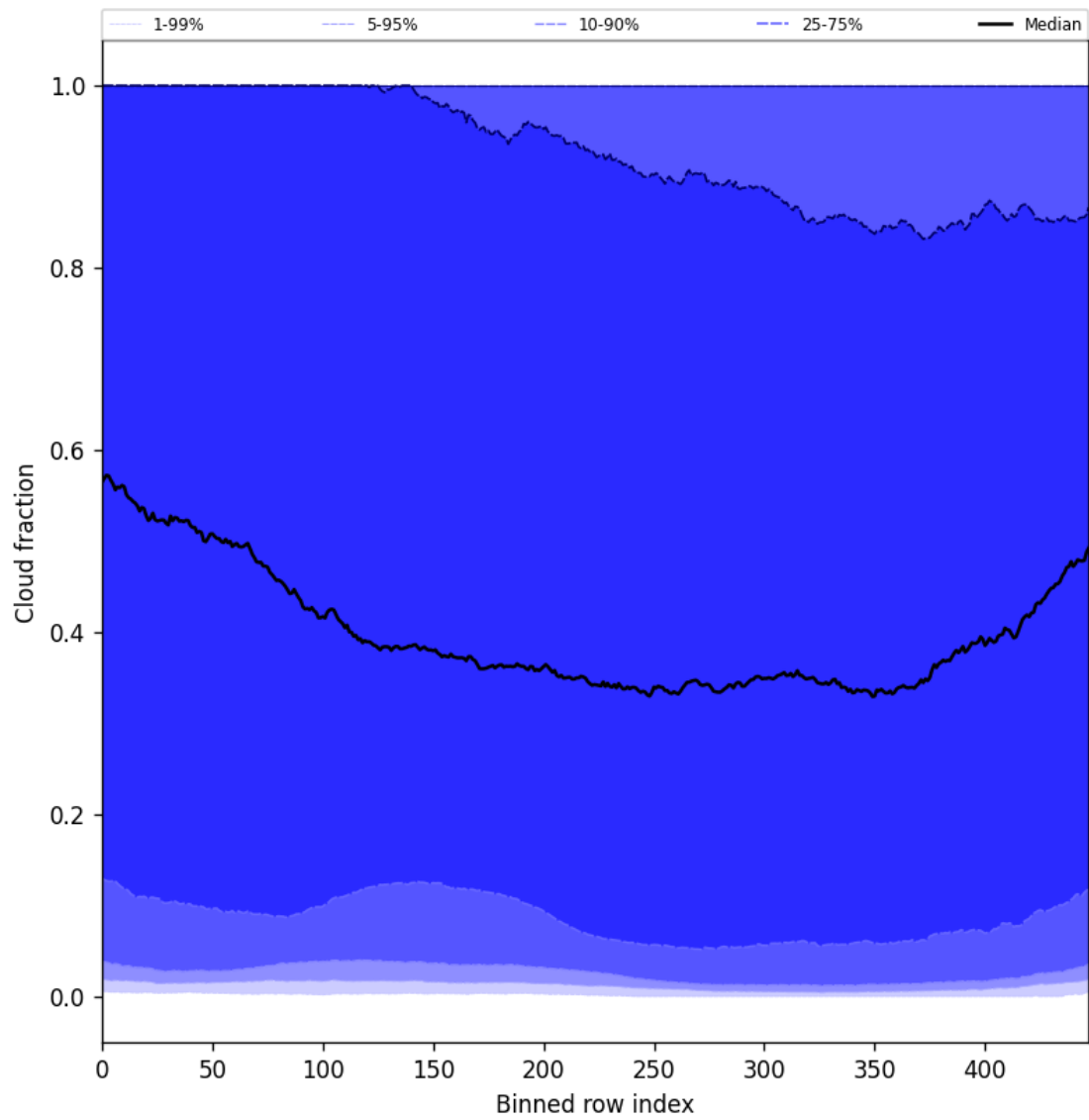
Figure 49: Along track statistics of “Cloud fraction” for 2025-01-08 to 2025-01-10
