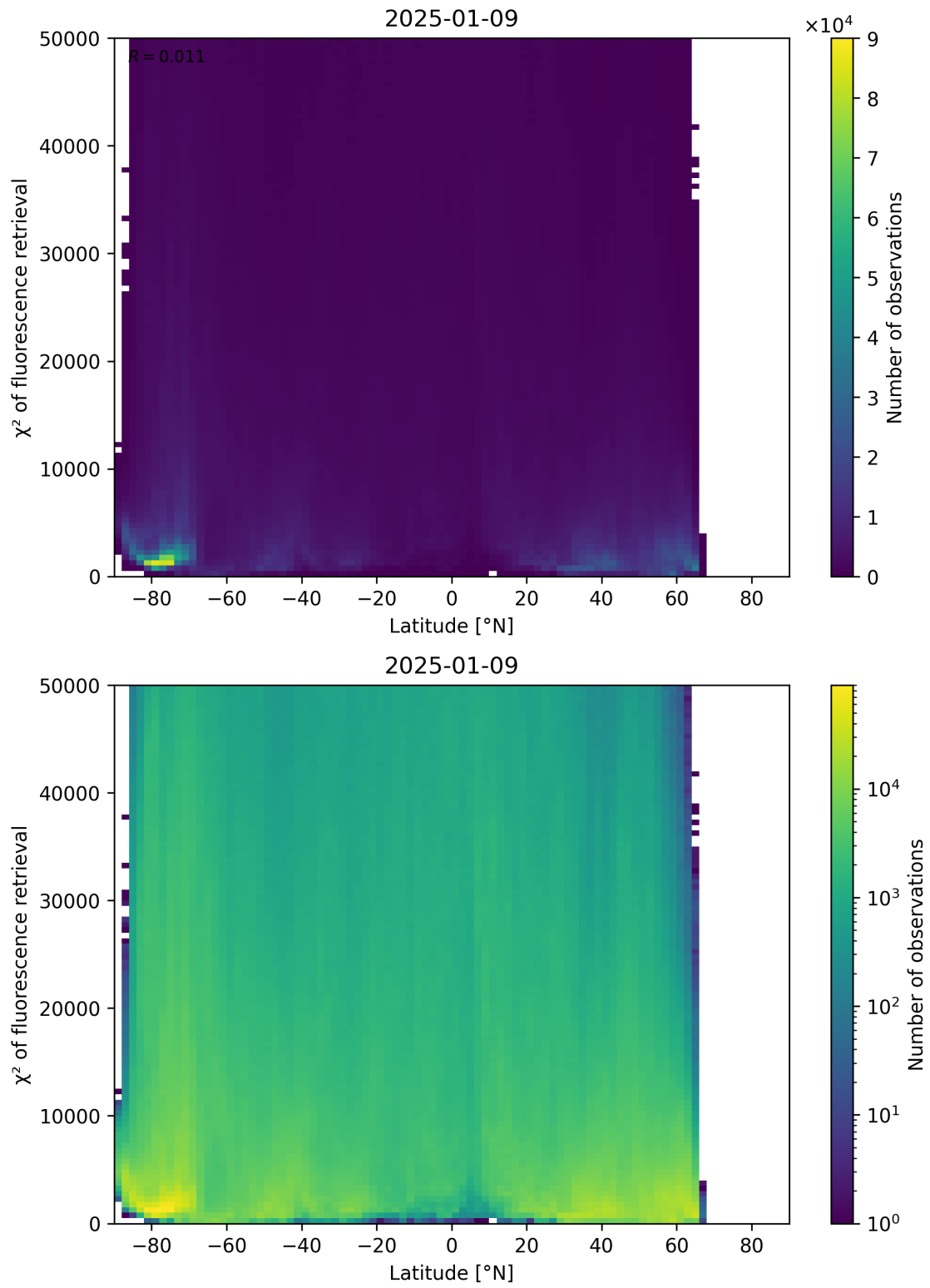
Figure 89: Scatter density plot of “Latitude” against “ \chi^2 of fluorescence retrieval” for 2025-01-08 to 2025-01-10.
