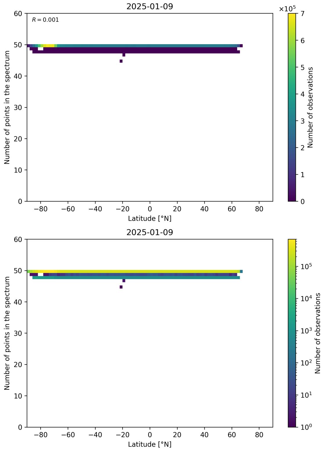
Figure 94: Scatter density plot of “Latitude” against “Number of points in the spectrum” for 2025-01-08 to 2025-01-10.
