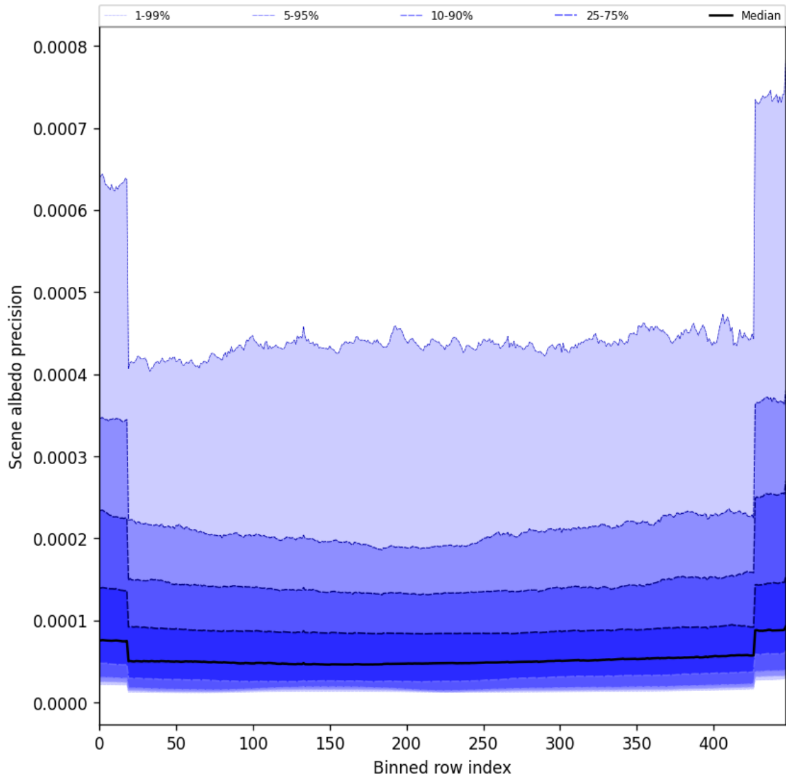
Figure 52: Along track statistics of “Scene albedo precision” for 2025-01-08 to 2025-01-10
