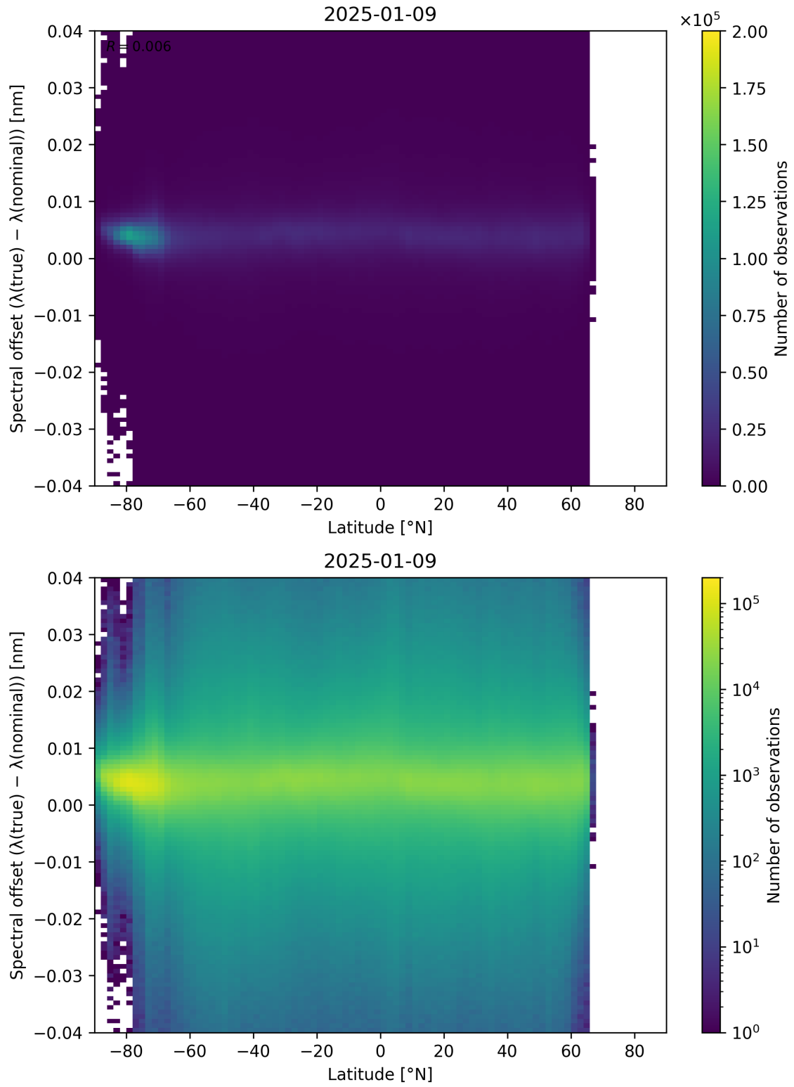
Figure 96: Scatter density plot of “Latitude” against “Spectral offset ( \lambda_{\text{true}} - \lambda_{\text{nominal}} )” for 2025-01-08 to 2025-01-10.
