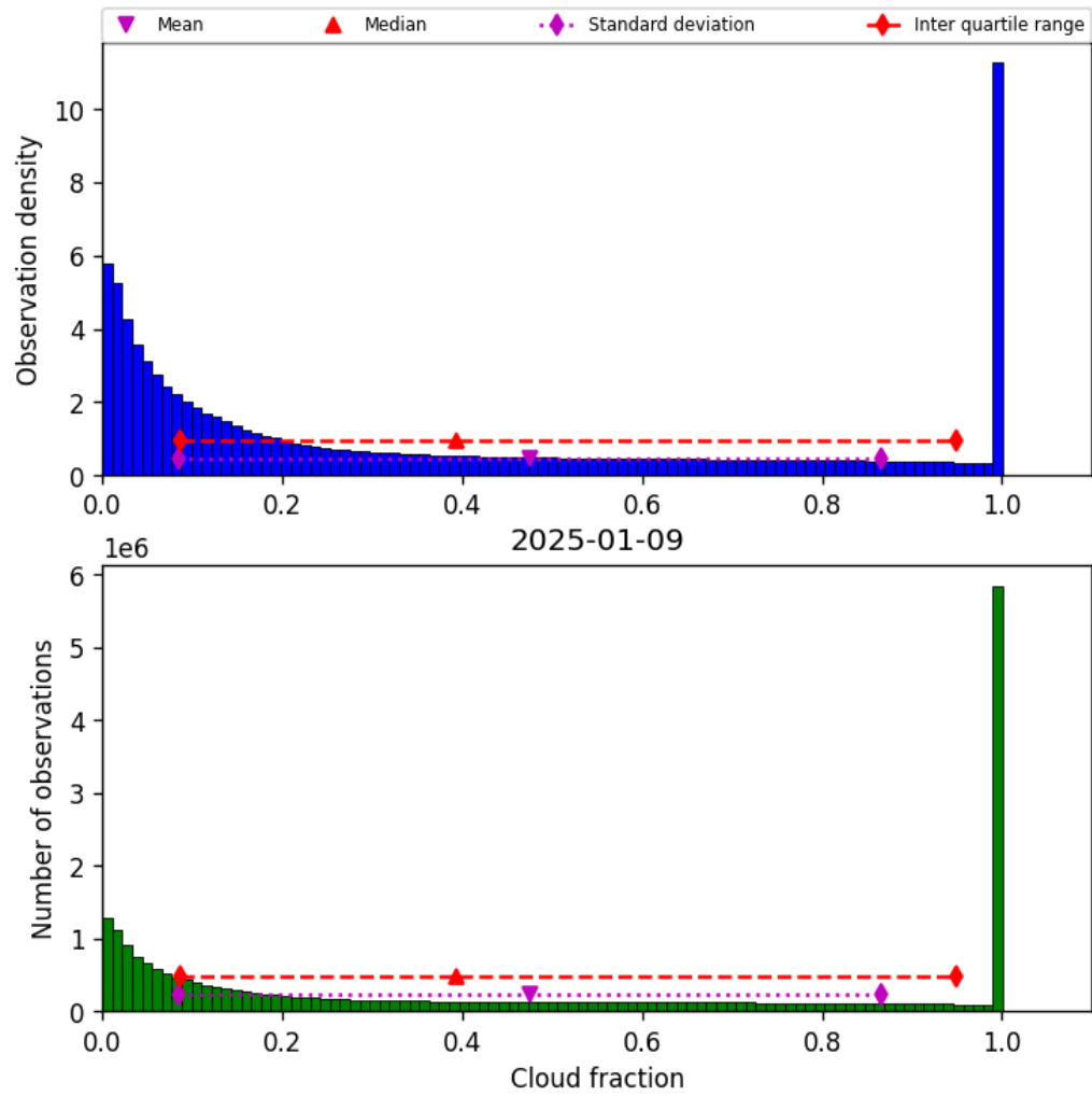
Figure 32: Histogram of “Cloud fraction” for 2025-01-08 to 2025-01-10
