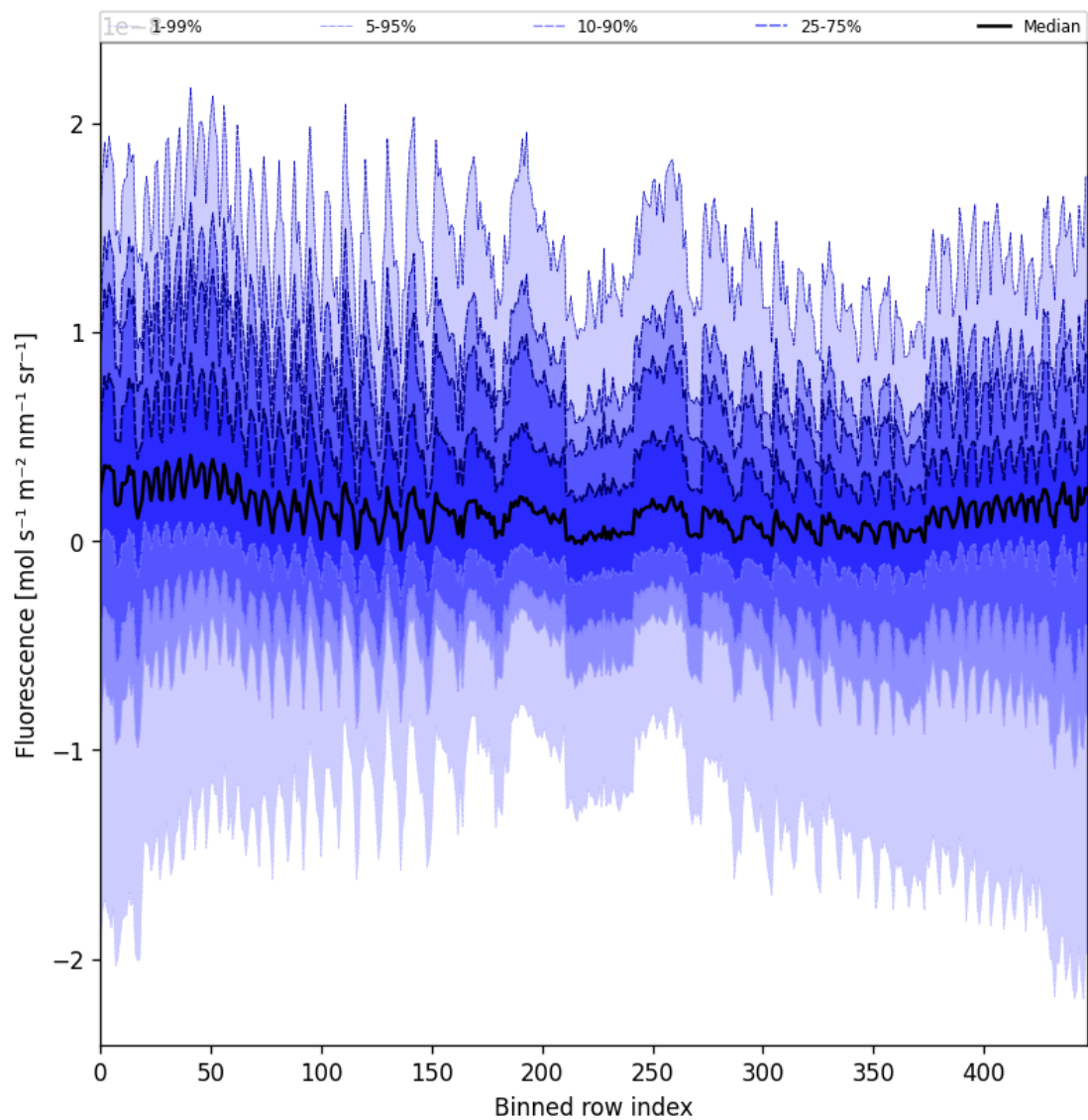
Figure 57: Along track statistics of “Fluorescence” for 2025-01-08 to 2025-01-10
