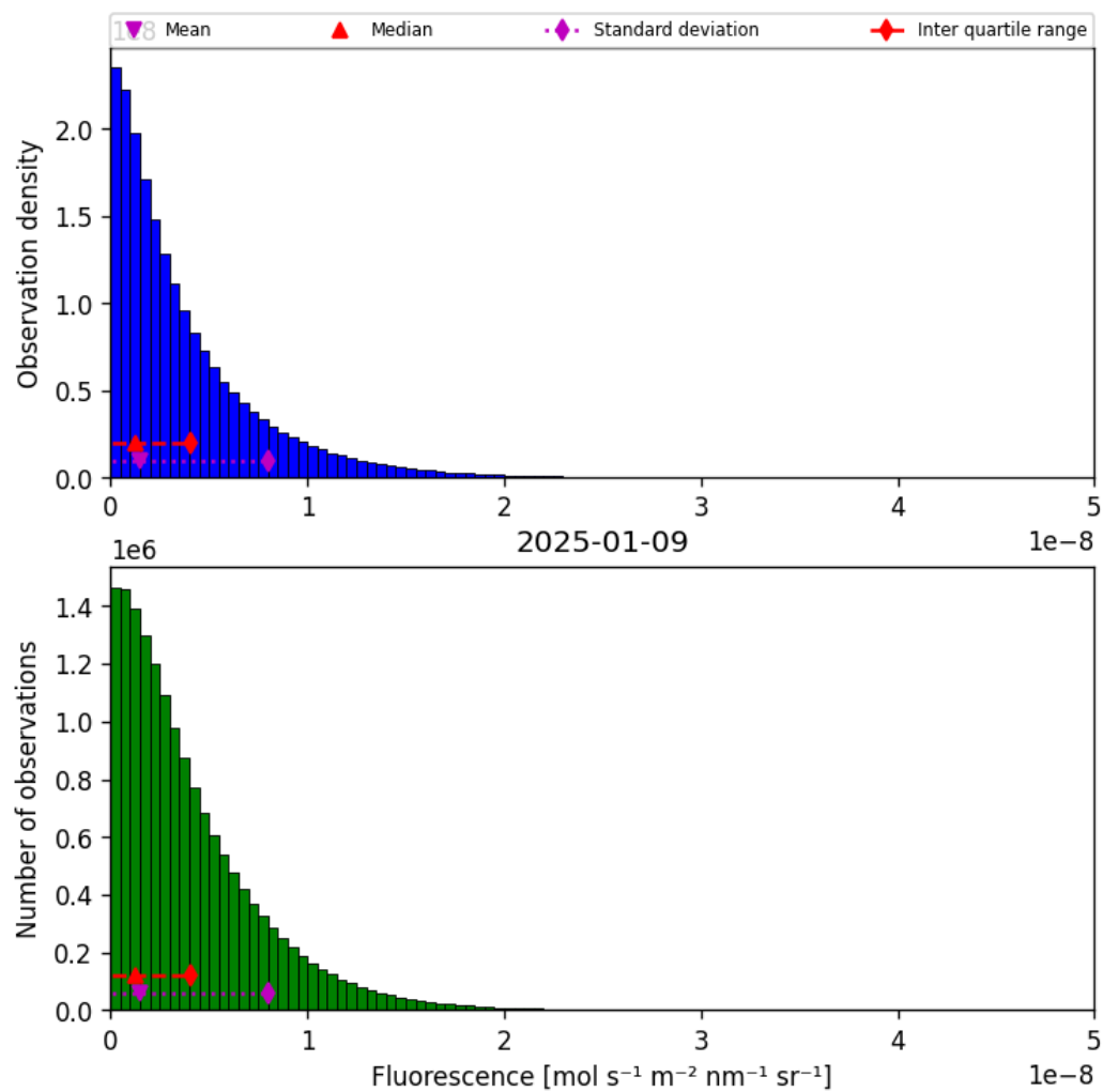
Figure 40: Histogram of “Fluorescence” for 2025-01-08 to 2025-01-10
