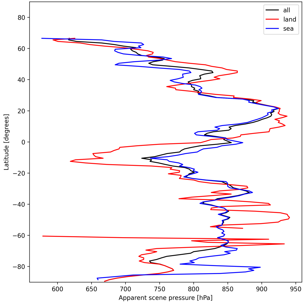
Figure 19: Zonal average of “Apparent scene pressure” for 2025-01-08 to 2025-01-10.
