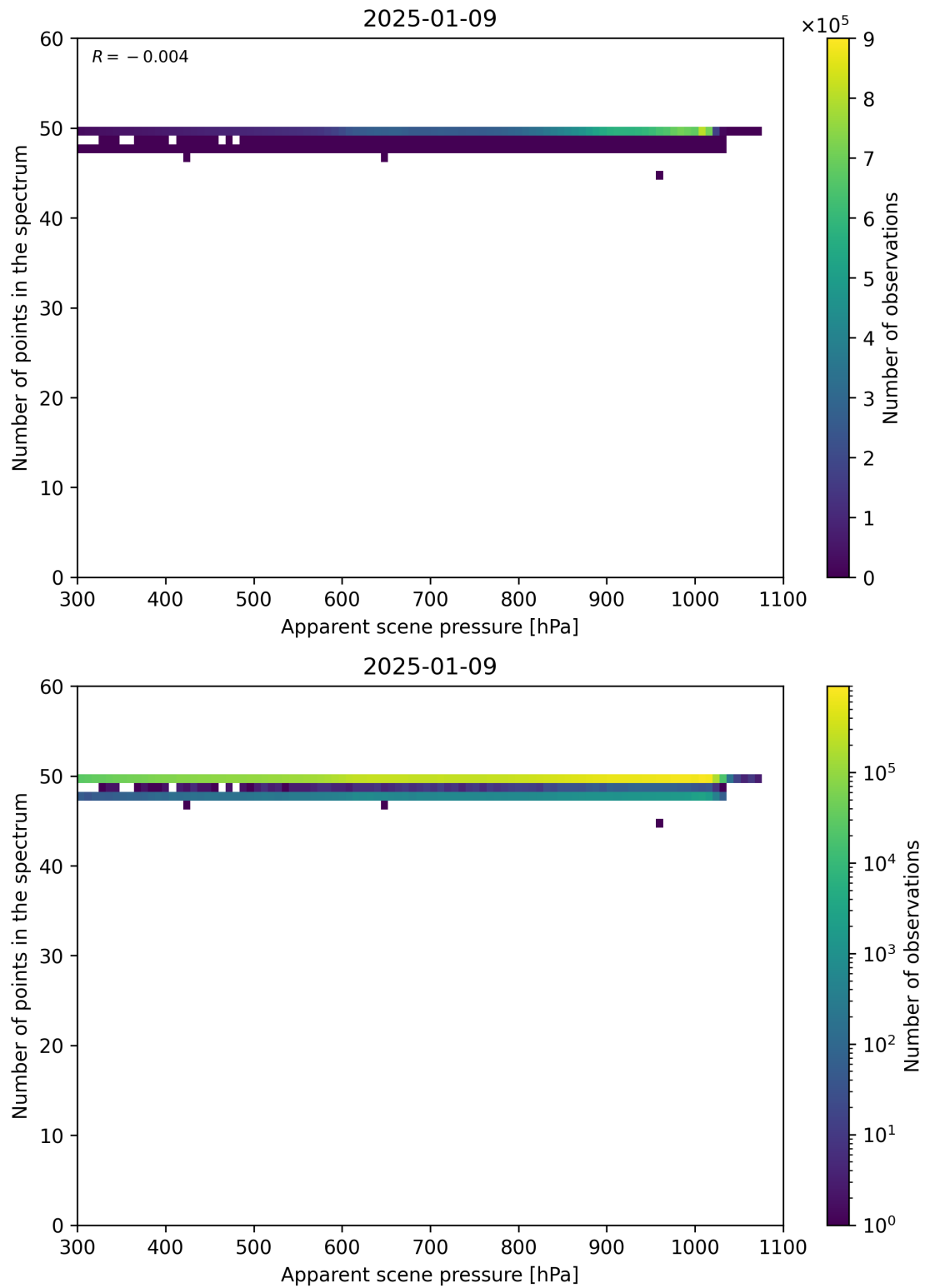
Figure 66: Scatter density plot of “Apparent scene pressure” against “Number of points in the spectrum” for 2025-01-08 to 2025-01-10.
