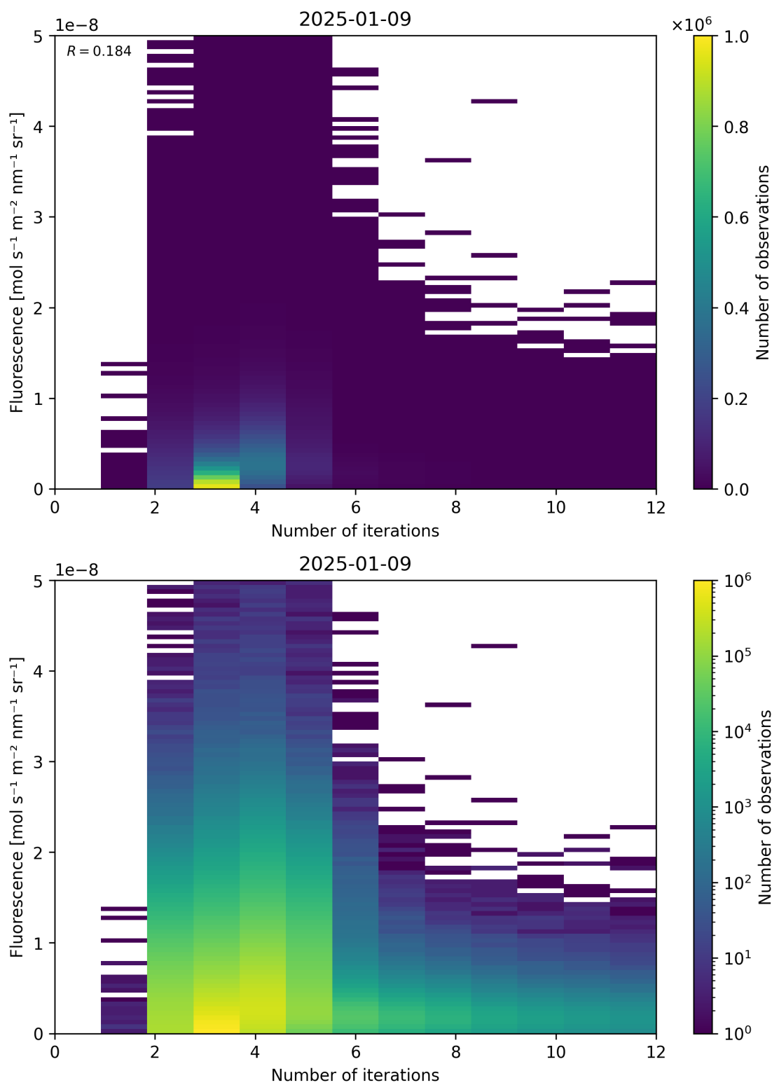
Figure 98: Scatter density plot of “Number of iterations” against “Fluorescence” for 2025-01-08 to 2025-01-10.
