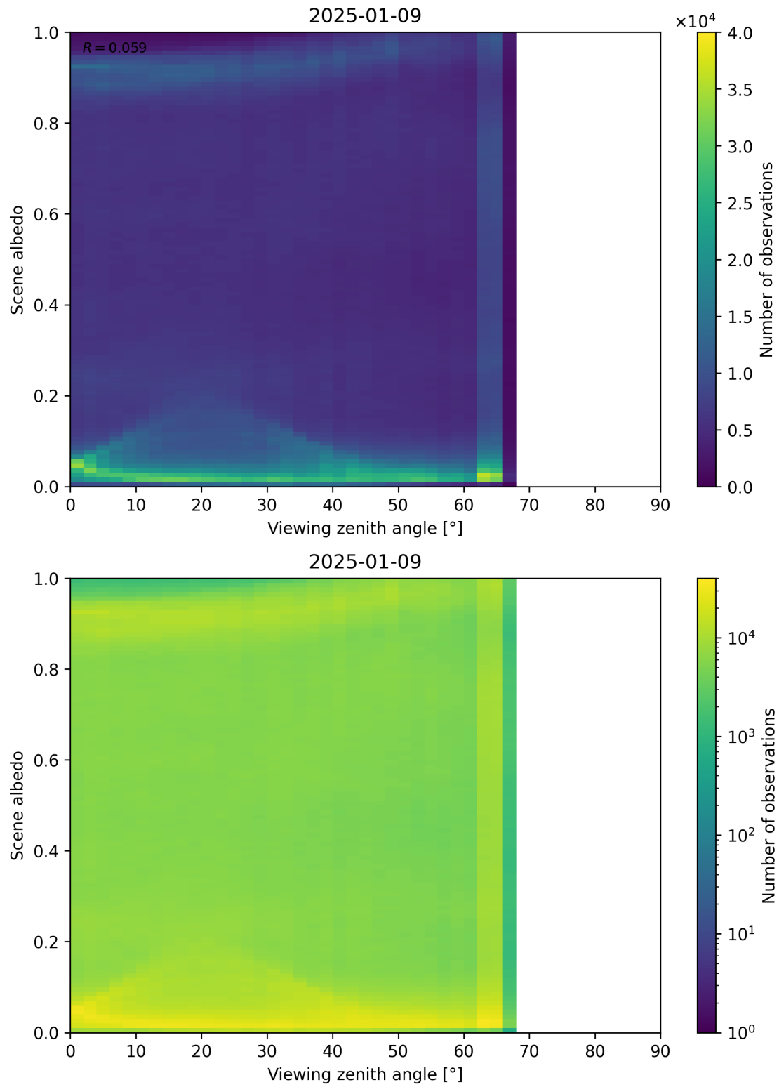
Figure 126: Scatter density plot of “Viewing zenith angle” against “Scene albedo” for 2025-01-08 to 2025-01-10.
