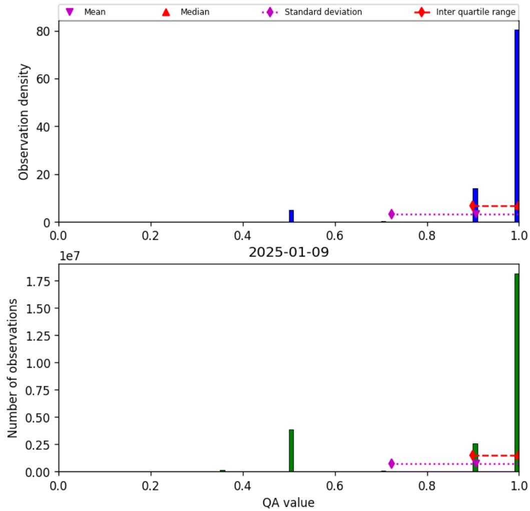
Figure 29: Histogram of “QA value” for 2025-01-08 to 2025-01-10
