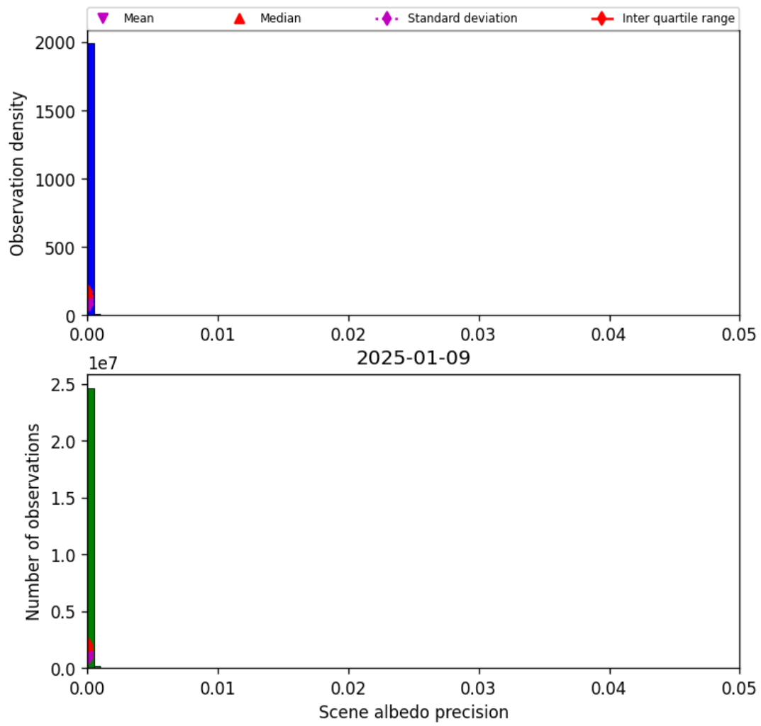
Figure 35: Histogram of “Scene albedo precision” for 2025-01-08 to 2025-01-10
