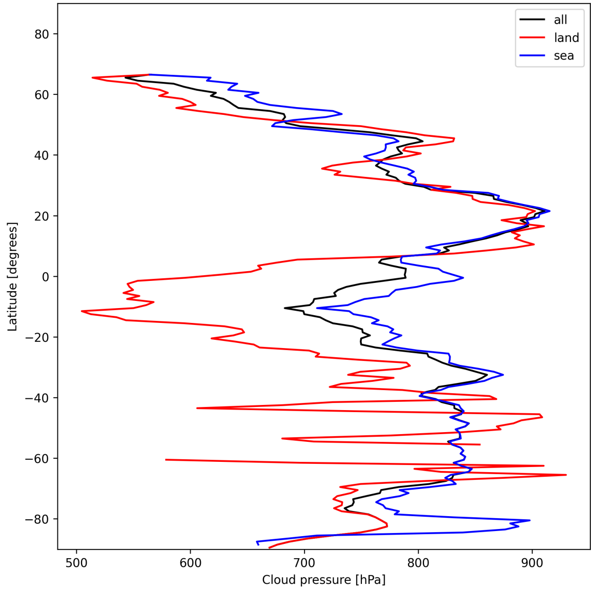
Figure 13: Zonal average of “Cloud pressure” for 2025-01-08 to 2025-01-10.
