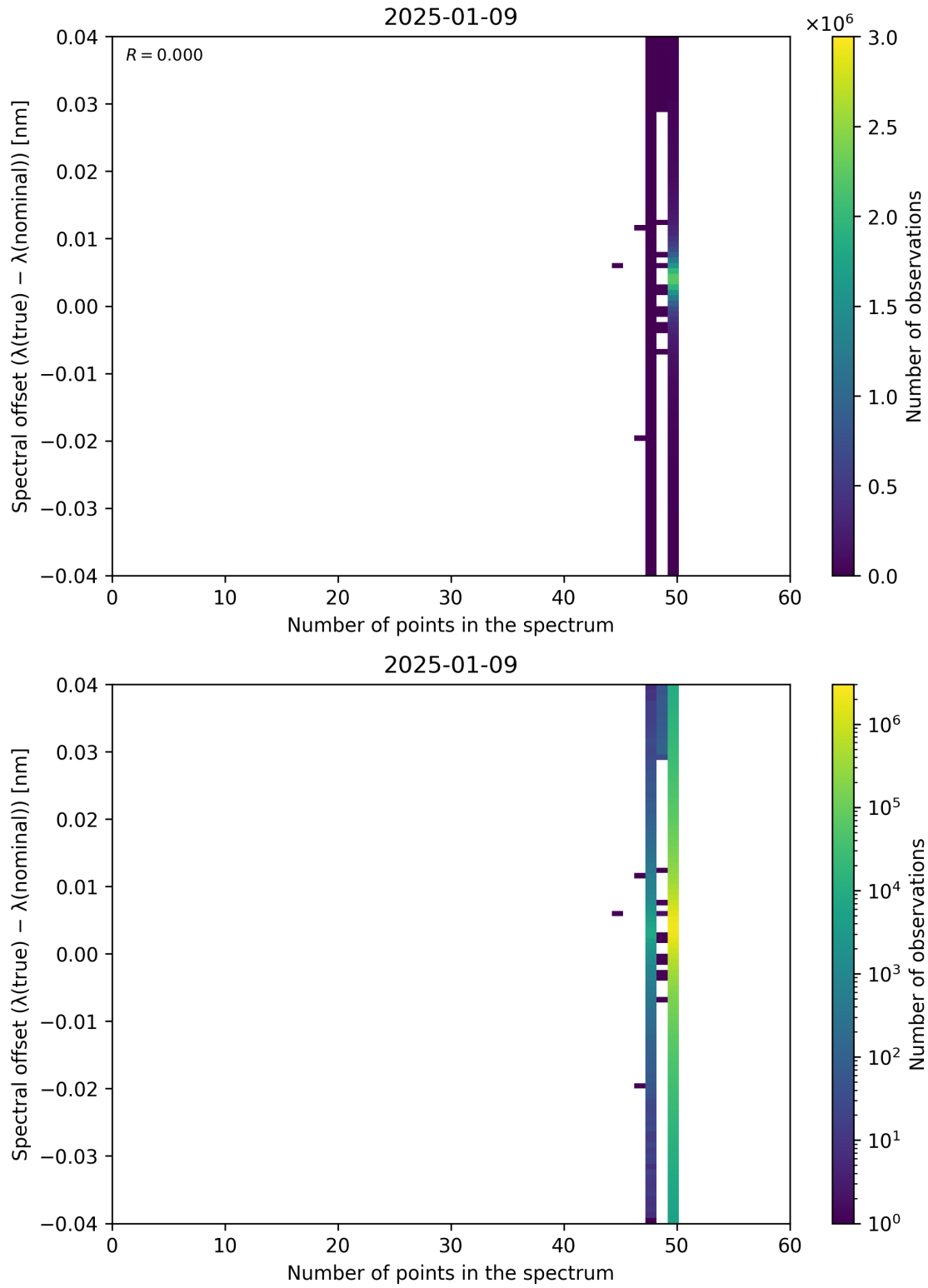
Figure 101: Scatter density plot of “Number of points in the spectrum” against “Spectral offset ( \lambda_{\text{true}} - \lambda_{\text{nominal}} )” for 2025-01-08 to 2025-01-10.
