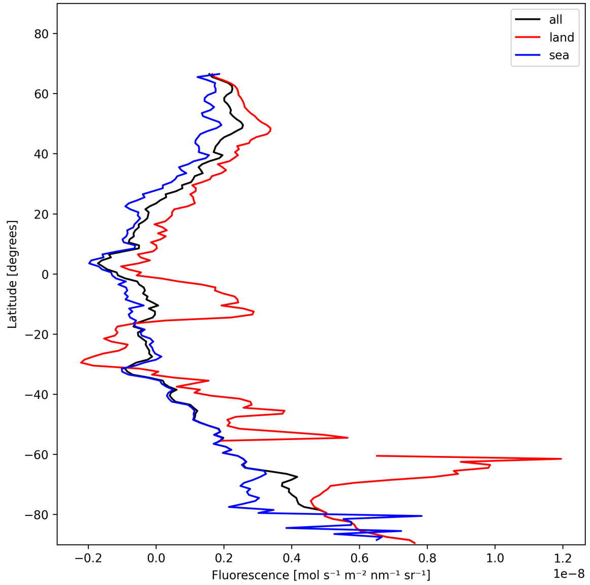
Figure 23: Zonal average of “Fluorescence” for 2025-01-08 to 2025-01-10.
