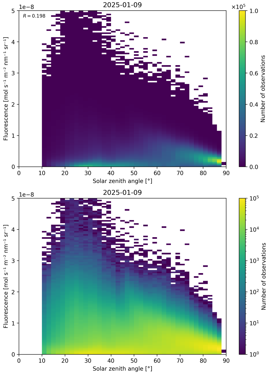
Figure 112: Scatter density plot of “Solar zenith angle” against “Fluorescence” for 2025-01-08 to 2025-01-10.
