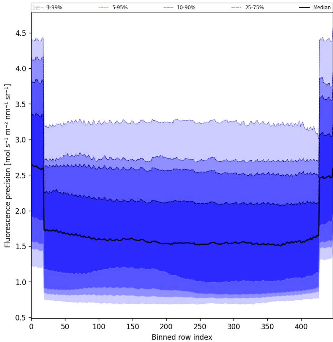
Figure 58: Along track statistics of “Fluorescence precision” for 2025-01-08 to 2025-01-10
