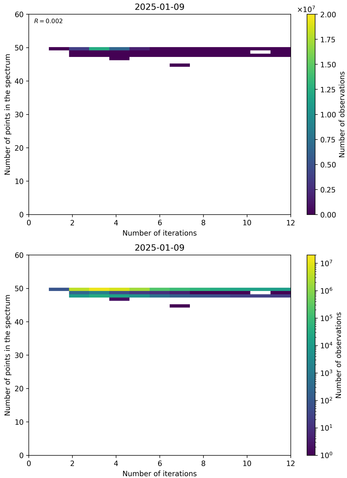
Figure 99: Scatter density plot of “Number of iterations” against “Number of points in the spectrum” for 2025-01-08 to 2025-01-10.
