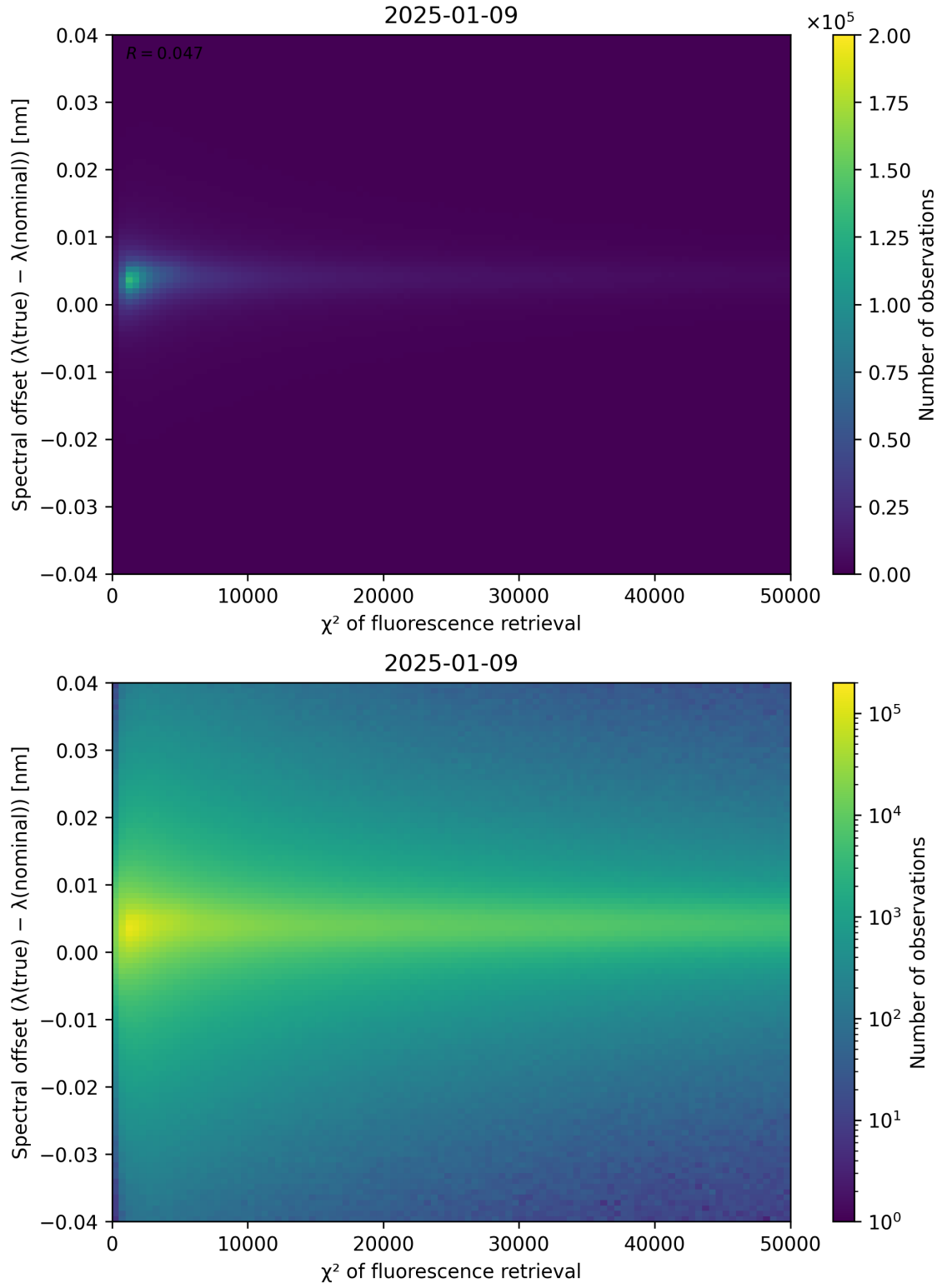
Figure 69: Scatter density plot of “ \chi^2 of fluorescence retrieval” against “Spectral offset ( \lambda_{\text{true}} - \lambda_{\text{nominal}} )” for 2025-01-08 to 2025-01-10.
