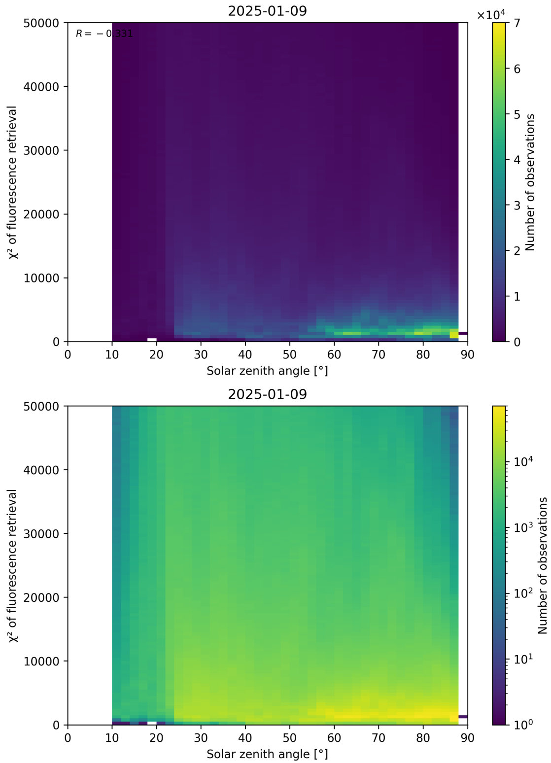
Figure 109: Scatter density plot of “Solar zenith angle” against “ \chi^2 of fluorescence retrieval” for 2025-01-08 to 2025-01-10.
