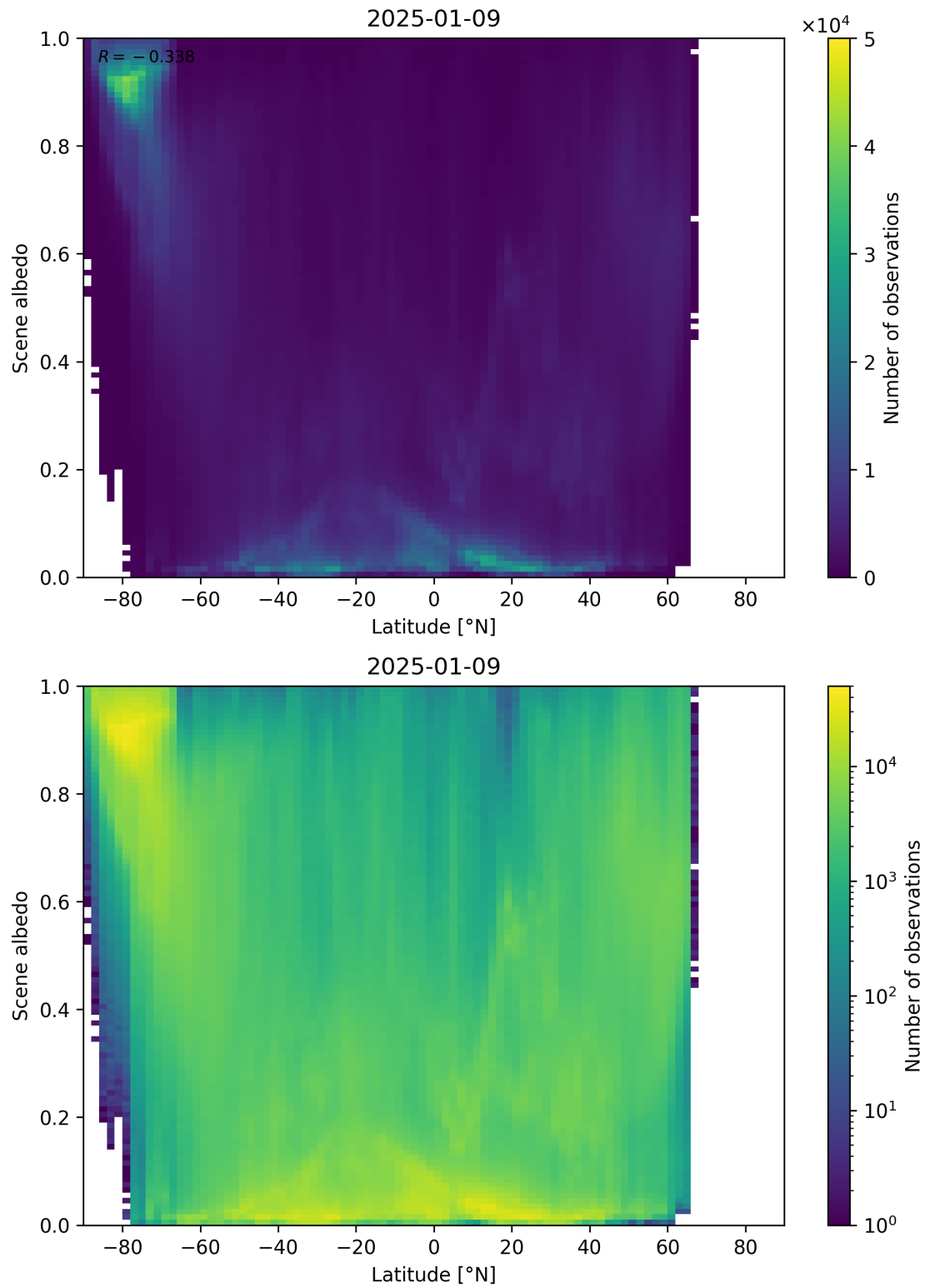
Figure 95: Scatter density plot of “Latitude” against “Scene albedo” for 2025-01-08 to 2025-01-10.
