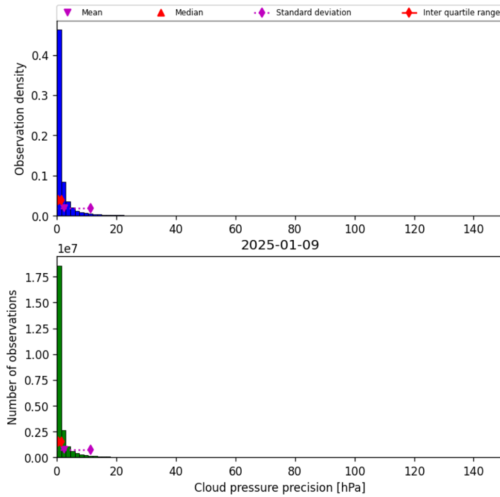
Figure 31: Histogram of “Cloud pressure precision” for 2025-01-08 to 2025-01-10
