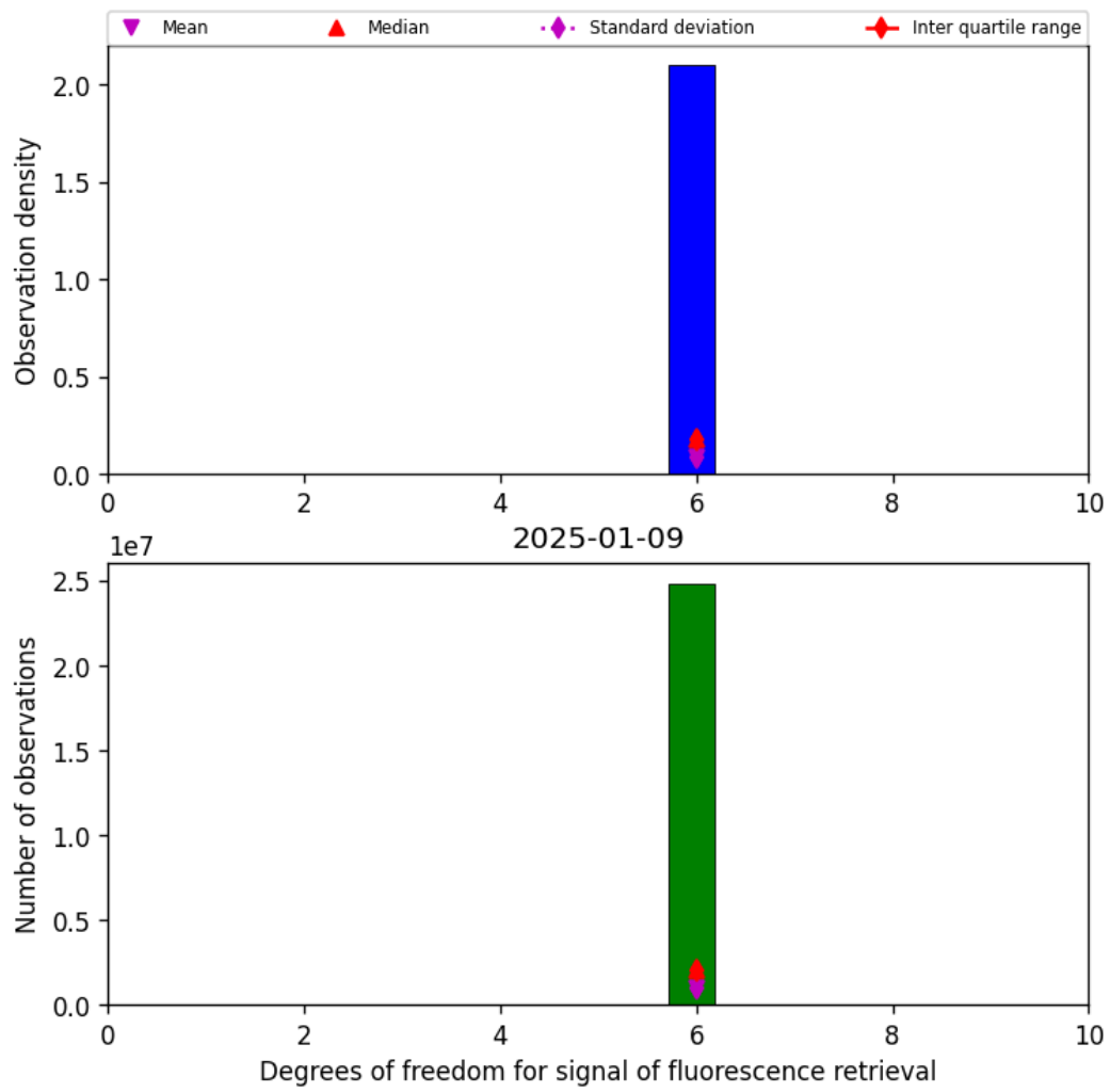
Figure 43: Histogram of “Degrees of freedom for signal of fluorescence retrieval” for 2025-01-08 to 2025-01-10
