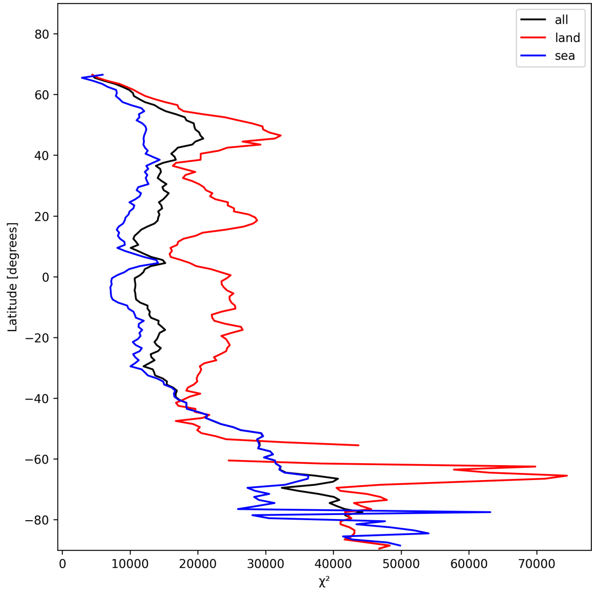
Figure 21: Zonal average of “ \chi^2 ” for 2025-01-08 to 2025-01-10.
