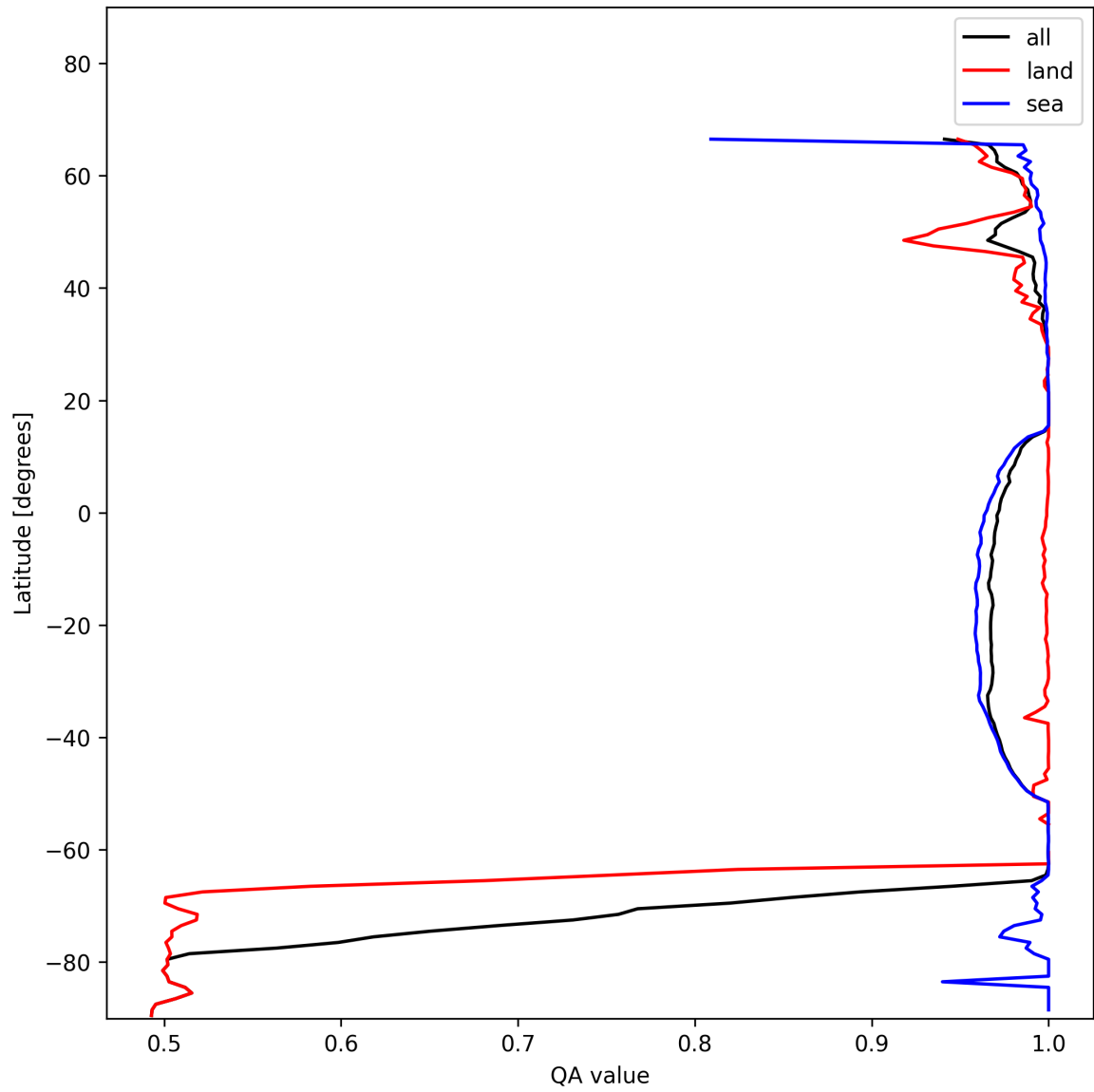
Figure 12: Zonal average of “QA value” for 2025-01-08 to 2025-01-10.
