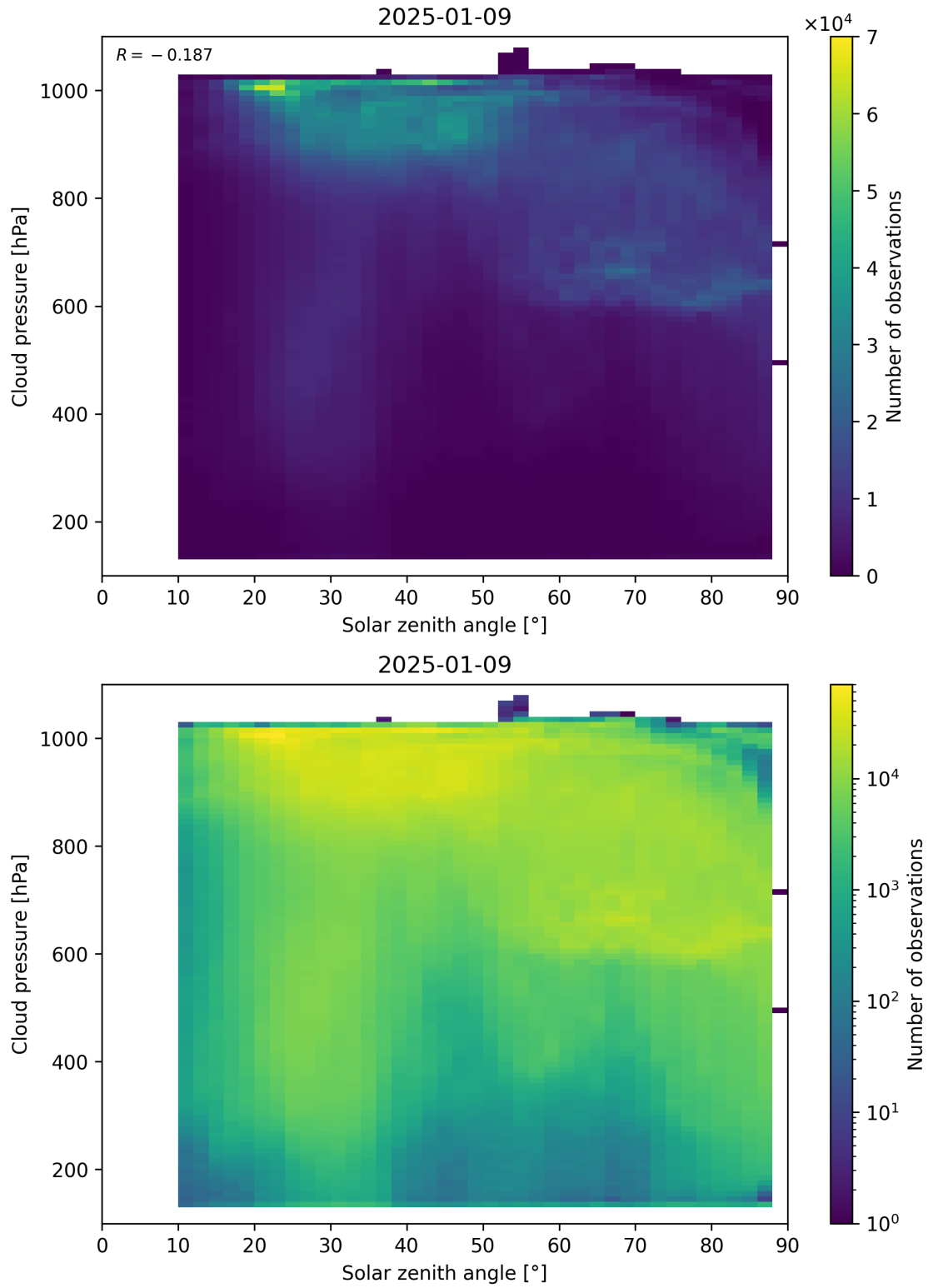
Figure 111: Scatter density plot of “Solar zenith angle” against “Cloud pressure” for 2025-01-08 to 2025-01-10.
