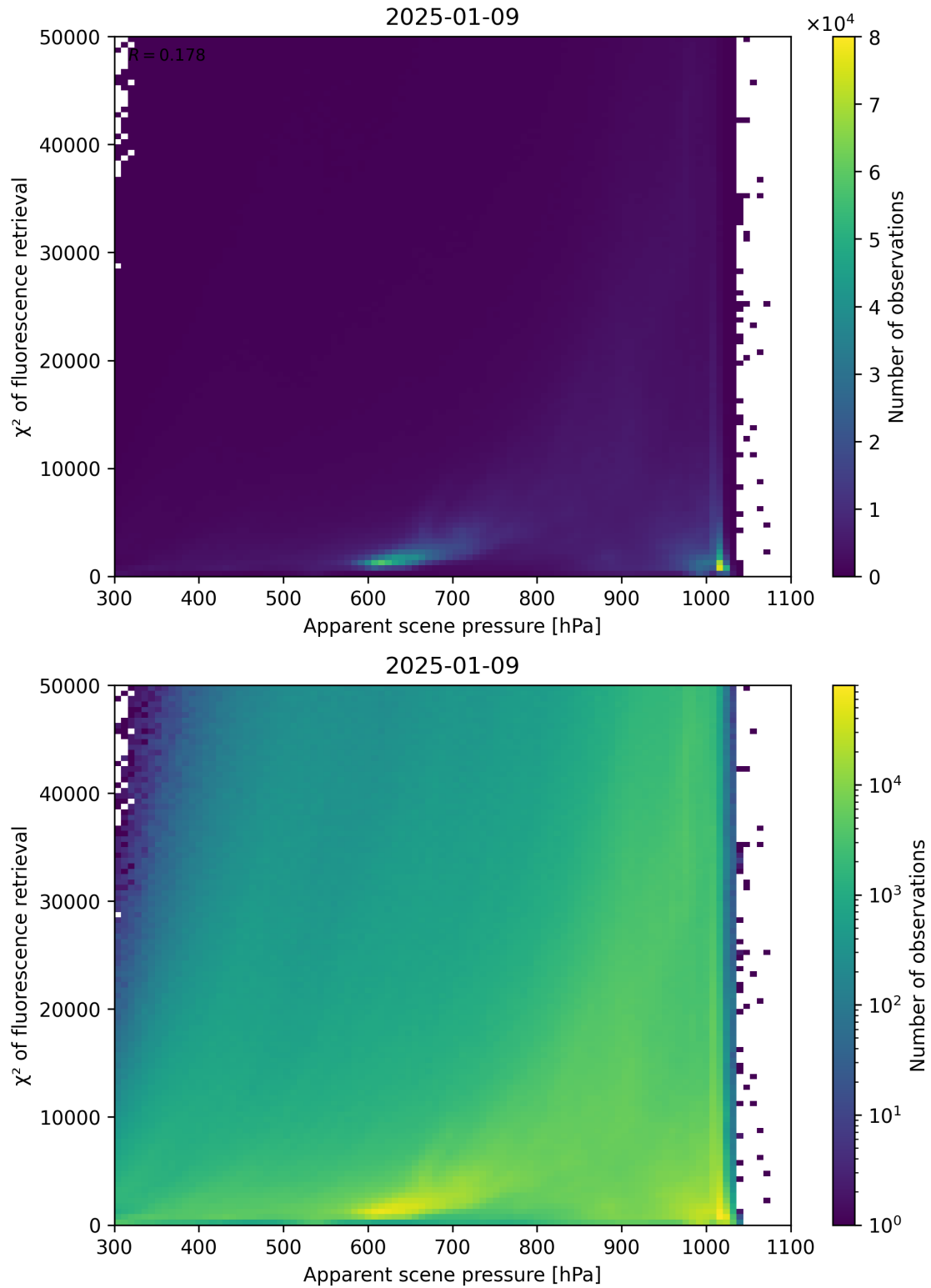
Figure 63: Scatter density plot of “Apparent scene pressure” against “ \chi^2 of fluorescence retrieval” for 2025-01-08 to 2025-01-10.
