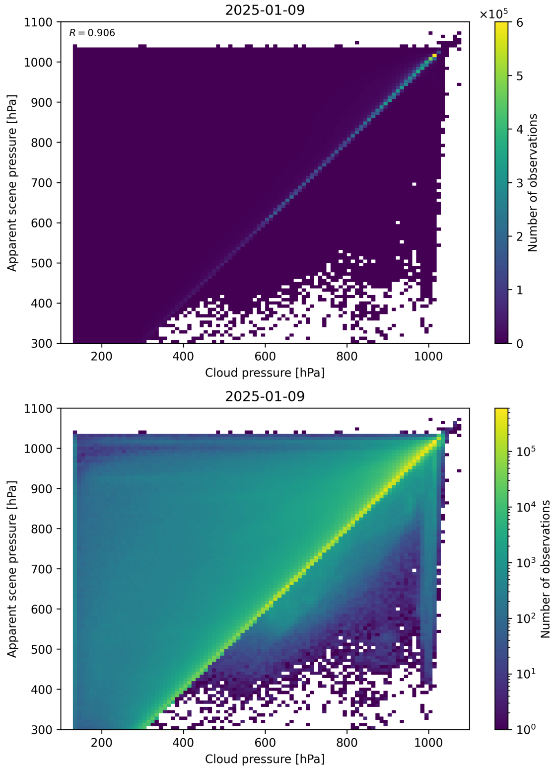
Figure 77: Scatter density plot of “Cloud pressure” against “Apparent scene pressure” for 2025-01-08 to 2025-01-10.
