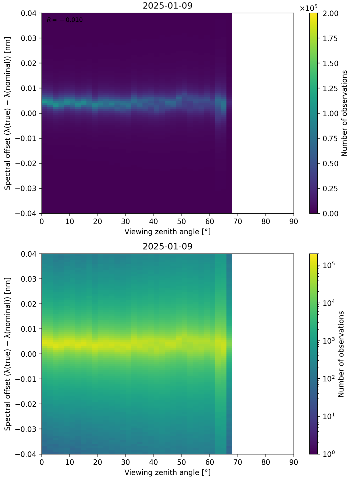
Figure 128: Scatter density plot of “Viewing zenith angle” against “Spectral offset ( \lambda_{\text{true}} - \lambda_{\text{nominal}} )” for 2025-01-08 to 2025-01-10.
