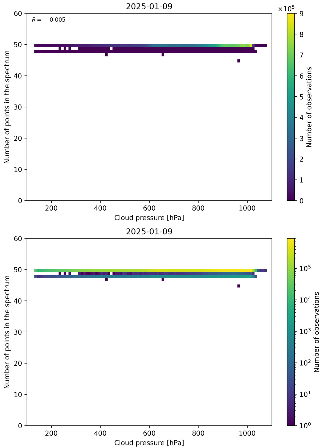
Figure 82: Scatter density plot of “Cloud pressure” against “Number of points in the spectrum” for 2025-01-08 to 2025-01-10.
