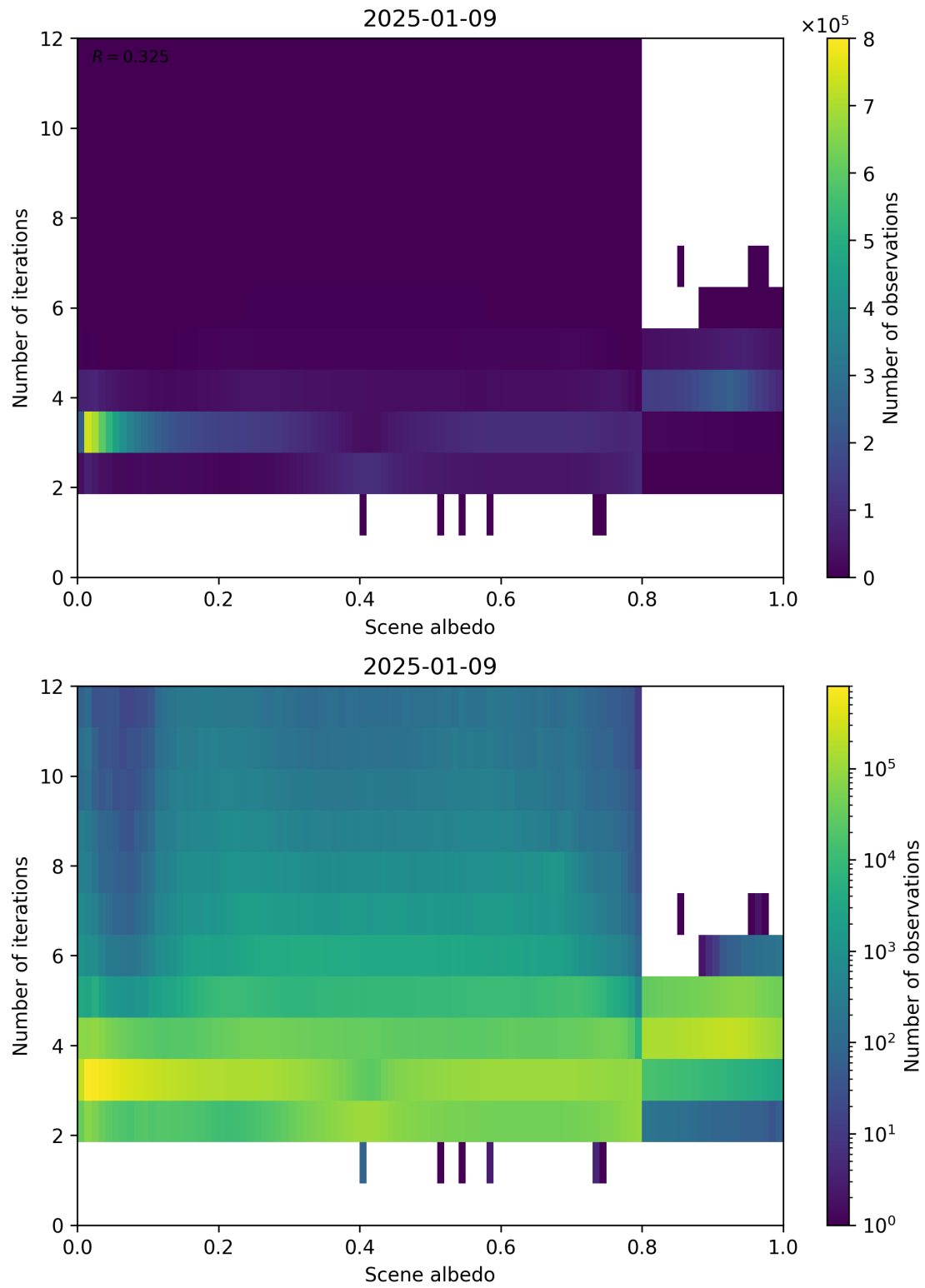
Figure 105: Scatter density plot of “Scene albedo” against “Number of iterations” for 2025-01-08 to 2025-01-10.
