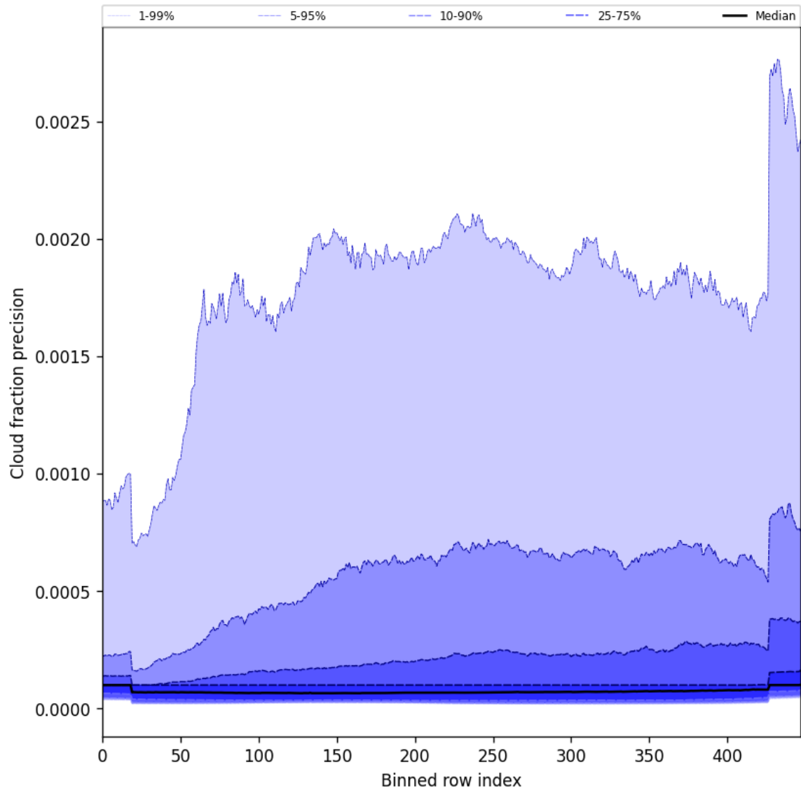
Figure 50: Along track statistics of “Cloud fraction precision” for 2025-01-08 to 2025-01-10
