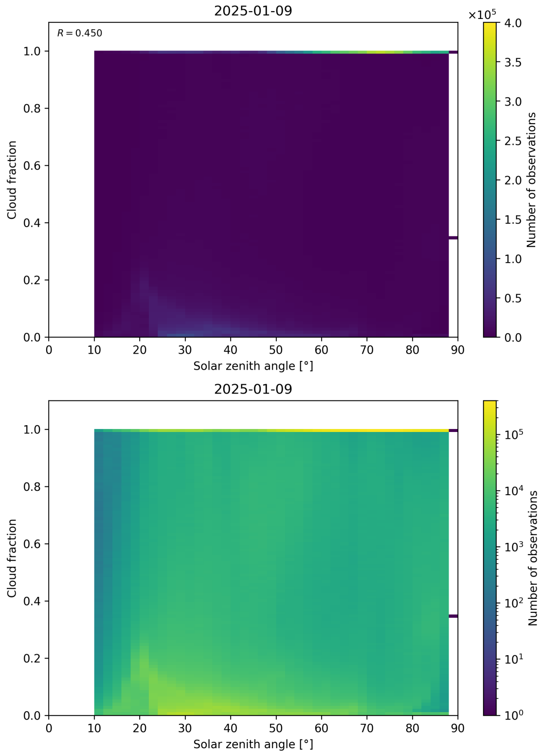
Figure 110: Scatter density plot of “Solar zenith angle” against “Cloud fraction” for 2025-01-08 to 2025-01-10.
