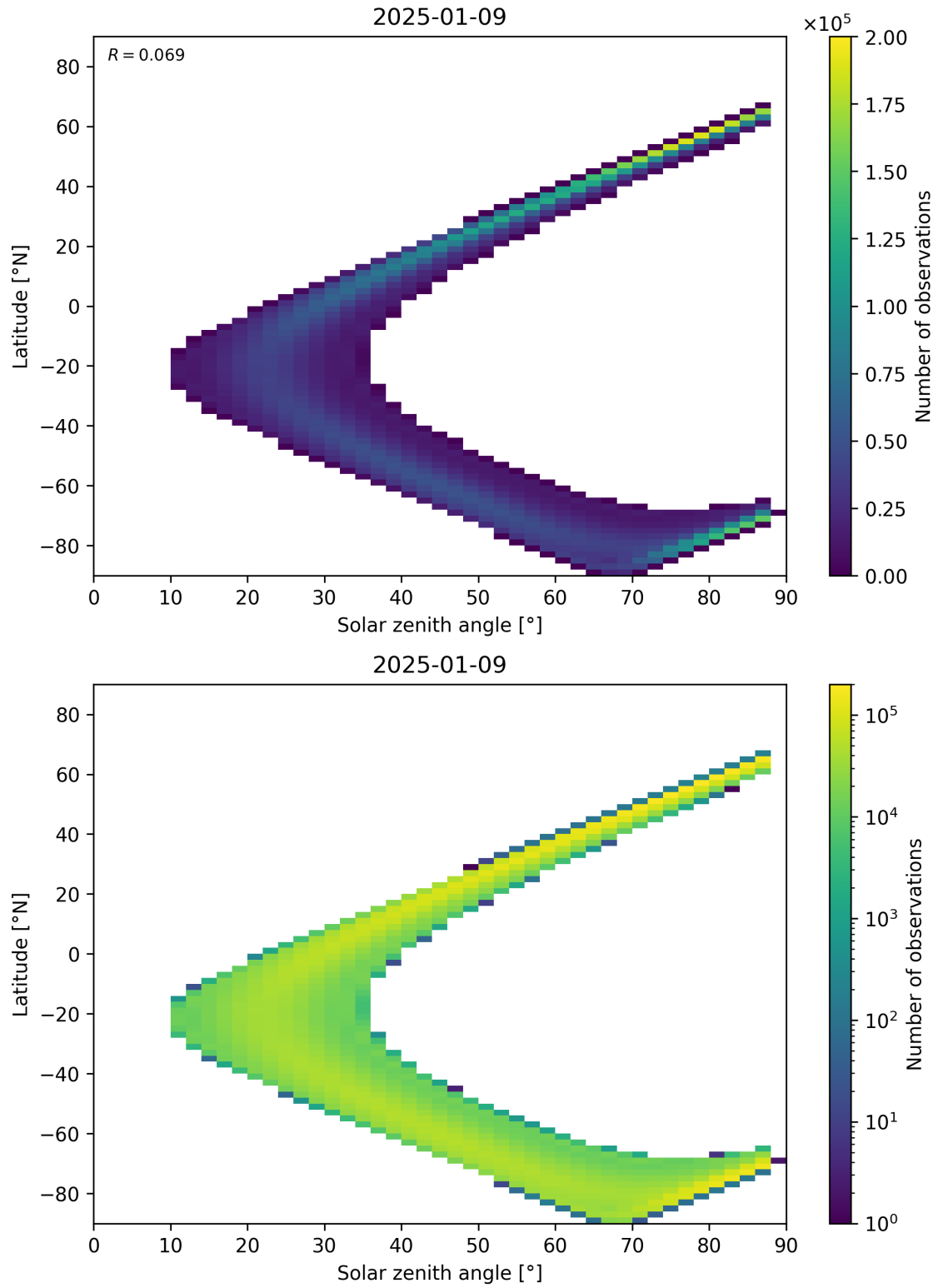
Figure 113: Scatter density plot of “Solar zenith angle” against “Latitude” for 2025-01-08 to 2025-01-10.
