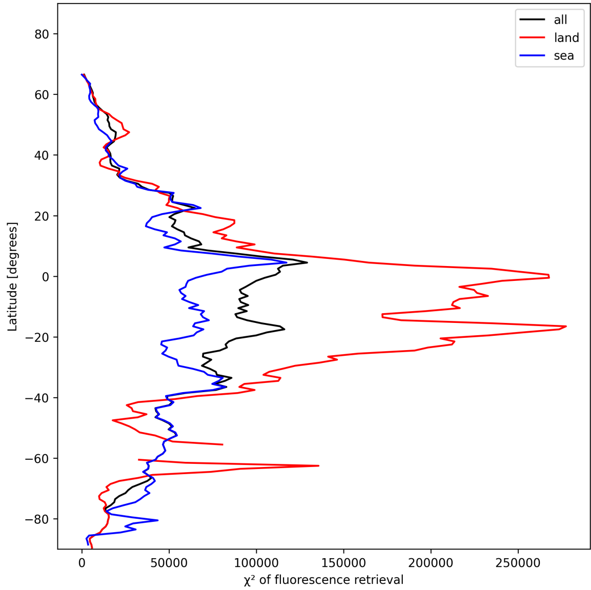
Figure 25: Zonal average of “ \chi^2 of fluorescence retrieval” for 2025-01-08 to 2025-01-10.
