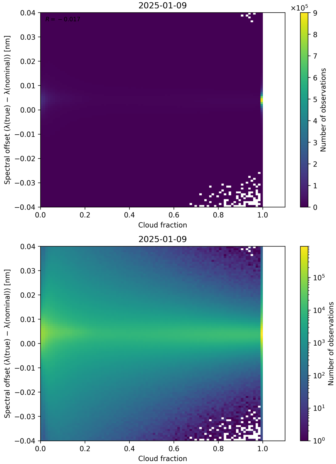
Figure 76: Scatter density plot of “Cloud fraction” against “Spectral offset ( \lambda_{\text{true}} - \lambda_{\text{nominal}} )” for 2025-01-08 to 2025-01-10.
