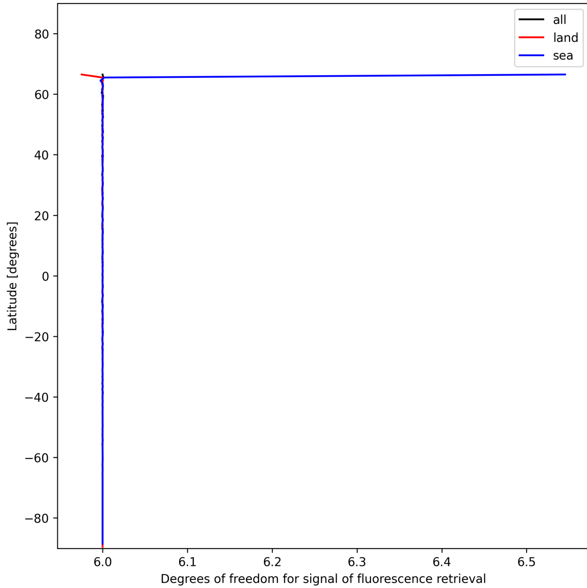
Figure 26: Zonal average of “Degrees of freedom for signal of fluorescence retrieval” for 2025-01-08 to 2025-01-10.
