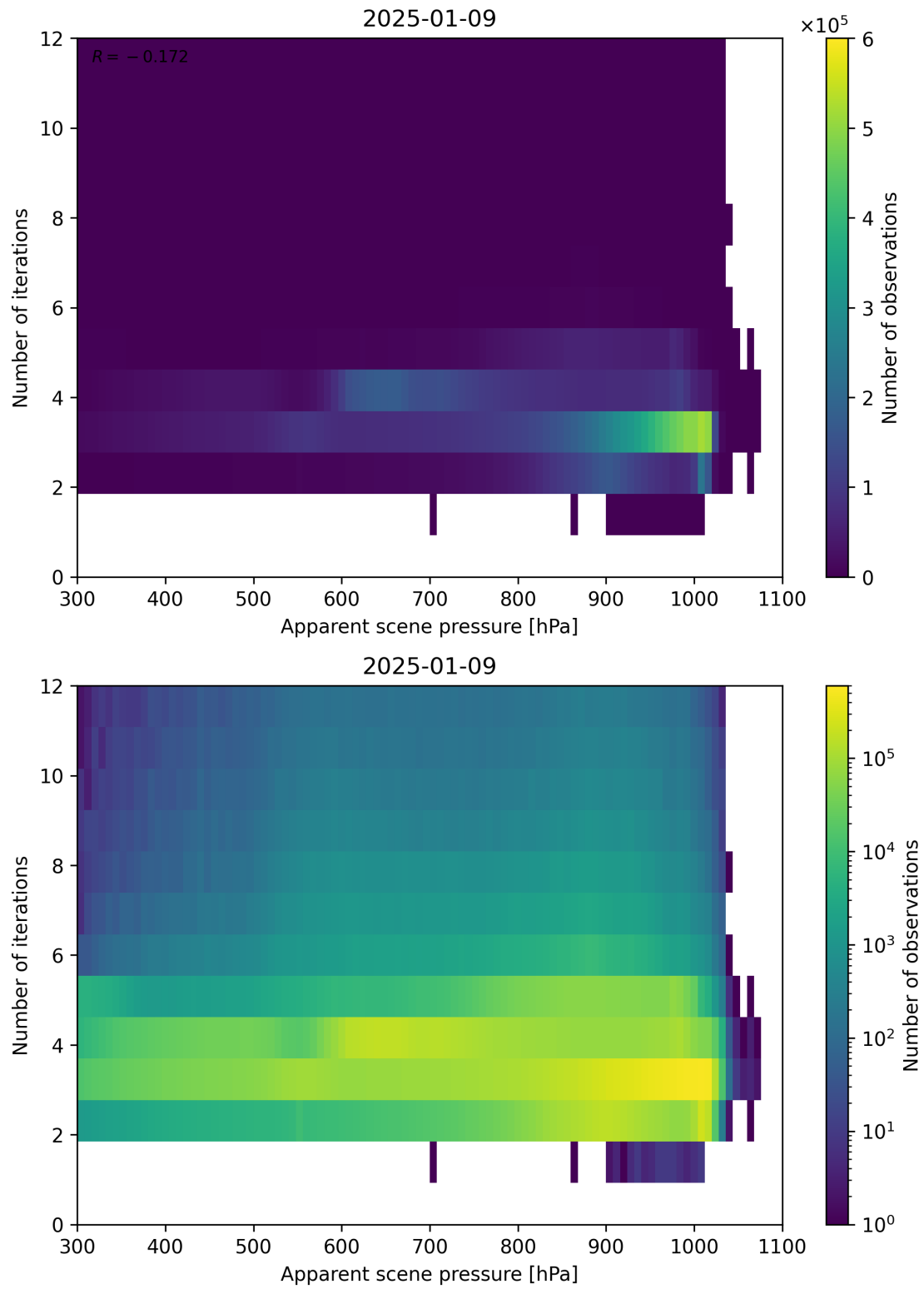
Figure 65: Scatter density plot of “Apparent scene pressure” against “Number of iterations” for 2025-01-08 to 2025-01-10.
