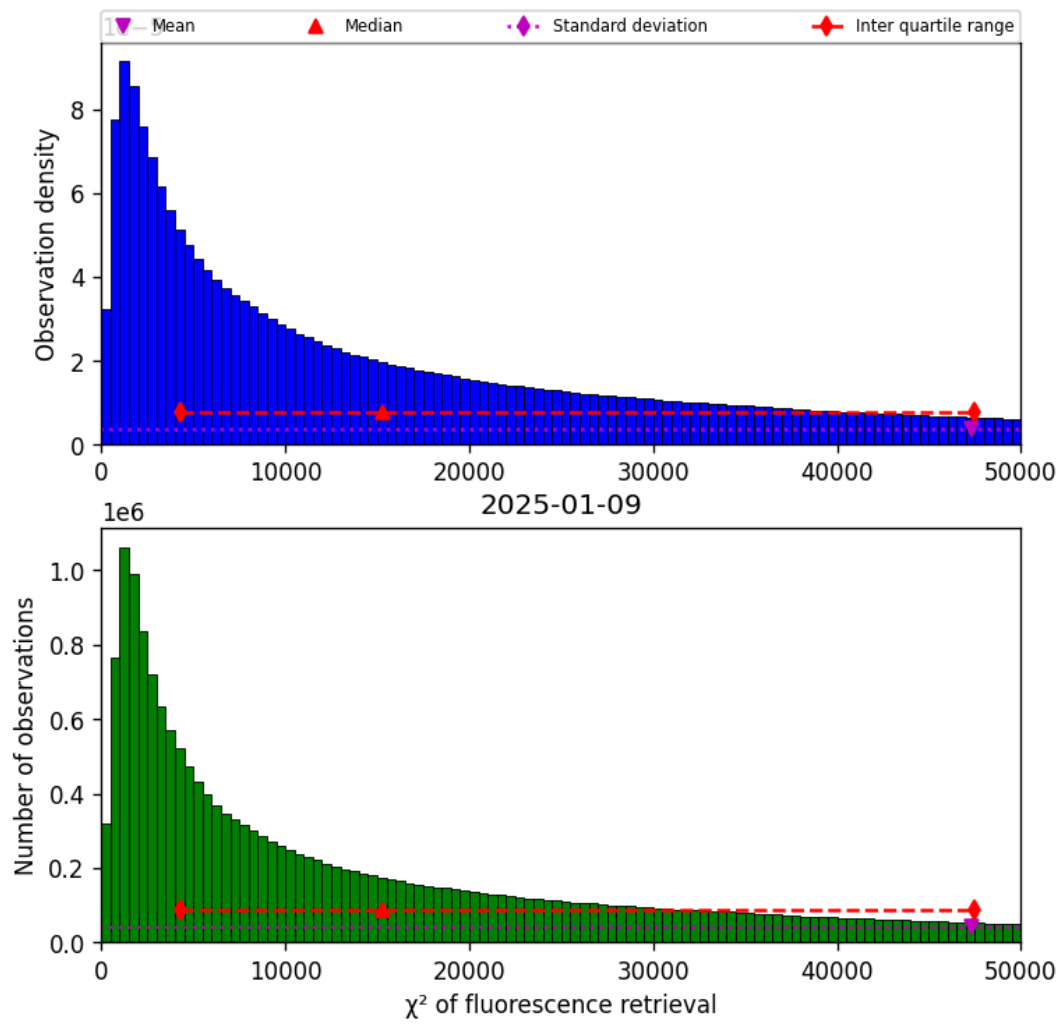
Figure 42: Histogram of “ \chi^2 of fluorescence retrieval” for 2025-01-08 to 2025-01-10
