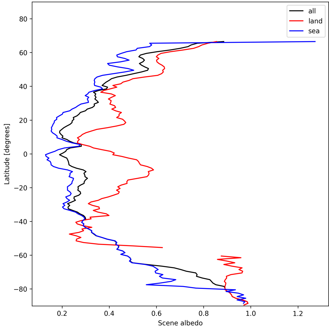
Figure 17: Zonal average of “Scene albedo” for 2025-01-08 to 2025-01-10.
