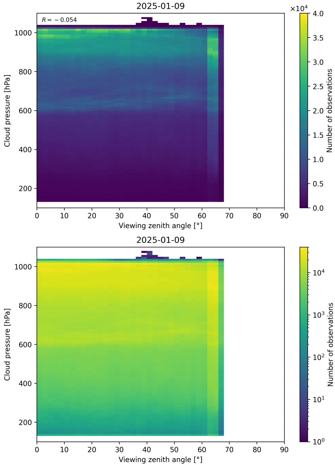
Figure 121: Scatter density plot of “Viewing zenith angle” against “Cloud pressure” for 2025-01-08 to 2025-01-10.
