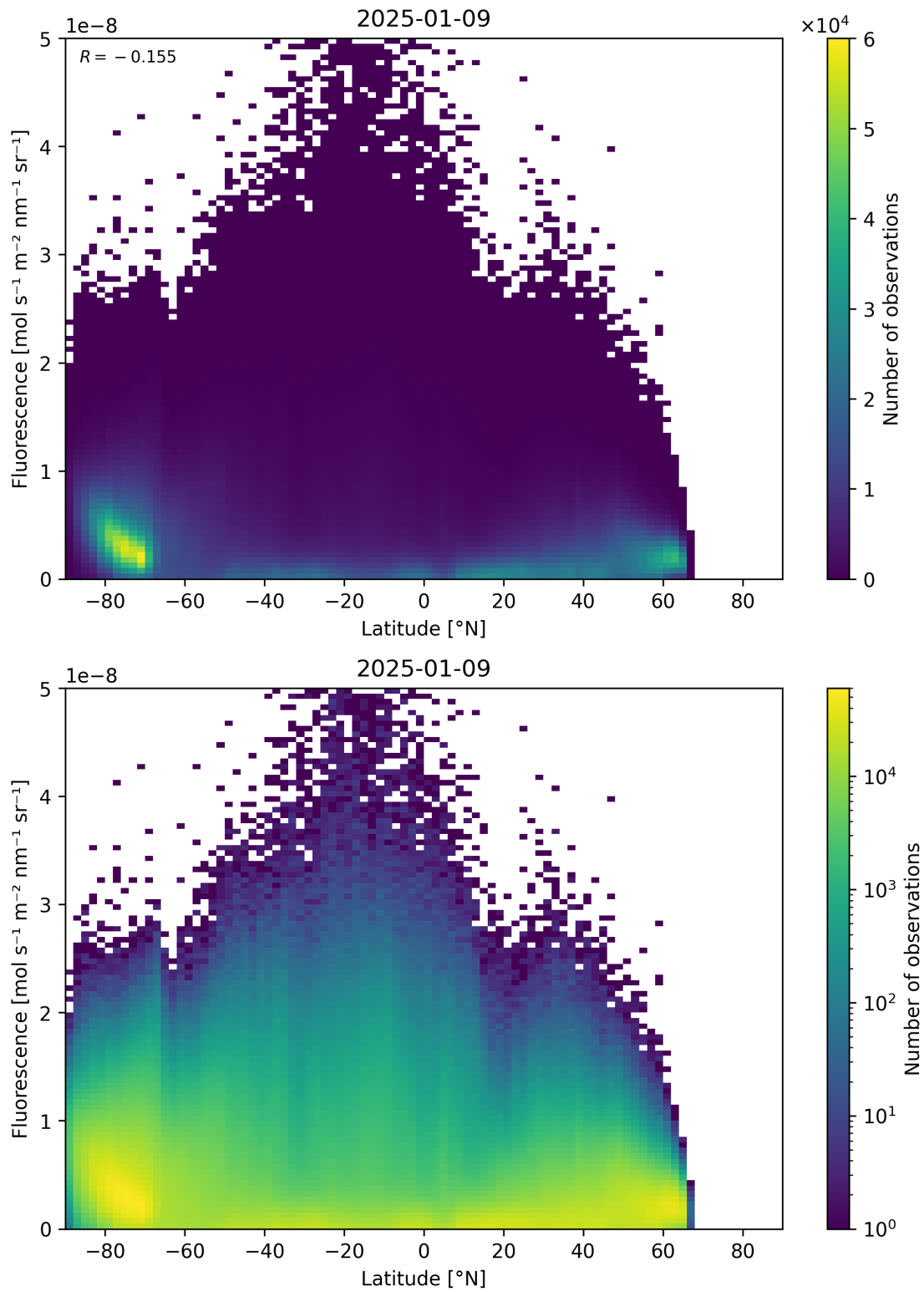
Figure 92: Scatter density plot of “Latitude” against “Fluorescence” for 2025-01-08 to 2025-01-10.
