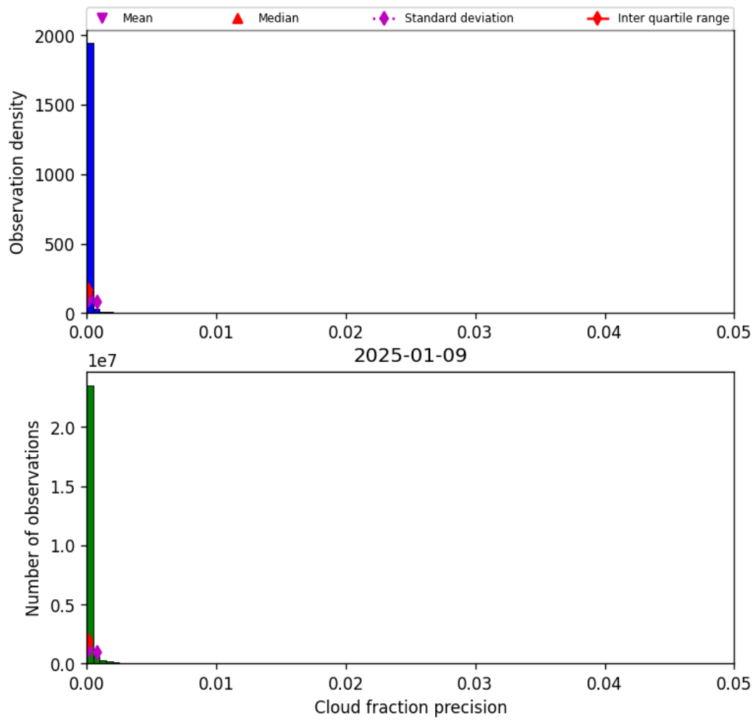
Figure 33: Histogram of “Cloud fraction precision” for 2025-01-08 to 2025-01-10
