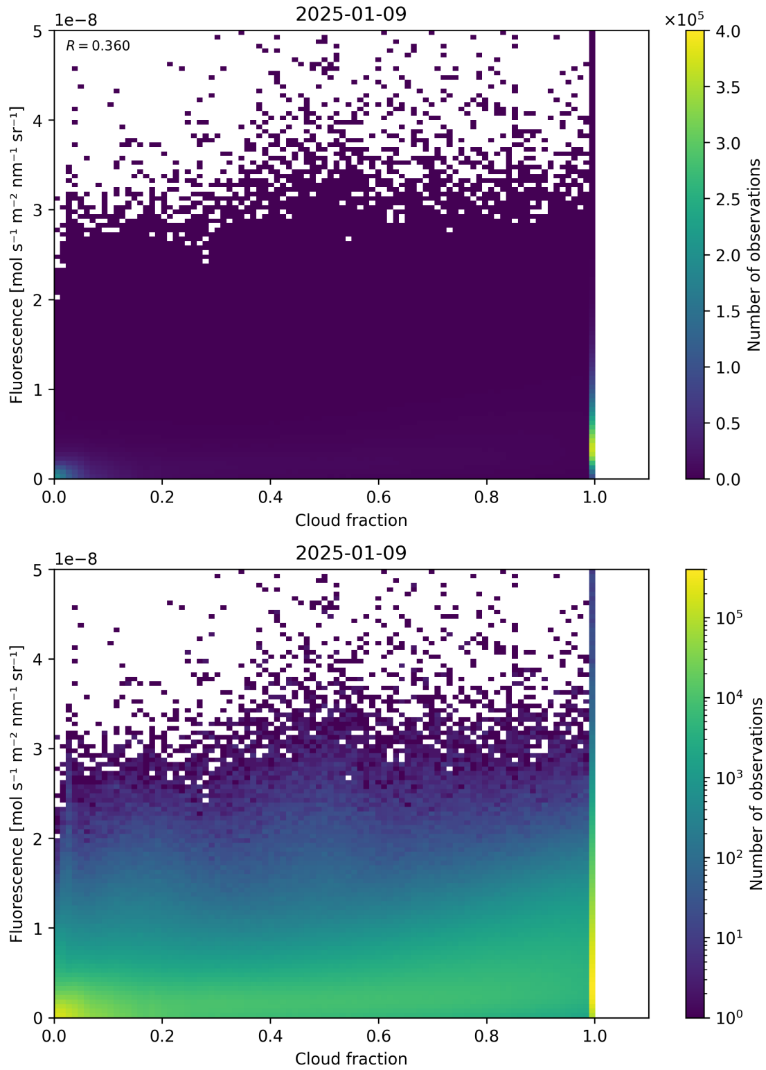
Figure 72: Scatter density plot of “Cloud fraction” against “Fluorescence” for 2025-01-08 to 2025-01-10.
