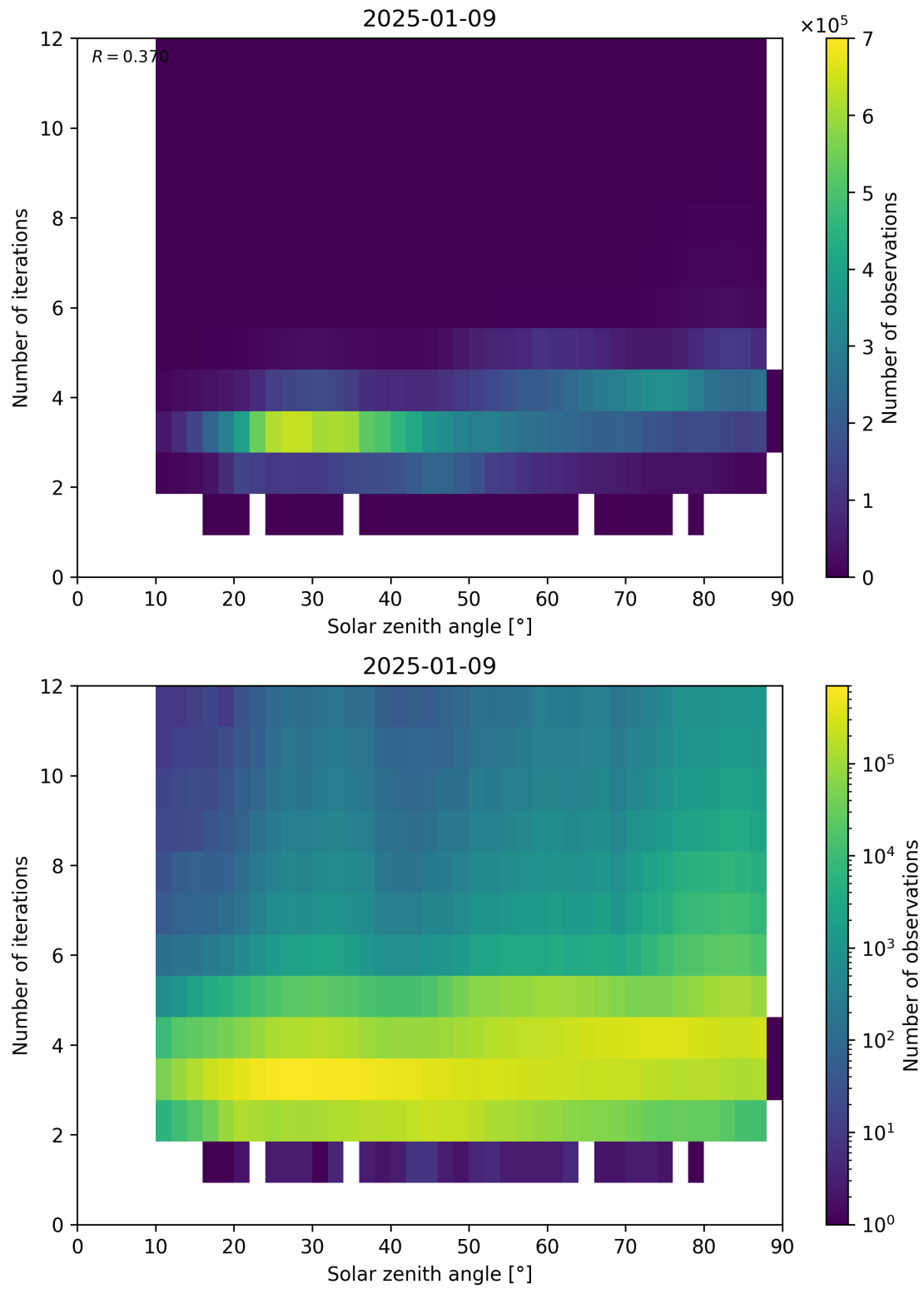
Figure 114: Scatter density plot of “Solar zenith angle” against “Number of iterations” for 2025-01-08 to 2025-01-10.
