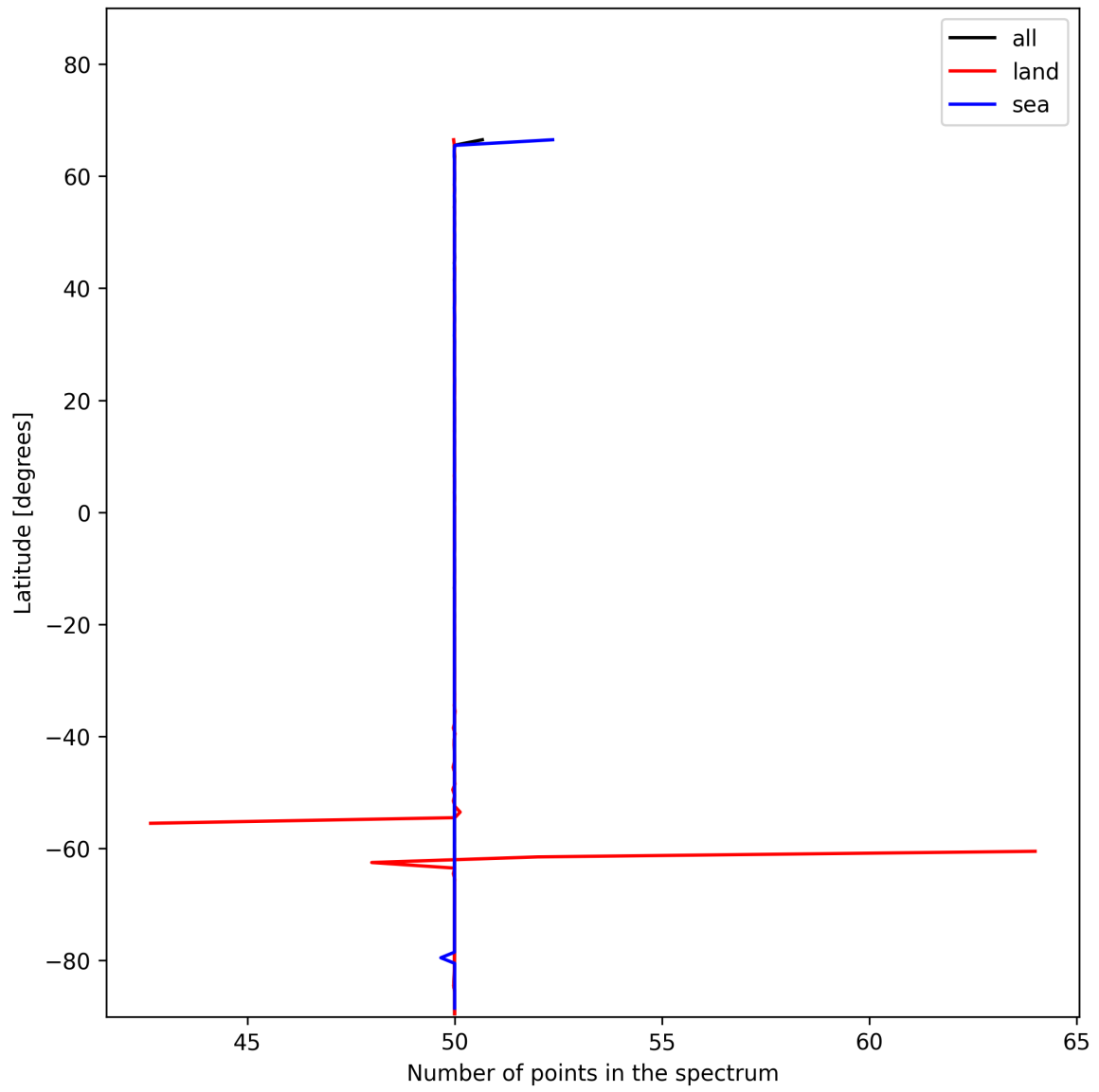
Figure 27: Zonal average of “Number of points in the spectrum” for 2025-01-08 to 2025-01-10.
