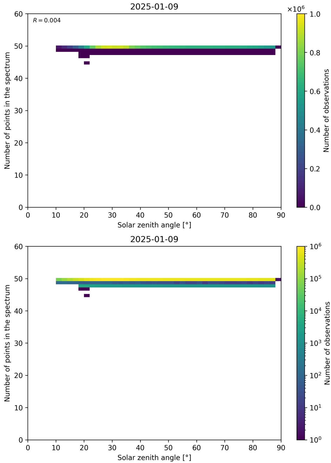
Figure 115: Scatter density plot of “Solar zenith angle” against “Number of points in the spectrum” for 2025-01-08 to 2025-01-10.
