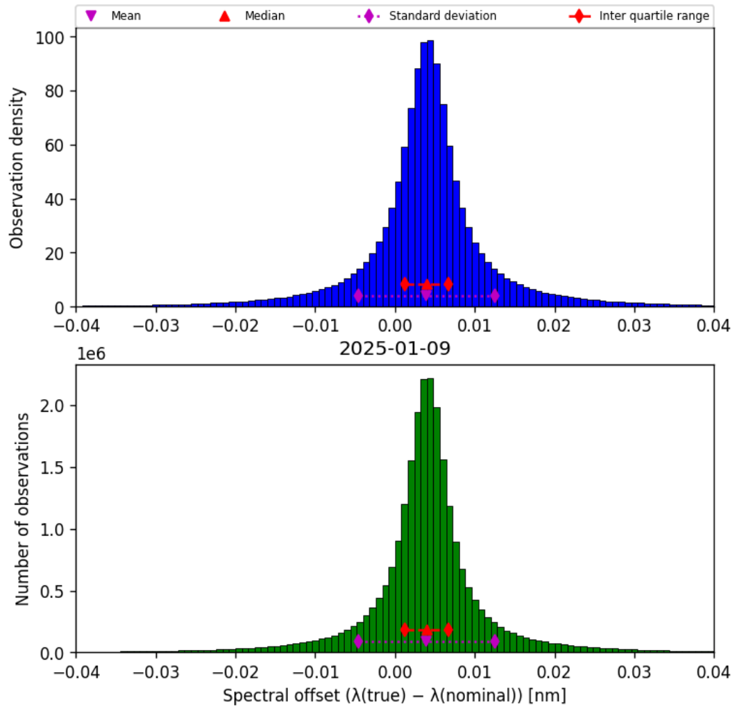
Figure 45: Histogram of “Spectral offset ( \lambda_{\text{true}} - \lambda_{\text{nominal}} )” for 2025-01-08 to 2025-01-10
