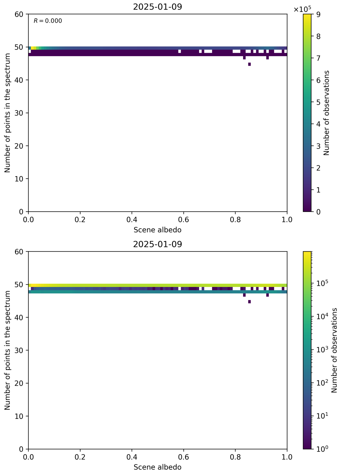
Figure 106: Scatter density plot of “Scene albedo” against “Number of points in the spectrum” for 2025-01-08 to 2025-01-10.
