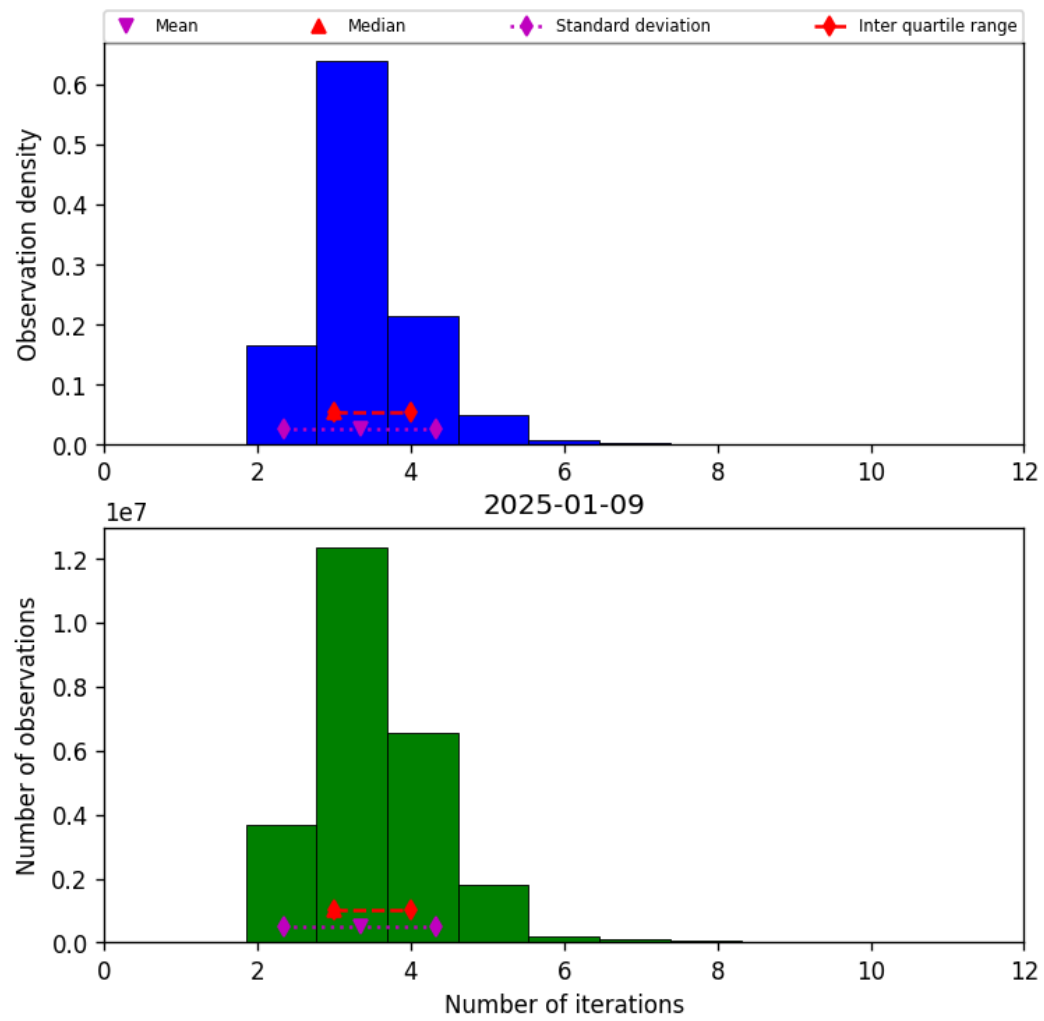
Figure 39: Histogram of “Number of iterations” for 2025-01-08 to 2025-01-10
