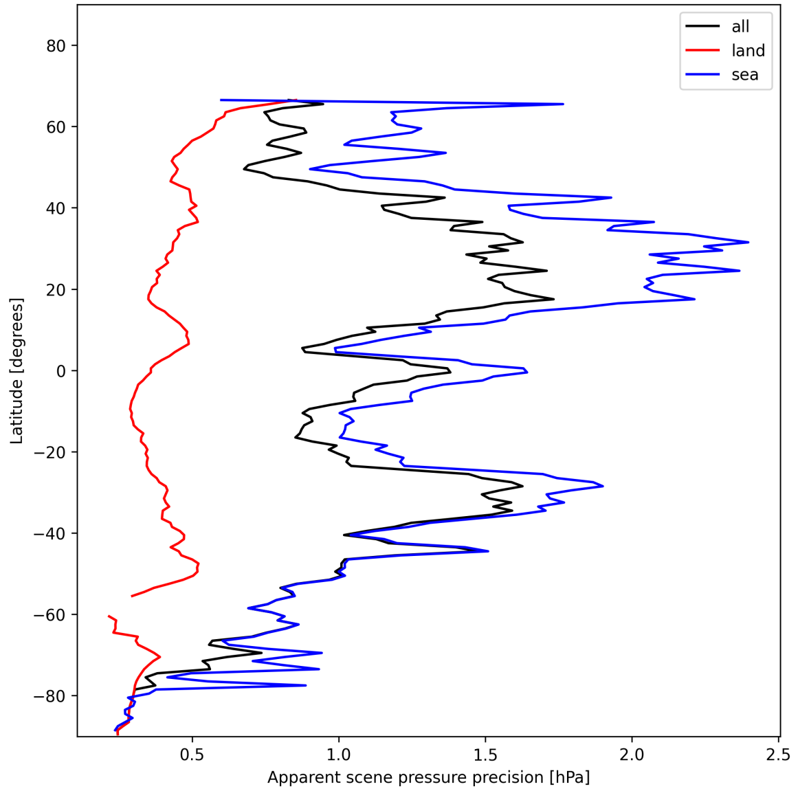
Figure 20: Zonal average of “Apparent scene pressure precision” for 2025-01-08 to 2025-01-10.
