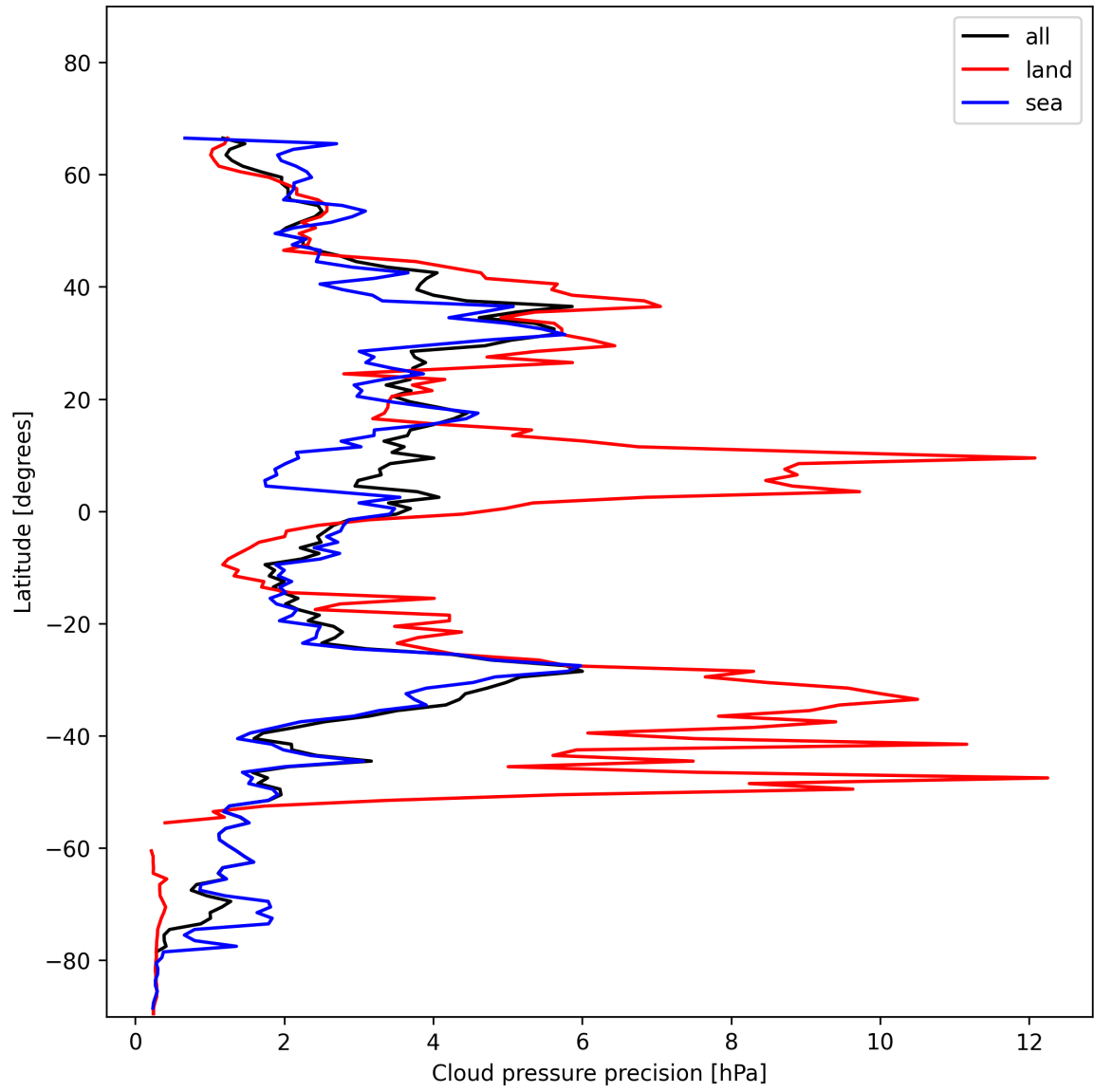
Figure 14: Zonal average of “Cloud pressure precision” for 2025-01-08 to 2025-01-10.
