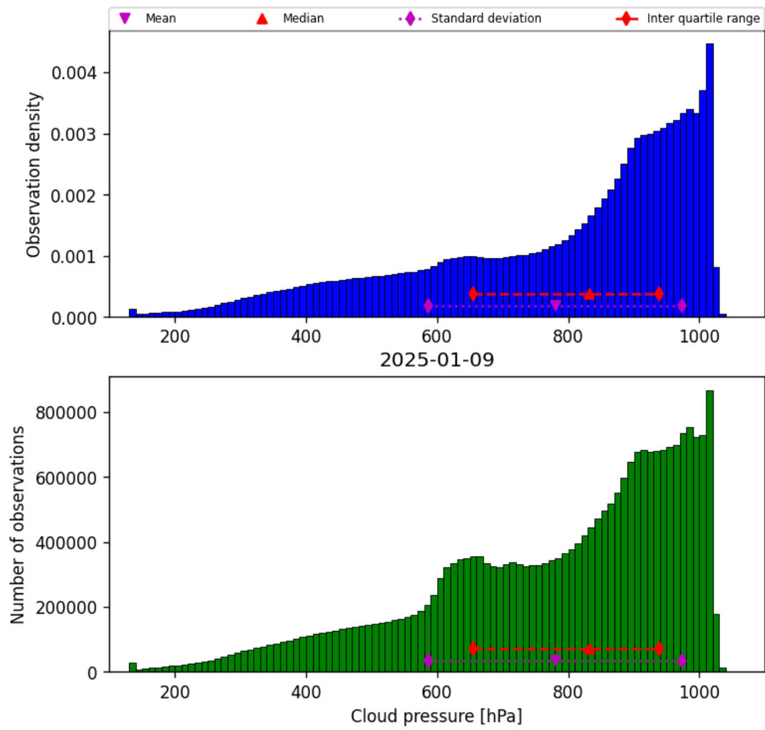
Figure 30: Histogram of “Cloud pressure” for 2025-01-08 to 2025-01-10
