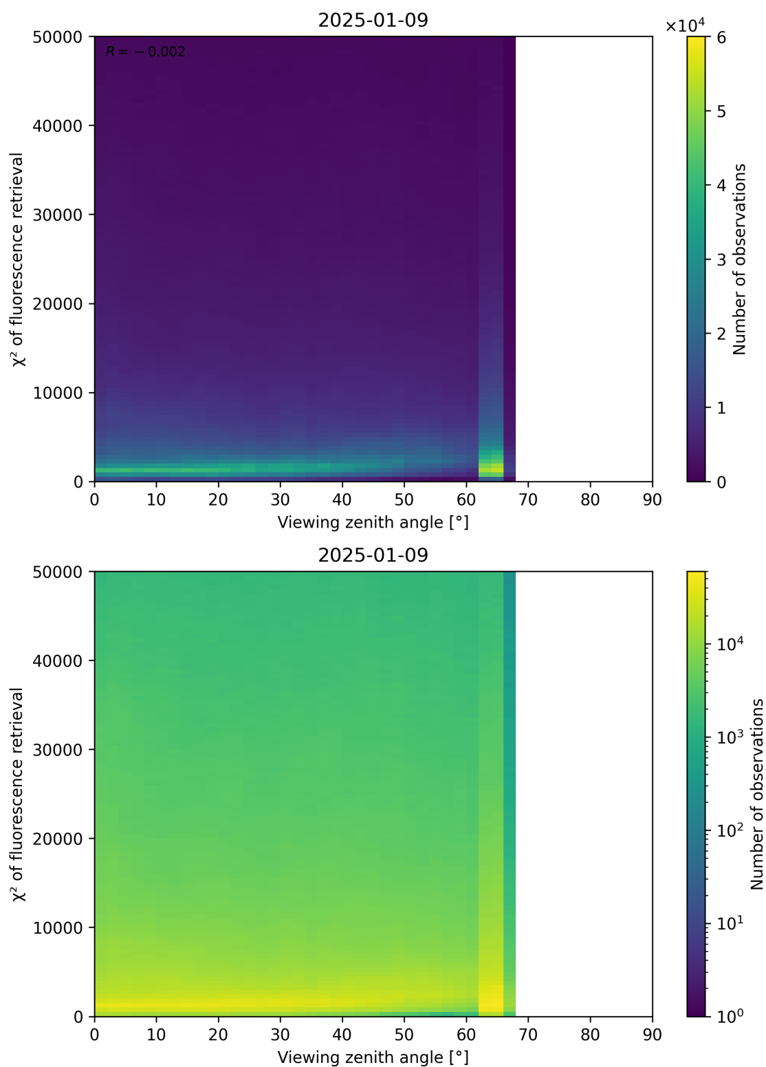
Figure 119: Scatter density plot of “Viewing zenith angle” against “ \chi^2 of fluorescence retrieval” for 2025-01-08 to 2025-01-10.
