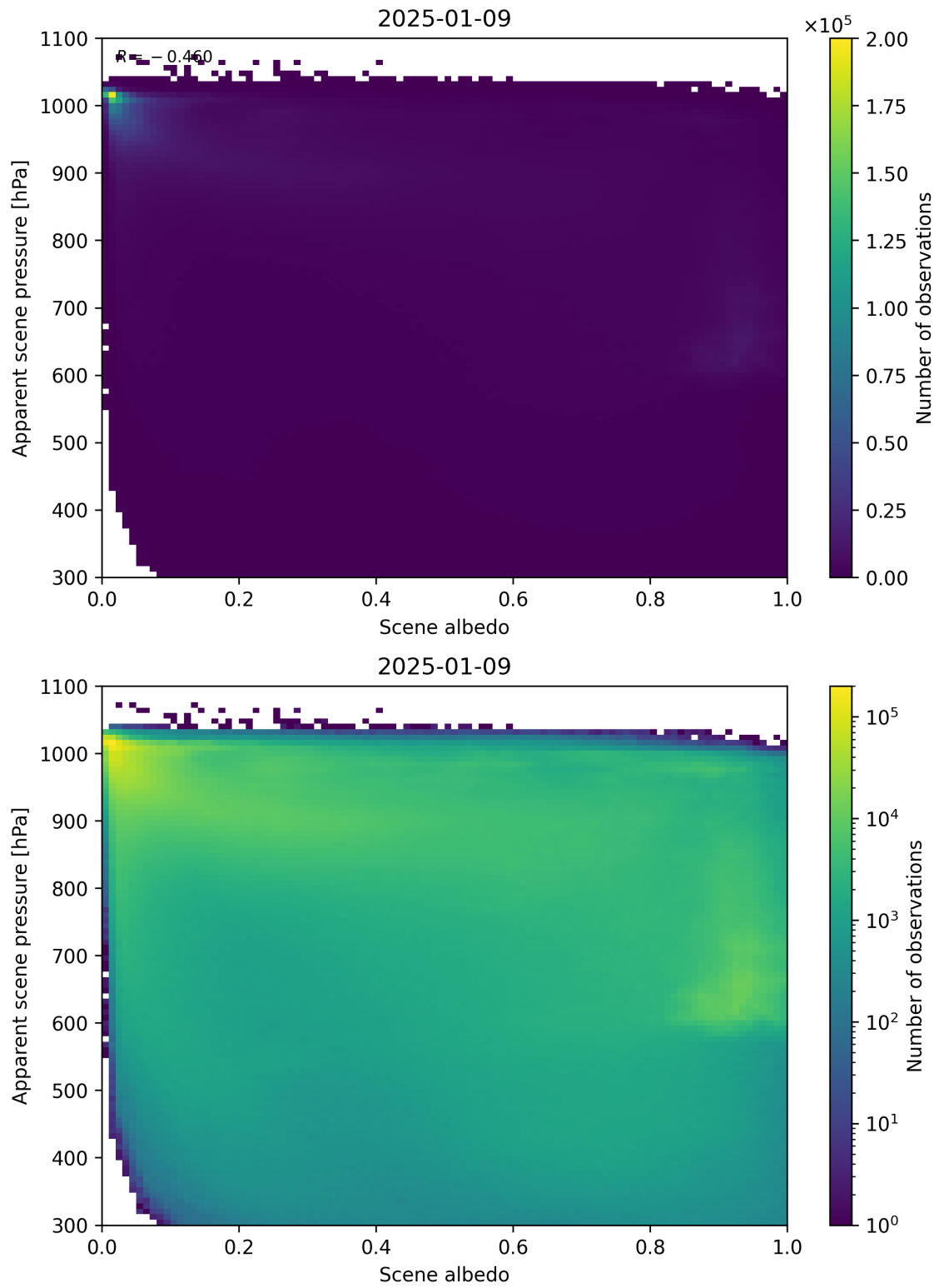
Figure 102: Scatter density plot of “Scene albedo” against “Apparent scene pressure” for 2025-01-08 to 2025-01-10.
