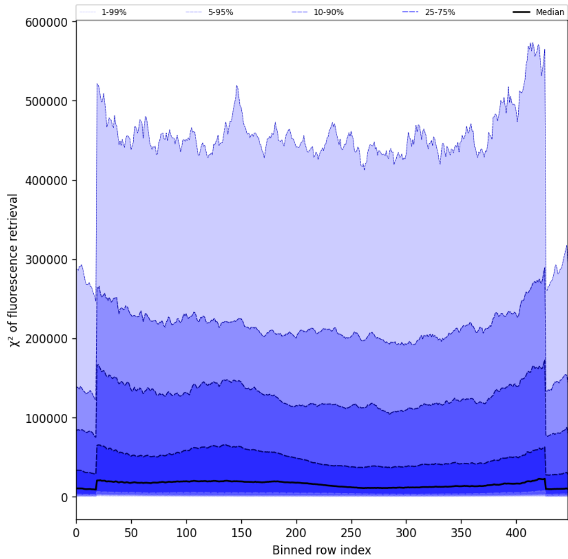
Figure 59: Along track statistics of “ \chi^2 of fluorescence retrieval” for 2025-01-08 to 2025-01-10
