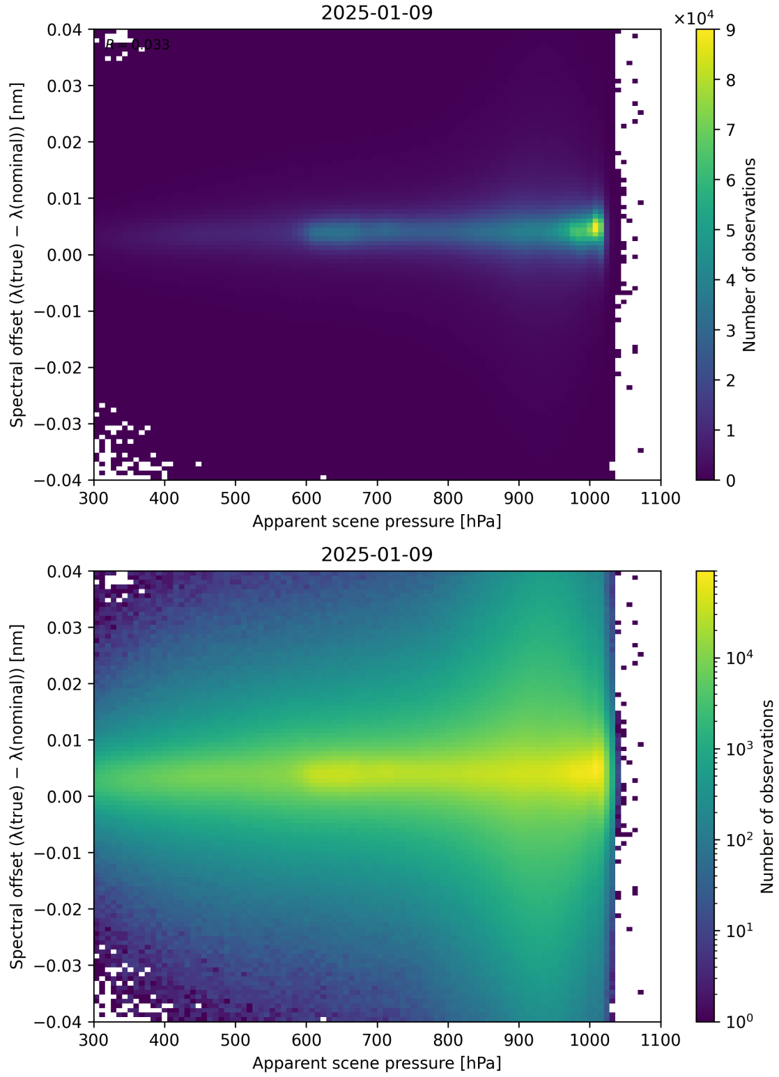
Figure 67: Scatter density plot of “Apparent scene pressure” against “Spectral offset ( \lambda_{\text{true}} - \lambda_{\text{nominal}} )” for 2025-01-08 to 2025-01-10.
