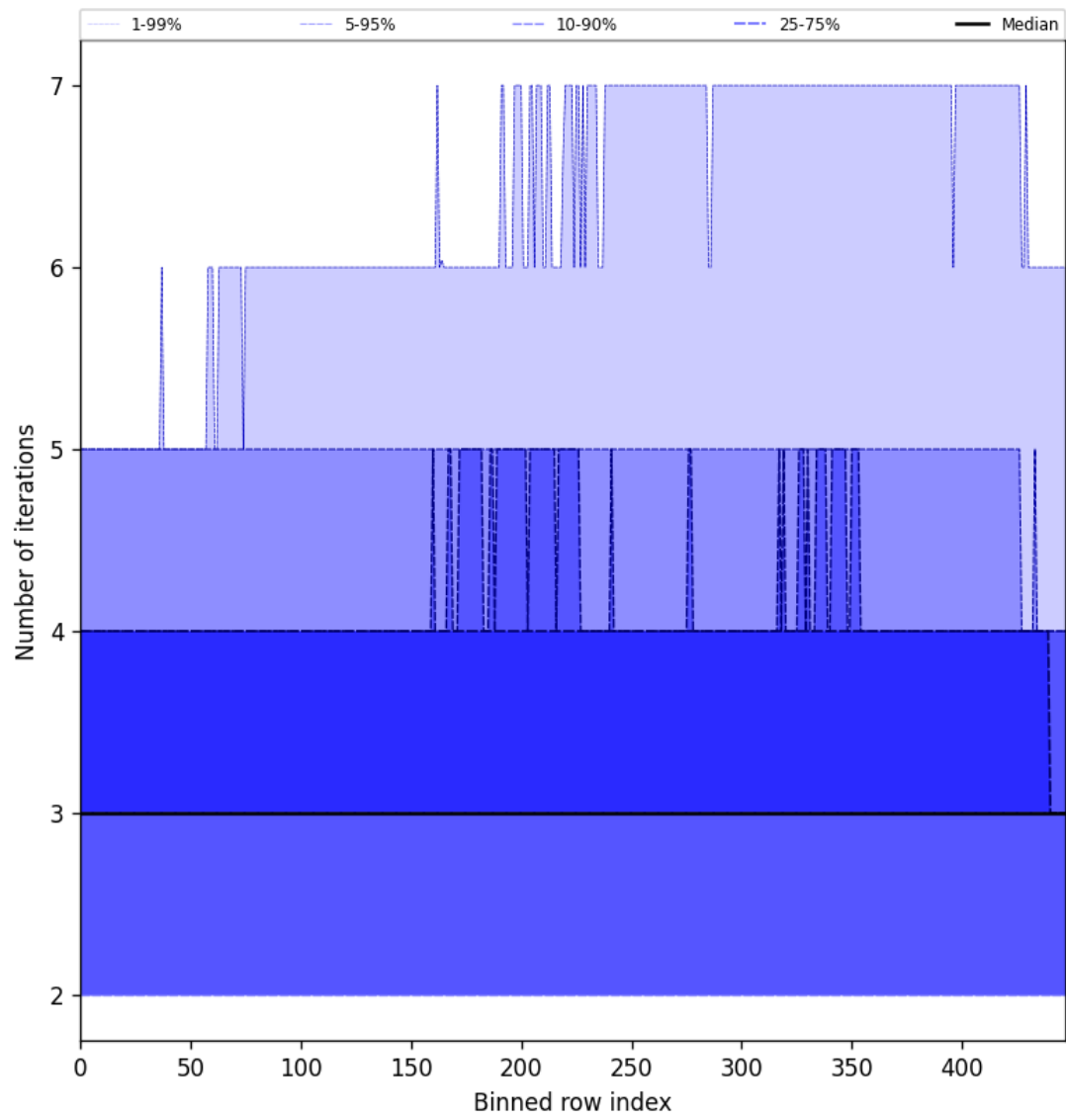
Figure 56: Along track statistics of “Number of iterations” for 2025-01-08 to 2025-01-10
