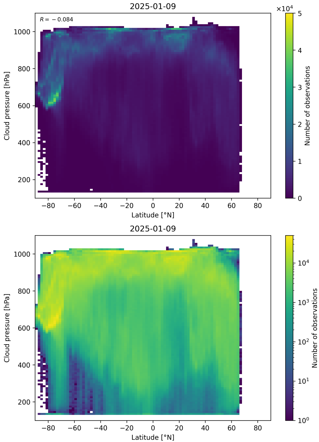
Figure 91: Scatter density plot of “Latitude” against “Cloud pressure” for 2025-01-08 to 2025-01-10.
