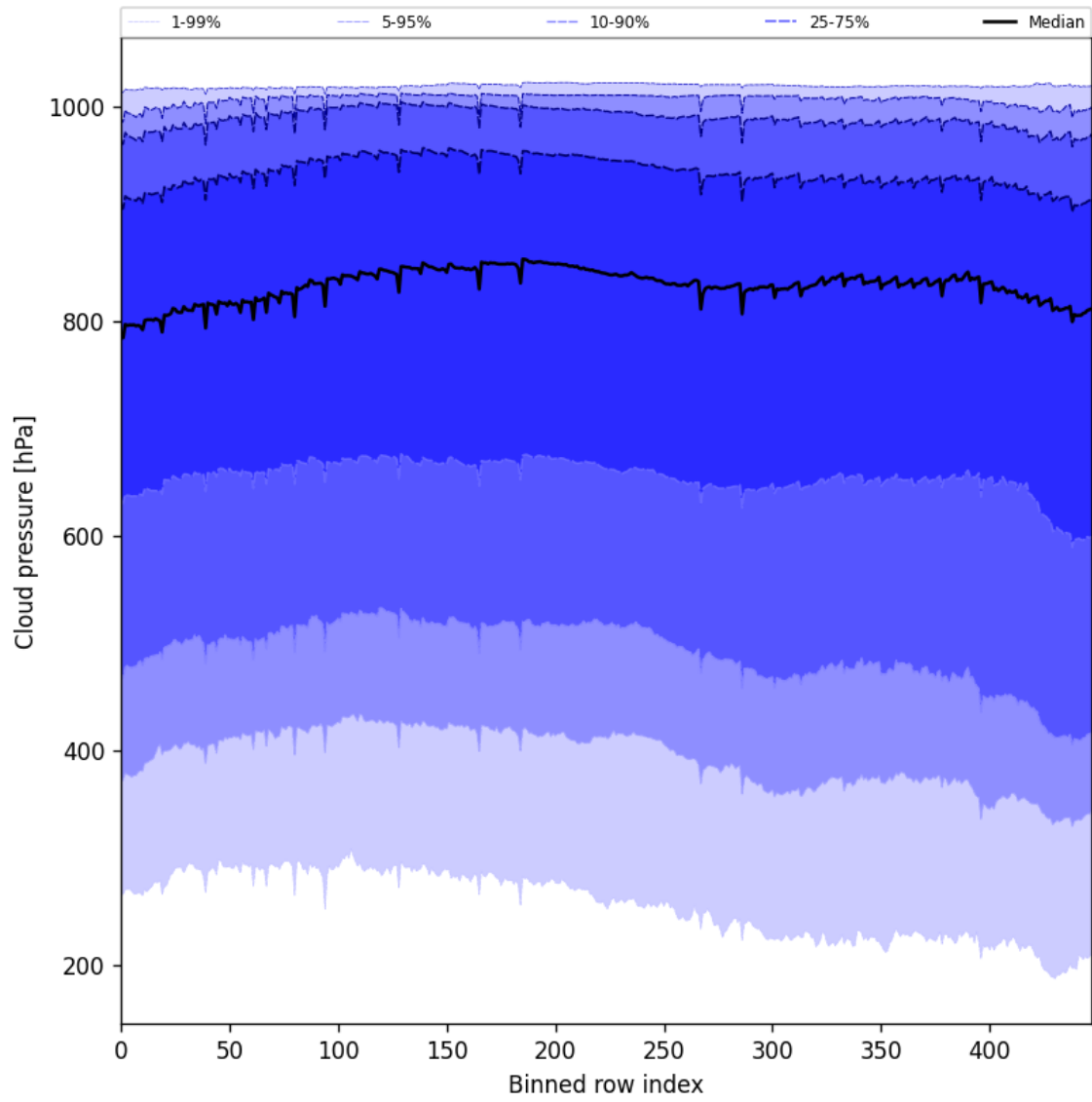
Figure 47: Along track statistics of “Cloud pressure” for 2025-01-08 to 2025-01-10
