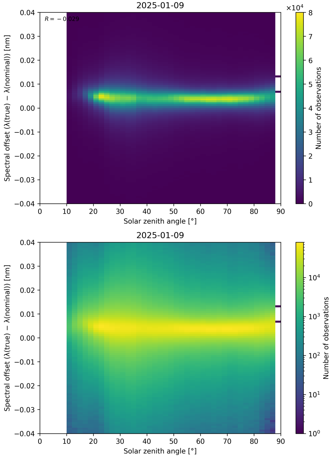
Figure 117: Scatter density plot of “Solar zenith angle” against “Spectral offset ( \lambda_{\text{true}} - \lambda_{\text{nominal}} )” for 2025-01-08 to 2025-01-10.
