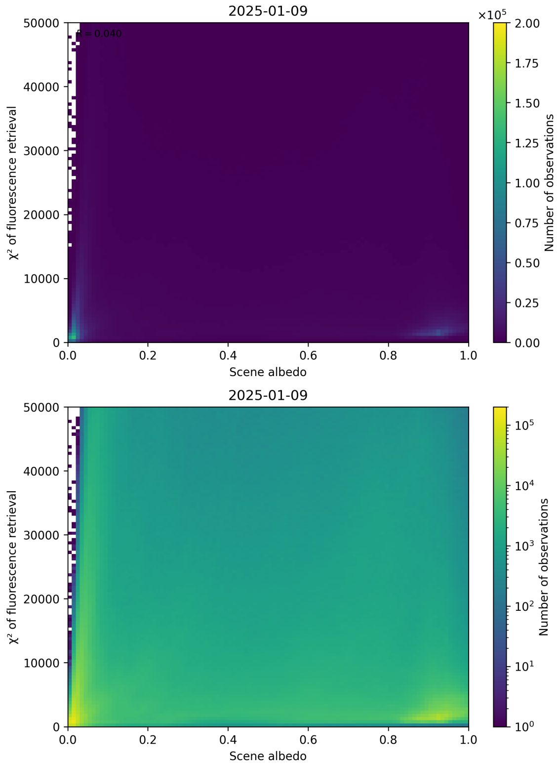
Figure 103: Scatter density plot of “Scene albedo” against “ \chi^2 of fluorescence retrieval” for 2025-01-08 to 2025-01-10.
