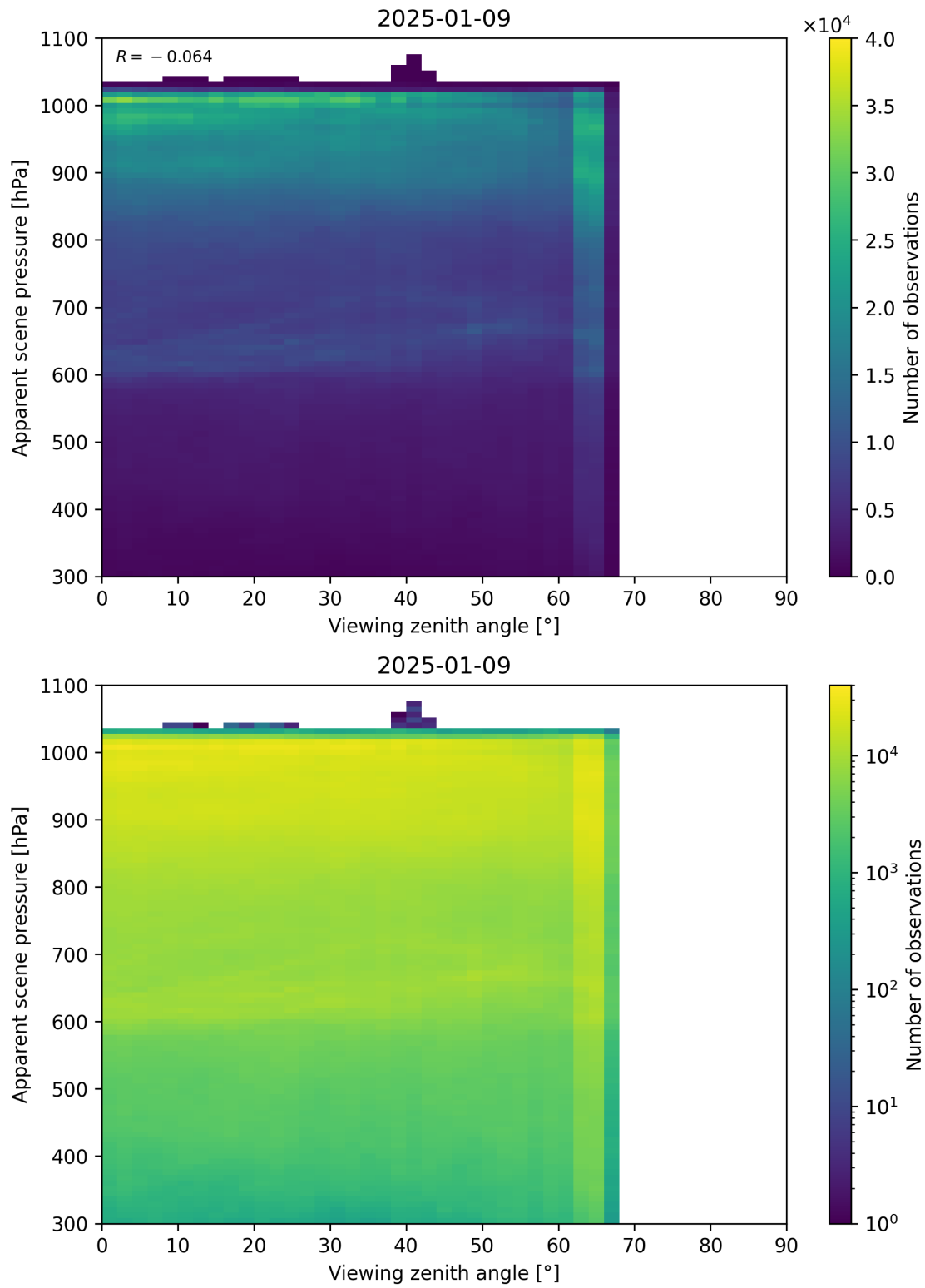
Figure 118: Scatter density plot of “Viewing zenith angle” against “Apparent scene pressure” for 2025-01-08 to 2025-01-10.
