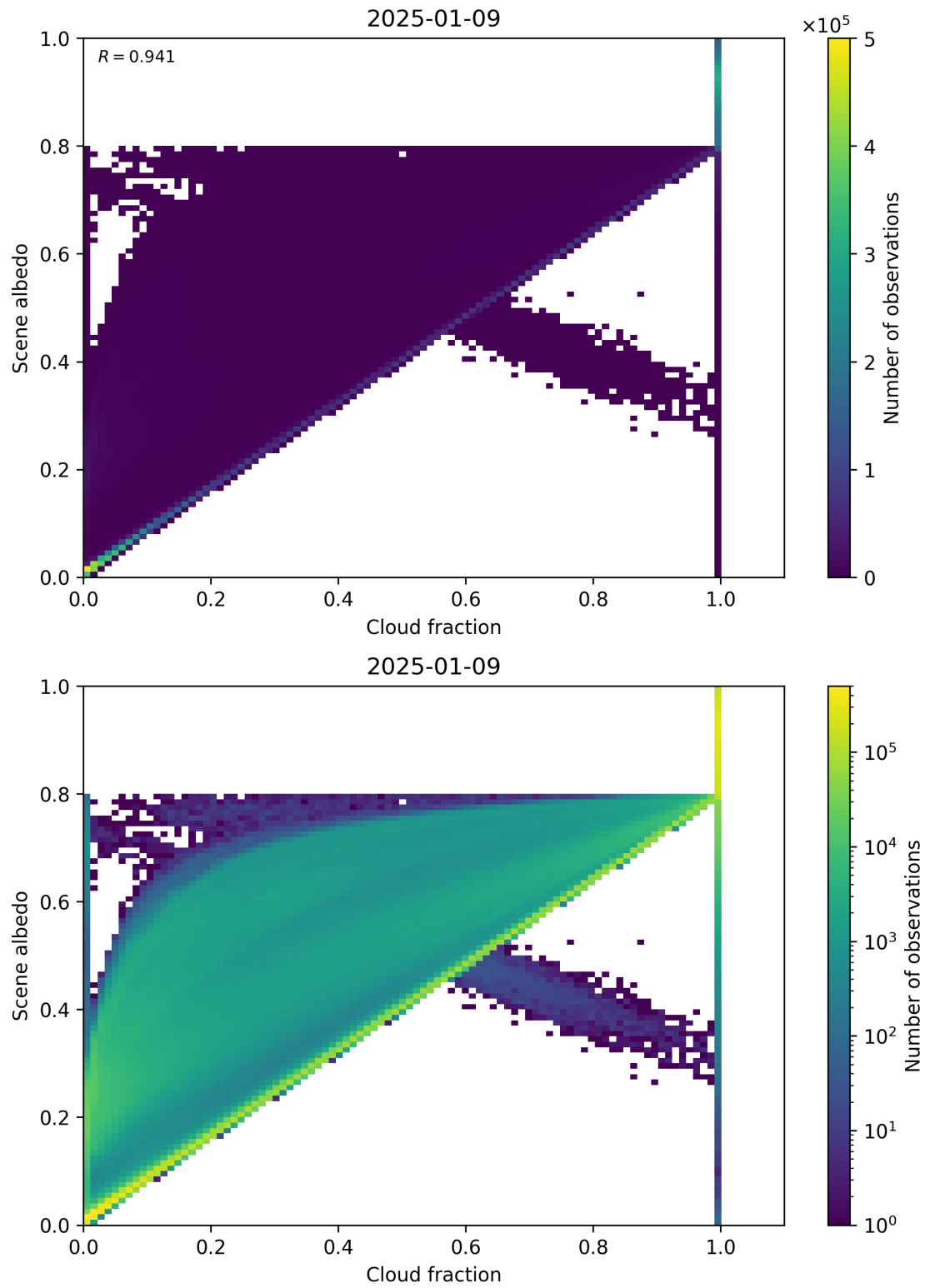
Figure 75: Scatter density plot of “Cloud fraction” against “Scene albedo” for 2025-01-08 to 2025-01-10.
