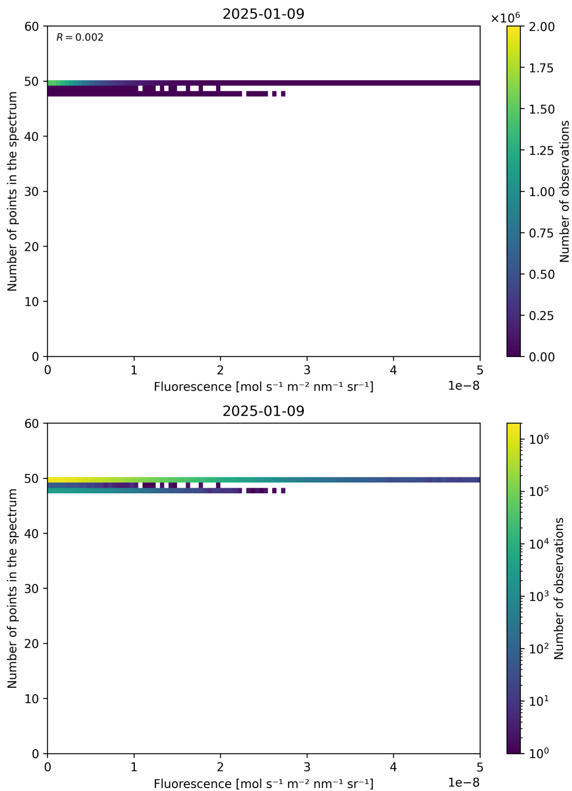
Figure 86: Scatter density plot of “Fluorescence” against “Number of points in the spectrum” for 2025-01-08 to 2025-01-10.
