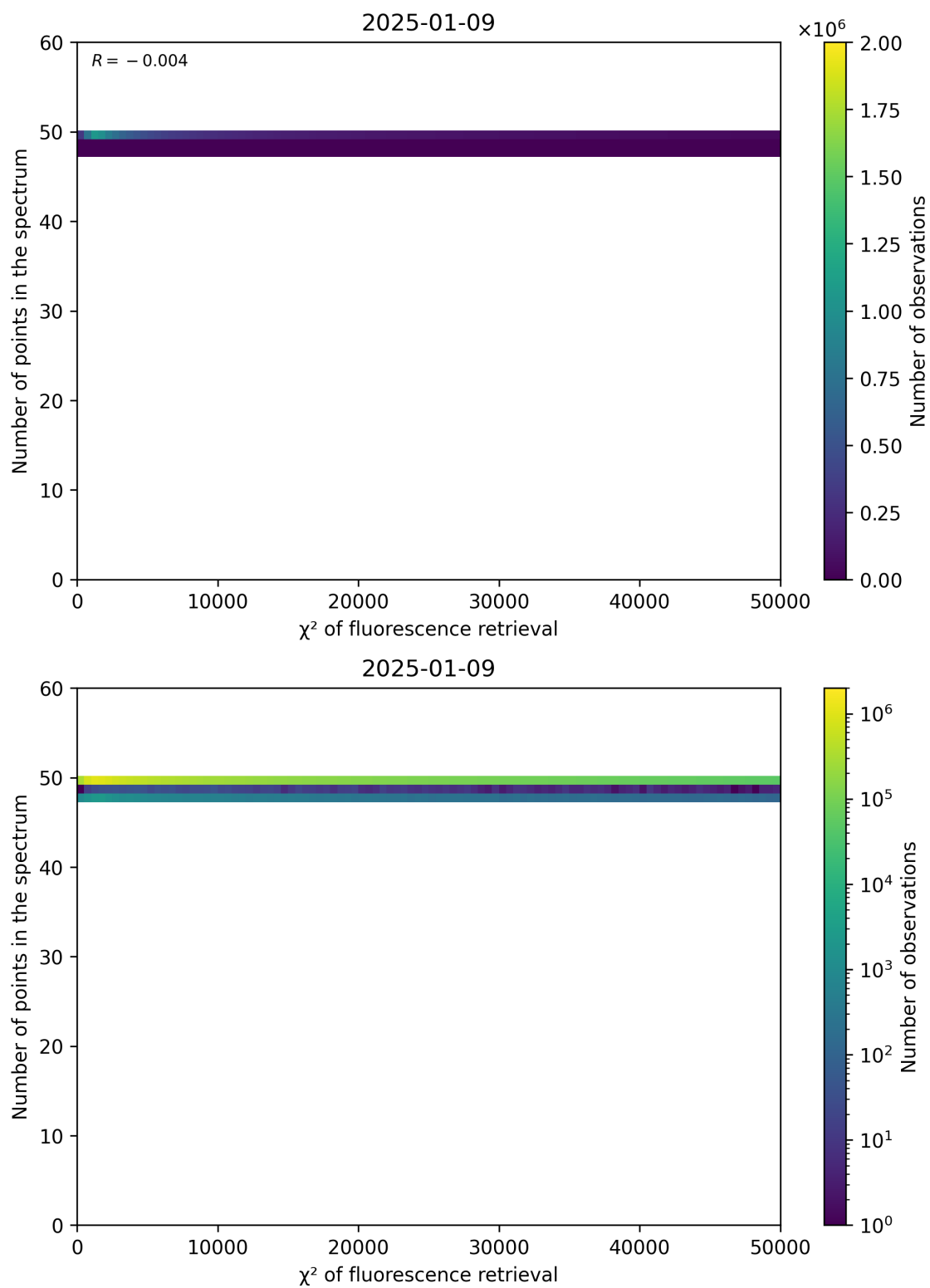
Figure 68: Scatter density plot of “ \chi^2 of fluorescence retrieval” against “Number of points in the spectrum” for 2025-01-08 to 2025-01-10.
