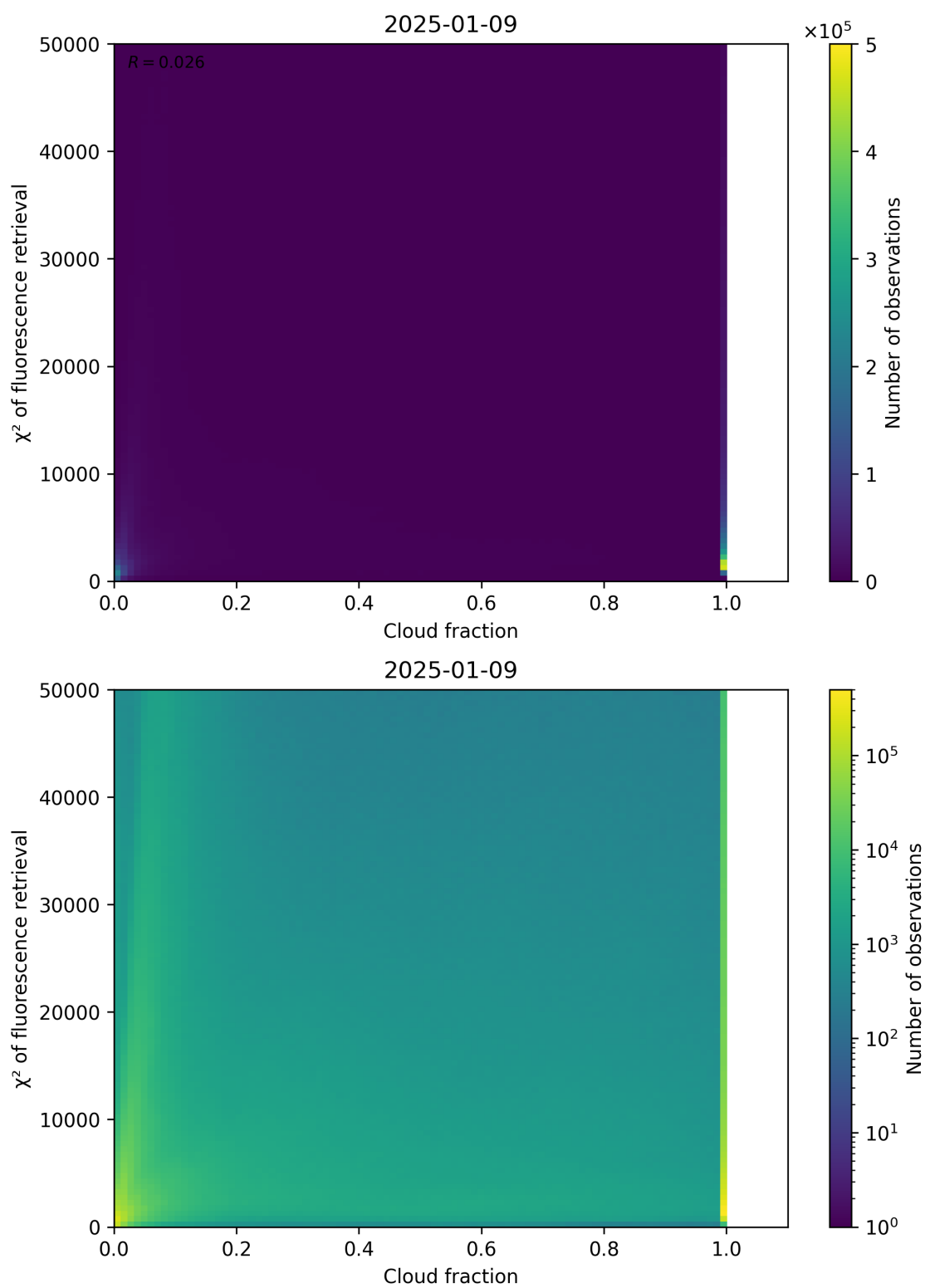
Figure 71: Scatter density plot of “Cloud fraction” against “ \chi^2 of fluorescence retrieval” for 2025-01-08 to 2025-01-10.
