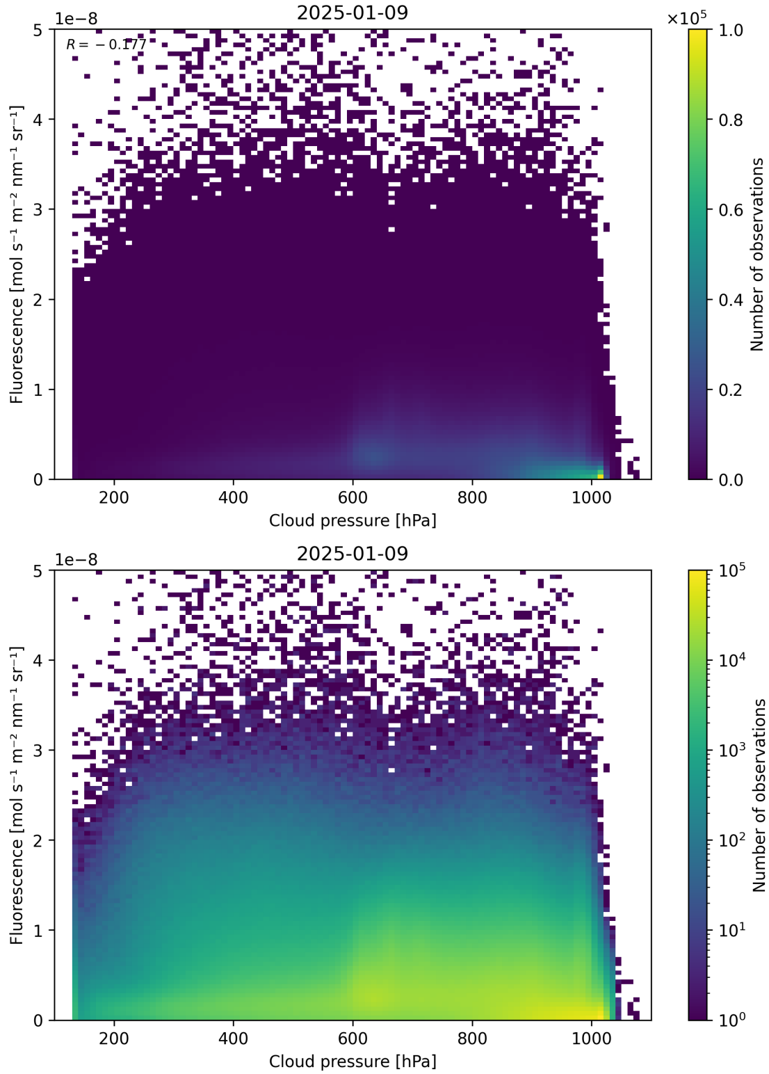
Figure 80: Scatter density plot of “Cloud pressure” against “Fluorescence” for 2025-01-08 to 2025-01-10.
