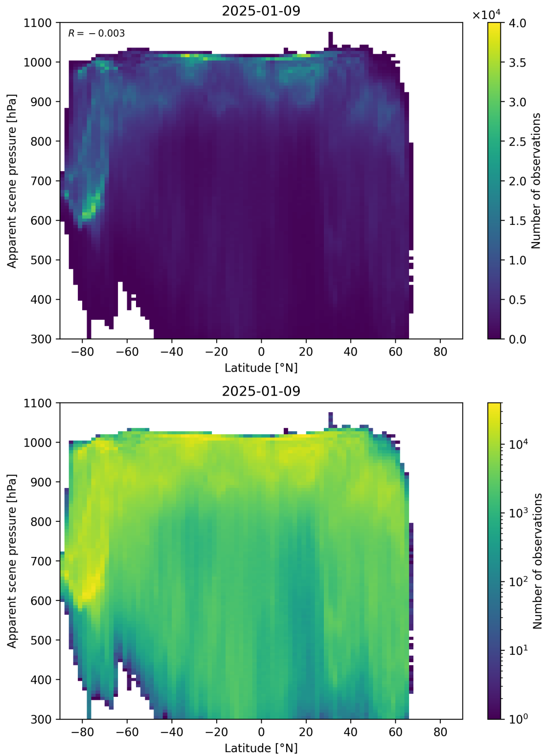
Figure 88: Scatter density plot of “Latitude” against “Apparent scene pressure” for 2025-01-08 to 2025-01-10.
