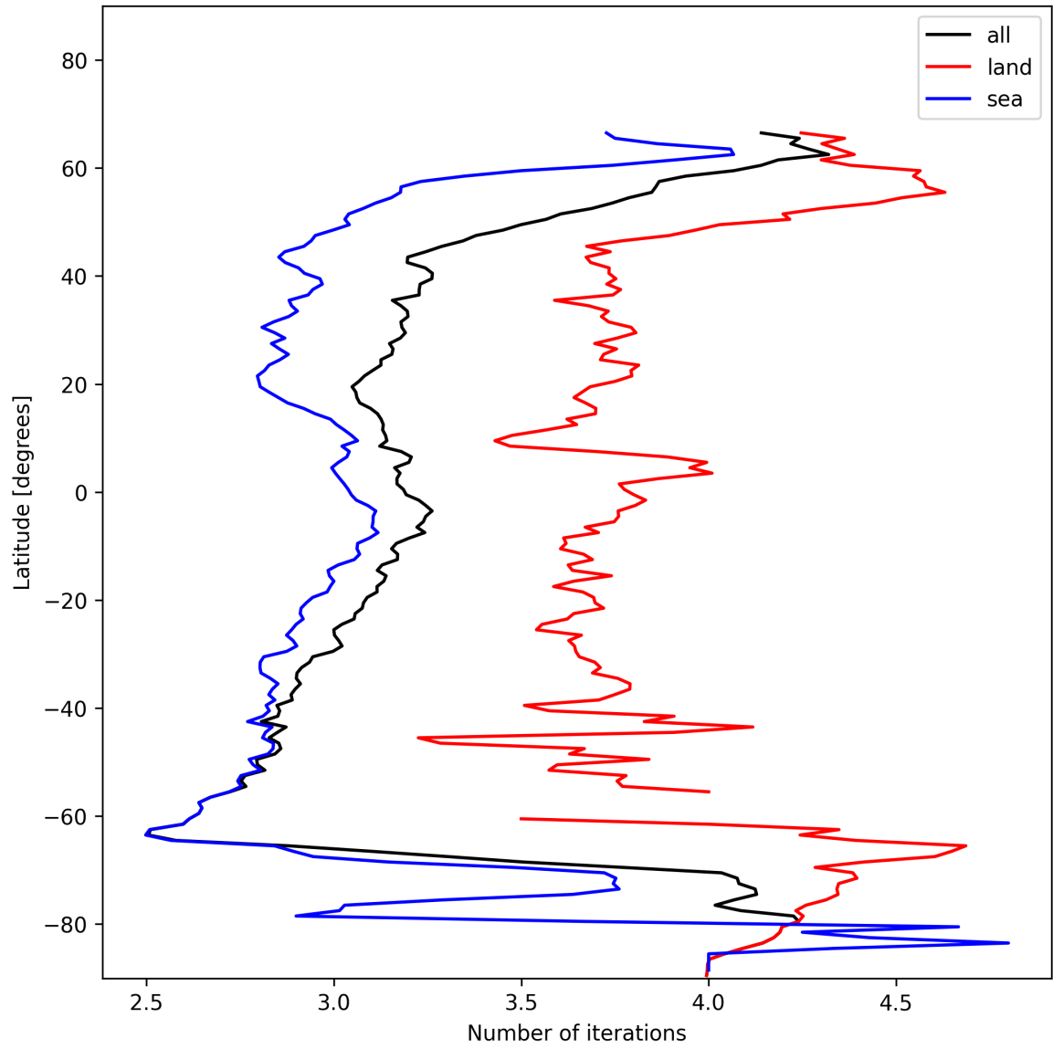
Figure 22: Zonal average of “Number of iterations” for 2025-01-08 to 2025-01-10.
