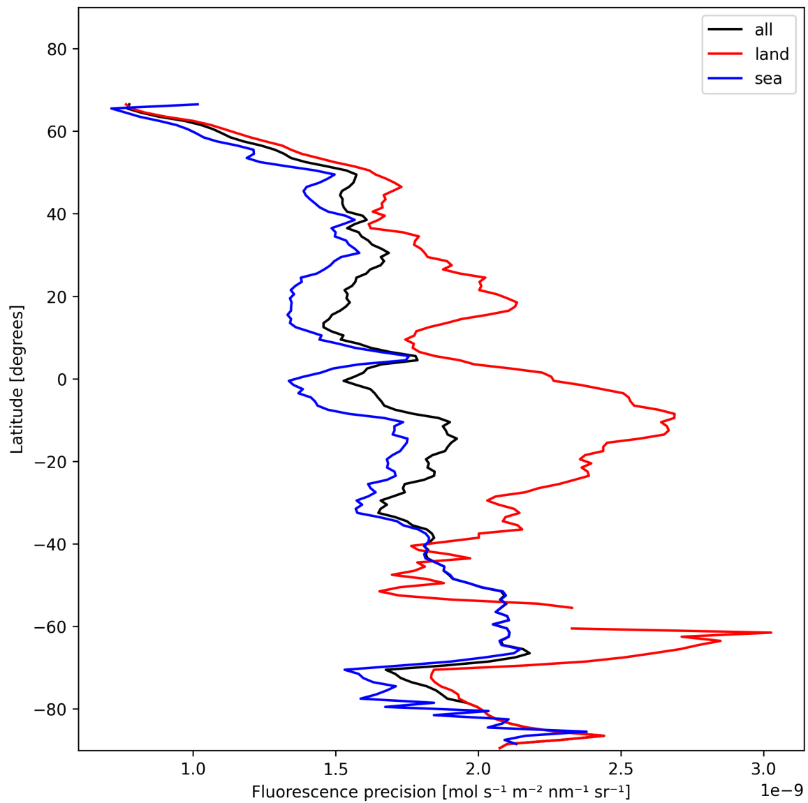
Figure 24: Zonal average of “Fluorescence precision” for 2025-01-08 to 2025-01-10.
