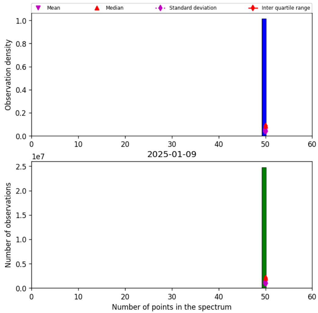
Figure 44: Histogram of “Number of points in the spectrum” for 2025-01-08 to 2025-01-10
