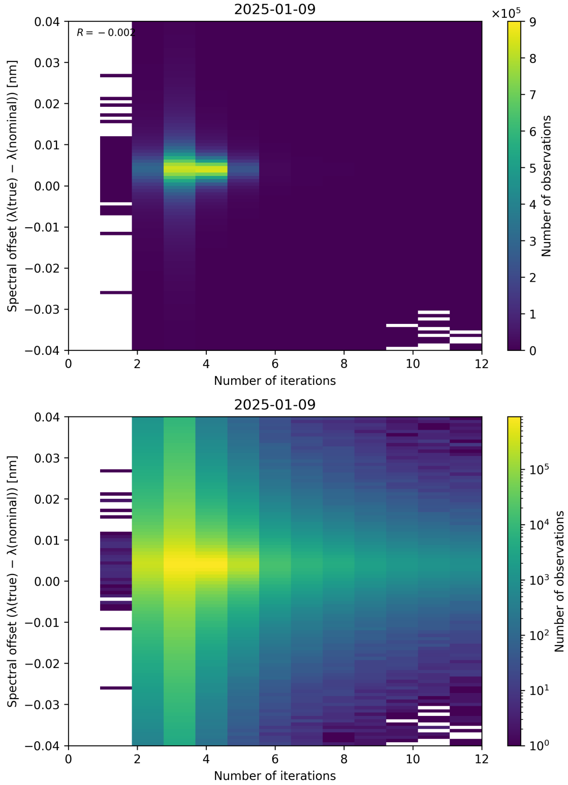
Figure 100: Scatter density plot of “Number of iterations” against “Spectral offset ( \lambda_{\text{true}} - \lambda_{\text{nominal}} )” for 2025-01-08 to 2025-01-10.
