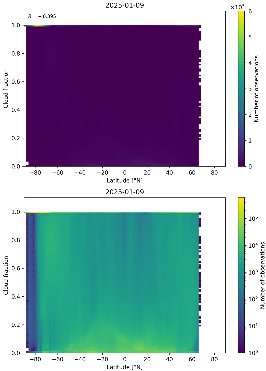
Figure 90: Scatter density plot of “Latitude” against “Cloud fraction” for 2025-01-08 to 2025-01-10.
