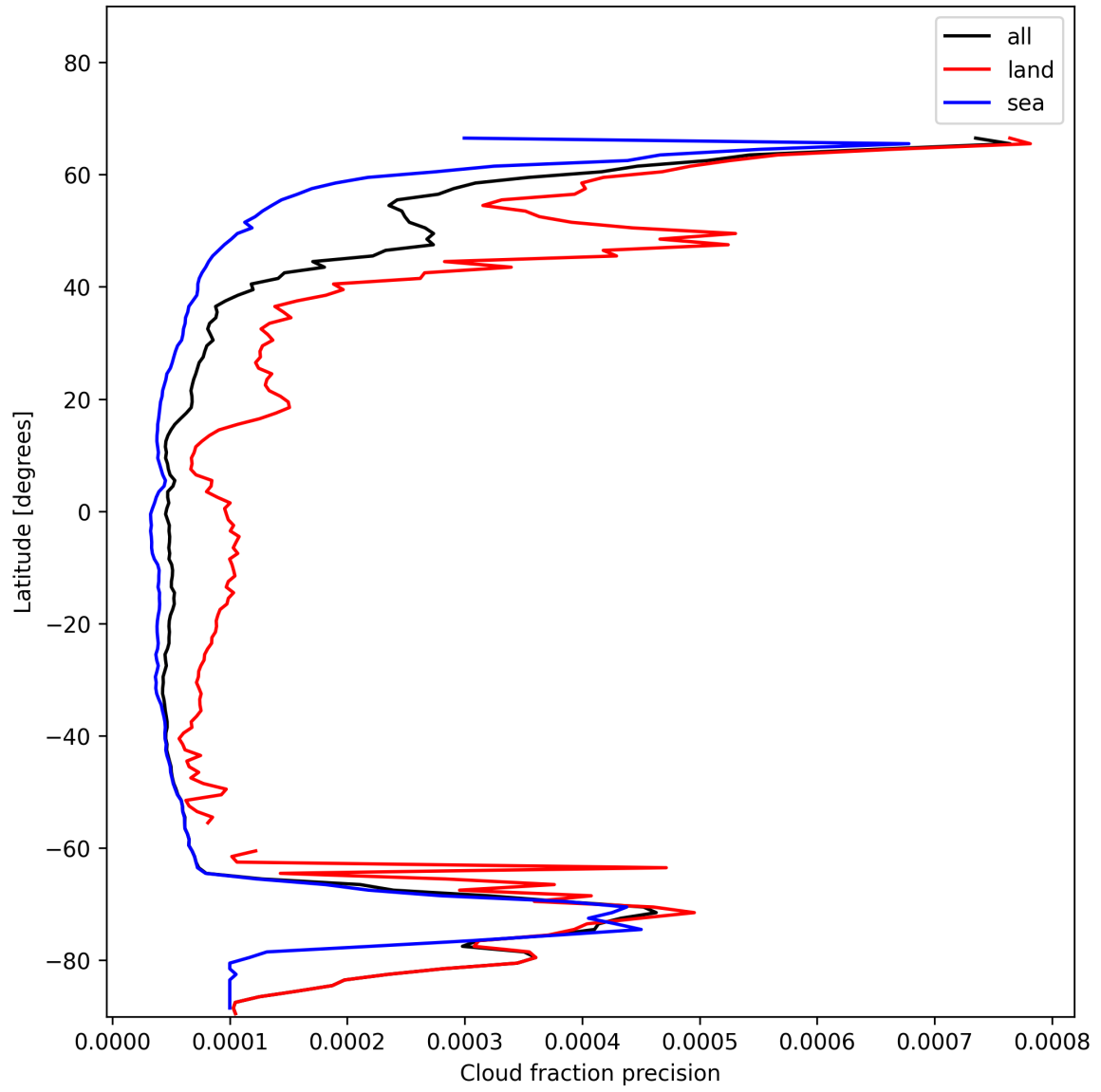
Figure 16: Zonal average of “Cloud fraction precision” for 2025-01-08 to 2025-01-10.
