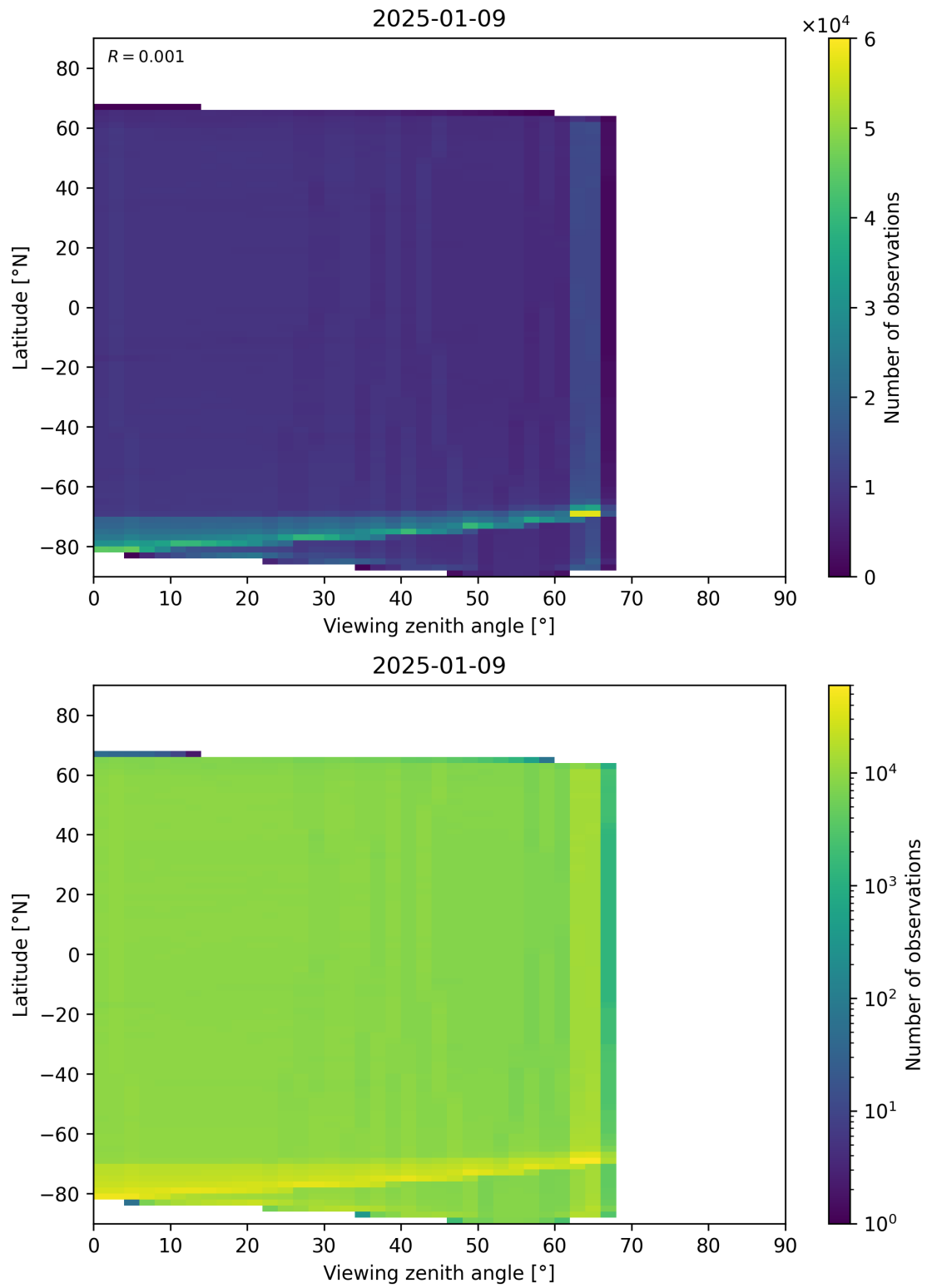
Figure 123: Scatter density plot of “Viewing zenith angle” against “Latitude” for 2025-01-08 to 2025-01-10.
