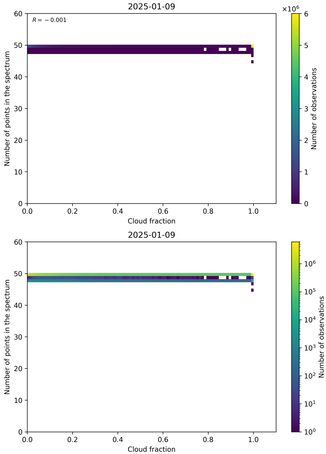
Figure 74: Scatter density plot of “Cloud fraction” against “Number of points in the spectrum” for 2025-01-08 to 2025-01-10.
