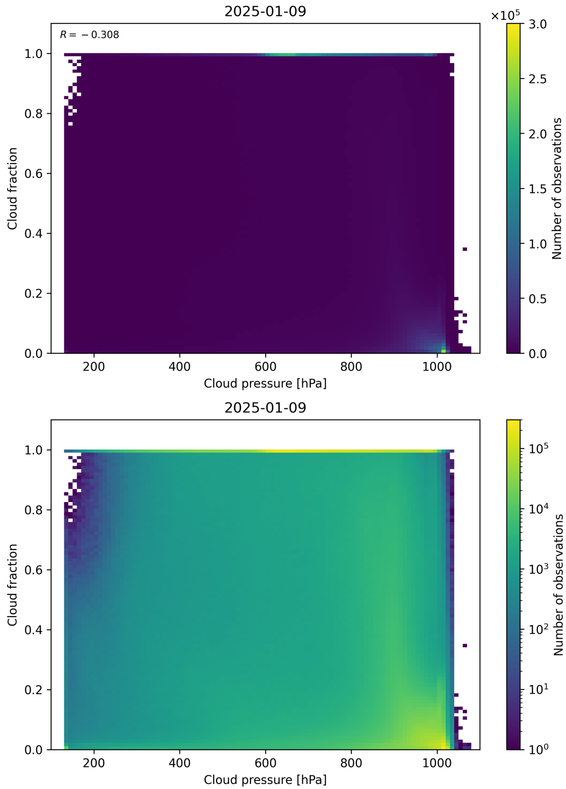
Figure 79: Scatter density plot of “Cloud pressure” against “Cloud fraction” for 2025-01-08 to 2025-01-10.
