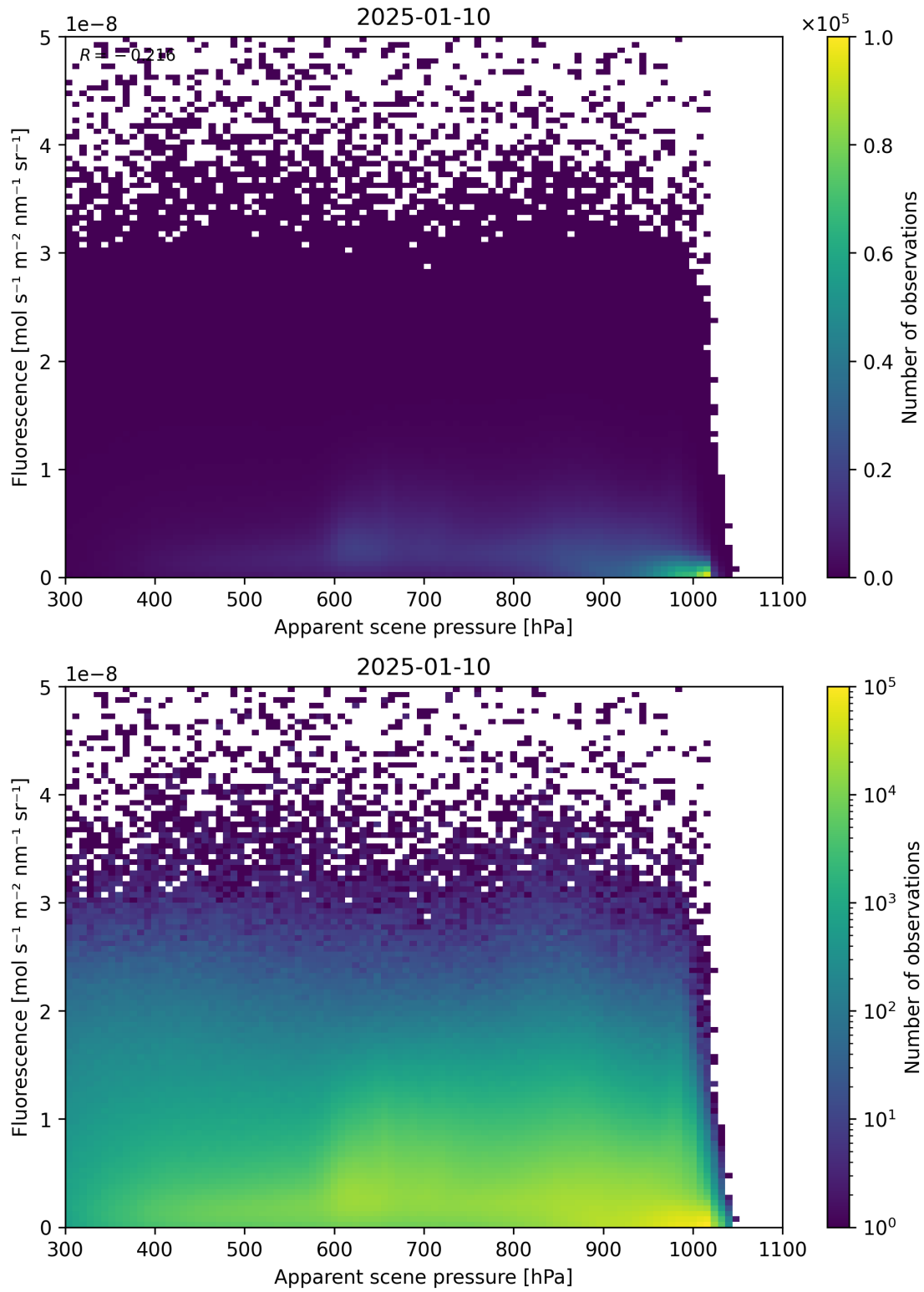
Figure 64: Scatter density plot of “Apparent scene pressure” against “Fluorescence” for 2025-01-09 to 2025-01-11.
