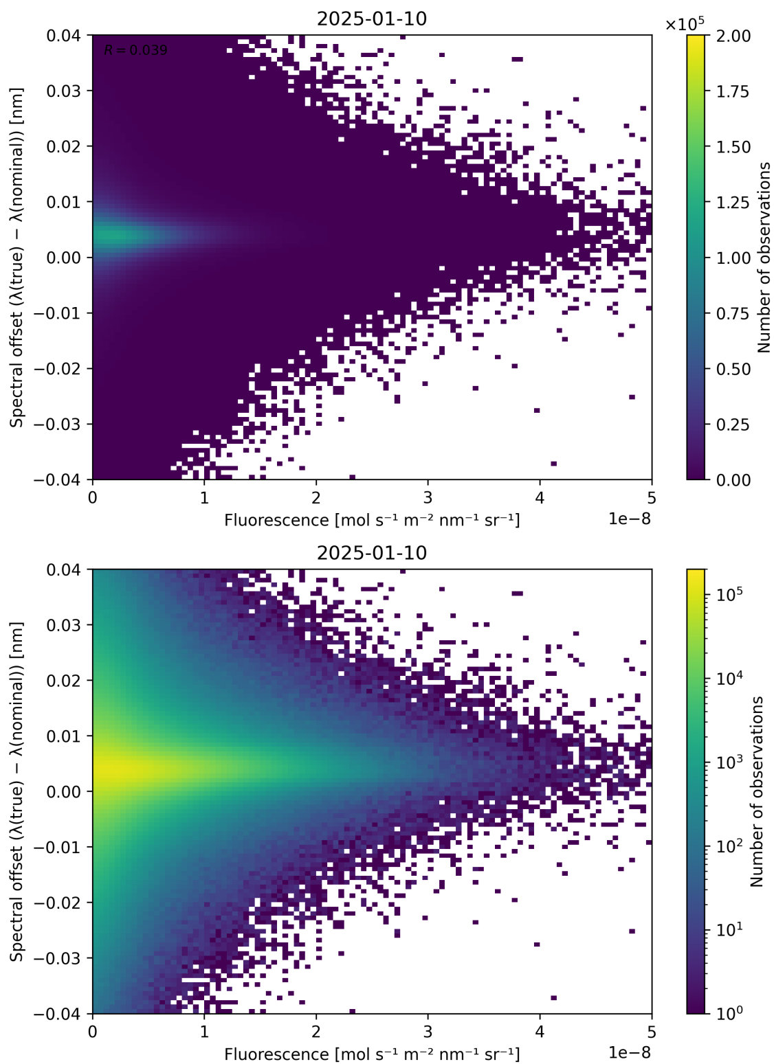
Figure 87: Scatter density plot of “Fluorescence” against “Spectral offset ( \lambda_{\text{true}} - \lambda_{\text{nominal}} )” for 2025-01-09 to 2025-01-11.
