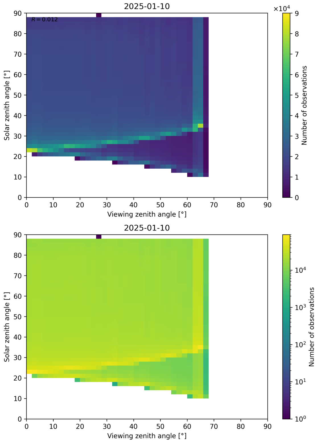
Figure 127: Scatter density plot of “Viewing zenith angle” against “Solar zenith angle” for 2025-01-09 to 2025-01-11.
