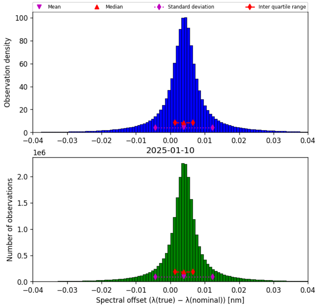
Figure 45: Histogram of “Spectral offset ( \lambda_{\text{true}} - \lambda_{\text{nominal}} )” for 2025-01-09 to 2025-01-11
