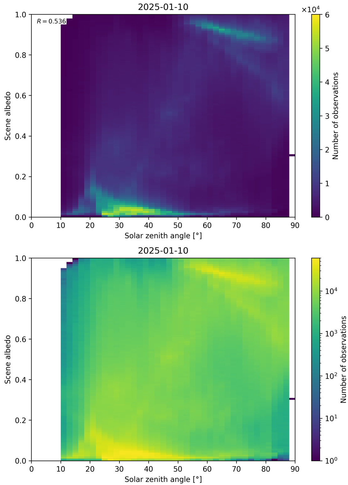
Figure 116: Scatter density plot of “Solar zenith angle” against “Scene albedo” for 2025-01-09 to 2025-01-11.
