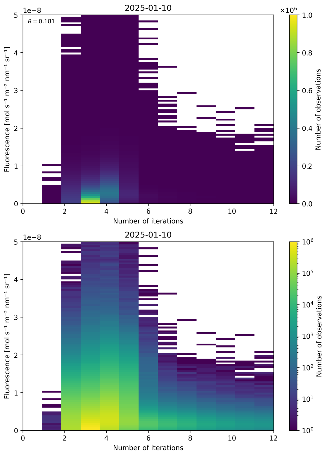
Figure 98: Scatter density plot of “Number of iterations” against “Fluorescence” for 2025-01-09 to 2025-01-11.
