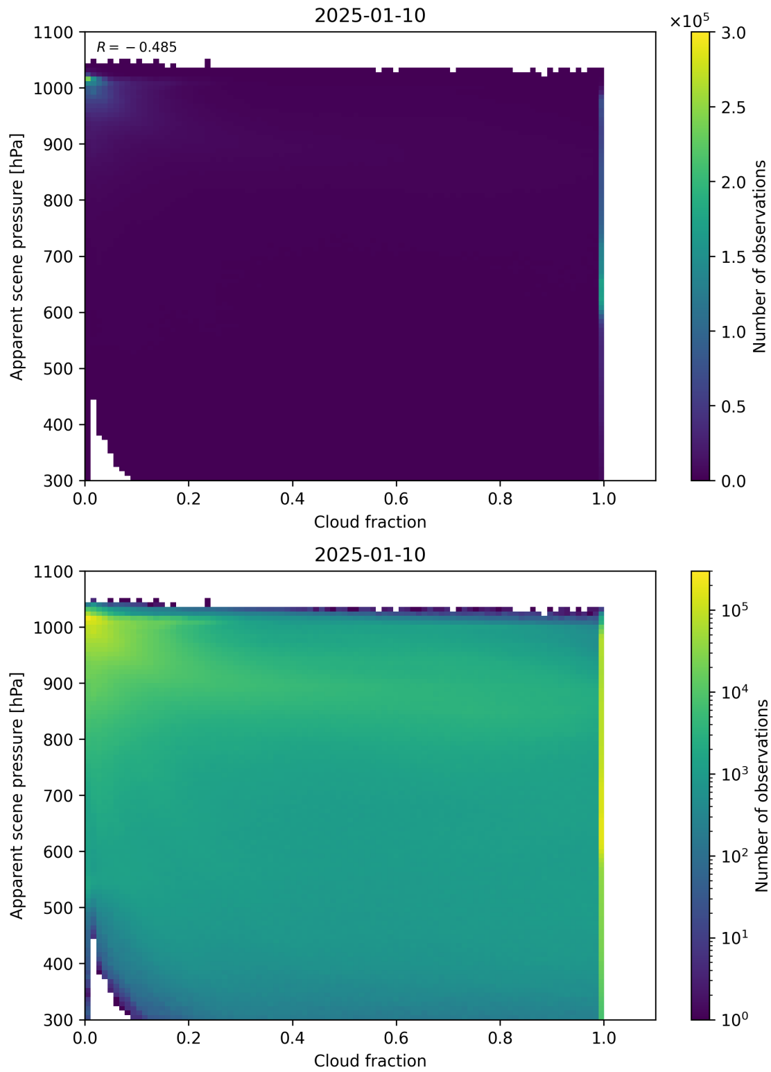
Figure 70: Scatter density plot of “Cloud fraction” against “Apparent scene pressure” for 2025-01-09 to 2025-01-11.
