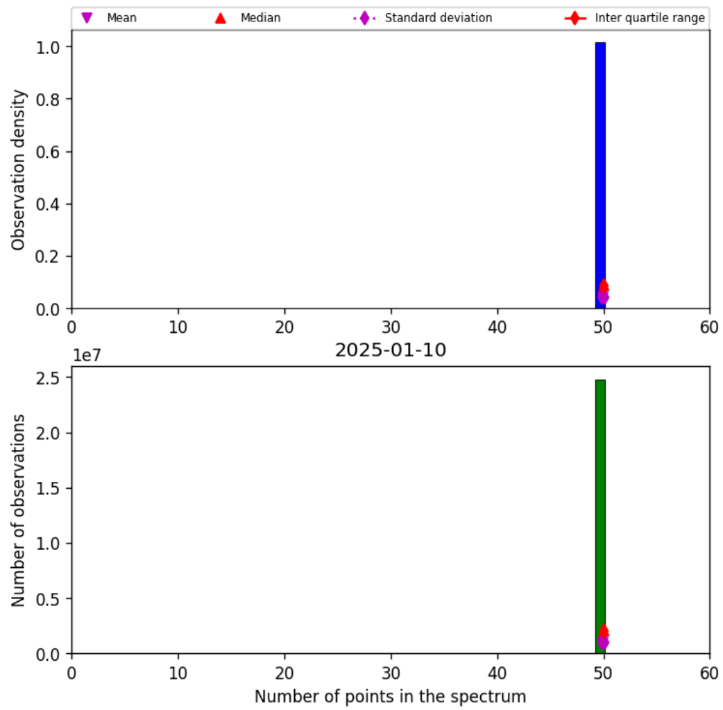
Figure 44: Histogram of “Number of points in the spectrum” for 2025-01-09 to 2025-01-11
