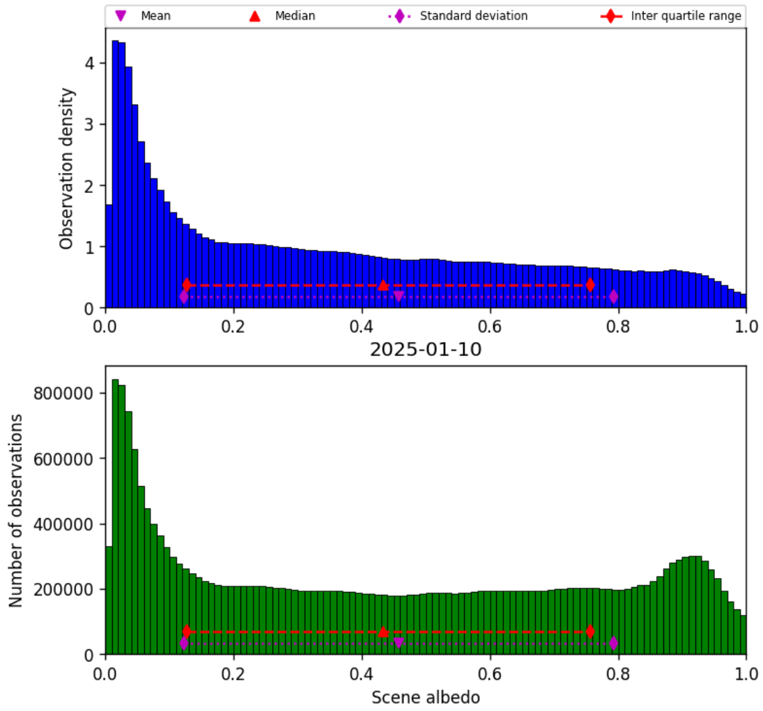
Figure 34: Histogram of “Scene albedo” for 2025-01-09 to 2025-01-11
