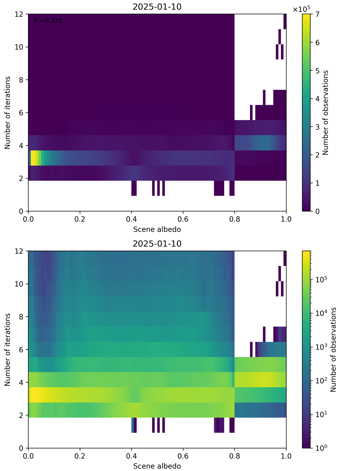
Figure 105: Scatter density plot of “Scene albedo” against “Number of iterations” for 2025-01-09 to 2025-01-11.
