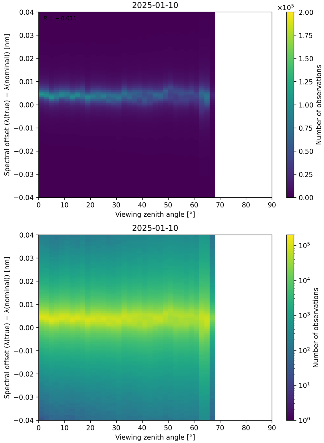
Figure 128: Scatter density plot of “Viewing zenith angle” against “Spectral offset ( \lambda_{\text{true}} - \lambda_{\text{nominal}} )” for 2025-01-09 to 2025-01-11.
