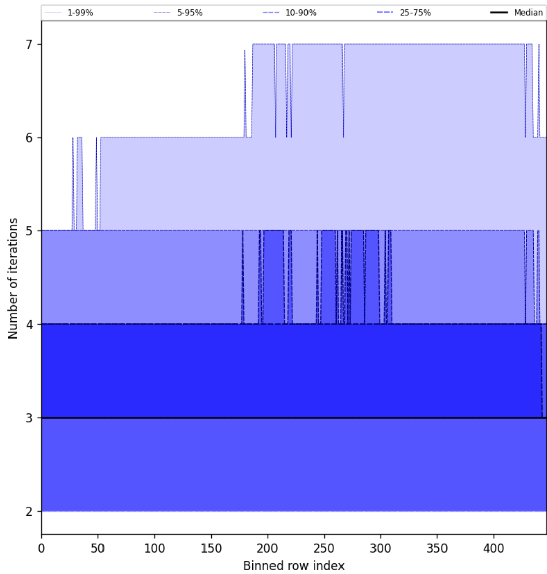
Figure 56: Along track statistics of “Number of iterations” for 2025-01-09 to 2025-01-11
