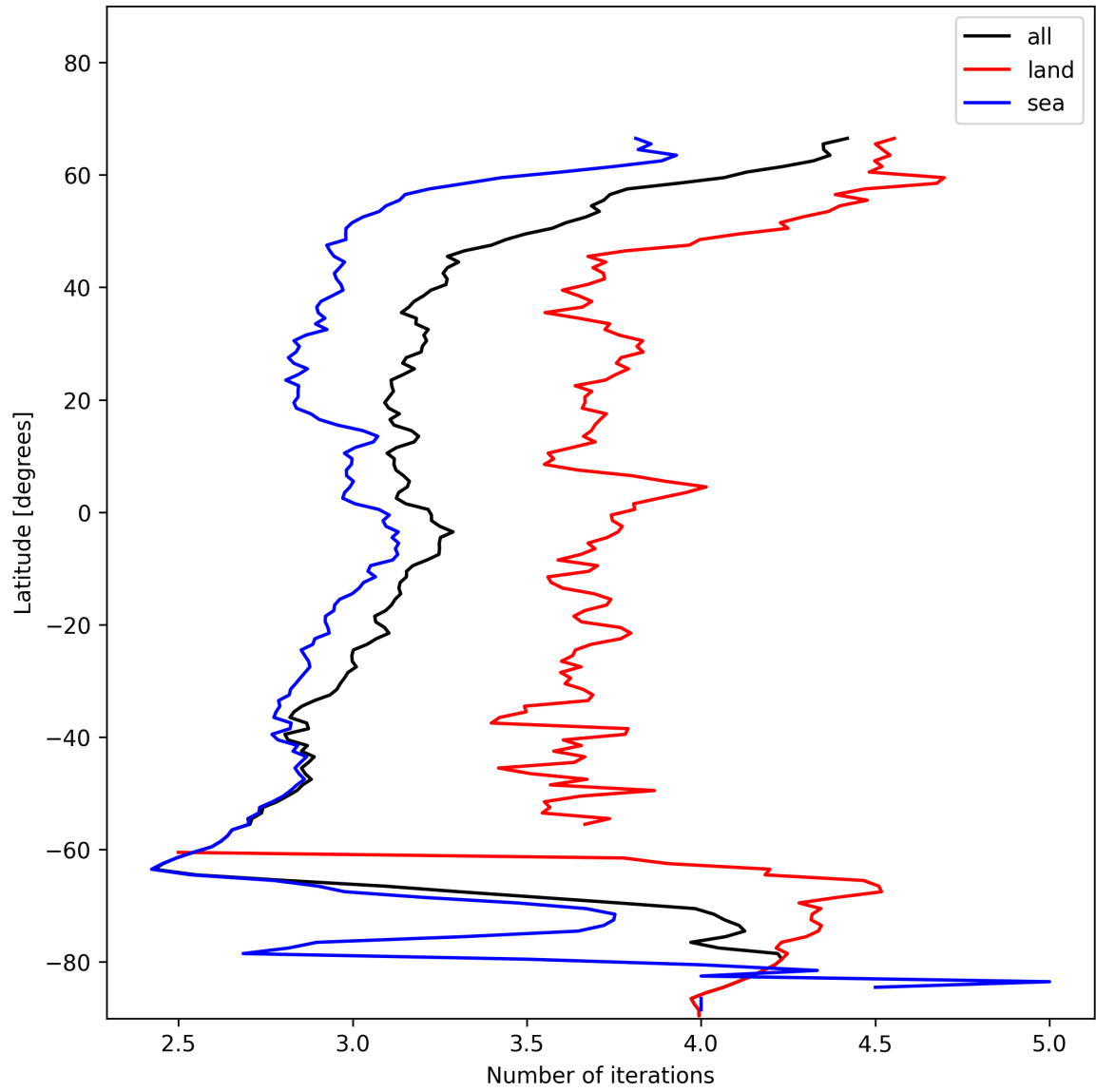
Figure 22: Zonal average of “Number of iterations” for 2025-01-09 to 2025-01-11.
