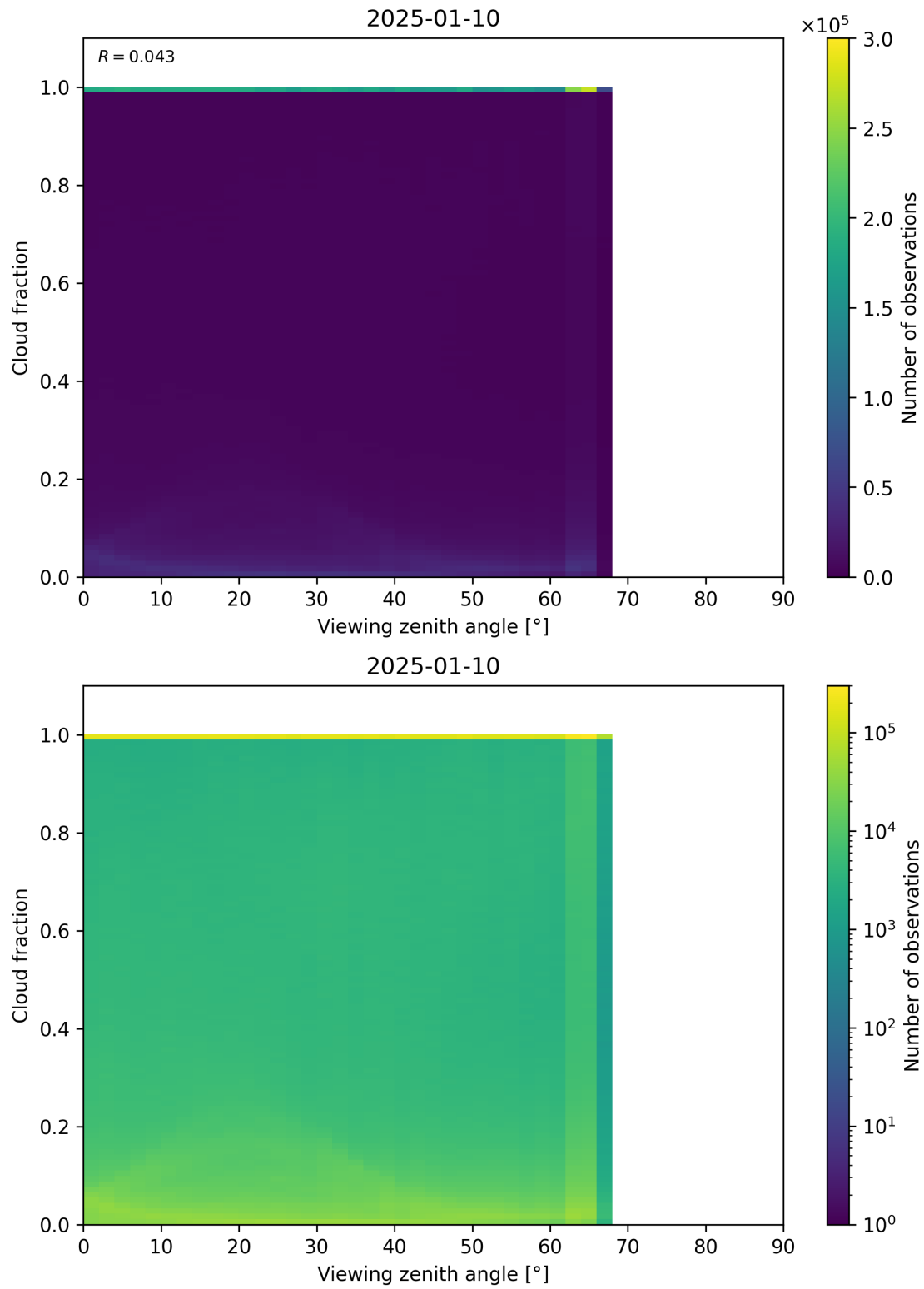
Figure 120: Scatter density plot of “Viewing zenith angle” against “Cloud fraction” for 2025-01-09 to 2025-01-11.
