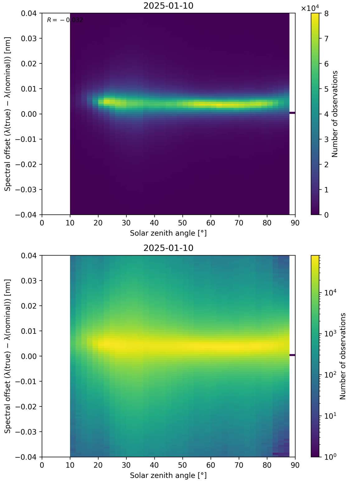
Figure 117: Scatter density plot of “Solar zenith angle” against “Spectral offset ( \lambda_{\text{true}} - \lambda_{\text{nominal}} )” for 2025-01-09 to 2025-01-11.
