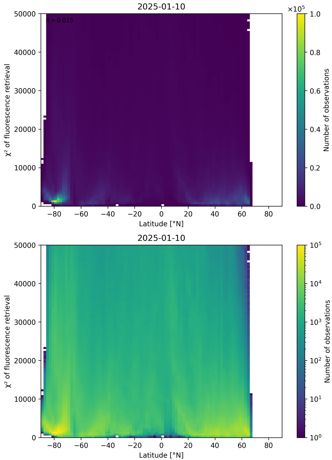
Figure 89: Scatter density plot of “Latitude” against “ \chi^2 of fluorescence retrieval” for 2025-01-09 to 2025-01-11.
