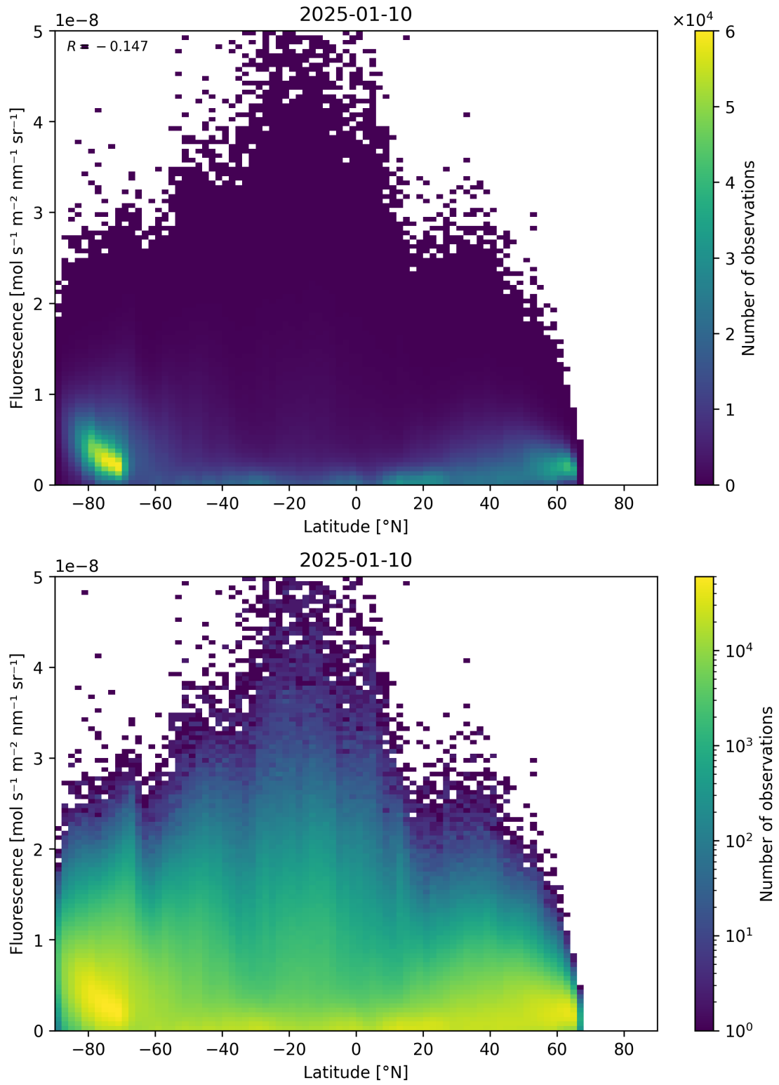
Figure 92: Scatter density plot of “Latitude” against “Fluorescence” for 2025-01-09 to 2025-01-11.
