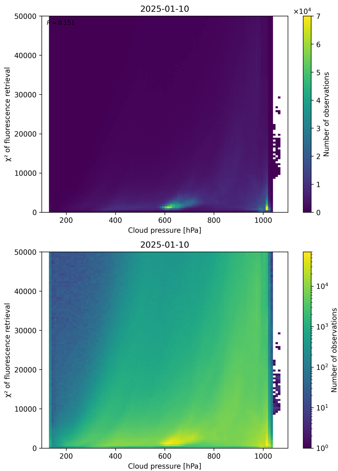
Figure 78: Scatter density plot of “Cloud pressure” against “ \chi^2 of fluorescence retrieval” for 2025-01-09 to 2025-01-11.
