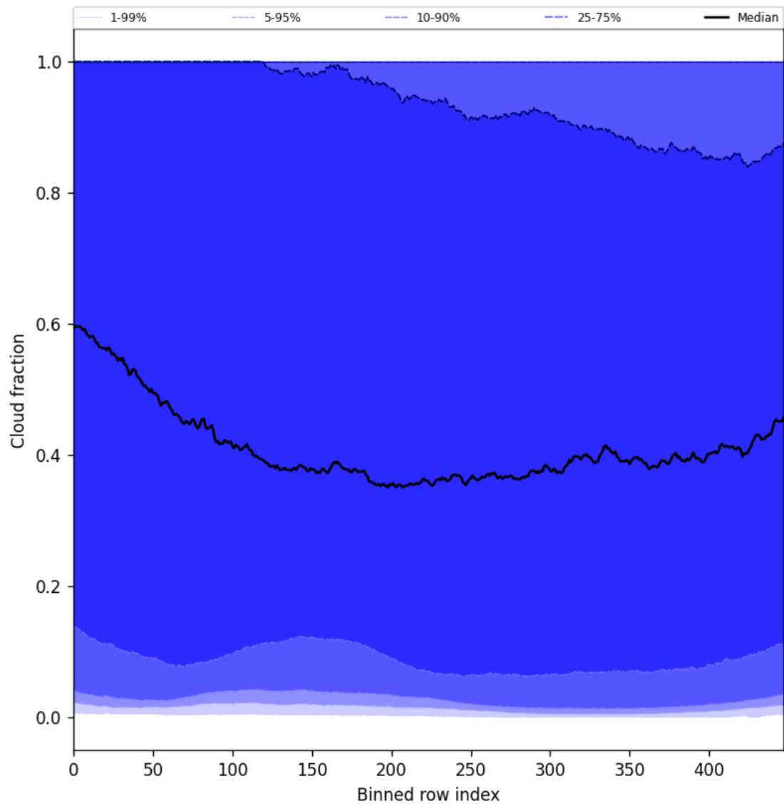
Figure 49: Along track statistics of “Cloud fraction” for 2025-01-09 to 2025-01-11
