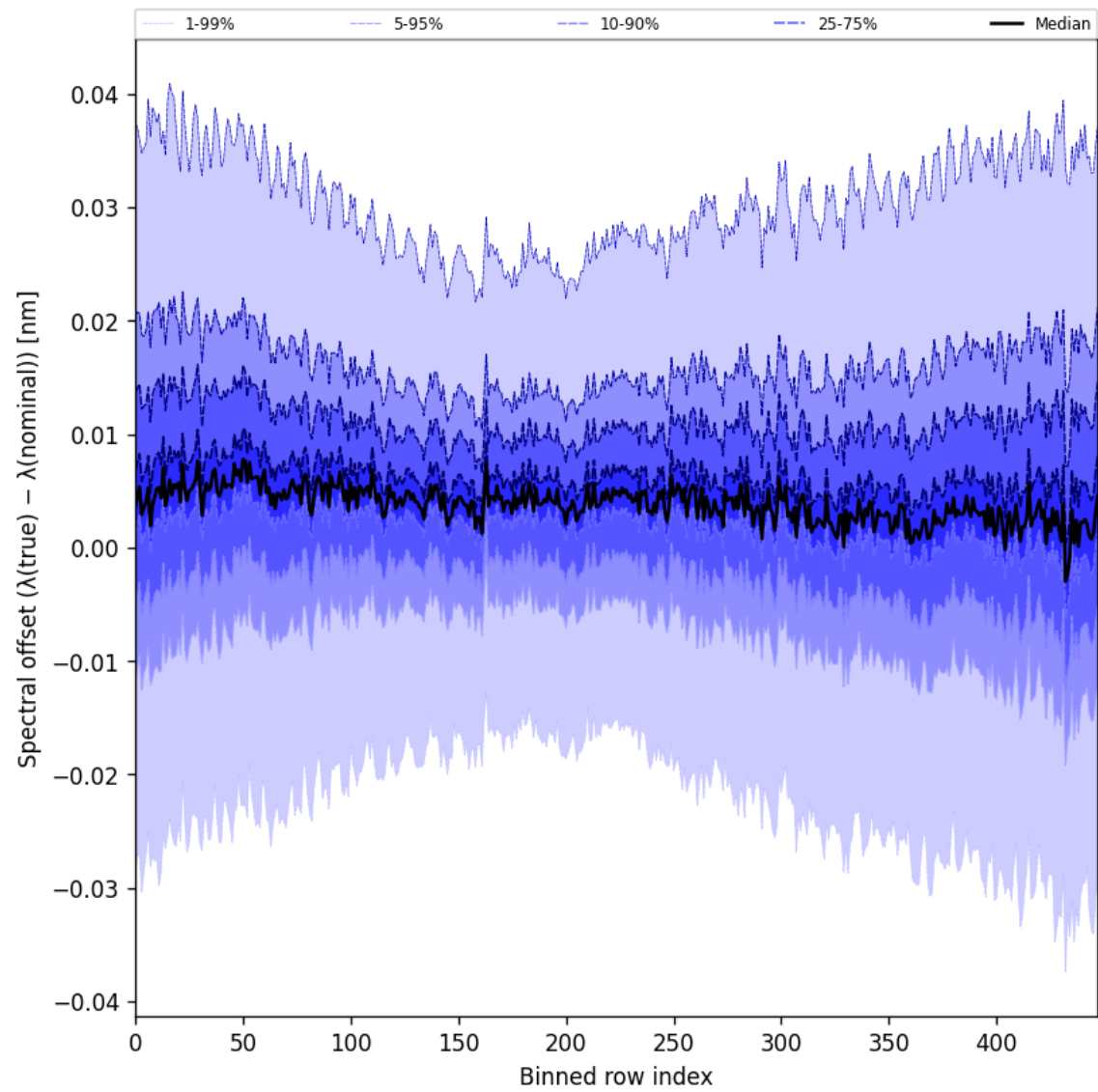
Figure 62: Along track statistics of “Spectral offset ( \lambda_{\text{true}} - \lambda_{\text{nominal}} )” for 2025-01-09 to 2025-01-11
