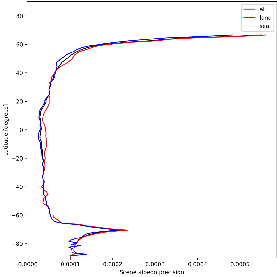
Figure 18: Zonal average of “Scene albedo precision” for 2025-01-09 to 2025-01-11.
