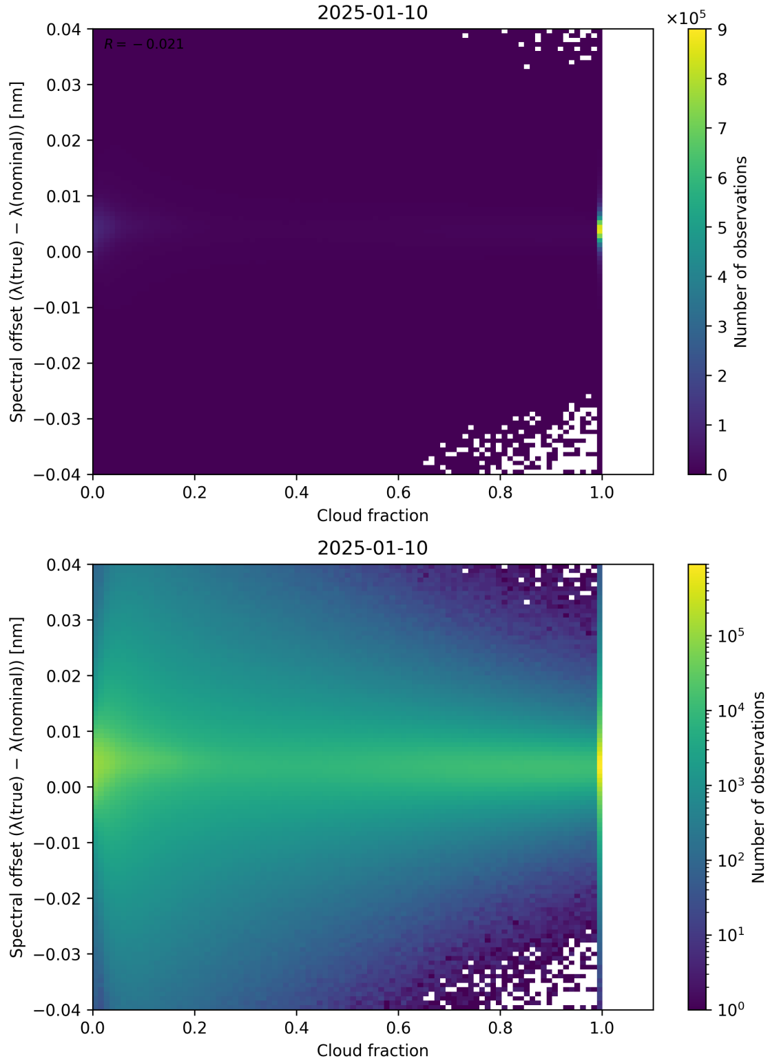
Figure 76: Scatter density plot of “Cloud fraction” against “Spectral offset ( \lambda_{\text{true}} - \lambda_{\text{nominal}} )” for 2025-01-09 to 2025-01-11.
