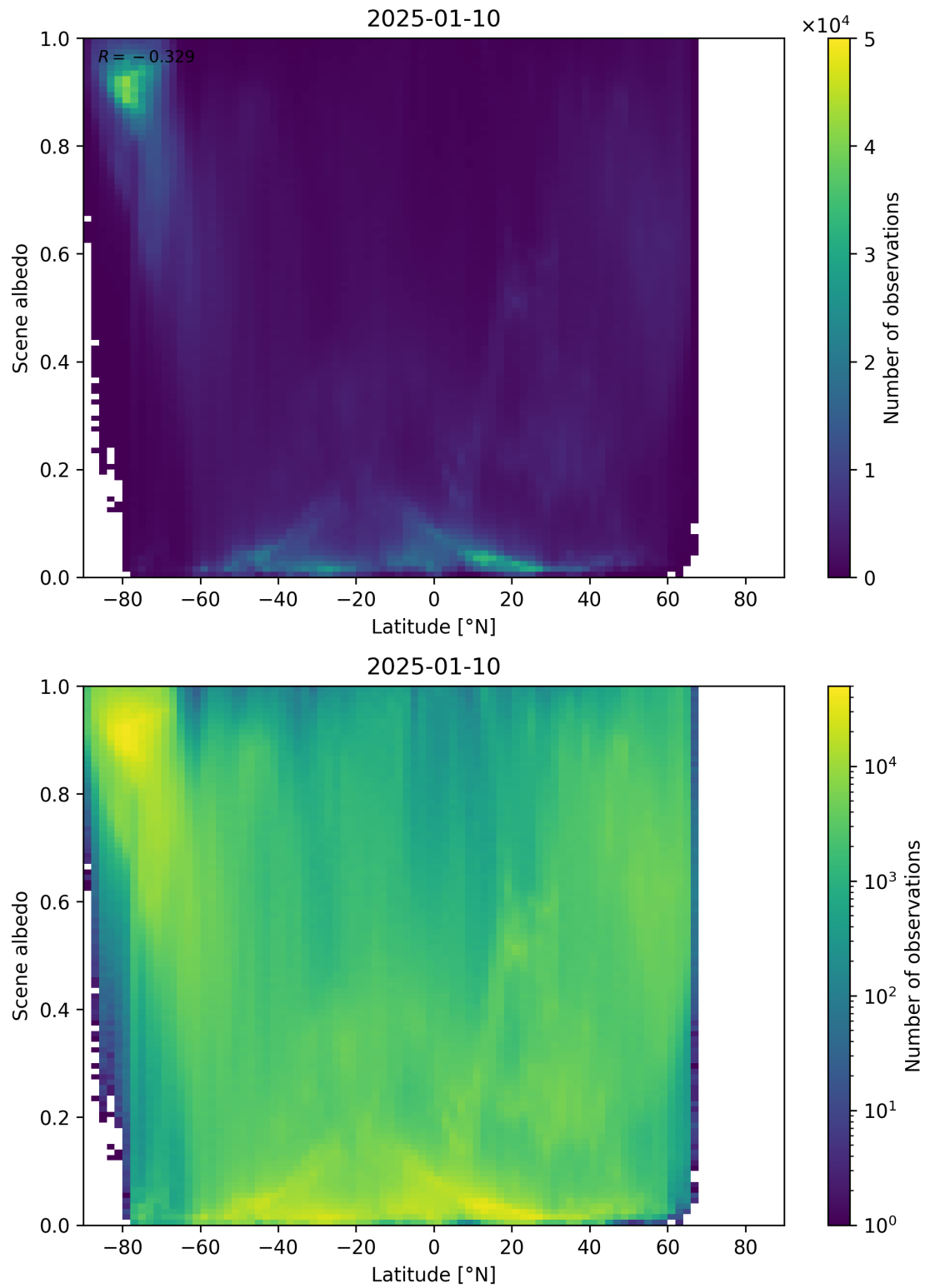
Figure 95: Scatter density plot of “Latitude” against “Scene albedo” for 2025-01-09 to 2025-01-11.
