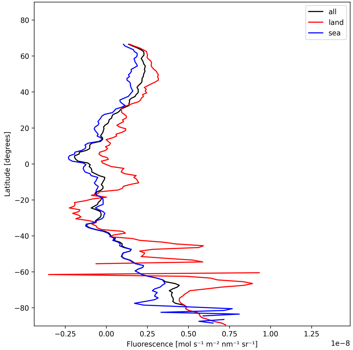
Figure 23: Zonal average of “Fluorescence” for 2025-01-09 to 2025-01-11.
