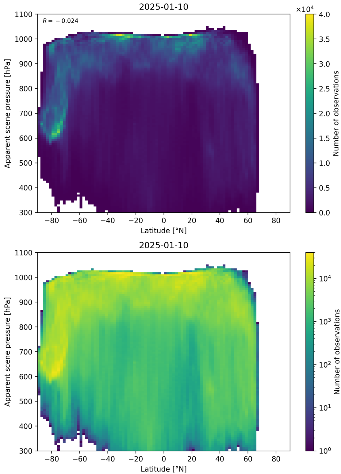
Figure 88: Scatter density plot of “Latitude” against “Apparent scene pressure” for 2025-01-09 to 2025-01-11.
