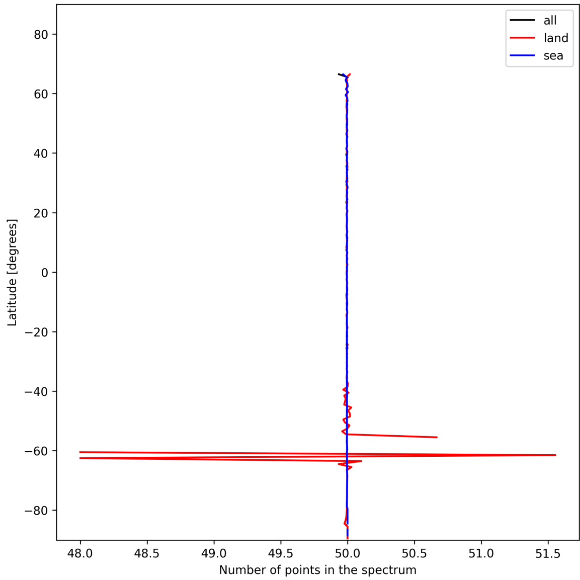
Figure 27: Zonal average of “Number of points in the spectrum” for 2025-01-09 to 2025-01-11.
