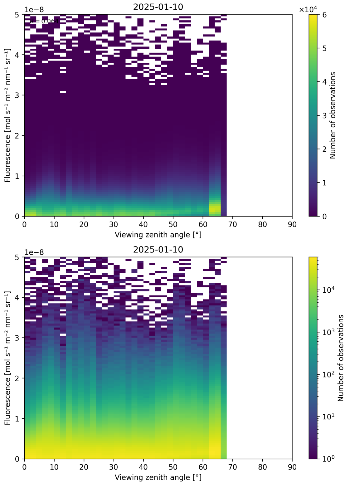
Figure 122: Scatter density plot of “Viewing zenith angle” against “Fluorescence” for 2025-01-09 to 2025-01-11.
