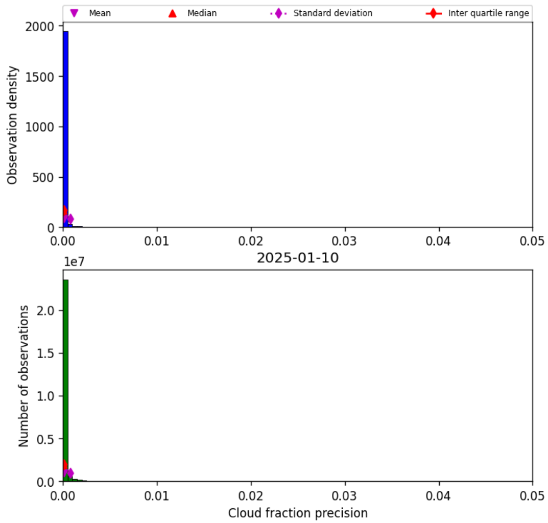
Figure 33: Histogram of “Cloud fraction precision” for 2025-01-09 to 2025-01-11
