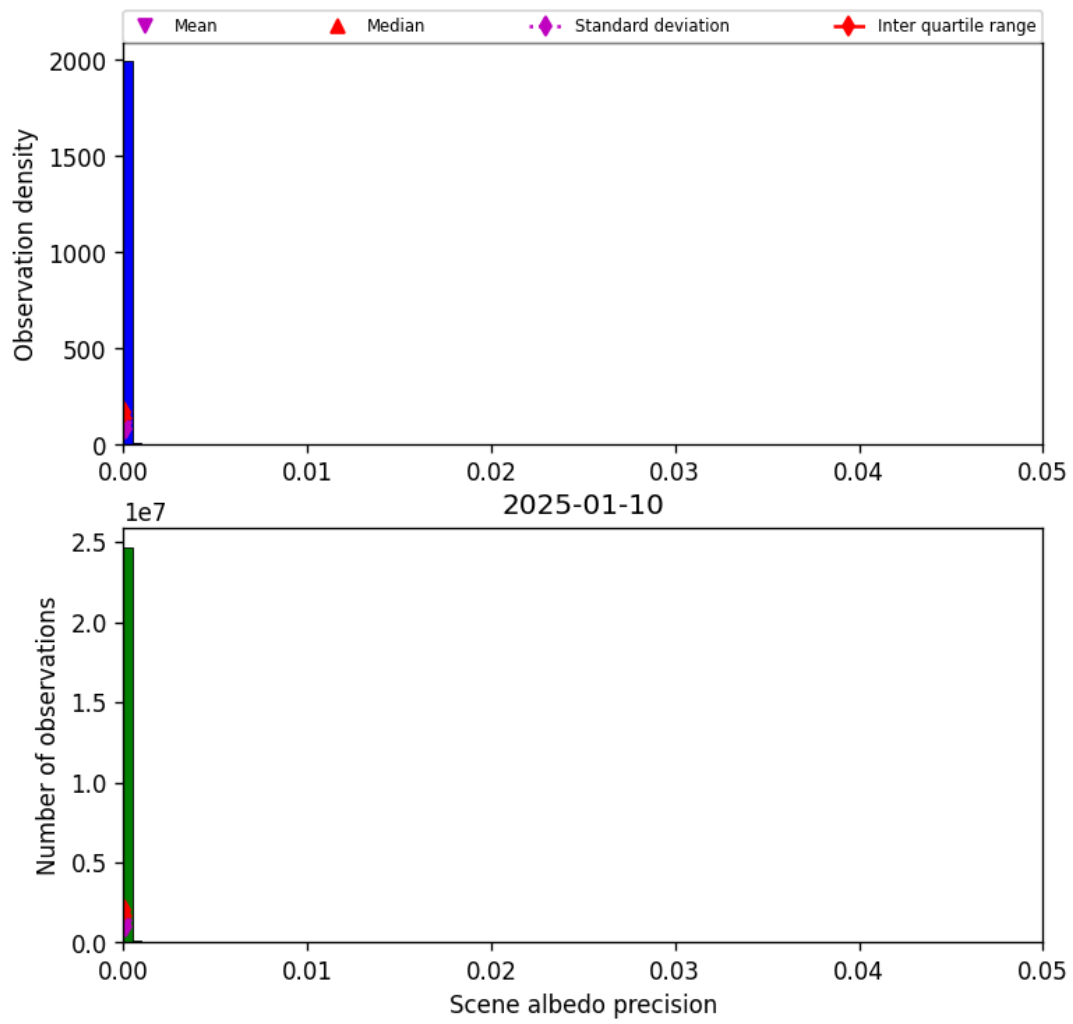
Figure 35: Histogram of “Scene albedo precision” for 2025-01-09 to 2025-01-11
