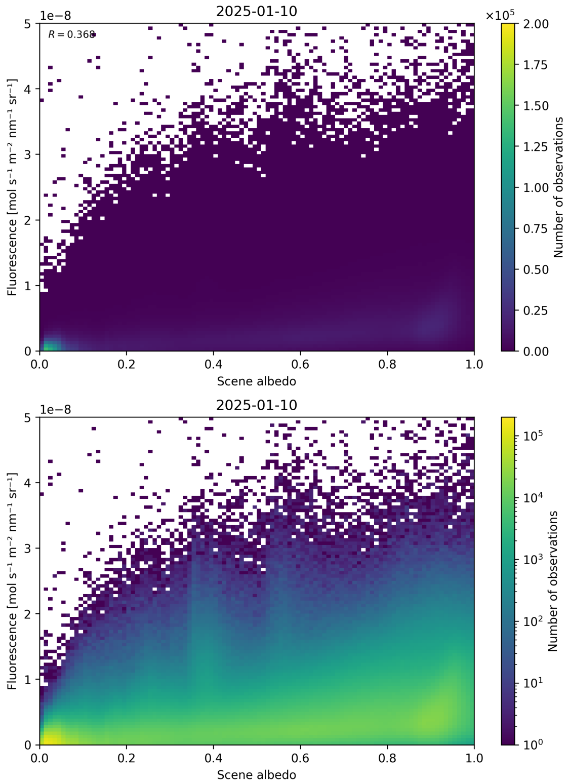
Figure 104: Scatter density plot of “Scene albedo” against “Fluorescence” for 2025-01-09 to 2025-01-11.
