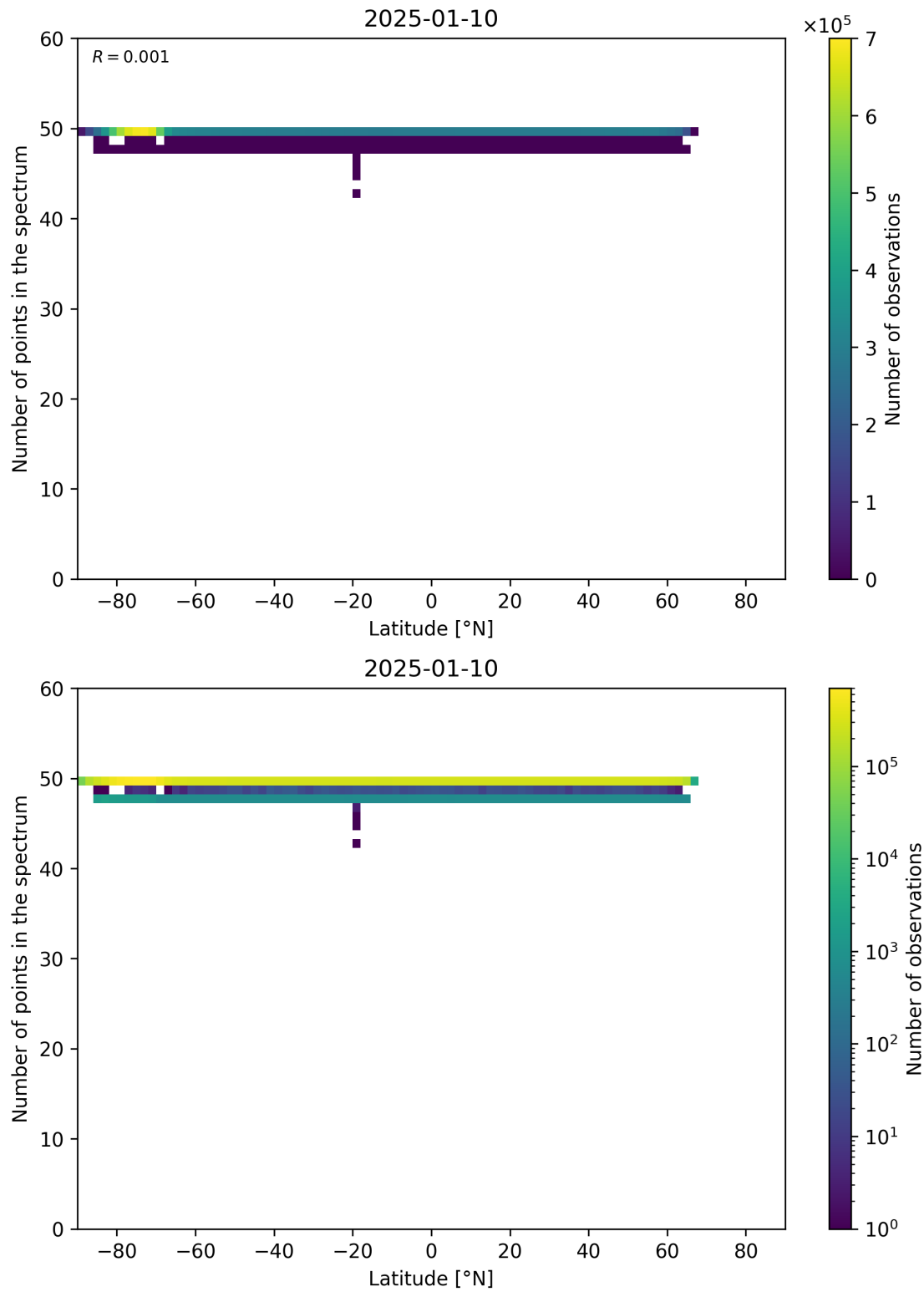
Figure 94: Scatter density plot of “Latitude” against “Number of points in the spectrum” for 2025-01-09 to 2025-01-11.
