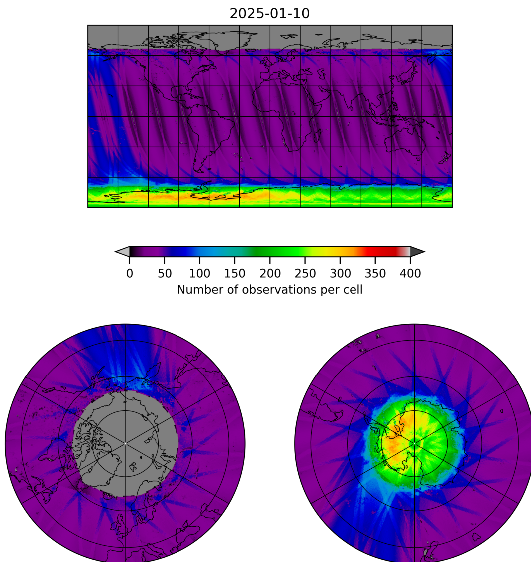
Figure 11: Map of the number of observations for 2025-01-09 to 2025-01-11
