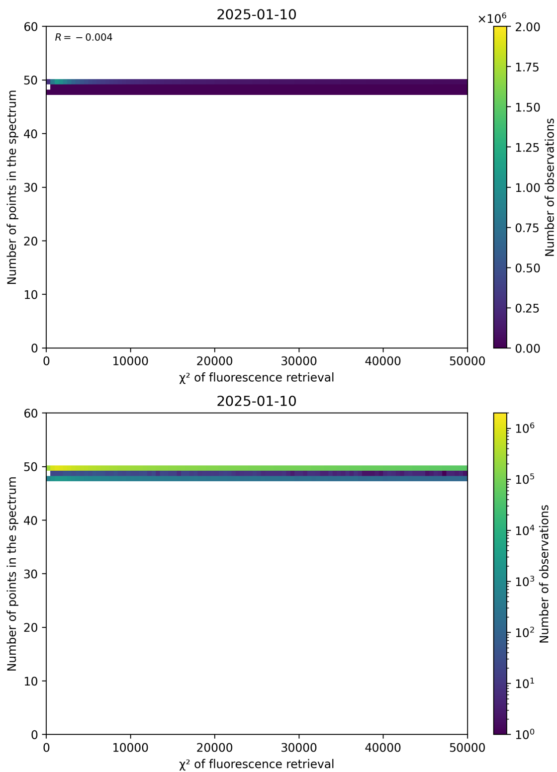
Figure 68: Scatter density plot of “ \chi^2 of fluorescence retrieval” against “Number of points in the spectrum” for 2025-01-09 to 2025-01-11.
