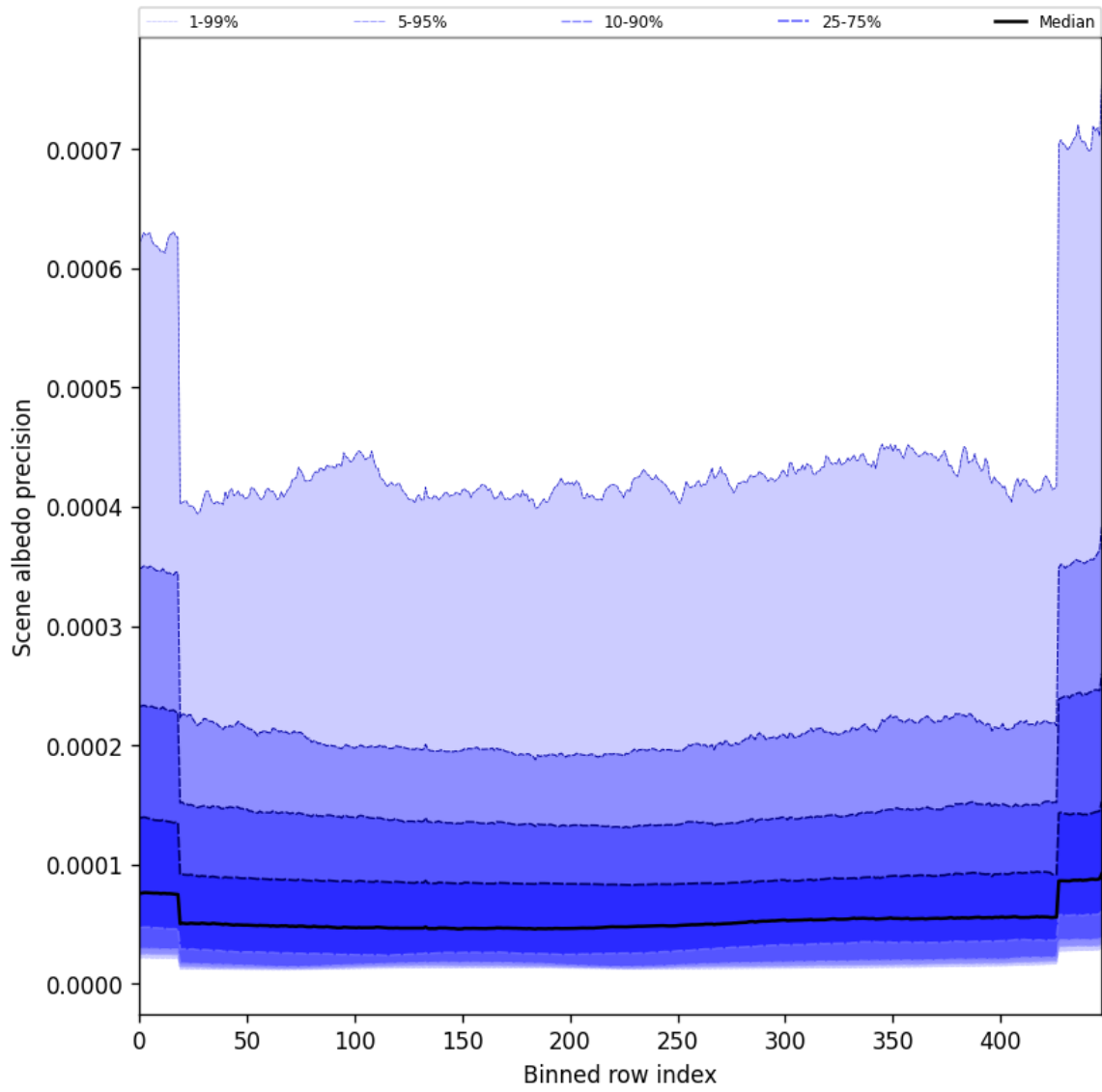
Figure 52: Along track statistics of “Scene albedo precision” for 2025-01-09 to 2025-01-11
