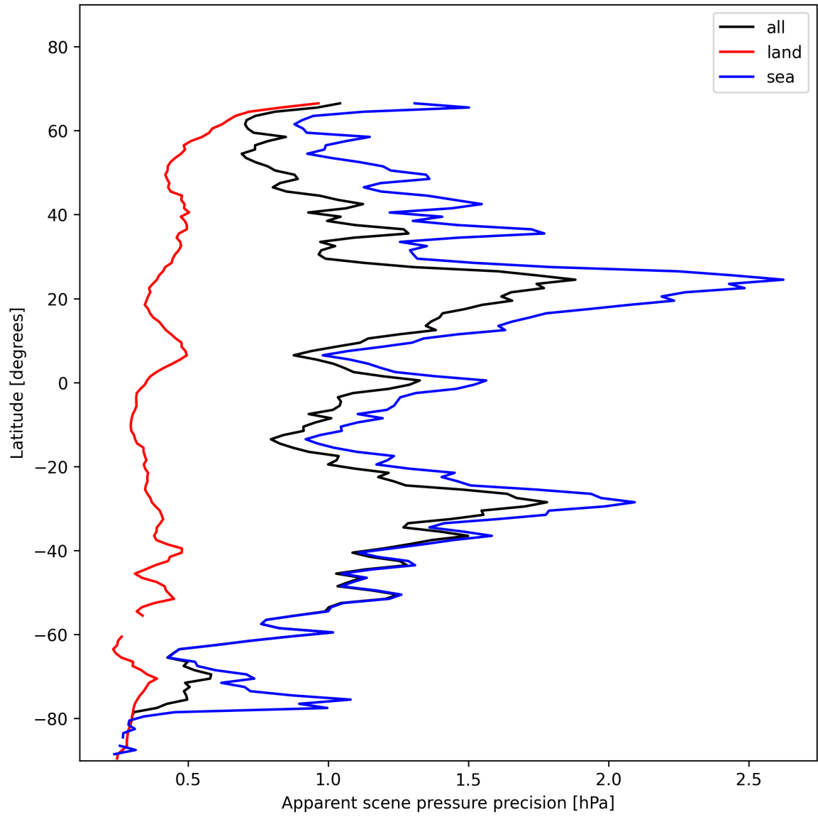
Figure 20: Zonal average of “Apparent scene pressure precision” for 2025-01-09 to 2025-01-11.
