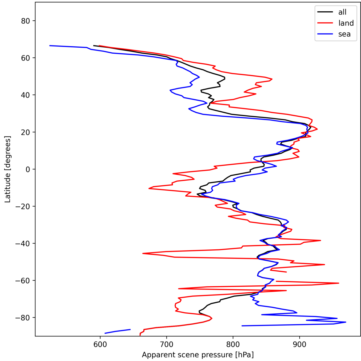
Figure 19: Zonal average of “Apparent scene pressure” for 2025-01-09 to 2025-01-11.
