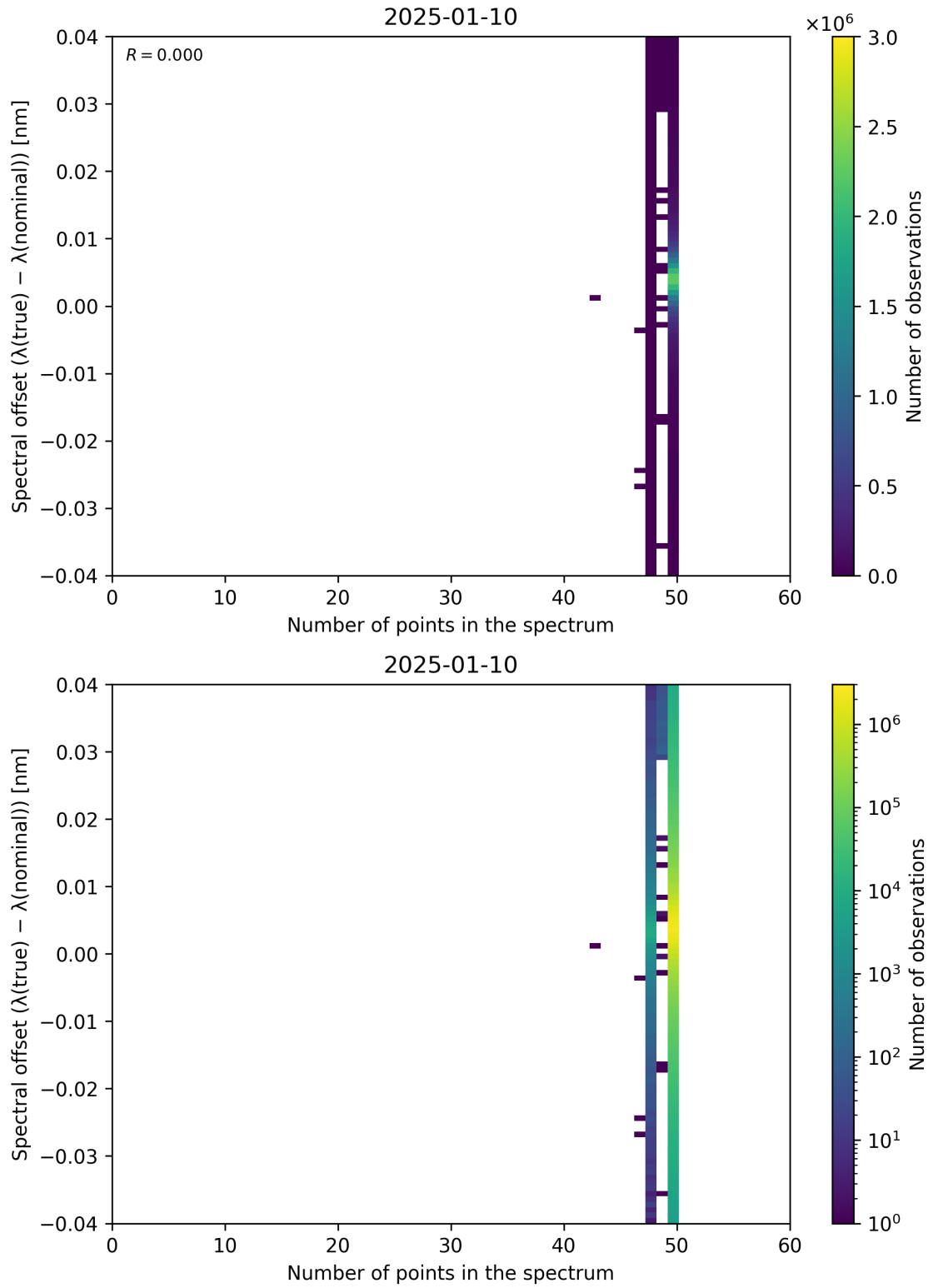
Figure 101: Scatter density plot of “Number of points in the spectrum” against “Spectral offset ( \lambda_{\text{true}} - \lambda_{\text{nominal}} )” for 2025-01-09 to 2025-01-11.
