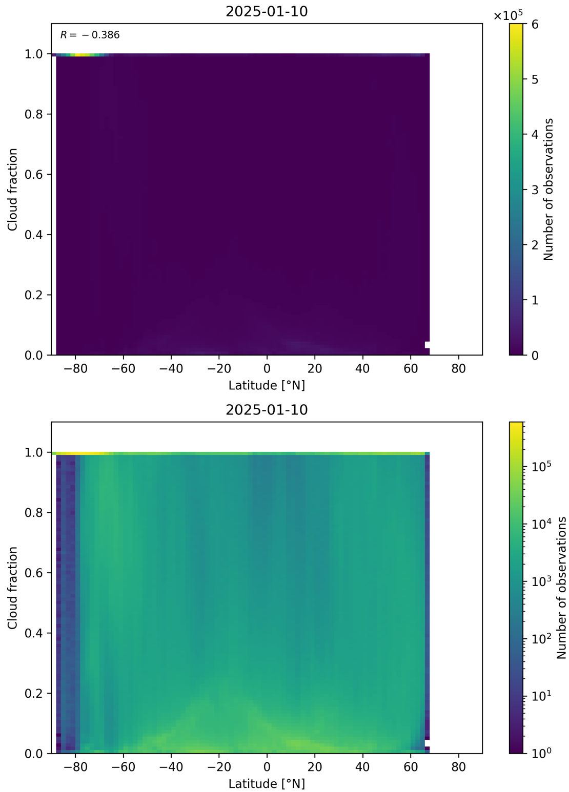
Figure 90: Scatter density plot of “Latitude” against “Cloud fraction” for 2025-01-09 to 2025-01-11.
