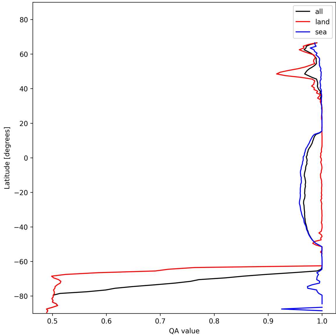
Figure 12: Zonal average of “QA value” for 2025-01-09 to 2025-01-11.
