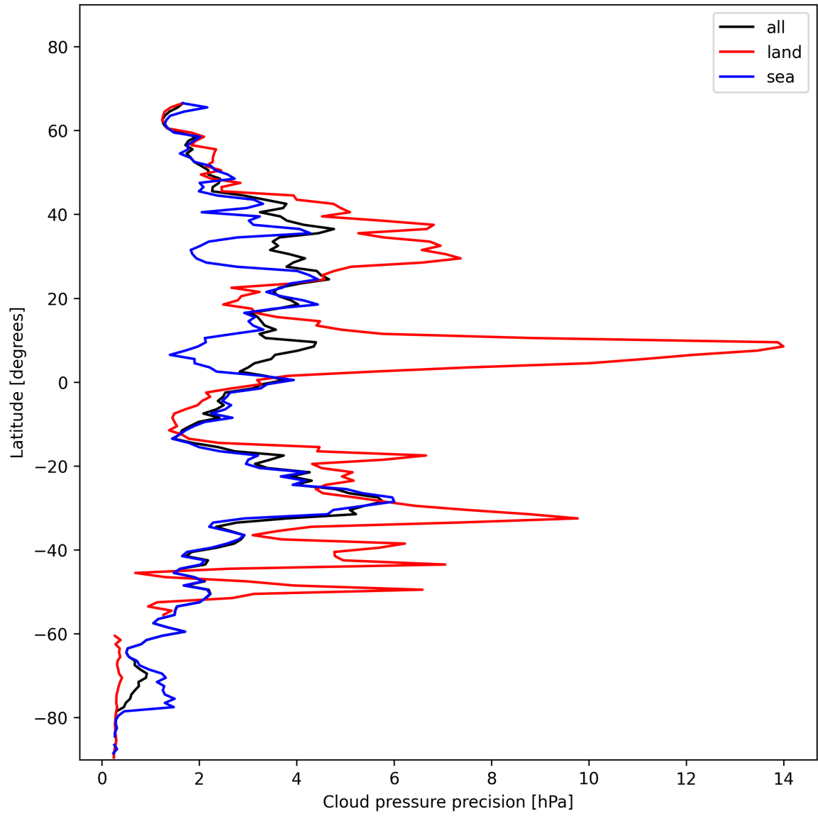
Figure 14: Zonal average of “Cloud pressure precision” for 2025-01-09 to 2025-01-11.
