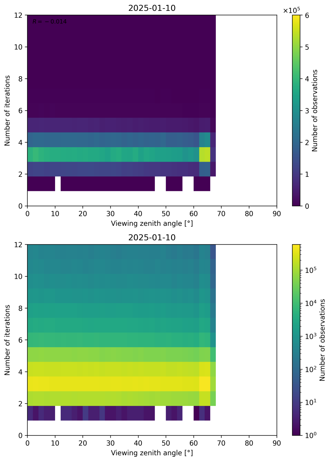
Figure 124: Scatter density plot of “Viewing zenith angle” against “Number of iterations” for 2025-01-09 to 2025-01-11.
