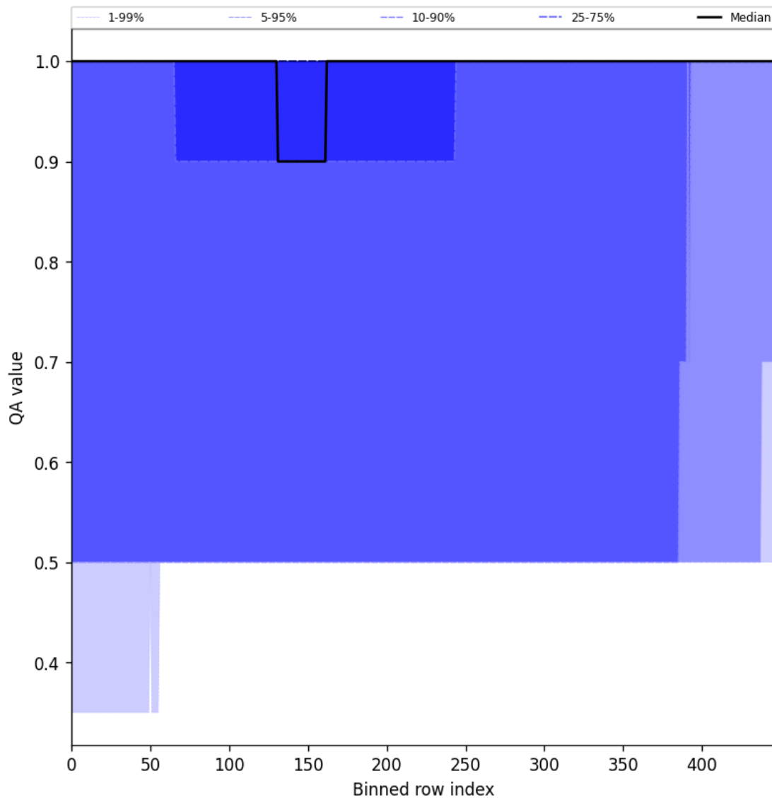
Figure 46: Along track statistics of “QA value” for 2025-01-09 to 2025-01-11
