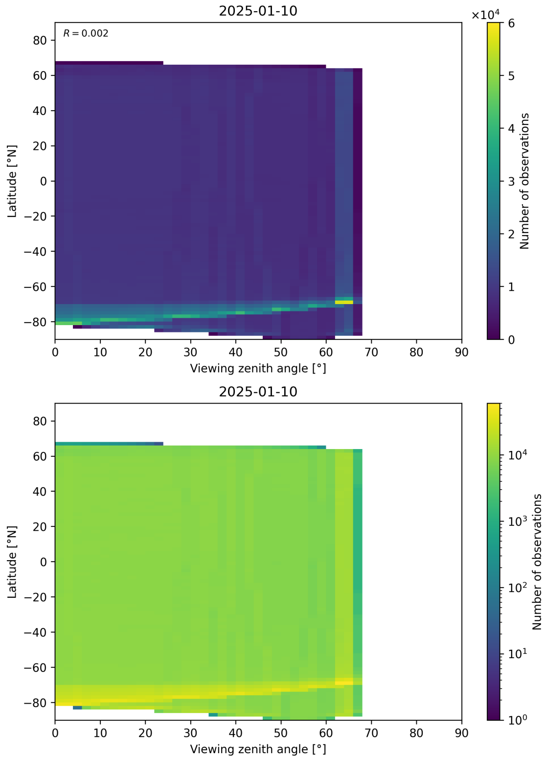
Figure 123: Scatter density plot of “Viewing zenith angle” against “Latitude” for 2025-01-09 to 2025-01-11.
