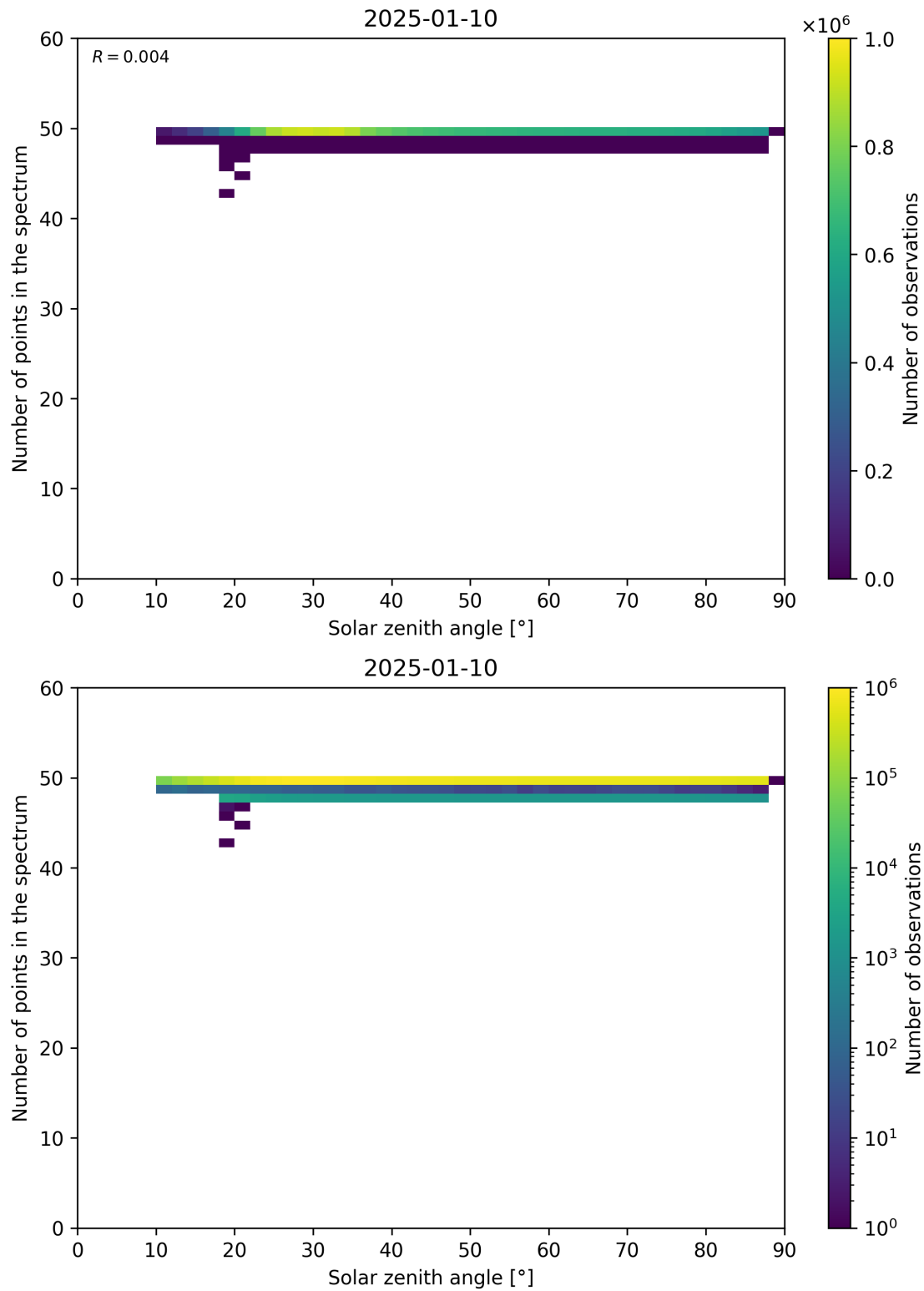
Figure 115: Scatter density plot of “Solar zenith angle” against “Number of points in the spectrum” for 2025-01-09 to 2025-01-11.
