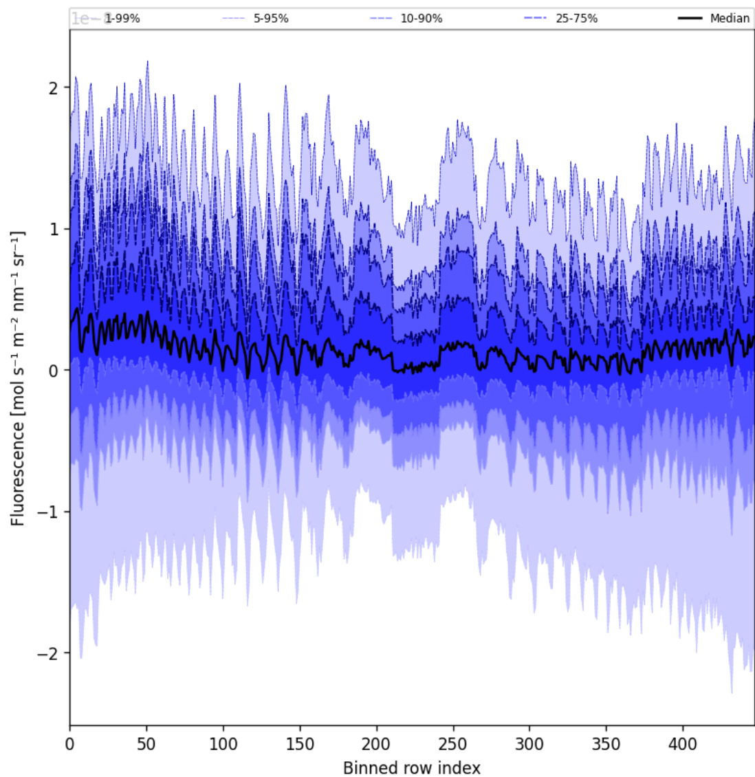
Figure 57: Along track statistics of “Fluorescence” for 2025-01-09 to 2025-01-11
