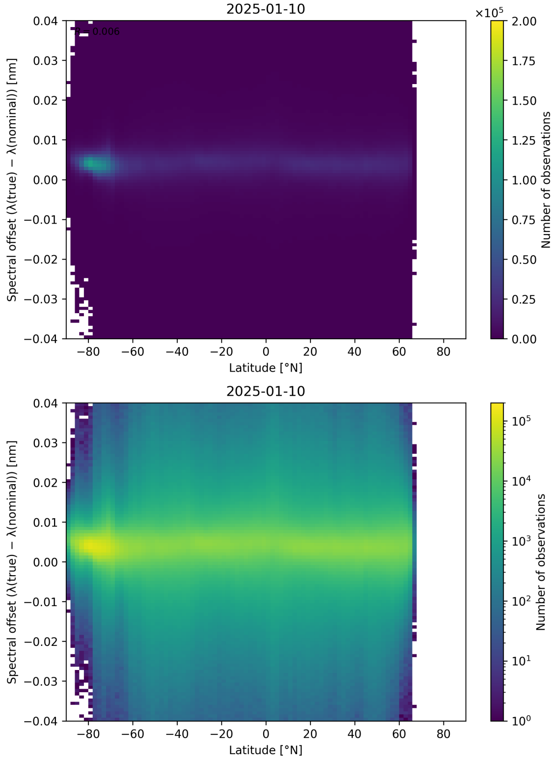
Figure 96: Scatter density plot of “Latitude” against “Spectral offset ( \lambda_{\text{true}} - \lambda_{\text{nominal}} )” for 2025-01-09 to 2025-01-11.
