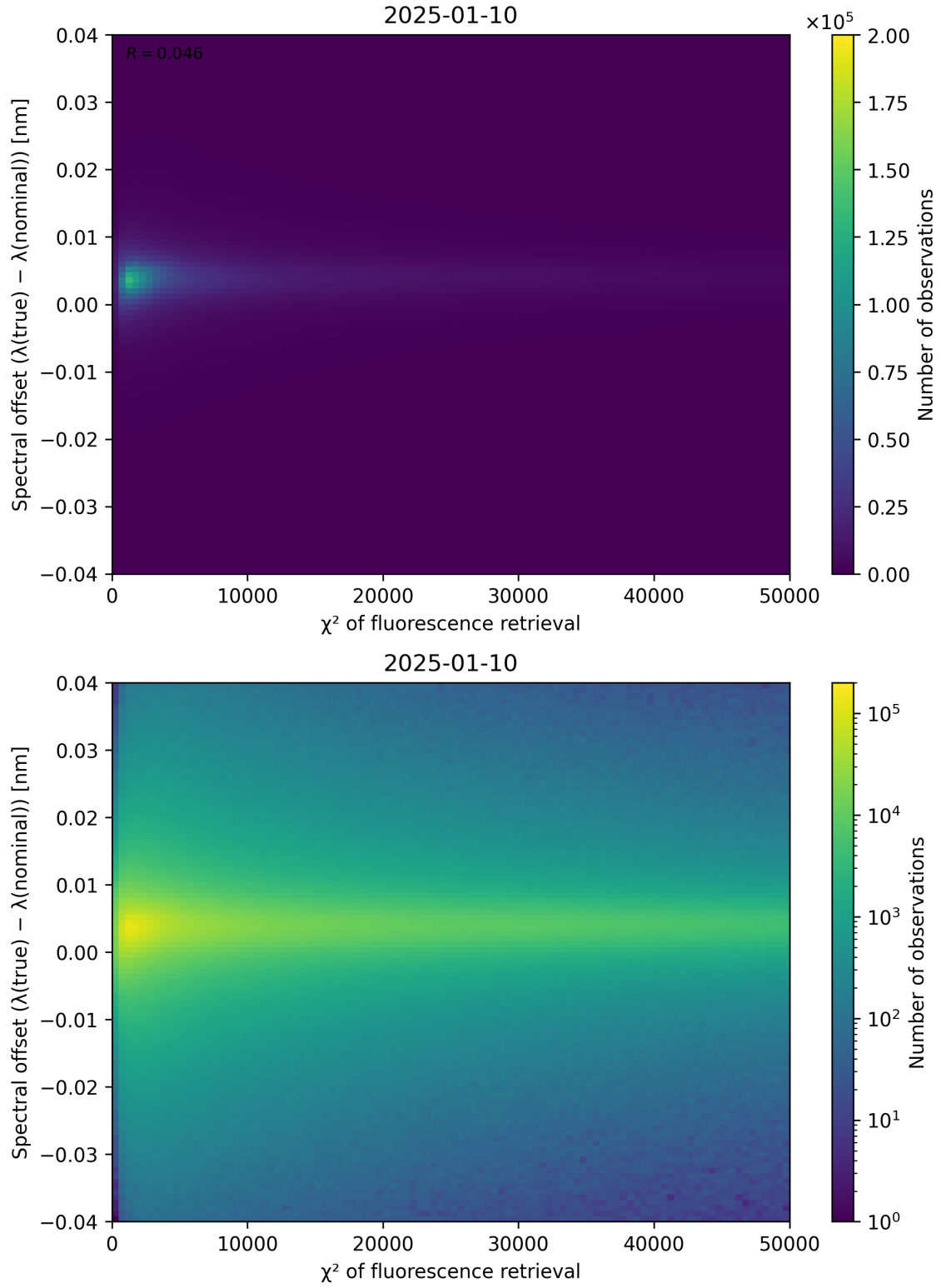
Figure 69: Scatter density plot of “ \chi^2 of fluorescence retrieval” against “Spectral offset ( \lambda_{\text{true}} - \lambda_{\text{nominal}} )” for 2025-01-09 to 2025-01-11.
