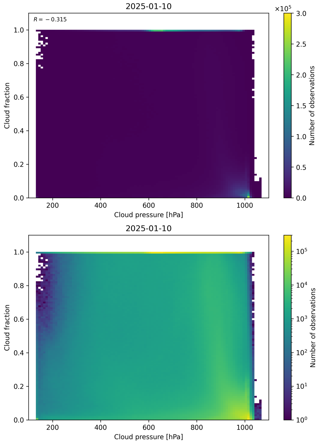
Figure 79: Scatter density plot of “Cloud pressure” against “Cloud fraction” for 2025-01-09 to 2025-01-11.
