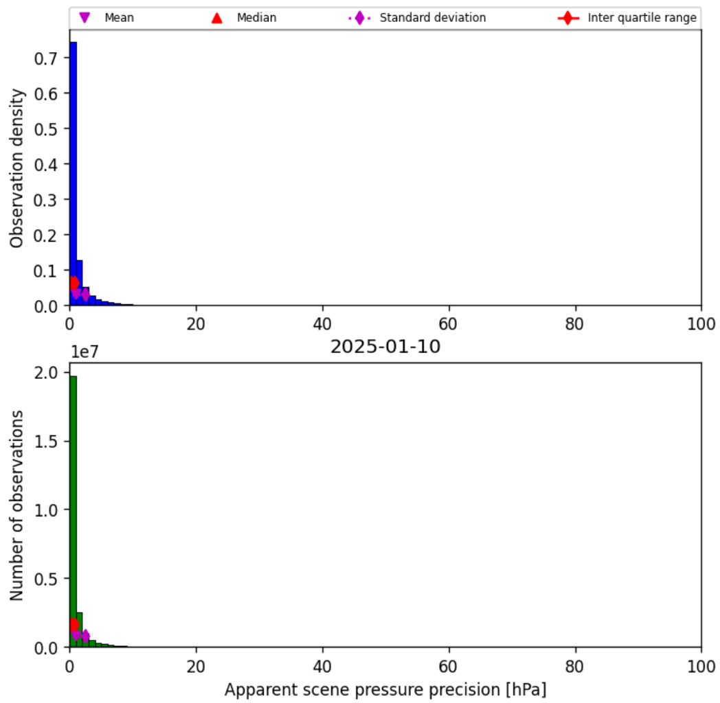
Figure 37: Histogram of “Apparent scene pressure precision” for 2025-01-09 to 2025-01-11
