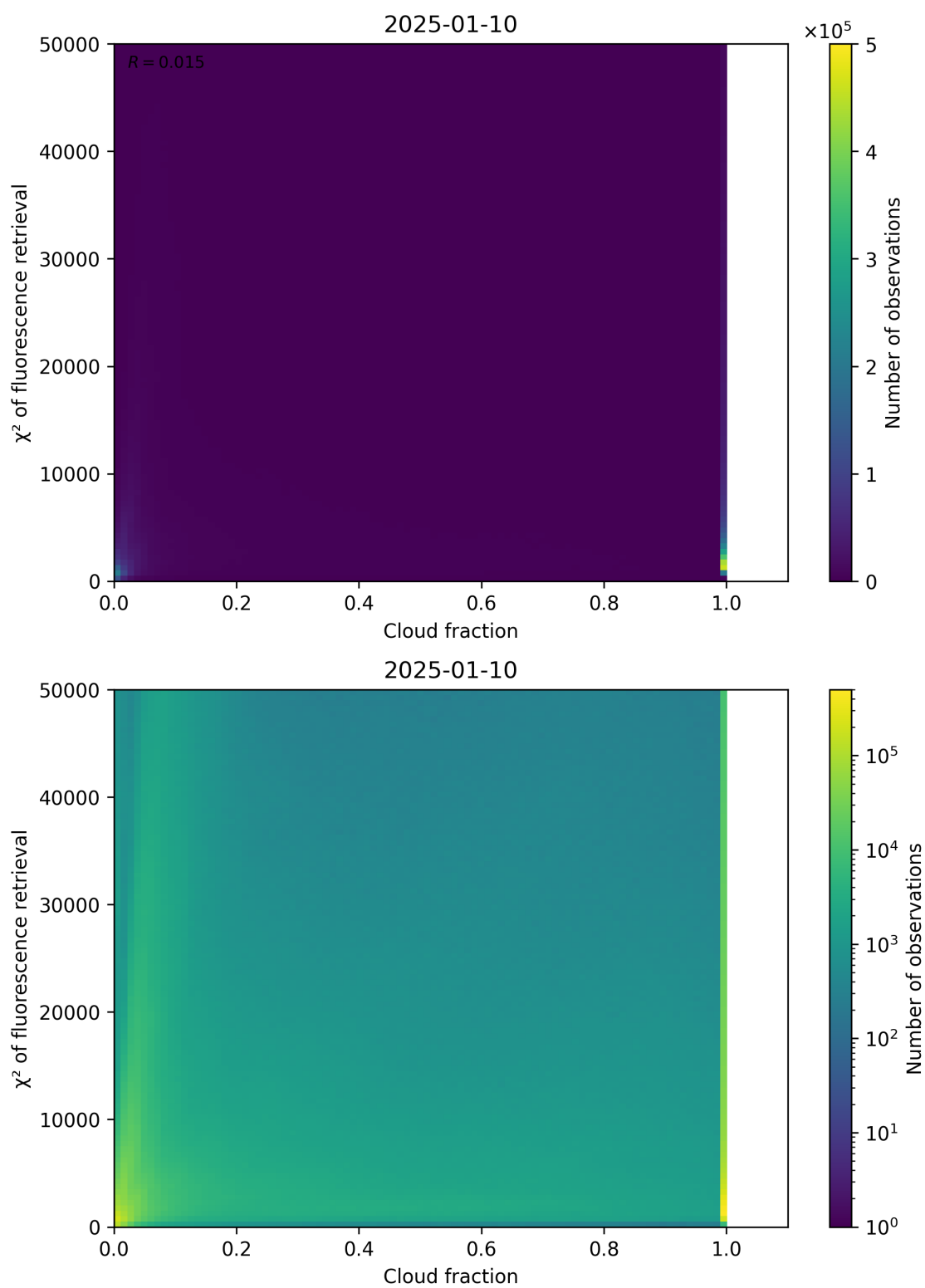
Figure 71: Scatter density plot of “Cloud fraction” against “ \chi^2 of fluorescence retrieval” for 2025-01-09 to 2025-01-11.
