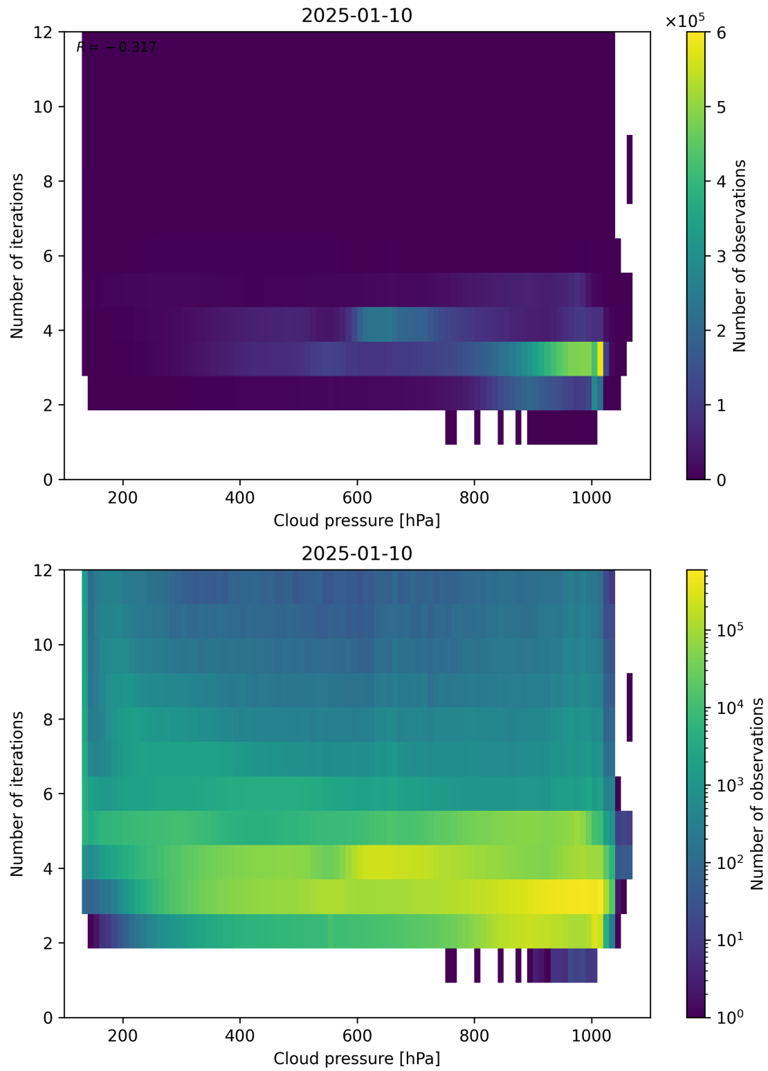
Figure 81: Scatter density plot of “Cloud pressure” against “Number of iterations” for 2025-01-09 to 2025-01-11.
