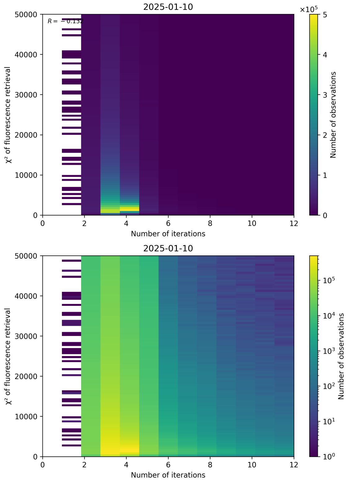
Figure 97: Scatter density plot of “Number of iterations” against “ \chi^2 of fluorescence retrieval” for 2025-01-09 to 2025-01-11.
