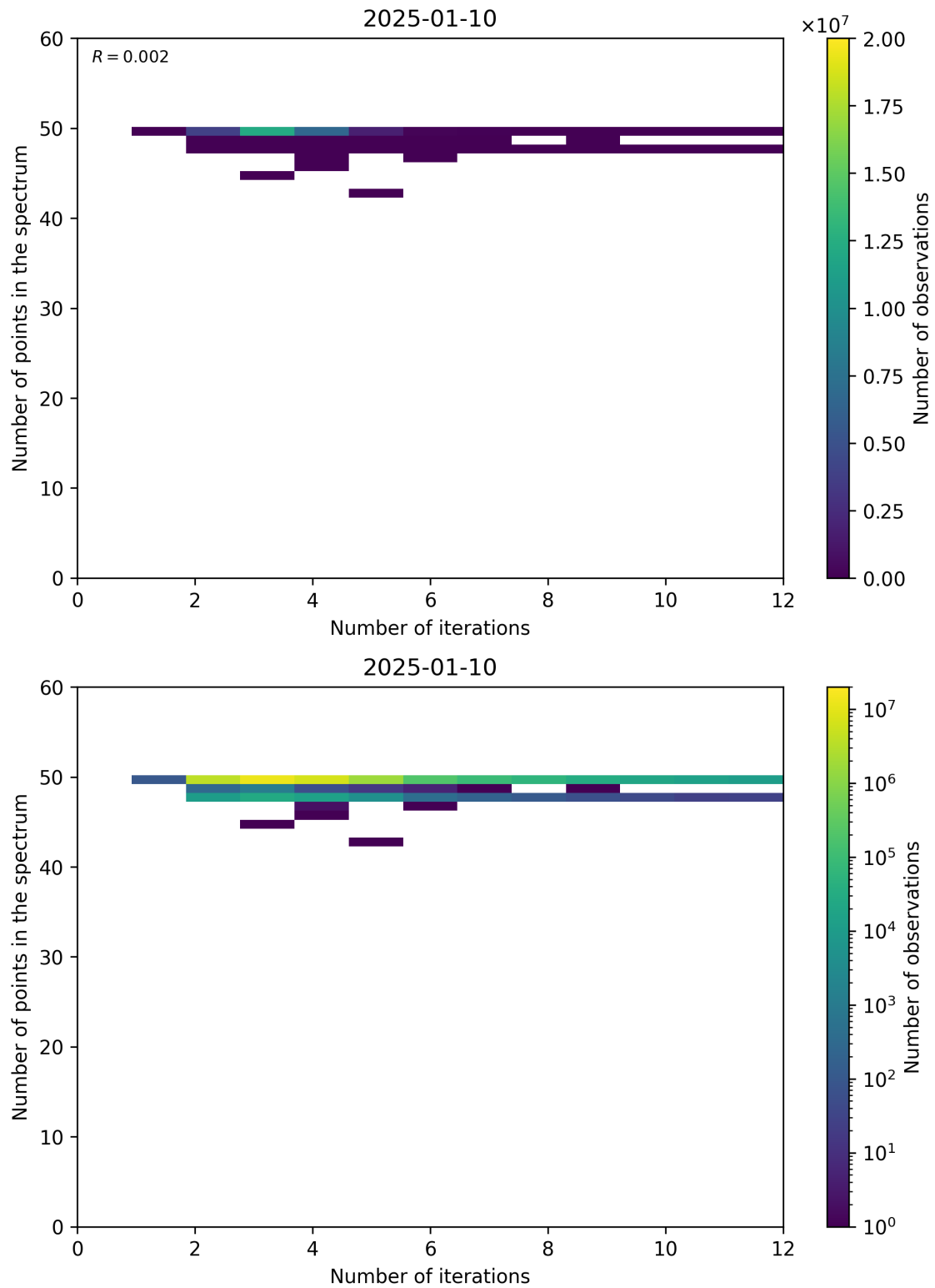
Figure 99: Scatter density plot of “Number of iterations” against “Number of points in the spectrum” for 2025-01-09 to 2025-01-11.
