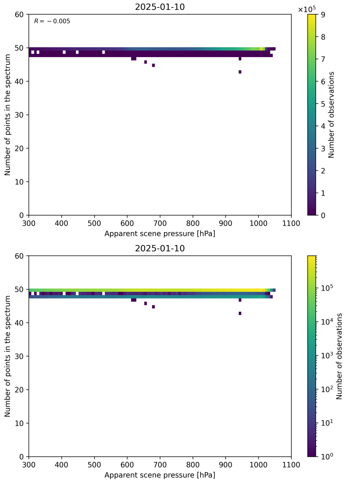
Figure 66: Scatter density plot of “Apparent scene pressure” against “Number of points in the spectrum” for 2025-01-09 to 2025-01-11.
