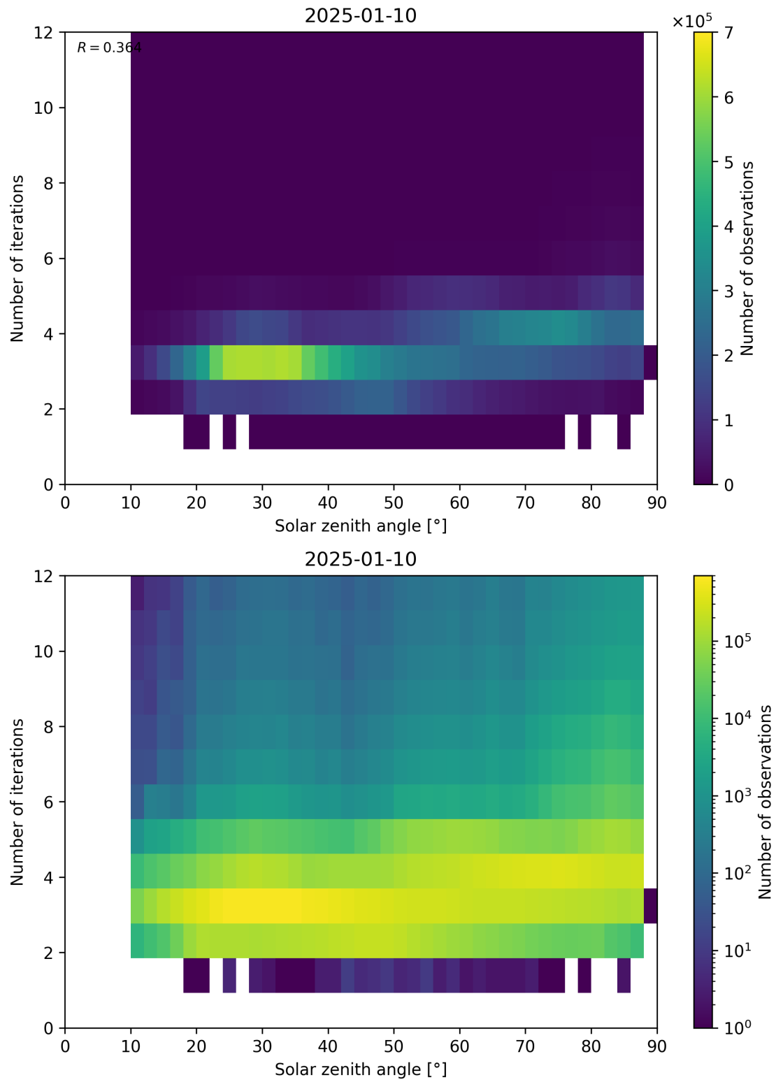
Figure 114: Scatter density plot of “Solar zenith angle” against “Number of iterations” for 2025-01-09 to 2025-01-11.
