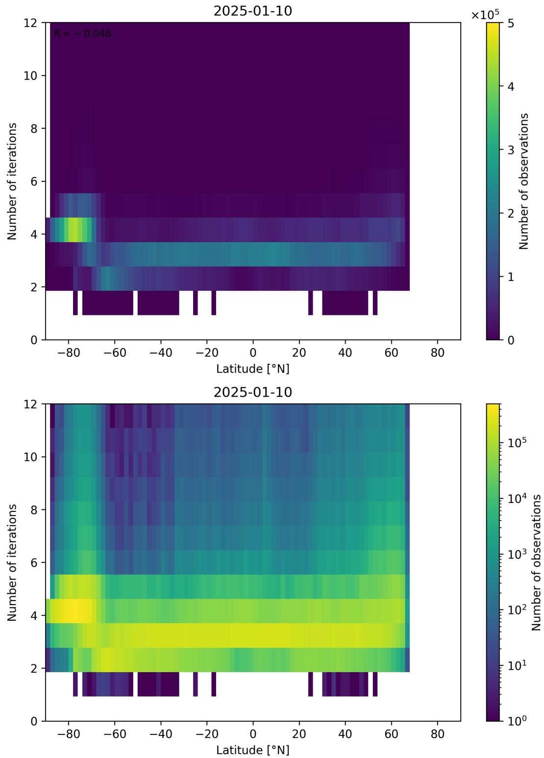
Figure 93: Scatter density plot of “Latitude” against “Number of iterations” for 2025-01-09 to 2025-01-11.
