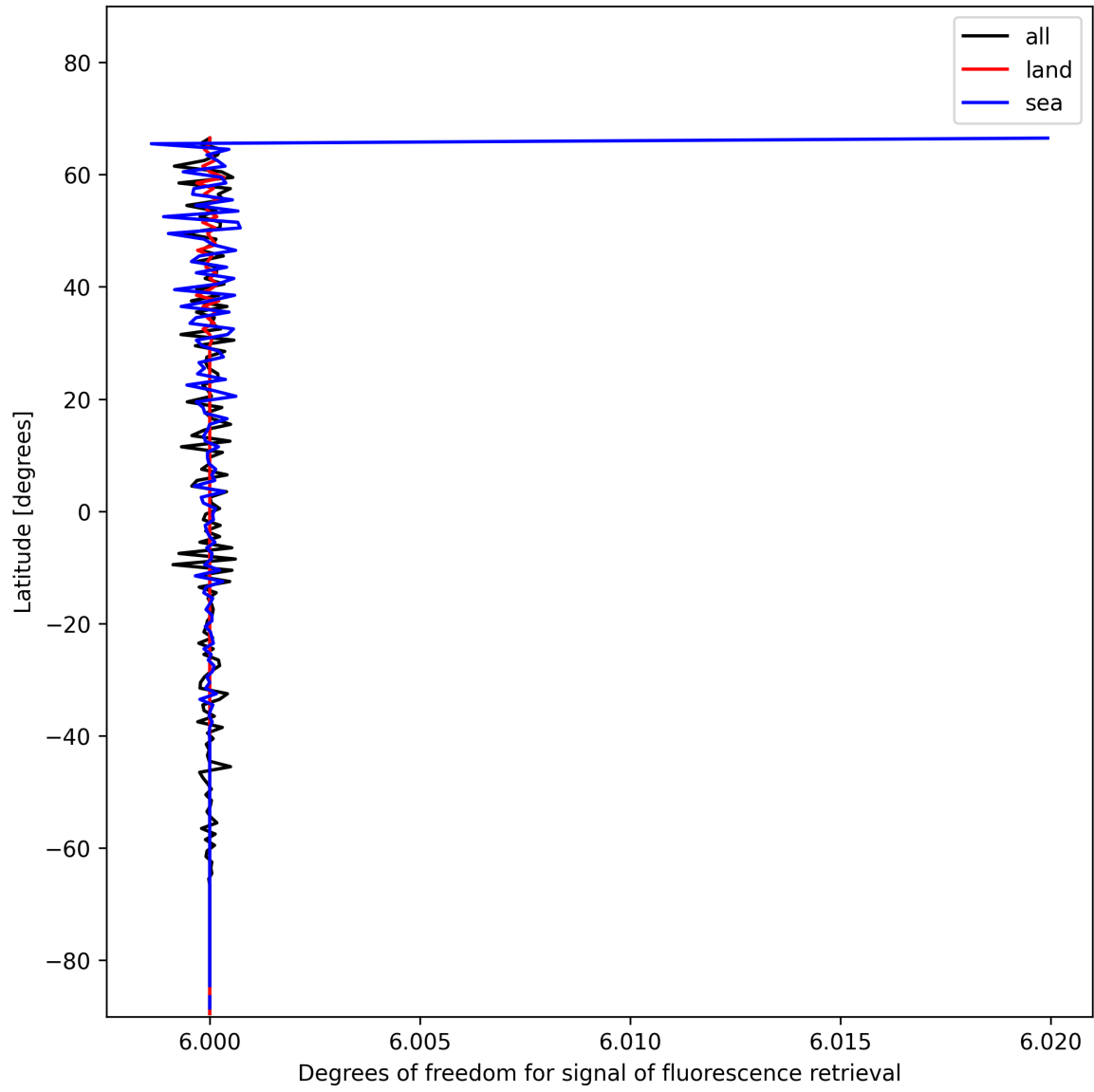
Figure 26: Zonal average of “Degrees of freedom for signal of fluorescence retrieval” for 2025-01-09 to 2025-01-11.
