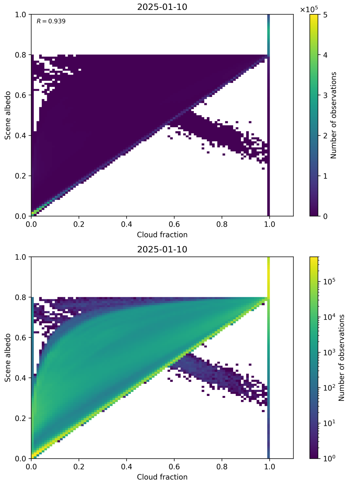
Figure 75: Scatter density plot of “Cloud fraction” against “Scene albedo” for 2025-01-09 to 2025-01-11.
