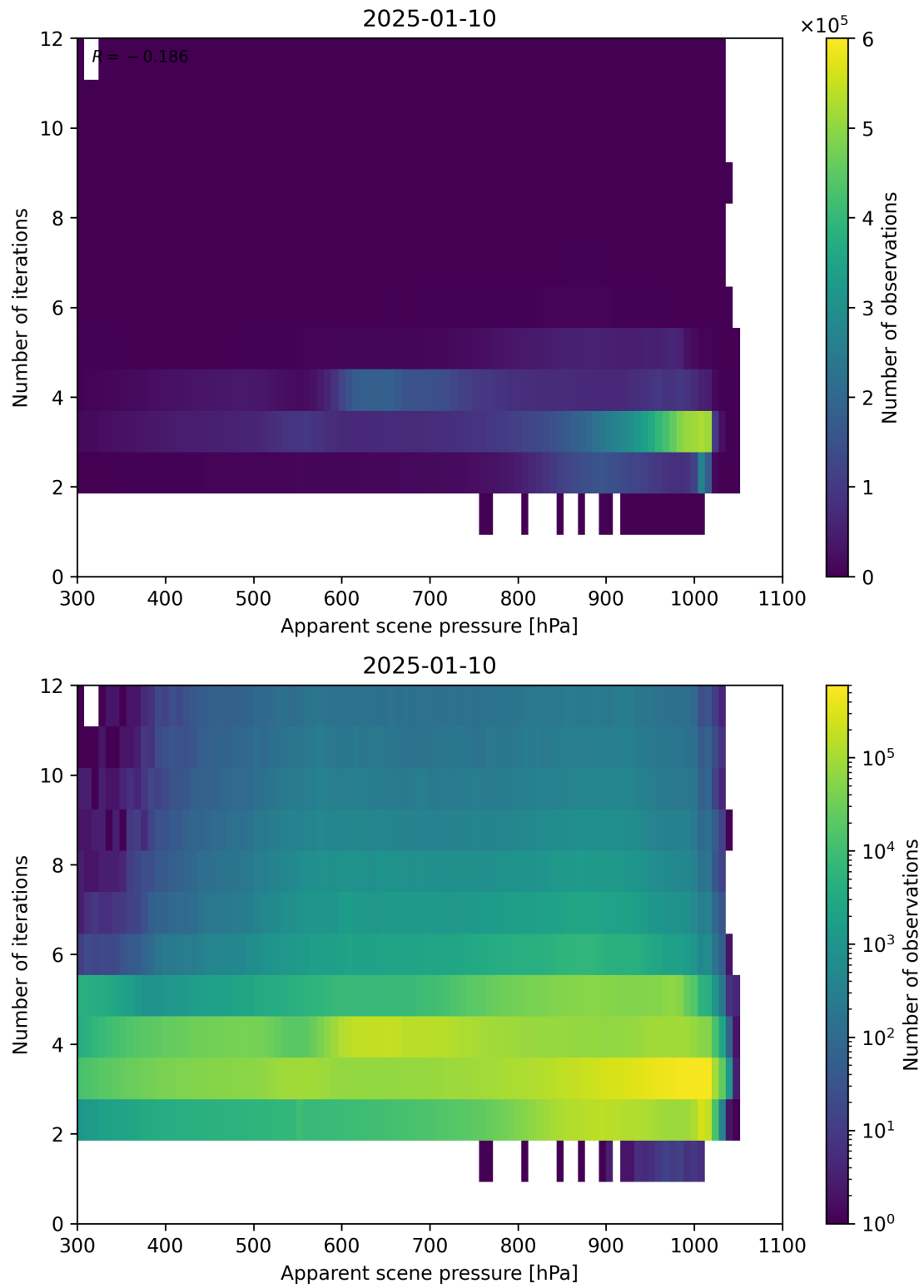
Figure 65: Scatter density plot of “Apparent scene pressure” against “Number of iterations” for 2025-01-09 to 2025-01-11.
