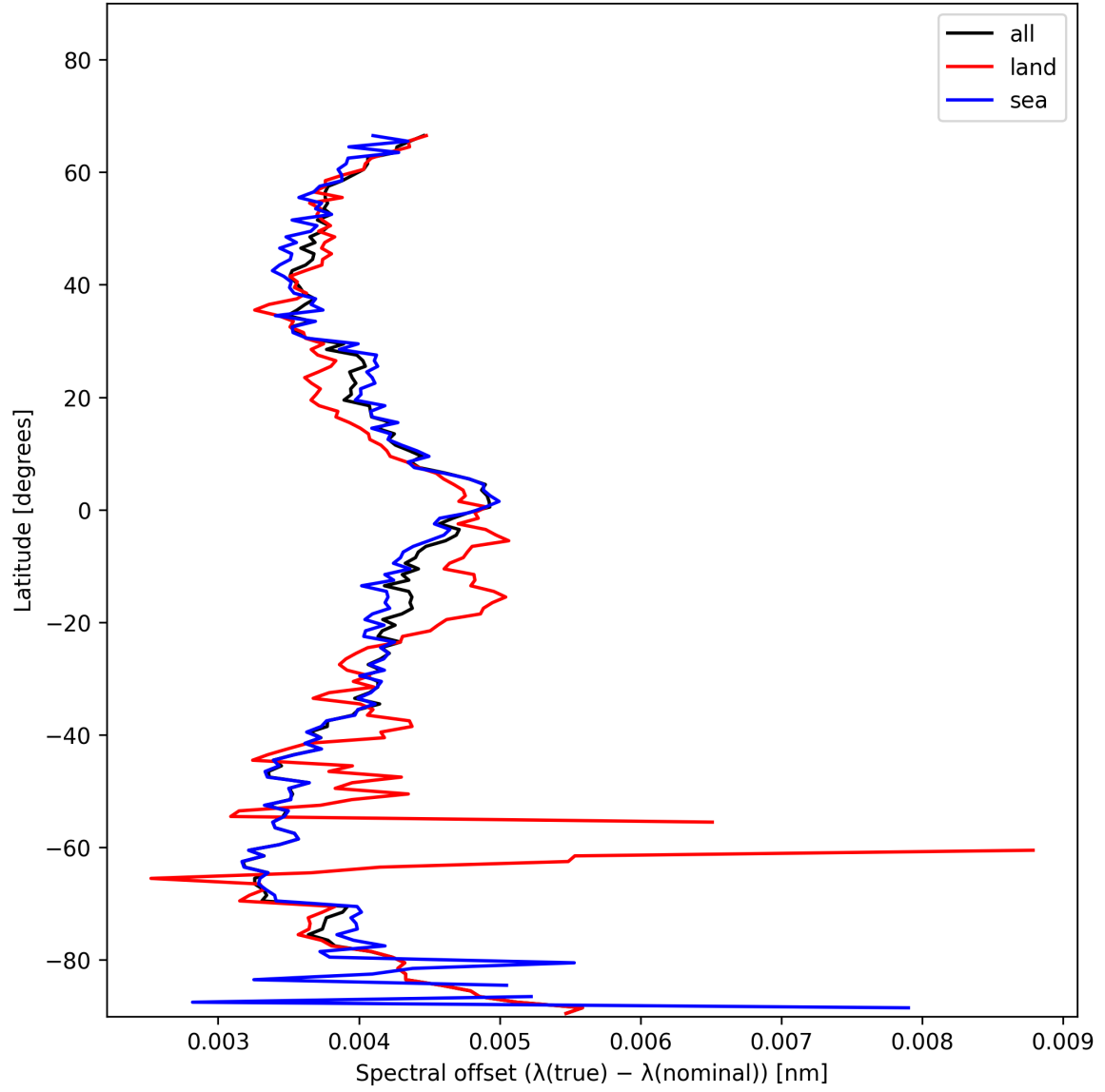
Figure 28: Zonal average of “Spectral offset ( \lambda_{\text{true}} - \lambda_{\text{nominal}} )” for 2025-01-09 to 2025-01-11.
