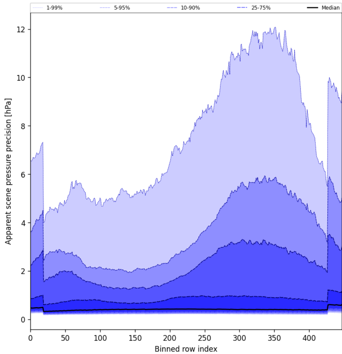
Figure 54: Along track statistics of “Apparent scene pressure precision” for 2025-01-09 to 2025-01-11
