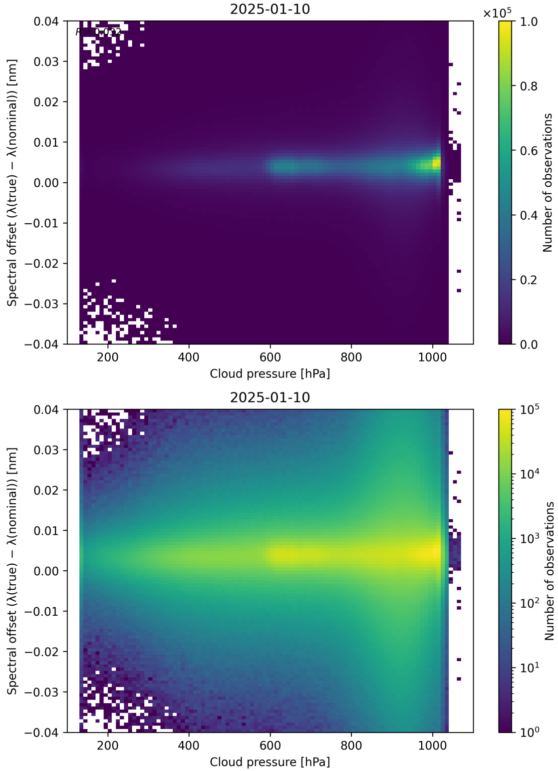
Figure 84: Scatter density plot of “Cloud pressure” against “Spectral offset ( \lambda_{\text{true}} - \lambda_{\text{nominal}} )” for 2025-01-09 to 2025-01-11.
