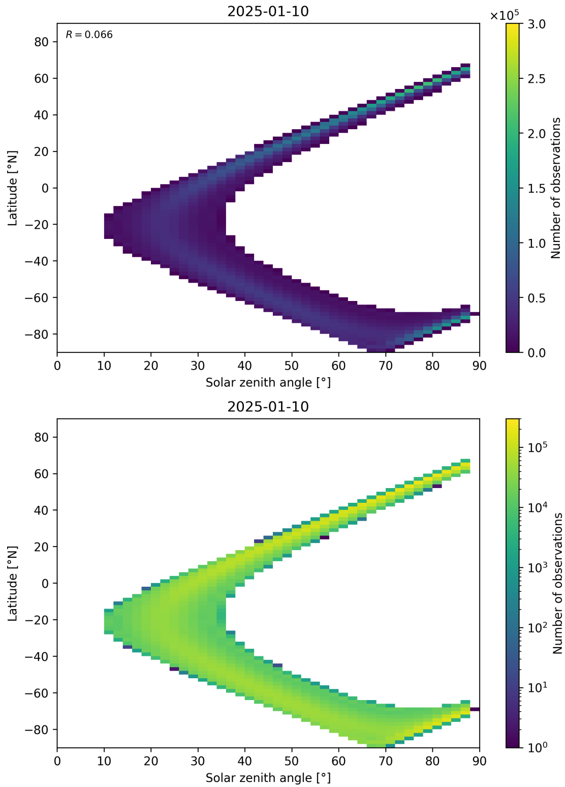
Figure 113: Scatter density plot of “Solar zenith angle” against “Latitude” for 2025-01-09 to 2025-01-11.
