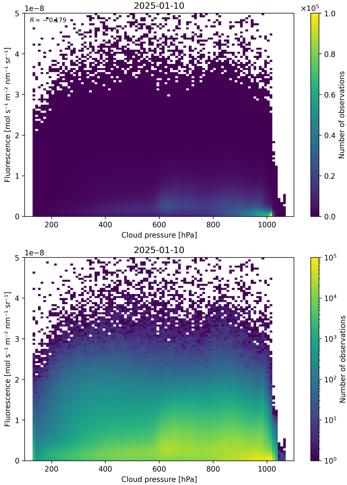
Figure 80: Scatter density plot of “Cloud pressure” against “Fluorescence” for 2025-01-09 to 2025-01-11.
