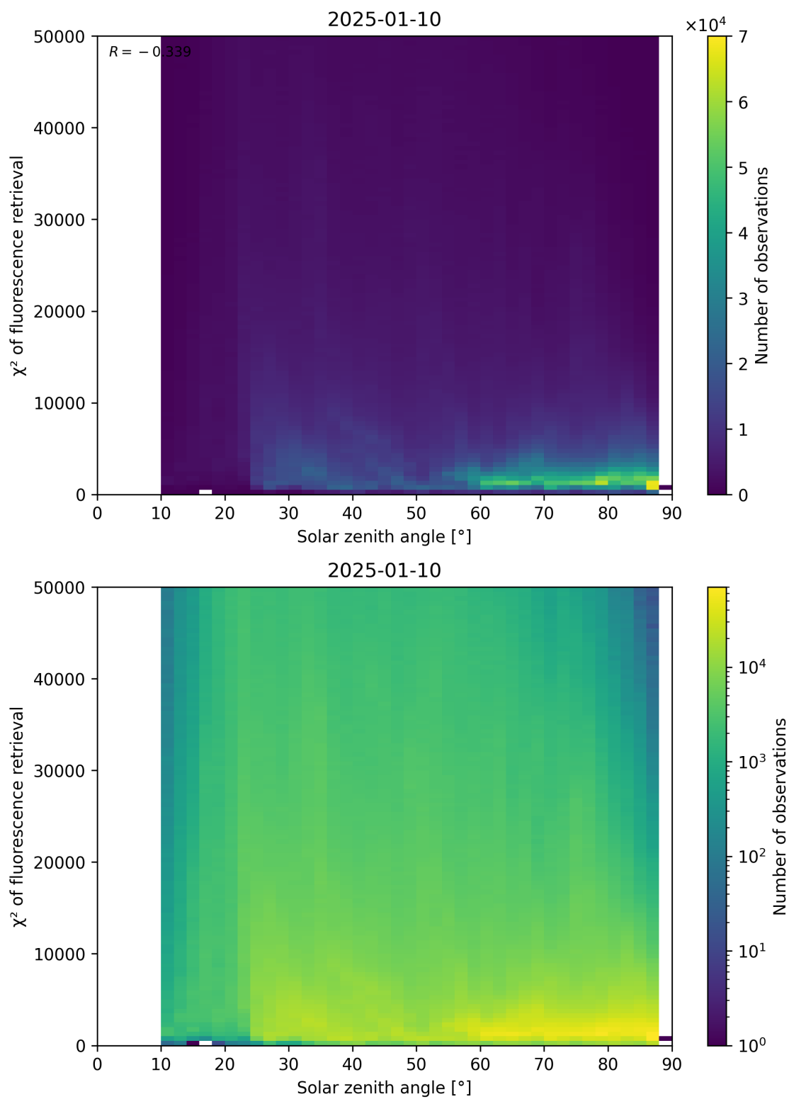
Figure 109: Scatter density plot of “Solar zenith angle” against “ \chi^2 of fluorescence retrieval” for 2025-01-09 to 2025-01-11.
