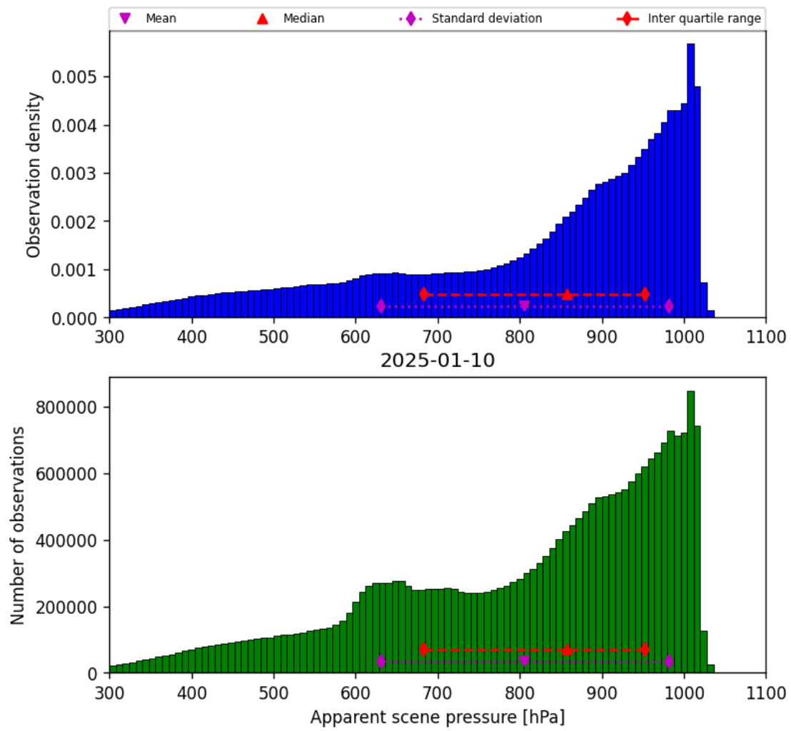
Figure 36: Histogram of “Apparent scene pressure” for 2025-01-09 to 2025-01-11
