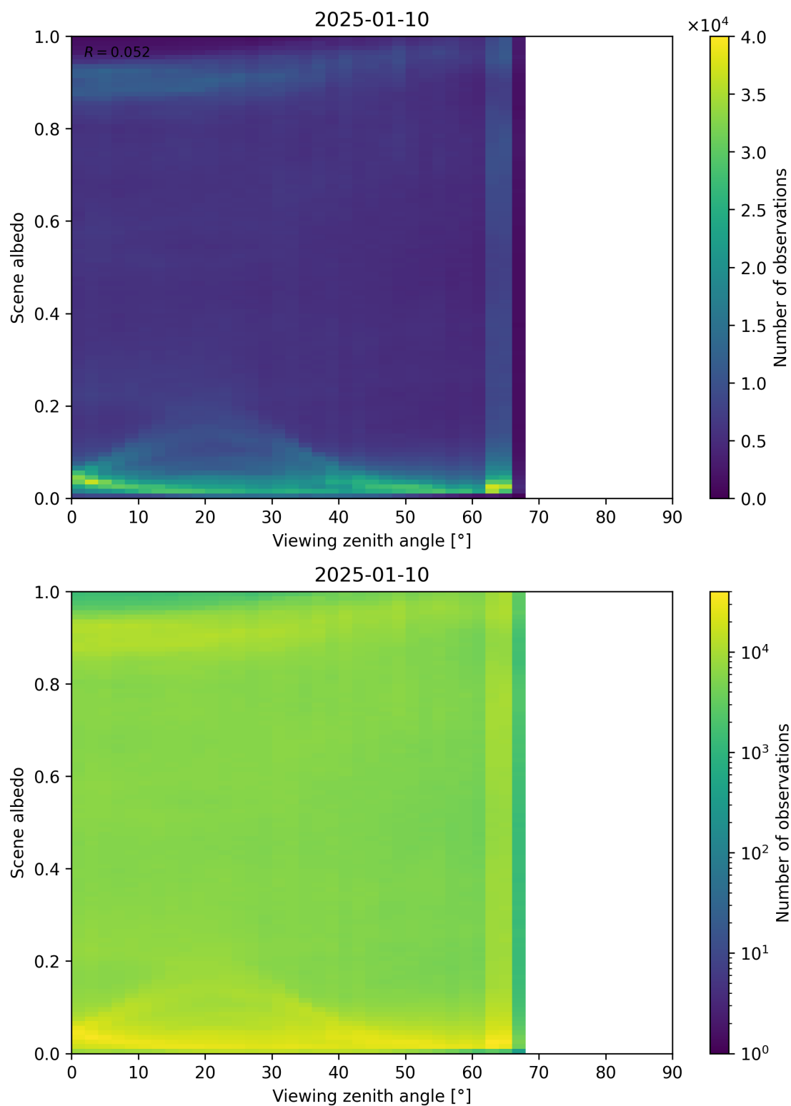
Figure 126: Scatter density plot of “Viewing zenith angle” against “Scene albedo” for 2025-01-09 to 2025-01-11.
