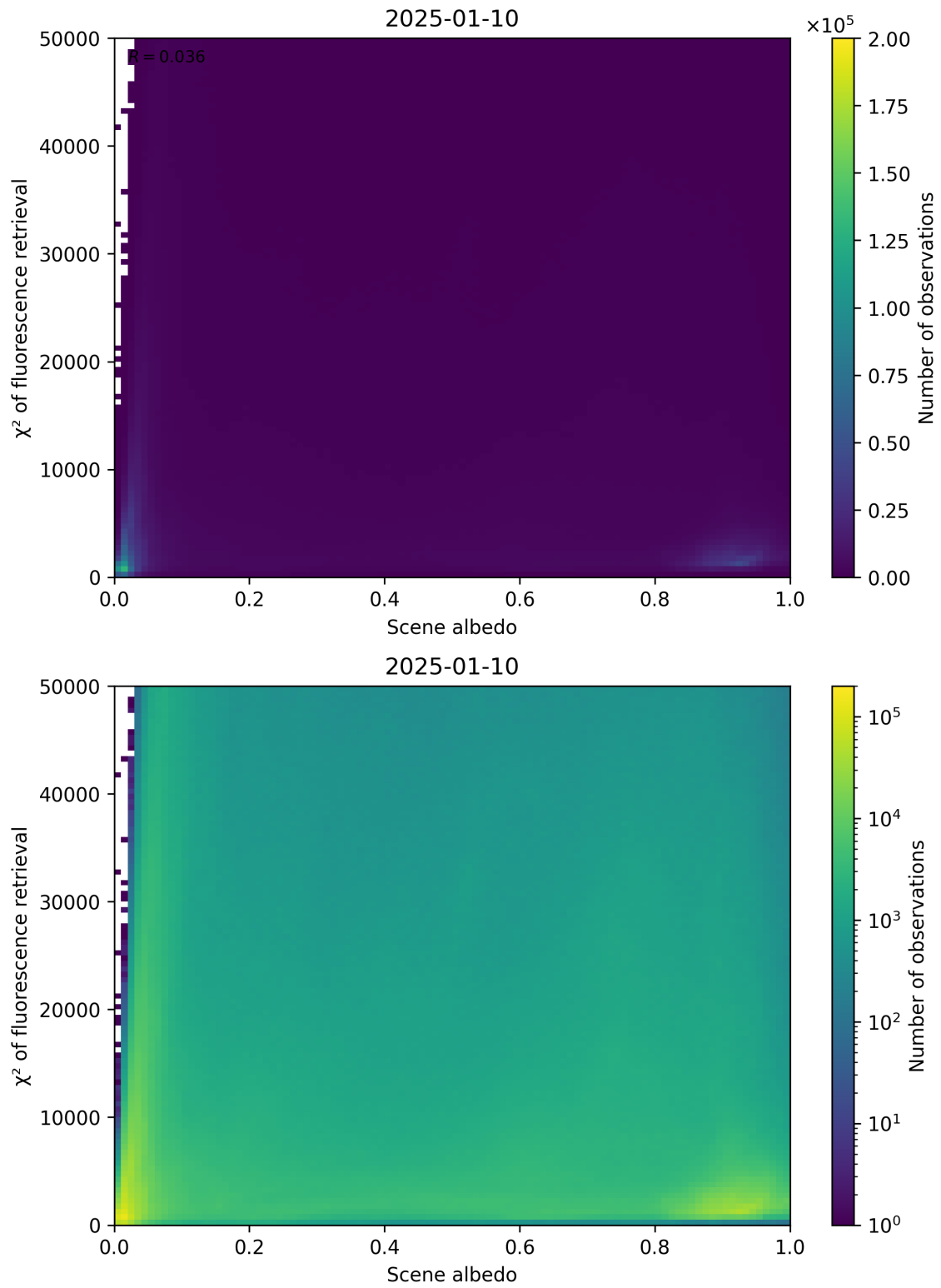
Figure 103: Scatter density plot of “Scene albedo” against “ \chi^2 of fluorescence retrieval” for 2025-01-09 to 2025-01-11.
