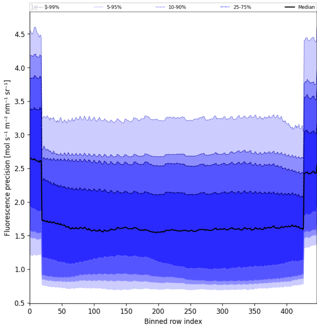
Figure 58: Along track statistics of “Fluorescence precision” for 2025-01-09 to 2025-01-11
