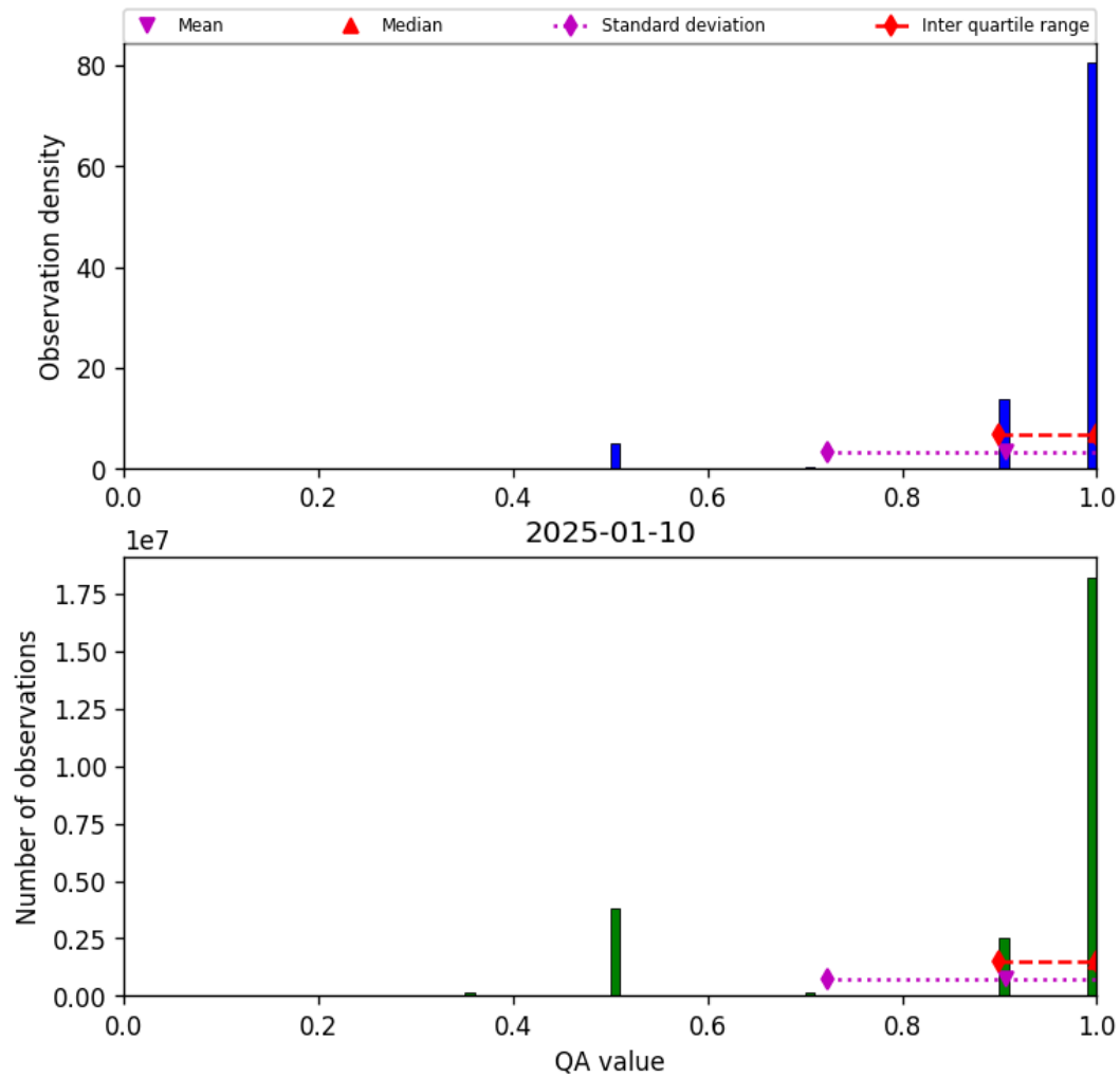
Figure 29: Histogram of “QA value” for 2025-01-09 to 2025-01-11
