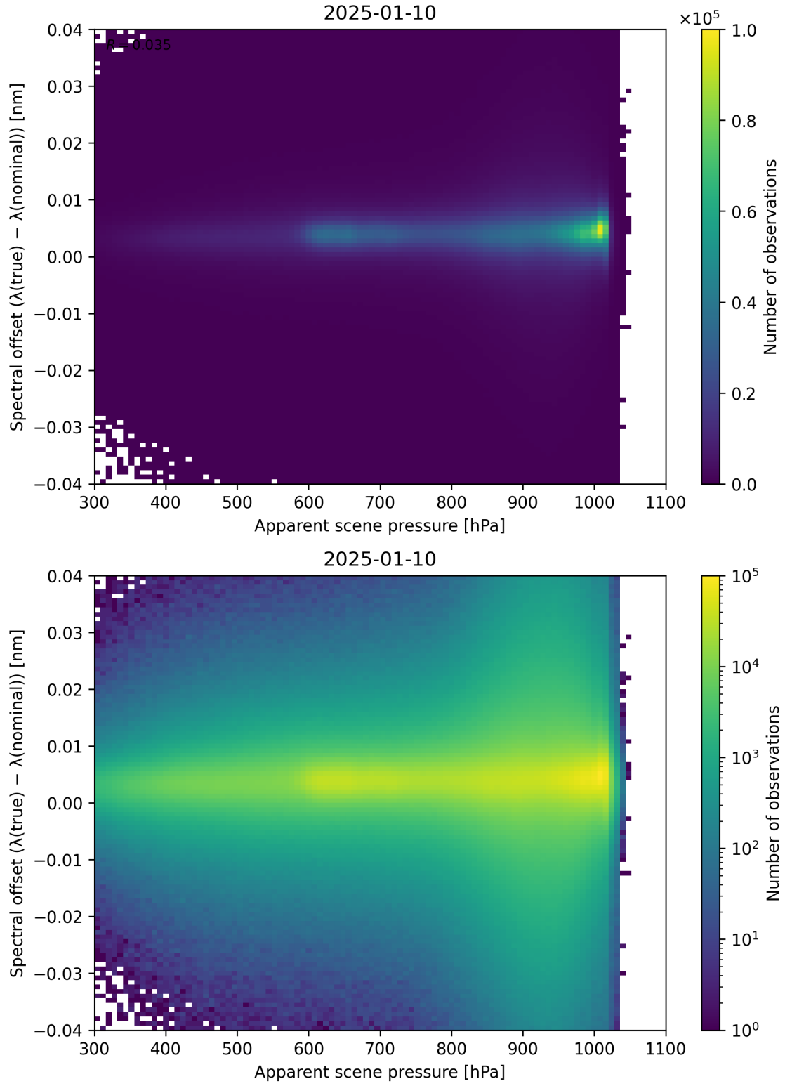
Figure 67: Scatter density plot of “Apparent scene pressure” against “Spectral offset ( \lambda_{\text{true}} - \lambda_{\text{nominal}} )” for 2025-01-09 to 2025-01-11.
