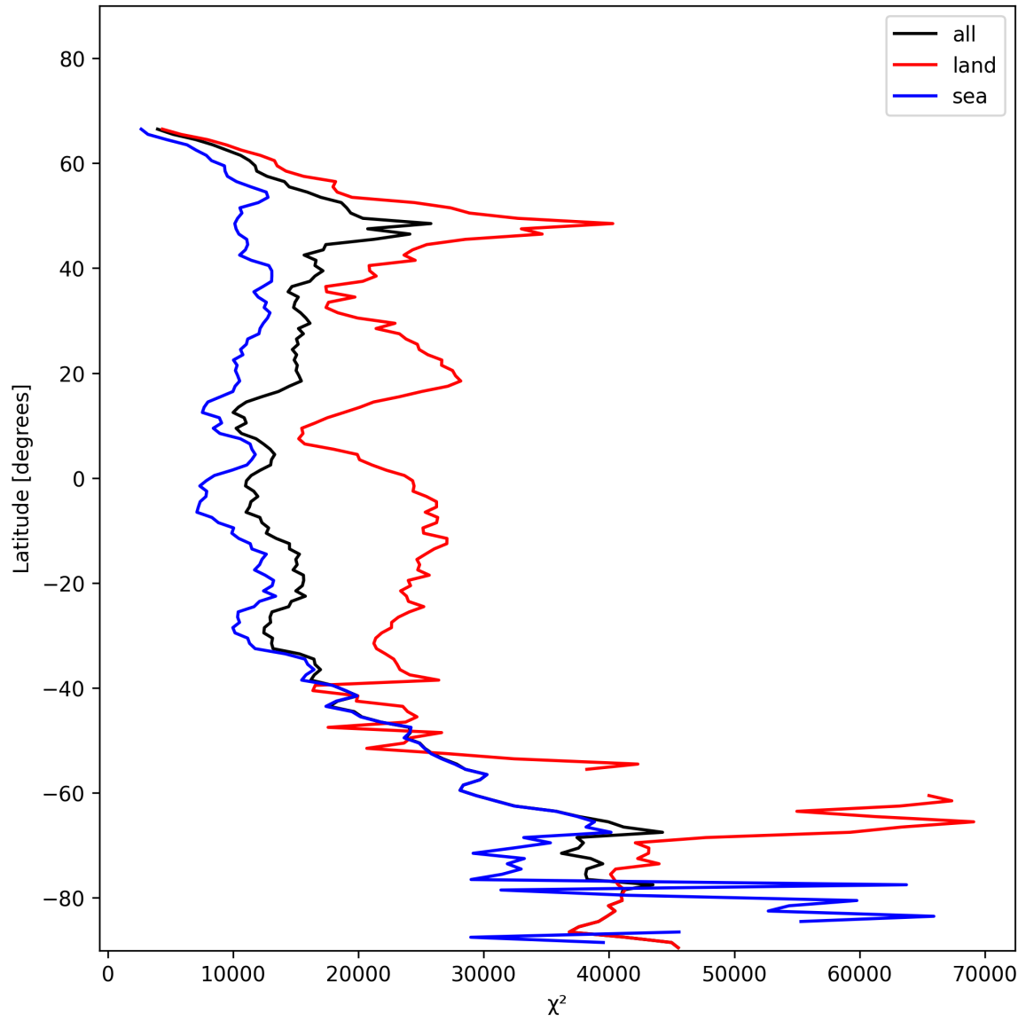
Figure 21: Zonal average of “ \chi^2 ” for 2025-01-09 to 2025-01-11.
