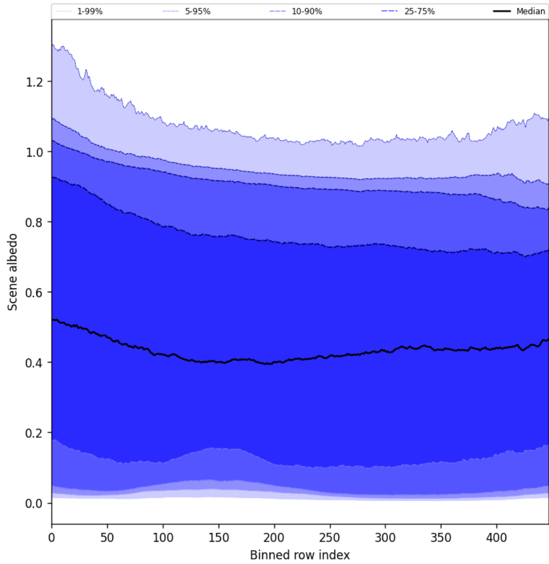
Figure 51: Along track statistics of “Scene albedo” for 2025-01-09 to 2025-01-11
