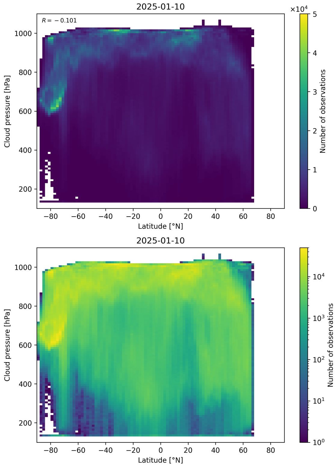
Figure 91: Scatter density plot of “Latitude” against “Cloud pressure” for 2025-01-09 to 2025-01-11.
