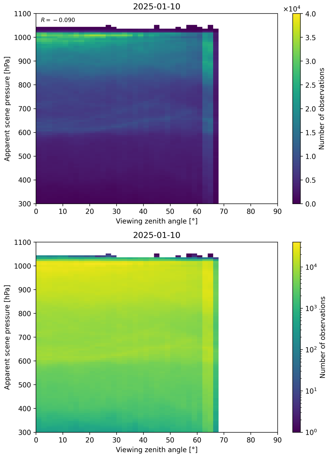
Figure 118: Scatter density plot of “Viewing zenith angle” against “Apparent scene pressure” for 2025-01-09 to 2025-01-11.
