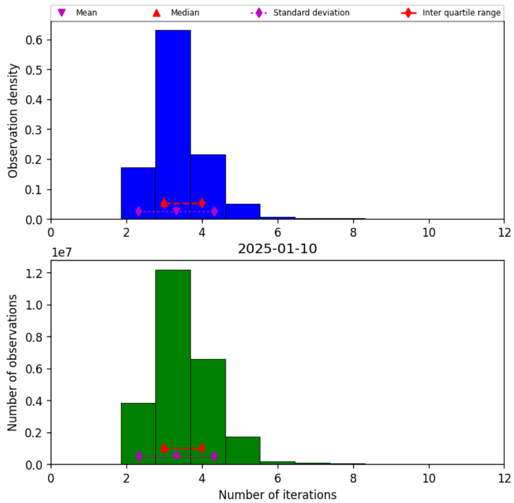
Figure 39: Histogram of “Number of iterations” for 2025-01-09 to 2025-01-11
