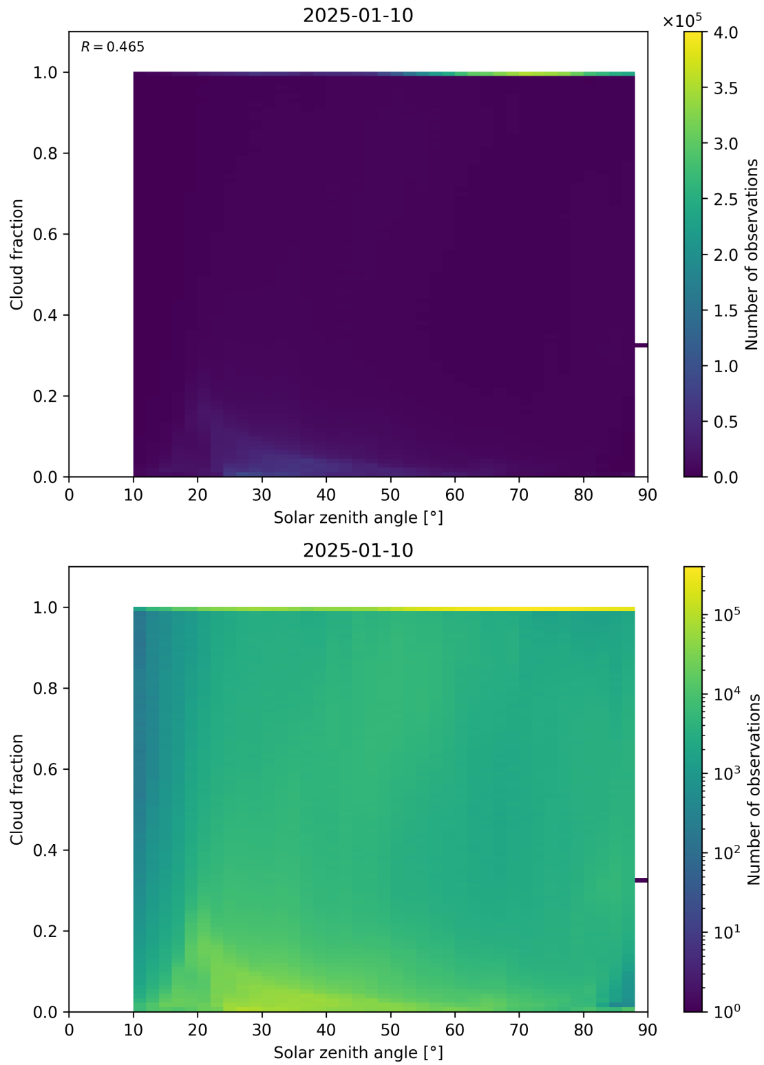
Figure 110: Scatter density plot of “Solar zenith angle” against “Cloud fraction” for 2025-01-09 to 2025-01-11.
