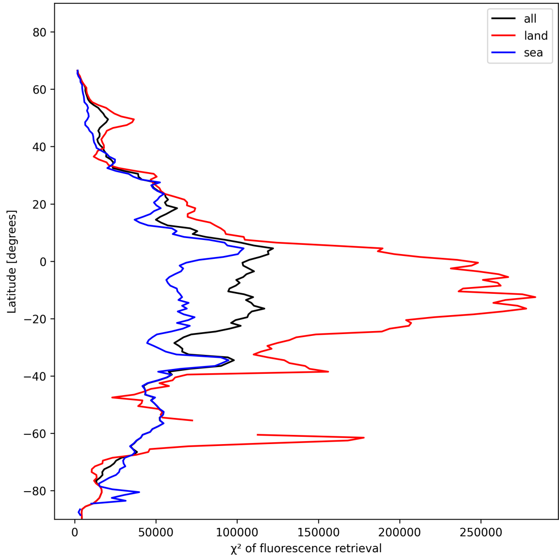
Figure 25: Zonal average of “ \chi^2 of fluorescence retrieval” for 2025-01-09 to 2025-01-11.
