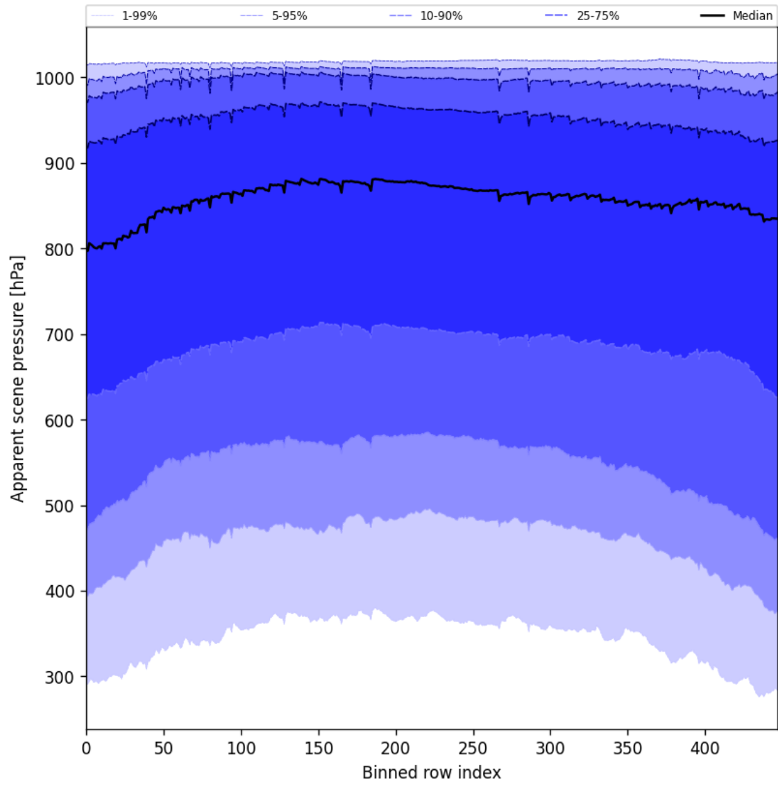
Figure 53: Along track statistics of “Apparent scene pressure” for 2025-01-09 to 2025-01-11
