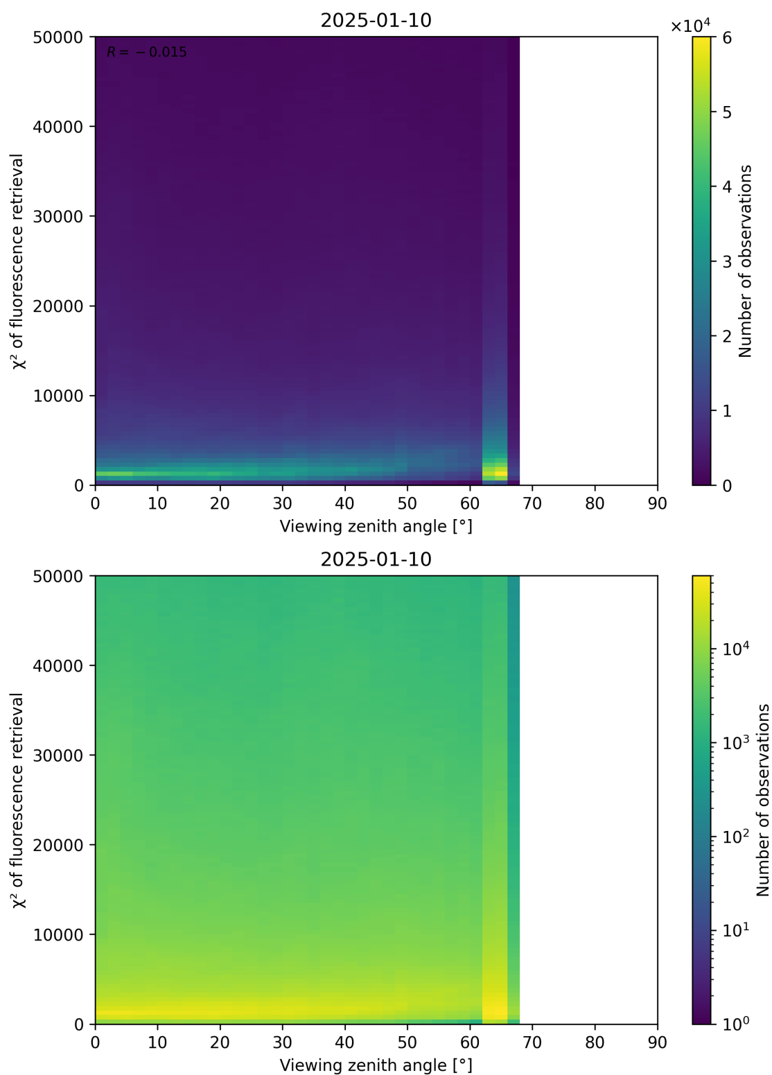
Figure 119: Scatter density plot of “Viewing zenith angle” against “ \chi^2 of fluorescence retrieval” for 2025-01-09 to 2025-01-11.
