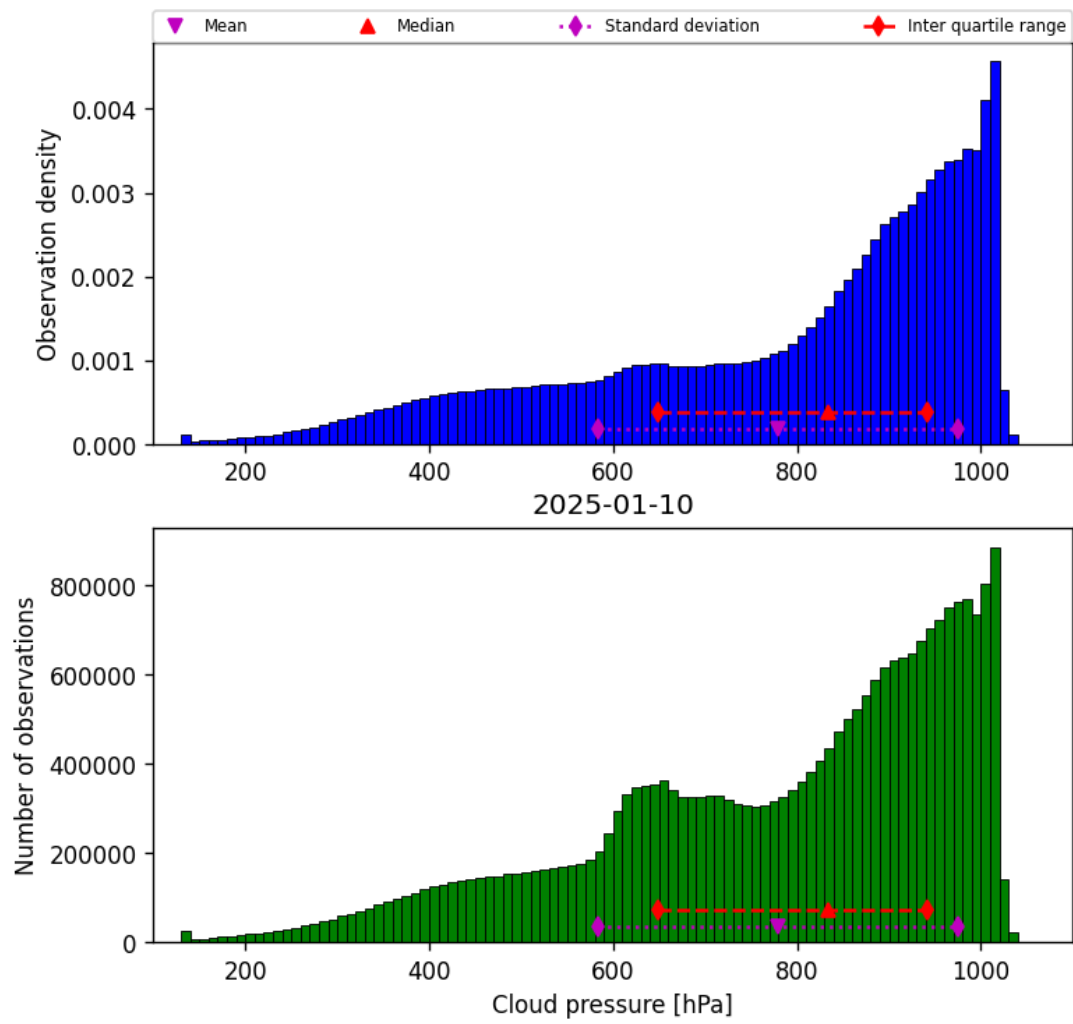
Figure 30: Histogram of “Cloud pressure” for 2025-01-09 to 2025-01-11
