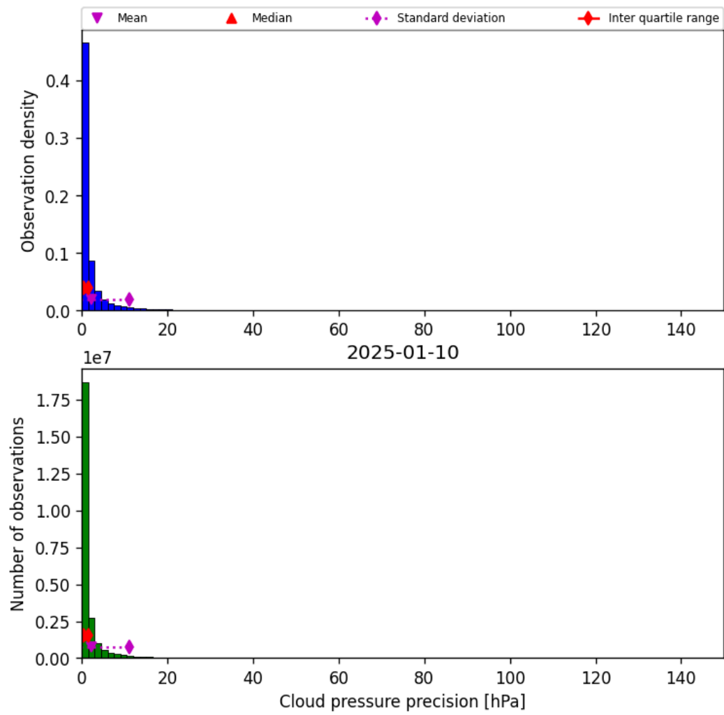
Figure 31: Histogram of “Cloud pressure precision” for 2025-01-09 to 2025-01-11
