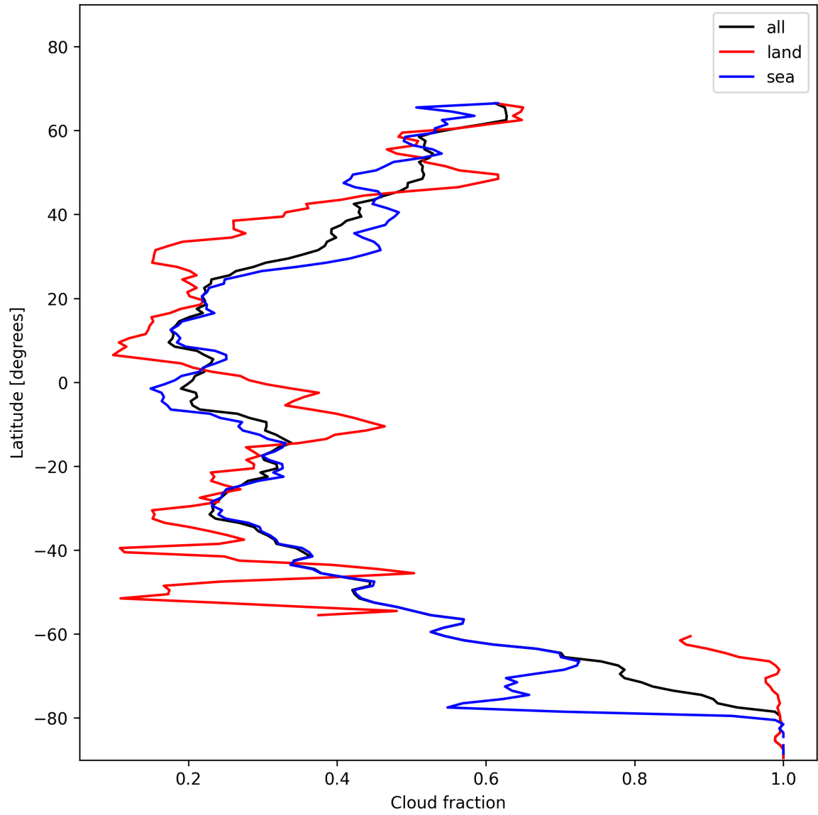
Figure 15: Zonal average of “Cloud fraction” for 2025-01-09 to 2025-01-11.
