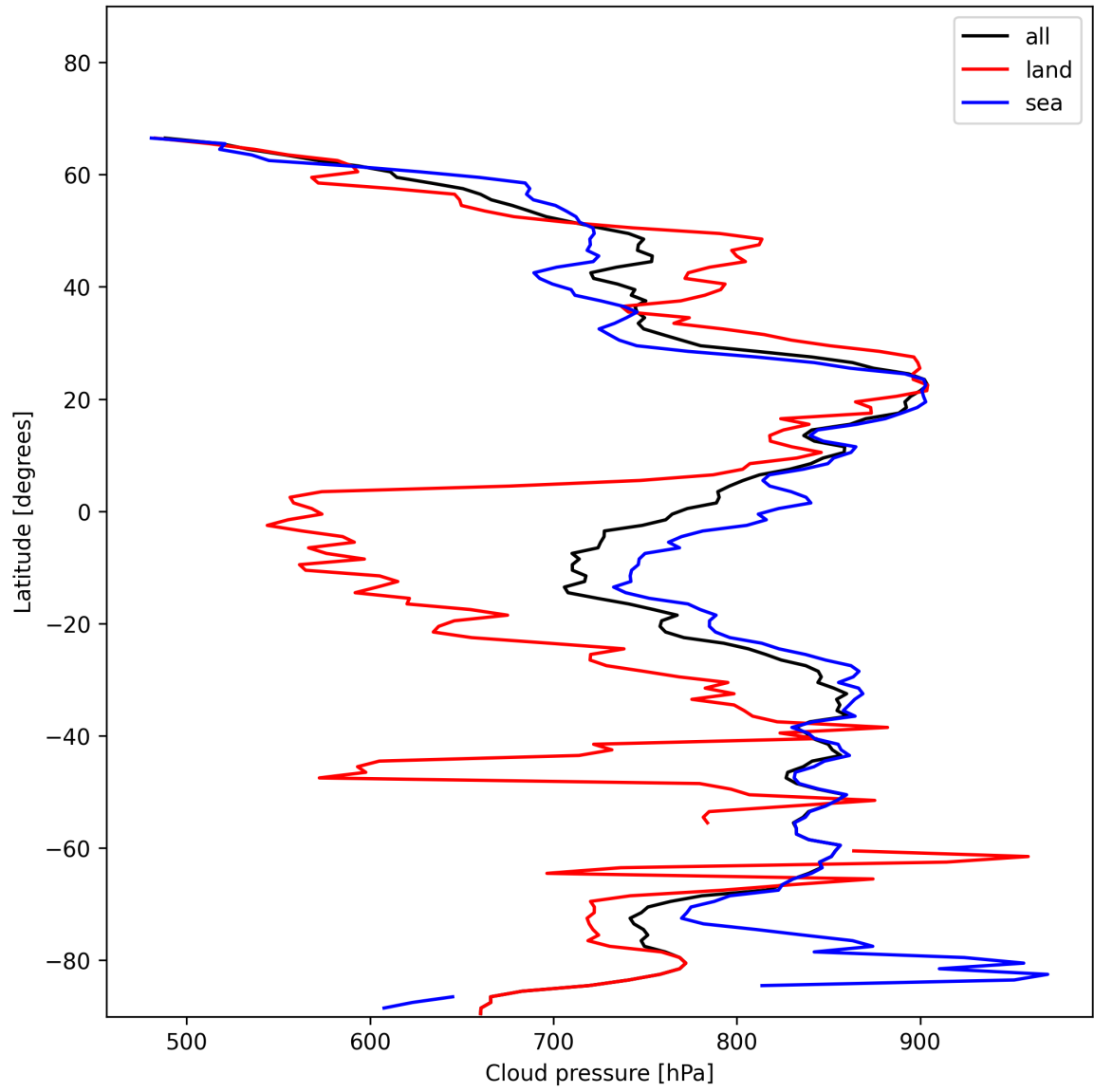
Figure 13: Zonal average of “Cloud pressure” for 2025-01-09 to 2025-01-11.
