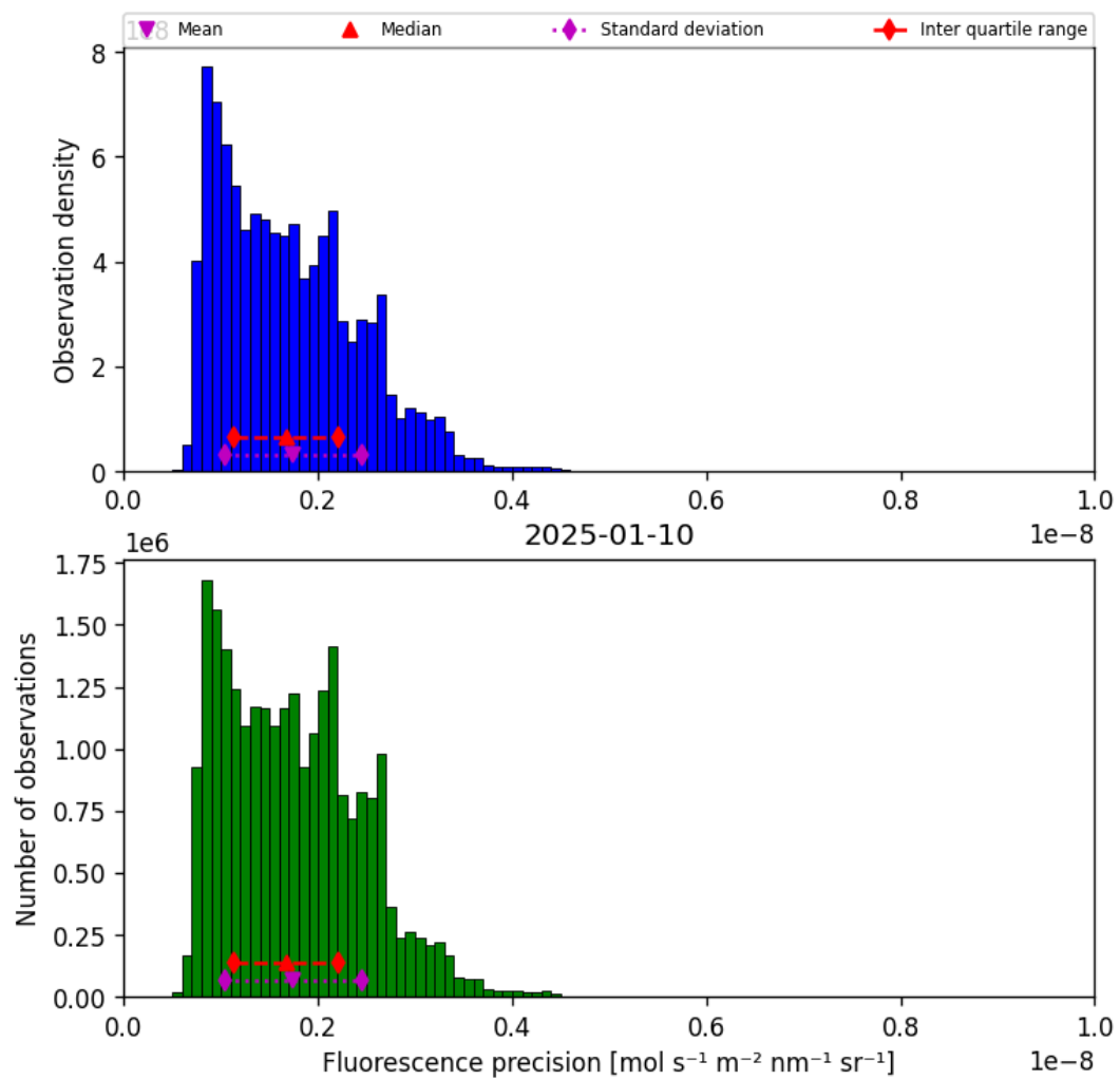
Figure 41: Histogram of “Fluorescence precision” for 2025-01-09 to 2025-01-11
