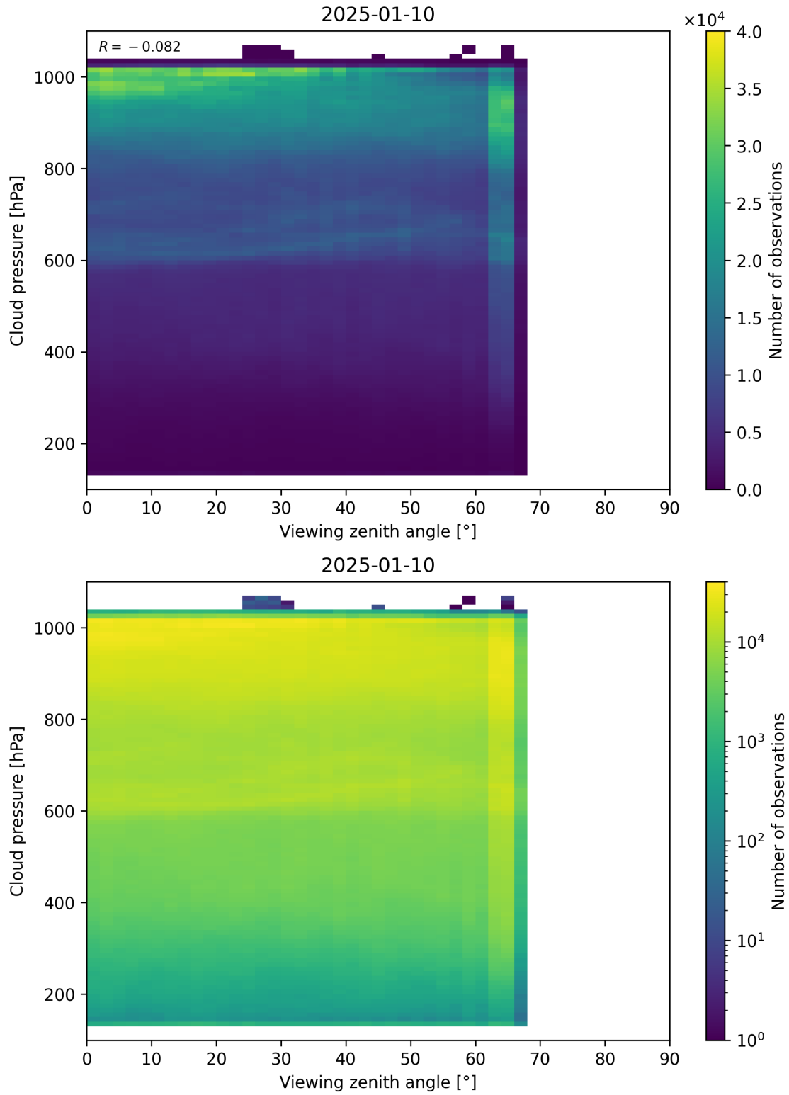
Figure 121: Scatter density plot of “Viewing zenith angle” against “Cloud pressure” for 2025-01-09 to 2025-01-11.
