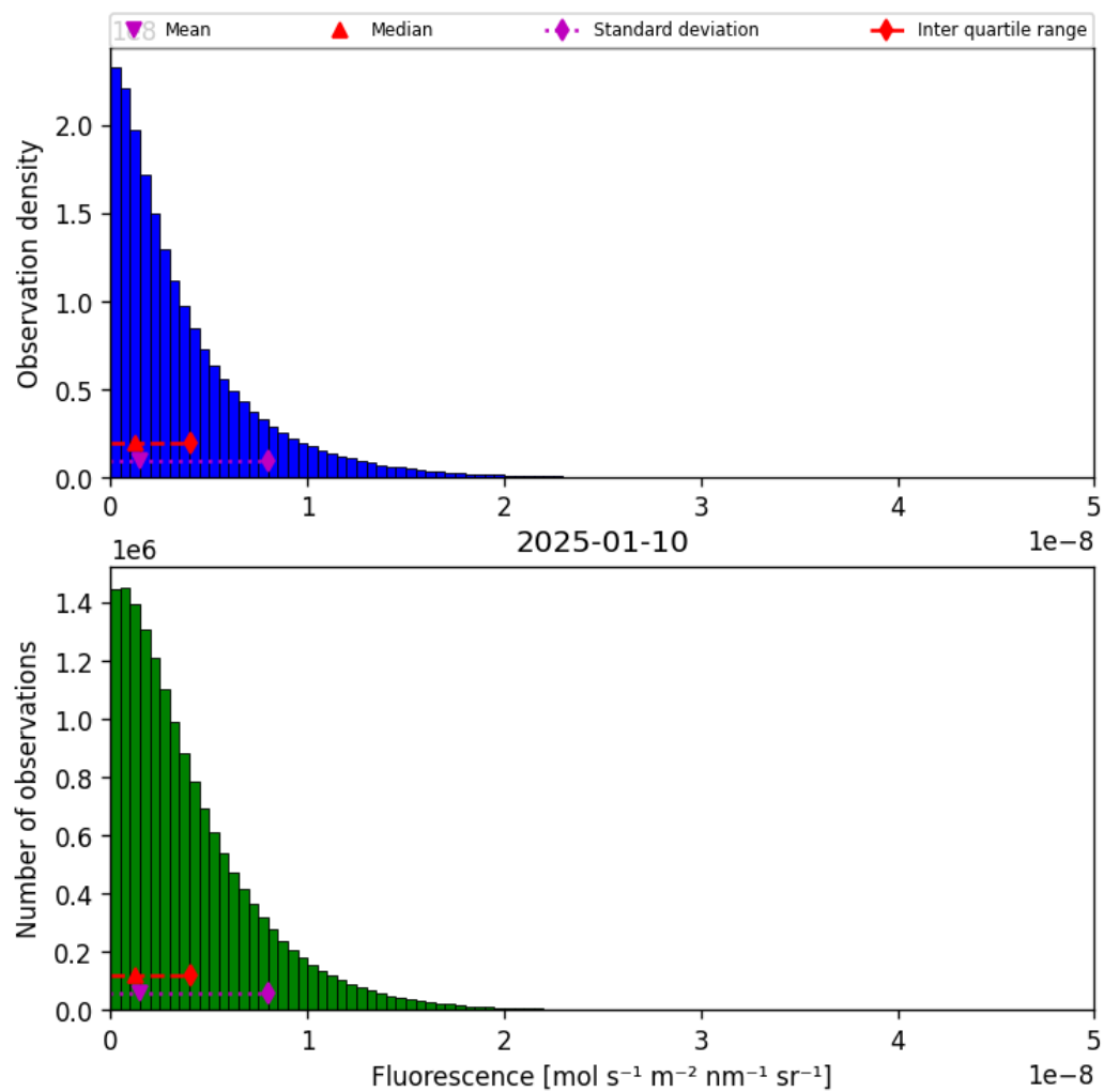
Figure 40: Histogram of “Fluorescence” for 2025-01-09 to 2025-01-11
