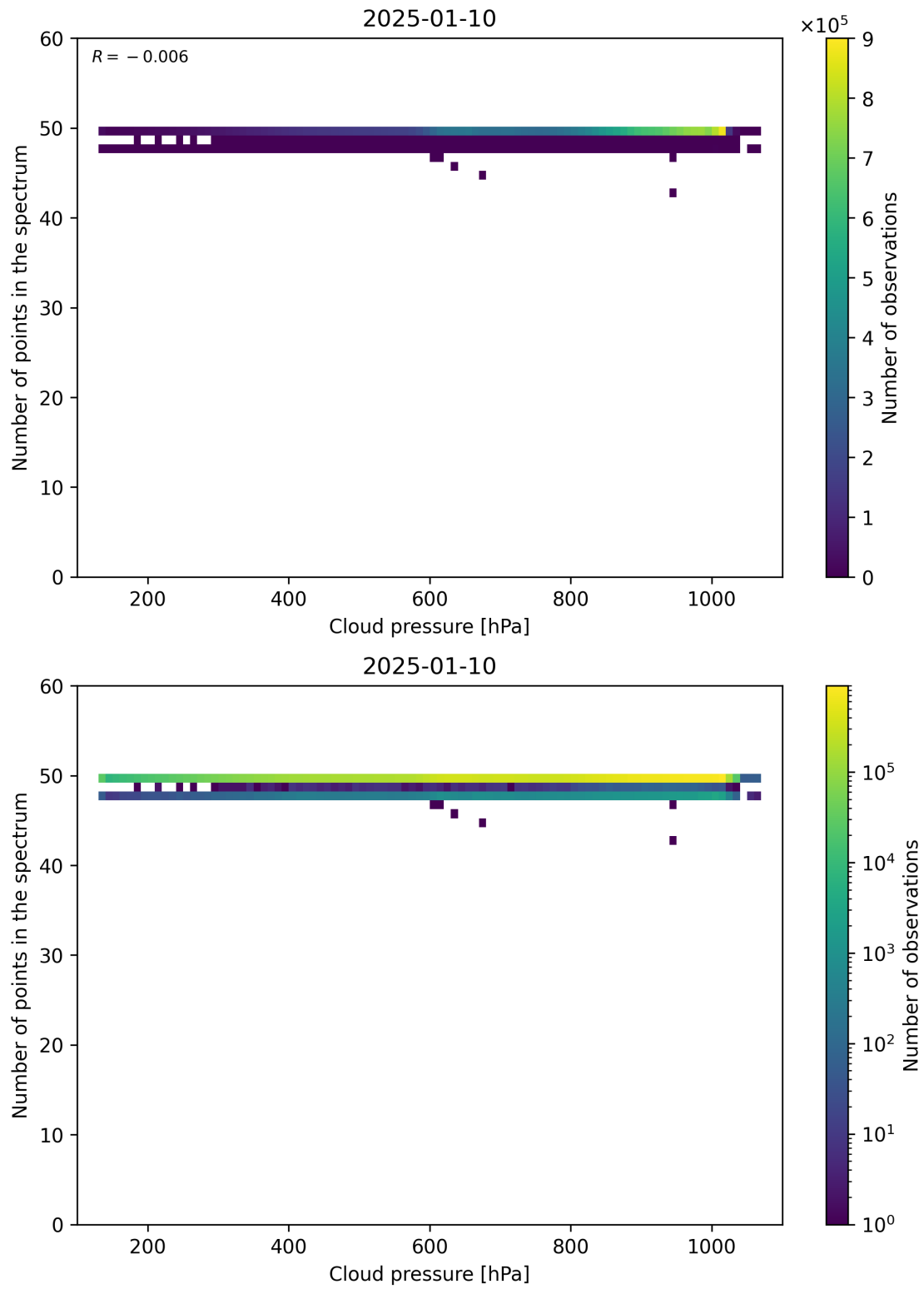
Figure 82: Scatter density plot of “Cloud pressure” against “Number of points in the spectrum” for 2025-01-09 to 2025-01-11.
