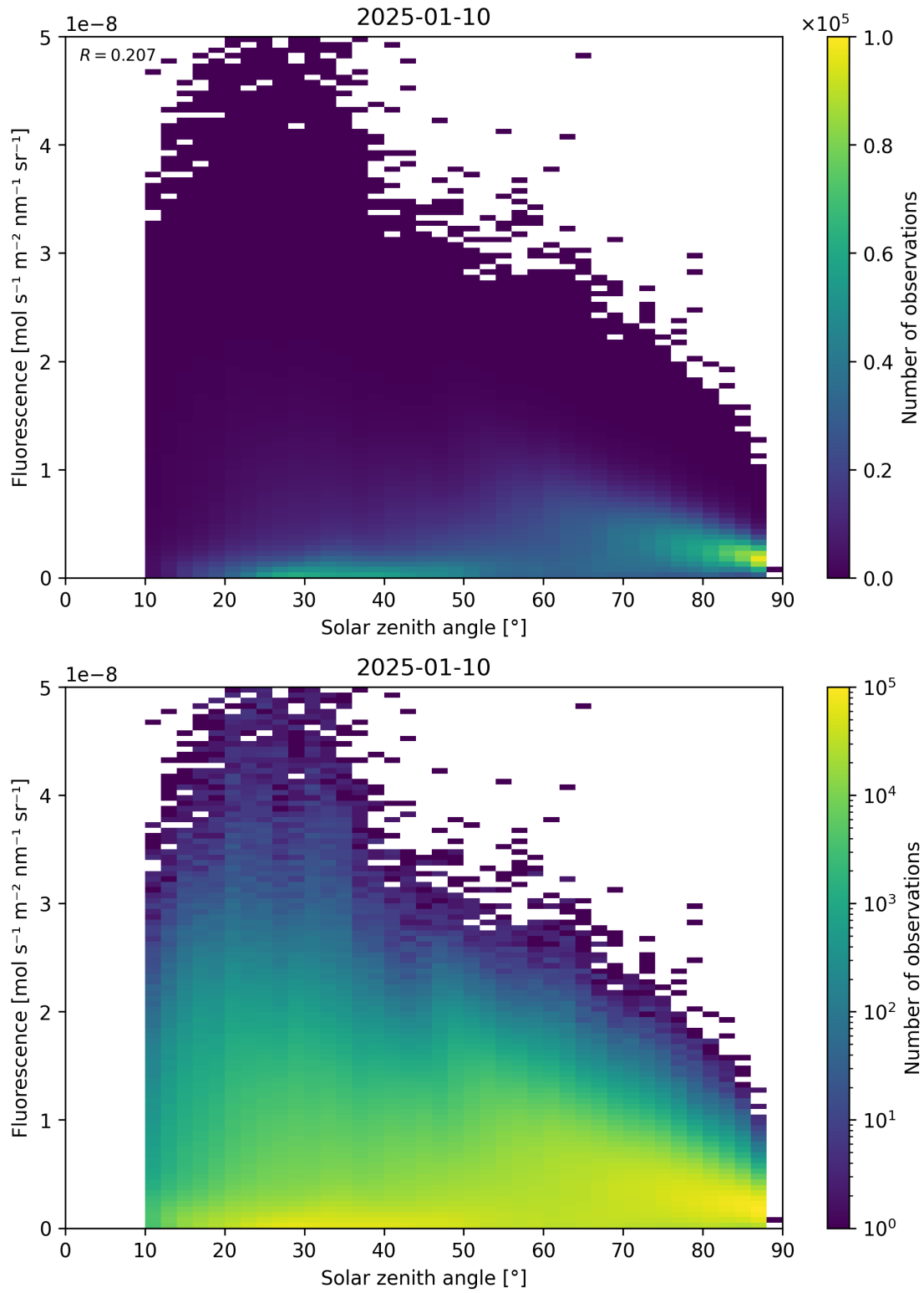
Figure 112: Scatter density plot of “Solar zenith angle” against “Fluorescence” for 2025-01-09 to 2025-01-11.
