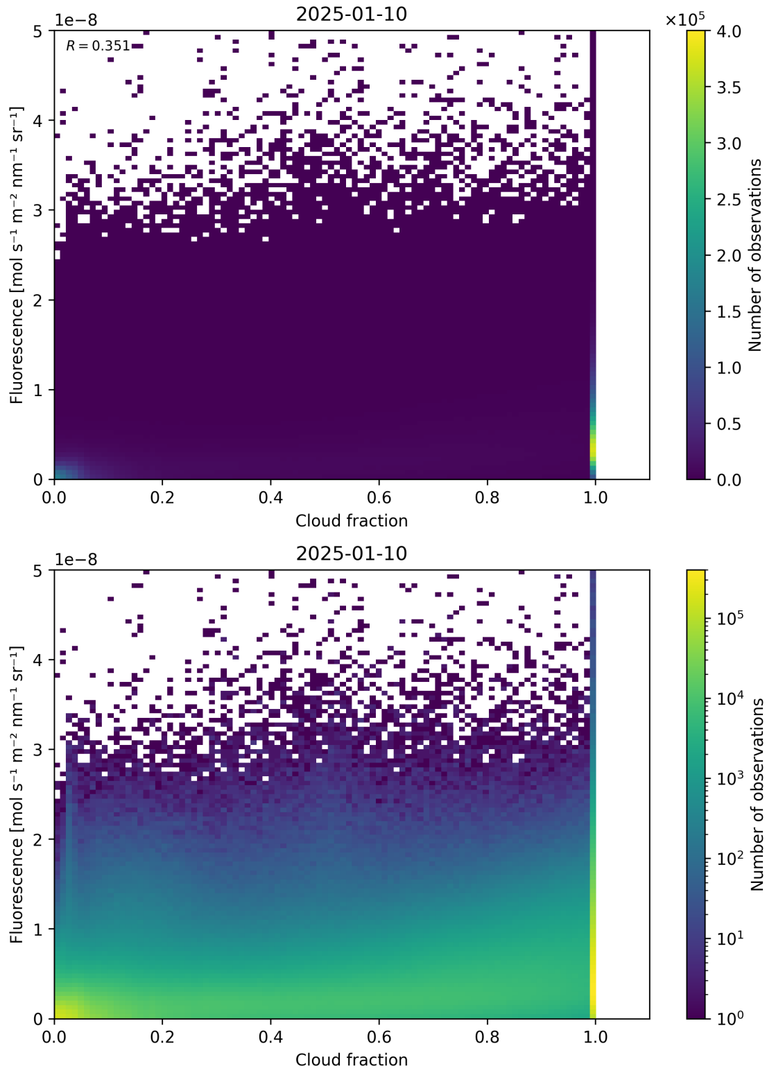
Figure 72: Scatter density plot of “Cloud fraction” against “Fluorescence” for 2025-01-09 to 2025-01-11.
