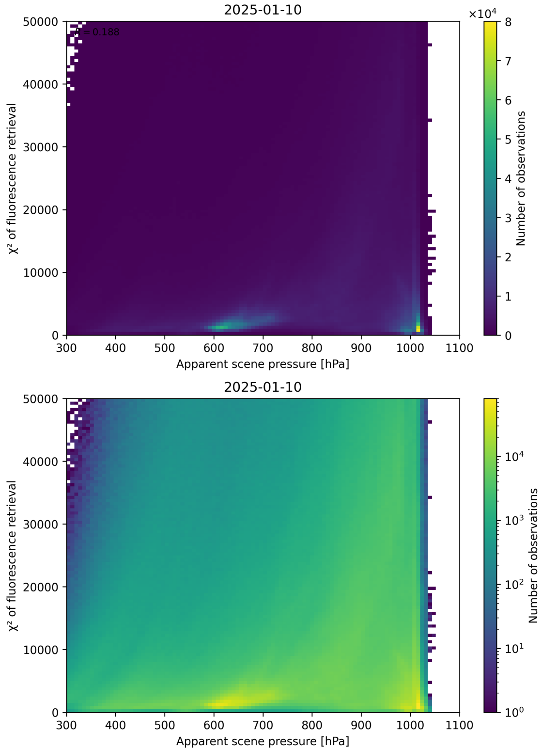
Figure 63: Scatter density plot of “Apparent scene pressure” against “ \chi^2 of fluorescence retrieval” for 2025-01-09 to 2025-01-11.
