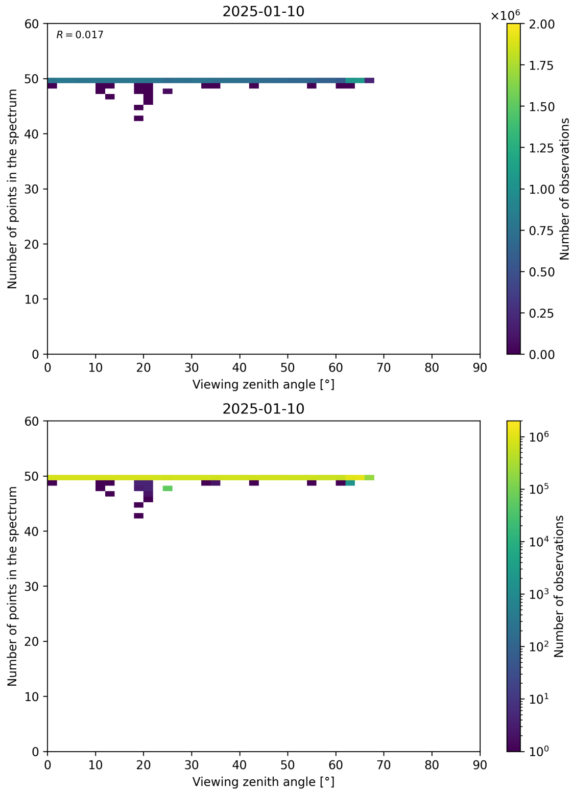
Figure 125: Scatter density plot of “Viewing zenith angle” against “Number of points in the spectrum” for 2025-01-09 to 2025-01-11.
