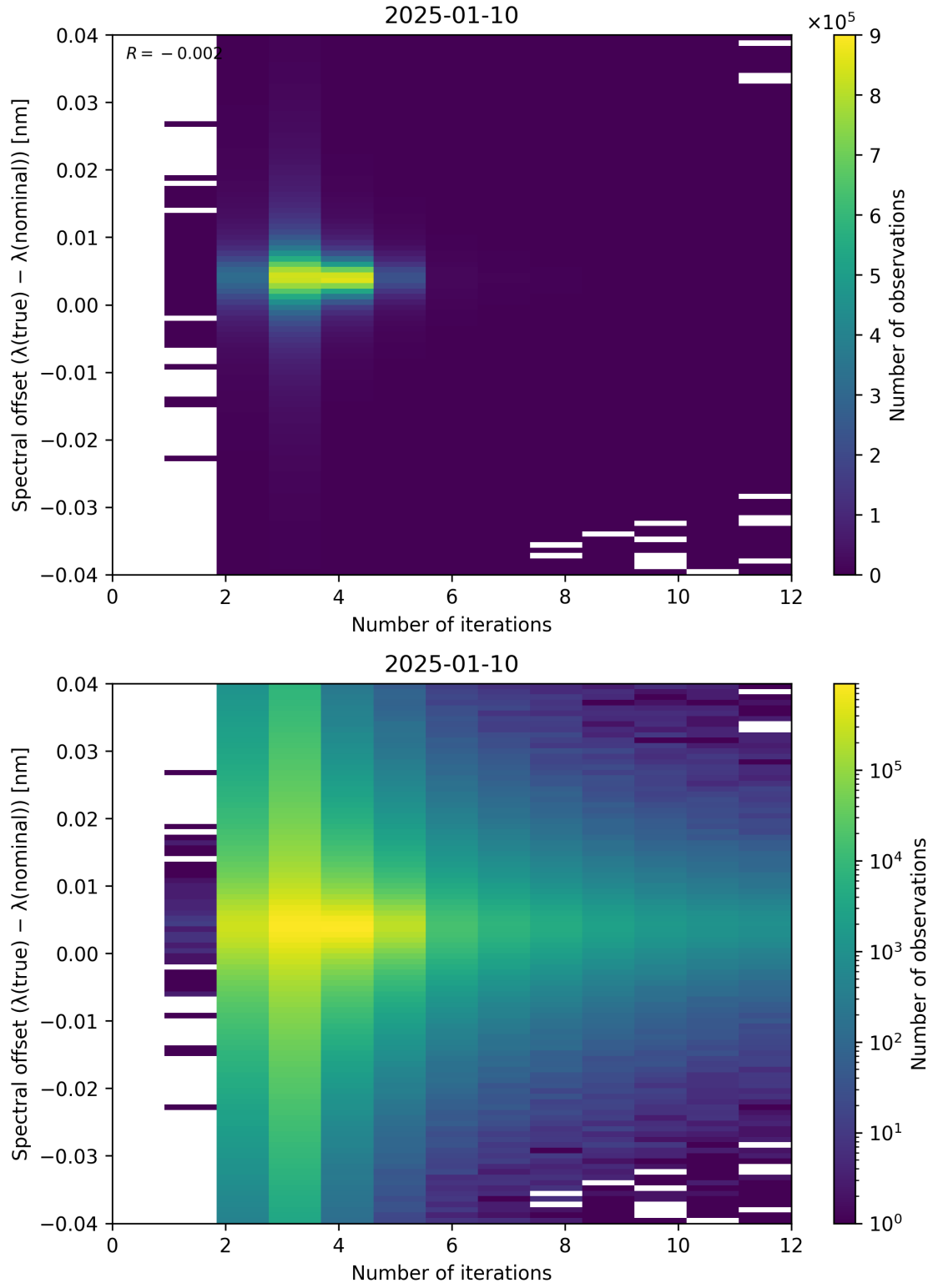
Figure 100: Scatter density plot of “Number of iterations” against “Spectral offset ( \lambda_{\text{true}} - \lambda_{\text{nominal}} )” for 2025-01-09 to 2025-01-11.
