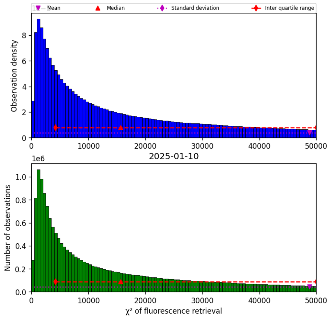
Figure 42: Histogram of “ \chi^2 of fluorescence retrieval” for 2025-01-09 to 2025-01-11
