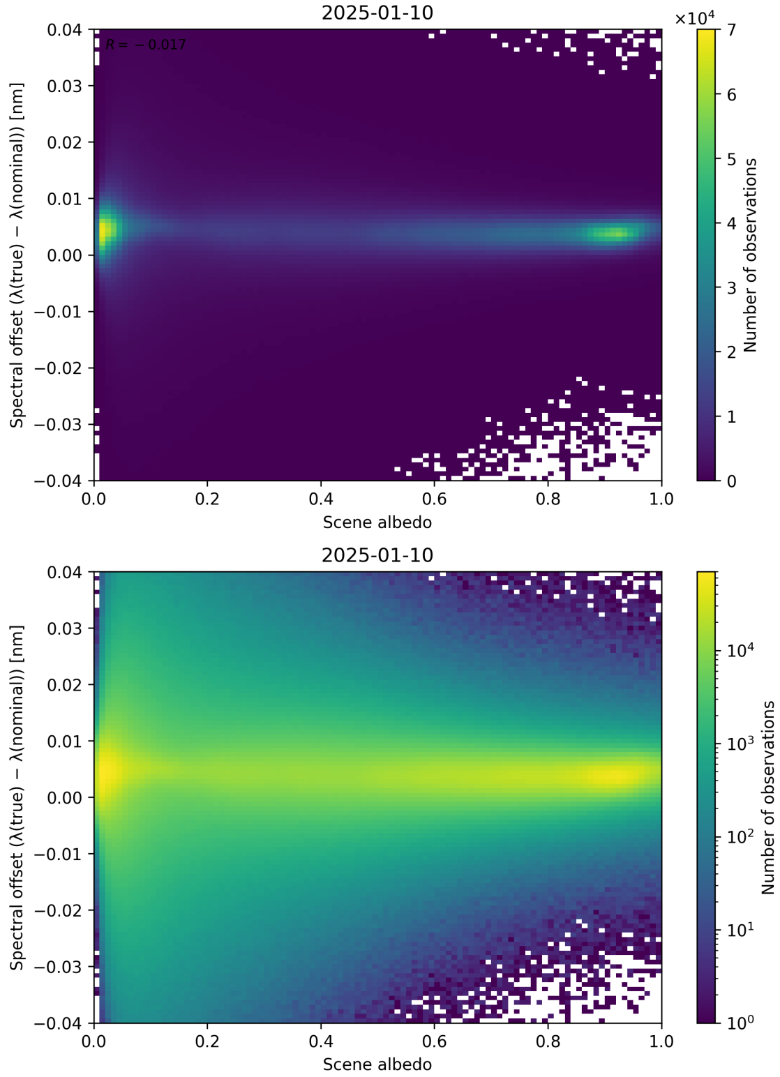
Figure 107: Scatter density plot of “Scene albedo” against “Spectral offset ( \lambda_{\text{true}} - \lambda_{\text{nominal}} )” for 2025-01-09 to 2025-01-11.
