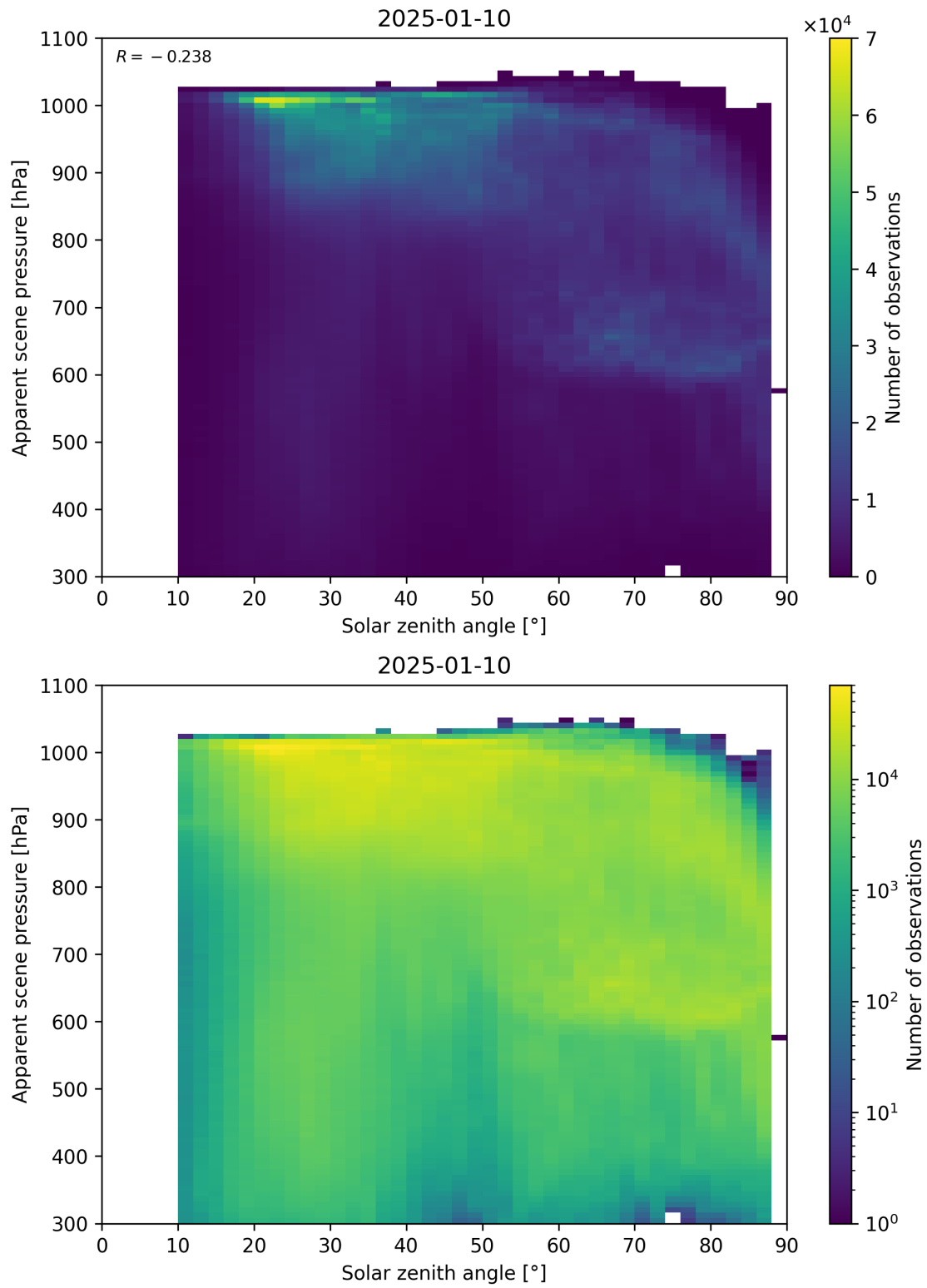
Figure 108: Scatter density plot of “Solar zenith angle” against “Apparent scene pressure” for 2025-01-09 to 2025-01-11.
