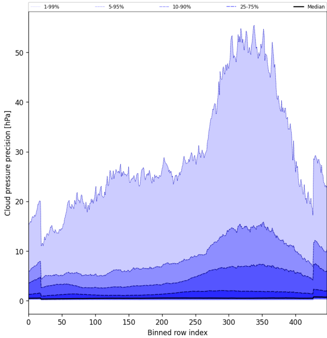
Figure 48: Along track statistics of “Cloud pressure precision” for 2025-01-09 to 2025-01-11
