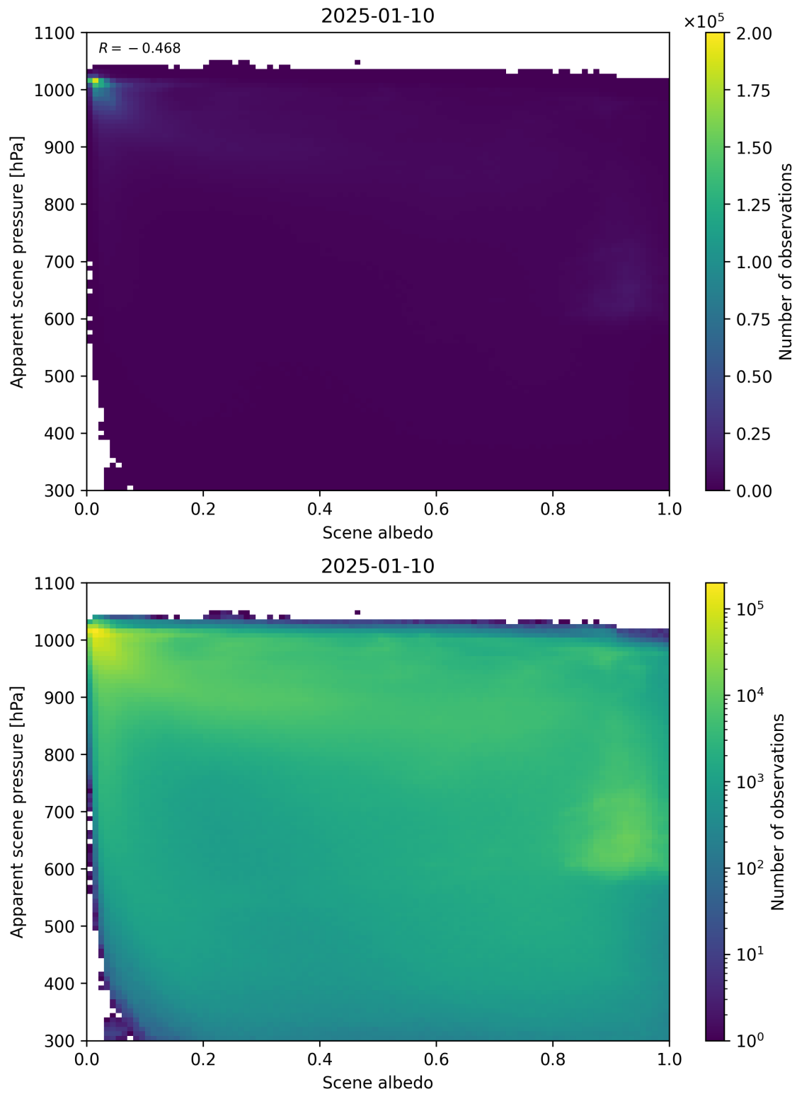
Figure 102: Scatter density plot of “Scene albedo” against “Apparent scene pressure” for 2025-01-09 to 2025-01-11.
