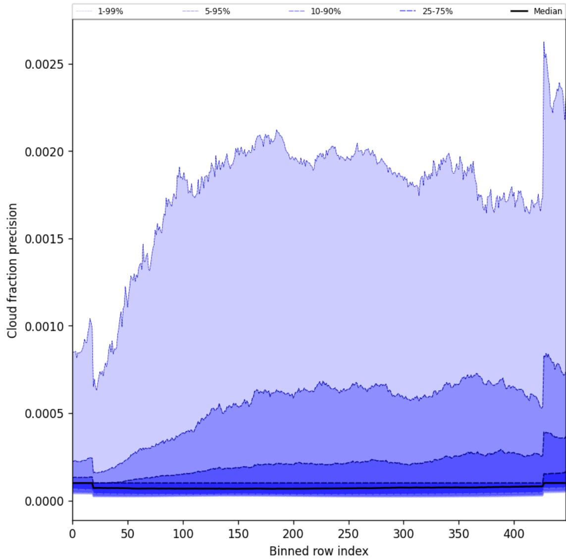
Figure 50: Along track statistics of “Cloud fraction precision” for 2025-01-09 to 2025-01-11
