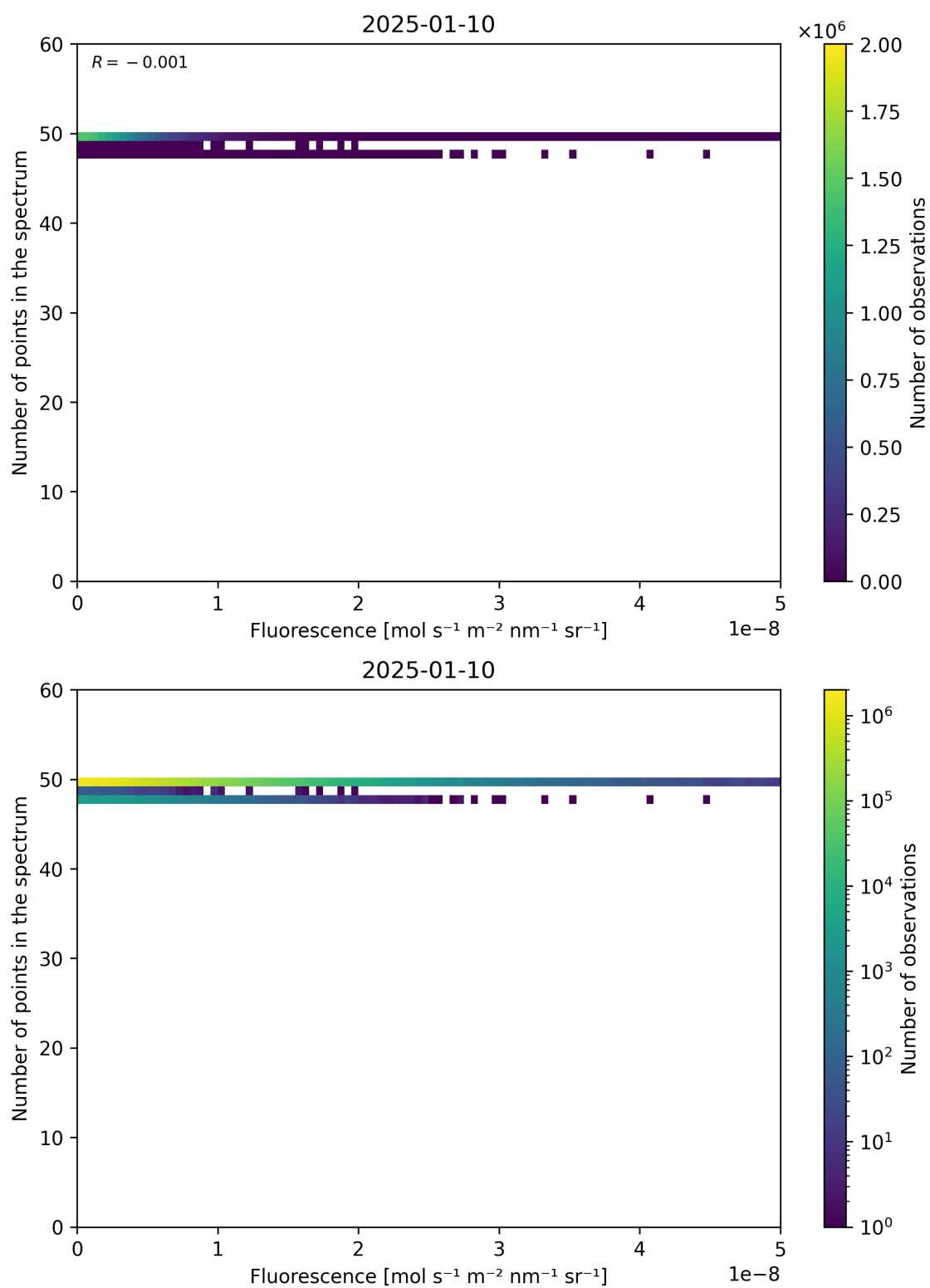
Figure 86: Scatter density plot of “Fluorescence” against “Number of points in the spectrum” for 2025-01-09 to 2025-01-11.
