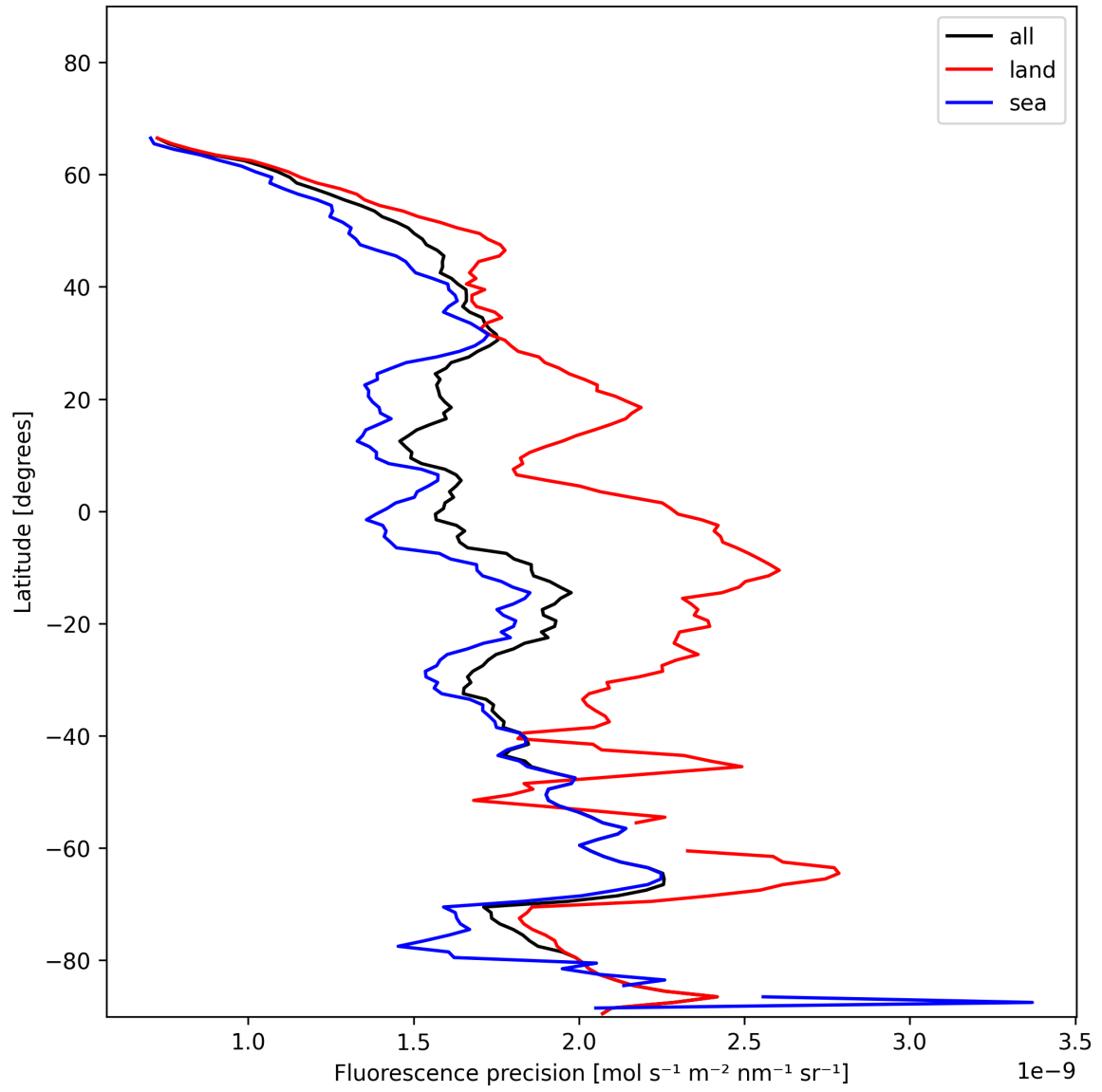
Figure 24: Zonal average of “Fluorescence precision” for 2025-01-09 to 2025-01-11.
