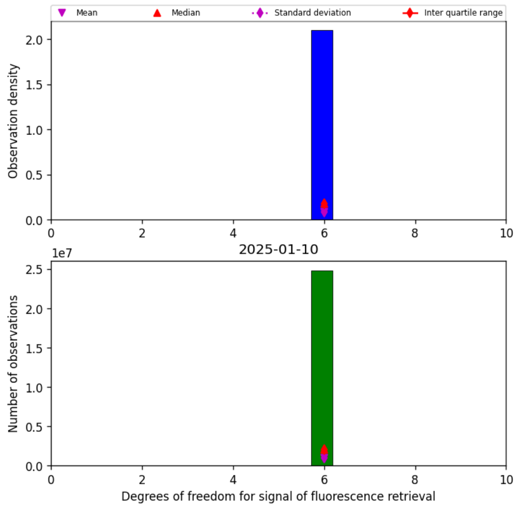
Figure 43: Histogram of "Degrees of freedom for signal of fluorescence retrieval" for 2025-01-09 to 2025-01-11
