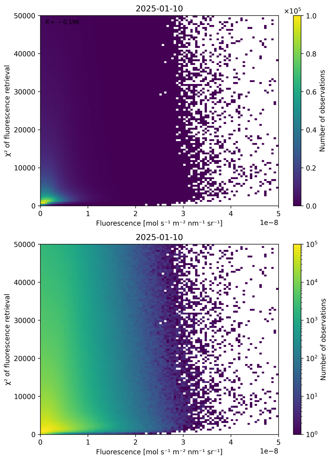
Figure 85: Scatter density plot of “Fluorescence” against “ \chi^2 of fluorescence retrieval” for 2025-01-09 to 2025-01-11.
