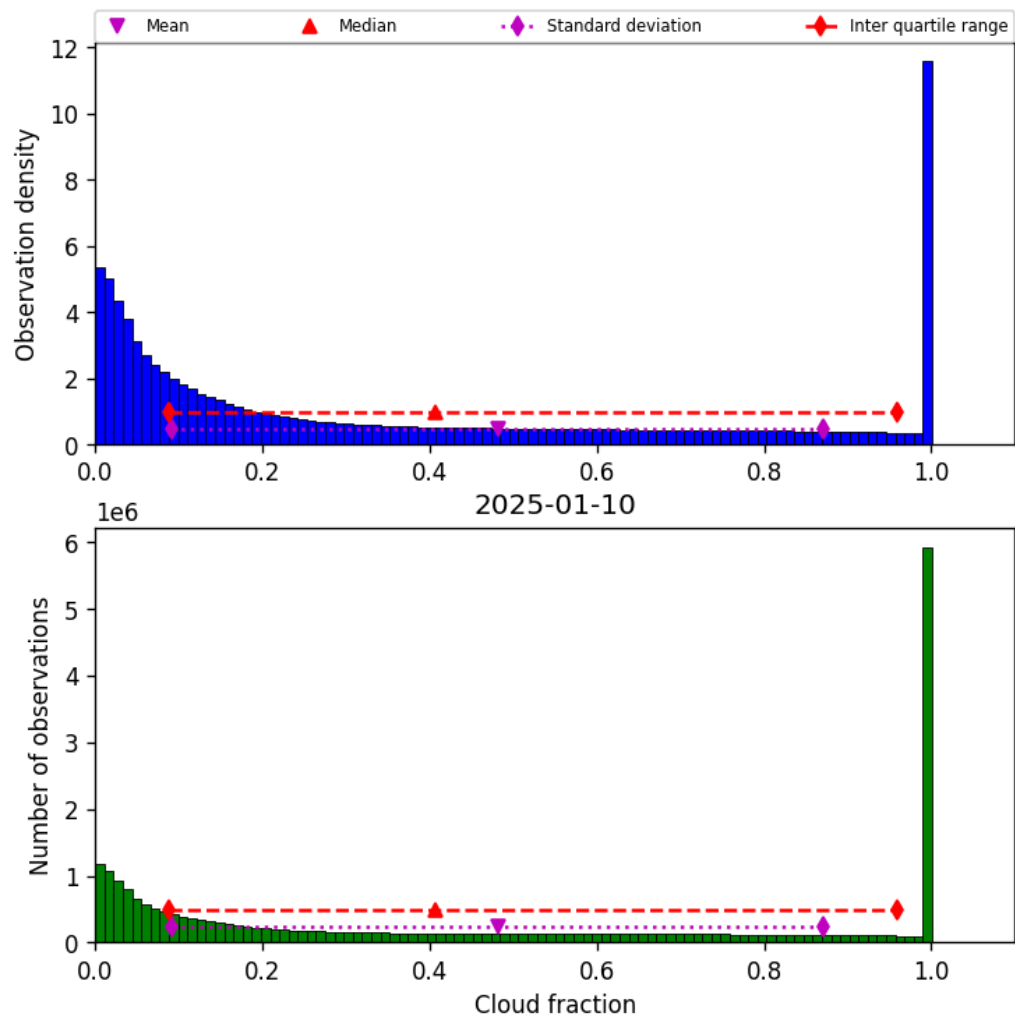
Figure 32: Histogram of “Cloud fraction” for 2025-01-09 to 2025-01-11
