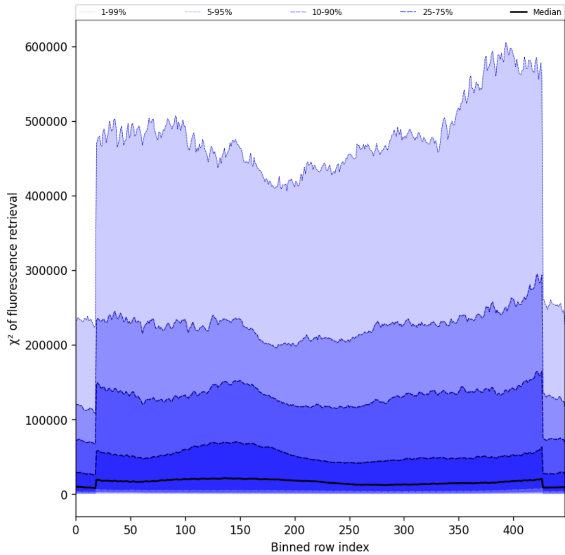
Figure 59: Along track statistics of “ \chi^2 of fluorescence retrieval” for 2025-01-09 to 2025-01-11
