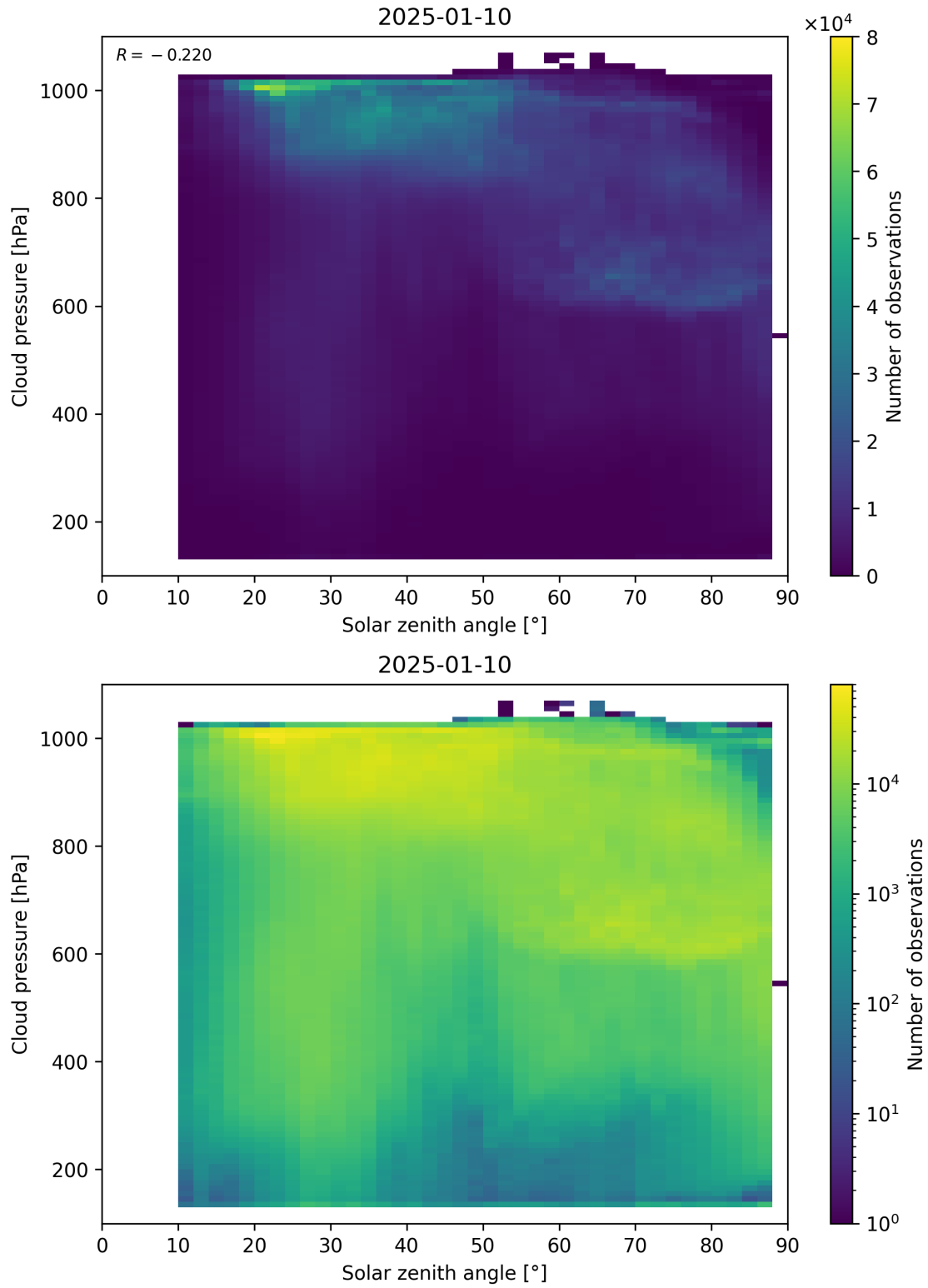
Figure 111: Scatter density plot of “Solar zenith angle” against “Cloud pressure” for 2025-01-09 to 2025-01-11.
