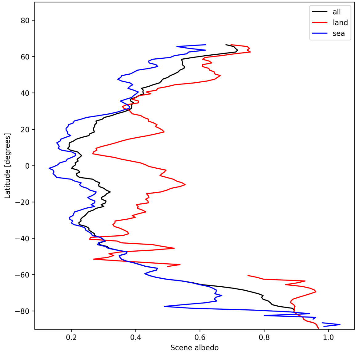
Figure 17: Zonal average of "Scene albedo" for 2025-01-09 to 2025-01-11.
