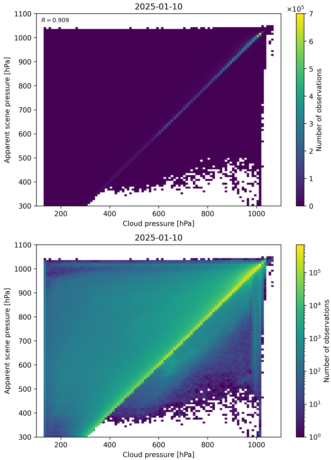
Figure 77: Scatter density plot of “Cloud pressure” against “Apparent scene pressure” for 2025-01-09 to 2025-01-11.
