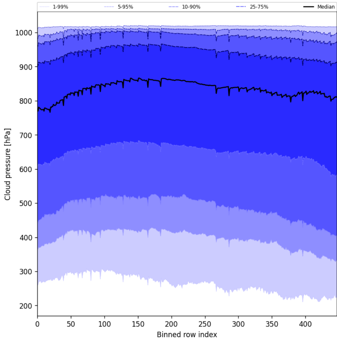
Figure 47: Along track statistics of “Cloud pressure” for 2025-01-09 to 2025-01-11
