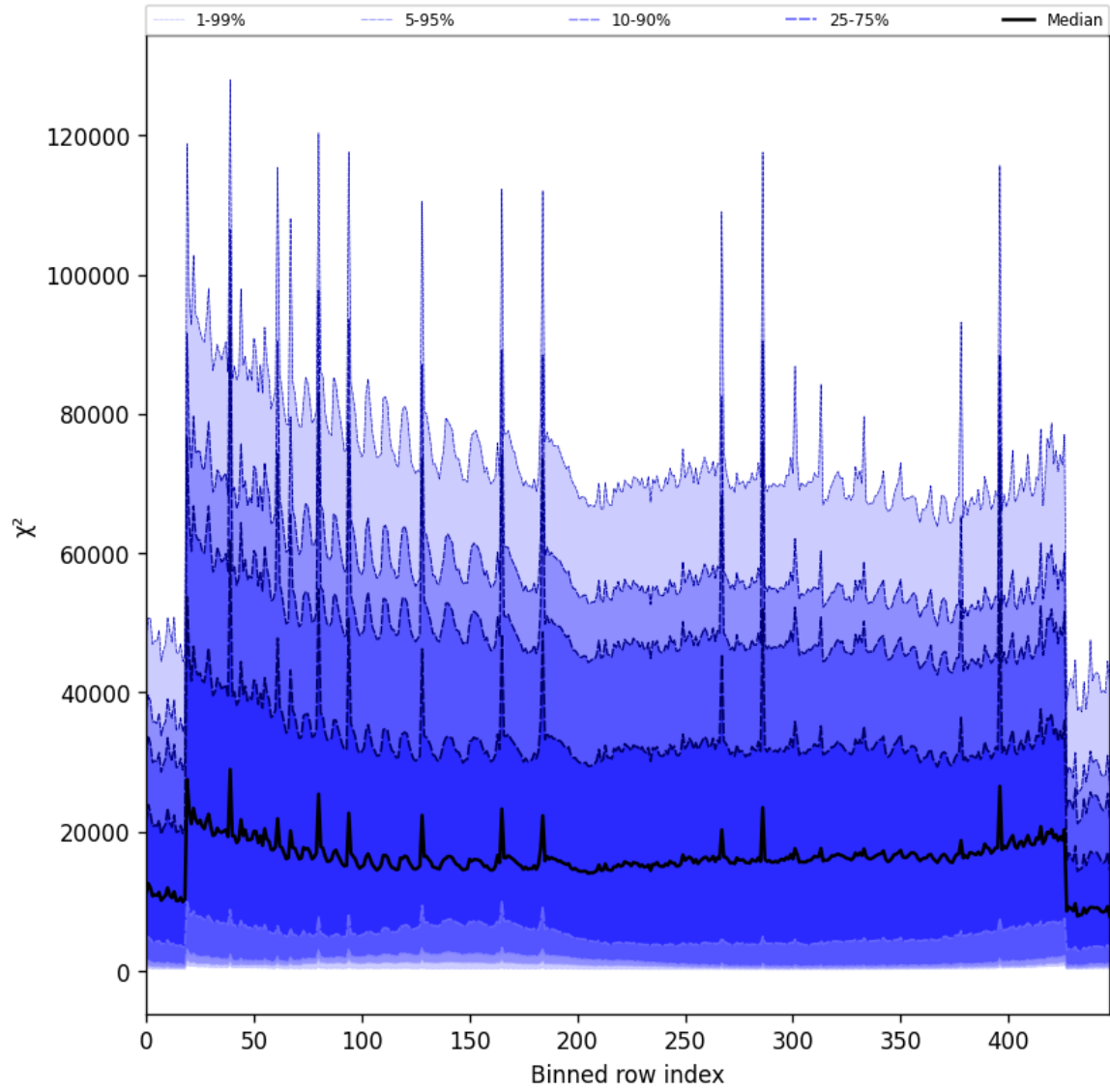
Figure 55: Along track statistics of “ \chi^2 ” for 2025-01-09 to 2025-01-11
