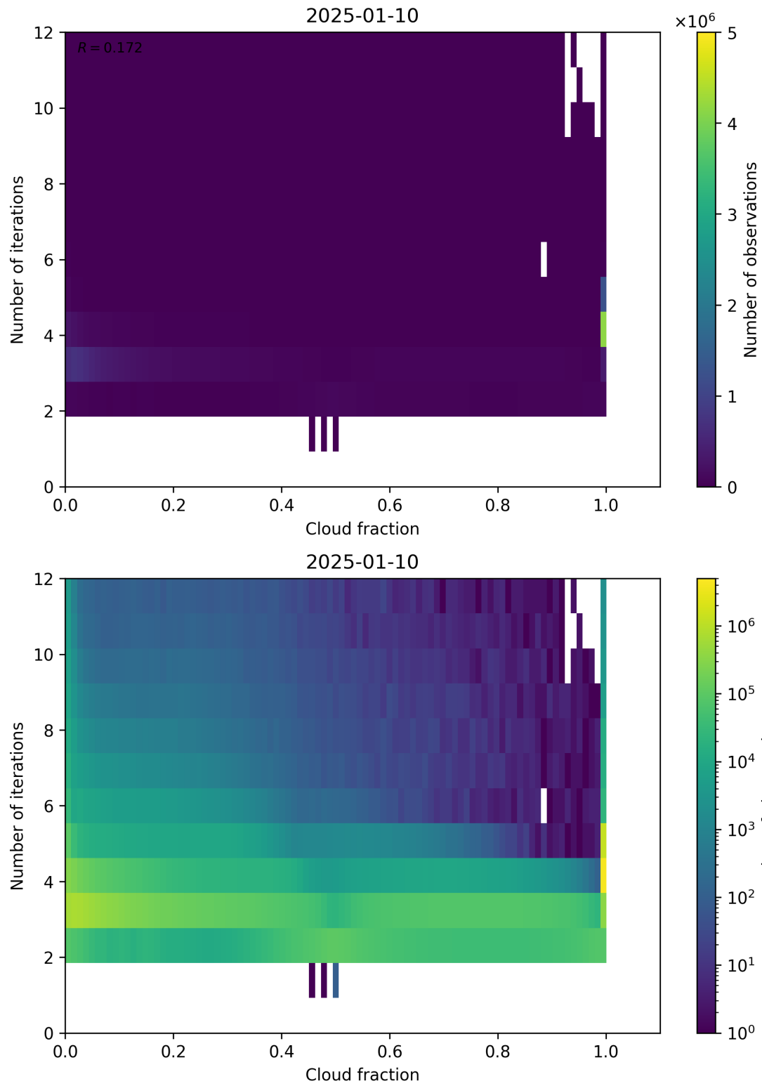
Figure 73: Scatter density plot of “Cloud fraction” against “Number of iterations” for 2025-01-09 to 2025-01-11.
