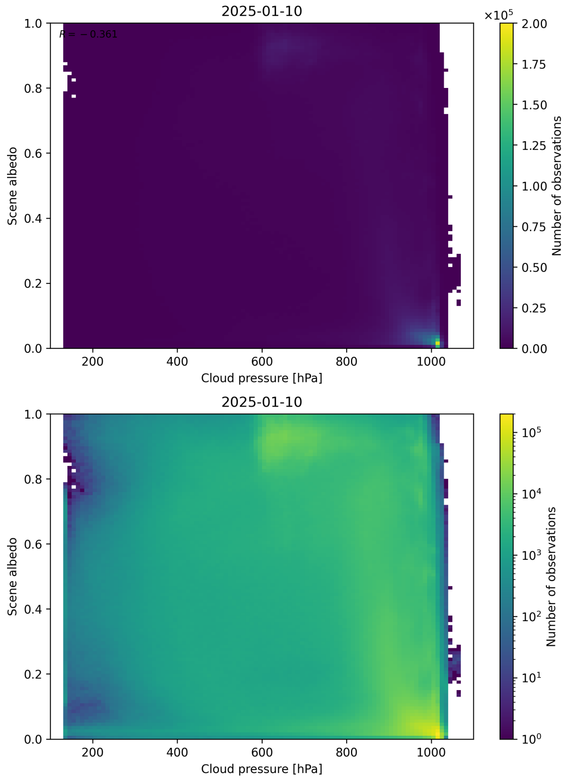
Figure 83: Scatter density plot of “Cloud pressure” against “Scene albedo” for 2025-01-09 to 2025-01-11.
