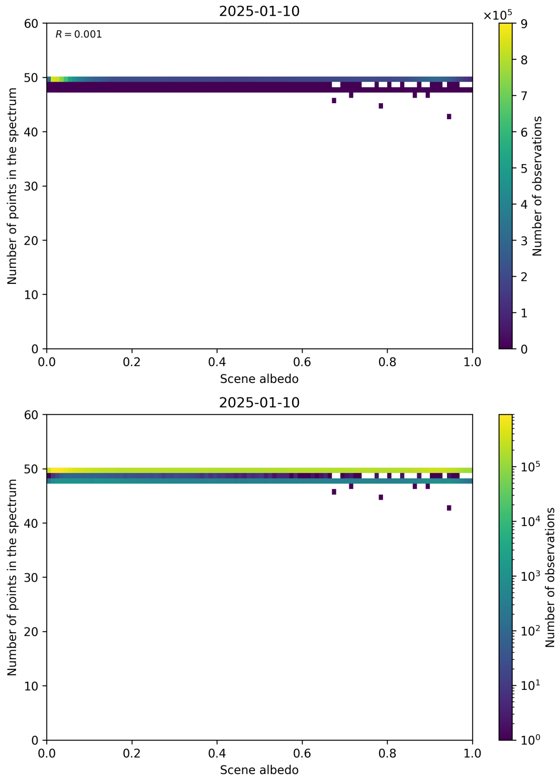
Figure 106: Scatter density plot of “Scene albedo” against “Number of points in the spectrum” for 2025-01-09 to 2025-01-11.
