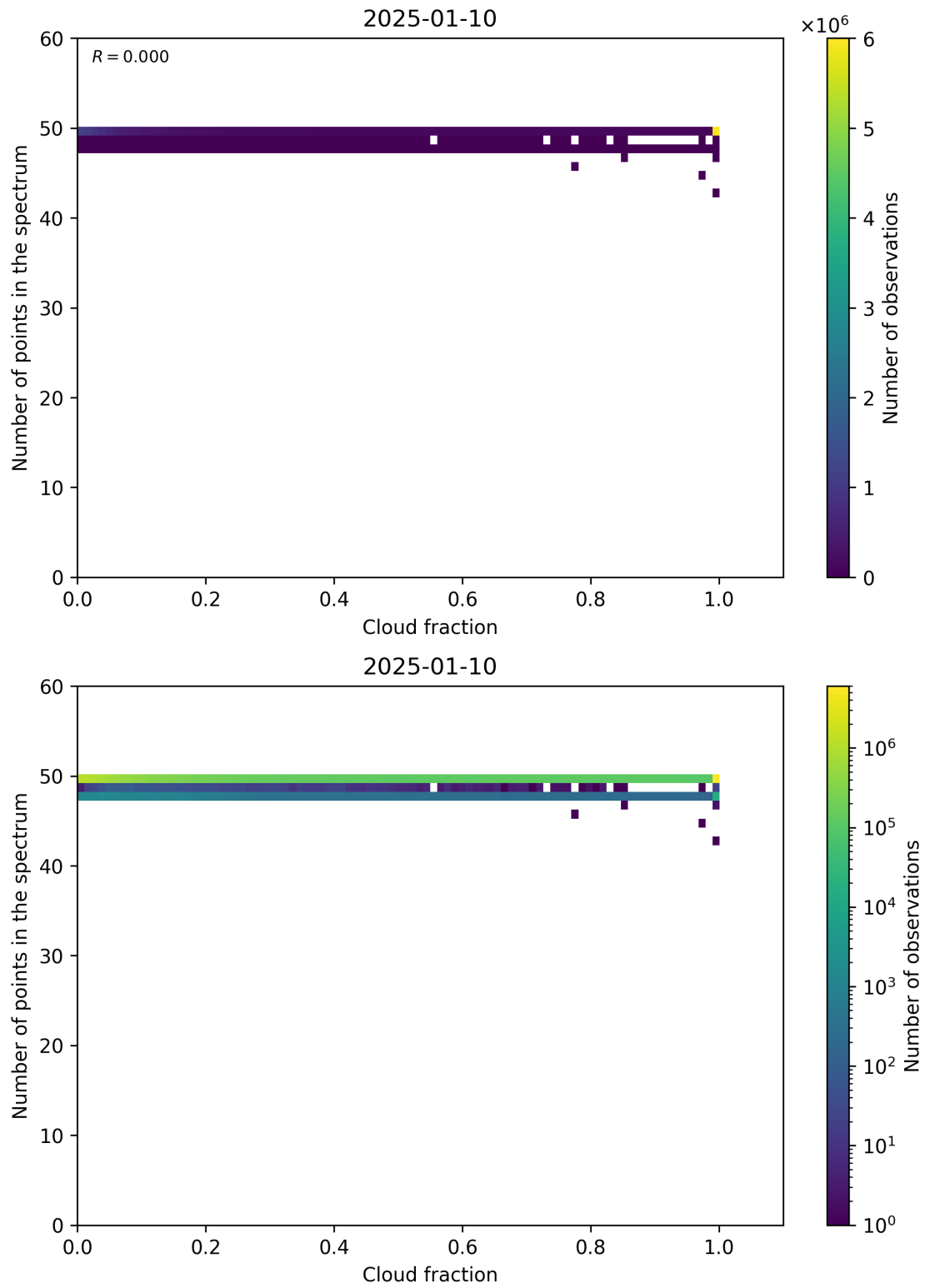
Figure 74: Scatter density plot of “Cloud fraction” against “Number of points in the spectrum” for 2025-01-09 to 2025-01-11.
