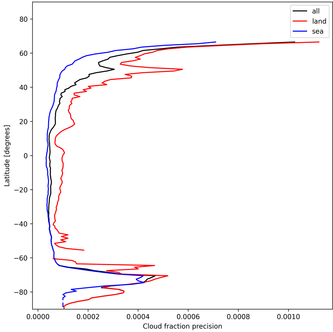
Figure 16: Zonal average of “Cloud fraction precision” for 2025-01-09 to 2025-01-11.
