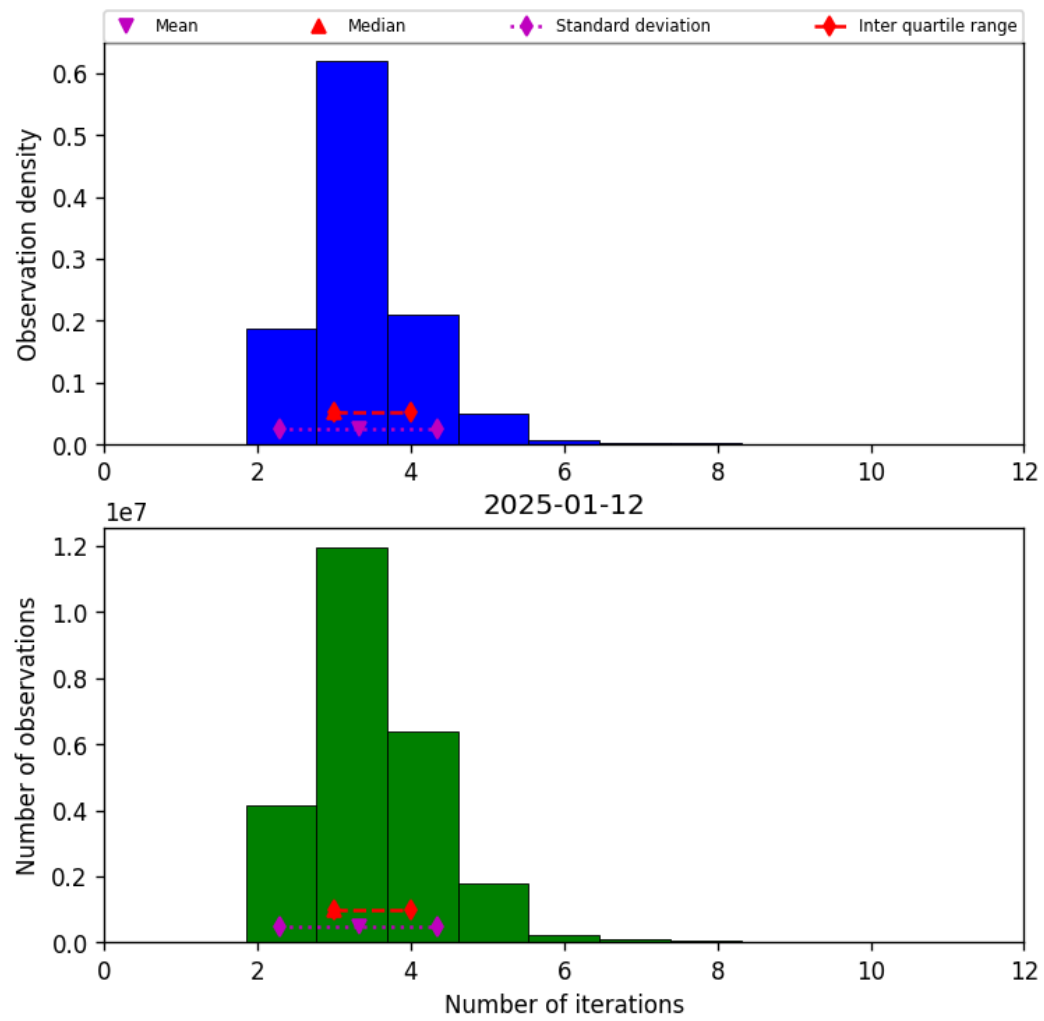
Figure 39: Histogram of “Number of iterations” for 2025-01-12 to 2025-01-13
