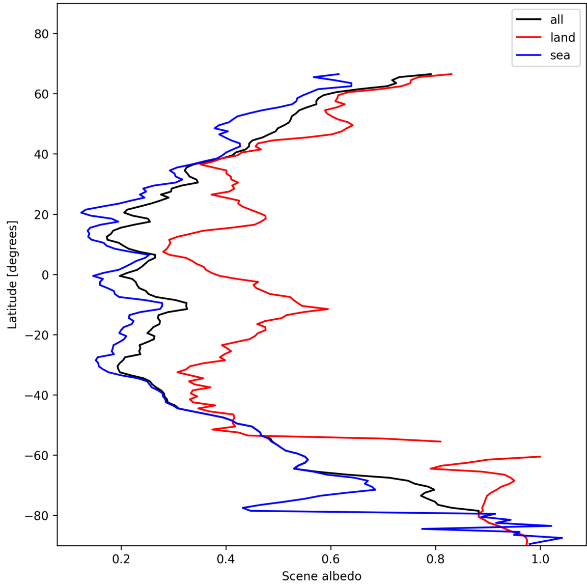
Figure 17: Zonal average of “Scene albedo” for 2025-01-12 to 2025-01-13.
