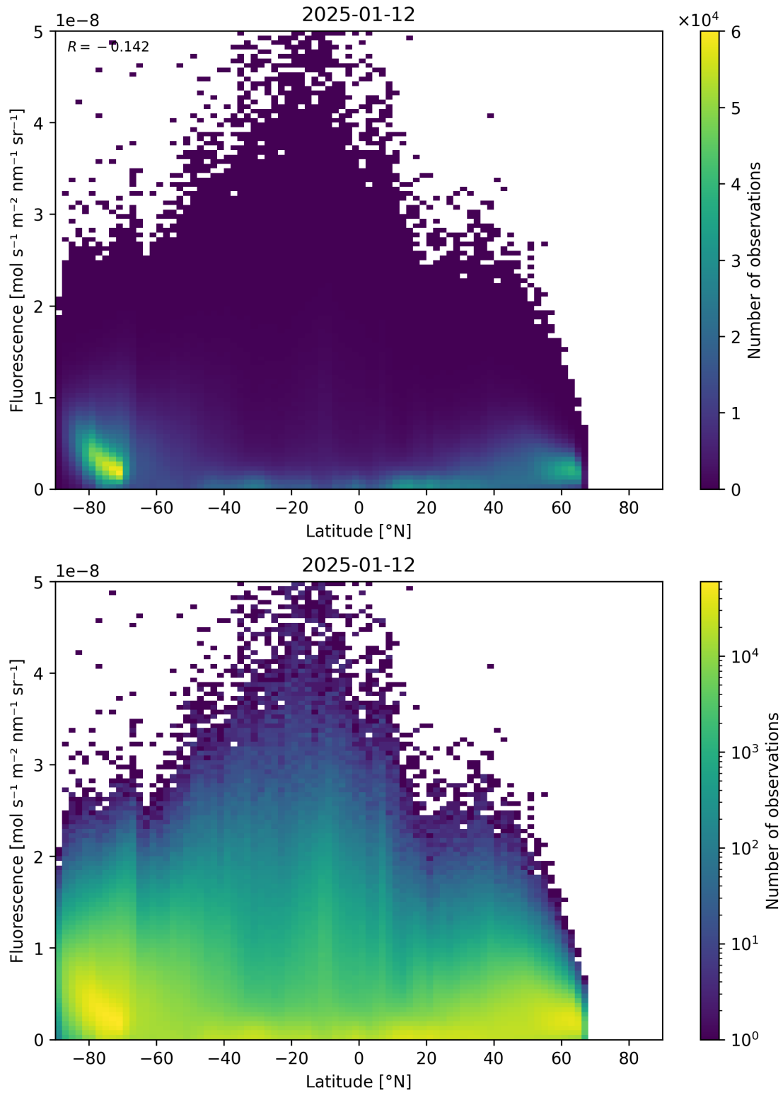
Figure 92: Scatter density plot of “Latitude” against “Fluorescence” for 2025-01-12 to 2025-01-13.
