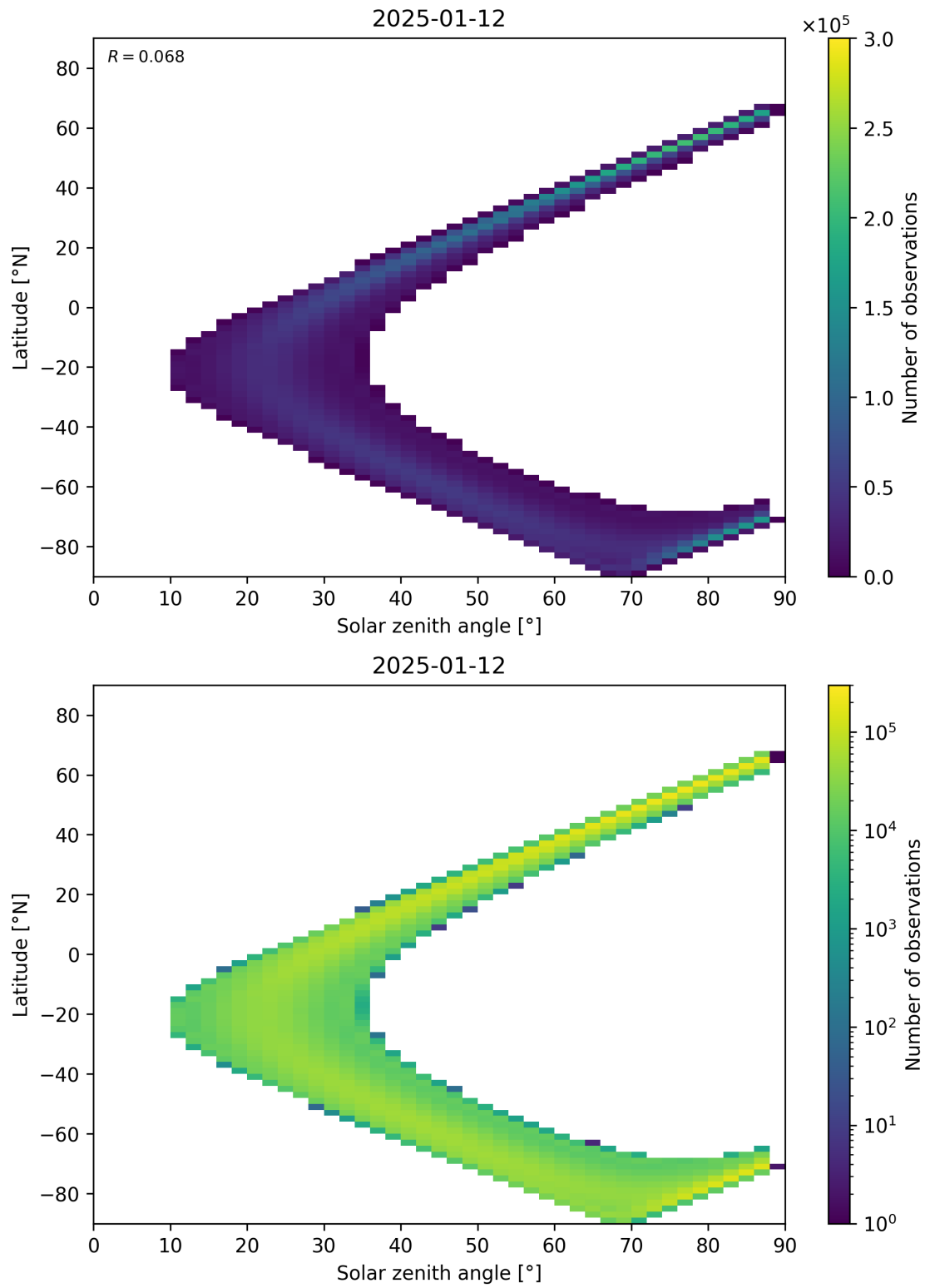
Figure 113: Scatter density plot of “Solar zenith angle” against “Latitude” for 2025-01-12 to 2025-01-13.
