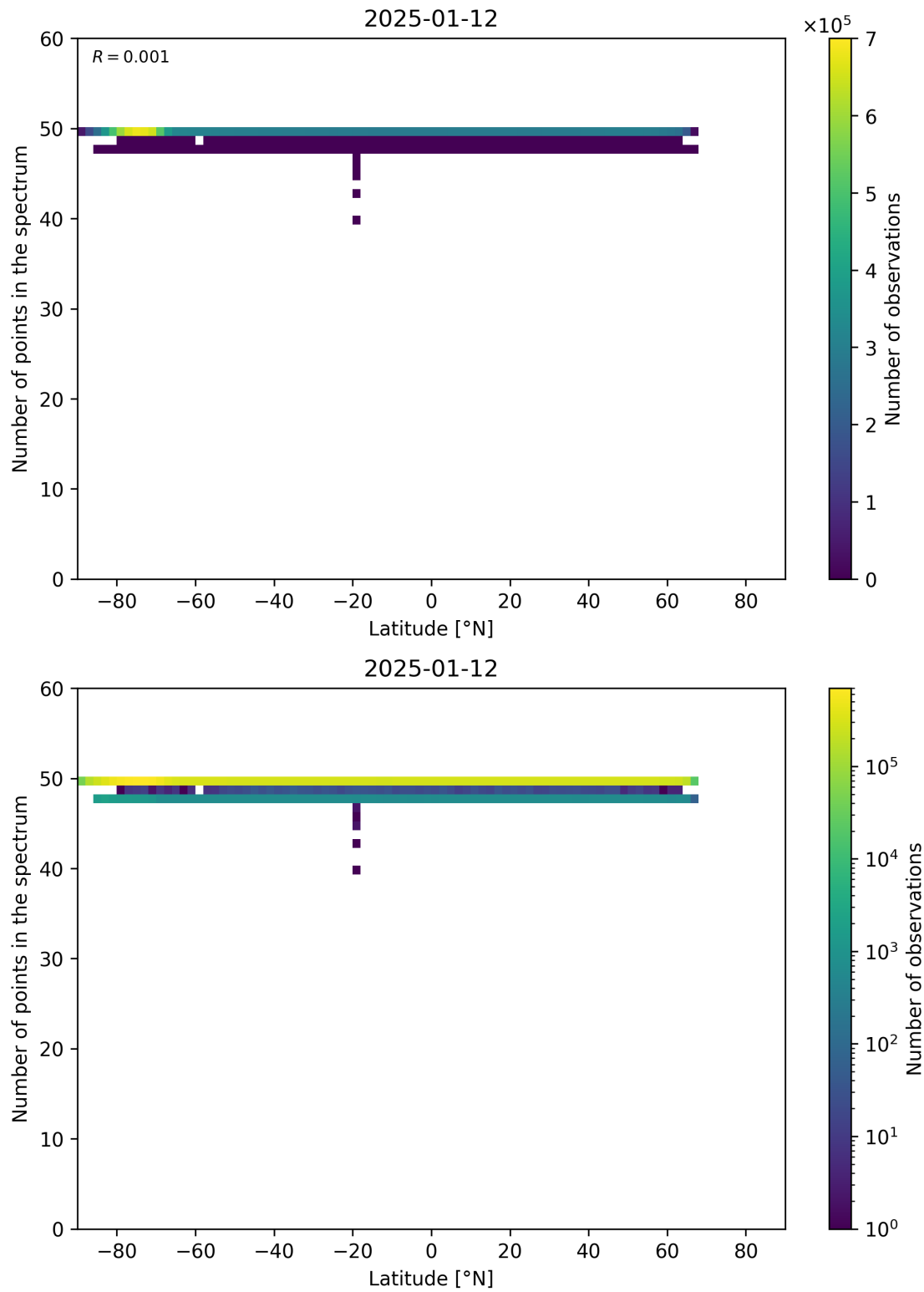
Figure 94: Scatter density plot of “Latitude” against “Number of points in the spectrum” for 2025-01-12 to 2025-01-13.
