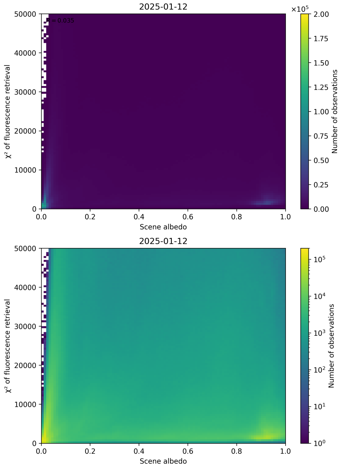
Figure 103: Scatter density plot of “Scene albedo” against “ \chi^2 of fluorescence retrieval” for 2025-01-12 to 2025-01-13.
