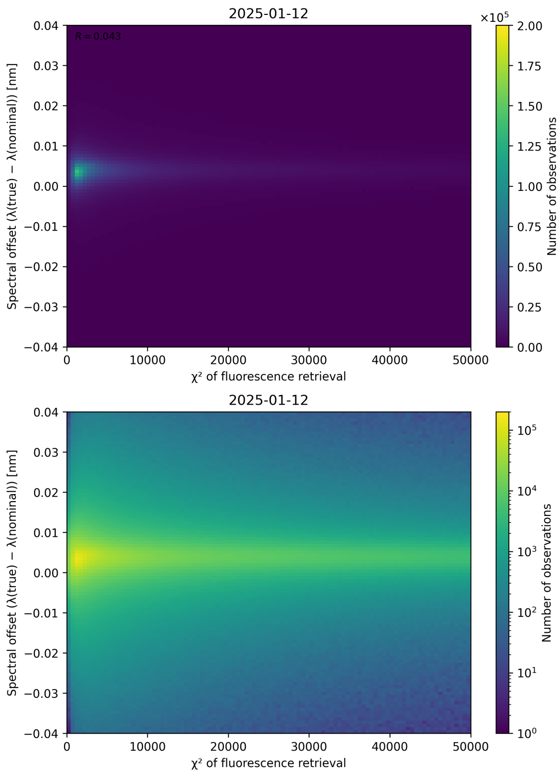
Figure 69: Scatter density plot of “ \chi^2 of fluorescence retrieval” against “Spectral offset ( \lambda_{\text{true}} - \lambda_{\text{nominal}} )” for 2025-01-12 to 2025-01-13.
