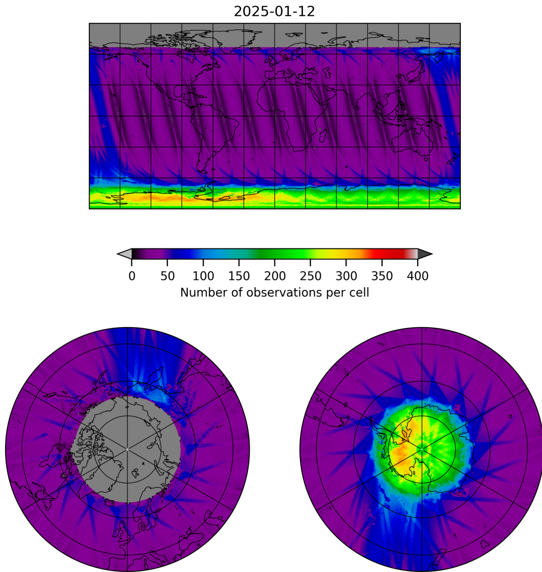
Figure 11: Map of the number of observations for 2025-01-12 to 2025-01-13
