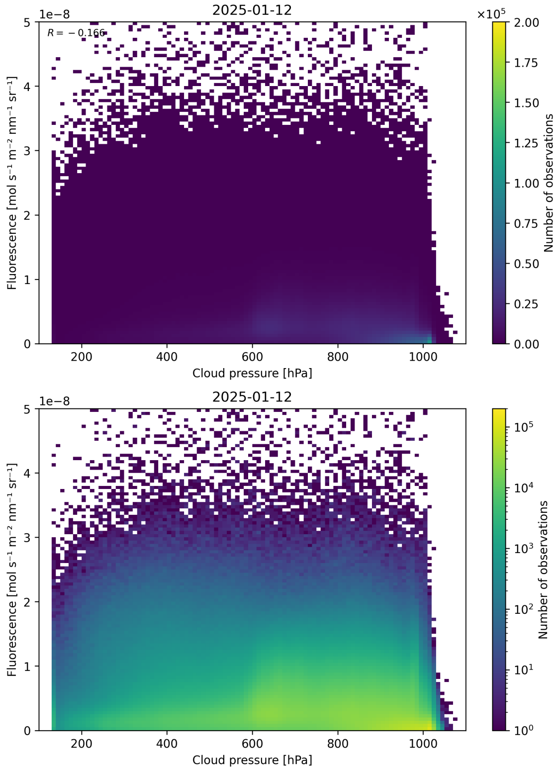
Figure 80: Scatter density plot of “Cloud pressure” against “Fluorescence” for 2025-01-12 to 2025-01-13.
