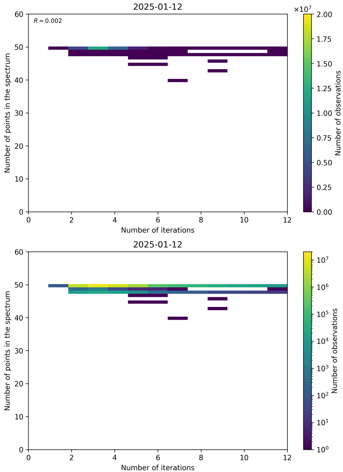
Figure 99: Scatter density plot of “Number of iterations” against “Number of points in the spectrum” for 2025-01-12 to 2025-01-13.
