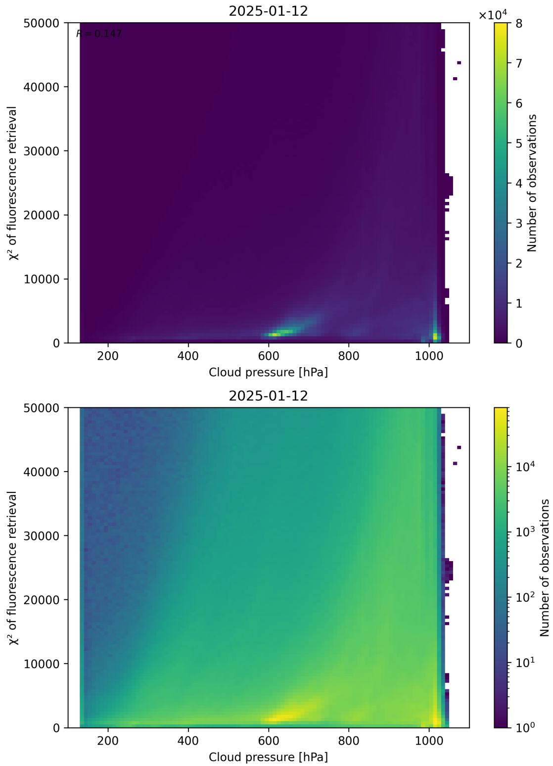
Figure 78: Scatter density plot of “Cloud pressure” against “ \chi^2 of fluorescence retrieval” for 2025-01-12 to 2025-01-13.
