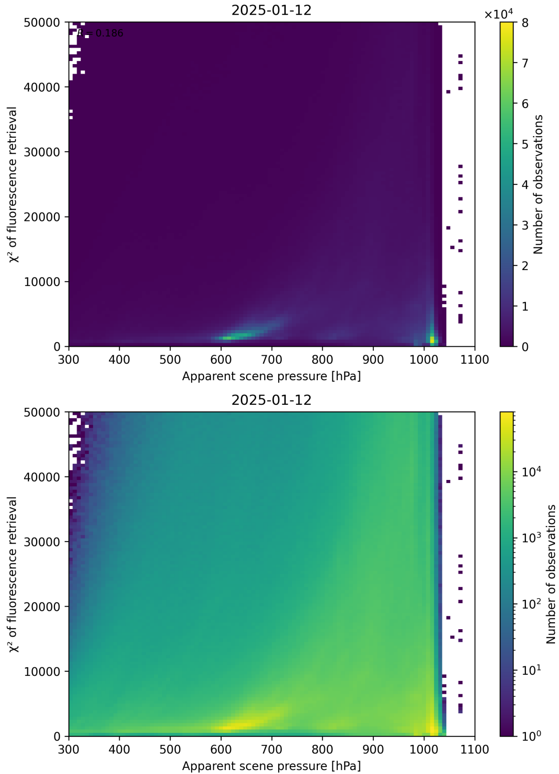
Figure 63: Scatter density plot of “Apparent scene pressure” against “ \chi^2 of fluorescence retrieval” for 2025-01-12 to 2025-01-13.
