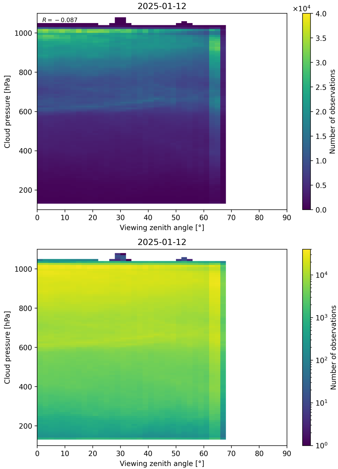
Figure 121: Scatter density plot of “Viewing zenith angle” against “Cloud pressure” for 2025-01-12 to 2025-01-13.
