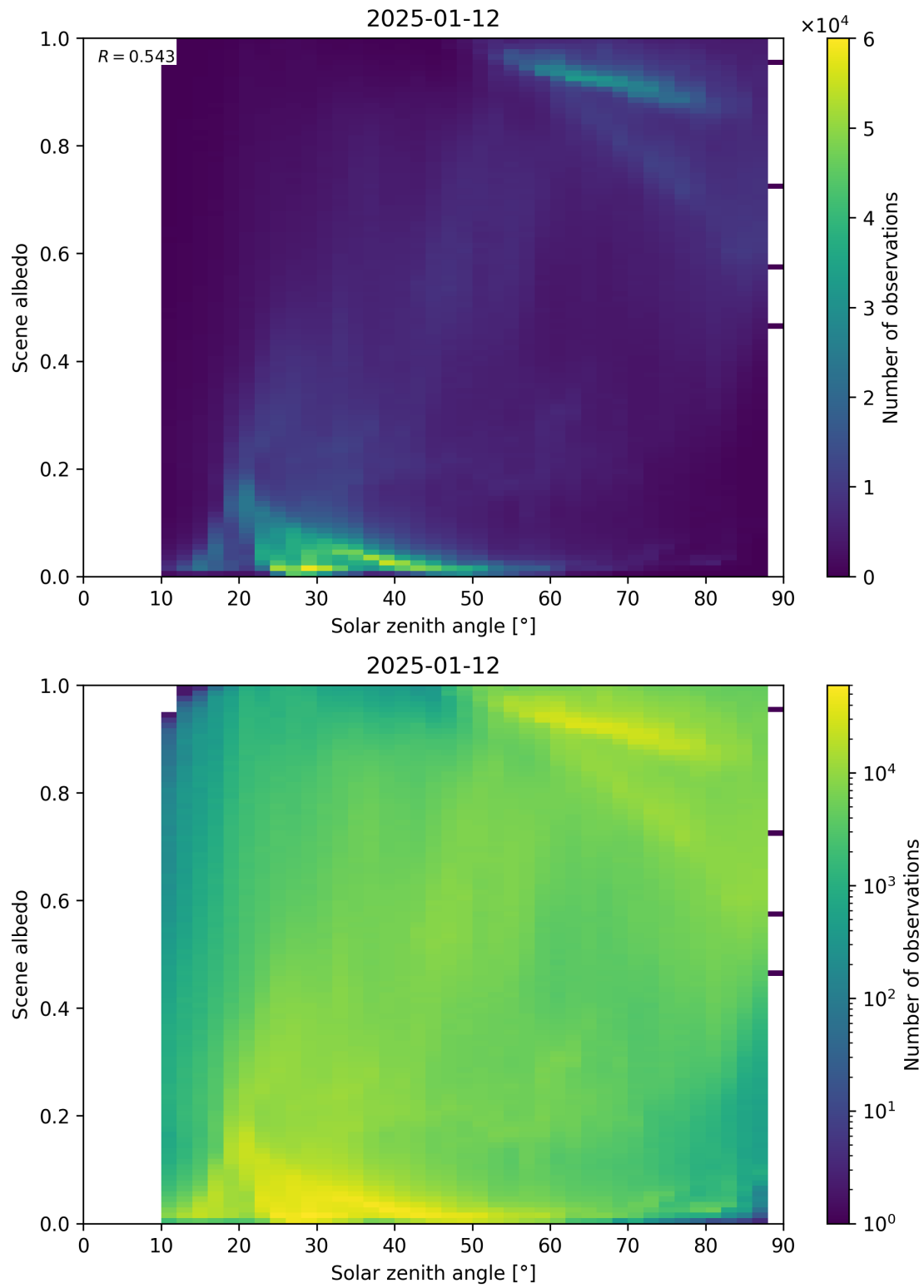
Figure 116: Scatter density plot of “Solar zenith angle” against “Scene albedo” for 2025-01-12 to 2025-01-13.
