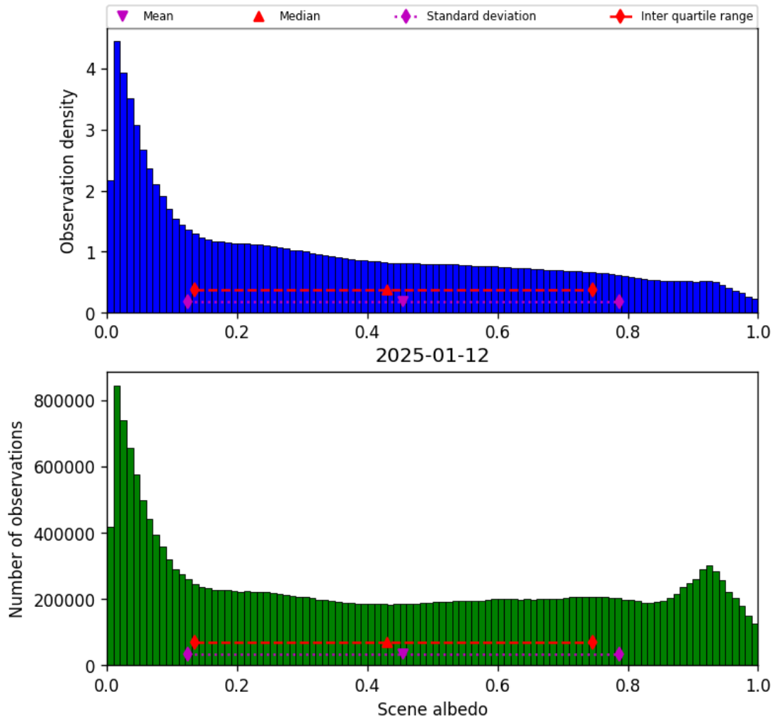
Figure 34: Histogram of “Scene albedo” for 2025-01-12 to 2025-01-13
