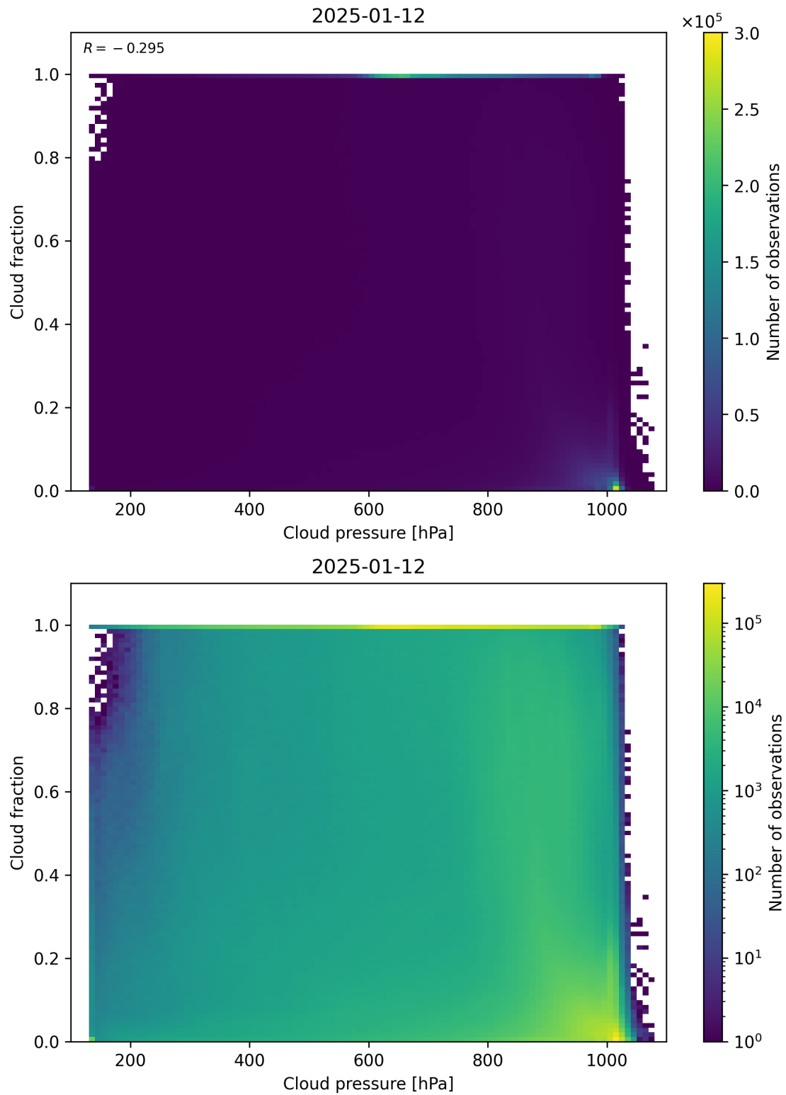
Figure 79: Scatter density plot of “Cloud pressure” against “Cloud fraction” for 2025-01-12 to 2025-01-13.
