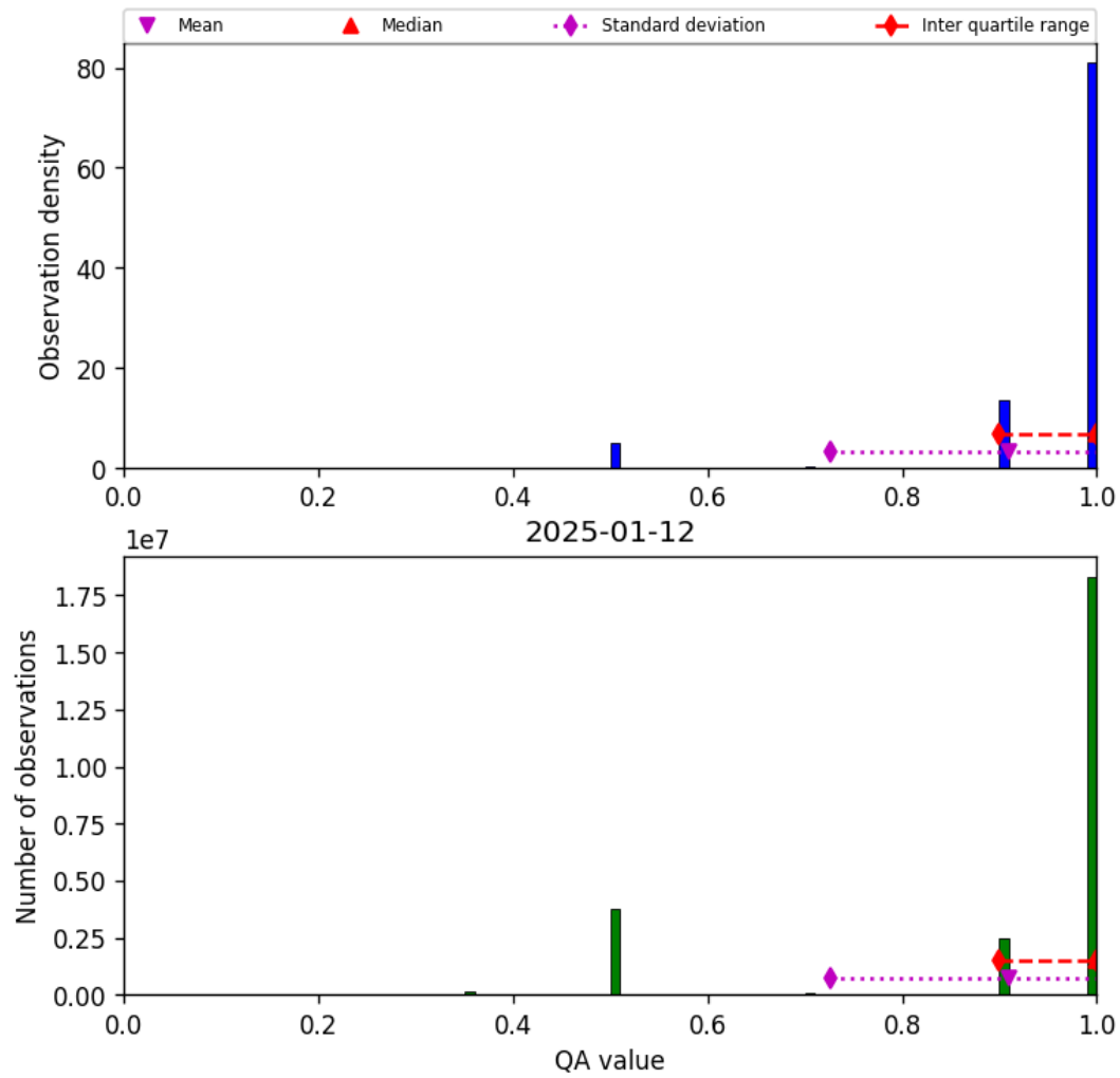
Figure 29: Histogram of “QA value” for 2025-01-12 to 2025-01-13
