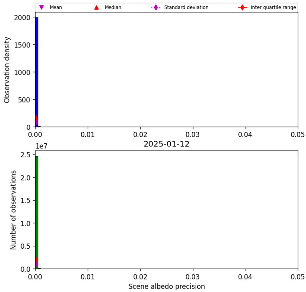
Figure 35: Histogram of “Scene albedo precision” for 2025-01-12 to 2025-01-13
