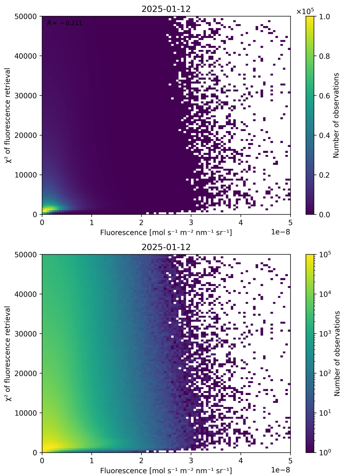
Figure 85: Scatter density plot of “Fluorescence” against “ \chi^2 of fluorescence retrieval” for 2025-01-12 to 2025-01-13.
