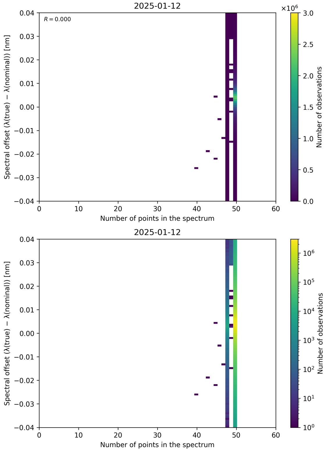
Figure 101: Scatter density plot of “Number of points in the spectrum” against “Spectral offset ( \lambda_{\text{true}} - \lambda_{\text{nominal}} )” for 2025-01-12 to 2025-01-13.
