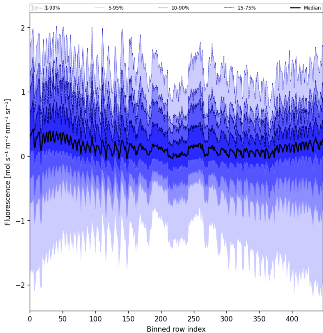
Figure 57: Along track statistics of "Fluorescence" for 2025-01-12 to 2025-01-13
