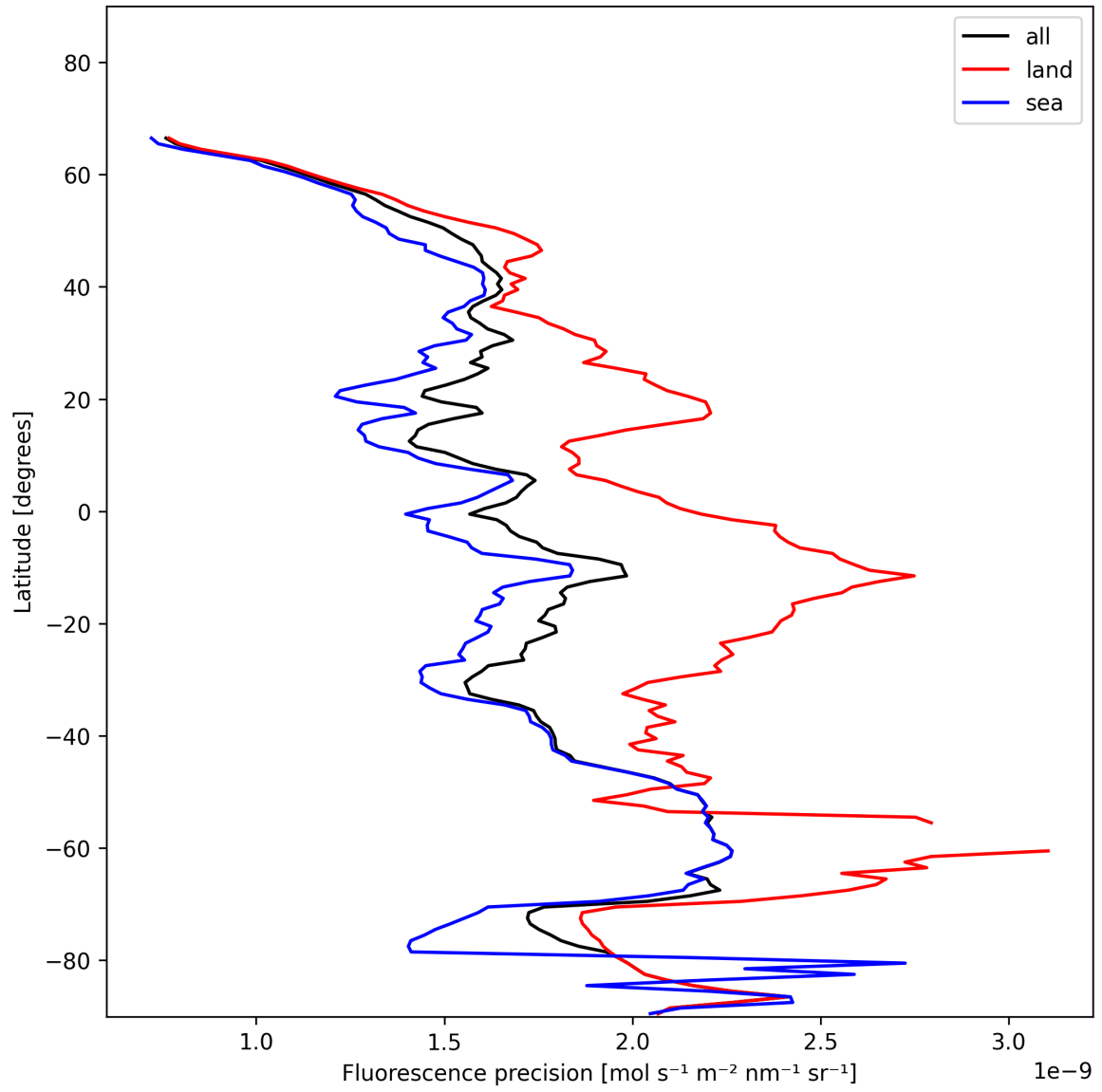
Figure 24: Zonal average of “Fluorescence precision” for 2025-01-12 to 2025-01-13.
