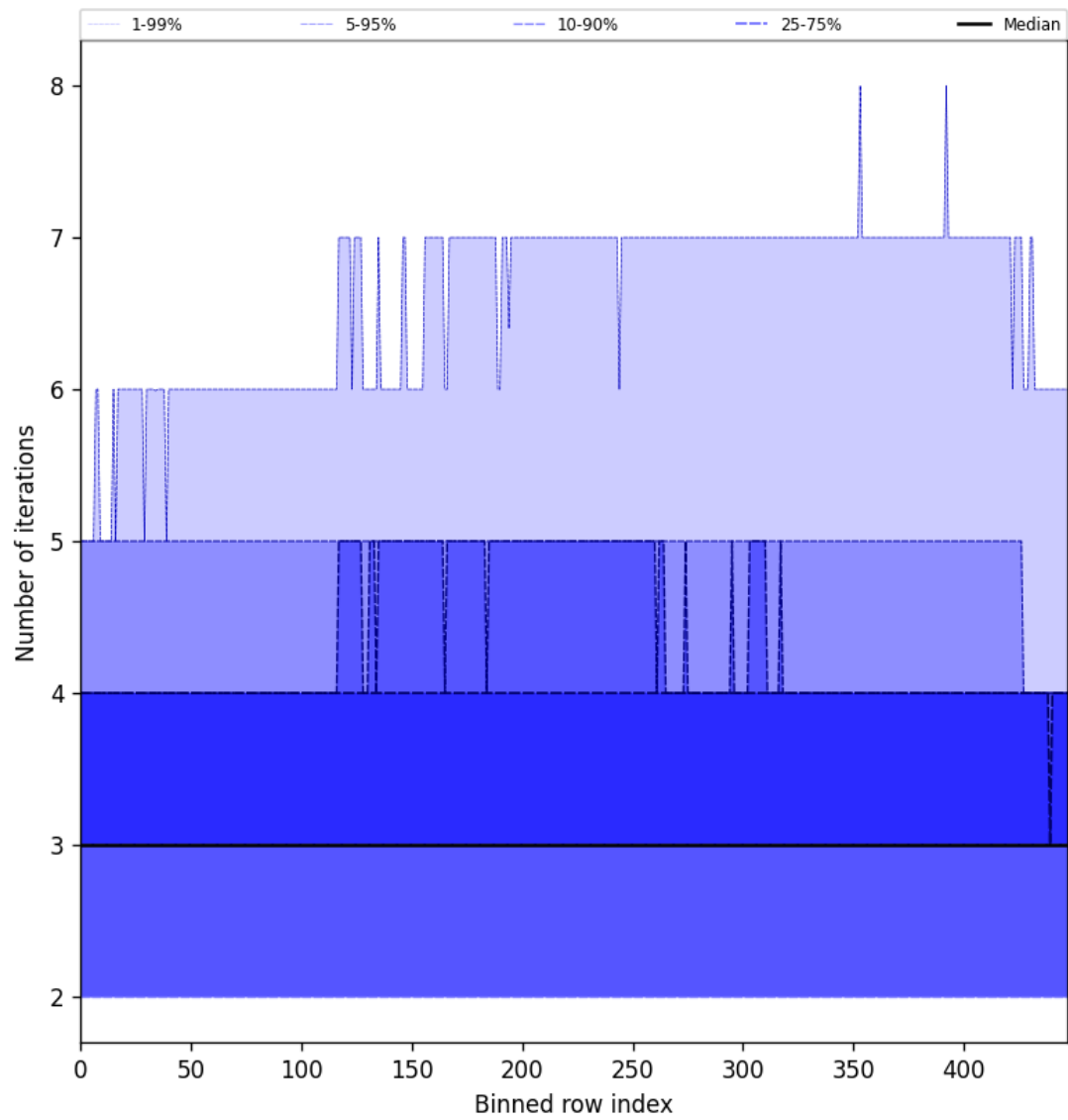
Figure 56: Along track statistics of “Number of iterations” for 2025-01-12 to 2025-01-13
