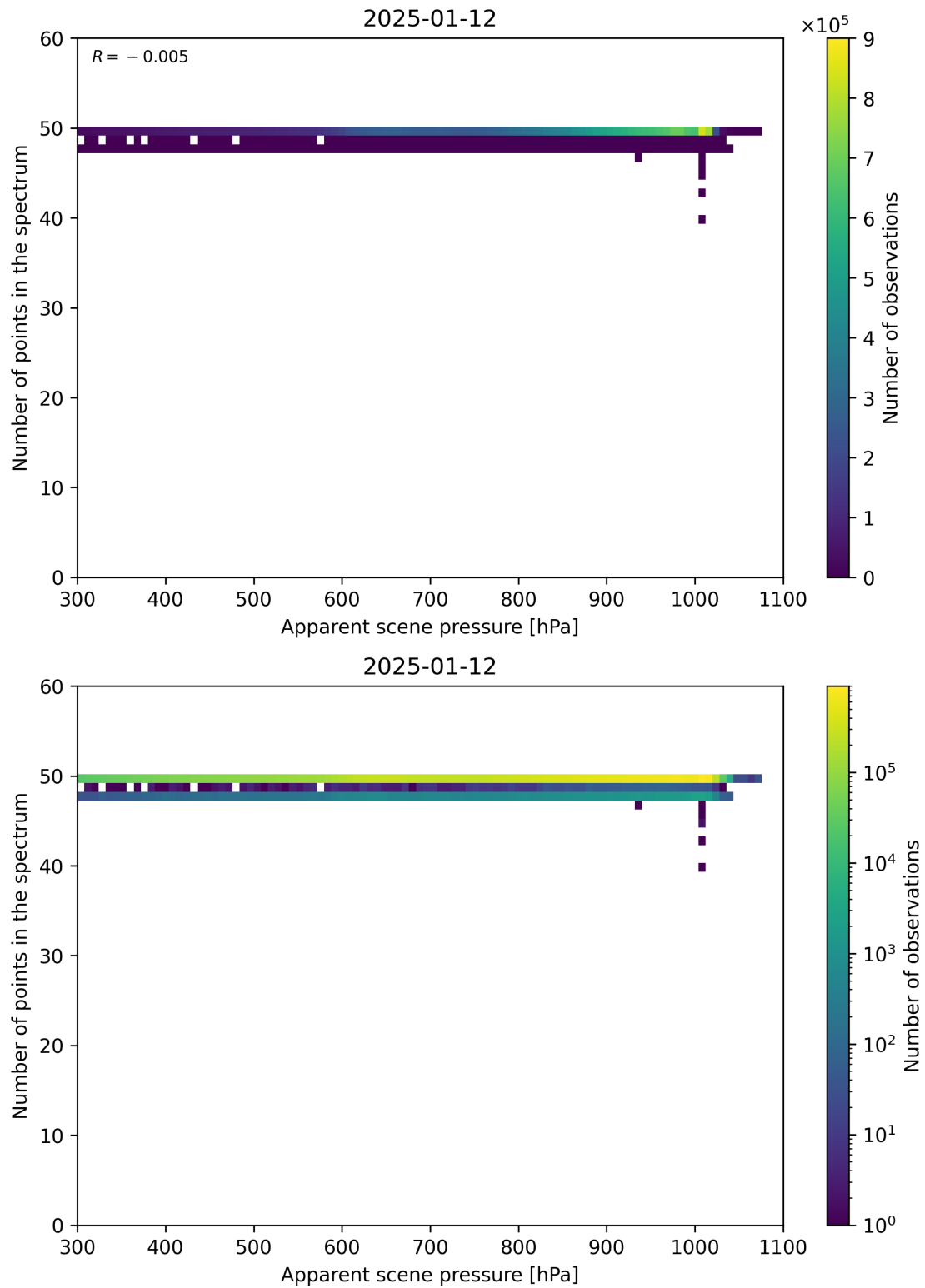
Figure 66: Scatter density plot of “Apparent scene pressure” against “Number of points in the spectrum” for 2025-01-12 to 2025-01-13.
