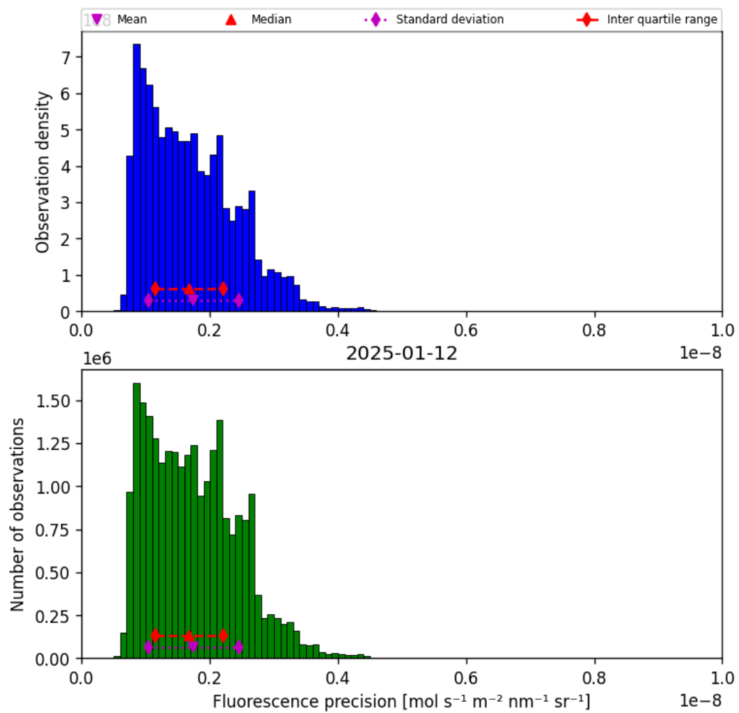
Figure 41: Histogram of “Fluorescence precision” for 2025-01-12 to 2025-01-13
