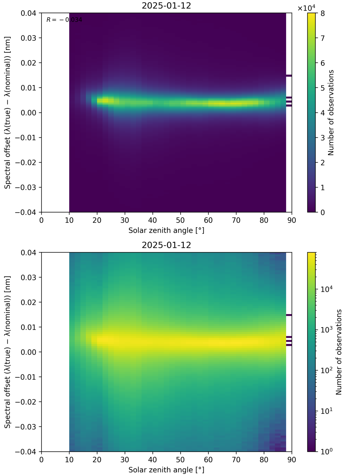
Figure 117: Scatter density plot of “Solar zenith angle” against “Spectral offset ( \lambda_{\text{true}} - \lambda_{\text{nominal}} )” for 2025-01-12 to 2025-01-13.
