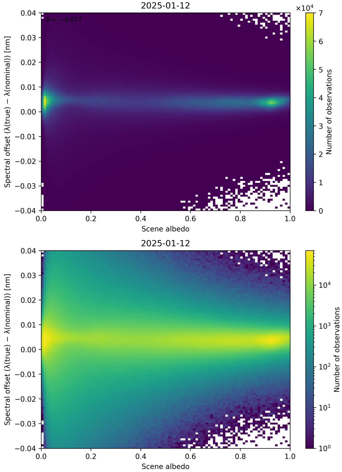
Figure 107: Scatter density plot of “Scene albedo” against “Spectral offset ( \lambda_{\text{true}} - \lambda_{\text{nominal}} )” for 2025-01-12 to 2025-01-13.
