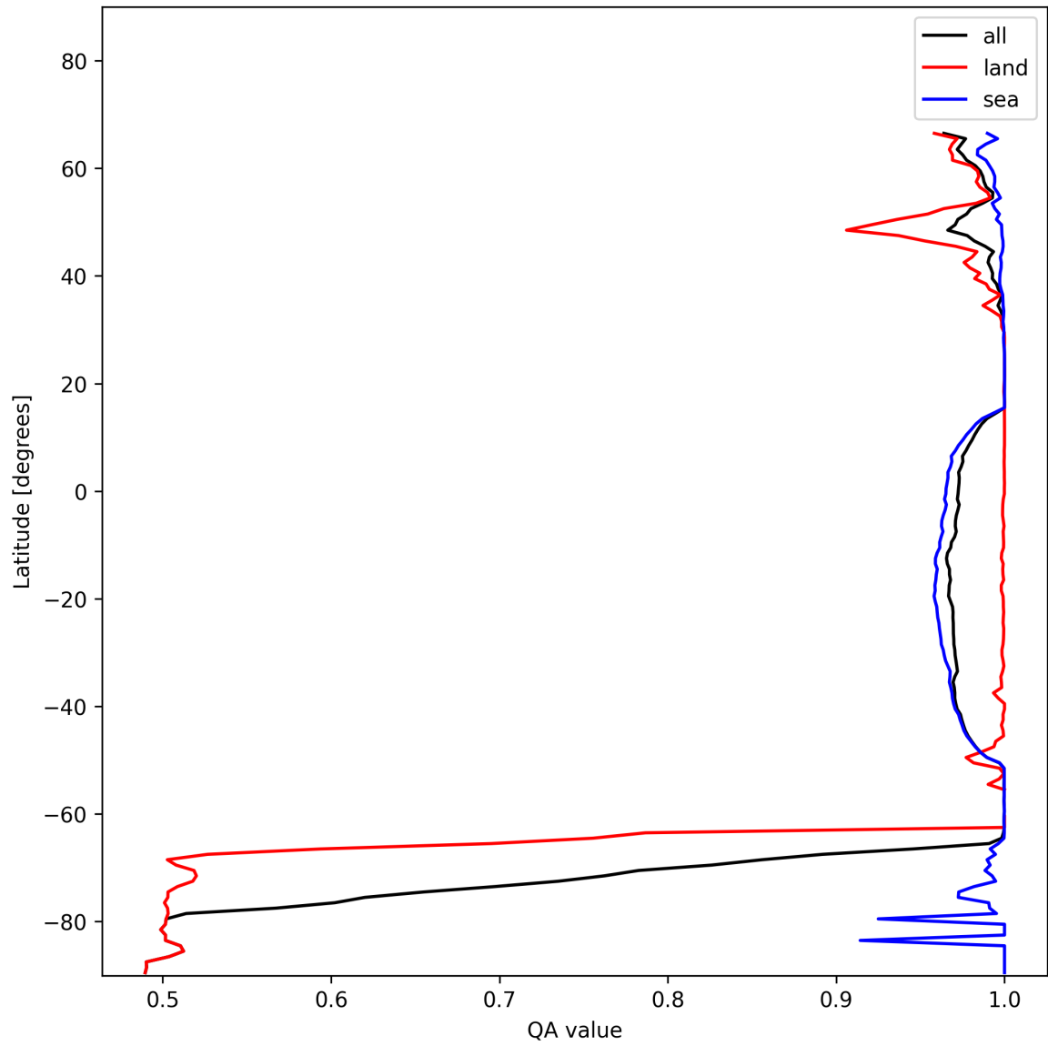
Figure 12: Zonal average of “QA value” for 2025-01-12 to 2025-01-13.
