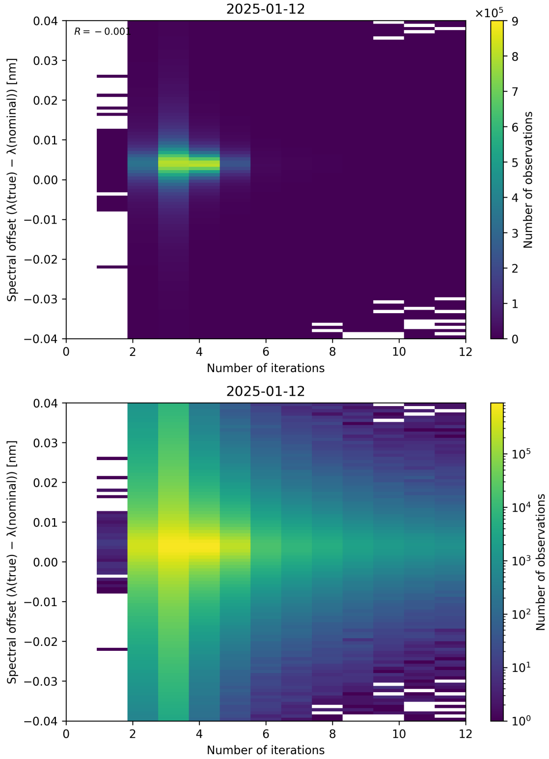
Figure 100: Scatter density plot of “Number of iterations” against “Spectral offset ( \lambda_{\text{true}} - \lambda_{\text{nominal}} )” for 2025-01-12 to 2025-01-13.
