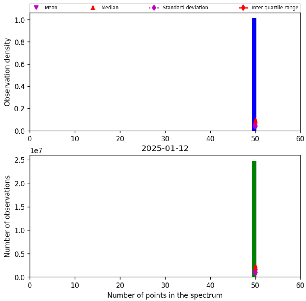
Figure 44: Histogram of “Number of points in the spectrum” for 2025-01-12 to 2025-01-13
