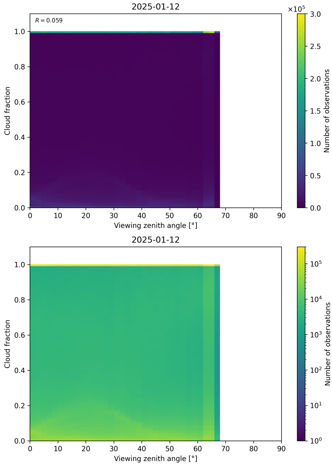
Figure 120: Scatter density plot of “Viewing zenith angle” against “Cloud fraction” for 2025-01-12 to 2025-01-13.
