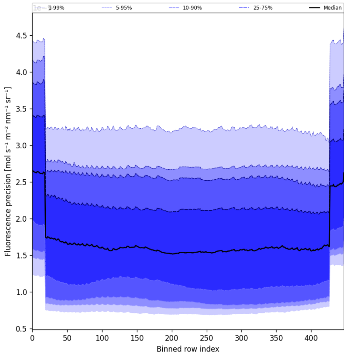
Figure 58: Along track statistics of “Fluorescence precision” for 2025-01-12 to 2025-01-13
