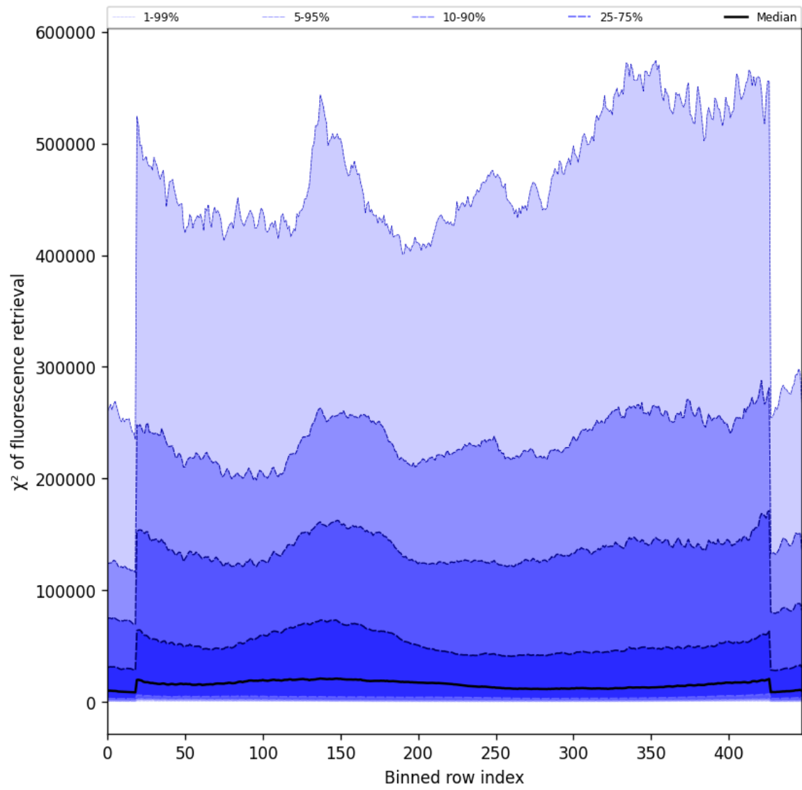
Figure 59: Along track statistics of “ \chi^2 of fluorescence retrieval” for 2025-01-12 to 2025-01-13
