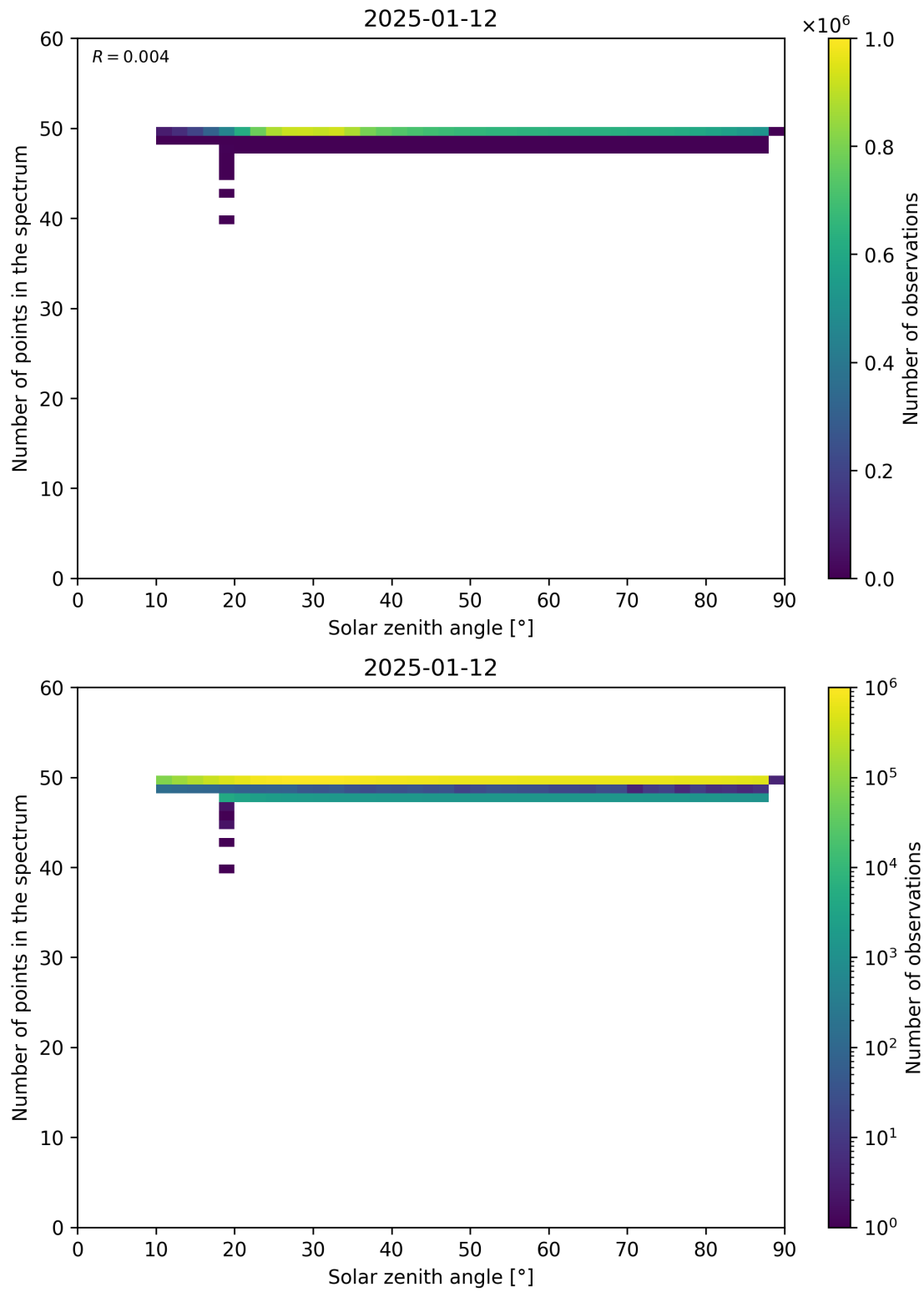
Figure 115: Scatter density plot of “Solar zenith angle” against “Number of points in the spectrum” for 2025-01-12 to 2025-01-13.
