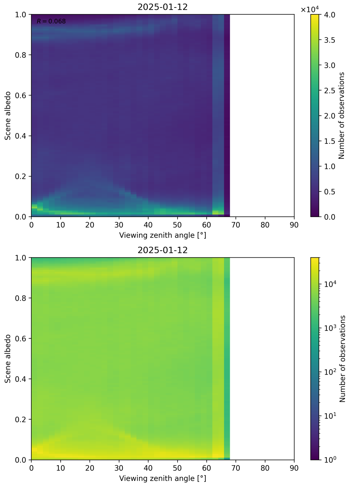
Figure 126: Scatter density plot of “Viewing zenith angle” against “Scene albedo” for 2025-01-12 to 2025-01-13.
