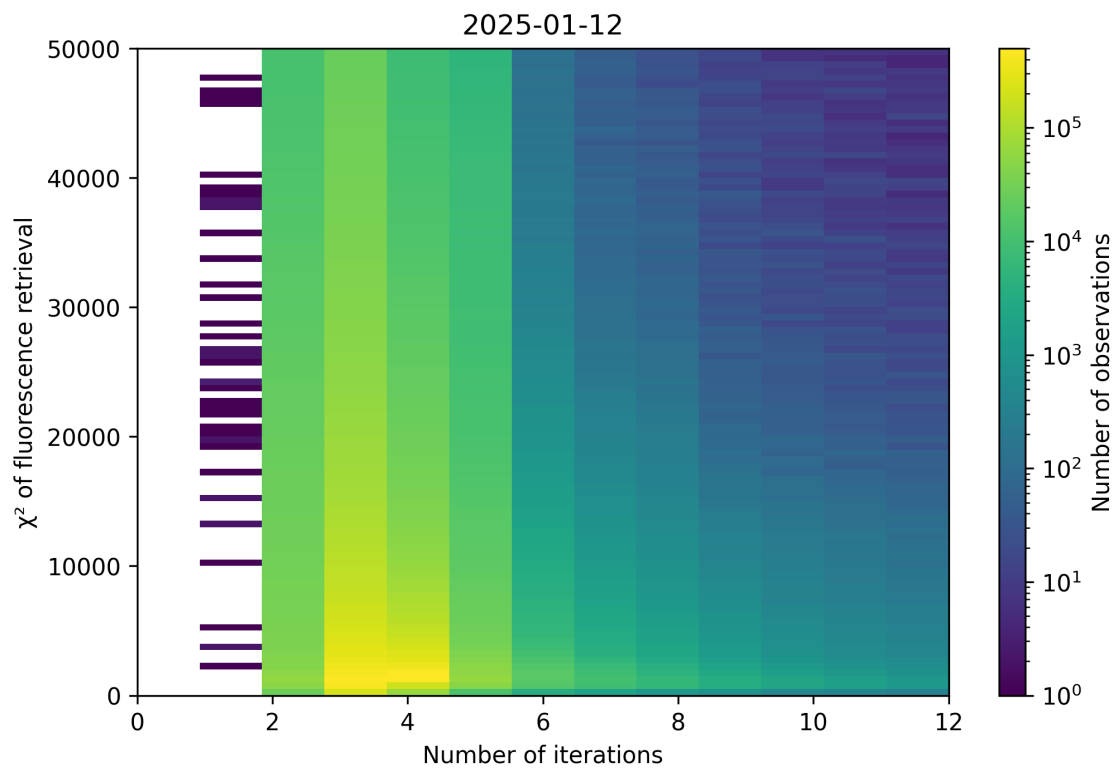
Figure 97: Scatter density plot of “Number of iterations” against “ \chi^2 of fluorescence retrieval” for 2025-01-12 to 2025-01-13.
