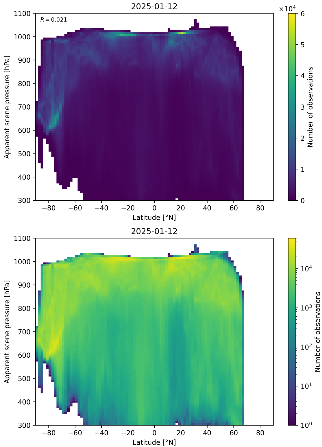
Figure 88: Scatter density plot of “Latitude” against “Apparent scene pressure” for 2025-01-12 to 2025-01-13.
