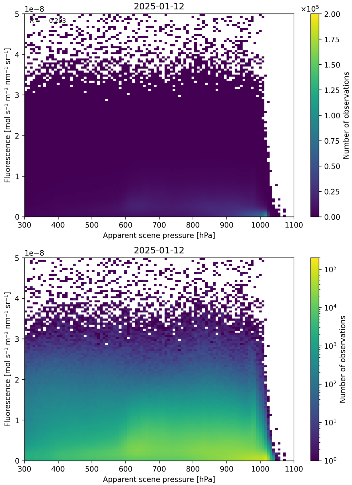
Figure 64: Scatter density plot of “Apparent scene pressure” against “Fluorescence” for 2025-01-12 to 2025-01-13.
