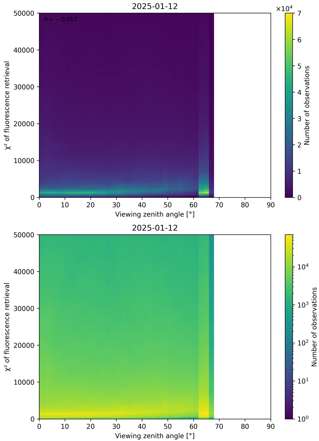
Figure 119: Scatter density plot of “Viewing zenith angle” against “ \chi^2 of fluorescence retrieval” for 2025-01-12 to 2025-01-13.
