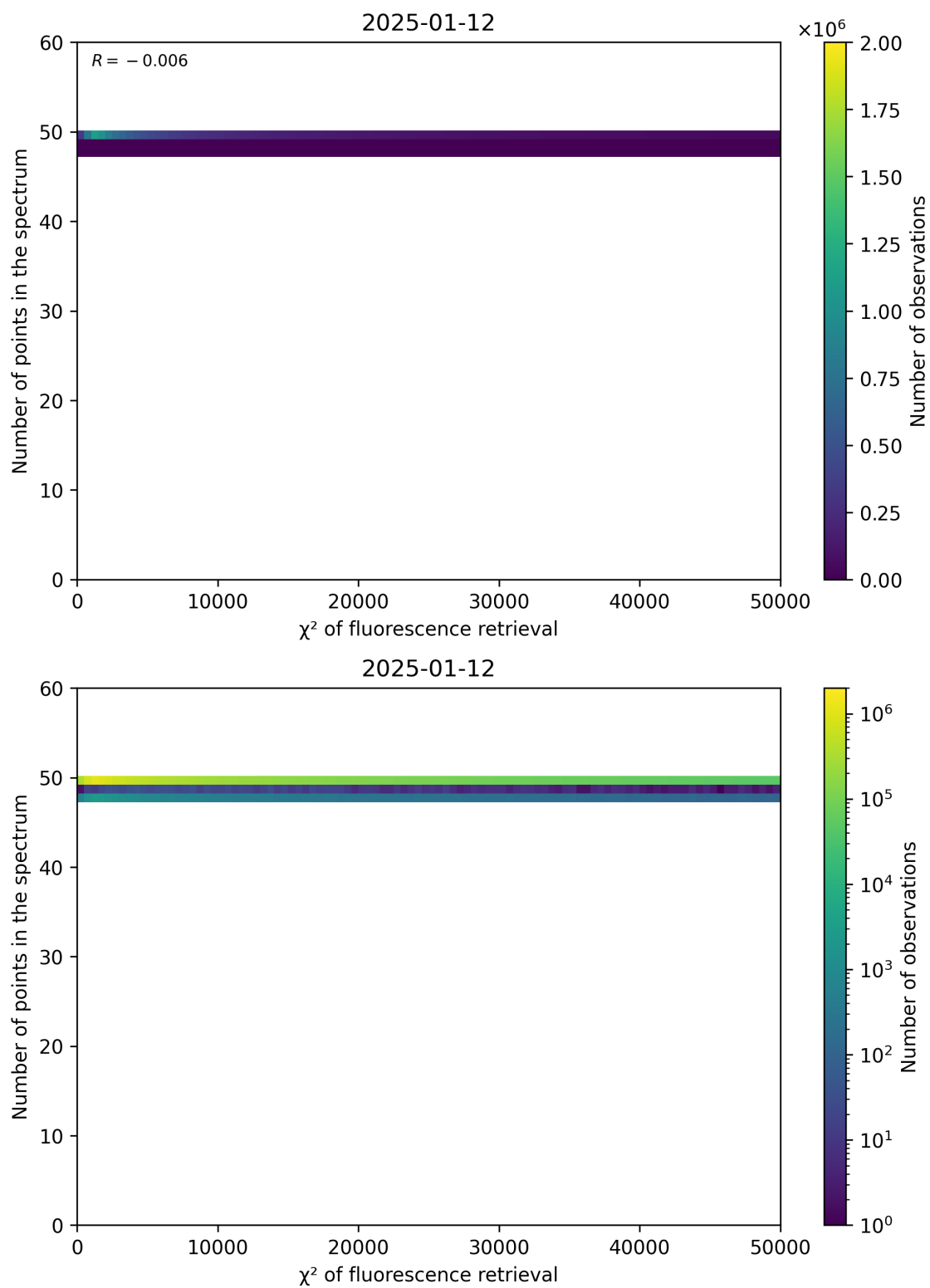
Figure 68: Scatter density plot of “ \chi^2 of fluorescence retrieval” against “Number of points in the spectrum” for 2025-01-12 to 2025-01-13.
