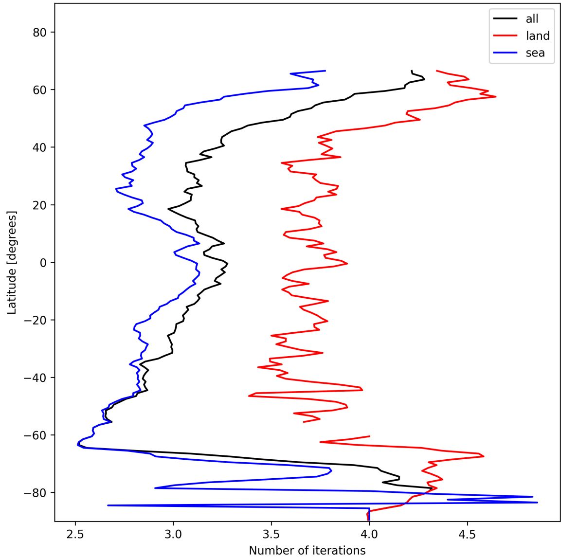
Figure 22: Zonal average of “Number of iterations” for 2025-01-12 to 2025-01-13.
