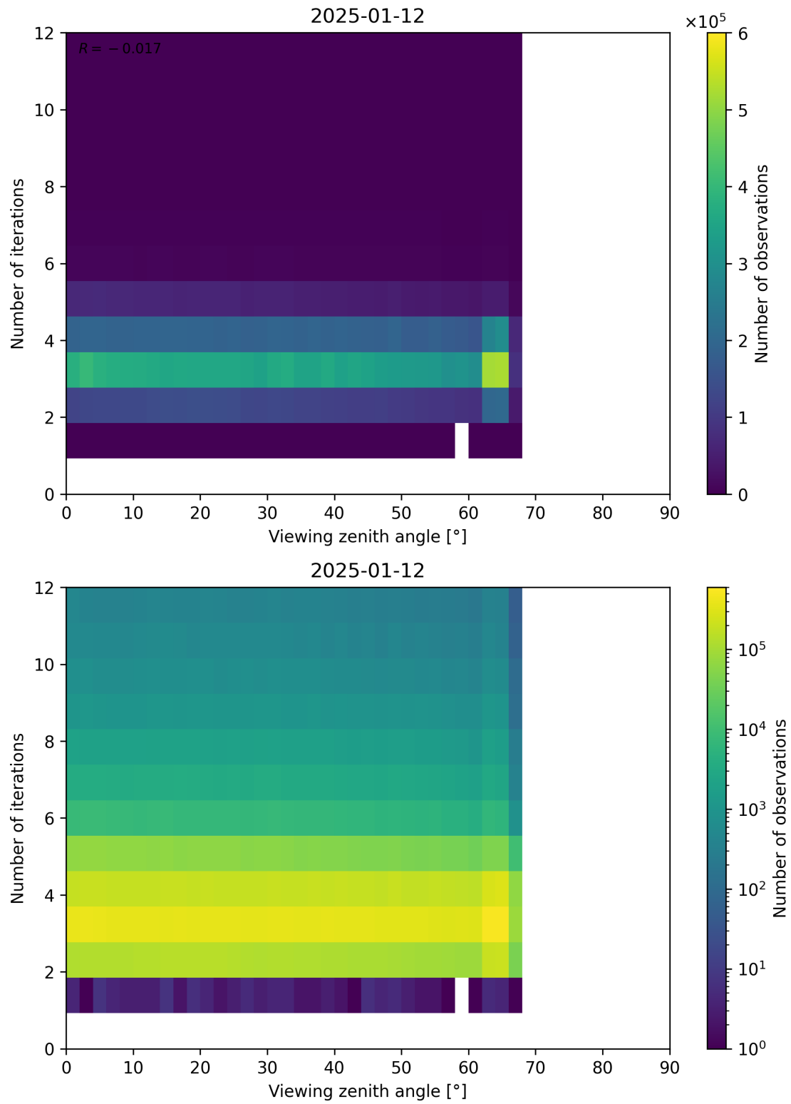
Figure 124: Scatter density plot of “Viewing zenith angle” against “Number of iterations” for 2025-01-12 to 2025-01-13.
