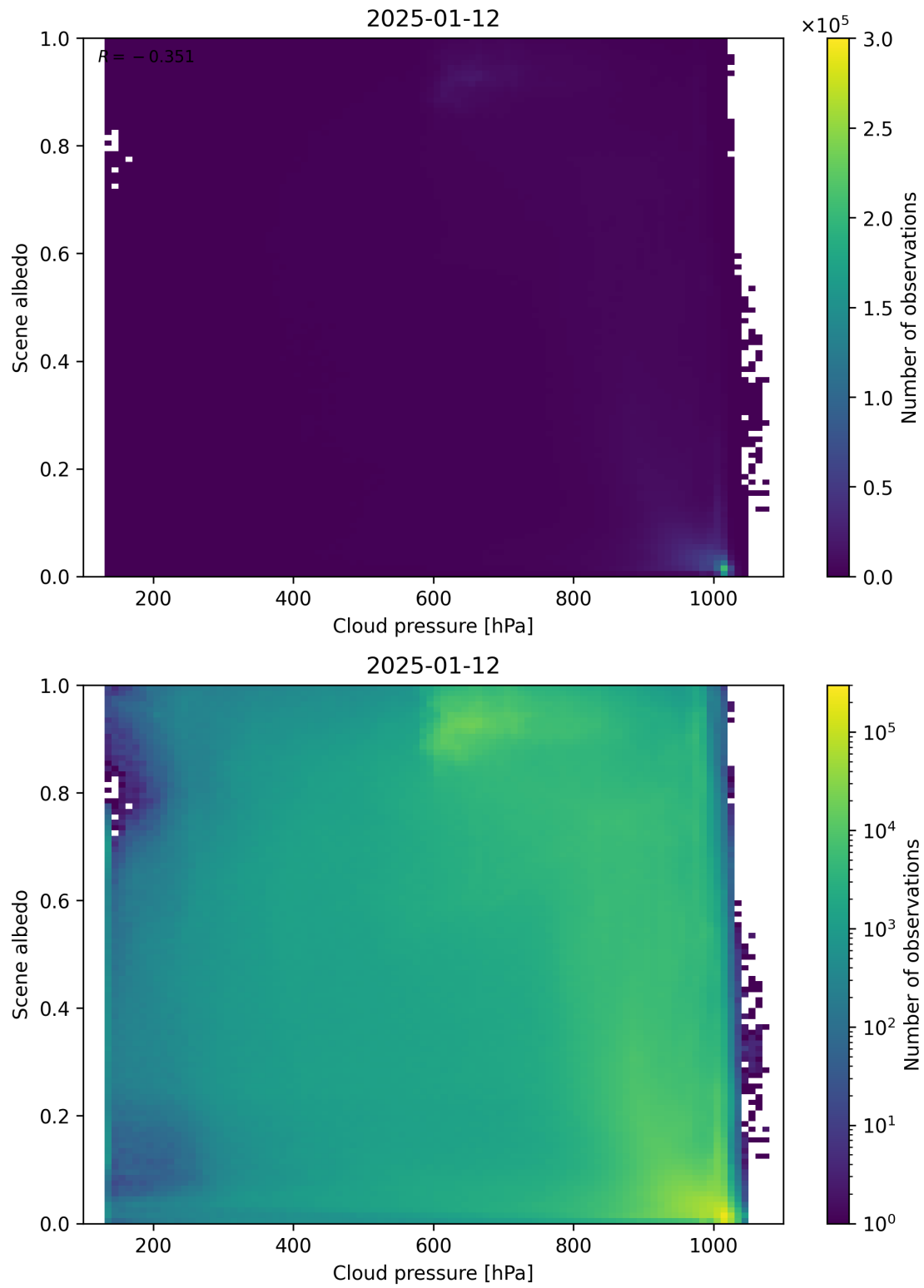
Figure 83: Scatter density plot of “Cloud pressure” against “Scene albedo” for 2025-01-12 to 2025-01-13.
