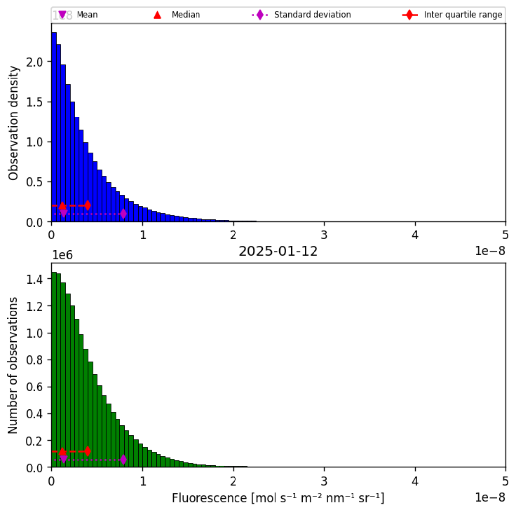
Figure 40: Histogram of “Fluorescence” for 2025-01-12 to 2025-01-13
