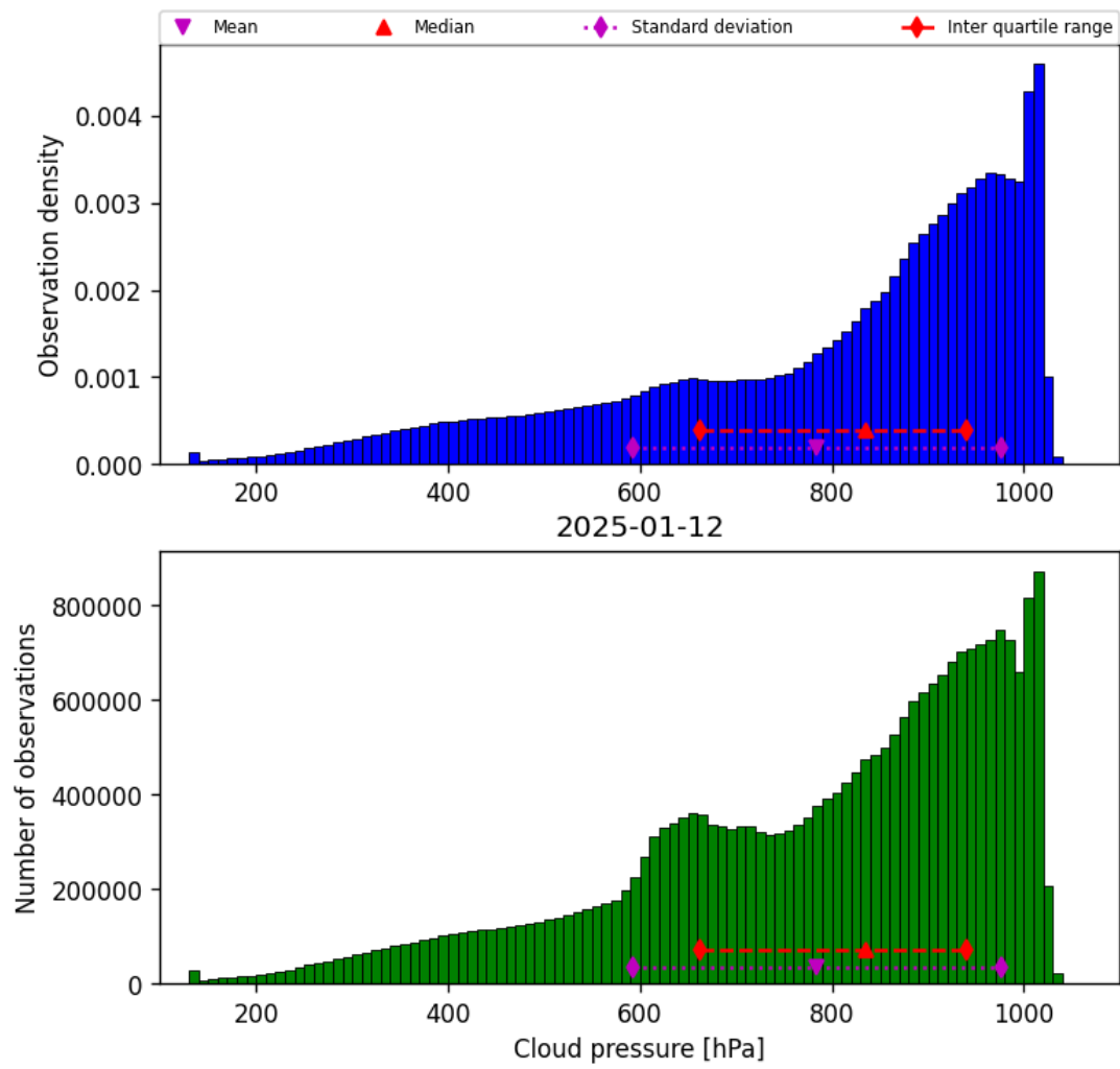
Figure 30: Histogram of “Cloud pressure” for 2025-01-12 to 2025-01-13
