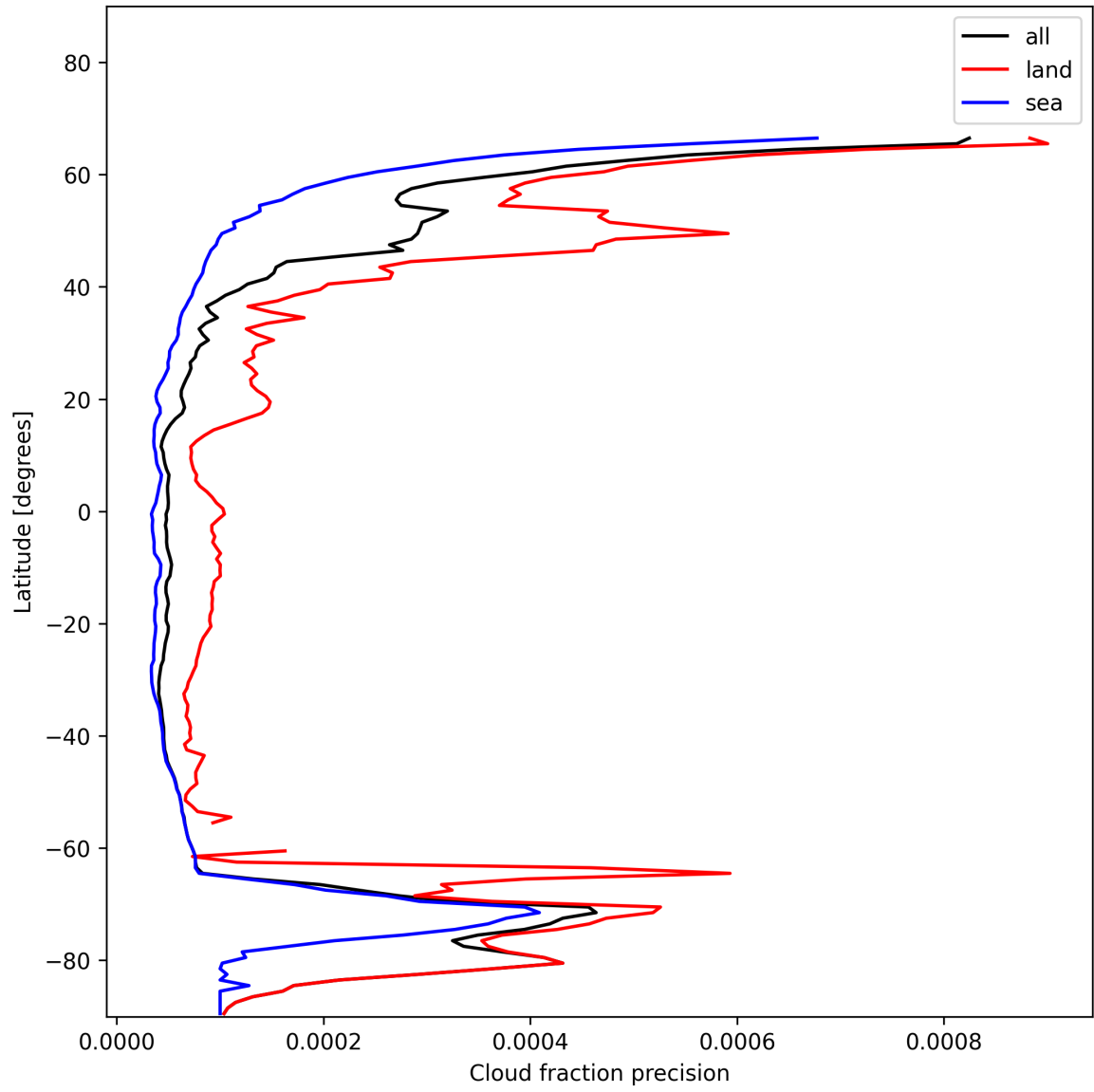
Figure 16: Zonal average of “Cloud fraction precision” for 2025-01-12 to 2025-01-13.
