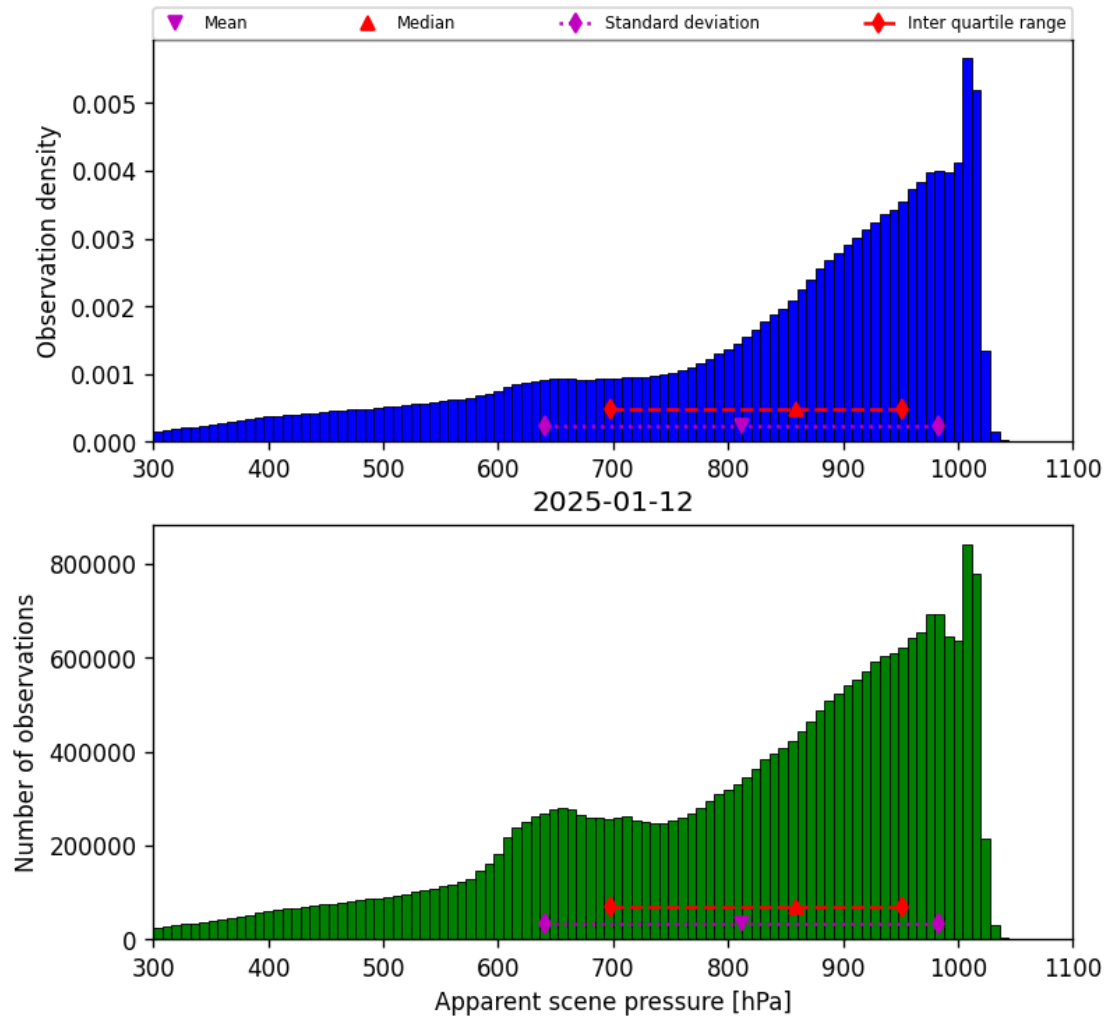
Figure 36: Histogram of “Apparent scene pressure” for 2025-01-12 to 2025-01-13
