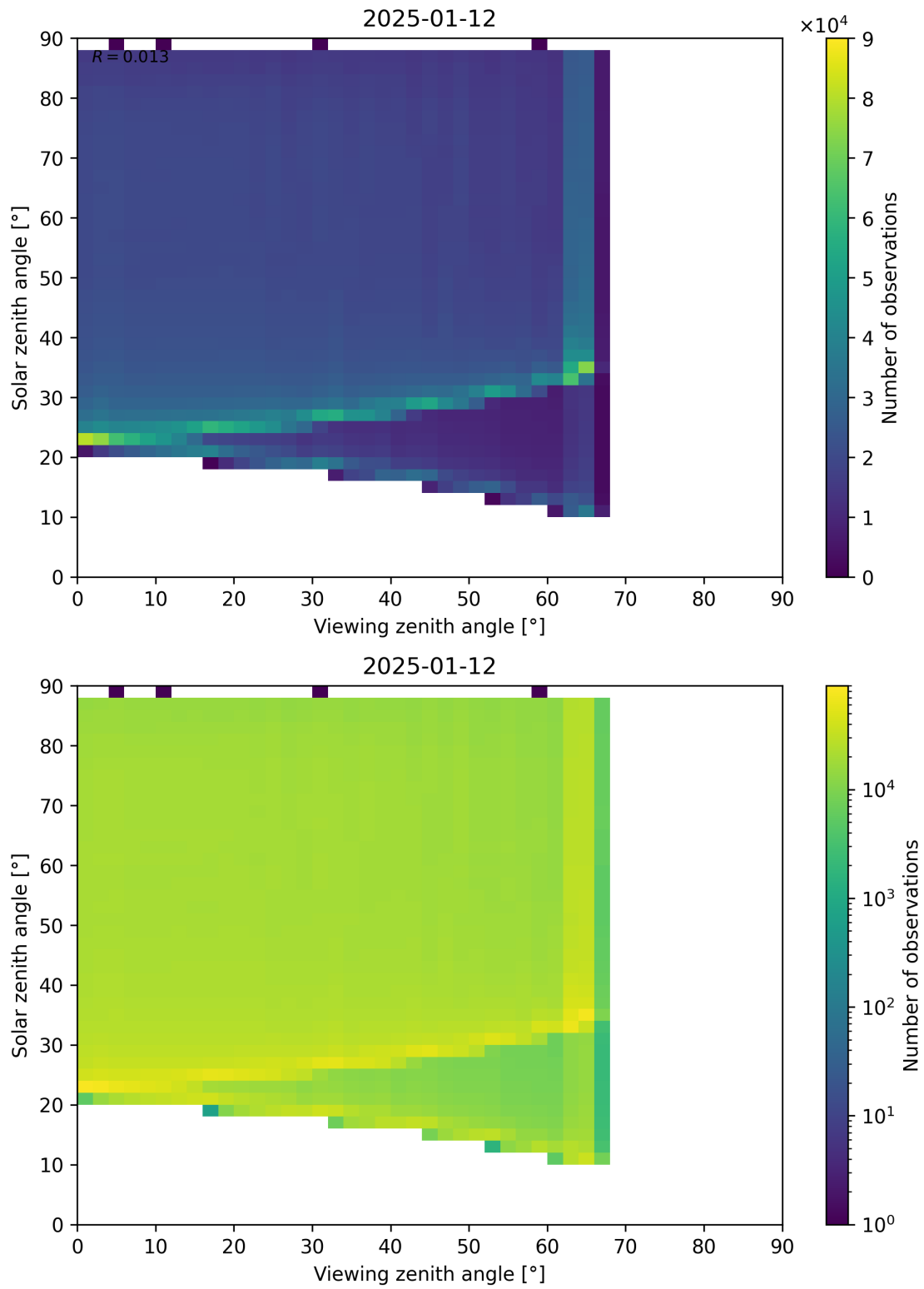
Figure 127: Scatter density plot of “Viewing zenith angle” against “Solar zenith angle” for 2025-01-12 to 2025-01-13.
