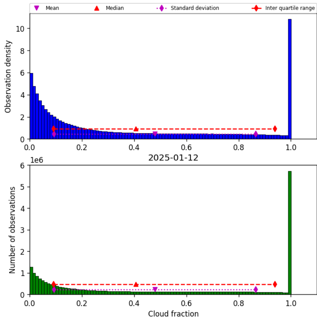
Figure 32: Histogram of “Cloud fraction” for 2025-01-12 to 2025-01-13
