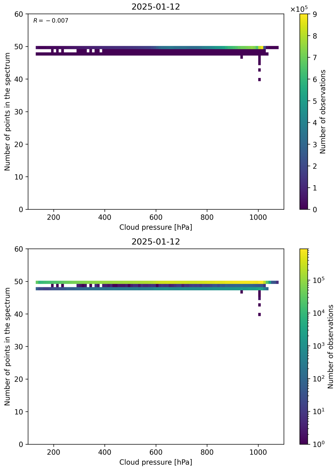
Figure 82: Scatter density plot of “Cloud pressure” against “Number of points in the spectrum” for 2025-01-12 to 2025-01-13.
