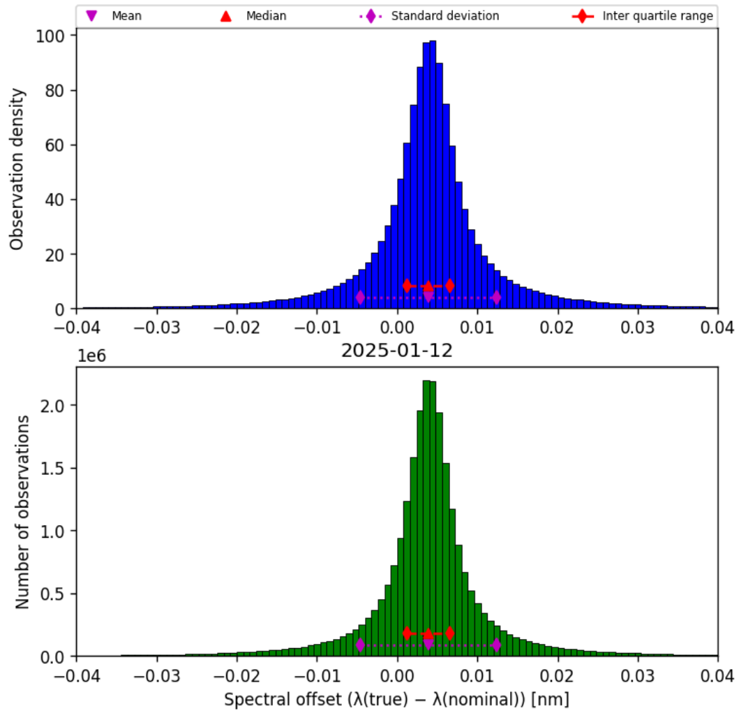
Figure 45: Histogram of “Spectral offset ( \lambda_{\text{true}} - \lambda_{\text{nominal}} )” for 2025-01-12 to 2025-01-13
