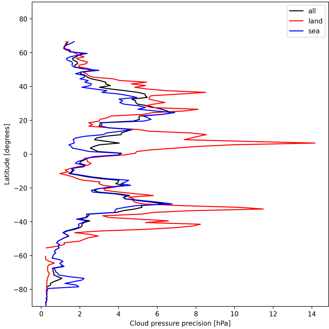
Figure 14: Zonal average of “Cloud pressure precision” for 2025-01-12 to 2025-01-13.
