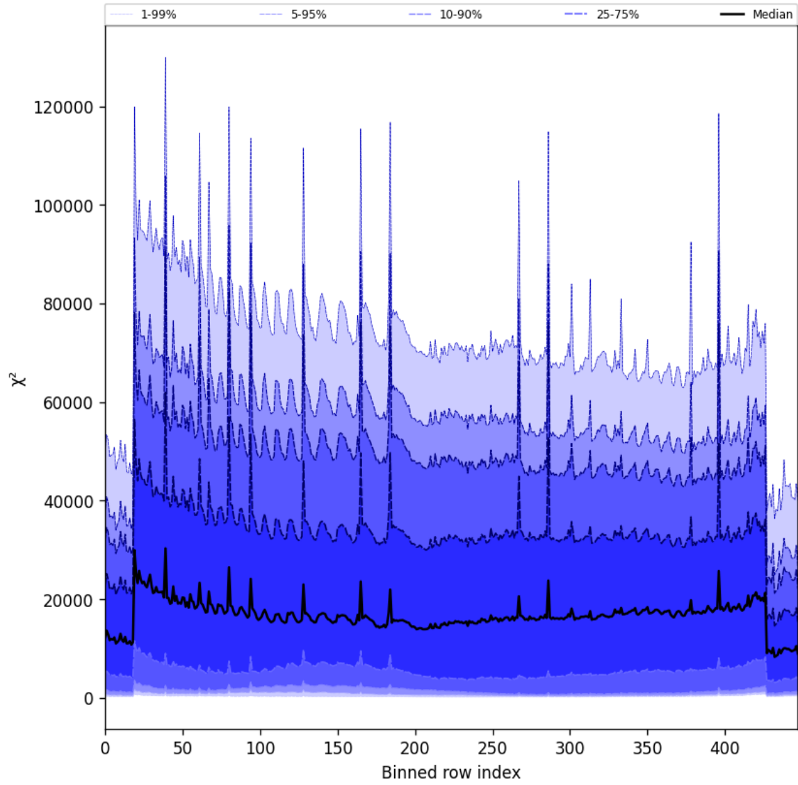
Figure 55: Along track statistics of “ \chi^2 ” for 2025-01-12 to 2025-01-13
