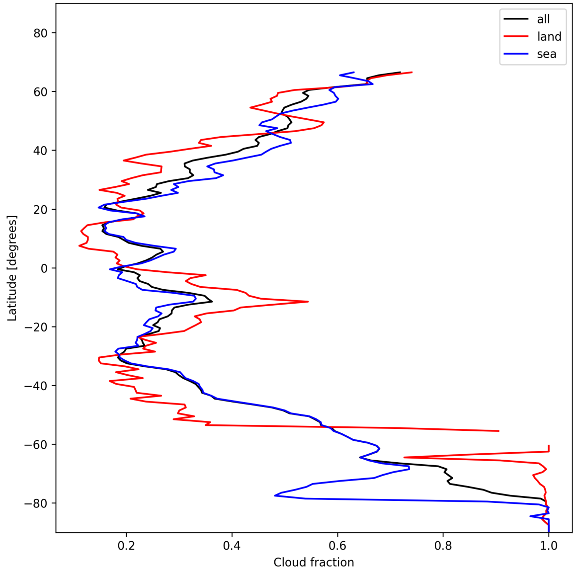
Figure 15: Zonal average of “Cloud fraction” for 2025-01-12 to 2025-01-13.
