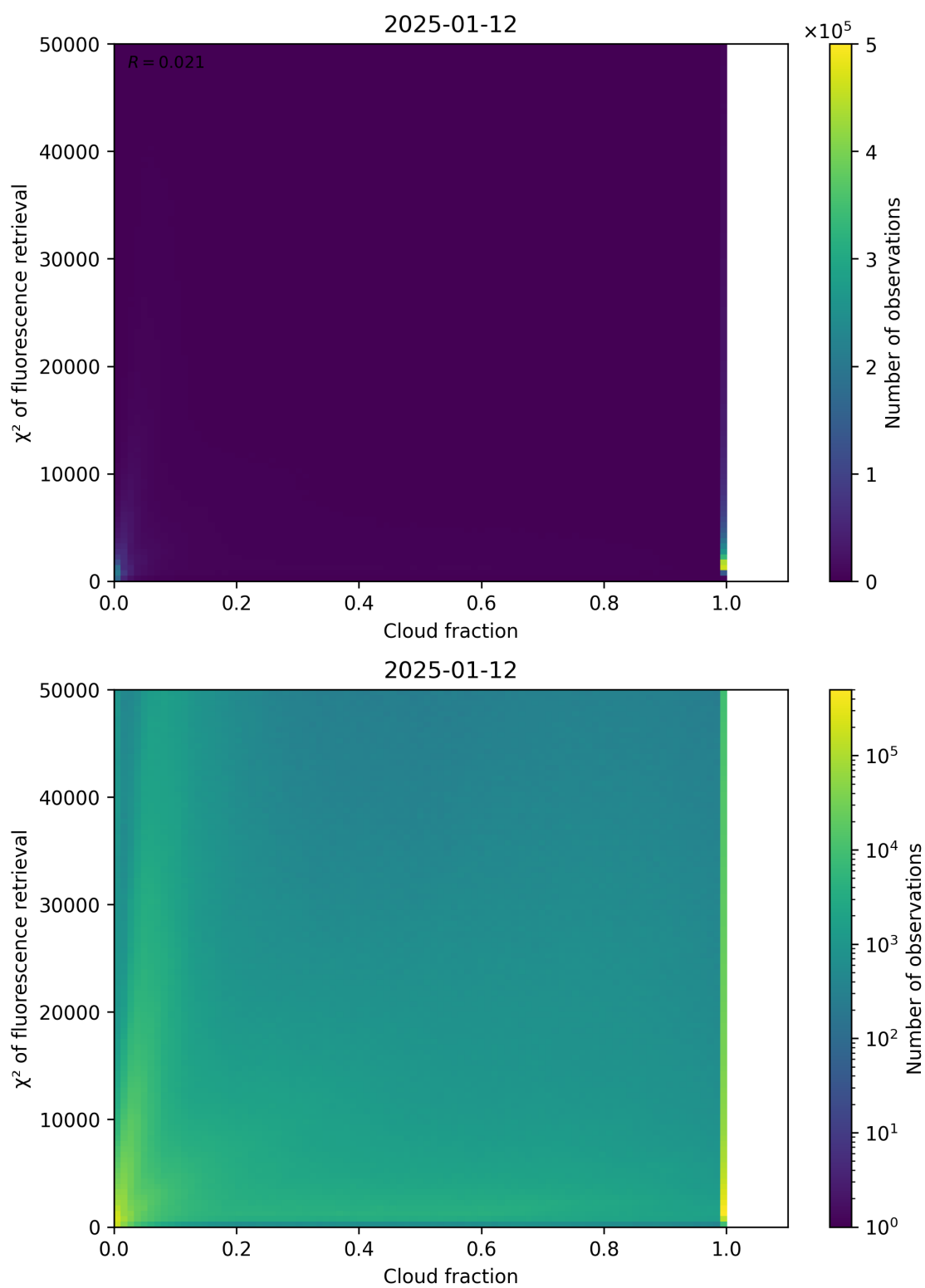
Figure 71: Scatter density plot of “Cloud fraction” against “ \chi^2 of fluorescence retrieval” for 2025-01-12 to 2025-01-13.
