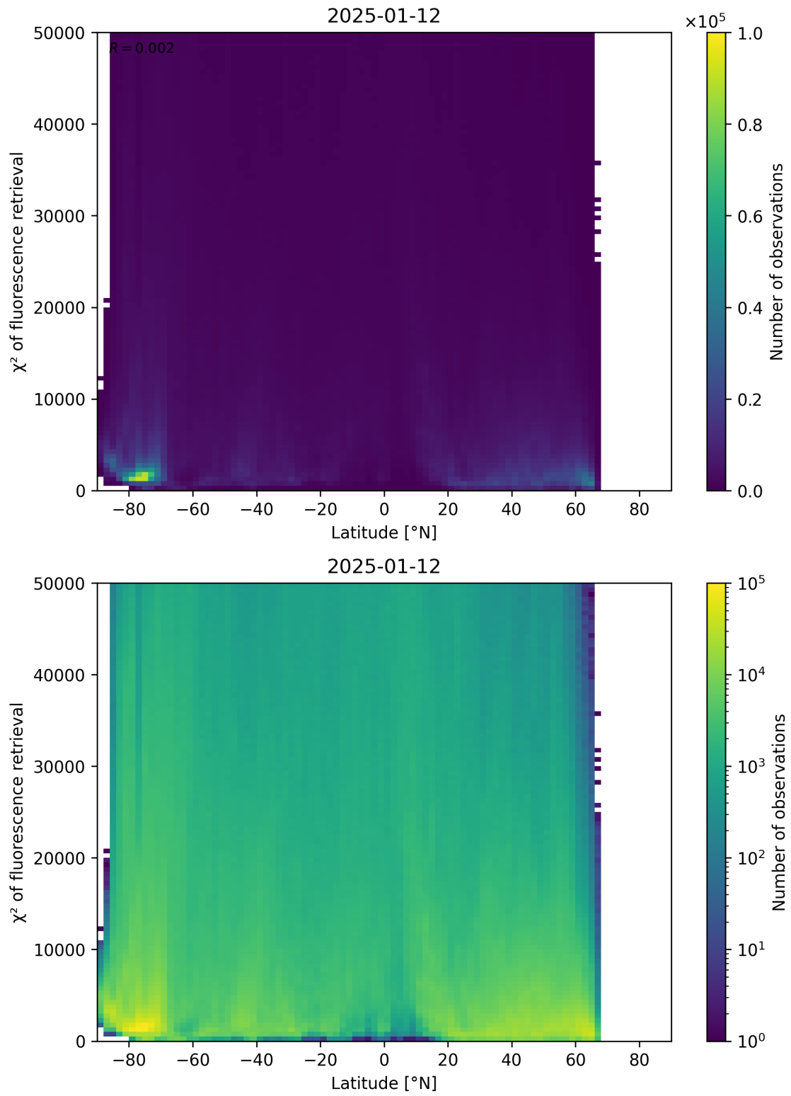
Figure 89: Scatter density plot of “Latitude” against “ \chi^2 of fluorescence retrieval” for 2025-01-12 to 2025-01-13.
