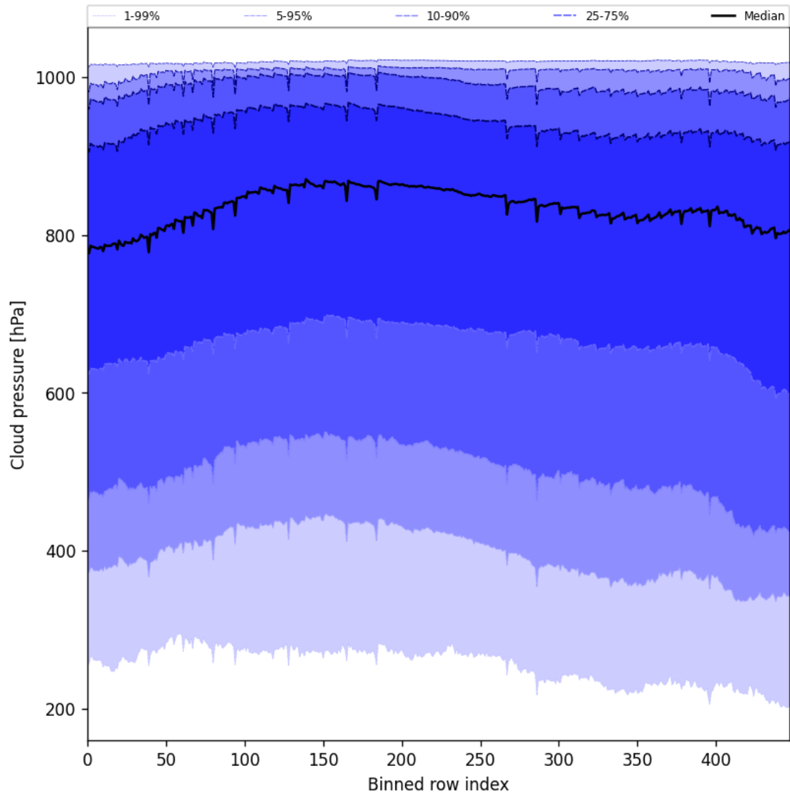
Figure 47: Along track statistics of “Cloud pressure” for 2025-01-12 to 2025-01-13
