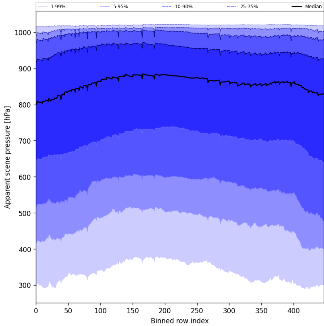
Figure 53: Along track statistics of “Apparent scene pressure” for 2025-01-12 to 2025-01-13
