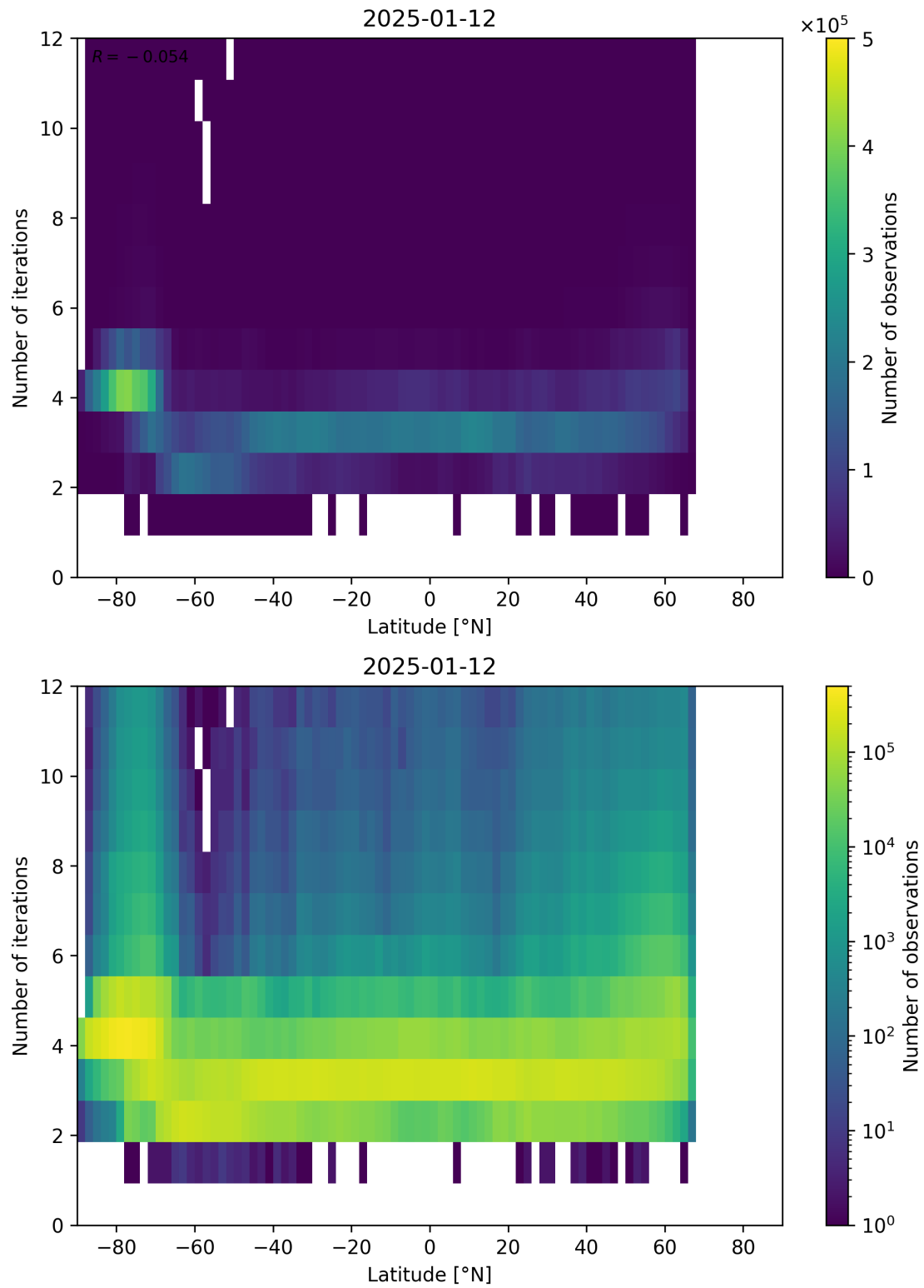
Figure 93: Scatter density plot of “Latitude” against “Number of iterations” for 2025-01-12 to 2025-01-13.
