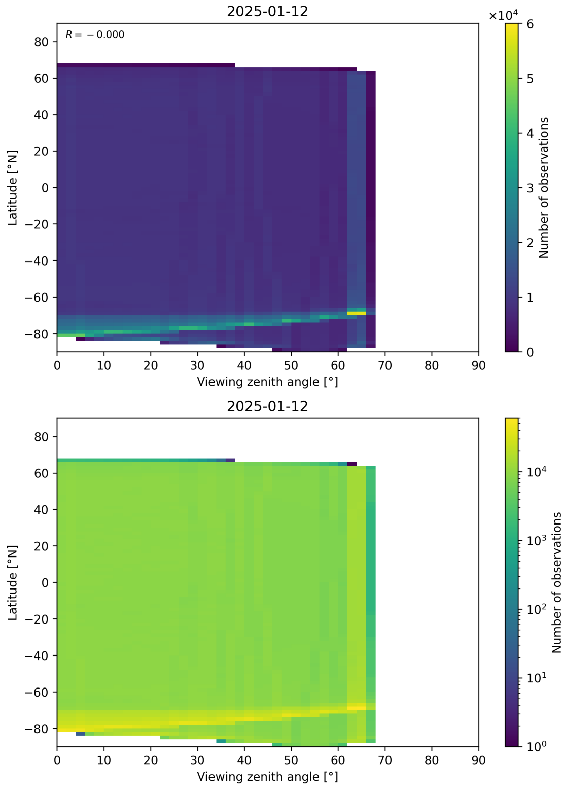
Figure 123: Scatter density plot of “Viewing zenith angle” against “Latitude” for 2025-01-12 to 2025-01-13.
