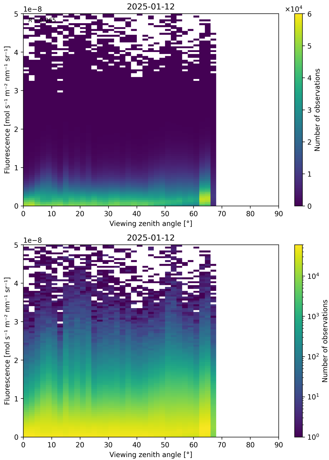
Figure 122: Scatter density plot of "Viewing zenith angle" against "Fluorescence" for 2025-01-12 to 2025-01-13.
