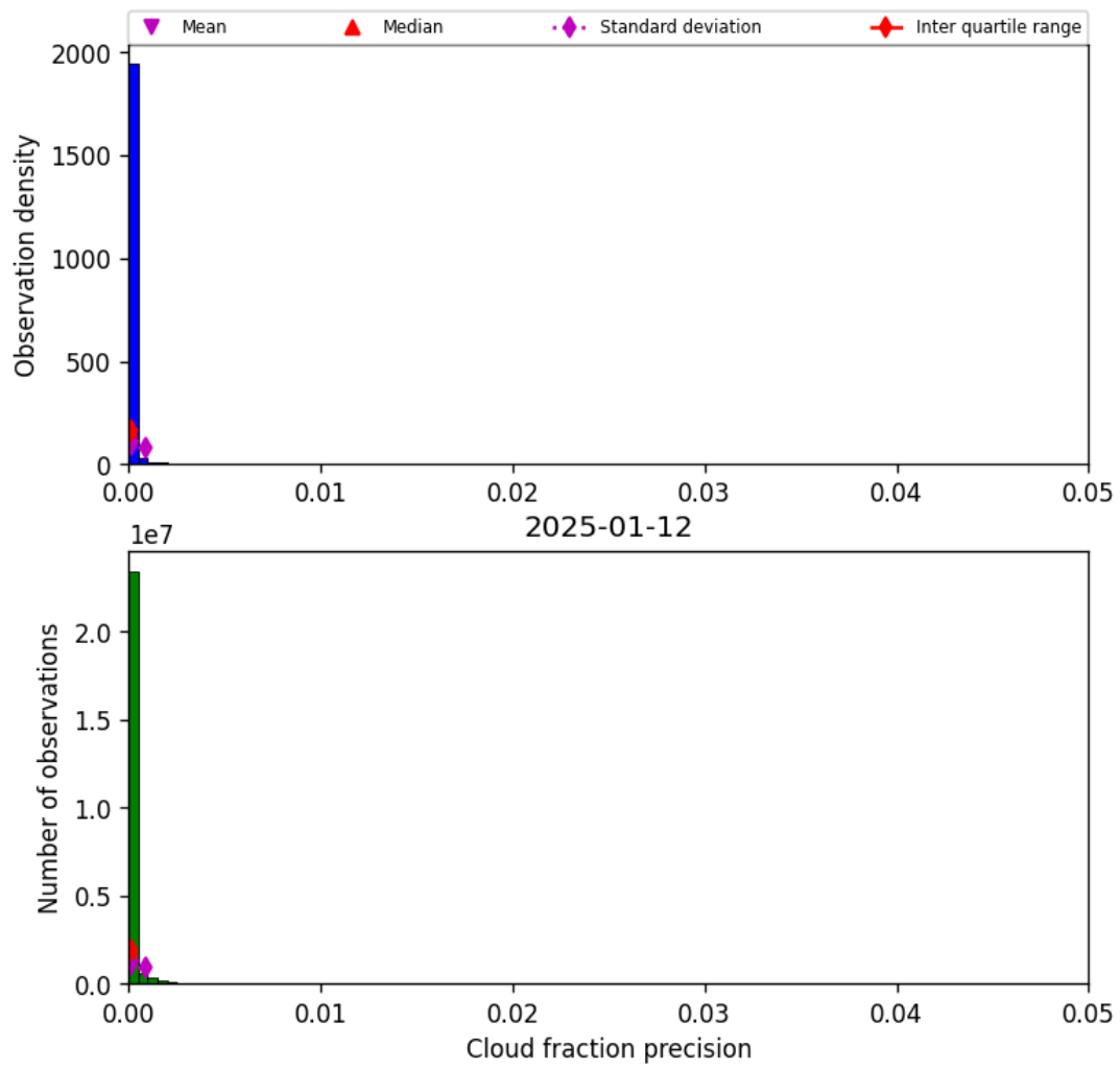
Figure 33: Histogram of “Cloud fraction precision” for 2025-01-12 to 2025-01-13
