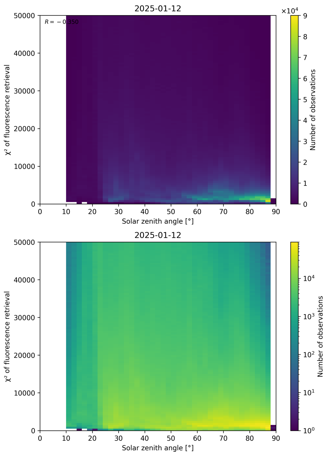
Figure 109: Scatter density plot of “Solar zenith angle” against “ \chi^2 of fluorescence retrieval” for 2025-01-12 to 2025-01-13.
