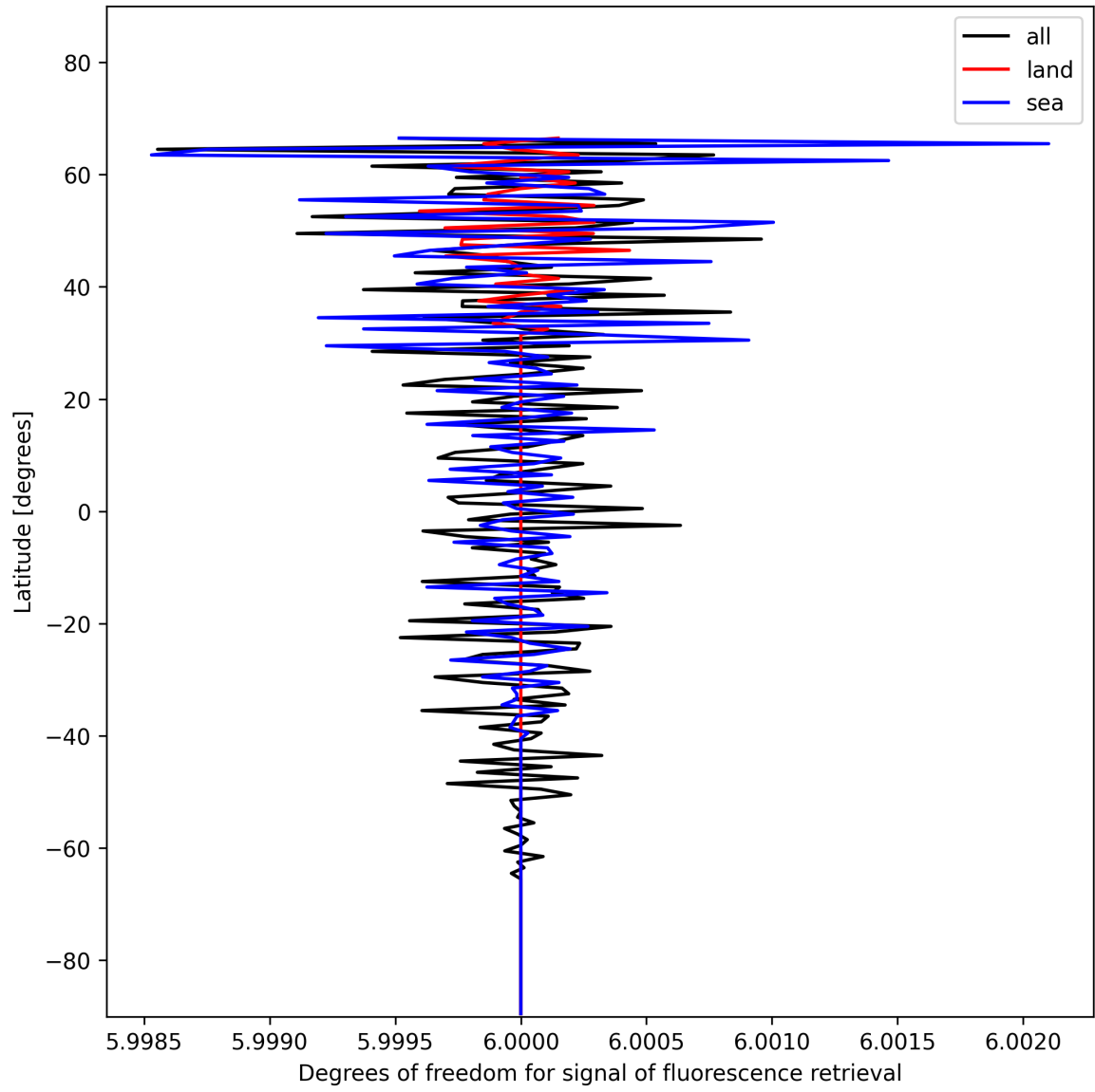
Figure 26: Zonal average of “Degrees of freedom for signal of fluorescence retrieval” for 2025-01-12 to 2025-01-13.
