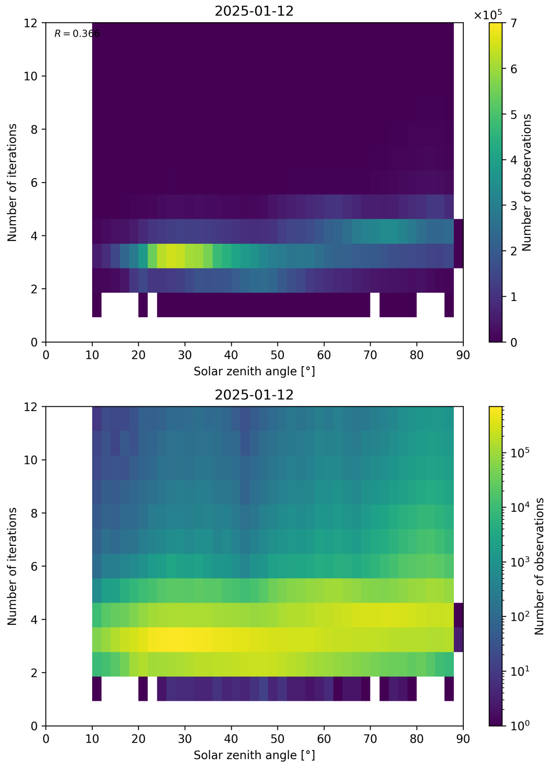
Figure 114: Scatter density plot of “Solar zenith angle” against “Number of iterations” for 2025-01-12 to 2025-01-13.
