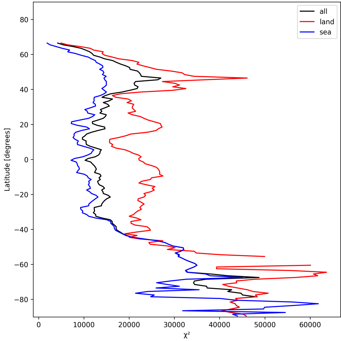
Figure 21: Zonal average of “ \chi^2 ” for 2025-01-12 to 2025-01-13.
