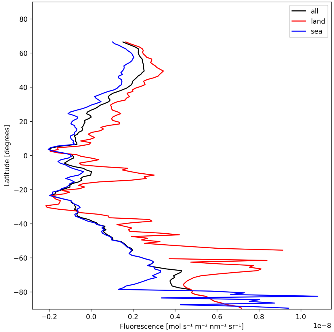
Figure 23: Zonal average of “Fluorescence” for 2025-01-12 to 2025-01-13.
