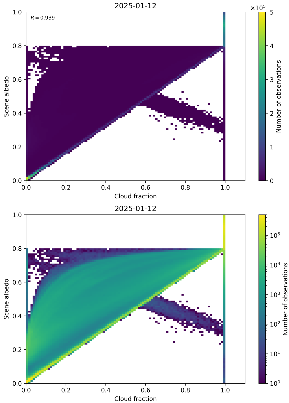
Figure 75: Scatter density plot of “Cloud fraction” against “Scene albedo” for 2025-01-12 to 2025-01-13.
