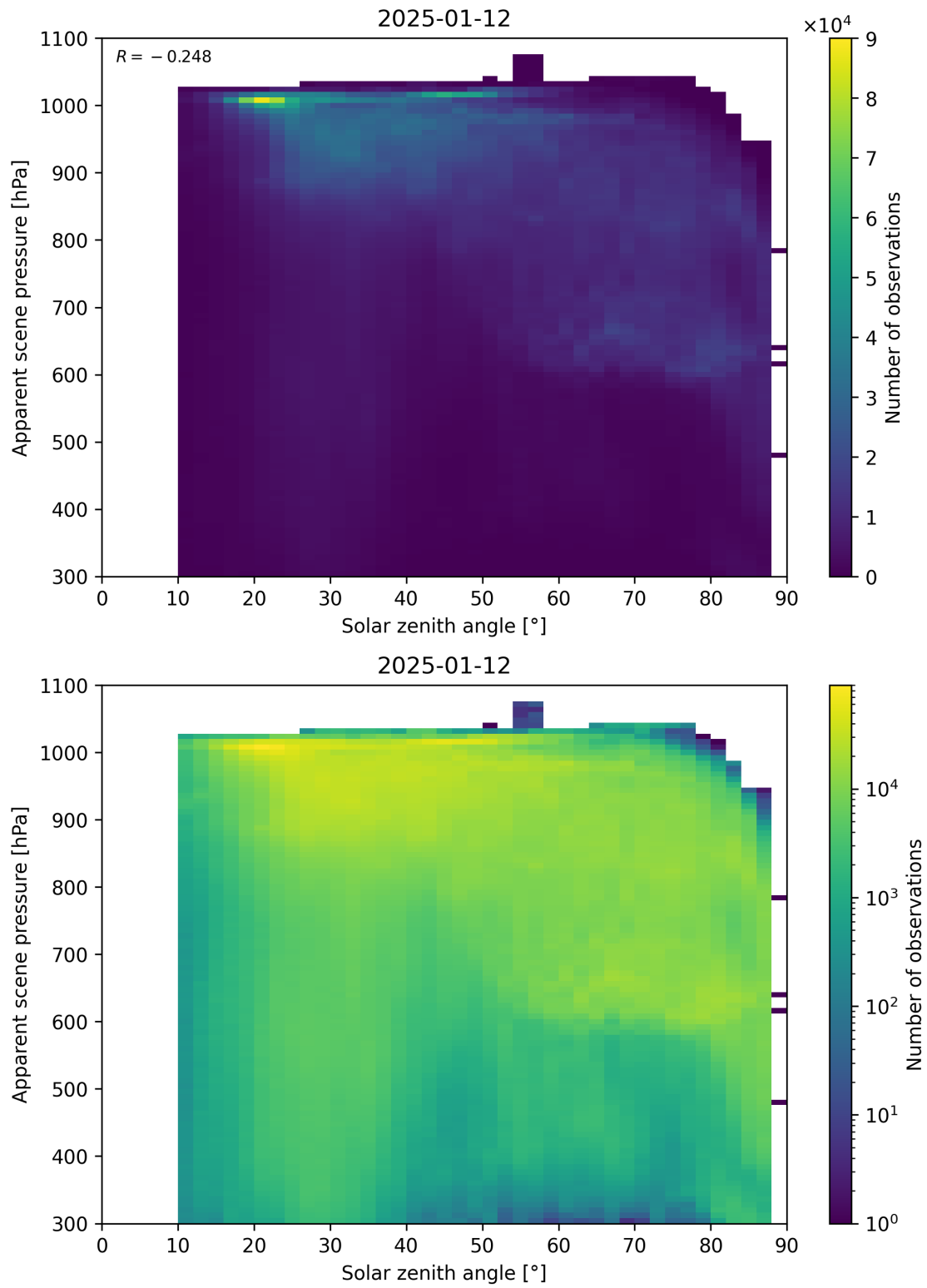
Figure 108: Scatter density plot of “Solar zenith angle” against “Apparent scene pressure” for 2025-01-12 to 2025-01-13.
