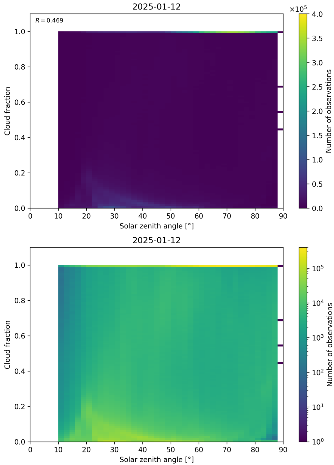
Figure 110: Scatter density plot of “Solar zenith angle” against “Cloud fraction” for 2025-01-12 to 2025-01-13.
