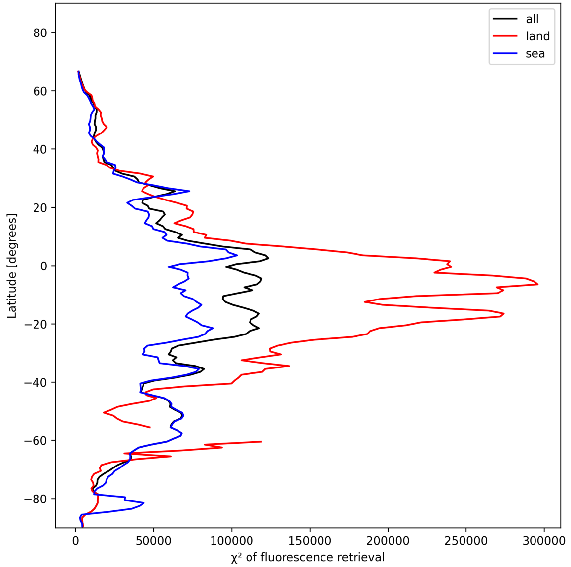
Figure 25: Zonal average of “ \chi^2 of fluorescence retrieval” for 2025-01-12 to 2025-01-13.
