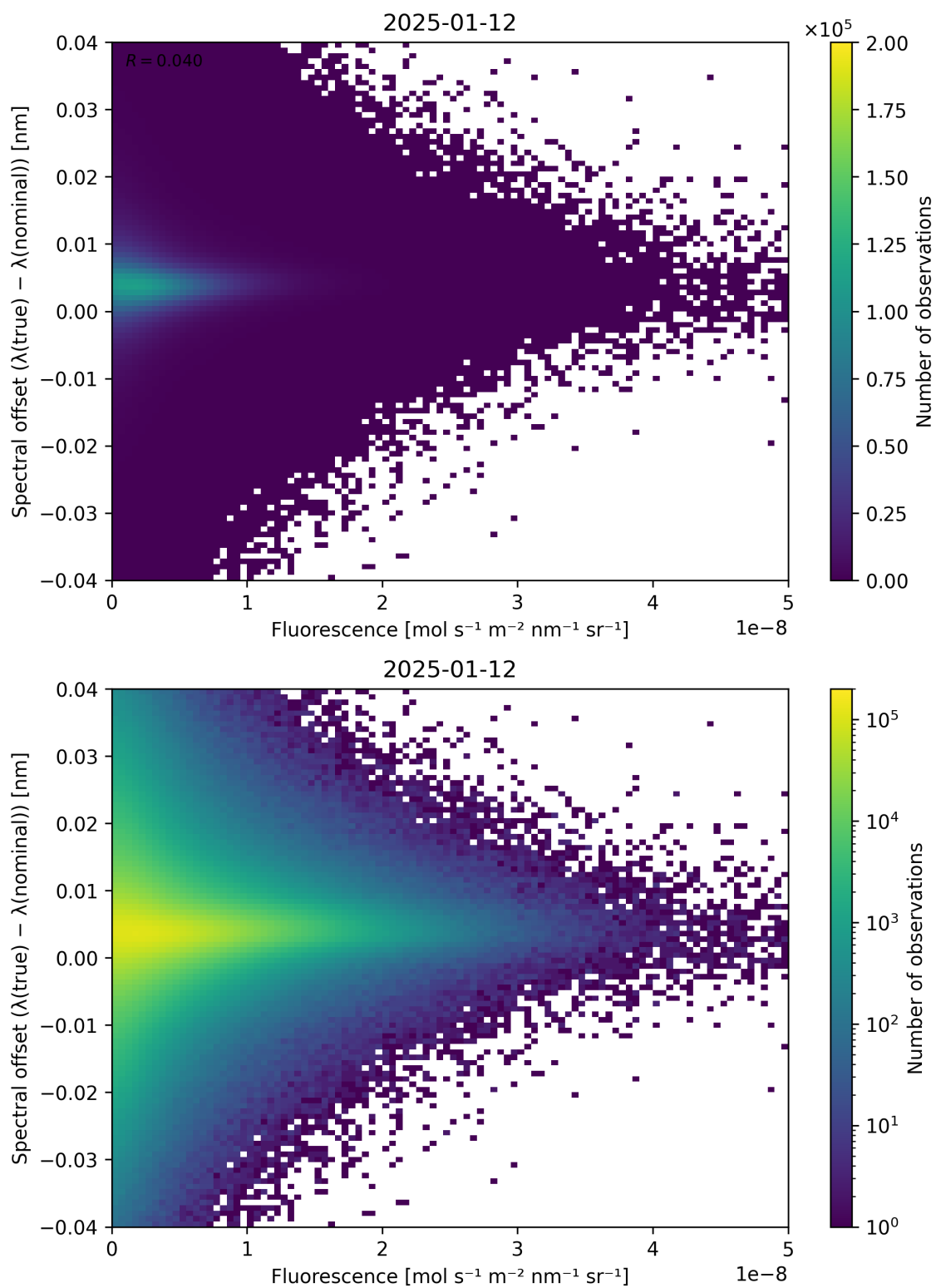
Figure 87: Scatter density plot of “Fluorescence” against “Spectral offset ( \lambda_{\text{true}} - \lambda_{\text{nominal}} )” for 2025-01-12 to 2025-01-13.
