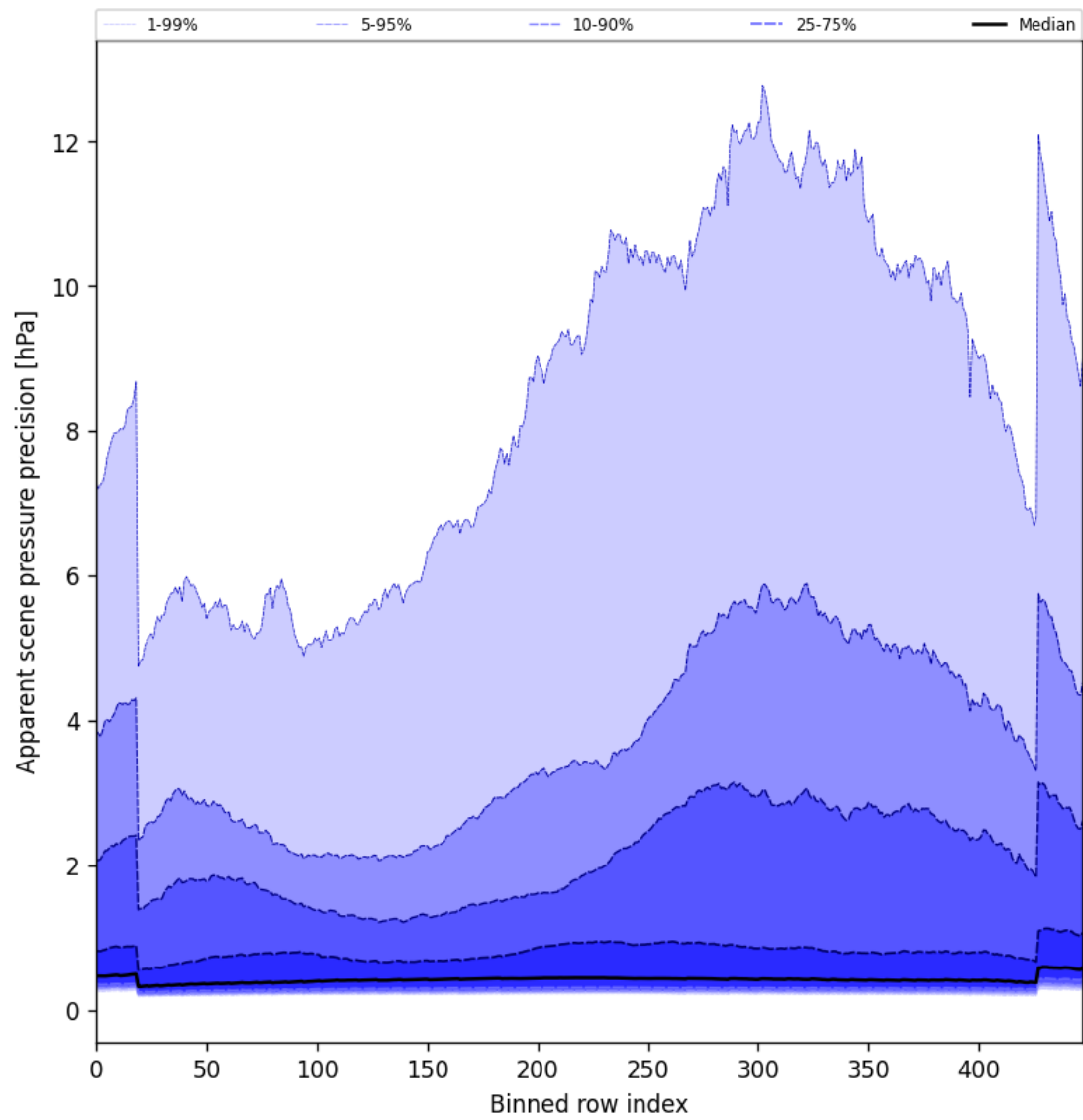
Figure 54: Along track statistics of “Apparent scene pressure precision” for 2025-01-12 to 2025-01-13
