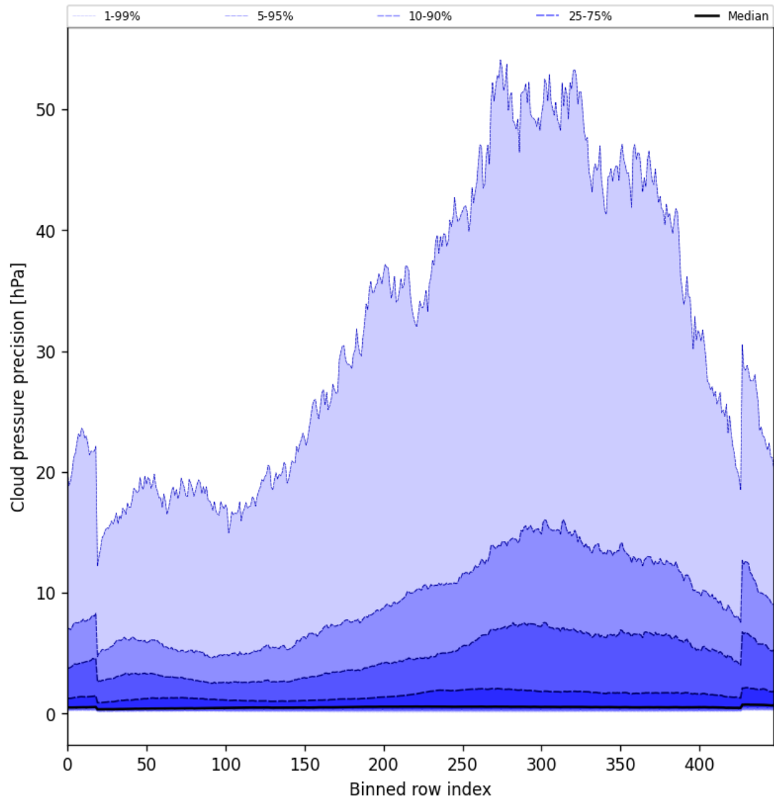
Figure 48: Along track statistics of “Cloud pressure precision” for 2025-01-12 to 2025-01-13
