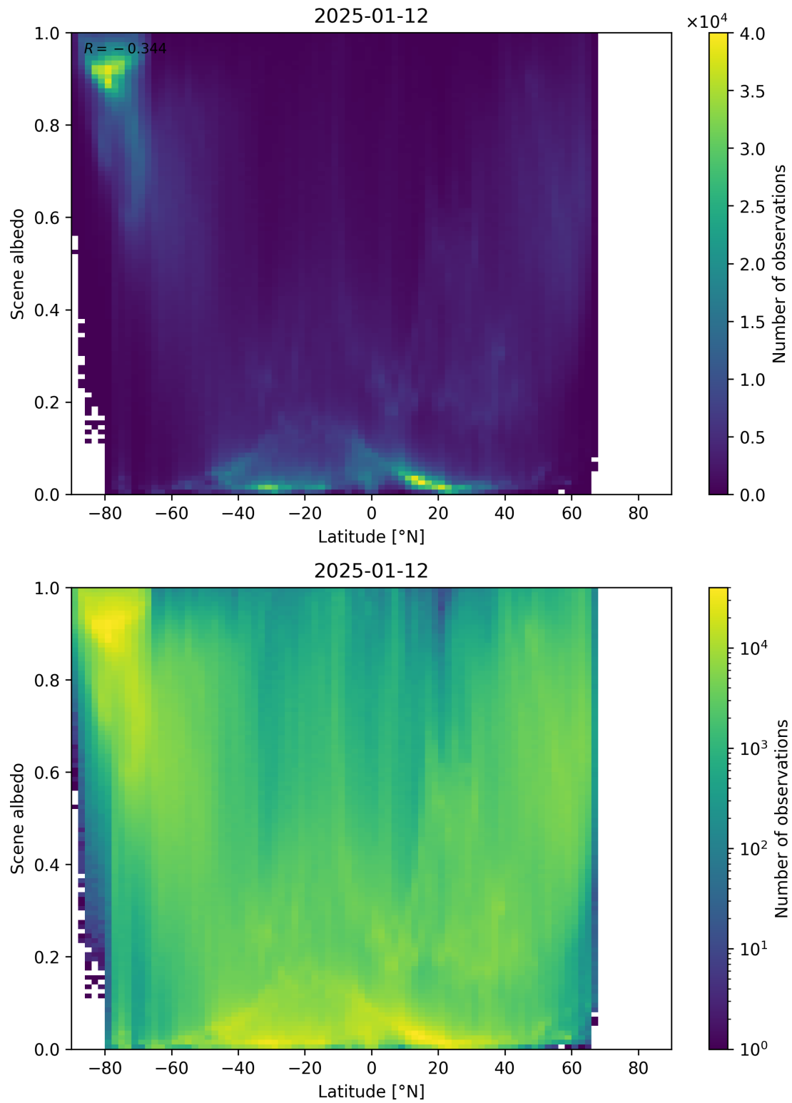
Figure 95: Scatter density plot of “Latitude” against “Scene albedo” for 2025-01-12 to 2025-01-13.
