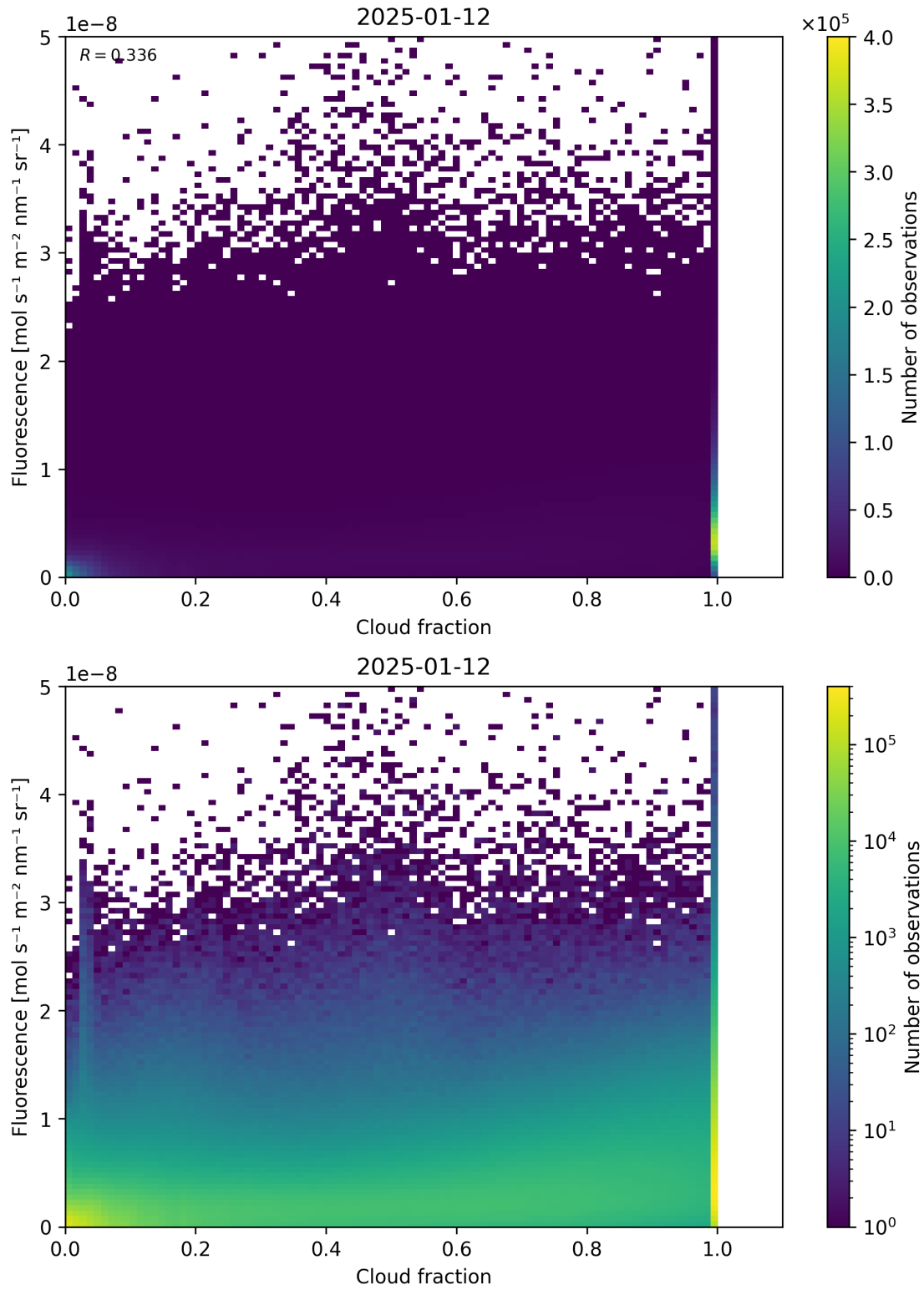
Figure 72: Scatter density plot of “Cloud fraction” against “Fluorescence” for 2025-01-12 to 2025-01-13.
