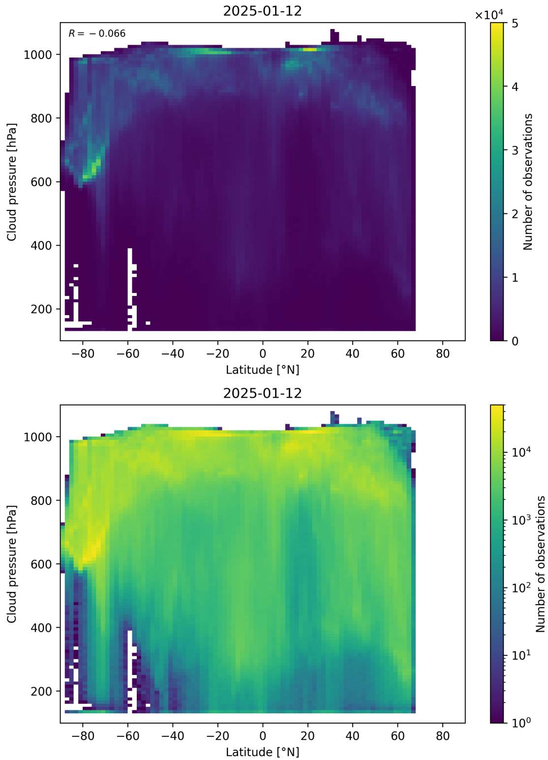
Figure 91: Scatter density plot of “Latitude” against “Cloud pressure” for 2025-01-12 to 2025-01-13.
