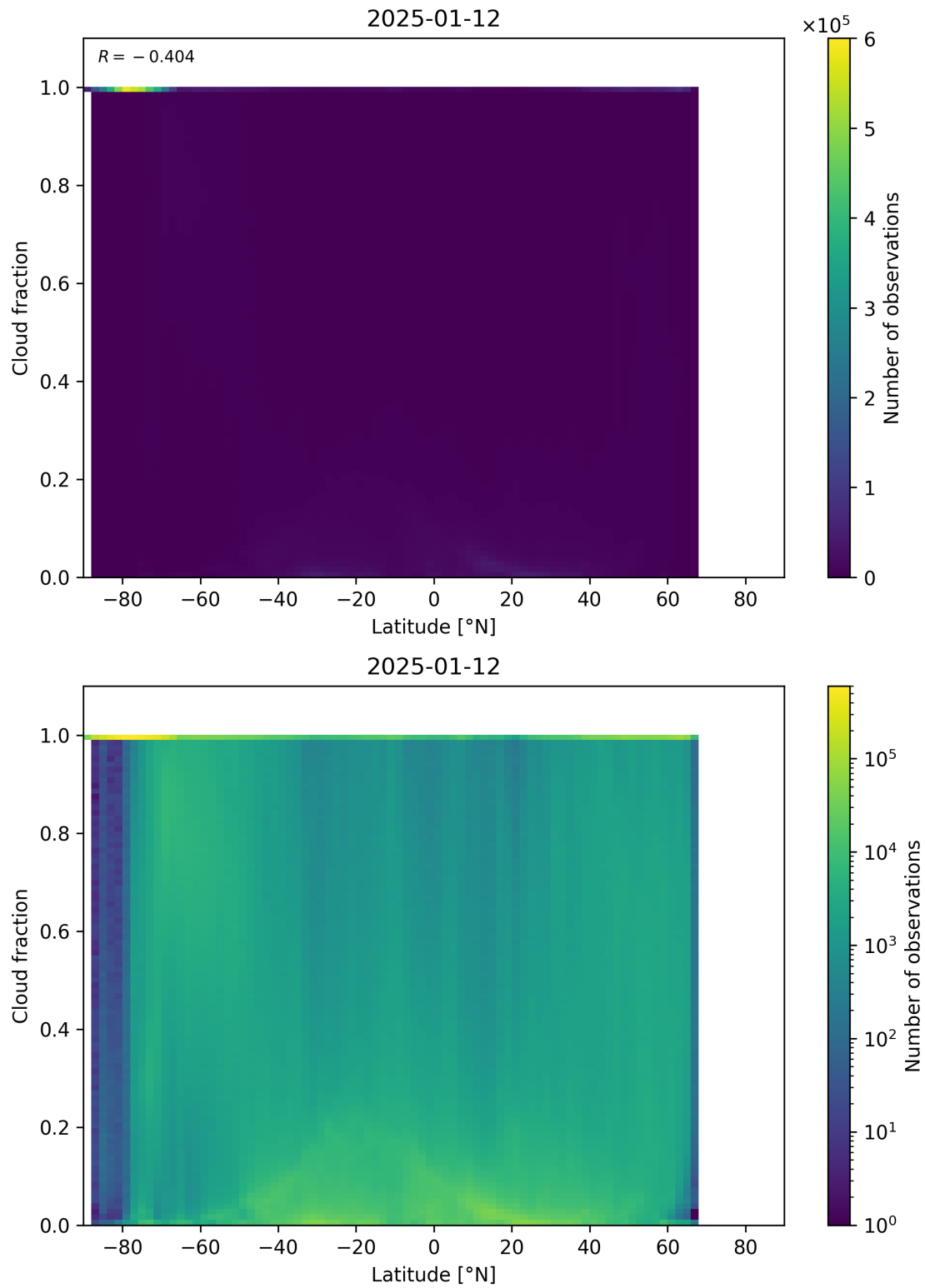
Figure 90: Scatter density plot of “Latitude” against “Cloud fraction” for 2025-01-12 to 2025-01-13.
