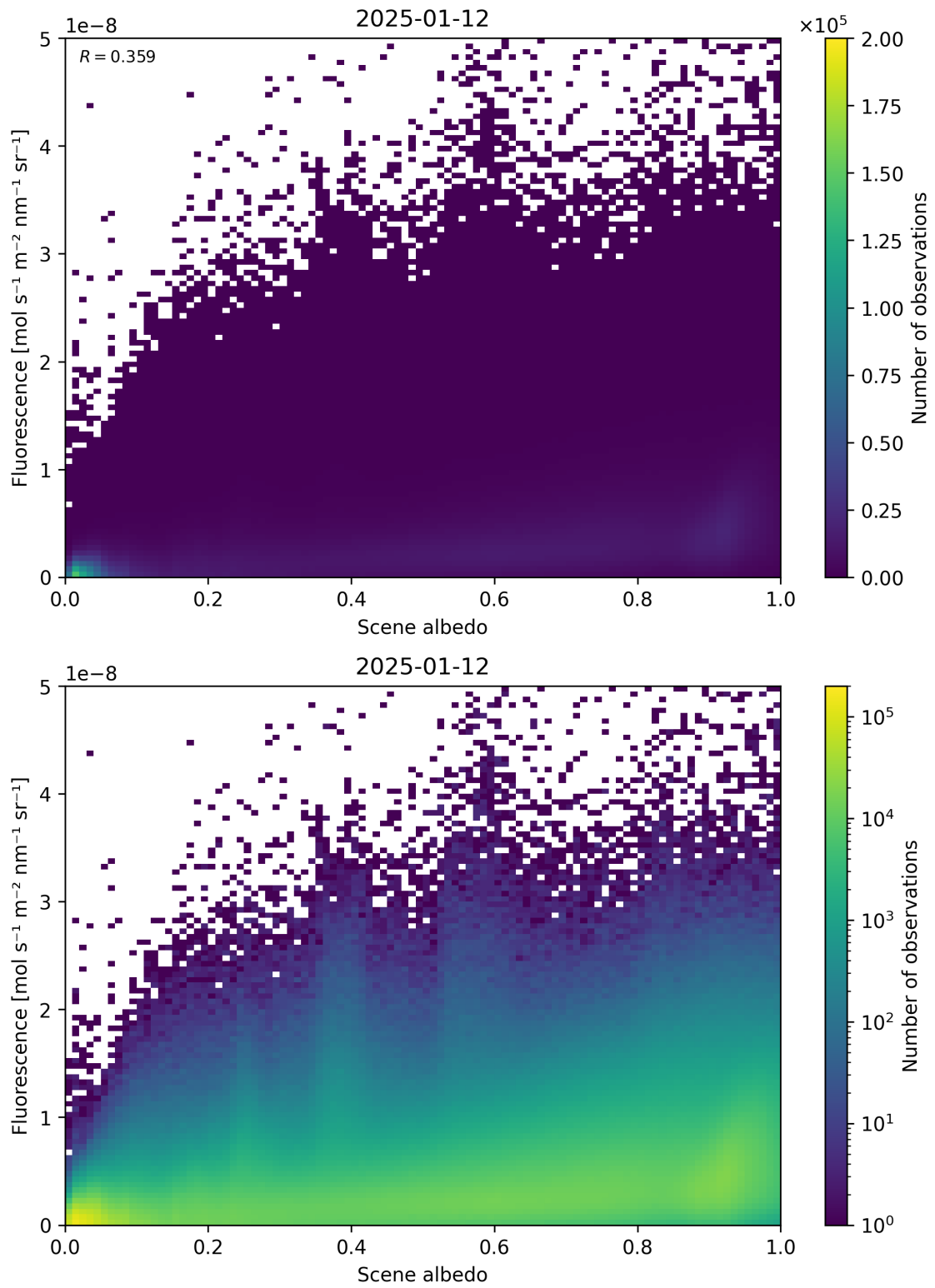
Figure 104: Scatter density plot of “Scene albedo” against “Fluorescence” for 2025-01-12 to 2025-01-13.
