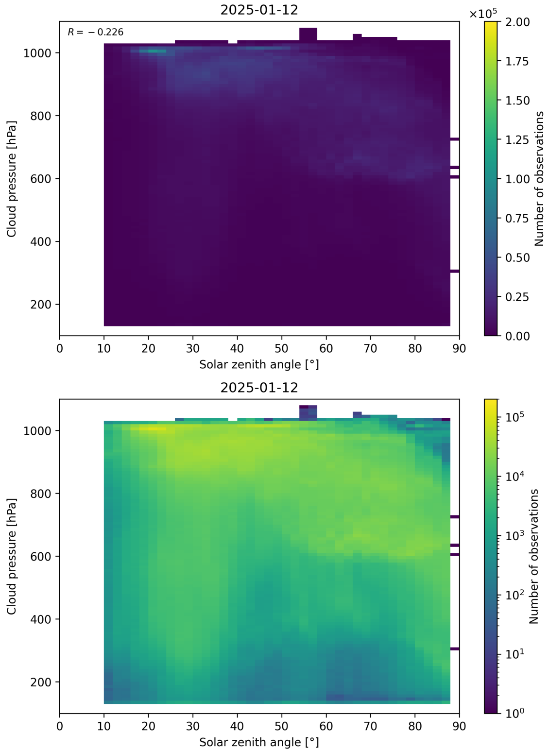
Figure 111: Scatter density plot of “Solar zenith angle” against “Cloud pressure” for 2025-01-12 to 2025-01-13.
