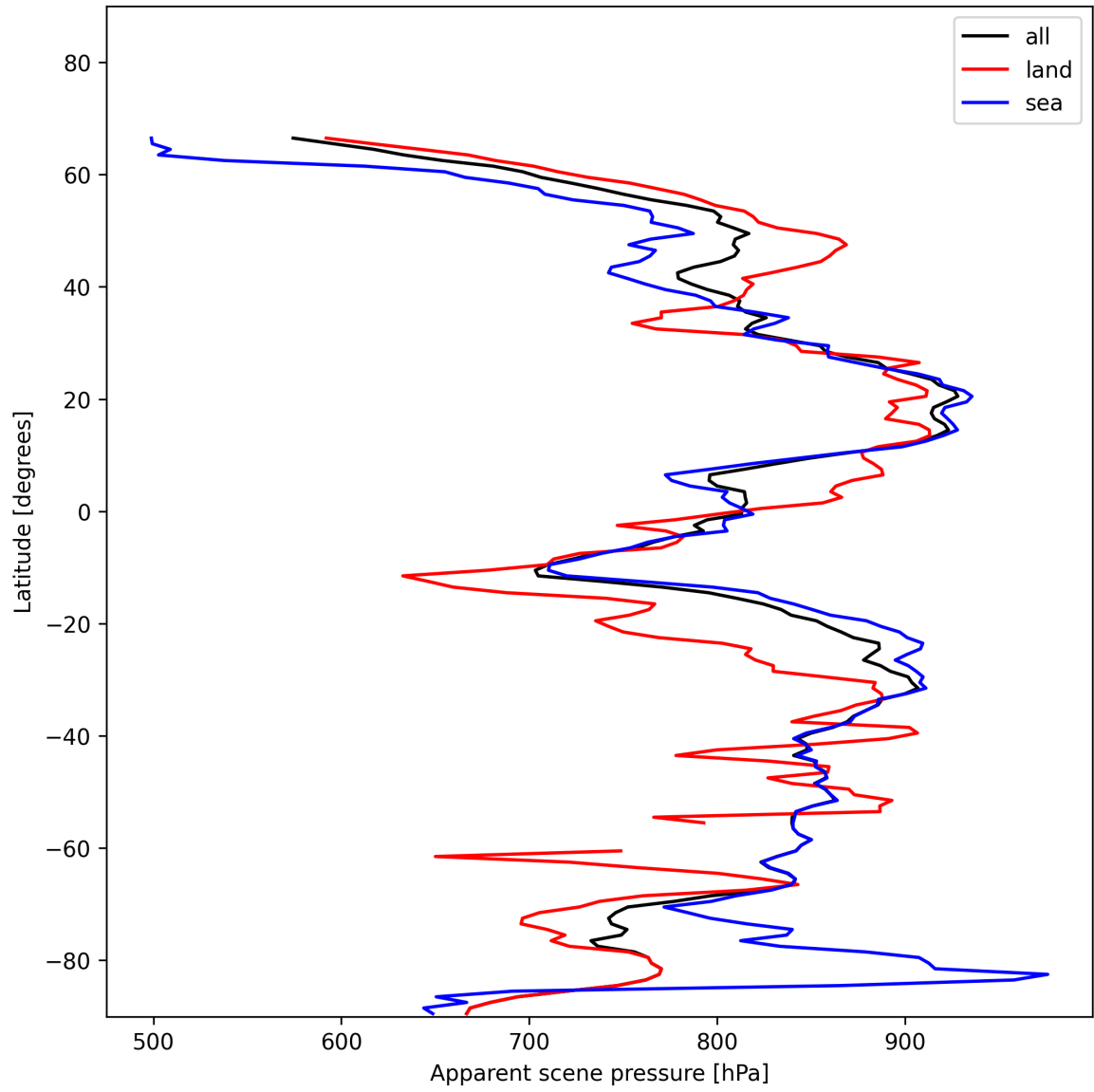
Figure 19: Zonal average of “Apparent scene pressure” for 2025-01-12 to 2025-01-13.
