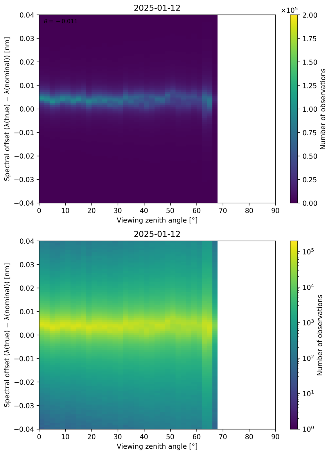
Figure 128: Scatter density plot of “Viewing zenith angle” against “Spectral offset ( \lambda_{\text{true}} - \lambda_{\text{nominal}} )” for 2025-01-12 to 2025-01-13.
