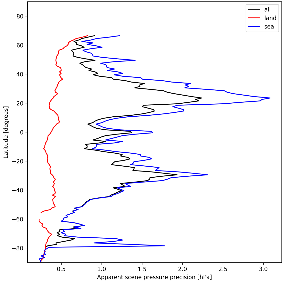
Figure 20: Zonal average of “Apparent scene pressure precision” for 2025-01-12 to 2025-01-13.
