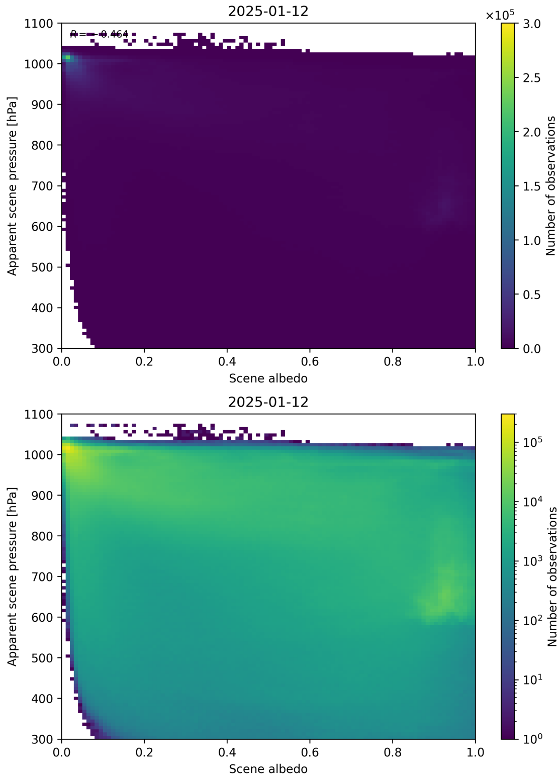
Figure 102: Scatter density plot of “Scene albedo” against “Apparent scene pressure” for 2025-01-12 to 2025-01-13.
