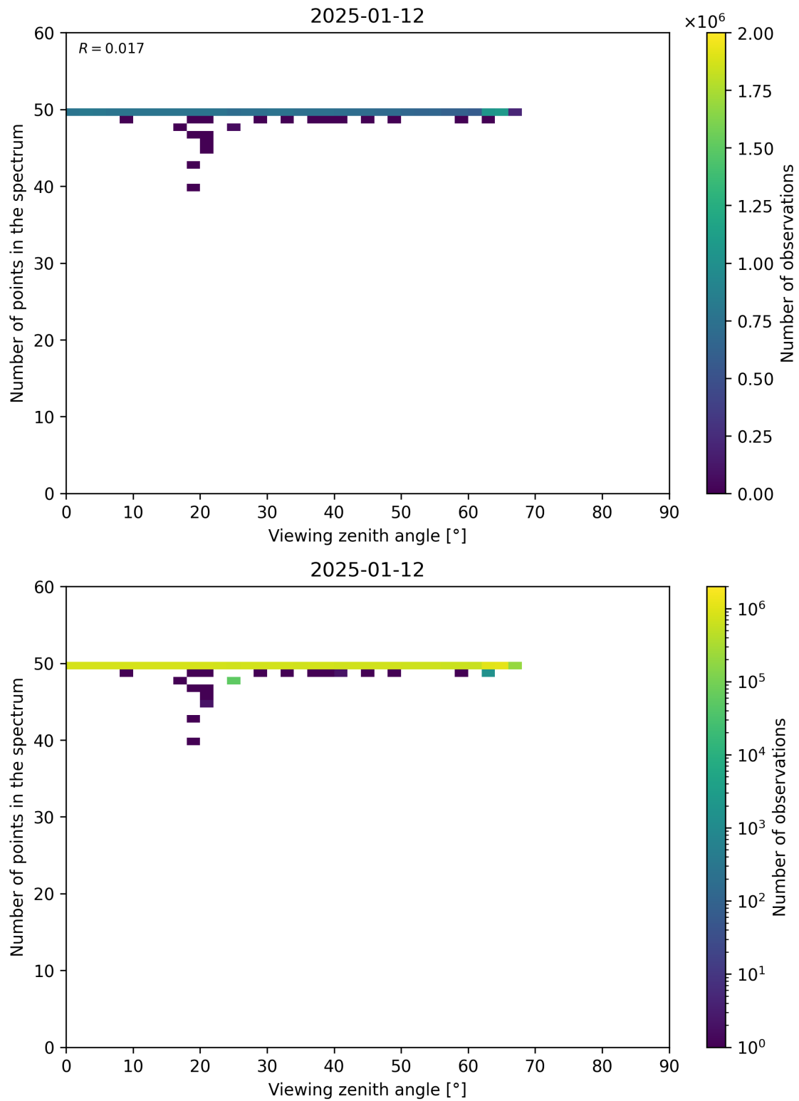
Figure 125: Scatter density plot of “Viewing zenith angle” against “Number of points in the spectrum” for 2025-01-12 to 2025-01-13.
