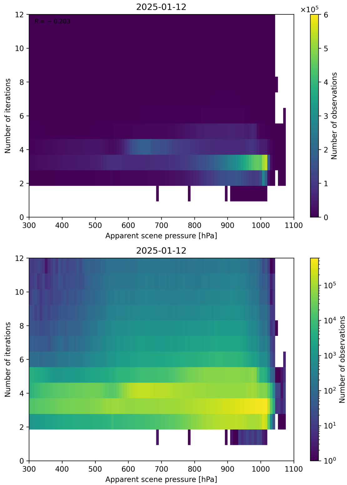
Figure 65: Scatter density plot of “Apparent scene pressure” against “Number of iterations” for 2025-01-12 to 2025-01-13.
