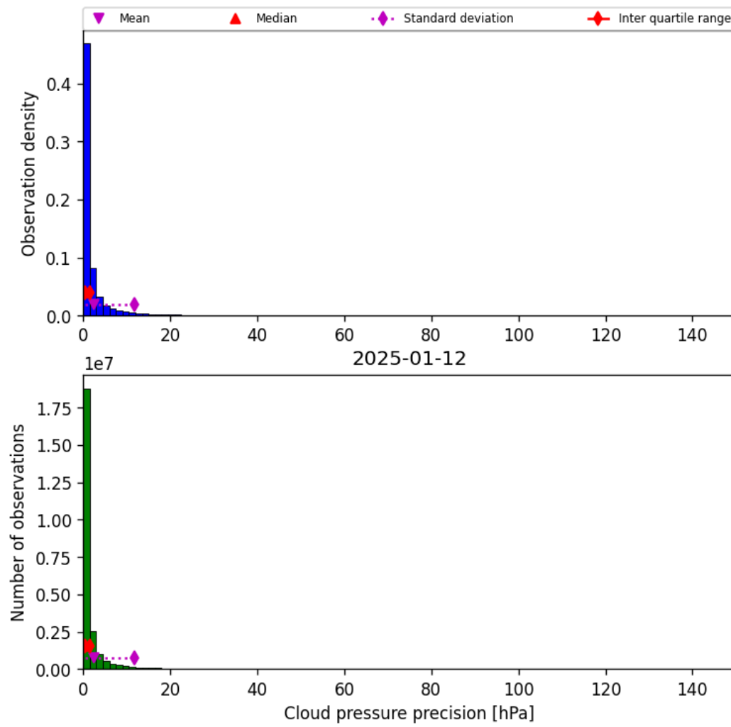
Figure 31: Histogram of “Cloud pressure precision” for 2025-01-12 to 2025-01-13
