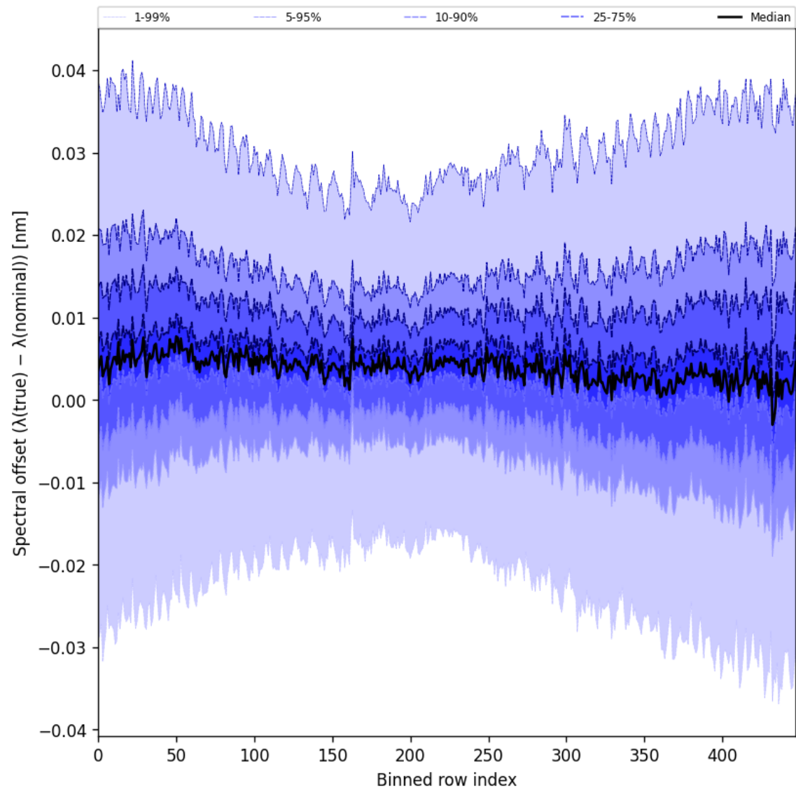
Figure 62: Along track statistics of “Spectral offset ( \lambda_{\text{true}} - \lambda_{\text{nominal}} )” for 2025-01-12 to 2025-01-13
