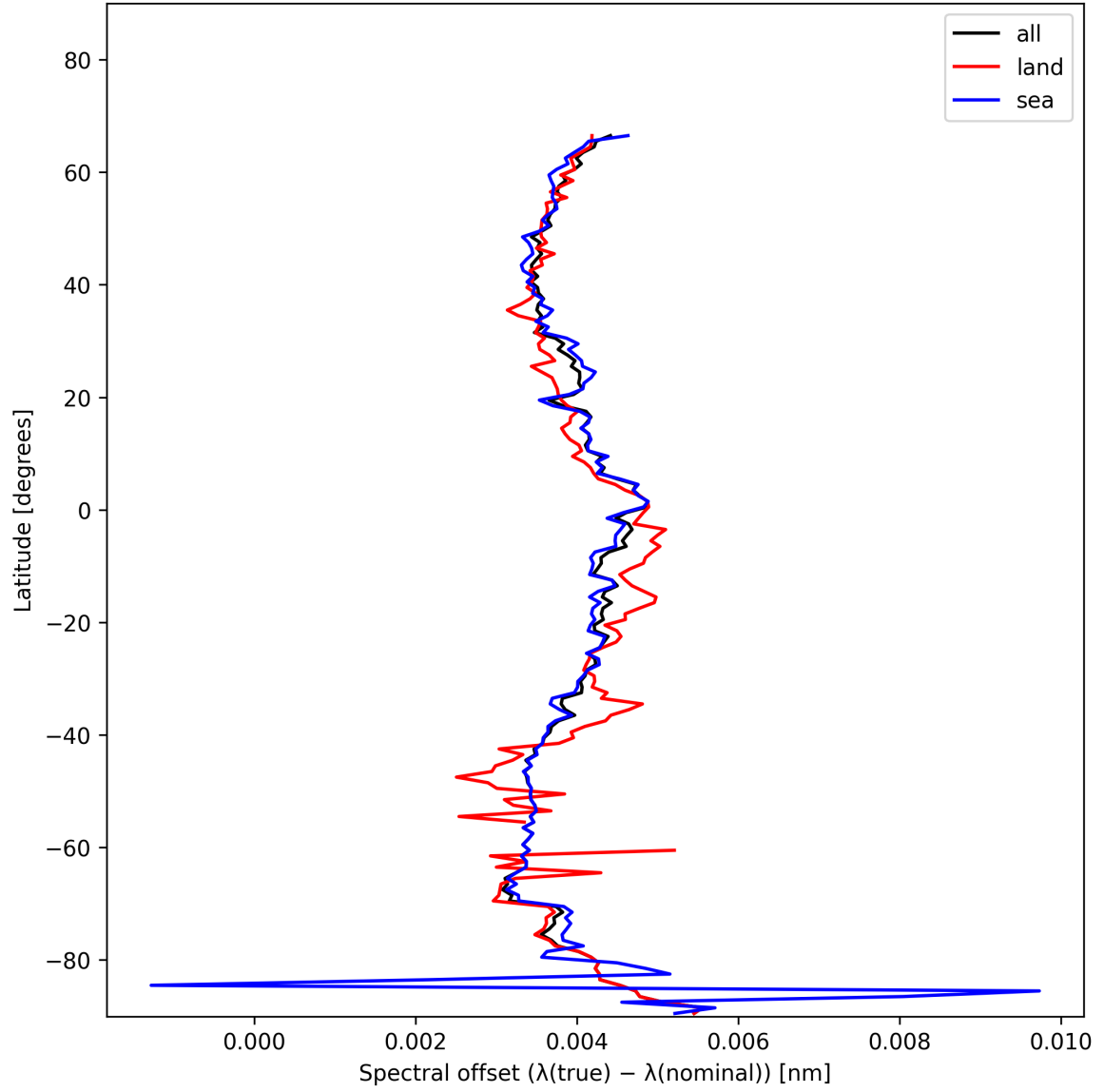
Figure 28: Zonal average of “Spectral offset ( \lambda_{\text{true}} - \lambda_{\text{nominal}} )” for 2025-01-12 to 2025-01-13.
