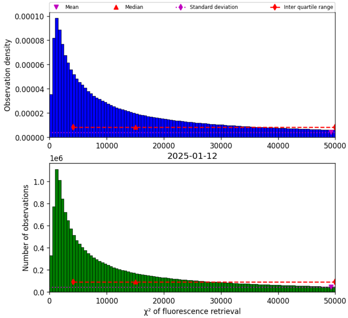
Figure 42: Histogram of “ \chi^2 of fluorescence retrieval” for 2025-01-12 to 2025-01-13
