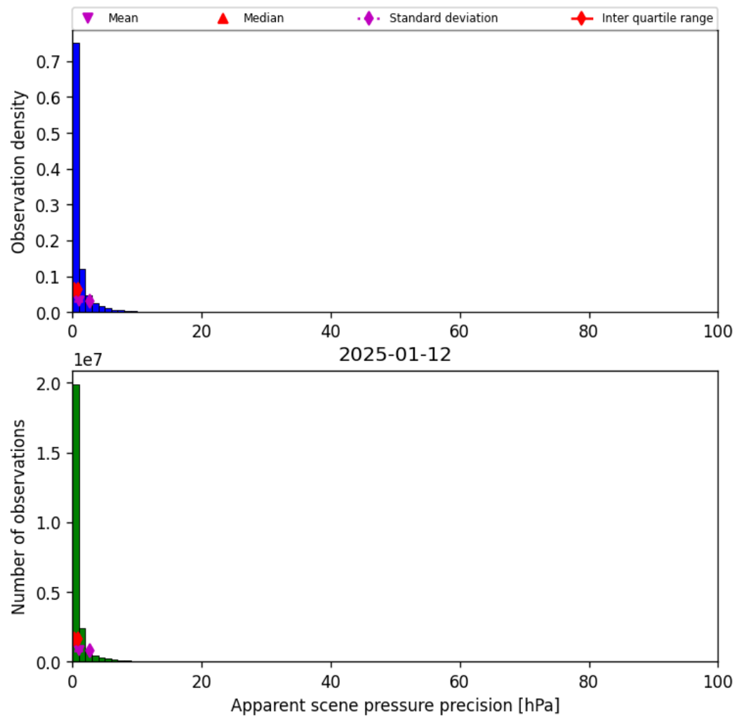
Figure 37: Histogram of “Apparent scene pressure precision” for 2025-01-12 to 2025-01-13
