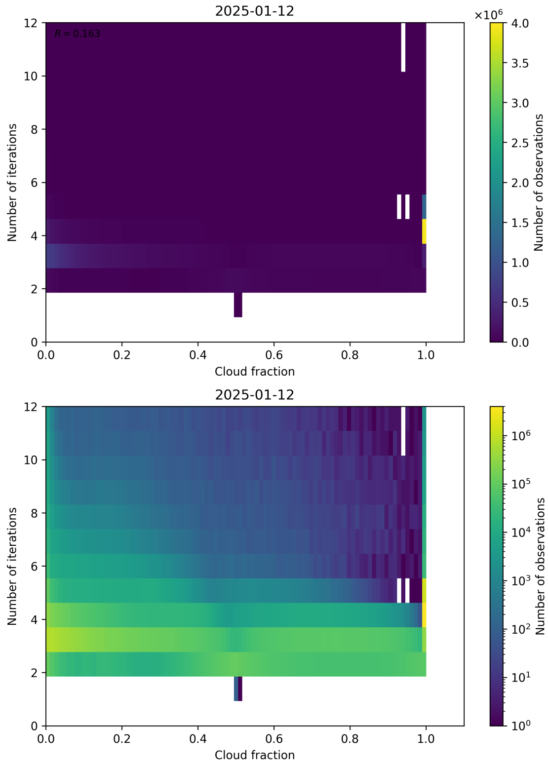
Figure 73: Scatter density plot of “Cloud fraction” against “Number of iterations” for 2025-01-12 to 2025-01-13.
