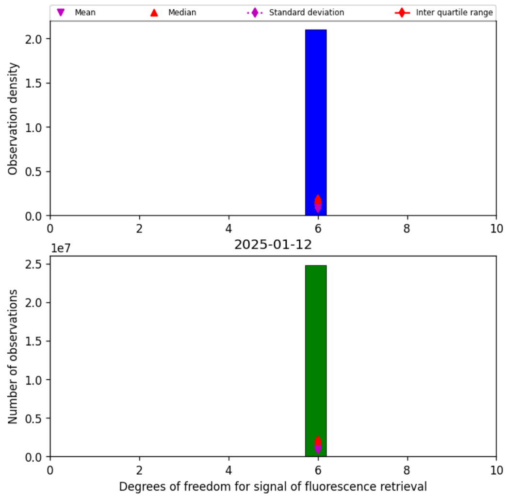
Figure 43: Histogram of “Degrees of freedom for signal of fluorescence retrieval” for 2025-01-12 to 2025-01-13
