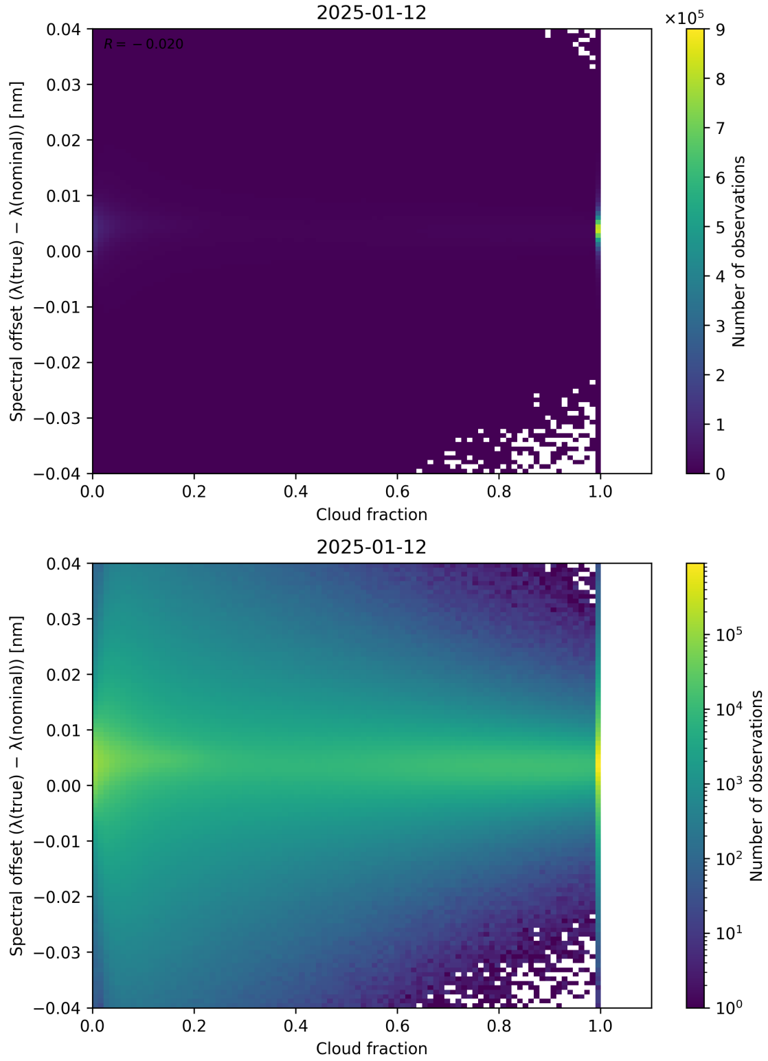
Figure 76: Scatter density plot of “Cloud fraction” against “Spectral offset ( \lambda_{\text{true}} - \lambda_{\text{nominal}} )” for 2025-01-12 to 2025-01-13.
