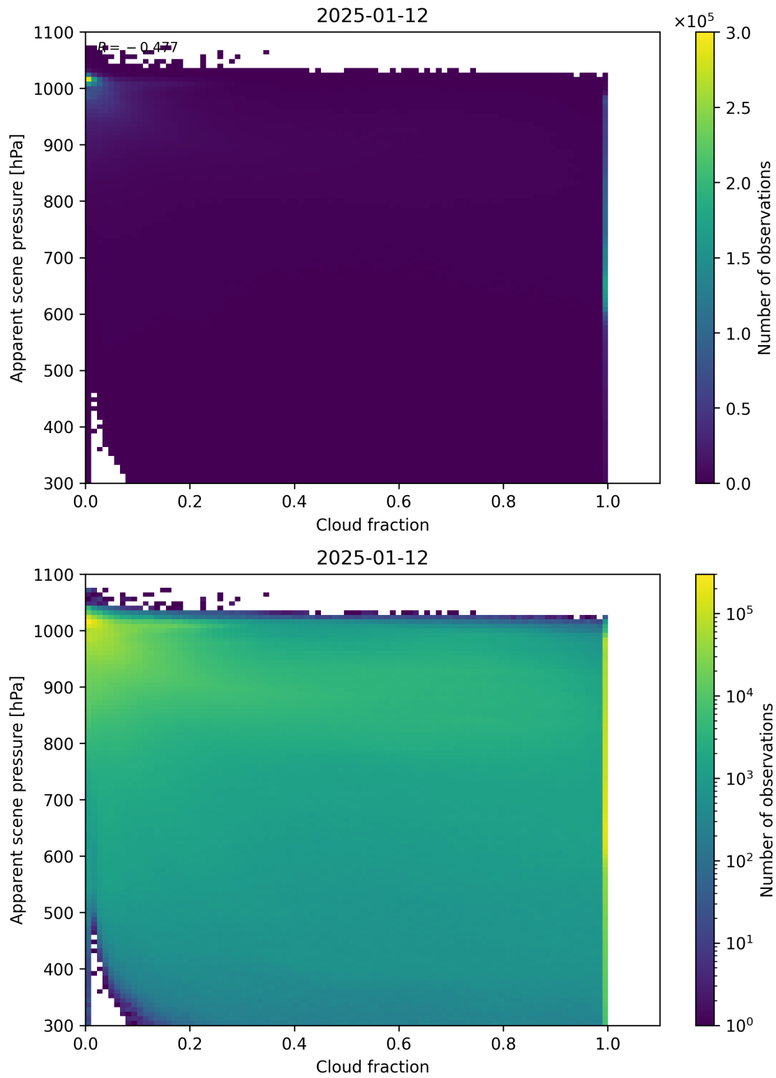
Figure 70: Scatter density plot of “Cloud fraction” against “Apparent scene pressure” for 2025-01-12 to 2025-01-13.
