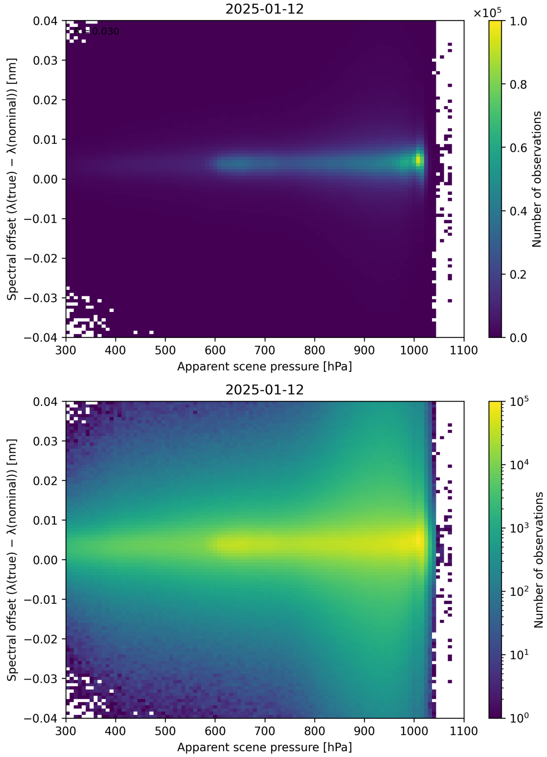
Figure 67: Scatter density plot of “Apparent scene pressure” against “Spectral offset ( \lambda_{\text{true}} - \lambda_{\text{nominal}} )” for 2025-01-12 to 2025-01-13.
