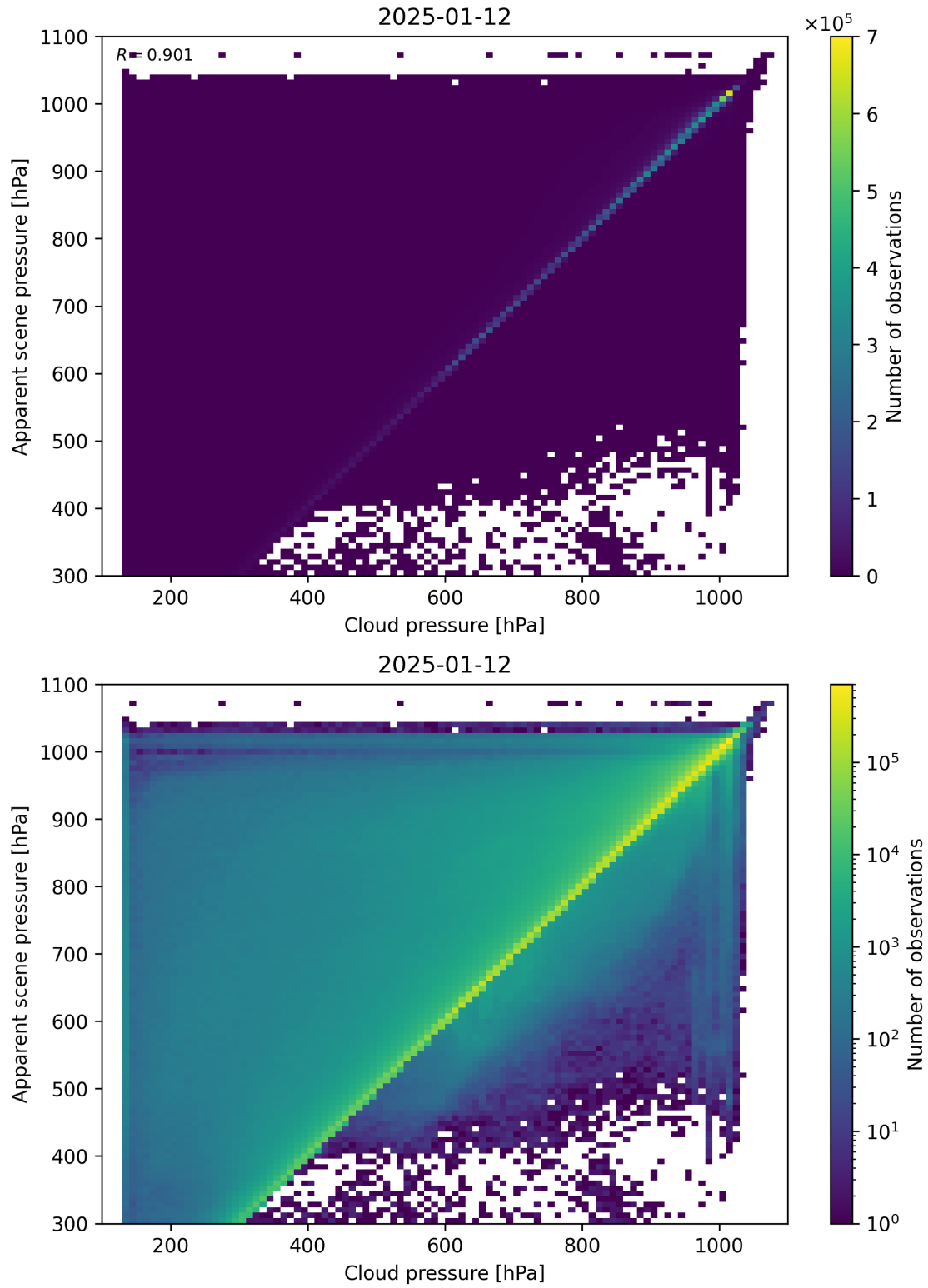
Figure 77: Scatter density plot of “Cloud pressure” against “Apparent scene pressure” for 2025-01-12 to 2025-01-13.
