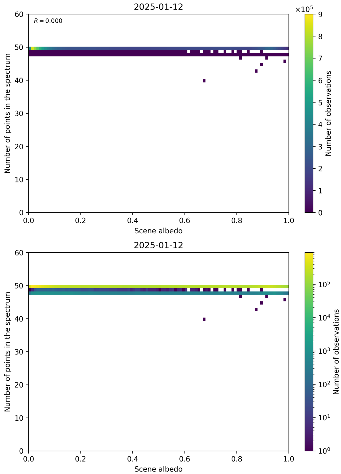
Figure 106: Scatter density plot of “Scene albedo” against “Number of points in the spectrum” for 2025-01-12 to 2025-01-13.
