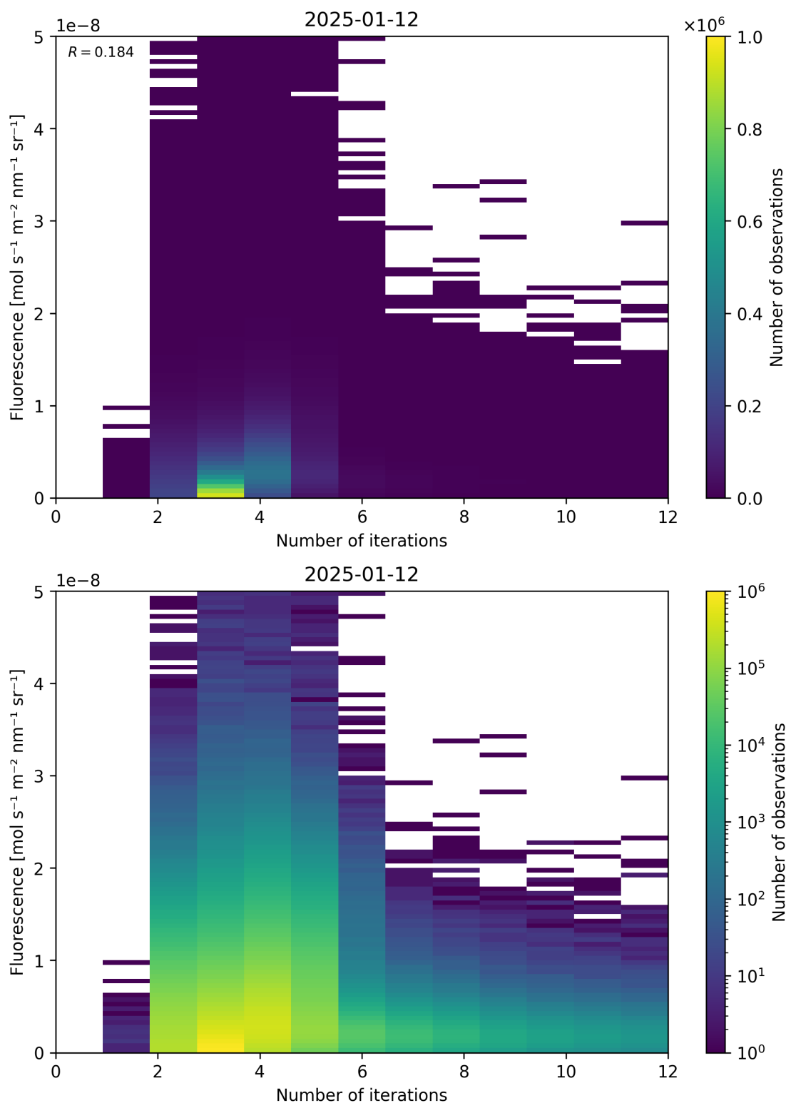
Figure 98: Scatter density plot of “Number of iterations” against “Fluorescence” for 2025-01-12 to 2025-01-13.
