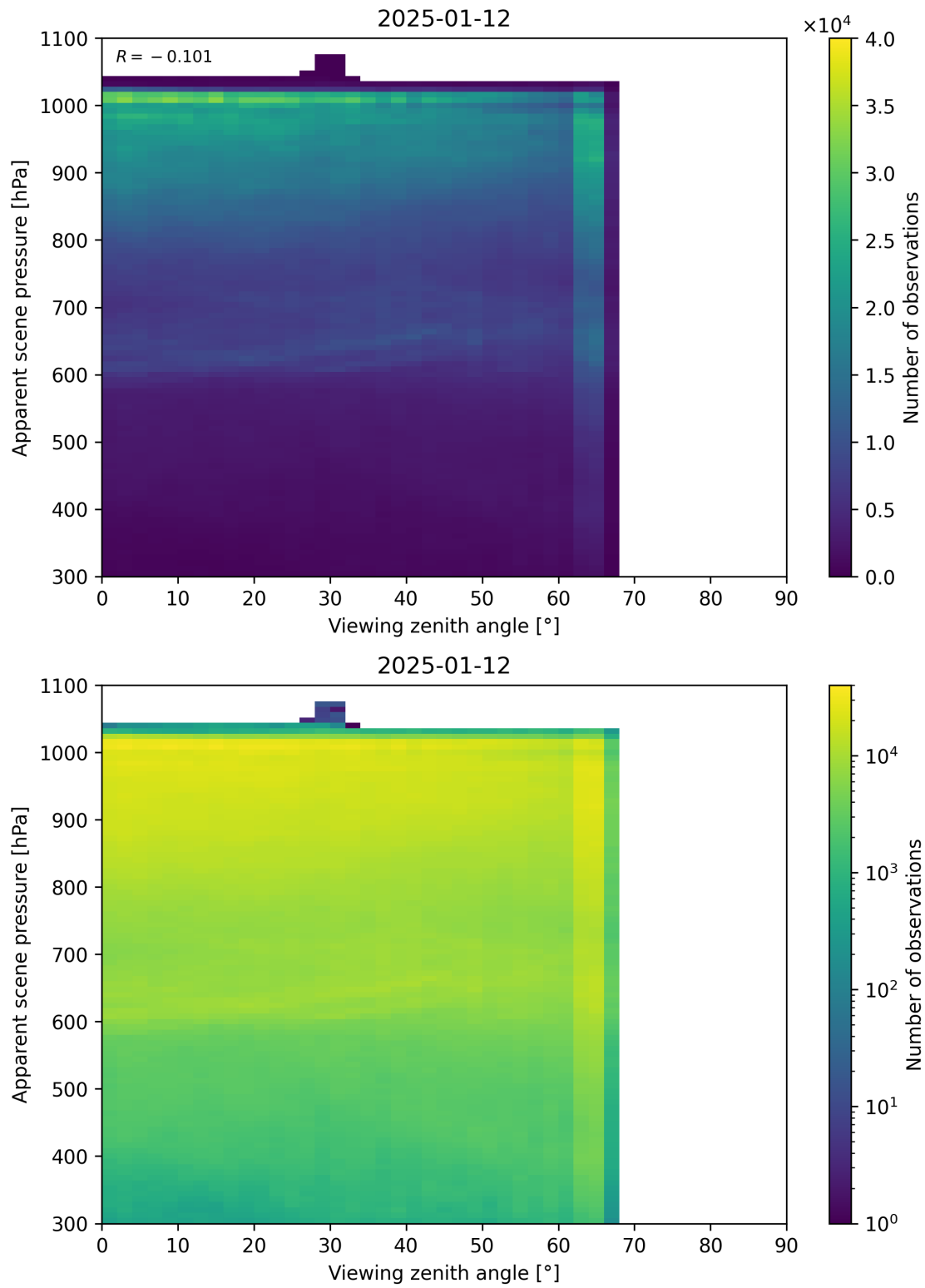
Figure 118: Scatter density plot of “Viewing zenith angle” against “Apparent scene pressure” for 2025-01-12 to 2025-01-13.
