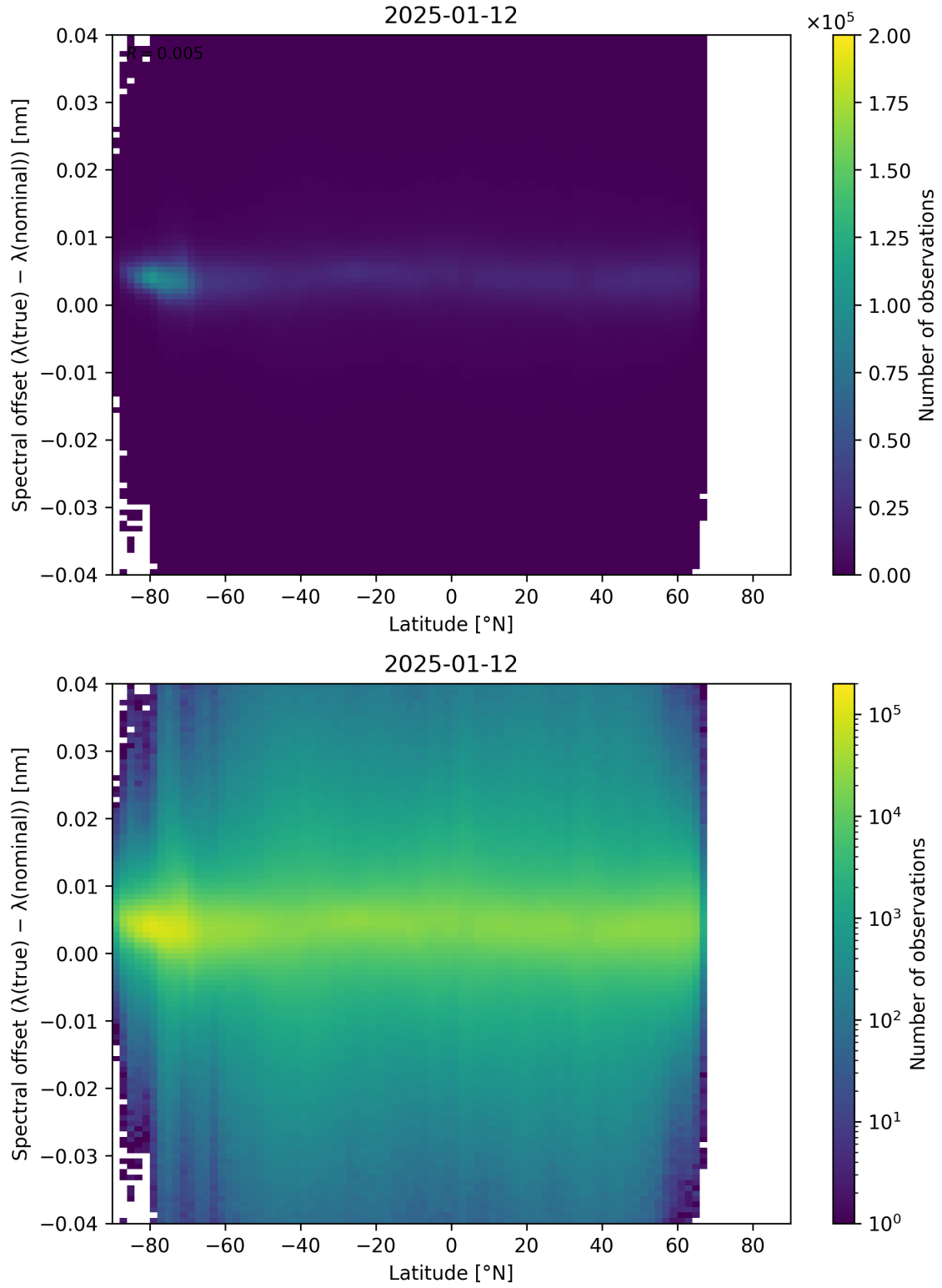
Figure 96: Scatter density plot of “Latitude” against “Spectral offset ( \lambda_{\text{true}} - \lambda_{\text{nominal}} )” for 2025-01-12 to 2025-01-13.
