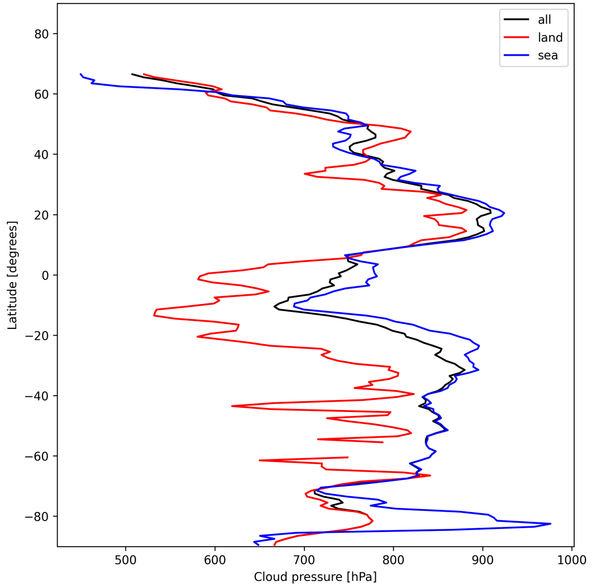
Figure 13: Zonal average of “Cloud pressure” for 2025-01-12 to 2025-01-13.
