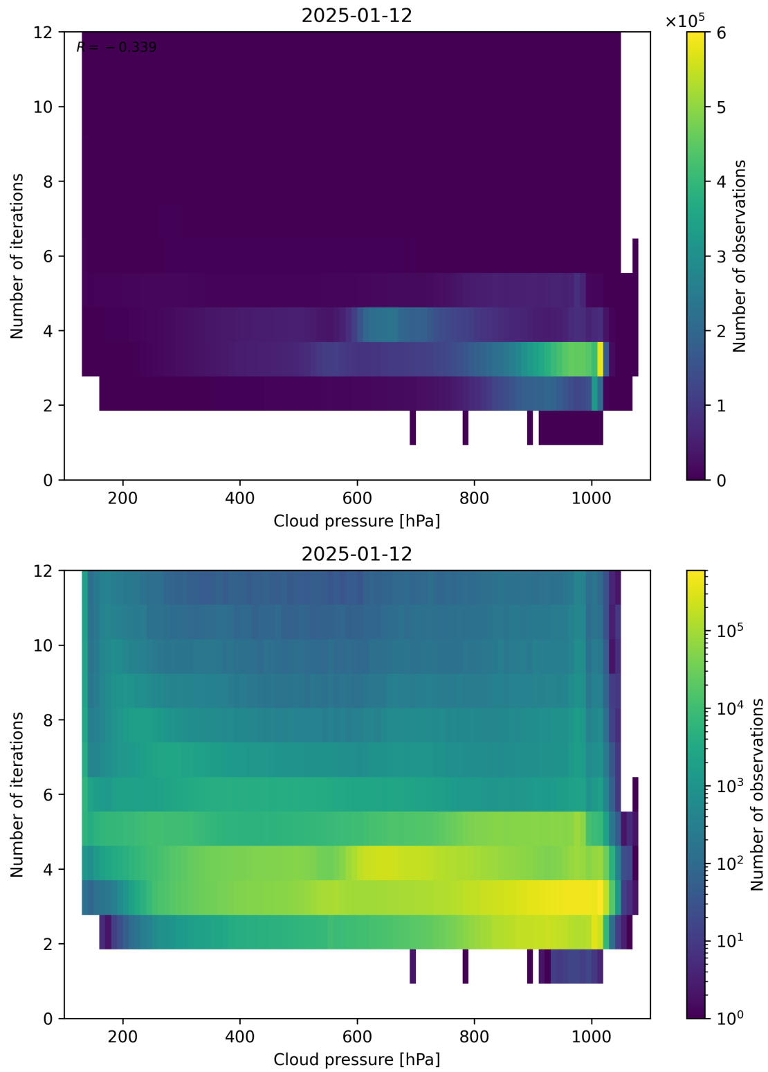
Figure 81: Scatter density plot of “Cloud pressure” against “Number of iterations” for 2025-01-12 to 2025-01-13.
