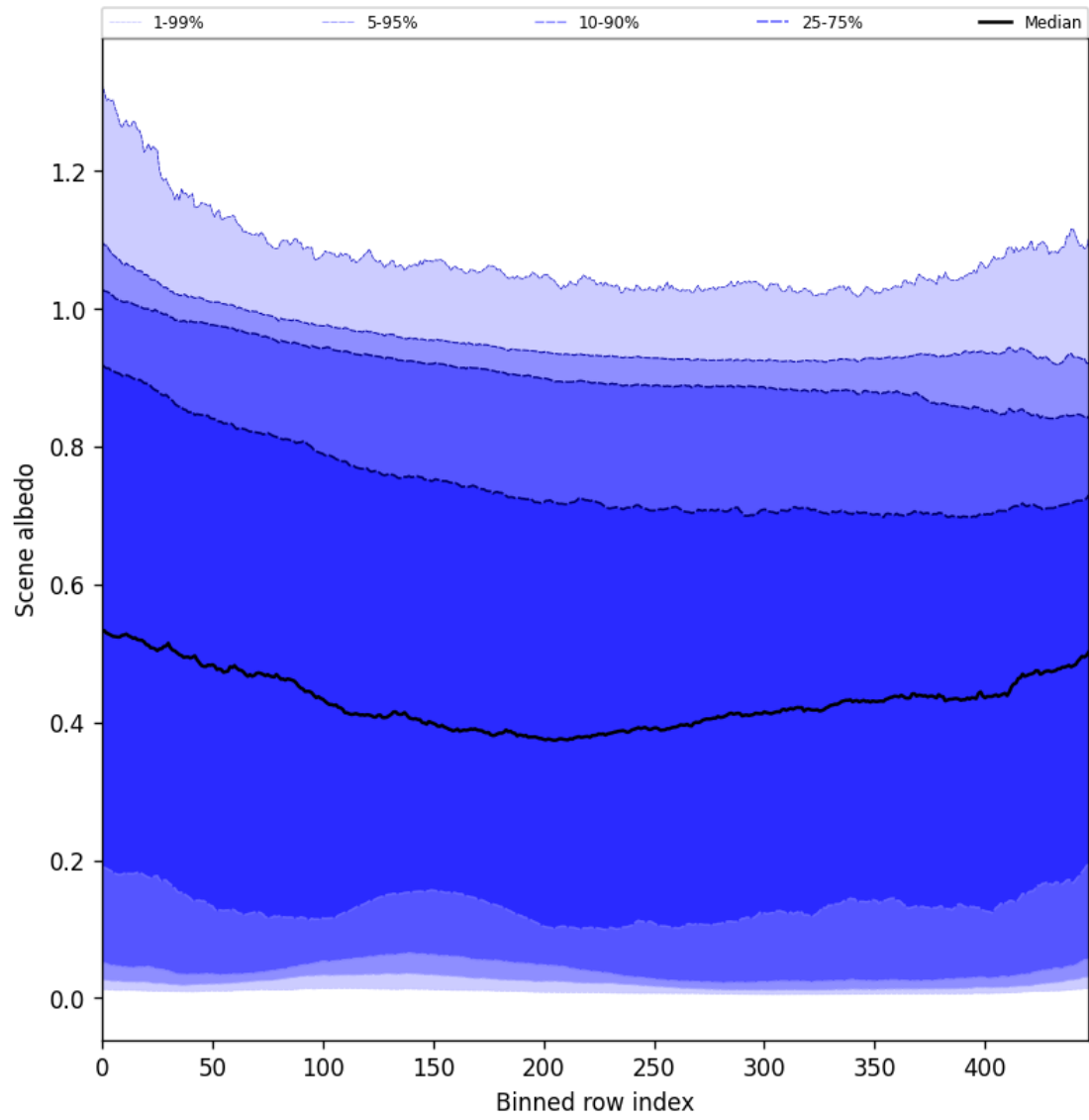
Figure 51: Along track statistics of “Scene albedo” for 2025-01-12 to 2025-01-13
