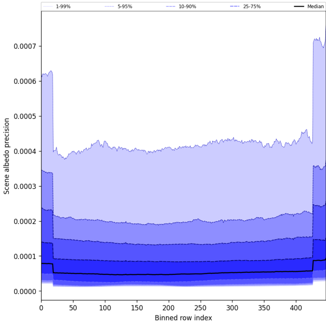
Figure 52: Along track statistics of “Scene albedo precision” for 2025-01-12 to 2025-01-13
