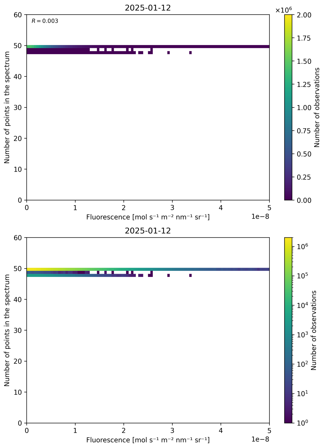
Figure 86: Scatter density plot of “Fluorescence” against “Number of points in the spectrum” for 2025-01-12 to 2025-01-13.
