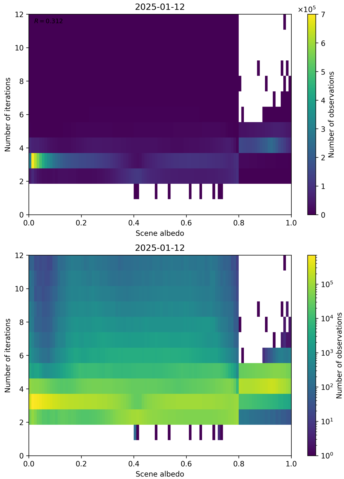
Figure 105: Scatter density plot of “Scene albedo” against “Number of iterations” for 2025-01-12 to 2025-01-13.
