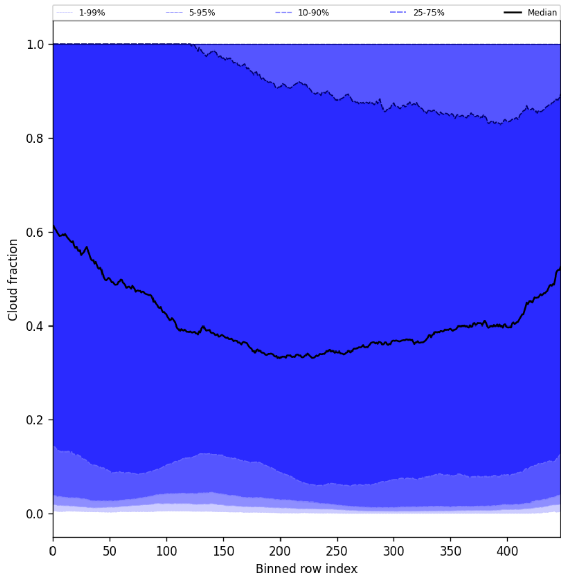
Figure 49: Along track statistics of “Cloud fraction” for 2025-01-12 to 2025-01-13
