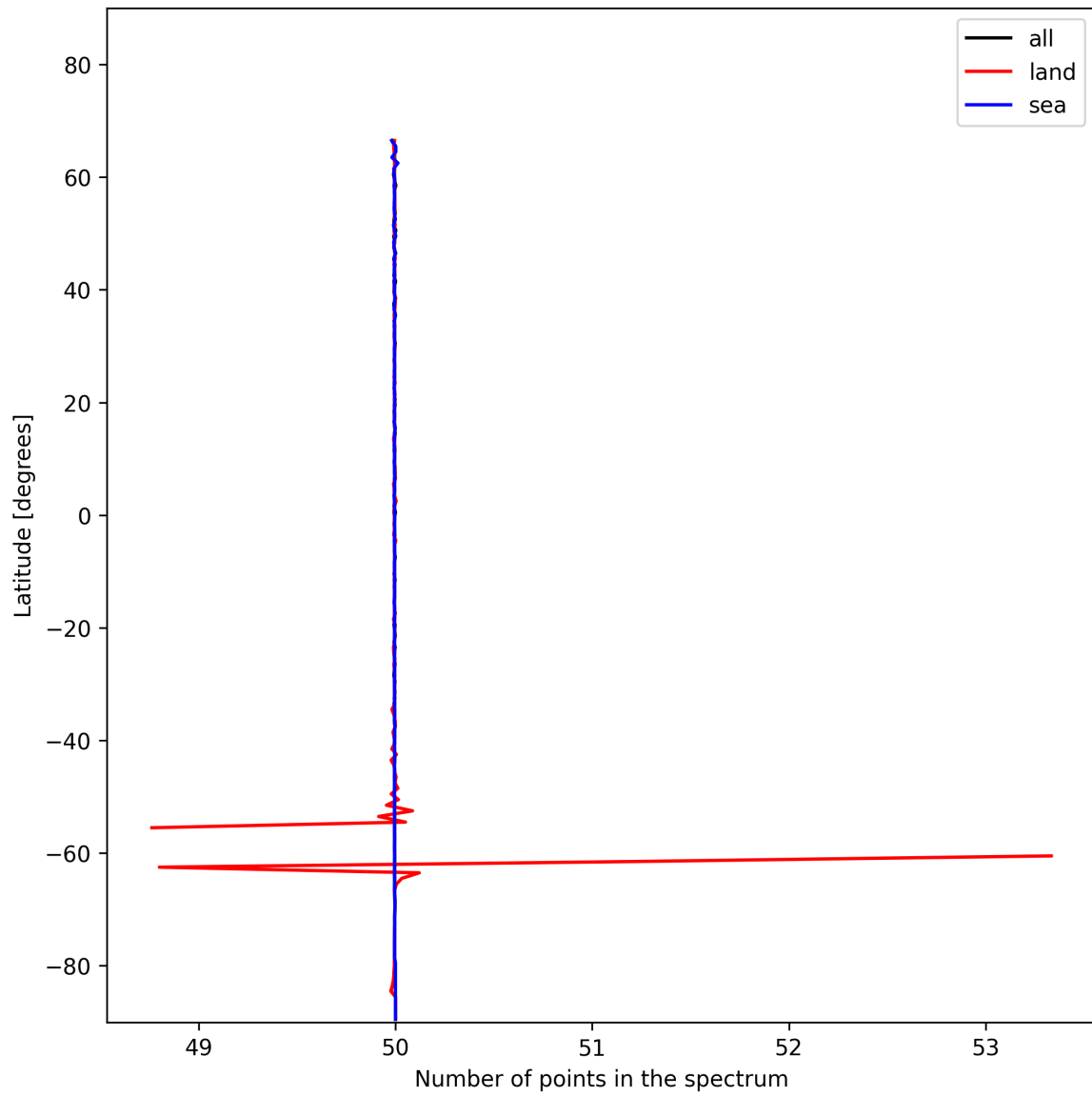
Figure 27: Zonal average of “Number of points in the spectrum” for 2025-01-12 to 2025-01-13.
