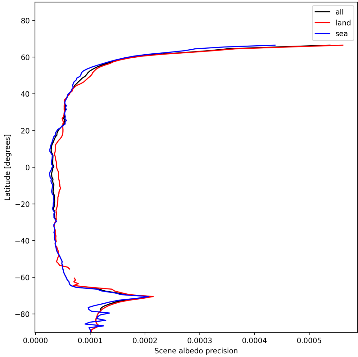
Figure 18: Zonal average of “Scene albedo precision” for 2025-01-12 to 2025-01-13.
