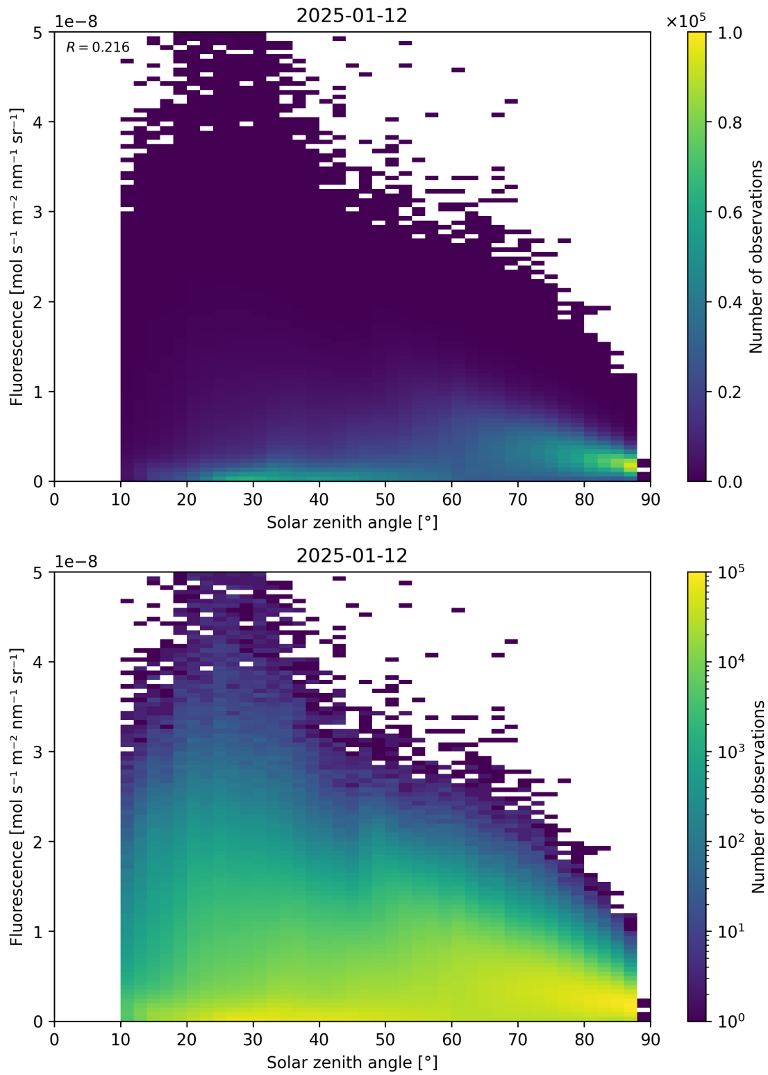
Figure 112: Scatter density plot of “Solar zenith angle” against “Fluorescence” for 2025-01-12 to 2025-01-13.
