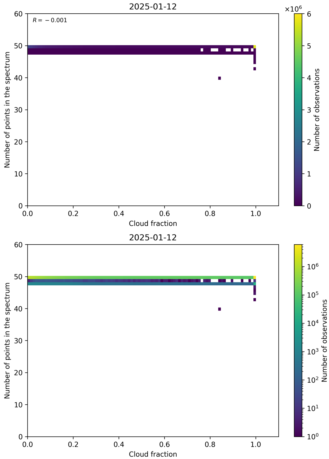
Figure 74: Scatter density plot of “Cloud fraction” against “Number of points in the spectrum” for 2025-01-12 to 2025-01-13.
