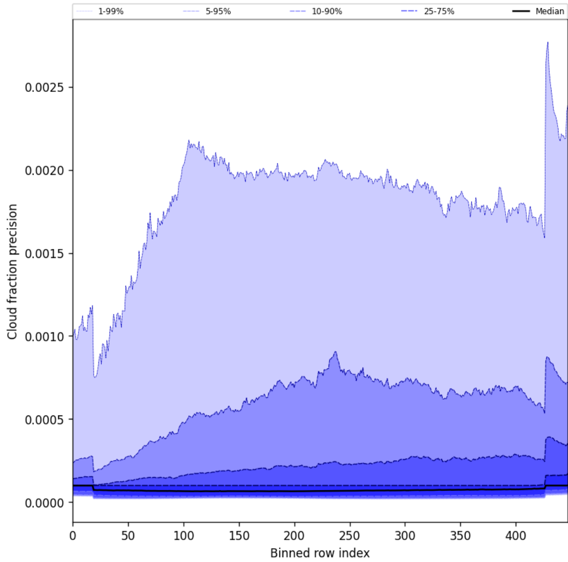
Figure 50: Along track statistics of “Cloud fraction precision” for 2025-01-12 to 2025-01-13
