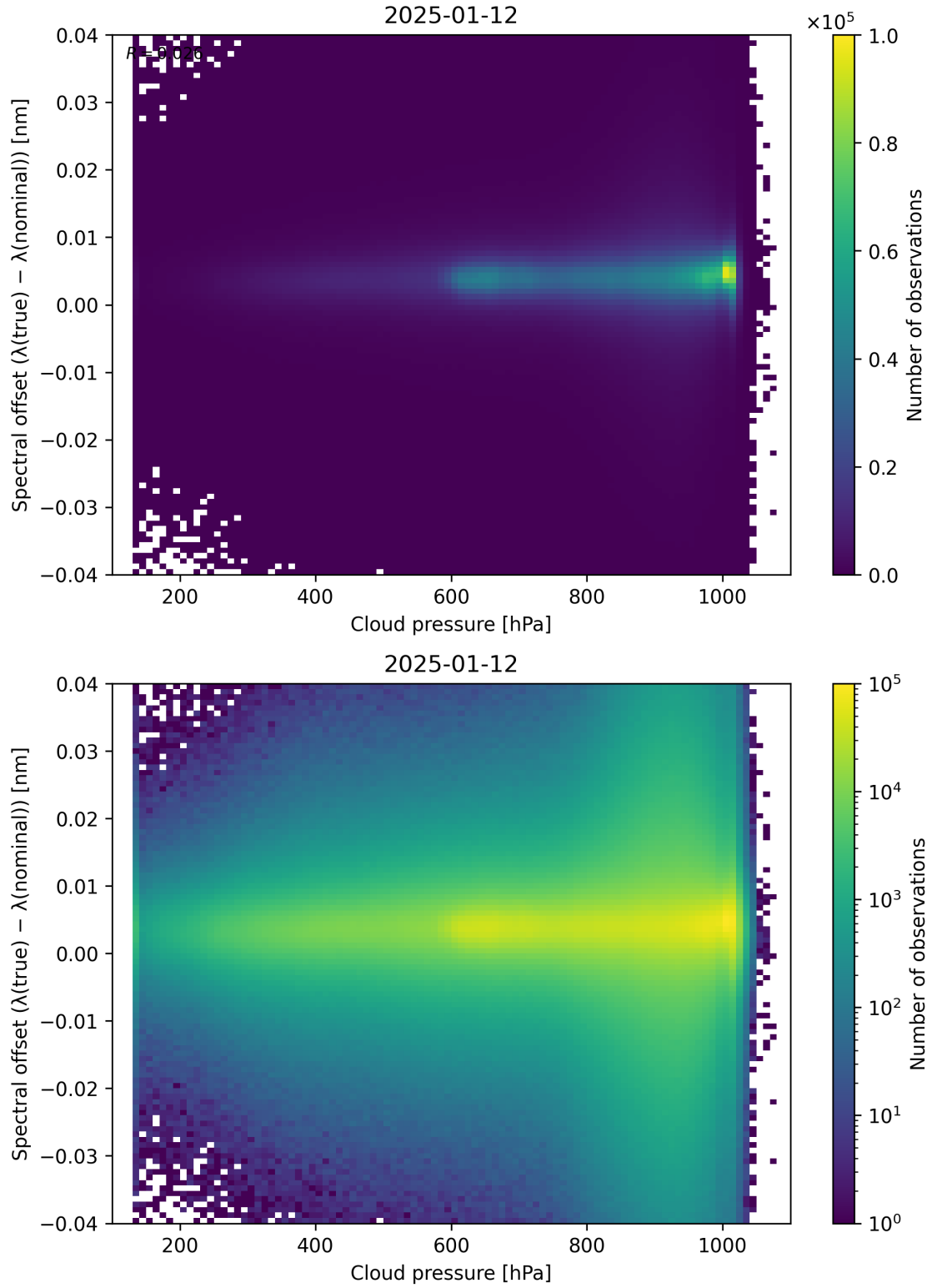
Figure 84: Scatter density plot of “Cloud pressure” against “Spectral offset ( \lambda_{\text{true}} - \lambda_{\text{nominal}} )” for 2025-01-12 to 2025-01-13.
