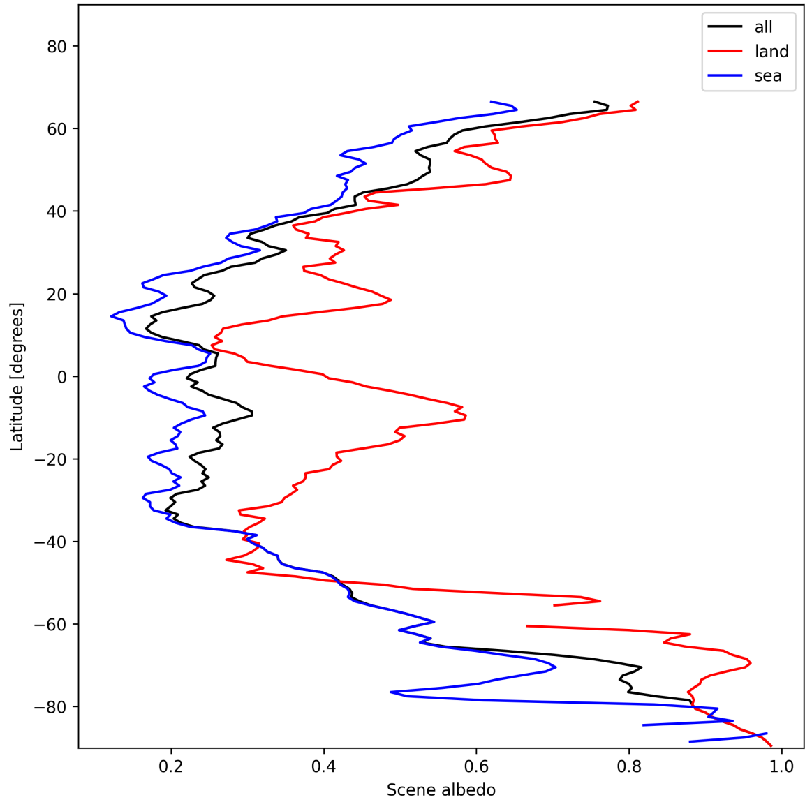
Figure 17: Zonal average of “Scene albedo” for 2025-01-12 to 2025-01-14.
