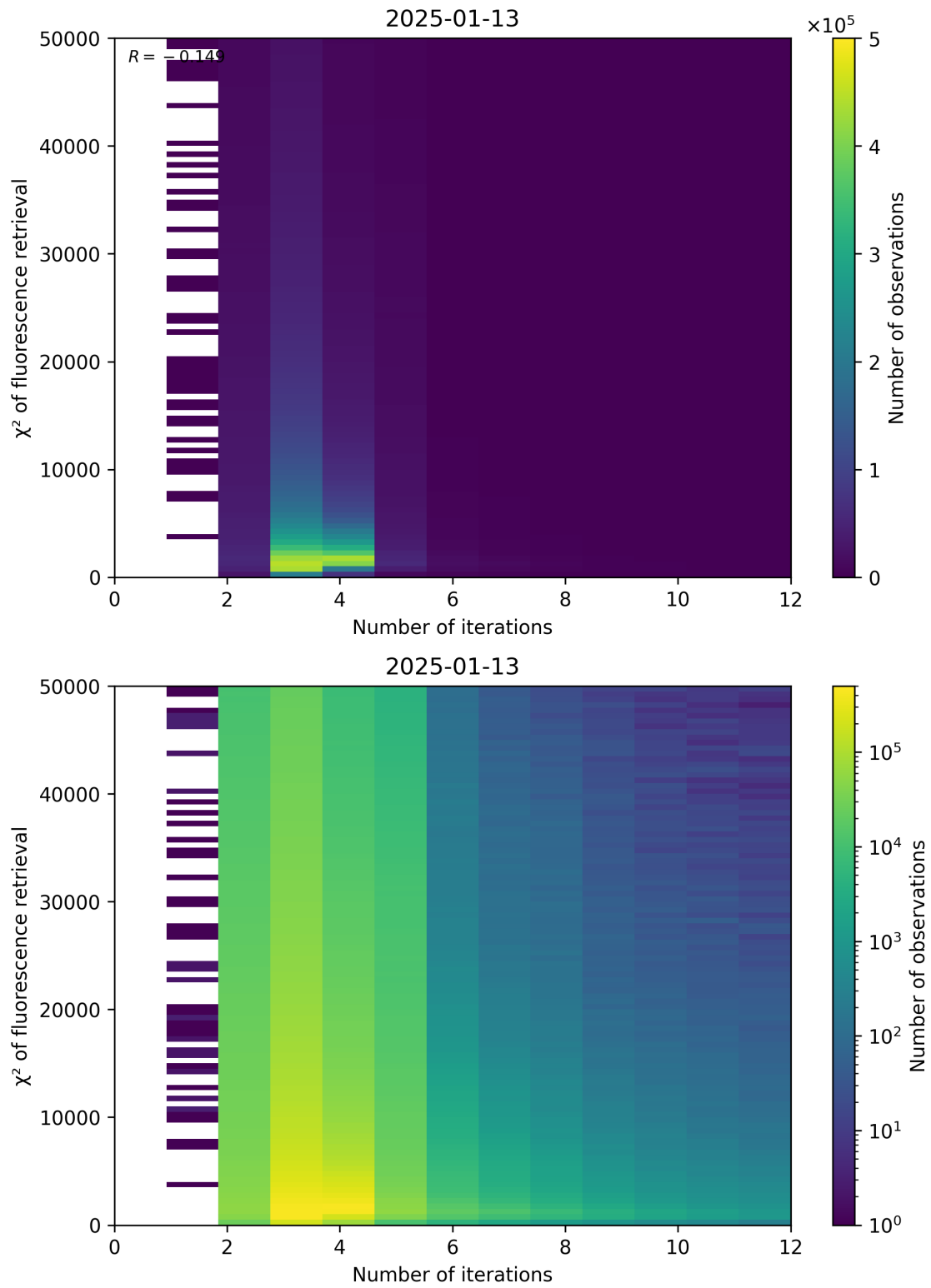
Figure 97: Scatter density plot of “Number of iterations” against “ \chi^2 of fluorescence retrieval” for 2025-01-12 to 2025-01-14.
