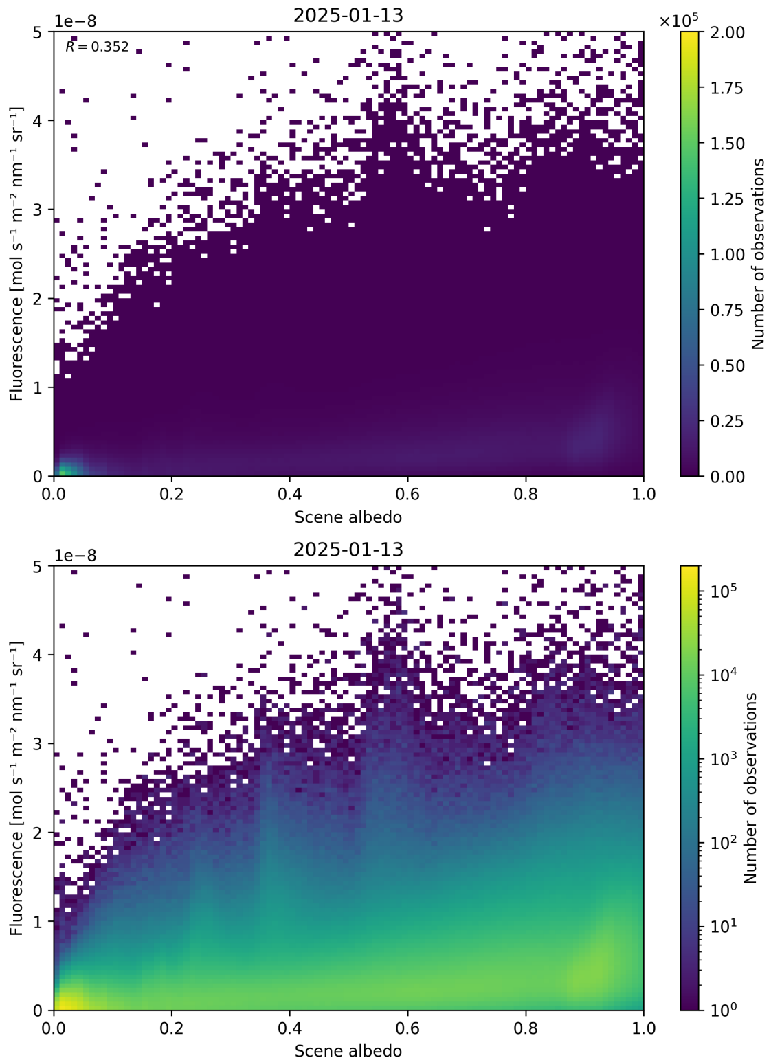
Figure 104: Scatter density plot of “Scene albedo” against “Fluorescence” for 2025-01-12 to 2025-01-14.
