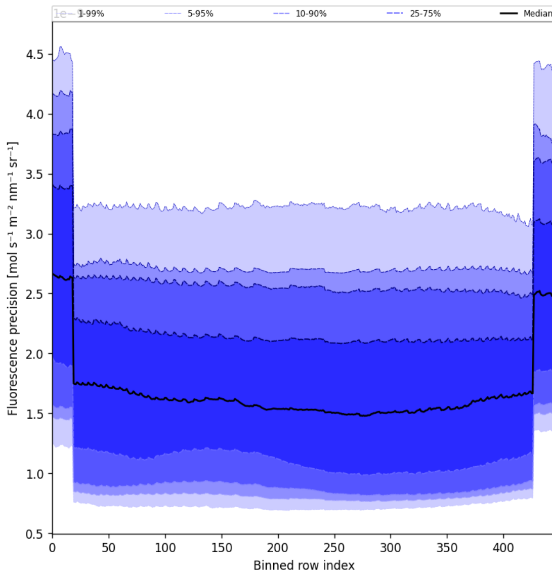
Figure 58: Along track statistics of “Fluorescence precision” for 2025-01-12 to 2025-01-14
