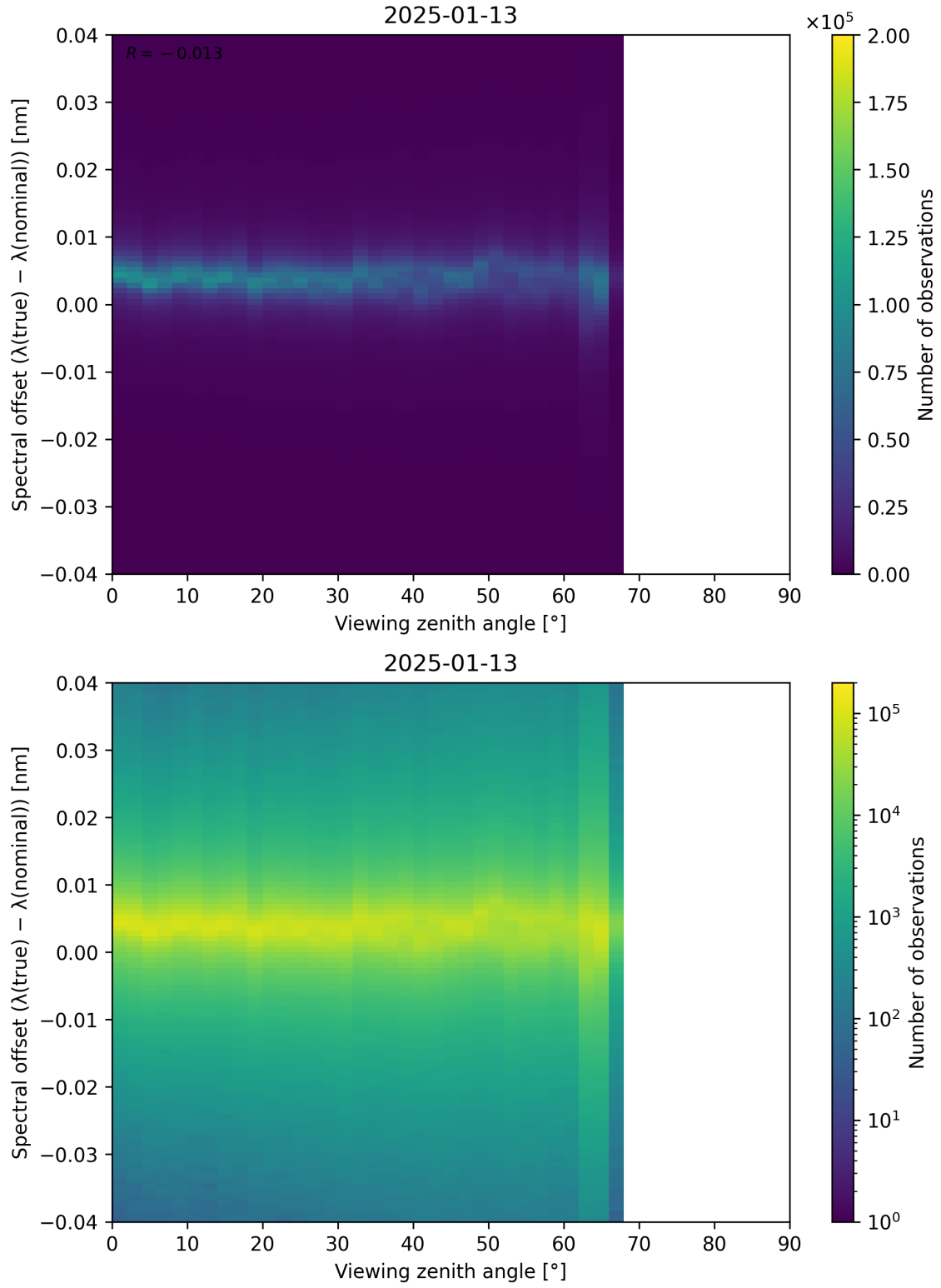
Figure 128: Scatter density plot of “Viewing zenith angle” against “Spectral offset ( \lambda_{\text{true}} - \lambda_{\text{nominal}} )” for 2025-01-12 to 2025-01-14.
