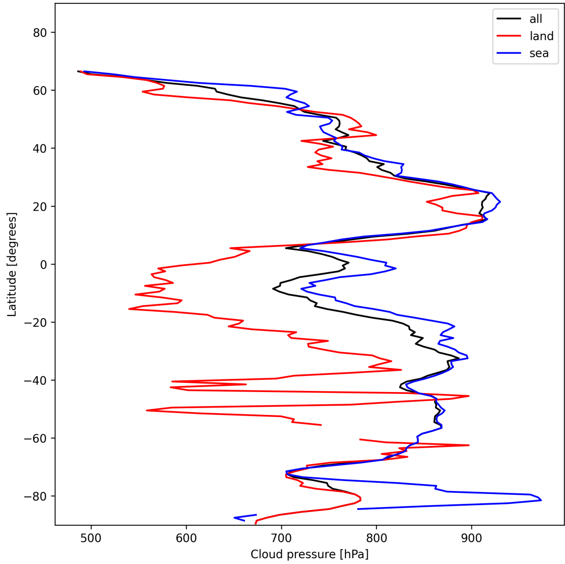
Figure 13: Zonal average of “Cloud pressure” for 2025-01-12 to 2025-01-14.
