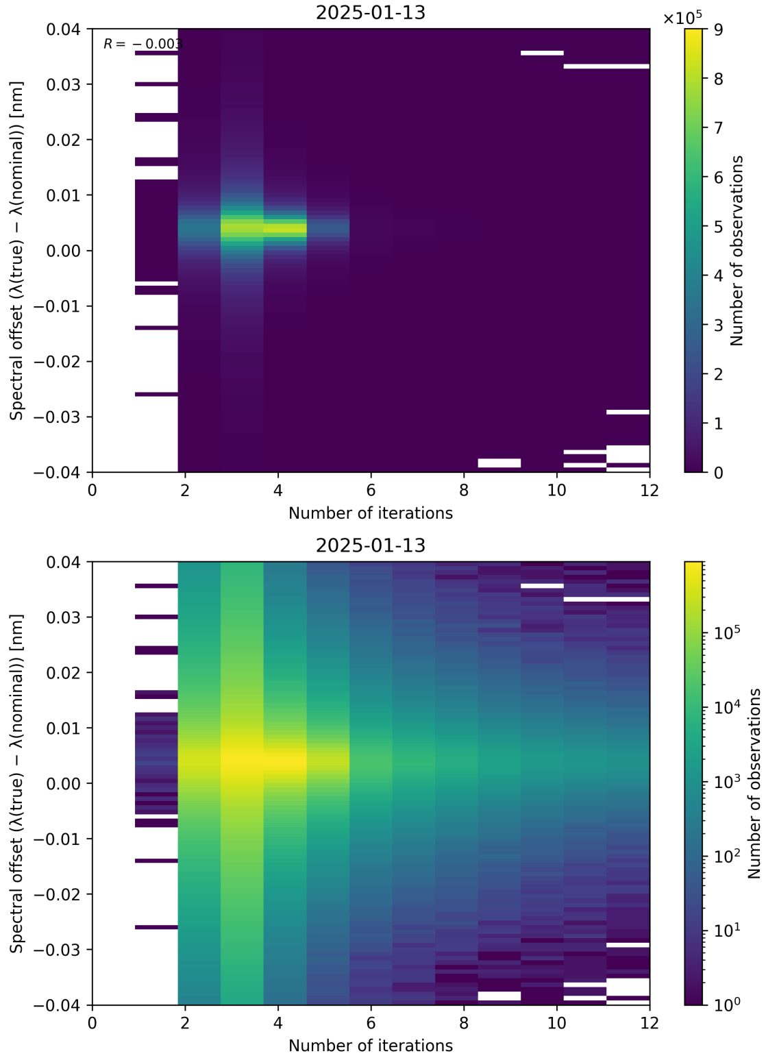
Figure 100: Scatter density plot of “Number of iterations” against “Spectral offset ( \lambda_{\text{true}} - \lambda_{\text{nominal}} )” for 2025-01-12 to 2025-01-14.
