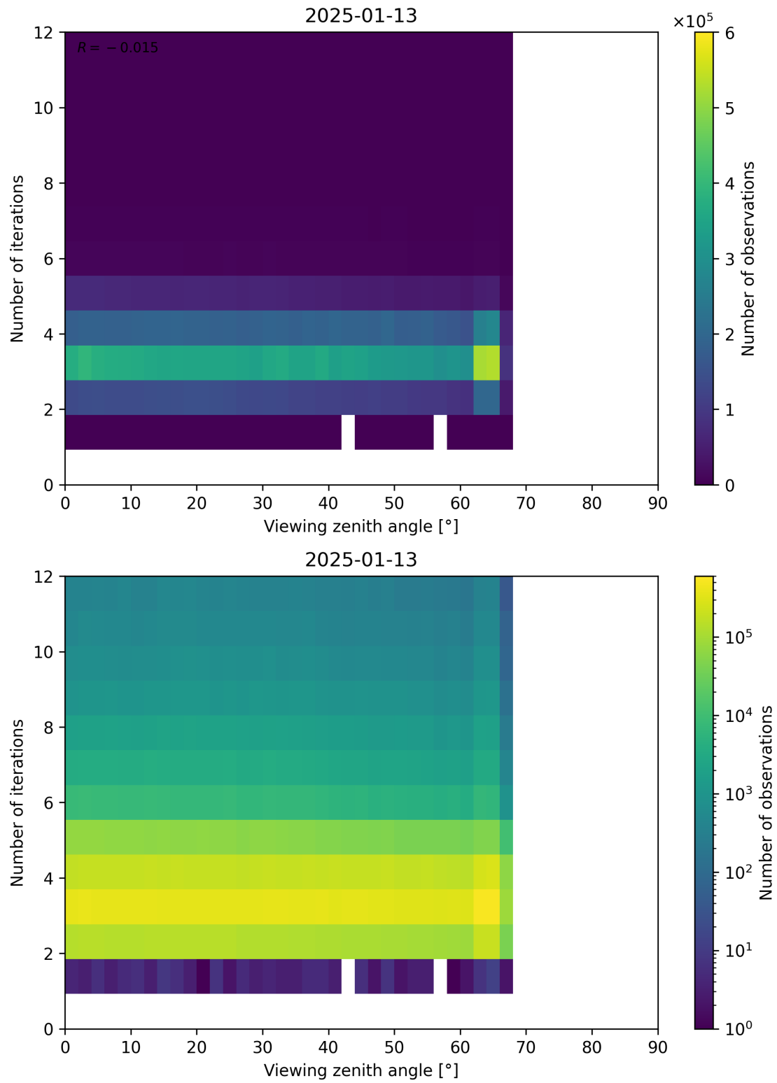
Figure 124: Scatter density plot of “Viewing zenith angle” against “Number of iterations” for 2025-01-12 to 2025-01-14.
