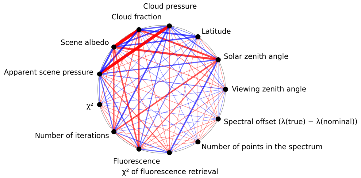
Figure 1: Map of correlation graph for 2025-01-12 to 2025-01-14.
