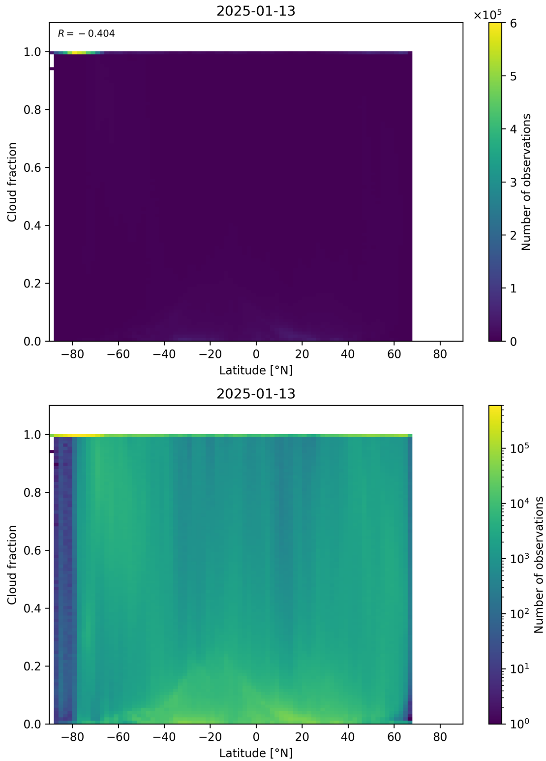
Figure 90: Scatter density plot of “Latitude” against “Cloud fraction” for 2025-01-12 to 2025-01-14.
