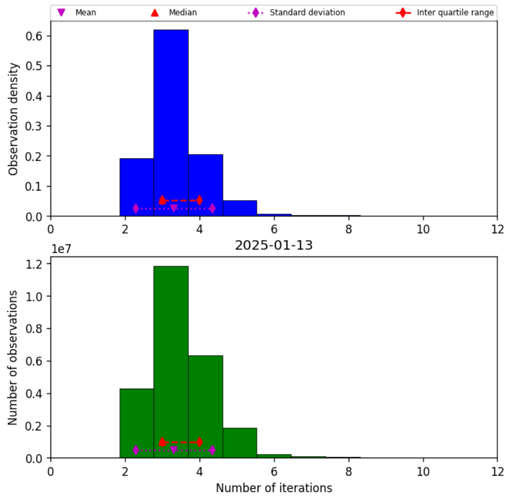
Figure 39: Histogram of “Number of iterations” for 2025-01-12 to 2025-01-14
