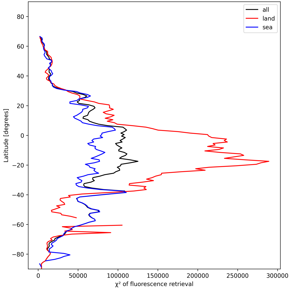
Figure 25: Zonal average of “ \chi^2 of fluorescence retrieval” for 2025-01-12 to 2025-01-14.
