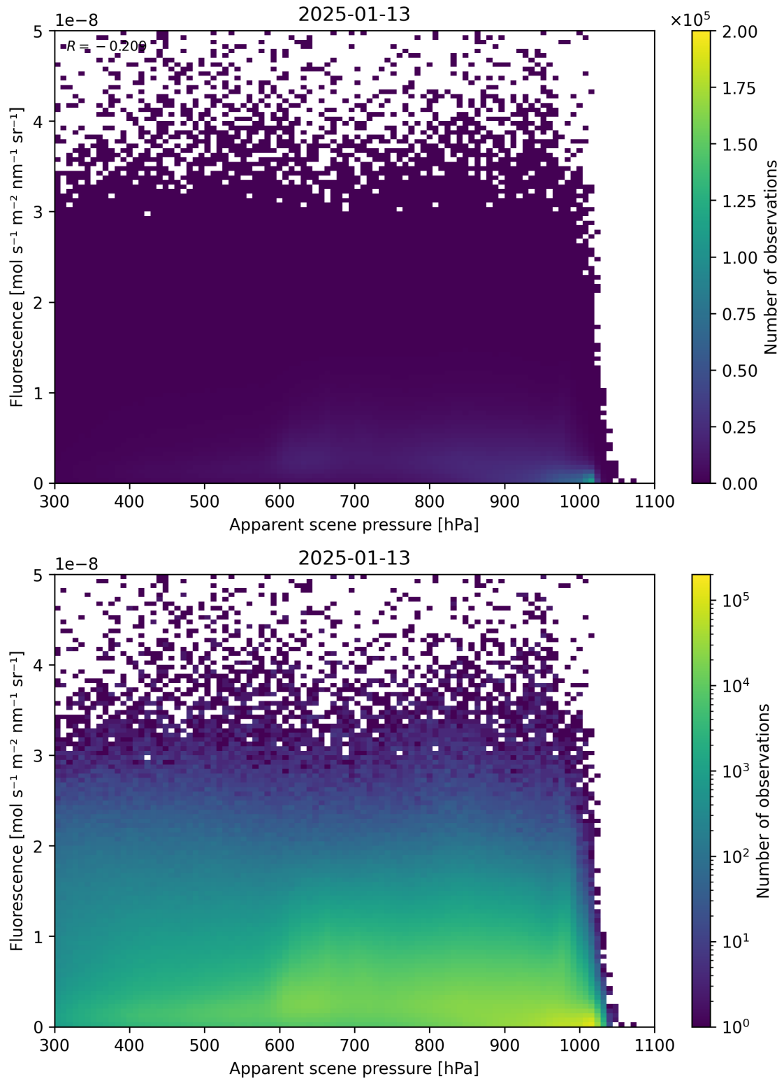
Figure 64: Scatter density plot of “Apparent scene pressure” against “Fluorescence” for 2025-01-12 to 2025-01-14.
