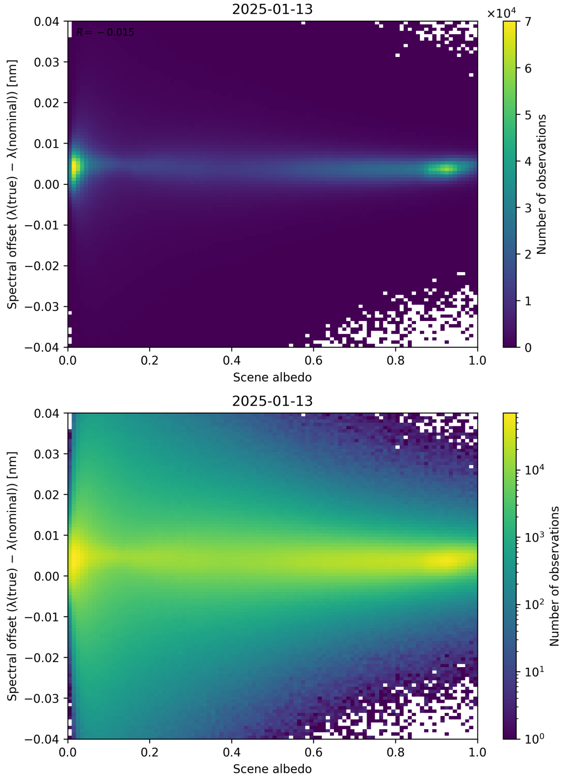
Figure 107: Scatter density plot of “Scene albedo” against “Spectral offset ( \lambda_{\text{true}} - \lambda_{\text{nominal}} )” for 2025-01-12 to 2025-01-14.
