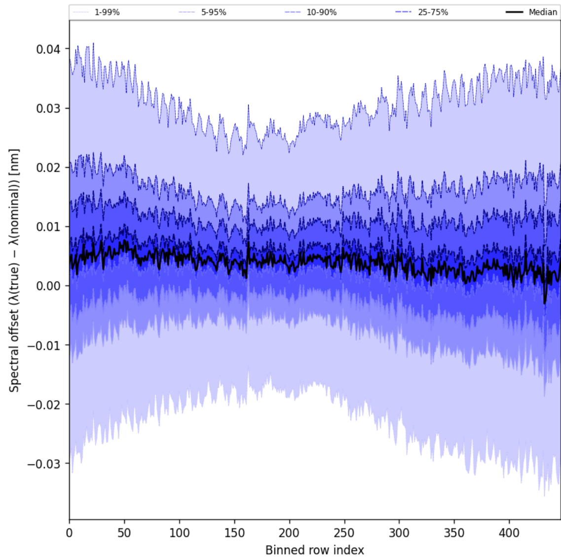
Figure 62: Along track statistics of “Spectral offset ( \lambda_{\text{true}} - \lambda_{\text{nominal}} )” for 2025-01-12 to 2025-01-14
