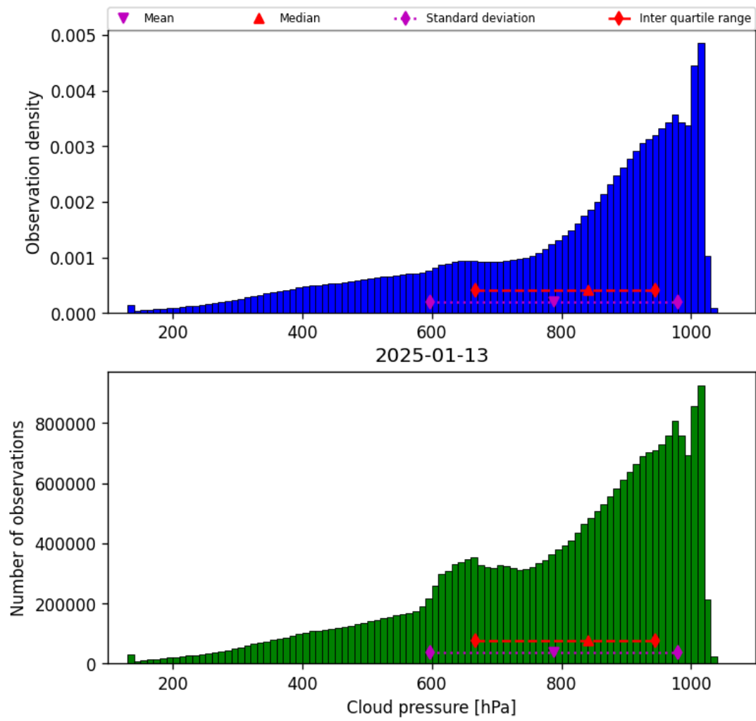
Figure 30: Histogram of “Cloud pressure” for 2025-01-12 to 2025-01-14
