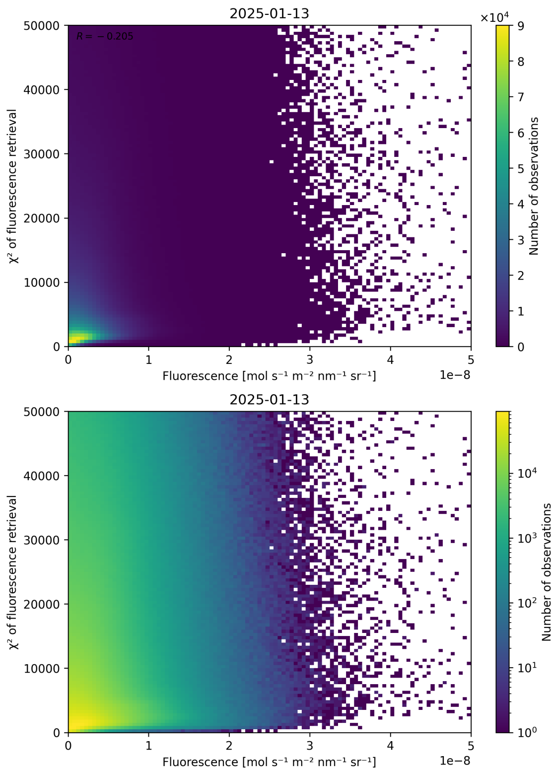
Figure 85: Scatter density plot of “Fluorescence” against “ \chi^2 of fluorescence retrieval” for 2025-01-12 to 2025-01-14.
