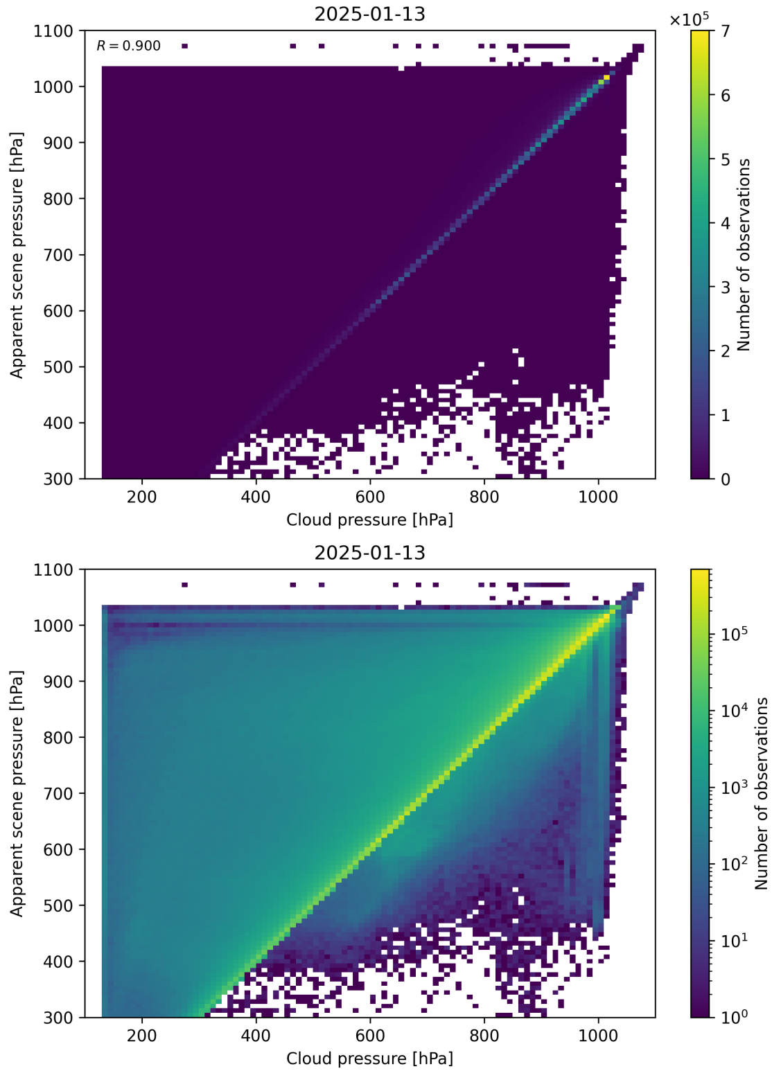
Figure 77: Scatter density plot of “Cloud pressure” against “Apparent scene pressure” for 2025-01-12 to 2025-01-14.
