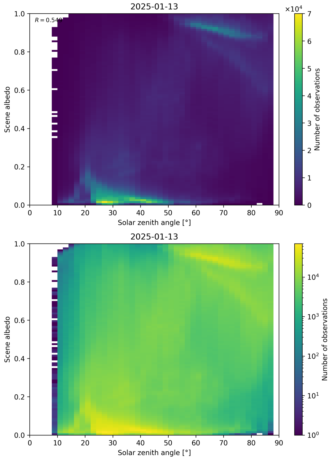
Figure 116: Scatter density plot of “Solar zenith angle” against “Scene albedo” for 2025-01-12 to 2025-01-14.
