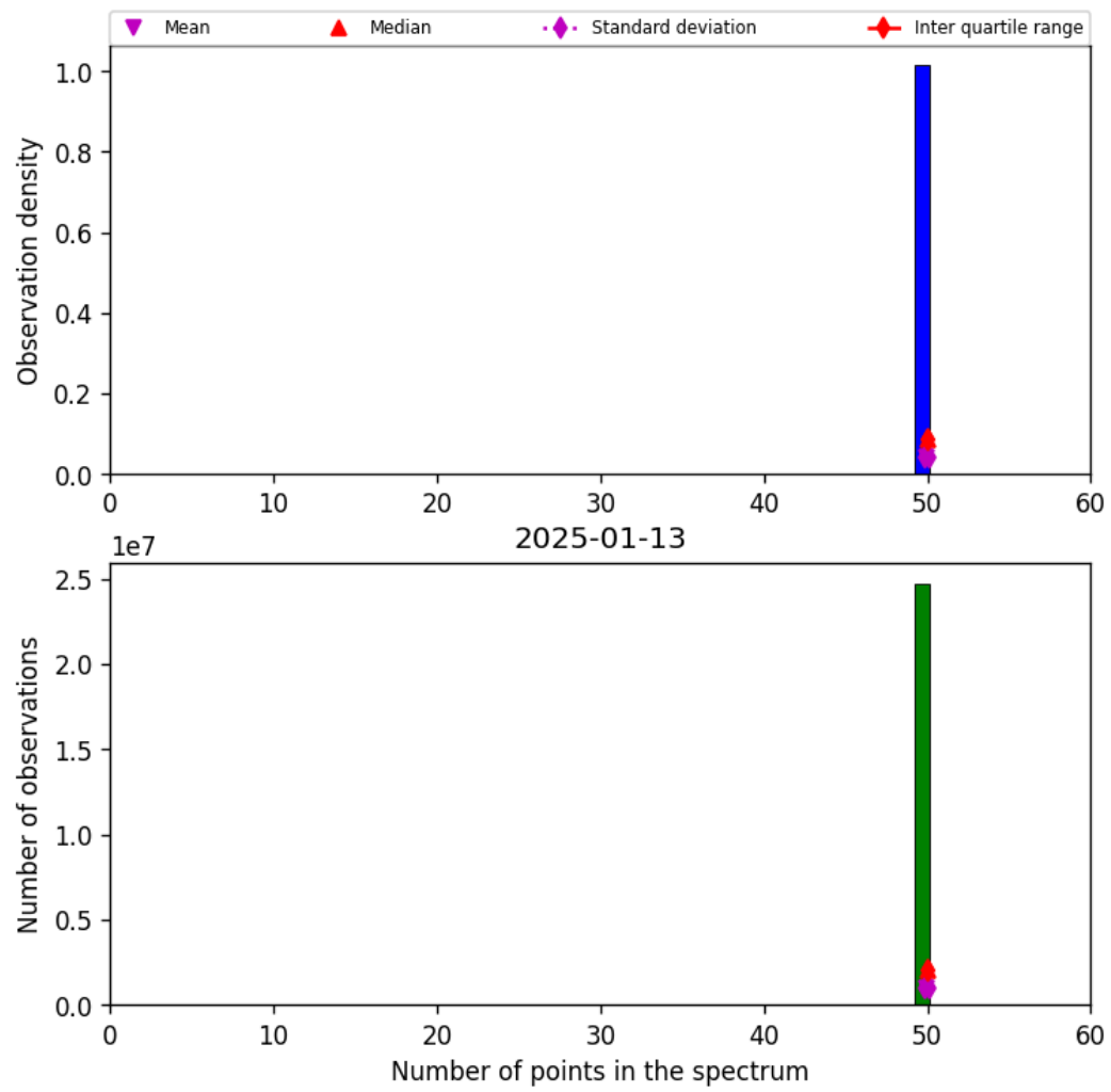
Figure 44: Histogram of “Number of points in the spectrum” for 2025-01-12 to 2025-01-14
