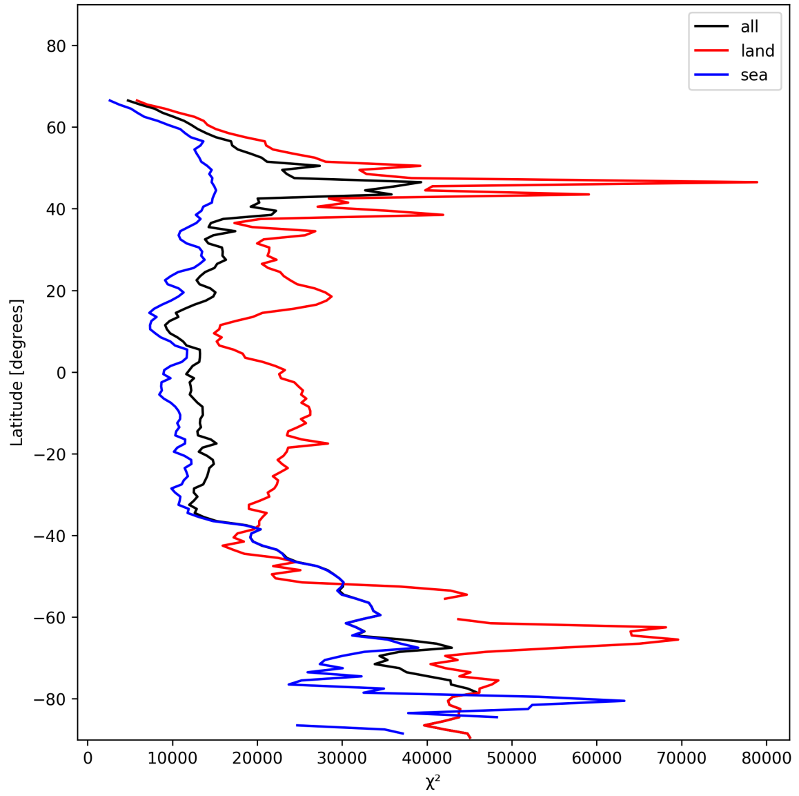
Figure 21: Zonal average of “ \chi^2 ” for 2025-01-12 to 2025-01-14.
