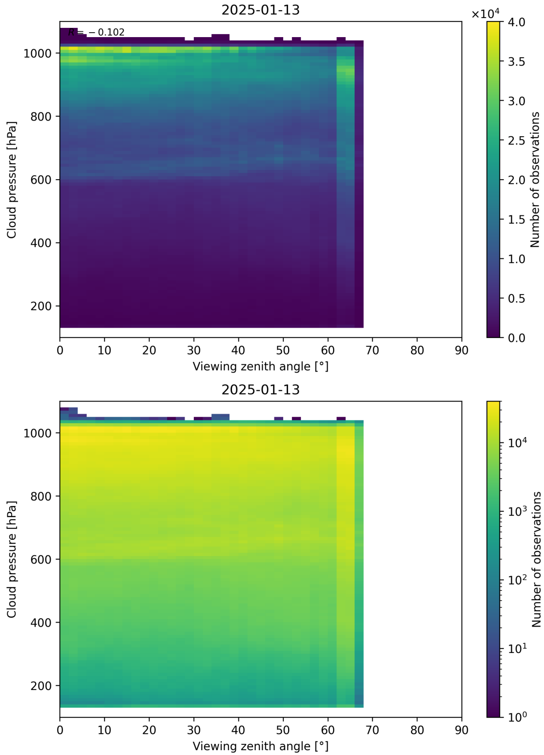
Figure 121: Scatter density plot of “Viewing zenith angle” against “Cloud pressure” for 2025-01-12 to 2025-01-14.
