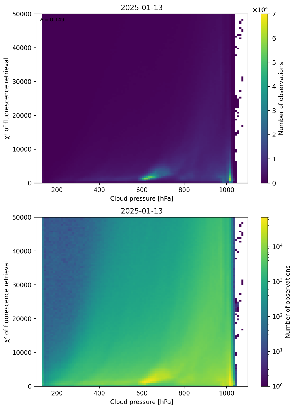
Figure 78: Scatter density plot of “Cloud pressure” against “ \chi^2 of fluorescence retrieval” for 2025-01-12 to 2025-01-14.
