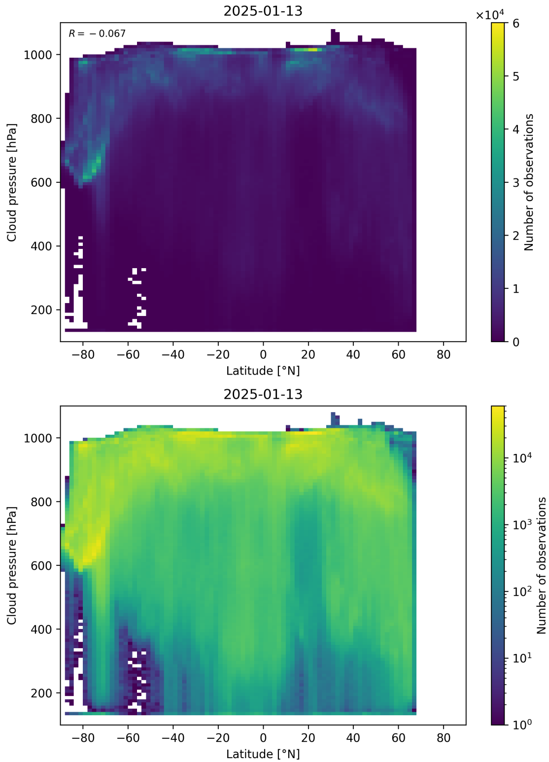
Figure 91: Scatter density plot of “Latitude” against “Cloud pressure” for 2025-01-12 to 2025-01-14.
