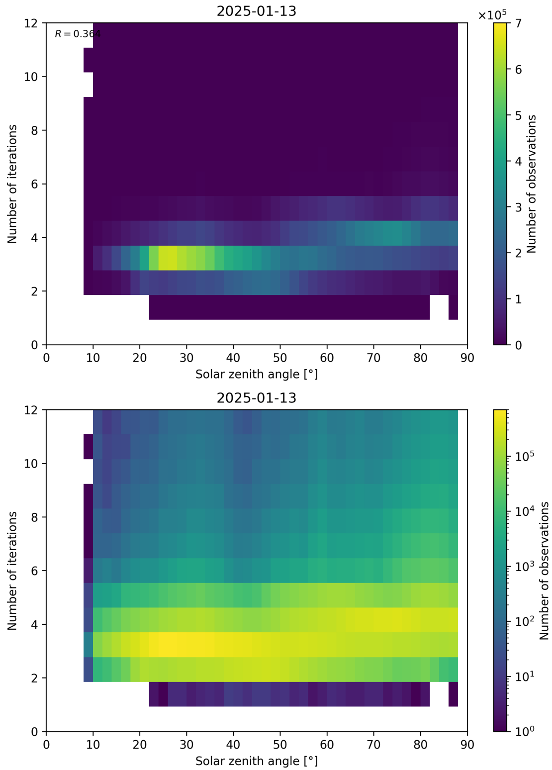
Figure 114: Scatter density plot of “Solar zenith angle” against “Number of iterations” for 2025-01-12 to 2025-01-14.
