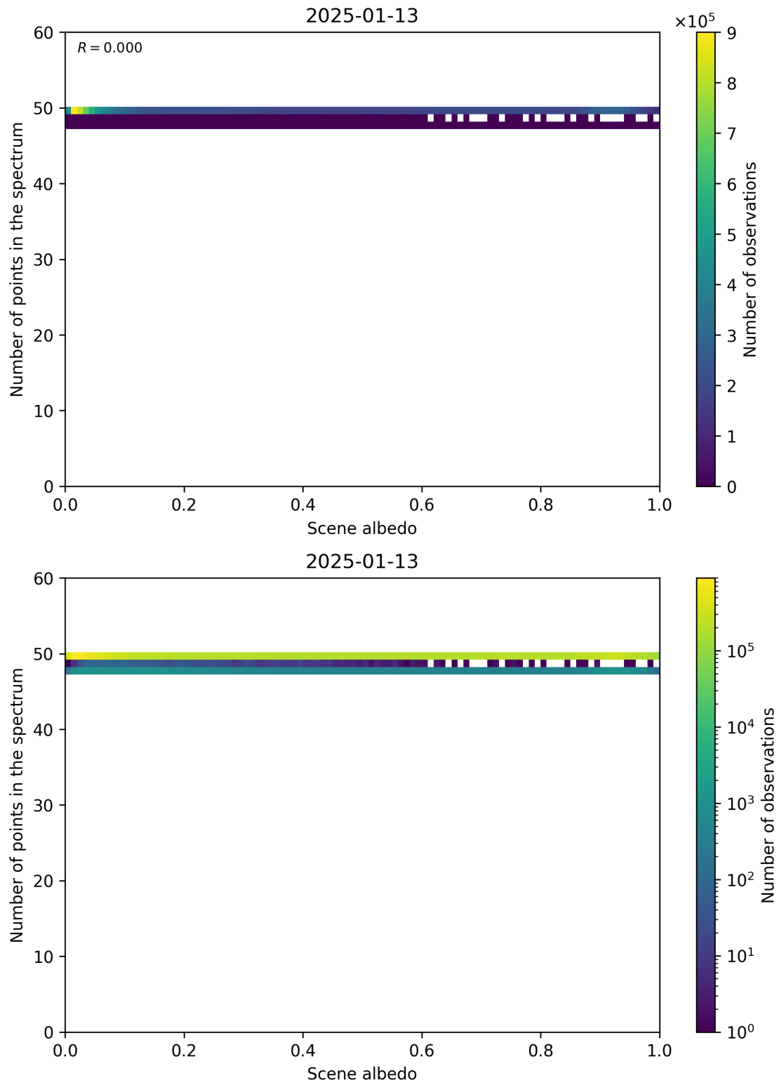
Figure 106: Scatter density plot of “Scene albedo” against “Number of points in the spectrum” for 2025-01-12 to 2025-01-14.
