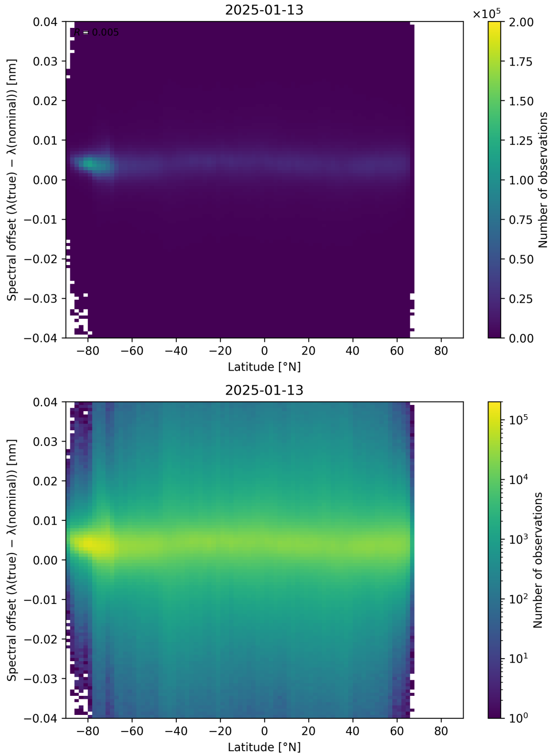
Figure 96: Scatter density plot of “Latitude” against “Spectral offset ( \lambda_{\text{true}} - \lambda_{\text{nominal}} )” for 2025-01-12 to 2025-01-14.
