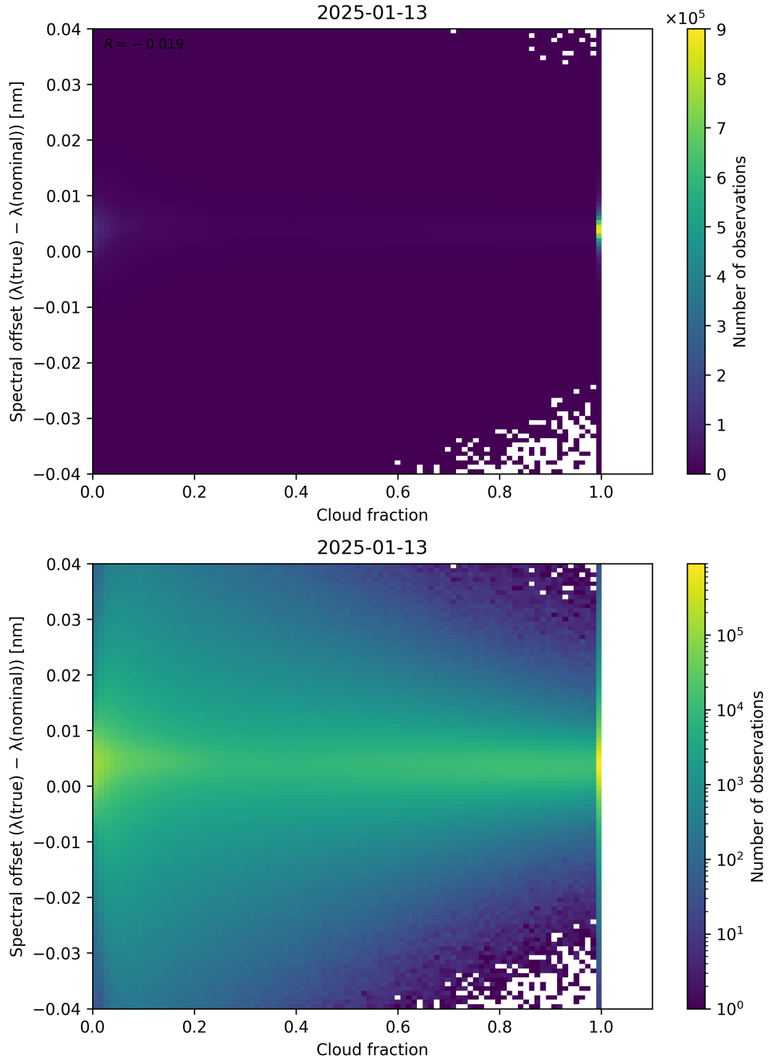
Figure 76: Scatter density plot of “Cloud fraction” against “Spectral offset ( \lambda_{\text{true}} - \lambda_{\text{nominal}} )” for 2025-01-12 to 2025-01-14.
