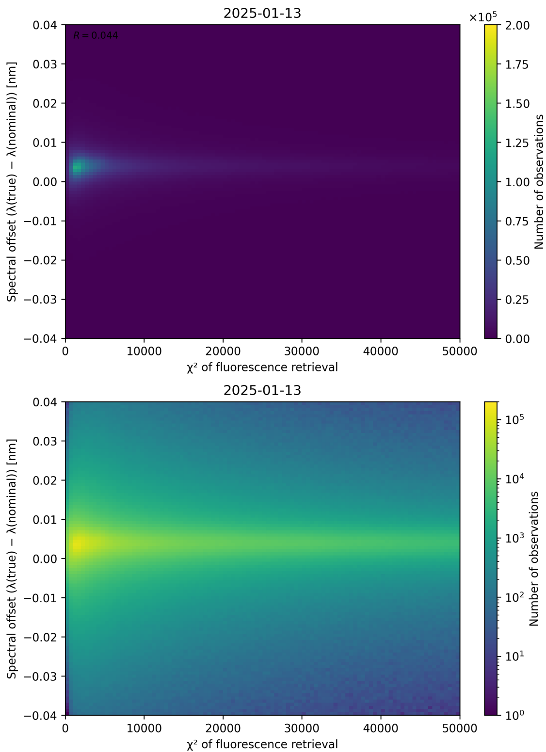
Figure 69: Scatter density plot of “ \chi^2 of fluorescence retrieval” against “Spectral offset ( \lambda_{\text{true}} - \lambda_{\text{nominal}} )” for 2025-01-12 to 2025-01-14.
