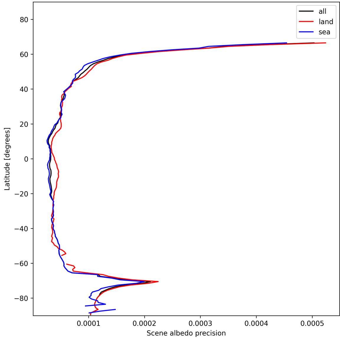
Figure 18: Zonal average of “Scene albedo precision” for 2025-01-12 to 2025-01-14.
