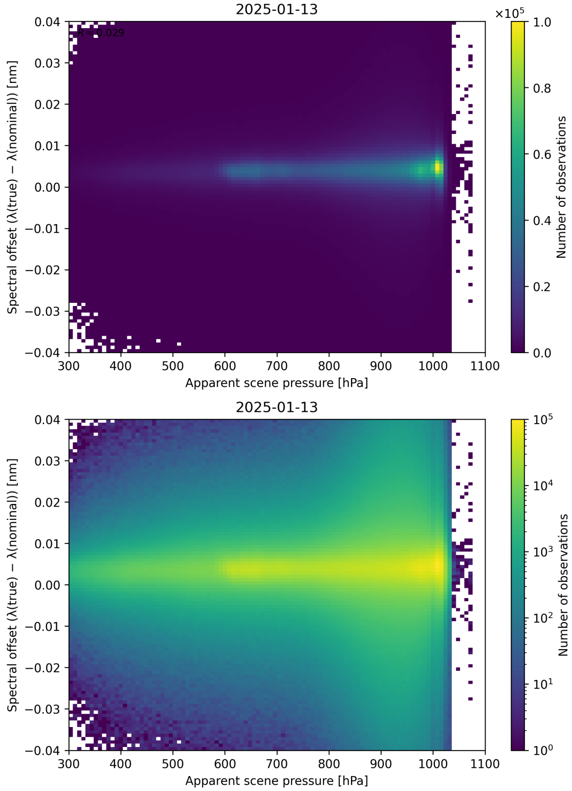
Figure 67: Scatter density plot of “Apparent scene pressure” against “Spectral offset ( \lambda_{\text{true}} - \lambda_{\text{nominal}} )” for 2025-01-12 to 2025-01-14.
