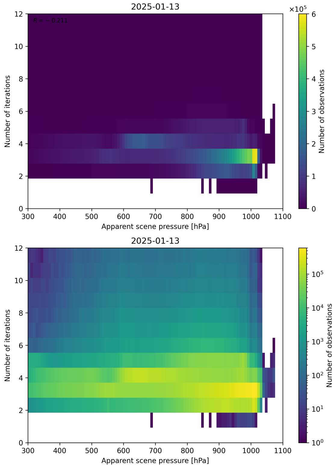
Figure 65: Scatter density plot of “Apparent scene pressure” against “Number of iterations” for 2025-01-12 to 2025-01-14.
