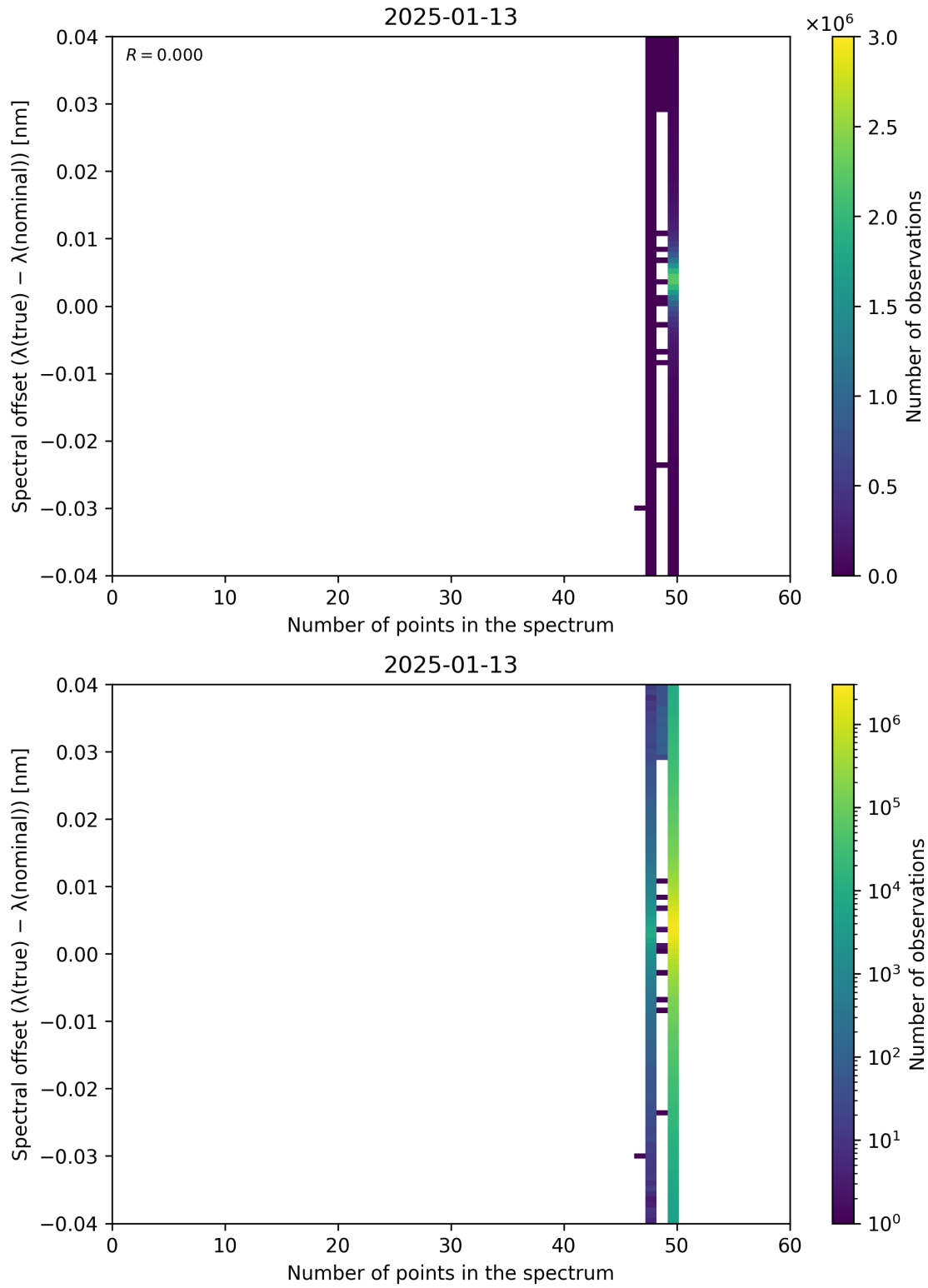
Figure 101: Scatter density plot of “Number of points in the spectrum” against “Spectral offset ( \lambda_{\text{true}} - \lambda_{\text{nominal}} )” for 2025-01-12 to 2025-01-14.
