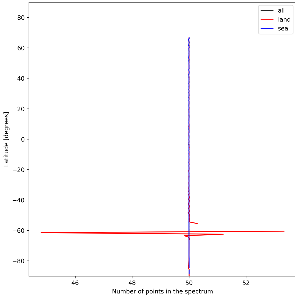
Figure 27: Zonal average of “Number of points in the spectrum” for 2025-01-12 to 2025-01-14.
