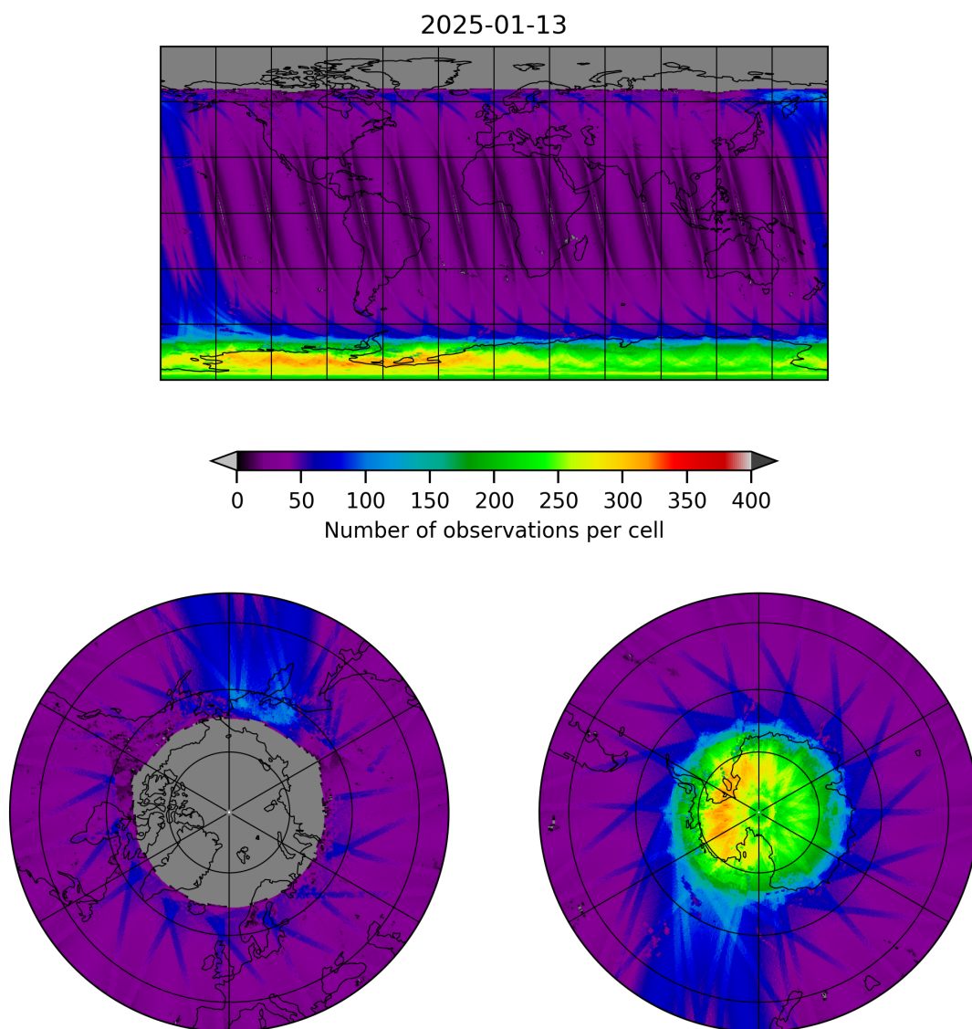
Figure 11: Map of the number of observations for 2025-01-12 to 2025-01-14
