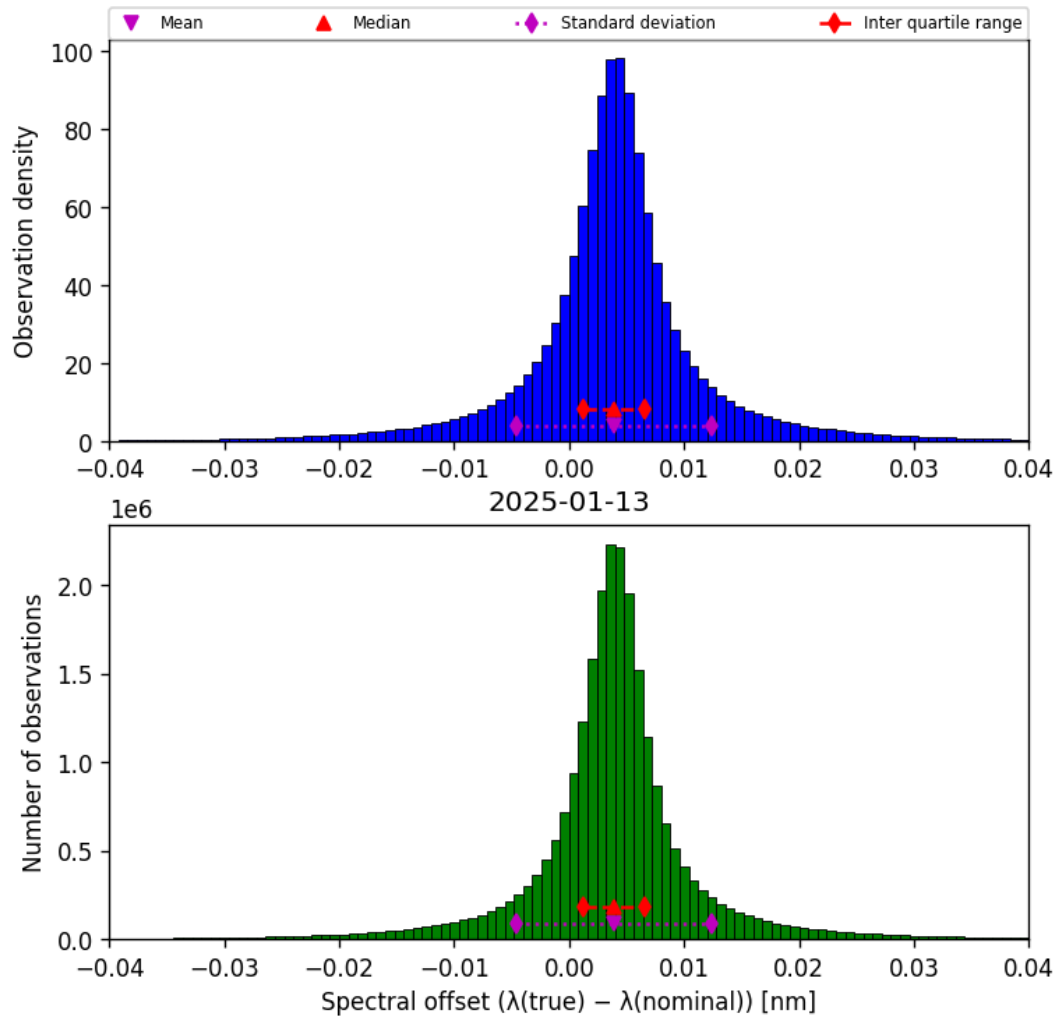
Figure 45: Histogram of “Spectral offset ( \lambda_{\text{true}} - \lambda_{\text{nominal}} )” for 2025-01-12 to 2025-01-14
