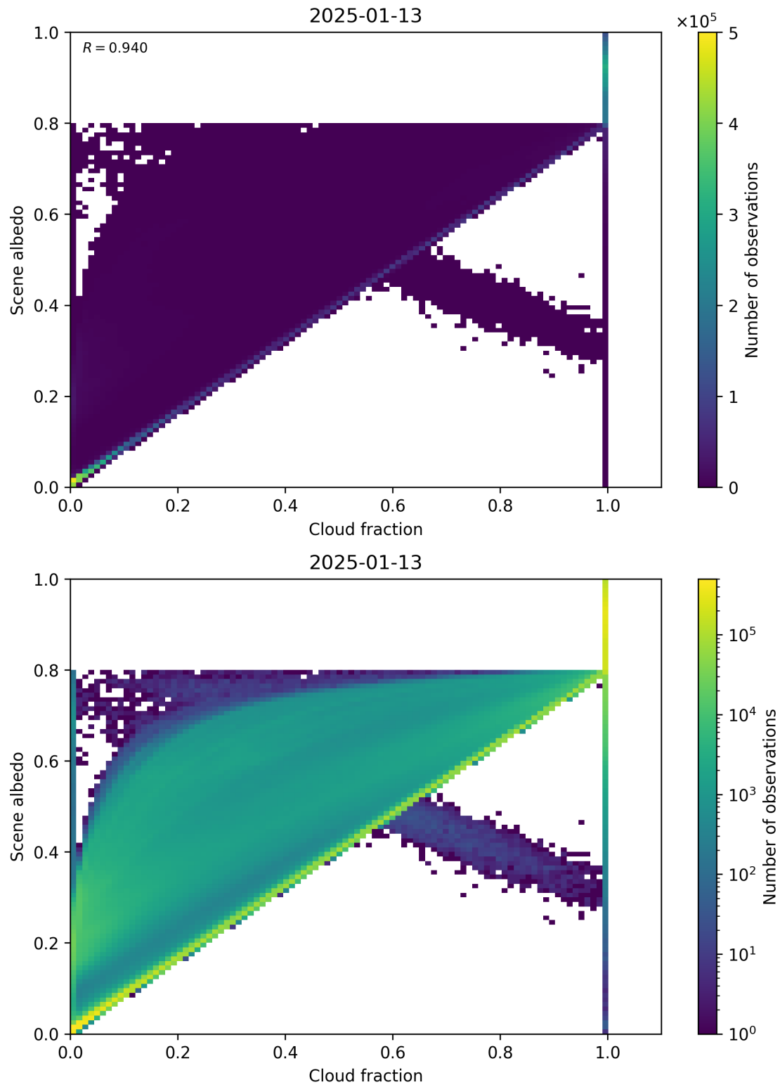
Figure 75: Scatter density plot of “Cloud fraction” against “Scene albedo” for 2025-01-12 to 2025-01-14.
