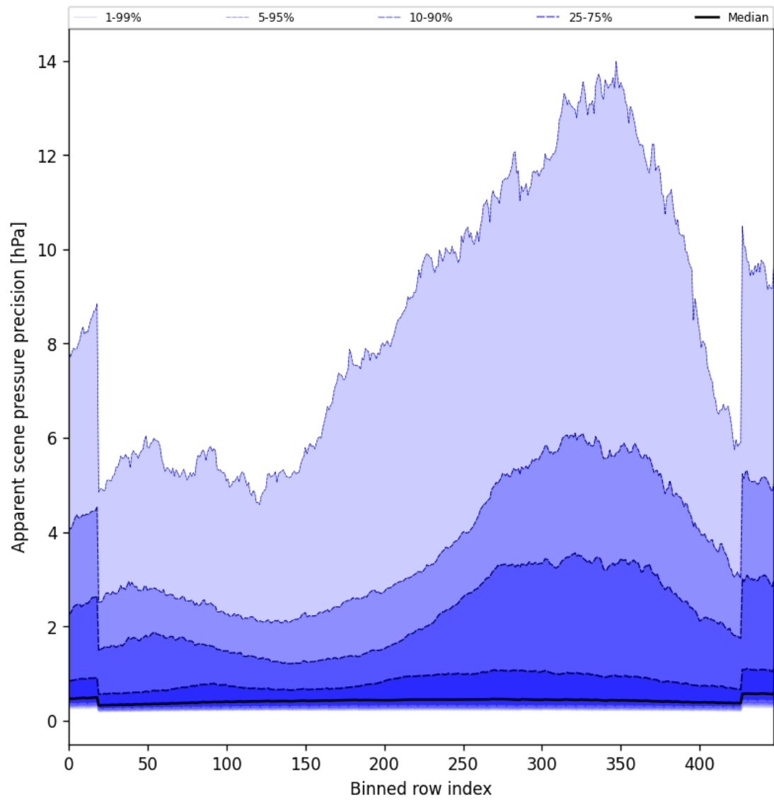
Figure 54: Along track statistics of “Apparent scene pressure precision” for 2025-01-12 to 2025-01-14
