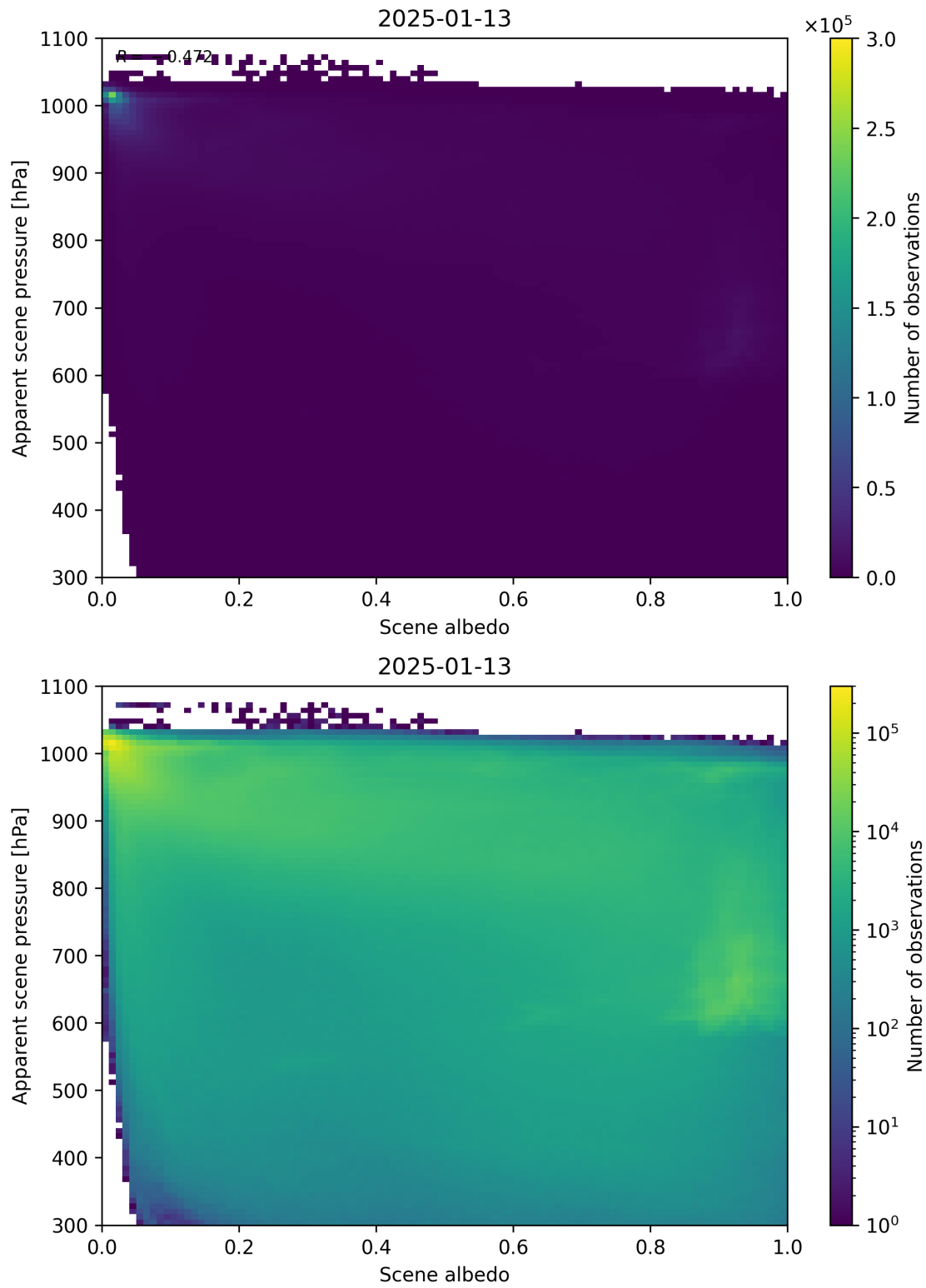
Figure 102: Scatter density plot of “Scene albedo” against “Apparent scene pressure” for 2025-01-12 to 2025-01-14.
