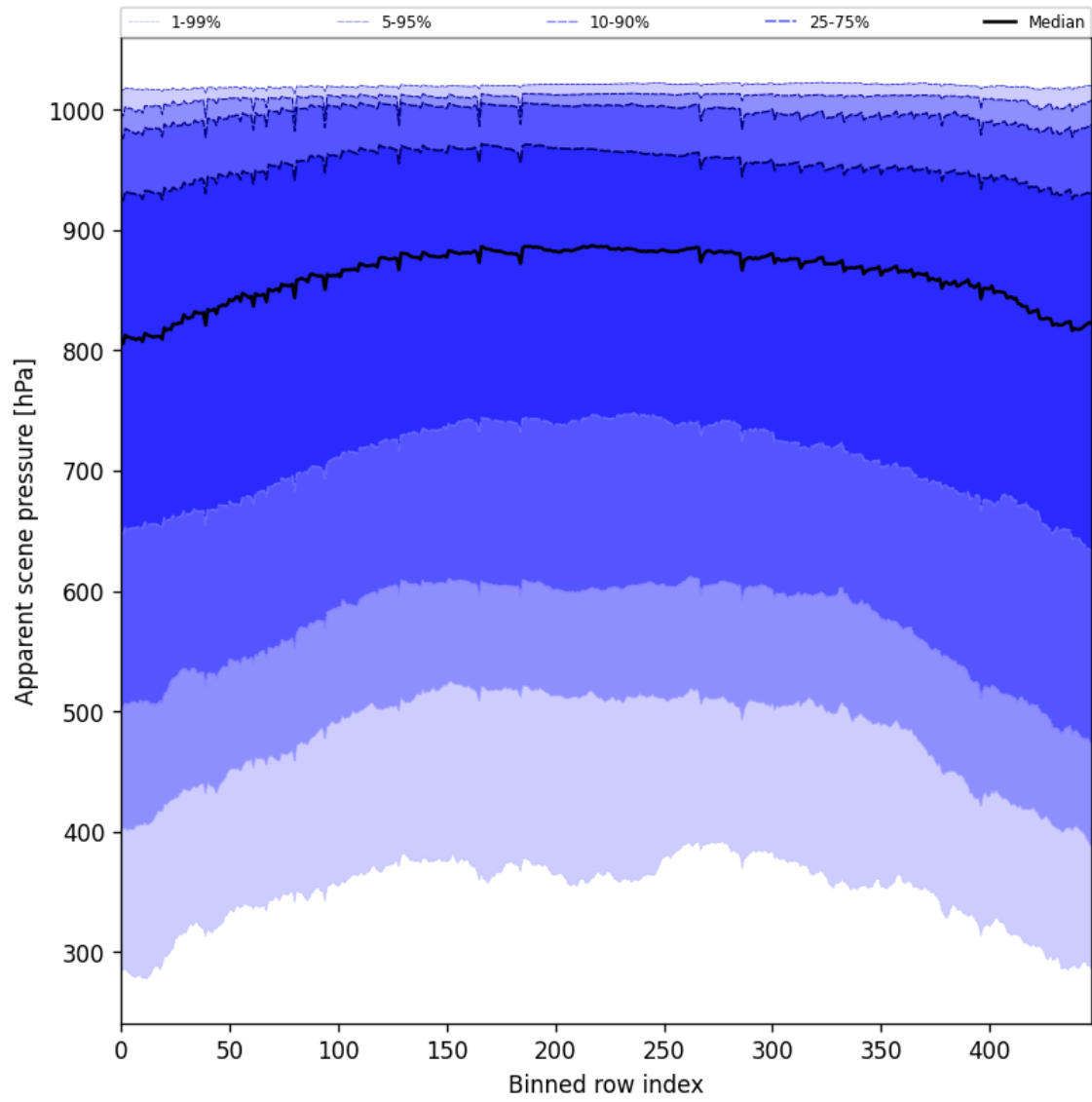
Figure 53: Along track statistics of “Apparent scene pressure” for 2025-01-12 to 2025-01-14
