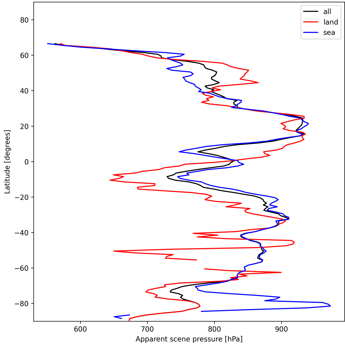
Figure 19: Zonal average of “Apparent scene pressure” for 2025-01-12 to 2025-01-14.
