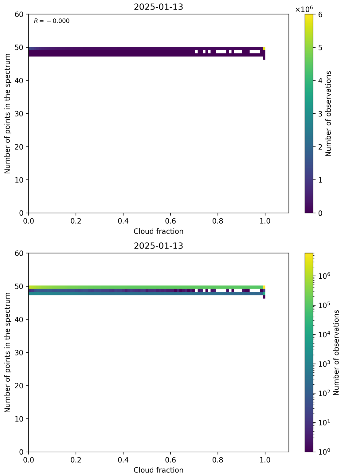
Figure 74: Scatter density plot of “Cloud fraction” against “Number of points in the spectrum” for 2025-01-12 to 2025-01-14.
