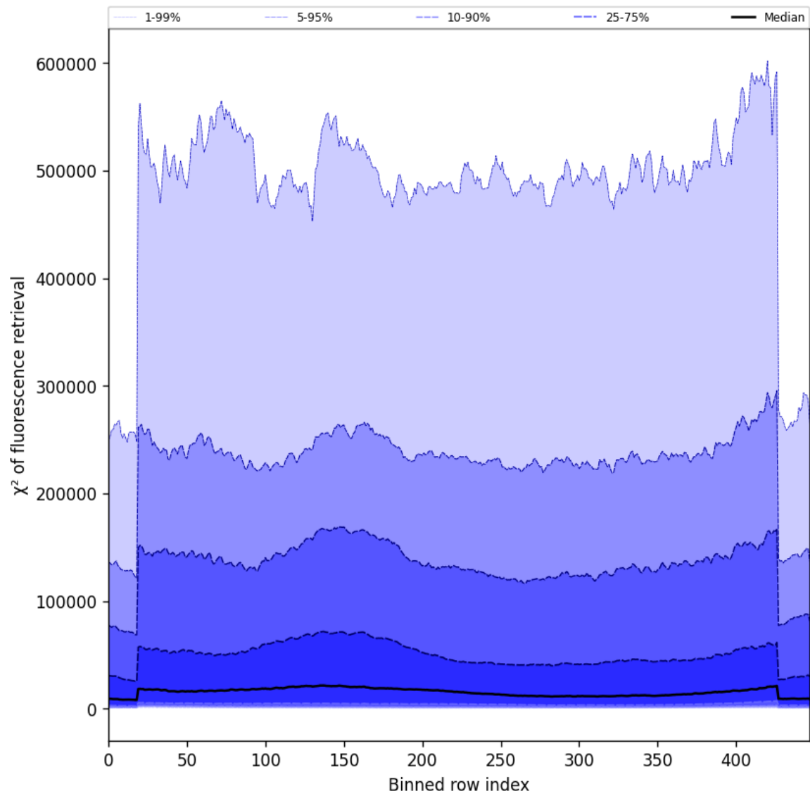
Figure 59: Along track statistics of “ \chi^2 of fluorescence retrieval” for 2025-01-12 to 2025-01-14
