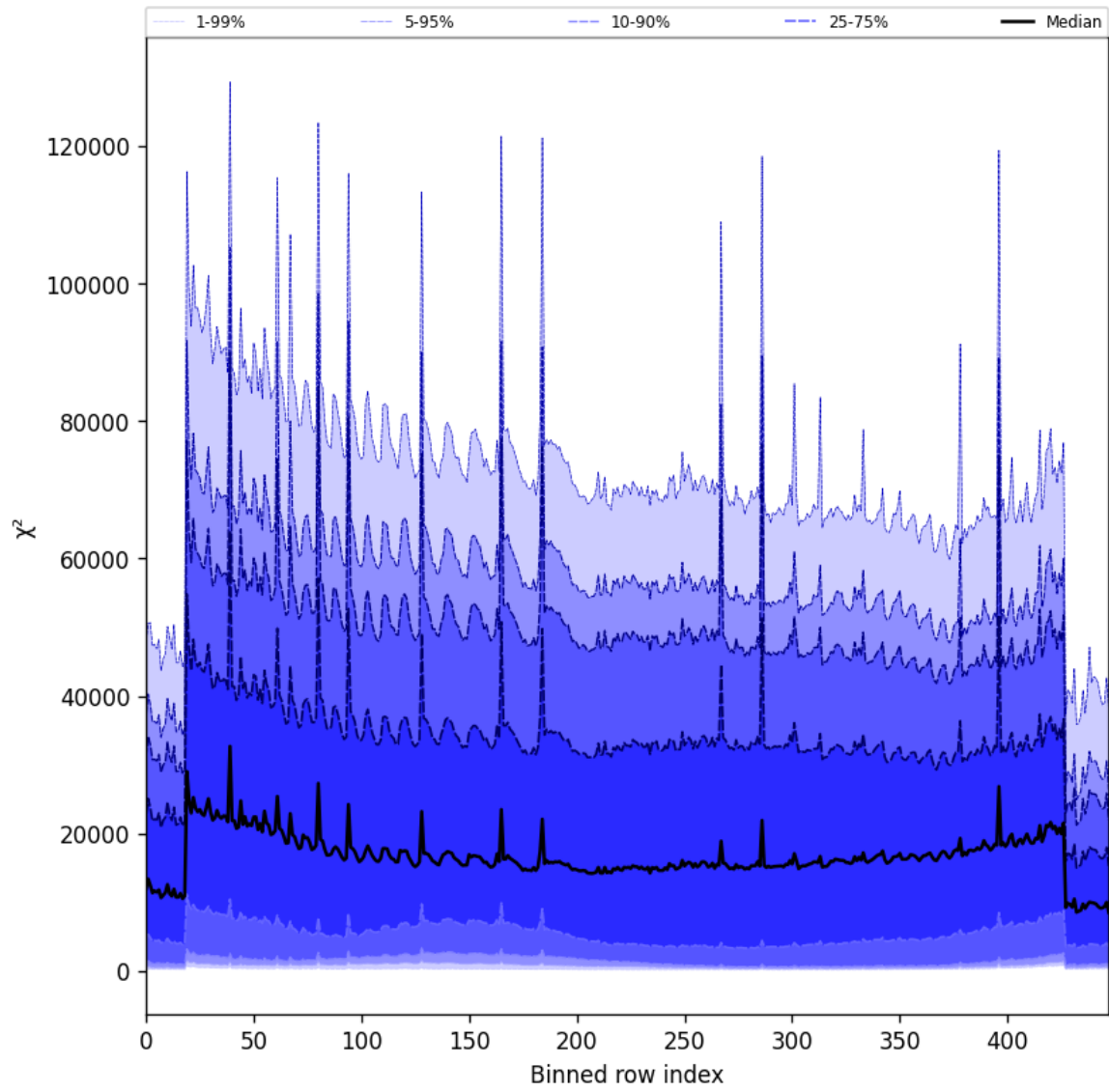
Figure 55: Along track statistics of “ \chi^2 ” for 2025-01-12 to 2025-01-14
