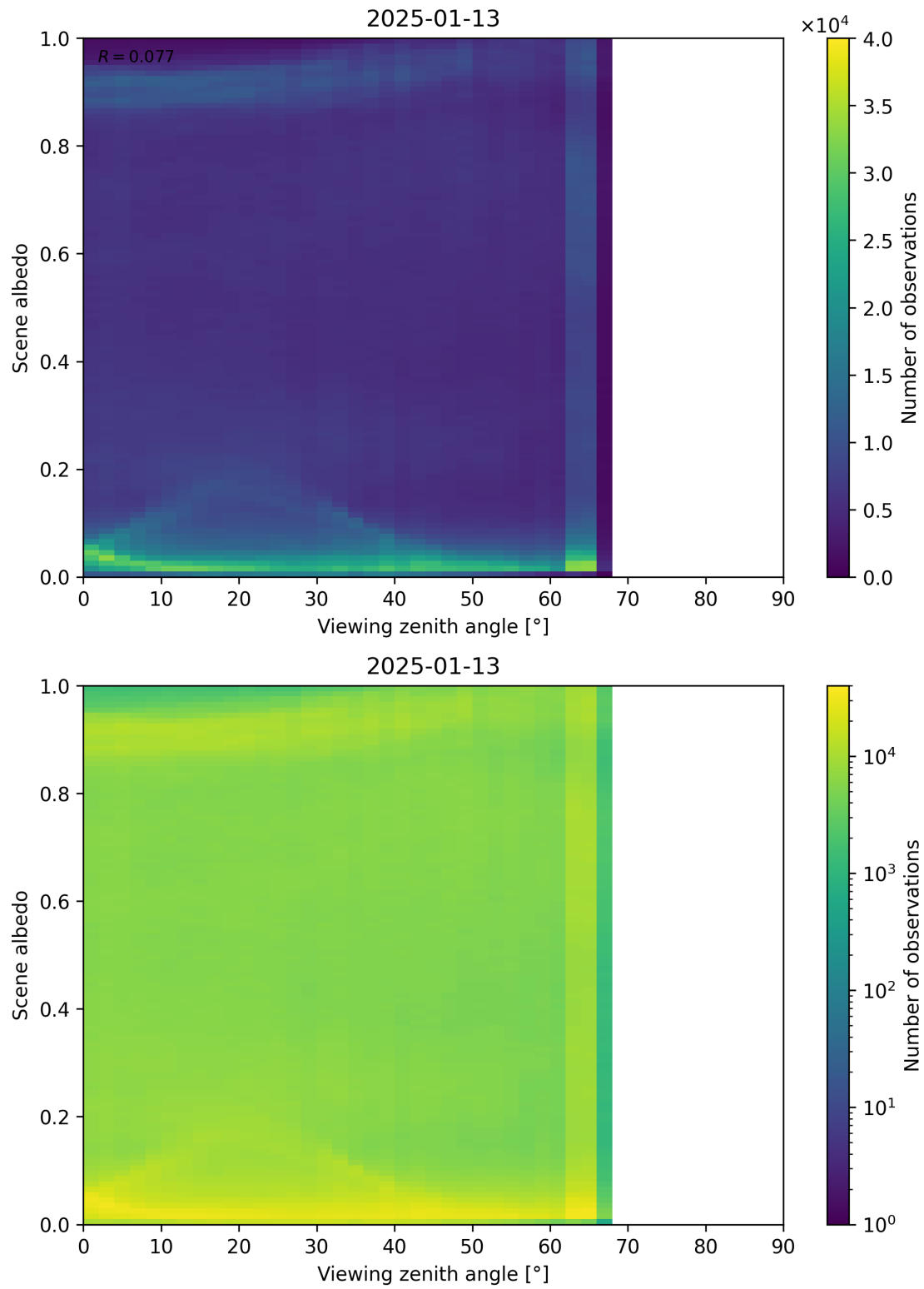
Figure 126: Scatter density plot of “Viewing zenith angle” against “Scene albedo” for 2025-01-12 to 2025-01-14.
