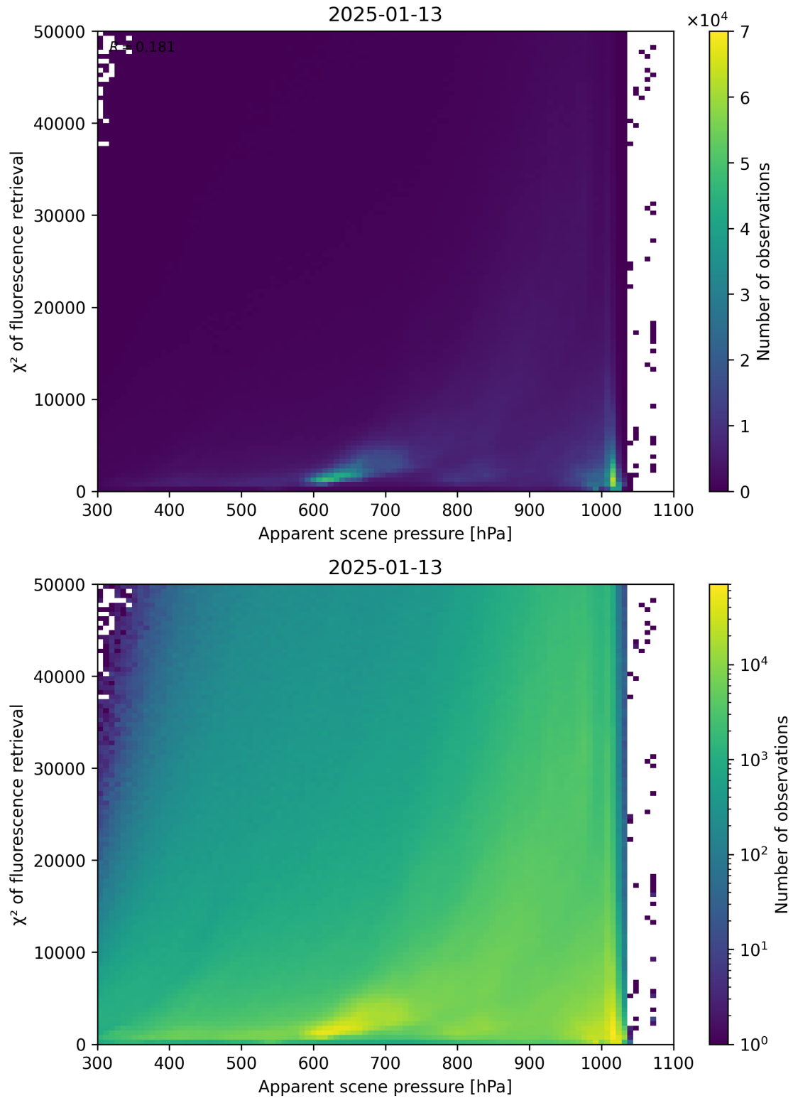
Figure 63: Scatter density plot of “Apparent scene pressure” against “ \chi^2 of fluorescence retrieval” for 2025-01-12 to 2025-01-14.
