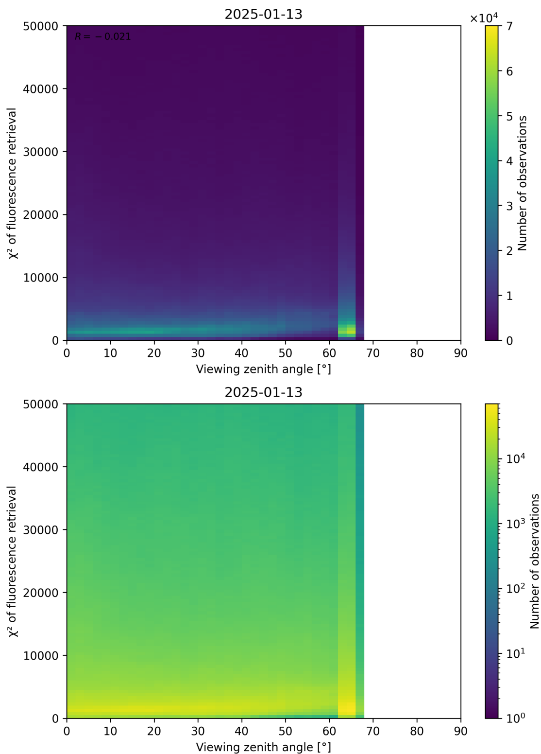
Figure 119: Scatter density plot of “Viewing zenith angle” against “ \chi^2 of fluorescence retrieval” for 2025-01-12 to 2025-01-14.
