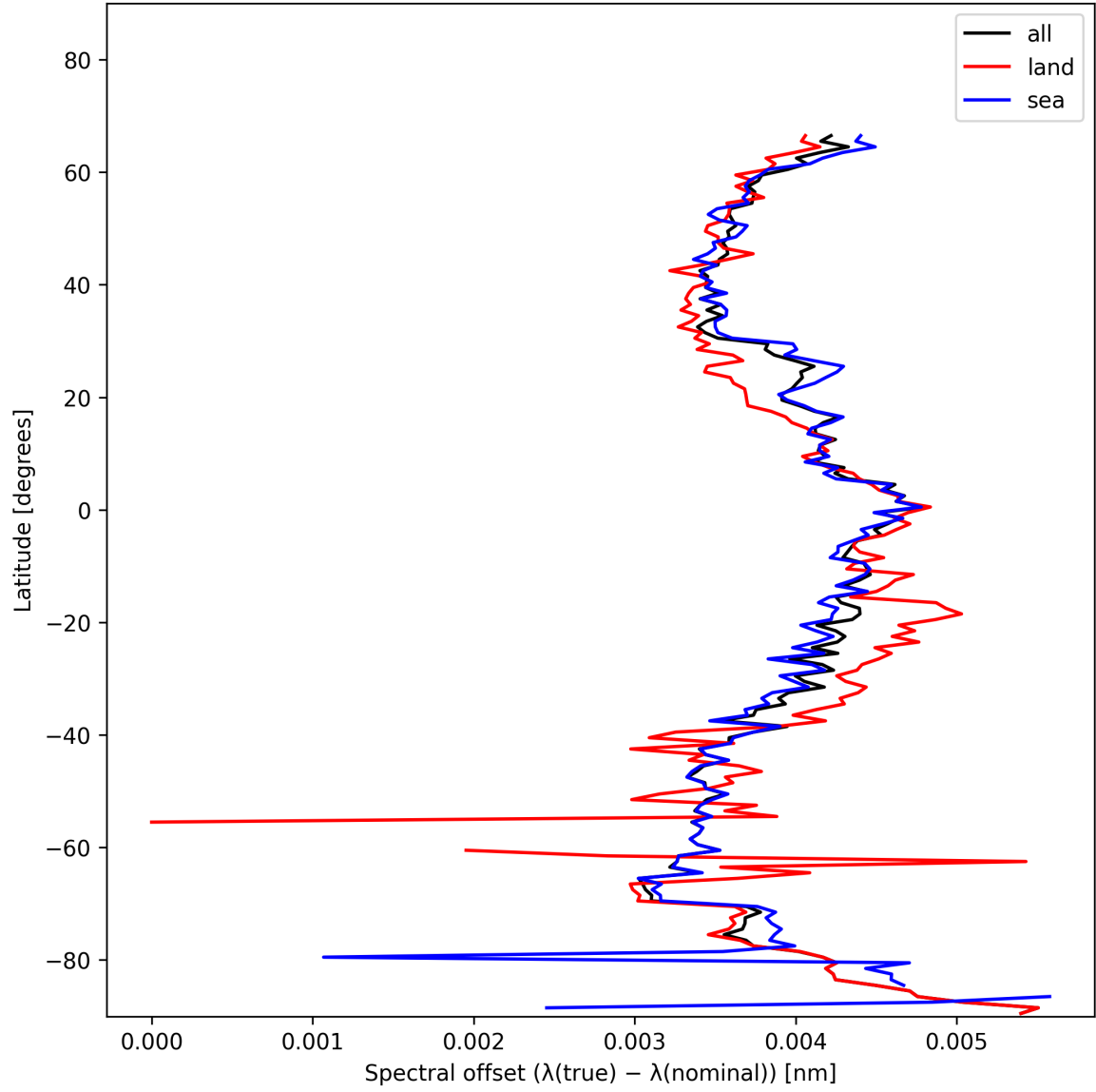
Figure 28: Zonal average of “Spectral offset ( \lambda_{\text{true}} - \lambda_{\text{nominal}} )” for 2025-01-12 to 2025-01-14.
