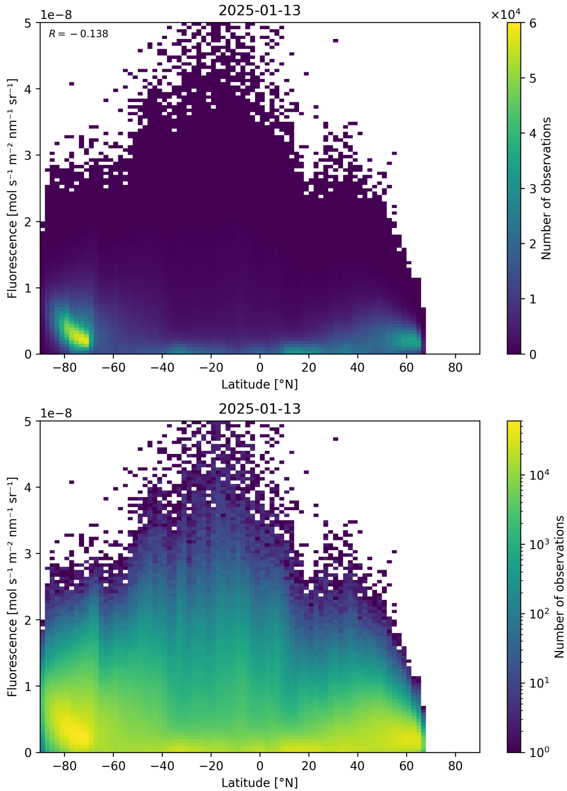
Figure 92: Scatter density plot of “Latitude” against “Fluorescence” for 2025-01-12 to 2025-01-14.
