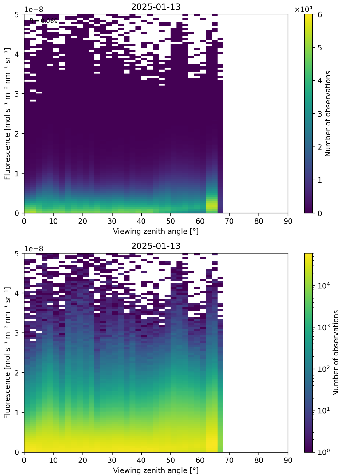
Figure 122: Scatter density plot of “Viewing zenith angle” against “Fluorescence” for 2025-01-12 to 2025-01-14.
