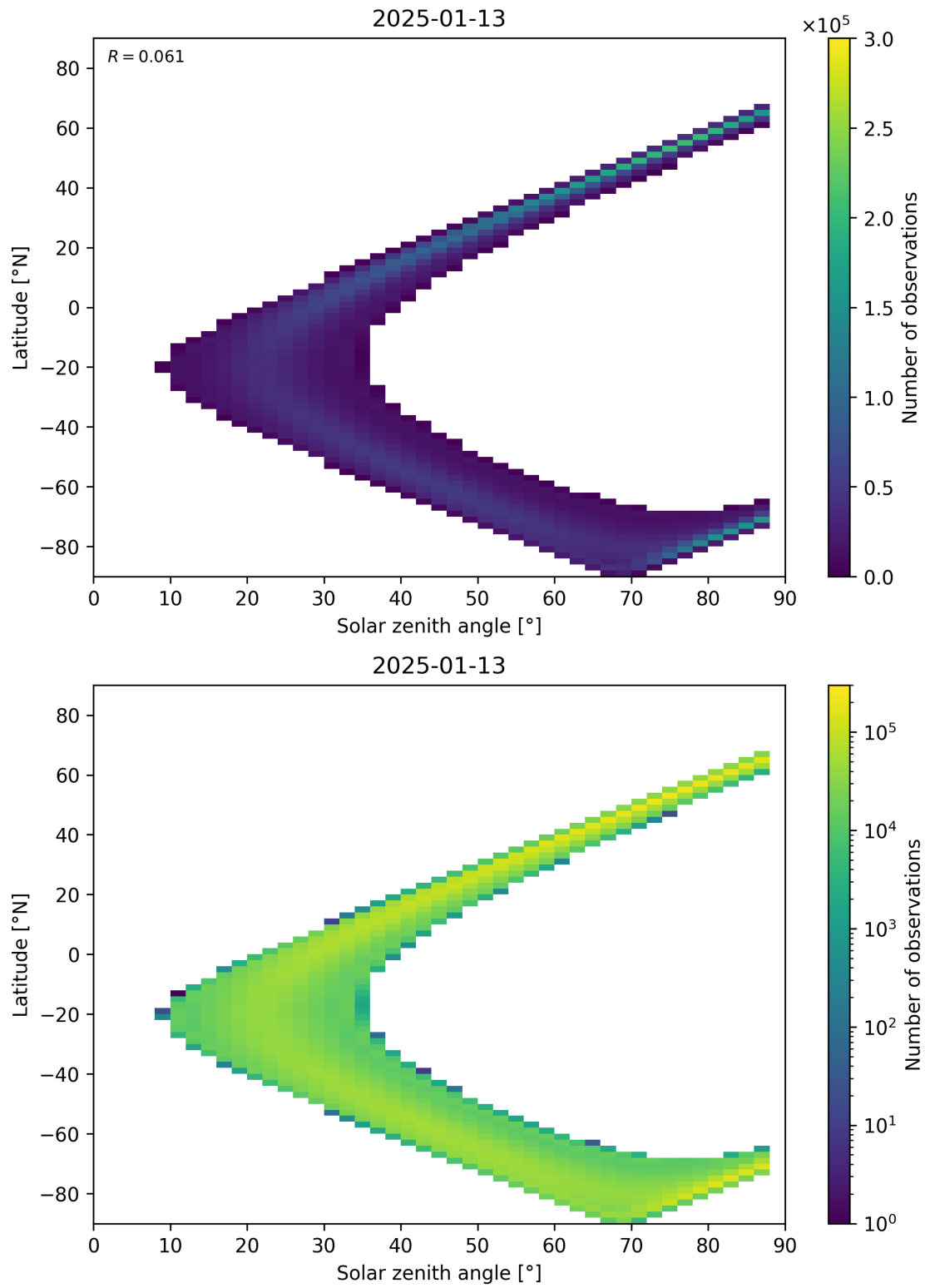
Figure 113: Scatter density plot of “Solar zenith angle” against “Latitude” for 2025-01-12 to 2025-01-14.
