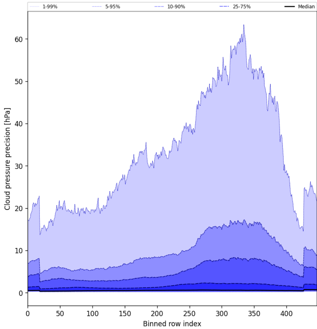
Figure 48: Along track statistics of “Cloud pressure precision” for 2025-01-12 to 2025-01-14
