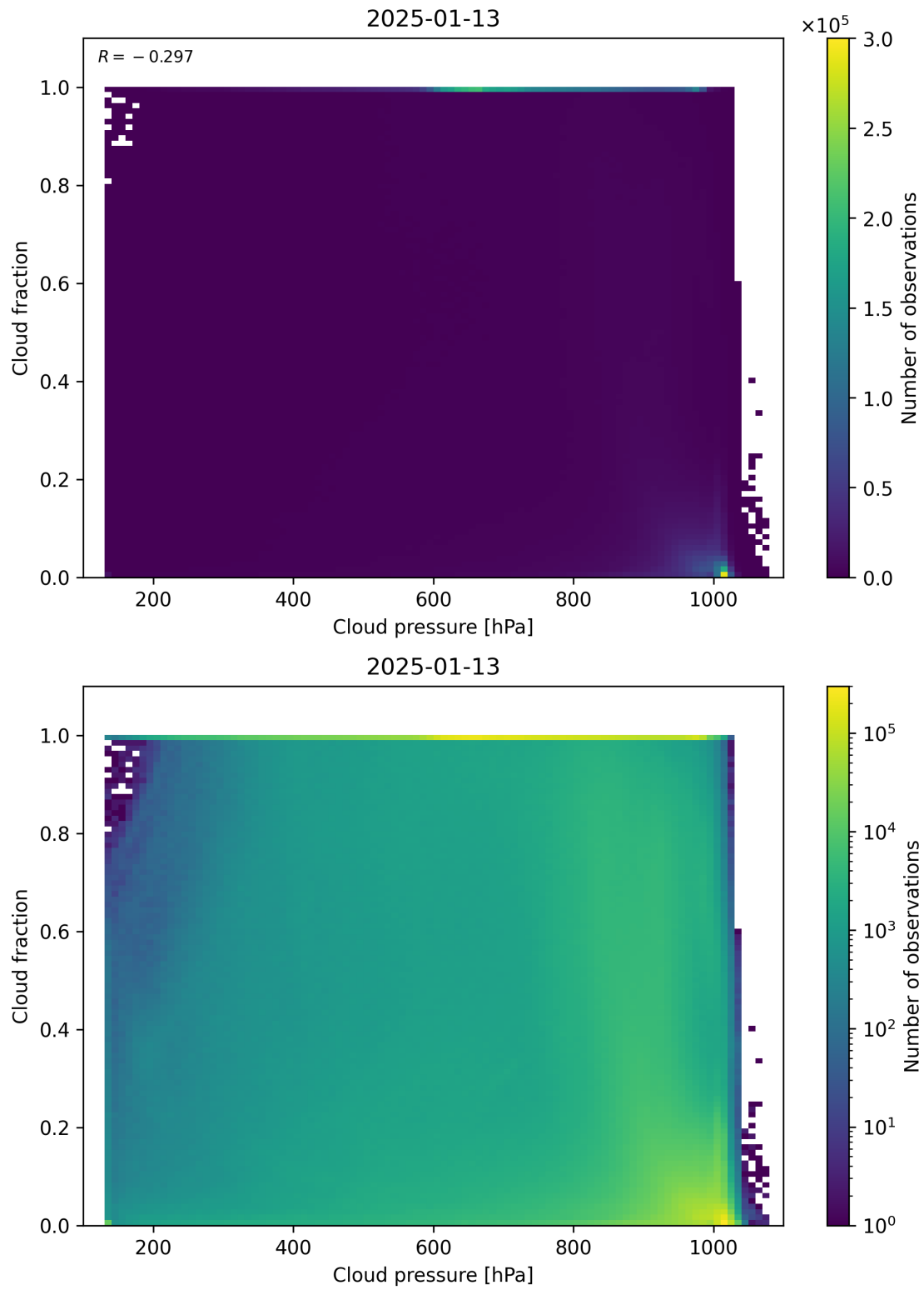
Figure 79: Scatter density plot of “Cloud pressure” against “Cloud fraction” for 2025-01-12 to 2025-01-14.
