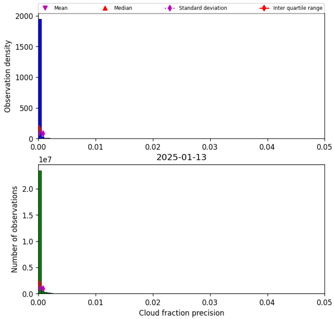
Figure 33: Histogram of “Cloud fraction precision” for 2025-01-12 to 2025-01-14
