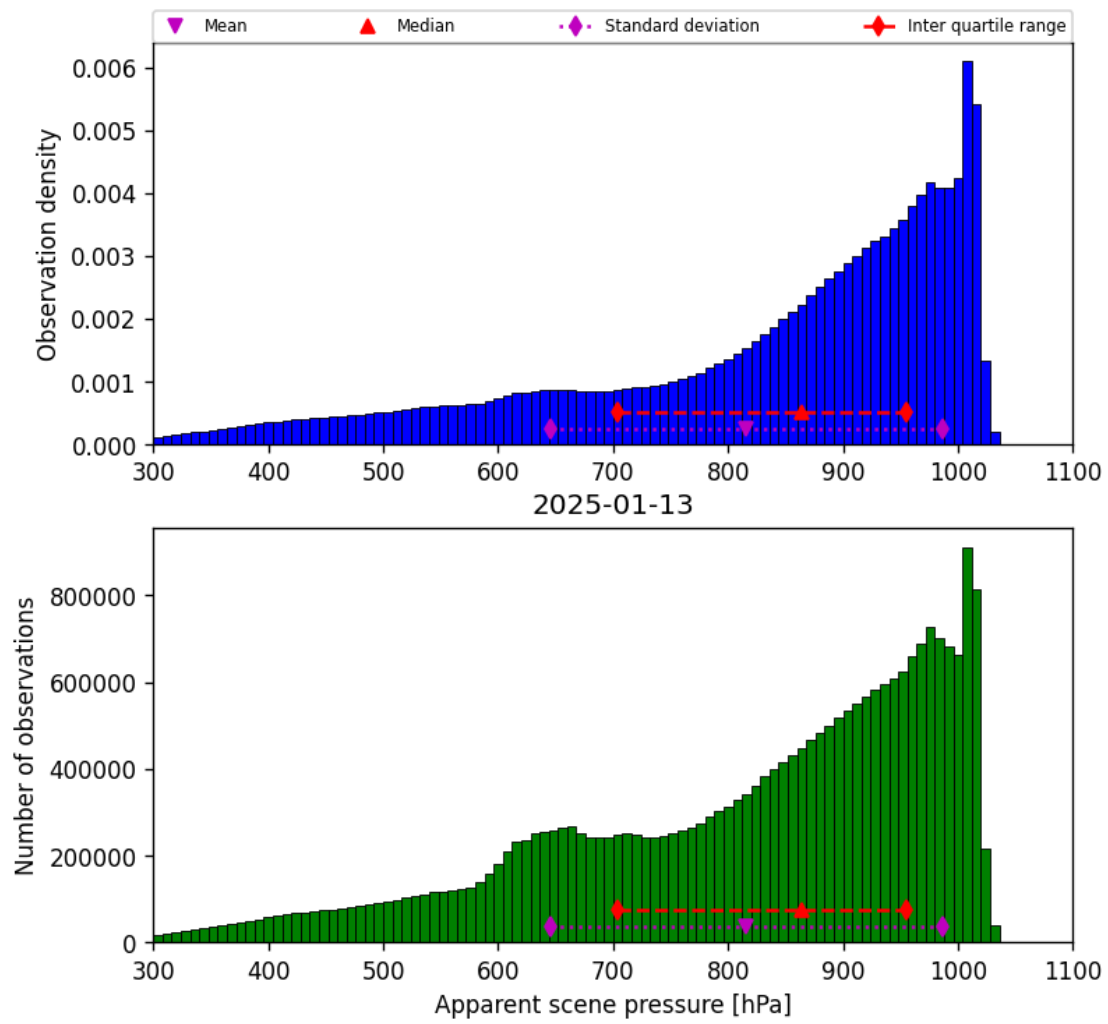
Figure 36: Histogram of "Apparent scene pressure" for 2025-01-12 to 2025-01-14
