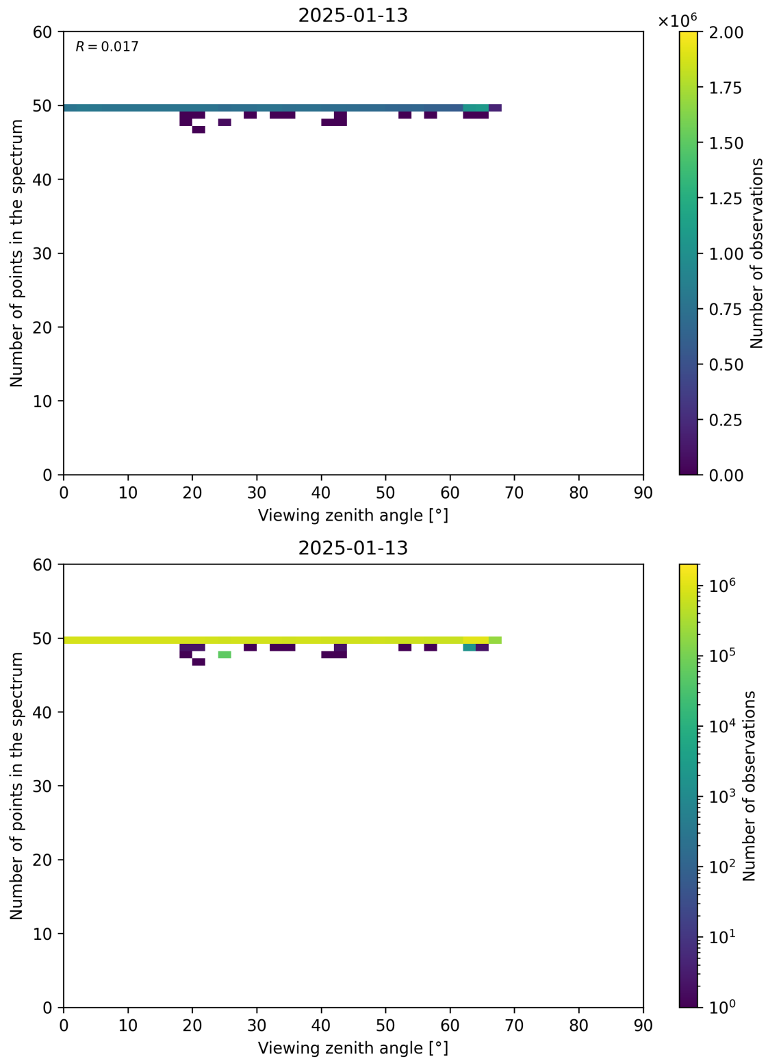
Figure 125: Scatter density plot of “Viewing zenith angle” against “Number of points in the spectrum” for 2025-01-12 to 2025-01-14.
