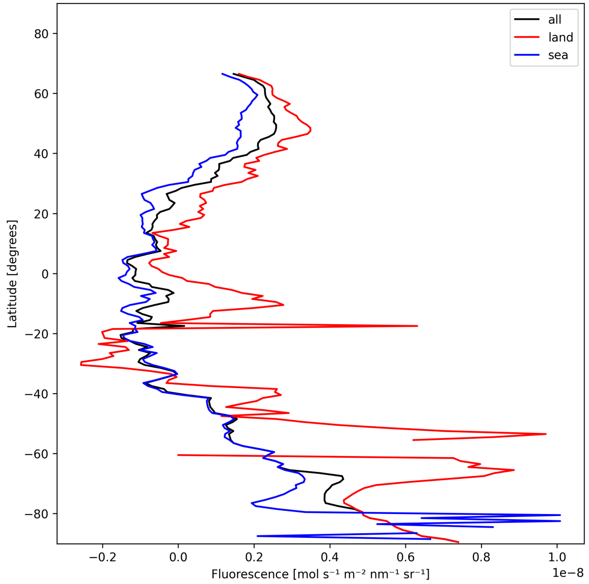
Figure 23: Zonal average of “Fluorescence” for 2025-01-12 to 2025-01-14.
