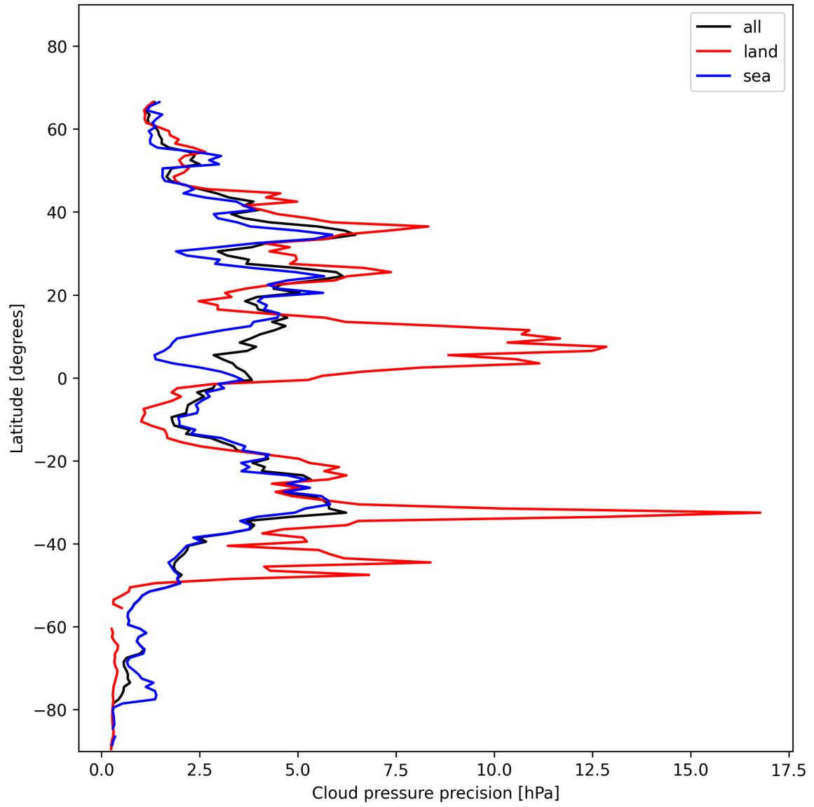
Figure 14: Zonal average of “Cloud pressure precision” for 2025-01-12 to 2025-01-14.
