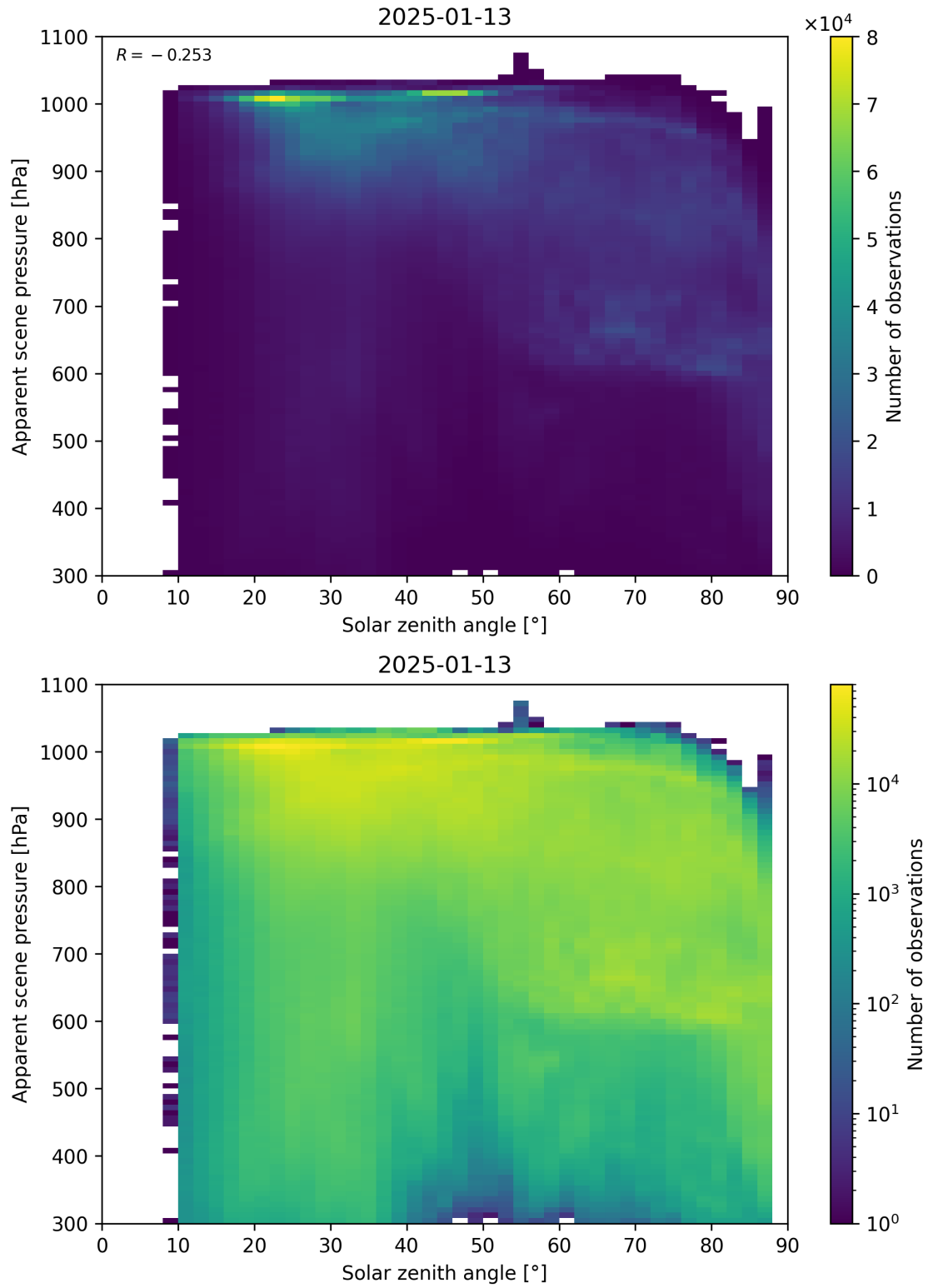
Figure 108: Scatter density plot of “Solar zenith angle” against “Apparent scene pressure” for 2025-01-12 to 2025-01-14.
