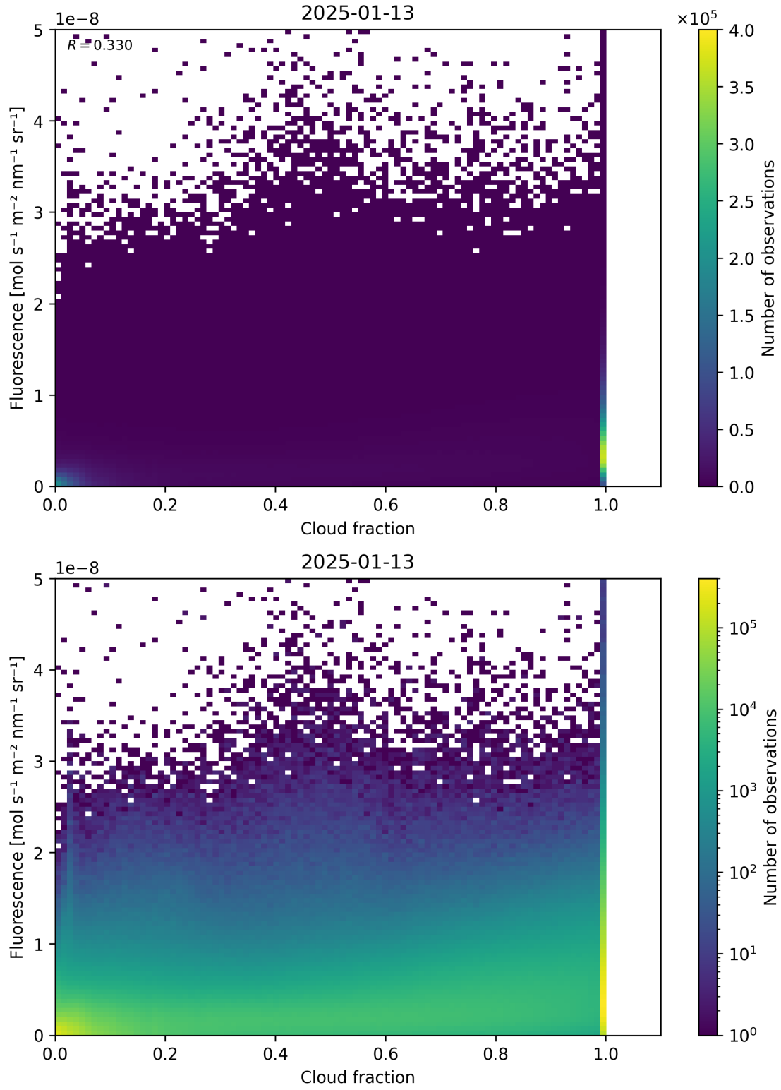
Figure 72: Scatter density plot of “Cloud fraction” against “Fluorescence” for 2025-01-12 to 2025-01-14.
