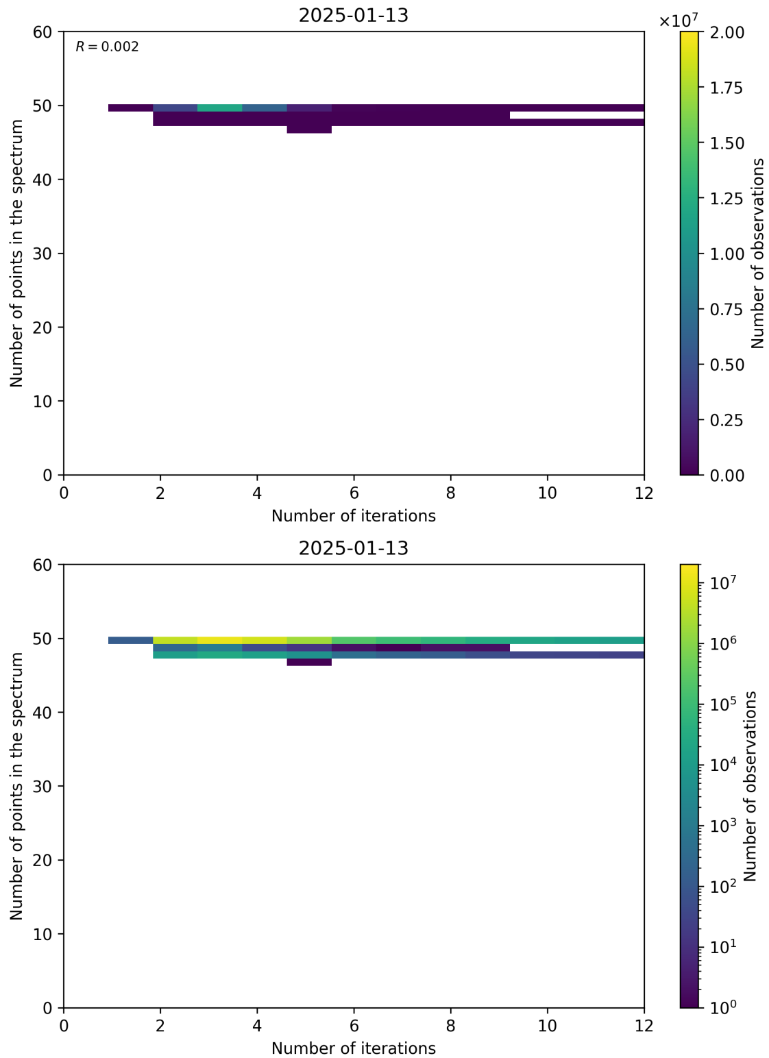
Figure 99: Scatter density plot of “Number of iterations” against “Number of points in the spectrum” for 2025-01-12 to 2025-01-14.
