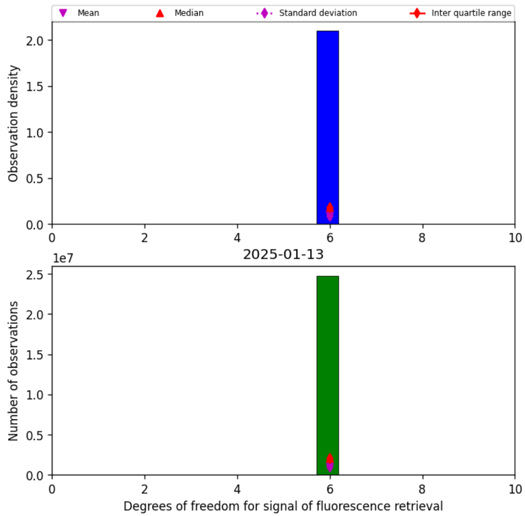
Figure 43: Histogram of “Degrees of freedom for signal of fluorescence retrieval” for 2025-01-12 to 2025-01-14
