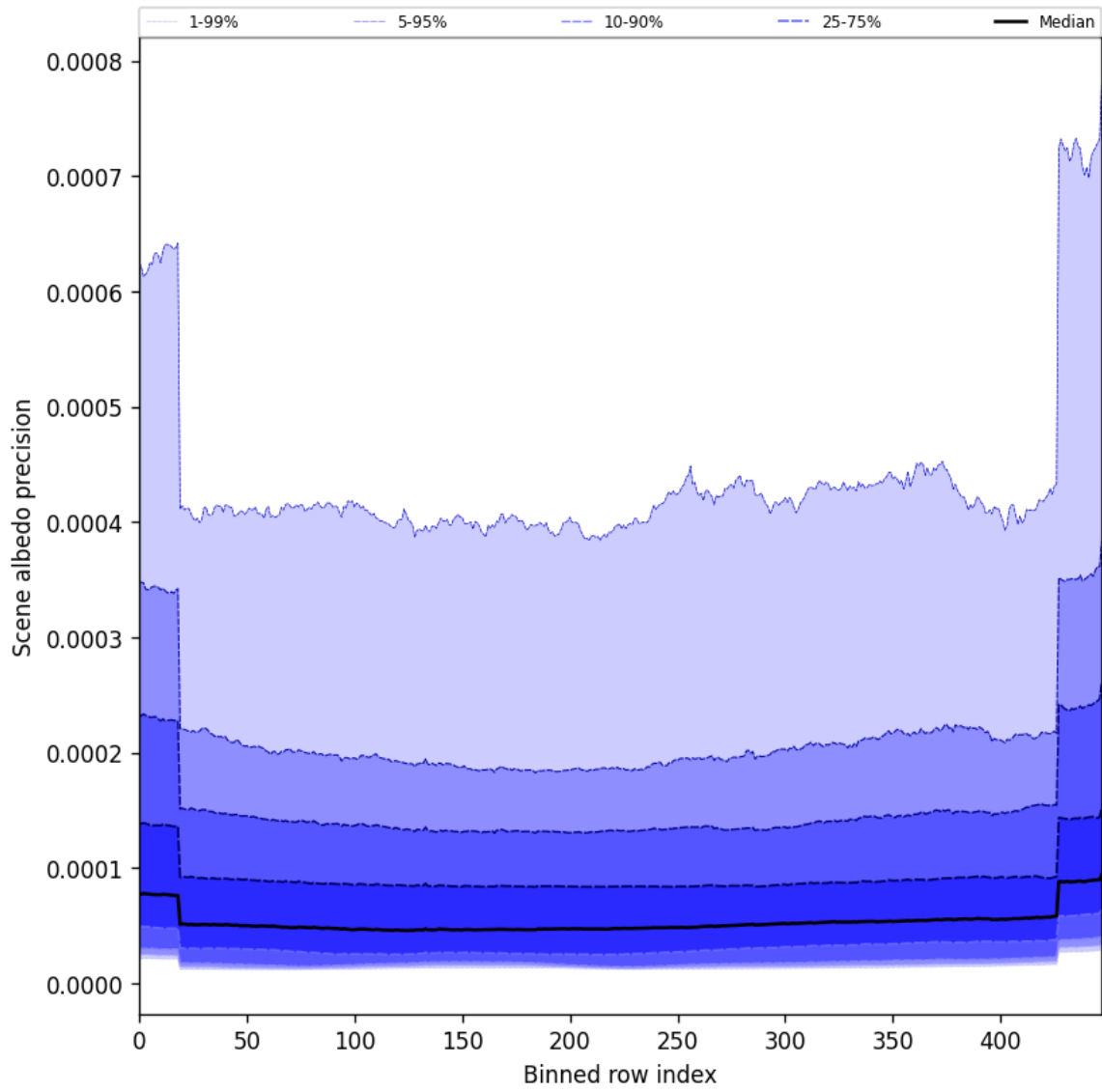
Figure 52: Along track statistics of “Scene albedo precision” for 2025-01-12 to 2025-01-14
