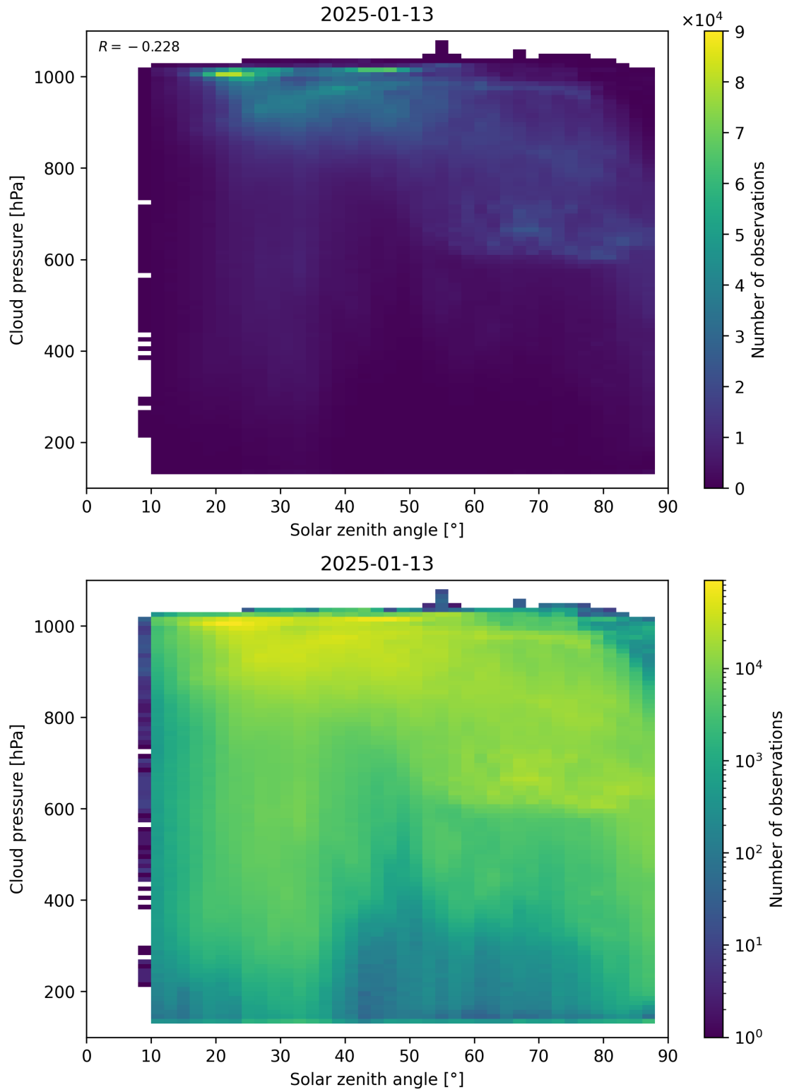
Figure 111: Scatter density plot of “Solar zenith angle” against “Cloud pressure” for 2025-01-12 to 2025-01-14.
