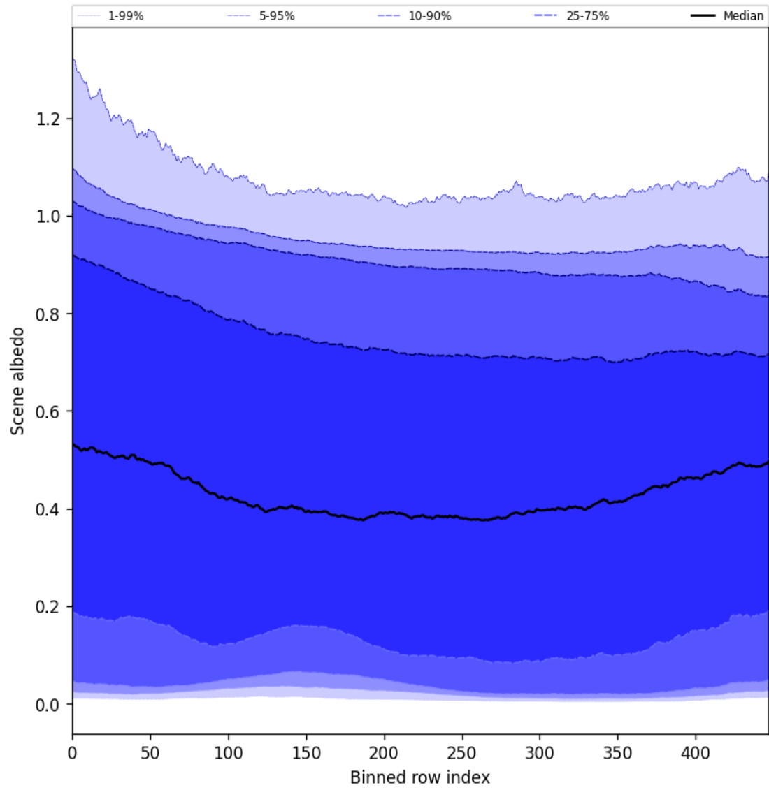
Figure 51: Along track statistics of “Scene albedo” for 2025-01-12 to 2025-01-14
