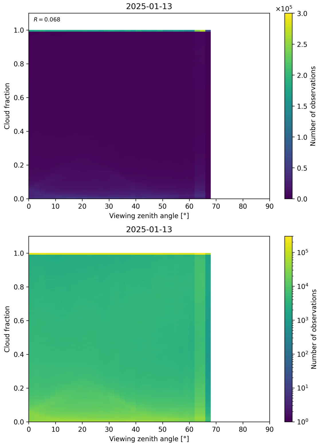
Figure 120: Scatter density plot of “Viewing zenith angle” against “Cloud fraction” for 2025-01-12 to 2025-01-14.
