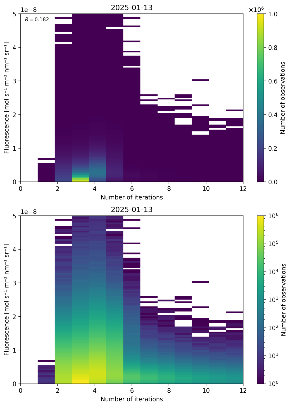
Figure 98: Scatter density plot of “Number of iterations” against “Fluorescence” for 2025-01-12 to 2025-01-14.
