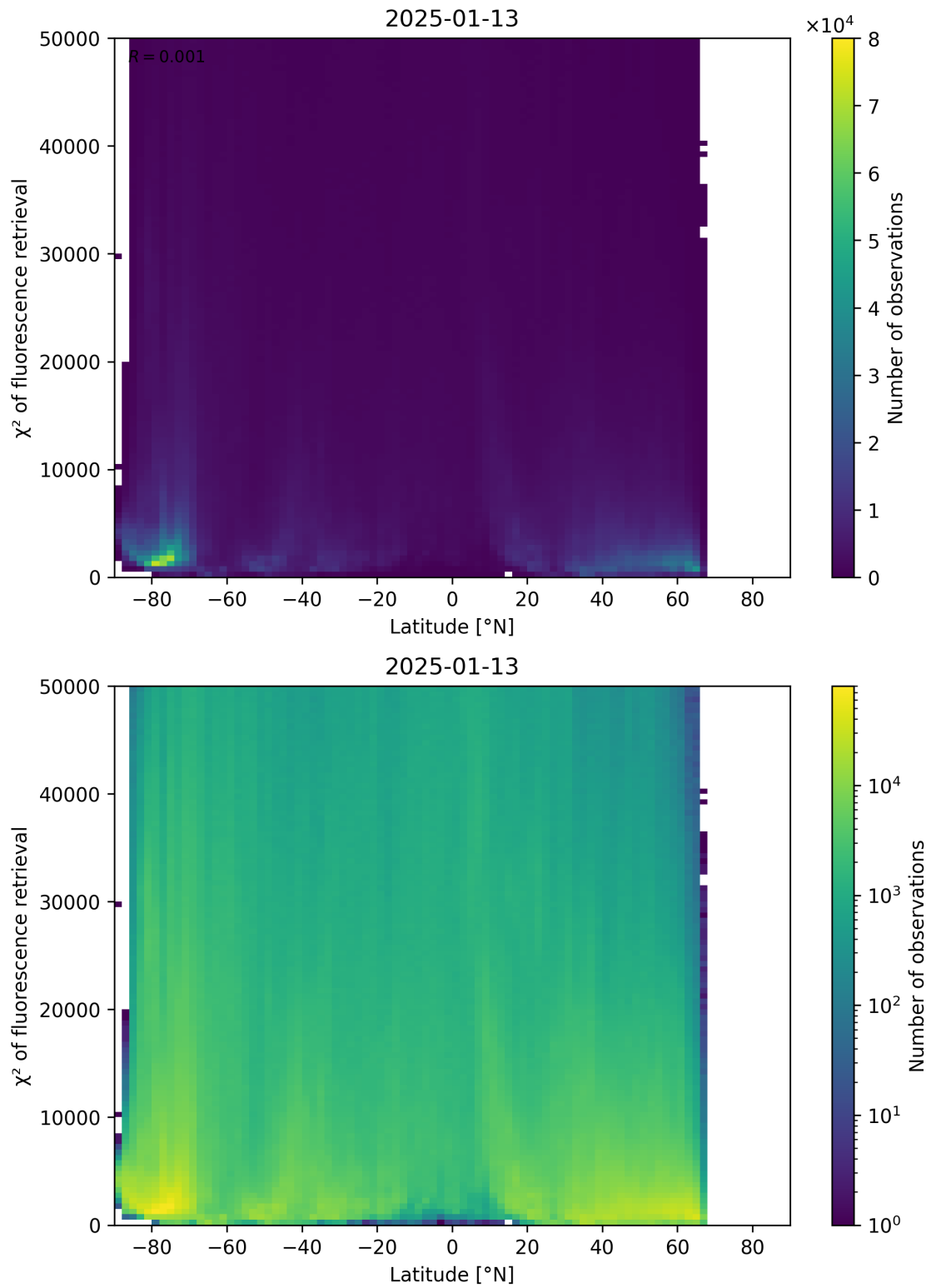
Figure 89: Scatter density plot of “Latitude” against “ \chi^2 of fluorescence retrieval” for 2025-01-12 to 2025-01-14.
