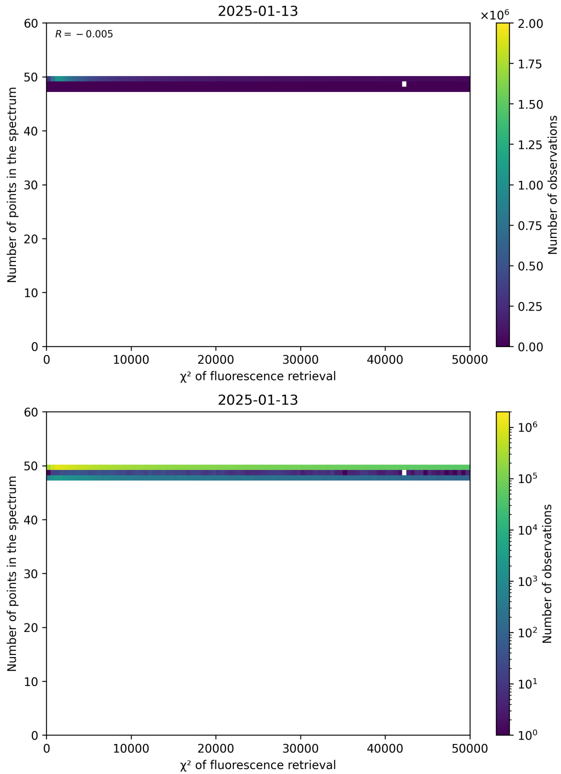
Figure 68: Scatter density plot of " \chi^2 of fluorescence retrieval" against "Number of points in the spectrum" for 2025-01-12 to 2025-01-14.
