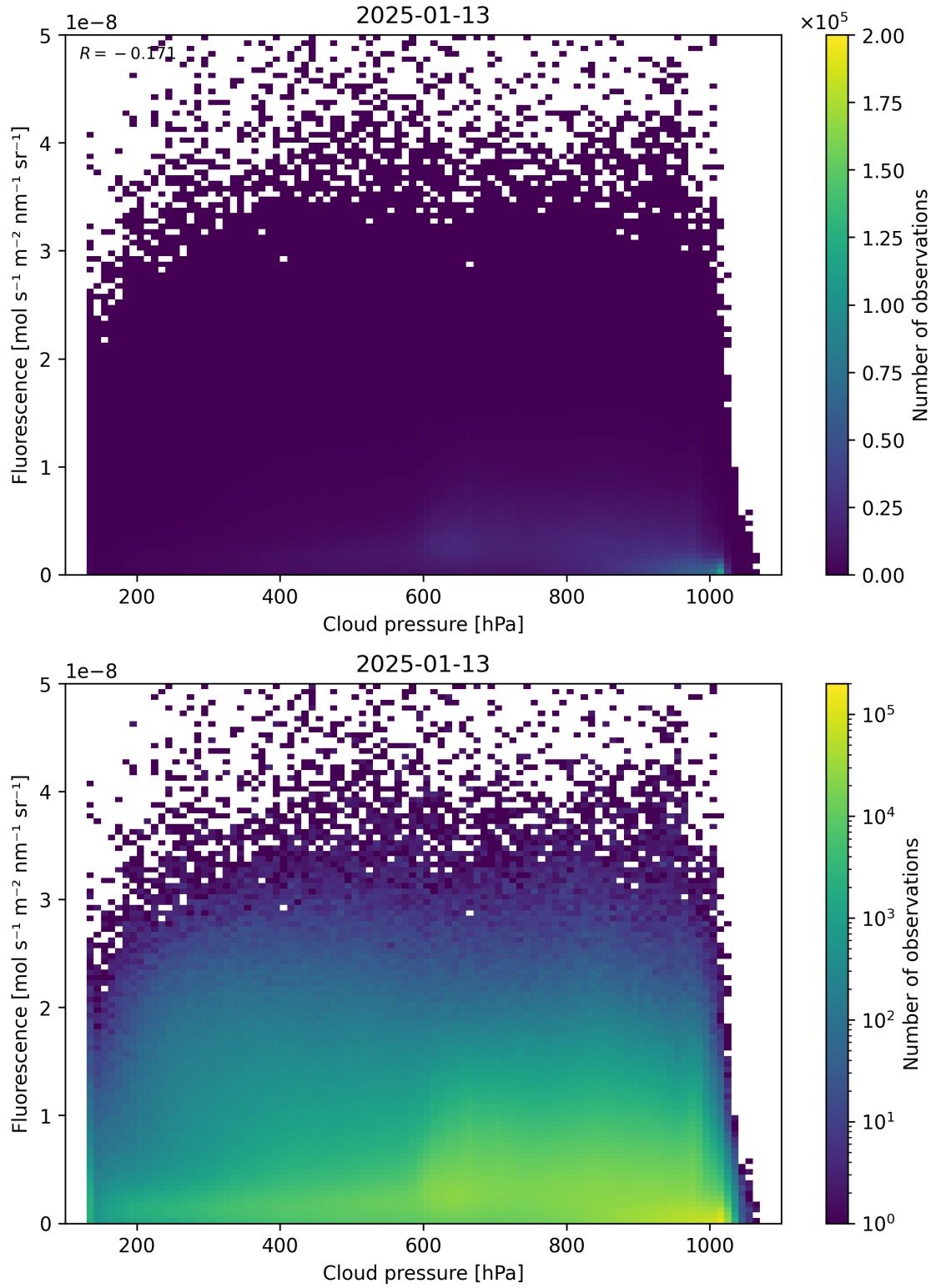
Figure 80: Scatter density plot of “Cloud pressure” against “Fluorescence” for 2025-01-12 to 2025-01-14.
