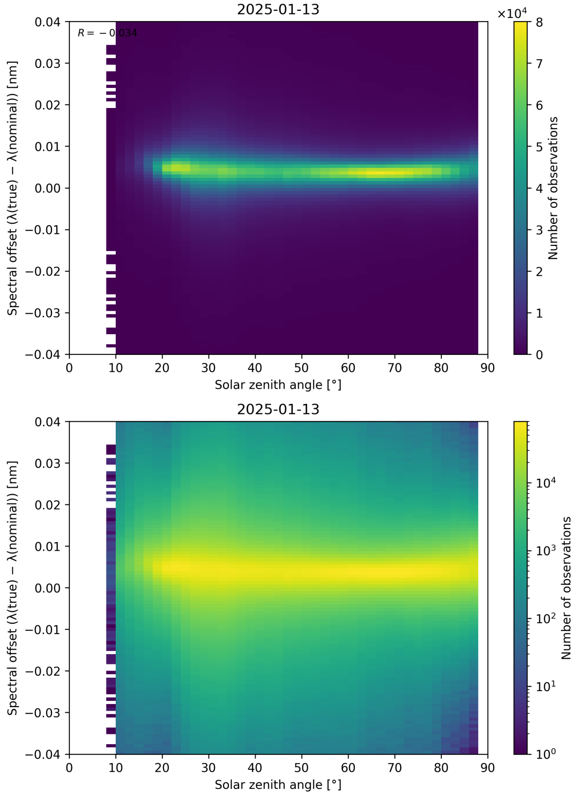
Figure 117: Scatter density plot of “Solar zenith angle” against “Spectral offset ( \lambda_{\text{true}} - \lambda_{\text{nominal}} )” for 2025-01-12 to 2025-01-14.
