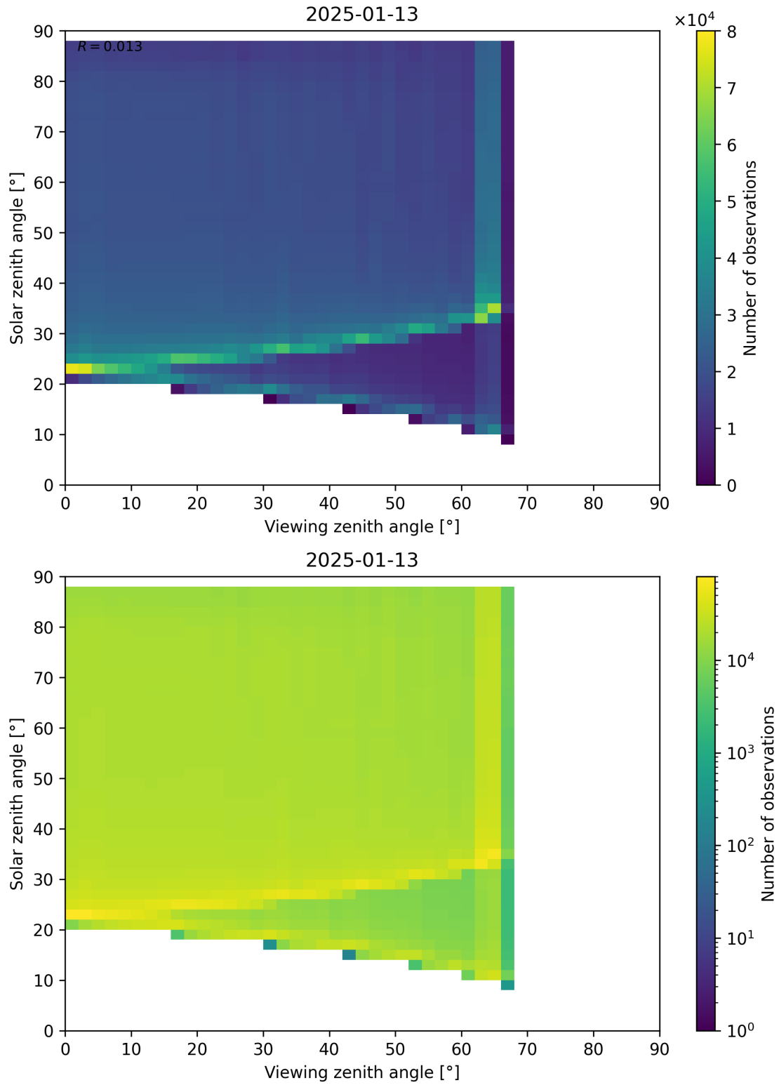
Figure 127: Scatter density plot of “Viewing zenith angle” against “Solar zenith angle” for 2025-01-12 to 2025-01-14.
