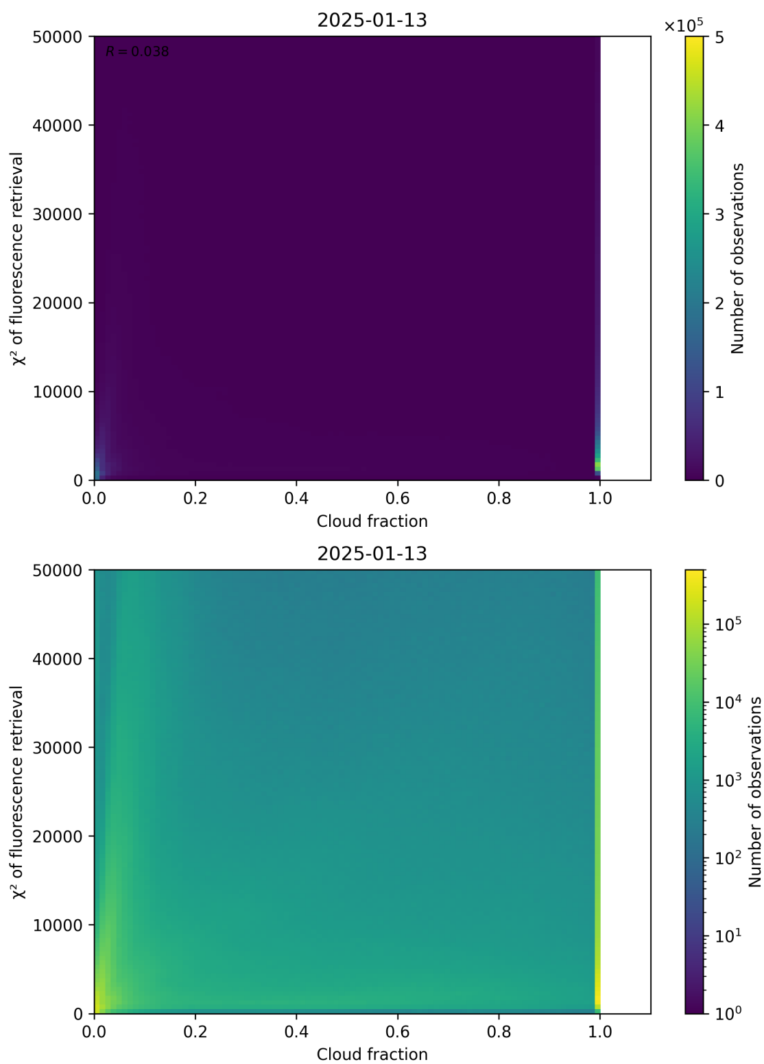
Figure 71: Scatter density plot of “Cloud fraction” against “ \chi^2 of fluorescence retrieval” for 2025-01-12 to 2025-01-14.
