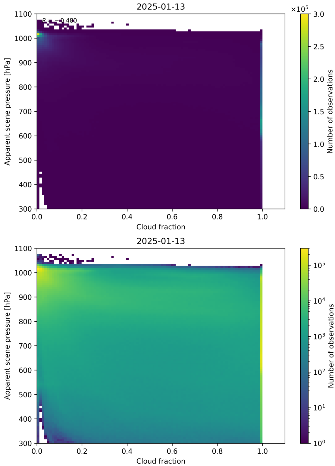
Figure 70: Scatter density plot of “Cloud fraction” against “Apparent scene pressure” for 2025-01-12 to 2025-01-14.
