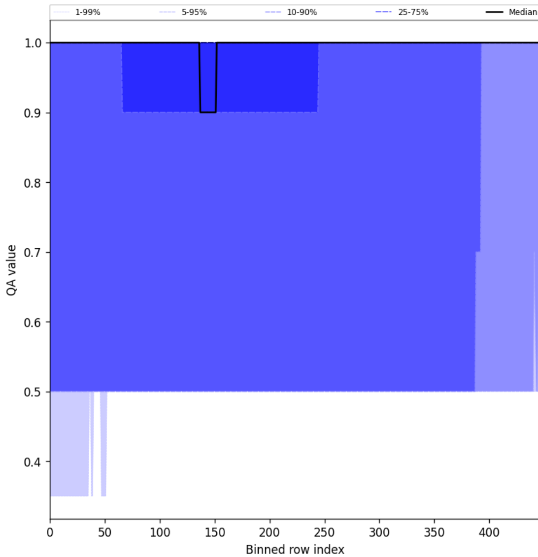
Figure 46: Along track statistics of “QA value” for 2025-01-12 to 2025-01-14
