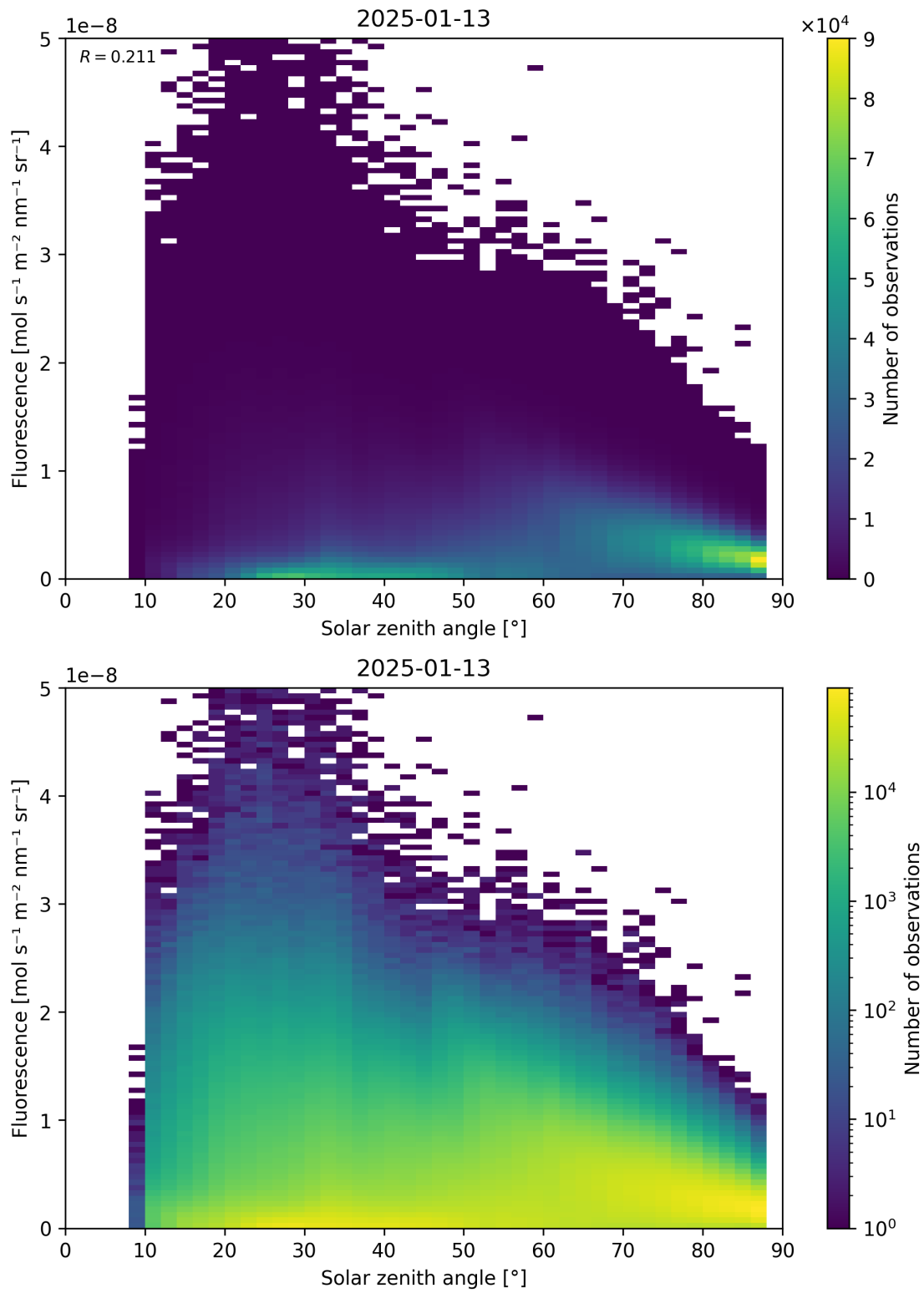
Figure 112: Scatter density plot of “Solar zenith angle” against “Fluorescence” for 2025-01-12 to 2025-01-14.
