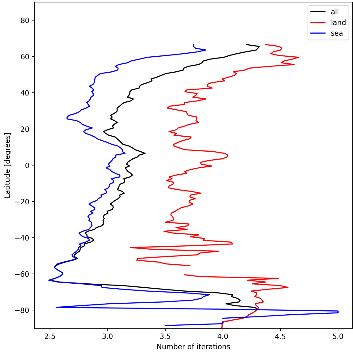
Figure 22: Zonal average of “Number of iterations” for 2025-01-12 to 2025-01-14.
