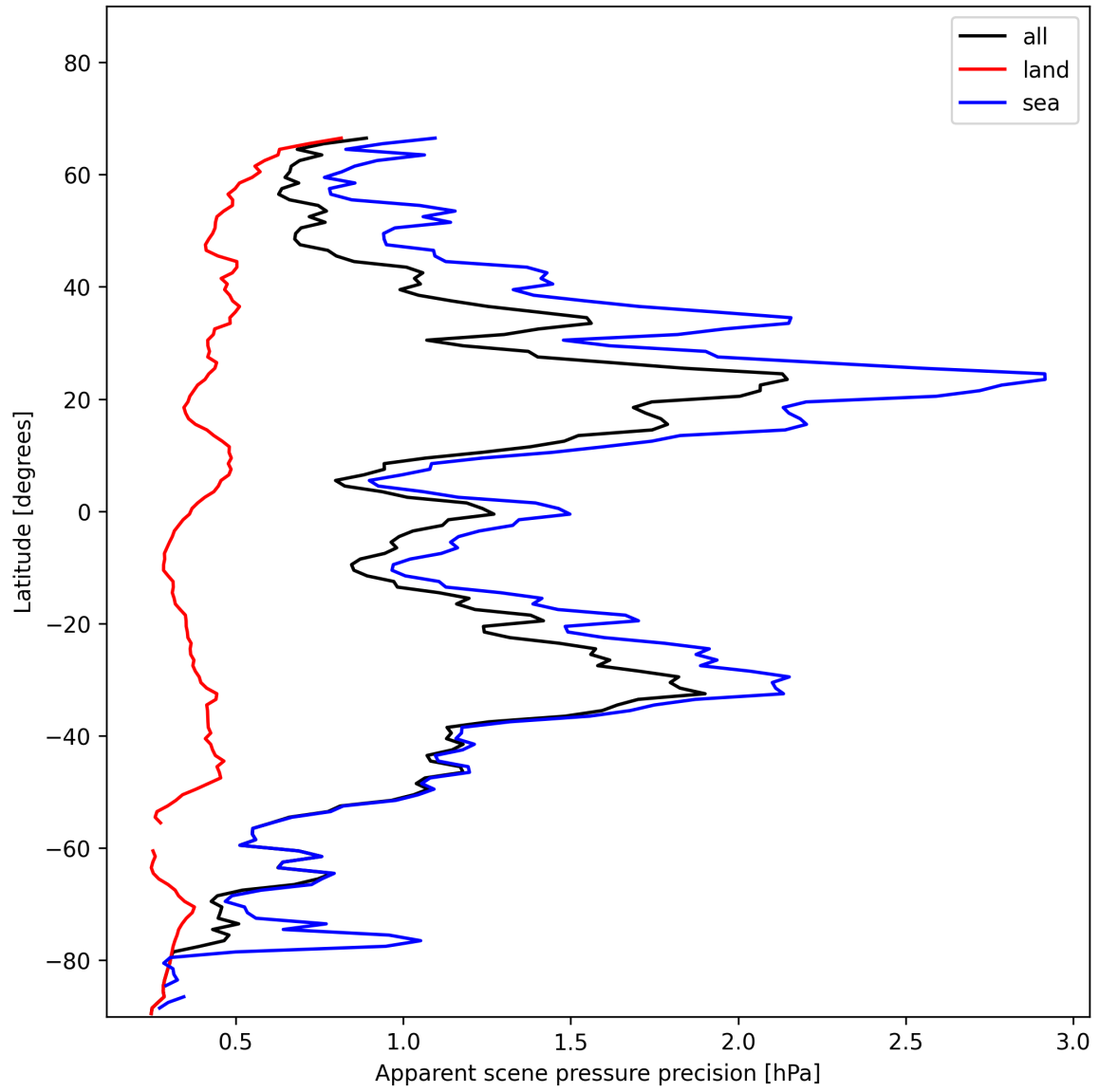
Figure 20: Zonal average of “Apparent scene pressure precision” for 2025-01-12 to 2025-01-14.
