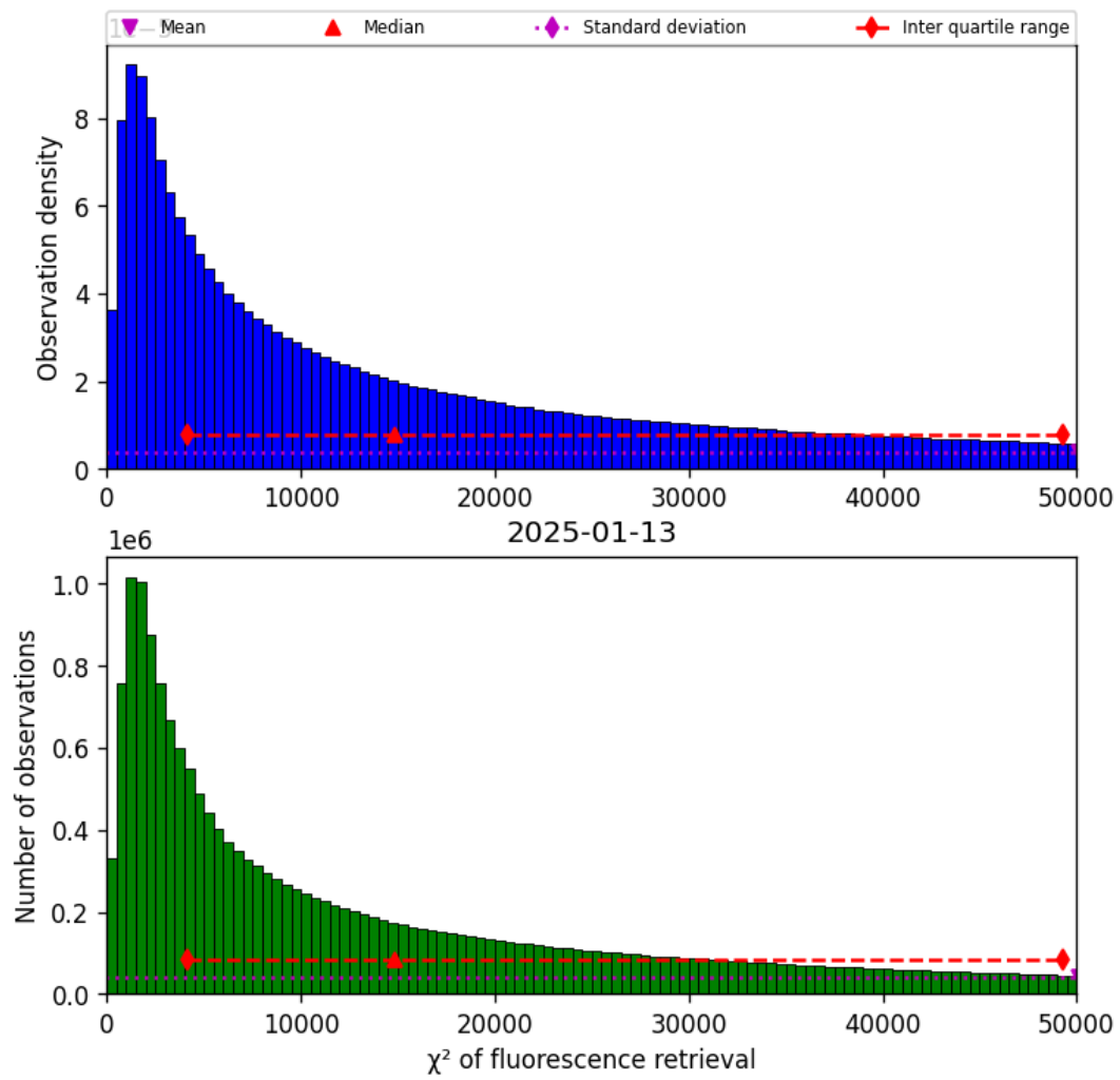
Figure 42: Histogram of “ \chi^2 of fluorescence retrieval” for 2025-01-12 to 2025-01-14
