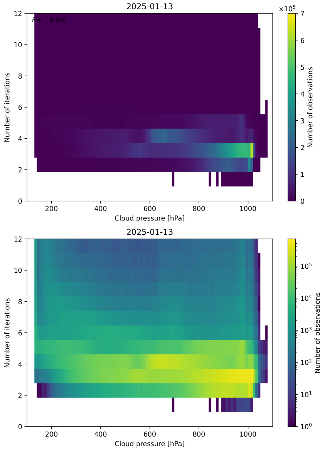
Figure 81: Scatter density plot of “Cloud pressure” against “Number of iterations” for 2025-01-12 to 2025-01-14.
