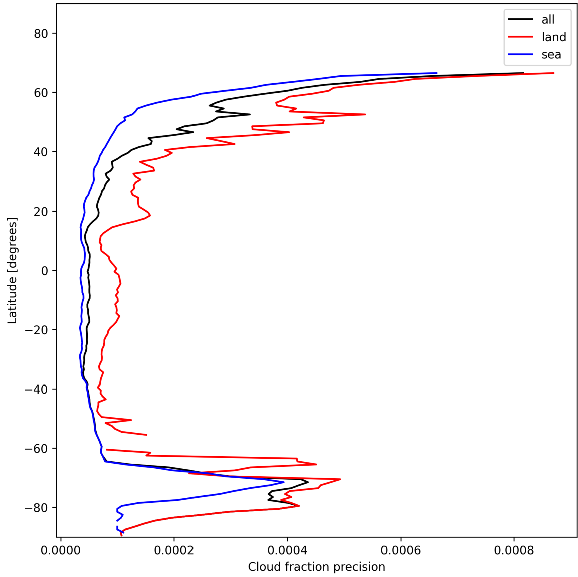
Figure 16: Zonal average of “Cloud fraction precision” for 2025-01-12 to 2025-01-14.
