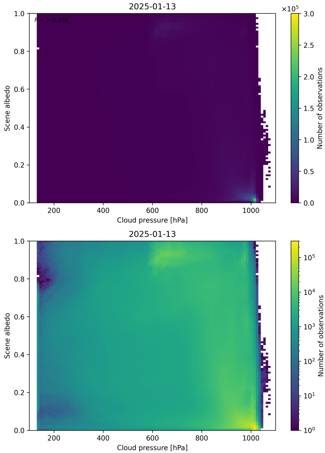
Figure 83: Scatter density plot of “Cloud pressure” against “Scene albedo” for 2025-01-12 to 2025-01-14.
