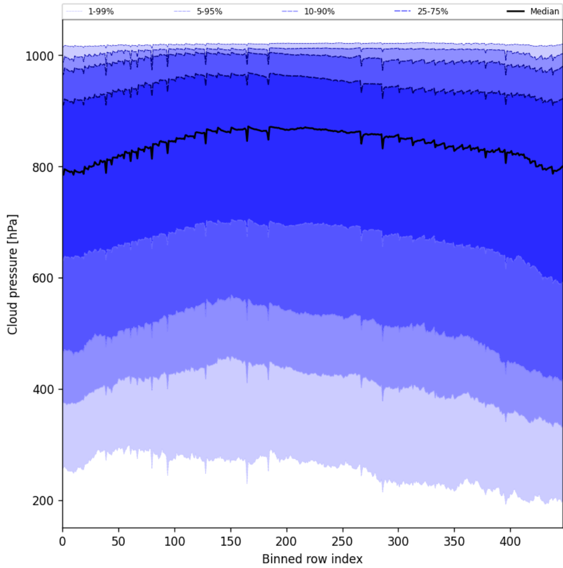
Figure 47: Along track statistics of “Cloud pressure” for 2025-01-12 to 2025-01-14
