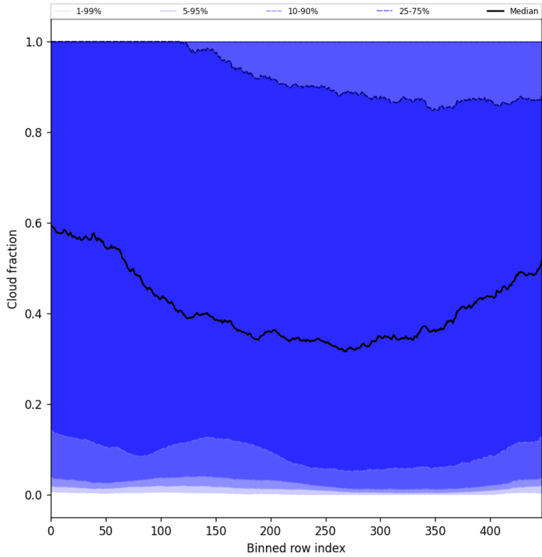
Figure 49: Along track statistics of “Cloud fraction” for 2025-01-12 to 2025-01-14
