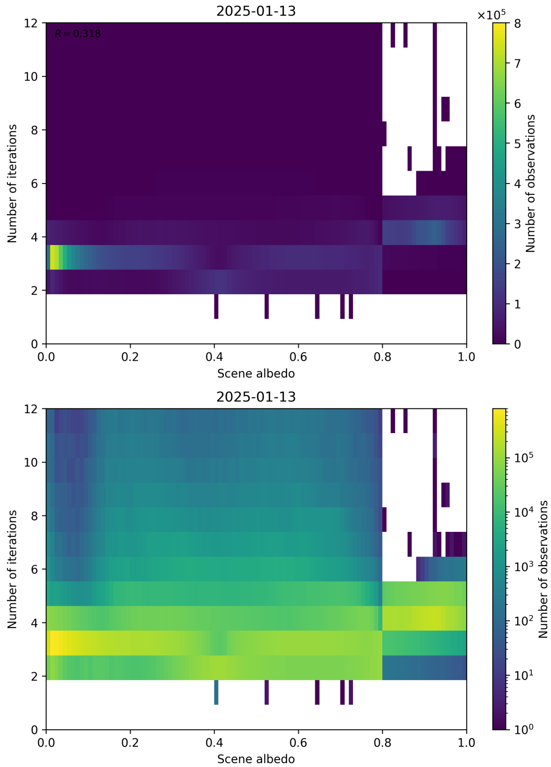
Figure 105: Scatter density plot of “Scene albedo” against “Number of iterations” for 2025-01-12 to 2025-01-14.
