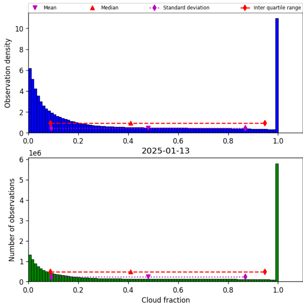
Figure 32: Histogram of “Cloud fraction” for 2025-01-12 to 2025-01-14
