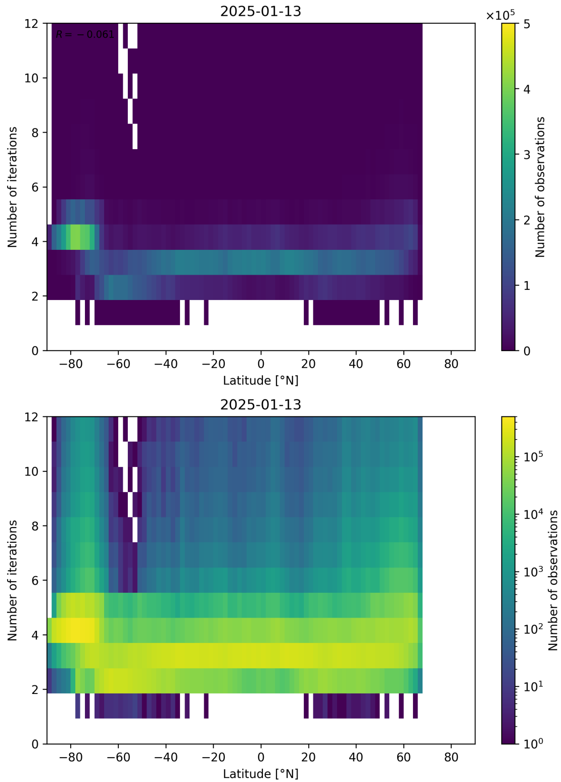
Figure 93: Scatter density plot of “Latitude” against “Number of iterations” for 2025-01-12 to 2025-01-14.
