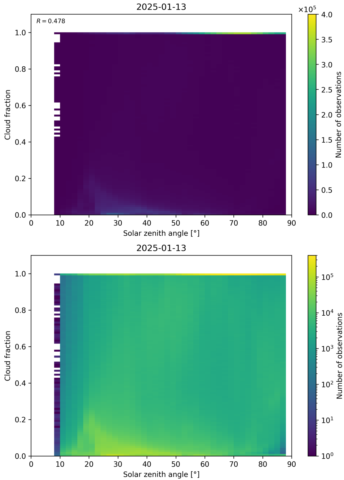
Figure 110: Scatter density plot of “Solar zenith angle” against “Cloud fraction” for 2025-01-12 to 2025-01-14.
