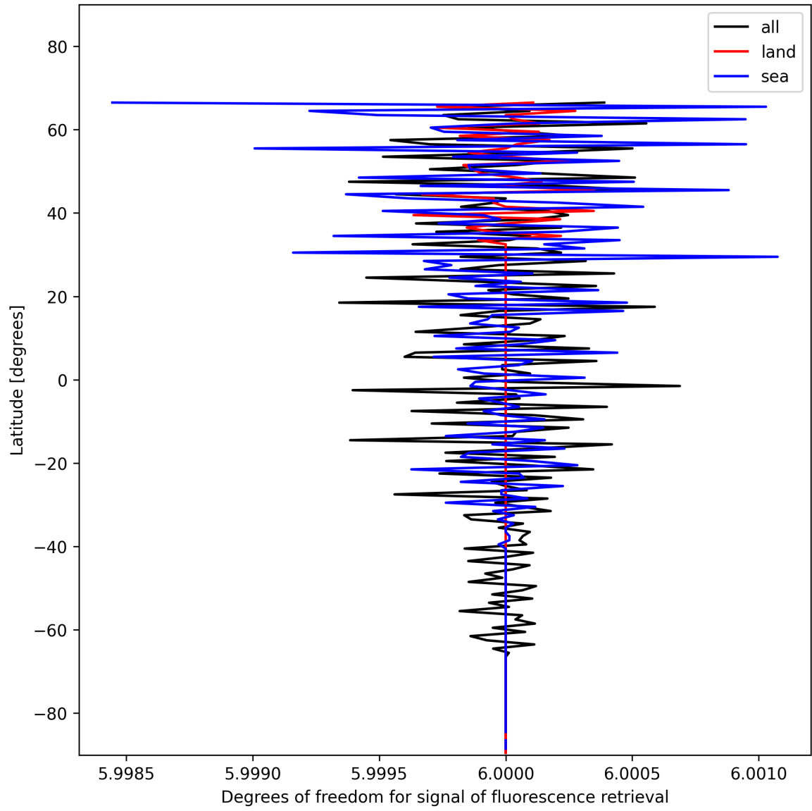
Figure 26: Zonal average of “Degrees of freedom for signal of fluorescence retrieval” for 2025-01-12 to 2025-01-14.
