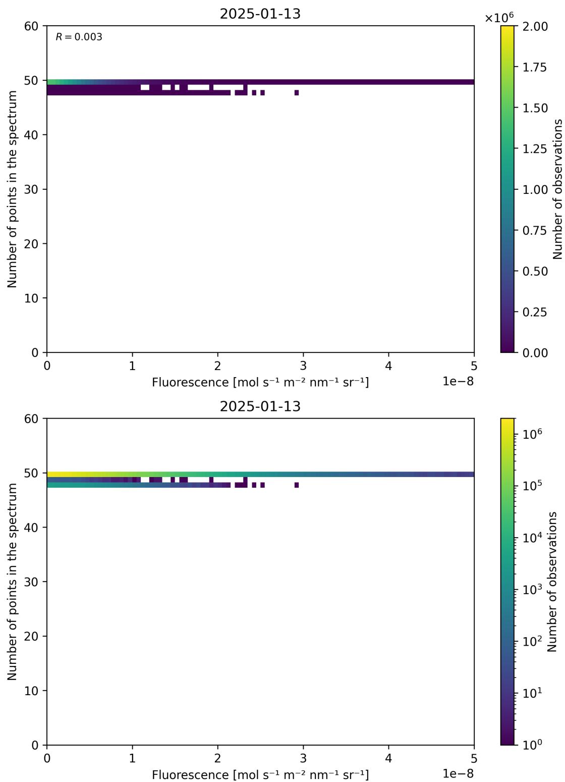
Figure 86: Scatter density plot of “Fluorescence” against “Number of points in the spectrum” for 2025-01-12 to 2025-01-14.
