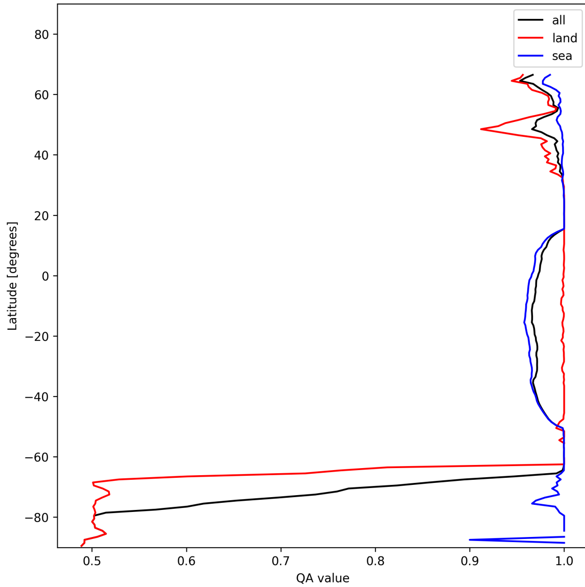
Figure 12: Zonal average of “QA value” for 2025-01-12 to 2025-01-14.
