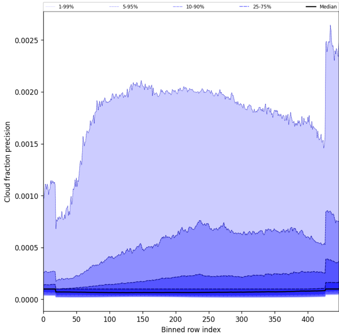
Figure 50: Along track statistics of “Cloud fraction precision” for 2025-01-12 to 2025-01-14
