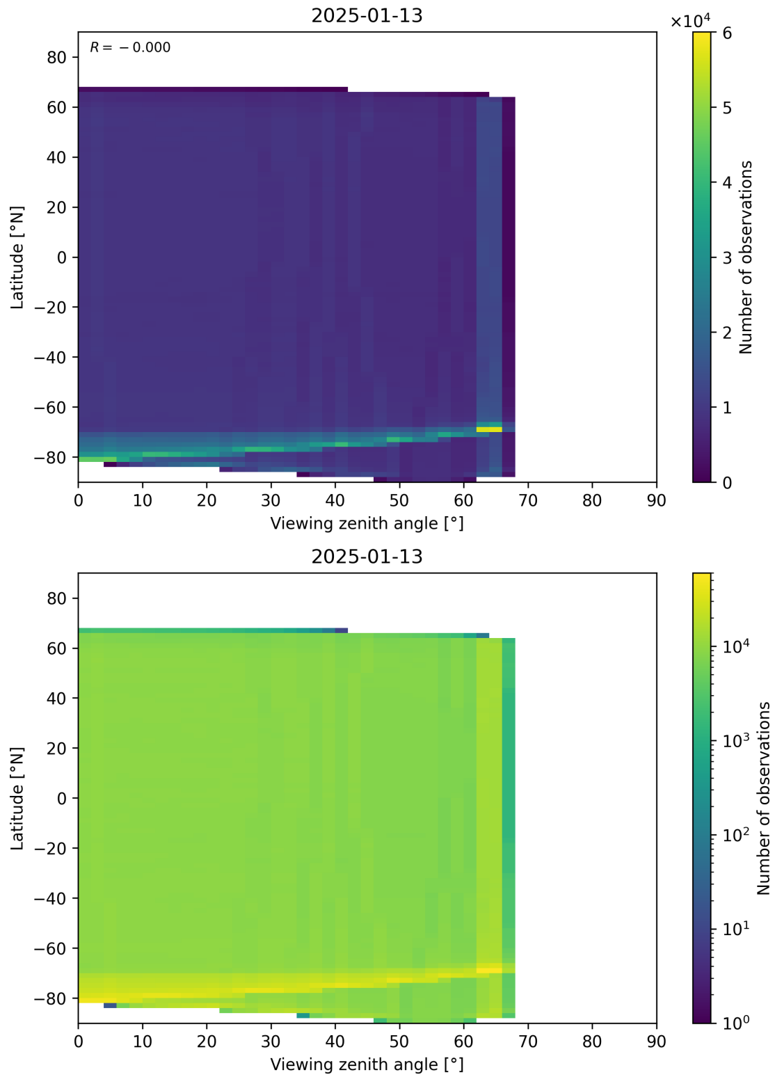
Figure 123: Scatter density plot of “Viewing zenith angle” against “Latitude” for 2025-01-12 to 2025-01-14.
