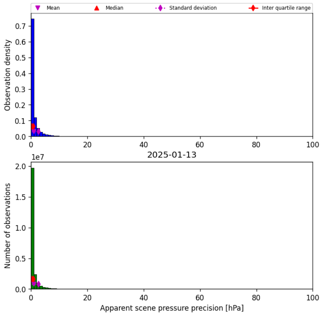
Figure 37: Histogram of “Apparent scene pressure precision” for 2025-01-12 to 2025-01-14
