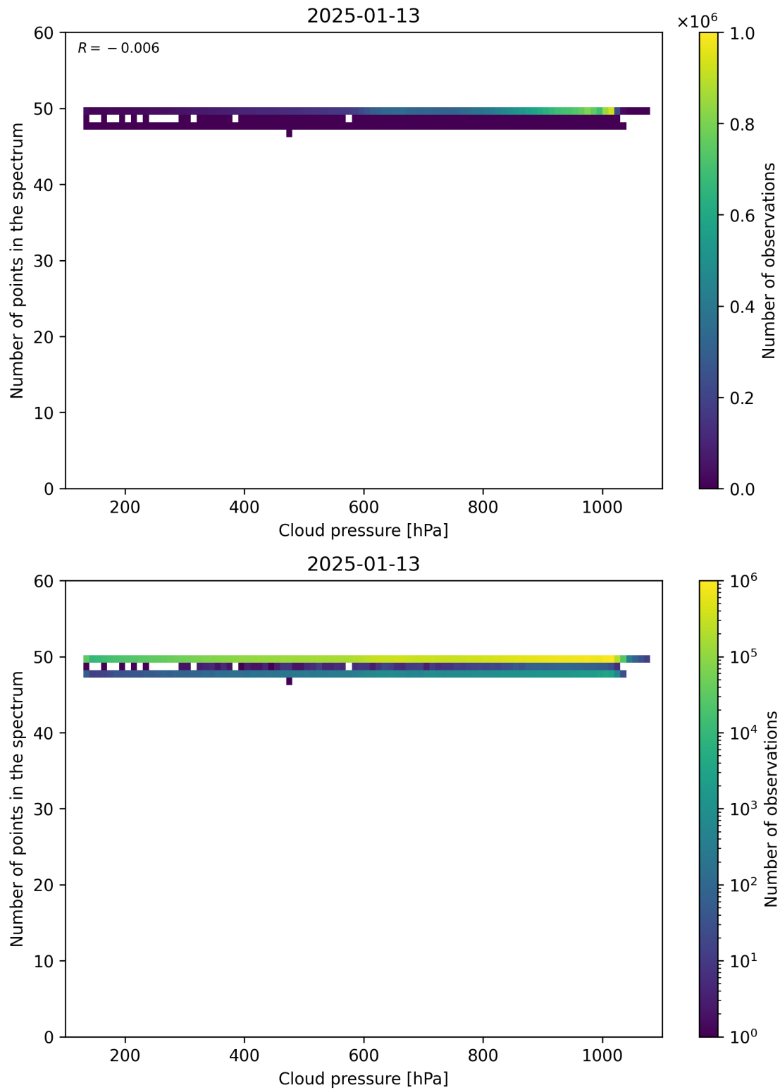
Figure 82: Scatter density plot of “Cloud pressure” against “Number of points in the spectrum” for 2025-01-12 to 2025-01-14.
