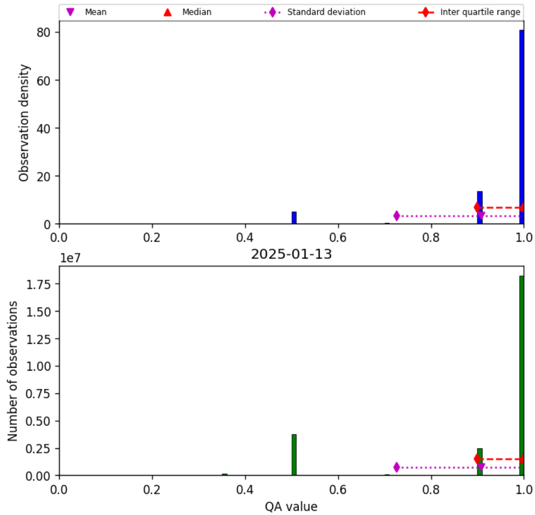
Figure 29: Histogram of “QA value” for 2025-01-12 to 2025-01-14
