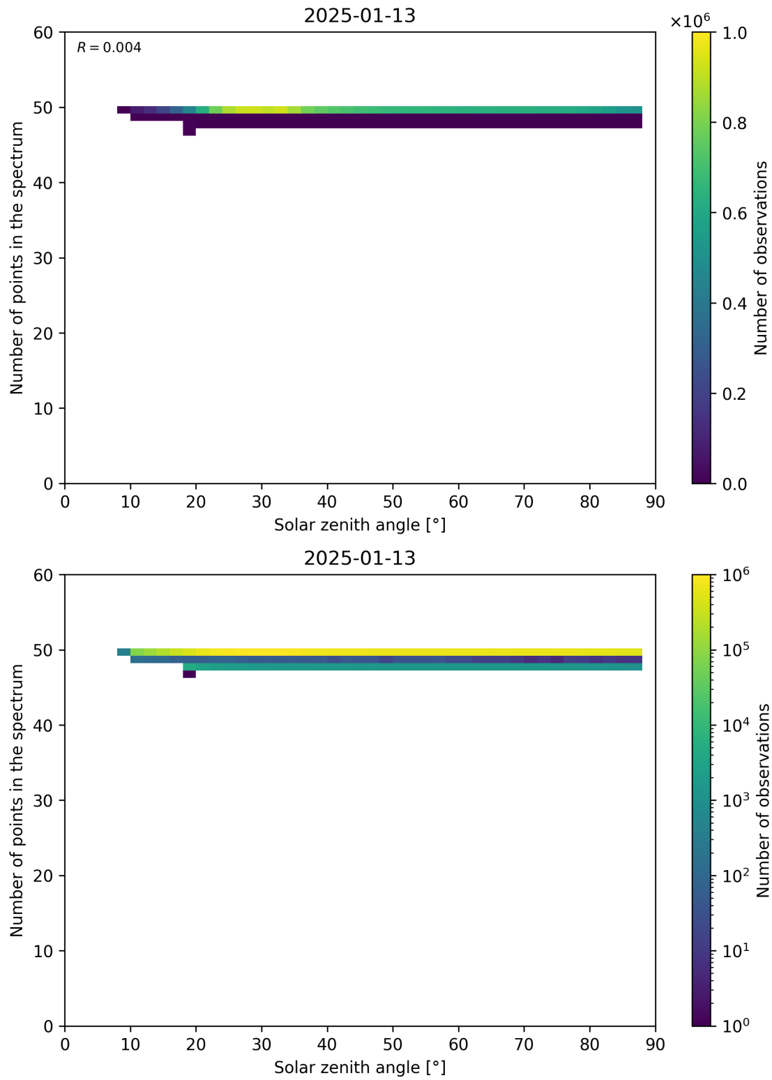
Figure 115: Scatter density plot of “Solar zenith angle” against “Number of points in the spectrum” for 2025-01-12 to 2025-01-14.
