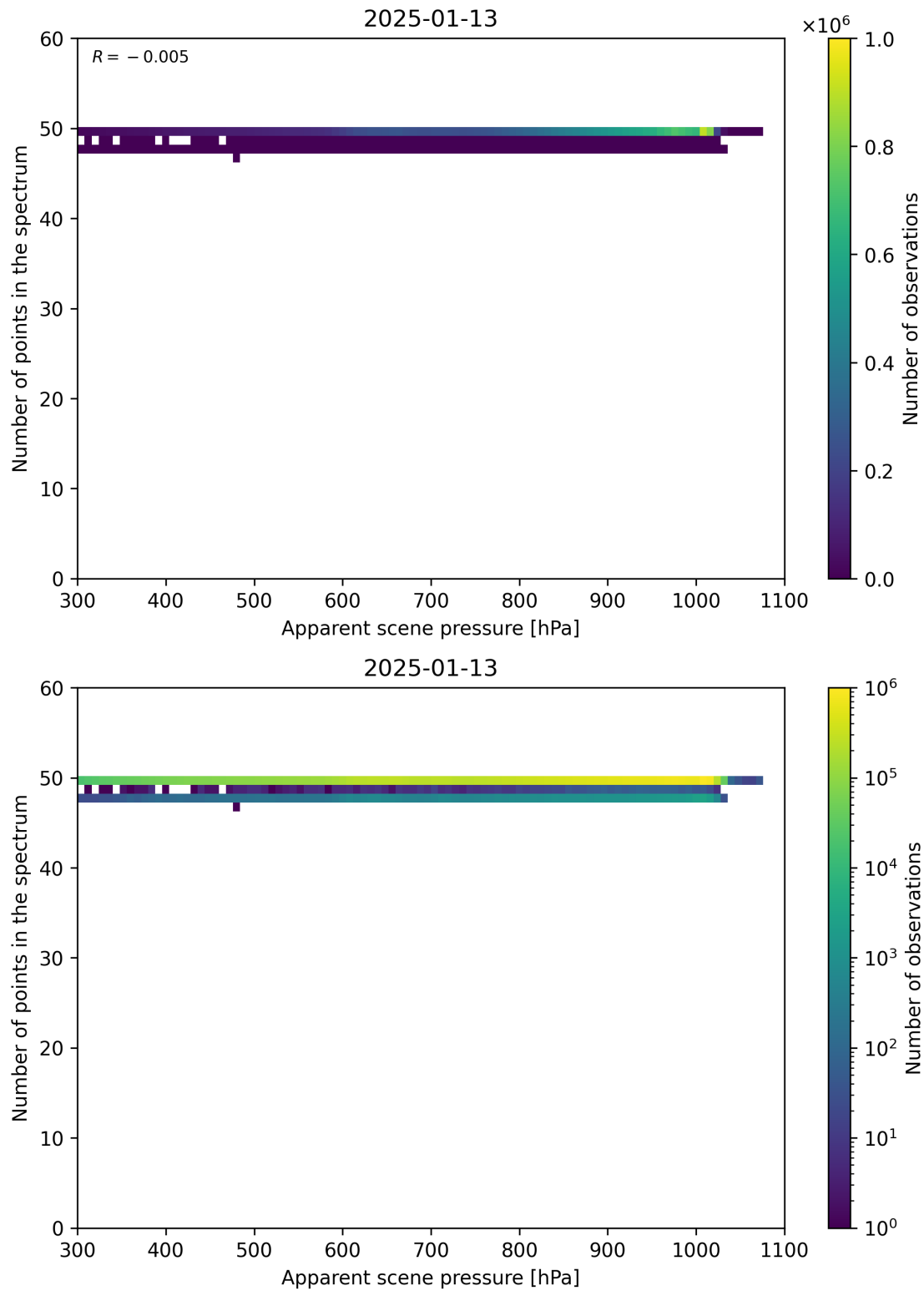
Figure 66: Scatter density plot of “Apparent scene pressure” against “Number of points in the spectrum” for 2025-01-12 to 2025-01-14.
