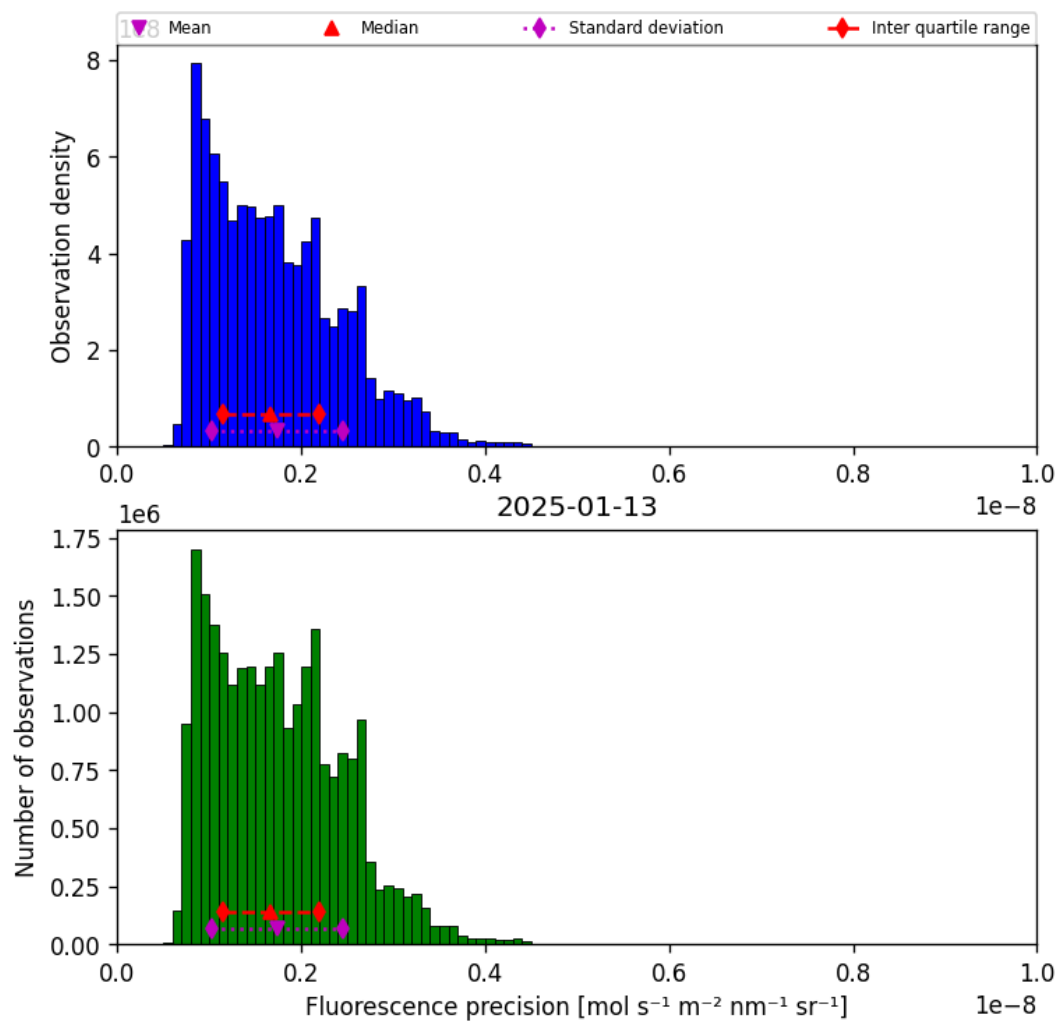
Figure 41: Histogram of “Fluorescence precision” for 2025-01-12 to 2025-01-14
