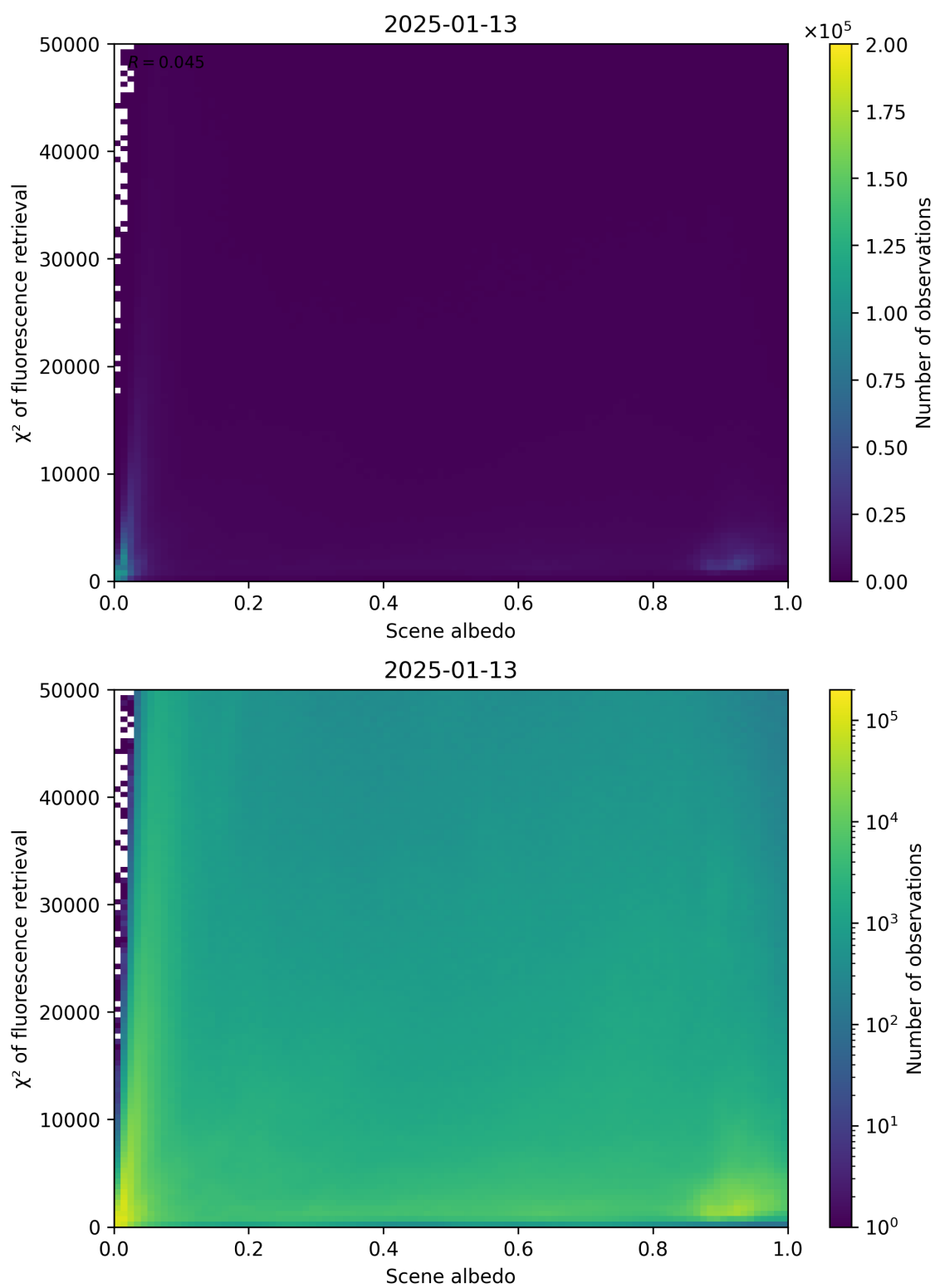
Figure 103: Scatter density plot of “Scene albedo” against “ \chi^2 of fluorescence retrieval” for 2025-01-12 to 2025-01-14.
