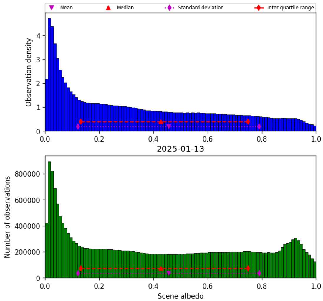
Figure 34: Histogram of “Scene albedo” for 2025-01-12 to 2025-01-14
