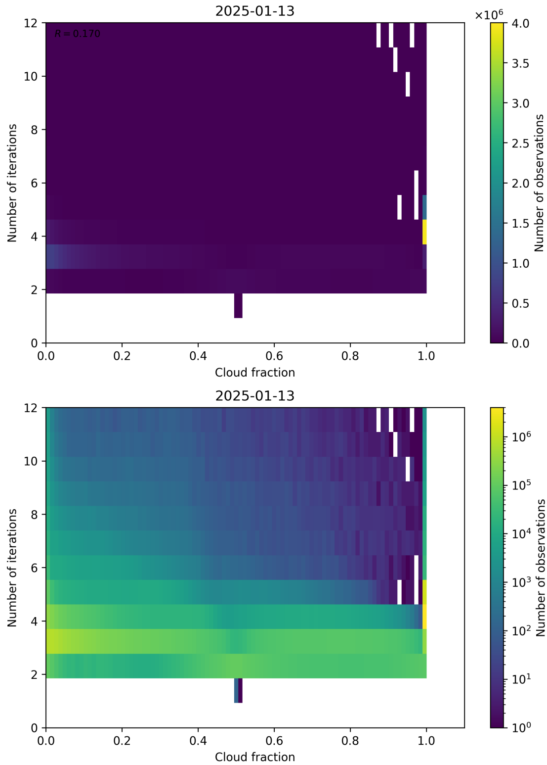
Figure 73: Scatter density plot of “Cloud fraction” against “Number of iterations” for 2025-01-12 to 2025-01-14.
