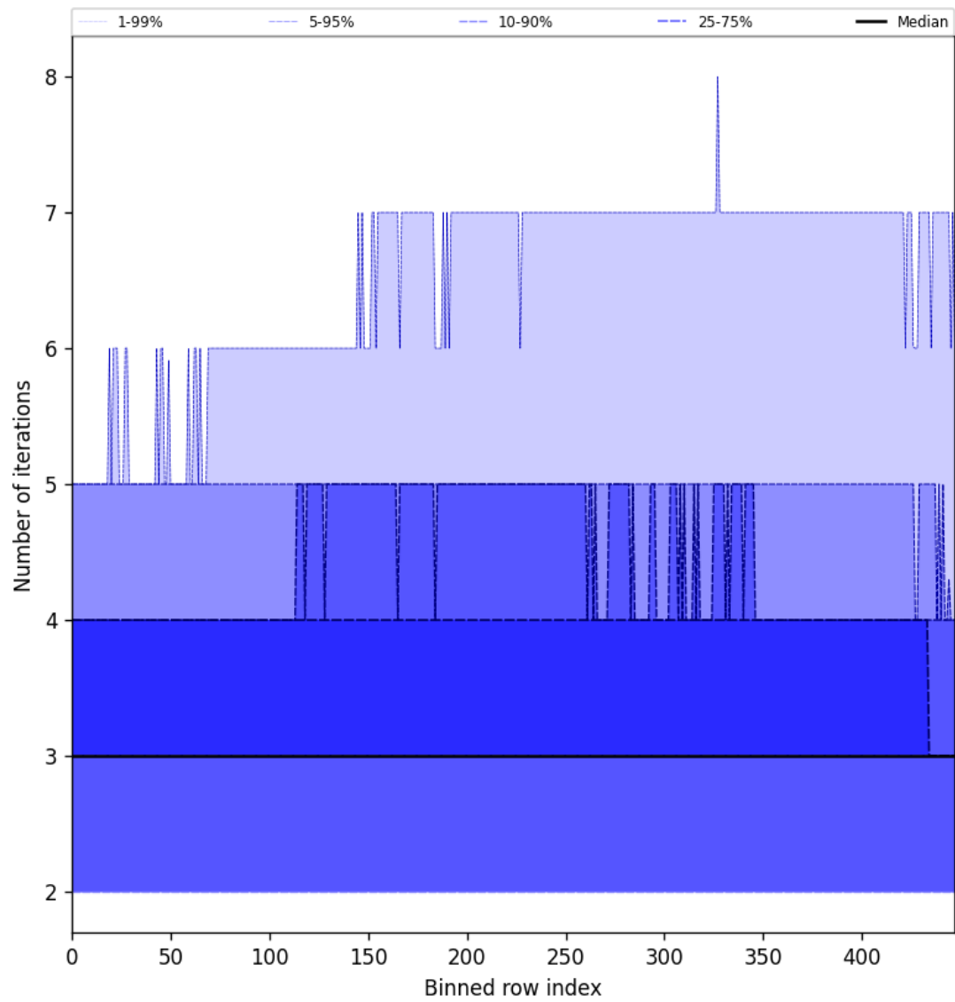
Figure 56: Along track statistics of “Number of iterations” for 2025-01-12 to 2025-01-14
