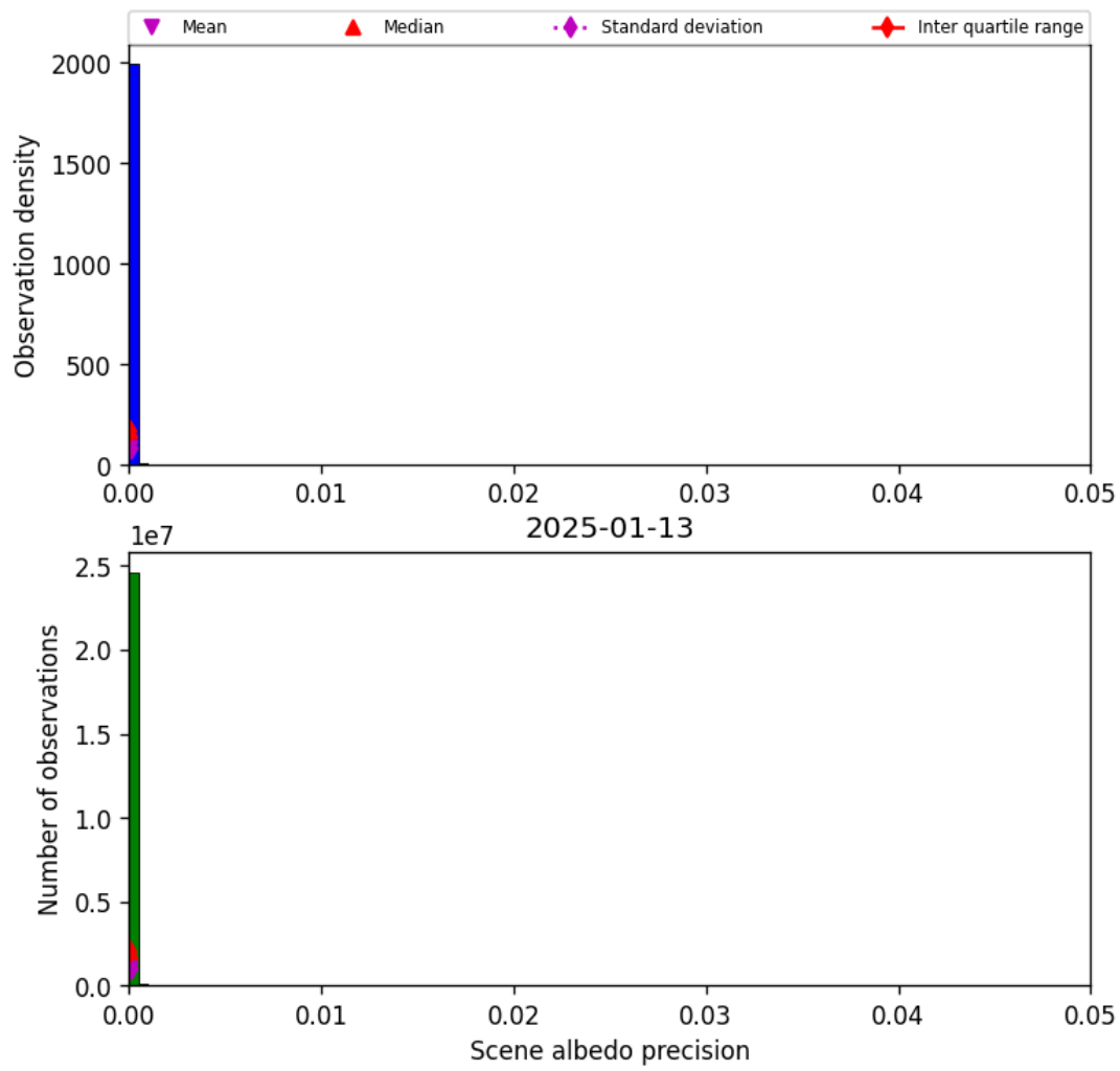
Figure 35: Histogram of “Scene albedo precision” for 2025-01-12 to 2025-01-14
