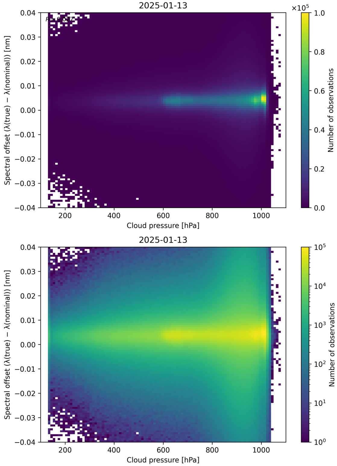
Figure 84: Scatter density plot of “Cloud pressure” against “Spectral offset ( \lambda_{\text{true}} - \lambda_{\text{nominal}} )” for 2025-01-12 to 2025-01-14.
