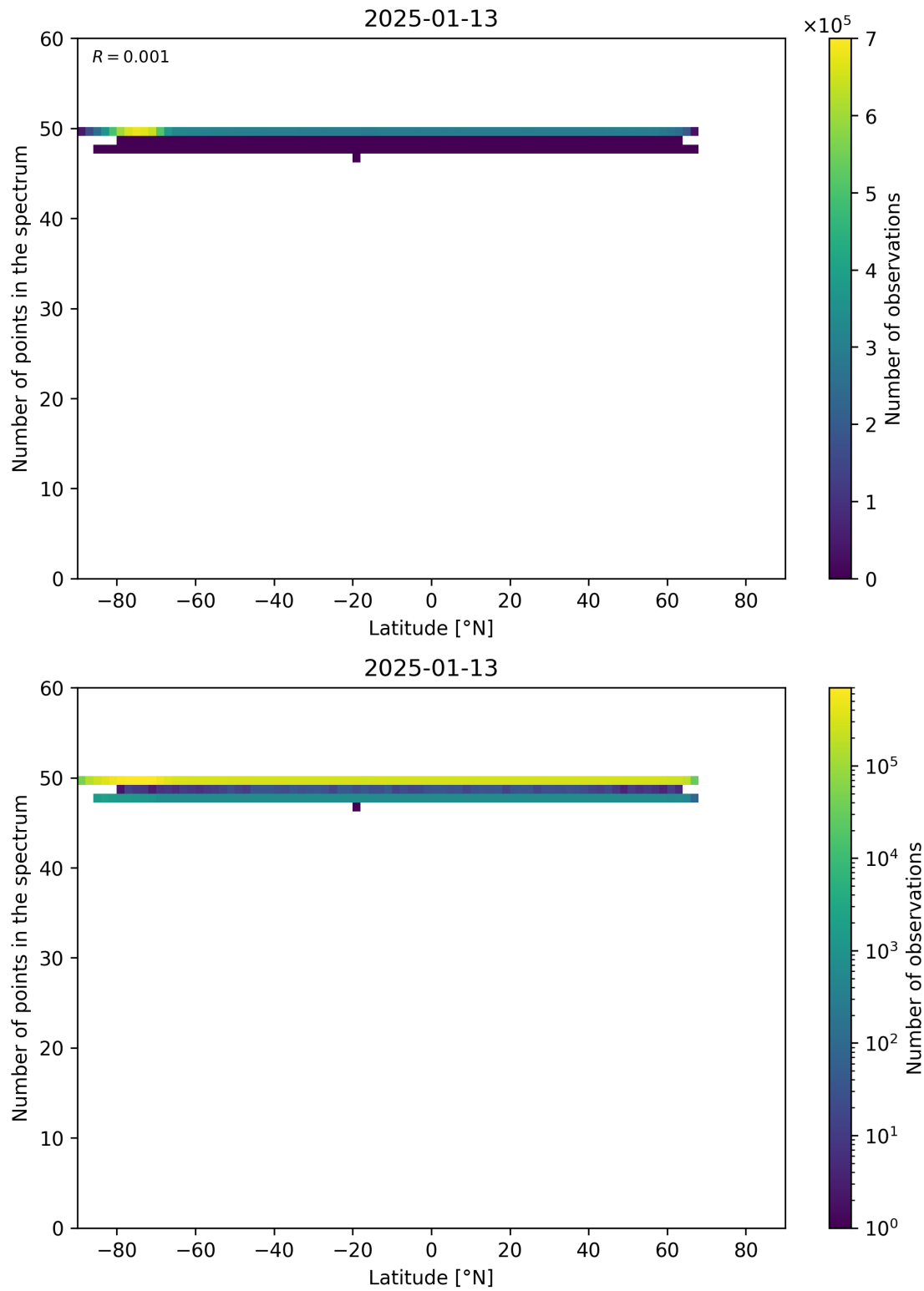
Figure 94: Scatter density plot of “Latitude” against “Number of points in the spectrum” for 2025-01-12 to 2025-01-14.
