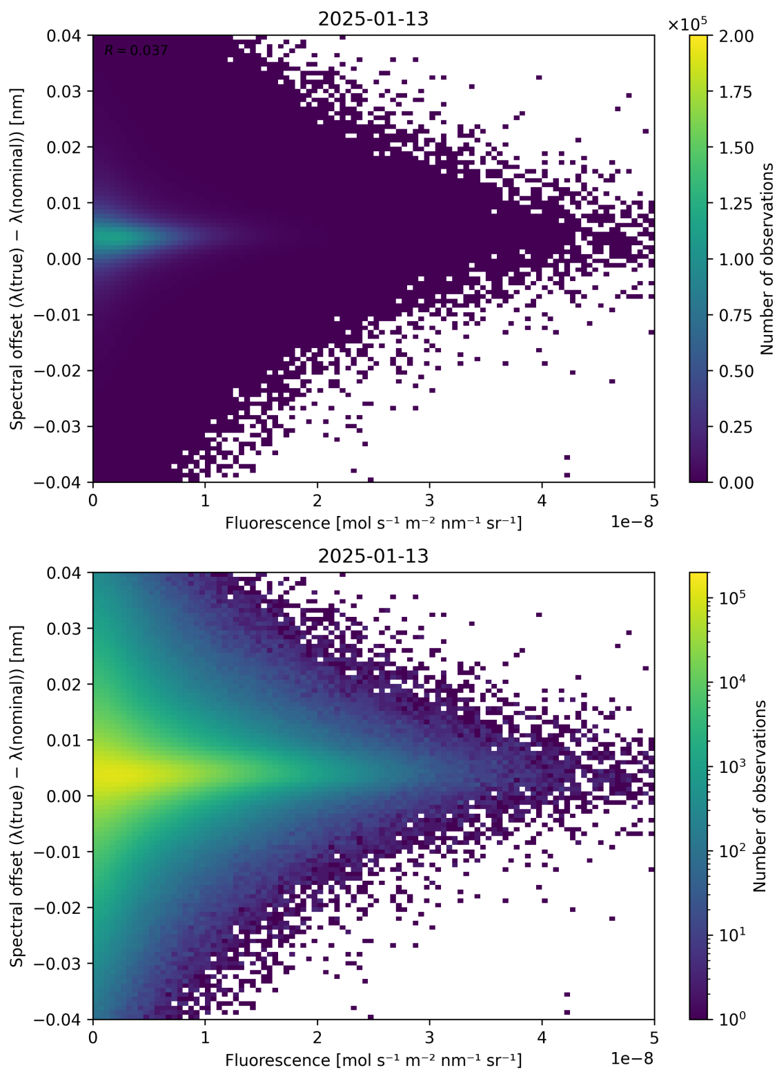
Figure 87: Scatter density plot of “Fluorescence” against “Spectral offset ( \lambda_{\text{true}} - \lambda_{\text{nominal}} )” for 2025-01-12 to 2025-01-14.
