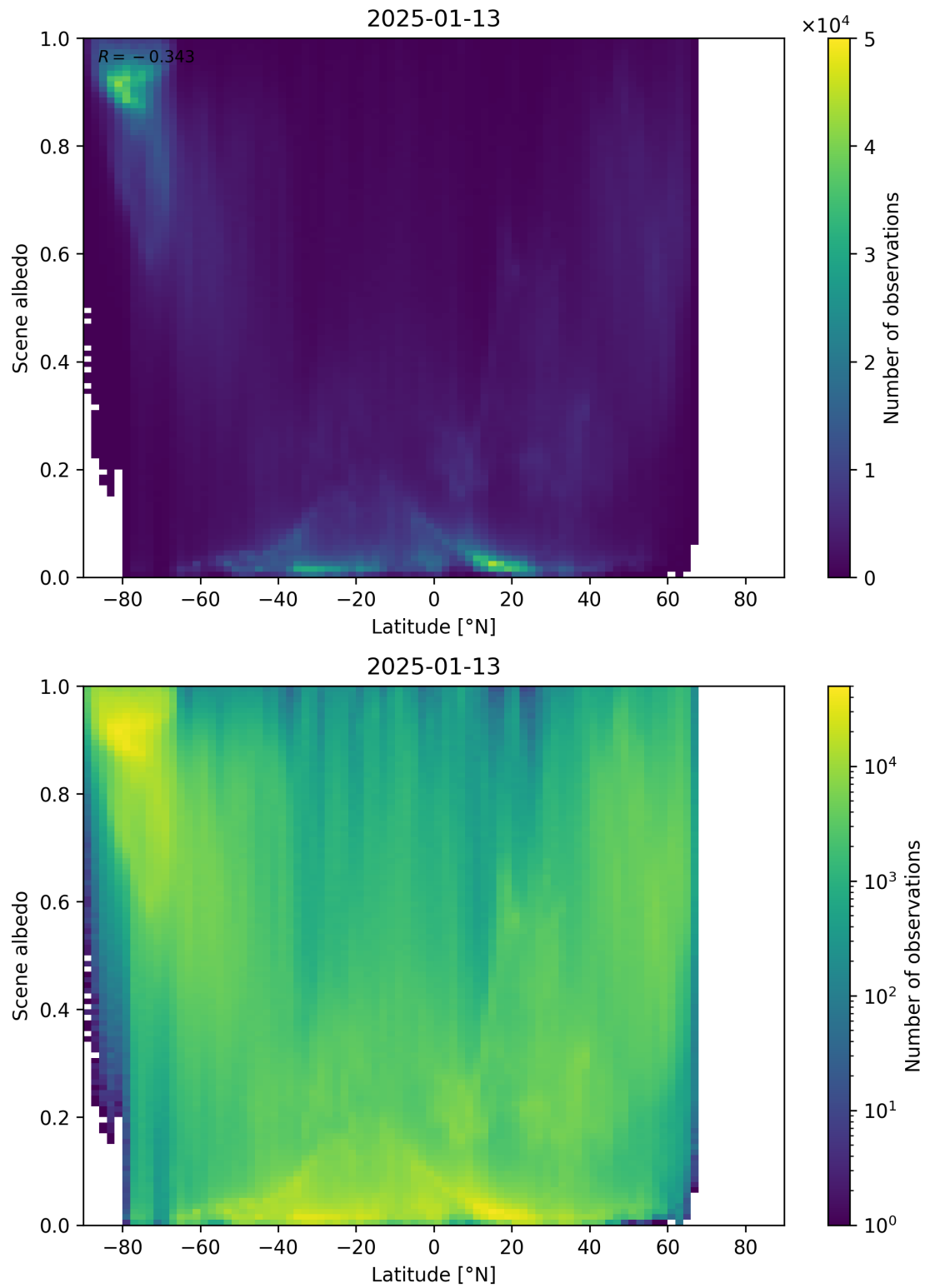
Figure 95: Scatter density plot of “Latitude” against “Scene albedo” for 2025-01-12 to 2025-01-14.
