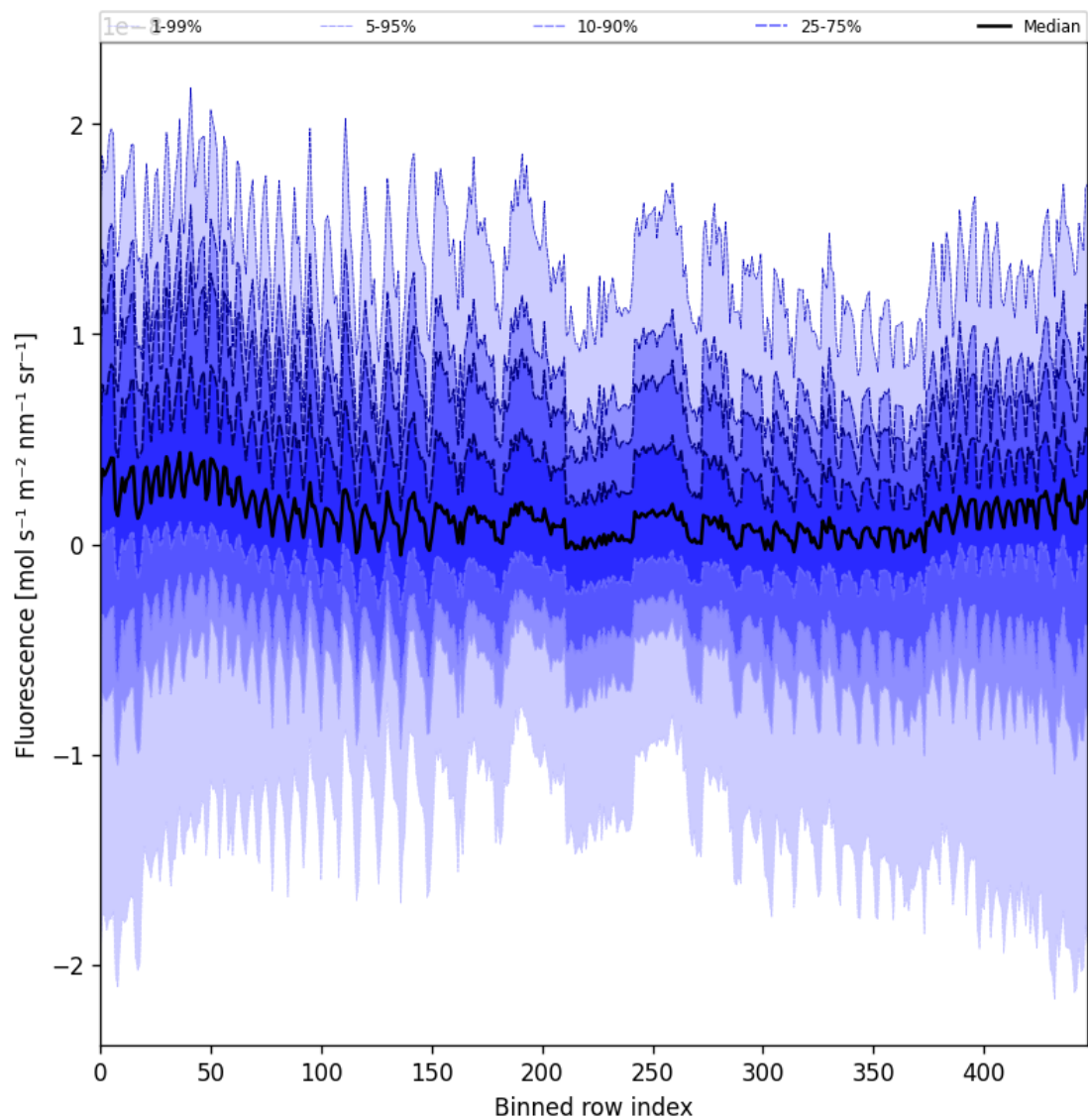
Figure 57: Along track statistics of “Fluorescence” for 2025-01-12 to 2025-01-14
