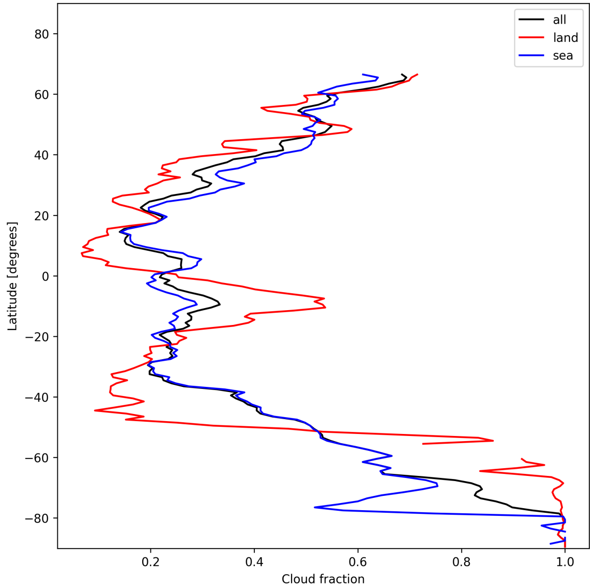
Figure 15: Zonal average of “Cloud fraction” for 2025-01-12 to 2025-01-14.
