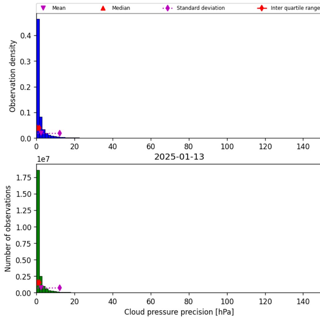
Figure 31: Histogram of “Cloud pressure precision” for 2025-01-12 to 2025-01-14
