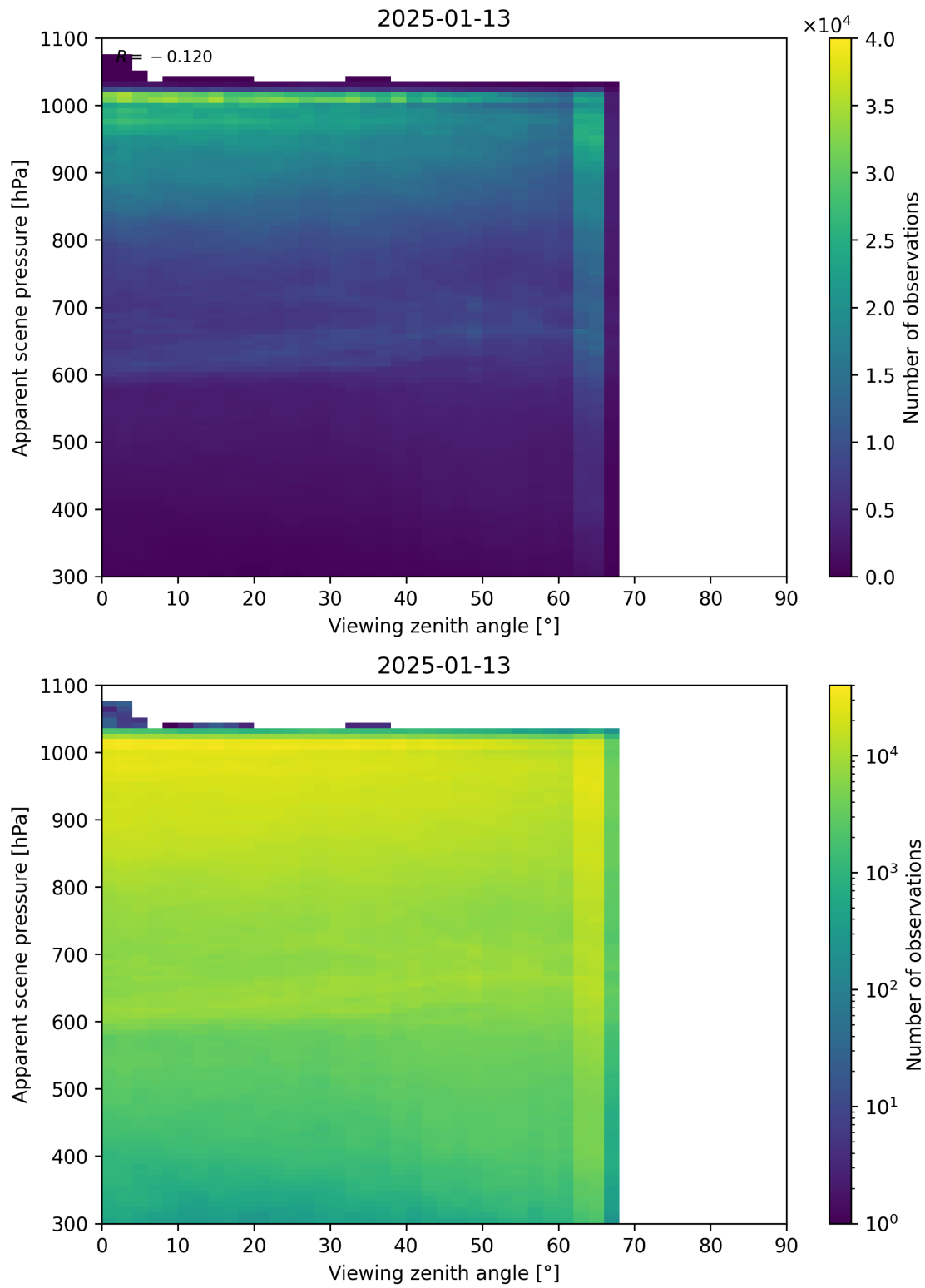
Figure 118: Scatter density plot of “Viewing zenith angle” against “Apparent scene pressure” for 2025-01-12 to 2025-01-14.
