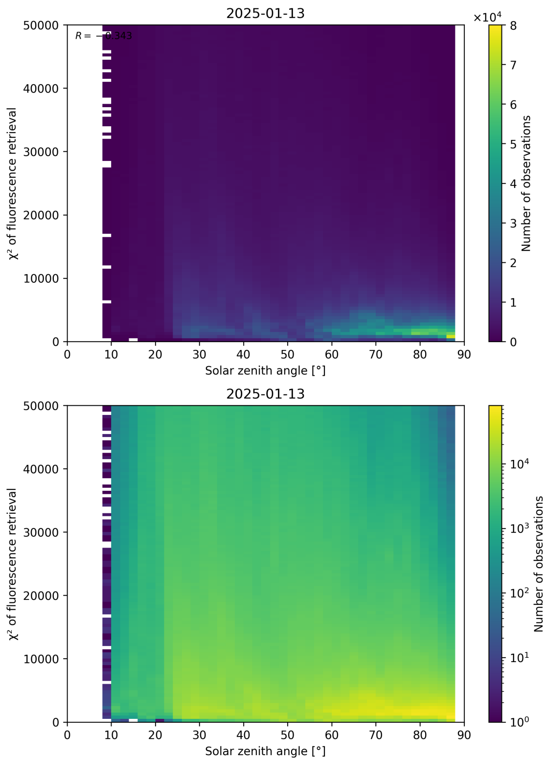
Figure 109: Scatter density plot of “Solar zenith angle” against “ \chi^2 of fluorescence retrieval” for 2025-01-12 to 2025-01-14.
