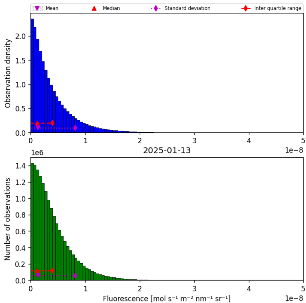
Figure 40: Histogram of “Fluorescence” for 2025-01-12 to 2025-01-14
