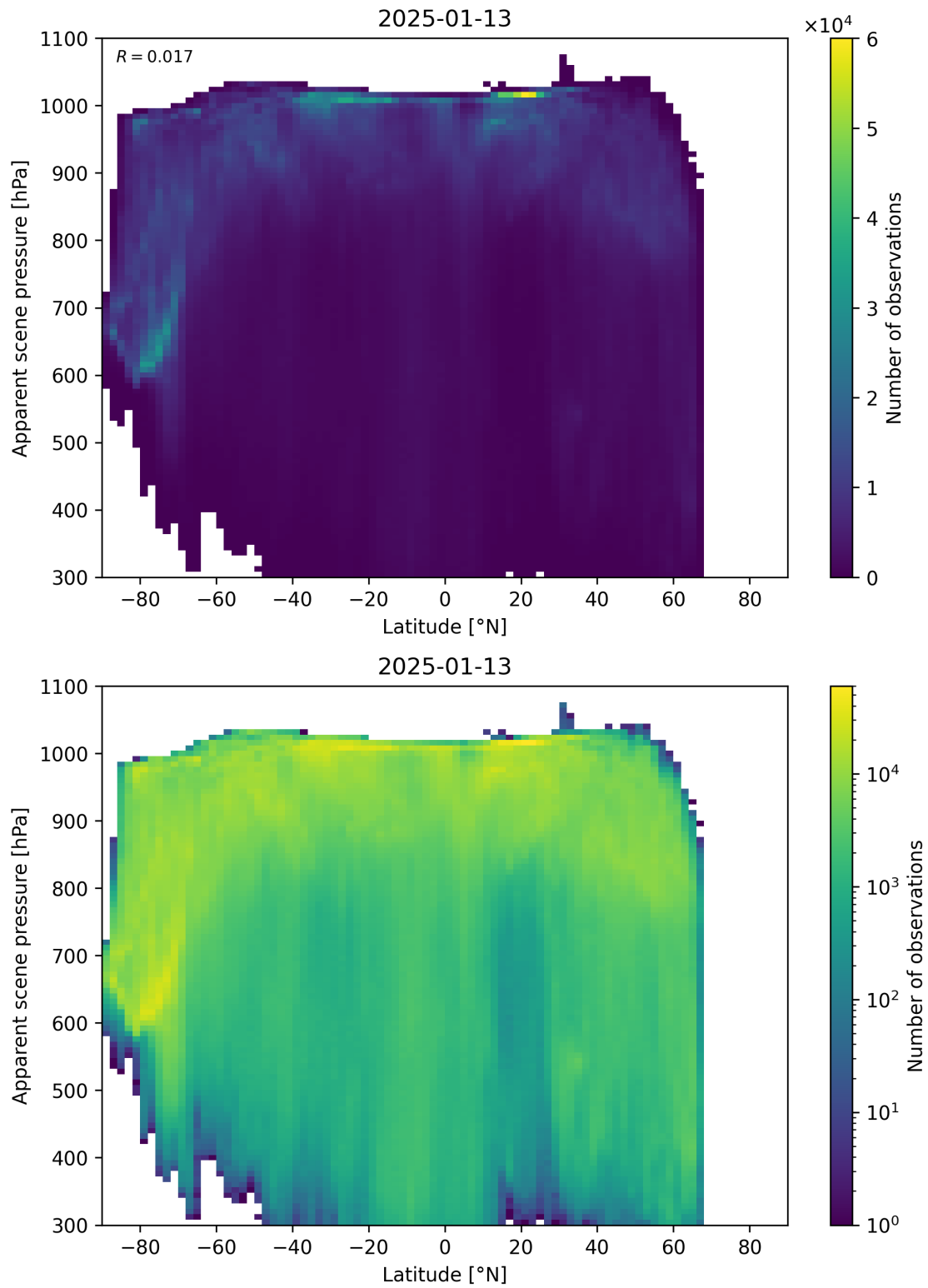
Figure 88: Scatter density plot of “Latitude” against “Apparent scene pressure” for 2025-01-12 to 2025-01-14.
