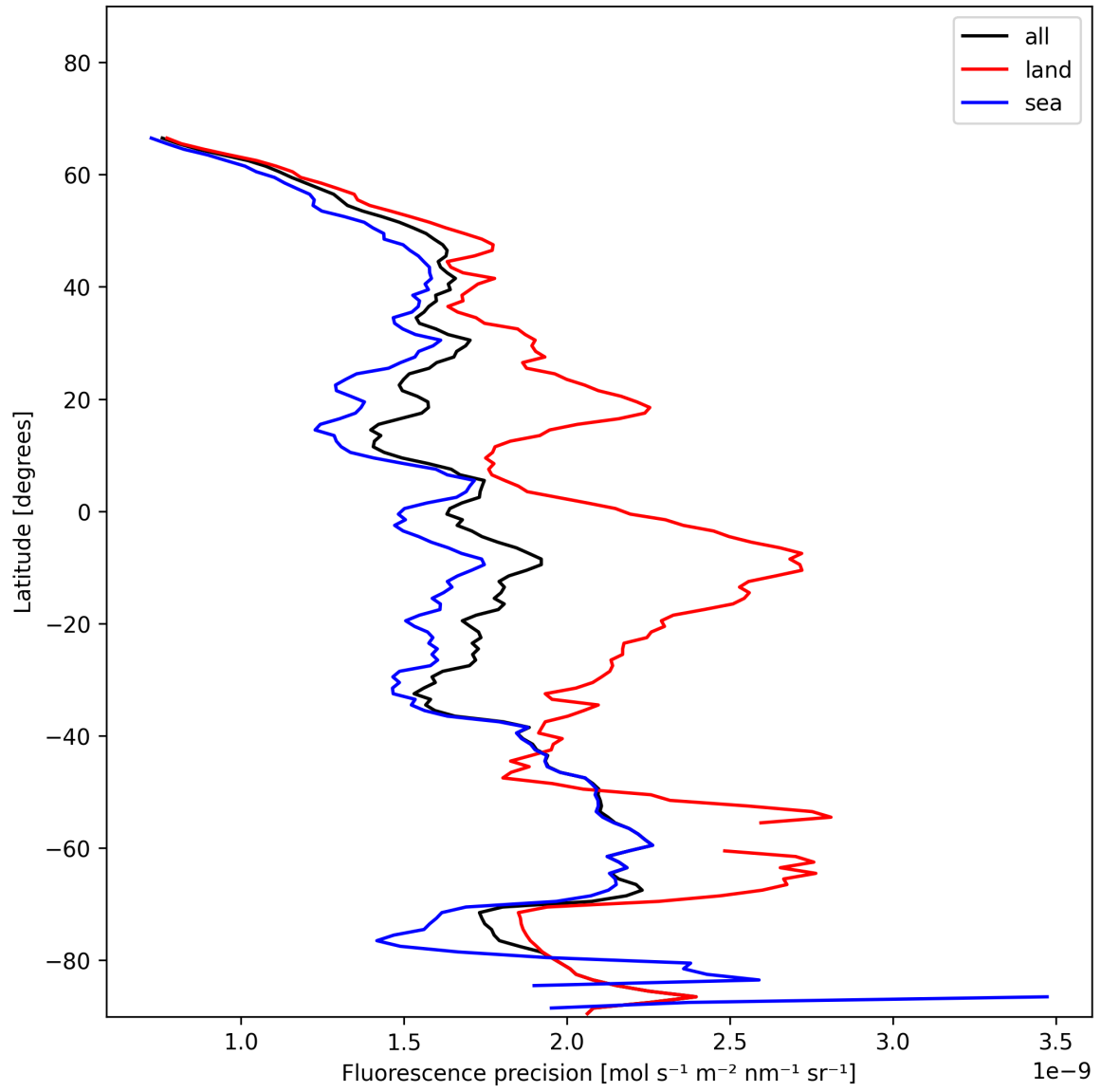
Figure 24: Zonal average of “Fluorescence precision” for 2025-01-12 to 2025-01-14.
